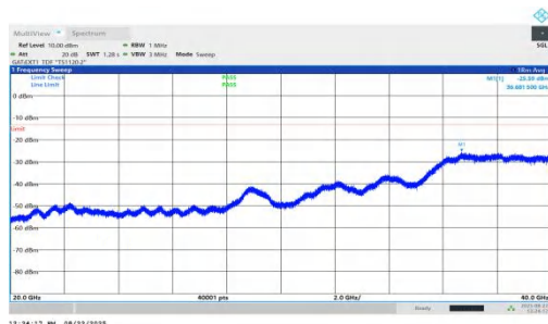
NTV-n78(3450-3550)-PC1.5-30-50-L-DFT-BPSK-Inner_1RB_Right-2 0000-40000-PASS
