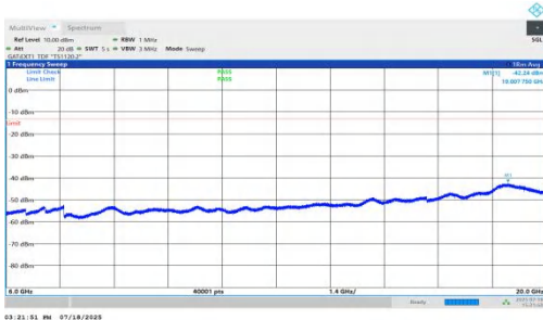
NTNV-n78(3450-3550)-PC1.5-30-70-L-DFT-BPSK-Inner_1RB_Right-6000-20000-PASS
