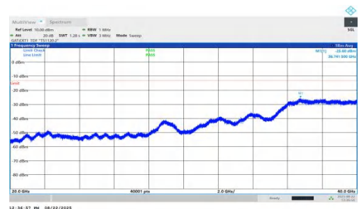
NTNV-n78(3450-3550)-PC1.5-30-60-H-DFT-QPSK-Inner_1RB_Right-2 0000-40000-PASS
