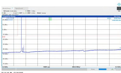
NTNV-n78(3450-3550)-PC1.5-30-60-H-DFT-QPSK-Inner_1RB_Left-3000-6000-PASS
