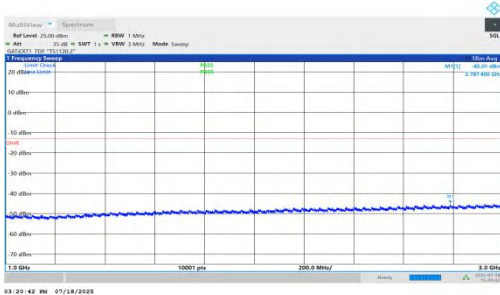
NTNV-n78(3450-3550)-PC1.5-30-70-L-DFT-BPSK-Inner_1RB_Right-1000-3000-PASS
