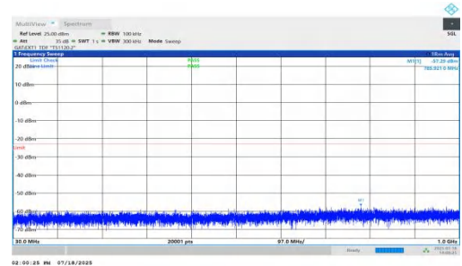
NTNV-n78(3450-3550)-PC1.5-30-40-H-DFT-QPSK-Inner_1RB_Right-3 0-1000-PASS
