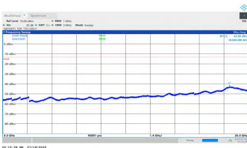
NTNV-n78(3450-3550)-PC1.5-30-60-H-DFT-QPSK-Inner_1RB_Right- 6000-20000-PASS
