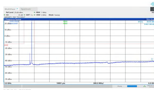
NTNV-n78(3450-3550)-PC1.5-30-40-H-DFT-BPSK-Inner_1RB_Right-3 000-6000-PASS
