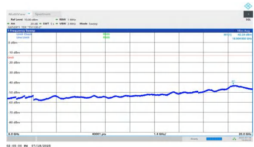
NTNV-n78(3450-3550)-PC1.5-30-50-L-DFT-BPSK-Inner_1RB_Left-6000-20000-PASS
