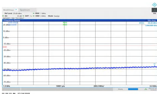
NTNV-n78(3450-3550)-PC1.5-30-60-M-DFT-BPSK-Inner_1RB_Right-1000-3000-PASS
