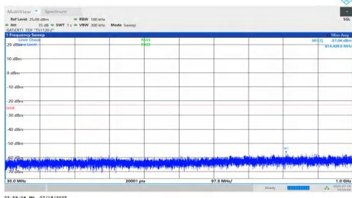
NTNV-n78(3450-3550)-PC1.5-30-60-M-DFT-QPSK-Inner_1RB_Left-3 0-1000-PASS
