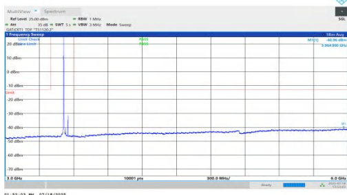
NTNV-n78(3450-3550)-PC1.5-30-40-H-DFT-BPSK-Inner_1RB_Left-3 000-6000-PASS
