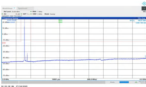
NTNV-n78(3450-3550)-PC1.5-30-60-M-DFT-BPSK-Inner_1RB_Left-3000-6000-PASS
