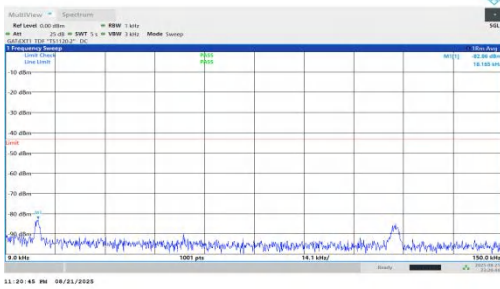
NTNV-n78(3450-3550)-PC1.5-30-50-H-DFT-BPSK-Inner_1RB_Left-0.009-0.15-PASS
