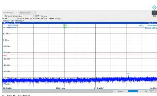
NTNV-n78(3450-3550)-PC1.5-30-50-M-DFT-BPSK-Inner_1RB_Left-30-1000-PASS
