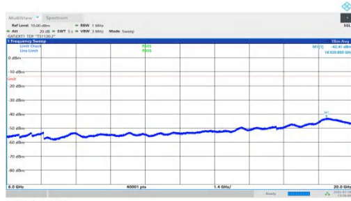
NTNV-n78(3450-3550)-PC1.5-30-40-H-DFT-QPSK-Inner_1RB_Left-6000-20000-PASS
