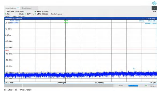
NTNV-n78(3450-3550)-PC1.5-30-60-H-DFT-QPSK-Inner_1RB_Right-3 0-1000-PASS
