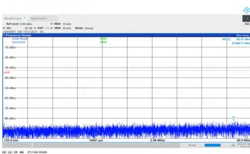
NTV-n78(3450-3550)-PC1.5-30-50-L-DFT-QPSK-Inner_1RB_Right- 0.15-30-PASS
