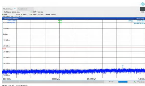
NTNV-n78(3450-3550)-PC1.5-30-60-H-DFT-QPSK-Inner_1RB_Left-30-1000-PASS
