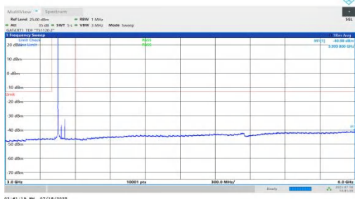
NTNV-n78(3450-3550)-PC1.5-30-60-L-DFT-BPSK-Inner_1RB_Left-30 00-6000-PASS
