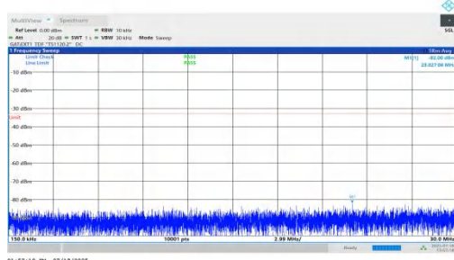
NTNV-n78(3450-3550)-PC1.5-30-40-H-DFT-QPSK-Inner_1RB_Left-0.15-30-PASS
