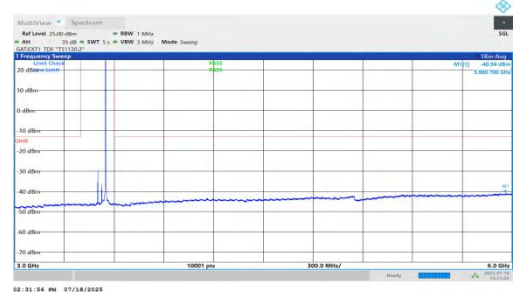
NTNV-n78(3450-3550)-PC1.5-30-50-H-DFT-BPSK-Inner_1RB_Right-3 000-6000-PASS
