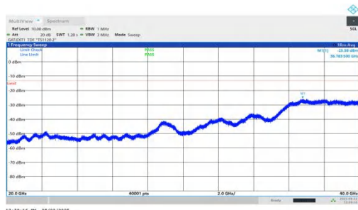
NTNV-n78(3450-3550)-PC1.5-30-70-L-DFT-QPSK-Inner_1RB_Right-20000-40000-PASS
