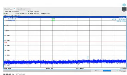
NTV-n78(3450-3550)-PC1.5-30-50-L-DFT-QPSK-Inner_1RB_Right-3 0-1000-PASS
