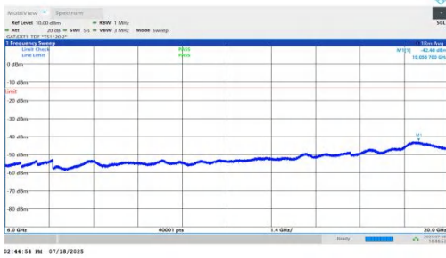
NTNV-n78(3450-3550)-PC1.5-30-60-L-DFT-BPSK-Inner_1RB_Right-6000-20000-PASS
