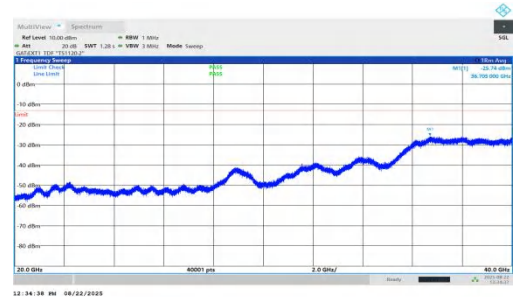
NTNV-n78(3450-3550)-PC1.5-30-60-M-DFT-QPSK-Inner_1RB_Right-20000-40000-PASS
