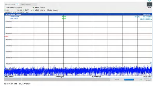
NTNV-n78(3450-3550)-PC1.5-30-50-H-DFT-BPSK-Inner_1RB_Left-0.15-30-PASS
