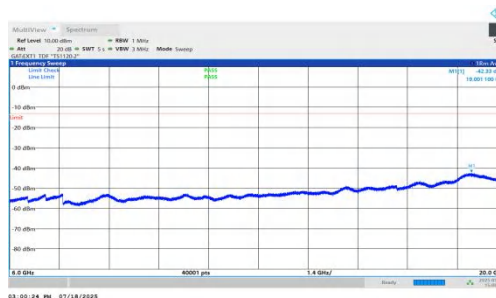
NTNV-n78(3450-3550)-PC1.5-30-60-M-DFT-QPSK-Inner_1RB_Left-60 00-20000-PASS
