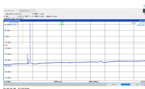
NTNV-n78(3450-3550)-PC1.5-30-60-H-DFT-BPSK-Inner_1RB_Right-3 000-6000-PASS
