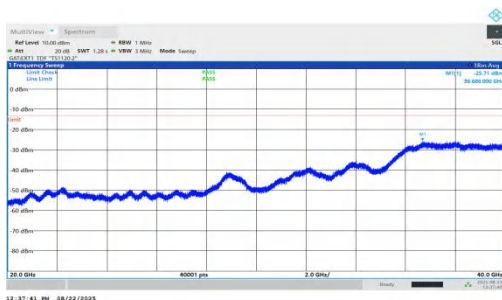
NTNV-n78(3450-3550)-PC1.5-30-70-L-DFT-BPSK-Inner_1RB_Left-20000-40000-PASS
