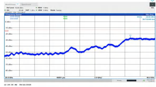
NTNV-n78(3450-3550)-PC1.5-30-50-M-DFT-BPSK-Inner_1RB_Right-20000-40000-PASS
