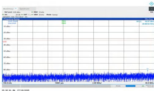
NTNV-n78(3450-3550)-PC1.5-30-70-M-DFT-BPSK-Inner_1RB_Right- 0.15-30-PASS
