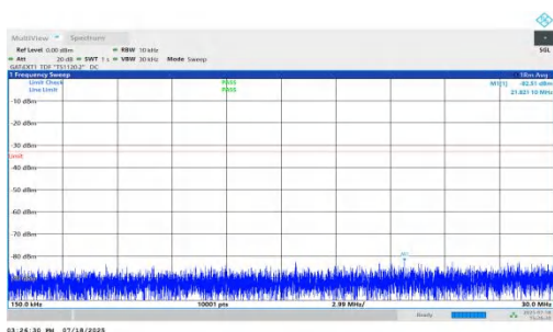
NTNV-n78(3450-3550)-PC1.5-30-70-L-DFT-QPSK-Inner_1RB_Right- 0.15-30-PASS
