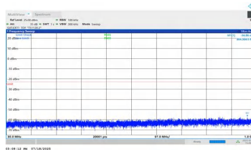
NTNV-n78(3450-3550)-PC1.5-30-60-H-DFT-BPSK-Inner_1RB_Right-3 0-1000-PASS
