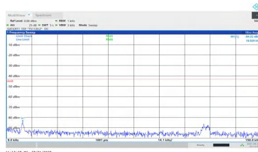
NTNV-n78(3450-3550)-PC1.5-30-40-H-DFT-BPSK-Inner_1RB_Right-0 .009-0.15-PASS
