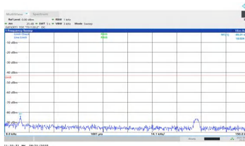
NTNV-n78(3450-3550)-PC1.5-30-50-H-DFT-QPSK-Inner_1RB_Right-0 .009-0.15-PASS
