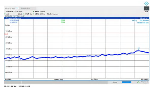
NTNV-n78(3450-3550)-PC1.5-30-70-L-DFT-BPSK-Inner_1RB_Left-6000-20000-PASS
