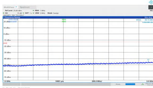
NTNV-n78(3450-3550)-PC1.5-30-40-H-DFT-QPSK-Inner_1RB_Left-1000-3000-PASS
