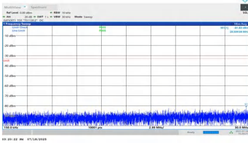
NTNV-n78(3450-3550)-PC1.5-30-70-L-DFT-BPSK-Inner_1RB_Right-0.15-30-PASS
