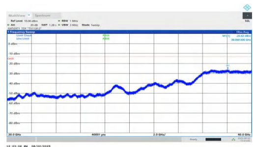
NTNV-n78(3450-3550)-PC1.5-30-40-H-DFT-QPSK-Inner_1RB_Right-2 0000-40000-PASS
