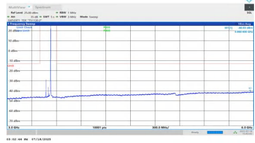
NTNV-n78(3450-3550)-PC1.5-30-60-M-DFT-QPSK-Inner_1RB_Right-3000-6000-PASS
