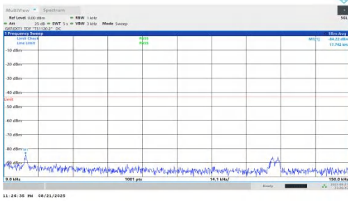
NTNV-n78(3450-3550)-PC1.5-30-60-M-DFT-BPSK-Inner_1RB_Left-0.009-0.15-PASS
