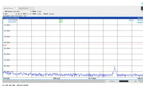
NTNV-n78(3450-3550)-PC1.5-30-60-M-DFT-QPSK-Inner_1RB_Right- 0.009-0.15-PASS
