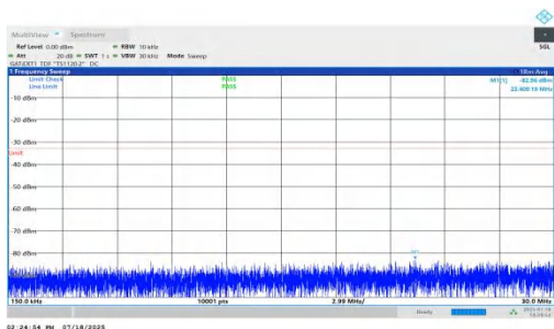
NTNV-n78(3450-3550)-PC1.5-30-50-M-DFT-QPSK-Inner_1RB_Right- 0.15-30-PASS
