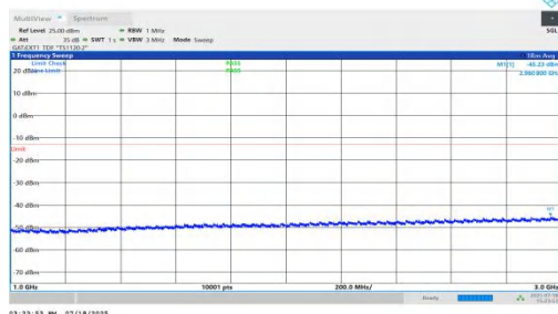
NTNV-n78(3450-3550)-PC1.5-30-70-L-DFT-QPSK-Inner_1RB_Left-10 00-3000-PASS
