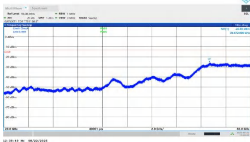
NTNV-n78(3450-3550)-PC1.5-30-70-L-DFT-QPSK-Inner_1RB_Left-2 0000-40000-PASS
