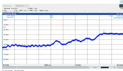
NTNV-n78(3450-3550)-PC1.5-30-70-M-DFT-BPSK-Inner_1RB_Right-20000-40000-PASS
