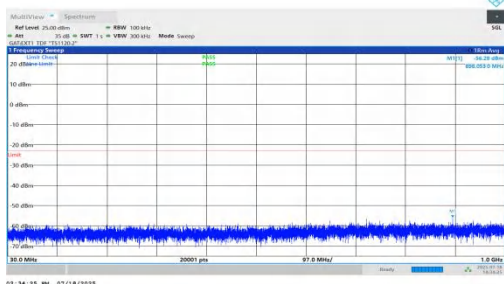
NTNV-n78(3450-3550)-PC1.5-30-50-H-DFT-QPSK-Inner_1RB_Left-3 0-1000-PASS
