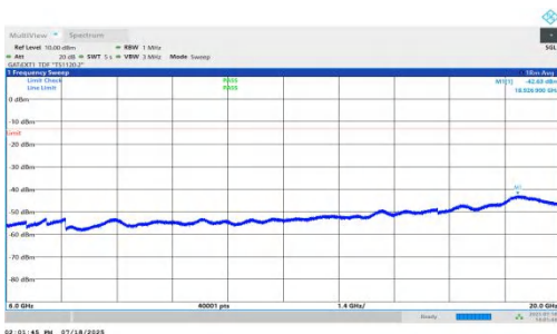
NTNV-n78(3450-3550)-PC1.5-30-40-H-DFT-QPSK-Inner_1RB_Right- 6000-20000-PASS
