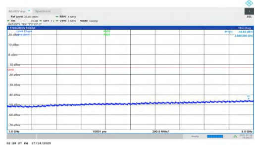
NTNV-n78(3450-3550)-PC1.5-30-50-H-DFT-BPSK-Inner_1RB_Left-1000-3000-PASS
