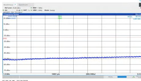
NTNV-n78(3450-3550)-PC1.5-30-60-M-DFT-QPSK-Inner_1RB_Left-10 00-3000-PASS
