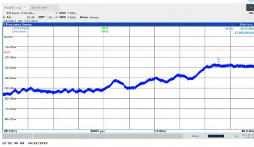
NTNV-n78(3450-3550)-PC1.5-30-40-H-DFT-QPSK-Inner_1RB_Left-2 0000-40000-PASS
