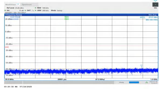
NTNV-n78(3450-3550)-PC1.5-30-70-L-DFT-BPSK-Inner_1RB_Right-3 0-1000-PASS
