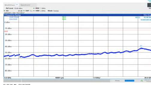
NTNV-n78(3450-3550)-PC1.5-30-40-H-DFT-BPSK-Inner_1RB_Left-60 00-20000-PASS
