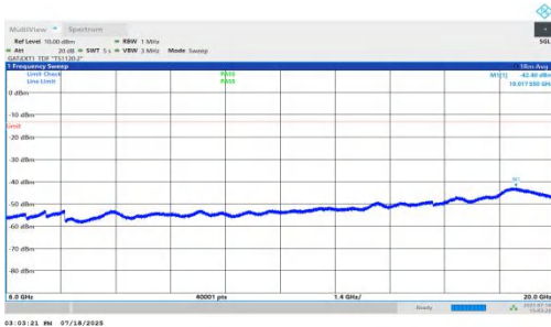
NTNV-n78(3450-3550)-PC1.5-30-60-M-DFT-QPSK-Inner_1RB_Right-6000-20000-PASS
