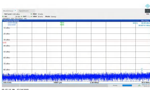
NTNV-n78(3450-3550)-PC1.5-30-50-H-DFT-QPSK-Inner_1RB_Right- 0.15-30-PASS
