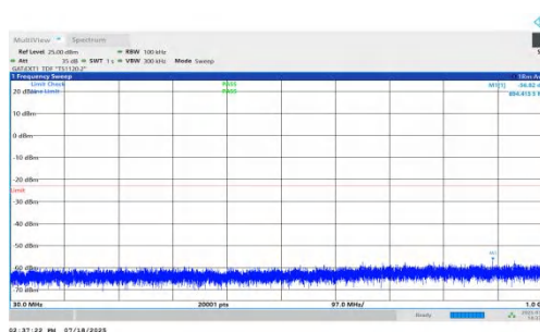
NTNV-n78(3450-3550)-PC1.5-30-50-H-DFT-QPSK-Inner_1RB_Right-3 0-1000-PASS
