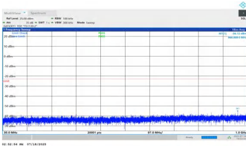
NTNV-n78(3450-3550)-PC1.5-30-60-M-DFT-BPSK-Inner_1RB_Left-30-1000-PASS
