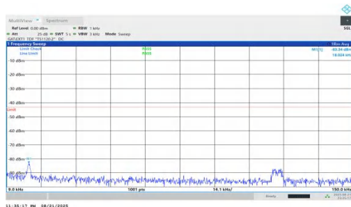
NTNV-n78(3450-3550)-PC1.5-30-70-M-DFT-BPSK-Inner_1RB_Right-0 .009-0.15-PASS
