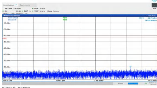
NTNV-n78(3450-3550)-PC1.5-30-60-M-DFT-BPSK-Inner_1RB_Right-0.15-30-PASS
