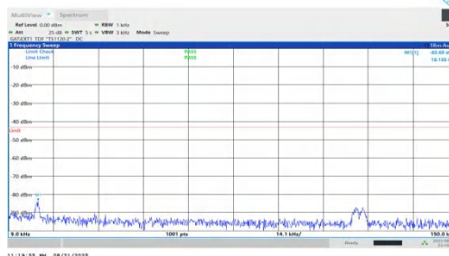
NTNV-n78(3450-3550)-PC1.5-30-50-M-DFT-QPSK-Inner_1RB_Right- 0.009-0.15-PASS
