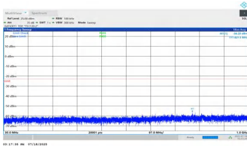
NTNV-n78(3450-3550)-PC1.5-30-70-L-DFT-BPSK-Inner_1RB_Left-30-1000-PASS
