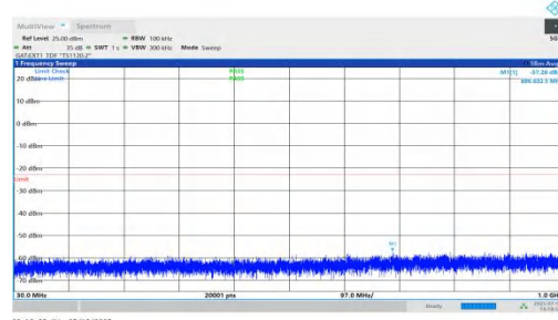
NTNV-n78(3450-3550)-PC1.5-30-50-M-DFT-BPSK-Inner_1RB_Right-3 0-1000-PASS
