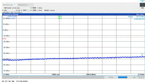
NTNV-n78(3450-3550)-PC1.5-30-50-H-DFT-QPSK-Inner_1RB_Right-1000-3000-PASS
