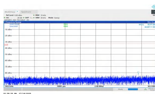
NTNV-n78(3450-3550)-PC1.5-30-60-M-DFT-QPSK-Inner_1RB_Left-0 15-30-PASS
