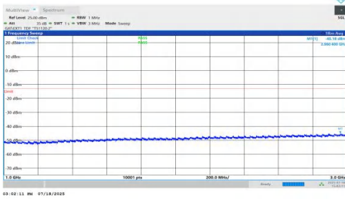
NTNV-n78(3450-3550)-PC1.5-30-60-M-DFT-QPSK-Inner_1RB_Right-1000-3000-PASS
