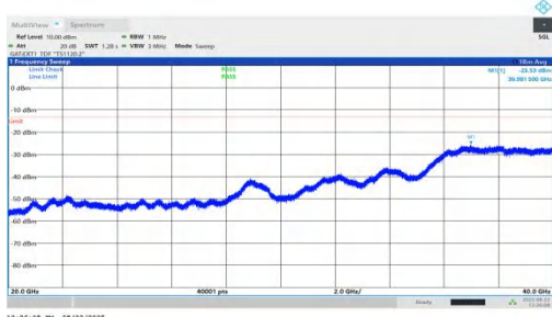
NTNV-n78(3450-3550)-PC1.5-30-50-M-DFT-BPSK-Inner_1RB_Left-2 0000-40000-PASS
