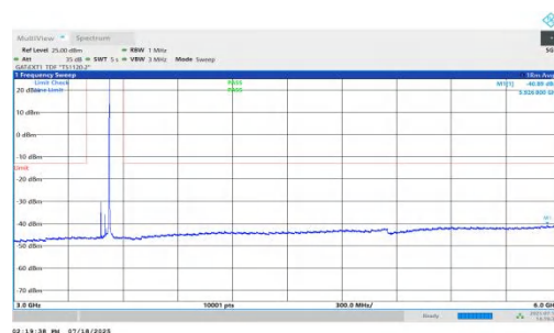
NTNV-n78(3450-3550)-PC1.5-30-50-M-DFT-BPSK-Inner_1RB_Right-3 000-6000-PASS
