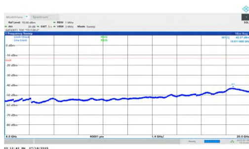
NTNV-n78(3450-3550)-PC1.5-30-60-H-DFT-QPSK-Inner_1RB_Left-6000-20000-PASS
