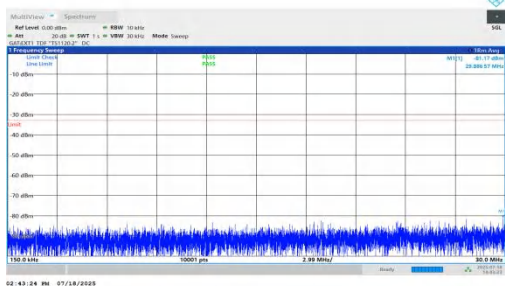
NTNV-n78(3450-3550)-PC1.5-30-60-L-DFT-BPSK-Inner_1RB_Right- 0.15-30-PASS
