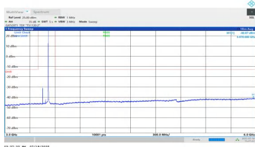
NTNV-n78(3450-3550)-PC1.5-30-70-L-DFT-QPSK-Inner_1RB_Right-3000-6000-PASS
