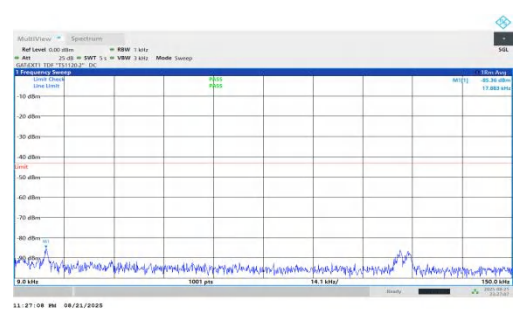
NTNV-n78(3450-3550)-PC1.5-30-60-M-DFT-BPSK-Inner_1RB_Right-0.009-0.15-PASS
