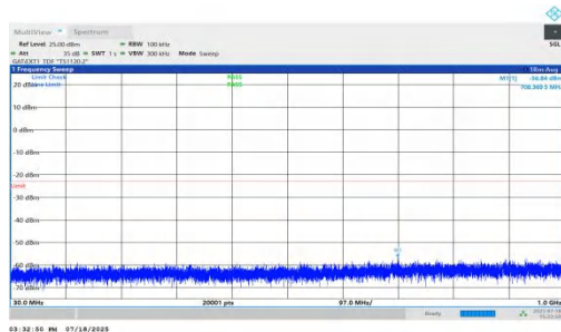
NTNV-n78(3450-3550)-PC1.5-30-70-M-DFT-BPSK-Inner_1RB_Right-3 0-1000-PASS
