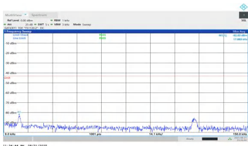
NTNV-n78(3450-3550)-PC1.5-30-70-M-DFT-BPSK-Inner_1RB_Left-0.009-0.15-PASS
