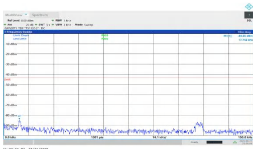
NTNV-n78(3450-3550)-PC1.5-30-70-M-DFT-QPSK-Inner_1RB_Left-0.009-0.15-PASS
