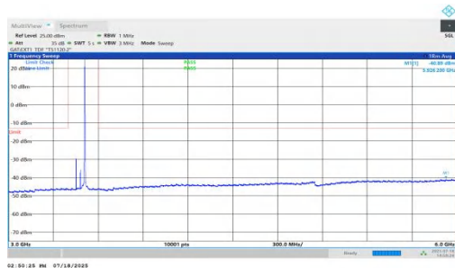
NTNV-n78(3450-3550)-PC1.5-30-60-L-DFT-QPSK-Inner_1RB_Right-3 000-6000-PASS
