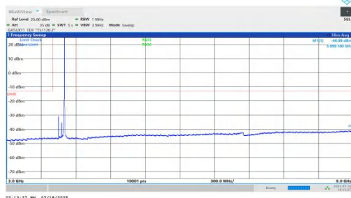
NTNV-n78(3450-3550)-PC1.5-30-50-L-DFT-QPSK-Inner_1RB_Right-3000-6000-PASS
