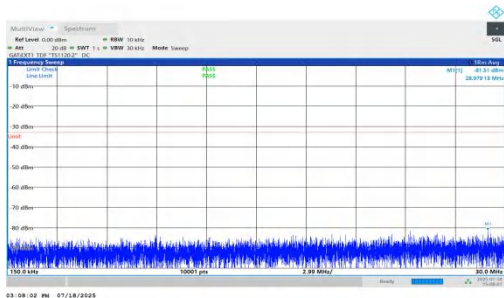
NTNV-n78(3450-3550)-PC1.5-30-60-H-DFT-BPSK-Inner_1RB_Right- 0.15-30-PASS
