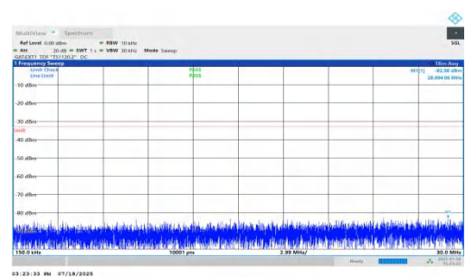
NTNV-n78(3450-3550)-PC1.5-30-70-L-DFT-QPSK-Inner_1RB_Left-0.1 5-30-PASS
