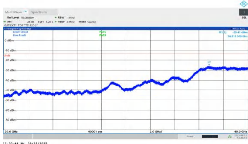
NTNV-n78(3450-3550)-PC1.5-30-60-L-DFT-BPSK-Inner_1RB_Left-20 000-40000-PASS
