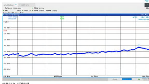
NTNV-n78(3450-3550)-PC1.5-30-70-M-DFT-BPSK-Inner_1RB_Left-60 00-20000-PASS
