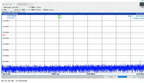
NTNV-n78(3450-3550)-PC1.5-30-50-H-DFT-BPSK-Inner_1RB_Right-0.15-30-PASS
