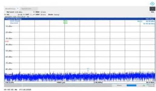
NTNV-n78(3450-3550)-PC1.5-30-60-H-DFT-BPSK-Inner_1RB_Left-0.15-30-PASS
