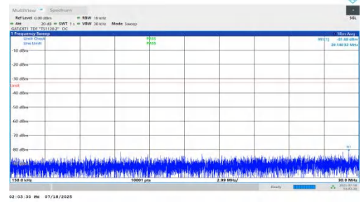
NTNV-n78(3450-3550)-PC1.5-30-50-L-DFT-BPSK-Inner_1RB_Left-0.15-30-PASS
