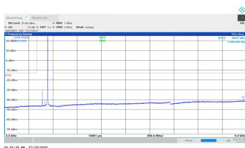
NTNV-n78(3450-3550)-PC1.5-30-70-M-DFT-BPSK-Inner_1RB_Right-3 000-6000-PASS
