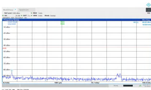
NTNV-n78(3450-3550)-PC1.5-30-50-M-DFT-BPSK-Inner_1RB_Left-0.009-0.15-PASS
