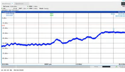
NTNV-n78(3450-3550)-PC1.5-30-60-H-DFT-QPSK-Inner_1RB_Left-2 0000-40000-PASS
