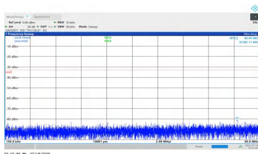
NTNV-n78(3450-3550)-PC1.5-30-50-M-DFT-BPSK-Inner_1RB_Left-0.15-30-PASS
