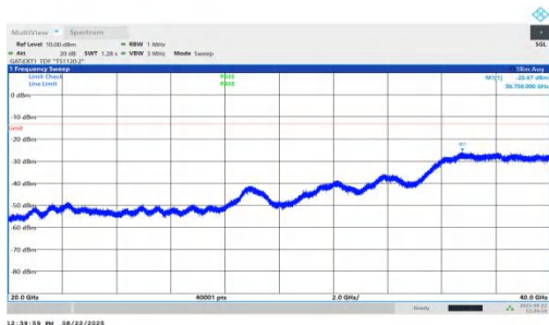
NTNV-n78(3450-3550)-PC1.5-30-70-M-DFT-BPSK-Inner_1RB_Left-2 0000-40000-PASS
