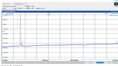
NTNV-n78(3450-3550)-PC1.5-30-50-M-DFT-BPSK-Inner_1RB_Left-3 000-6000-PASS
