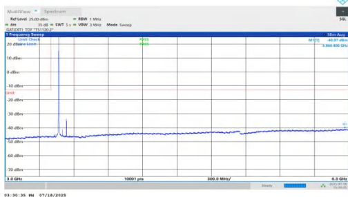
NTNV-n78(3450-3550)-PC1.5-30-70-M-DFT-BPSK-Inner_1RB_Left-3 000-6000-PASS
