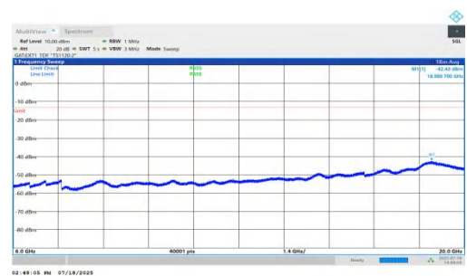
NTNV-n78(3450-3550)-PC1.5-30-60-L-DFT-QPSK-Inner_1RB_Left-6000-20000-PASS
