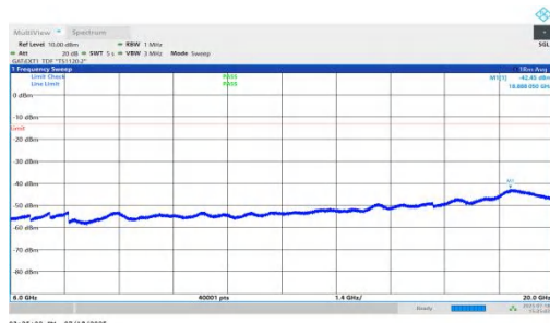
NTNV-n78(3450-3550)-PC1.5-30-70-L-DFT-QPSK-Inner_1RB_Left-60 00-20000-PASS
