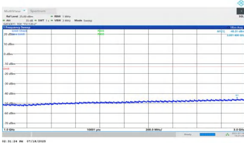
NTNV-n78(3450-3550)-PC1.5-30-50-H-DFT-BPSK-Inner_1RB_Right-1000-3000-PASS
