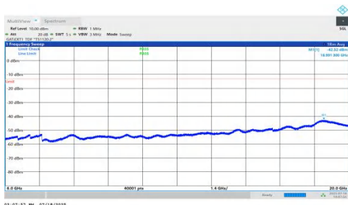
NTV-n78(3450-3550)-PC1.5-30-50-L-DFT-BPSK-Inner_1RB_Right-6000-20000-PASS
