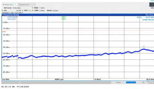
NTNV-n78(3450-3550)-PC1.5-30-50-M-DFT-BPSK-Inner_1RB_Right-6000-20000-PASS
