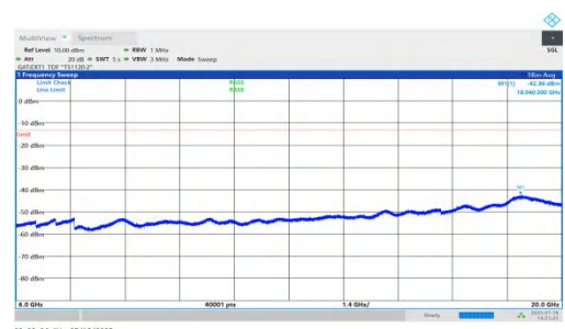
NTNV-n78(3450-3550)-PC1.5-30-50-M-DFT-QPSK-Inner_1RB_Left-6000-20000-PASS
