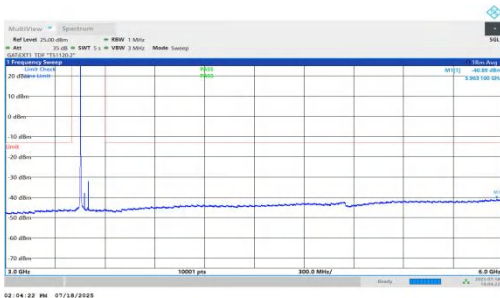
NTNV-n78(3450-3550)-PC1.5-30-50-L-DFT-BPSK-Inner_1RB_Left-3000-6000-PASS
