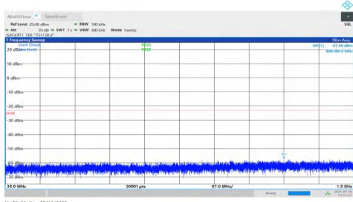
NTNV-n78(3450-3550)-PC1.5-30-40-H-DFT-QPSK-Inner_1RB_Left-30-1000-PASS
