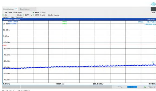
NTV-n78(3450-3550)-PC1.5-30-50-L-DFT-BPSK-Inner_1RB_Right-1000-3000-PASS
