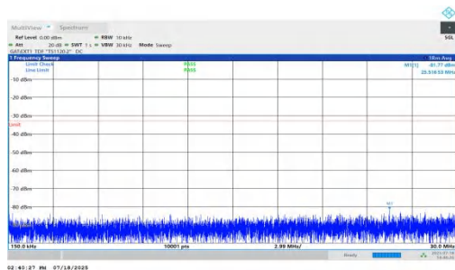
NTNV-n78(3450-3550)-PC1.5-30-60-L-DFT-BPSK-Inner_1RB_Left-0.15-30-PASS
