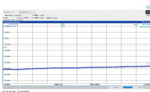
NTNV-n78(3450-3550)-PC1.5-30-50-M-DFT-BPSK-Inner_1RB_Left-1000-3000-PASS
