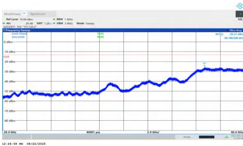
NTV-n78(3450-3550)-PC1.5-30-50-L-DFT-QPSK-Inner_1RB_Left-2 0000-40000-PASS
