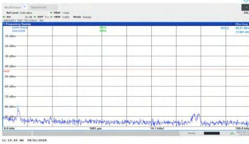
NTNV-n78(3450-3550)-PC1.5-30-50-L-DFT-BPSK-Inner_1RB_Left-0.009-0.15-PASS
