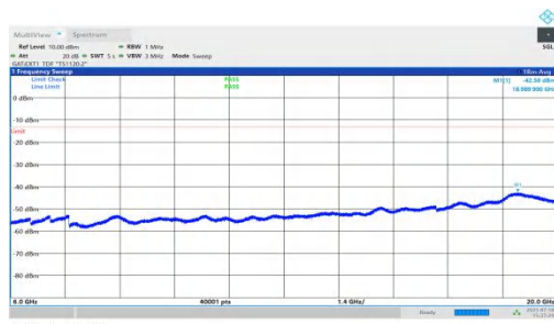
NTNV-n78(3450-3550)-PC1.5-30-70-M-DFT-QPSK-Inner_1RB_Left-6000-20000-PASS
