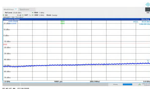
NTNV-n78(3450-3550)-PC1.5-30-60-L-DFT-BPSK-Inner_1RB_Left-1000-3000-PASS
