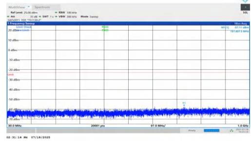
NTNV-n78(3450-3550)-PC1.5-30-50-H-DFT-BPSK-Inner_1RB_Right-3 0-1000-PASS
