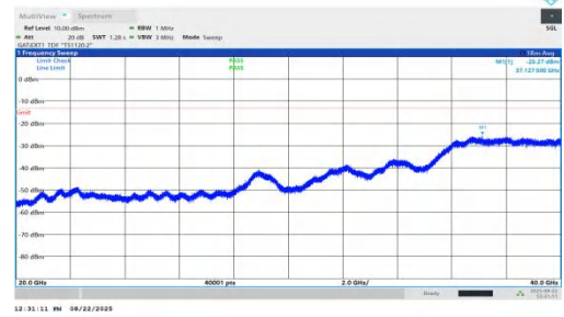
NTNV-n78(3450-3550)-PC1.5-30-60-L-DFT-BPSK-Inner_1RB_Right-20000-40000-PASS
