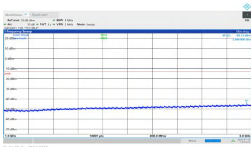
NTNV-n78(3450-3550)-PC1.5-30-40-H-DFT-BPSK-Inner_1RB_Right- 1000-3000-PASS
