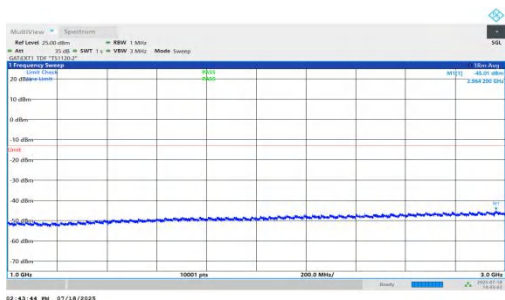
NTNV-n78(3450-3550)-PC1.5-30-60-L-DFT-BPSK-Inner_1RB_Right- 1000-3000-PASS
