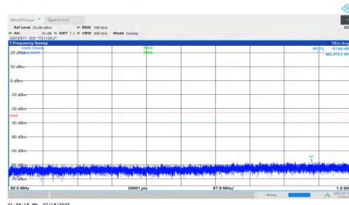
NTNV-n78(3450-3550)-PC1.5-30-40-H-DFT-BPSK-Inner_1RB_Right-3 0-1000-PASS
