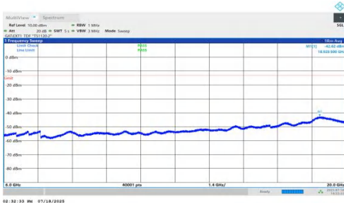
NTNV-n78(3450-3550)-PC1.5-30-50-H-DFT-BPSK-Inner_1RB_Right-6000-20000-PASS
