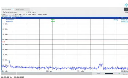
NTNV-n78(3450-3550)-PC1.5-30-70-L-DFT-QPSK-Inner_1RB_Left-0.009-0.15-PASS
