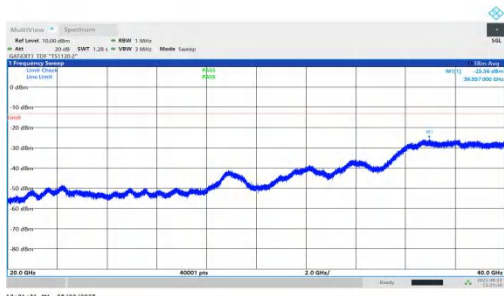
NTNV-n78(3450-3550)-PC1.5-30-40-H-DFT-BPSK-Inner_1RB_Left-2 0000-40000-PASS
