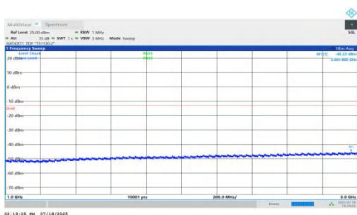
NTNV-n78(3450-3550)-PC1.5-30-50-M-DFT-BPSK-Inner_1RB_Right- 1000-3000-PASS
