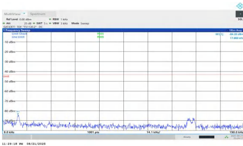
NTNV-n78(3450-3550)-PC1.5-30-60-H-DFT-BPSK-Inner_1RB_Left-0.009-0.15-PASS
