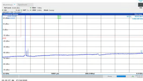
NTNV-n78(3450-3550)-PC1.5-30-60-H-DFT-BPSK-Inner_1RB_Left-3 000-6000-PASS
