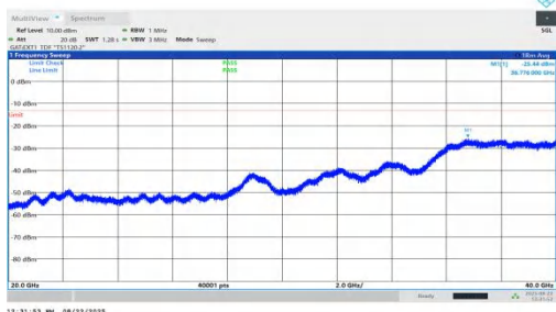
NTNV-n78(3450-3550)-PC1.5-30-60-L-DFT-QPSK-Inner_1RB_Left-2 0000-40000-PASS
