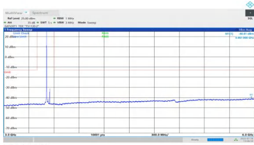
NTNV-n78(3450-3550)-PC1.5-30-40-H-DFT-QPSK-Inner_1RB_Left-3000-6000-PASS
