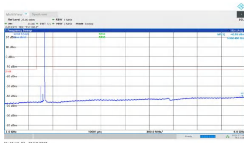
NTV-n78(3450-3550)-PC1.5-30-50-L-DFT-BPSK-Inner_1RB_Right-3 000-6000-PASS
