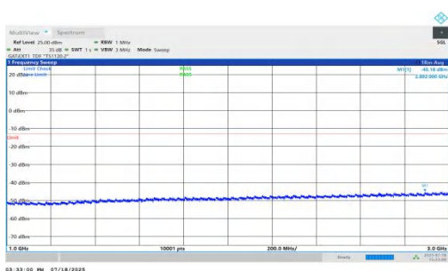
NTNV-n78(3450-3550)-PC1.5-30-70-M-DFT-BPSK-Inner_1RB_Right- 1000-3000-PASS
