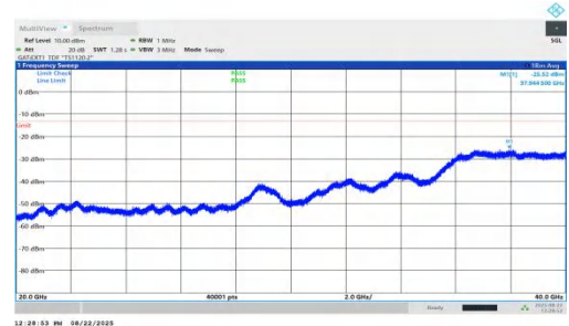
NTNV-n78(3450-3550)-PC1.5-30-50-H-DFT-BPSK-Inner_1RB_Right-2 0000-40000-PASS
