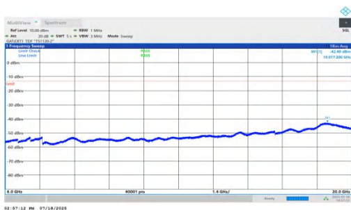
NTNV-n78(3450-3550)-PC1.5-30-60-M-DFT-BPSK-Inner_1RB_Right-6000-20000-PASS
