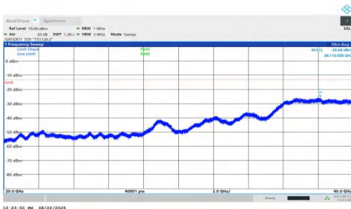
NTNV-n78(3450-3550)-PC1.5-30-50-L-DFT-BPSK-Inner_1RB_Left-20000-40000-PASS
