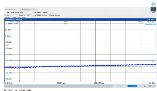
NTNV-n78(3450-3550)-PC1.5-30-50-M-DFT-QPSK-Inner_1RB_Left-1000-3000-PASS
