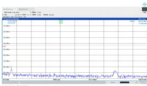
NTV-n78(3450-3550)-PC1.5-30-50-L-DFT-QPSK-Inner_1RB_Left-0.009-0.15-PASS
