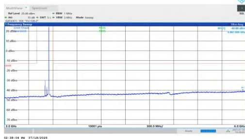
NTNV-n78(3450-3550)-PC1.5-30-50-H-DFT-QPSK-Inner_1RB_Right-3000-6000-PASS
