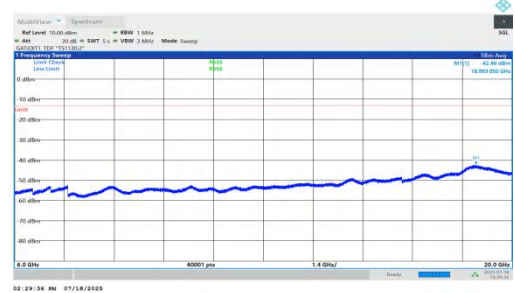
NTNV-n78(3450-3550)-PC1.5-30-50-H-DFT-BPSK-Inner_1RB_Left-6000-20000-PASS
