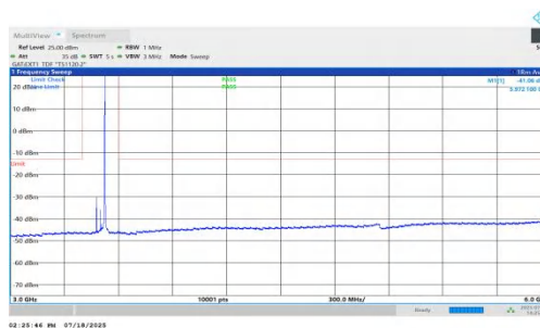
NTNV-n78(3450-3550)-PC1.5-30-50-M-DFT-QPSK-Inner_1RB_Right- 3000-6000-PASS
