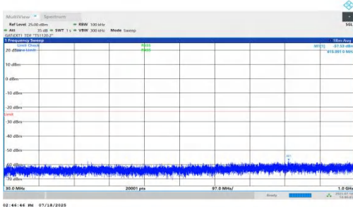
NTNV-n78(3450-3550)-PC1.5-30-60-L-DFT-QPSK-Inner_1RB_Left-30-1000-PASS
