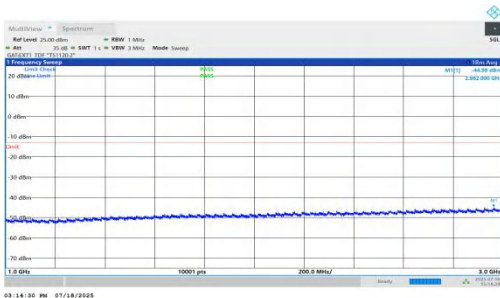
NTNV-n78(3450-3550)-PC1.5-30-60-H-DFT-QPSK-Inner_1RB_Right- 1000-3000-PASS
