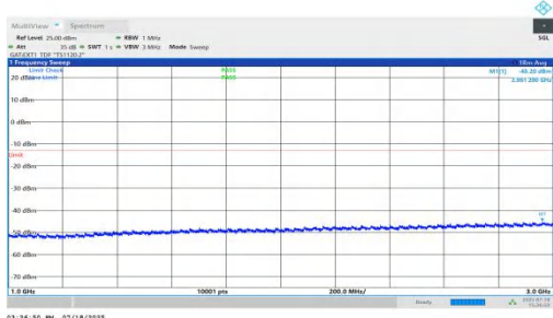
NTNV-n78(3450-3550)-PC1.5-30-70-L-DFT-QPSK-Inner_1RB_Right-1000-3000-PASS
