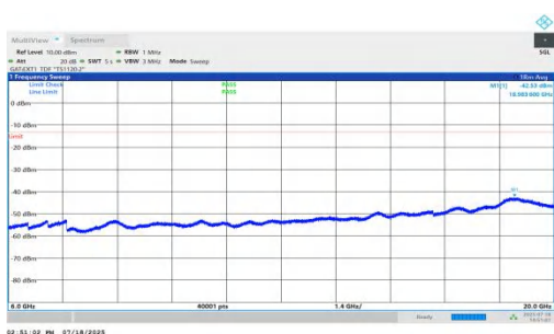
NTNV-n78(3450-3550)-PC1.5-30-60-L-DFT-QPSK-Inner_1RB_Right- 6000-20000-PASS
