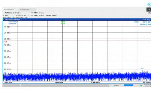
NTV-n78(3450-3550)-PC1.5-30-50-L-DFT-QPSK-Inner_1RB_Left-0.1 5-30-PASS
