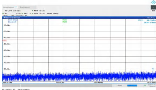
NTV-n78(3450-3550)-PC1.5-30-50-L-DFT-BPSK-Inner_1RB_Right-0.15-30-PASS
