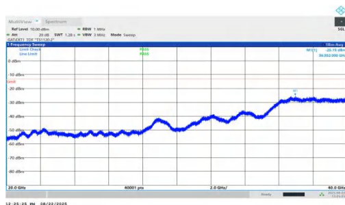
NTNV-n78(3450-3550)-PC1.5-30-50-L-DFT-QPSK-Inner_1RB_Right-20000-40000-PASS
