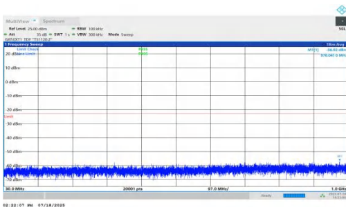
NTNV-n78(3450-3550)-PC1.5-30-50-M-DFT-QPSK-Inner_1RB_Left-30-1000-PASS
