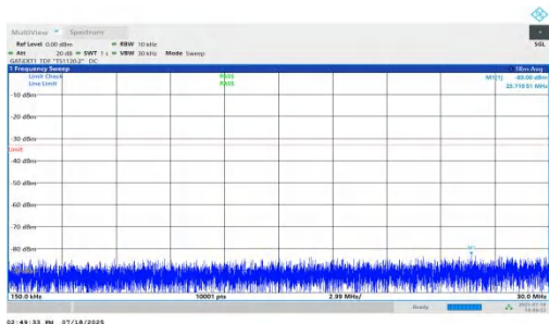
NTNV-n78(3450-3550)-PC1.5-30-60-L-DFT-QPSK-Inner_1RB_Right- 0.15-30-PASS
