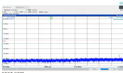
NTNV-n78(3450-3550)-PC1.5-30-60-L-DFT-QPSK-Inner_1RB_Right-3 0-1000-PASS
