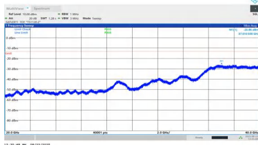
NTNV-n78(3450-3550)-PC1.5-30-60-H-DFT-BPSK-Inner_1RB_Right-20000-40000-PASS
