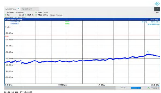
NTNV-n78(3450-3550)-PC1.5-30-60-M-DFT-BPSK-Inner_1RB_Left-6000-20000-PASS
