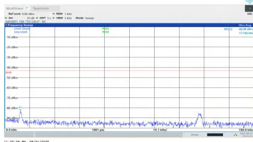
NTNV-n78(3450-3550)-PC1.5-30-60-L-DFT-QPSK-Inner_1RB_Right-0 .009-0.15-PASS
