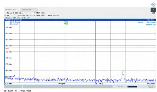
NTNV-n78(3450-3550)-PC1.5-30-50-H-DFT-BPSK-Inner_1RB_Right-0.009-0.15-PASS
