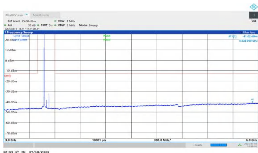
NTNV-n78(3450-3550)-PC1.5-30-60-M-DFT-QPSK-Inner_1RB_Left-3 000-6000-PASS
