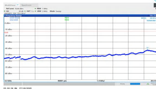
NTNV-n78(3450-3550)-PC1.5-30-60-H-DFT-BPSK-Inner_1RB_Left-60 00-20000-PASS
