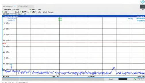
NTNV-n78(3450-3550)-PC1.5-30-40-H-DFT-QPSK-Inner_1RB_Left-0.009-0.15-PASS
