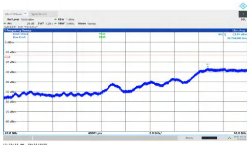
NTNV-n78(3450-3550)-PC1.5-30-50-H-DFT-QPSK-Inner_1RB_Left-2 0000-40000-PASS
