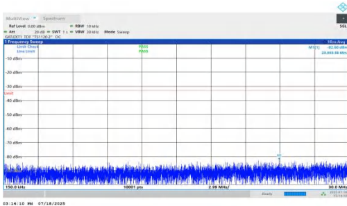
NTNV-n78(3450-3550)-PC1.5-30-60-H-DFT-QPSK-Inner_1RB_Right- 0.15-30-PASS
