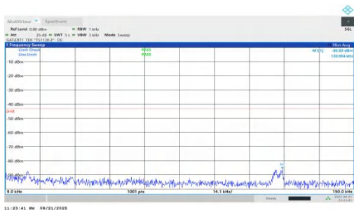
NTNV-n78(3450-3550)-PC1.5-30-60-L-DFT-BPSK-Inner_1RB_Left-0.009-0.15-PASS
