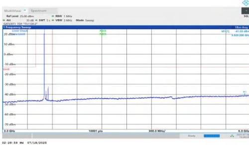
NTNV-n78(3450-3550)-PC1.5-30-50-H-DFT-BPSK-Inner_1RB_Left-3000-6000-PASS
