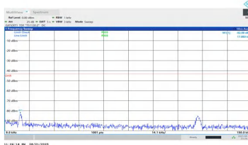
NTNV-n78(3450-3550)-PC1.5-30-60-L-DFT-BPSK-Inner_1RB_Right-0. 009-0.15-PASS
