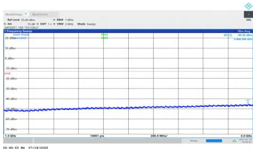
NTNV-n78(3450-3550)-PC1.5-30-60-L-DFT-QPSK-Inner_1RB_Right- 1000-3000-PASS
