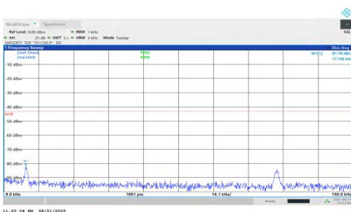
NTNV-n78(3450-3550)-PC1.5-30-50-H-DFT-QPSK-Inner_1RB_Left-0.009-0.15-PASS
