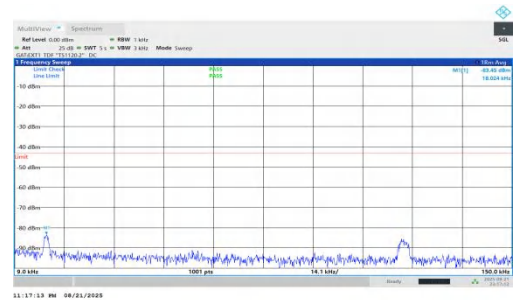
NTV-n78(3450-3550)-PC1.5-30-50-L-DFT-QPSK-Inner_1RB_Right-0 .009-0.15-PASS
