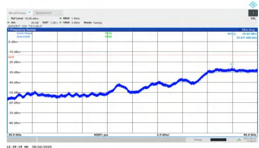
NTNV-n78(3450-3550)-PC1.5-30-70-L-DFT-BPSK-Inner_1RB_Right-2 0000-40000-PASS
