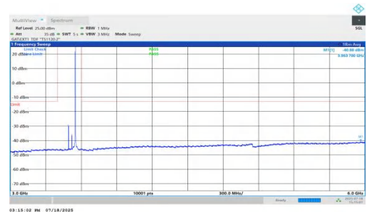
NTNV-n78(3450-3550)-PC1.5-30-60-H-DFT-QPSK-Inner_1RB_Right-3 000-6000-PASS
