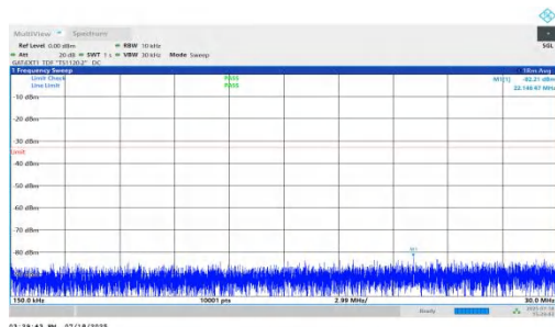
NTNV-n78(3450-3550)-PC1.5-30-70-M-DFT-BPSK-Inner_1RB_Left-0.15-30-PASS
