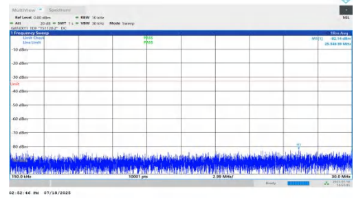
NTNV-n78(3450-3550)-PC1.5-30-60-M-DFT-BPSK-Inner_1RB_Left-0.15-30-PASS
