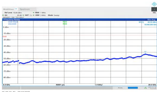
NTNV-n78(3450-3550)-PC1.5-30-70-L-DFT-QPSK-Inner_1RB_Right-6000-20000-PASS
