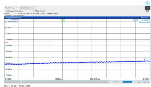
NTNV-n78(3450-3550)-PC1.5-30-50-L-DFT-BPSK-Inner_1RB_Left-1000-3000-PASS
