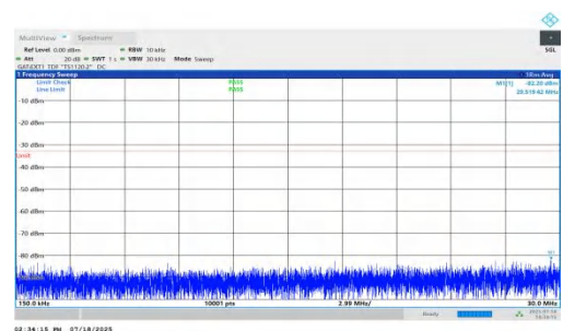
NTNV-n78(3450-3550)-PC1.5-30-50-H-DFT-QPSK-Inner_1RB_Left-0.15-30-PASS
