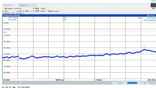
NTNV-n78(3450-3550)-PC1.5-30-40-H-DFT-BPSK-Inner_1RB_Right-6000-20000-PASS
