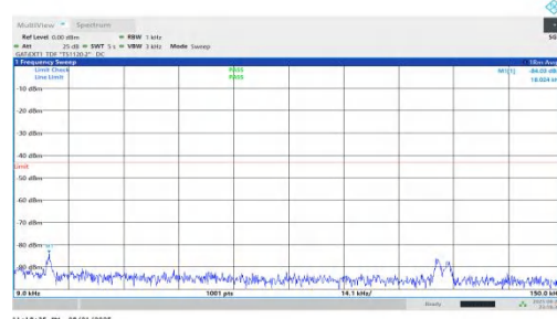
NTNV-n78(3450-3550)-PC1.5-30-50-M-DFT-BPSK-Inner_1RB_Right-0 .009-0.15-PASS
