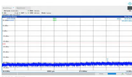
NTNV-n78(3450-3550)-PC1.5-30-70-M-DFT-QPSK-Inner_1RB_Left-30-1000-PASS
