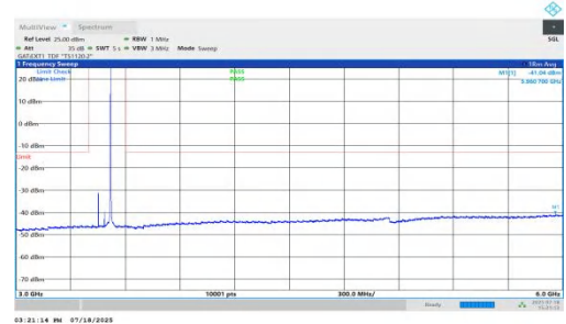
NTNV-n78(3450-3550)-PC1.5-30-70-L-DFT-BPSK-Inner_1RB_Right-3 000-6000-PASS
