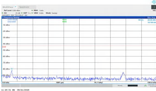
NTNV-n78(3450-3550)-PC1.5-30-60-L-DFT-QPSK-Inner_1RB_Left-0.009-0.15-PASS
