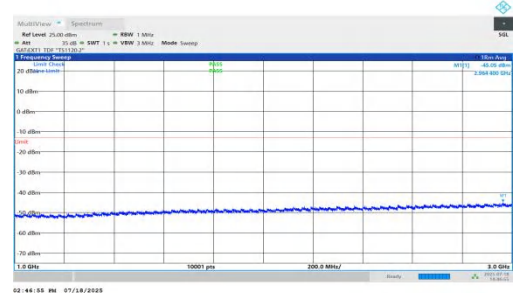
NTNV-n78(3450-3550)-PC1.5-30-60-L-DFT-QPSK-Inner_1RB_Left-1000-3000-PASS
