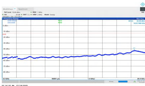
NTNV-n78(3450-3550)-PC1.5-30-50-L-DFT-QPSK-Inner_1RB_Right-6000-20000-PASS
