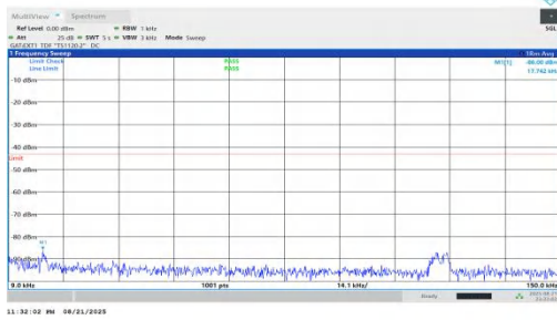
NTNV-n78(3450-3550)-PC1.5-30-70-L-DFT-BPSK-Inner_1RB_Left-0.009-0.15-PASS
