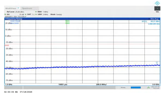
NTNV-n78(3450-3550)-PC1.5-30-60-M-DFT-BPSK-Inner_1RB_Left-1000-3000-PASS
