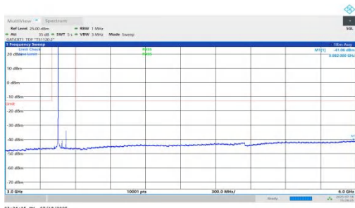
NTNV-n78(3450-3550)-PC1.5-30-70-L-DFT-QPSK-Inner_1RB_Left-3 000-6000-PASS
