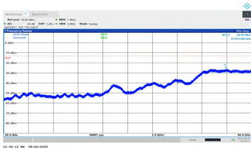
NTNV-n78(3450-3550)-PC1.5-30-60-M-DFT-QPSK-Inner_1RB_Left-2 0000-40000-PASS
