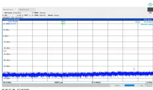
NTNV-n78(3450-3550)-PC1.5-30-60-L-DFT-BPSK-Inner_1RB_Left-30-1000-PASS
