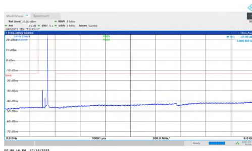
NTNV-n78(3450-3550)-PC1.5-30-60-L-DFT-BPSK-Inner_1RB_Right-3 000-6000-PASS
