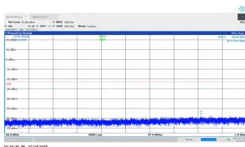
NTNV-n78(3450-3550)-PC1.5-30-70-L-DFT-QPSK-Inner_1RB_Right-3 0-1000-PASS
