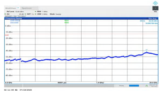
NTV-n78(3450-3550)-PC1.5-30-50-L-DFT-QPSK-Inner_1RB_Left-60 00-20000-PASS
