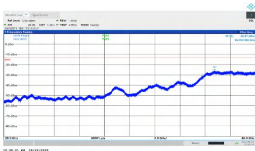
NTNV-n78(3450-3550)-PC1.5-30-60-H-DFT-BPSK-Inner_1RB_Left-2 0000-40000-PASS
