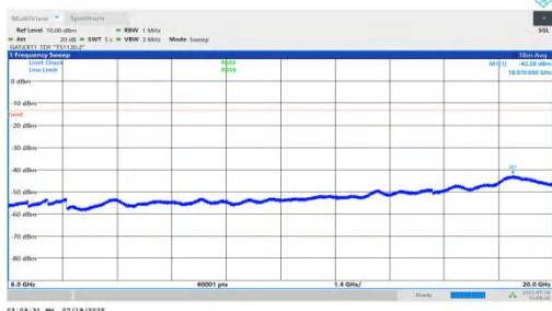
NTNV-n78(3450-3550)-PC1.5-30-60-H-DFT-BPSK-Inner_1RB_Right-6000-20000-PASS
