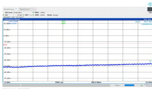
NTNV-n78(3450-3550)-PC1.5-30-70-M-DFT-QPSK-Inner_1RB_Left-1000-3000-PASS
