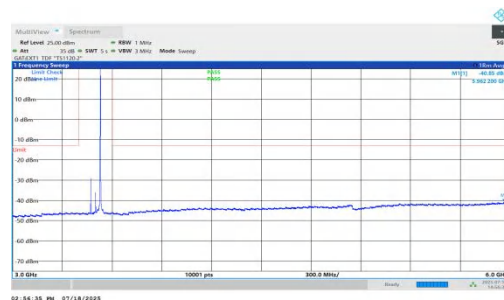
NTNV-n78(3450-3550)-PC1.5-30-60-M-DFT-BPSK-Inner_1RB_Right-3 000-6000-PASS
