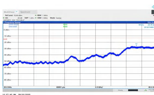
NTNV-n78(3450-3550)-PC1.5-30-50-M-DFT-QPSK-Inner_1RB_Right- 20000-40000-PASS
