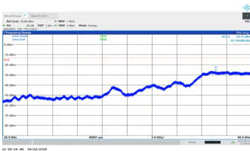
NTNV-n78(3450-3550)-PC1.5-30-50-H-DFT-BPSK-Inner_1RB_Left-20000-40000-PASS
