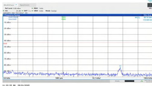
NTNV-n78(3450-3550)-PC1.5-30-70-L-DFT-QPSK-Inner_1RB_Right-0 .009-0.15-PASS
