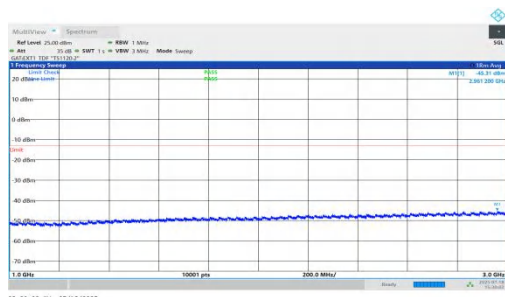
NTNV-n78(3450-3550)-PC1.5-30-70-M-DFT-BPSK-Inner_1RB_Left-1000-3000-PASS
