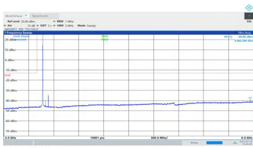
NTNV-n78(3450-3550)-PC1.5-30-70-M-DFT-QPSK-Inner_1RB_Left-3000-6000-PASS
