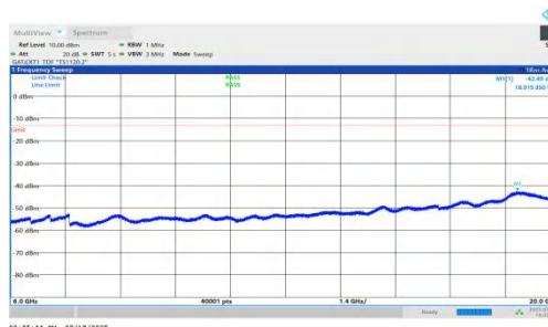
NTNV-n78(3450-3550)-PC1.5-30-50-H-DFT-QPSK-Inner_1RB_Left-60 00-20000-PASS
