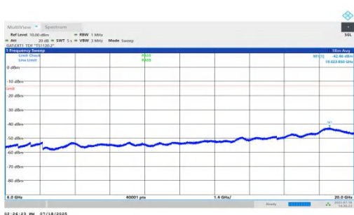
NTNV-n78(3450-3550)-PC1.5-30-50-M-DFT-QPSK-Inner_1RB_Right- 6000-20000-PASS
