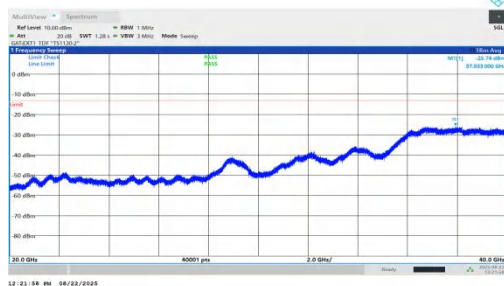
NTNV-n78(3450-3550)-PC1.5-30-40-H-DFT-BPSK-Inner_1RB_Right-20000-40000-PASS
