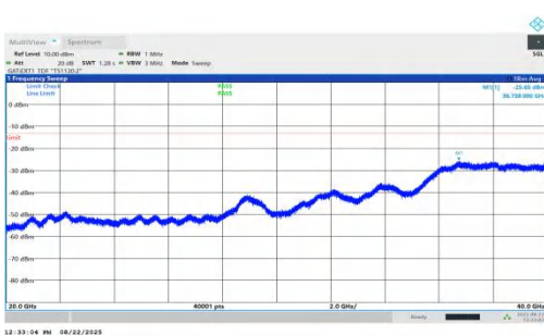
NTNV-n78(3450-3550)-PC1.5-30-60-M-DFT-BPSK-Inner_1RB_Left-20000-40000-PASS
