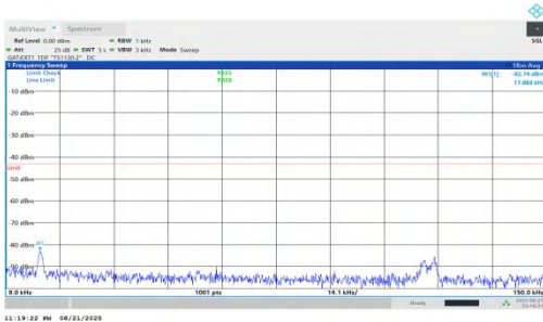
NTNV-n78(3450-3550)-PC1.5-30-50-M-DFT-QPSK-Inner_1RB_Left-0.009-0.15-PASS
