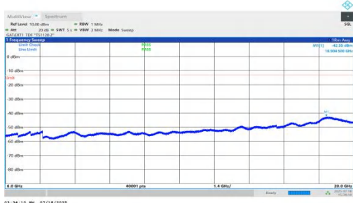
NTNV-n78(3450-3550)-PC1.5-30-70-M-DFT-BPSK-Inner_1RB_Right-6000-20000-PASS
