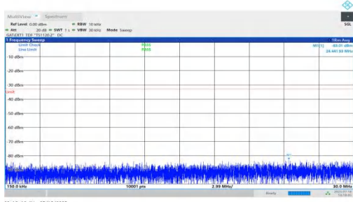
NTNV-n78(3450-3550)-PC1.5-30-50-M-DFT-BPSK-Inner_1RB_Right- 0.15-30-PASS
