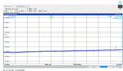
NTNV-n78(3450-3550)-PC1.5-30-70-L-DFT-BPSK-Inner_1RB_Left-1000-3000-PASS
