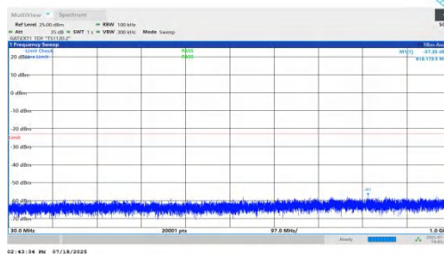
NTNV-n78(3450-3550)-PC1.5-30-60-L-DFT-BPSK-Inner_1RB_Right-3 0-1000-PASS
