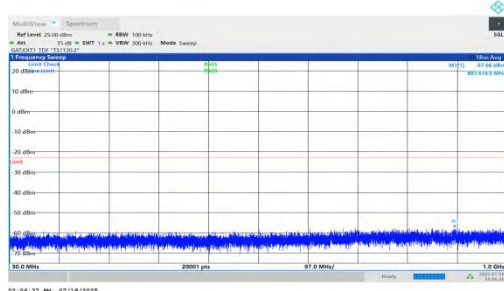
NTV-n78(3450-3550)-PC1.5-30-50-L-DFT-BPSK-Inner_1RB_Right-3 0-1000-PASS
