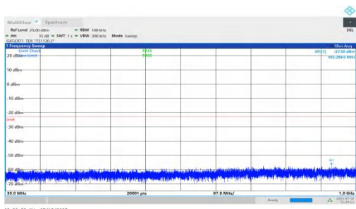
NTNV-n78(3450-3550)-PC1.5-30-70-M-DFT-BPSK-Inner_1RB_Left-30-1000-PASS
