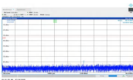
NTNV-n78(3450-3550)-PC1.5-30-60-M-DFT-QPSK-Inner_1RB_Right- 0.15-30-PASS
