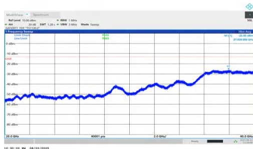
NTNV-n78(3450-3550)-PC1.5-30-50-H-DFT-QPSK-Inner_1RB_Right-20000-40000-PASS
