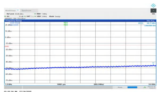
NTNV-n78(3450-3550)-PC1.5-30-60-H-DFT-BPSK-Inner_1RB_Left-1000-3000-PASS
