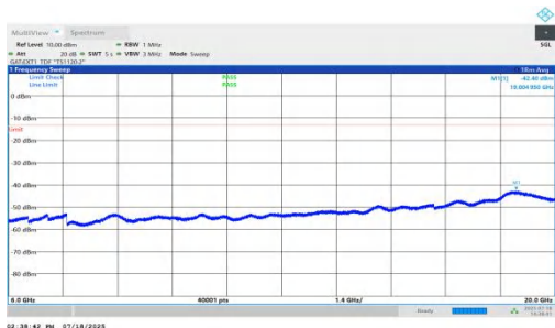
NTNV-n78(3450-3550)-PC1.5-30-50-H-DFT-QPSK-Inner_1RB_Right-6000-20000-PASS
