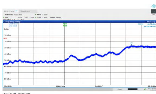
NTNV-n78(3450-3550)-PC1.5-30-60-L-DFT-QPSK-Inner_1RB_Right-2 0000-40000-PASS
