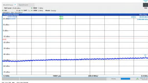
NTNV-n78(3450-3550)-PC1.5-30-50-L-DFT-QPSK-Inner_1RB_Right-1000-3000-PASS
