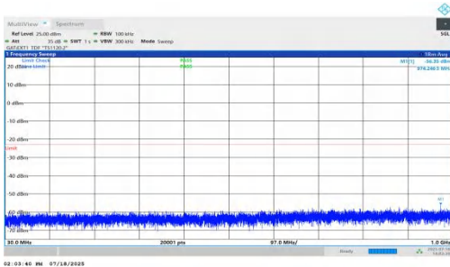
NTNV-n78(3450-3550)-PC1.5-30-50-L-DFT-BPSK-Inner_1RB_Left-30-1000-PASS
