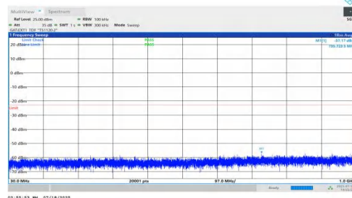
NTNV-n78(3450-3550)-PC1.5-30-60-M-DFT-BPSK-Inner_1RB_Right-3 0-1000-PASS
