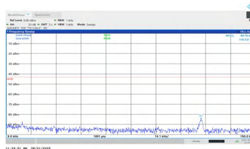
NTNV-n78(3450-3550)-PC1.5-30-60-H-DFT-BPSK-Inner_1RB_Right-0 .009-0.15-PASS
