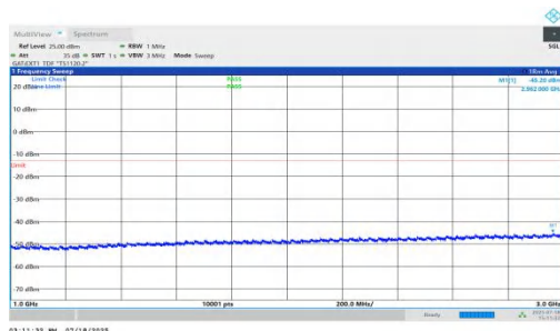
NTNV-n78(3450-3550)-PC1.5-30-60-H-DFT-QPSK-Inner_1RB_Left-1000-3000-PASS
