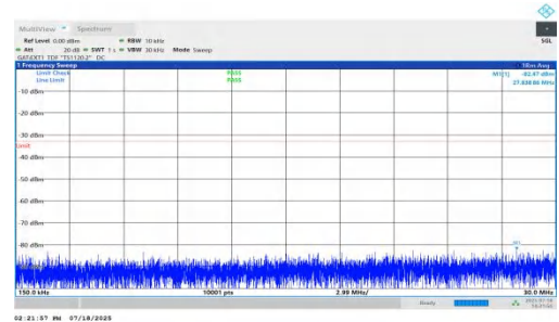
NTNV-n78(3450-3550)-PC1.5-30-50-M-DFT-QPSK-Inner_1RB_Left-0.15-30-PASS
