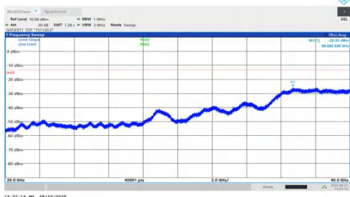
NTNV-n78(3450-3550)-PC1.5-30-50-M-DFT-QPSK-Inner_1RB_Left-2 0000-40000-PASS
