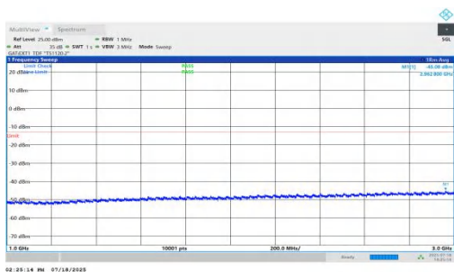
NTNV-n78(3450-3550)-PC1.5-30-50-M-DFT-QPSK-Inner_1RB_Right- 1000-3000-PASS
