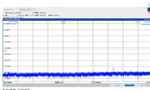
NTNV-n78(3450-3550)-PC1.5-30-50-M-DFT-QPSK-Inner_1RB_Right- 30-1000-PASS
