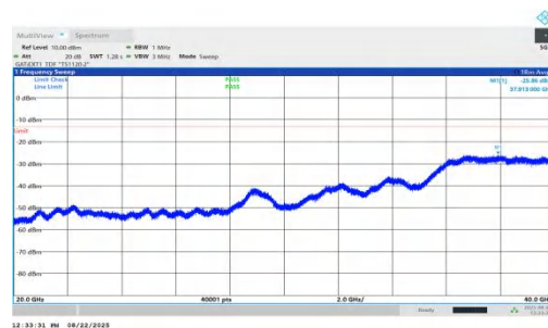
NTNV-n78(3450-3550)-PC1.5-30-60-M-DFT-BPSK-Inner_1RB_Right-2 0000-40000-PASS
