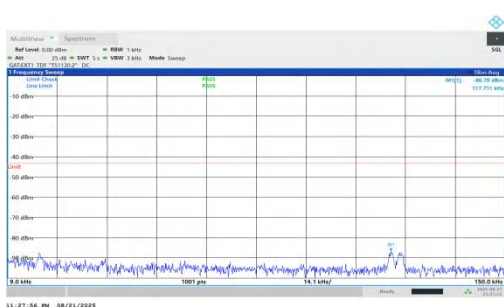
NTNV-n78(3450-3550)-PC1.5-30-60-M-DFT-QPSK-Inner_1RB_Left-0 .009-0.15-PASS
