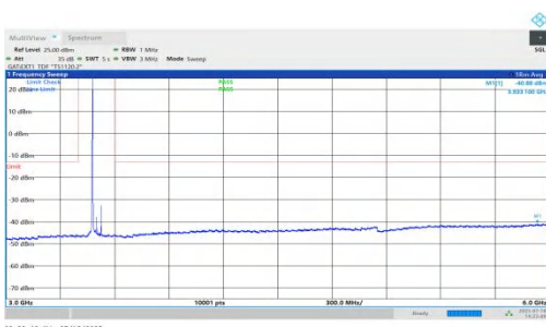
NTNV-n78(3450-3550)-PC1.5-30-50-M-DFT-QPSK-Inner_1RB_Left-3000-6000-PASS
