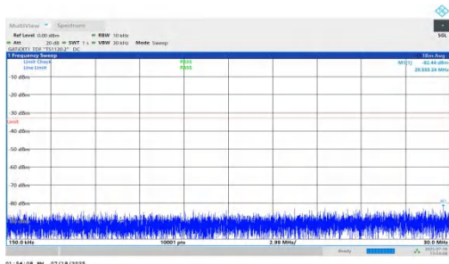
NTNV-n78(3450-3550)-PC1.5-30-40-H-DFT-BPSK-Inner_1RB_Right- 0.15-30-PASS
