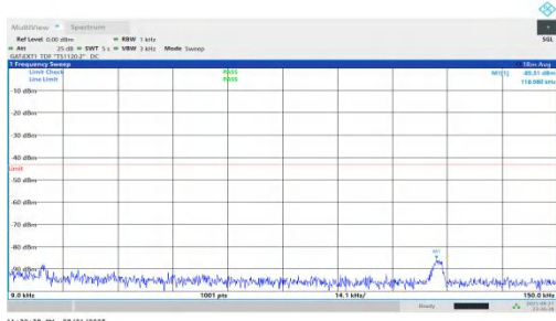
NTNV-n78(3450-3550)-PC1.5-30-60-H-DFT-QPSK-Inner_1RB_Left-0.009-0.15-PASS
