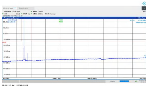
NTNV-n78(3450-3550)-PC1.5-30-70-L-DFT-BPSK-Inner_1RB_Left-3000-6000-PASS
