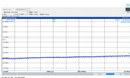
NTNV-n78(3450-3550)-PC1.5-30-60-H-DFT-BPSK-Inner_1RB_Right- 1000-3000-PASS
