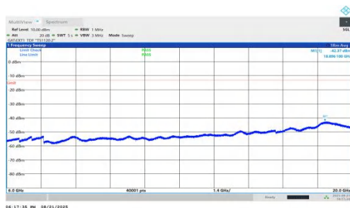
NTNV-n78(3450-3550)-PC1.5-30-25-M-DFT-QPSK-Inner_1RB_Left-60 00-20000-PASS
