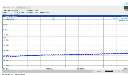
NTNV-n78(3450-3550)-PC1.5-30-25-H-DFT-QPSK-Inner_1RB_Left-1000-3000-PASS
