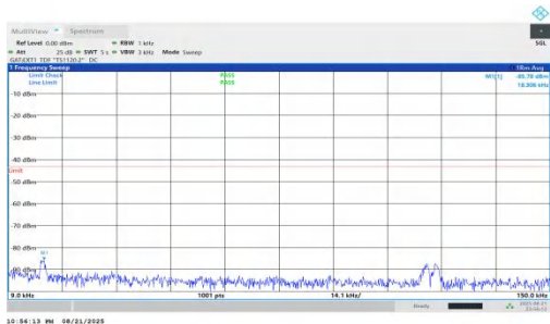
NTNV-n78(3450-3550)-PC1.5-30-25-H-DFT-BPSK-Inner_1RB_Left-0.009-0.15-PASS
