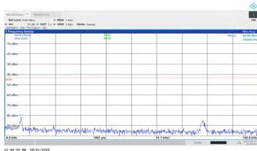
NTNV-n78(3450-3550)-PC1.5-30-20-H-DFT-QPSK-Inner_1RB_Right-0 .009-0.15-PASS
