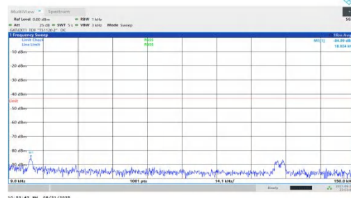
NTVN-n78(3450-3550)-PC1.5-30-25-L-DFT-QPSK-Inner_1RB_Right-0 .009-0.15-PASS
