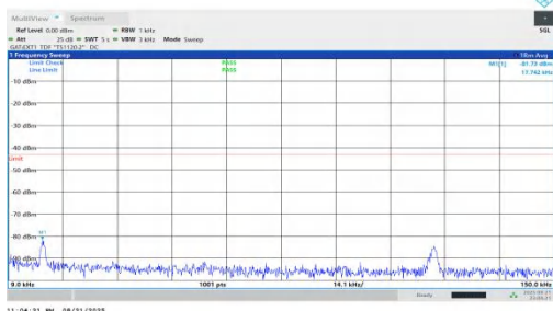
NTNV-n78(3450-3550)-PC1.5-30-30-H-DFT-BPSK-Inner_1RB_Left-0.009-0.15-PASS
