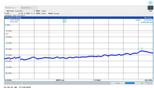
NTNV-n78(3450-3550)-PC1.5-30-40-M-DFT-BPSK-Inner_1RB_Left-6000-20000-PASS
