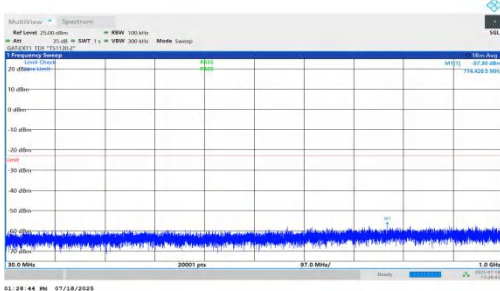
NTVN-n78(3450-3550)-PC1.5-30-40-L-DFT-QPSK-Inner_1RB_Left-30-1000-PASS
