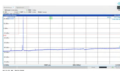
NTNV-n78(3450-3550)-PC1.5-30-25-M-DFT-BPSK-Inner_1RB_Right-3 000-6000-PASS
