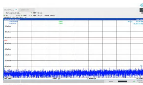
NTNV-n78(3450-3550)-PC1.5-30-25-M-DFT-QPSK-Inner_1RB_Left-0 15-30-PASS
