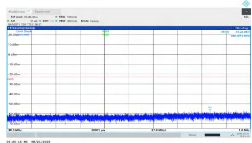
NTNV-n78(3450-3550)-PC1.5-30-25-H-DFT-BPSK-Inner_1RB_Right-3 0-1000-PASS
