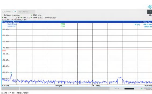
NTNV-n78(3450-3550)-PC1.5-30-30-L-DFT-QPSK-Inner_1RB_Left-0.009-0.15-PASS
