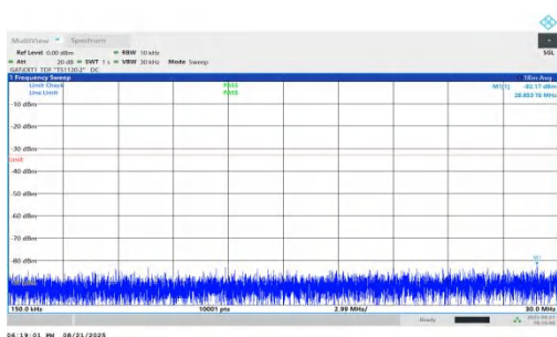
NTNV-n78(3450-3550)-PC1.5-30-25-M-DFT-QPSK-Inner_1RB_Right- 0.15-30-PASS
