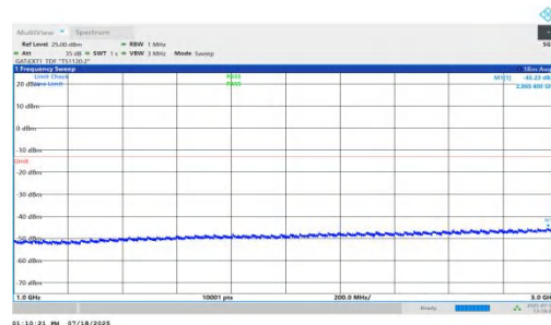
NTNV-n78(3450-3550)-PC1.5-30-30-H-DFT-BPSK-Inner_1RB_Left-1000-3000-PASS
