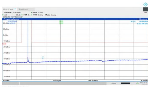
NTNV-n78(3450-3550)-PC1.5-30-25-H-DFT-QPSK-Inner_1RB_Left-3000-6000-PASS
