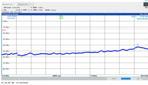
NTVN-n78(3450-3550)-PC1.5-30-40-L-DFT-BPSK-Inner_1RB_Right-6000-20000-PASS
