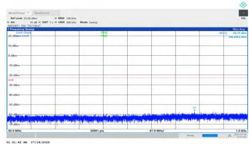
NTNV-n78(3450-3550)-PC1.5-30-40-L-DFT-QPSK-Inner_1RB_Right-3 0-1000-PASS
