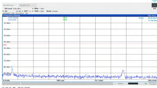
NTNV-n78(3450-3550)-PC1.5-30-25-M-DFT-BPSK-Inner_1RB_Left-0.009-0.15-PASS
