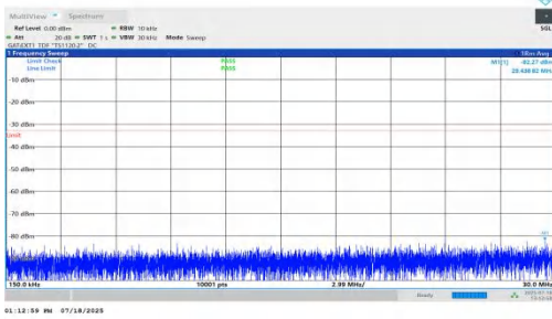
NTNV-n78(3450-3550)-PC1.5-30-30-H-DFT-BPSK-Inner_1RB_Right-0.15-30-PASS
