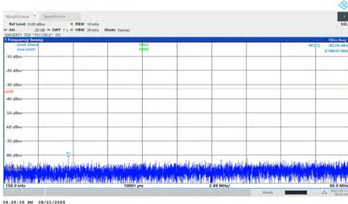
NTNV-n78(3450-3550)-PC1.5-30-25-H-DFT-BPSK-Inner_1RB_Right- 0.15-30-PASS
