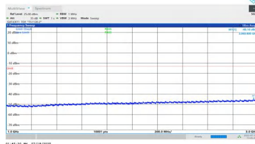
NTNV-n78(3450-3550)-PC1.5-30-40-M-DFT-QPSK-Inner_1RB_Left-10 00-3000-PASS
