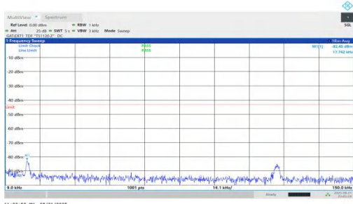
NTNV-n78(3450-3550)-PC1.5-30-30-M-DFT-QPSK-Inner_1RB_Left-0.009-0.15-PASS
