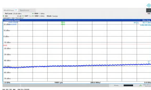
NTNV-n78(3450-3550)-PC1.5-30-25-H-DFT-BPSK-Inner_1RB_Left-1000-3000-PASS
