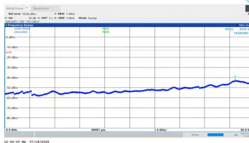
NTNV-n78(3450-3550)-PC1.5-30-30-M-DFT-BPSK-Inner_1RB_Left-60 00-20000-PASS
