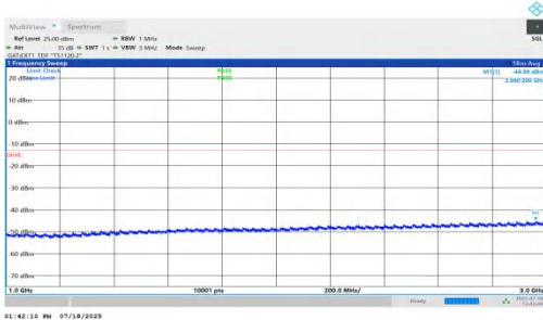
NTNV-n78(3450-3550)-PC1.5-30-40-M-DFT-BPSK-Inner_1RB_Right-1000-3000-PASS
