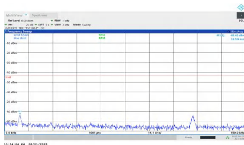
NTNV-n78(3450-3550)-PC1.5-30-25-M-DFT-BPSK-Inner_1RB_Right-0.009-0.15-PASS
