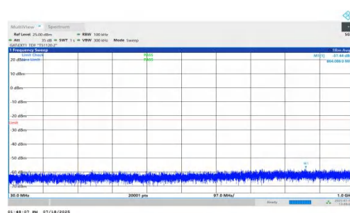
NTNV-n78(3450-3550)-PC1.5-30-40-M-DFT-QPSK-Inner_1RB_Right- 30-1000-PASS
