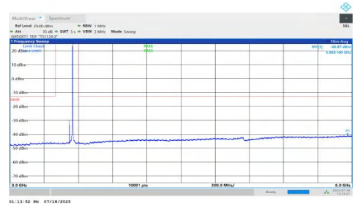
NTNV-n78(3450-3550)-PC1.5-30-30-H-DFT-BPSK-Inner_1RB_Right-3 000-6000-PASS
