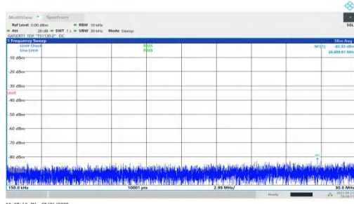
NTNV-n78(3450-3550)-PC1.5-30-25-H-DFT-QPSK-Inner_1RB_Left-0.15-30-PASS
