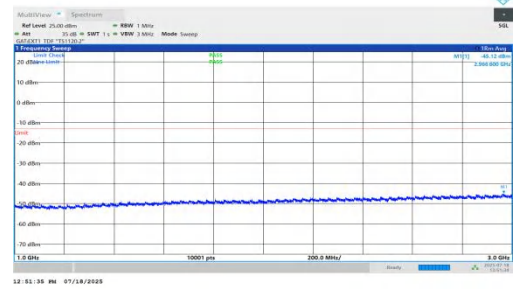
NTNV-n78(3450-3550)-PC1.5-30-30-L-DFT-QPSK-Inner_1RB_Left-10 00-3000-PASS
