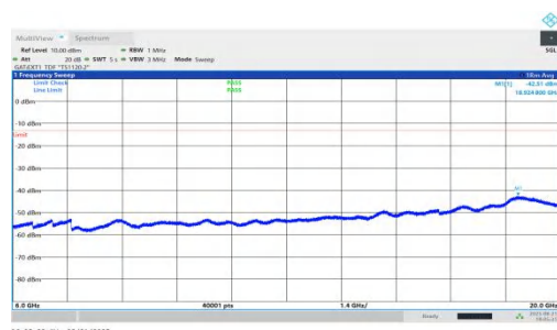
NTNV-n78(3450-3550)-PC1.5-30-25-L-DFT-QPSK-Inner_1RB_Left-60 00-20000-PASS
