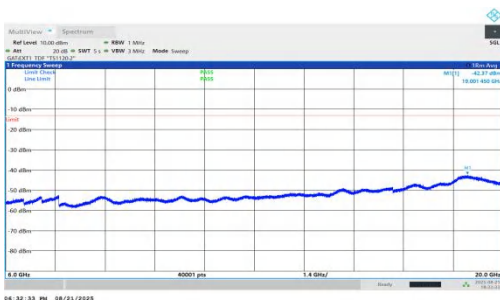
NTNV-n78(3450-3550)-PC1.5-30-25-H-DFT-QPSK-Inner_1RB_Right- 6000-20000-PASS
