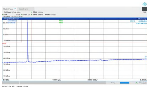
NTNV-n78(3450-3550)-PC1.5-30-30-H-DFT-BPSK-Inner_1RB_Left-3000-6000-PASS
