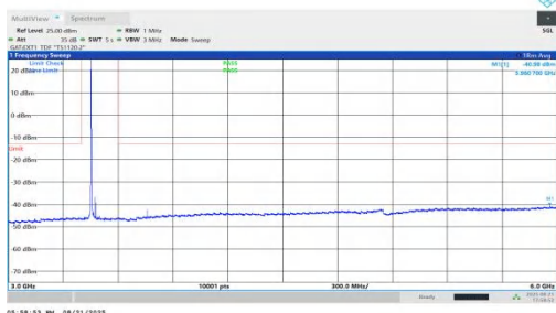
NTNV-n78(3450-3550)-PC1.5-30-25-L-DFT-BPSK-Inner_1RB_Left-30 00-6000-PASS
