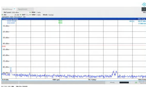
NTNV-n78(3450-3550)-PC1.5-30-40-M-DFT-QPSK-Inner_1RB_Left-0 .009-0.15-PASS
