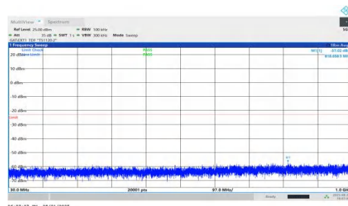
NTVN-n78(3450-3550)-PC1.5-30-25-L-DFT-QPSK-Inner_1RB_Right-3 0-1000-PASS
