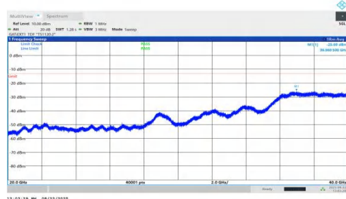
NTNV-n78(3450-3550)-PC1.5-30-25-L-DFT-BPSK-Inner_1RB_Right-2 0000-40000-PASS
