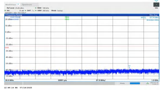
NTNV-n78(3450-3550)-PC1.5-30-30-L-DFT-BPSK-Inner_1RB_Right-3 0-1000-PASS
