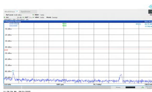
NTNV-n78(3450-3550)-PC1.5-30-30-H-DFT-BPSK-Inner_1RB_Right-0.009-0.15-PASS
