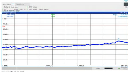
NTNV-n78(3450-3550)-PC1.5-30-25-H-DFT-BPSK-Inner_1RB_Right-6000-20000-PASS
