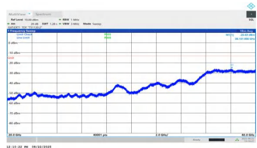
NTNV-n78(3450-3550)-PC1.5-30-30-L-DFT-BPSK-Inner_1RB_Right-2 0000-40000-PASS
