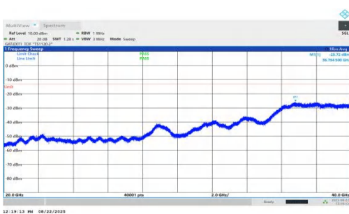
NTNV-n78(3450-3550)-PC1.5-30-40-M-DFT-BPSK-Inner_1RB_Left-20000-40000-PASS
