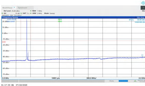
NTNV-n78(3450-3550)-PC1.5-30-30-H-DFT-QPSK-Inner_1RB_Left-3 000-6000-PASS
