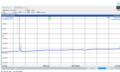
NTVN-n78(3450-3550)-PC1.5-30-40-L-DFT-QPSK-Inner_1RB_Left-3000-6000-PASS
