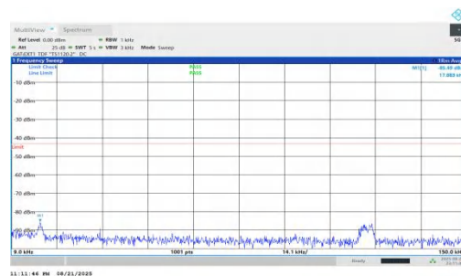
NTNV-n78(3450-3550)-PC1.5-30-40-M-DFT-QPSK-Inner_1RB_Right- 0.009-0.15-PASS
