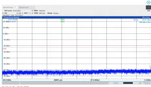
NTNV-n78(3450-3550)-PC1.5-30-25-M-DFT-BPSK-Inner_1RB_Left-30-1000-PASS
