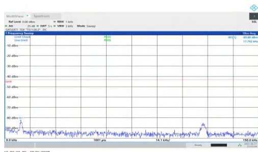
NTNV-n78(3450-3550)-PC1.5-30-25-L-DFT-QPSK-Inner_1RB_Left-0. 009-0.15-PASS
