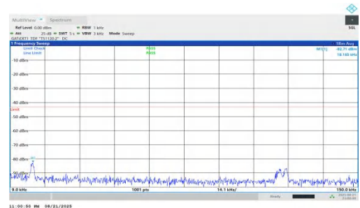
NTNV-n78(3450-3550)-PC1.5-30-30-L-DFT-QPSK-Inner_1RB_Right-0 .009-0.15-PASS
