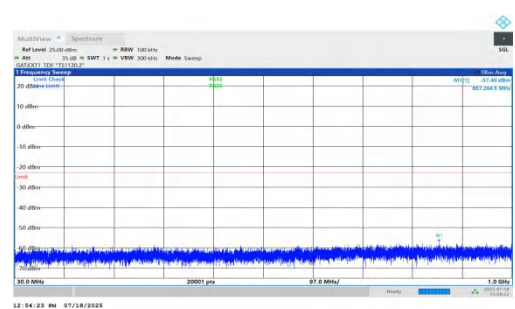
NTNV-n78(3450-3550)-PC1.5-30-30-L-DFT-QPSK-Inner_1RB_Right-3 0-1000-PASS
