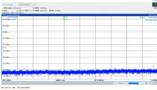
NTNV-n78(3450-3550)-PC1.5-30-30-H-DFT-QPSK-Inner_1RB_Left-3 0-1000-PASS
