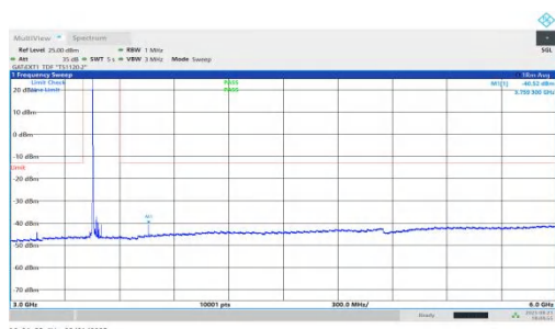
NTNV-n78(3450-3550)-PC1.5-30-25-L-DFT-QPSK-Inner_1RB_Left-3 000-6000-PASS
