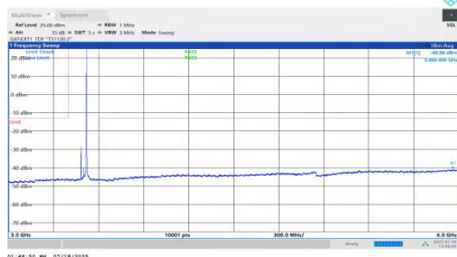
NTNV-n78(3450-3550)-PC1.5-30-40-M-DFT-QPSK-Inner_1RB_Right-3000-6000-PASS
