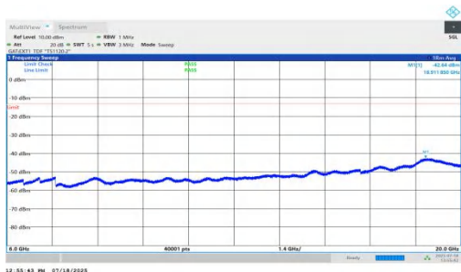
NTNV-n78(3450-3550)-PC1.5-30-30-L-DFT-QPSK-Inner_1RB_Right-6000-20000-PASS
