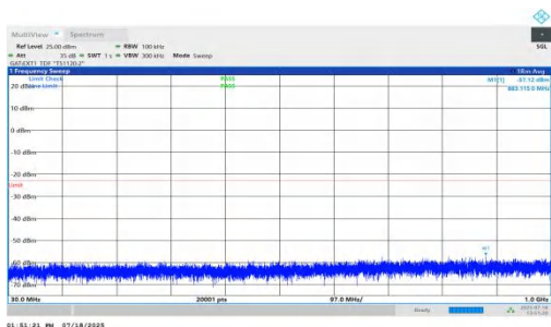
NTNV-n78(3450-3550)-PC1.5-30-40-H-DFT-BPSK-Inner_1RB_Left-300-1000-PASS
