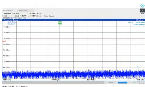
NTNV-n78(3450-3550)-PC1.5-30-20-H-DFT-QPSK-Inner_1RB_Right- 0.15-30-PASS
