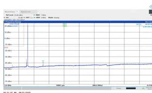
NTNV-n78(3450-3550)-PC1.5-30-25-L-DFT-BPSK-Inner_1RB_Right-3 000-6000-PASS
