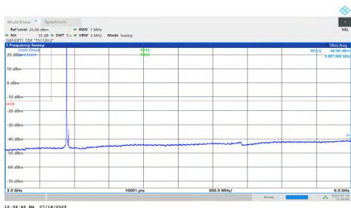
NTNV-n78(3450-3550)-PC1.5-30-20-H-DFT-QPSK-Inner_1RB_Left-3 000-6000-PASS
