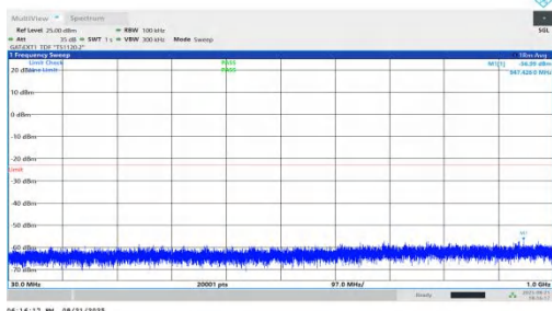
NTNV-n78(3450-3550)-PC1.5-30-25-M-DFT-QPSK-Inner_1RB_Left-3 0-1000-PASS
