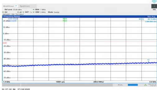
NTNV-n78(3450-3550)-PC1.5-30-30-M-DFT-QPSK-Inner_1RB_Right- 1000-3000-PASS
