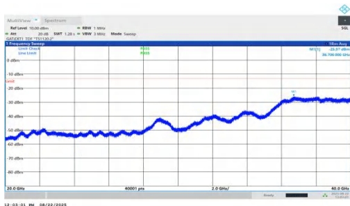
NTNV-n78(3450-3550)-PC1.5-30-25-L-DFT-BPSK-Inner_1RB_Left-20 000-40000-PASS
