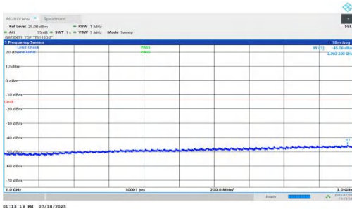
NTNV-n78(3450-3550)-PC1.5-30-30-H-DFT-BPSK-Inner_1RB_Right-1000-3000-PASS
