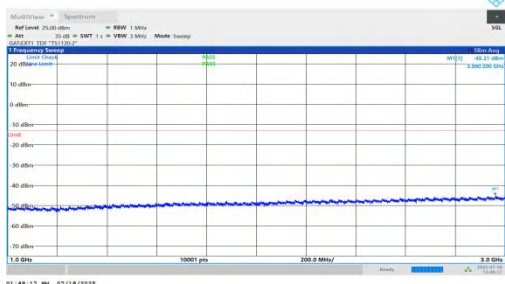
NTNV-n78(3450-3550)-PC1.5-30-40-M-DFT-QPSK-Inner_1RB_Right-1000-3000-PASS
