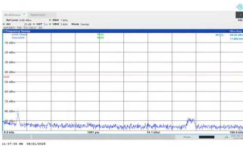
NTNV-n78(3450-3550)-PC1.5-30-40-L-DFT-BPSK-Inner_1RB_Left-0.009-0.15-PASS
