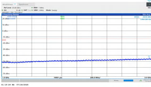
NTNV-n78(3450-3550)-PC1.5-30-30-H-DFT-QPSK-Inner_1RB_Right-1000-3000-PASS
