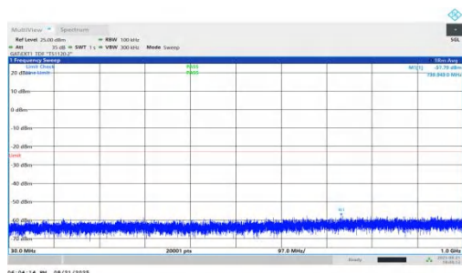
NTNV-n78(3450-3550)-PC1.5-30-25-L-DFT-QPSK-Inner_1RB_Left-3 0-1000-PASS
