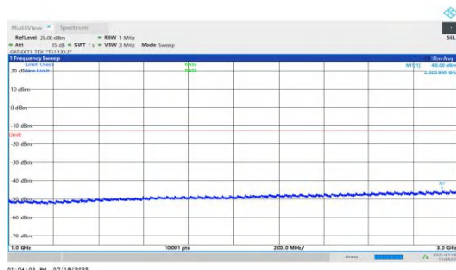
NTNV-n78(3450-3550)-PC1.5-30-30-M-DFT-QPSK-Inner_1RB_Left-1000-3000-PASS
