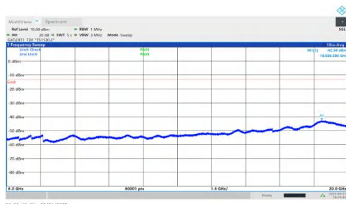
NTNV-n78(3450-3550)-PC1.5-30-25-H-DFT-QPSK-Inner_1RB_Left-6000-20000-PASS
