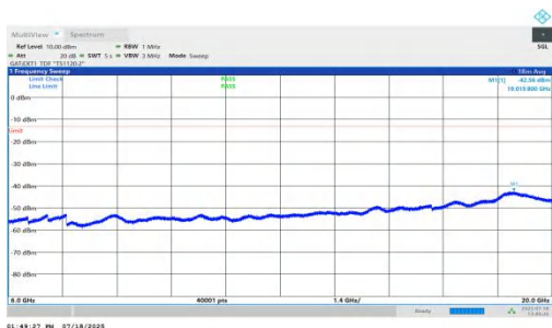
NTNV-n78(3450-3550)-PC1.5-30-40-M-DFT-QPSK-Inner_1RB_Right-6000-20000-PASS
