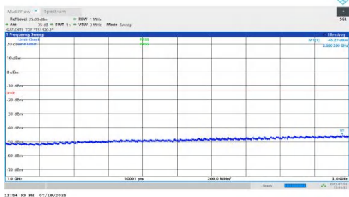
NTNV-n78(3450-3550)-PC1.5-30-30-L-DFT-QPSK-Inner_1RB_Right-1000-3000-PASS
