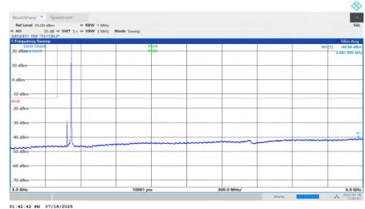
NTNV-n78(3450-3550)-PC1.5-30-40-M-DFT-BPSK-Inner_1RB_Right-3 000-6000-PASS
