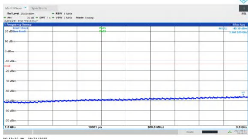
NTNV-n78(3450-3550)-PC1.5-30-25-M-DFT-QPSK-Inner_1RB_Right-1000-3000-PASS
