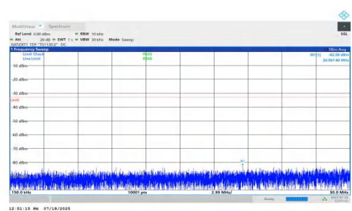
NTNV-n78(3450-3550)-PC1.5-30-30-L-DFT-QPSK-Inner_1RB_Left-0.1 5-30-PASS
