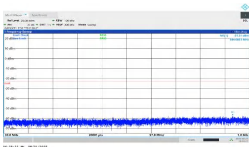
NTNV-n78(3450-3550)-PC1.5-30-25-H-DFT-QPSK-Inner_1RB_Left-30-1000-PASS
