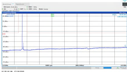
NTNV-n78(3450-3550)-PC1.5-30-30-M-DFT-BPSK-Inner_1RB_Left-3 000-6000-PASS
