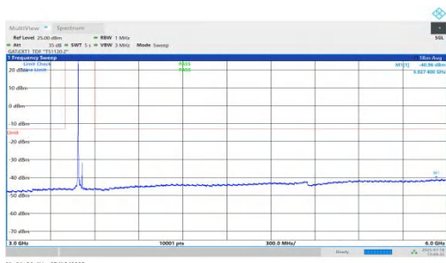
NTNV-n78(3450-3550)-PC1.5-30-30-M-DFT-QPSK-Inner_1RB_Left-3000-6000-PASS
