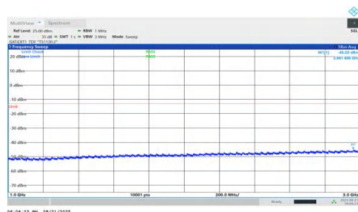
NTNV-n78(3450-3550)-PC1.5-30-25-L-DFT-QPSK-Inner_1RB_Left-10 00-3000-PASS
