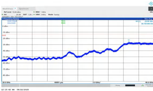
NTNV-n78(3450-3550)-PC1.5-30-30-H-DFT-QPSK-Inner_1RB_Left-2 0000-40000-PASS
