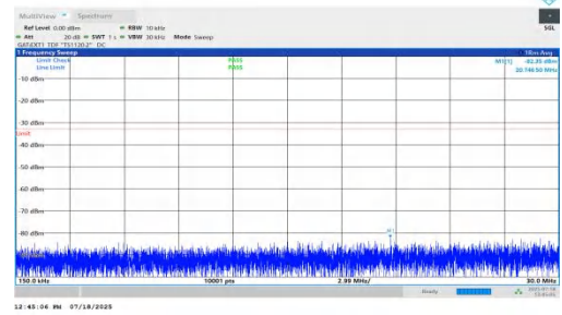
NTNV-n78(3450-3550)-PC1.5-30-30-L-DFT-BPSK-Inner_1RB_Left-0.15-30-PASS
