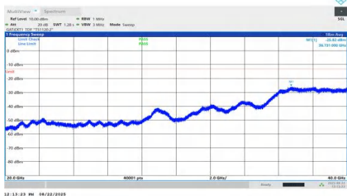
NTNV-n78(3450-3550)-PC1.5-30-30-M-DFT-QPSK-Inner_1RB_Left-2 0000-40000-PASS
