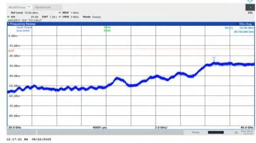
NTVN-n78(3450-3550)-PC1.5-30-40-L-DFT-BPSK-Inner_1RB_Right-20000-40000-PASS
