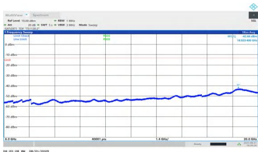
NTNV-n78(3450-3550)-PC1.5-30-25-M-DFT-QPSK-Inner_1RB_Right-6000-20000-PASS
