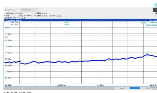
NTNV-n78(3450-3550)-PC1.5-30-40-M-DFT-QPSK-Inner_1RB_Left-60 00-20000-PASS
