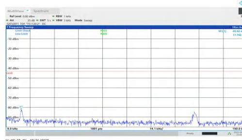
NTVN-n78(3450-3550)-PC1.5-30-40-L-DFT-BPSK-Inner_1RB_Right-0. 009-0.15-PASS
