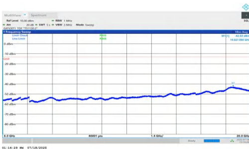
NTNV-n78(3450-3550)-PC1.5-30-30-H-DFT-BPSK-Inner_1RB_Right-6000-20000-PASS
