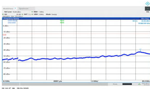
NTNV-n78(3450-3550)-PC1.5-30-25-M-DFT-BPSK-Inner_1RB_Right-6000-20000-PASS
