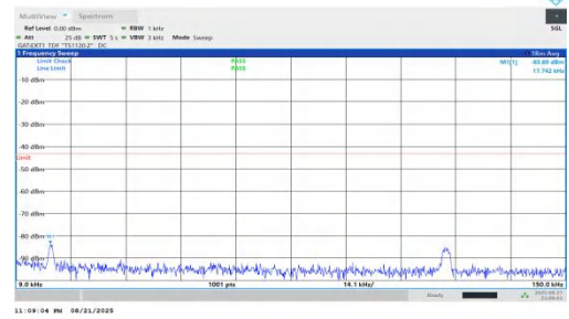
NTNV-n78(3450-3550)-PC1.5-30-40-L-DFT-QPSK-Inner_1RB_Right-0 .009-0.15-PASS
