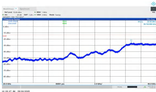
NTNV-n78(3450-3550)-PC1.5-30-25-M-DFT-QPSK-Inner_1RB_Left-2 0000-40000-PASS
