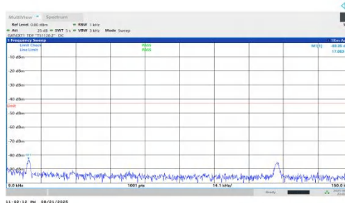
NTNV-n78(3450-3550)-PC1.5-30-30-M-DFT-BPSK-Inner_1RB_Right-0 .009-0.15-PASS
