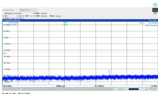
NTNV-n78(3450-3550)-PC1.5-30-25-L-DFT-BPSK-Inner_1RB_Left-30-1000-PASS
