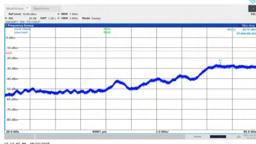
NTNV-n78(3450-3550)-PC1.5-30-30-M-DFT-BPSK-Inner_1RB_Right-20000-40000-PASS
