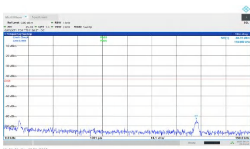
NTNV-n78(3450-3550)-PC1.5-30-25-M-DFT-QPSK-Inner_1RB_Left-0 .009-0.15-PASS
