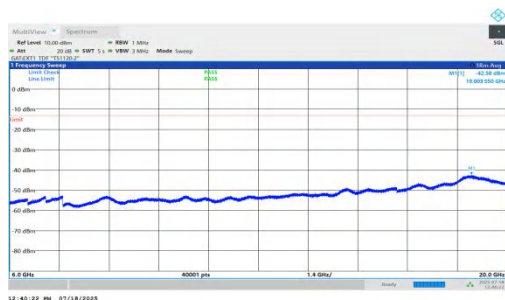
NTNV-n78(3450-3550)-PC1.5-30-20-H-DFT-QPSK-Inner_1RB_Left-60 00-20000-PASS
