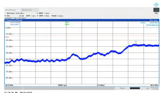
NTNV-n78(3450-3550)-PC1.5-30-40-L-DFT-QPSK-Inner_1RB_Right-2 0000-40000-PASS
