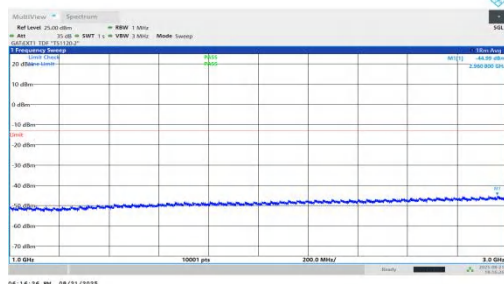
NTNV-n78(3450-3550)-PC1.5-30-25-M-DFT-QPSK-Inner_1RB_Left-10 00-3000-PASS
