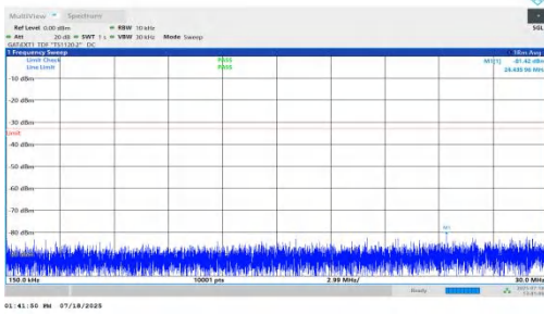
NTNV-n78(3450-3550)-PC1.5-30-40-M-DFT-BPSK-Inner_1RB_Right-0.15-30-PASS
