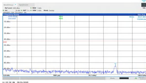
NTNV-n78(3450-3550)-PC1.5-30-30-M-DFT-QPSK-Inner_1RB_Right- 0.009-0.15-PASS
