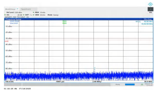
NTNV-n78(3450-3550)-PC1.5-30-40-L-DFT-BPSK-Inner_1RB_Left-0.15-30-PASS
