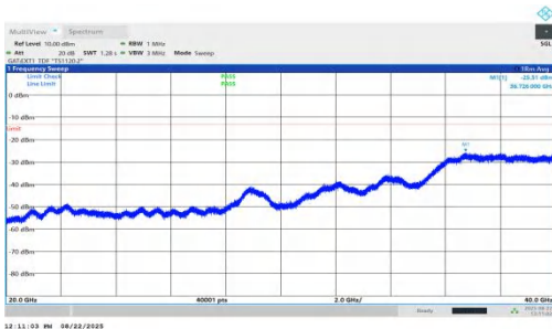
NTNV-n78(3450-3550)-PC1.5-30-30-L-DFT-QPSK-Inner_1RB_Left-2 0000-40000-PASS
