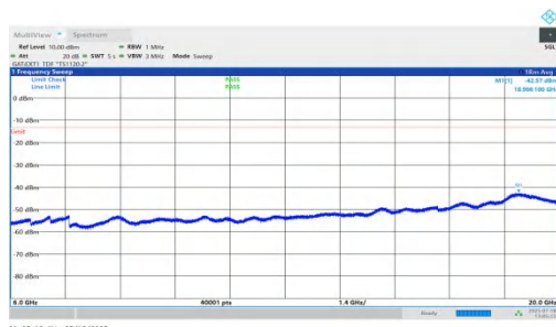
NTNV-n78(3450-3550)-PC1.5-30-30-M-DFT-QPSK-Inner_1RB_Left-6000-20000-PASS
