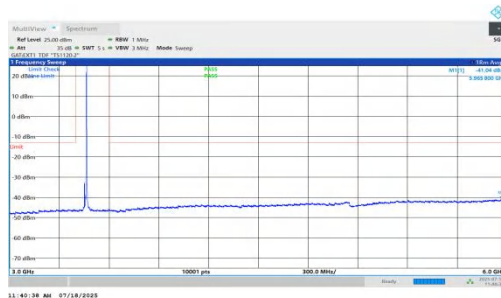
NTNV-n78(3450-3550)-PC1.5-30-15-L-DFT-QPSK-Inner_1RB_Right-3 000-6000-PASS
