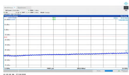
NTNV-n78(3450-3550)-PC1.5-30-20-M-DFT-QPSK-Inner_1RB_Left-1000-3000-PASS
