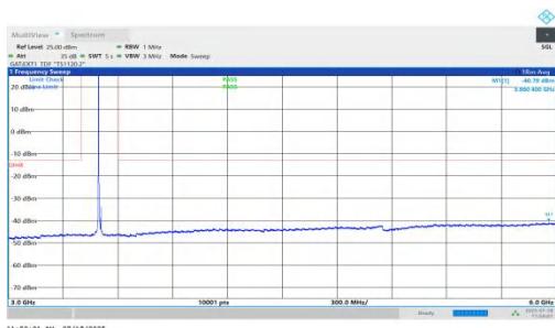
NTNV-n78(3450-3550)-PC1.5-30-15-M-DFT-QPSK-Inner_1RB_Left-3 000-6000-PASS
