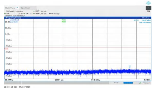
NTV-n78(3450-3550)-PC1.5-30-10-M-DFT-QPSK-Inner_1RB_Right- 30-1000-PASS
