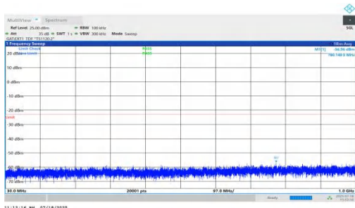
NTNV-n78(3450-3550)-PC1.5-30-10-M-DFT-QPSK-Inner_1RB_Left-30-1000-PASS
