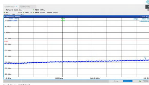
NTNV-n78(3450-3550)-PC1.5-30-10-H-DFT-BPSK-Inner_1RB_Left-1000-3000-PASS
