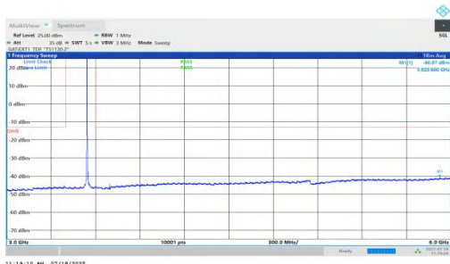
NTNV-n78(3450-3550)-PC1.5-30-10-H-DFT-BPSK-Inner_1RB_Left-3000-6000-PASS
