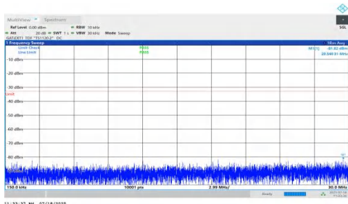
NTNV-n78(3450-3550)-PC1.5-30-15-L-DFT-BPSK-Inner_1RB_Right- 0.15-30-PASS
