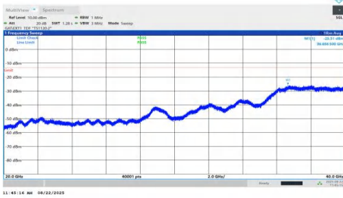
NTV-n78(3450-3550)-PC1.5-30-10-M-DFT-QPSK-Inner_1RB_Left-2 0000-40000-PASS
