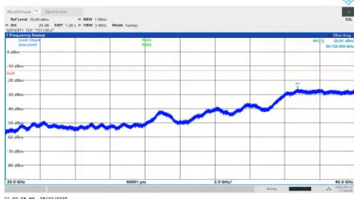
NTNV-n78(3450-3550)-PC1.5-30-15-L-DFT-QPSK-Inner_1RB_Left-2 0000-40000-PASS
