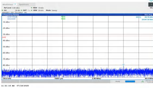
NTNV-n78(3450-3550)-PC1.5-30-10-H-DFT-BPSK-Inner_1RB_Right-0.15-30-PASS
