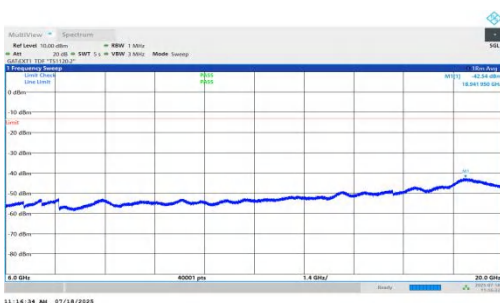
NTV-n78(3450-3550)-PC1.5-30-10-M-DFT-QPSK-Inner_1RB_Right- 6000-20000-PASS
