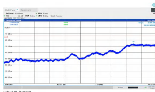
NTNV-n78(3450-3550)-PC1.5-30-10-L-DFT-BPSK-Inner_1RB_Right-2 0000-40000-PASS
