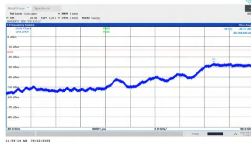
NTNV-n78(3450-3550)-PC1.5-30-15-H-DFT-BPSK-Inner_1RB_Right-20000-40000-PASS
