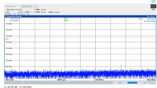
NTNV-n78(3450-3550)-PC1.5-30-15-L-DFT-QPSK-Inner_1RB_Left-0.15-5-30-PASS
