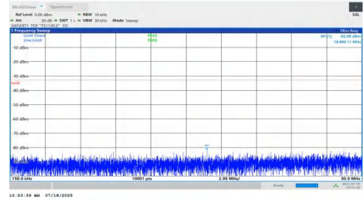
NTNV-n78(3450-3550)-PC1.5-30-10-L-DFT-BPSK-Inner_1RB_Left-0.15-30-PASS
