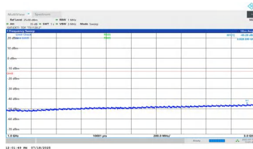
NTNV-n78(3450-3550)-PC1.5-30-15-H-DFT-QPSK-Inner_1RB_Left-1000-3000-PASS
