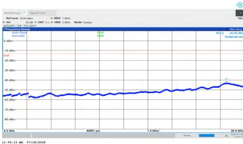
NTNV-n78(3450-3550)-PC1.5-30-10-L-DFT-QPSK-Inner_1RB_Right-6000-20000-PASS
