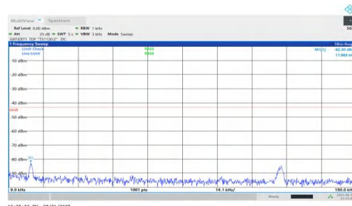
NTNV-n78(3450-3550)-PC1.5-30-15-L-DFT-BPSK-Inner_1RB_Right-0 009-0.15-PASS
