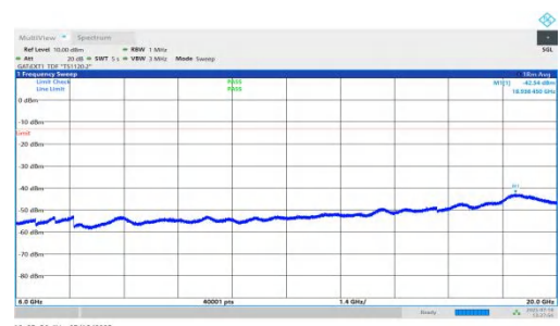
NTNV-n78(3450-3550)-PC1.5-30-20-M-DFT-QPSK-Inner_1RB_Left-6000-20000-PASS
