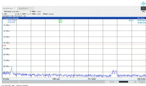
NTNV-n78(3450-3550)-PC1.5-30-15-H-DFT-BPSK-Inner_1RB_Left-0.009-0.15-PASS
