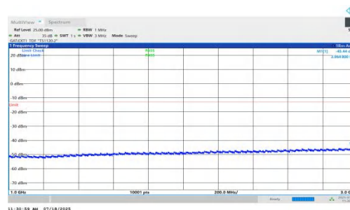
NTNV-n78(3450-3550)-PC1.5-30-15-L-DFT-BPSK-Inner_1RB_Left-1000-3000-PASS
