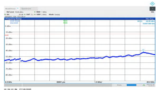
NTNV-n78(3450-3550)-PC1.5-30-20-H-DFT-BPSK-Inner_1RB_Left-6000-20000-PASS
