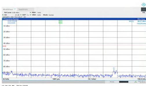
NTNV-n78(3450-3550)-PC1.5-30-15-L-DFT-BPSK-Inner_1RB_Left-0.009-0.15-PASS
