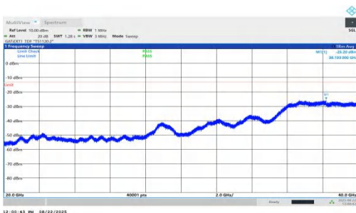
NTNV-n78(3450-3550)-PC1.5-30-20-H-DFT-BPSK-Inner_1RB_Left-20000-40000-PASS
