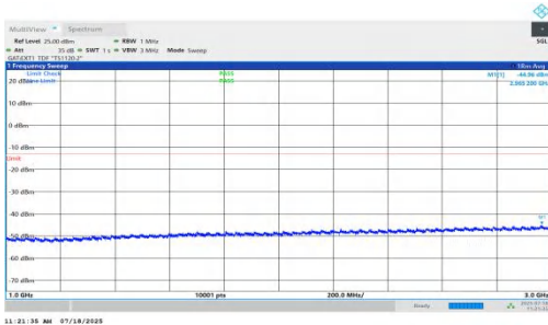
NTNV-n78(3450-3550)-PC1.5-30-10-H-DFT-BPSK-Inner_1RB_Right-1000-3000-PASS
