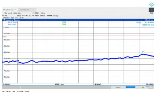
NTNV-n78(3450-3550)-PC1.5-30-10-H-DFT-QPSK-Inner_1RB_Right-6000-20000-PASS
