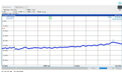
NTNV-n78(3450-3550)-PC1.5-30-20-L-DFT-QPSK-Inner_1RB_Right-6000-20000-PASS
