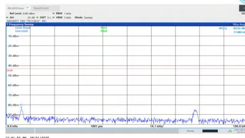
NTNV-n78(3450-3550)-PC1.5-30-15-H-DFT-QPSK-Inner_1RB_Right-0 .009-0.15-PASS
