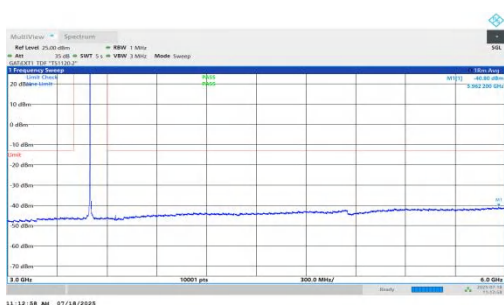
NTNV-n78(3450-3550)-PC1.5-30-10-M-DFT-QPSK-Inner_1RB_Left-3000-6000-PASS
