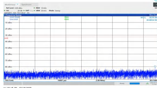
NTNV-n78(3450-3550)-PC1.5-30-10-H-DFT-BPSK-Inner_1RB_Left-0.15-30-PASS
