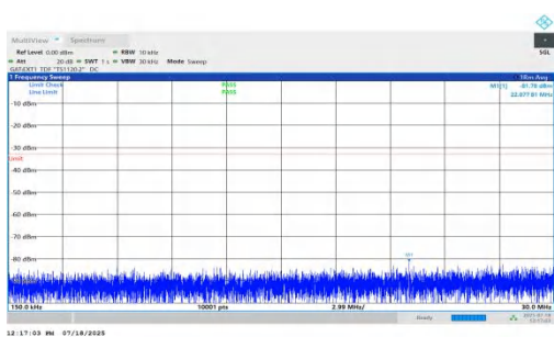
NTV-n78(3450-3550)-PC1.5-30-20-L-DFT-QPSK-Inner_1RB_Right- 0.15-30-PASS
