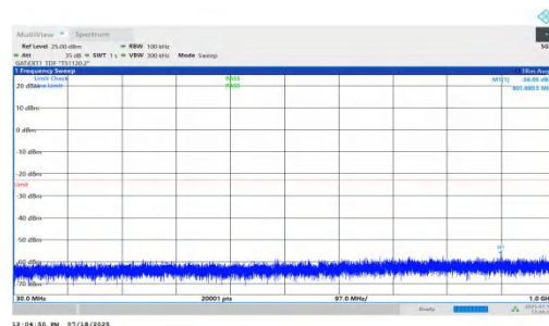
NTNV-n78(3450-3550)-PC1.5-30-15-H-DFT-QPSK-Inner_1RB_Right-3 0-1000-PASS
