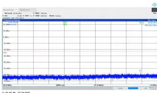
NTNV-n78(3450-3550)-PC1.5-30-15-L-DFT-BPSK-Inner_1RB_Left-30-1000-PASS
