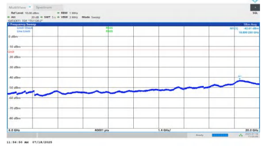
NTNV-n78(3450-3550)-PC1.5-30-15-H-DFT-BPSK-Inner_1RB_Left-60 00-20000-PASS
