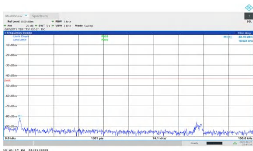
NTNV-n78(3450-3550)-PC1.5-30-15-H-DFT-QPSK-Inner_1RB_Left-0.009-0.15-PASS
