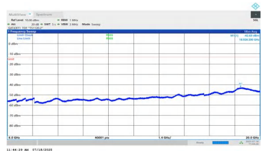
NTNV-n78(3450-3550)-PC1.5-30-15-M-DFT-BPSK-Inner_1RB_Left-6000-20000-PASS
