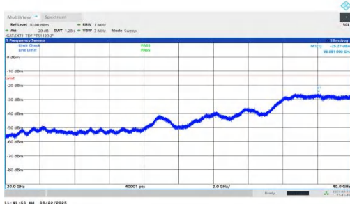
NTNV-n78(3450-3550)-PC1.5-30-10-L-DFT-BPSK-Inner_1RB_Left-20000-40000-PASS
