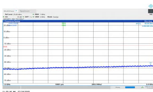
NTNV-n78(3450-3550)-PC1.5-30-15-H-DFT-BPSK-Inner_1RB_Left-1000-3000-PASS
