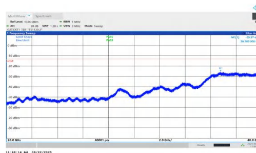
NTNV-n78(3450-3550)-PC1.5-30-10-H-DFT-QPSK-Inner_1RB_Right-20000-40000-PASS
