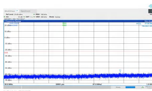
NTNV-n78(3450-3550)-PC1.5-30-15-M-DFT-QPSK-Inner_1RB_Right- 30-1000-PASS
