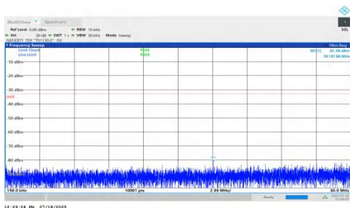
NTNV-n78(3450-3550)-PC1.5-30-20-M-DFT-QPSK-Inner_1RB_Right- 0.15-30-PASS
