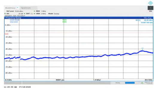
NTNV-n78(3450-3550)-PC1.5-30-10-H-DFT-QPSK-Inner_1RB_Left-60 00-20000-PASS
