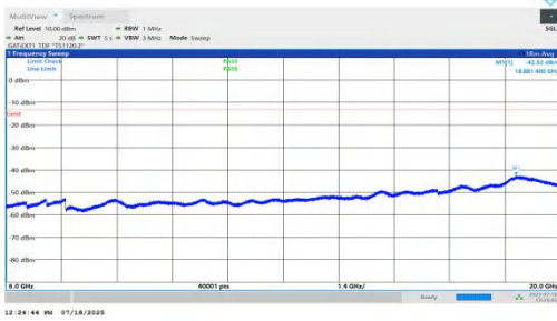
NTNV-n78(3450-3550)-PC1.5-30-20-M-DFT-BPSK-Inner_1RB_Right-6000-20000-PASS
