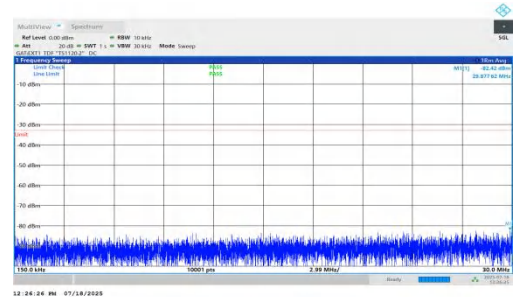
NTNV-n78(3450-3550)-PC1.5-30-20-M-DFT-QPSK-Inner_1RB_Left-0.15-30-PASS
