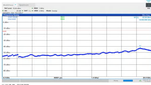
NTNV-n78(3450-3550)-PC1.5-30-10-M-DFT-BPSK-Inner_1RB_Right-6000-20000-PASS
