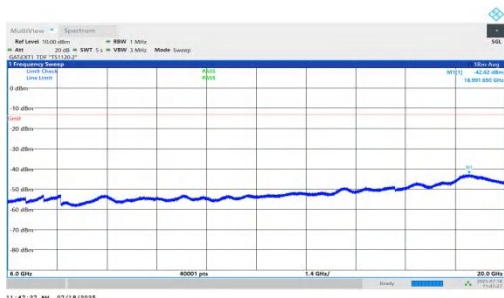
NTNV-n78(3450-3550)-PC1.5-30-15-M-DFT-BPSK-Inner_1RB_Right-6000-20000-PASS
