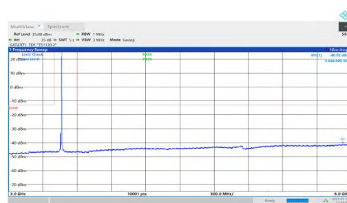
NTNV-n78(3450-3550)-PC1.5-30-15-L-DFT-BPSK-Inner_1RB_Right-3 000-6000-PASS
