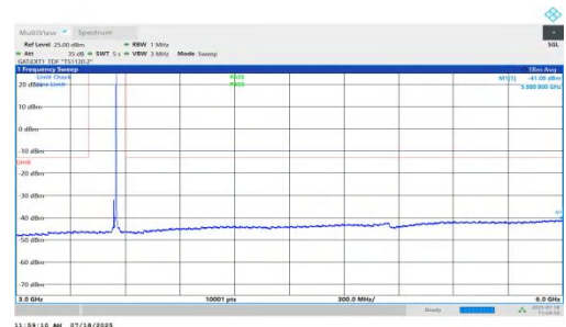
NTNV-n78(3450-3550)-PC1.5-30-15-H-DFT-BPSK-Inner_1RB_Right-3 000-6000-PASS
