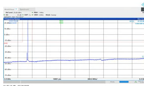
NTNV-n78(3450-3550)-PC1.5-30-20-M-DFT-QPSK-Inner_1RB_Right- 3000-6000-PASS
