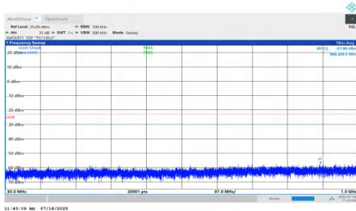
NTNV-n78(3450-3550)-PC1.5-30-15-M-DFT-BPSK-Inner_1RB_Left-30-1000-PASS
