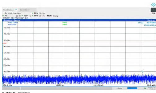
NTNV-n78(3450-3550)-PC1.5-30-15-L-DFT-QPSK-Inner_1RB_Right- 0.15-30-PASS
