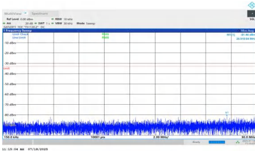
NTV-n78(3450-3550)-PC1.5-30-10-M-DFT-QPSK-Inner_1RB_Right- 0.15-30-PASS
