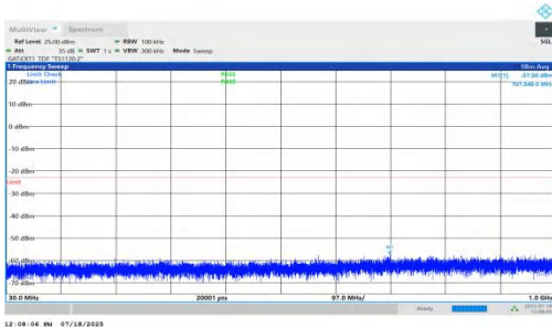
NTNV-n78(3450-3550)-PC1.5-30-20-L-DFT-BPSK-Inner_1RB_Left-30-1000-PASS
