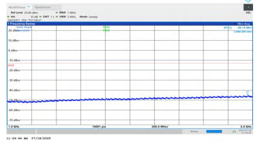
NTNV-n78(3450-3550)-PC1.5-30-10-H-DFT-QPSK-Inner_1RB_Left-10 00-3000-PASS
