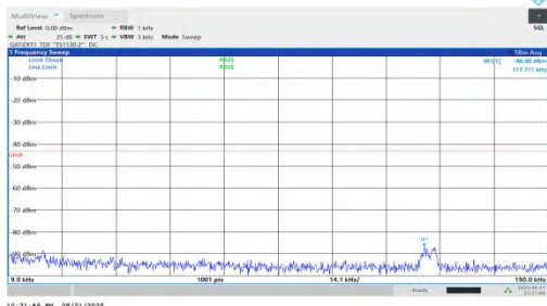
NTNV-n78(3450-3550)-PC1.5-30-10-H-DFT-BPSK-Inner_1RB_Left-0.009-0.15-PASS
