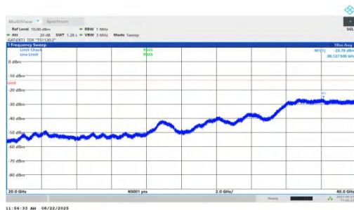
NTNV-n78(3450-3550)-PC1.5-30-20-L-DFT-BPSK-Inner_1RB_Right-2 0000-40000-PASS
