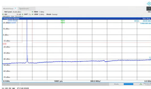
NTNV-n78(3450-3550)-PC1.5-30-15-M-DFT-BPSK-Inner_1RB_Left-3000-6000-PASS
