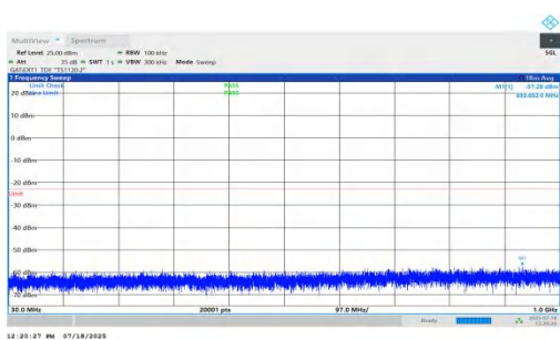
NTNV-n78(3450-3550)-PC1.5-30-20-M-DFT-BPSK-Inner_1RB_Left-30-1000-PASS
