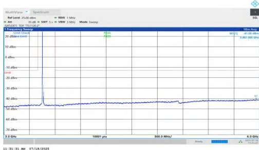
NTNV-n78(3450-3550)-PC1.5-30-15-L-DFT-BPSK-Inner_1RB_Left-30 00-6000-PASS
