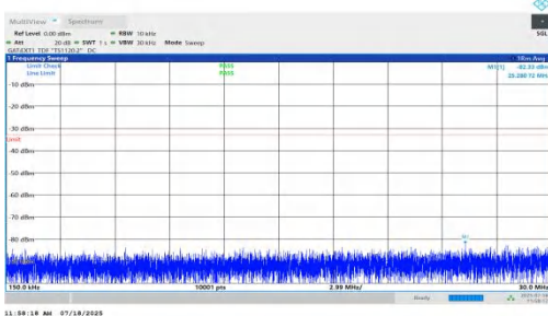
NTNV-n78(3450-3550)-PC1.5-30-15-H-DFT-BPSK-Inner_1RB_Right- 0.15-30-PASS
