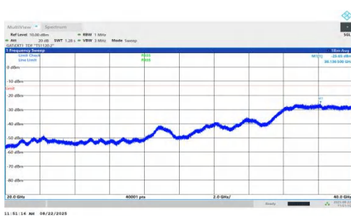
NTNV-n78(3450-3550)-PC1.5-30-15-M-DFT-BPSK-Inner_1RB_Left-20000-40000-PASS
