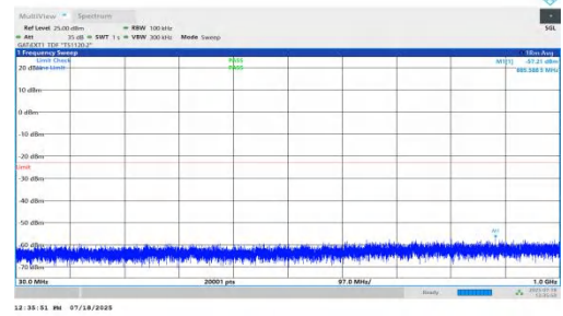
NTNV-n78(3450-3550)-PC1.5-30-20-H-DFT-BPSK-Inner_1RB_Right-3 0-1000-PASS
