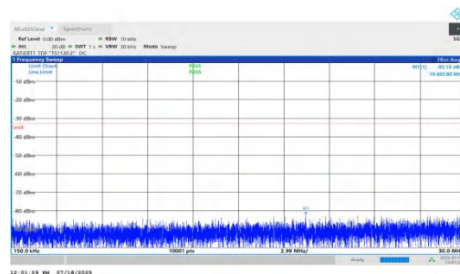
NTNV-n78(3450-3550)-PC1.5-30-15-H-DFT-QPSK-Inner_1RB_Left-0.15-30-PASS
