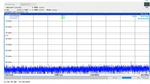
NTNV-n78(3450-3550)-PC1.5-30-15-M-DFT-BPSK-Inner_1RB_Left-0.15-30-PASS
