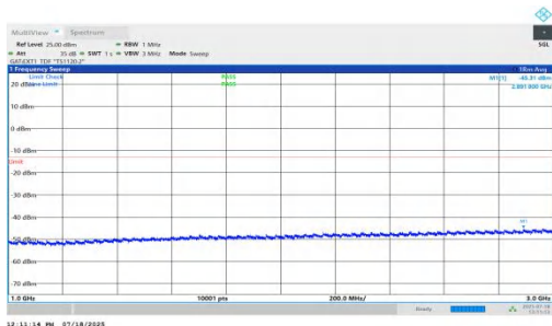
NTNV-n78(3450-3550)-PC1.5-30-20-L-DFT-BPSK-Inner_1RB_Right-1000-3000-PASS
