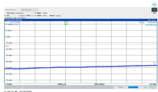
NTNV-n78(3450-3550)-PC1.5-30-10-M-DFT-BPSK-Inner_1RB_Left-1000-3000-PASS
