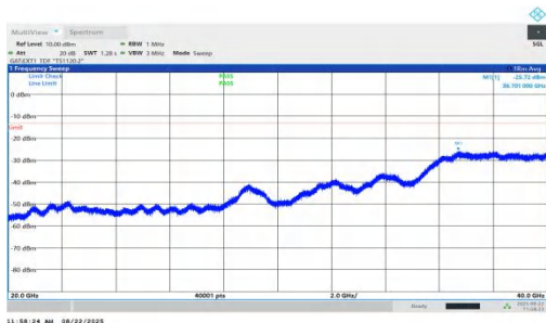
NTNV-n78(3450-3550)-PC1.5-30-20-M-DFT-BPSK-Inner_1RB_Left-2 0000-40000-PASS
