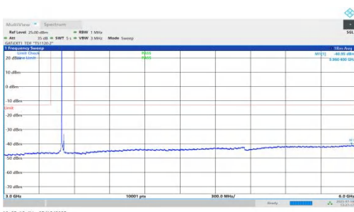
NTNV-n78(3450-3550)-PC1.5-30-20-M-DFT-QPSK-Inner_1RB_Left-3000-6000-PASS
