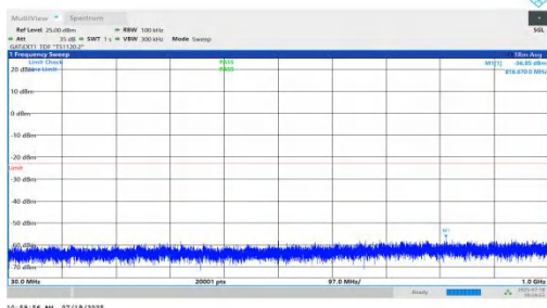
NTVN-n78(3450-3550)-PC1.5-30-10-L-DFT-QPSK-Inner_1RB_Left-3 0-1000-PASS
