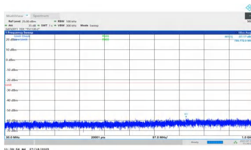
NTNV-n78(3450-3550)-PC1.5-30-15-L-DFT-QPSK-Inner_1RB_Right-3 0-1000-PASS
