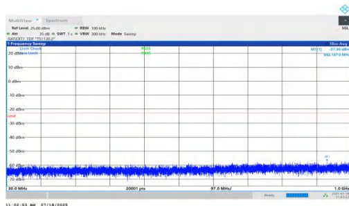
NTVN-n78(3450-3550)-PC1.5-30-10-L-DFT-QPSK-Inner_1RB_Right-3 0-1000-PASS
