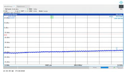
NTNV-n78(3450-3550)-PC1.5-30-10-L-DFT-BPSK-Inner_1RB_Left-1000-3000-PASS
