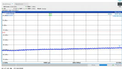
NTNV-n78(3450-3550)-PC1.5-30-20-L-DFT-QPSK-Inner_1RB_Right-1000-3000-PASS
