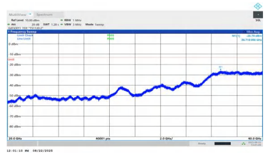
NTNV-n78(3450-3550)-PC1.5-30-20-H-DFT-BPSK-Inner_1RB_Right-2 0000-40000-PASS
