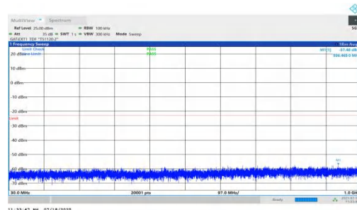
NTNV-n78(3450-3550)-PC1.5-30-15-L-DFT-BPSK-Inner_1RB_Right-3 0-1000-PASS
