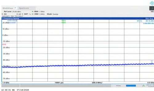
NTNV-n78(3450-3550)-PC1.5-30-20-H-DFT-BPSK-Inner_1RB_Right-1000-3000-PASS
