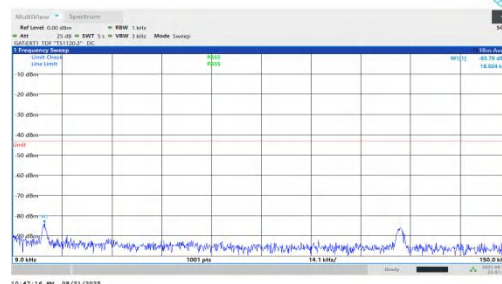
NTNV-n78(3450-3550)-PC1.5-30-20-M-DFT-QPSK-Inner_1RB_Right- 0.009-0.15-PASS
