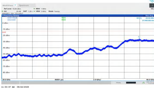
NTNV-n78(3450-3550)-PC1.5-30-15-H-DFT-BPSK-Inner_1RB_Left-2 0000-40000-PASS
