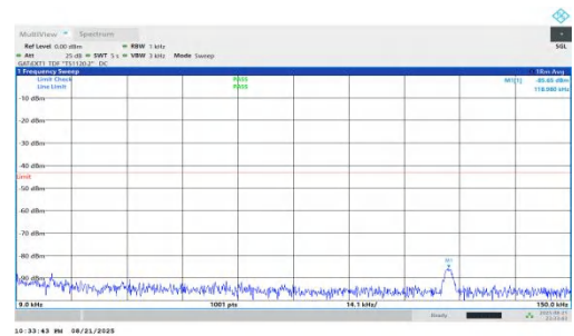
NTNV-n78(3450-3550)-PC1.5-30-10-H-DFT-QPSK-Inner_1RB_Right-0 .009-0.15-PASS
