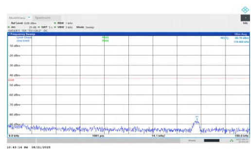
NTNV-n78(3450-3550)-PC1.5-30-20-L-DFT-BPSK-Inner_1RB_Right-0.009-0.15-PASS
