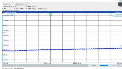
NTVN-n78(3450-3550)-PC1.5-30-10-L-DFT-QPSK-Inner_1RB_Left-10 00-3000-PASS
