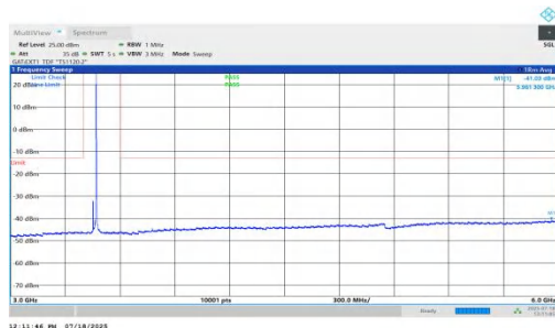
NTNV-n78(3450-3550)-PC1.5-30-20-L-DFT-BPSK-Inner_1RB_Right-3 000-6000-PASS
