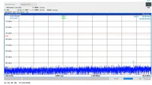
NTNV-n78(3450-3550)-PC1.5-30-20-H-DFT-BPSK-Inner_1RB_Left-0.15-30-PASS
