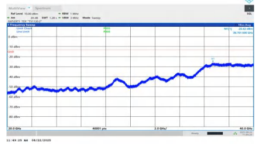
NTNV-n78(3450-3550)-PC1.5-30-15-L-DFT-BPSK-Inner_1RB_Right-20000-40000-PASS
