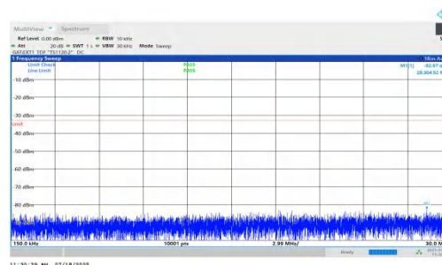
NTNV-n78(3450-3550)-PC1.5-30-15-L-DFT-BPSK-Inner_1RB_Left-0.15-5-30-PASS
