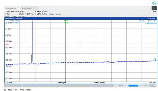
NTNV-n78(3450-3550)-PC1.5-30-20-H-DFT-BPSK-Inner_1RB_Right-3 000-6000-PASS
