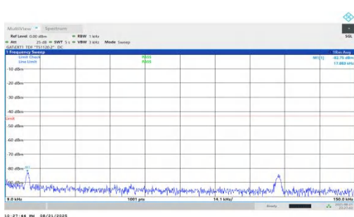
NTNV-n78(3450-3550)-PC1.5-30-10-L-DFT-QPSK-Inner_1RB_Left-0.009-0.15-PASS
