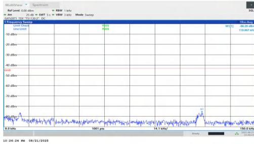
NTNV-n78(3450-3550)-PC1.5-30-10-L-DFT-BPSK-Inner_1RB_Left-0.009-0.15-PASS
