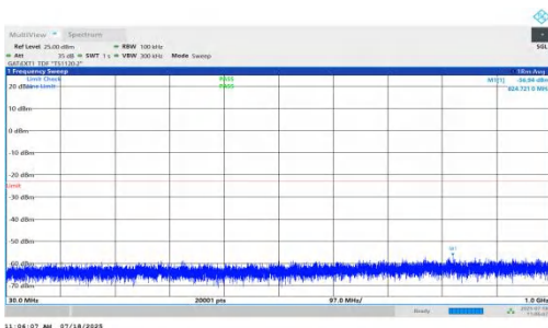
NTNV-n78(3450-3550)-PC1.5-30-10-M-DFT-BPSK-Inner_1RB_Left-30-1000-PASS
