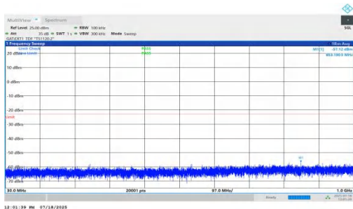
NTNV-n78(3450-3550)-PC1.5-30-15-H-DFT-QPSK-Inner_1RB_Left-30-1000-PASS
