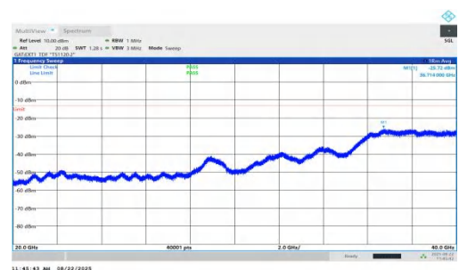
NTV-n78(3450-3550)-PC1.5-30-10-M-DFT-QPSK-Inner_1RB_Right- 20000-40000-PASS
