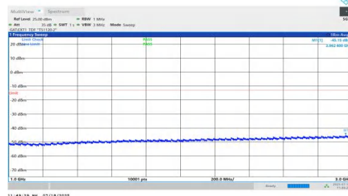
NTNV-n78(3450-3550)-PC1.5-30-15-M-DFT-QPSK-Inner_1RB_Left-10 00-3000-PASS
