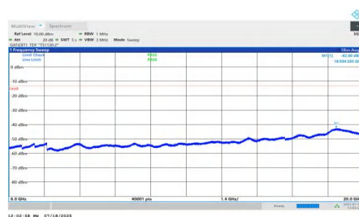
NTNV-n78(3450-3550)-PC1.5-30-15-H-DFT-QPSK-Inner_1RB_Left-6000-20000-PASS
