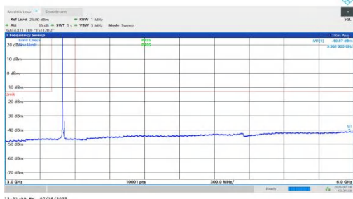
NTNV-n78(3450-3550)-PC1.5-30-20-M-DFT-BPSK-Inner_1RB_Left-3 000-6000-PASS
