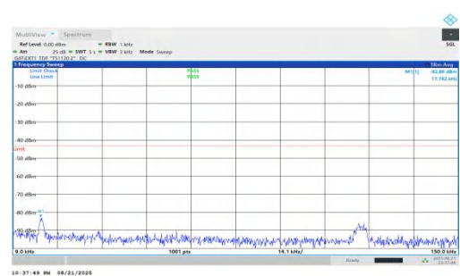
NTNV-n78(3450-3550)-PC1.5-30-15-M-DFT-BPSK-Inner_1RB_Right-0.009-0.15-PASS
