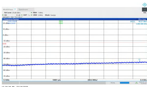
NTNV-n78(3450-3550)-PC1.5-30-20-M-DFT-QPSK-Inner_1RB_Right- 1000-3000-PASS
