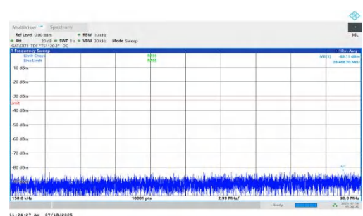
NTNV-n78(3450-3550)-PC1.5-30-10-H-DFT-QPSK-Inner_1RB_Left-0.15-30-PASS
