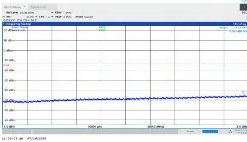
NTNV-n78(3450-3550)-PC1.5-30-10-L-DFT-QPSK-Inner_1RB_Right-1000-3000-PASS
