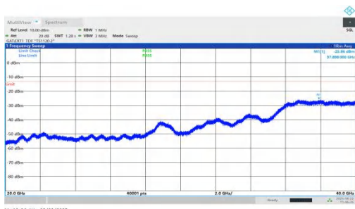
NTNV-n78(3450-3550)-PC1.5-30-10-H-DFT-BPSK-Inner_1RB_Left-20000-40000-PASS
