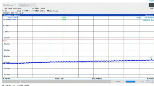
NTNV-n78(3450-3550)-PC1.5-30-10-H-DFT-QPSK-Inner_1RB_Right-1000-3000-PASS
