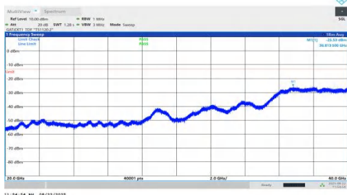
NTNV-n78(3450-3550)-PC1.5-30-15-H-DFT-QPSK-Inner_1RB_Left-2 0000-40000-PASS
