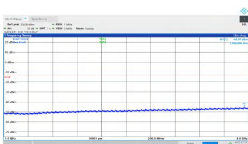
NTNV-n78(3450-3550)-PC1.5-30-10-M-DFT-BPSK-Inner_1RB_Right- 1000-3000-PASS
