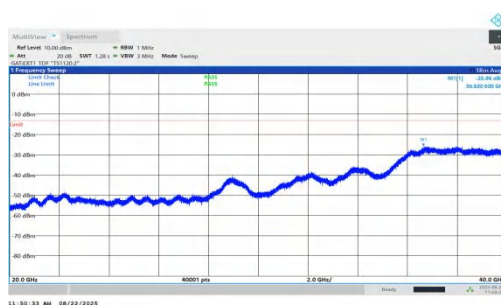
NTNV-n78(3450-3550)-PC1.5-30-15-L-DFT-QPSK-Inner_1RB_Right-2 0000-40000-PASS
