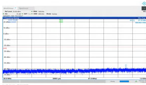
NTNV-n78(3450-3550)-PC1.5-30-10-M-DFT-BPSK-Inner_1RB_Right-3 0-1000-PASS
