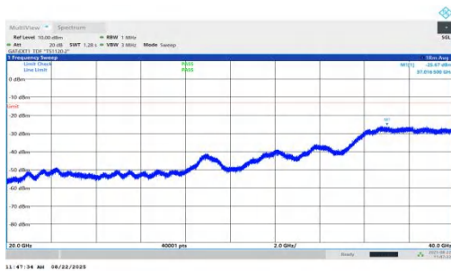
NTNV-n78(3450-3550)-PC1.5-30-10-H-DFT-QPSK-Inner_1RB_Left-2 0000-40000-PASS
