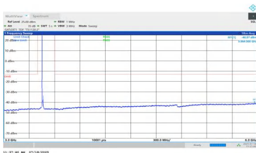
NTNV-n78(3450-3550)-PC1.5-30-15-L-DFT-QPSK-Inner_1RB_Left-3000-6000-PASS
