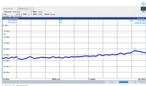
NTNV-n78(3450-3550)-PC1.5-30-15-M-DFT-QPSK-Inner_1RB_Right-6000-20000-PASS
