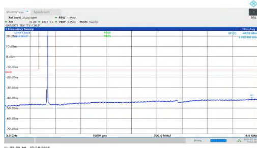
NTNV-n78(3450-3550)-PC1.5-30-15-M-DFT-QPSK-Inner_1RB_Right-3000-6000-PASS
