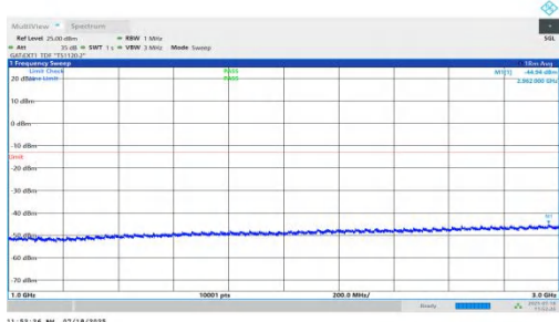
NTNV-n78(3450-3550)-PC1.5-30-15-M-DFT-QPSK-Inner_1RB_Right-1000-3000-PASS
