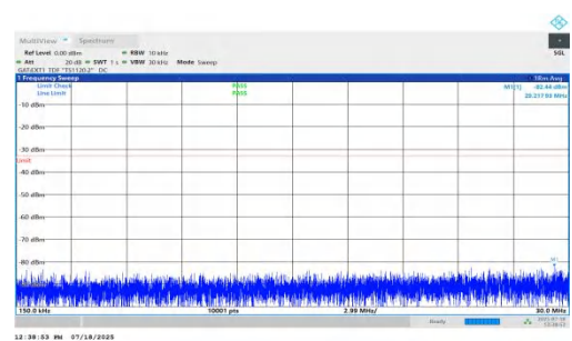
NTNV-n78(3450-3550)-PC1.5-30-20-H-DFT-QPSK-Inner_1RB_Left-0.15-30-PASS
