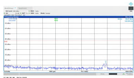
NTNV-n78(3450-3550)-PC1.5-30-20-H-DFT-BPSK-Inner_1RB_Right-0.009-0.15-PASS
