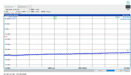
NTNV-n78(3450-3550)-PC1.5-30-20-L-DFT-BPSK-Inner_1RB_Left-1000-3000-PASS
