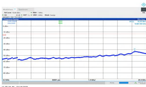
NTNV-n78(3450-3550)-PC1.5-30-10-L-DFT-BPSK-Inner_1RB_Right-6000-20000-PASS
