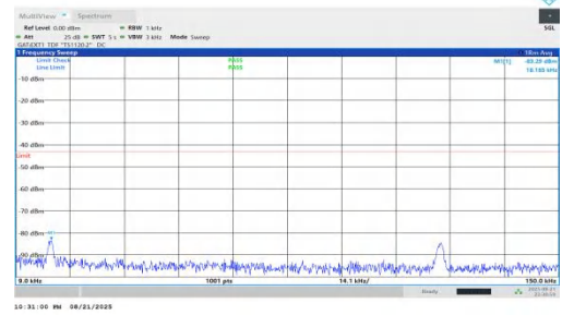
NTV-n78(3450-3550)-PC1.5-30-10-M-DFT-QPSK-Inner_1RB_Right- 0.009-0.15-PASS
