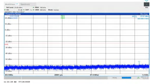
NTNV-n78(3450-3550)-PC1.5-30-10-H-DFT-BPSK-Inner_1RB_Right-3 0-1000-PASS
