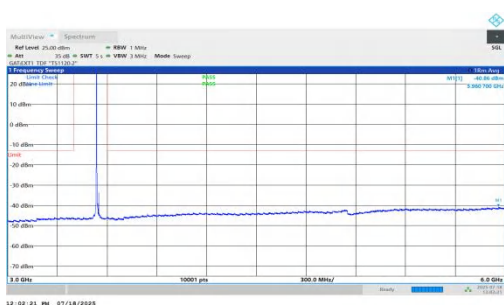
NTNV-n78(3450-3550)-PC1.5-30-15-H-DFT-QPSK-Inner_1RB_Left-3000-6000-PASS
