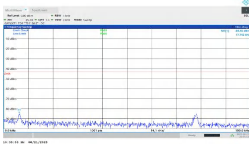
NTNV-n78(3450-3550)-PC1.5-30-15-L-DFT-QPSK-Inner_1RB_Left-0.009-0.15-PASS
