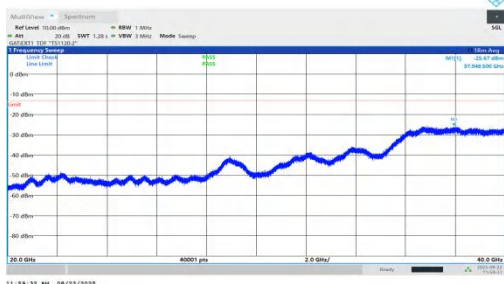
NTNV-n78(3450-3550)-PC1.5-30-20-M-DFT-QPSK-Inner_1RB_Left-2 0000-40000-PASS
