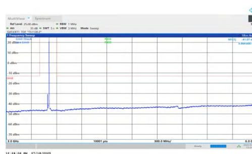
NTNV-n78(3450-3550)-PC1.5-30-20-M-DFT-BPSK-Inner_1RB_Right-3 000-6000-PASS
