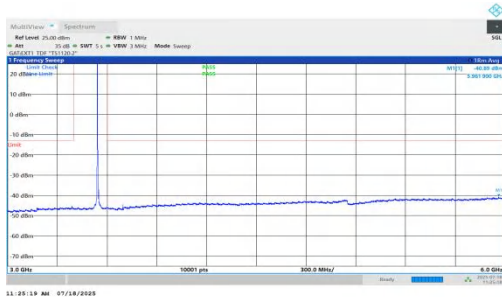
NTNV-n78(3450-3550)-PC1.5-30-10-H-DFT-QPSK-Inner_1RB_Left-3 000-6000-PASS
