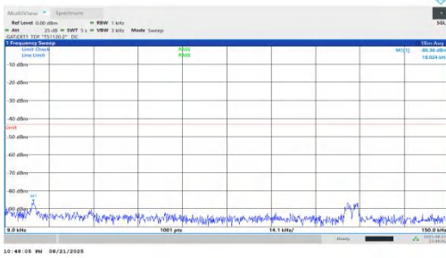
NTNV-n78(3450-3550)-PC1.5-30-20-H-DFT-BPSK-Inner_1RB_Left-0.009-0.15-PASS
