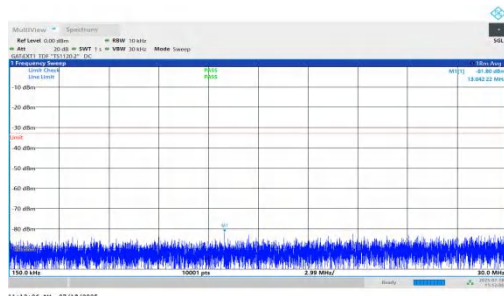
NTNV-n78(3450-3550)-PC1.5-30-10-M-DFT-QPSK-Inner_1RB_Left-0.15-30-PASS
