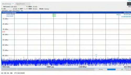
NTNV-n78(3450-3550)-PC1.5-30-20-H-DFT-BPSK-Inner_1RB_Right-0.15-30-PASS
