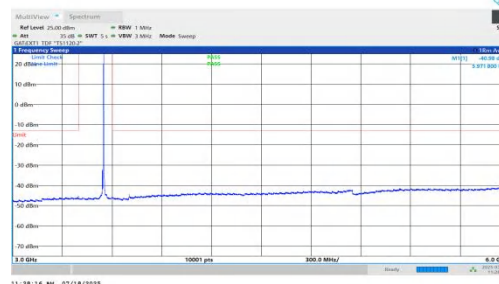
NTNV-n78(3450-3550)-PC1.5-30-10-H-DFT-QPSK-Inner_1RB_Right-3000-6000-PASS
