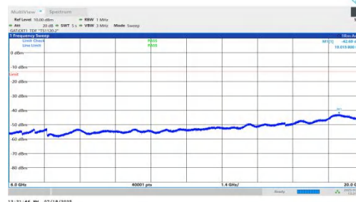
NTNV-n78(3450-3550)-PC1.5-30-20-M-DFT-BPSK-Inner_1RB_Left-60 00-20000-PASS
