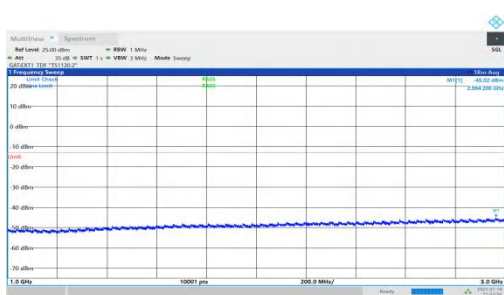
NTNV-n78(3450-3550)-PC1.5-30-15-L-DFT-BPSK-Inner_1RB_Right- 1000-3000-PASS
