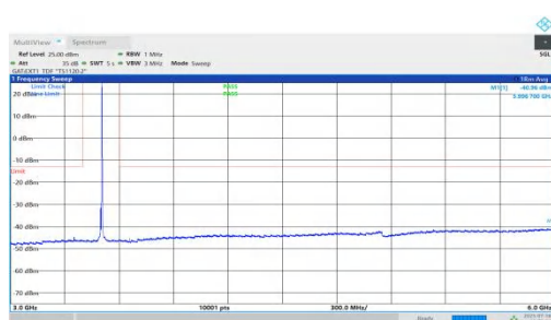
NTNV-n78(3450-3550)-PC1.5-30-10-M-DFT-BPSK-Inner_1RB_Right-3 000-6000-PASS
