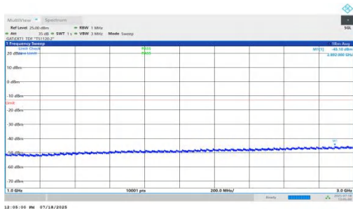
NTNV-n78(3450-3550)-PC1.5-30-15-H-DFT-QPSK-Inner_1RB_Right- 1000-3000-PASS
