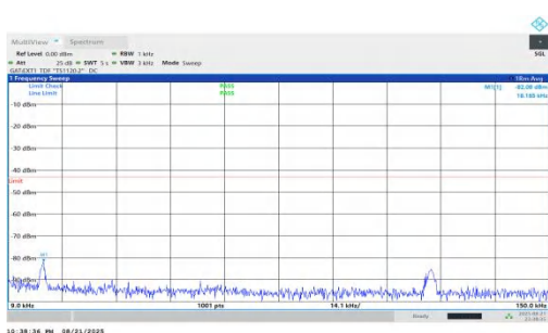
NTNV-n78(3450-3550)-PC1.5-30-15-M-DFT-QPSK-Inner_1RB_Left-0.009-0.15-PASS
