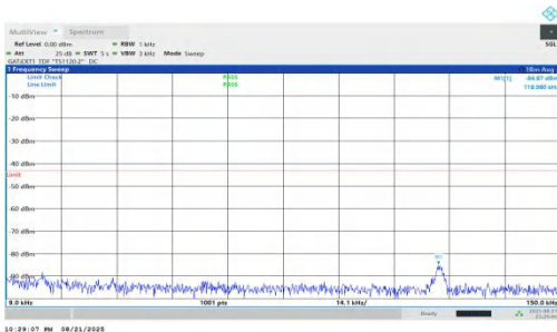
NTNV-n78(3450-3550)-PC1.5-30-10-M-DFT-BPSK-Inner_1RB_Left-0.009-0.15-PASS
