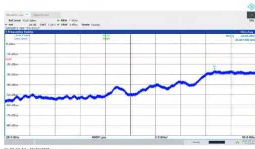
NTNV-n78(3450-3550)-PC1.5-30-15-M-DFT-QPSK-Inner_1RB_Right-20000-40000-PASS
