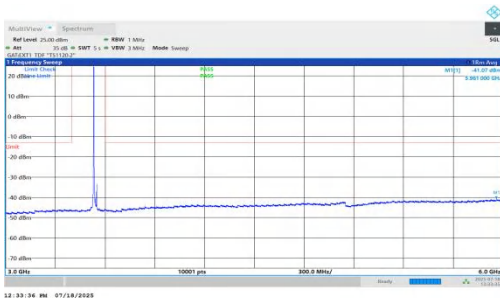
NTNV-n78(3450-3550)-PC1.5-30-20-H-DFT-BPSK-Inner_1RB_Left-3000-6000-PASS
