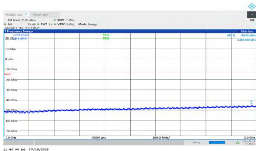
NTNV-n78(3450-3550)-PC1.5-30-15-L-DFT-QPSK-Inner_1RB_Right- 1000-3000-PASS
