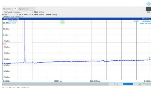
NTVN-n78(3450-3550)-PC1.5-30-10-L-DFT-QPSK-Inner_1RB_Left-3 000-6000-PASS
