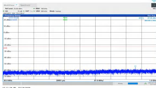
NTNV-n78(3450-3550)-PC1.5-30-20-L-DFT-BPSK-Inner_1RB_Right-3 0-1000-PASS
