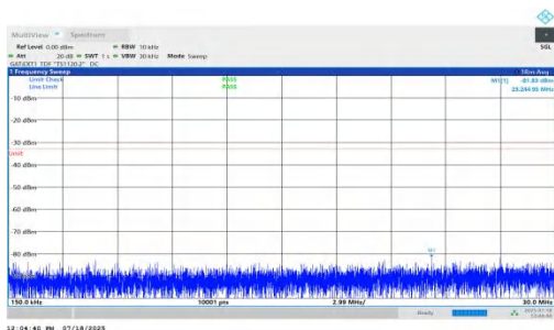
NTNV-n78(3450-3550)-PC1.5-30-15-H-DFT-QPSK-Inner_1RB_Right- 0.15-30-PASS
