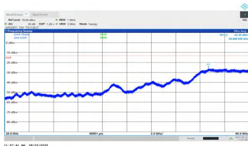
NTNV-n78(3450-3550)-PC1.5-30-20-L-DFT-QPSK-Inner_1RB_Right-20000-40000-PASS
