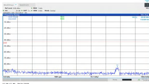
NTVN-n78(3450-3550)-PC1.5-30-10-L-DFT-QPSK-Inner_1RB_Right-0 .009-0.15-PASS
