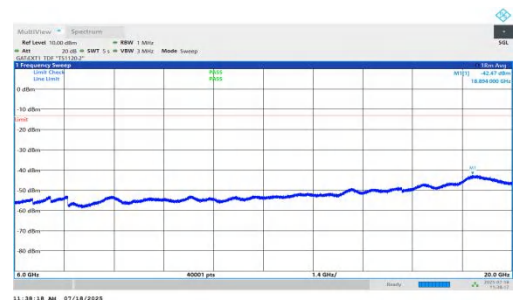
NTNV-n78(3450-3550)-PC1.5-30-15-L-DFT-QPSK-Inner_1RB_Left-6000-20000-PASS
