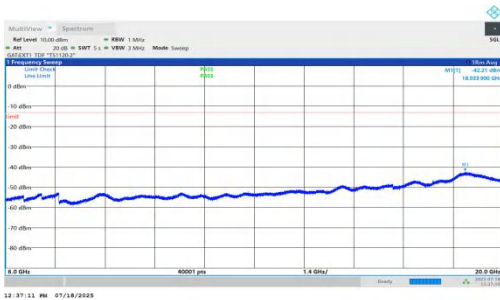
NTNV-n78(3450-3550)-PC1.5-30-20-H-DFT-BPSK-Inner_1RB_Right-6000-20000-PASS
