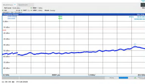
NTNV-n78(3450-3550)-PC1.5-30-15-L-DFT-BPSK-Inner_1RB_Right-6000-20000-PASS
