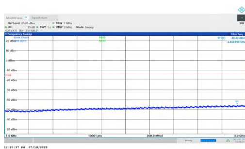
NTNV-n78(3450-3550)-PC1.5-30-20-M-DFT-BPSK-Inner_1RB_Left-1000-3000-PASS
