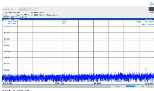
NTVN-n78(3450-3550)-PC1.5-30-10-L-DFT-QPSK-Inner_1RB_Right- 0.15-30-PASS
