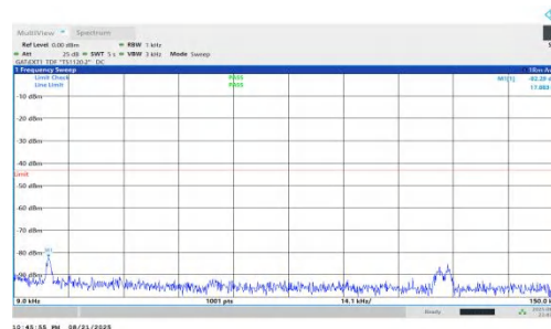
NTNV-n78(3450-3550)-PC1.5-30-20-M-DFT-BPSK-Inner_1RB_Right-0 .009-0.15-PASS
