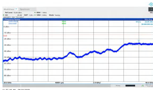
NTNV-n78(3450-3550)-PC1.5-30-15-M-DFT-BPSK-Inner_1RB_Right-2 0000-40000-PASS
