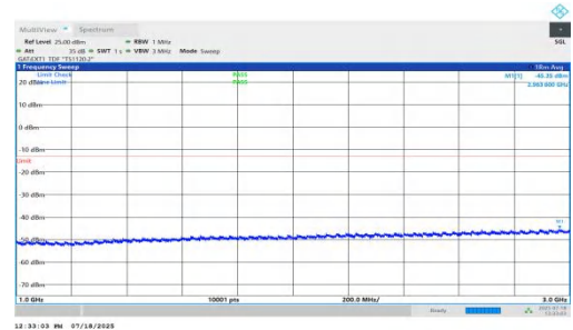
NTNV-n78(3450-3550)-PC1.5-30-20-H-DFT-BPSK-Inner_1RB_Left-1000-3000-PASS
