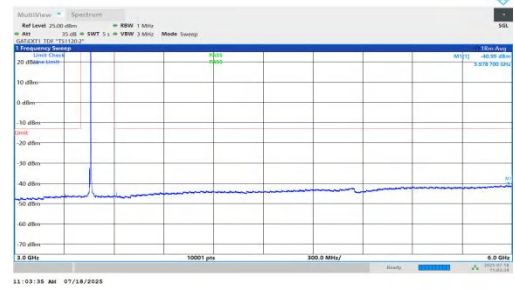
NTNV-n78(3450-3550)-PC1.5-30-10-L-DFT-QPSK-Inner_1RB_Right-3000-6000-PASS
