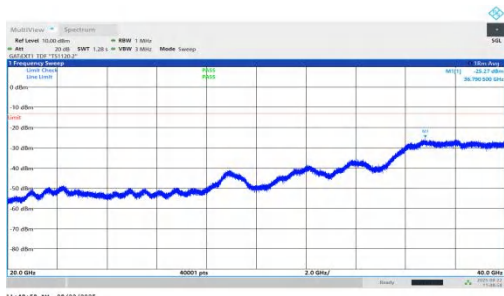
NTNV-n78(3450-3550)-PC1.5-30-15-L-DFT-BPSK-Inner_1RB_Left-20 000-40000-PASS
