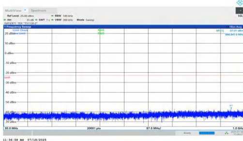
NTNV-n78(3450-3550)-PC1.5-30-15-L-DFT-QPSK-Inner_1RB_Left-30-1000-PASS
