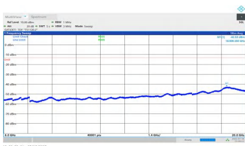
NTNV-n78(3450-3550)-PC1.5-30-20-M-DFT-QPSK-Inner_1RB_Right- 6000-20000-PASS
