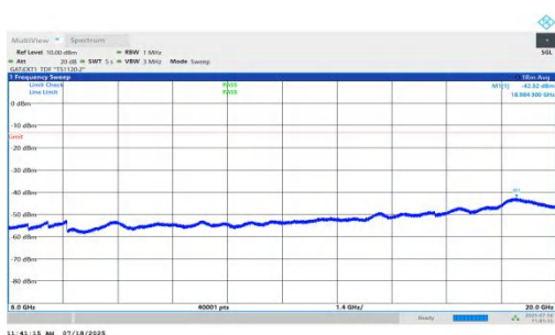
NTNV-n78(3450-3550)-PC1.5-30-15-L-DFT-QPSK-Inner_1RB_Right- 6000-20000-PASS
