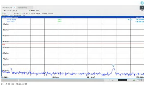
NTNV-n78(3450-3550)-PC1.5-30-20-M-DFT-QPSK-Inner_1RB_Left-0.009-0.15-PASS
