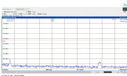
NTNV-n78(3450-3550)-PC1.5-30-20-L-DFT-QPSK-Inner_1RB_Left-0.009-0.15-PASS
