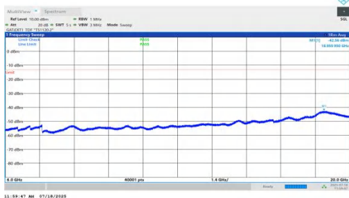
NTNV-n78(3450-3550)-PC1.5-30-15-H-DFT-BPSK-Inner_1RB_Right-6000-20000-PASS
