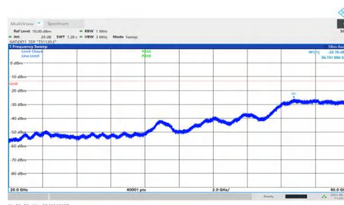
NTNV-n78(3450-3550)-PC1.5-30-20-M-DFT-QPSK-Inner_1RB_Right- 20000-40000-PASS
