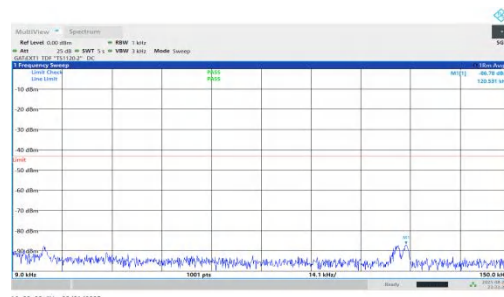
NTNV-n78(3450-3550)-PC1.5-30-10-H-DFT-BPSK-Inner_1RB_Right-0.009-0.15-PASS
