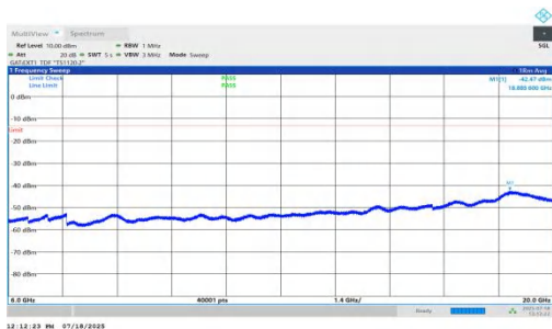
NTNV-n78(3450-3550)-PC1.5-30-20-L-DFT-BPSK-Inner_1RB_Right-6000-20000-PASS
