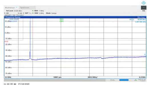
NTNV-n78(3450-3550)-PC1.5-30-10-H-DFT-BPSK-Inner_1RB_Right-3 000-6000-PASS
