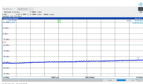
NTNV-n78(3450-3550)-PC1.5-30-10-L-DFT-BPSK-Inner_1RB_Right-1000-3000-PASS
