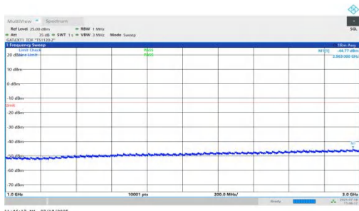
NTNV-n78(3450-3550)-PC1.5-30-15-M-DFT-BPSK-Inner_1RB_Right-1000-3000-PASS
