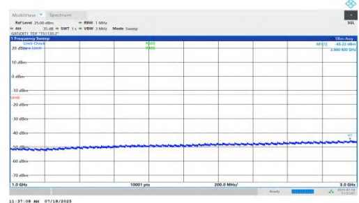
NTNV-n78(3450-3550)-PC1.5-30-15-L-DFT-QPSK-Inner_1RB_Left-1000-3000-PASS
