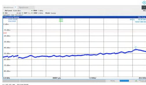
NTNV-n78(3450-3550)-PC1.5-30-10-M-DFT-BPSK-Inner_1RB_Left-60 00-20000-PASS
