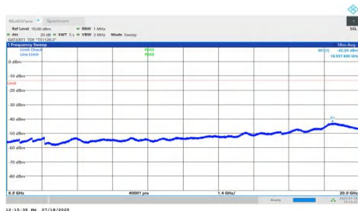
NTV-n78(3450-3550)-PC1.5-30-20-L-DFT-QPSK-Inner_1RB_Left-60 00-20000-PASS
