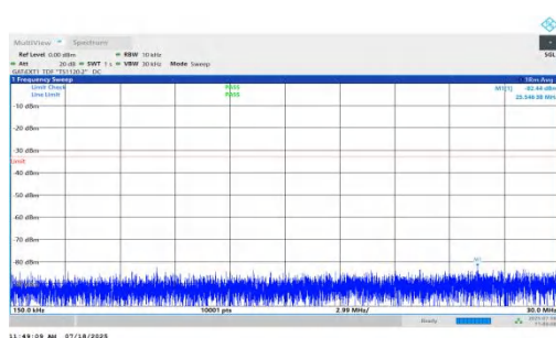
NTNV-n78(3450-3550)-PC1.5-30-15-M-DFT-QPSK-Inner_1RB_Left-0.15-30-PASS
