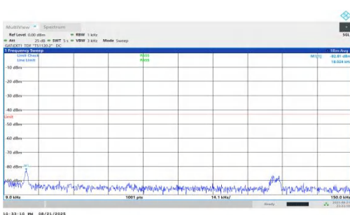
NTNV-n78(3450-3550)-PC1.5-30-10-H-DFT-QPSK-Inner_1RB_Left-0.009-0.15-PASS
