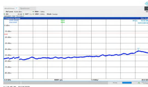
NTNV-n78(3450-3550)-PC1.5-30-10-H-DFT-BPSK-Inner_1RB_Left-6000-20000-PASS
