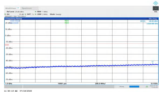
NTNV-n78(3450-3550)-PC1.5-30-15-M-DFT-BPSK-Inner_1RB_Left-1000-3000-PASS
