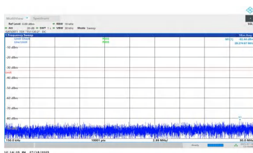
NTNV-n78(3450-3550)-PC1.5-30-20-L-DFT-QPSK-Inner_1RB_Left-0.1 5-30-PASS
