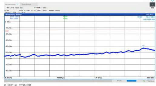
NTNV-n78(3450-3550)-PC1.5-30-10-L-DFT-BPSK-Inner_1RB_Left-6000-20000-PASS
