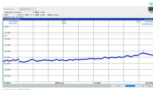
NTVN-n78(3450-3550)-PC1.5-30-10-L-DFT-QPSK-Inner_1RB_Left-60 00-20000-PASS
