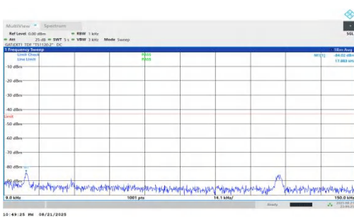
NTNV-n78(3450-3550)-PC1.5-30-20-H-DFT-QPSK-Inner_1RB_Left-0.009-0.15-PASS
