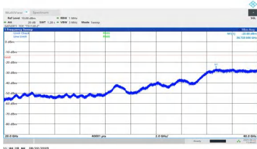
NTNV-n78(3450-3550)-PC1.5-30-10-M-DFT-BPSK-Inner_1RB_Left-2 0000-40000-PASS
