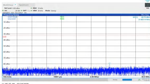
NTNV-n78(3450-3550)-PC1.5-30-15-M-DFT-BPSK-Inner_1RB_Right-0.15-30-PASS
