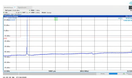
NTNV-n78(3450-3550)-PC1.5-30-15-H-DFT-QPSK-Inner_1RB_Right-3 000-6000-PASS
