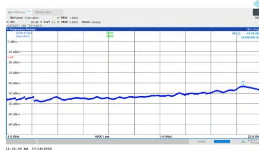
NTNV-n78(3450-3550)-PC1.5-30-15-L-DFT-BPSK-Inner_1RB_Left-60 00-20000-PASS
