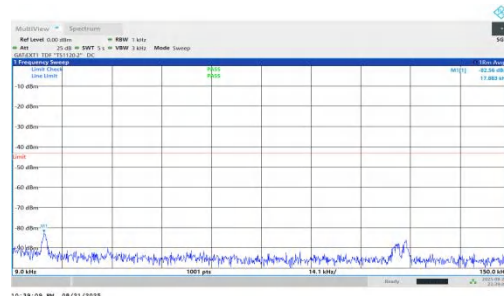
NTNV-n78(3450-3550)-PC1.5-30-15-M-DFT-QPSK-Inner_1RB_Right- 0.009-0.15-PASS
