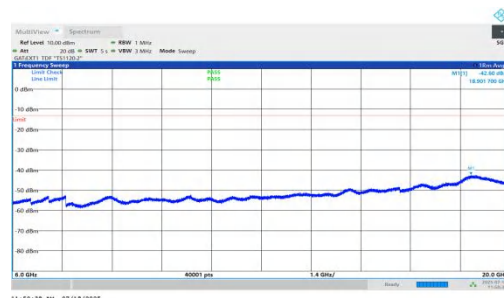
NTNV-n78(3450-3550)-PC1.5-30-15-M-DFT-QPSK-Inner_1RB_Left-60 00-20000-PASS
