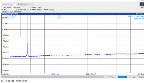
NTNV-n78(3450-3550)-PC1.5-30-15-H-DFT-BPSK-Inner_1RB_Left-3 000-6000-PASS
