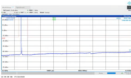
NTNV-n78(3450-3550)-PC1.5-30-20-L-DFT-BPSK-Inner_1RB_Left-3000-6000-PASS
