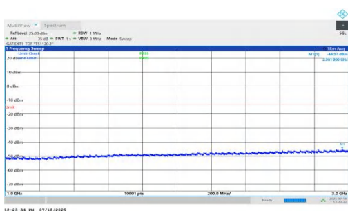
NTNV-n78(3450-3550)-PC1.5-30-20-M-DFT-BPSK-Inner_1RB_Right- 1000-3000-PASS
