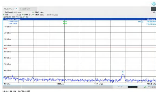
NTV-n78(3450-3550)-PC1.5-30-20-L-DFT-QPSK-Inner_1RB_Right-0 .009-0.15-PASS
