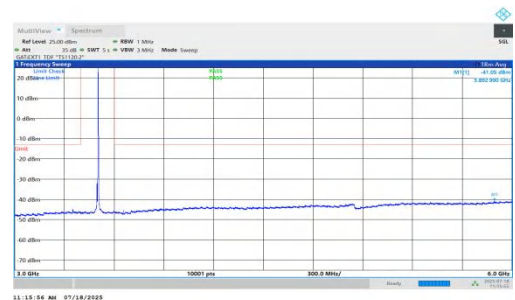
NTV-n78(3450-3550)-PC1.5-30-10-M-DFT-QPSK-Inner_1RB_Right- 3000-6000-PASS
