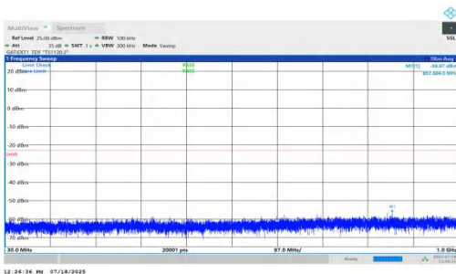
NTNV-n78(3450-3550)-PC1.5-30-20-M-DFT-QPSK-Inner_1RB_Left-30-1000-PASS
