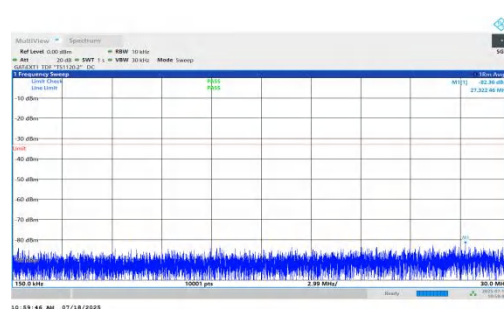
NTNV-n78(3450-3550)-PC1.5-30-10-L-DFT-QPSK-Inner_1RB_Left-0.1 5-30-PASS
