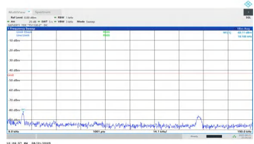
NTNV-n78(3450-3550)-PC1.5-30-10-L-DFT-BPSK-Inner_1RB_Right-0.009-0.15-PASS
