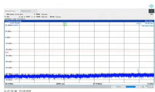
NTNV-n78(3450-3550)-PC1.5-30-10-H-DFT-QPSK-Inner_1RB_Right-3 0-1000-PASS
