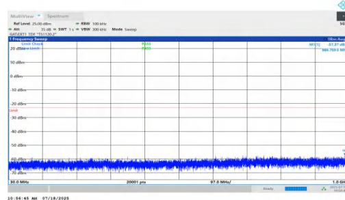
NTNV-n78(3450-3550)-PC1.5-30-10-L-DFT-BPSK-Inner_1RB_Right-3 0-1000-PASS
