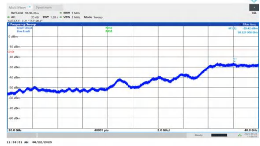
NTNV-n78(3450-3550)-PC1.5-30-20-M-DFT-BPSK-Inner_1RB_Right-20000-40000-PASS
