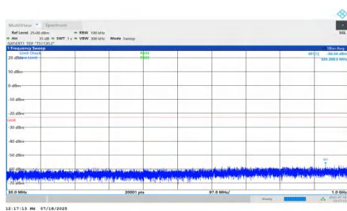
NTV-n78(3450-3550)-PC1.5-30-20-L-DFT-QPSK-Inner_1RB_Right-3 0-1000-PASS
