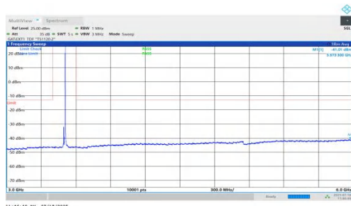
NTNV-n78(3450-3550)-PC1.5-30-15-M-DFT-BPSK-Inner_1RB_Right-3 000-6000-PASS
