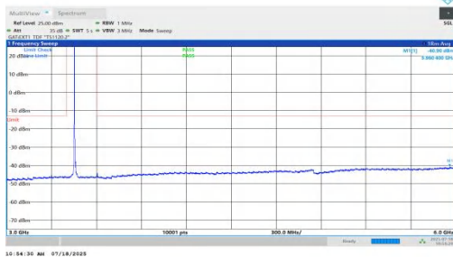
NTNV-n78(3450-3550)-PC1.5-30-10-L-DFT-BPSK-Inner_1RB_Left-3000-6000-PASS
