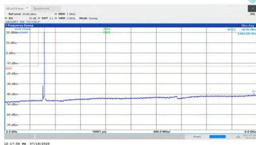
NTNV-n78(3450-3550)-PC1.5-30-20-L-DFT-QPSK-Inner_1RB_Right-3000-6000-PASS
