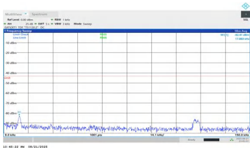
NTNV-n78(3450-3550)-PC1.5-30-20-M-DFT-BPSK-Inner_1RB_Left-0.009-0.15-PASS
