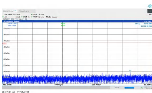
NTNV-n78(3450-3550)-PC1.5-30-10-H-DFT-QPSK-Inner_1RB_Right- 0.15-30-PASS
