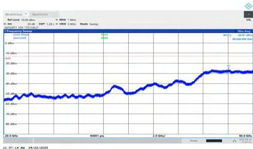
NTV-n78(3450-3550)-PC1.5-30-20-L-DFT-QPSK-Inner_1RB_Left-2 0000-40000-PASS
