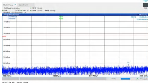
NTNV-n78(3450-3550)-PC1.5-30-20-L-DFT-BPSK-Inner_1RB_Right-0.15-30-PASS
