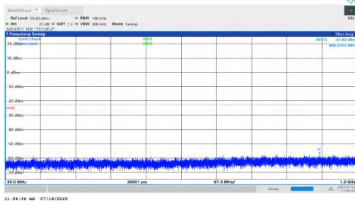
NTNV-n78(3450-3550)-PC1.5-30-10-H-DFT-QPSK-Inner_1RB_Left-3 0-1000-PASS
