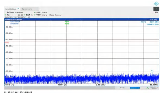
NTNV-n78(3450-3550)-PC1.5-30-10-M-DFT-BPSK-Inner_1RB_Left-0.15-30-PASS
