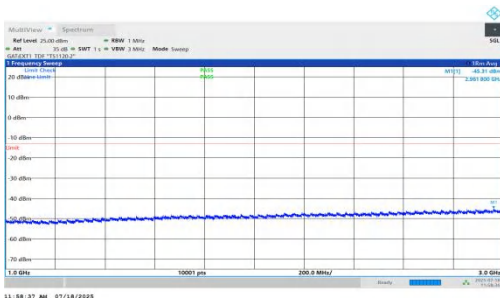
NTNV-n78(3450-3550)-PC1.5-30-15-H-DFT-BPSK-Inner_1RB_Right- 1000-3000-PASS
