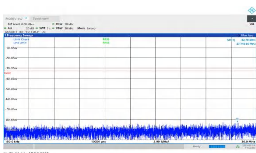
NTNV-n78(3450-3550)-PC1.5-30-15-M-DFT-QPSK-Inner_1RB_Right- 0.15-30-PASS
