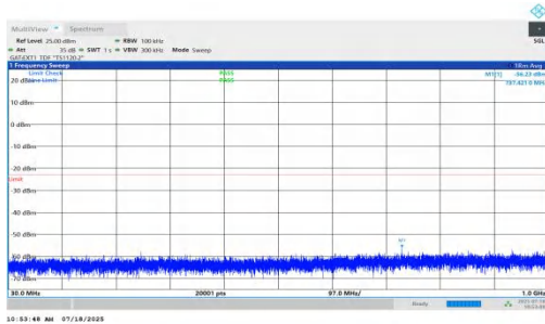
NTNV-n78(3450-3550)-PC1.5-30-10-L-DFT-BPSK-Inner_1RB_Left-30-1000-PASS
