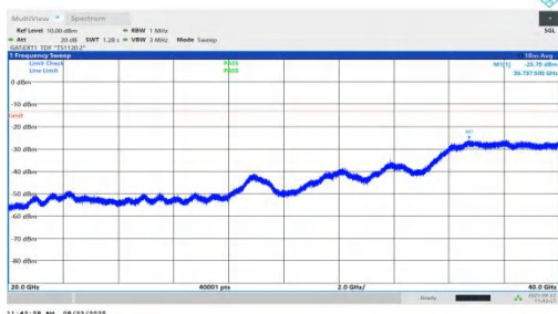
NTVN-n78(3450-3550)-PC1.5-30-10-L-DFT-QPSK-Inner_1RB_Left-2 0000-40000-PASS
