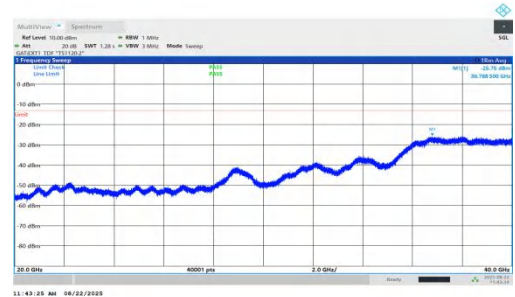
NTNV-n78(3450-3550)-PC1.5-30-10-L-DFT-QPSK-Inner_1RB_Right-20000-40000-PASS
