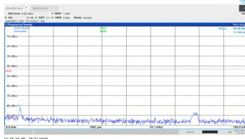
NTNV-n78(3450-3550)-PC1.5-30-15-L-DFT-QPSK-Inner_1RB_Right-0 .009-0.15-PASS
