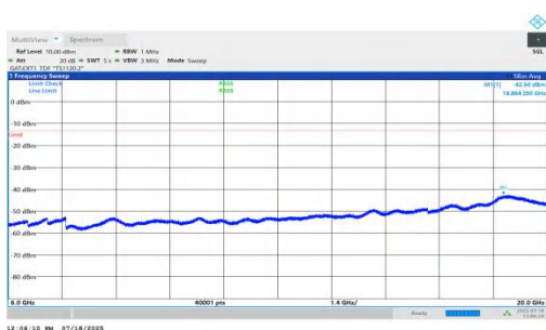
NTNV-n78(3450-3550)-PC1.5-30-15-H-DFT-QPSK-Inner_1RB_Right- 6000-20000-PASS
