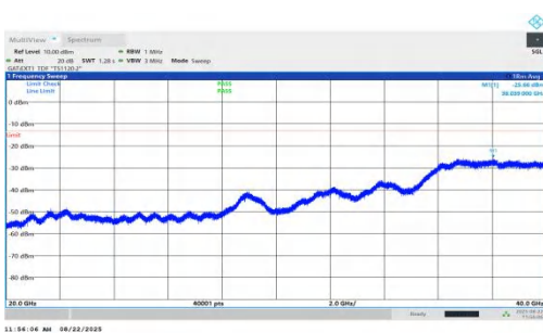
NTNV-n78(3450-3550)-PC1.5-30-20-L-DFT-BPSK-Inner_1RB_Left-20000-40000-PASS
