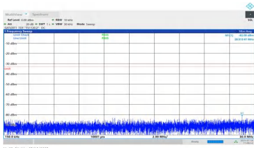
NTNV-n78(3450-3550)-PC1.5-30-10-M-DFT-BPSK-Inner_1RB_Right- 0.15-30-PASS
