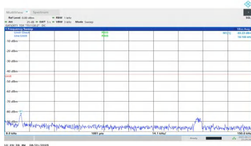
NTNV-n78(3450-3550)-PC1.5-30-10-M-DFT-BPSK-Inner_1RB_Right-0 .009-0.15-PASS
