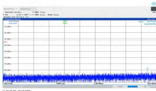
NTNV-n78(3450-3550)-PC1.5-30-15-H-DFT-BPSK-Inner_1RB_Left-0.15-5-30-PASS
