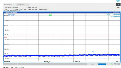
NTNV-n77(3700-3980)-PC1.5-30-100-H-DFT-BPSK-Inner_1RB_Right-30-1000-PASS
