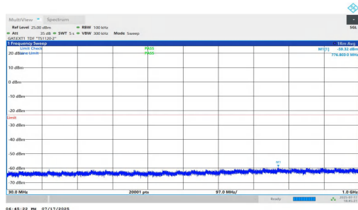
NTNV-n77(3700-3980)-PC1.5-30-100-M-DFT-QPSK-Inner_1RB_Right-30-1000-PASS
