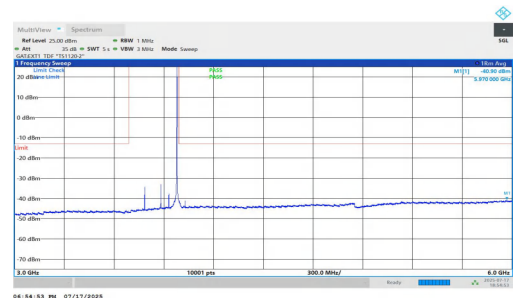
NTNV-n77(3700-3980)-PC1.5-30-100-H-DFT-BPSK-Inner_1RB_Right-3000-6000-PASS
