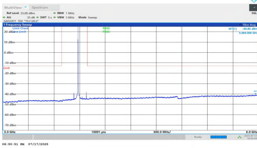
NTNV-n77(3700-3980)-PC1.5-30-100-H-DFT-BPSK-Inner_1RB_Left-3000-6000-PASS
