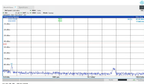
NTNV-n77(3700-3980)-PC1.5-30-100-M-DFT-QPSK-Inner_1RB_Right-0.009-0.15-PASS
