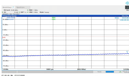
NTNV-n77(3700-3980)-PC1.5-30-100-H-DFT-QPSK-Inner_1RB_Right-1000-3000-PASS
