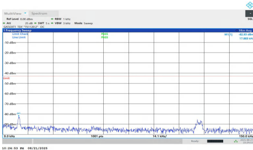
NTNV-n77(3700-3980)-PC1.5-30-100-H-DFT-QPSK-Inner_1RB_Left- 0.009-0.15-PASS
