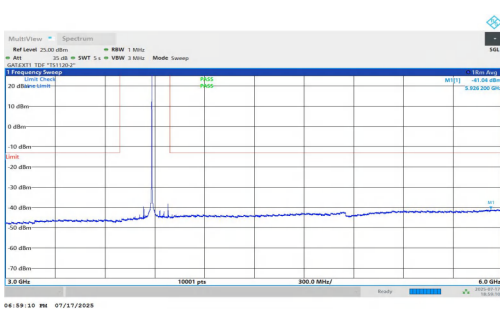
NTNV-n77(3700-3980)-PC1.5-30-100-H-DFT-QPSK-Inner_1RB_Left- 3000-6000-PASS
