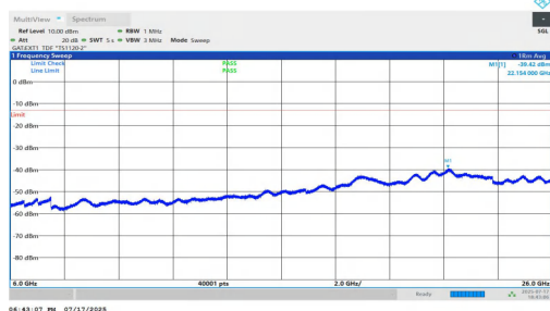
NTNV-n77(3700-3980)-PC1.5-30-100-M-DFT-QPSK-Inner_1RB_Left-6000-26000-PASS
