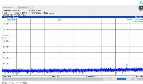
NTNV-n77(3700-3980)-PC1.5-30-100-H-DFT-QPSK-Inner_1RB_Right-0.15-30-PASS
