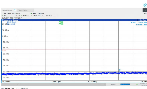
NTNV-n77(3700-3980)-PC1.5-30-100-H-DFT-BPSK-Inner_1RB_Left- 30-1000-PASS
