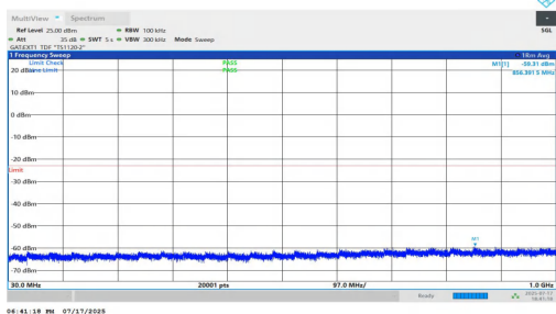
NTNV-n77(3700-3980)-PC1.5-30-100-M-DFT-QPSK-Inner_1RB_Left-30-1000-PASS
