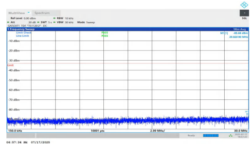
NTNV-n77(3700-3980)-PC1.5-30-100-H-DFT-QPSK-Inner_1RB_Left-0 .15-30-PASS
