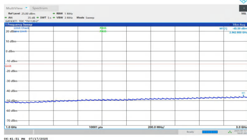
NTNV-n77(3700-3980)-PC1.5-30-100-M-DFT-QPSK-Inner_1RB_Left-1000-3000-PASS
