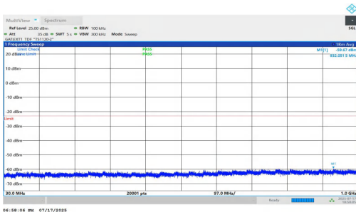
NTNV-n77(3700-3980)-PC1.5-30-100-H-DFT-QPSK-Inner_1RB_Left- 30-1000-PASS
