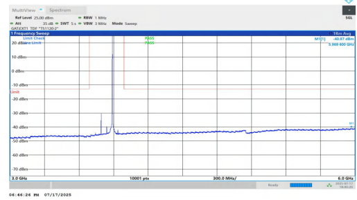
NTNV-n77(3700-3980)-PC1.5-30-100-M-DFT-QPSK-Inner_1RB_Right -3000-6000-PASS
