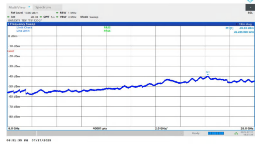
NTNV-n77(3700-3980)-PC1.5-30-100-H-DFT-BPSK-Inner_1RB_Left-6000-26000-PASS
