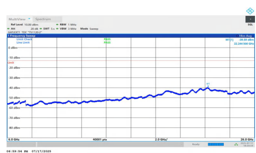
NTNV-n77(3700-3980)-PC1.5-30-100-H-DFT-QPSK-Inner_1RB_Left-6 000-26000-PASS
