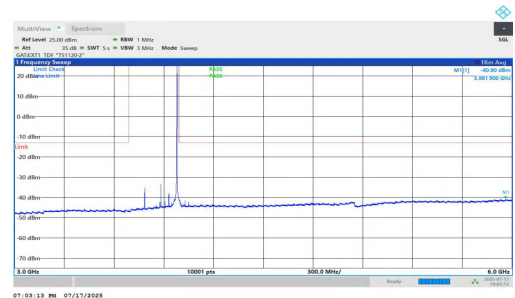
NTNV-n77(3700-3980)-PC1.5-30-100-H-DFT-QPSK-Inner_1RB_Right-3000-6000-PASS
