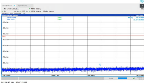
NTNV-n77(3700-3980)-PC1.5-30-100-H-DFT-BPSK-Inner_1RB_Right-0.15-30-PASS
