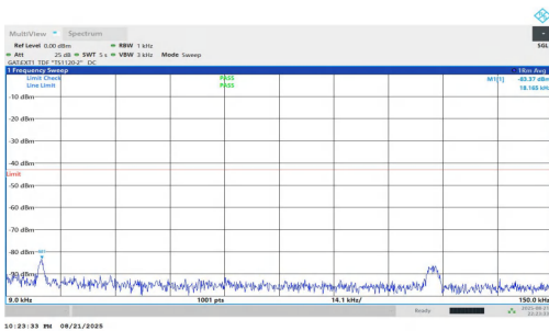
NTNV-n77(3700-3980)-PC1.5-30-100-H-DFT-BPSK-Inner_1RB_Left- 0.009-0.15-PASS
