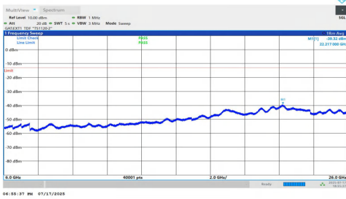
NTNV-n77(3700-3980)-PC1.5-30-100-H-DFT-BPSK-Inner_1RB_Right -6000-26000-PASS
