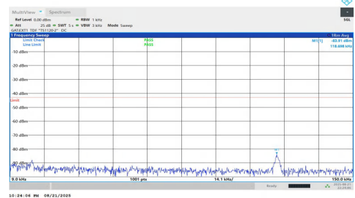
NTNV-n77(3700-3980)-PC1.5-30-100-H-DFT-BPSK-Inner_1RB_Right-0.009-0.15-PASS
