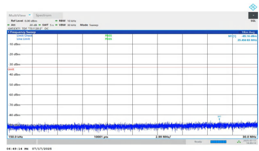
NTNV-n77(3700-3980)-PC1.5-30-100-H-DFT-BPSK-Inner_1RB_Left-0. 15-30-PASS
