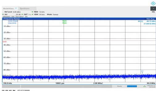
NTNV-n77(3700-3980)-PC1.5-30-100-M-DFT-QPSK-Inner_1RB_Right-t0.15-30-PASS
