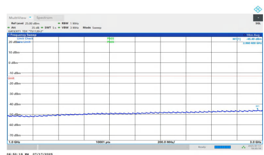
NTNV-n77(3700-3980)-PC1.5-30-100-H-DFT-BPSK-Inner_1RB_Left-1 000-3000-PASS
