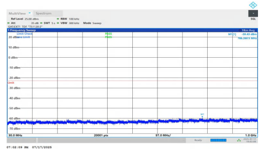
NTNV-n77(3700-3980)-PC1.5-30-100-H-DFT-QPSK-Inner_1RB_Right-30-1000-PASS
