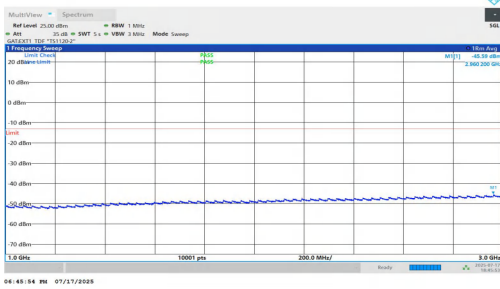
NTNV-n77(3700-3980)-PC1.5-30-100-M-DFT-QPSK-Inner_1RB_Right t-1000-3000-PASS
