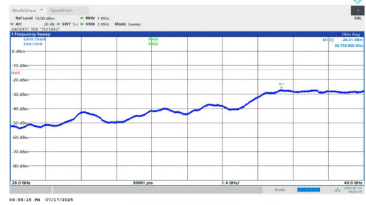
NTNV-n77(3700-3980)-PC1.5-30-100-H-DFT-BPSK-Inner_1RB_Right- 26000-40000-PASS
