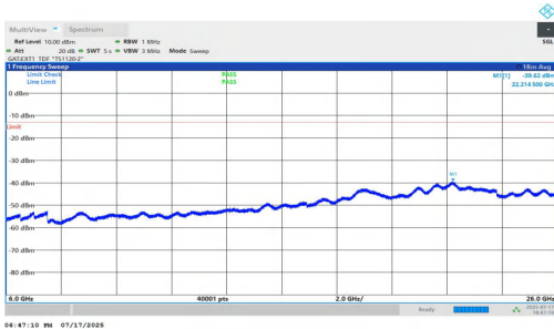
NTNV-n77(3700-3980)-PC1.5-30-100-M-DFT-QPSK-Inner_1RB_Right t-6000-26000-PASS
