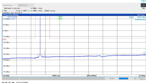
NTNV-n77(3700-3980)-PC1.5-30-100-M-DFT-QPSK-Inner_1RB_Left-3000-6000-PASS
