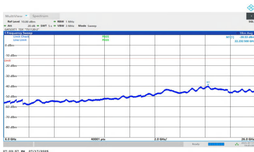
NTNV-n77(3700-3980)-PC1.5-30-100-H-DFT-QPSK-Inner_1RB_Right-6000-26000-PASS
