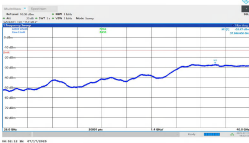
NTNV-n77(3700-3980)-PC1.5-30-100-H-DFT-BPSK-Inner_1RB_Left-26000-40000-PASS
