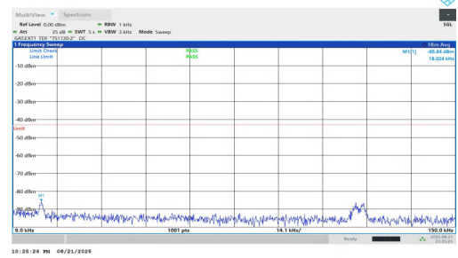
NTNV-n77(3700-3980)-PC1.5-30-100-H-DFT-QPSK-Inner_1RB_Right-0.009-0.15-PASS
