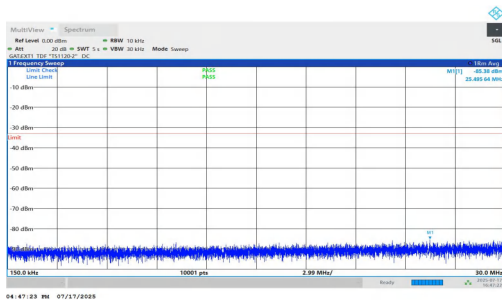
NTVN-n77(3700-3980)-PC1.5-30-80-L-DFT-QPSK-Inner_1RB_Right- 0.15-30-PASS
