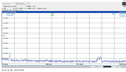
NTNV-n77(3700-3980)-PC1.5-30-90-L-DFT-BPSK-Inner_1RB_Left-0.009-0.15-PASS
