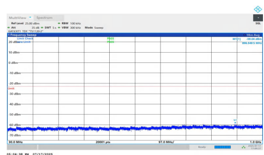
NTNV-n77(3700-3980)-PC1.5-30-80-M-DFT-QPSK-Inner_1RB_Right- 30-1000-PASS
