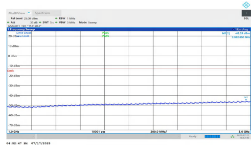
NTNV-n77(3700-3980)-PC1.5-30-80-M-DFT-BPSK-Inner_1RB_Left-1000-3000-PASS
