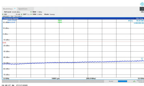
NTVN-n77(3700-3980)-PC1.5-30-80-L-DFT-QPSK-Inner_1RB_Right- 1000-3000-PASS
