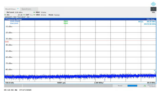
NTNV-n77(3700-3980)-PC1.5-30-80-H-DFT-QPSK-Inner_1RB_Left-0.15-30-PASS
