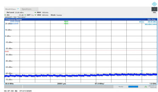
NTVN-n77(3700-3980)-PC1.5-30-80-L-DFT-QPSK-Inner_1RB_Right-3 0-1000-PASS
