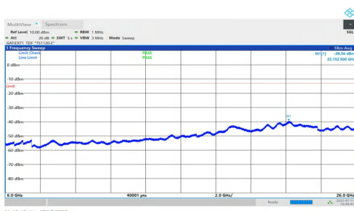
NTVN-n77(3700-3980)-PC1.5-30-80-L-DFT-QPSK-Inner_1RB_Right- 6000-26000-PASS
