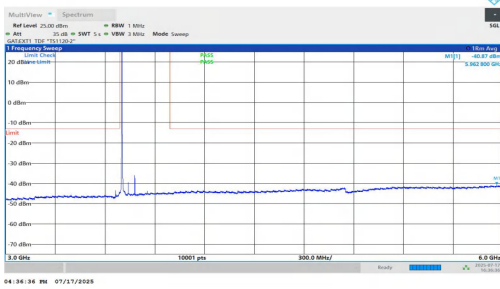
NTNV-n77(3700-3980)-PC1.5-30-80-L-DFT-BPSK-Inner_1RB_Left-30 00-6000-PASS
