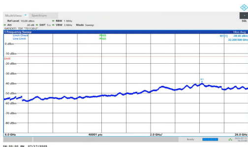
NTNV-n77(3700-3980)-PC1.5-30-70-H-DFT-QPSK-Inner_1RB_Right-6000-26000-PASS
