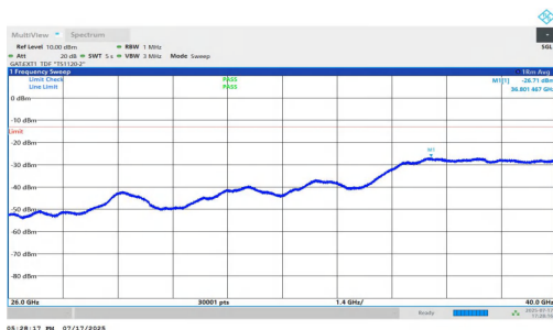
NTNV-n77(3700-3980)-PC1.5-30-90-L-DFT-BPSK-Inner_1RB_Left-26000-40000-PASS
