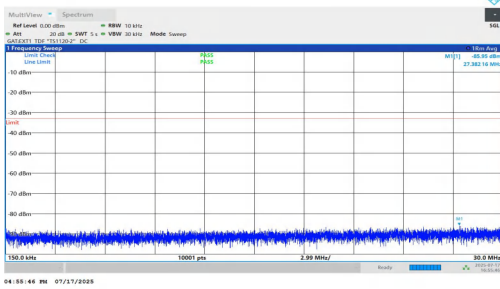
NTNV-n77(3700-3980)-PC1.5-30-80-M-DFT-BPSK-Inner_1RB_Right-0.15-30-PASS
