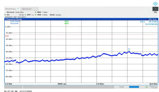
NTNV-n77(3700-3980)-PC1.5-30-90-L-DFT-BPSK-Inner_1RB_Left-6000-26000-PASS
