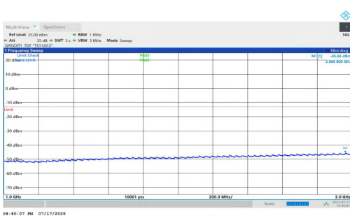
NTNV-n77(3700-3980)-PC1.5-30-80-L-DFT-BPSK-Inner_1RB_Right- 1000-3000-PASS
