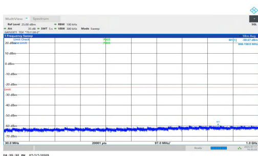
NTNV-n77(3700-3980)-PC1.5-30-80-L-DFT-BPSK-Inner_1RB_Left-30-1000-PASS
