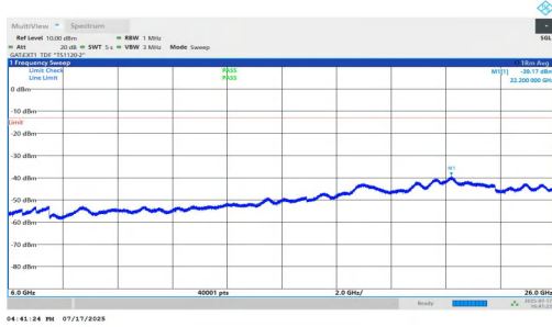
NTVN-n77(3700-3980)-PC1.5-30-80-L-DFT-BPSK-Inner_1RB_Right-6000-26000-PASS
