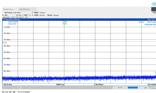
NTNV-n77(3700-3980)-PC1.5-30-80-H-DFT-QPSK-Inner_1RB_Right- 0.15-30-PASS
