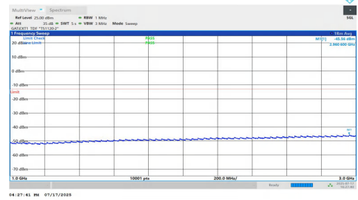
NTNV-n77(3700-3980)-PC1.5-30-70-H-DFT-QPSK-Inner_1RB_Left-10 00-3000-PASS
