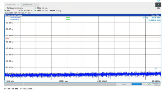
NTNV-n77(3700-3980)-PC1.5-30-80-M-DFT-BPSK-Inner_1RB_Left-0.15-30-PASS
