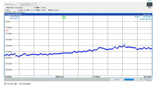
NTNV-n77(3700-3980)-PC1.5-30-80-H-DFT-BPSK-Inner_1RB_Left-60 00-26000-PASS
