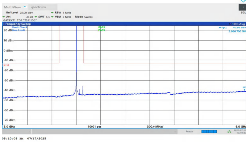
NTNV-n77(3700-3980)-PC1.5-30-80-H-DFT-BPSK-Inner_1RB_Left-3 000-6000-PASS
