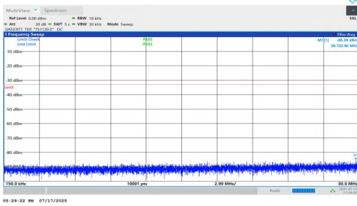
NTNV-n77(3700-3980)-PC1.5-30-90-L-DFT-BPSK-Inner_1RB_Right-0.15-30-PASS
