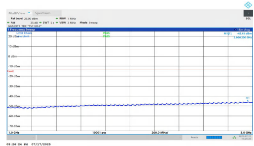
NTNV-n77(3700-3980)-PC1.5-30-90-L-DFT-BPSK-Inner_1RB_Left-1000-3000-PASS
