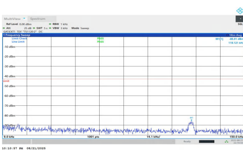
NTNV-n77(3700-3980)-PC1.5-30-90-L-DFT-QPSK-Inner_1RB_Left-0.009-0.15-PASS
