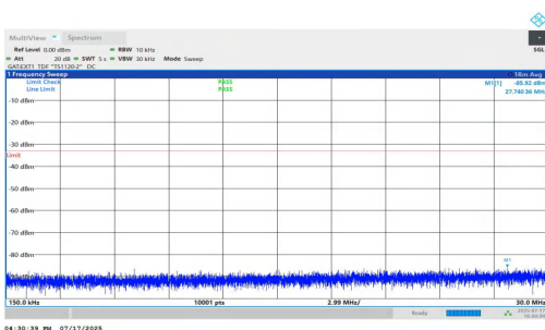
NTNV-n77(3700-3980)-PC1.5-30-70-H-DFT-QPSK-Inner_1RB_Right- 0.15-30-PASS
