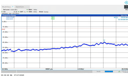
NTNV-n77(3700-3980)-PC1.5-30-80-M-DFT-QPSK-Inner_1RB_Right-6000-26000-PASS
