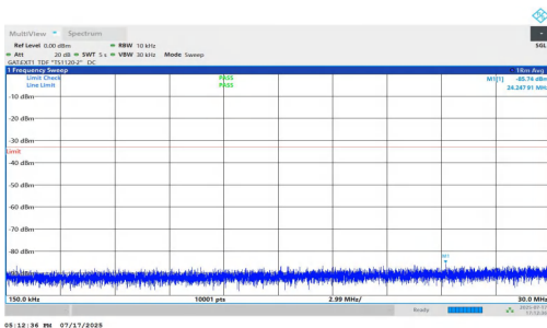
NTNV-n77(3700-3980)-PC1.5-30-80-H-DFT-BPSK-Inner_1RB_Right- 0.15-30-PASS
