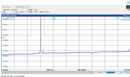
NTNV-n77(3700-3980)-PC1.5-30-70-H-DFT-QPSK-Inner_1RB_Left-3 000-6000-PASS
