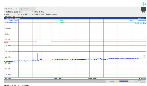
NTVN-n77(3700-3980)-PC1.5-30-80-L-DFT-QPSK-Inner_1RB_Right-3 000-6000-PASS
