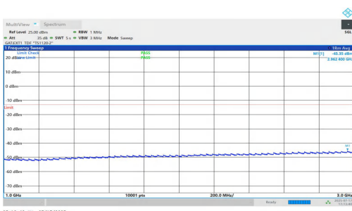
NTNV-n77(3700-3980)-PC1.5-30-80-H-DFT-BPSK-Inner_1RB_Right- 1000-3000-PASS
