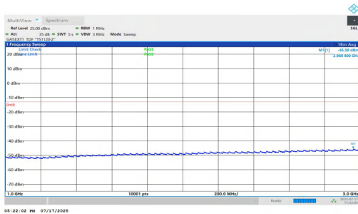
NTNV-n77(3700-3980)-PC1.5-30-80-H-DFT-QPSK-Inner_1RB_Right- 1000-3000-PASS
