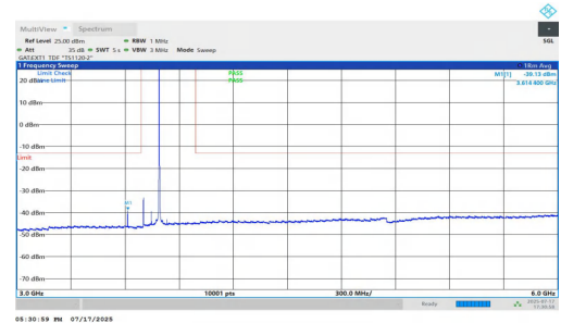
NTNV-n77(3700-3980)-PC1.5-30-90-L-DFT-BPSK-Inner_1RB_Right-3 000-6000-PASS
