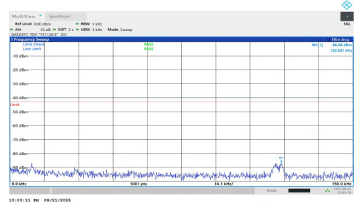
NTVN-n77(3700-3980)-PC1.5-30-80-L-DFT-QPSK-Inner_1RB_Right-0 .009-0.15-PASS
