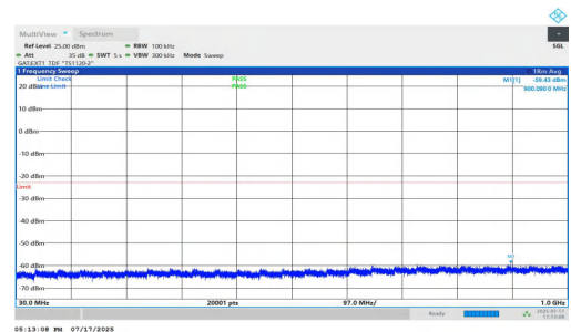
NTNV-n77(3700-3980)-PC1.5-30-80-H-DFT-BPSK-Inner_1RB_Right-3 0-1000-PASS
