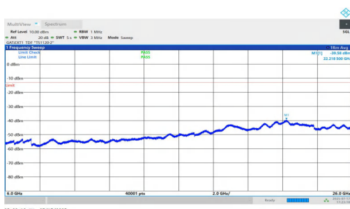
NTNV-n77(3700-3980)-PC1.5-30-80-H-DFT-QPSK-Inner_1RB_Right- 6000-26000-PASS
