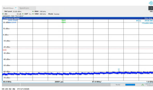
NTNV-n77(3700-3980)-PC1.5-30-90-L-DFT-BPSK-Inner_1RB_Left-30-1000-PASS
