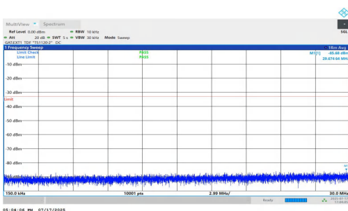
NTNV-n77(3700-3980)-PC1.5-30-80-M-DFT-QPSK-Inner_1RB_Right- 0.15-30-PASS
