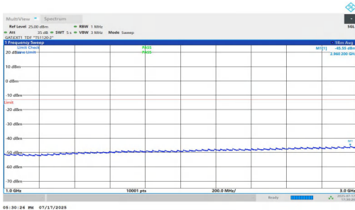
NTNV-n77(3700-3980)-PC1.5-30-90-L-DFT-BPSK-Inner_1RB_Right-1000-3000-PASS
