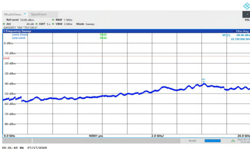
NTNV-n77(3700-3980)-PC1.5-30-90-L-DFT-BPSK-Inner_1RB_Right-6000-26000-PASS
