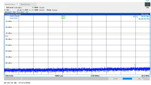
NTNV-n77(3700-3980)-PC1.5-30-90-L-DFT-BPSK-Inner_1RB_Left-0.15-30-PASS
