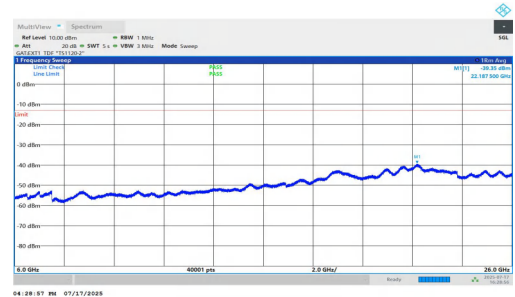
NTNV-n77(3700-3980)-PC1.5-30-70-H-DFT-QPSK-Inner_1RB_Left-60 00-26000-PASS
