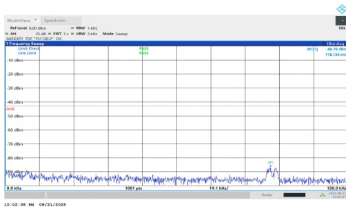
NTVN-n77(3700-3980)-PC1.5-30-80-L-DFT-QPSK-Inner_1RB_Left-0.009-0.15-PASS
