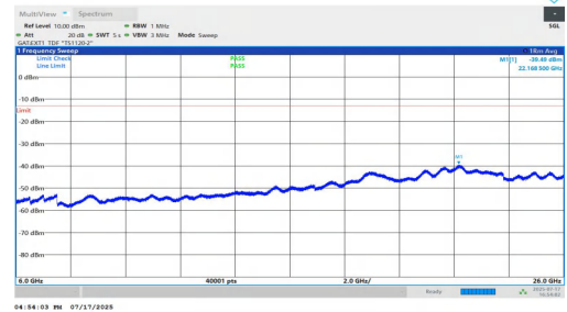
NTNV-n77(3700-3980)-PC1.5-30-80-M-DFT-BPSK-Inner_1RB_Left-6000-26000-PASS
