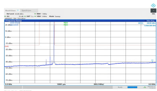
NTNV-n77(3700-3980)-PC1.5-30-80-H-DFT-BPSK-Inner_1RB_Right-3 000-6000-PASS
