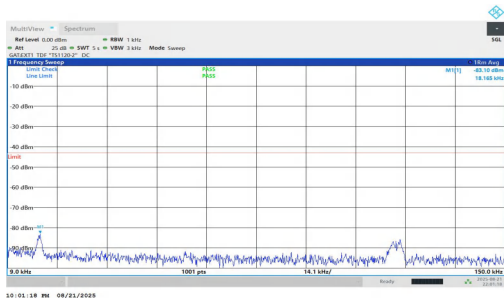
NTNV-n77(3700-3980)-PC1.5-30-80-L-DFT-BPSK-Inner_1RB_Left-0.009-0.15-PASS
