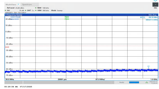
NTNV-n77(3700-3980)-PC1.5-30-90-L-DFT-BPSK-Inner_1RB_Right-3 0-1000-PASS
