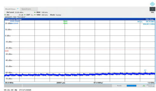
NTNV-n77(3700-3980)-PC1.5-30-80-H-DFT-QPSK-Inner_1RB_Right-3 0-1000-PASS
