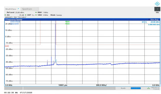
NTNV-n77(3700-3980)-PC1.5-30-80-H-DFT-QPSK-Inner_1RB_Right-3 000-6000-PASS
