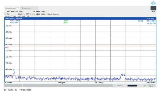
NTNV-n77(3700-3980)-PC1.5-30-80-L-DFT-BPSK-Inner_1RB_Right-0. 009-0.15-PASS
