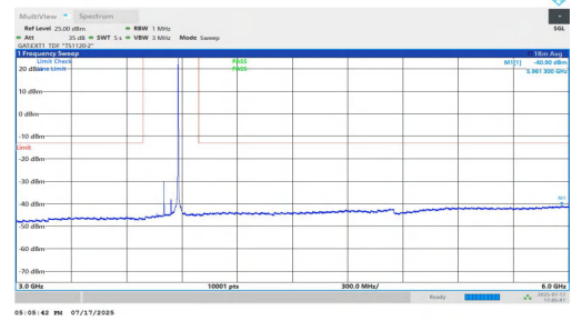
NTNV-n77(3700-3980)-PC1.5-30-80-M-DFT-QPSK-Inner_1RB_Right-3000-6000-PASS
