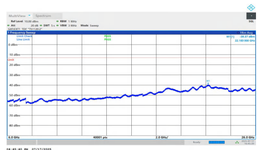
NTVN-n77(3700-3980)-PC1.5-30-80-L-DFT-QPSK-Inner_1RB_Left-6000-26000-PASS
