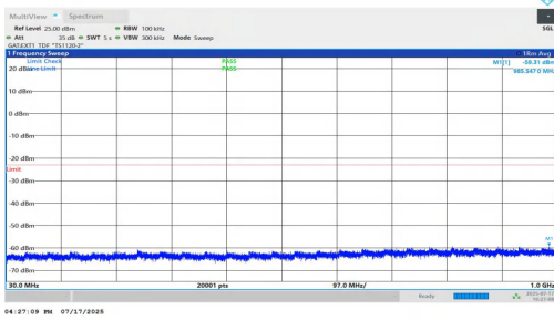
NTNV-n77(3700-3980)-PC1.5-30-70-H-DFT-QPSK-Inner_1RB_Left-3 0-1000-PASS
