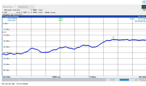
NTNV-n77(3700-3980)-PC1.5-30-80-H-DFT-QPSK-Inner_1RB_Left-2 6000-40000-PASS
