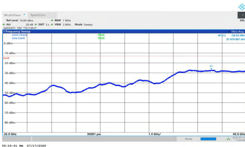
NTNV-n77(3700-3980)-PC1.5-30-80-M-DFT-QPSK-Inner_1RB_Left-2 6000-40000-PASS
