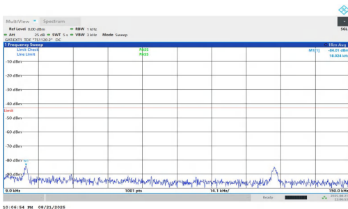
NTNV-n77(3700-3980)-PC1.5-30-80-H-DFT-BPSK-Inner_1RB_Left-0.009-0.15-PASS
