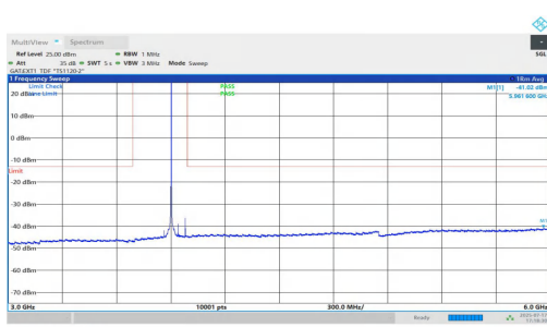
NTNV-n77(3700-3980)-PC1.5-30-80-H-DFT-QPSK-Inner_1RB_Left-3000-6000-PASS
