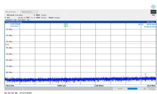
NTNV-n77(3700-3980)-PC1.5-30-90-L-DFT-QPSK-Inner_1RB_Left-0.1 5-30-PASS
