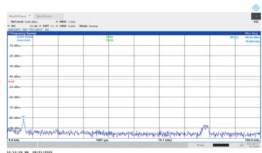
NTNV-n77(3700-3980)-PC1.5-30-90-L-DFT-BPSK-Inner_1RB_Right-0.009-0.15-PASS
