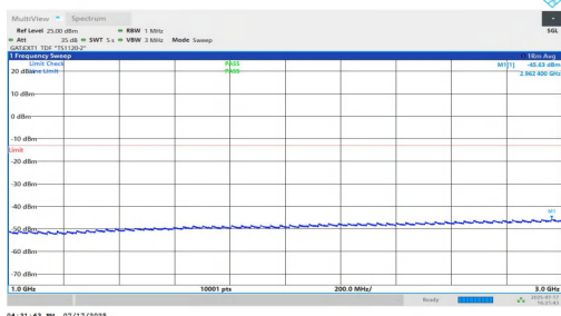
NTNV-n77(3700-3980)-PC1.5-30-70-H-DFT-QPSK-Inner_1RB_Right-1000-3000-PASS
