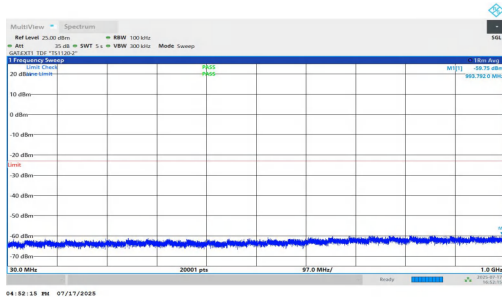
NTNV-n77(3700-3980)-PC1.5-30-80-M-DFT-BPSK-Inner_1RB_Left-30-1000-PASS
