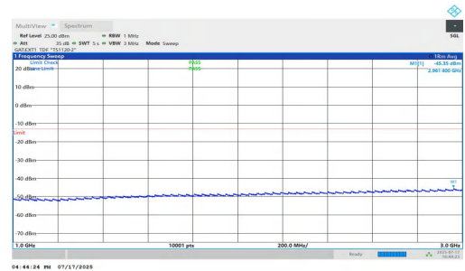
NTVN-n77(3700-3980)-PC1.5-30-80-L-DFT-QPSK-Inner_1RB_Left-1000-3000-PASS
