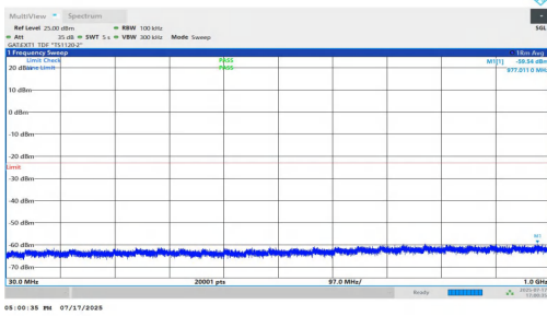
NTNV-n77(3700-3980)-PC1.5-30-80-M-DFT-QPSK-Inner_1RB_Left-3 0-1000-PASS
