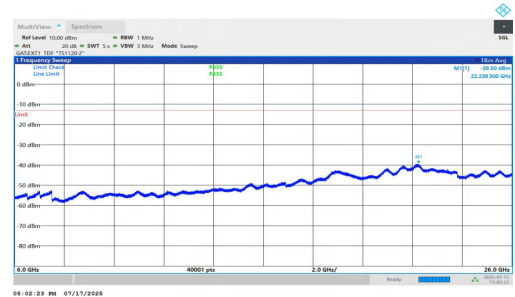
NTNV-n77(3700-3980)-PC1.5-30-80-M-DFT-QPSK-Inner_1RB_Left-60 00-26000-PASS
