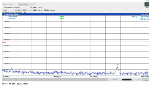
NTNV-n77(3700-3980)-PC1.5-30-80-M-DFT-BPSK-Inner_1RB_Left-0.009-0.15-PASS
