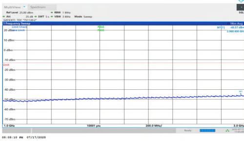
NTNV-n77(3700-3980)-PC1.5-30-80-M-DFT-QPSK-Inner_1RB_Right-1000-3000-PASS
