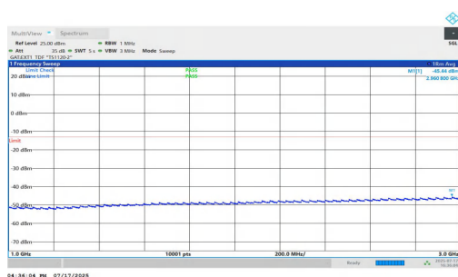
NTNV-n77(3700-3980)-PC1.5-30-80-L-DFT-BPSK-Inner_1RB_Left-1000-3000-PASS
