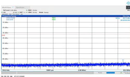
NTNV-n77(3700-3980)-PC1.5-30-80-L-DFT-BPSK-Inner_1RB_Right- 0.15-30-PASS
