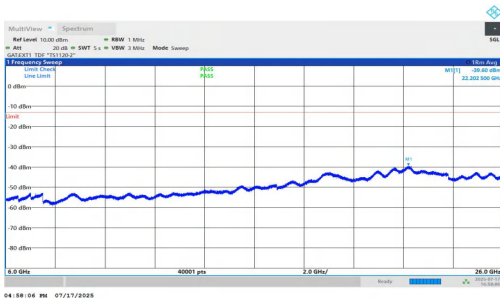
NTNV-n77(3700-3980)-PC1.5-30-80-M-DFT-BPSK-Inner_1RB_Right-6000-26000-PASS
