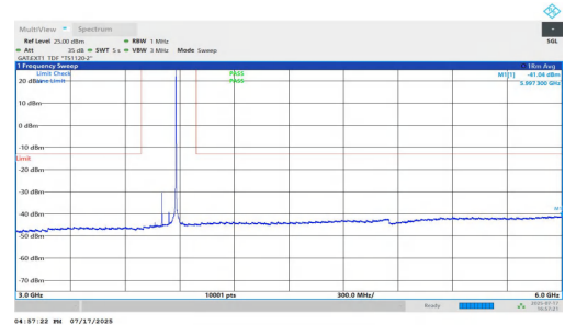
NTNV-n77(3700-3980)-PC1.5-30-80-M-DFT-BPSK-Inner_1RB_Right-3 000-6000-PASS
