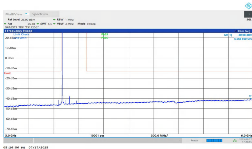
NTNV-n77(3700-3980)-PC1.5-30-90-L-DFT-BPSK-Inner_1RB_Left-3000-6000-PASS
