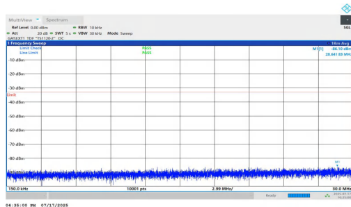
NTNV-n77(3700-3980)-PC1.5-30-80-L-DFT-BPSK-Inner_1RB_Left-0.15-5-30-PASS
