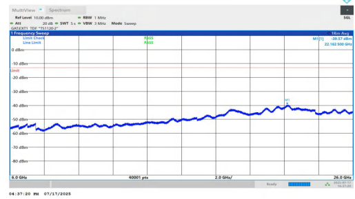
NTNV-n77(3700-3980)-PC1.5-30-80-L-DFT-BPSK-Inner_1RB_Left-60 00-26000-PASS
