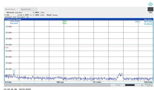
NTNV-n77(3700-3980)-PC1.5-30-80-M-DFT-QPSK-Inner_1RB_Right- 0.009-0.15-PASS
