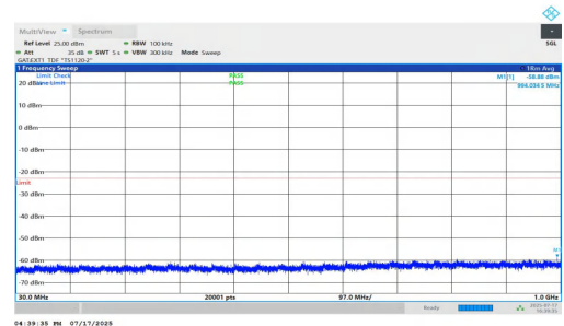
NTNV-n77(3700-3980)-PC1.5-30-80-L-DFT-BPSK-Inner_1RB_Right-3 0-1000-PASS
