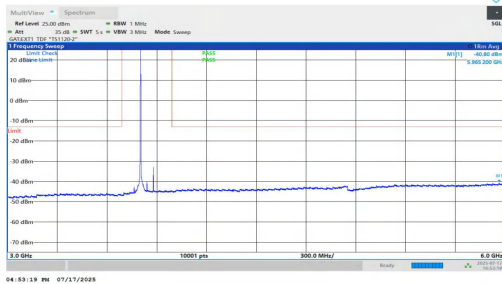
NTNV-n77(3700-3980)-PC1.5-30-80-M-DFT-BPSK-Inner_1RB_Left-3000-6000-PASS
