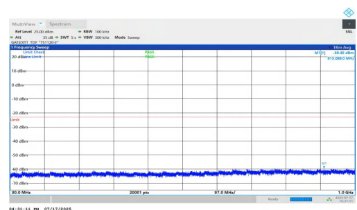
NTNV-n77(3700-3980)-PC1.5-30-70-H-DFT-QPSK-Inner_1RB_Right-3 0-1000-PASS
