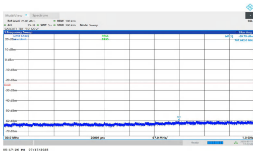
NTNV-n77(3700-3980)-PC1.5-30-80-H-DFT-QPSK-Inner_1RB_Left-30-1000-PASS
