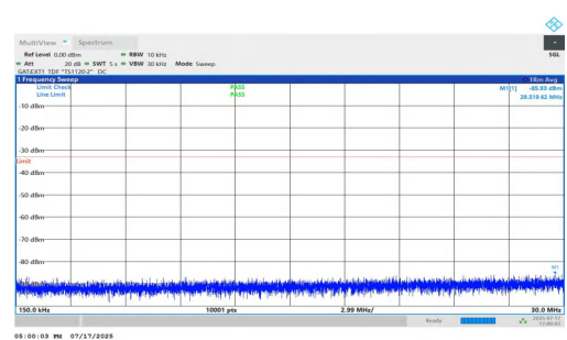
NTNV-n77(3700-3980)-PC1.5-30-80-M-DFT-QPSK-Inner_1RB_Left-0 15-30-PASS
