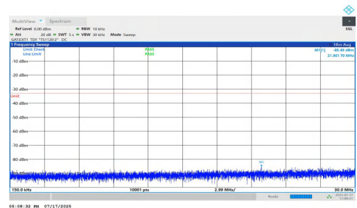
NTNV-n77(3700-3980)-PC1.5-30-80-H-DFT-BPSK-Inner_1RB_Left-0.15-5-30-PASS
