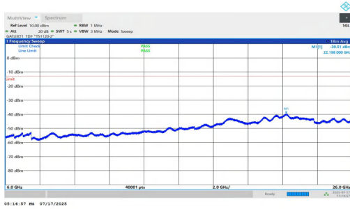
NTNV-n77(3700-3980)-PC1.5-30-80-H-DFT-BPSK-Inner_1RB_Right-6000-26000-PASS
