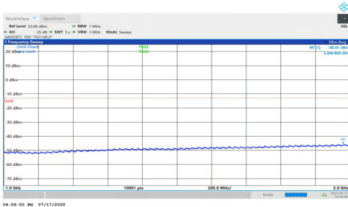
NTNV-n77(3700-3980)-PC1.5-30-80-M-DFT-BPSK-Inner_1RB_Right-1000-3000-PASS
