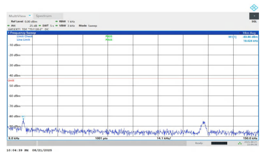
NTNV-n77(3700-3980)-PC1.5-30-80-M-DFT-BPSK-Inner_1RB_Right-0.009-0.15-PASS
