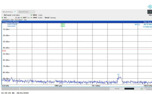
NTNV-n77(3700-3980)-PC1.5-30-80-M-DFT-QPSK-Inner_1RB_Left-0 .009-0.15-PASS
