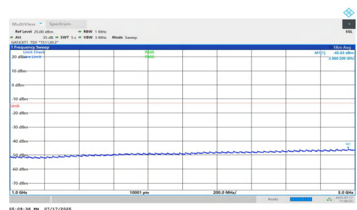
NTNV-n77(3700-3980)-PC1.5-30-80-H-DFT-BPSK-Inner_1RB_Left-1000-3000-PASS
