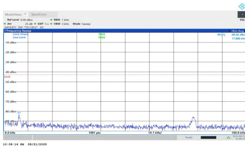
NTNV-n77(3700-3980)-PC1.5-30-80-H-DFT-QPSK-Inner_1RB_Left-0.009-0.15-PASS
