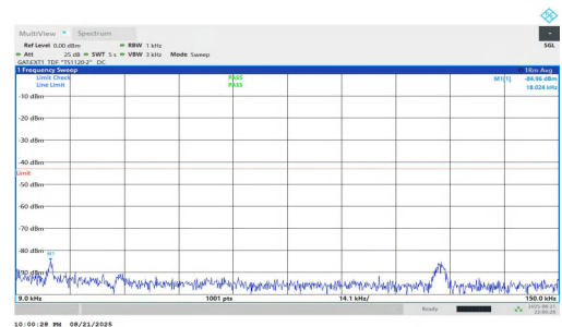
NTNV-n77(3700-3980)-PC1.5-30-70-H-DFT-QPSK-Inner_1RB_Right-0 .009-0.15-PASS
