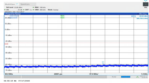
NTNV-n77(3700-3980)-PC1.5-30-80-M-DFT-BPSK-Inner_1RB_Right-3 0-1000-PASS
