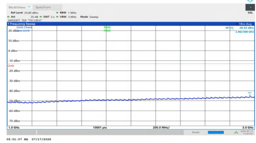
NTNV-n77(3700-3980)-PC1.5-30-80-M-DFT-QPSK-Inner_1RB_Left-10 00-3000-PASS
