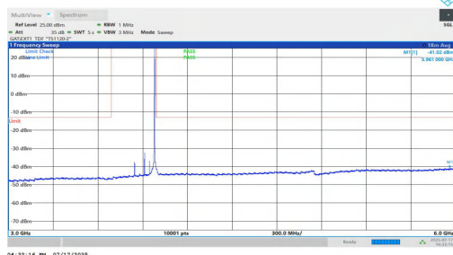
NTNV-n77(3700-3980)-PC1.5-30-70-H-DFT-QPSK-Inner_1RB_Right-3000-6000-PASS
