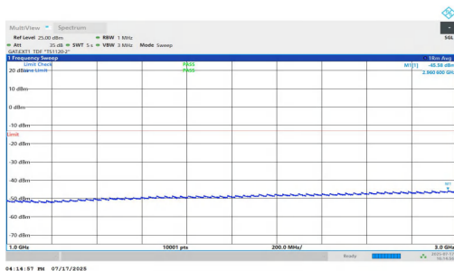
NTNV-n77(3700-3980)-PC1.5-30-70-M-DFT-QPSK-Inner_1RB_Right- 1000-3000-PASS
