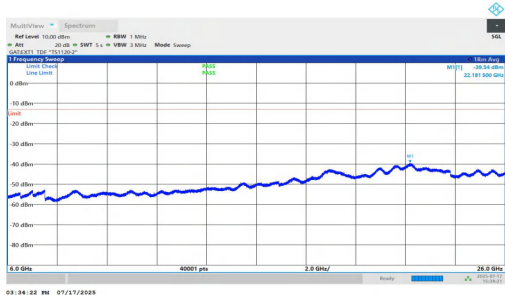
NTNV-n77(3700-3980)-PC1.5-30-60-H-DFT-BPSK-Inner_1RB_Right-6000-26000-PASS
