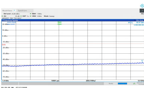
NTNV-n77(3700-3980)-PC1.5-30-60-H-DFT-BPSK-Inner_1RB_Right- 1000-3000-PASS
