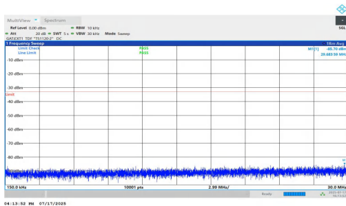
NTNV-n77(3700-3980)-PC1.5-30-70-M-DFT-QPSK-Inner_1RB_Right- 0.15-30-PASS
