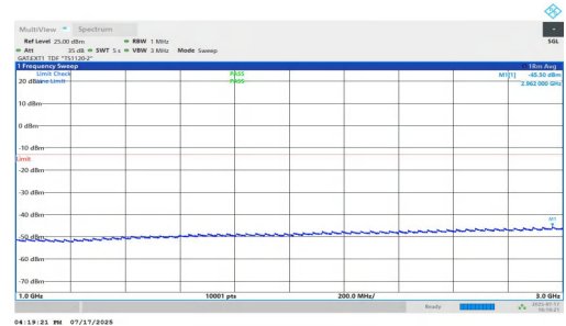
NTNV-n77(3700-3980)-PC1.5-30-70-H-DFT-BPSK-Inner_1RB_Left-1000-3000-PASS
