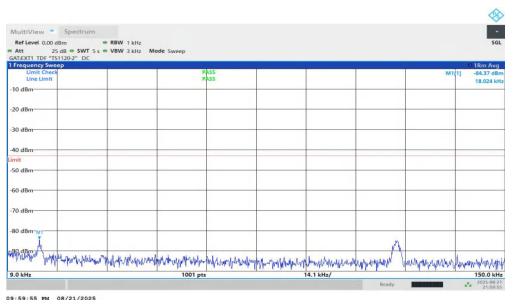
NTNV-n77(3700-3980)-PC1.5-30-70-H-DFT-QPSK-Inner_1RB_Left-0.009-0.15-PASS
