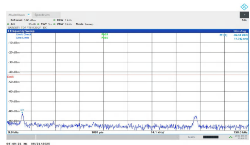
NTNV-n77(3700-3980)-PC1.5-30-60-M-DFT-QPSK-Inner_1RB_Right- 0.009-0.15-PASS
