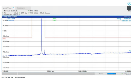
NTNV-n77(3700-3980)-PC1.5-30-70-H-DFT-BPSK-Inner_1RB_Left-3000-6000-PASS
