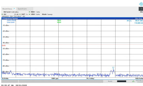
NTNV-n77(3700-3980)-PC1.5-30-70-M-DFT-BPSK-Inner_1RB_Left-0.009-0.15-PASS
