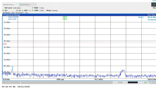
NTV-n77(3700-3980)-PC1.5-30-70-L-DFT-BPSK-Inner_1RB_Left-0.009-0.15-PASS
