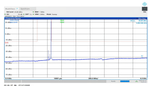
NTNV-n77(3700-3980)-PC1.5-30-60-H-DFT-QPSK-Inner_1RB_Right-3 000-6000-PASS
