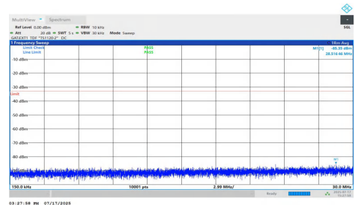
NTNV-n77(3700-3980)-PC1.5-30-60-H-DFT-BPSK-Inner_1RB_Left-0.15-5-30-PASS
