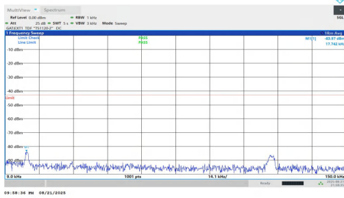
NTNV-n77(3700-3980)-PC1.5-30-70-H-DFT-BPSK-Inner_1RB_Left-0.009-0.15-PASS
