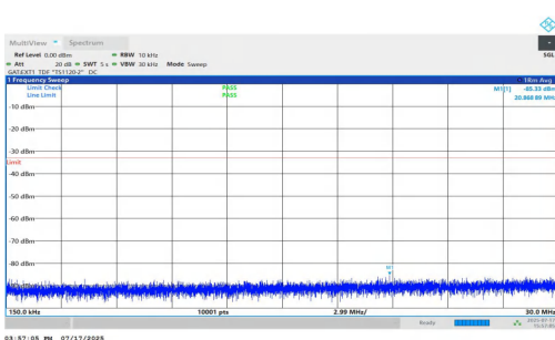
NTNV-n77(3700-3980)-PC1.5-30-70-L-DFT-QPSK-Inner_1RB_Right- 0.15-30-PASS
