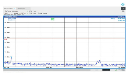
NTNV-n77(3700-3980)-PC1.5-30-70-H-DFT-BPSK-Inner_1RB_Right-0.009-0.15-PASS
