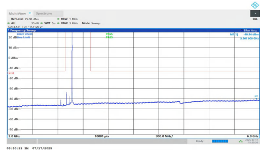
NTNV-n77(3700-3980)-PC1.5-30-70-L-DFT-BPSK-Inner_1RB_Right-3 000-6000-PASS
