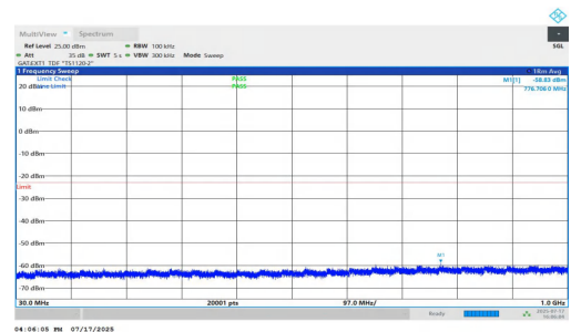
NTNV-n77(3700-3980)-PC1.5-30-70-M-DFT-BPSK-Inner_1RB_Right-3 0-1000-PASS
