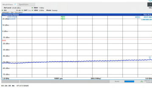
NTNV-n77(3700-3980)-PC1.5-30-60-M-DFT-QPSK-Inner_1RB_Right-1000-3000-PASS
