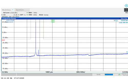
NTNV-n77(3700-3980)-PC1.5-30-70-M-DFT-QPSK-Inner_1RB_Left-3000-6000-PASS
