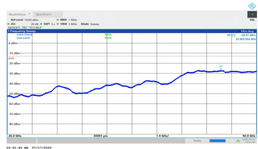
NTNV-n77(3700-3980)-PC1.5-30-70-L-DFT-BPSK-Inner_1RB_Right-2 6000-40000-PASS
