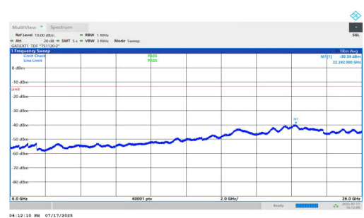
NTNV-n77(3700-3980)-PC1.5-30-70-M-DFT-QPSK-Inner_1RB_Left-6000-26000-PASS
