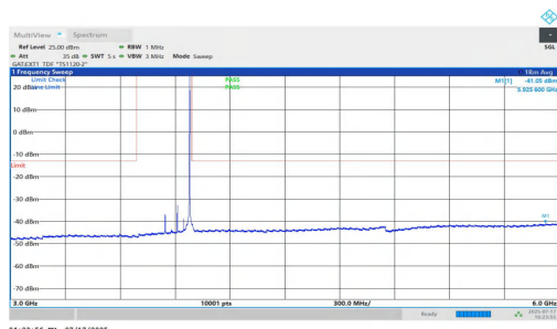
NTNV-n77(3700-3980)-PC1.5-30-70-H-DFT-BPSK-Inner_1RB_Right-3 000-6000-PASS
