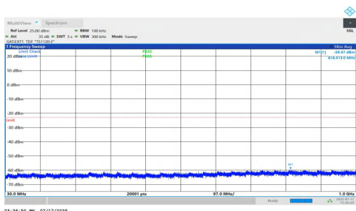
NTNV-n77(3700-3980)-PC1.5-30-60-H-DFT-QPSK-Inner_1RB_Left-30-1000-PASS
