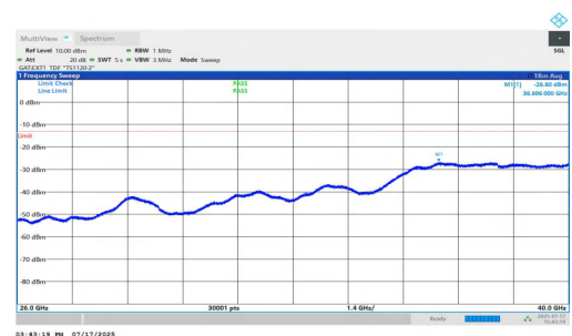
NTNV-n77(3700-3980)-PC1.5-30-60-H-DFT-QPSK-Inner_1RB_Right-2 6000-40000-PASS
