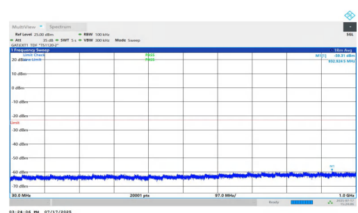
NTNV-n77(3700-3980)-PC1.5-30-60-M-DFT-QPSK-Inner_1RB_Right- 30-1000-PASS
