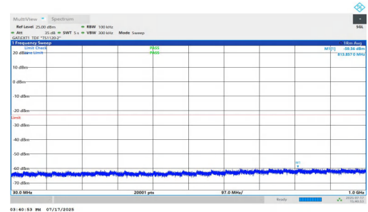
NTNV-n77(3700-3980)-PC1.5-30-60-H-DFT-QPSK-Inner_1RB_Right-3 0-1000-PASS
