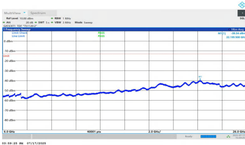
NTNV-n77(3700-3980)-PC1.5-30-70-L-DFT-QPSK-Inner_1RB_Right-6000-26000-PASS
