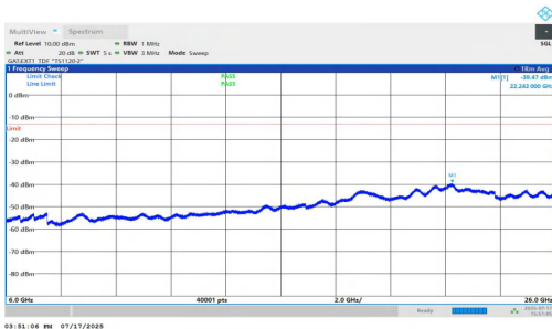
NTNV-n77(3700-3980)-PC1.5-30-70-L-DFT-BPSK-Inner_1RB_Right-6000-26000-PASS
