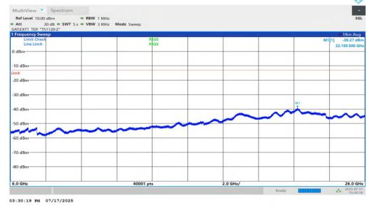
NTNV-n77(3700-3980)-PC1.5-30-60-H-DFT-BPSK-Inner_1RB_Left-60 00-26000-PASS
