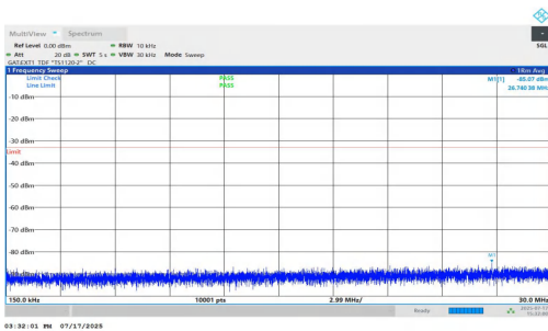
NTNV-n77(3700-3980)-PC1.5-30-60-H-DFT-BPSK-Inner_1RB_Right- 0.15-30-PASS
