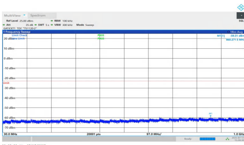
NTNV-n77(3700-3980)-PC1.5-30-60-H-DFT-BPSK-Inner_1RB_Left-30-1000-PASS
