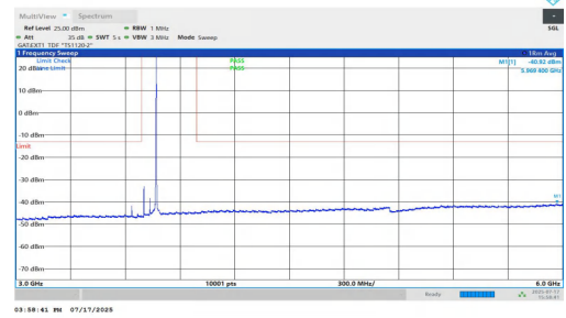
NTNV-n77(3700-3980)-PC1.5-30-70-L-DFT-QPSK-Inner_1RB_Right-3000-6000-PASS
