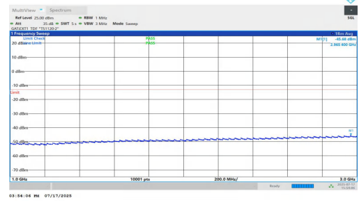
NTNV-n77(3700-3980)-PC1.5-30-70-L-DFT-QPSK-Inner_1RB_Left-10 00-3000-PASS
