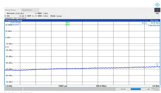
NTNV-n77(3700-3980)-PC1.5-30-60-H-DFT-BPSK-Inner_1RB_Left-1000-3000-PASS
