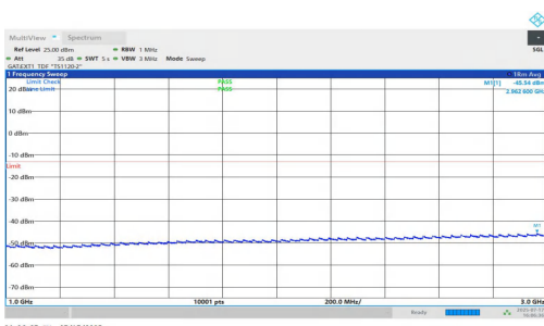
NTNV-n77(3700-3980)-PC1.5-30-70-M-DFT-BPSK-Inner_1RB_Right- 1000-3000-PASS
