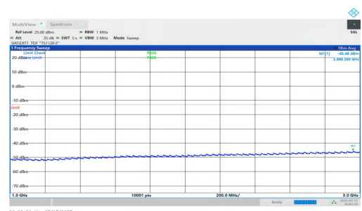
NTNV-n77(3700-3980)-PC1.5-30-70-M-DFT-BPSK-Inner_1RB_Left-1000-3000-PASS
