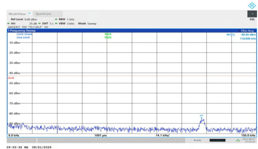
NTV-n77(3700-3980)-PC1.5-30-70-L-DFT-BPSK-Inner_1RB_Right-0.009-0.15-PASS
