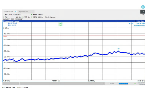
NTNV-n77(3700-3980)-PC1.5-30-60-H-DFT-QPSK-Inner_1RB_Left-6000-26000-PASS
