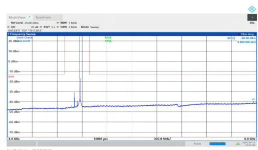
NTNV-n77(3700-3980)-PC1.5-30-70-M-DFT-BPSK-Inner_1RB_Right-3 000-6000-PASS
