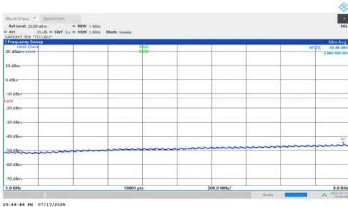
NTNV-n77(3700-3980)-PC1.5-30-70-L-DFT-BPSK-Inner_1RB_Right-1000-3000-PASS
