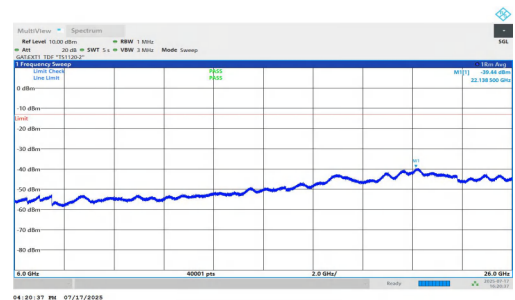
NTNV-n77(3700-3980)-PC1.5-30-70-H-DFT-BPSK-Inner_1RB_Left-6000-26000-PASS
