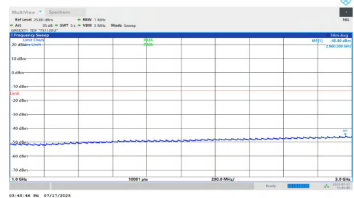
NTV-n77(3700-3980)-PC1.5-30-70-L-DFT-BPSK-Inner_1RB_Left-1000-3000-PASS
