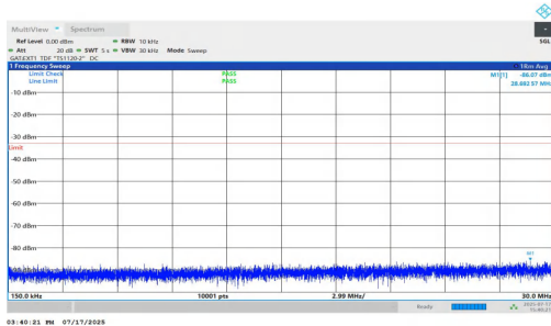
NTNV-n77(3700-3980)-PC1.5-30-60-H-DFT-QPSK-Inner_1RB_Right- 0.15-30-PASS
