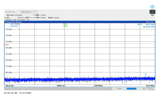
NTNV-n77(3700-3980)-PC1.5-30-70-L-DFT-QPSK-Inner_1RB_Left-0.1 5-30-PASS
