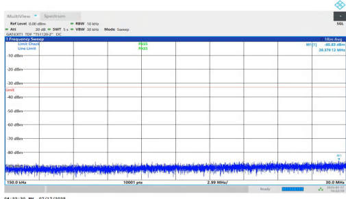
NTNV-n77(3700-3980)-PC1.5-30-70-H-DFT-BPSK-Inner_1RB_Right-0.15-30-PASS
