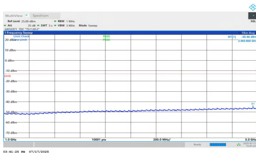
NTNV-n77(3700-3980)-PC1.5-30-60-H-DFT-QPSK-Inner_1RB_Right- 1000-3000-PASS
