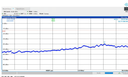
NTNV-n77(3700-3980)-PC1.5-30-60-H-DFT-QPSK-Inner_1RB_Right- 6000-26000-PASS
