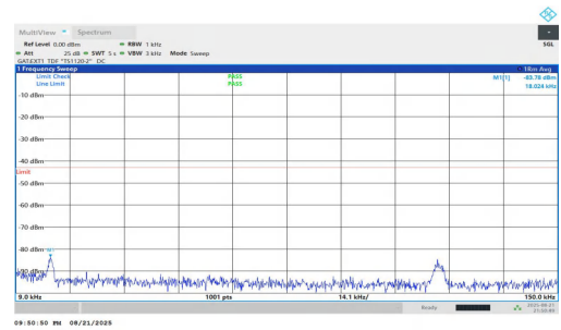
NTNV-n77(3700-3980)-PC1.5-30-60-H-DFT-BPSK-Inner_1RB_Right-0 .009-0.15-PASS
