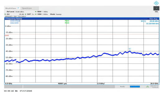
NTNV-n77(3700-3980)-PC1.5-30-70-L-DFT-QPSK-Inner_1RB_Left-60 00-26000-PASS
