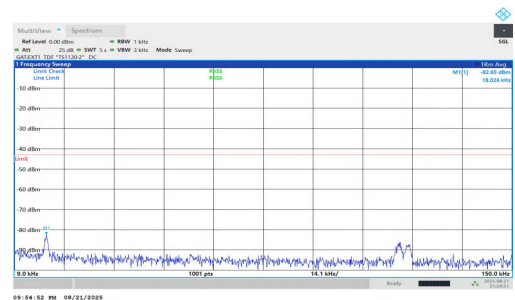
NTNV-n77(3700-3980)-PC1.5-30-70-L-DFT-QPSK-Inner_1RB_Right-0 .009-0.15-PASS
