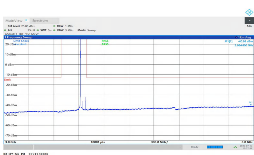
NTNV-n77(3700-3980)-PC1.5-30-60-H-DFT-QPSK-Inner_1RB_Left-3000-6000-PASS
