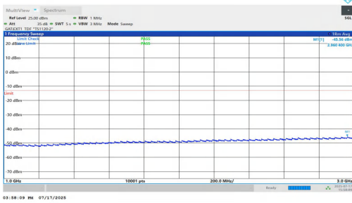
NTNV-n77(3700-3980)-PC1.5-30-70-L-DFT-QPSK-Inner_1RB_Right-1000-3000-PASS
