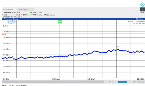
NTNV-n77(3700-3980)-PC1.5-30-70-H-DFT-BPSK-Inner_1RB_Right-6000-26000-PASS
