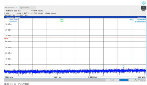
NTNV-n77(3700-3980)-PC1.5-30-70-M-DFT-QPSK-Inner_1RB_Left-0.15-30-PASS
