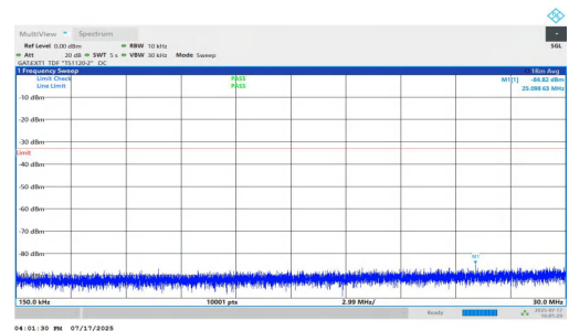
NTNV-n77(3700-3980)-PC1.5-30-70-M-DFT-BPSK-Inner_1RB_Left-0.15-30-PASS
