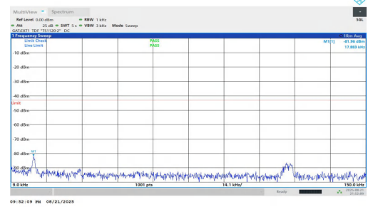
NTNV-n77(3700-3980)-PC1.5-30-60-H-DFT-QPSK-Inner_1RB_Right-0 .009-0.15-PASS
