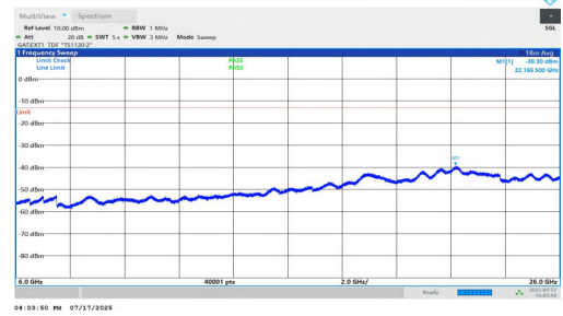
NTNV-n77(3700-3980)-PC1.5-30-70-M-DFT-BPSK-Inner_1RB_Left-60 00-26000-PASS
