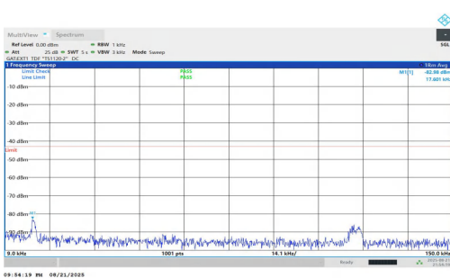
NTNV-n77(3700-3980)-PC1.5-30-70-L-DFT-QPSK-Inner_1RB_Left-0.009-0.15-PASS
