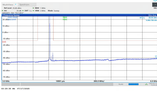
NTNV-n77(3700-3980)-PC1.5-30-60-H-DFT-BPSK-Inner_1RB_Left-3 000-6000-PASS
