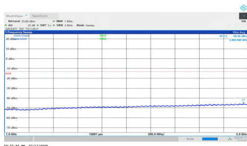
NTNV-n77(3700-3980)-PC1.5-30-60-H-DFT-QPSK-Inner_1RB_Left-1000-3000-PASS
