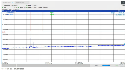
NTV-n77(3700-3980)-PC1.5-30-70-L-DFT-BPSK-Inner_1RB_Left-3000-6000-PASS
