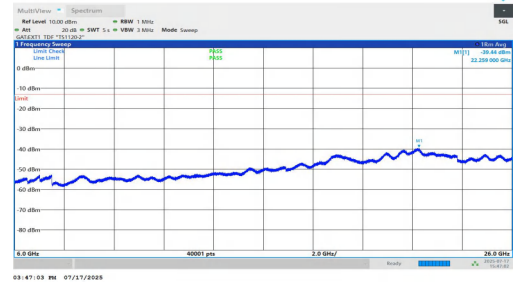
NTV-n77(3700-3980)-PC1.5-30-70-L-DFT-BPSK-Inner_1RB_Left-6000-26000-PASS
