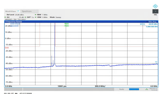
NTNV-n77(3700-3980)-PC1.5-30-60-H-DFT-BPSK-Inner_1RB_Right-3 000-6000-PASS
