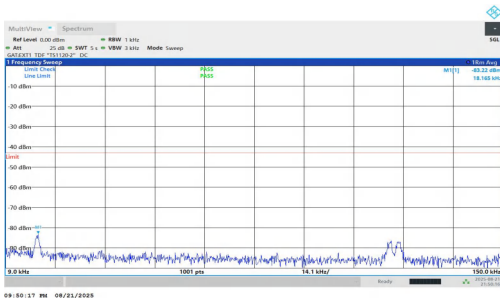
NTNV-n77(3700-3980)-PC1.5-30-60-H-DFT-BPSK-Inner_1RB_Left-0.009-0.15-PASS
