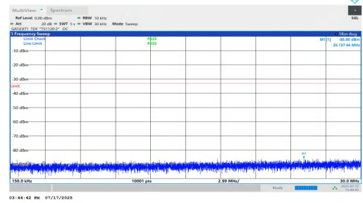
NTV-n77(3700-3980)-PC1.5-30-70-L-DFT-BPSK-Inner_1RB_Left-0.15-30-PASS
