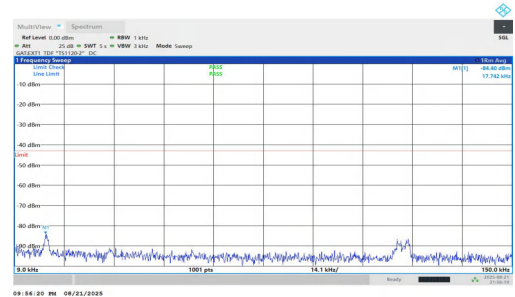
NTNV-n77(3700-3980)-PC1.5-30-70-M-DFT-BPSK-Inner_1RB_Right-0 .009-0.15-PASS
