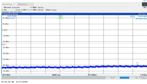
NTNV-n77(3700-3980)-PC1.5-30-60-M-DFT-QPSK-Inner_1RB_Left-3 0-1000-PASS
