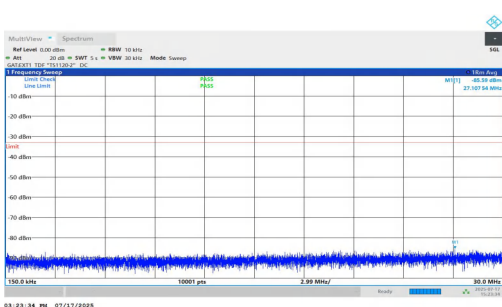
NTNV-n77(3700-3980)-PC1.5-30-60-M-DFT-QPSK-Inner_1RB_Right- 0.15-30-PASS
