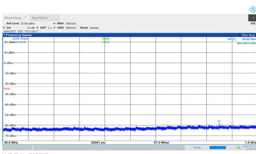
NTNV-n77(3700-3980)-PC1.5-30-70-M-DFT-BPSK-Inner_1RB_Left-30-1000-PASS
