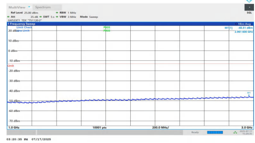
NTNV-n77(3700-3980)-PC1.5-30-60-M-DFT-QPSK-Inner_1RB_Left-10 00-3000-PASS
