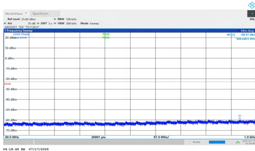
NTNV-n77(3700-3980)-PC1.5-30-70-H-DFT-BPSK-Inner_1RB_Left-3000-1000-PASS
