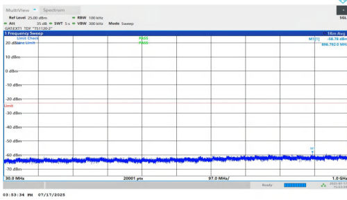
NTNV-n77(3700-3980)-PC1.5-30-70-L-DFT-QPSK-Inner_1RB_Left-3 0-1000-PASS
