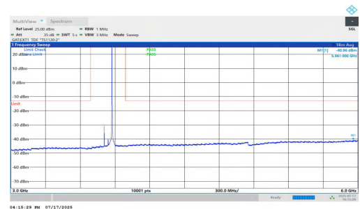
NTNV-n77(3700-3980)-PC1.5-30-70-M-DFT-QPSK-Inner_1RB_Right- 3000-6000-PASS
