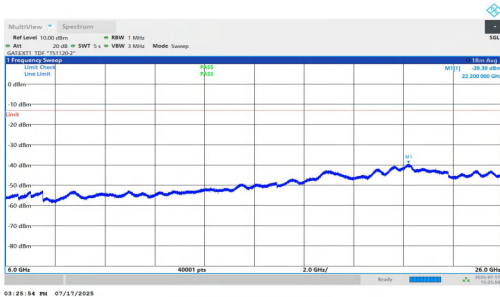
NTNV-n77(3700-3980)-PC1.5-30-60-M-DFT-QPSK-Inner_1RB_Right-6000-26000-PASS
