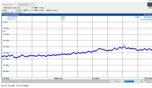
NTNV-n77(3700-3980)-PC1.5-30-70-M-DFT-BPSK-Inner_1RB_Right-6000-26000-PASS
