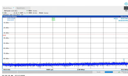
NTNV-n77(3700-3980)-PC1.5-30-60-H-DFT-QPSK-Inner_1RB_Left-0.15-30-PASS
