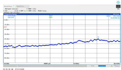
NTNV-n77(3700-3980)-PC1.5-30-60-M-DFT-QPSK-Inner_1RB_Left-60 00-26000-PASS
