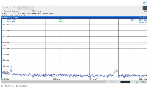
NTNV-n77(3700-3980)-PC1.5-30-70-M-DFT-QPSK-Inner_1RB_Left-0.009-0.15-PASS
