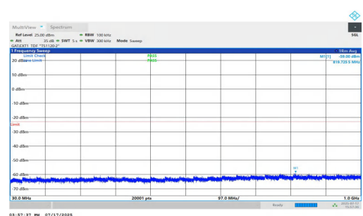
NTNV-n77(3700-3980)-PC1.5-30-70-L-DFT-QPSK-Inner_1RB_Right-3 0-1000-PASS
