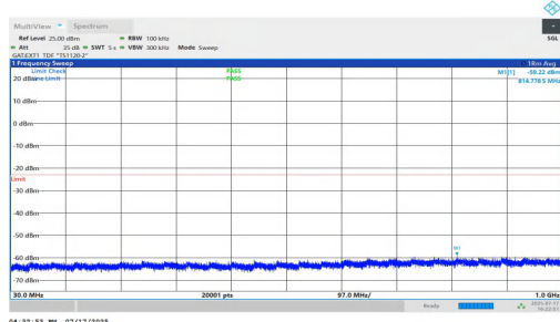
NTNV-n77(3700-3980)-PC1.5-30-70-H-DFT-BPSK-Inner_1RB_Right-3 0-1000-PASS
