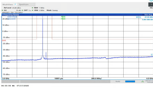
NTNV-n77(3700-3980)-PC1.5-30-70-M-DFT-BPSK-Inner_1RB_Left-3 000-6000-PASS
