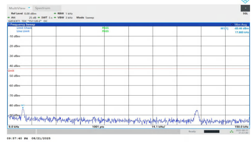
NTNV-n77(3700-3980)-PC1.5-30-70-M-DFT-QPSK-Inner_1RB_Right- 0.009-0.15-PASS
