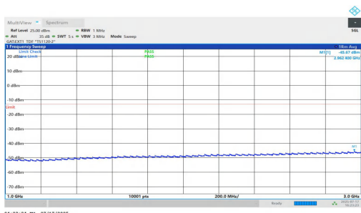
NTNV-n77(3700-3980)-PC1.5-30-70-H-DFT-BPSK-Inner_1RB_Right-1000-3000-PASS
