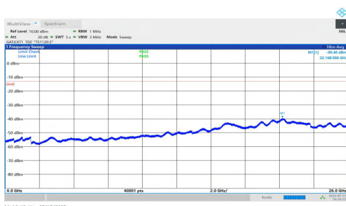
NTNV-n77(3700-3980)-PC1.5-30-70-M-DFT-QPSK-Inner_1RB_Right- 6000-26000-PASS
