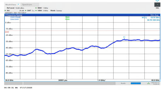
NTNV-n77(3700-3980)-PC1.5-30-70-M-DFT-BPSK-Inner_1RB_Right-26000-40000-PASS
