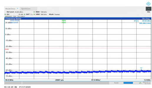
NTNV-n77(3700-3980)-PC1.5-30-70-M-DFT-QPSK-Inner_1RB_Right- 30-1000-PASS
