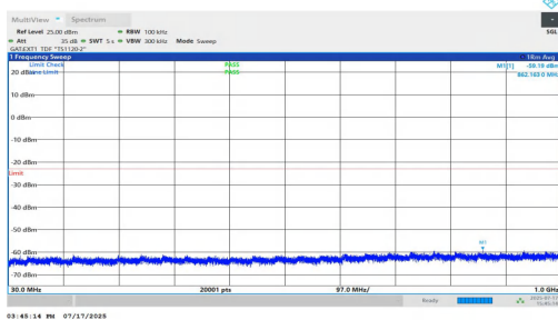
NTV-n77(3700-3980)-PC1.5-30-70-L-DFT-BPSK-Inner_1RB_Left-30-1000-PASS
