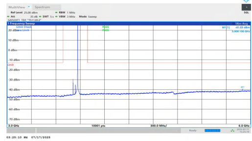
NTNV-n77(3700-3980)-PC1.5-30-60-M-DFT-QPSK-Inner_1RB_Right-3000-6000-PASS
