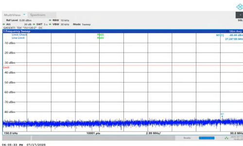
NTNV-n77(3700-3980)-PC1.5-30-70-M-DFT-BPSK-Inner_1RB_Right- 0.15-30-PASS
