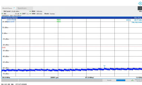
NTNV-n77(3700-3980)-PC1.5-30-70-M-DFT-QPSK-Inner_1RB_Left-30-1000-PASS
