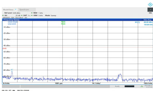
NTNV-n77(3700-3980)-PC1.5-30-60-H-DFT-QPSK-Inner_1RB_Left-0.009-0.15-PASS
