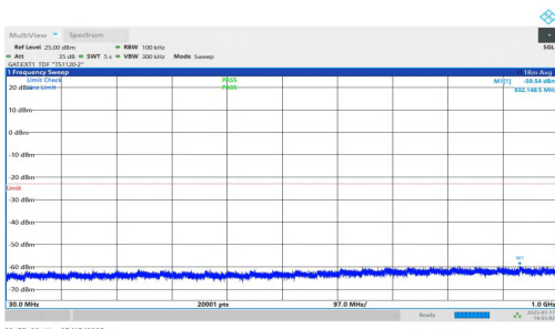
NTNV-n77(3700-3980)-PC1.5-30-60-L-DFT-BPSK-Inner_1RB_Left-30-1000-PASS
