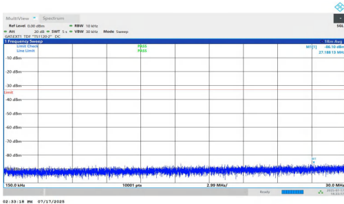
NTNV-n77(3700-3980)-PC1.5-30-50-M-DFT-QPSK-Inner_1RB_Right- 0.15-30-PASS
