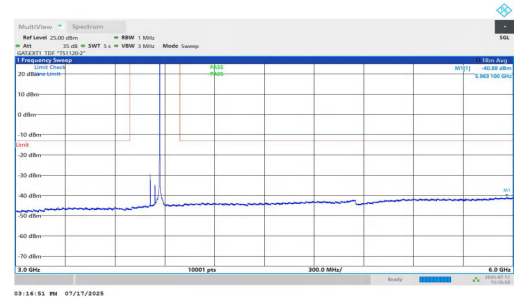
NTNV-n77(3700-3980)-PC1.5-30-60-M-DFT-BPSK-Inner_1RB_Right-3 000-6000-PASS
