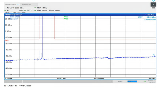
NTNV-n77(3700-3980)-PC1.5-30-50-L-DFT-QPSK-Inner_1RB_Right-3000-6000-PASS
