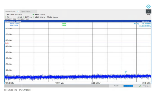
NTNV-n77(3700-3980)-PC1.5-30-60-M-DFT-QPSK-Inner_1RB_Left-0 15-30-PASS
