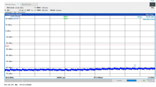
NTNV-n77(3700-3980)-PC1.5-30-60-M-DFT-BPSK-Inner_1RB_Right-3 0-1000-PASS
