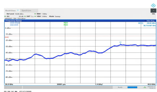
NTNV-n77(3700-3980)-PC1.5-30-50-M-DFT-QPSK-Inner_1RB_Right- 26000-40000-PASS
