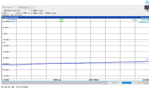
NTNV-n77(3700-3980)-PC1.5-30-50-H-DFT-BPSK-Inner_1RB_Right-1000-3000-PASS
