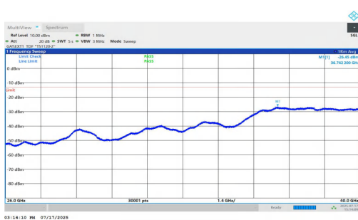
NTNV-n77(3700-3980)-PC1.5-30-60-M-DFT-BPSK-Inner_1RB_Left-26000-40000-PASS
