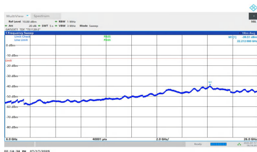
NTVN-n77(3700-3980)-PC1.5-30-50-L-DFT-QPSK-Inner_1RB_Left-60 00-26000-PASS
