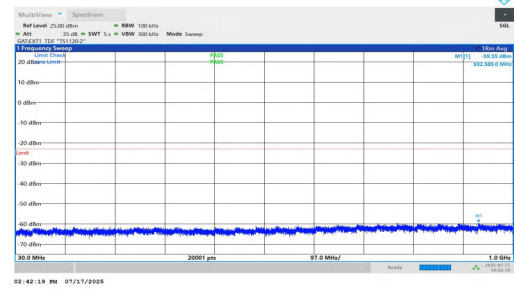
NTNV-n77(3700-3980)-PC1.5-30-50-H-DFT-BPSK-Inner_1RB_Right-3 0-1000-PASS
