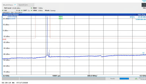
NTNV-n77(3700-3980)-PC1.5-30-50-H-DFT-BPSK-Inner_1RB_Left-3000-6000-PASS
