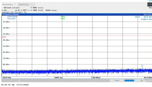
NTNV-n77(3700-3980)-PC1.5-30-50-H-DFT-BPSK-Inner_1RB_Right-0.15-30-PASS
