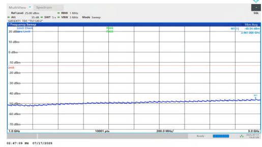
NTNV-n77(3700-3980)-PC1.5-30-50-H-DFT-QPSK-Inner_1RB_Left-10 00-3000-PASS
