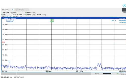
NTNV-n77(3700-3980)-PC1.5-30-60-M-DFT-QPSK-Inner_1RB_Left-0 .009-0.15-PASS
