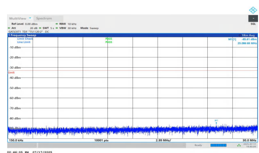
NTNV-n77(3700-3980)-PC1.5-30-50-H-DFT-QPSK-Inner_1RB_Left-0.15-30-PASS
