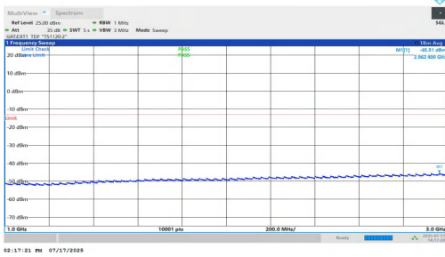
NTNV-n77(3700-3980)-PC1.5-30-50-L-DFT-QPSK-Inner_1RB_Right-1000-3000-PASS
