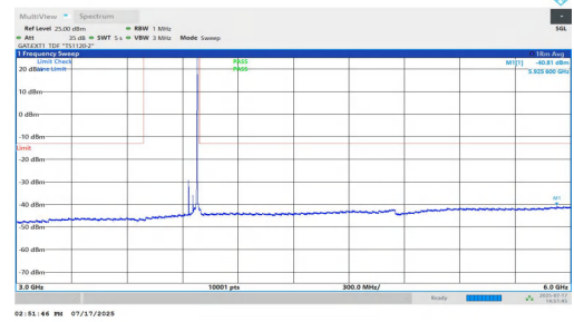
NTNV-n77(3700-3980)-PC1.5-30-50-H-DFT-QPSK-Inner_1RB_Right-3000-6000-PASS
