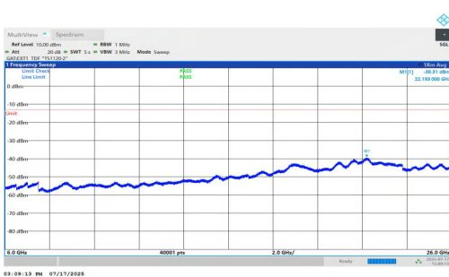
NTNV-n77(3700-3980)-PC1.5-30-60-L-DFT-QPSK-Inner_1RB_Right- 6000-26000-PASS
