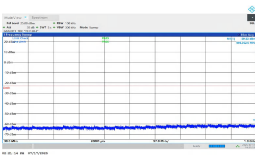
NTNV-n77(3700-3980)-PC1.5-30-50-M-DFT-BPSK-Inner_1RB_Left-30-1000-PASS
