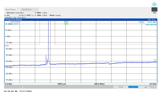
NTNV-n77(3700-3980)-PC1.5-30-50-M-DFT-QPSK-Inner_1RB_Right- 3000-6000-PASS
