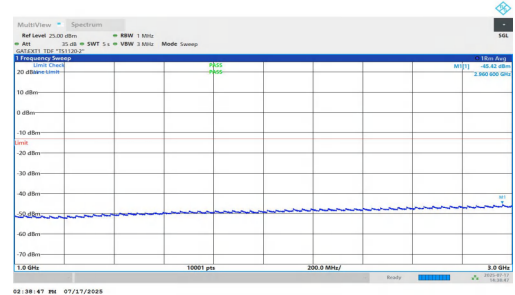
NTNV-n77(3700-3980)-PC1.5-30-50-H-DFT-BPSK-Inner_1RB_Left-1000-3000-PASS
