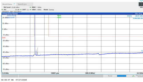
NTNV-n77(3700-3980)-PC1.5-30-60-L-DFT-BPSK-Inner_1RB_Left-30 00-6000-PASS
