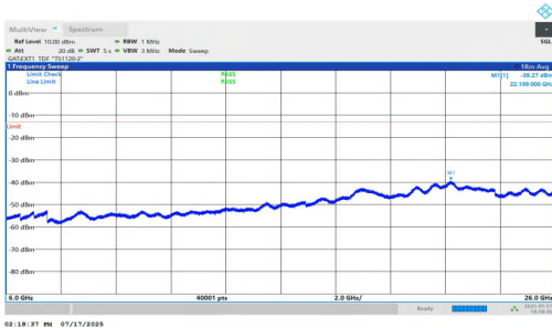
NTNV-n77(3700-3980)-PC1.5-30-50-L-DFT-QPSK-Inner_1RB_Right-6000-26000-PASS
