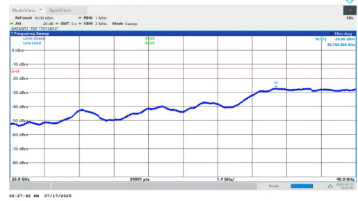
NTNV-n77(3700-3980)-PC1.5-30-50-M-DFT-BPSK-Inner_1RB_Right-26000-40000-PASS
