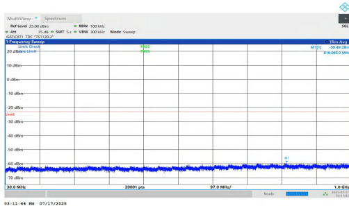
NTNV-n77(3700-3980)-PC1.5-30-60-M-DFT-BPSK-Inner_1RB_Left-30-1000-PASS
