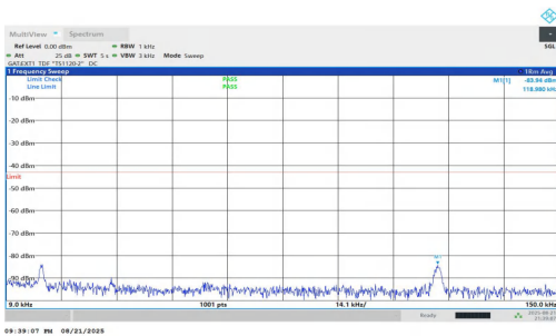
NTNV-n77(3700-3980)-PC1.5-30-50-M-DFT-BPSK-Inner_1RB_Left-0.009-0.15-PASS
