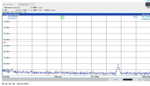
NTNV-n77(3700-3980)-PC1.5-30-50-H-DFT-BPSK-Inner_1RB_Left-0.009-0.15-PASS
