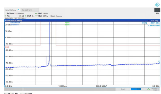
NTNV-n77(3700-3980)-PC1.5-30-50-M-DFT-BPSK-Inner_1RB_Right-3 000-6000-PASS
