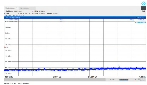
NTNV-n77(3700-3980)-PC1.5-30-50-M-DFT-BPSK-Inner_1RB_Right-3 0-1000-PASS
