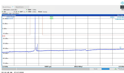
NTNV-n77(3700-3980)-PC1.5-30-60-M-DFT-BPSK-Inner_1RB_Left-3000-6000-PASS
