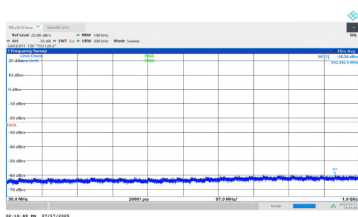
NTVN-n77(3700-3980)-PC1.5-30-50-L-DFT-QPSK-Inner_1RB_Right-3 0-1000-PASS
