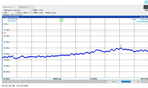
NTVN-n77(3700-3980)-PC1.5-30-60-L-DFT-BPSK-Inner_1RB_Right-6000-26000-PASS
