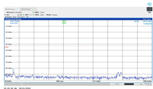
NTNV-n77(3700-3980)-PC1.5-30-50-H-DFT-QPSK-Inner_1RB_Right-0 .009-0.15-PASS
