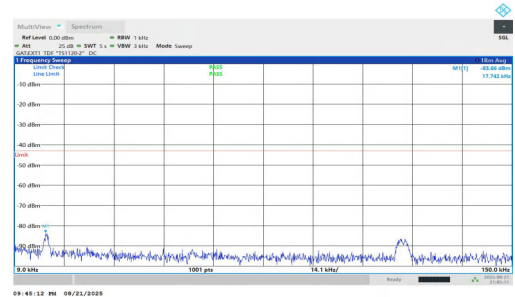
NTNV-n77(3700-3980)-PC1.5-30-60-L-DFT-BPSK-Inner_1RB_Right-0. 009-0.15-PASS
