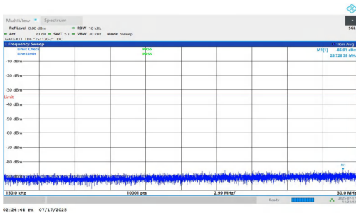
NTNV-n77(3700-3980)-PC1.5-30-50-M-DFT-BPSK-Inner_1RB_Right- 0.15-30-PASS
