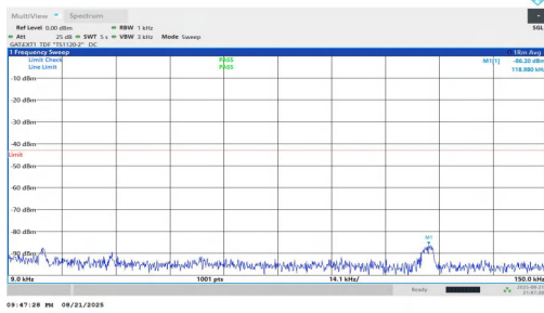
NTNV-n77(3700-3980)-PC1.5-30-60-M-DFT-BPSK-Inner_1RB_Left-0.009-0.15-PASS
