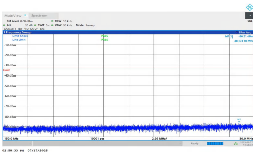
NTNV-n77(3700-3980)-PC1.5-30-60-L-DFT-BPSK-Inner_1RB_Right- 0.15-30-PASS
