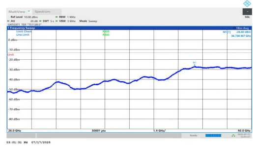
NTVN-n77(3700-3980)-PC1.5-30-60-L-DFT-BPSK-Inner_1RB_Right-26000-40000-PASS
