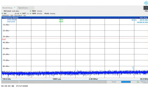
NTNV-n77(3700-3980)-PC1.5-30-60-L-DFT-QPSK-Inner_1RB_Right- 0.15-30-PASS
