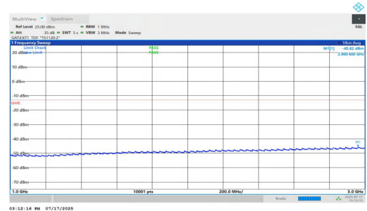
NTNV-n77(3700-3980)-PC1.5-30-60-M-DFT-BPSK-Inner_1RB_Left-1000-3000-PASS
