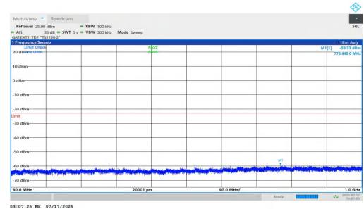
NTNV-n77(3700-3980)-PC1.5-30-60-L-DFT-QPSK-Inner_1RB_Right-3 0-1000-PASS
