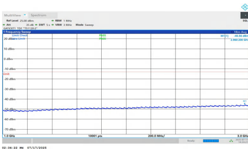
NTNV-n77(3700-3980)-PC1.5-30-50-M-DFT-QPSK-Inner_1RB_Right- 1000-3000-PASS
