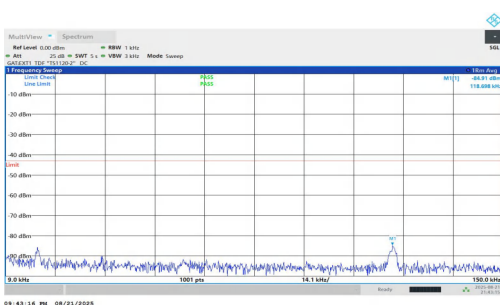
NTNV-n77(3700-3980)-PC1.5-30-50-H-DFT-QPSK-Inner_1RB_Left-0.009-0.15-PASS
