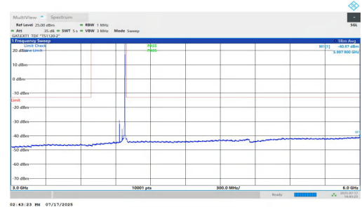
NTNV-n77(3700-3980)-PC1.5-30-50-H-DFT-BPSK-Inner_1RB_Right-3 000-6000-PASS
