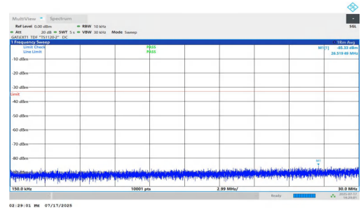
NTNV-n77(3700-3980)-PC1.5-30-50-M-DFT-QPSK-Inner_1RB_Left-0.15-30-PASS
