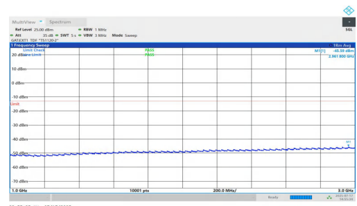
NTNV-n77(3700-3980)-PC1.5-30-60-L-DFT-BPSK-Inner_1RB_Left-1000-3000-PASS
