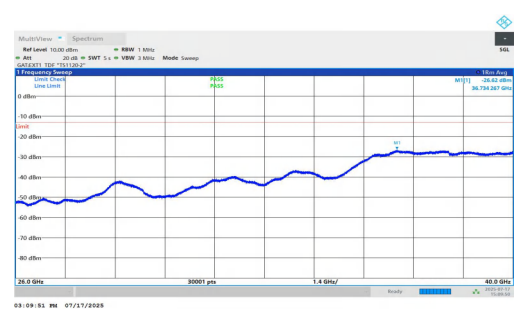
NTNV-n77(3700-3980)-PC1.5-30-60-L-DFT-QPSK-Inner_1RB_Right-2 6000-40000-PASS
