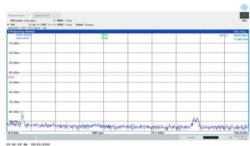
NTNV-n77(3700-3980)-PC1.5-30-50-H-DFT-BPSK-Inner_1RB_Right-0.009-0.15-PASS
