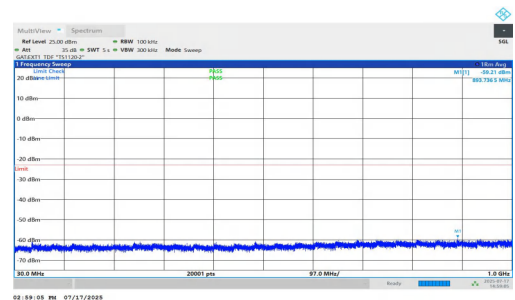
NTNV-n77(3700-3980)-PC1.5-30-60-L-DFT-BPSK-Inner_1RB_Right-3 0-1000-PASS
