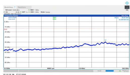
NTNV-n77(3700-3980)-PC1.5-30-60-M-DFT-BPSK-Inner_1RB_Left-6000-26000-PASS
