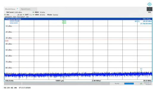
NTNV-n77(3700-3980)-PC1.5-30-50-M-DFT-BPSK-Inner_1RB_Left-0.15-30-PASS
