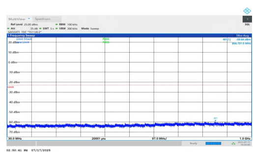
NTNV-n77(3700-3980)-PC1.5-30-50-H-DFT-QPSK-Inner_1RB_Right-3 0-1000-PASS
