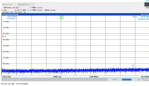
NTNV-n77(3700-3980)-PC1.5-30-60-M-DFT-BPSK-Inner_1RB_Right-0.15-30-PASS
