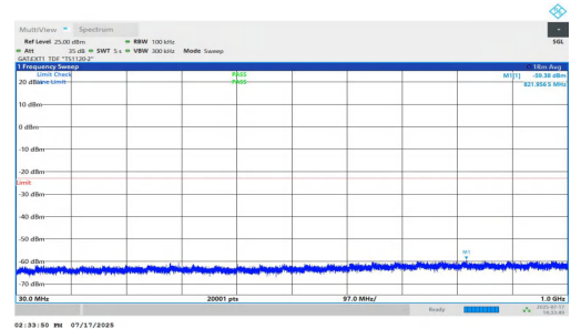
NTNV-n77(3700-3980)-PC1.5-30-50-M-DFT-QPSK-Inner_1RB_Right- 30-1000-PASS
