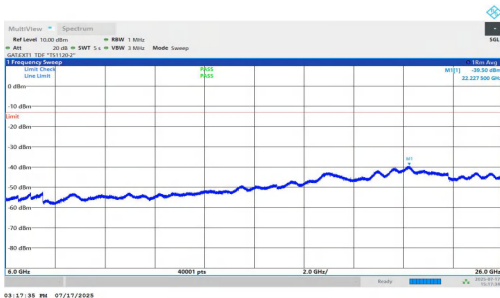
NTNV-n77(3700-3980)-PC1.5-30-60-M-DFT-BPSK-Inner_1RB_Right-6000-26000-PASS
