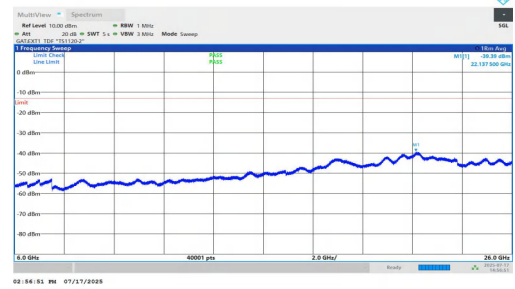
NTNV-n77(3700-3980)-PC1.5-30-60-L-DFT-BPSK-Inner_1RB_Left-60 00-26000-PASS
