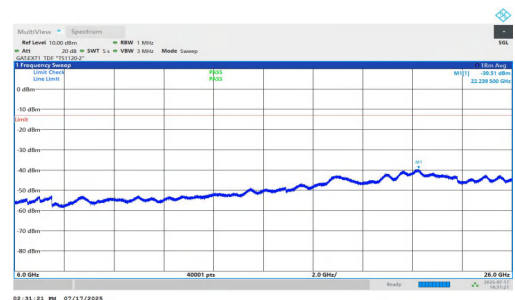
NTNV-n77(3700-3980)-PC1.5-30-50-M-DFT-QPSK-Inner_1RB_Left-6000-26000-PASS
