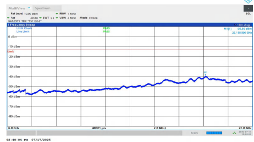
NTNV-n77(3700-3980)-PC1.5-30-50-H-DFT-BPSK-Inner_1RB_Left-6000-26000-PASS
