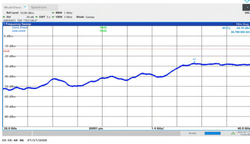
NTNV-n77(3700-3980)-PC1.5-30-60-L-DFT-QPSK-Inner_1RB_Left-2 6000-40000-PASS
