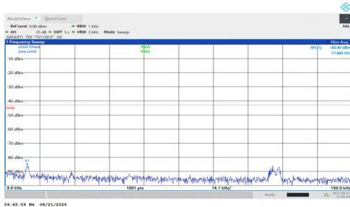
NTVN-n77(3700-3980)-PC1.5-30-60-L-DFT-QPSK-Inner_1RB_Left-0.009-0.15-PASS
