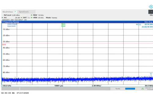
NTNV-n77(3700-3980)-PC1.5-30-50-H-DFT-QPSK-Inner_1RB_Right- 0.15-30-PASS
