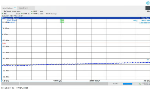
NTNV-n77(3700-3980)-PC1.5-30-60-M-DFT-BPSK-Inner_1RB_Right-1000-3000-PASS
