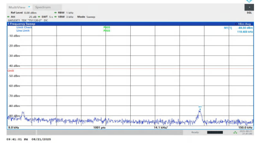
NTNV-n77(3700-3980)-PC1.5-30-50-M-DFT-QPSK-Inner_1RB_Right- 0.009-0.15-PASS
