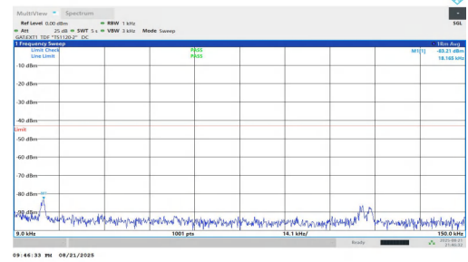
NTNV-n77(3700-3980)-PC1.5-30-60-L-DFT-QPSK-Inner_1RB_Right-0 .009-0.15-PASS
