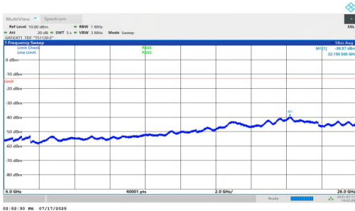
NTNV-n77(3700-3980)-PC1.5-30-50-H-DFT-QPSK-Inner_1RB_Right-6000-26000-PASS
