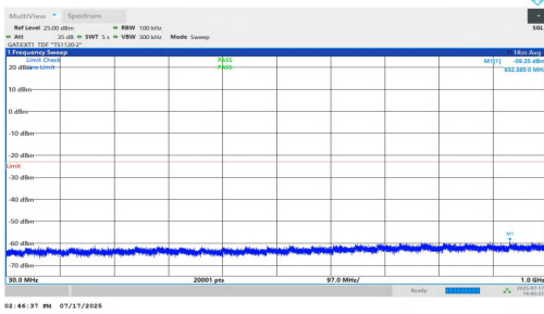
NTNV-n77(3700-3980)-PC1.5-30-50-H-DFT-QPSK-Inner_1RB_Left-3 0-1000-PASS
