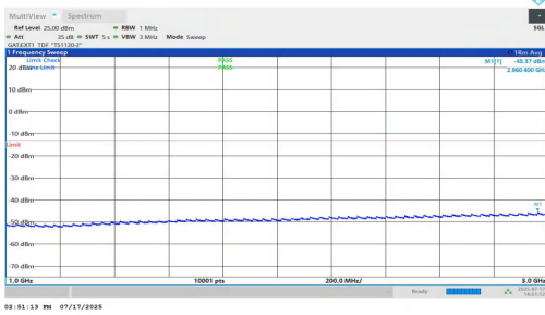
NTNV-n77(3700-3980)-PC1.5-30-50-H-DFT-QPSK-Inner_1RB_Right-1000-3000-PASS
