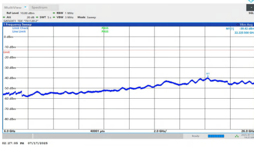
NTNV-n77(3700-3980)-PC1.5-30-50-M-DFT-BPSK-Inner_1RB_Right-6000-26000-PASS
