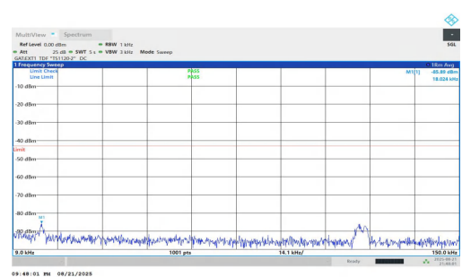
NTNV-n77(3700-3980)-PC1.5-30-60-M-DFT-BPSK-Inner_1RB_Right-0.009-0.15-PASS
