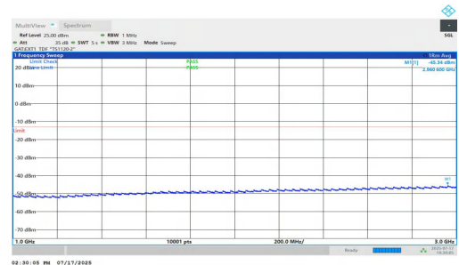
NTNV-n77(3700-3980)-PC1.5-30-50-M-DFT-QPSK-Inner_1RB_Left-1000-3000-PASS
