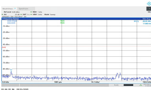
NTNV-n77(3700-3980)-PC1.5-30-60-L-DFT-BPSK-Inner_1RB_Left-0.009-0.15-PASS
