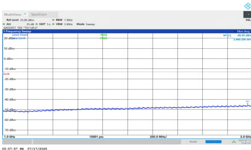
NTNV-n77(3700-3980)-PC1.5-30-60-L-DFT-QPSK-Inner_1RB_Right- 1000-3000-PASS
