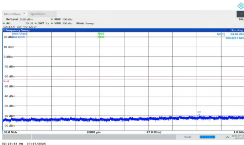
NTNV-n77(3700-3980)-PC1.5-30-50-M-DFT-QPSK-Inner_1RB_Left-30-1000-PASS
