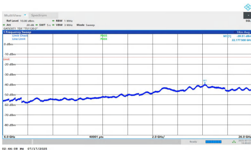
NTNV-n77(3700-3980)-PC1.5-30-50-H-DFT-BPSK-Inner_1RB_Right-6000-26000-PASS
