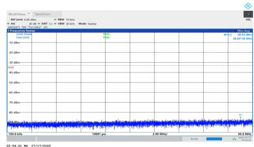
NTNV-n77(3700-3980)-PC1.5-30-60-L-DFT-BPSK-Inner_1RB_Left-0.15-5-30-PASS
