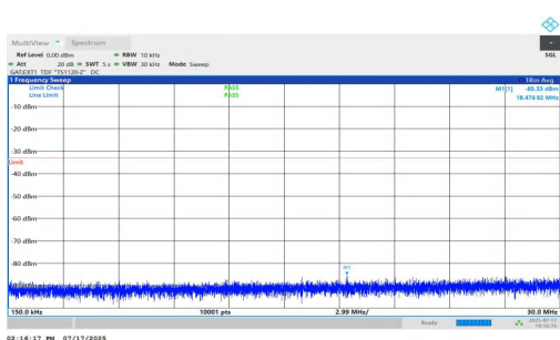
NTVN-n77(3700-3980)-PC1.5-30-50-L-DFT-QPSK-Inner_1RB_Right- 0.15-30-PASS
