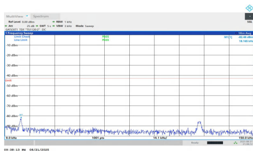
NTVN-n77(3700-3980)-PC1.5-30-50-L-DFT-QPSK-Inner_1RB_Right-0 .009-0.15-PASS
