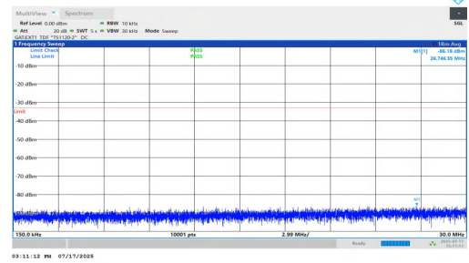
NTNV-n77(3700-3980)-PC1.5-30-60-M-DFT-BPSK-Inner_1RB_Left-0.15-30-PASS
