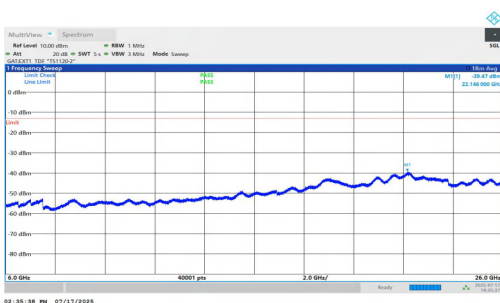
NTNV-n77(3700-3980)-PC1.5-30-50-M-DFT-QPSK-Inner_1RB_Right- 6000-26000-PASS
