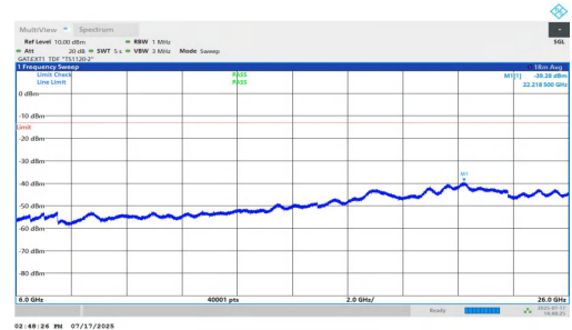
NTNV-n77(3700-3980)-PC1.5-30-50-H-DFT-QPSK-Inner_1RB_Left-60 00-26000-PASS
