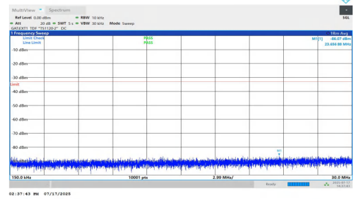
NTNV-n77(3700-3980)-PC1.5-30-50-H-DFT-BPSK-Inner_1RB_Left-0.15-30-PASS
