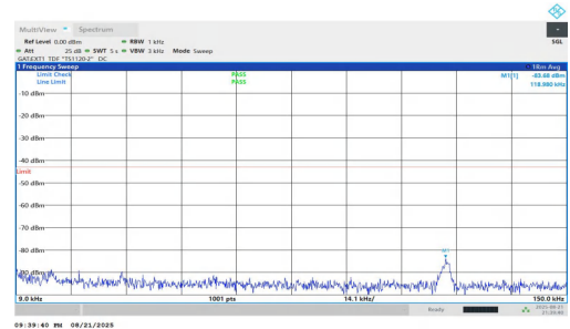
NTNV-n77(3700-3980)-PC1.5-30-50-M-DFT-BPSK-Inner_1RB_Right-0 .009-0.15-PASS
