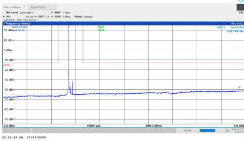
NTNV-n77(3700-3980)-PC1.5-30-50-M-DFT-BPSK-Inner_1RB_Left-3 000-6000-PASS
