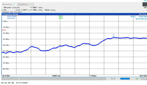
NTNV-n77(3700-3980)-PC1.5-30-50-M-DFT-QPSK-Inner_1RB_Left-2 6000-40000-PASS
