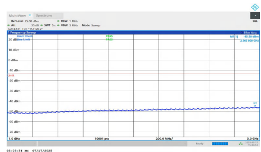
NTVN-n77(3700-3980)-PC1.5-30-60-L-DFT-QPSK-Inner_1RB_Left-1000-3000-PASS
