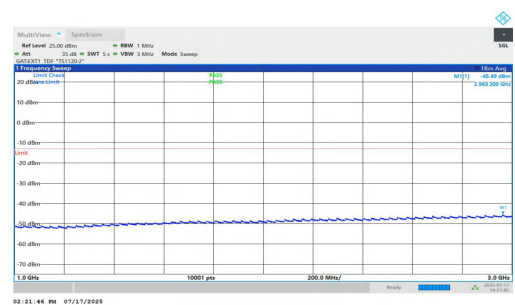
NTNV-n77(3700-3980)-PC1.5-30-50-M-DFT-BPSK-Inner_1RB_Left-1000-3000-PASS
