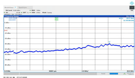
NTV-n77(3700-3980)-PC1.5-30-50-L-DFT-BPSK-Inner_1RB_Left-6000-26000-PASS
