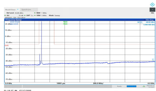
NTNV-n77(3700-3980)-PC1.5-30-40-L-DFT-BPSK-Inner_1RB_Right-3 000-6000-PASS
