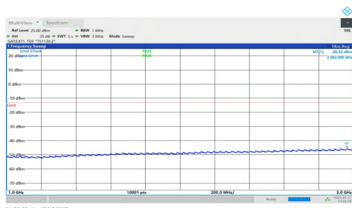
NTNV-n77(3700-3980)-PC1.5-30-40-H-DFT-QPSK-Inner_1RB_Left-1000-3000-PASS
