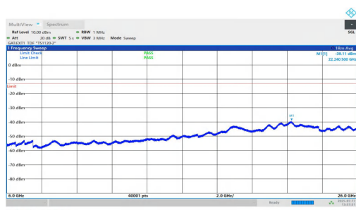
NTNV-n77(3700-3980)-PC1.5-30-40-H-DFT-QPSK-Inner_1RB_Left-6000-26000-PASS
