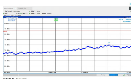
NTNV-n77(3700-3980)-PC1.5-30-40-M-DFT-QPSK-Inner_1RB_Left-60 00-26000-PASS
