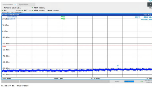
NTNV-n77(3700-3980)-PC1.5-30-30-H-DFT-QPSK-Inner_1RB_Left-3 0-1000-PASS
