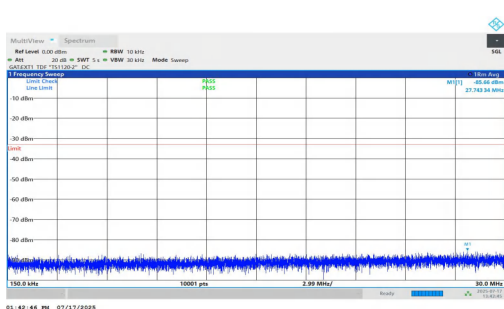
NTNV-n77(3700-3980)-PC1.5-30-40-M-DFT-QPSK-Inner_1RB_Right- 0.15-30-PASS
