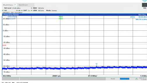
NTNV-n77(3700-3980)-PC1.5-30-40-M-DFT-QPSK-Inner_1RB_Left-3 0-1000-PASS
