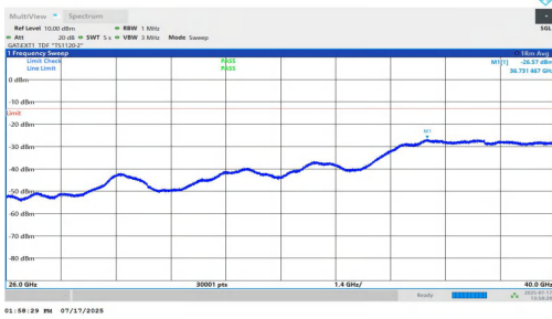
NTNV-n77(3700-3980)-PC1.5-30-40-H-DFT-QPSK-Inner_1RB_Left-2 6000-40000-PASS
