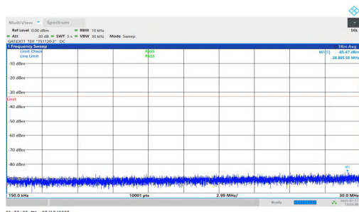
NTNV-n77(3700-3980)-PC1.5-30-40-H-DFT-QPSK-Inner_1RB_Left-0.15-30-PASS
