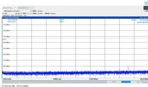
NTVN-n77(3700-3980)-PC1.5-30-40-L-DFT-QPSK-Inner_1RB_Right- 0.15-30-PASS
