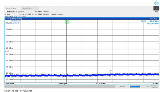
NTNV-n77(3700-3980)-PC1.5-30-40-H-DFT-QPSK-Inner_1RB_Right-3 0-1000-PASS
