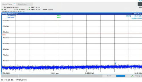
NTNV-n77(3700-3980)-PC1.5-30-40-M-DFT-BPSK-Inner_1RB_Right-0.15-30-PASS
