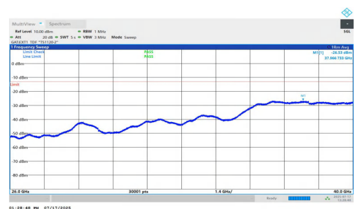
NTVN-n77(3700-3980)-PC1.5-30-40-L-DFT-QPSK-Inner_1RB_Right-2 6000-40000-PASS
