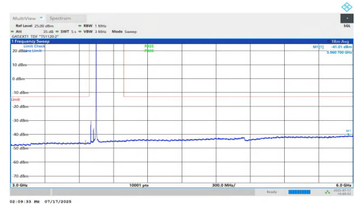
NTNV-n77(3700-3980)-PC1.5-30-50-L-DFT-BPSK-Inner_1RB_Right-3 000-6000-PASS
