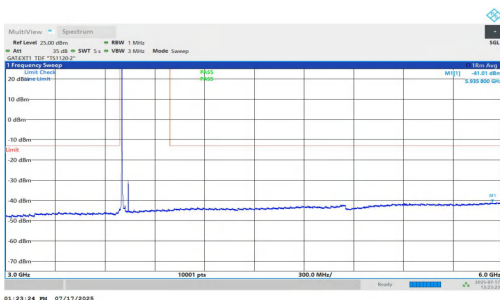
NTNV-n77(3700-3980)-PC1.5-30-40-L-DFT-QPSK-Inner_1RB_Left-30000-60000-PASS
