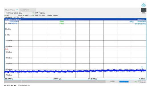
NTNV-n77(3700-3980)-PC1.5-30-30-H-DFT-QPSK-Inner_1RB_Right-3 0-1000-PASS
