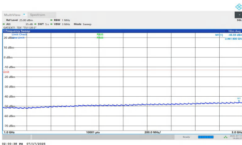
NTNV-n77(3700-3980)-PC1.5-30-40-H-DFT-QPSK-Inner_1RB_Right-1000-3000-PASS
