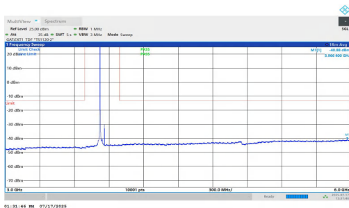
NTNV-n77(3700-3980)-PC1.5-30-40-M-DFT-BPSK-Inner_1RB_Left-3000-6000-PASS
