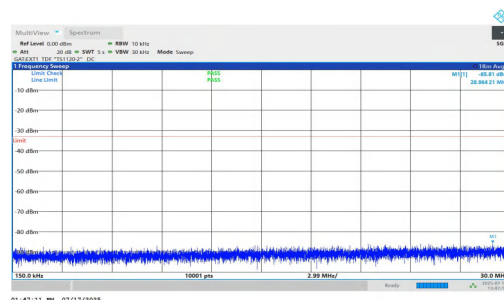
NTNV-n77(3700-3980)-PC1.5-30-40-H-DFT-BPSK-Inner_1RB_Left-0.15-5-30-PASS
