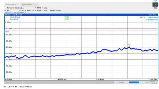
NTNV-n77(3700-3980)-PC1.5-30-40-L-DFT-BPSK-Inner_1RB_Left-60 00-26000-PASS
