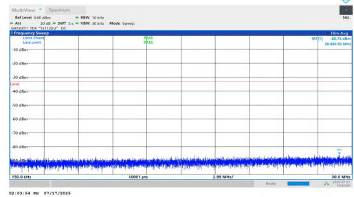
NTV-n77(3700-3980)-PC1.5-30-50-L-DFT-BPSK-Inner_1RB_Left-0.15-30-PASS
