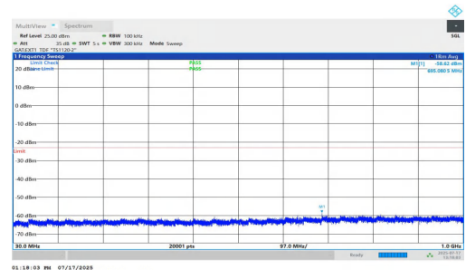
NTNV-n77(3700-3980)-PC1.5-30-40-L-DFT-BPSK-Inner_1RB_Right-3 0-1000-PASS
