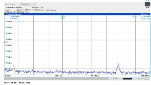
NTVN-n77(3700-3980)-PC1.5-30-40-L-DFT-QPSK-Inner_1RB_Right-0 .009-0.15-PASS
