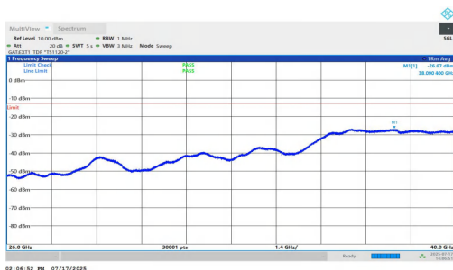
NTV-n77(3700-3980)-PC1.5-30-50-L-DFT-BPSK-Inner_1RB_Left-26000-40000-PASS
