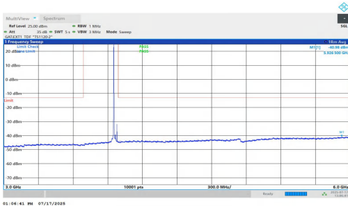
NTNV-n77(3700-3980)-PC1.5-30-30-H-DFT-QPSK-Inner_1RB_Left-3 000-6000-PASS
