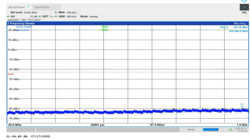
NTNV-n77(3700-3980)-PC1.5-30-40-M-DFT-BPSK-Inner_1RB_Right-3 0-1000-PASS
