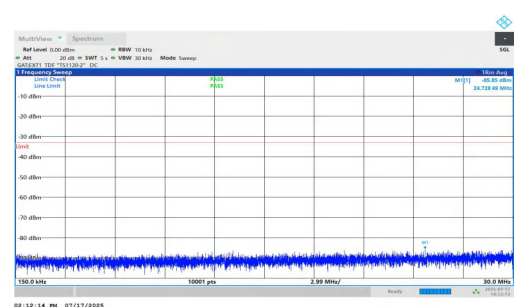
NTNV-n77(3700-3980)-PC1.5-30-50-L-DFT-QPSK-Inner_1RB_Left-0.1 5-30-PASS
