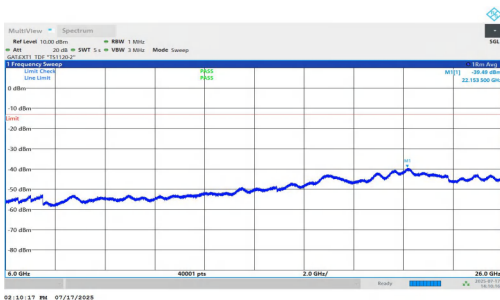
NTNV-n77(3700-3980)-PC1.5-30-50-L-DFT-BPSK-Inner_1RB_Right-6000-26000-PASS
