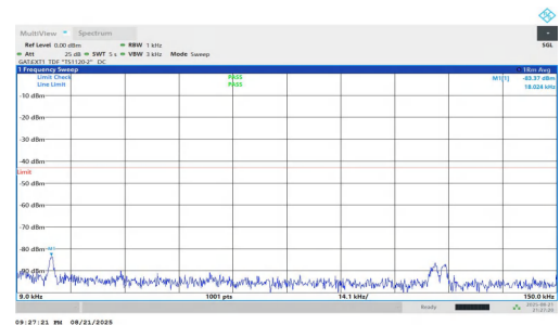
NTNV-n77(3700-3980)-PC1.5-30-30-H-DFT-QPSK-Inner_1RB_Right-0 .009-0.15-PASS
