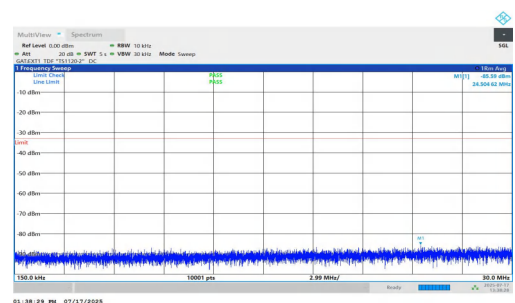
NTNV-n77(3700-3980)-PC1.5-30-40-M-DFT-QPSK-Inner_1RB_Left-0.15-30-PASS
