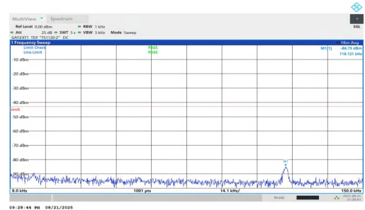
NTNV-n77(3700-3980)-PC1.5-30-40-L-DFT-BPSK-Inner_1RB_Right-0 009-0.15-PASS
