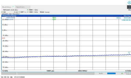
NTNV-n77(3700-3980)-PC1.5-30-50-L-DFT-BPSK-Inner_1RB_Right-1000-3000-PASS
