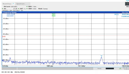
NTNV-n77(3700-3980)-PC1.5-30-40-M-DFT-BPSK-Inner_1RB_Left-0.009-0.15-PASS
