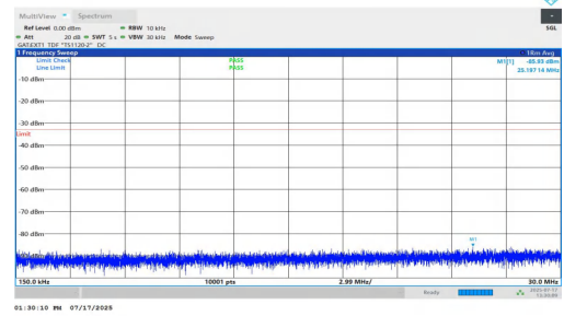
NTNV-n77(3700-3980)-PC1.5-30-40-M-DFT-BPSK-Inner_1RB_Left-0.15-30-PASS
