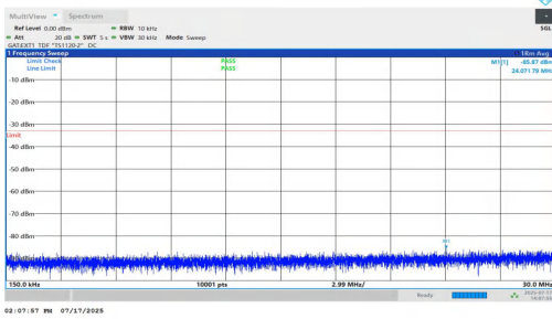
NTNV-n77(3700-3980)-PC1.5-30-50-L-DFT-BPSK-Inner_1RB_Right-0.15-30-PASS
