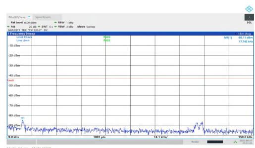
NTNV-n77(3700-3980)-PC1.5-30-40-M-DFT-BPSK-Inner_1RB_Right-0.009-0.15-PASS
