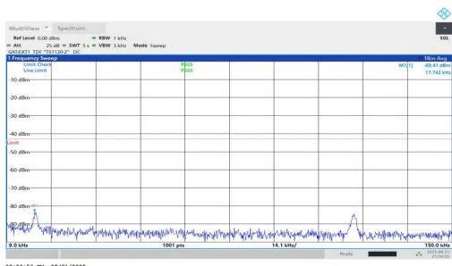
NTNV-n77(3700-3980)-PC1.5-30-40-H-DFT-QPSK-Inner_1RB_Left-0.009-0.15-PASS
