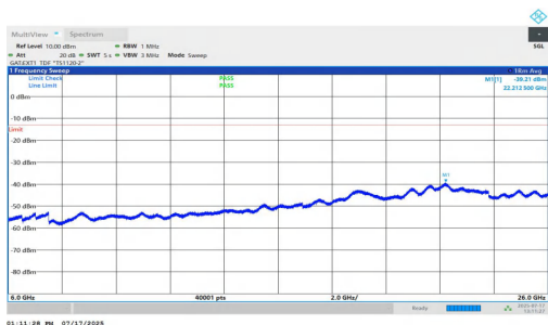
NTNV-n77(3700-3980)-PC1.5-30-30-H-DFT-QPSK-Inner_1RB_Right-6000-26000-PASS
