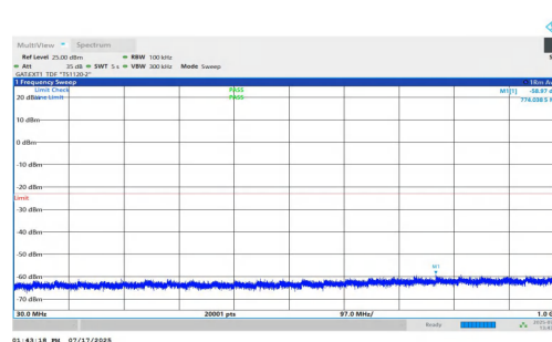
NTNV-n77(3700-3980)-PC1.5-30-40-M-DFT-QPSK-Inner_1RB_Right- 30-1000-PASS
