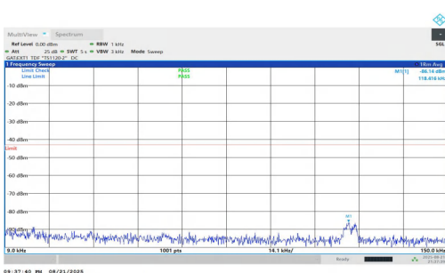
NTNV-n77(3700-3980)-PC1.5-30-50-L-DFT-QPSK-Inner_1RB_Left-0.009-0.15-PASS
