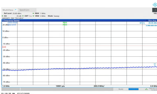
NTNV-n77(3700-3980)-PC1.5-30-40-L-DFT-BPSK-Inner_1RB_Right- 1000-3000-PASS
