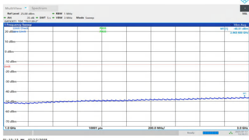
NTNV-n77(3700-3980)-PC1.5-30-30-H-DFT-QPSK-Inner_1RB_Right-1000-3000-PASS
