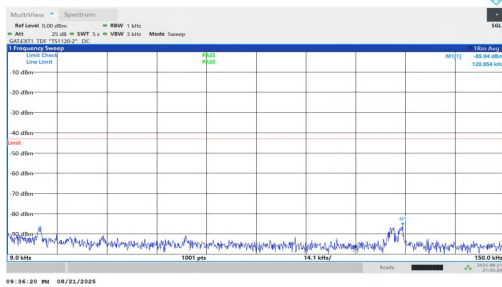
NTV-n77(3700-3980)-PC1.5-30-50-L-DFT-BPSK-Inner_1RB_Left-0.009-0.15-PASS
