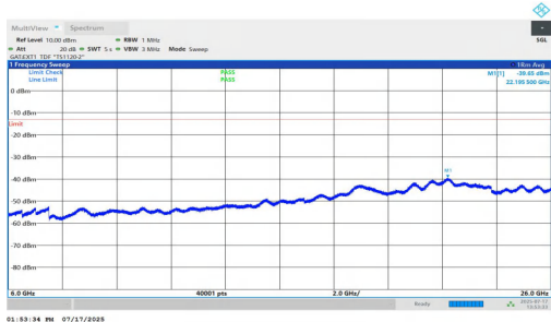
NTNV-n77(3700-3980)-PC1.5-30-40-H-DFT-BPSK-Inner_1RB_Right-6000-26000-PASS
