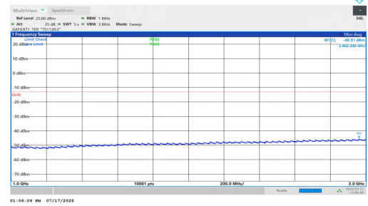
NTNV-n77(3700-3980)-PC1.5-30-30-H-DFT-QPSK-Inner_1RB_Left-10 00-3000-PASS
