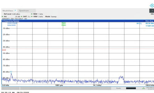
NTNV-n77(3700-3980)-PC1.5-30-40-M-DFT-QPSK-Inner_1RB_Left-0.009-0.15-PASS
