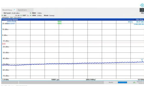
NTNV-n77(3700-3980)-PC1.5-30-40-H-DFT-BPSK-Inner_1RB_Right- 1000-3000-PASS
