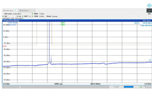
NTNV-n77(3700-3980)-PC1.5-30-40-H-DFT-QPSK-Inner_1RB_Left-3000-6000-PASS
