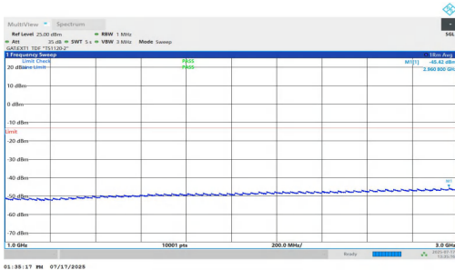
NTNV-n77(3700-3980)-PC1.5-30-40-M-DFT-BPSK-Inner_1RB_Right-1000-3000-PASS
