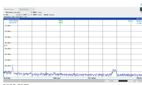
NTNV-n77(3700-3980)-PC1.5-30-40-M-DFT-QPSK-Inner_1RB_Right- 0.009-0.15-PASS
