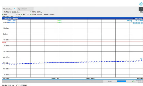
NTVN-n77(3700-3980)-PC1.5-30-40-L-DFT-QPSK-Inner_1RB_Right- 1000-3000-PASS
