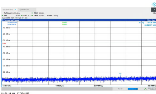
NTNV-n77(3700-3980)-PC1.5-30-40-H-DFT-BPSK-Inner_1RB_Right- 0.15-30-PASS
