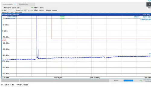
NTNV-n77(3700-3980)-PC1.5-30-40-L-DFT-BPSK-Inner_1RB_Left-30 00-6000-PASS
