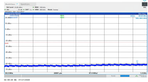
NTNV-n77(3700-3980)-PC1.5-30-50-L-DFT-BPSK-Inner_1RB_Right-3 0-1000-PASS
