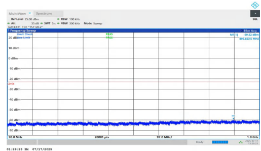
NTVN-n77(3700-3980)-PC1.5-30-40-L-DFT-QPSK-Inner_1RB_Right-3 0-1000-PASS
