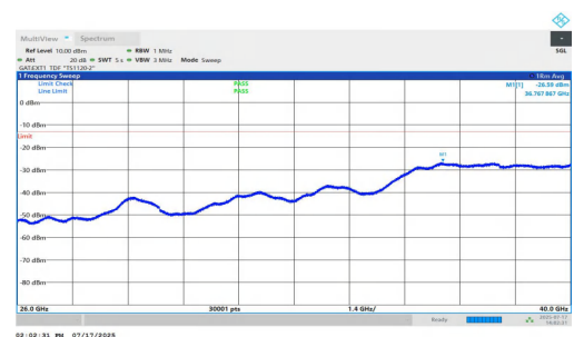
NTNV-n77(3700-3980)-PC1.5-30-40-H-DFT-QPSK-Inner_1RB_Right-2 6000-40000-PASS
