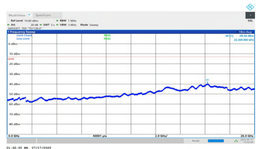
NTNV-n77(3700-3980)-PC1.5-30-40-M-DFT-BPSK-Inner_1RB_Left-6000-26000-PASS
