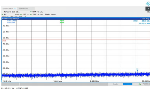
NTNV-n77(3700-3980)-PC1.5-30-40-L-DFT-BPSK-Inner_1RB_Right- 0.15-30-PASS
