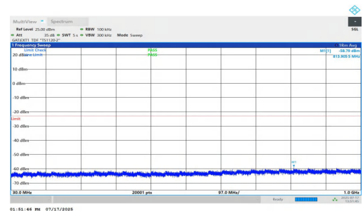
NTNV-n77(3700-3980)-PC1.5-30-40-H-DFT-BPSK-Inner_1RB_Right-3 0-1000-PASS
