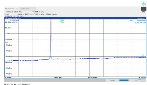
NTNV-n77(3700-3980)-PC1.5-30-40-H-DFT-QPSK-Inner_1RB_Right-3 000-6000-PASS
