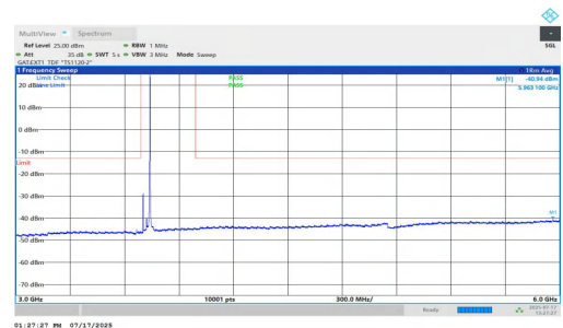
NTVN-n77(3700-3980)-PC1.5-30-40-L-DFT-QPSK-Inner_1RB_Right-3 000-6000-PASS
