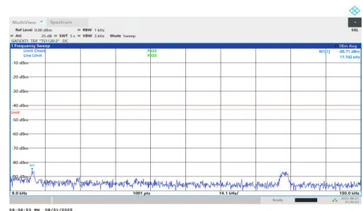
NTV-n77(3700-3980)-PC1.5-30-50-L-DFT-BPSK-Inner_1RB_Right-0.009-0.15-PASS
