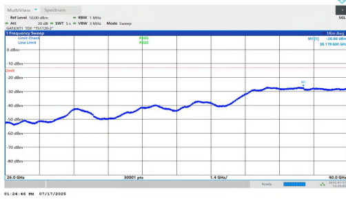
NTVN-n77(3700-3980)-PC1.5-30-40-L-DFT-QPSK-Inner_1RB_Left-2 6000-40000-PASS
