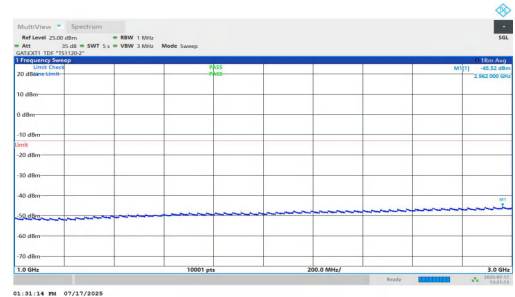
NTNV-n77(3700-3980)-PC1.5-30-40-M-DFT-BPSK-Inner_1RB_Left-1000-3000-PASS
