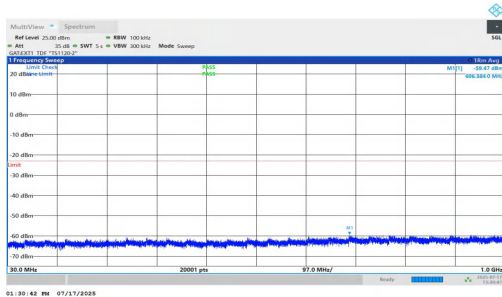
NTNV-n77(3700-3980)-PC1.5-30-40-M-DFT-BPSK-Inner_1RB_Left-30-1000-PASS
