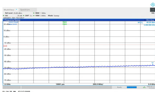
NTNV-n77(3700-3980)-PC1.5-30-40-L-DFT-BPSK-Inner_1RB_Left-1.00-3.00-PASS
