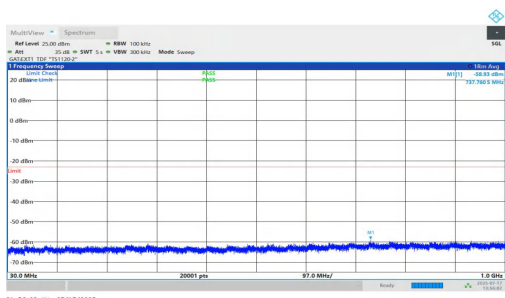
NTNV-n77(3700-3980)-PC1.5-30-40-H-DFT-QPSK-Inner_1RB_Left-30-1000-PASS
