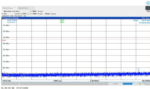
NTNV-n77(3700-3980)-PC1.5-30-40-H-DFT-QPSK-Inner_1RB_Right-0.15-30-PASS
