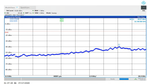
NTNV-n77(3700-3980)-PC1.5-30-30-H-DFT-QPSK-Inner_1RB_Left-60 00-26000-PASS
