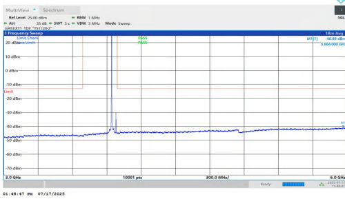
NTNV-n77(3700-3980)-PC1.5-30-40-H-DFT-BPSK-Inner_1RB_Left-3 000-6000-PASS
