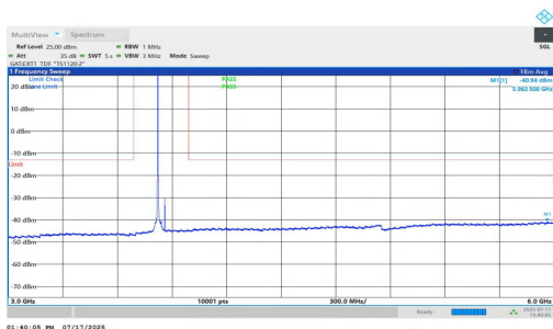
NTNV-n77(3700-3980)-PC1.5-30-40-M-DFT-QPSK-Inner_1RB_Left-3 000-6000-PASS
