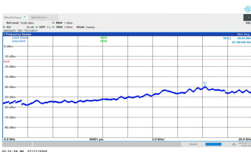
NTNV-n77(3700-3980)-PC1.5-30-40-H-DFT-QPSK-Inner_1RB_Right-6000-26000-PASS
