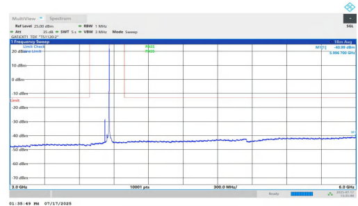
NTNV-n77(3700-3980)-PC1.5-30-40-M-DFT-BPSK-Inner_1RB_Right-3 000-6000-PASS
