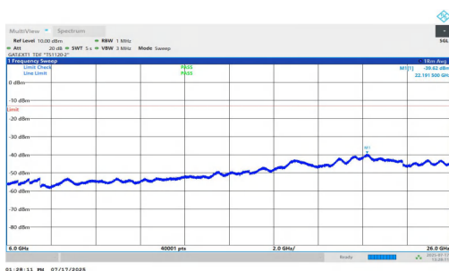
NTVN-n77(3700-3980)-PC1.5-30-40-L-DFT-QPSK-Inner_1RB_Right- 6000-26000-PASS
