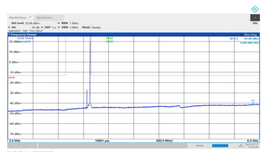
NTNV-n77(3700-3980)-PC1.5-30-40-H-DFT-BPSK-Inner_1RB_Right-3 000-6000-PASS
