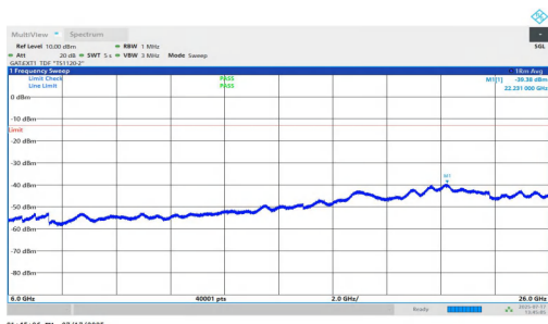
NTNV-n77(3700-3980)-PC1.5-30-40-M-DFT-QPSK-Inner_1RB_Right-6000-26000-PASS
