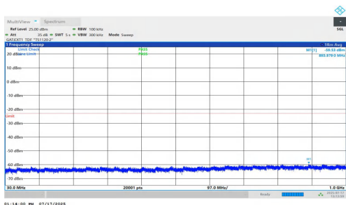
NTNV-n77(3700-3980)-PC1.5-30-40-L-DFT-BPSK-Inner_1RB_Left-0.30-1.00-PASS
