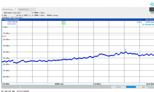
NTNV-n77(3700-3980)-PC1.5-30-40-M-DFT-BPSK-Inner_1RB_Right-6000-26000-PASS
