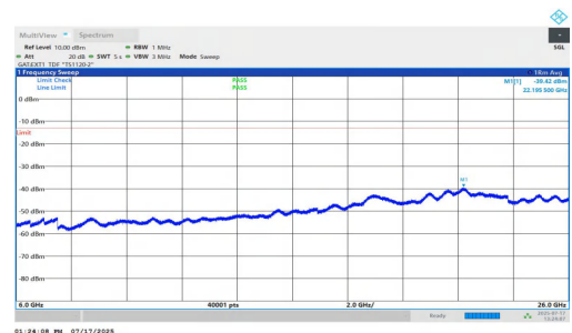
NTNV-n77(3700-3980)-PC1.5-30-40-L-DFT-QPSK-Inner_1RB_Left-60000-260000-PASS
