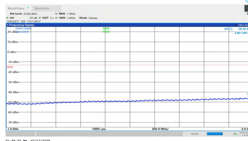
NTNV-n77(3700-3980)-PC1.5-30-40-M-DFT-QPSK-Inner_1RB_Left-10 00-3000-PASS
