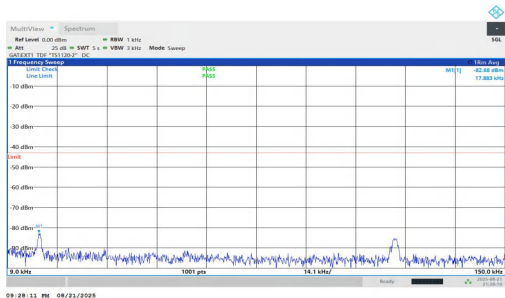
NTNV-n77(3700-3980)-PC1.5-30-40-L-DFT-BPSK-Inner_1RB_Left-0.009-0.15-PASS
