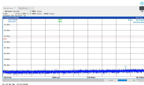
NTNV-n77(3700-3980)-PC1.5-30-40-L-DFT-BPSK-Inner_1RB_Left-0.15-0.30-PASS
