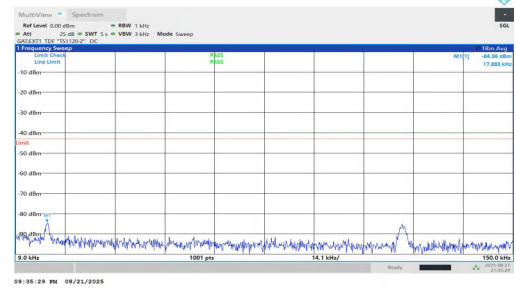
NTNV-n77(3700-3980)-PC1.5-30-40-H-DFT-QPSK-Inner_1RB_Right-0 .009-0.15-PASS
