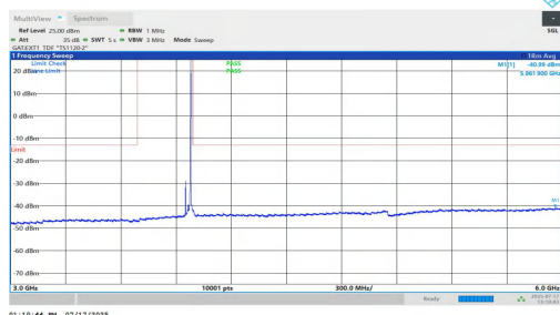
NTNV-n77(3700-3980)-PC1.5-30-30-H-DFT-QPSK-Inner_1RB_Right-3000-6000-PASS
