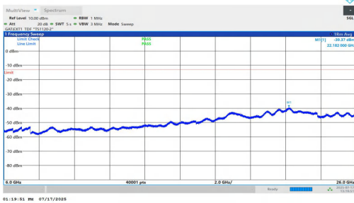
NTNV-n77(3700-3980)-PC1.5-30-40-L-DFT-BPSK-Inner_1RB_Right-6000-26000-PASS
