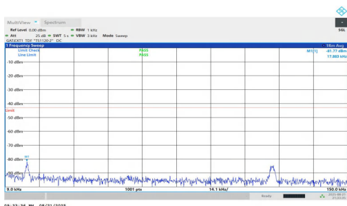
NTNV-n77(3700-3980)-PC1.5-30-40-H-DFT-BPSK-Inner_1RB_Left-0.009-0.15-PASS
