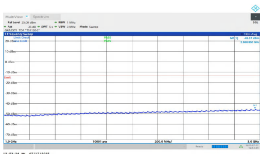
NTNV-n77(3700-3980)-PC1.5-30-30-M-DFT-QPSK-Inner_1RB_Right- 1000-3000-PASS
