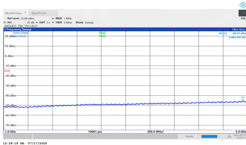
NTNV-n77(3700-3980)-PC1.5-30-30-L-DFT-BPSK-Inner_1RB_Right-1000-3000-PASS
