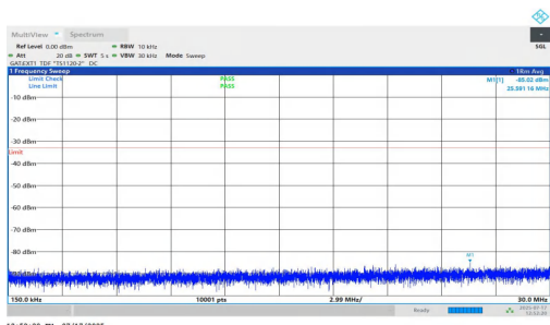
NTNV-n77(3700-3980)-PC1.5-30-30-M-DFT-QPSK-Inner_1RB_Right- 0.15-30-PASS
