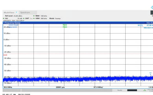
NTNV-n77(3700-3980)-PC1.5-30-25-M-DFT-QPSK-Inner_1RB_Right- 30-1000-PASS
