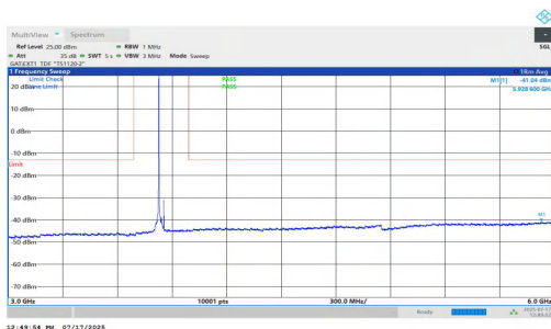
NTNV-n77(3700-3980)-PC1.5-30-30-M-DFT-QPSK-Inner_1RB_Left-3000-6000-PASS
