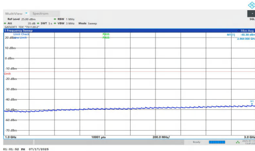
NTNV-n77(3700-3980)-PC1.5-30-30-H-DFT-BPSK-Inner_1RB_Right-1000-3000-PASS
