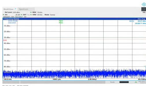
NTNV-n77(3700-3980)-PC1.5-30-25-H-DFT-QPSK-Inner_1RB_Left-0.15-30-PASS
