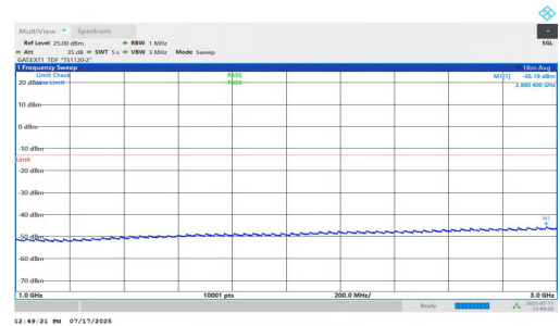
NTNV-n77(3700-3980)-PC1.5-30-30-M-DFT-QPSK-Inner_1RB_Left-1000-3000-PASS
