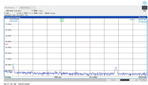
NTNV-n77(3700-3980)-PC1.5-30-25-H-DFT-BPSK-Inner_1RB_Right-0 .009-0.15-PASS
