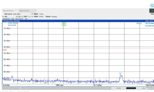
NTNV-n77(3700-3980)-PC1.5-30-30-H-DFT-QPSK-Inner_1RB_Left-0.009-0.15-PASS
