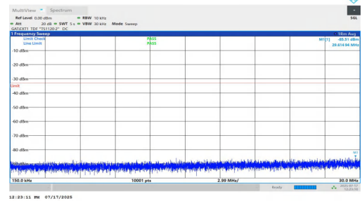
NTV-n77(3700-3980)-PC1.5-30-30-L-DFT-BPSK-Inner_1RB_Left-0.15-30-PASS
