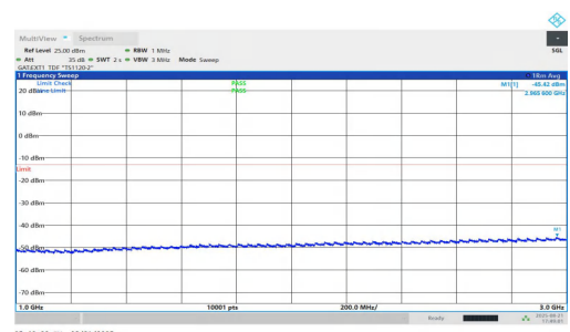
NTNV-n77(3700-3980)-PC1.5-30-25-H-DFT-BPSK-Inner_1RB_Left-1000-3000-PASS
