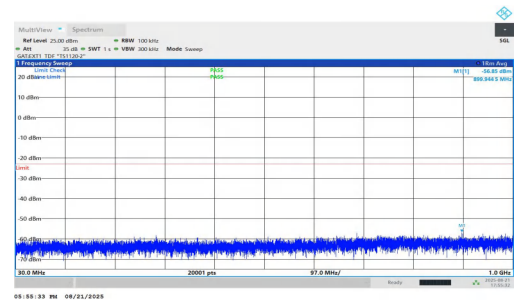
NTNV-n77(3700-3980)-PC1.5-30-25-H-DFT-QPSK-Inner_1RB_Right-3 0-1000-PASS
