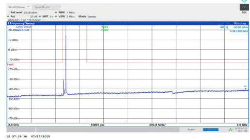
NTNV-n77(3700-3980)-PC1.5-30-30-L-DFT-QPSK-Inner_1RB_Right-3000-6000-PASS
