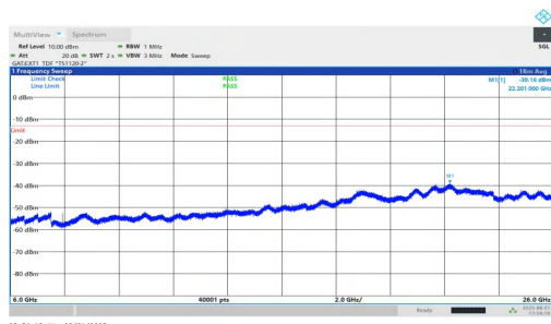
NTNV-n77(3700-3980)-PC1.5-30-25-H-DFT-QPSK-Inner_1RB_Left-6000-26000-PASS
