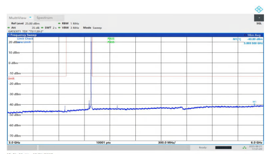
NTNV-n77(3700-3980)-PC1.5-30-25-H-DFT-BPSK-Inner_1RB_Right-3 000-6000-PASS
