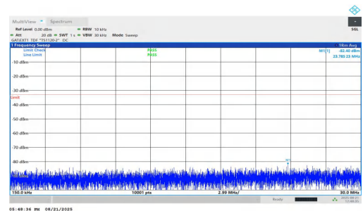
NTNV-n77(3700-3980)-PC1.5-30-25-H-DFT-BPSK-Inner_1RB_Left-0.15-5-30-PASS
