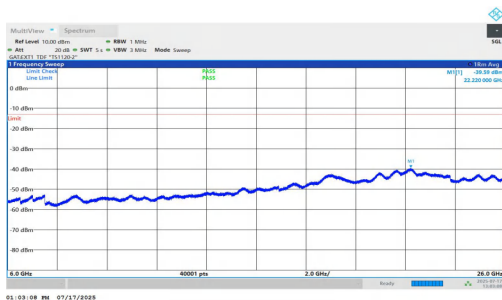
NTNV-n77(3700-3980)-PC1.5-30-30-H-DFT-BPSK-Inner_1RB_Right-6000-26000-PASS
