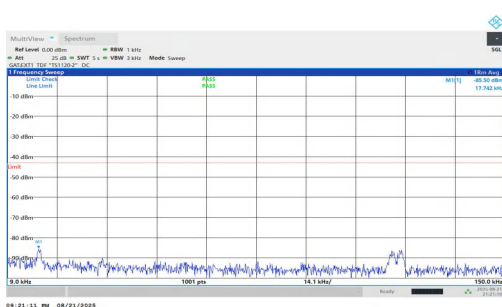
NTNV-n77(3700-3980)-PC1.5-30-30-L-DFT-QPSK-Inner_1RB_Left-0.009-0.15-PASS
