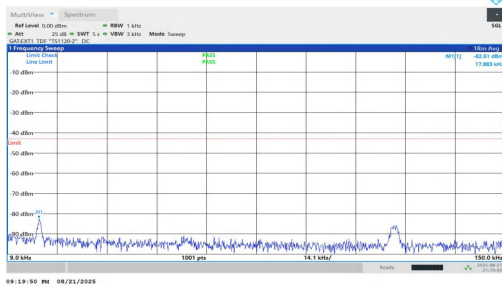
NTV-n77(3700-3980)-PC1.5-30-30-L-DFT-BPSK-Inner_1RB_Left-0.009-0.15-PASS
