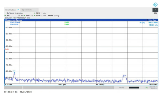
NTV-n77(3700-3980)-PC1.5-30-30-L-DFT-BPSK-Inner_1RB_Right-0.009-0.15-PASS
