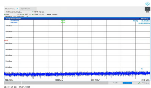
NTNV-n77(3700-3980)-PC1.5-30-30-M-DFT-QPSK-Inner_1RB_Left-0.15-30-PASS
