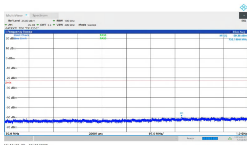
NTNV-n77(3700-3980)-PC1.5-30-30-M-DFT-QPSK-Inner_1RB_Right- 30-1000-PASS
