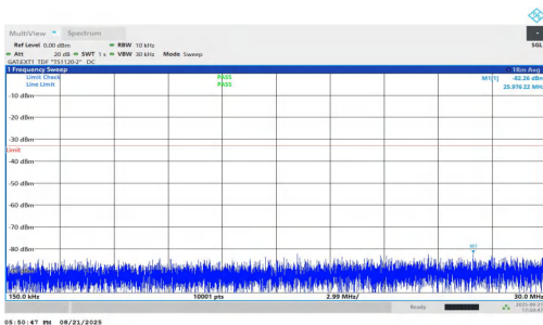
NTNV-n77(3700-3980)-PC1.5-30-25-H-DFT-BPSK-Inner_1RB_Right- 0.15-30-PASS
