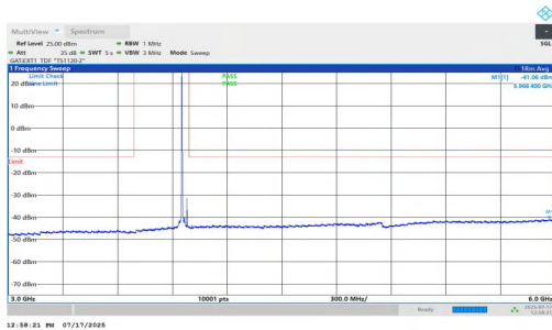
NTNV-n77(3700-3980)-PC1.5-30-30-H-DFT-BPSK-Inner_1RB_Left-3000-6000-PASS
