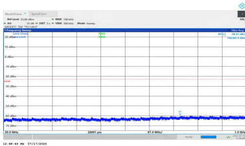
NTNV-n77(3700-3980)-PC1.5-30-30-M-DFT-QPSK-Inner_1RB_Left-30-1000-PASS
