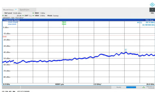
NTNV-n77(3700-3980)-PC1.5-30-30-M-DFT-QPSK-Inner_1RB_Right- 6000-26000-PASS
