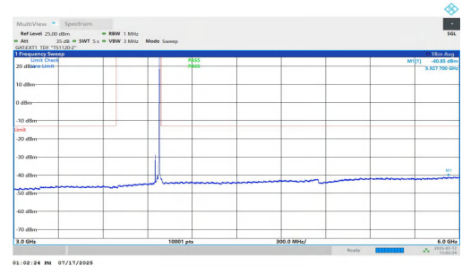
NTNV-n77(3700-3980)-PC1.5-30-30-H-DFT-BPSK-Inner_1RB_Right-3 000-6000-PASS
