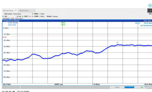
NTNV-n77(3700-3980)-PC1.5-30-30-H-DFT-BPSK-Inner_1RB_Left-26000-40000-PASS
