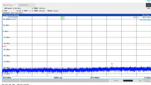
NTNV-n77(3700-3980)-PC1.5-30-25-M-DFT-QPSK-Inner_1RB_Left-3 0-1000-PASS
