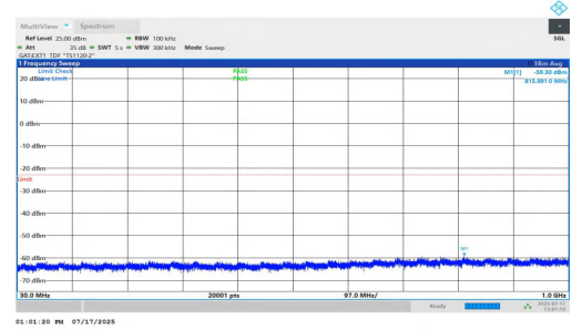
NTNV-n77(3700-3980)-PC1.5-30-30-H-DFT-BPSK-Inner_1RB_Right-3 0-1000-PASS
