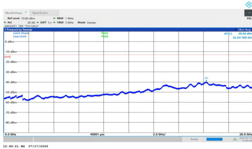
NTNV-n77(3700-3980)-PC1.5-30-30-M-DFT-BPSK-Inner_1RB_Right-6000-26000-PASS
