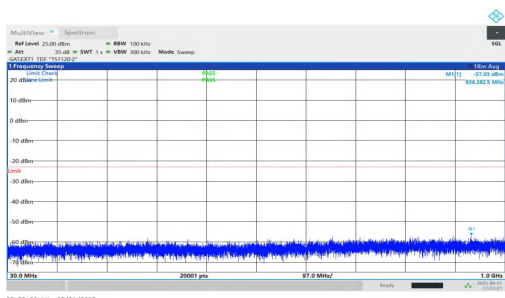
NTNV-n77(3700-3980)-PC1.5-30-25-H-DFT-QPSK-Inner_1RB_Left-30-1000-PASS
