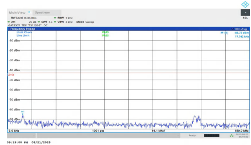
NTNV-n77(3700-3980)-PC1.5-30-25-H-DFT-QPSK-Inner_1RB_Right-0 .009-0.15-PASS
