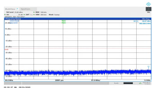
NTNV-n77(3700-3980)-PC1.5-30-25-H-DFT-BPSK-Inner_1RB_Right-3 0-1000-PASS
