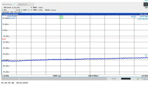
NTNV-n77(3700-3980)-PC1.5-30-25-M-DFT-QPSK-Inner_1RB_Right-1000-3000-PASS
