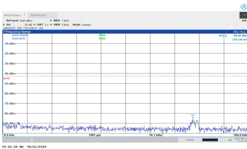
NTNV-n77(3700-3980)-PC1.5-30-30-M-DFT-BPSK-Inner_1RB_Left-0.009-0.15-PASS
