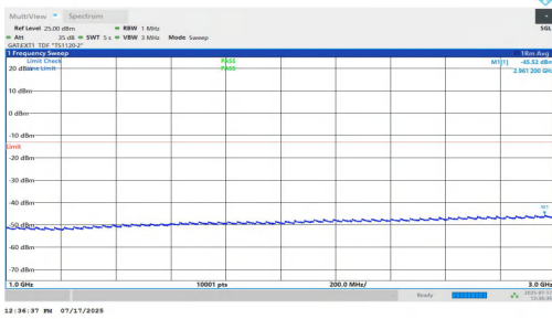
NTNV-n77(3700-3980)-PC1.5-30-30-L-DFT-QPSK-Inner_1RB_Right-1000-3000-PASS
