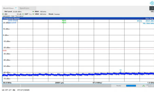
NTNV-n77(3700-3980)-PC1.5-30-30-H-DFT-BPSK-Inner_1RB_Left-3000-1000-PASS
