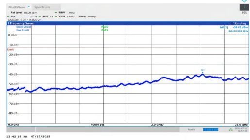
NTNV-n77(3700-3980)-PC1.5-30-30-M-DFT-BPSK-Inner_1RB_Left-60 00-26000-PASS
