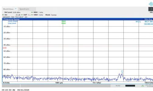
NTNV-n77(3700-3980)-PC1.5-30-30-M-DFT-QPSK-Inner_1RB_Left-0.009-0.15-PASS
