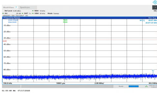
NTNV-n77(3700-3980)-PC1.5-30-30-H-DFT-BPSK-Inner_1RB_Right-0.15-30-PASS
