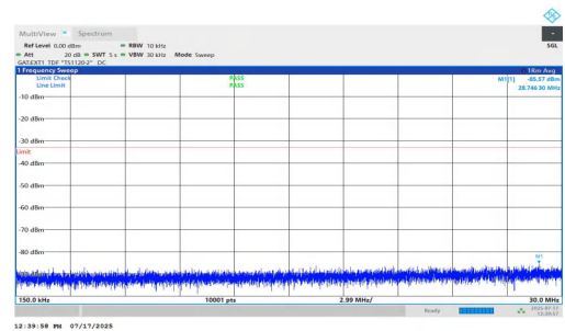
NTNV-n77(3700-3980)-PC1.5-30-30-M-DFT-BPSK-Inner_1RB_Left-0.15-30-PASS
