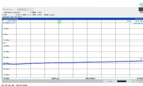
NTNV-n77(3700-3980)-PC1.5-30-25-H-DFT-QPSK-Inner_1RB_Right-1000-3000-PASS
