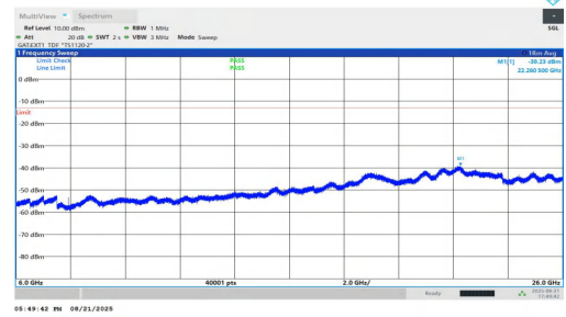
NTNV-n77(3700-3980)-PC1.5-30-25-H-DFT-BPSK-Inner_1RB_Left-60 00-26000-PASS
