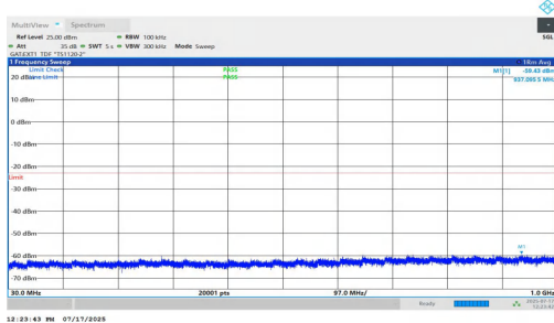
NTV-n77(3700-3980)-PC1.5-30-30-L-DFT-BPSK-Inner_1RB_Left-30-1000-PASS
