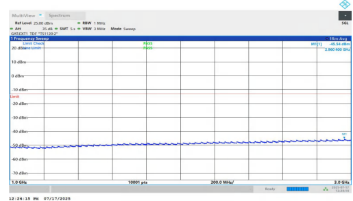
NTV-n77(3700-3980)-PC1.5-30-30-L-DFT-BPSK-Inner_1RB_Left-1000-3000-PASS
