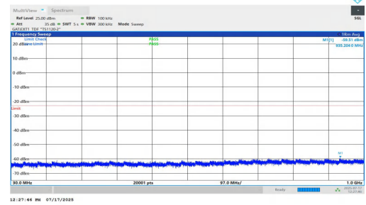
NTNV-n77(3700-3980)-PC1.5-30-30-L-DFT-BPSK-Inner_1RB_Right-3 0-1000-PASS
