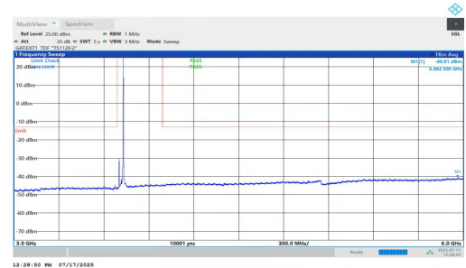
NTNV-n77(3700-3980)-PC1.5-30-30-L-DFT-BPSK-Inner_1RB_Right-3 000-6000-PASS
