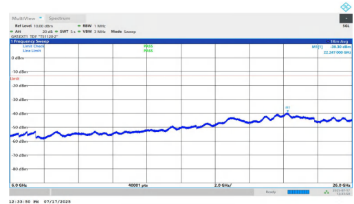
NTVN-n77(3700-3980)-PC1.5-30-30-L-DFT-QPSK-Inner_1RB_Left-60 00-26000-PASS
