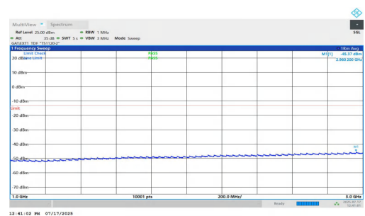
NTNV-n77(3700-3980)-PC1.5-30-30-M-DFT-BPSK-Inner_1RB_Left-1000-3000-PASS
