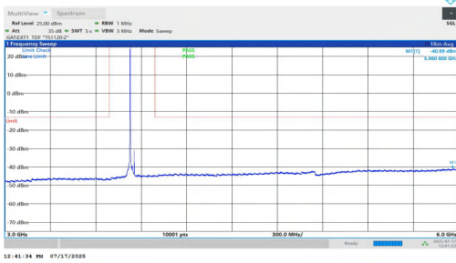
NTNV-n77(3700-3980)-PC1.5-30-30-M-DFT-BPSK-Inner_1RB_Left-3 000-6000-PASS
