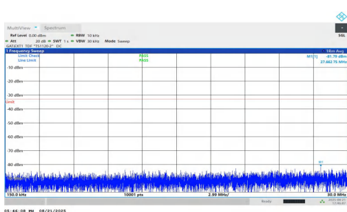
NTNV-n77(3700-3980)-PC1.5-30-25-M-DFT-QPSK-Inner_1RB_Right- 0.15-30-PASS
