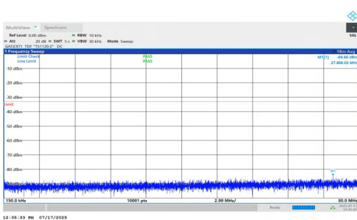
NTVN-n77(3700-3980)-PC1.5-30-30-L-DFT-QPSK-Inner_1RB_Right- 0.15-30-PASS
