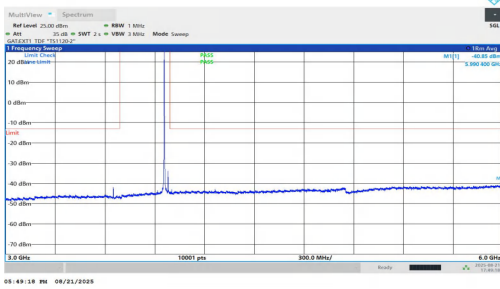
NTNV-n77(3700-3980)-PC1.5-30-25-H-DFT-BPSK-Inner_1RB_Left-3 000-6000-PASS
