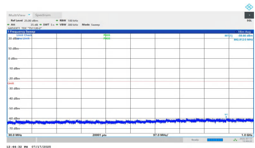
NTNV-n77(3700-3980)-PC1.5-30-30-M-DFT-BPSK-Inner_1RB_Right-3 0-1000-PASS
