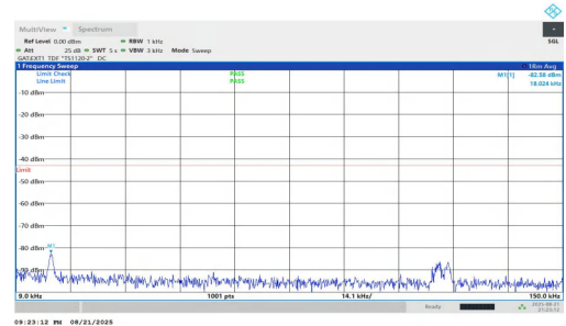
NTNV-n77(3700-3980)-PC1.5-30-30-M-DFT-BPSK-Inner_1RB_Right-0 .009-0.15-PASS
