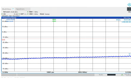
NTNV-n77(3700-3980)-PC1.5-30-25-H-DFT-BPSK-Inner_1RB_Right- 1000-3000-PASS
