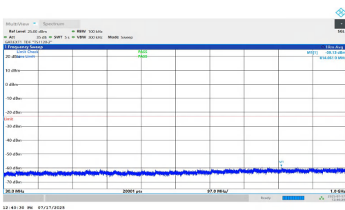
NTNV-n77(3700-3980)-PC1.5-30-30-M-DFT-BPSK-Inner_1RB_Left-30-1000-PASS
