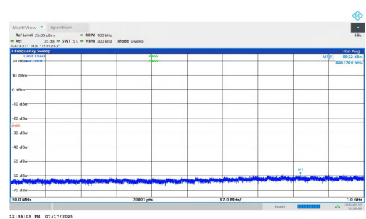
NTVN-n77(3700-3980)-PC1.5-30-30-L-DFT-QPSK-Inner_1RB_Right-3 0-1000-PASS
