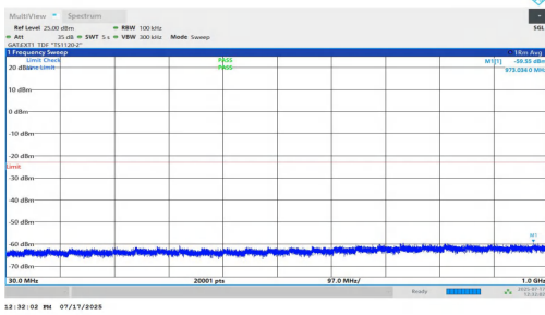
NTVN-n77(3700-3980)-PC1.5-30-30-L-DFT-QPSK-Inner_1RB_Left-3 0-1000-PASS
