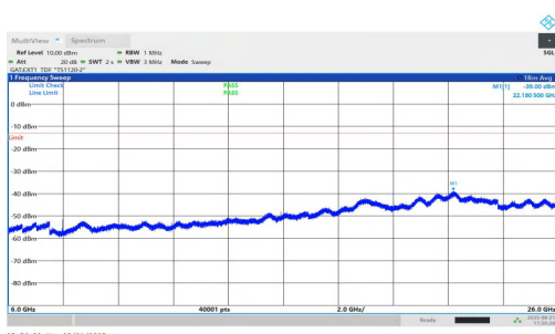
NTNV-n77(3700-3980)-PC1.5-30-25-H-DFT-QPSK-Inner_1RB_Right-6000-26000-PASS
