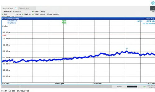
NTNV-n77(3700-3980)-PC1.5-30-25-M-DFT-QPSK-Inner_1RB_Right-6000-26000-PASS
