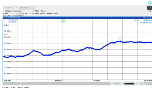
NTNV-n77(3700-3980)-PC1.5-30-25-H-DFT-BPSK-Inner_1RB_Right-26000-40000-PASS
