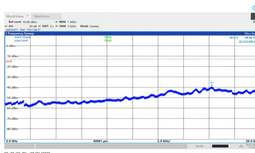
NTNV-n77(3700-3980)-PC1.5-30-25-M-DFT-QPSK-Inner_1RB_Left-60 00-26000-PASS
