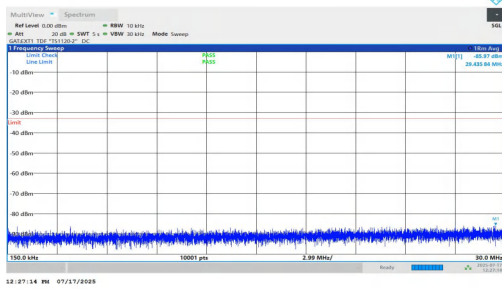
NTNV-n77(3700-3980)-PC1.5-30-30-L-DFT-BPSK-Inner_1RB_Right-0.15-30-PASS
