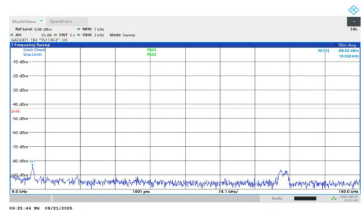
NTVN-n77(3700-3980)-PC1.5-30-30-L-DFT-QPSK-Inner_1RB_Right-0 .009-0.15-PASS
