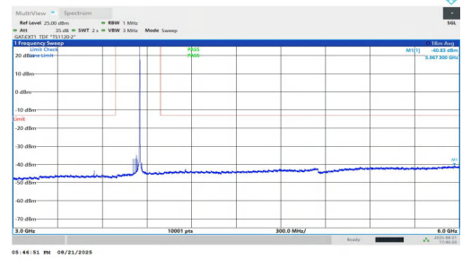
NTNV-n77(3700-3980)-PC1.5-30-25-M-DFT-QPSK-Inner_1RB_Right-3000-6000-PASS
