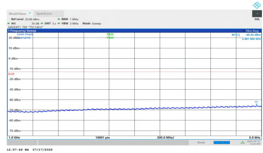
NTNV-n77(3700-3980)-PC1.5-30-30-H-DFT-BPSK-Inner_1RB_Left-1000-3000-PASS
