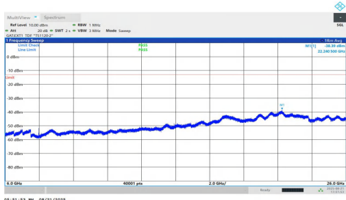
NTNV-n77(3700-3980)-PC1.5-30-25-H-DFT-BPSK-Inner_1RB_Right-6000-26000-PASS
