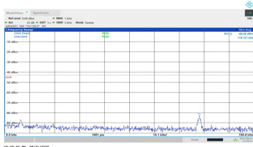
NTNV-n77(3700-3980)-PC1.5-30-30-M-DFT-QPSK-Inner_1RB_Right- 0.009-0.15-PASS
