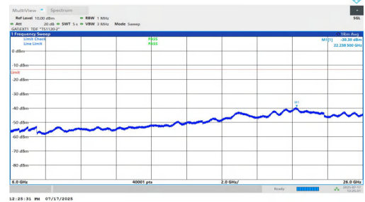
NTV-n77(3700-3980)-PC1.5-30-30-L-DFT-BPSK-Inner_1RB_Left-6000-26000-PASS
