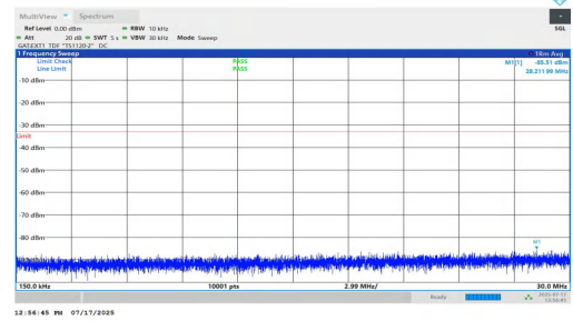
NTNV-n77(3700-3980)-PC1.5-30-30-H-DFT-BPSK-Inner_1RB_Left-0.15-30-PASS
