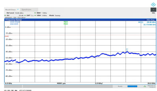
NTNV-n77(3700-3980)-PC1.5-30-30-M-DFT-QPSK-Inner_1RB_Left-6000-26000-PASS
