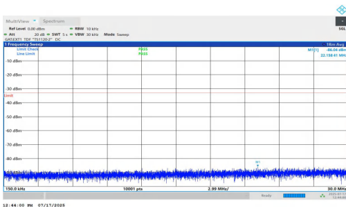
NTNV-n77(3700-3980)-PC1.5-30-30-M-DFT-BPSK-Inner_1RB_Right- 0.15-30-PASS
