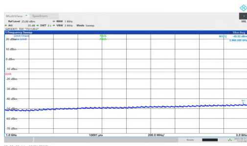
NTNV-n77(3700-3980)-PC1.5-30-25-H-DFT-QPSK-Inner_1RB_Left-1000-3000-PASS
