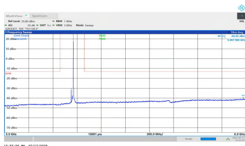
NTNV-n77(3700-3980)-PC1.5-30-30-M-DFT-QPSK-Inner_1RB_Right- 3000-6000-PASS
