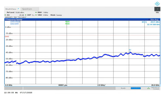
NTNV-n77(3700-3980)-PC1.5-30-30-H-DFT-BPSK-Inner_1RB_Left-6000-26000-PASS
