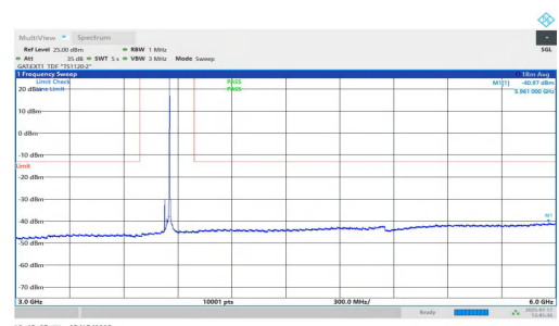
NTNV-n77(3700-3980)-PC1.5-30-30-M-DFT-BPSK-Inner_1RB_Right-3 000-6000-PASS
