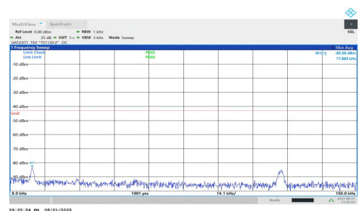
NTNV-n77(3700-3980)-PC1.5-30-30-H-DFT-BPSK-Inner_1RB_Right-0.009-0.15-PASS
