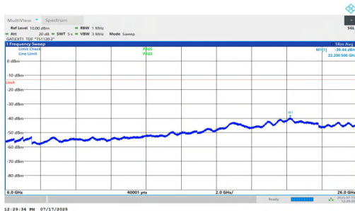
NTNV-n77(3700-3980)-PC1.5-30-30-L-DFT-BPSK-Inner_1RB_Right-6000-26000-PASS
