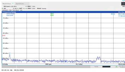
NTNV-n77(3700-3980)-PC1.5-30-30-H-DFT-BPSK-Inner_1RB_Left-0.009-0.15-PASS
