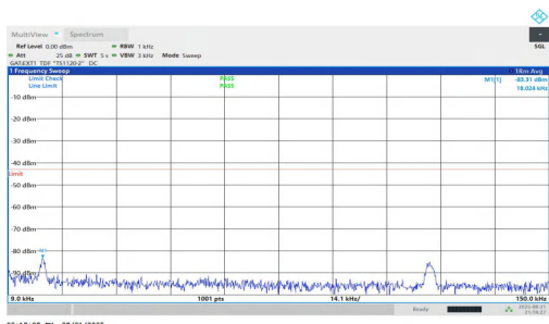
NTNV-n77(3700-3980)-PC1.5-30-25-H-DFT-QPSK-Inner_1RB_Left-0.009-0.15-PASS
