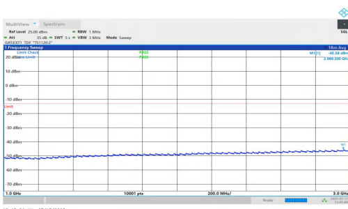
NTNV-n77(3700-3980)-PC1.5-30-30-M-DFT-BPSK-Inner_1RB_Right- 1000-3000-PASS
