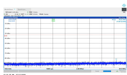
NTNV-n77(3700-3980)-PC1.5-30-30-L-DFT-QPSK-Inner_1RB_Left-0.1 5-30-PASS
