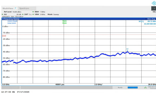
NTNV-n77(3700-3980)-PC1.5-30-30-L-DFT-QPSK-Inner_1RB_Right-6000-26000-PASS
