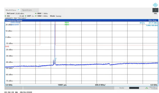
NTNV-n77(3700-3980)-PC1.5-30-25-H-DFT-QPSK-Inner_1RB_Right-3 000-6000-PASS
