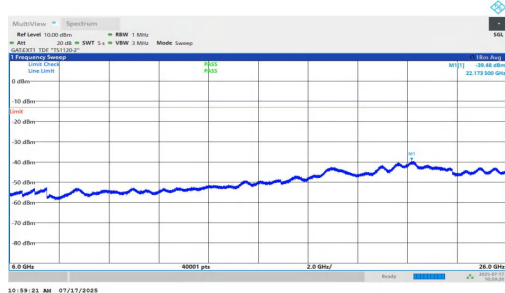
NTVN-n77(3700-3980)-PC1.5-30-15-H-DFT-BPSK-Inner_1RB_Left-60 00-26000-PASS
