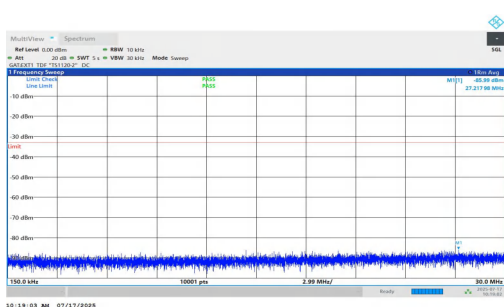
NTNV-n77(3700-3980)-PC1.5-30-10-H-DFT-QPSK-Inner_1RB_Right- 0.15-30-PASS
