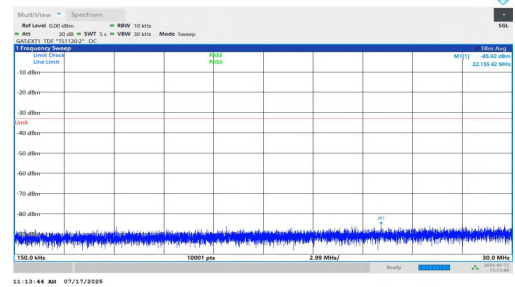
NTV-n77(3700-3980)-PC1.5-30-20-L-DFT-BPSK-Inner_1RB_Left-0.15-30-PASS
