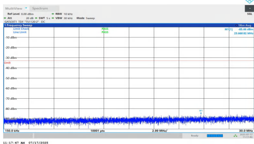
NTNV-n77(3700-3980)-PC1.5-30-20-L-DFT-BPSK-Inner_1RB_Right-0.15-30-PASS
