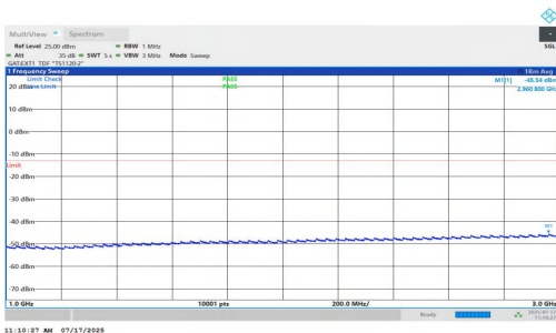
NTNV-n77(3700-3980)-PC1.5-30-15-H-DFT-QPSK-Inner_1RB_Right-1000-3000-PASS
