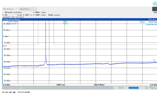
NTNV-n77(3700-3980)-PC1.5-30-15-M-DFT-BPSK-Inner_1RB_Left-3000-6000-PASS
