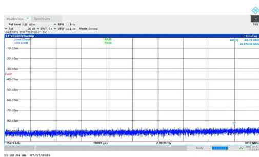
NTNV-n77(3700-3980)-PC1.5-30-20-L-DFT-QPSK-Inner_1RB_Left-0.1 5-30-PASS
