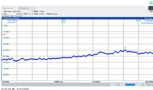
NTNV-n77(3700-3980)-PC1.5-30-10-H-DFT-QPSK-Inner_1RB_Right-6000-26000-PASS
