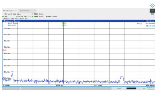
NTNV-n77(3700-3980)-PC1.5-30-15-M-DFT-QPSK-Inner_1RB_Left-0 .009-0.15-PASS
