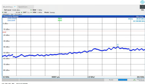
NTVN-n77(3700-3980)-PC1.5-30-15-L-DFT-BPSK-Inner_1RB_Right-6000-26000-PASS
