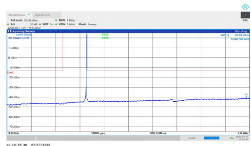
NTNV-n77(3700-3980)-PC1.5-30-15-H-DFT-QPSK-Inner_1RB_Right-3 000-6000-PASS
