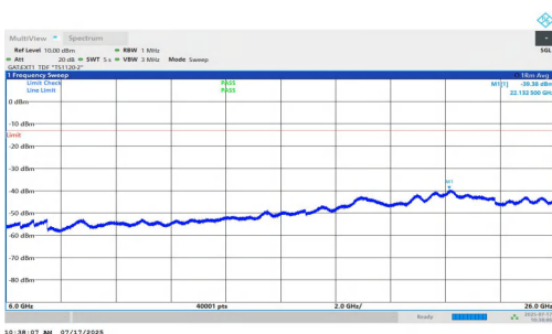
NTNV-n77(3700-3980)-PC1.5-30-15-L-DFT-QPSK-Inner_1RB_Right- 6000-26000-PASS
