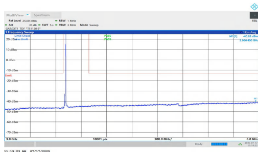
NTNV-n77(3700-3980)-PC1.5-30-20-L-DFT-BPSK-Inner_1RB_Right-3 000-6000-PASS
