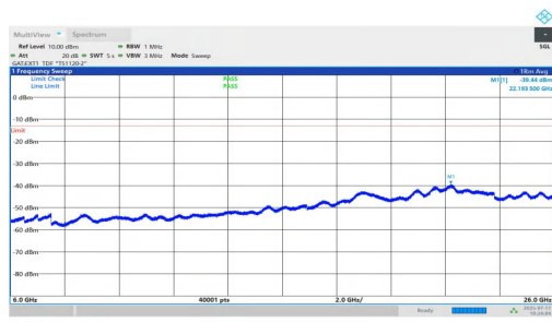
NTVN-n77(3700-3980)-PC1.5-30-15-L-DFT-QPSK-Inner_1RB_Left-6000-26000-PASS
