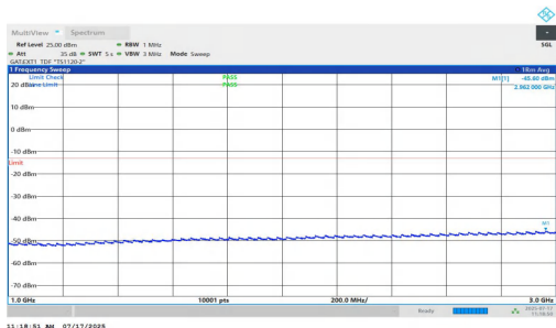
NTNV-n77(3700-3980)-PC1.5-30-20-L-DFT-BPSK-Inner_1RB_Right-1000-3000-PASS
