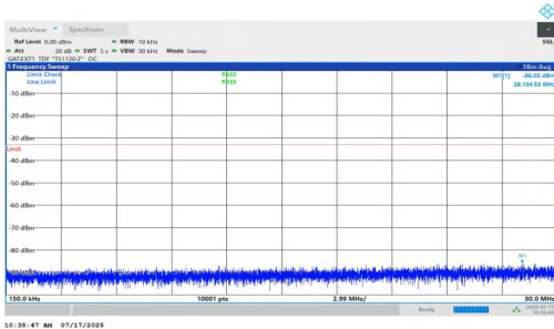
NTNV-n77(3700-3980)-PC1.5-30-15-L-DFT-QPSK-Inner_1RB_Right- 0.15-30-PASS
