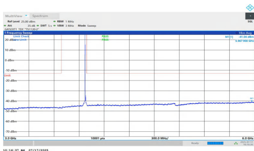
NTNV-n77(3700-3980)-PC1.5-30-10-H-DFT-QPSK-Inner_1RB_Left-3 000-6000-PASS
