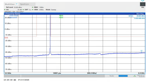
NTNV-n77(3700-3980)-PC1.5-30-10-H-DFT-QPSK-Inner_1RB_Right-3000-6000-PASS
