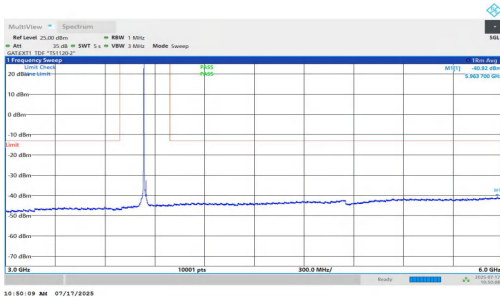
NTNV-n77(3700-3980)-PC1.5-30-15-M-DFT-QPSK-Inner_1RB_Left-3 000-6000-PASS
