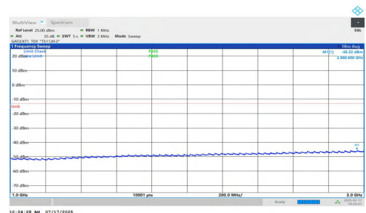
NTNV-n77(3700-3980)-PC1.5-30-15-L-DFT-BPSK-Inner_1RB_Left-1000-3000-PASS
