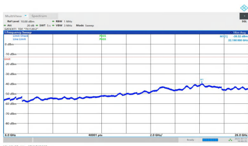
NTNV-n77(3700-3980)-PC1.5-30-15-M-DFT-BPSK-Inner_1RB_Right-6000-26000-PASS
