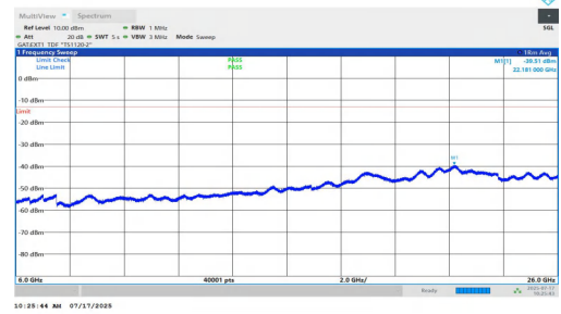
NTNV-n77(3700-3980)-PC1.5-30-15-L-DFT-BPSK-Inner_1RB_Left-60 00-26000-PASS
