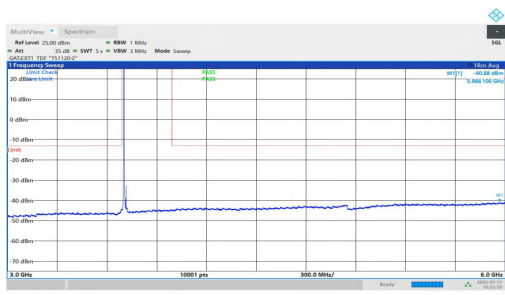
NTVN-n77(3700-3980)-PC1.5-30-15-L-DFT-QPSK-Inner_1RB_Left-3000-6000-PASS
