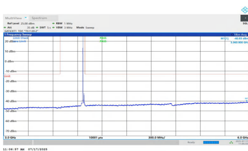
NTNV-n77(3700-3980)-PC1.5-30-15-H-DFT-QPSK-Inner_1RB_Left-3000-6000-PASS
