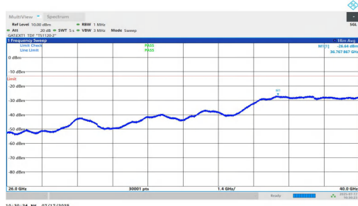
NTVN-n77(3700-3980)-PC1.5-30-15-L-DFT-BPSK-Inner_1RB_Right-26000-40000-PASS
