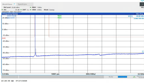
NTNV-n77(3700-3980)-PC1.5-30-15-L-DFT-BPSK-Inner_1RB_Left-30 00-6000-PASS
