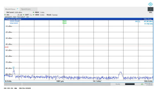
NTNV-n77(3700-3980)-PC1.5-30-15-M-DFT-QPSK-Inner_1RB_Right- 0.009-0.15-PASS
