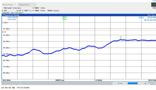
NTNV-n77(3700-3980)-PC1.5-30-15-L-DFT-QPSK-Inner_1RB_Left-2 6000-40000-PASS
