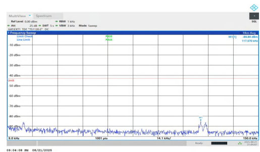
NTV-n77(3700-3980)-PC1.5-30-20-L-DFT-BPSK-Inner_1RB_Right-0.009-0.15-PASS
