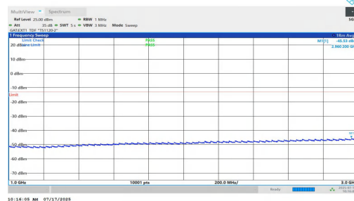
NTNV-n77(3700-3980)-PC1.5-30-10-H-DFT-QPSK-Inner_1RB_Left-10 00-3000-PASS
