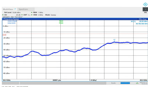
NTVN-n77(3700-3980)-PC1.5-30-15-H-DFT-BPSK-Inner_1RB_Left-2 6000-40000-PASS
