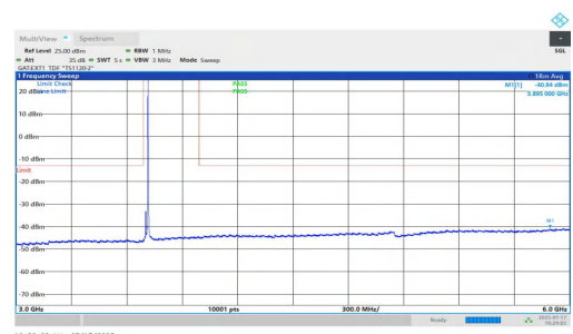
NTNV-n77(3700-3980)-PC1.5-30-15-L-DFT-BPSK-Inner_1RB_Right-3 000-6000-PASS
