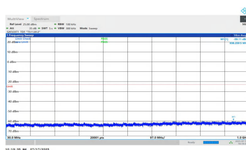
NTNV-n77(3700-3980)-PC1.5-30-10-H-DFT-QPSK-Inner_1RB_Right-3 0-1000-PASS
