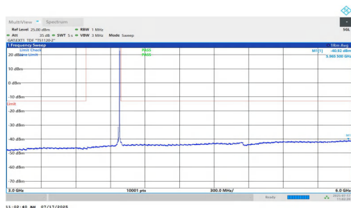
NTVN-n77(3700-3980)-PC1.5-30-15-H-DFT-BPSK-Inner_1RB_Right-3 000-6000-PASS
