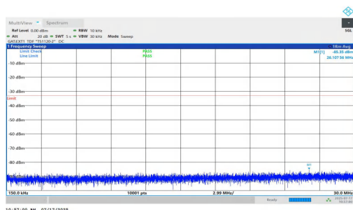
NTNV-n77(3700-3980)-PC1.5-30-15-H-DFT-BPSK-Inner_1RB_Left-0.15-5-30-PASS
