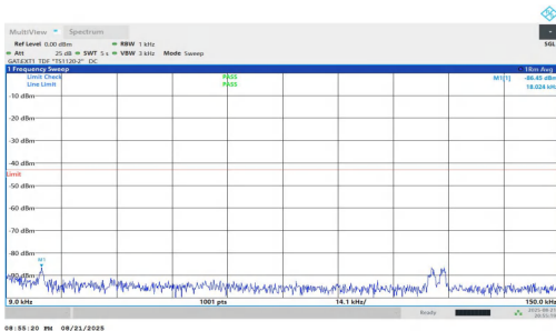
NTNV-n77(3700-3980)-PC1.5-30-15-L-DFT-BPSK-Inner_1RB_Left-0.009-0.15-PASS
