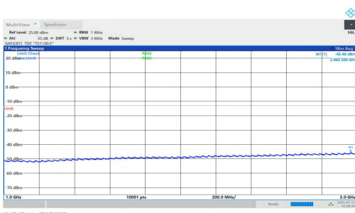
NTNV-n77(3700-3980)-PC1.5-30-15-L-DFT-BPSK-Inner_1RB_Right- 1000-3000-PASS
