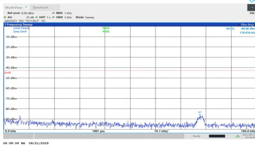
NTNV-n77(3700-3980)-PC1.5-30-15-M-DFT-BPSK-Inner_1RB_Left-0.009-0.15-PASS
