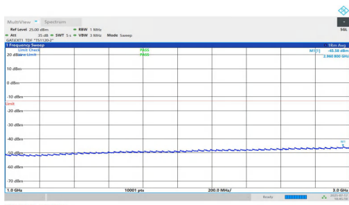
NTNV-n77(3700-3980)-PC1.5-30-15-M-DFT-BPSK-Inner_1RB_Right-1000-3000-PASS
