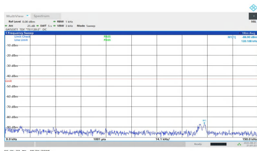
NTVN-n77(3700-3980)-PC1.5-30-15-H-DFT-BPSK-Inner_1RB_Right-0 .009-0.15-PASS
