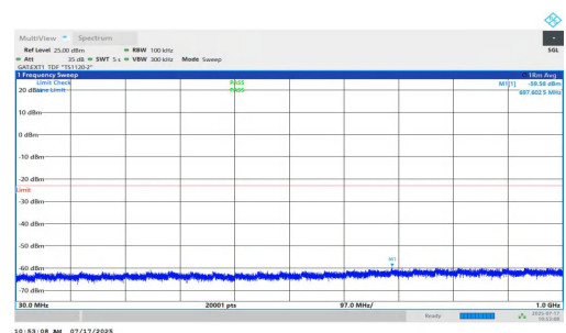
NTNV-n77(3700-3980)-PC1.5-30-15-M-DFT-QPSK-Inner_1RB_Right- 30-1000-PASS
