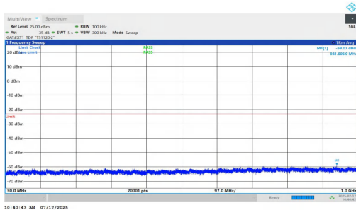
NTNV-n77(3700-3980)-PC1.5-30-15-M-DFT-BPSK-Inner_1RB_Left-30-1000-PASS
