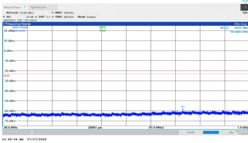
NTNV-n77(3700-3980)-PC1.5-30-15-M-DFT-QPSK-Inner_1RB_Left-3 0-1000-PASS
