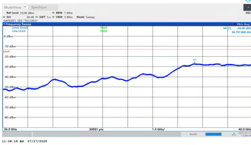
NTNV-n77(3700-3980)-PC1.5-30-15-H-DFT-QPSK-Inner_1RB_Left-2 6000-40000-PASS
