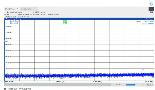
NTNV-n77(3700-3980)-PC1.5-30-15-H-DFT-QPSK-Inner_1RB_Left-0.15-30-PASS
