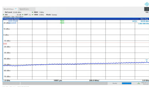
NTVN-n77(3700-3980)-PC1.5-30-15-L-DFT-QPSK-Inner_1RB_Left-1000-3000-PASS
