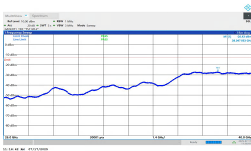
NTV-n77(3700-3980)-PC1.5-30-20-L-DFT-BPSK-Inner_1RB_Left-26000-40000-PASS
