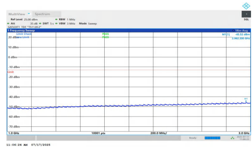
NTNV-n77(3700-3980)-PC1.5-30-15-H-DFT-QPSK-Inner_1RB_Left-1000-3000-PASS
