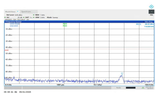
NTNV-n77(3700-3980)-PC1.5-30-15-M-DFT-BPSK-Inner_1RB_Right-0.009-0.15-PASS
