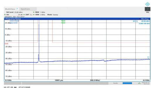
NTNV-n77(3700-3980)-PC1.5-30-15-L-DFT-QPSK-Inner_1RB_Right-3 000-6000-PASS
