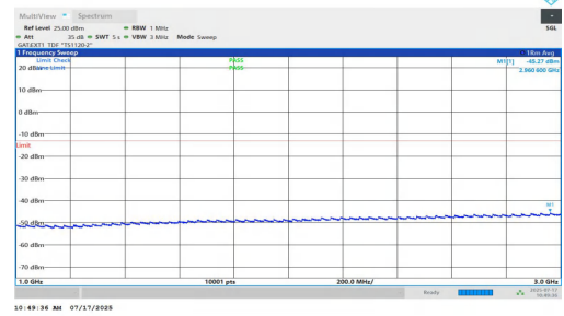
NTNV-n77(3700-3980)-PC1.5-30-15-M-DFT-QPSK-Inner_1RB_Left-10 00-3000-PASS
