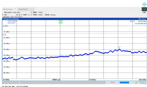
NTNV-n77(3700-3980)-PC1.5-30-15-M-DFT-QPSK-Inner_1RB_Right-6000-26000-PASS
