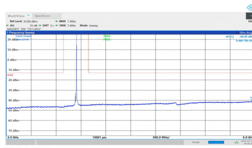
NTNV-n77(3700-3980)-PC1.5-30-15-M-DFT-BPSK-Inner_1RB_Right-3 000-6000-PASS
