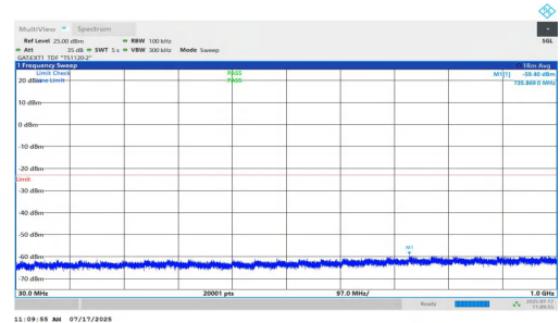
NTNV-n77(3700-3980)-PC1.5-30-15-H-DFT-QPSK-Inner_1RB_Right-3 0-1000-PASS
