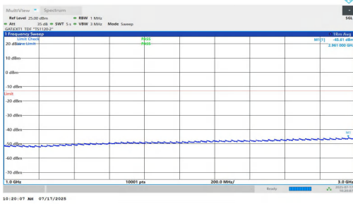
NTNV-n77(3700-3980)-PC1.5-30-10-H-DFT-QPSK-Inner_1RB_Right-1000-3000-PASS
