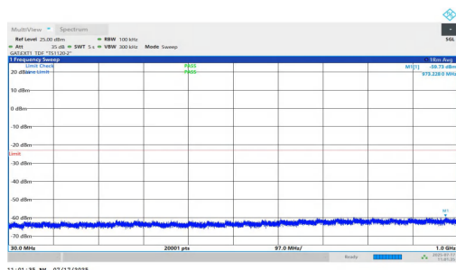
NTVN-n77(3700-3980)-PC1.5-30-15-H-DFT-BPSK-Inner_1RB_Right-3 0-1000-PASS
