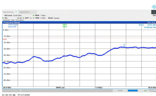
NTNV-n77(3700-3980)-PC1.5-30-15-M-DFT-BPSK-Inner_1RB_Left-26000-40000-PASS
