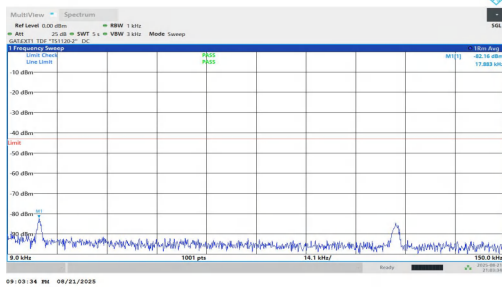
NTV-n77(3700-3980)-PC1.5-30-20-L-DFT-BPSK-Inner_1RB_Left-0.009-0.15-PASS
