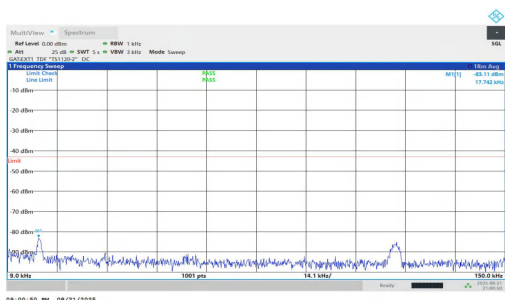
NTNV-n77(3700-3980)-PC1.5-30-15-H-DFT-BPSK-Inner_1RB_Left-0.009-0.15-PASS
