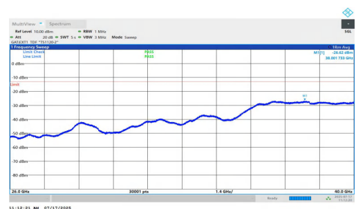
NTNV-n77(3700-3980)-PC1.5-30-15-H-DFT-QPSK-Inner_1RB_Right-2 6000-40000-PASS
