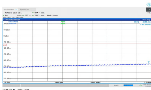
NTNV-n77(3700-3980)-PC1.5-30-15-H-DFT-BPSK-Inner_1RB_Left-1000-3000-PASS
