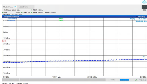
NTNV-n77(3700-3980)-PC1.5-30-15-M-DFT-QPSK-Inner_1RB_Right-1000-3000-PASS
