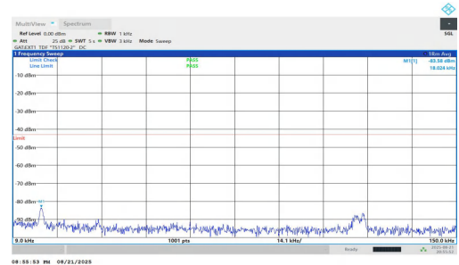
NTNV-n77(3700-3980)-PC1.5-30-15-L-DFT-BPSK-Inner_1RB_Right-0. 009-0.15-PASS
