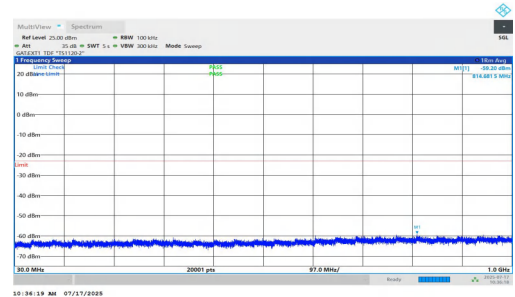
NTNV-n77(3700-3980)-PC1.5-30-15-L-DFT-QPSK-Inner_1RB_Right-3 0-1000-PASS
