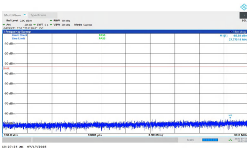
NTNV-n77(3700-3980)-PC1.5-30-15-L-DFT-BPSK-Inner_1RB_Right- 0.15-30-PASS
