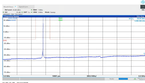
NTNV-n77(3700-3980)-PC1.5-30-15-M-DFT-QPSK-Inner_1RB_Right-3000-6000-PASS
