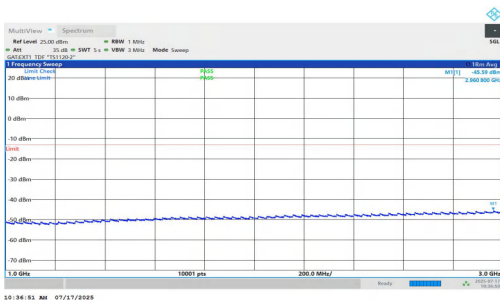
NTNV-n77(3700-3980)-PC1.5-30-15-L-DFT-QPSK-Inner_1RB_Right- 1000-3000-PASS
