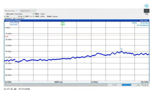
NTNV-n77(3700-3980)-PC1.5-30-15-H-DFT-QPSK-Inner_1RB_Left-6000-26000-PASS
