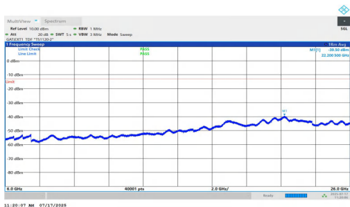
NTNV-n77(3700-3980)-PC1.5-30-20-L-DFT-BPSK-Inner_1RB_Right-6000-26000-PASS
