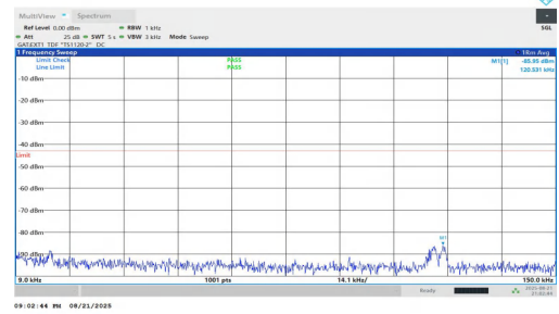
NTNV-n77(3700-3980)-PC1.5-30-15-H-DFT-QPSK-Inner_1RB_Right-0 .009-0.15-PASS
