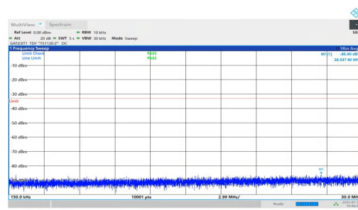
NTNV-n77(3700-3980)-PC1.5-30-15-M-DFT-QPSK-Inner_1RB_Left-0 15-30-PASS
