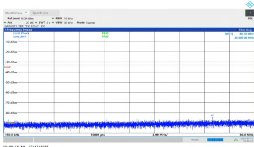
NTNV-n77(3700-3980)-PC1.5-30-15-M-DFT-BPSK-Inner_1RB_Right-0.15-30-PASS
