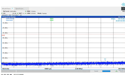
NTNV-n77(3700-3980)-PC1.5-30-15-M-DFT-QPSK-Inner_1RB_Right- 0.15-30-PASS
