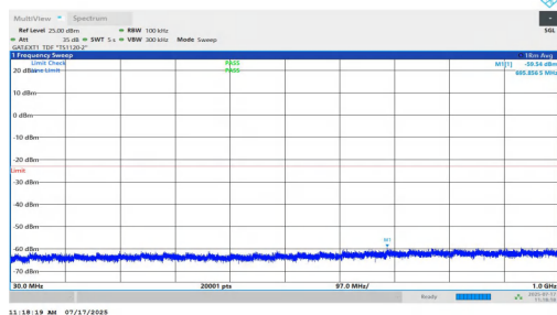
NTNV-n77(3700-3980)-PC1.5-30-20-L-DFT-BPSK-Inner_1RB_Right-3 0-1000-PASS
