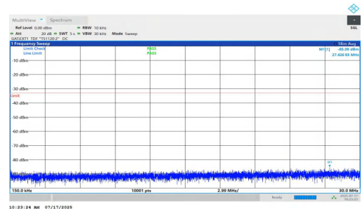
NTNV-n77(3700-3980)-PC1.5-30-15-L-DFT-BPSK-Inner_1RB_Left-0.15-5-30-PASS
