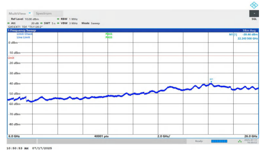
NTNV-n77(3700-3980)-PC1.5-30-15-M-DFT-QPSK-Inner_1RB_Left-60 00-26000-PASS
