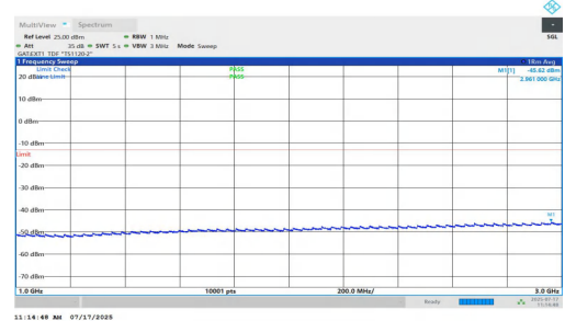
NTV-n77(3700-3980)-PC1.5-30-20-L-DFT-BPSK-Inner_1RB_Left-1000-3000-PASS
