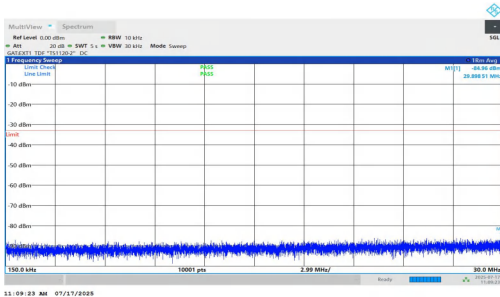
NTNV-n77(3700-3980)-PC1.5-30-15-H-DFT-QPSK-Inner_1RB_Right-0.15-30-PASS
