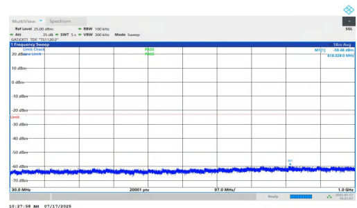
NTNV-n77(3700-3980)-PC1.5-30-15-L-DFT-BPSK-Inner_1RB_Right-3 0-1000-PASS
