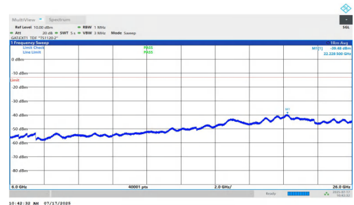
NTNV-n77(3700-3980)-PC1.5-30-15-M-DFT-BPSK-Inner_1RB_Left-6000-26000-PASS
