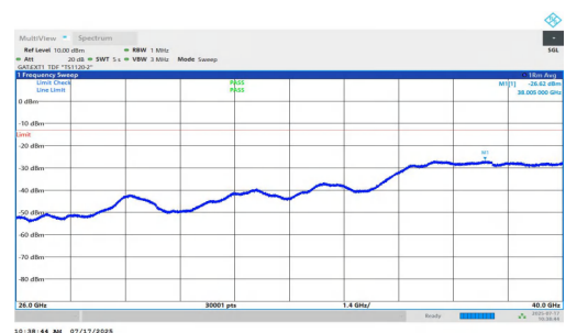
NTNV-n77(3700-3980)-PC1.5-30-15-L-DFT-QPSK-Inner_1RB_Right-2 6000-40000-PASS
