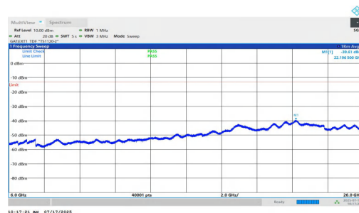
NTNV-n77(3700-3980)-PC1.5-30-10-H-DFT-QPSK-Inner_1RB_Left-60 00-26000-PASS
