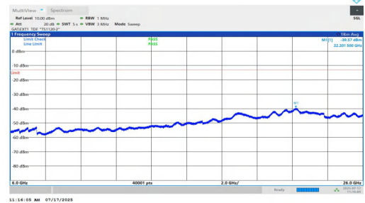
NTV-n77(3700-3980)-PC1.5-30-20-L-DFT-BPSK-Inner_1RB_Left-6000-26000-PASS
