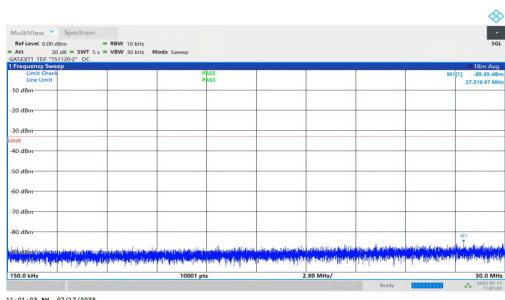
NTVN-n77(3700-3980)-PC1.5-30-15-H-DFT-BPSK-Inner_1RB_Right- 0.15-30-PASS
