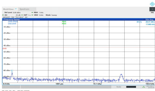
NTVN-n77(3700-3980)-PC1.5-30-15-L-DFT-QPSK-Inner_1RB_Left-0.009-0.15-PASS
