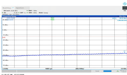
NTVN-n77(3700-3980)-PC1.5-30-15-H-DFT-BPSK-Inner_1RB_Right- 1000-3000-PASS
