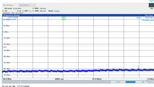
NTNV-n77(3700-3980)-PC1.5-30-10-H-DFT-QPSK-Inner_1RB_Left-3 0-1000-PASS
