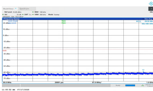
NTNV-n77(3700-3980)-PC1.5-30-15-H-DFT-QPSK-Inner_1RB_Left-30-1000-PASS
