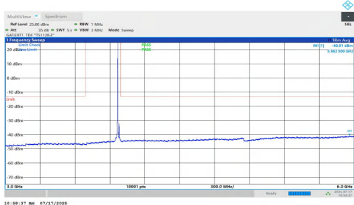
NTVN-n77(3700-3980)-PC1.5-30-15-H-DFT-BPSK-Inner_1RB_Left-3 000-6000-PASS
