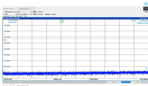
NTVN-n77(3700-3980)-PC1.5-30-15-L-DFT-QPSK-Inner_1RB_Left-0.15-5-30-PASS
