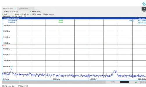
NTNV-n77(3700-3980)-PC1.5-30-15-H-DFT-QPSK-Inner_1RB_Left-0.009-0.15-PASS
