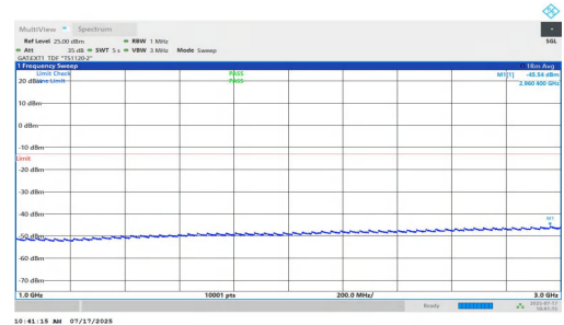
NTNV-n77(3700-3980)-PC1.5-30-15-M-DFT-BPSK-Inner_1RB_Left-1000-3000-PASS
