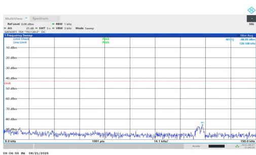
NTNV-n77(3700-3980)-PC1.5-30-20-L-DFT-QPSK-Inner_1RB_Left-0.009-0.15-PASS
