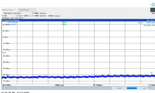
NTNV-n77(3700-3980)-PC1.5-30-15-L-DFT-BPSK-Inner_1RB_Left-30-1000-PASS
