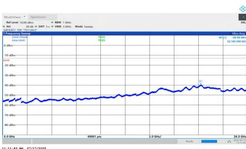
NTNV-n77(3700-3980)-PC1.5-30-15-H-DFT-QPSK-Inner_1RB_Right-6000-26000-PASS
