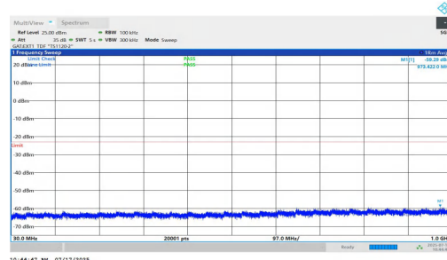
NTNV-n77(3700-3980)-PC1.5-30-15-M-DFT-BPSK-Inner_1RB_Right-3 0-1000-PASS
