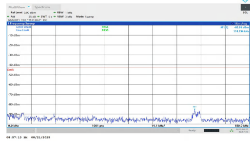
NTNV-n77(3700-3980)-PC1.5-30-15-L-DFT-QPSK-Inner_1RB_Right-0 .009-0.15-PASS
