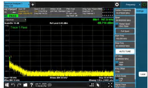
NTNV-n77(3700-3980)-PC2-30-30-L-DFT-BPSK-Inner_1RB_Left-0.15- 30-PASS
