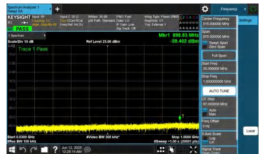
NTNV-n77(3700-3980)-PC2-30-30-M-DFT-QPSK-Inner_1RB_Right-30-1000-PASS
