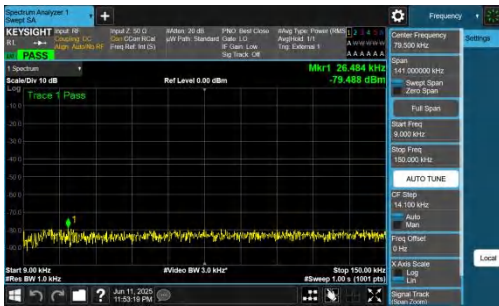
NTNV-n77(3700-3980)-PC2-30-30-L-DFT-BPSK-Inner_1RB_Left-0.00 9-0.15-PASS
