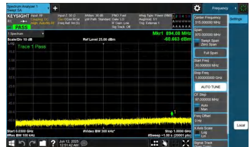
NTNV-n77(3700-3980)-PC2-30-40-L-DFT-BPSK-Inner_1RB_Right-30- 1000-PASS
