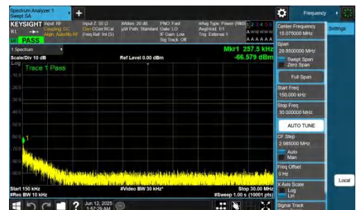
NTNV-n77(3700-3980)-PC2-30-50-M-DFT-BPSK-Inner_1RB_Left-0.15 -30-PASS
