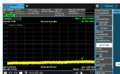
NTNV-n77(3700-3980)-PC2-30-50-L-DFT-QPSK-Inner_1RB_Right-30-1000-PASS
