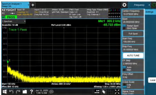
NTNV-n77(3700-3980)-PC2-30-40-M-DFT-BPSK-Inner_1RB_Right-0. 15-30-PASS
