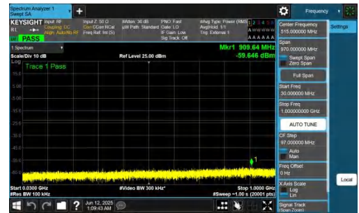
NTNV-n77(3700-3980)-PC2-30-40-M-DFT-BPSK-Inner_1RB_Right-30- 1000-PASS
