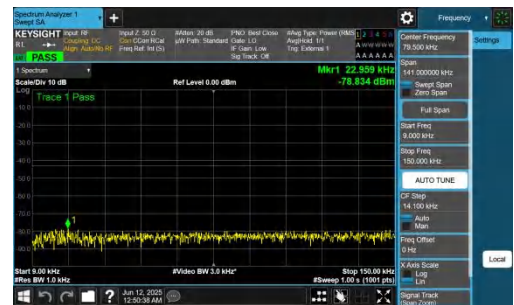
NTNV-n77(3700-3980)-PC2-30-40-L-DFT-BPSK-Inner_1RB_Right-0.0 09-0.15-PASS
