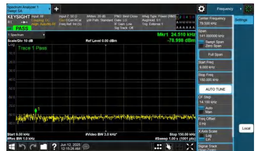
NTNV-n77(3700-3980)-PC2-30-30-M-DFT-BPSK-Inner_1RB_Right-0.0 09-0.15-PASS
