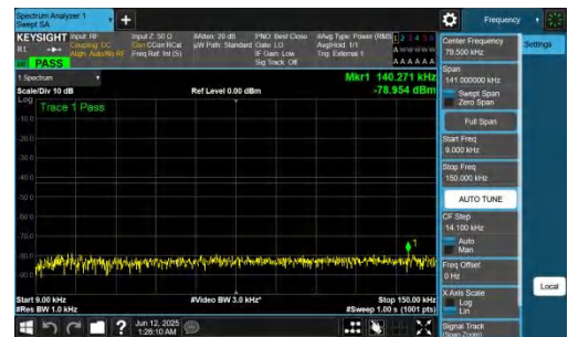
NTNV-n77(3700-3980)-PC2-30-40-H-DFT-BPSK-Inner_1RB_Right-0.0 09-0.15-PASS
