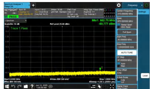
NTNV-n77(3700-3980)-PC2-30-40-L-DFT-QPSK-Inner_1RB_Right-30-1000-PASS
