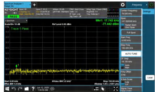
NTNV-n77(3700-3980)-PC2-30-40-H-DFT-QPSK-Inner_1RB_Right-0.0 09-0.15-PASS
