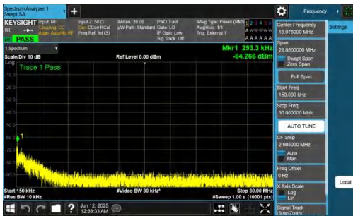
NTNV-n77(3700-3980)-PC2-30-30-H-DFT-BPSK-Inner_1RB_Right-0.15-30-PASS
