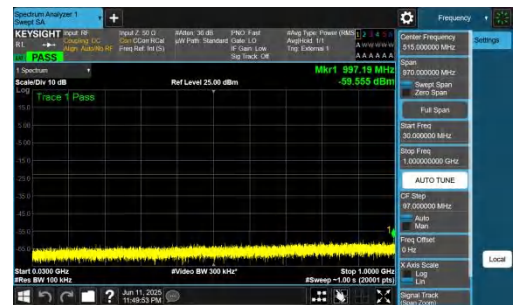
NTNV-n77(3700-3980)-PC2-30-25-H-DFT-QPSK-Inner_1RB_Right-30-1000-PASS
