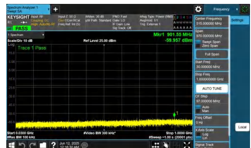
NTNV-n77(3700-3980)-PC2-30-30-M-DFT-BPSK-Inner_1RB_Right-30- 1000-PASS
