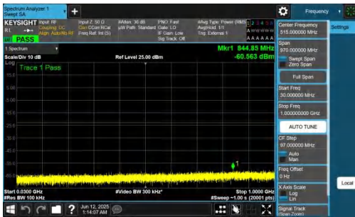
NTNV-n77(3700-3980)-PC2-30-40-M-DFT-QPSK-Inner_1RB_Left-30-1000-PASS
