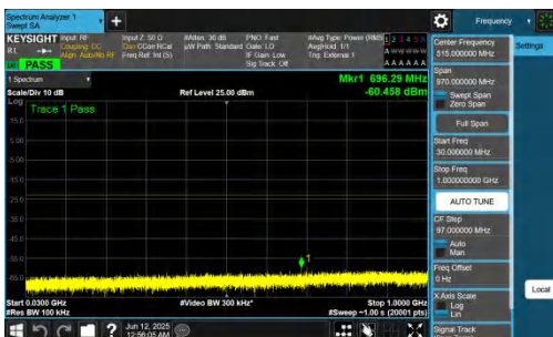
NTNV-n77(3700-3980)-PC2-30-40-L-DFT-QPSK-Inner_1RB_Left-30-1000-PASS
