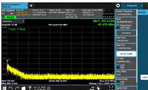
NTNV-n77(3700-3980)-PC2-30-30-M-DFT-BPSK-Inner_1RB_Right-0. 15-30-PASS
