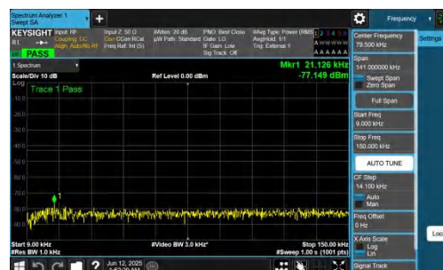
NTNV-n77(3700-3980)-PC2-30-50-L-DFT-QPSK-Inner_1RB_Right-0.009-0.15-PASS
