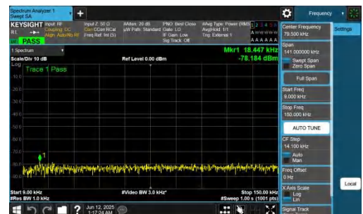
NTNV-n77(3700-3980)-PC2-30-40-M-DFT-QPSK-Inner_1RB_Right-0.09-0.15-PASS
