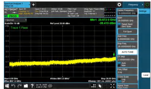
NTNV-n77(3700-3980)-PC2-30-30-M-DFT-BPSK-Inner_1RB_Left-600 0-26000-PASS
