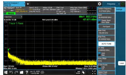
NTNV-n77(3700-3980)-PC2-30-40-M-DFT-BPSK-Inner_1RB_Left-0.15 -30-PASS
