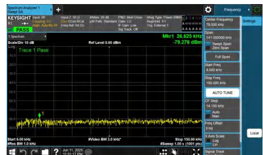
NTNV-n77(3700-3980)-PC2-30-25-M-DFT-QPSK-Inner_1RB_Right-0.09-0.15-PASS
