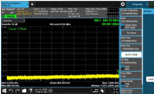
NTNV-n77(3700-3980)-PC2-30-30-H-DFT-QPSK-Inner_1RB_Left-30-1000-PASS
