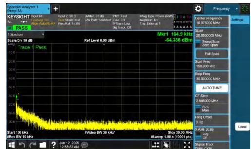
NTNV-n77(3700-3980)-PC2-30-40-L-DFT-QPSK-Inner_1RB_Left-0.15-30-PASS
