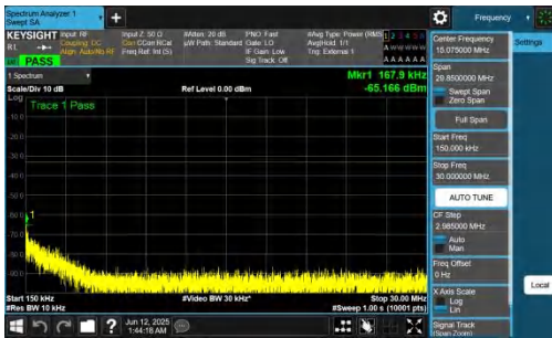
NTVN-n77(3700-3980)-PC2-30-50-L-DFT-BPSK-Inner_1RB_Right-0.15-30-PASS
