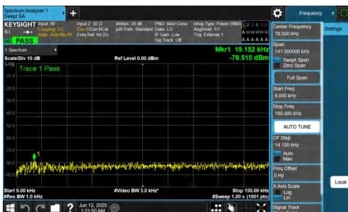
NTNV-n77(3700-3980)-PC2-30-40-H-DFT-BPSK-Inner_1RB_Left-0.009-0.15-PASS
