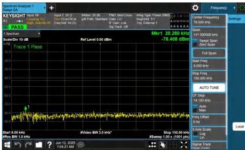
NTNV-n77(3700-3980)-PC2-30-40-M-DFT-BPSK-Inner_1RB_Left-0.0 09-0.15-PASS
