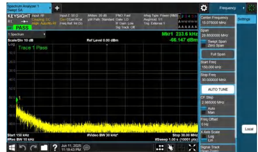
NTNV-n77(3700-3980)-PC2-30-25-M-DFT-BPSK-Inner_1RB_Left-0.15 -30-PASS
