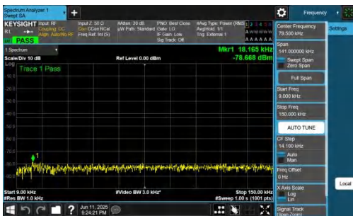
NTNV-n77(3700-3980)-PC2-30-15-L-DFT-QPSK-Inner_1RB_Left-0.009-0.15-PASS
