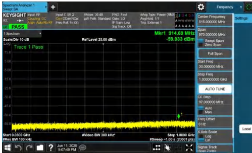
NTVN-n77(3700-3980)-PC2-30-10-H-DFT-QPSK-Inner_1RB_Left-30-1000-PASS
