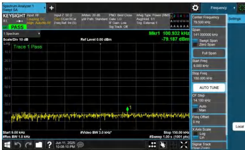
NTNV-n77(3700-3980)-PC2-30-20-L-DFT-BPSK-Inner_1RB_Left-0.00 9-0.15-PASS
