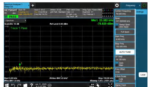
NTVN-n77(3700-3980)-PC2-30-10-H-DFT-QPSK-Inner_1RB_Right-0.09-0.15-PASS
