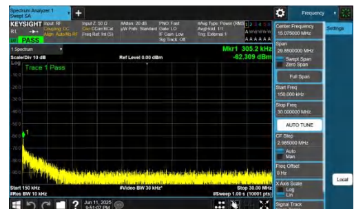
NTNV-n77(3700-3980)-PC2-30-15-H-DFT-BPSK-Inner_1RB_Left-0.15- 30-PASS
