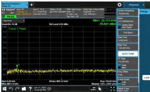
NTNV-n77(3700-3980)-PC2-30-20-H-DFT-BPSK-Inner_1RB_Left-0.0 09-0.15-PASS
