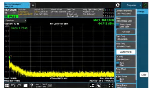
NTNV-n77(3700-3980)-PC2-30-15-L-DFT-QPSK-Inner_1RB_Left-0.15-30-PASS
