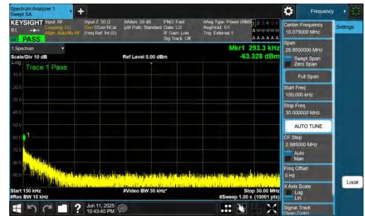
NTNV-n77(3700-3980)-PC2-30-20-H-DFT-BPSK-Inner_1RB_Left-0.15- 30-PASS
