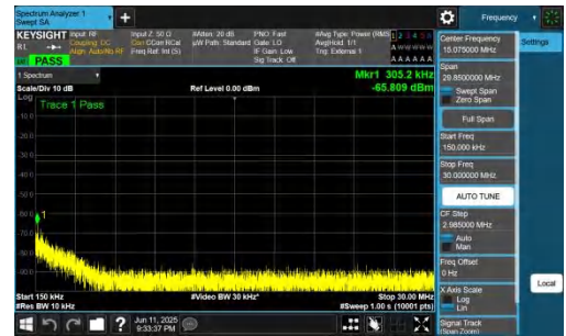
NTNV-n77(3700-3980)-PC2-30-15-M-DFT-BPSK-Inner_1RB_Left-0.15 -30-PASS
