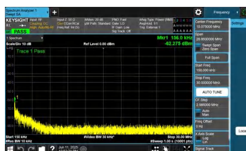
NTNV-n77(3700-3980)-PC2-30-20-H-DFT-QPSK-Inner_1RB_Left-0.15 -30-PASS
