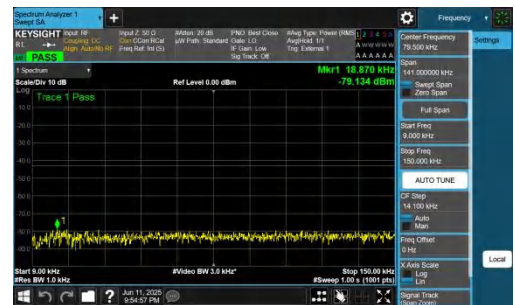
NTNV-n77(3700-3980)-PC2-30-15-H-DFT-BPSK-Inner_1RB_Right-0.0 09-0.15-PASS
