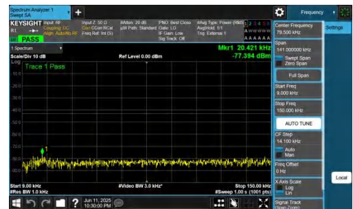
NTNV-n77(3700-3980)-PC2-30-20-M-DFT-BPSK-Inner_1RB_Right-0.0 09-0.15-PASS
