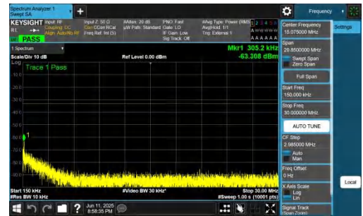
NTNV-n77(3700-3980)-PC2-30-10-H-DFT-BPSK-Inner_1RB_Left-0.15- 30-PASS
