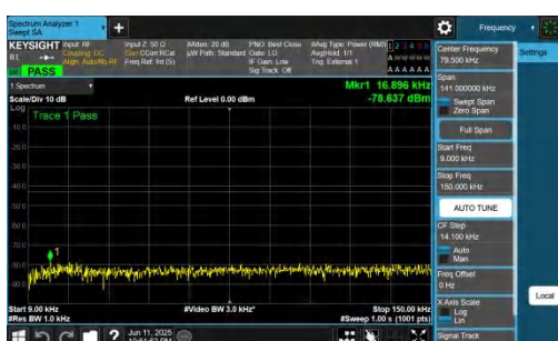
NTNV-n77(3700-3980)-PC2-30-20-H-DFT-QPSK-Inner_1RB_Left-0.0 09-0.15-PASS
