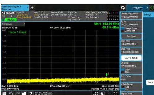
NTNV-n77(3700-3980)-PC2-30-25-L-DFT-BPSK-Inner_1RB_Left-30-1 000-PASS
