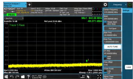
NTNV-n77(3700-3980)-PC2-30-15-L-DFT-QPSK-Inner_1RB_Right-30-1000-PASS
