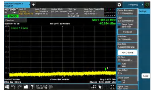
NTNV-n77(3700-3980)-PC2-30-15-M-DFT-BPSK-Inner_1RB_Right-30-1000-PASS
