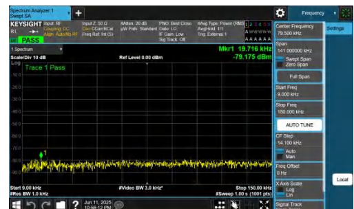
NTNV-n77(3700-3980)-PC2-30-20-H-DFT-QPSK-Inner_1RB_Right-0.009-0.15-PASS
