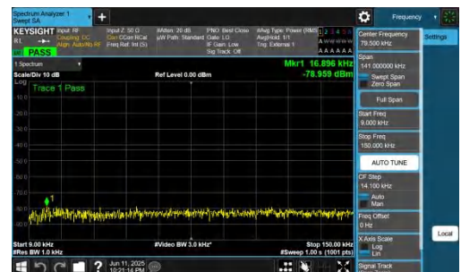
NTNV-n77(3700-3980)-PC2-30-20-L-DFT-QPSK-Inner_1RB_Right-0.0-09-0.15-PASS
