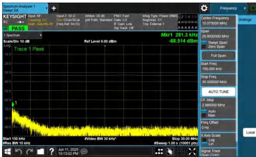
NTNV-n77(3700-3980)-PC2-30-20-L-DFT-BPSK-Inner_1RB_Right-0.15-30-PASS
