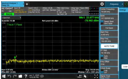
NTNV-n77(3700-3980)-PC2-30-15-M-DFT-BPSK-Inner_1RB_Left-0.0 09-0.15-PASS
