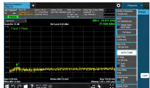
NTNV-n77(3700-3980)-PC2-30-15-M-DFT-QPSK-Inner_1RB_Right-0.09-0.15-PASS
