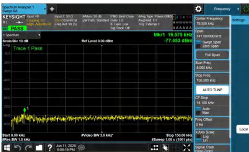
NTNV-n77(3700-3980)-PC2-30-15-H-DFT-QPSK-Inner_1RB_Left-0.009-0.15-PASS
