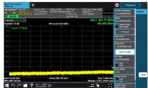
NTNV-n77(3700-3980)-PC2-30-10-M-DFT-QPSK-Inner_1RB_Right-30 -1000-PASS
