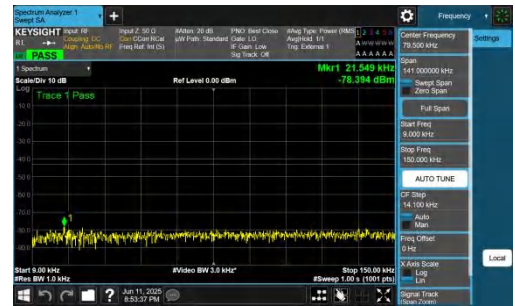
NTNV-n77(3700-3980)-PC2-30-10-M-DFT-QPSK-Inner_1RB_Right-0.0 09-0.15-PASS
