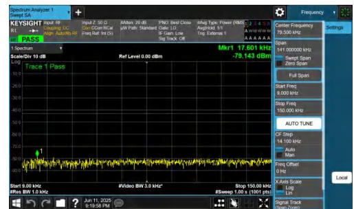
NTNV-n77(3700-3980)-PC2-30-15-L-DFT-BPSK-Inner_1RB_Right-0.0 09-0.15-PASS
