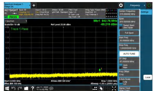
NTNV-n77(3700-3980)-PC2-30-25-L-DFT-QPSK-Inner_1RB_Right-30.30 1000-PASS
