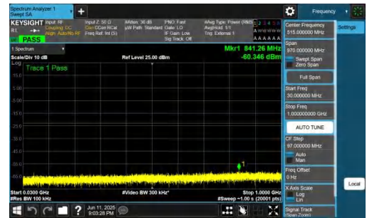
NTNV-n77(3700-3980)-PC2-30-10-H-DFT-BPSK-Inner_1RB_Right-30-1000-PASS
