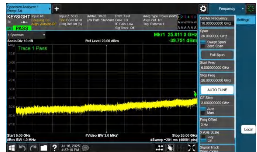
NTNV-n77(3700-3980)-PC2-30-15-M-DFT-QPSK-Inner_1RB_Left-6000-26000-PASS
