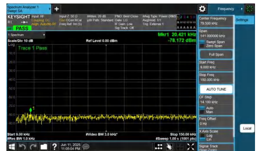
NTNV-n77(3700-3980)-PC2-30-25-L-DFT-BPSK-Inner_1RB_Right-0.0 09-0.15-PASS
