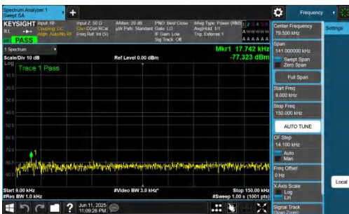
NTNV-n77(3700-3980)-PC2-30-25-L-DFT-QPSK-Inner_1RB_Left-0.009-0.15-PASS
