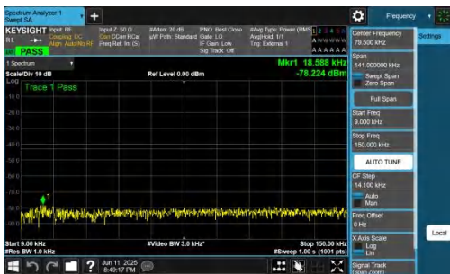
NTNV-n77(3700-3980)-PC2-30-10-M-DFT-QPSK-Inner_1RB_Left-0.009-0.15-PASS
