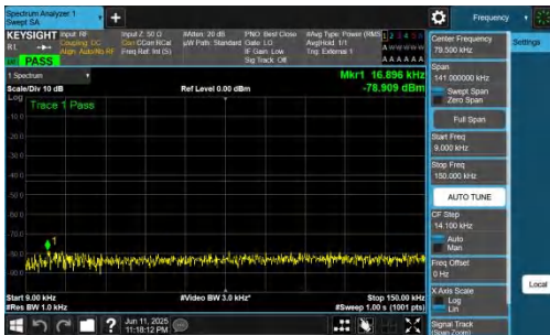
NTNV-n77(3700-3980)-PC2-30-25-M-DFT-BPSK-Inner_1RB_Left-0.0 09-0.15-PASS
