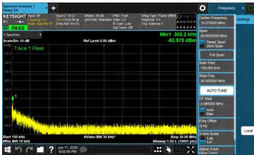
NTNV-n77(3700-3980)-PC2-30-10-H-DFT-BPSK-Inner_1RB_Right-0.15-30-PASS
