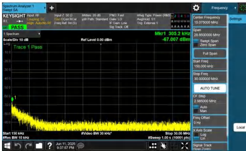
NTNV-n77(3700-3980)-PC2-30-15-M-DFT-BPSK-Inner_1RB_Right-0.15-30-PASS
