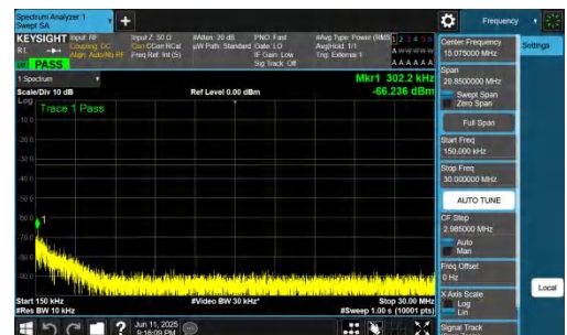
NTNV-n77(3700-3980)-PC2-30-15-L-DFT-BPSK-Inner_1RB_Left-0.15- 30-PASS
