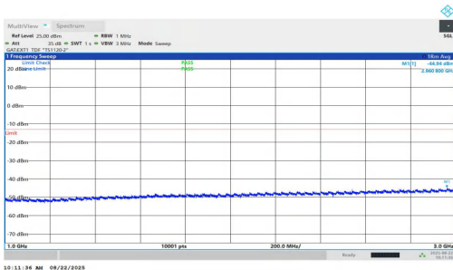
NTNV-n77(3450-3550)-PC1.5-30-100-M-DFT-QPSK-Inner_1RB_Right-t1000-3000-PASS
