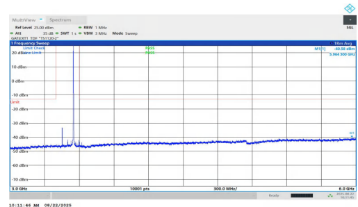
NTNV-n77(3450-3550)-PC1.5-30-100-M-DFT-QPSK-Inner_1RB_Right-3000-6000-PASS
