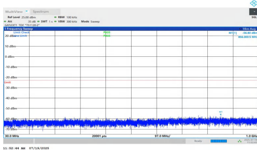
NTNV-n77(3450-3550)-PC1.5-30-90-H-DFT-BPSK-Inner_1RB_Left-3000-1000-PASS
