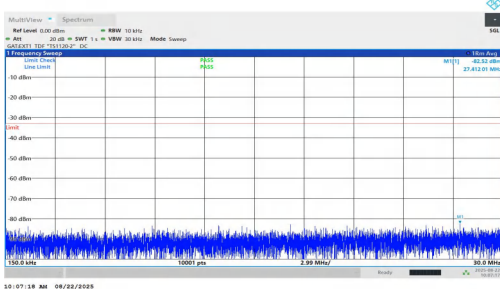
NTNV-n77(3450-3550)-PC1.5-30-100-M-DFT-BPSK-Inner_1RB_Right-0.15-30-PASS
