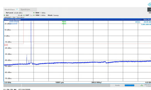
NTNV-n77(3450-3550)-PC1.5-30-90-H-DFT-BPSK-Inner_1RB_Right-3 000-6000-PASS
