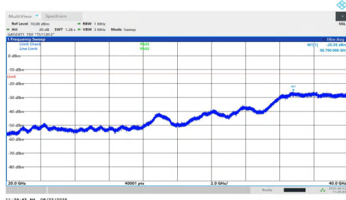
NTNV-n77(3450-3550)-PC1.5-30-100-M-DFT-BPSK-Inner_1RB_Right- 20000-40000-PASS
