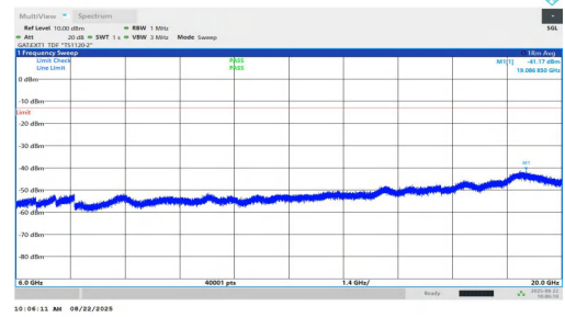
NTNV-n77(3450-3550)-PC1.5-30-100-M-DFT-BPSK-Inner_1RB_Left-6000-20000-PASS
