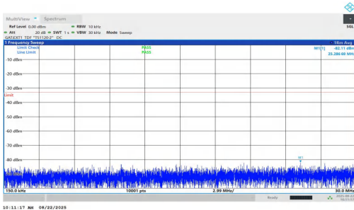
NTNV-n77(3450-3550)-PC1.5-30-100-M-DFT-QPSK-Inner_1RB_Right-t0.15-30-PASS
