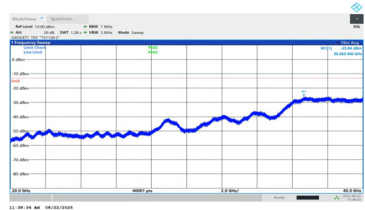
NTNV-n77(3450-3550)-PC1.5-30-90-H-DFT-QPSK-Inner_1RB_Right-20000-40000-PASS
