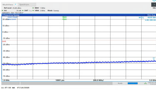
NTNV-n77(3450-3550)-PC1.5-30-90-H-DFT-QPSK-Inner_1RB_Right-1000-3000-PASS
