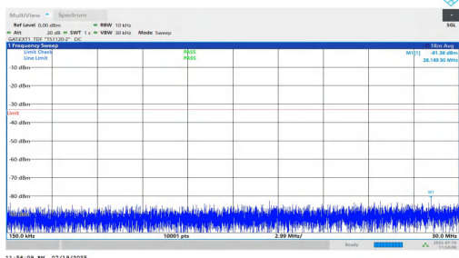
NTNV-n77(3450-3550)-PC1.5-30-90-H-DFT-BPSK-Inner_1RB_Right-0.15-30-PASS
