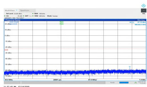
NTNV-n77(3450-3550)-PC1.5-30-90-H-DFT-QPSK-Inner_1RB_Right-3 0-1000-PASS
