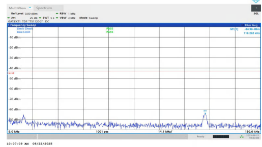
NTNV-n77(3450-3550)-PC1.5-30-100-M-DFT-BPSK-Inner_1RB_Right-0.009-0.15-PASS
