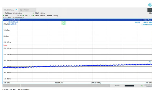
NTNV-n77(3450-3550)-PC1.5-30-100-M-DFT-QPSK-Inner_1RB_Left-1 000-3000-PASS
