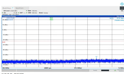
NTNV-n77(3450-3550)-PC1.5-30-100-M-DFT-QPSK-Inner_1RB_Left- 30-1000-PASS
