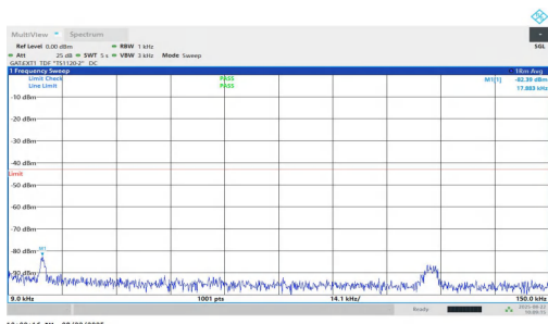
NTNV-n77(3450-3550)-PC1.5-30-100-M-DFT-QPSK-Inner_1RB_Left- 0.009-0.15-PASS
