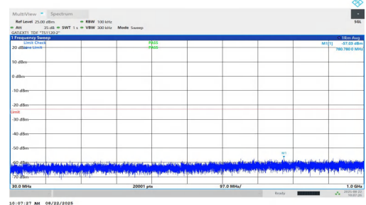
NTNV-n77(3450-3550)-PC1.5-30-100-M-DFT-BPSK-Inner_1RB_Right-30-1000-PASS
