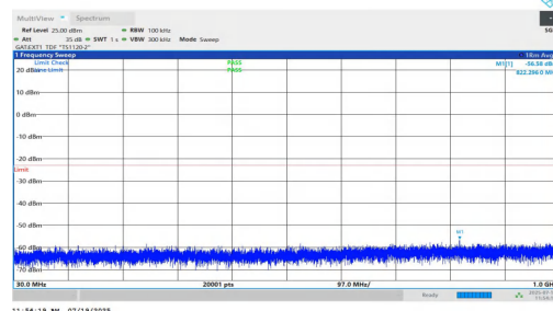
NTNV-n77(3450-3550)-PC1.5-30-90-H-DFT-BPSK-Inner_1RB_Right-3 0-1000-PASS
