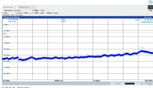
NTNV-n77(3450-3550)-PC1.5-30-100-M-DFT-BPSK-Inner_1RB_Right -6000-20000-PASS
