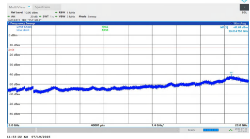
NTNV-n77(3450-3550)-PC1.5-30-90-H-DFT-BPSK-Inner_1RB_Left-6000-20000-PASS
