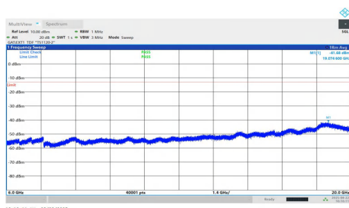
NTNV-n77(3450-3550)-PC1.5-30-100-M-DFT-QPSK-Inner_1RB_Left-6 000-20000-PASS
