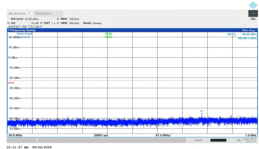
NTNV-n77(3450-3550)-PC1.5-30-100-M-DFT-QPSK-Inner_1RB_Right-30-1000-PASS
