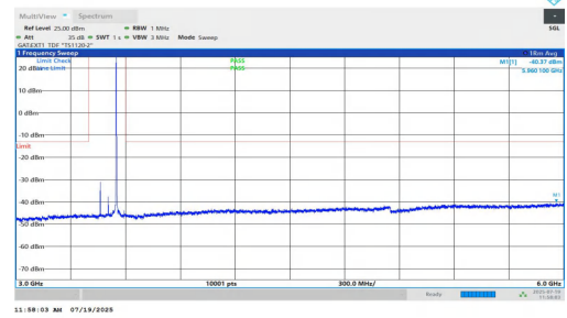
NTNV-n77(3450-3550)-PC1.5-30-90-H-DFT-QPSK-Inner_1RB_Right-3000-6000-PASS
