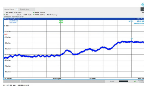
NTNV-n77(3450-3550)-PC1.5-30-90-H-DFT-BPSK-Inner_1RB_Right-2 0000-40000-PASS
