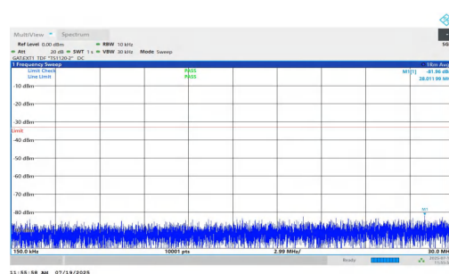
NTNV-n77(3450-3550)-PC1.5-30-90-H-DFT-QPSK-Inner_1RB_Left-0.15-30-PASS
