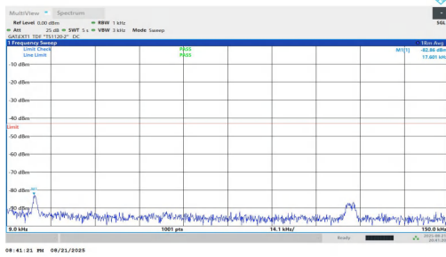
NTNV-n77(3450-3550)-PC1.5-30-90-H-DFT-BPSK-Inner_1RB_Left-0.009-0.15-PASS
