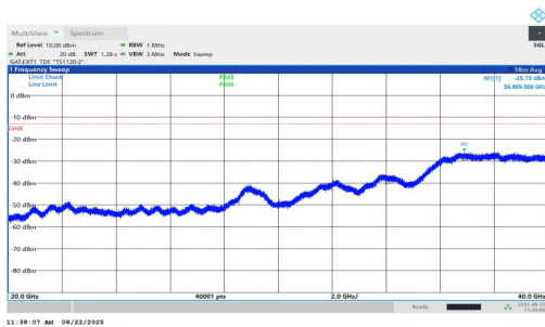
NTNV-n77(3450-3550)-PC1.5-30-90-H-DFT-QPSK-Inner_1RB_Left-2 0000-40000-PASS
