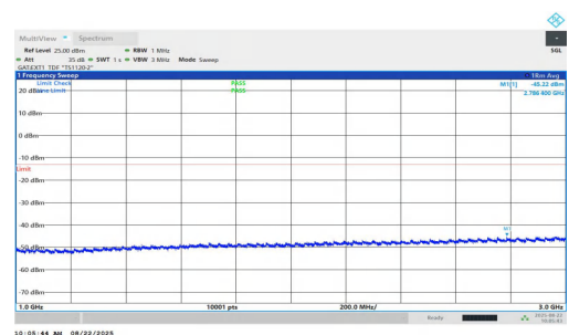
NTNV-n77(3450-3550)-PC1.5-30-100-M-DFT-BPSK-Inner_1RB_Left-1000-3000-PASS
