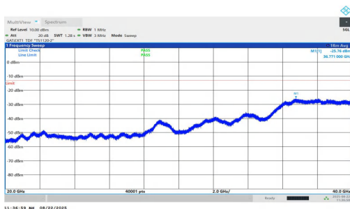
NTNV-n77(3450-3550)-PC1.5-30-90-H-DFT-BPSK-Inner_1RB_Left-20000-40000-PASS
