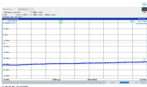
NTNV-n77(3450-3550)-PC1.5-30-90-H-DFT-BPSK-Inner_1RB_Right-1000-3000-PASS
