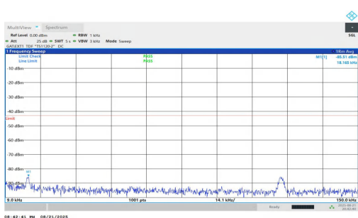
NTNV-n77(3450-3550)-PC1.5-30-90-H-DFT-QPSK-Inner_1RB_Left-0.009-0.15-PASS
