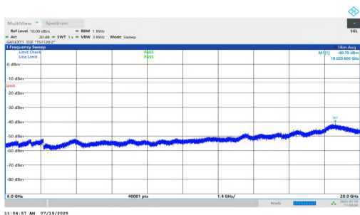
NTNV-n77(3450-3550)-PC1.5-30-90-H-DFT-BPSK-Inner_1RB_Right-6000-20000-PASS
