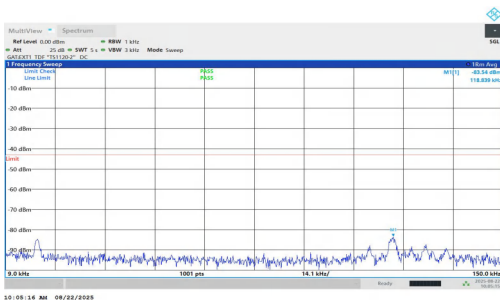
NTNV-n77(3450-3550)-PC1.5-30-100-M-DFT-BPSK-Inner_1RB_Left-0.009-0.15-PASS
