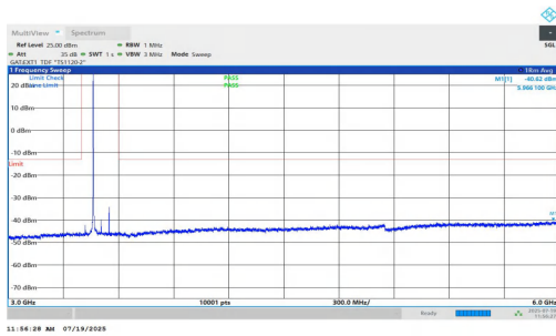
NTNV-n77(3450-3550)-PC1.5-30-90-H-DFT-QPSK-Inner_1RB_Left-3 000-6000-PASS
