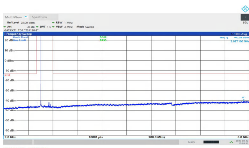
NTNV-n77(3450-3550)-PC1.5-30-100-M-DFT-QPSK-Inner_1RB_Left- 3000-6000-PASS
