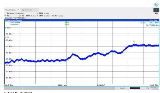
NTNV-n77(3450-3550)-PC1.5-30-100-M-DFT-QPSK-Inner_1RB_Right-20000-40000-PASS
