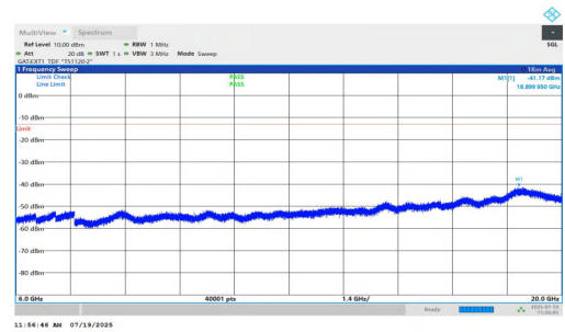
NTNV-n77(3450-3550)-PC1.5-30-90-H-DFT-QPSK-Inner_1RB_Left-60 00-20000-PASS
