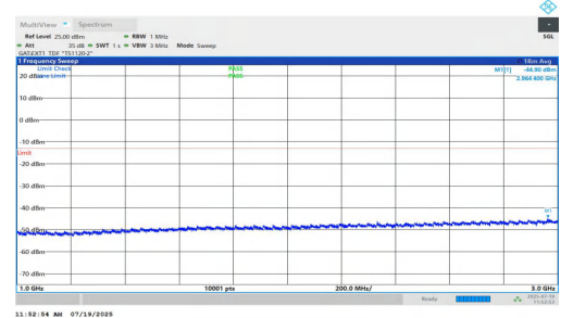
NTNV-n77(3450-3550)-PC1.5-30-90-H-DFT-BPSK-Inner_1RB_Left-1000-3000-PASS
