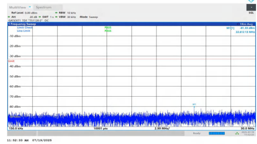
NTNV-n77(3450-3550)-PC1.5-30-90-H-DFT-BPSK-Inner_1RB_Left-0.15-30-PASS
