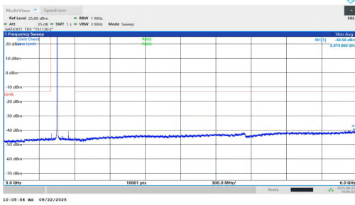
NTNV-n77(3450-3550)-PC1.5-30-100-M-DFT-BPSK-Inner_1RB_Left-3000-6000-PASS
