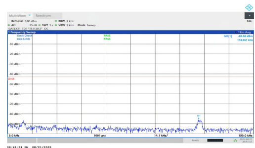
NTNV-n77(3450-3550)-PC1.5-30-90-H-DFT-BPSK-Inner_1RB_Right-0.009-0.15-PASS
