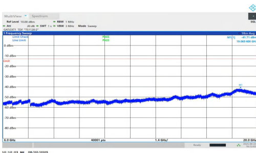
NTNV-n77(3450-3550)-PC1.5-30-100-M-DFT-QPSK-Inner_1RB_Right-t6000-20000-PASS
