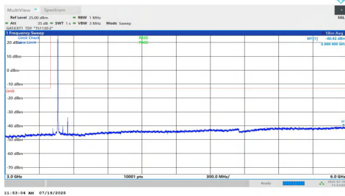
NTNV-n77(3450-3550)-PC1.5-30-90-H-DFT-BPSK-Inner_1RB_Left-3000-6000-PASS
