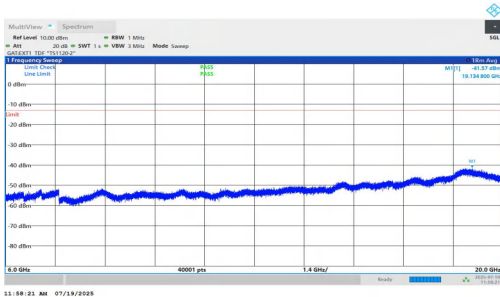
NTNV-n77(3450-3550)-PC1.5-30-90-H-DFT-QPSK-Inner_1RB_Right-6000-20000-PASS
