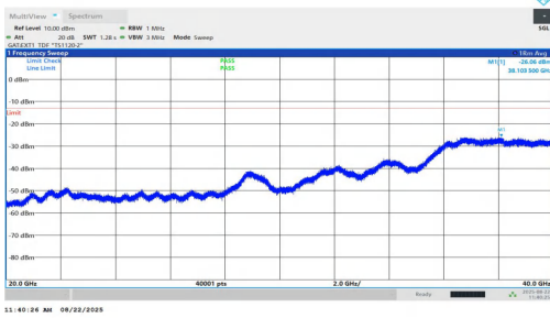
NTNV-n77(3450-3550)-PC1.5-30-100-M-DFT-QPSK-Inner_1RB_Left-20000-40000-PASS
