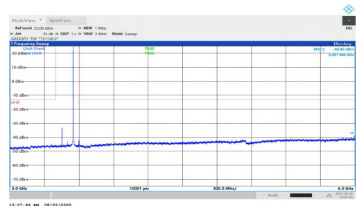
NTNV-n77(3450-3550)-PC1.5-30-100-M-DFT-BPSK-Inner_1RB_Right-3000-6000-PASS
