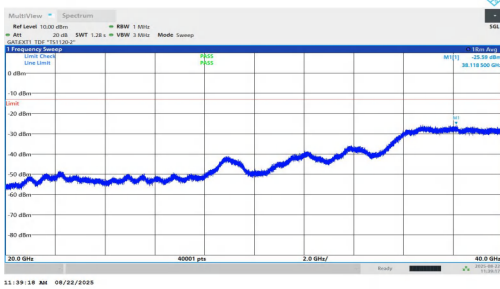
NTNV-n77(3450-3550)-PC1.5-30-100-M-DFT-BPSK-Inner_1RB_Left-20000-40000-PASS
