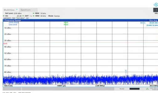
NTNV-n77(3450-3550)-PC1.5-30-100-M-DFT-QPSK-Inner_1RB_Left-0 .15-30-PASS
