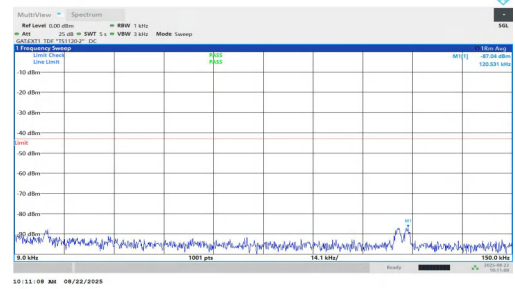
NTNV-n77(3450-3550)-PC1.5-30-100-M-DFT-QPSK-Inner_1RB_Right-0.009-0.15-PASS
