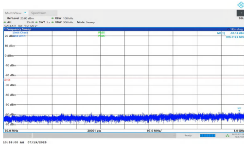
NTV-n77(3450-3550)-PC1.5-30-70-L-DFT-BPSK-Inner_1RB_Left-30-1000-PASS
