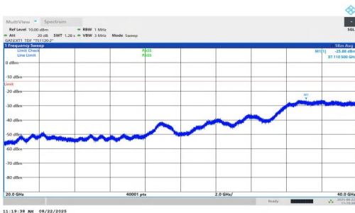
NTVN-n77(3450-3550)-PC1.5-30-70-L-DFT-QPSK-Inner_1RB_Left-2 0000-40000-PASS
