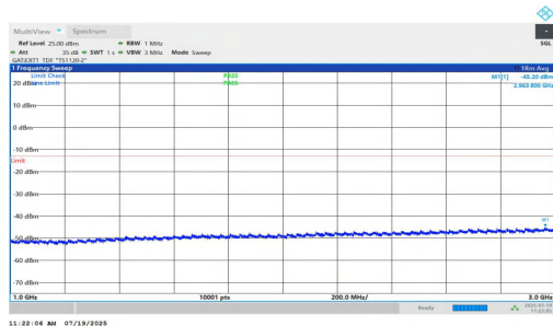
NTNV-n77(3450-3550)-PC1.5-30-80-L-DFT-QPSK-Inner_1RB_Left-1000-3000-PASS
