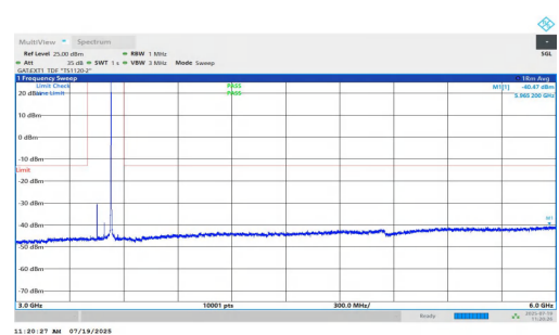
NTVN-n77(3450-3550)-PC1.5-30-80-L-DFT-BPSK-Inner_1RB_Right-3 000-6000-PASS
