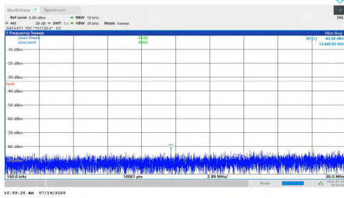
NTNV-n77(3450-3550)-PC1.5-30-70-L-DFT-BPSK-Inner_1RB_Right-0.15-30-PASS
