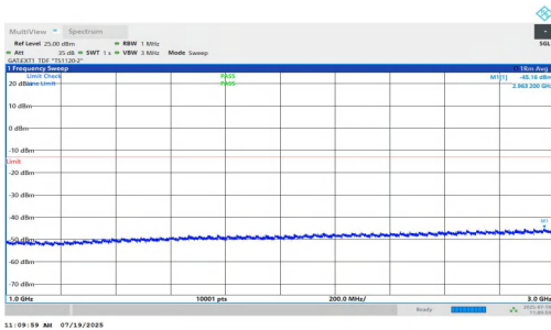
NTNV-n77(3450-3550)-PC1.5-30-70-M-DFT-QPSK-Inner_1RB_Right- 1000-3000-PASS
