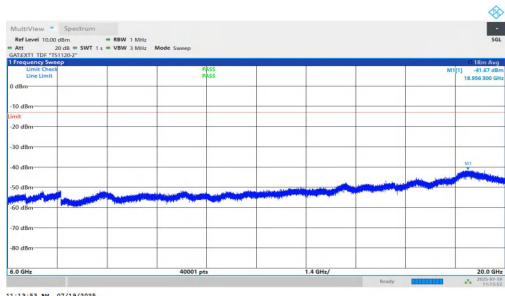
NTNV-n77(3450-3550)-PC1.5-30-70-H-DFT-BPSK-Inner_1RB_Right-6000-20000-PASS
