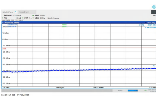
NTVN-n77(3450-3550)-PC1.5-30-80-L-DFT-BPSK-Inner_1RB_Right- 1000-3000-PASS
