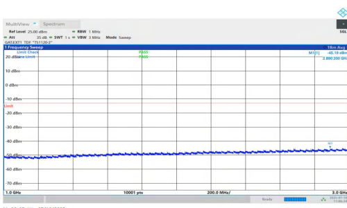
NTNV-n77(3450-3550)-PC1.5-30-70-M-DFT-BPSK-Inner_1RB_Right- 1000-3000-PASS
