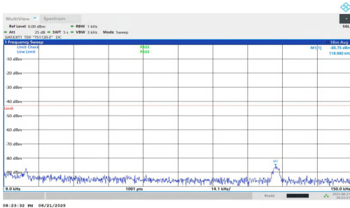
NTNV-n77(3450-3550)-PC1.5-30-70-M-DFT-QPSK-Inner_1RB_Left-0.009-0.15-PASS
