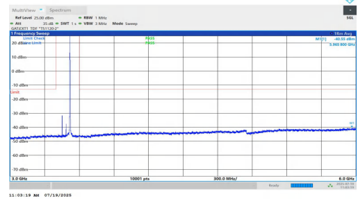
NTNV-n77(3450-3550)-PC1.5-30-70-L-DFT-QPSK-Inner_1RB_Right-3000-6000-PASS
