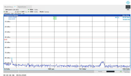
NTNV-n77(3450-3550)-PC1.5-30-70-M-DFT-BPSK-Inner_1RB_Right-0 .009-0.15-PASS
