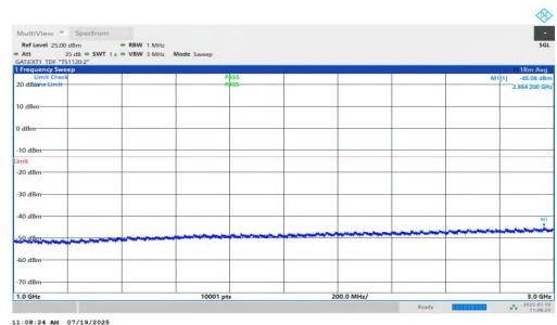
NTNV-n77(3450-3550)-PC1.5-30-70-M-DFT-QPSK-Inner_1RB_Left-1000-3000-PASS
