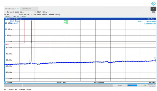
NTNV-n77(3450-3550)-PC1.5-30-70-M-DFT-QPSK-Inner_1RB_Right- 3000-6000-PASS
