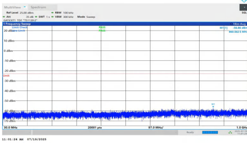
NTVN-n77(3450-3550)-PC1.5-30-70-L-DFT-QPSK-Inner_1RB_Left-3 0-1000-PASS
