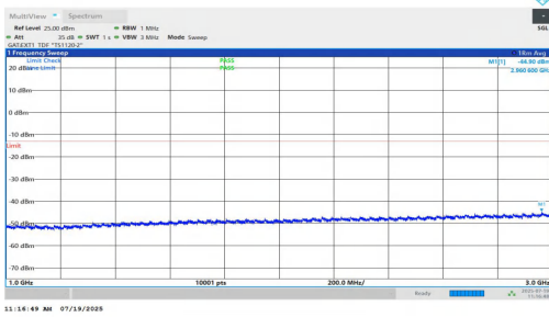
NTNV-n77(3450-3550)-PC1.5-30-70-H-DFT-QPSK-Inner_1RB_Right-1000-3000-PASS
