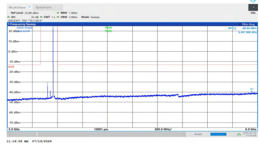
NTNV-n77(3450-3550)-PC1.5-30-70-H-DFT-QPSK-Inner_1RB_Right-3000-6000-PASS
