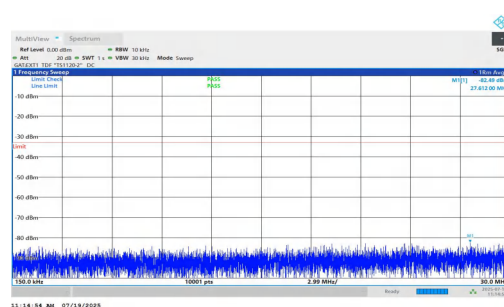
NTNV-n77(3450-3550)-PC1.5-30-70-H-DFT-QPSK-Inner_1RB_Left-0.15-30-PASS
