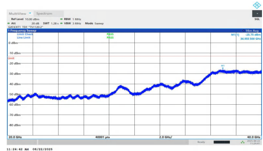
NTNV-n77(3450-3550)-PC1.5-30-70-H-DFT-QPSK-Inner_1RB_Right-20000-40000-PASS
