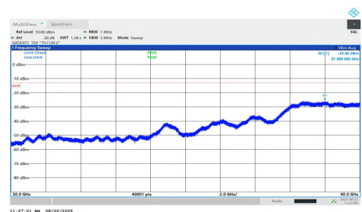
NTNV-n77(3450-3550)-PC1.5-30-80-L-DFT-QPSK-Inner_1RB_Right-2 0000-40000-PASS
