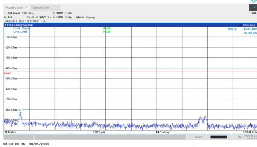
NTV-n77(3450-3550)-PC1.5-30-70-L-DFT-BPSK-Inner_1RB_Left-0.009-0.15-PASS
