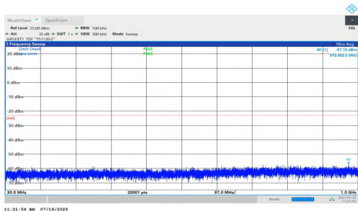
NTNV-n77(3450-3550)-PC1.5-30-80-L-DFT-QPSK-Inner_1RB_Left-30-1000-PASS
