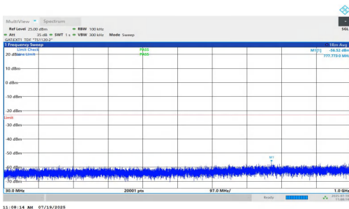
NTNV-n77(3450-3550)-PC1.5-30-70-M-DFT-QPSK-Inner_1RB_Left-30-1000-PASS
