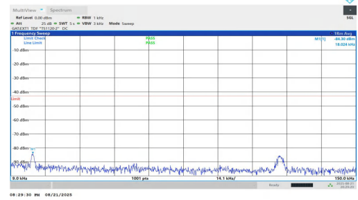
NTNV-n77(3450-3550)-PC1.5-30-80-L-DFT-QPSK-Inner_1RB_Right-0 .009-0.15-PASS
