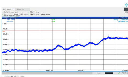
NTNV-n77(3450-3550)-PC1.5-30-70-H-DFT-BPSK-Inner_1RB_Left-20000-40000-PASS
