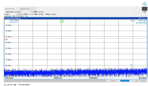
NTNV-n77(3450-3550)-PC1.5-30-80-L-DFT-BPSK-Inner_1RB_Left-0.15-5-30-PASS
