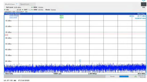
NTV-n77(3450-3550)-PC1.5-30-70-L-DFT-BPSK-Inner_1RB_Left-0.15-30-PASS
