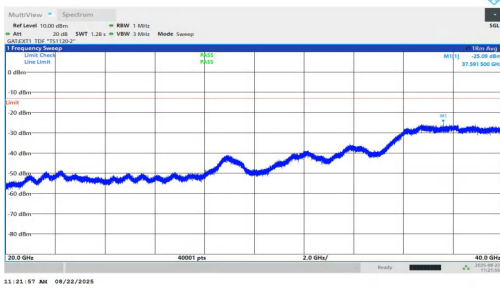
NTNV-n77(3450-3550)-PC1.5-30-70-M-DFT-QPSK-Inner_1RB_Left-2 0000-40000-PASS
