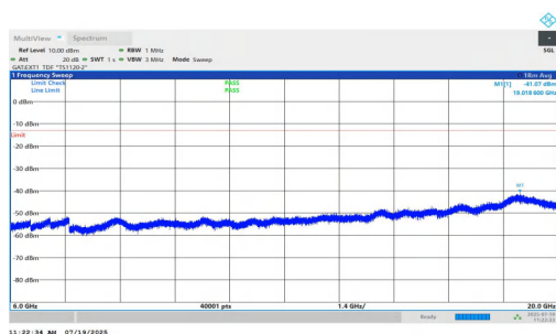
NTNV-n77(3450-3550)-PC1.5-30-80-L-DFT-QPSK-Inner_1RB_Left-6000-20000-PASS
