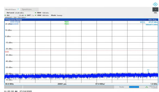
NTVN-n77(3450-3550)-PC1.5-30-80-L-DFT-BPSK-Inner_1RB_Right-3 0-1000-PASS
