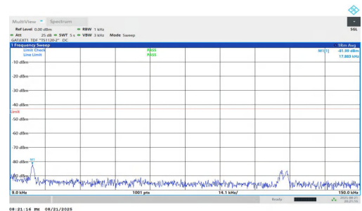
NTVN-n77(3450-3550)-PC1.5-30-70-L-DFT-QPSK-Inner_1RB_Right-0 .009-0.15-PASS
