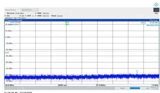
NTNV-n77(3450-3550)-PC1.5-30-70-H-DFT-QPSK-Inner_1RB_Right-3 0-1000-PASS
