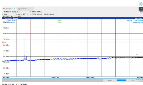
NTNV-n77(3450-3550)-PC1.5-30-70-H-DFT-BPSK-Inner_1RB_Left-3000-6000-PASS
