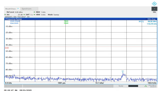
NTNV-n77(3450-3550)-PC1.5-30-70-H-DFT-QPSK-Inner_1RB_Right-0 .009-0.15-PASS
