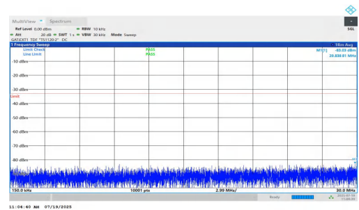
NTNV-n77(3450-3550)-PC1.5-30-70-M-DFT-BPSK-Inner_1RB_Left-0.15-30-PASS
