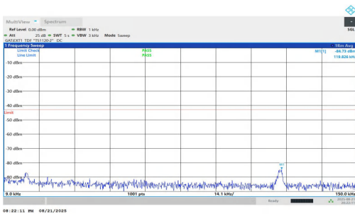
NTNV-n77(3450-3550)-PC1.5-30-70-M-DFT-BPSK-Inner_1RB_Left-0.009-0.15-PASS
