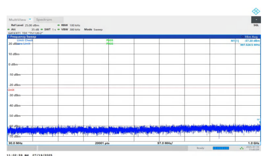
NTVN-n77(3450-3550)-PC1.5-30-70-L-DFT-QPSK-Inner_1RB_Right-3 0-1000-PASS
