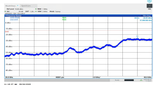
NTNV-n77(3450-3550)-PC1.5-30-70-L-DFT-BPSK-Inner_1RB_Right-2 0000-40000-PASS
