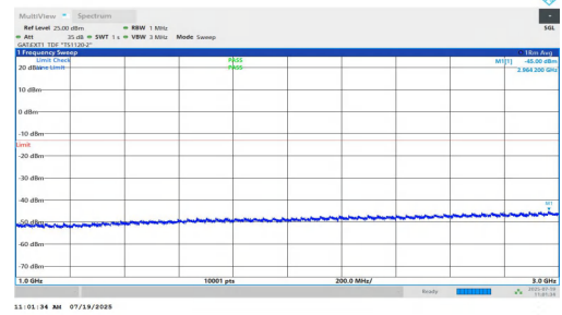
NTVN-n77(3450-3550)-PC1.5-30-70-L-DFT-QPSK-Inner_1RB_Left-10 00-3000-PASS
