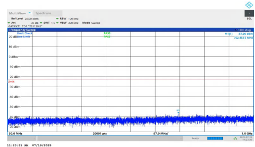
NTNV-n77(3450-3550)-PC1.5-30-80-L-DFT-QPSK-Inner_1RB_Right-3 0-1000-PASS
