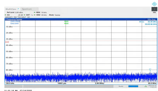
NTNV-n77(3450-3550)-PC1.5-30-70-L-DFT-QPSK-Inner_1RB_Left-0.1 5-30-PASS
