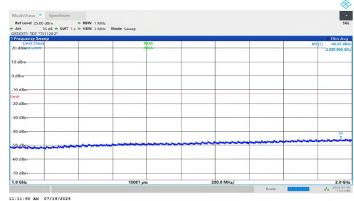
NTNV-n77(3450-3550)-PC1.5-30-70-H-DFT-BPSK-Inner_1RB_Left-1000-3000-PASS
