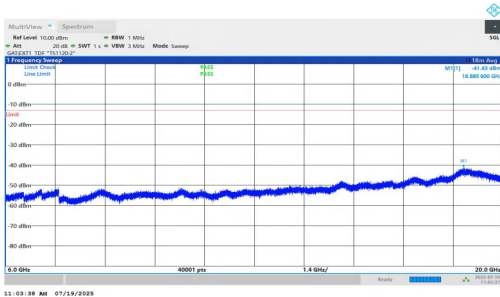
NTNV-n77(3450-3550)-PC1.5-30-70-L-DFT-QPSK-Inner_1RB_Right-6000-20000-PASS
