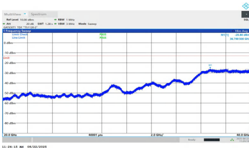
NTNV-n77(3450-3550)-PC1.5-30-70-H-DFT-QPSK-Inner_1RB_Left-2 0000-40000-PASS
