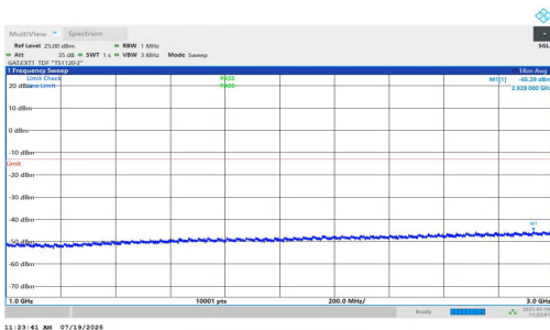
NTNV-n77(3450-3550)-PC1.5-30-80-L-DFT-QPSK-Inner_1RB_Right- 1000-3000-PASS
