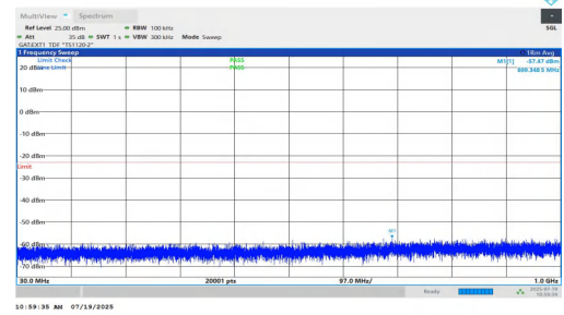
NTNV-n77(3450-3550)-PC1.5-30-70-L-DFT-BPSK-Inner_1RB_Right-3 0-1000-PASS
