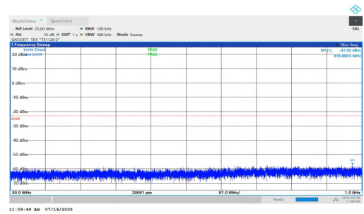
NTNV-n77(3450-3550)-PC1.5-30-70-M-DFT-QPSK-Inner_1RB_Right- 30-1000-PASS
