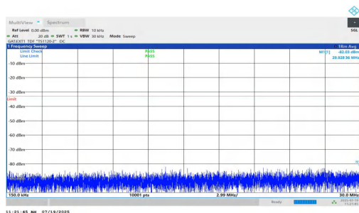
NTNV-n77(3450-3550)-PC1.5-30-80-L-DFT-QPSK-Inner_1RB_Left-0.15-5-30-PASS
