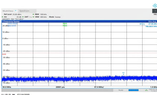
NTNV-n77(3450-3550)-PC1.5-30-80-L-DFT-BPSK-Inner_1RB_Left-30-1000-PASS
