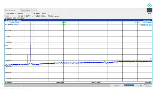
NTNV-n77(3450-3550)-PC1.5-30-70-M-DFT-BPSK-Inner_1RB_Right-3 000-6000-PASS
