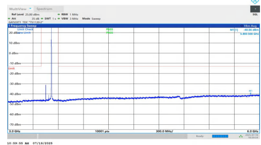
NTNV-n77(3450-3550)-PC1.5-30-70-L-DFT-BPSK-Inner_1RB_Right-3 000-6000-PASS
