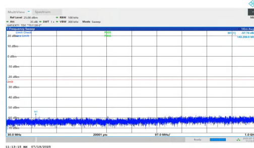
NTNV-n77(3450-3550)-PC1.5-30-70-H-DFT-BPSK-Inner_1RB_Right-3 0-1000-PASS
