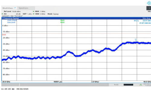
NTVN-n77(3450-3550)-PC1.5-30-80-L-DFT-BPSK-Inner_1RB_Left-20 000-40000-PASS
