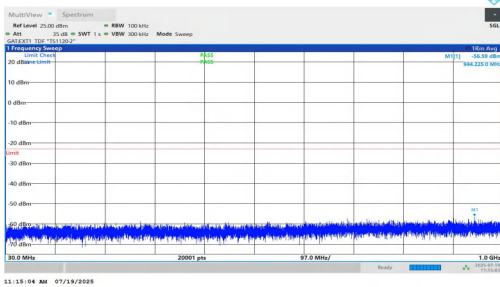
NTNV-n77(3450-3550)-PC1.5-30-70-H-DFT-QPSK-Inner_1RB_Left-3 0-1000-PASS
