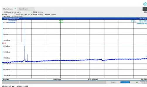
NTV-n77(3450-3550)-PC1.5-30-70-L-DFT-BPSK-Inner_1RB_Left-3000-6000-PASS
