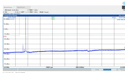
NTNV-n77(3450-3550)-PC1.5-30-70-H-DFT-BPSK-Inner_1RB_Right-3 000-6000-PASS
