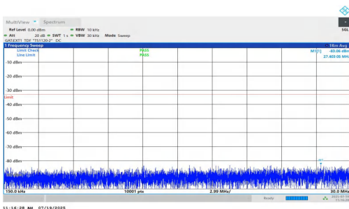
NTNV-n77(3450-3550)-PC1.5-30-70-H-DFT-QPSK-Inner_1RB_Right- 0.15-30-PASS
