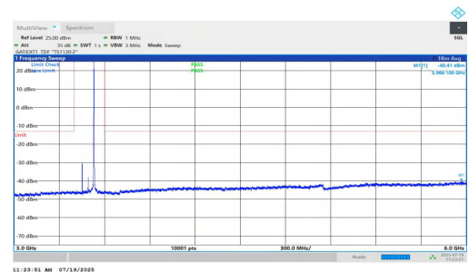
NTNV-n77(3450-3550)-PC1.5-30-80-L-DFT-QPSK-Inner_1RB_Right-3 000-6000-PASS
