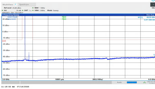
NTVN-n77(3450-3550)-PC1.5-30-80-L-DFT-BPSK-Inner_1RB_Left-30 00-6000-PASS
