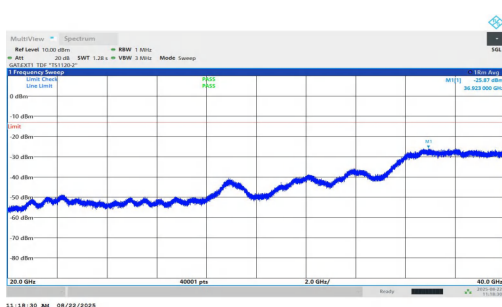
NTV-n77(3450-3550)-PC1.5-30-70-L-DFT-BPSK-Inner_1RB_Left-20000-40000-PASS
