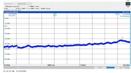
NTVN-n77(3450-3550)-PC1.5-30-80-L-DFT-BPSK-Inner_1RB_Left-60 00-20000-PASS
