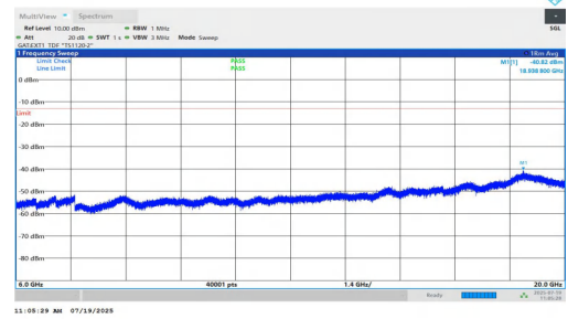
NTNV-n77(3450-3550)-PC1.5-30-70-M-DFT-BPSK-Inner_1RB_Left-60 00-20000-PASS
