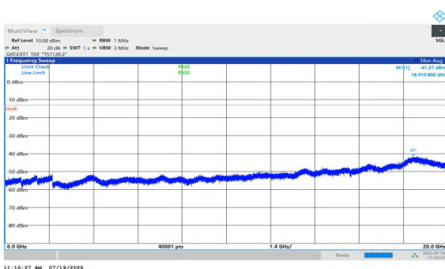
NTNV-n77(3450-3550)-PC1.5-30-70-M-DFT-QPSK-Inner_1RB_Right- 6000-20000-PASS
