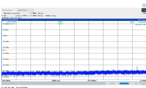
NTNV-n77(3450-3550)-PC1.5-30-70-M-DFT-BPSK-Inner_1RB_Left-30-1000-PASS
