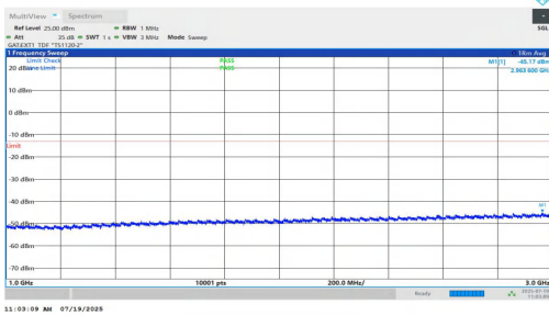
NTNV-n77(3450-3550)-PC1.5-30-70-L-DFT-QPSK-Inner_1RB_Right-1000-3000-PASS
