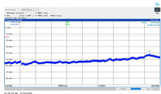
NTV-n77(3450-3550)-PC1.5-30-70-L-DFT-BPSK-Inner_1RB_Left-6000-20000-PASS
