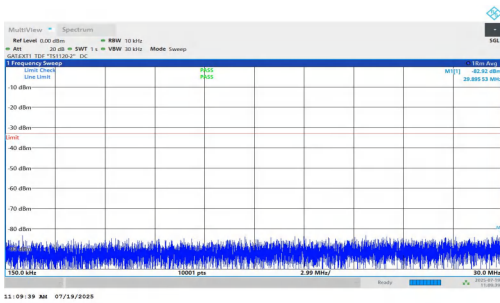
NTNV-n77(3450-3550)-PC1.5-30-70-M-DFT-QPSK-Inner_1RB_Right- 0.15-30-PASS
