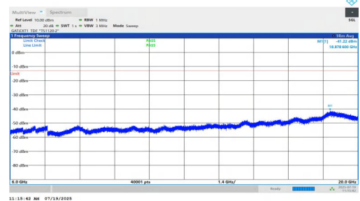
NTNV-n77(3450-3550)-PC1.5-30-70-H-DFT-QPSK-Inner_1RB_Left-60 00-20000-PASS
