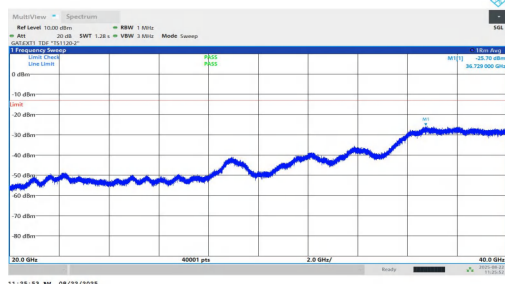
NTNV-n77(3450-3550)-PC1.5-30-80-L-DFT-BPSK-Inner_1RB_Right-20000-40000-PASS
