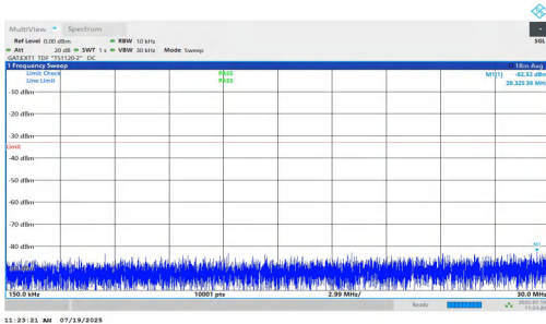
NTNV-n77(3450-3550)-PC1.5-30-80-L-DFT-QPSK-Inner_1RB_Right- 0.15-30-PASS
