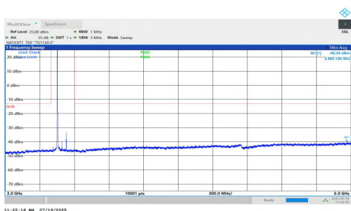
NTNV-n77(3450-3550)-PC1.5-30-80-L-DFT-QPSK-Inner_1RB_Left-3000-6000-PASS
