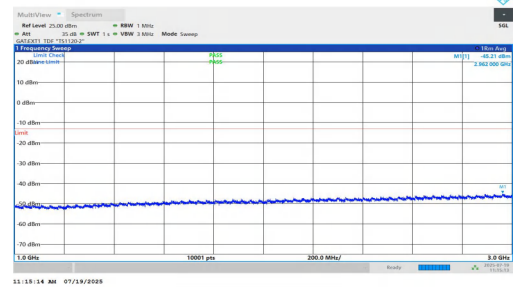
NTNV-n77(3450-3550)-PC1.5-30-70-H-DFT-QPSK-Inner_1RB_Left-10 00-3000-PASS
