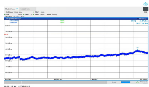
NTNV-n77(3450-3550)-PC1.5-30-70-H-DFT-BPSK-Inner_1RB_Left-6000-20000-PASS
