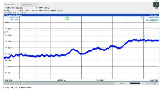
NTNV-n77(3450-3550)-PC1.5-30-70-M-DFT-BPSK-Inner_1RB_Right-20000-40000-PASS
