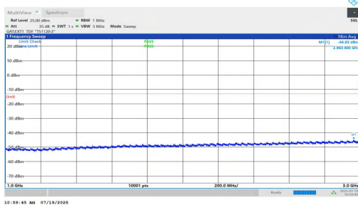
NTNV-n77(3450-3550)-PC1.5-30-70-L-DFT-BPSK-Inner_1RB_Right-1000-3000-PASS
