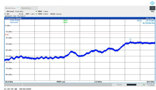
NTNV-n77(3450-3550)-PC1.5-30-70-L-DFT-QPSK-Inner_1RB_Right-20000-40000-PASS
