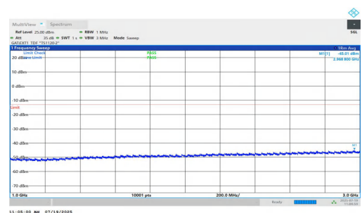
NTNV-n77(3450-3550)-PC1.5-30-70-M-DFT-BPSK-Inner_1RB_Left-1000-3000-PASS
