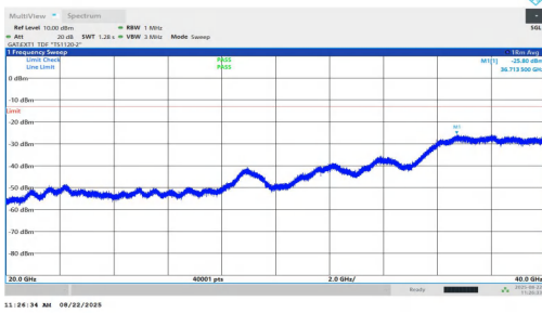
NTNV-n77(3450-3550)-PC1.5-30-80-L-DFT-QPSK-Inner_1RB_Left-2 0000-40000-PASS
