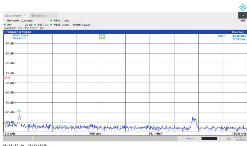
NTNV-n77(3450-3550)-PC1.5-30-80-L-DFT-QPSK-Inner_1RB_Left-0.009-0.15-PASS
