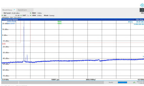
NTNV-n77(3450-3550)-PC1.5-30-70-M-DFT-QPSK-Inner_1RB_Left-3000-6000-PASS
