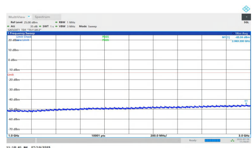
NTNV-n77(3450-3550)-PC1.5-30-80-L-DFT-BPSK-Inner_1RB_Left-1000-3000-PASS
