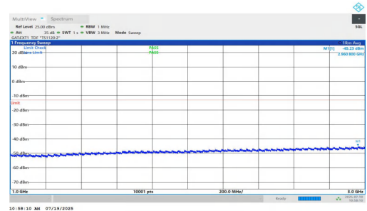
NTV-n77(3450-3550)-PC1.5-30-70-L-DFT-BPSK-Inner_1RB_Left-1000-3000-PASS
