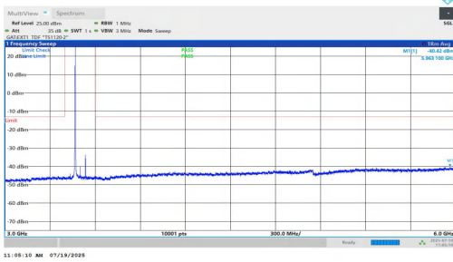
NTNV-n77(3450-3550)-PC1.5-30-70-M-DFT-BPSK-Inner_1RB_Left-3 000-6000-PASS
