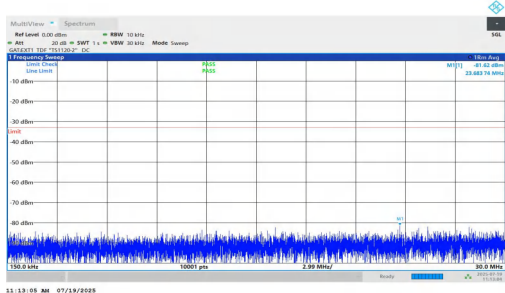
NTNV-n77(3450-3550)-PC1.5-30-70-H-DFT-BPSK-Inner_1RB_Right-0.15-30-PASS
