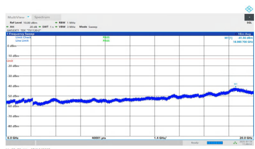
NTNV-n77(3450-3550)-PC1.5-30-70-M-DFT-QPSK-Inner_1RB_Left-6000-20000-PASS
