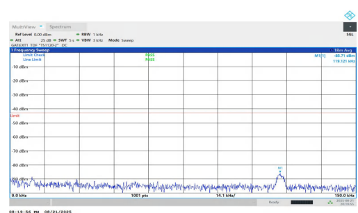
NTV-n77(3450-3550)-PC1.5-30-70-L-DFT-BPSK-Inner_1RB_Right-0.009-0.15-PASS
