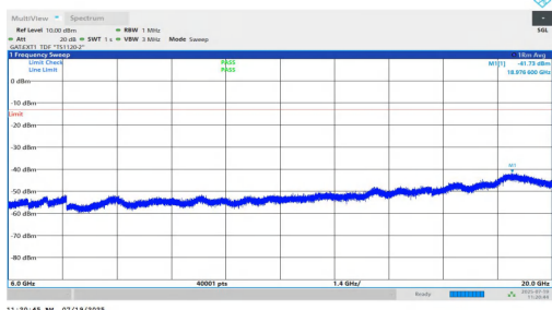
NTNV-n77(3450-3550)-PC1.5-30-80-L-DFT-BPSK-Inner_1RB_Right-6000-20000-PASS
