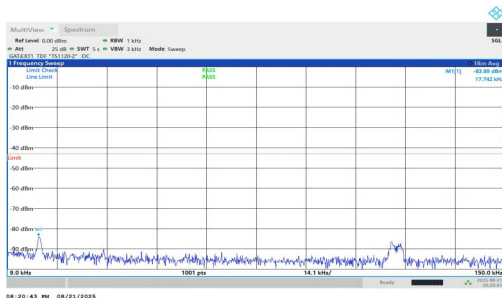
NTNV-n77(3450-3550)-PC1.5-30-70-L-DFT-QPSK-Inner_1RB_Left-0.009-0.15-PASS
