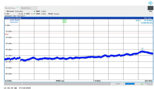
NTVN-n77(3450-3550)-PC1.5-30-70-L-DFT-QPSK-Inner_1RB_Left-60 00-20000-PASS
