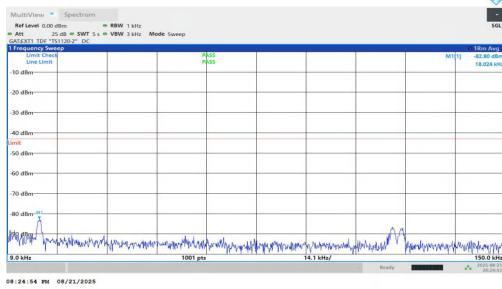
NTNV-n77(3450-3550)-PC1.5-30-70-H-DFT-BPSK-Inner_1RB_Left-0.009-0.15-PASS
