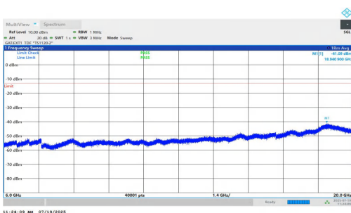
NTNV-n77(3450-3550)-PC1.5-30-80-L-DFT-QPSK-Inner_1RB_Right- 6000-20000-PASS
