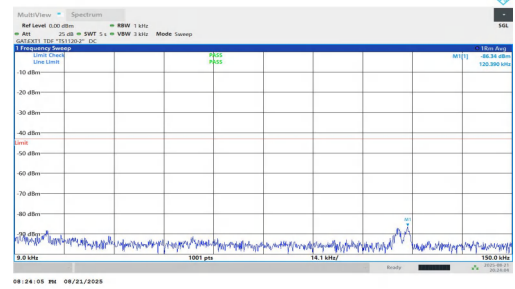
NTNV-n77(3450-3550)-PC1.5-30-70-M-DFT-QPSK-Inner_1RB_Right- 0.009-0.15-PASS
