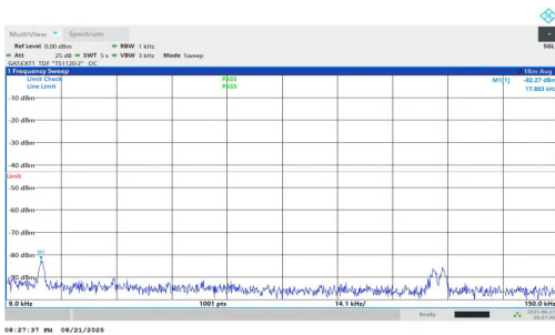
NTNV-n77(3450-3550)-PC1.5-30-80-L-DFT-BPSK-Inner_1RB_Left-0.009-0.15-PASS
