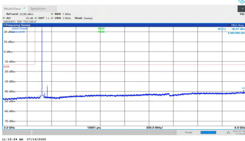
NTNV-n77(3450-3550)-PC1.5-30-70-H-DFT-QPSK-Inner_1RB_Left-3 000-6000-PASS
