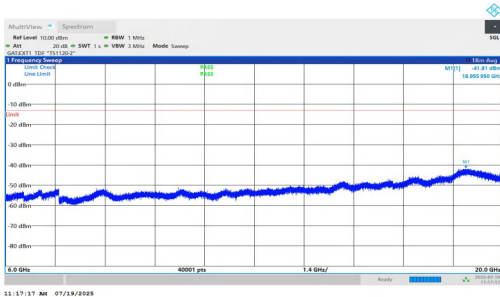
NTNV-n77(3450-3550)-PC1.5-30-70-H-DFT-QPSK-Inner_1RB_Right-6000-20000-PASS
