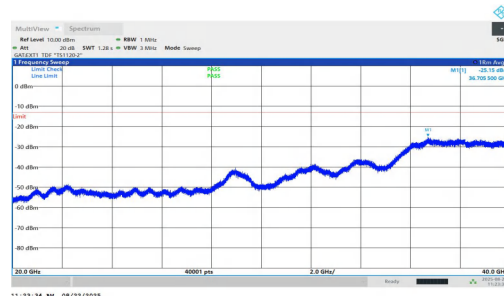
NTNV-n77(3450-3550)-PC1.5-30-70-H-DFT-BPSK-Inner_1RB_Right-2 0000-40000-PASS
