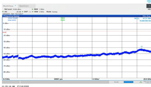
NTNV-n77(3450-3550)-PC1.5-30-70-L-DFT-BPSK-Inner_1RB_Right-6000-20000-PASS
