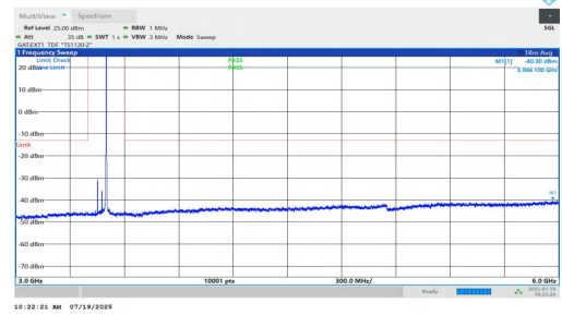
NTNV-n77(3450-3550)-PC1.5-30-50-L-DFT-QPSK-Inner_1RB_Right-3000-6000-PASS
