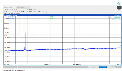
NTNV-n77(3450-3550)-PC1.5-30-40-H-DFT-QPSK-Inner_1RB_Right-3 000-6000-PASS
