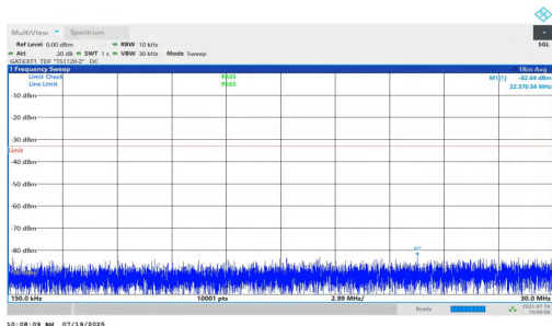
NTNV-n77(3450-3550)-PC1.5-30-40-M-DFT-QPSK-Inner_1RB_Right- 0.15-30-PASS
