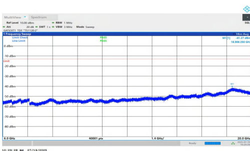
NTNV-n77(3450-3550)-PC1.5-30-50-M-DFT-QPSK-Inner_1RB_Right- 6000-20000-PASS
