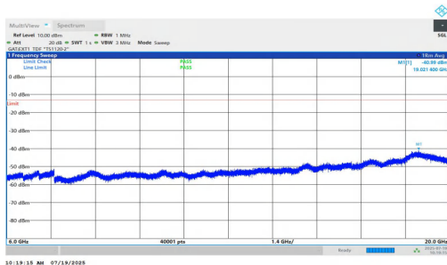
NTNV-n77(3450-3550)-PC1.5-30-50-L-DFT-BPSK-Inner_1RB_Right-6000-20000-PASS
