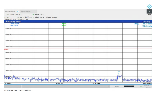
NTNV-n77(3450-3550)-PC1.5-30-40-M-DFT-BPSK-Inner_1RB_Right-0.009-0.15-PASS
