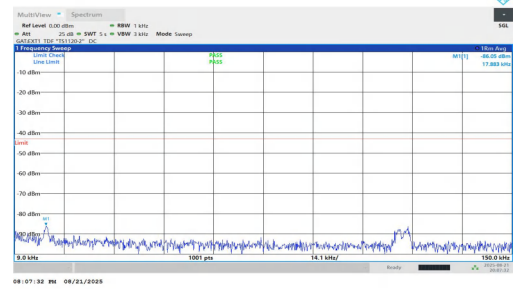
NTNV-n77(3450-3550)-PC1.5-30-50-M-DFT-QPSK-Inner_1RB_Right- 0.009-0.15-PASS
