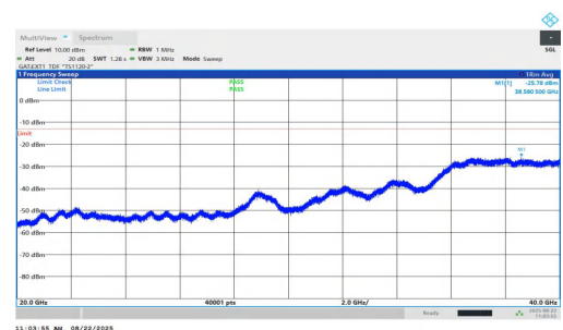
NTNV-n77(3450-3550)-PC1.5-30-40-H-DFT-QPSK-Inner_1RB_Right-2 0000-40000-PASS
