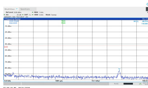
NTNV-n77(3450-3550)-PC1.5-30-40-M-DFT-QPSK-Inner_1RB_Right- 0.009-0.15-PASS
