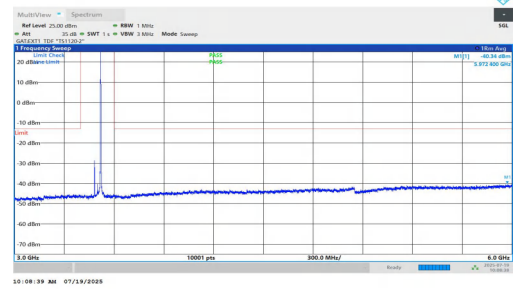
NTNV-n77(3450-3550)-PC1.5-30-40-M-DFT-QPSK-Inner_1RB_Right-3000-6000-PASS
