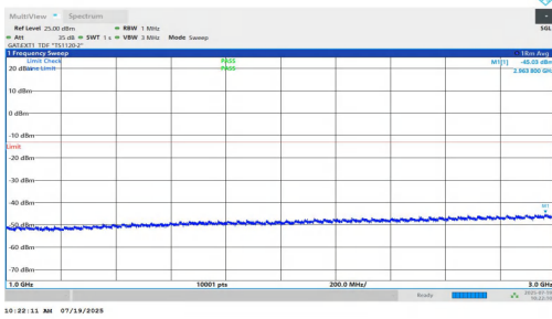
NTNV-n77(3450-3550)-PC1.5-30-50-L-DFT-QPSK-Inner_1RB_Right-1000-3000-PASS
