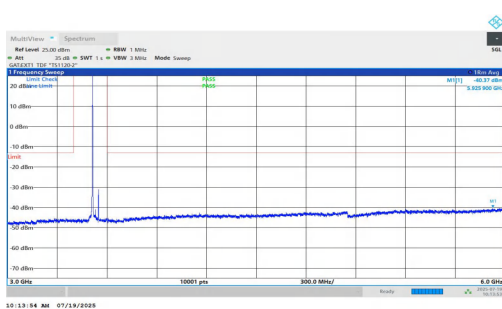
NTNV-n77(3450-3550)-PC1.5-30-40-H-DFT-QPSK-Inner_1RB_Left-3000-6000-PASS
