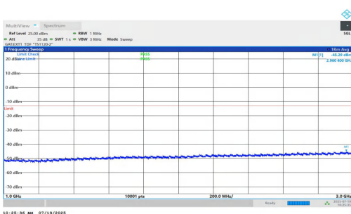
NTNV-n77(3450-3550)-PC1.5-30-50-M-DFT-BPSK-Inner_1RB_Right- 1000-3000-PASS
