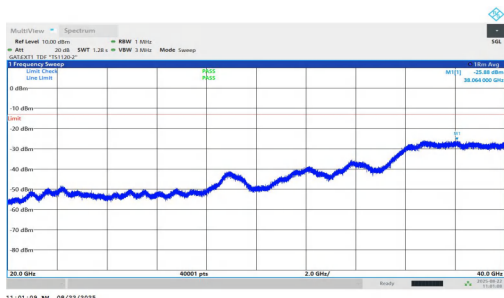
NTNV-n77(3450-3550)-PC1.5-30-40-M-DFT-QPSK-Inner_1RB_Left-2 0000-40000-PASS
