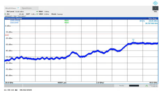
NTNV-n77(3450-3550)-PC1.5-30-50-L-DFT-QPSK-Inner_1RB_Right-20000-40000-PASS
