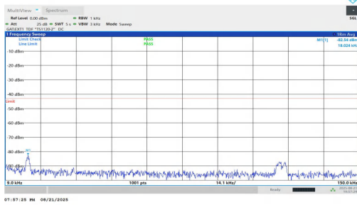
NTNV-n77(3450-3550)-PC1.5-30-40-M-DFT-BPSK-Inner_1RB_Left-0.009-0.15-PASS
