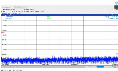
NTNV-n77(3450-3550)-PC1.5-30-50-M-DFT-QPSK-Inner_1RB_Right- 0.15-30-PASS
