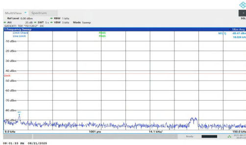
NTNV-n77(3450-3550)-PC1.5-30-40-H-DFT-QPSK-Inner_1RB_Left-0.009-0.15-PASS
