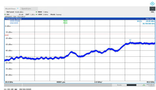
NTNV-n77(3450-3550)-PC1.5-30-40-M-DFT-BPSK-Inner_1RB_Right-2 0000-40000-PASS
