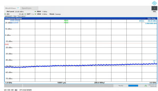
NTNV-n77(3450-3550)-PC1.5-30-40-M-DFT-BPSK-Inner_1RB_Left-1000-3000-PASS
