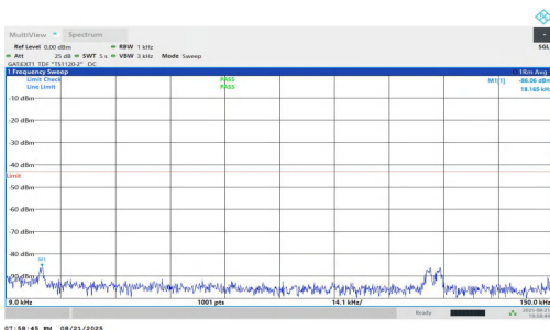
NTNV-n77(3450-3550)-PC1.5-30-40-M-DFT-QPSK-Inner_1RB_Left-0 .009-0.15-PASS
