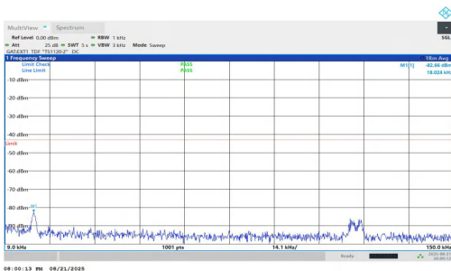
NTNV-n77(3450-3550)-PC1.5-30-40-H-DFT-BPSK-Inner_1RB_Left-0.009-0.15-PASS
