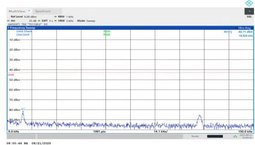
NTNV-n77(3450-3550)-PC1.5-30-40-H-DFT-BPSK-Inner_1RB_Right-0 .009-0.15-PASS
