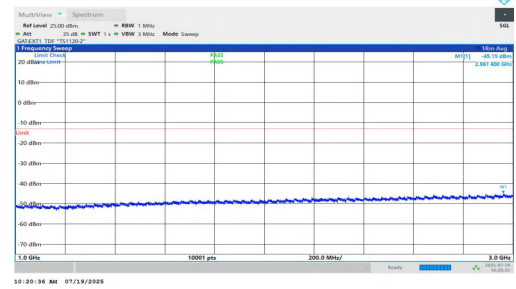
NTNV-n77(3450-3550)-PC1.5-30-50-L-DFT-QPSK-Inner_1RB_Left-10 00-3000-PASS
