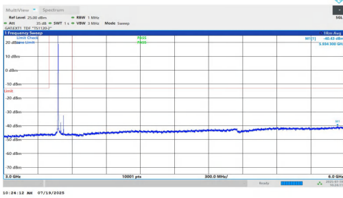
NTNV-n77(3450-3550)-PC1.5-30-50-M-DFT-BPSK-Inner_1RB_Left-3 000-6000-PASS
