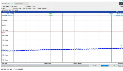
NTNV-n77(3450-3550)-PC1.5-30-40-M-DFT-QPSK-Inner_1RB_Right-1000-3000-PASS
