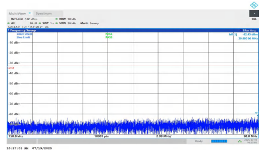
NTNV-n77(3450-3550)-PC1.5-30-50-M-DFT-QPSK-Inner_1RB_Left-0.15-30-PASS
