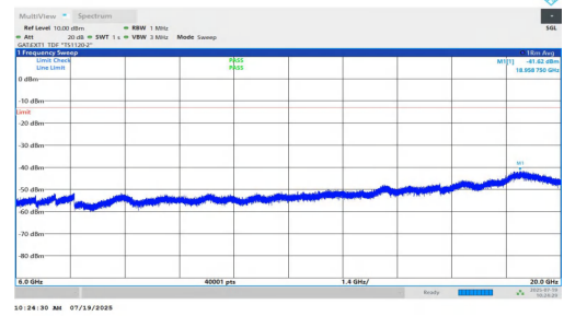
NTNV-n77(3450-3550)-PC1.5-30-50-M-DFT-BPSK-Inner_1RB_Left-60 00-20000-PASS
