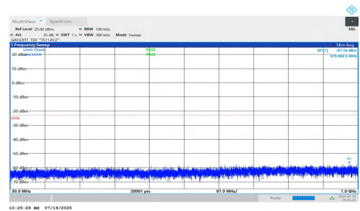
NTNV-n77(3450-3550)-PC1.5-30-50-M-DFT-BPSK-Inner_1RB_Right-3 0-1000-PASS
