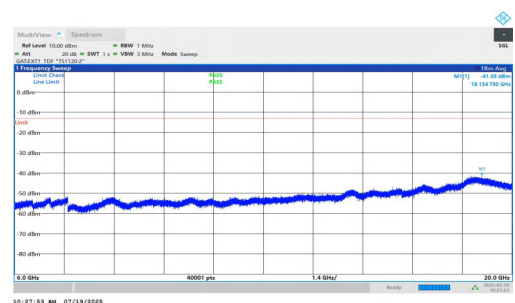
NTNV-n77(3450-3550)-PC1.5-30-50-M-DFT-QPSK-Inner_1RB_Left-6000-20000-PASS
