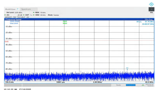
NTNV-n77(3450-3550)-PC1.5-30-40-H-DFT-BPSK-Inner_1RB_Left-0.15-5-30-PASS
