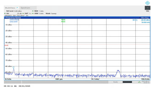
NTNV-n77(3450-3550)-PC1.5-30-50-M-DFT-BPSK-Inner_1RB_Right-0 .009-0.15-PASS
