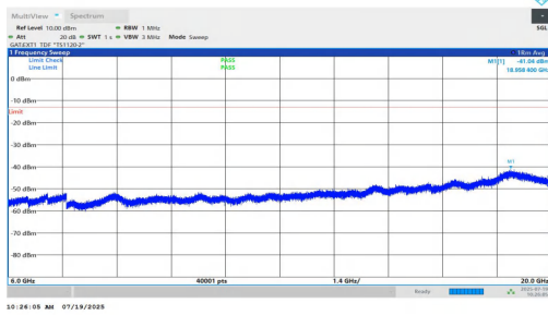
NTNV-n77(3450-3550)-PC1.5-30-50-M-DFT-BPSK-Inner_1RB_Right-6000-20000-PASS
