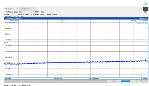
NTNV-n77(3450-3550)-PC1.5-30-50-M-DFT-QPSK-Inner_1RB_Left-1000-3000-PASS
