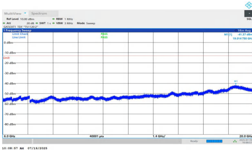
NTNV-n77(3450-3550)-PC1.5-30-40-M-DFT-QPSK-Inner_1RB_Right-6000-20000-PASS
