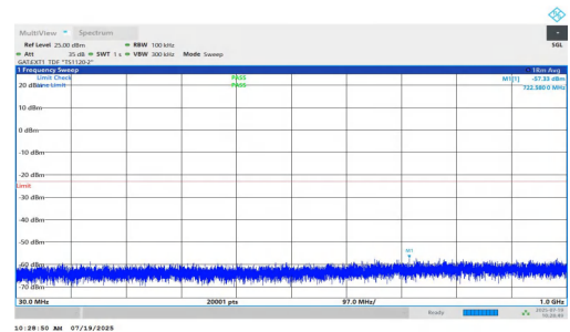
NTNV-n77(3450-3550)-PC1.5-30-50-M-DFT-QPSK-Inner_1RB_Right- 30-1000-PASS
