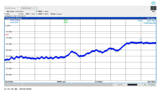
NTNV-n77(3450-3550)-PC1.5-30-40-M-DFT-QPSK-Inner_1RB_Right-20000-40000-PASS
