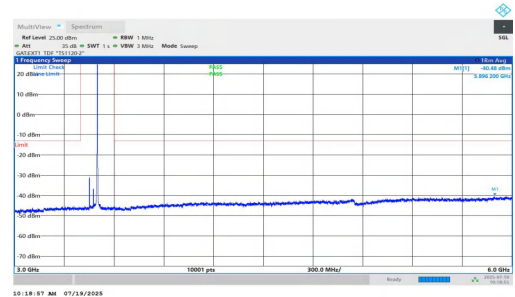
NTNV-n77(3450-3550)-PC1.5-30-50-L-DFT-BPSK-Inner_1RB_Right-3 000-6000-PASS
