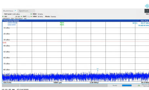
NTNV-n77(3450-3550)-PC1.5-30-50-L-DFT-QPSK-Inner_1RB_Right- 0.15-30-PASS
