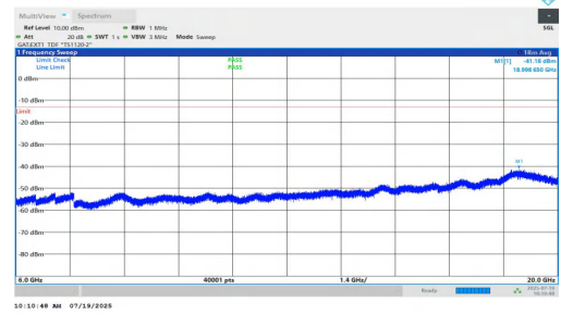
NTNV-n77(3450-3550)-PC1.5-30-40-H-DFT-BPSK-Inner_1RB_Left-60 00-20000-PASS
