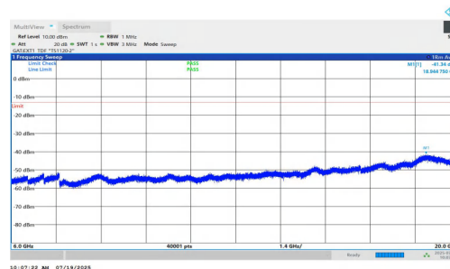
NTNV-n77(3450-3550)-PC1.5-30-40-M-DFT-QPSK-Inner_1RB_Left-60 00-20000-PASS
