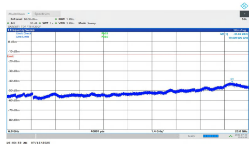
NTNV-n77(3450-3550)-PC1.5-30-40-M-DFT-BPSK-Inner_1RB_Left-6000-20000-PASS
