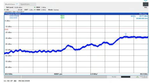
NTNV-n77(3450-3550)-PC1.5-30-40-H-DFT-BPSK-Inner_1RB_Right-20000-40000-PASS
