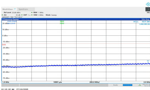
NTNV-n77(3450-3550)-PC1.5-30-40-H-DFT-QPSK-Inner_1RB_Right- 1000-3000-PASS
