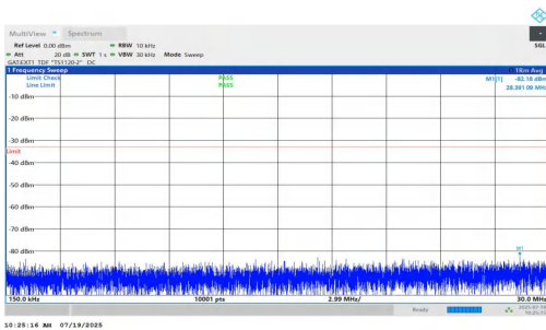
NTNV-n77(3450-3550)-PC1.5-30-50-M-DFT-BPSK-Inner_1RB_Right- 0.15-30-PASS
