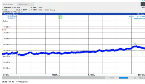
NTNV-n77(3450-3550)-PC1.5-30-40-H-DFT-BPSK-Inner_1RB_Right-6000-20000-PASS
