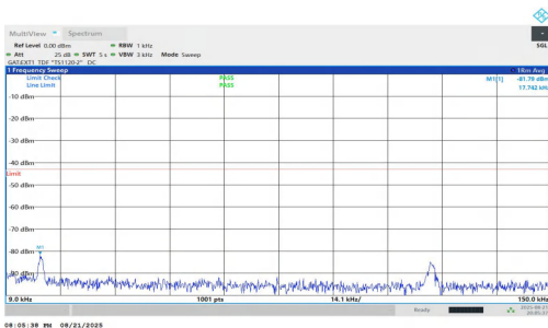
NTNV-n77(3450-3550)-PC1.5-30-50-M-DFT-BPSK-Inner_1RB_Left-0.009-0.15-PASS
