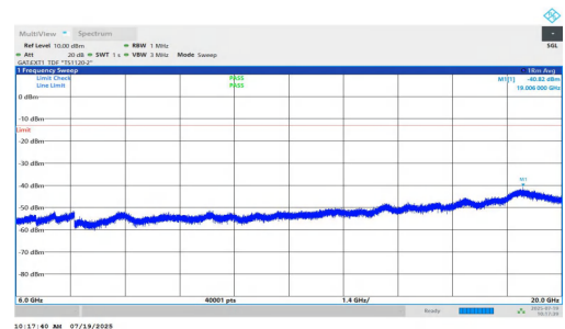
NTV-n77(3450-3550)-PC1.5-30-50-L-DFT-BPSK-Inner_1RB_Left-6000-20000-PASS
