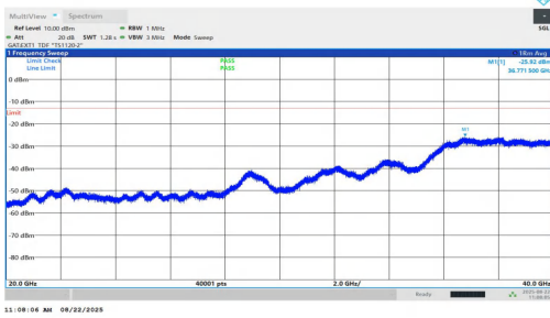
NTNV-n77(3450-3550)-PC1.5-30-50-M-DFT-QPSK-Inner_1RB_Left-2 0000-40000-PASS
