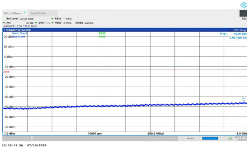
NTNV-n77(3450-3550)-PC1.5-30-40-M-DFT-BPSK-Inner_1RB_Right-1000-3000-PASS
