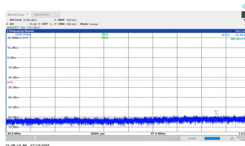
NTNV-n77(3450-3550)-PC1.5-30-40-M-DFT-QPSK-Inner_1RB_Right- 30-1000-PASS
