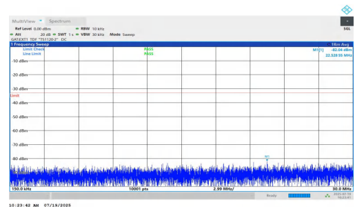
NTNV-n77(3450-3550)-PC1.5-30-50-M-DFT-BPSK-Inner_1RB_Left-0.15-30-PASS
