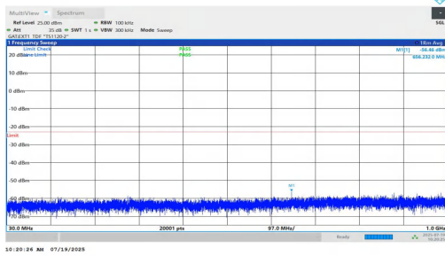
NTNV-n77(3450-3550)-PC1.5-30-50-L-DFT-QPSK-Inner_1RB_Left-3 0-1000-PASS
