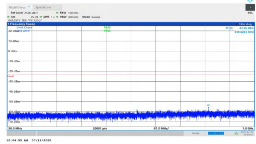
NTNV-n77(3450-3550)-PC1.5-30-40-M-DFT-BPSK-Inner_1RB_Right-3 0-1000-PASS
