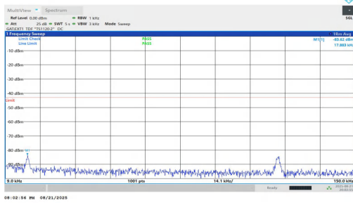
NTV-n77(3450-3550)-PC1.5-30-50-L-DFT-BPSK-Inner_1RB_Left-0.009-0.15-PASS
