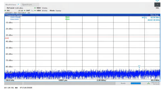
NTV-n77(3450-3550)-PC1.5-30-50-L-DFT-BPSK-Inner_1RB_Left-0.15-30-PASS
