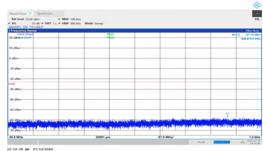
NTNV-n77(3450-3550)-PC1.5-30-40-H-DFT-QPSK-Inner_1RB_Right-3 0-1000-PASS
