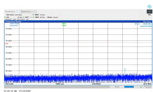
NTNV-n77(3450-3550)-PC1.5-30-50-L-DFT-QPSK-Inner_1RB_Left-0.1 5-30-PASS
