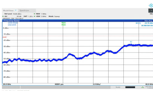
NTV-n77(3450-3550)-PC1.5-30-50-L-DFT-BPSK-Inner_1RB_Left-20000-40000-PASS
