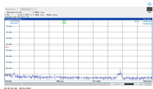
NTNV-n77(3450-3550)-PC1.5-30-50-L-DFT-QPSK-Inner_1RB_Right-0 .009-0.15-PASS
