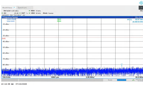
NTNV-n77(3450-3550)-PC1.5-30-40-H-DFT-QPSK-Inner_1RB_Right- 0.15-30-PASS
