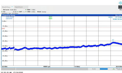
NTNV-n77(3450-3550)-PC1.5-30-40-M-DFT-BPSK-Inner_1RB_Right-6000-20000-PASS
