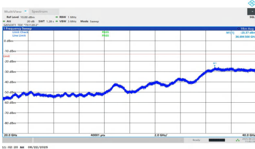
NTNV-n77(3450-3550)-PC1.5-30-40-H-DFT-BPSK-Inner_1RB_Left-2 0000-40000-PASS
