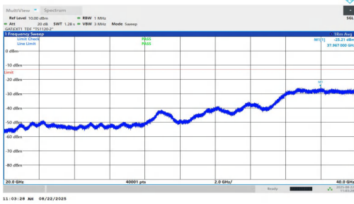
NTNV-n77(3450-3550)-PC1.5-30-40-H-DFT-QPSK-Inner_1RB_Left-2 0000-40000-PASS
