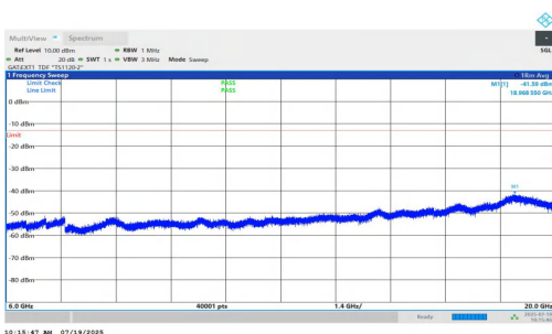
NTNV-n77(3450-3550)-PC1.5-30-40-H-DFT-QPSK-Inner_1RB_Right- 6000-20000-PASS
