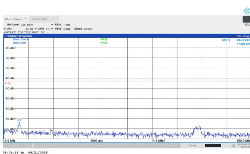
NTNV-n77(3450-3550)-PC1.5-30-50-L-DFT-QPSK-Inner_1RB_Left-0.009-0.15-PASS
