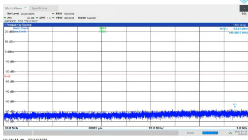
NTNV-n77(3450-3550)-PC1.5-30-40-M-DFT-QPSK-Inner_1RB_Left-3 0-1000-PASS
