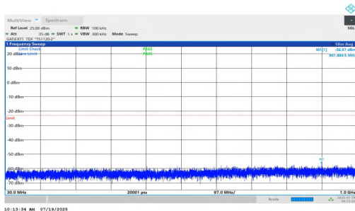
NTNV-n77(3450-3550)-PC1.5-30-40-H-DFT-QPSK-Inner_1RB_Left-30-1000-PASS
