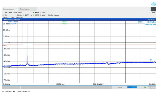
NTNV-n77(3450-3550)-PC1.5-30-40-M-DFT-QPSK-Inner_1RB_Left-3 000-6000-PASS
