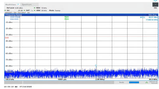
NTNV-n77(3450-3550)-PC1.5-30-40-M-DFT-BPSK-Inner_1RB_Left-0.15-30-PASS
