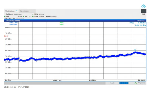
NTNV-n77(3450-3550)-PC1.5-30-40-H-DFT-QPSK-Inner_1RB_Left-6000-20000-PASS
