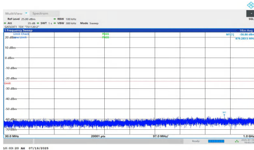
NTNV-n77(3450-3550)-PC1.5-30-40-M-DFT-BPSK-Inner_1RB_Left-30-1000-PASS
