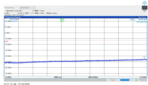
NTV-n77(3450-3550)-PC1.5-30-50-L-DFT-BPSK-Inner_1RB_Left-1000-3000-PASS
