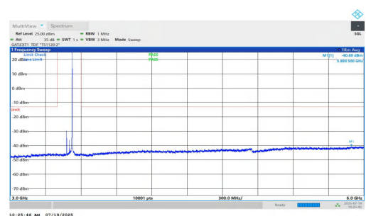
NTNV-n77(3450-3550)-PC1.5-30-50-M-DFT-BPSK-Inner_1RB_Right-3 000-6000-PASS
