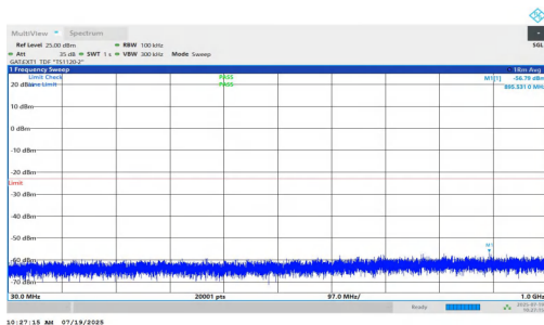
NTNV-n77(3450-3550)-PC1.5-30-50-M-DFT-QPSK-Inner_1RB_Left-30-1000-PASS
