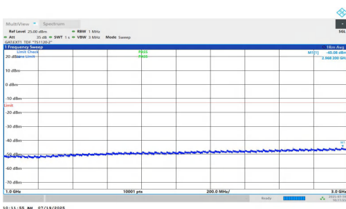
NTNV-n77(3450-3550)-PC1.5-30-40-H-DFT-BPSK-Inner_1RB_Right- 1000-3000-PASS
