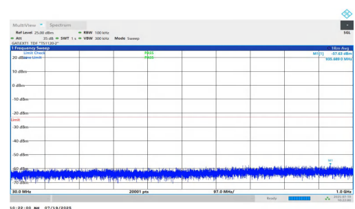
NTNV-n77(3450-3550)-PC1.5-30-50-L-DFT-QPSK-Inner_1RB_Right-3 0-1000-PASS
