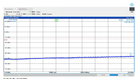
NTNV-n77(3450-3550)-PC1.5-30-50-M-DFT-BPSK-Inner_1RB_Left-1000-3000-PASS
