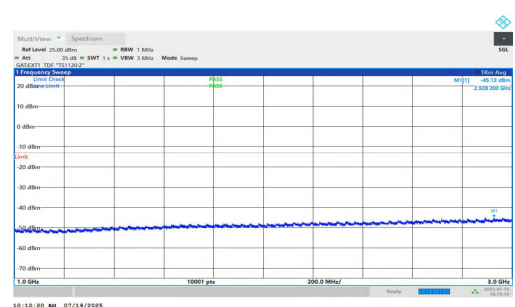
NTNV-n77(3450-3550)-PC1.5-30-40-H-DFT-BPSK-Inner_1RB_Left-1000-3000-PASS
