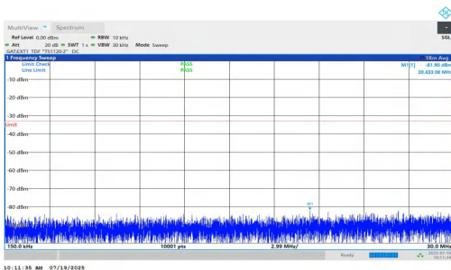
NTNV-n77(3450-3550)-PC1.5-30-40-H-DFT-BPSK-Inner_1RB_Right- 0.15-30-PASS
