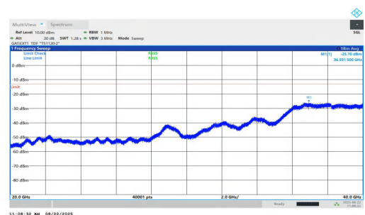
NTNV-n77(3450-3550)-PC1.5-30-50-M-DFT-QPSK-Inner_1RB_Right- 20000-40000-PASS
