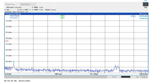
NTNV-n77(3450-3550)-PC1.5-30-40-H-DFT-QPSK-Inner_1RB_Right-0 .009-0.15-PASS
