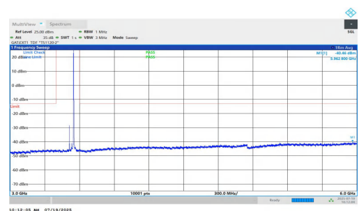
NTNV-n77(3450-3550)-PC1.5-30-40-H-DFT-BPSK-Inner_1RB_Right-3 000-6000-PASS
