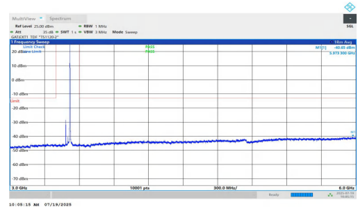
NTNV-n77(3450-3550)-PC1.5-30-40-M-DFT-BPSK-Inner_1RB_Right-3 000-6000-PASS
