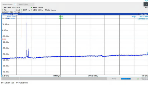
NTNV-n77(3450-3550)-PC1.5-30-40-H-DFT-BPSK-Inner_1RB_Left-3 000-6000-PASS
