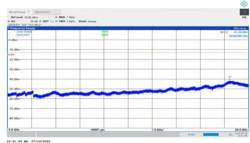
NTNV-n77(3450-3550)-PC1.5-30-50-L-DFT-QPSK-Inner_1RB_Left-60 00-20000-PASS
