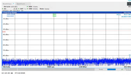
NTNV-n77(3450-3550)-PC1.5-30-50-L-DFT-BPSK-Inner_1RB_Right-0.15-30-PASS
