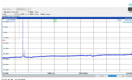
NTNV-n77(3450-3550)-PC1.5-30-50-M-DFT-QPSK-Inner_1RB_Left-3000-6000-PASS
