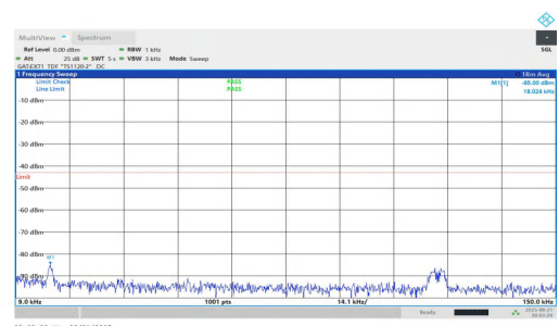
NTV-n77(3450-3550)-PC1.5-30-50-L-DFT-BPSK-Inner_1RB_Right-0.009-0.15-PASS
