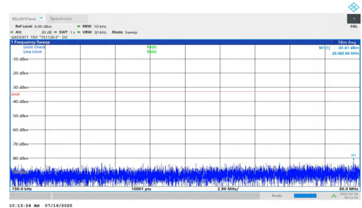
NTNV-n77(3450-3550)-PC1.5-30-40-H-DFT-QPSK-Inner_1RB_Left-0.15-30-PASS
