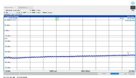
NTNV-n77(3450-3550)-PC1.5-30-40-H-DFT-QPSK-Inner_1RB_Left-1000-3000-PASS
