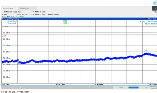
NTNV-n77(3450-3550)-PC1.5-30-50-L-DFT-QPSK-Inner_1RB_Right-6000-20000-PASS
