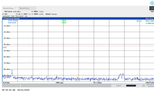
NTNV-n77(3450-3550)-PC1.5-30-50-M-DFT-QPSK-Inner_1RB_Left-0.009-0.15-PASS
