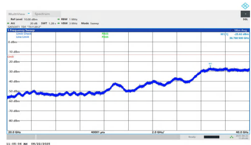
NTNV-n77(3450-3550)-PC1.5-30-50-L-DFT-BPSK-Inner_1RB_Right-2 0000-40000-PASS
