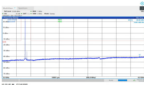
NTNV-n77(3450-3550)-PC1.5-30-40-M-DFT-BPSK-Inner_1RB_Left-3000-6000-PASS
