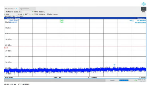
NTNV-n77(3450-3550)-PC1.5-30-40-H-DFT-BPSK-Inner_1RB_Right-3 0-1000-PASS
