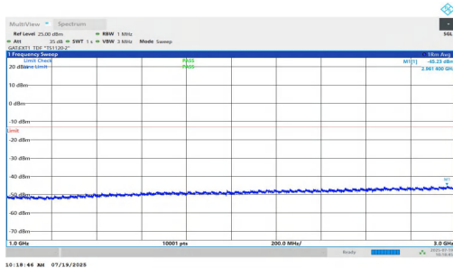
NTNV-n77(3450-3550)-PC1.5-30-50-L-DFT-BPSK-Inner_1RB_Right-1000-3000-PASS
