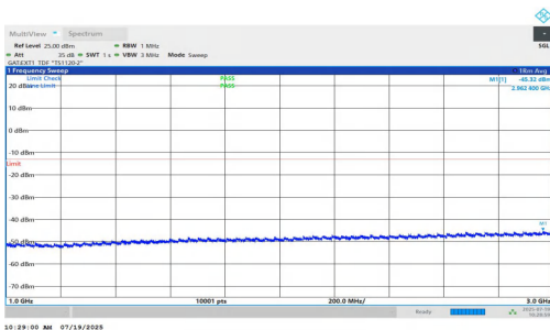
NTNV-n77(3450-3550)-PC1.5-30-50-M-DFT-QPSK-Inner_1RB_Right- 1000-3000-PASS
