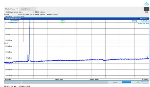
NTNV-n77(3450-3550)-PC1.5-30-50-M-DFT-QPSK-Inner_1RB_Right- 3000-6000-PASS
