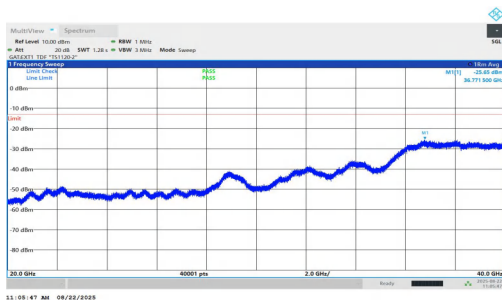
NTNV-n77(3450-3550)-PC1.5-30-50-L-DFT-QPSK-Inner_1RB_Left-2 0000-40000-PASS
