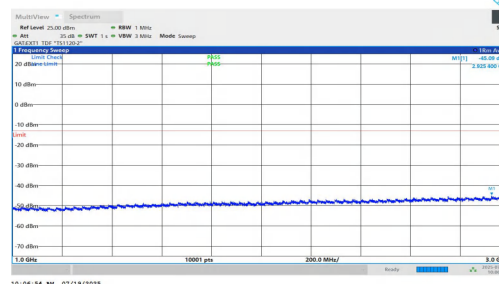
NTNV-n77(3450-3550)-PC1.5-30-40-M-DFT-QPSK-Inner_1RB_Left-10 00-3000-PASS
