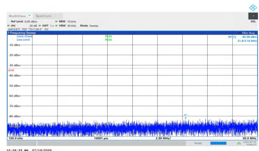
NTNV-n77(3450-3550)-PC1.5-30-40-M-DFT-QPSK-Inner_1RB_Left-0 15-30-PASS
