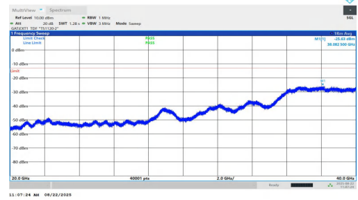
NTNV-n77(3450-3550)-PC1.5-30-50-M-DFT-BPSK-Inner_1RB_Right-20000-40000-PASS
