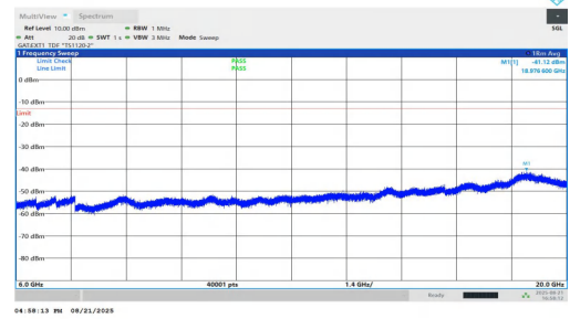
NTNV-n77(3450-3550)-PC1.5-30-25-L-DFT-BPSK-Inner_1RB_Left-60 00-20000-PASS
