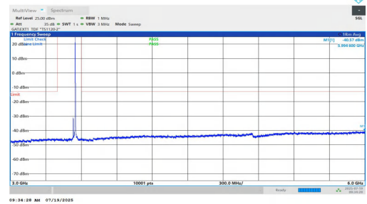
NTNV-n77(3450-3550)-PC1.5-30-20-H-DFT-QPSK-Inner_1RB_Right-3000-6000-PASS
