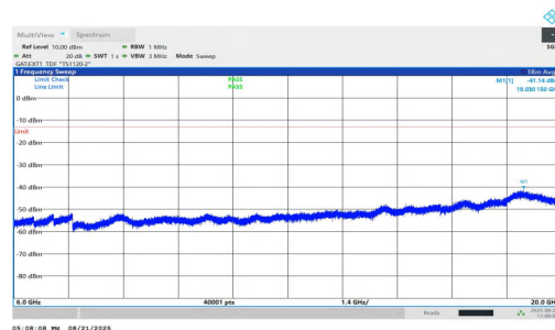
NTNV-n77(3450-3550)-PC1.5-30-25-M-DFT-QPSK-Inner_1RB_Left-60 00-20000-PASS
