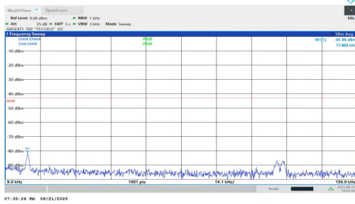
NTNV-n77(3450-3550)-PC1.5-30-20-H-DFT-BPSK-Inner_1RB_Left-0.009-0.15-PASS
