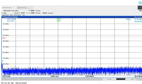
NTNV-n77(3450-3550)-PC1.5-30-25-H-DFT-QPSK-Inner_1RB_Right- 0.15-30-PASS
