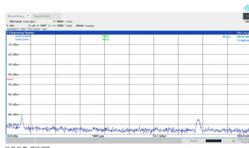
NTNV-n77(3450-3550)-PC1.5-30-25-M-DFT-QPSK-Inner_1RB_Right- 0.009-0.15-PASS
