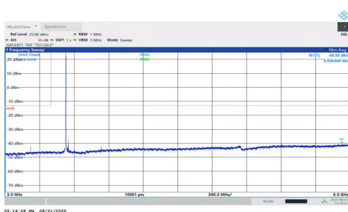
NTNV-n77(3450-3550)-PC1.5-30-25-H-DFT-QPSK-Inner_1RB_Left-3000-6000-PASS
