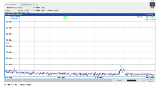
NTNV-n77(3450-3550)-PC1.5-30-25-H-DFT-QPSK-Inner_1RB_Right-0 .009-0.15-PASS
