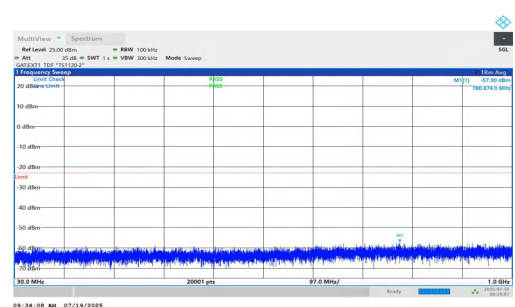
NTNV-n77(3450-3550)-PC1.5-30-20-H-DFT-QPSK-Inner_1RB_Right-3 0-1000-PASS
