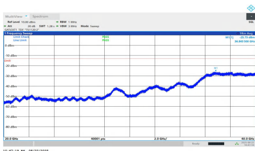
NTNV-n77(3450-3550)-PC1.5-30-25-M-DFT-QPSK-Inner_1RB_Left-2 0000-40000-PASS
