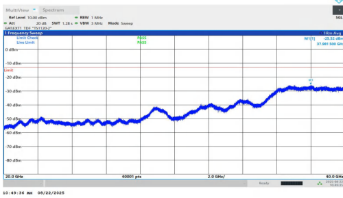
NTNV-n77(3450-3550)-PC1.5-30-25-H-DFT-QPSK-Inner_1RB_Left-2 0000-40000-PASS
