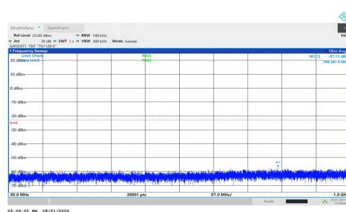
NTNV-n77(3450-3550)-PC1.5-30-25-M-DFT-QPSK-Inner_1RB_Right- 30-1000-PASS
