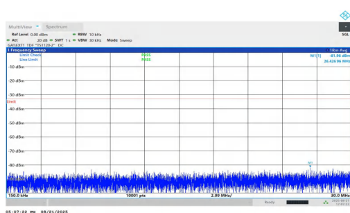
NTNV-n77(3450-3550)-PC1.5-30-25-M-DFT-QPSK-Inner_1RB_Left-0.15-30-PASS
