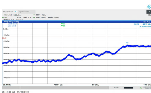
NTNV-n77(3450-3550)-PC1.5-30-25-M-DFT-BPSK-Inner_1RB_Left-20000-40000-PASS
