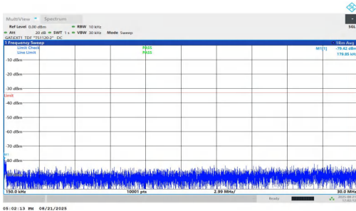
NTNV-n77(3450-3550)-PC1.5-30-25-L-DFT-QPSK-Inner_1RB_Right- 0.15-30-PASS
