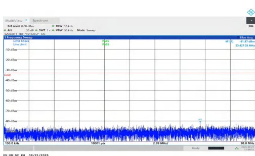
NTNV-n77(3450-3550)-PC1.5-30-25-M-DFT-QPSK-Inner_1RB_Right- 0.15-30-PASS
