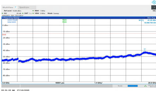
NTNV-n77(3450-3550)-PC1.5-30-20-H-DFT-BPSK-Inner_1RB_Right-6000-20000-PASS
