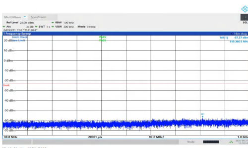
NTNV-n77(3450-3550)-PC1.5-30-25-H-DFT-BPSK-Inner_1RB_Left-30-1000-PASS
