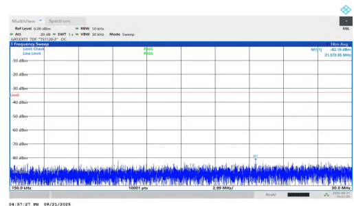
NTNV-n77(3450-3550)-PC1.5-30-25-L-DFT-BPSK-Inner_1RB_Left-0.15-5-30-PASS
