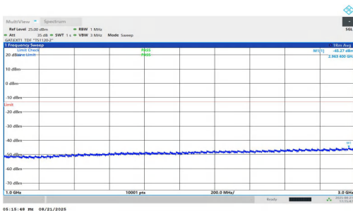
NTNV-n77(3450-3550)-PC1.5-30-25-H-DFT-QPSK-Inner_1RB_Right- 1000-3000-PASS
