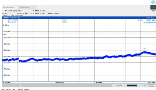
NTNV-n77(3450-3550)-PC1.5-30-25-L-DFT-BPSK-Inner_1RB_Right-6000-20000-PASS
