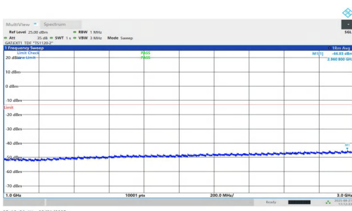
NTNV-n77(3450-3550)-PC1.5-30-25-H-DFT-BPSK-Inner_1RB_Right- 1000-3000-PASS
