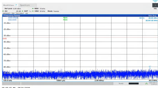
NTNV-n77(3450-3550)-PC1.5-30-25-M-DFT-BPSK-Inner_1RB_Right-0.15-30-PASS
