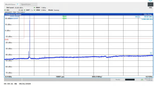
NTNV-n77(3450-3550)-PC1.5-30-25-M-DFT-QPSK-Inner_1RB_Right-3000-6000-PASS
