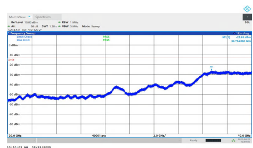
NTNV-n77(3450-3550)-PC1.5-30-25-H-DFT-QPSK-Inner_1RB_Right-2 0000-40000-PASS
