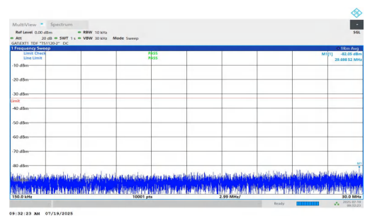
NTNV-n77(3450-3550)-PC1.5-30-20-H-DFT-QPSK-Inner_1RB_Left-0.15-30-PASS
