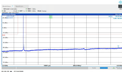
NTNV-n77(3450-3550)-PC1.5-30-20-H-DFT-BPSK-Inner_1RB_Left-3000-6000-PASS
