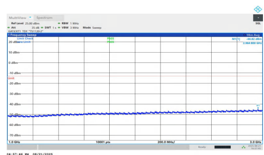
NTNV-n77(3450-3550)-PC1.5-30-25-L-DFT-BPSK-Inner_1RB_Left-1000-3000-PASS
