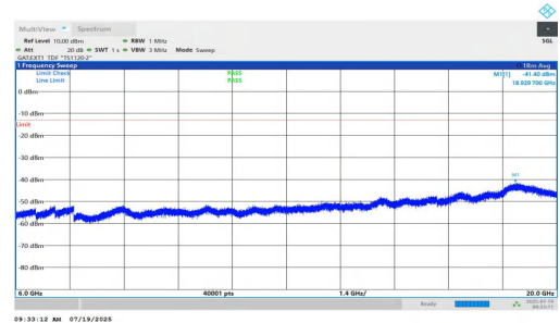
NTNV-n77(3450-3550)-PC1.5-30-20-H-DFT-QPSK-Inner_1RB_Left-60 00-20000-PASS
