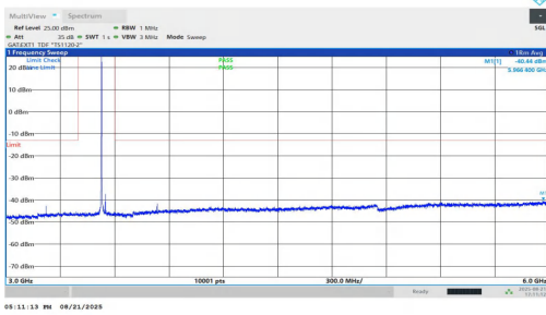
NTNV-n77(3450-3550)-PC1.5-30-25-H-DFT-BPSK-Inner_1RB_Left-3 000-6000-PASS
