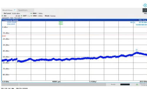
NTNV-n77(3450-3550)-PC1.5-30-25-H-DFT-QPSK-Inner_1RB_Right- 6000-20000-PASS
