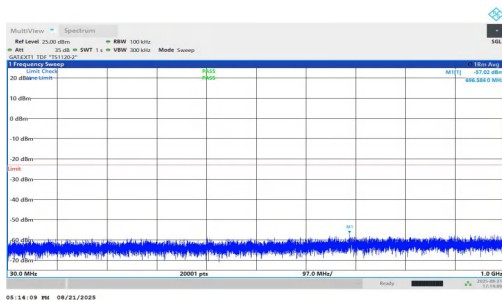
NTNV-n77(3450-3550)-PC1.5-30-25-H-DFT-QPSK-Inner_1RB_Left-30-1000-PASS
