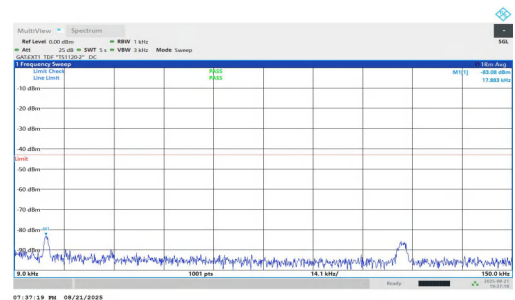
NTNV-n77(3450-3550)-PC1.5-30-20-H-DFT-QPSK-Inner_1RB_Right-0 .009-0.15-PASS
