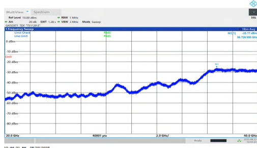
NTNV-n77(3450-3550)-PC1.5-30-25-L-DFT-BPSK-Inner_1RB_Right-20000-40000-PASS
