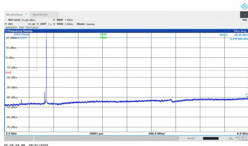
NTNV-n77(3450-3550)-PC1.5-30-25-M-DFT-BPSK-Inner_1RB_Right-3 000-6000-PASS
