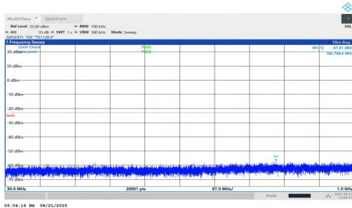
NTNV-n77(3450-3550)-PC1.5-30-25-M-DFT-BPSK-Inner_1RB_Left-30-1000-PASS
