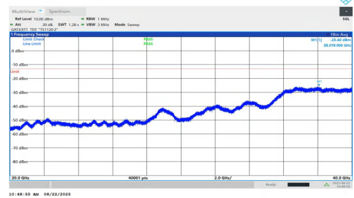
NTNV-n77(3450-3550)-PC1.5-30-25-H-DFT-BPSK-Inner_1RB_Right-20000-40000-PASS
