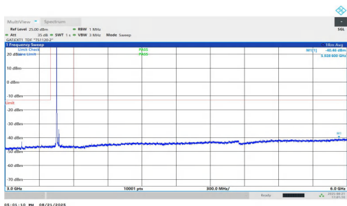
NTNV-n77(3450-3550)-PC1.5-30-25-L-DFT-QPSK-Inner_1RB_Left-30000-60000-PASS
