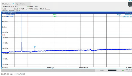
NTNV-n77(3450-3550)-PC1.5-30-25-L-DFT-BPSK-Inner_1RB_Left-30 00-6000-PASS
