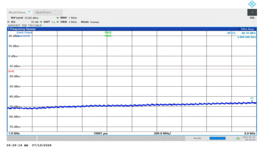
NTNV-n77(3450-3550)-PC1.5-30-20-H-DFT-BPSK-Inner_1RB_Left-1000-3000-PASS
