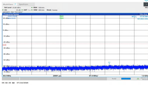
NTN-n77(3450-3550)-PC1.5-30-20-H-DFT-QPSK-Inner_1RB_Left-3 0-1000-PASS
