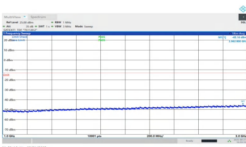
NTNV-n77(3450-3550)-PC1.5-30-25-L-DFT-BPSK-Inner_1RB_Right- 1000-3000-PASS
