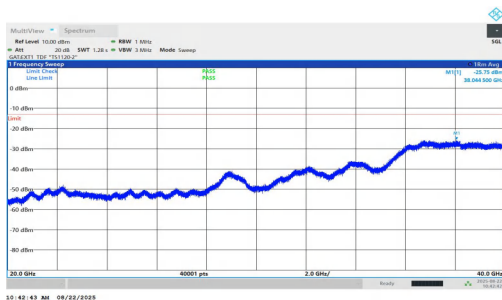
NTNV-n77(3450-3550)-PC1.5-30-20-H-DFT-QPSK-Inner_1RB_Left-2 0000-40000-PASS
