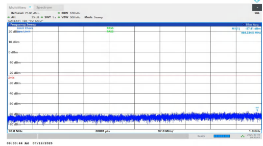
NTNV-n77(3450-3550)-PC1.5-30-20-H-DFT-BPSK-Inner_1RB_Right-3 0-1000-PASS
