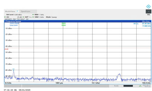
NTNV-n77(3450-3550)-PC1.5-30-25-M-DFT-BPSK-Inner_1RB_Right-0.009-0.15-PASS
