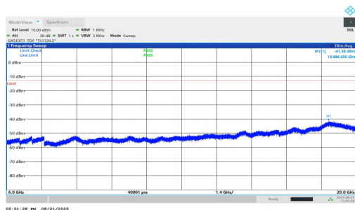
NTNV-n77(3450-3550)-PC1.5-30-25-L-DFT-QPSK-Inner_1RB_Left-60000-200000-PASS
