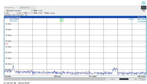
NTNV-n77(3450-3550)-PC1.5-30-25-H-DFT-BPSK-Inner_1RB_Right-0 .009-0.15-PASS
