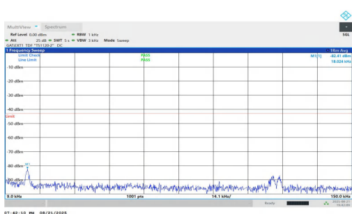
NTNV-n77(3450-3550)-PC1.5-30-25-M-DFT-QPSK-Inner_1RB_Left-0.009-0.15-PASS
