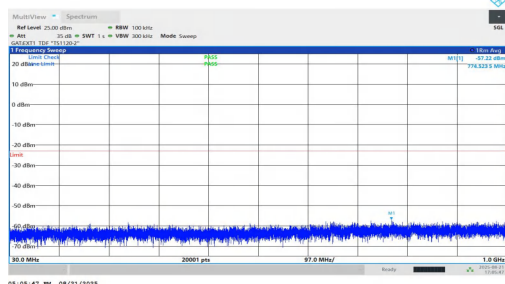
NTNV-n77(3450-3550)-PC1.5-30-25-M-DFT-BPSK-Inner_1RB_Right-3 0-1000-PASS
