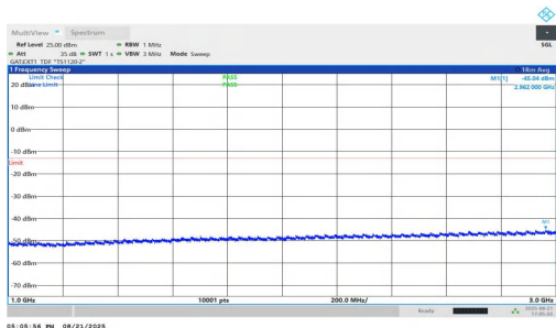
NTNV-n77(3450-3550)-PC1.5-30-25-M-DFT-BPSK-Inner_1RB_Right-1000-3000-PASS
