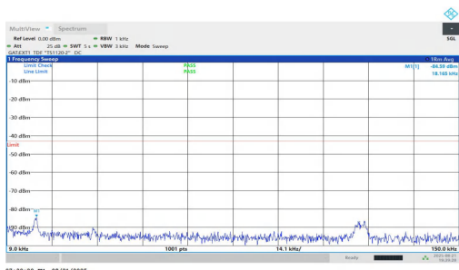
NTNV-n77(3450-3550)-PC1.5-30-25-L-DFT-QPSK-Inner_1RB_Left-0.009-0.15-PASS
