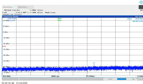
NTNV-n77(3450-3550)-PC1.5-30-20-H-DFT-BPSK-Inner_1RB_Left-300-1000-PASS
