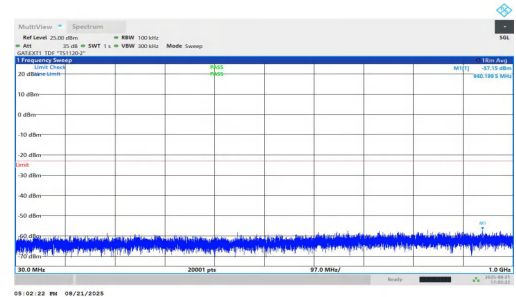
NTNV-n77(3450-3550)-PC1.5-30-25-L-DFT-QPSK-Inner_1RB_Right-3 0-1000-PASS
