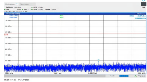
NTNV-n77(3450-3550)-PC1.5-30-20-H-DFT-BPSK-Inner_1RB_Left-0.15-30-PASS
