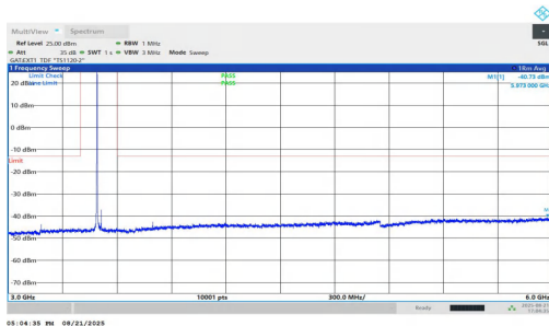
NTNV-n77(3450-3550)-PC1.5-30-25-M-DFT-BPSK-Inner_1RB_Left-3000-6000-PASS
