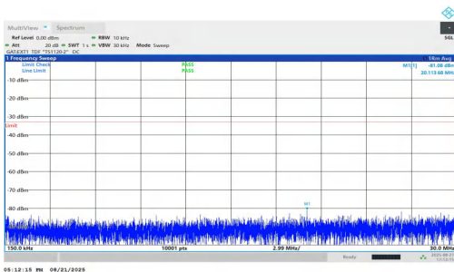
NTNV-n77(3450-3550)-PC1.5-30-25-H-DFT-BPSK-Inner_1RB_Right- 0.15-30-PASS
