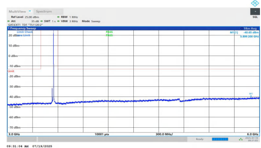
NTNV-n77(3450-3550)-PC1.5-30-20-H-DFT-BPSK-Inner_1RB_Right-3 000-6000-PASS
