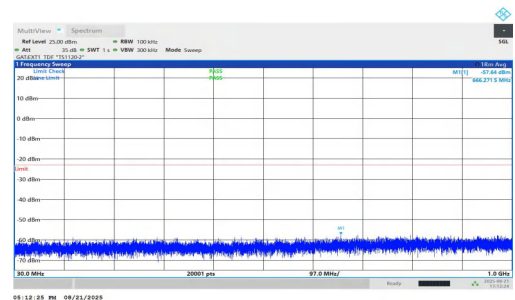
NTNV-n77(3450-3550)-PC1.5-30-25-H-DFT-BPSK-Inner_1RB_Right-3 0-1000-PASS
