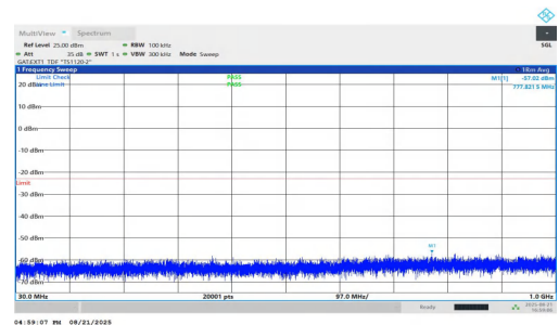
NTNV-n77(3450-3550)-PC1.5-30-25-L-DFT-BPSK-Inner_1RB_Right-3 0-1000-PASS
