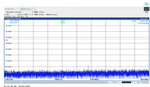
NTNV-n77(3450-3550)-PC1.5-30-25-H-DFT-BPSK-Inner_1RB_Left-0.15-5-30-PASS
