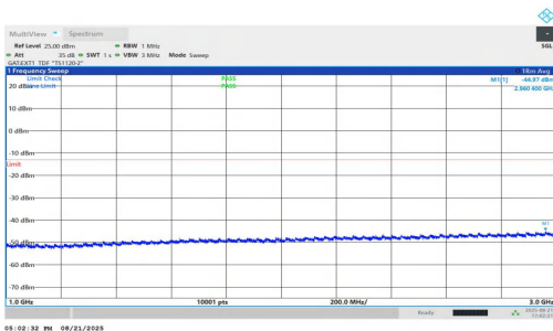
NTNV-n77(3450-3550)-PC1.5-30-25-L-DFT-QPSK-Inner_1RB_Right- 1000-3000-PASS
