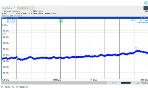
NTNV-n77(3450-3550)-PC1.5-30-25-M-DFT-QPSK-Inner_1RB_Right-6000-20000-PASS
