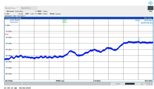
NTNV-n77(3450-3550)-PC1.5-30-20-H-DFT-QPSK-Inner_1RB_Right-20000-40000-PASS
