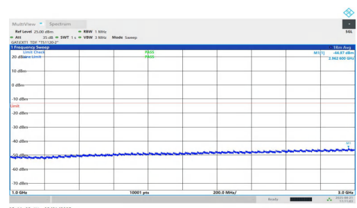
NTNV-n77(3450-3550)-PC1.5-30-25-H-DFT-BPSK-Inner_1RB_Left-1000-3000-PASS
