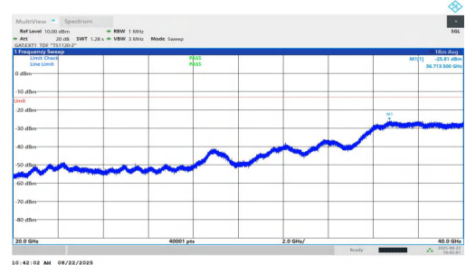
NTNV-n77(3450-3550)-PC1.5-30-20-H-DFT-BPSK-Inner_1RB_Right-2 0000-40000-PASS
