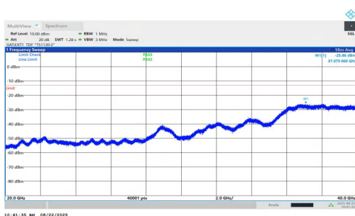
NTNV-n77(3450-3550)-PC1.5-30-20-H-DFT-BPSK-Inner_1RB_Left-20000-40000-PASS
