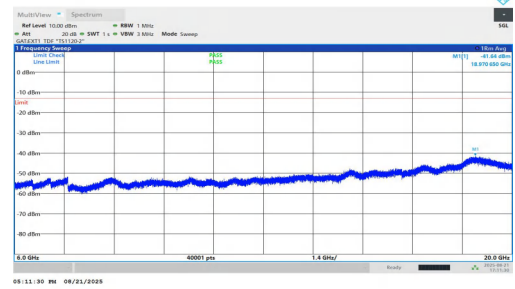
NTNV-n77(3450-3550)-PC1.5-30-25-H-DFT-BPSK-Inner_1RB_Left-60 00-20000-PASS
