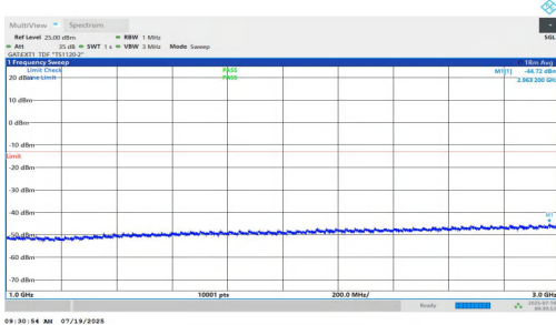
NTNV-n77(3450-3550)-PC1.5-30-20-H-DFT-BPSK-Inner_1RB_Right-1000-3000-PASS
