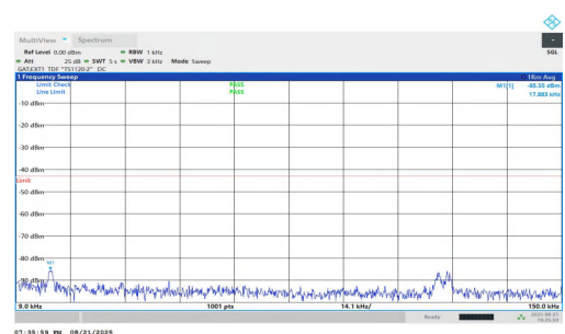
NTNV-n77(3450-3550)-PC1.5-30-20-H-DFT-BPSK-Inner_1RB_Right-0.009-0.15-PASS
