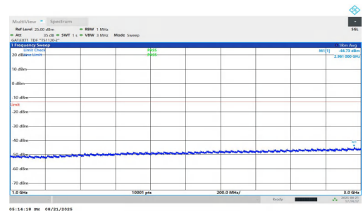
NTNV-n77(3450-3550)-PC1.5-30-25-H-DFT-QPSK-Inner_1RB_Left-1000-3000-PASS
