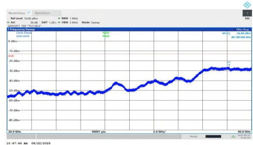
NTNV-n77(3450-3550)-PC1.5-30-25-M-DFT-QPSK-Inner_1RB_Right-20000-40000-PASS
