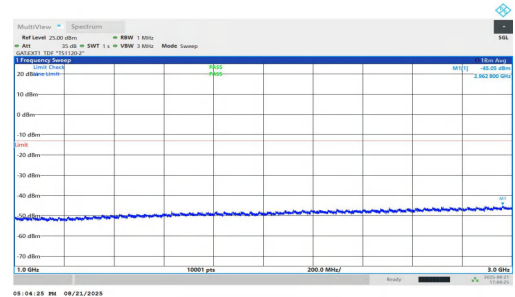
NTNV-n77(3450-3550)-PC1.5-30-25-M-DFT-BPSK-Inner_1RB_Left-1000-3000-PASS
