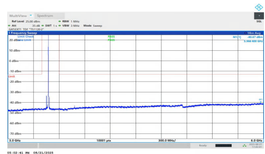
NTNV-n77(3450-3550)-PC1.5-30-25-L-DFT-QPSK-Inner_1RB_Right-3 000-6000-PASS
