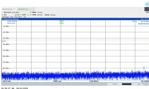
NTNV-n77(3450-3550)-PC1.5-30-25-L-DFT-BPSK-Inner_1RB_Right- 0.15-30-PASS
