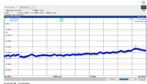
NTNV-n77(3450-3550)-PC1.5-30-20-H-DFT-BPSK-Inner_1RB_Left-6000-20000-PASS
