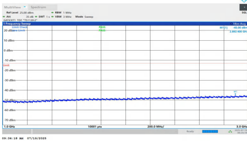
NTNV-n77(3450-3550)-PC1.5-30-20-H-DFT-QPSK-Inner_1RB_Right-1000-3000-PASS
