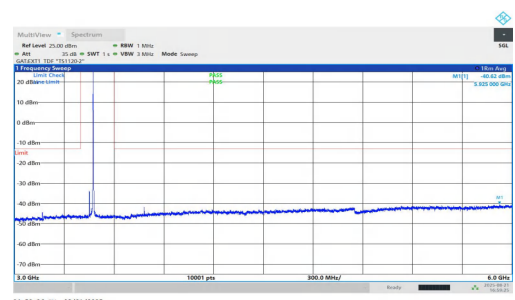
NTNV-n77(3450-3550)-PC1.5-30-25-L-DFT-BPSK-Inner_1RB_Right-3 000-6000-PASS
