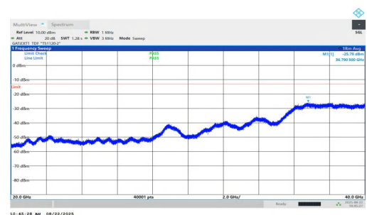
NTNV-n77(3450-3550)-PC1.5-30-25-L-DFT-QPSK-Inner_1RB_Right-2 0000-40000-PASS
