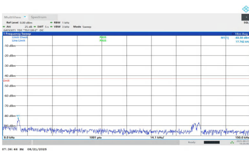
NTNV-n77(3450-3550)-PC1.5-30-20-H-DFT-QPSK-Inner_1RB_Left-0.009-0.15-PASS
