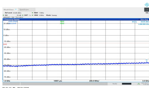
NTNV-n77(3450-3550)-PC1.5-30-25-L-DFT-QPSK-Inner_1RB_Left-10000-30000-PASS
