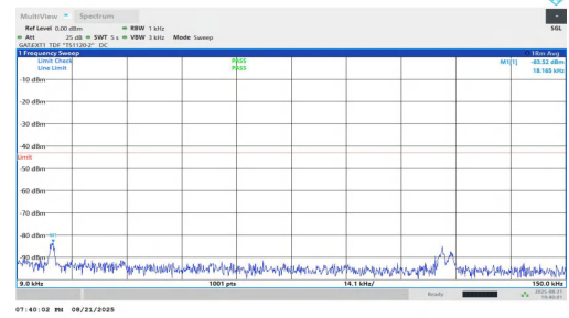
NTNV-n77(3450-3550)-PC1.5-30-25-L-DFT-QPSK-Inner_1RB_Right-0 .009-0.15-PASS
