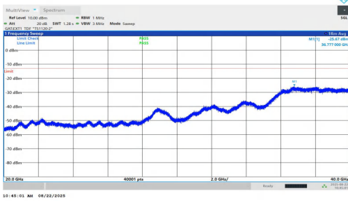
NTNV-n77(3450-3550)-PC1.5-30-25-L-DFT-QPSK-Inner_1RB_Left-2 0000-40000-PASS
