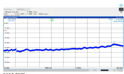
NTNV-n77(3450-3550)-PC1.5-30-25-H-DFT-QPSK-Inner_1RB_Left-6000-20000-PASS
