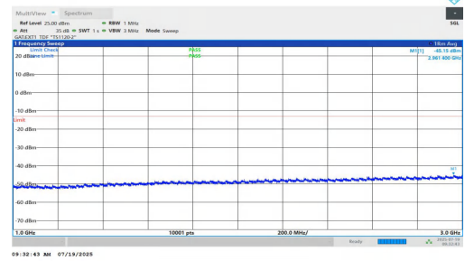
NTNV-n77(3450-3550)-PC1.5-30-20-H-DFT-QPSK-Inner_1RB_Left-10 00-3000-PASS
