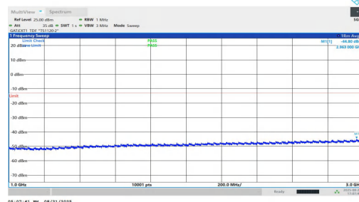
NTNV-n77(3450-3550)-PC1.5-30-25-M-DFT-QPSK-Inner_1RB_Left-10 00-3000-PASS
