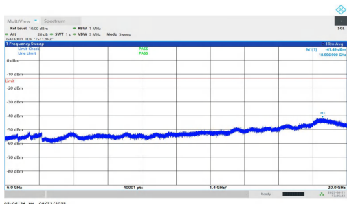
NTNV-n77(3450-3550)-PC1.5-30-25-M-DFT-BPSK-Inner_1RB_Right-6000-20000-PASS
