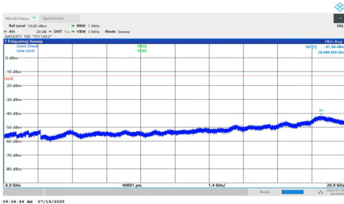
NTNV-n77(3450-3550)-PC1.5-30-20-H-DFT-QPSK-Inner_1RB_Right-6000-20000-PASS
