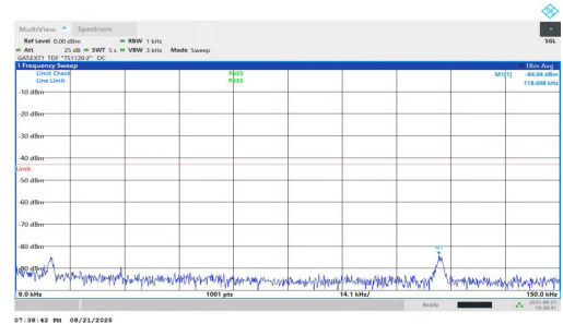
NTNV-n77(3450-3550)-PC1.5-30-25-L-DFT-BPSK-Inner_1RB_Right-0. 009-0.15-PASS
