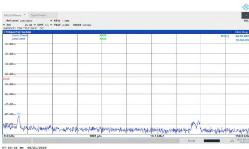
NTNV-n77(3450-3550)-PC1.5-30-25-H-DFT-BPSK-Inner_1RB_Left-0.009-0.15-PASS
