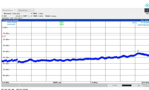
NTNV-n77(3450-3550)-PC1.5-30-25-L-DFT-QPSK-Inner_1RB_Right- 6000-20000-PASS
