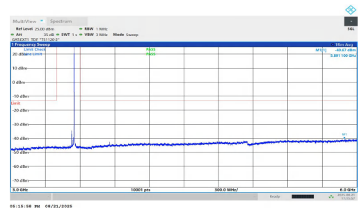
NTNV-n77(3450-3550)-PC1.5-30-25-H-DFT-QPSK-Inner_1RB_Right-3 000-6000-PASS
