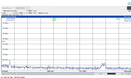
NTNV-n77(3450-3550)-PC1.5-30-25-L-DFT-BPSK-Inner_1RB_Left-0.009-0.15-PASS
