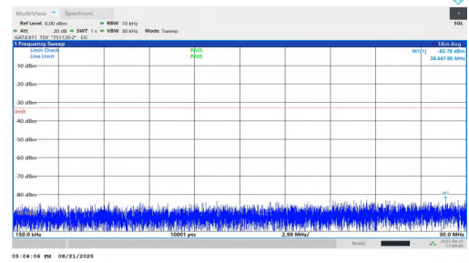
NTNV-n77(3450-3550)-PC1.5-30-25-M-DFT-BPSK-Inner_1RB_Left-0.15-30-PASS
