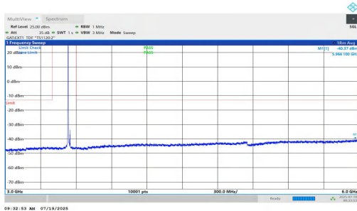
NTNV-n77(3450-3550)-PC1.5-30-20-H-DFT-QPSK-Inner_1RB_Left-3 000-6000-PASS
