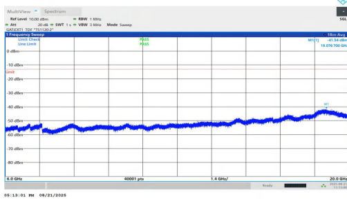
NTNV-n77(3450-3550)-PC1.5-30-25-H-DFT-BPSK-Inner_1RB_Right-6000-20000-PASS
