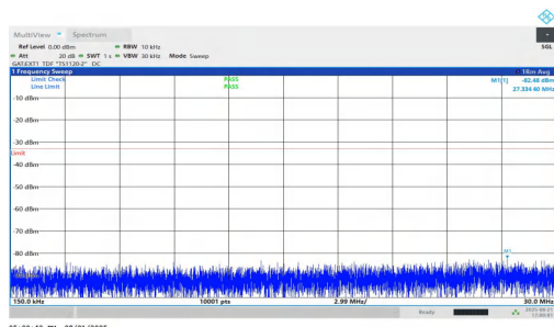
NTNV-n77(3450-3550)-PC1.5-30-25-L-DFT-QPSK-Inner_1RB_Left-0.15-0.30-PASS
