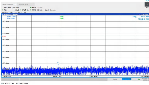
NTNV-n77(3450-3550)-PC1.5-30-20-H-DFT-BPSK-Inner_1RB_Right-0.15-30-PASS
