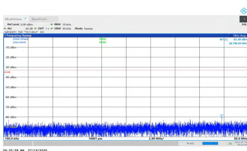
NTNV-n77(3450-3550)-PC1.5-30-20-H-DFT-QPSK-Inner_1RB_Right- 0.15-30-PASS
