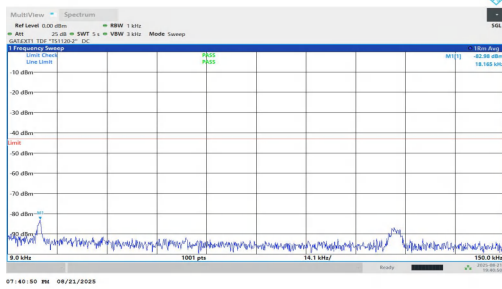
NTNV-n77(3450-3550)-PC1.5-30-25-M-DFT-BPSK-Inner_1RB_Left-0.009-0.15-PASS
