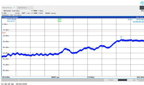
NTNV-n77(3450-3550)-PC1.5-30-25-H-DFT-BPSK-Inner_1RB_Left-2 0000-40000-PASS
