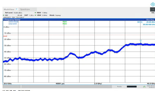
NTNV-n77(3450-3550)-PC1.5-30-25-M-DFT-BPSK-Inner_1RB_Right-2 0000-40000-PASS
