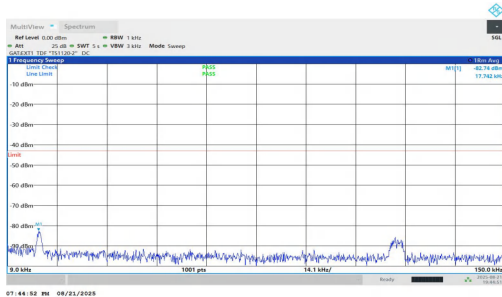
NTNV-n77(3450-3550)-PC1.5-30-25-H-DFT-QPSK-Inner_1RB_Left-0.009-0.15-PASS
