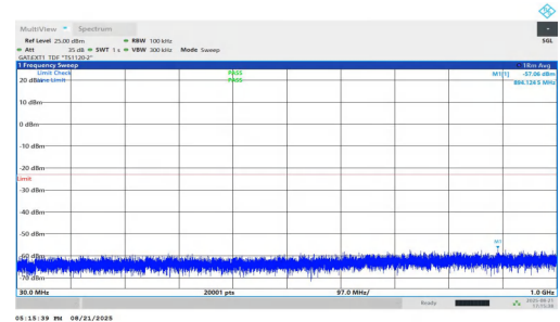
NTNV-n77(3450-3550)-PC1.5-30-25-H-DFT-QPSK-Inner_1RB_Right-3 0-1000-PASS
