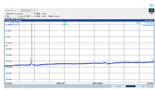
NTNV-n77(3450-3550)-PC1.5-30-25-H-DFT-BPSK-Inner_1RB_Right-3 000-6000-PASS
