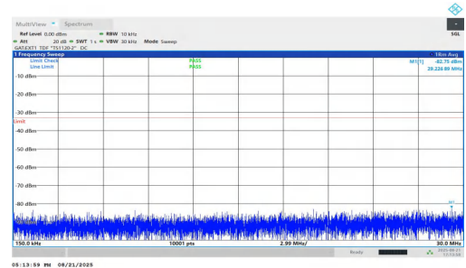
NTNV-n77(3450-3550)-PC1.5-30-25-H-DFT-QPSK-Inner_1RB_Left-0.15-30-PASS
