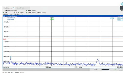
NTNV-n77(3450-3550)-PC1.5-30-15-M-DFT-QPSK-Inner_1RB_Right- 0.009-0.15-PASS
