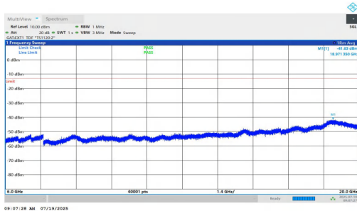
NTNV-n77(3450-3550)-PC1.5-30-15-M-DFT-QPSK-Inner_1RB_Right-6000-20000-PASS
