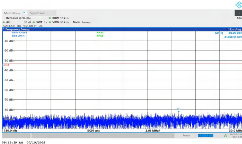
NTNV-n77(3450-3550)-PC1.5-30-15-H-DFT-QPSK-Inner_1RB_Right- 0.15-30-PASS
