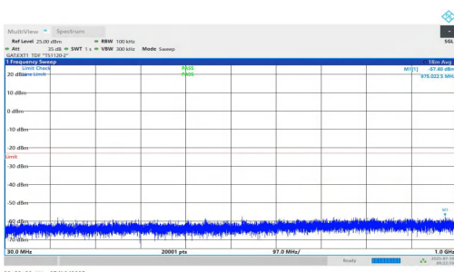
NTNV-n77(3450-3550)-PC1.5-30-20-M-DFT-BPSK-Inner_1RB_Left-30-1000-PASS
