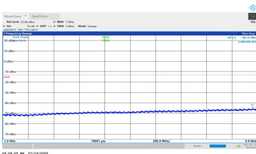
NTVN-n77(3450-3550)-PC1.5-30-20-M-DFT-BPSK-Inner_1RB_Right- 1000-3000-PASS
