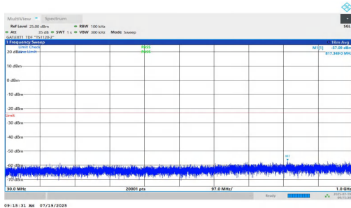
NTNV-n77(3450-3550)-PC1.5-30-20-L-DFT-BPSK-Inner_1RB_Left-30-1000-PASS
