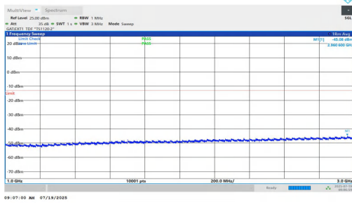
NTNV-n77(3450-3550)-PC1.5-30-15-M-DFT-QPSK-Inner_1RB_Right-1000-3000-PASS
