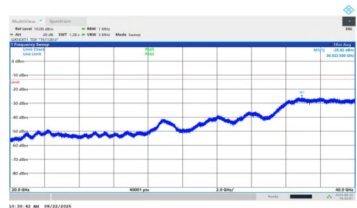
NTNV-n77(3450-3550)-PC1.5-30-15-M-DFT-BPSK-Inner_1RB_Right-2 0000-40000-PASS
