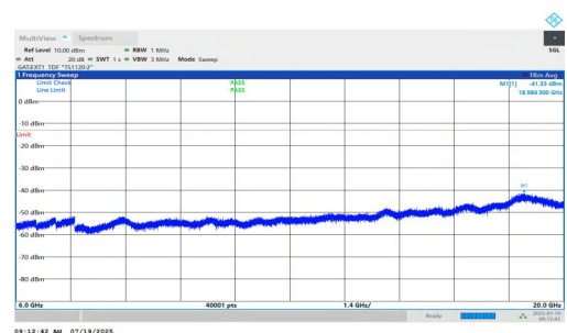
NTNV-n77(3450-3550)-PC1.5-30-15-H-DFT-QPSK-Inner_1RB_Left-6000-20000-PASS
