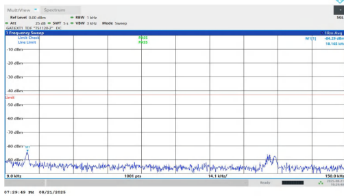
NTNV-n77(3450-3550)-PC1.5-30-20-L-DFT-BPSK-Inner_1RB_Left-0.009-0.15-PASS
