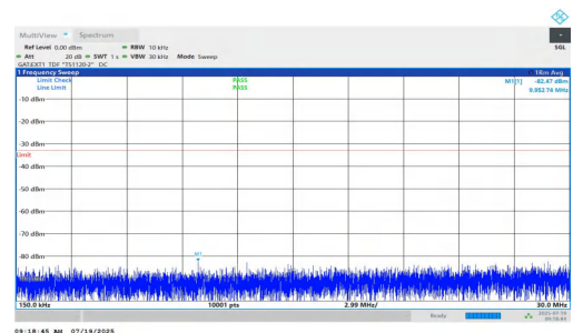
NTNV-n77(3450-3550)-PC1.5-30-20-L-DFT-QPSK-Inner_1RB_Left-0.1 5-30-PASS
