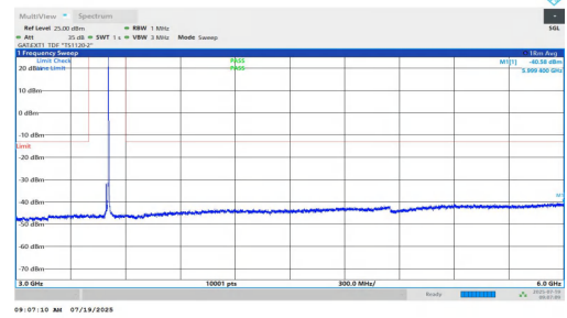
NTNV-n77(3450-3550)-PC1.5-30-15-M-DFT-QPSK-Inner_1RB_Right-3000-6000-PASS
