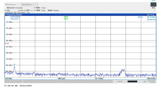
NTNV-n77(3450-3550)-PC1.5-30-15-H-DFT-QPSK-Inner_1RB_Right-0 .009-0.15-PASS
