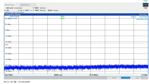
NTNV-n77(3450-3550)-PC1.5-30-20-L-DFT-BPSK-Inner_1RB_Right-3 0-1000-PASS
