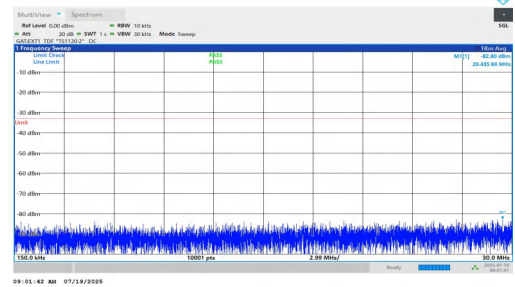
NTNV-n77(3450-3550)-PC1.5-30-15-M-DFT-BPSK-Inner_1RB_Left-0.15-30-PASS
