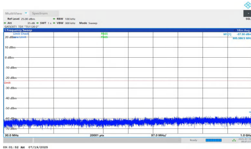
NTNV-n77(3450-3550)-PC1.5-30-15-M-DFT-BPSK-Inner_1RB_Left-30-1000-PASS
