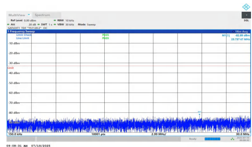
NTNV-n77(3450-3550)-PC1.5-30-15-H-DFT-BPSK-Inner_1RB_Left-0.15-5-30-PASS
