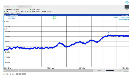
NTNV-n77(3450-3550)-PC1.5-30-15-M-DFT-QPSK-Inner_1RB_Right-20000-40000-PASS
