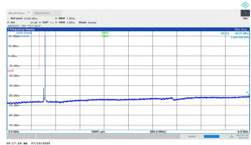
NTNV-n77(3450-3550)-PC1.5-30-20-L-DFT-BPSK-Inner_1RB_Right-3 000-6000-PASS
