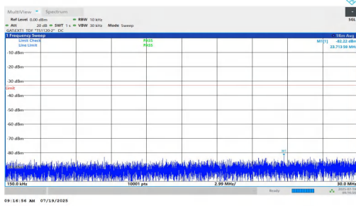
NTNV-n77(3450-3550)-PC1.5-30-20-L-DFT-BPSK-Inner_1RB_Right-0.15-30-PASS
