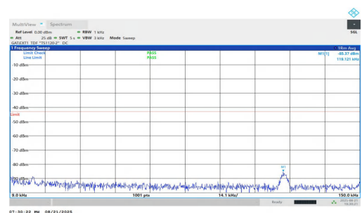
NTNV-n77(3450-3550)-PC1.5-30-20-L-DFT-BPSK-Inner_1RB_Right-0.009-0.15-PASS
