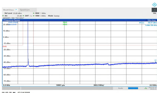
NTNV-n77(3450-3550)-PC1.5-30-15-M-DFT-QPSK-Inner_1RB_Left-3 000-6000-PASS
