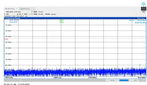
NTNV-n77(3450-3550)-PC1.5-30-20-M-DFT-BPSK-Inner_1RB_Left-0.15-30-PASS
