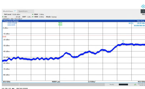
NTNV-n77(3450-3550)-PC1.5-30-15-M-DFT-BPSK-Inner_1RB_Left-20000-40000-PASS
