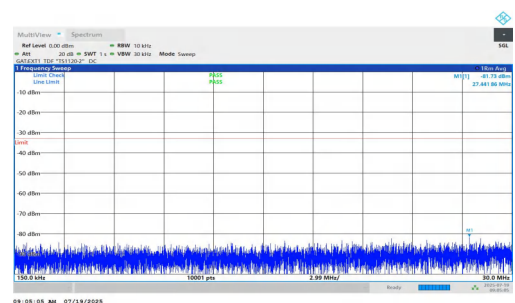
NTNV-n77(3450-3550)-PC1.5-30-15-M-DFT-QPSK-Inner_1RB_Left-0 15-30-PASS
