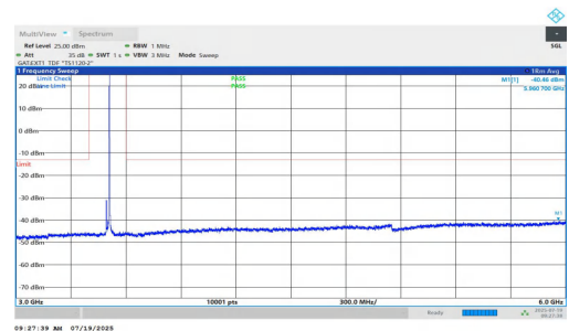
NTNV-n77(3450-3550)-PC1.5-30-20-M-DFT-QPSK-Inner_1RB_Right- 3000-6000-PASS
