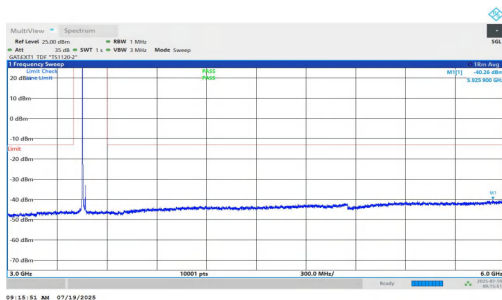
NTNV-n77(3450-3550)-PC1.5-30-20-L-DFT-BPSK-Inner_1RB_Left-3000-6000-PASS
