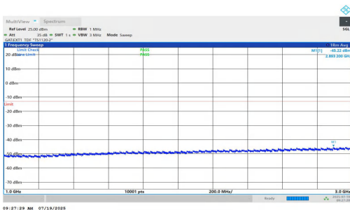
NTNV-n77(3450-3550)-PC1.5-30-20-M-DFT-QPSK-Inner_1RB_Right- 1000-3000-PASS
