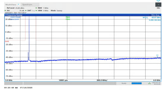
NTNV-n77(3450-3550)-PC1.5-30-20-L-DFT-QPSK-Inner_1RB_Right-3000-6000-PASS
