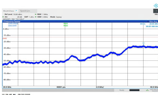
NTNV-n77(3450-3550)-PC1.5-30-20-L-DFT-BPSK-Inner_1RB_Left-20000-40000-PASS
