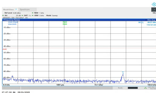
NTNV-n77(3450-3550)-PC1.5-30-15-H-DFT-BPSK-Inner_1RB_Left-0.009-0.15-PASS
