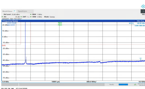
NTNV-n77(3450-3550)-PC1.5-30-20-M-DFT-QPSK-Inner_1RB_Left-3000-6000-PASS
