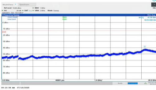
NTNV-n77(3450-3550)-PC1.5-30-15-H-DFT-BPSK-Inner_1RB_Right-6000-20000-PASS
