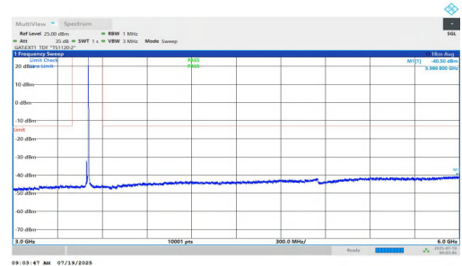
NTNV-n77(3450-3550)-PC1.5-30-15-M-DFT-BPSK-Inner_1RB_Right-3 000-6000-PASS
