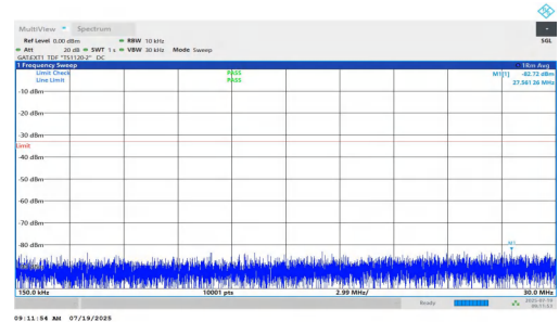
NTNV-n77(3450-3550)-PC1.5-30-15-H-DFT-QPSK-Inner_1RB_Left-0.15-30-PASS
