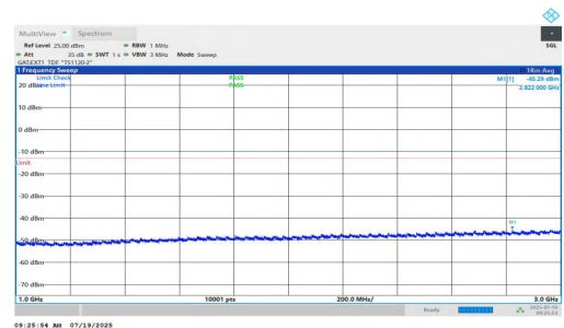
NTNV-n77(3450-3550)-PC1.5-30-20-M-DFT-QPSK-Inner_1RB_Left-1000-3000-PASS
