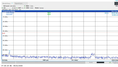
NTNV-n77(3450-3550)-PC1.5-30-15-M-DFT-BPSK-Inner_1RB_Left-0.009-0.15-PASS
