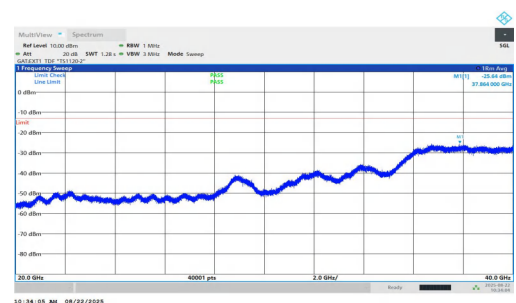
NTNV-n77(3450-3550)-PC1.5-30-15-H-DFT-QPSK-Inner_1RB_Right-2 0000-40000-PASS
