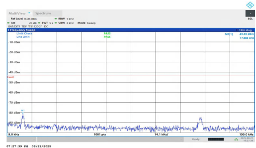
NTNV-n77(3450-3550)-PC1.5-30-15-H-DFT-BPSK-Inner_1RB_Right-0 .009-0.15-PASS
