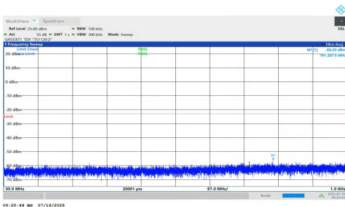
NTNV-n77(3450-3550)-PC1.5-30-20-M-DFT-QPSK-Inner_1RB_Left-30-1000-PASS
