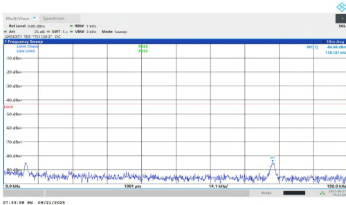
NTNV-n77(3450-3550)-PC1.5-30-20-M-DFT-QPSK-Inner_1RB_Left-0.009-0.15-PASS
