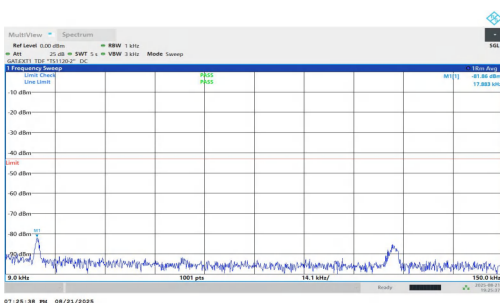
NTNV-n77(3450-3550)-PC1.5-30-15-M-DFT-QPSK-Inner_1RB_Left-0 .009-0.15-PASS
