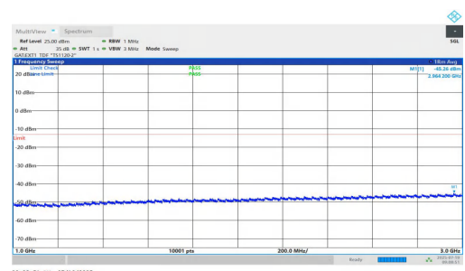
NTNV-n77(3450-3550)-PC1.5-30-15-H-DFT-BPSK-Inner_1RB_Left-1000-3000-PASS
