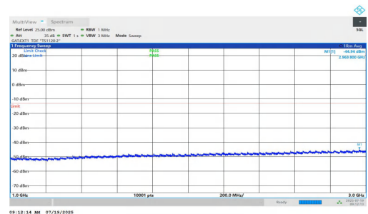
NTNV-n77(3450-3550)-PC1.5-30-15-H-DFT-QPSK-Inner_1RB_Left-1000-3000-PASS
