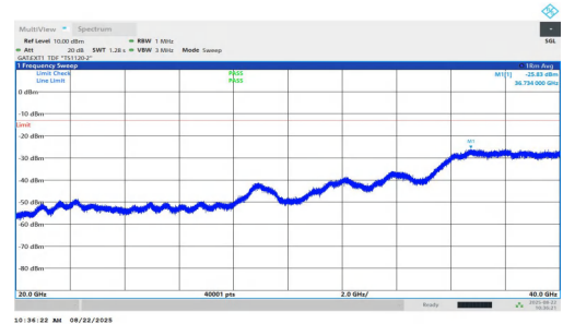
NTNV-n77(3450-3550)-PC1.5-30-20-L-DFT-QPSK-Inner_1RB_Right-20000-40000-PASS
