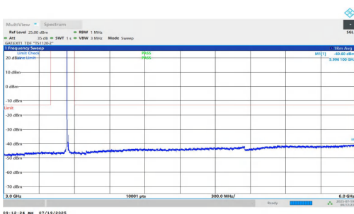
NTNV-n77(3450-3550)-PC1.5-30-15-H-DFT-QPSK-Inner_1RB_Left-3000-6000-PASS
