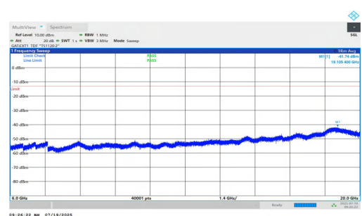
NTNV-n77(3450-3550)-PC1.5-30-20-M-DFT-QPSK-Inner_1RB_Left-6000-20000-PASS
