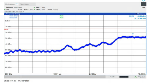
NTNV-n77(3450-3550)-PC1.5-30-15-H-DFT-BPSK-Inner_1RB_Right-20000-40000-PASS
