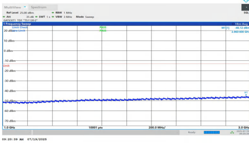
NTNV-n77(3450-3550)-PC1.5-30-20-L-DFT-QPSK-Inner_1RB_Right-1000-3000-PASS
