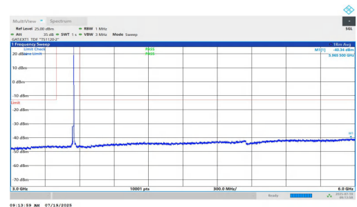
NTNV-n77(3450-3550)-PC1.5-30-15-H-DFT-QPSK-Inner_1RB_Right-3 000-6000-PASS
