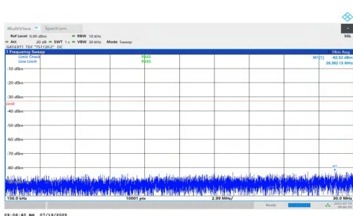
NTNV-n77(3450-3550)-PC1.5-30-15-M-DFT-QPSK-Inner_1RB_Right- 0.15-30-PASS
