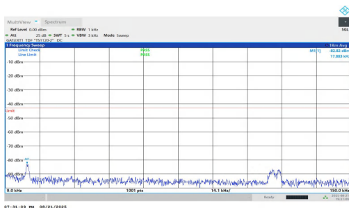
NTNV-n77(3450-3550)-PC1.5-30-20-L-DFT-QPSK-Inner_1RB_Left-0.009-0.15-PASS
