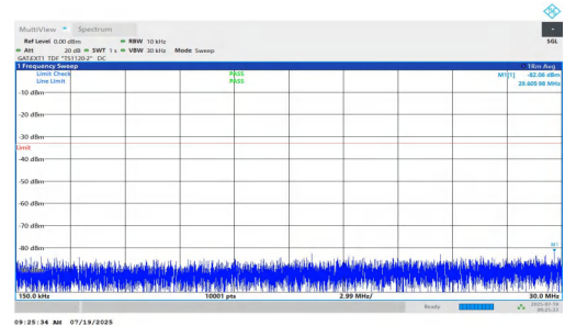
NTNV-n77(3450-3550)-PC1.5-30-20-M-DFT-QPSK-Inner_1RB_Left-0.15-30-PASS
