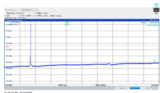
NTVN-n77(3450-3550)-PC1.5-30-20-M-DFT-BPSK-Inner_1RB_Right-3 000-6000-PASS
