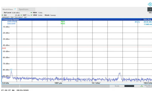
NTNV-n77(3450-3550)-PC1.5-30-20-M-DFT-BPSK-Inner_1RB_Left-0.009-0.15-PASS
