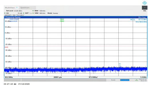
NTNV-n77(3450-3550)-PC1.5-30-20-M-DFT-QPSK-Inner_1RB_Right- 30-1000-PASS
