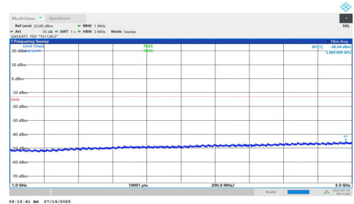
NTNV-n77(3450-3550)-PC1.5-30-20-L-DFT-BPSK-Inner_1RB_Left-1000-3000-PASS
