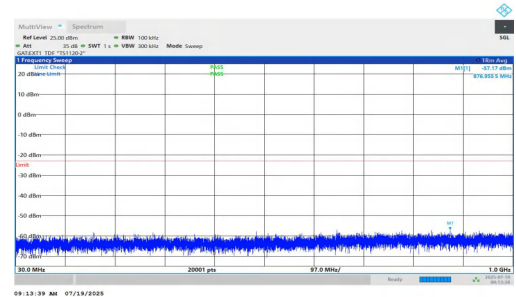
NTNV-n77(3450-3550)-PC1.5-30-15-H-DFT-QPSK-Inner_1RB_Right-3 0-1000-PASS
