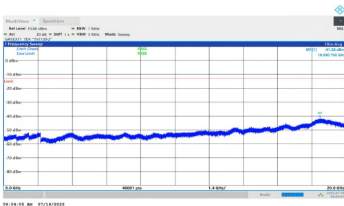
NTNV-n77(3450-3550)-PC1.5-30-15-M-DFT-BPSK-Inner_1RB_Right-6000-20000-PASS
