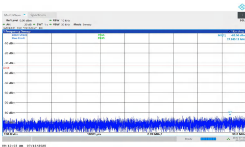
NTNV-n77(3450-3550)-PC1.5-30-15-H-DFT-BPSK-Inner_1RB_Right- 0.15-30-PASS
