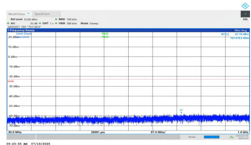
NTVN-n77(3450-3550)-PC1.5-30-20-M-DFT-BPSK-Inner_1RB_Right-3 0-1000-PASS
