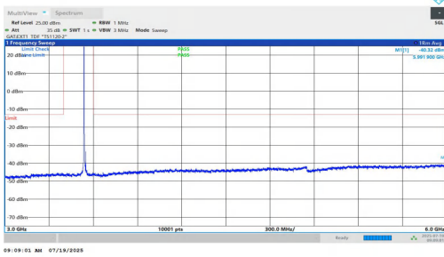
NTNV-n77(3450-3550)-PC1.5-30-15-H-DFT-BPSK-Inner_1RB_Left-3 000-6000-PASS
