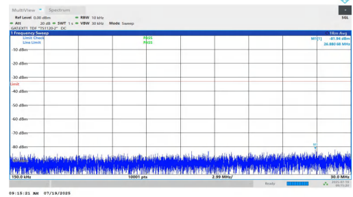
NTNV-n77(3450-3550)-PC1.5-30-20-L-DFT-BPSK-Inner_1RB_Left-0.15-30-PASS
