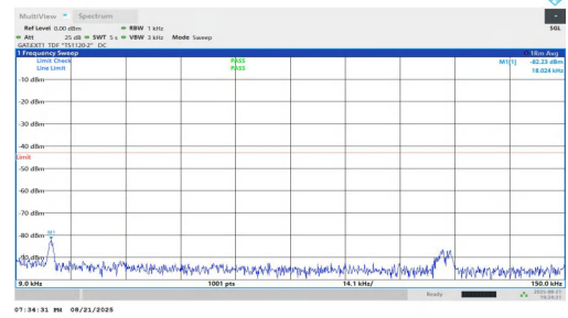
NTNV-n77(3450-3550)-PC1.5-30-20-M-DFT-QPSK-Inner_1RB_Right- 0.009-0.15-PASS
