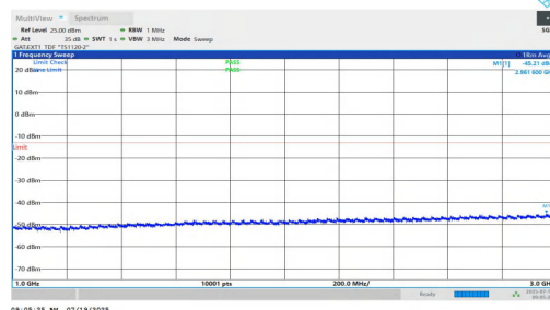
NTNV-n77(3450-3550)-PC1.5-30-15-M-DFT-QPSK-Inner_1RB_Left-10 00-3000-PASS
