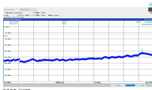
NTNV-n77(3450-3550)-PC1.5-30-15-M-DFT-QPSK-Inner_1RB_Left-60 00-20000-PASS
