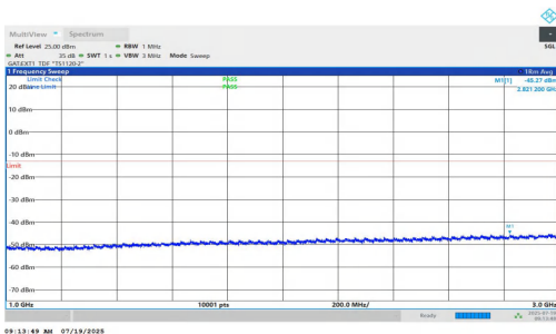
NTNV-n77(3450-3550)-PC1.5-30-15-H-DFT-QPSK-Inner_1RB_Right- 1000-3000-PASS
