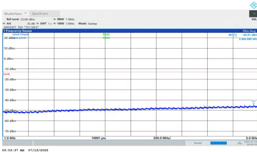
NTNV-n77(3450-3550)-PC1.5-30-15-M-DFT-BPSK-Inner_1RB_Right-1000-3000-PASS
