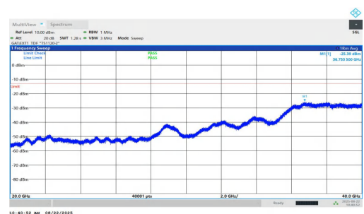
NTNV-n77(3450-3550)-PC1.5-30-20-M-DFT-QPSK-Inner_1RB_Right- 20000-40000-PASS
