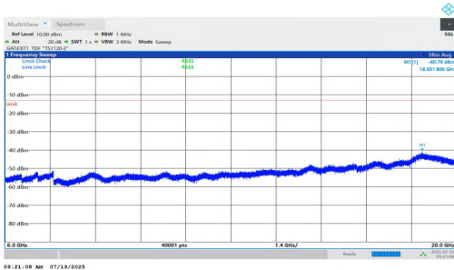
NTNV-n77(3450-3550)-PC1.5-30-20-L-DFT-QPSK-Inner_1RB_Right-6000-20000-PASS
