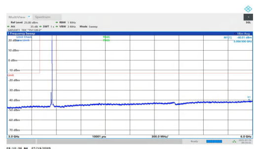
NTNV-n77(3450-3550)-PC1.5-30-15-H-DFT-BPSK-Inner_1RB_Right-3 000-6000-PASS
