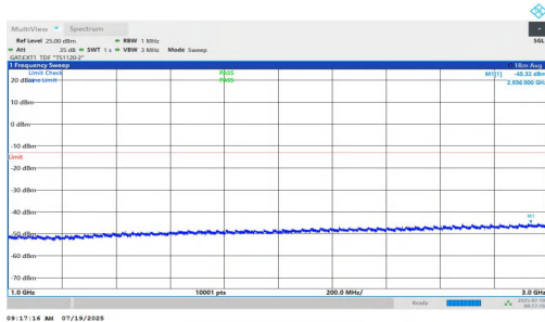
NTNV-n77(3450-3550)-PC1.5-30-20-L-DFT-BPSK-Inner_1RB_Right-1000-3000-PASS
