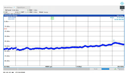
NTNV-n77(3450-3550)-PC1.5-30-20-L-DFT-BPSK-Inner_1RB_Left-6000-20000-PASS
