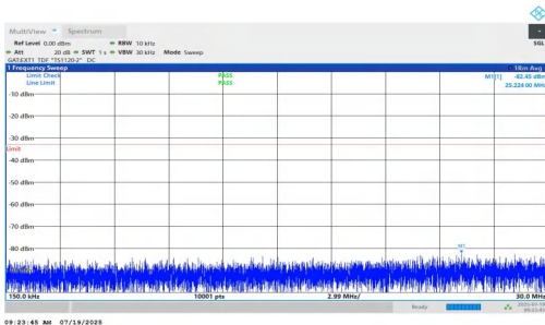
NTVN-n77(3450-3550)-PC1.5-30-20-M-DFT-BPSK-Inner_1RB_Right- 0.15-30-PASS
