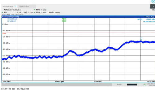
NTVN-n77(3450-3550)-PC1.5-30-20-M-DFT-BPSK-Inner_1RB_Left-2 0000-40000-PASS
