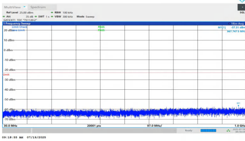
NTNV-n77(3450-3550)-PC1.5-30-20-L-DFT-QPSK-Inner_1RB_Left-3 0-1000-PASS
