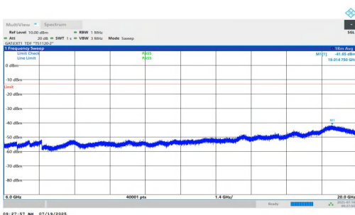
NTNV-n77(3450-3550)-PC1.5-30-20-M-DFT-QPSK-Inner_1RB_Right- 6000-20000-PASS
