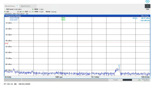
NTVN-n77(3450-3550)-PC1.5-30-20-M-DFT-BPSK-Inner_1RB_Right-0 .009-0.15-PASS
