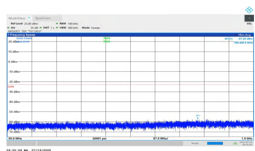
NTNV-n77(3450-3550)-PC1.5-30-20-L-DFT-QPSK-Inner_1RB_Right-3 0-1000-PASS
