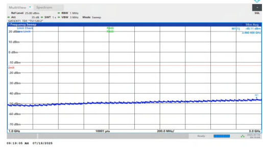
NTNV-n77(3450-3550)-PC1.5-30-20-L-DFT-QPSK-Inner_1RB_Left-10 00-3000-PASS
