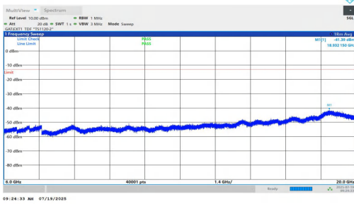
NTNV-n77(3450-3550)-PC1.5-30-20-M-DFT-BPSK-Inner_1RB_Right-6000-20000-PASS
