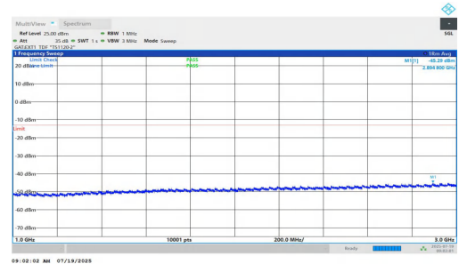
NTNV-n77(3450-3550)-PC1.5-30-15-M-DFT-BPSK-Inner_1RB_Left-1000-3000-PASS
