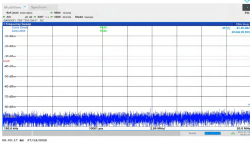
NTNV-n77(3450-3550)-PC1.5-30-15-M-DFT-BPSK-Inner_1RB_Right-0.15-30-PASS
