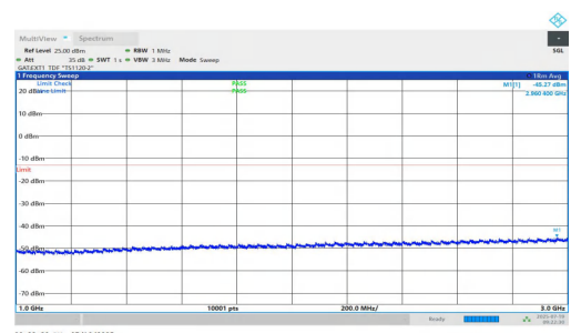
NTNV-n77(3450-3550)-PC1.5-30-20-M-DFT-BPSK-Inner_1RB_Left-1000-3000-PASS
