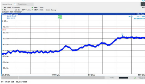
NTNV-n77(3450-3550)-PC1.5-30-20-M-DFT-QPSK-Inner_1RB_Left-2 0000-40000-PASS
