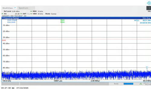
NTNV-n77(3450-3550)-PC1.5-30-20-M-DFT-QPSK-Inner_1RB_Right- 0.15-30-PASS
