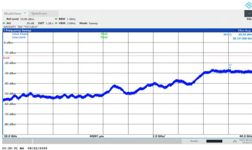
NTNV-n77(3450-3550)-PC1.5-30-15-H-DFT-BPSK-Inner_1RB_Left-2 0000-40000-PASS
