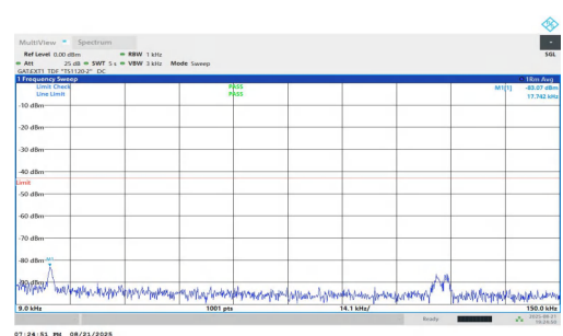
NTNV-n77(3450-3550)-PC1.5-30-15-M-DFT-BPSK-Inner_1RB_Right-0.009-0.15-PASS
