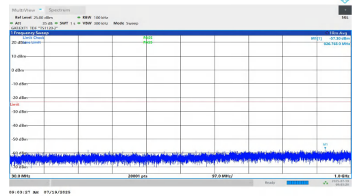
NTNV-n77(3450-3550)-PC1.5-30-15-M-DFT-BPSK-Inner_1RB_Right-3 0-1000-PASS
