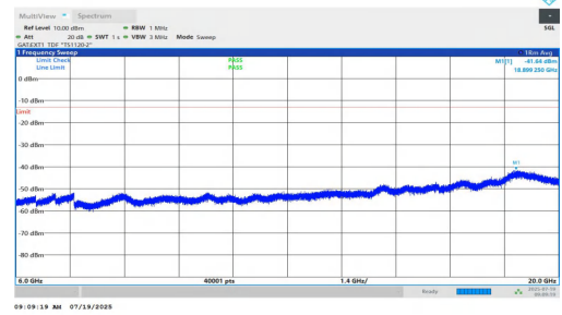
NTNV-n77(3450-3550)-PC1.5-30-15-H-DFT-BPSK-Inner_1RB_Left-60 00-20000-PASS
