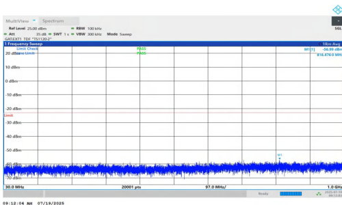
NTNV-n77(3450-3550)-PC1.5-30-15-H-DFT-QPSK-Inner_1RB_Left-30-1000-PASS
