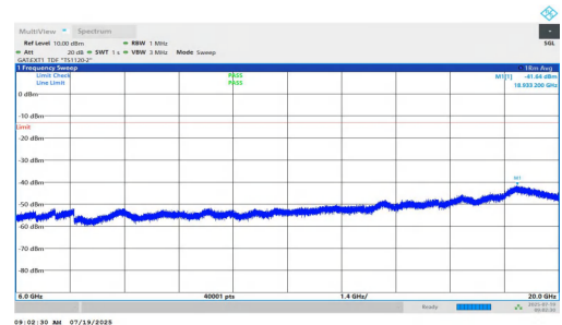
NTNV-n77(3450-3550)-PC1.5-30-15-M-DFT-BPSK-Inner_1RB_Left-6000-20000-PASS
