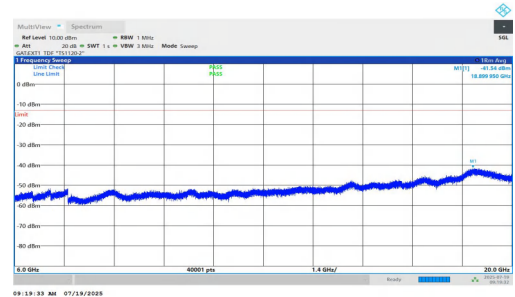
NTNV-n77(3450-3550)-PC1.5-30-20-L-DFT-QPSK-Inner_1RB_Left-60 00-20000-PASS
