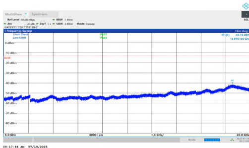
NTNV-n77(3450-3550)-PC1.5-30-20-L-DFT-BPSK-Inner_1RB_Right-6000-20000-PASS
