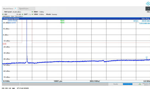
NTNV-n77(3450-3550)-PC1.5-30-15-M-DFT-BPSK-Inner_1RB_Left-3000-6000-PASS
