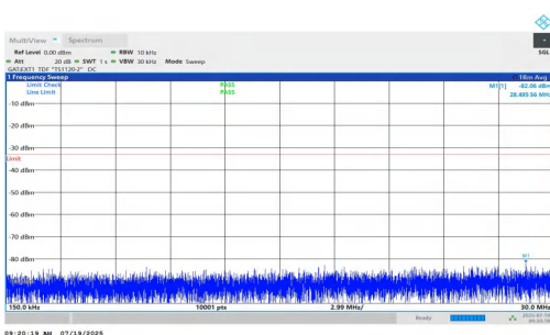
NTNV-n77(3450-3550)-PC1.5-30-20-L-DFT-QPSK-Inner_1RB_Right- 0.15-30-PASS
