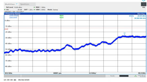
NTNV-n77(3450-3550)-PC1.5-30-20-M-DFT-BPSK-Inner_1RB_Right-20000-40000-PASS
