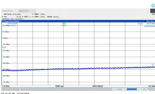
NTNV-n77(3450-3550)-PC1.5-30-15-H-DFT-BPSK-Inner_1RB_Right- 1000-3000-PASS
