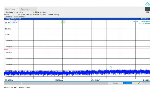
NTNV-n77(3450-3550)-PC1.5-30-15-H-DFT-BPSK-Inner_1RB_Right-3 0-1000-PASS
