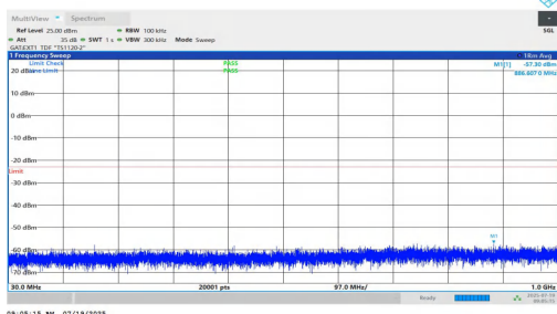
NTNV-n77(3450-3550)-PC1.5-30-15-M-DFT-QPSK-Inner_1RB_Left-3 0-1000-PASS
