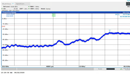
NTNV-n77(3450-3550)-PC1.5-30-15-L-DFT-QPSK-Inner_1RB_Left-2 0000-40000-PASS
