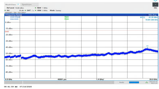
NTV-n77(3450-3550)-PC1.5-30-10-M-DFT-BPSK-Inner_1RB_Left-60 00-20000-PASS
