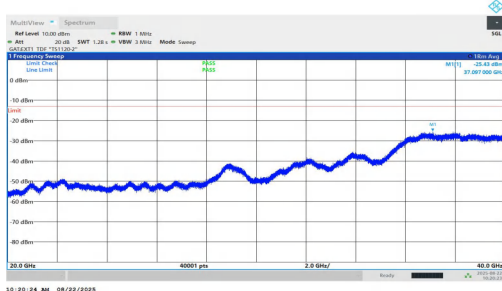
NTNV-n77(3450-3550)-PC1.5-30-10-L-DFT-BPSK-Inner_1RB_Left-20000-40000-PASS
