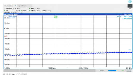
NTNV-n77(3450-3550)-PC1.5-30-10-H-DFT-BPSK-Inner_1RB_Left-1000-3000-PASS
