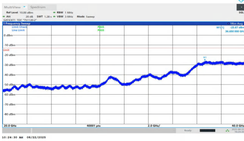
NTNV-n77(3450-3550)-PC1.5-30-10-M-DFT-QPSK-Inner_1RB_Left-2 0000-40000-PASS
