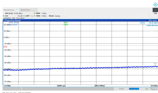
NTNV-n77(3450-3550)-PC1.5-30-10-L-DFT-BPSK-Inner_1RB_Right-1000-3000-PASS
