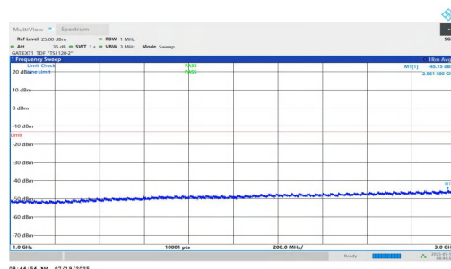
NTNV-n77(3450-3550)-PC1.5-30-10-M-DFT-QPSK-Inner_1RB_Left-1000-3000-PASS
