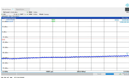
NTNV-n77(3450-3550)-PC1.5-30-15-L-DFT-BPSK-Inner_1RB_Right- 1000-3000-PASS
