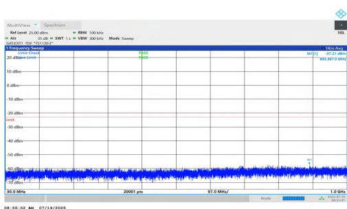
NTNV-n77(3450-3550)-PC1.5-30-15-L-DFT-BPSK-Inner_1RB_Left-30-1000-PASS
