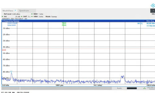
NTNV-n77(3450-3550)-PC1.5-30-10-H-DFT-QPSK-Inner_1RB_Left-0.009-0.15-PASS
