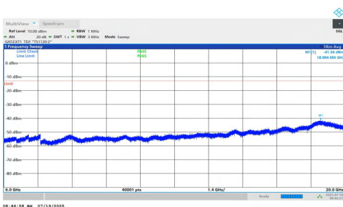
NTNV-n77(3450-3550)-PC1.5-30-10-M-DFT-QPSK-Inner_1RB_Right- 6000-20000-PASS
