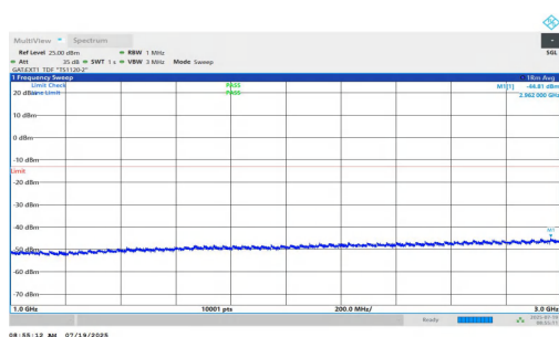
NTNV-n77(3450-3550)-PC1.5-30-15-L-DFT-BPSK-Inner_1RB_Left-1000-3000-PASS
