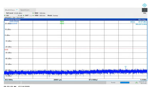
NTNV-n77(3450-3550)-PC1.5-30-10-H-DFT-QPSK-Inner_1RB_Right-3 0-1000-PASS
