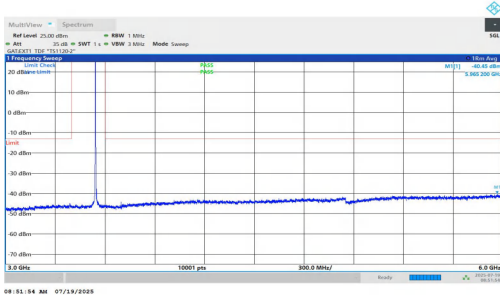
NTNV-n77(3450-3550)-PC1.5-30-10-H-DFT-QPSK-Inner_1RB_Left-3 000-6000-PASS
