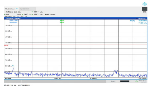
NTNV-n77(3450-3550)-PC1.5-30-10-L-DFT-QPSK-Inner_1RB_Right-0 .009-0.15-PASS
