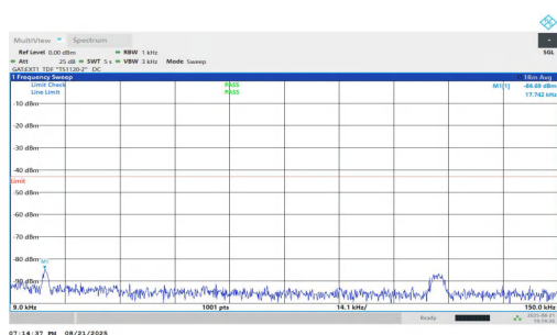
NTNV-n77(3450-3550)-PC1.5-30-10-L-DFT-QPSK-Inner_1RB_Left-0.009-0.15-PASS
