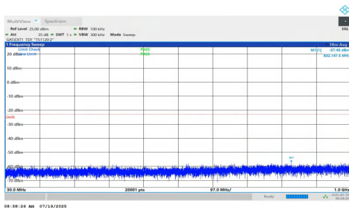
NTNV-n77(3450-3550)-PC1.5-30-15-L-DFT-QPSK-Inner_1RB_Left-30-1000-PASS
