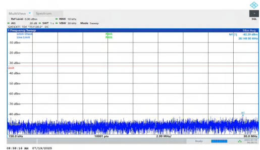
NTNV-n77(3450-3550)-PC1.5-30-15-L-DFT-QPSK-Inner_1RB_Left-0.15-5-30-PASS
