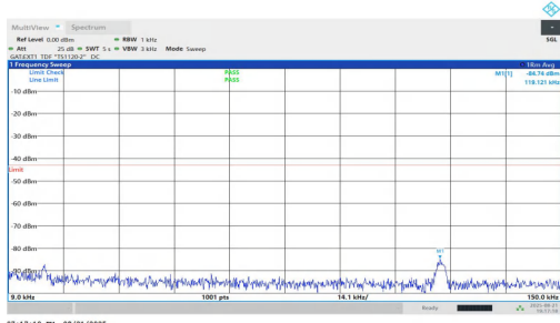
NTNV-n77(3450-3550)-PC1.5-30-10-M-DFT-QPSK-Inner_1RB_Left-0.009-0.15-PASS
