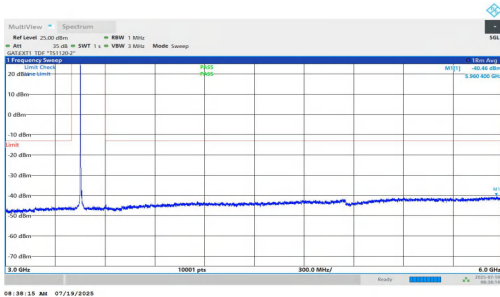
NTNV-n77(3450-3550)-PC1.5-30-10-L-DFT-QPSK-Inner_1RB_Left-3 000-6000-PASS
