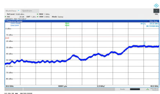
NTNV-n77(3450-3550)-PC1.5-30-15-L-DFT-QPSK-Inner_1RB_Right-2 0000-40000-PASS
