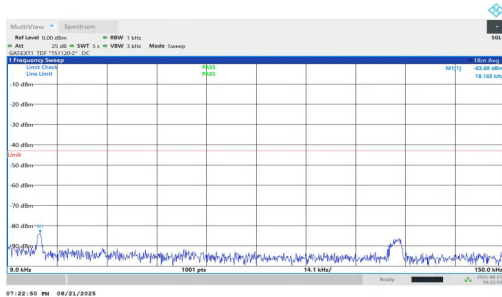
NTNV-n77(3450-3550)-PC1.5-30-15-L-DFT-QPSK-Inner_1RB_Left-0.009-0.15-PASS
