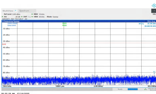
NTNV-n77(3450-3550)-PC1.5-30-10-H-DFT-QPSK-Inner_1RB_Right- 0.15-30-PASS
