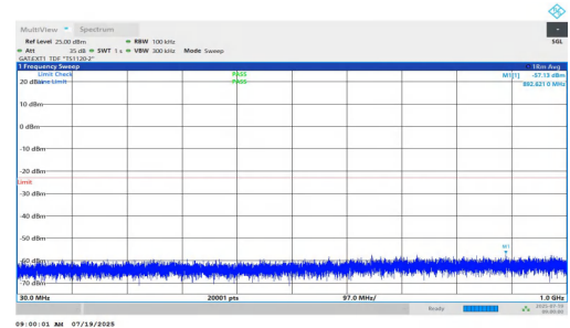
NTNV-n77(3450-3550)-PC1.5-30-15-L-DFT-QPSK-Inner_1RB_Right-3 0-1000-PASS
