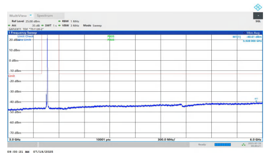
NTNV-n77(3450-3550)-PC1.5-30-15-L-DFT-QPSK-Inner_1RB_Right-3 000-6000-PASS
