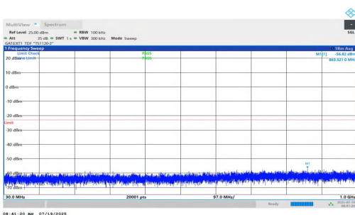
NTNV-n77(3450-3550)-PC1.5-30-10-M-DFT-BPSK-Inner_1RB_Left-30-1000-PASS
