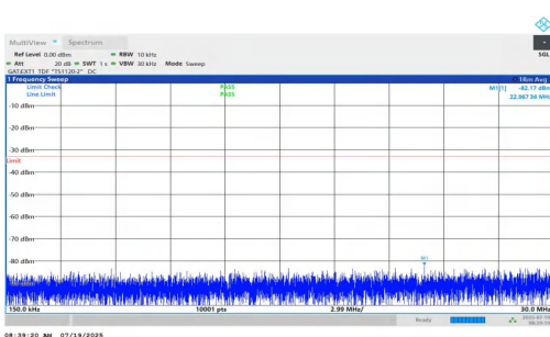
NTNV-n77(3450-3550)-PC1.5-30-10-L-DFT-QPSK-Inner_1RB_Right- 0.15-30-PASS
