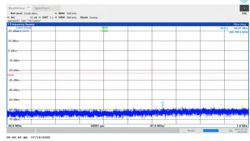
NTNV-n77(3450-3550)-PC1.5-30-10-H-DFT-BPSK-Inner_1RB_Right-3 0-1000-PASS
