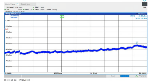
NTNV-n77(3450-3550)-PC1.5-30-10-L-DFT-BPSK-Inner_1RB_Left-6000-20000-PASS
