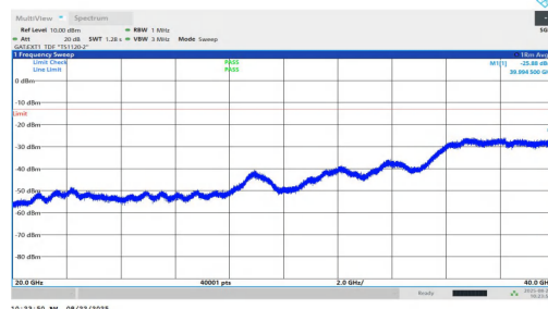
NTNV-n77(3450-3550)-PC1.5-30-10-M-DFT-BPSK-Inner_1RB_Right-20000-40000-PASS
