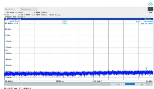
NTNV-n77(3450-3550)-PC1.5-30-15-L-DFT-BPSK-Inner_1RB_Right-3 0-1000-PASS
