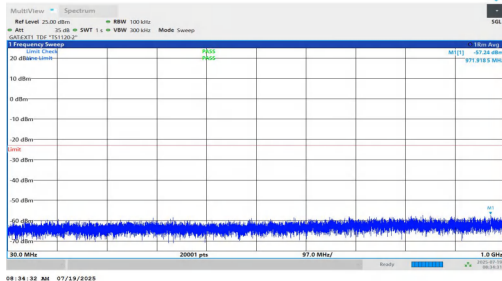
NTNV-n77(3450-3550)-PC1.5-30-10-L-DFT-BPSK-Inner_1RB_Left-30-1000-PASS
