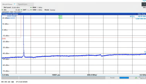
NTNV-n77(3450-3550)-PC1.5-30-15-L-DFT-BPSK-Inner_1RB_Left-30 00-6000-PASS
