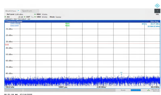
NTNV-n77(3450-3550)-PC1.5-30-10-H-DFT-QPSK-Inner_1RB_Left-0.15-30-PASS
