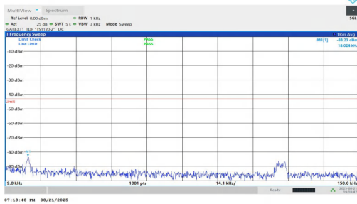
NTNV-n77(3450-3550)-PC1.5-30-10-H-DFT-BPSK-Inner_1RB_Left-0.009-0.15-PASS
