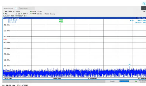
NTNV-n77(3450-3550)-PC1.5-30-15-L-DFT-BPSK-Inner_1RB_Left-0.15-5-30-PASS
