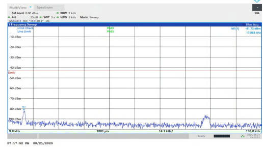
NTNV-n77(3450-3550)-PC1.5-30-10-M-DFT-QPSK-Inner_1RB_Right- 0.009-0.15-PASS
