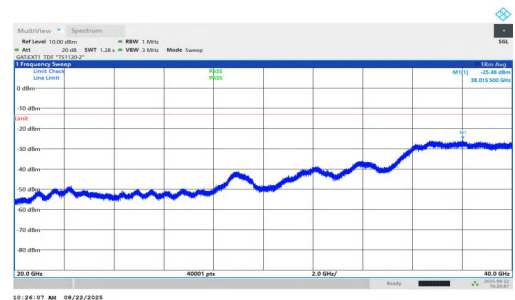
NTNV-n77(3450-3550)-PC1.5-30-10-H-DFT-BPSK-Inner_1RB_Right-2 0000-40000-PASS
