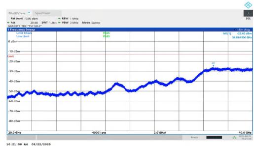
NTNV-n77(3450-3550)-PC1.5-30-10-L-DFT-QPSK-Inner_1RB_Right-20000-40000-PASS
