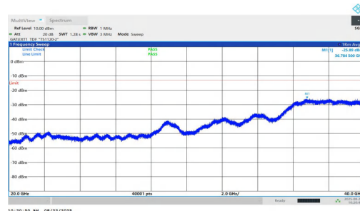
NTNV-n77(3450-3550)-PC1.5-30-10-L-DFT-BPSK-Inner_1RB_Right-2 0000-40000-PASS
