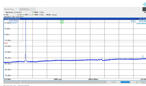
NTNV-n77(3450-3550)-PC1.5-30-10-L-DFT-BPSK-Inner_1RB_Right-3 000-6000-PASS
