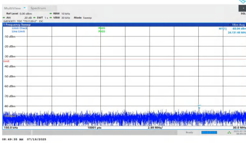
NTNV-n77(3450-3550)-PC1.5-30-10-H-DFT-BPSK-Inner_1RB_Right-0.15-30-PASS
