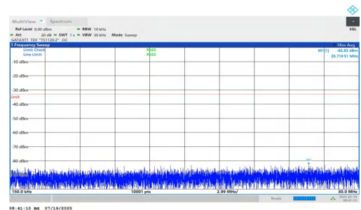
NTNV-n77(3450-3550)-PC1.5-30-10-M-DFT-BPSK-Inner_1RB_Left-0.15-30-PASS
