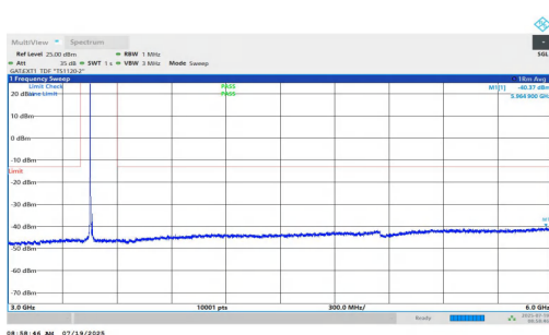
NTNV-n77(3450-3550)-PC1.5-30-15-L-DFT-QPSK-Inner_1RB_Left-3000-6000-PASS
