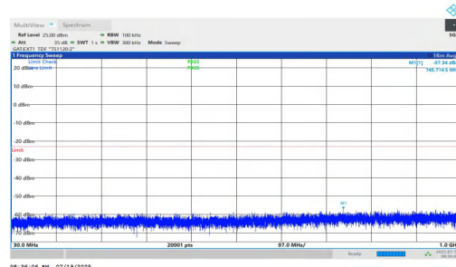
NTNV-n77(3450-3550)-PC1.5-30-10-L-DFT-BPSK-Inner_1RB_Right-3 0-1000-PASS
