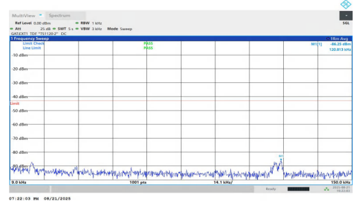
NTNV-n77(3450-3550)-PC1.5-30-15-L-DFT-BPSK-Inner_1RB_Right-0. 009-0.15-PASS
