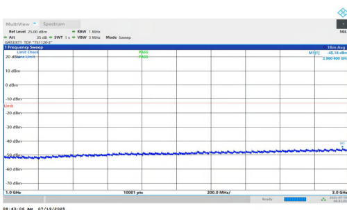
NTV-n77(3450-3550)-PC1.5-30-10-M-DFT-BPSK-Inner_1RB_Right- 1000-3000-PASS
