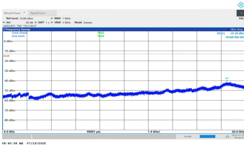
NTNV-n77(3450-3550)-PC1.5-30-10-L-DFT-QPSK-Inner_1RB_Right-6000-20000-PASS
