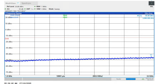
NTNV-n77(3450-3550)-PC1.5-30-10-L-DFT-BPSK-Inner_1RB_Left-1000-3000-PASS
