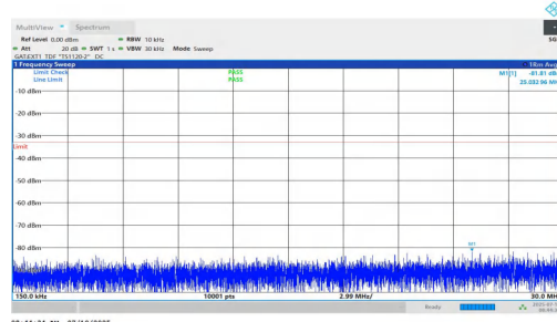
NTNV-n77(3450-3550)-PC1.5-30-10-M-DFT-QPSK-Inner_1RB_Left-0.15-30-PASS
