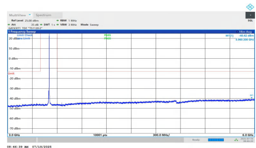
NTNV-n77(3450-3550)-PC1.5-30-10-M-DFT-QPSK-Inner_1RB_Right- 3000-6000-PASS
