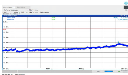
NTNV-n77(3450-3550)-PC1.5-30-10-L-DFT-BPSK-Inner_1RB_Right-6000-20000-PASS
