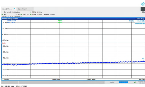
NTNV-n77(3450-3550)-PC1.5-30-10-M-DFT-QPSK-Inner_1RB_Right- 1000-3000-PASS
