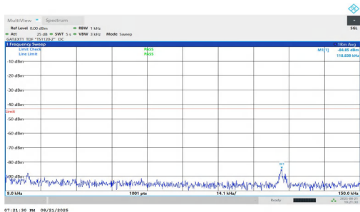
NTNV-n77(3450-3550)-PC1.5-30-15-L-DFT-BPSK-Inner_1RB_Left-0.009-0.15-PASS
