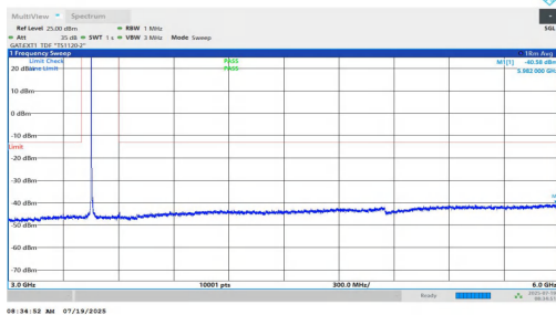
NTNV-n77(3450-3550)-PC1.5-30-10-L-DFT-BPSK-Inner_1RB_Left-3000-6000-PASS
