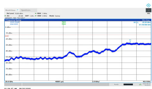
NTNV-n77(3450-3550)-PC1.5-30-10-M-DFT-QPSK-Inner_1RB_Right- 20000-40000-PASS
