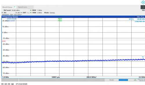
NTNV-n77(3450-3550)-PC1.5-30-10-H-DFT-BPSK-Inner_1RB_Right-1000-3000-PASS
