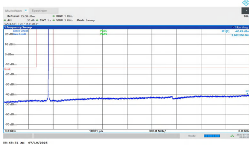
NTNV-n77(3450-3550)-PC1.5-30-10-H-DFT-BPSK-Inner_1RB_Left-3000-6000-PASS
