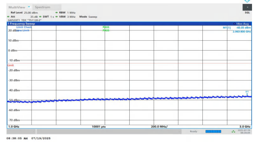
NTNV-n77(3450-3550)-PC1.5-30-10-L-DFT-QPSK-Inner_1RB_Left-10 00-3000-PASS
