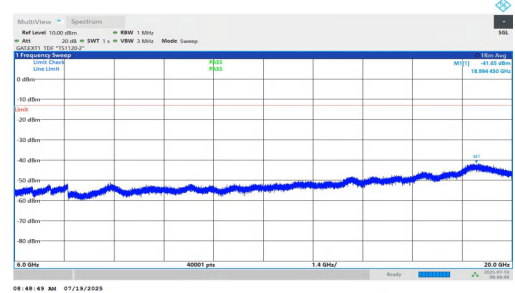
NTNV-n77(3450-3550)-PC1.5-30-10-H-DFT-BPSK-Inner_1RB_Left-6000-20000-PASS
