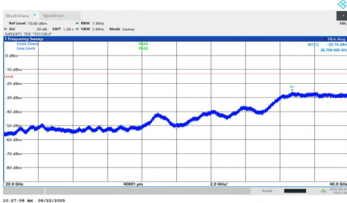
NTNV-n77(3450-3550)-PC1.5-30-15-L-DFT-BPSK-Inner_1RB_Left-20 000-40000-PASS
