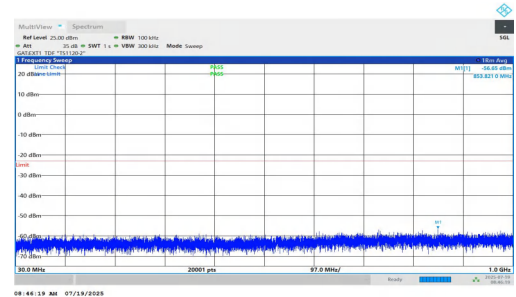
NTNV-n77(3450-3550)-PC1.5-30-10-M-DFT-QPSK-Inner_1RB_Right- 30-1000-PASS
