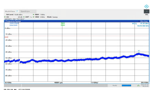
NTNV-n77(3450-3550)-PC1.5-30-15-L-DFT-QPSK-Inner_1RB_Left-6000-20000-PASS
