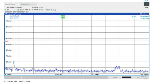
NTNV-n77(3450-3550)-PC1.5-30-15-L-DFT-QPSK-Inner_1RB_Right-0 .009-0.15-PASS
