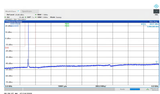
NTNV-n77(3450-3550)-PC1.5-30-15-L-DFT-BPSK-Inner_1RB_Right-3 000-6000-PASS
