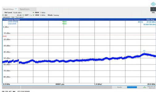
NTNV-n77(3450-3550)-PC1.5-30-10-H-DFT-QPSK-Inner_1RB_Right-6000-20000-PASS
