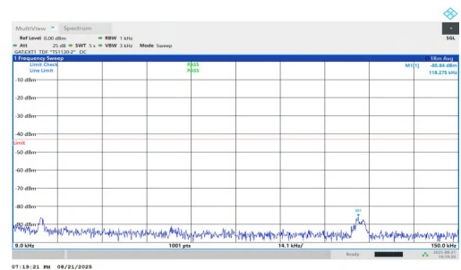
NTNV-n77(3450-3550)-PC1.5-30-10-H-DFT-BPSK-Inner_1RB_Right-0.009-0.15-PASS
