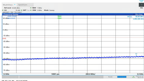
NTNV-n77(3450-3550)-PC1.5-30-10-H-DFT-QPSK-Inner_1RB_Right-1000-3000-PASS
