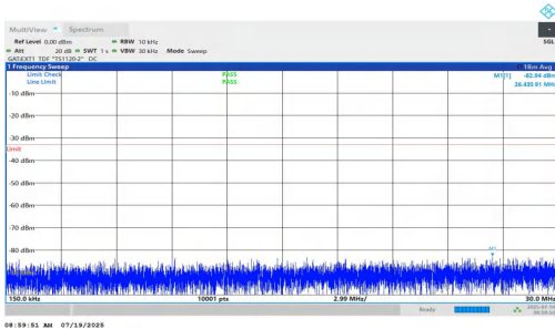
NTNV-n77(3450-3550)-PC1.5-30-15-L-DFT-QPSK-Inner_1RB_Right- 0.15-30-PASS
