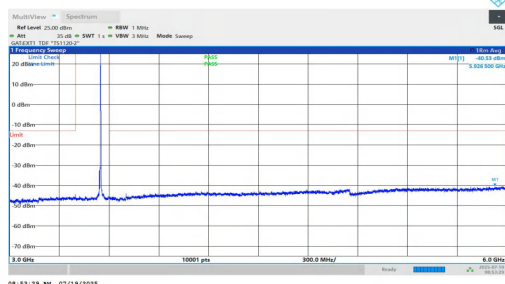
NTNV-n77(3450-3550)-PC1.5-30-10-H-DFT-QPSK-Inner_1RB_Right-3000-6000-PASS
