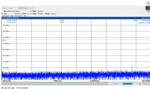
NTNV-n77(3450-3550)-PC1.5-30-10-M-DFT-QPSK-Inner_1RB_Right- 0.15-30-PASS
