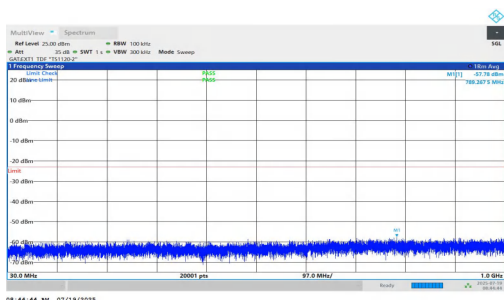
NTNV-n77(3450-3550)-PC1.5-30-10-M-DFT-QPSK-Inner_1RB_Left-30-1000-PASS
