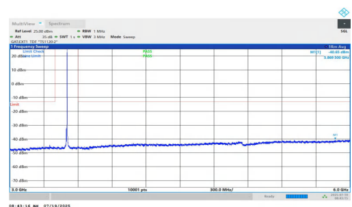
NTV-n77(3450-3550)-PC1.5-30-10-M-DFT-BPSK-Inner_1RB_Right-3 000-6000-PASS
