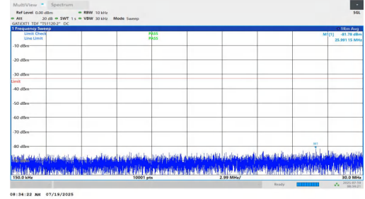
NTNV-n77(3450-3550)-PC1.5-30-10-L-DFT-BPSK-Inner_1RB_Left-0.15-30-PASS
