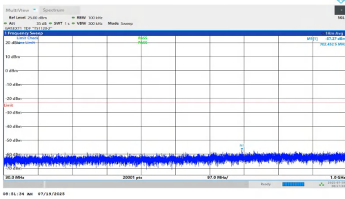
NTNV-n77(3450-3550)-PC1.5-30-10-H-DFT-QPSK-Inner_1RB_Left-3 0-1000-PASS
