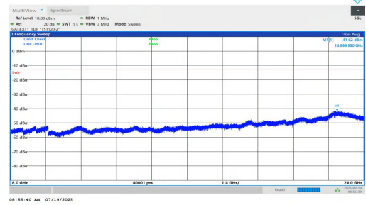
NTNV-n77(3450-3550)-PC1.5-30-15-L-DFT-BPSK-Inner_1RB_Left-60 00-20000-PASS
