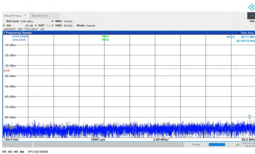
NTV-n77(3450-3550)-PC1.5-30-10-M-DFT-BPSK-Inner_1RB_Right- 0.15-30-PASS
