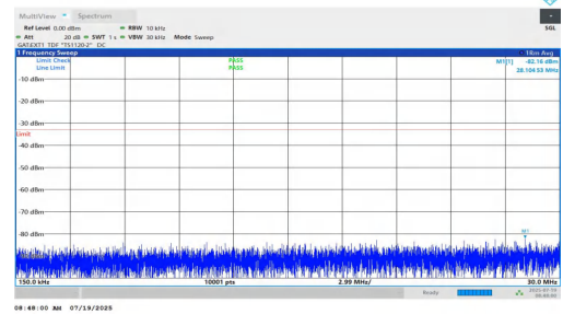
NTNV-n77(3450-3550)-PC1.5-30-10-H-DFT-BPSK-Inner_1RB_Left-0.15-30-PASS
