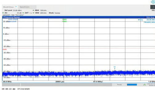
NTNV-n77(3450-3550)-PC1.5-30-10-H-DFT-BPSK-Inner_1RB_Left-300-1000-PASS
