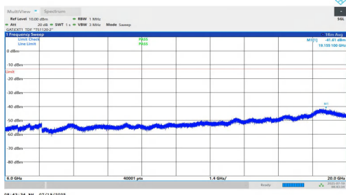
NTNV-n77(3450-3550)-PC1.5-30-10-M-DFT-BPSK-Inner_1RB_Right-6000-20000-PASS
