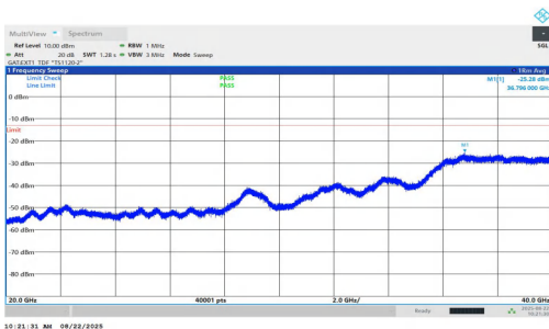
NTNV-n77(3450-3550)-PC1.5-30-10-L-DFT-QPSK-Inner_1RB_Left-2 0000-40000-PASS
