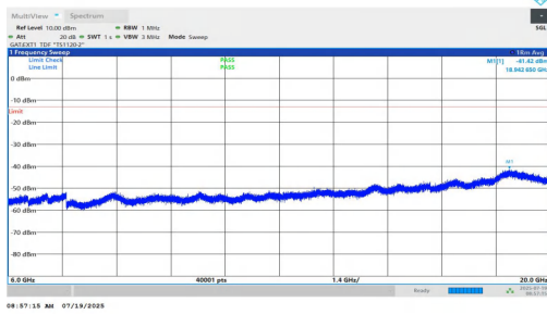
NTNV-n77(3450-3550)-PC1.5-30-15-L-DFT-BPSK-Inner_1RB_Right-6000-20000-PASS
