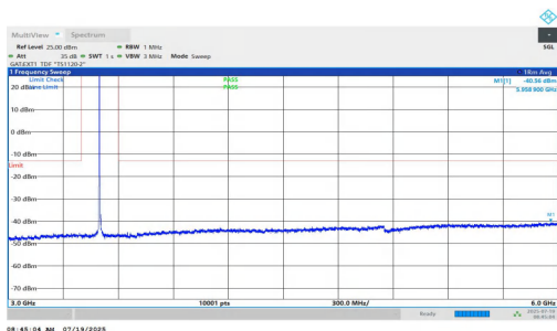
NTNV-n77(3450-3550)-PC1.5-30-10-M-DFT-QPSK-Inner_1RB_Left-3000-6000-PASS
