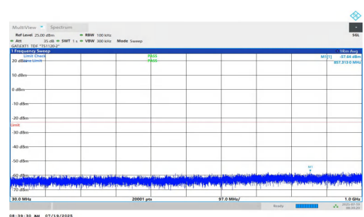
NTNV-n77(3450-3550)-PC1.5-30-10-L-DFT-QPSK-Inner_1RB_Right-3 0-1000-PASS
