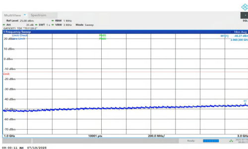
NTNV-n77(3450-3550)-PC1.5-30-15-L-DFT-QPSK-Inner_1RB_Right- 1000-3000-PASS
