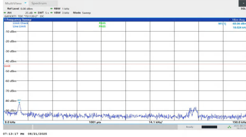
NTNV-n77(3450-3550)-PC1.5-30-10-L-DFT-BPSK-Inner_1RB_Left-0.009-0.15-PASS
