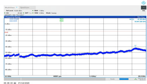
NTNV-n77(3450-3550)-PC1.5-30-10-L-DFT-QPSK-Inner_1RB_Left-60 00-20000-PASS
