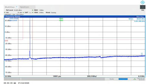
NTNV-n77(3450-3550)-PC1.5-30-10-H-DFT-BPSK-Inner_1RB_Right-3 000-6000-PASS
