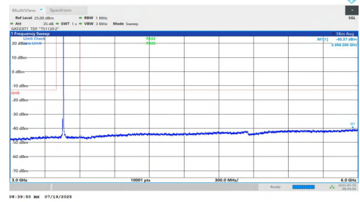
NTNV-n77(3450-3550)-PC1.5-30-10-L-DFT-QPSK-Inner_1RB_Right-3000-6000-PASS
