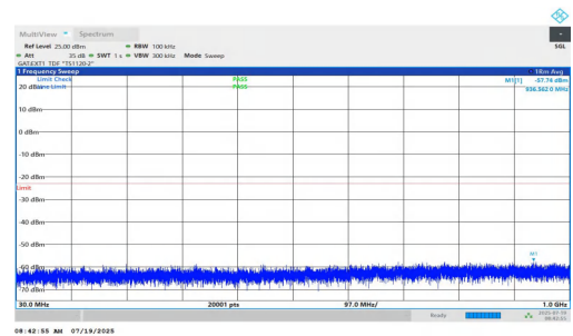
NTV-n77(3450-3550)-PC1.5-30-10-M-DFT-BPSK-Inner_1RB_Right-3 0-1000-PASS
