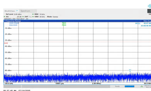
NTNV-n77(3450-3550)-PC1.5-30-10-L-DFT-QPSK-Inner_1RB_Left-0.1 5-30-PASS
