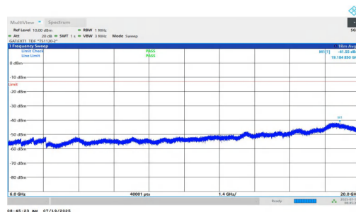
NTNV-n77(3450-3550)-PC1.5-30-10-M-DFT-QPSK-Inner_1RB_Left-6000-20000-PASS
