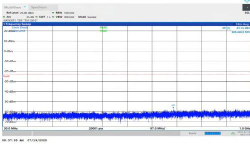
NTNV-n77(3450-3550)-PC1.5-30-10-L-DFT-QPSK-Inner_1RB_Left-3 0-1000-PASS
