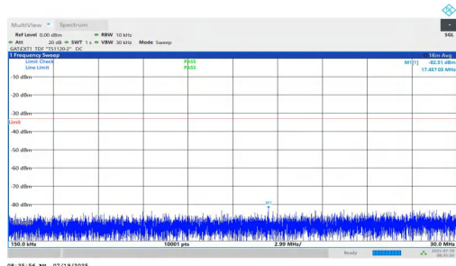
NTNV-n77(3450-3550)-PC1.5-30-10-L-DFT-BPSK-Inner_1RB_Right-0.15-30-PASS
