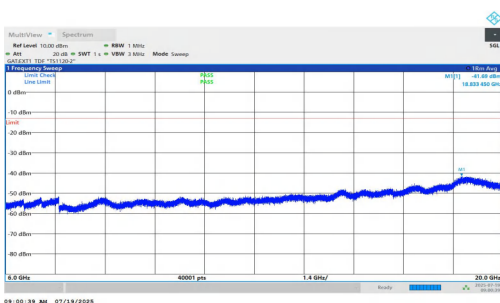
NTNV-n77(3450-3550)-PC1.5-30-15-L-DFT-QPSK-Inner_1RB_Right- 6000-20000-PASS
