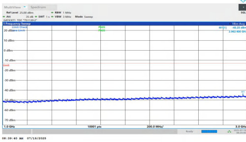
NTNV-n77(3450-3550)-PC1.5-30-10-L-DFT-QPSK-Inner_1RB_Right-1000-3000-PASS
