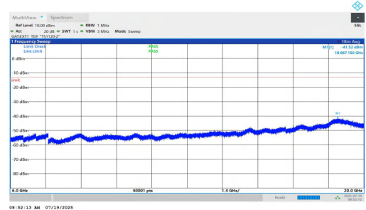
NTNV-n77(3450-3550)-PC1.5-30-10-H-DFT-QPSK-Inner_1RB_Left-60 00-20000-PASS
