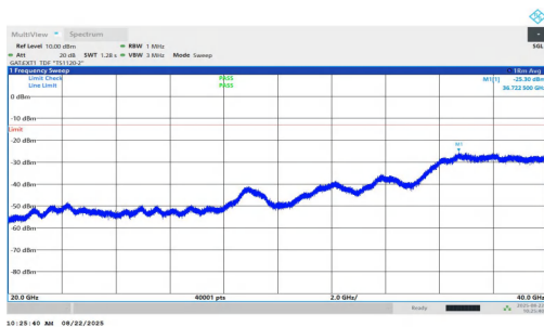
NTNV-n77(3450-3550)-PC1.5-30-10-H-DFT-BPSK-Inner_1RB_Left-20000-40000-PASS
