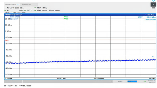
NTNV-n77(3450-3550)-PC1.5-30-10-H-DFT-QPSK-Inner_1RB_Left-10 00-3000-PASS
