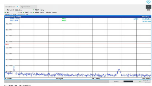
NTNV-n77(3450-3550)-PC1.5-30-10-L-DFT-BPSK-Inner_1RB_Right-0.009-0.15-PASS
