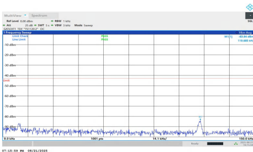
NTNV-n77(3450-3550)-PC1.5-30-10-M-DFT-BPSK-Inner_1RB_Left-0.009-0.15-PASS
