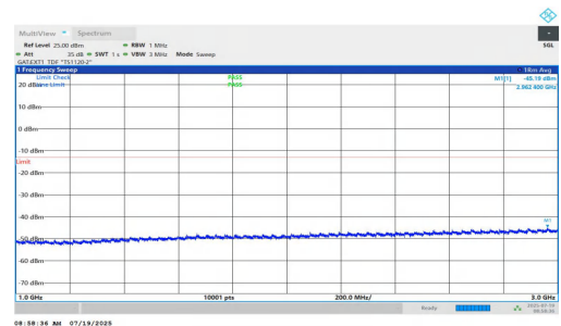
NTNV-n77(3450-3550)-PC1.5-30-15-L-DFT-QPSK-Inner_1RB_Left-1000-3000-PASS
