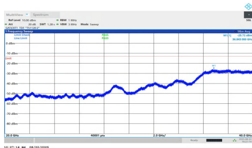
NTNV-n77(3450-3550)-PC1.5-30-10-H-DFT-QPSK-Inner_1RB_Right-20000-40000-PASS
