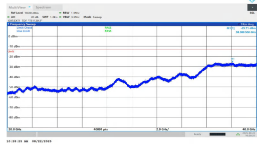
NTNV-n77(3450-3550)-PC1.5-30-15-L-DFT-BPSK-Inner_1RB_Right-20000-40000-PASS
