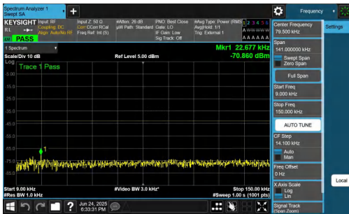
NTNV-n77(3450-3550)-PC2-30-10-H-DFT-BPSK-Inner_1RB_Left-0.0 09-0.15-PASS
