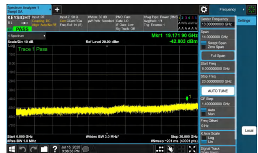
NTNV-n77(3450-3550)-PC2-30-10-H-DFT-BPSK-Inner_1RB_Left-6000 -20000-PASS
