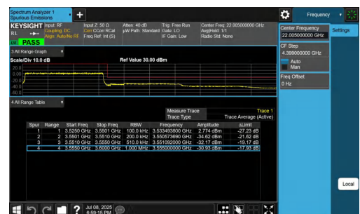
NTNV-n77(3450-3550)-PC2-30-25-H-DFT-QPSK-Outer_Full-PASS
