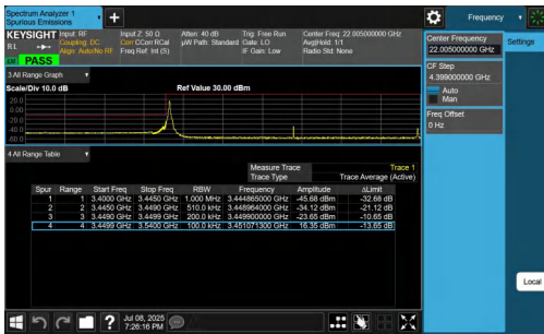
NTNV-n77(3450-3550)-PC2-30-90-L-DFT-BPSK-Edge_1RB_Left-PAS S
