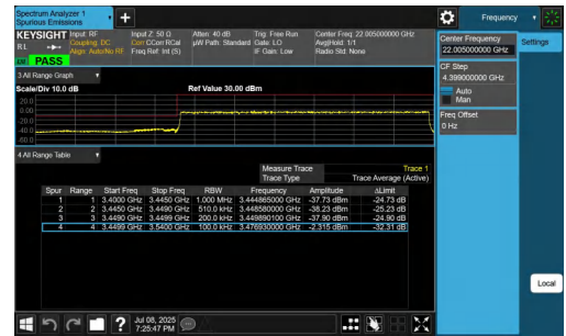
NTNV-n77(3450-3550)-PC2-30-90-L-DFT-BPSK-Outer_Full-PASS
