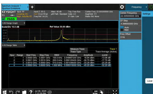
NTNV-n77(3450-3550)-PC2-30-50-H-DFT-QPSK-Edge_1RB_Right-PA SS
