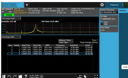
NTNV-n77(3450-3550)-PC2-30-25-H-DFT-BPSK-Edge_1RB_Right-PA SS
