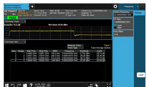
NTNV-n77(3450-3550)-PC2-30-90-H-DFT-QPSK-Outer_Full-PASS
