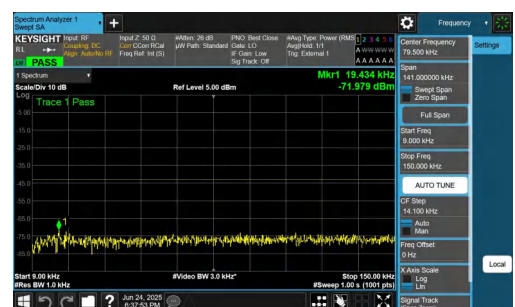
NTNV-n77(3450-3550)-PC2-30-10-H-DFT-BPSK-Inner_1RB_Right-0.0 09-0.15-PASS
