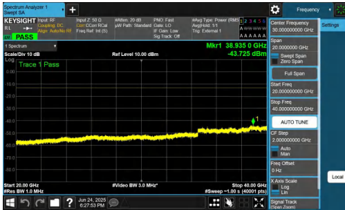
NTNV-n77(3450-3550)-PC2-30-10-M-DFT-QPSK-Inner_1RB_Left-20 000-40000-PASS
