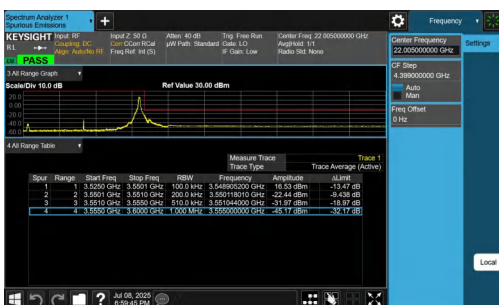
NTNV-n77(3450-3550)-PC2-30-25-H-DFT-QPSK-Edge_1RB_Right-PA SS
