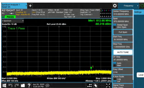
NTNV-n77(3450-3550)-PC2-30-10-H-DFT-BPSK-Inner_1RB_Left-30- 1000-PASS
