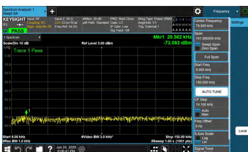
NTNV-n77(3450-3550)-PC2-30-10-L-DFT-QPSK-Inner_1RB_Left-0.09-0.15-PASS
