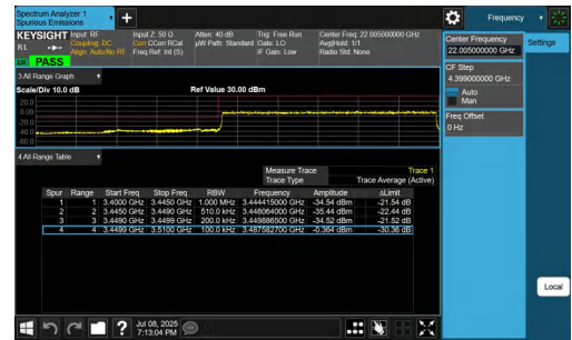
NTNV-n77(3450-3550)-PC2-30-60-L-DFT-BPSK-Outer_Full-PASS
