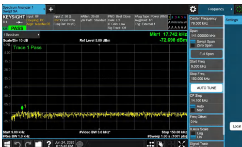
NTNV-n77(3450-3550)-PC2-30-10-M-DFT-BPSK-Inner_1RB_Left-0.0 09-0.15-PASS
