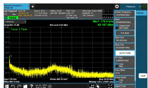
NTNV-n77(3450-3550)-PC2-30-10-L-DFT-QPSK-Inner_1RB_Left-0.15-30-PASS
