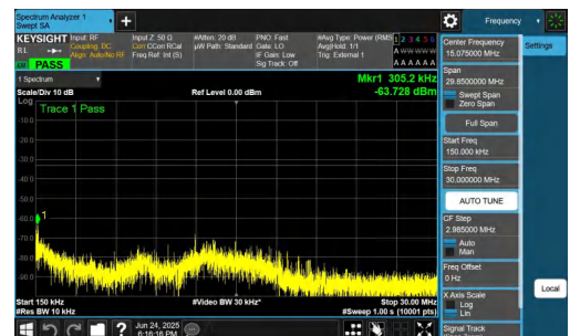
NTNV-n77(3450-3550)-PC2-30-10-M-DFT-BPSK-Inner_1RB_Left-0.15 -30-PASS
