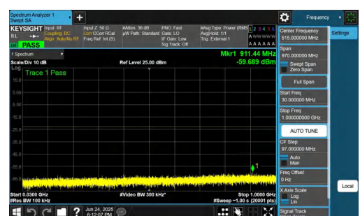
NTNV-n77(3450-3550)-PC2-30-10-L-DFT-QPSK-Inner_1RB_Right-30-1000-PASS
