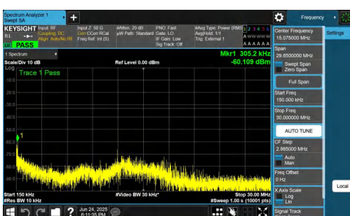
NTNV-n77(3450-3550)-PC2-30-10-L-DFT-QPSK-Inner_1RB_Right-0.15-30-PASS
