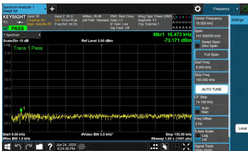
NTNV-n77(3450-3550)-PC2-30-10-M-DFT-QPSK-Inner_1RB_Left-0.0 09-0.15-PASS
