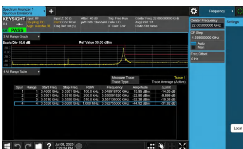
NTNV-n77(3450-3550)-PC2-30-90-H-DFT-QPSK-Edge_1RB_Right-PA SS
