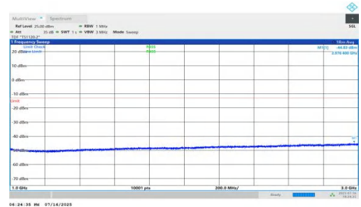
NTNV-n71-PC2-15-15-L-DFT-BPSK-Inner_1RB_Left-1000-3000-PASS
