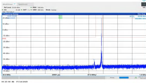
NTNV-n71-PC2-15-10-H-DFT-QPSK-Inner_1RB_Right-30-1000-PAS S
