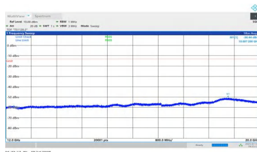
NTNV-n71-PC2-15-20-L-DFT-BPSK-Inner_1RB_Right-12000-20000-PASS
