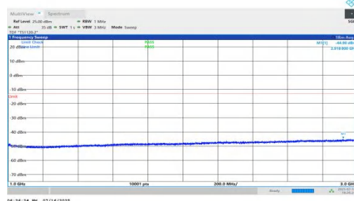
NTNV-n71-PC2-15-15-L-DFT-QPSK-Inner_1RB_Right-1000-3000-PASS S
