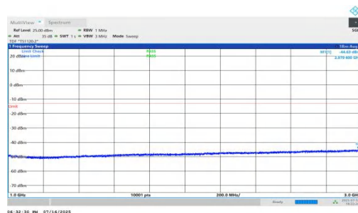
NTNV-n71-PC2-15-20-L-DFT-BPSK-Inner_1RB_Left-1000-3000-PASS
