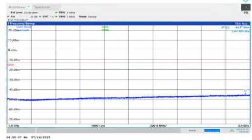
NTNV-n71-PC2-15-15-L-DFT-BPSK-Inner_1RB_Right-1000-3000-PASS
