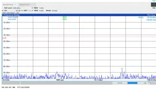
NTNV-n71-PC2-15-15-L-DFT-BPSK-Inner_1RB_Left-0.009-0.15-PAS S
