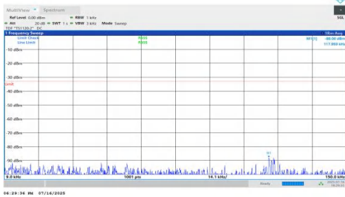
NTNV-n71-PC2-15-15-H-DFT-BPSK-Inner_1RB_Left-0.009-0.15-PAS S
