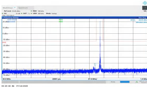
NTNV-n71-PC2-15-15-H-DFT-BPSK-Inner_1RB_Left-30-1000-PASS
