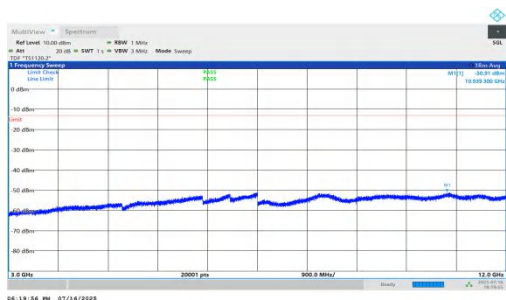
NTVN-n71-PC2-15-10-M-DFT-BPSK-Inner_1RB_Right-3000-12000-P ASS
