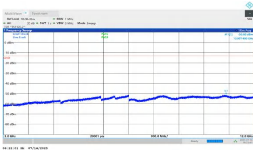
NTNV-n71-PC2-15-10-H-DFT-BPSK-Inner_1RB_Left-3000-12000-PA SS
