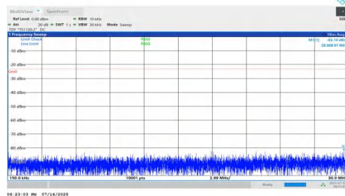
NTVN-n71-PC2-15-10-H-DFT-QPSK-Inner_1RB_Left-0.15-30-PASS
