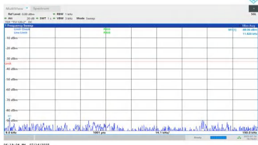
NTNV-n71-PC2-15-10-M-DFT-BPSK-Inner_1RB_Left-0.009-0.15-PAS S
