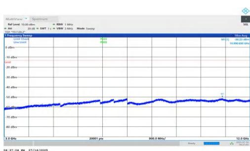
NTNV-n71-PC2-15-20-M-DFT-QPSK-Inner_1RB_Right-3000-12000-P ASS
