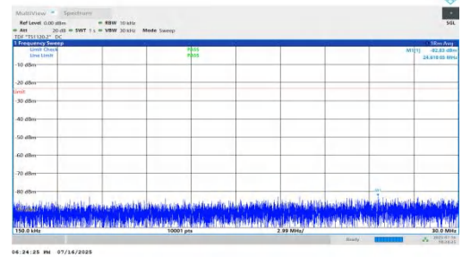
NTNV-n71-PC2-15-15-L-DFT-BPSK-Inner_1RB_Left-0.15-30-PASS
