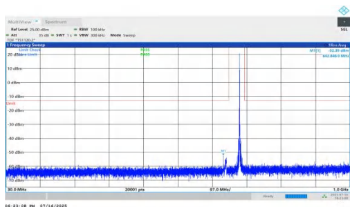
NTVN-n71-PC2-15-10-H-DFT-QPSK-Inner_1RB_Left-30-1000-PASS
