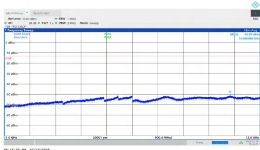
NTNV-n71-PC2-15-20-M-DFT-QPSK-Inner_1RB_Left-3000-12000-PA SS
