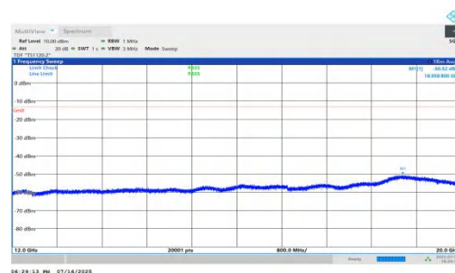
NTNV-n71-PC2-15-15-M-DFT-QPSK-Inner_1RB_Right-12000-20000-P ASS
