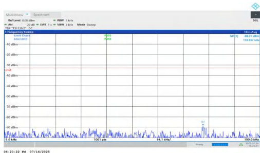
NTVN-n71-PC2-15-10-M-DFT-QPSK-Inner_1RB_Left-0.009-0.15-PA SS
