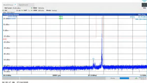
NTNV-n71-PC2-15-15-H-DFT-BPSK-Inner_1RB_Right-30-1000-PAS
