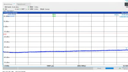
NTVN-n71-PC2-15-10-M-DFT-BPSK-Inner_1RB_Right-1000-3000-PA SS
