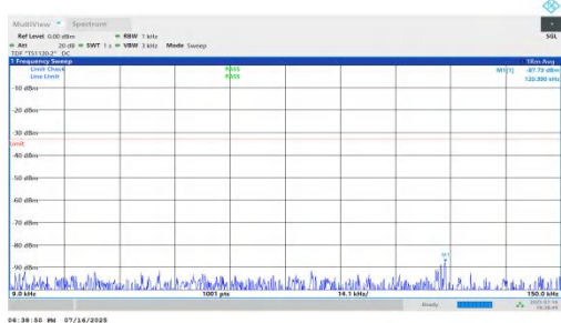
NTNV-n71-PC2-15-20-H-DFT-QPSK-Inner_1RB_Left-0.009-0.15-PAS
