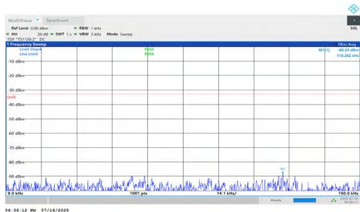
NTNV-n71-PC2-15-20-M-DFT-QPSK-Inner_1RB_Left-0.009-0.15-PA SS
