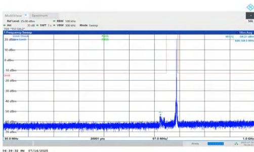
NTNV-n71-PC2-15-20-H-DFT-QPSK-Inner_1RB_Right-30-1000-PAS S
