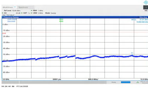
NTNV-n71-PC2-15-15-L-DFT-BPSK-Inner_1RB_Left-3000-12000-PA SS
