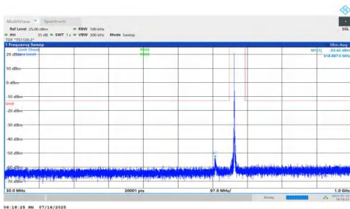
NTNV-n71-PC2-15-10-L-DFT-QPSK-Inner_1RB_Right-0.009-0.15-PA SS
