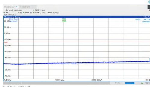
NTNV-n71-PC2-15-20-M-DFT-BPSK-Inner_1RB_Left-1000-3000-PAS S
