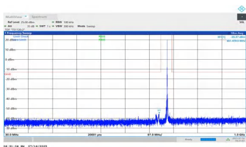
NTNV-n71-PC2-15-15-H-DFT-QPSK-Inner_1RB_Left-30-1000-PASS
