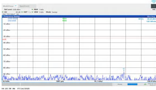
NTNV-n71-PC2-15-15-L-DFT-QPSK-Inner_1RB_Left-0.009-0.15-PASS
