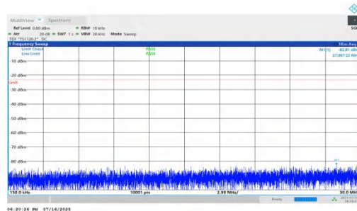
NTVN-n71-PC2-15-10-M-DFT-QPSK-Inner_1RB_Left-0.15-30-PASS
