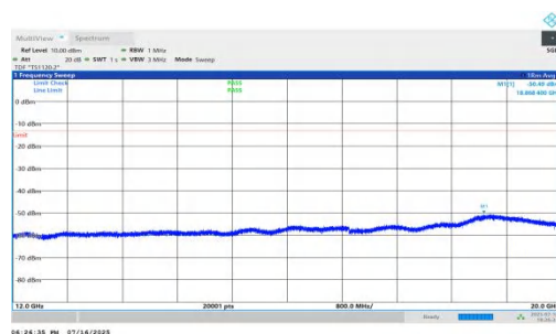
NTNV-n71-PC2-15-15-L-DFT-QPSK-Inner_1RB_Right-12000-20000-P ASS
