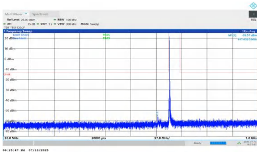
NTNV-n71-PC2-15-15-L-DFT-QPSK-Inner_1RB_Left-30-1000-PASS
