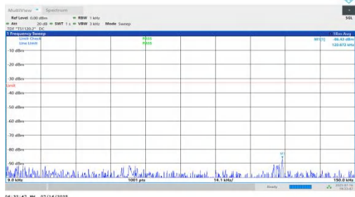
NTNV-n71-PC2-15-20-L-DFT-BPSK-Inner_1RB_Right-0.009-0.15-PA SS
