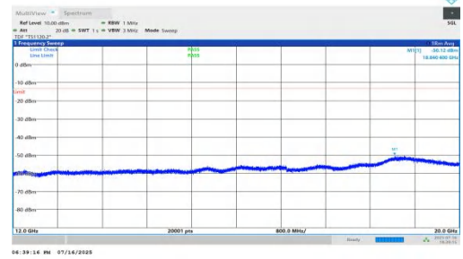
NTNV-n71-PC2-15-20-H-DFT-QPSK-Inner_1RB_Left-12000-20000-PA SS
