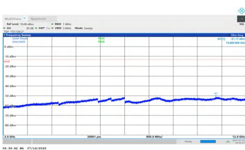
NTNV-n71-PC2-15-20-H-DFT-QPSK-Inner_1RB_Right-3000-12000-P ASS
