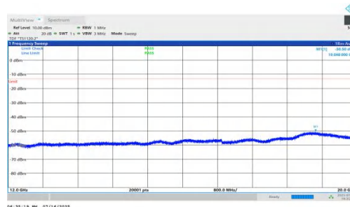
NTNV-n71-PC2-15-20-M-DFT-BPSK-Inner_1RB_Left-12000-20000-PA SS
