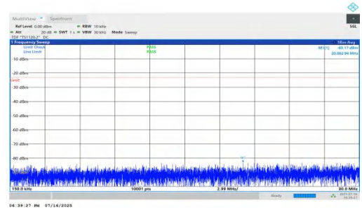
NTNV-n71-PC2-15-20-H-DFT-QPSK-Inner_1RB_Right-0.15-30-PASS
