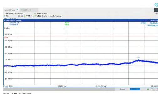
NTNV-n71-PC2-15-10-M-DFT-QPSK-Inner_1RB_Right-12000-20000-P ASS
