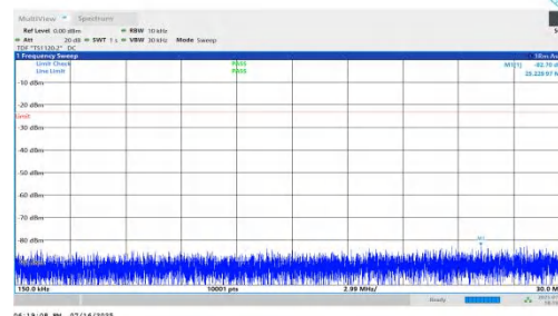
NTNV-n71-PC2-15-10-M-DFT-BPSK-Inner_1RB_Left-0.15-30-PASS
