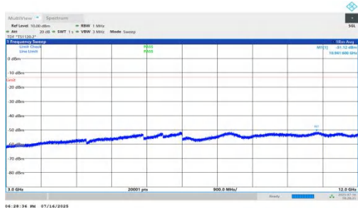
NTNV-n71-PC2-15-15-M-DFT-QPSK-Inner_1RB_Left-3000-12000-PA SS
