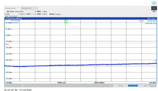
NTNV-n71-PC2-15-15-H-DFT-BPSK-Inner_1RB_Left-1000-3000-PASS
