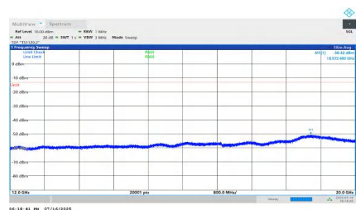
NTNV-n71-PC2-15-10-L-DFT-QPSK-Inner_1RB_Right-12000-20000-P ASS
