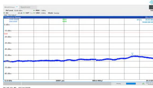
NTNV-n71-PC2-15-15-L-DFT-QPSK-Inner_1RB_Left-12000-20000-PA SS
