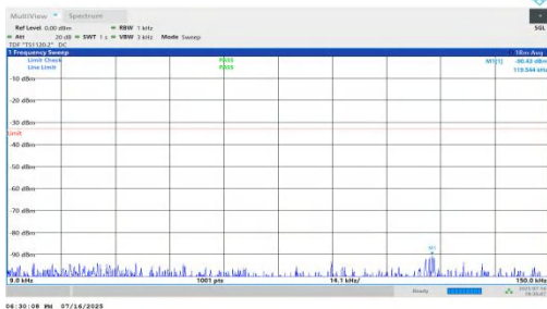
NTNV-n71-PC2-15-15-H-DFT-BPSK-Inner_1RB_Right-0.009-0.15-PA SS
