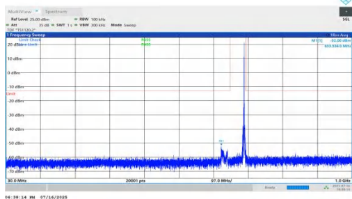
NTNV-n71-PC2-15-20-H-DFT-BPSK-Inner_1RB_Right-30-1000-PAS
