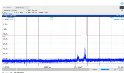
NTNV-n71-PC2-15-20-M-DFT-QPSK-Inner_1RB_Right-30-1000-PAS S
