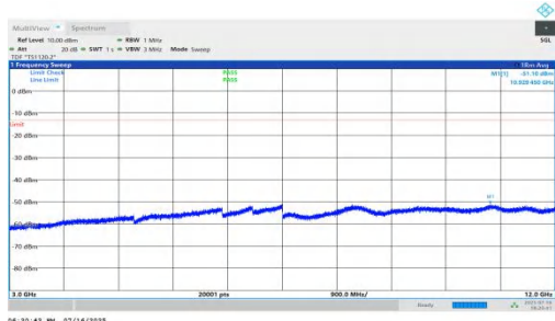
NTNV-n71-PC2-15-10-M-DFT-QPSK-Inner_1RB_Left-3000-12000-PA SS
