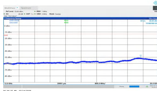
NTNV-n71-PC2-15-20-M-DFT-QPSK-Inner_1RB_Left-12000-20000-PA SS
