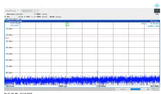
NTNV-n71-PC2-15-15-M-DFT-BPSK-Inner_1RB_Right-0.15-30-PASS
