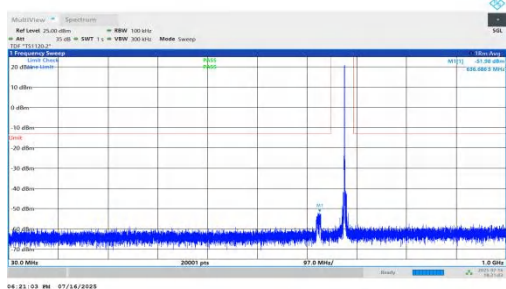
NTNV-n71-PC2-15-10-M-DFT-QPSK-Inner_1RB_Right-30-1000-PAS S
