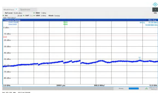
NTNV-n71-PC2-15-20-H-DFT-BPSK-Inner_1RB_Left-3000-12000-PA SS
