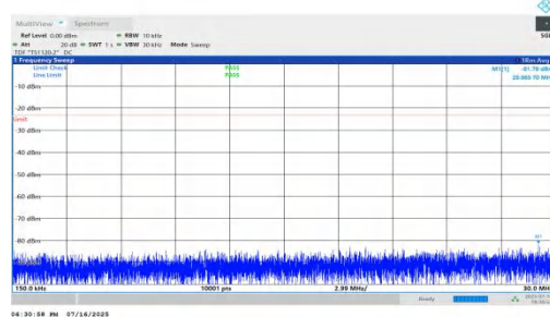
NTNV-n71-PC2-15-15-H-DFT-QPSK-Inner_1RB_Left-0.15-30-PASS
