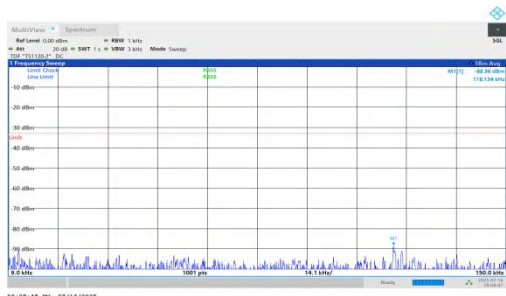
NTNV-n71-PC2-15-15-M-DFT-QPSK-Inner_1RB_Right-0.009-0.15-P ASS
