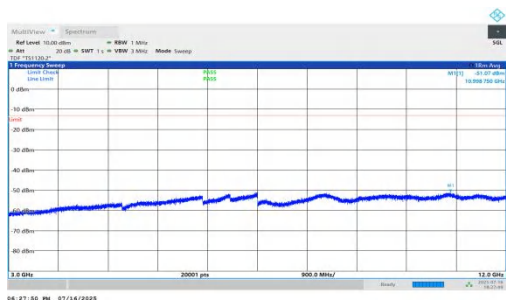
NTVN-n71-PC2-15-15-M-DFT-BPSK-Inner_1RB_Right-3000-12000-P ASS
