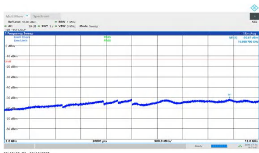
NTNV-n71-PC2-15-20-L-DFT-BPSK-Inner_1RB_Right-3000-12000-PASS
