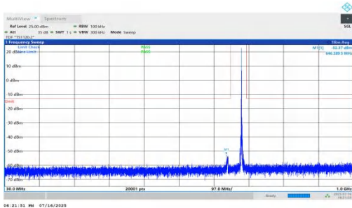
NTNV-n71-PC2-15-10-H-DFT-BPSK-Inner_1RB_Left-30-1000-PASS
