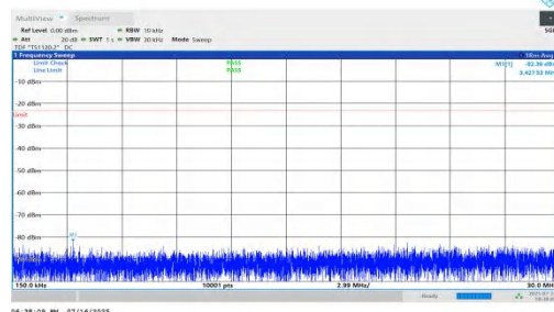
NTNV-n71-PC2-15-20-H-DFT-BPSK-Inner_1RB_Right-0.15-30-PASS
