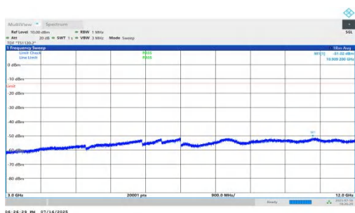
NTNV-n71-PC2-15-15-L-DFT-QPSK-Inner_1RB_Right-3000-12000-P ASS
