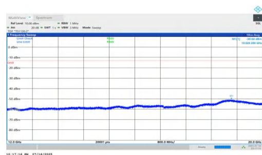
NTNV-n66-PC2-15-45-H-DFT-QPSK-Inner_1RB_Right-12000-200 00-PASS
