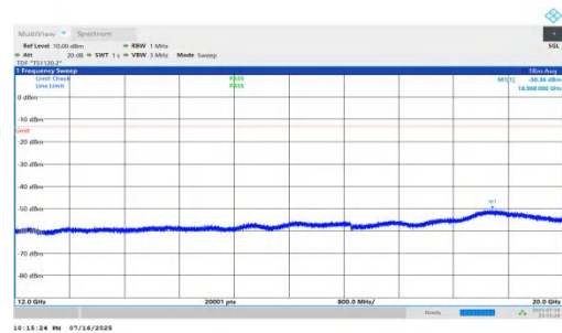
NTNV-n66-PC2-15-45-H-DFT-BPSK-Inner_1RB_Left-12000-20000-PASS
