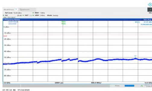
NTNV-n66-PC2-15-40-H-DFT-QPSK-Inner_1RB_Right-3000-12000-PASS
