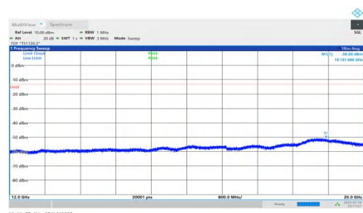
NTVN-n66-PC2-15-45-L-DFT-QPSK-Inner_1RB_Right-12000-20000-PASS 5-PASS
