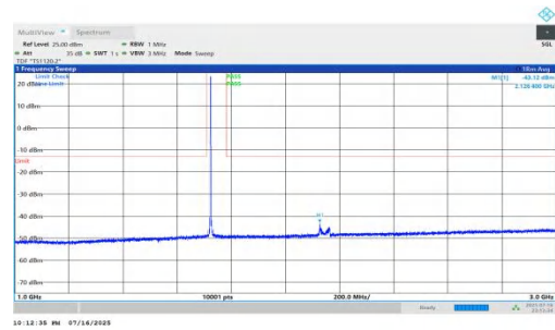
NTNV-n66-PC2-15-45-M-DFT-BPSK-Inner_1RB_Left-1000-3000-PASS
