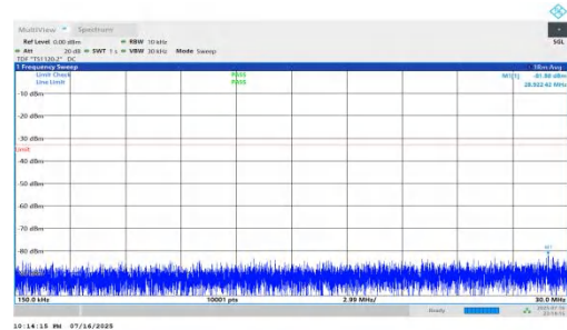
NTNV-n66-PC2-15-45-M-DFT-QPSK-Inner_1RB_Right-0.15-30-P ASS
