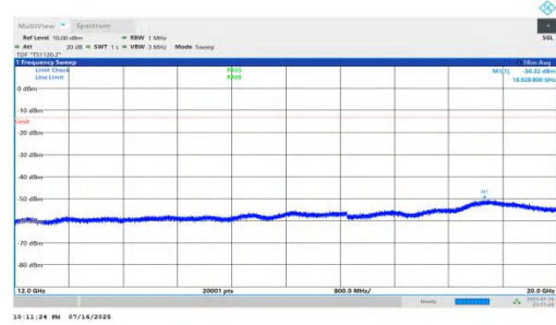
NTVN-n66-PC2-15-45-L-DFT-QPSK-Inner_1RB_Left-12000-2000 0-PASS
