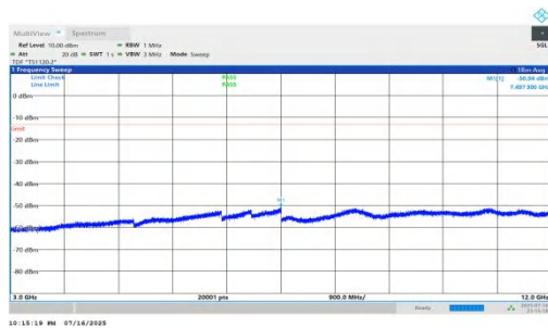
NTNV-n66-PC2-15-45-H-DFT-BPSK-Inner_1RB_Left-3000-12000-PASS
