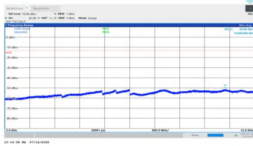
NTNV-n66-PC2-15-45-H-DFT-QPSK-Inner_1RB_Left-3000-1200 0-PASS
