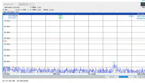
NTNV-n66-PC2-15-40-M-DFT-BPSK-Inner_1RB_Left-0.009-0.15-PASS
