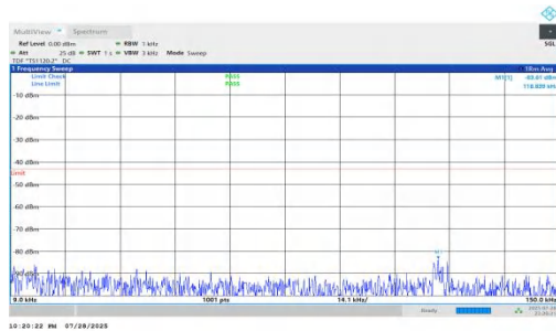
NTNV-n66-PC2-15-45-L-DFT-QPSK-Inner_1RB_Left-0.009-0.15- PASS
