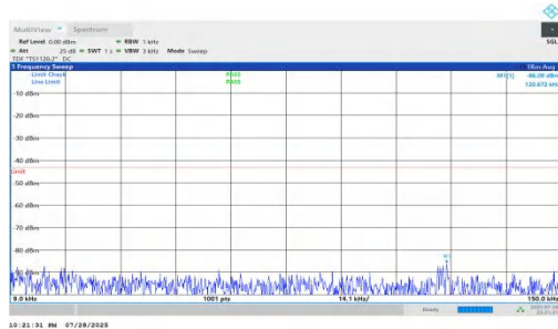
NTNV-n66-PC2-15-45-M-DFT-QPSK-Inner_1RB_Right-0.009-0.1 5-PASS
