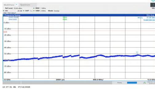
NTNV-n66-PC2-15-40-H-DFT-BPSK-Inner_1RB_Right-3000-12000-PASS
