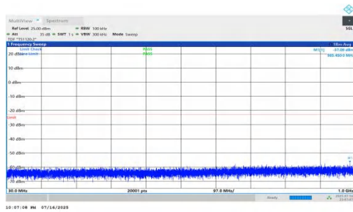
NTNV-n66-PC2-15-40-H-DFT-BPSK-Inner_1RB_Left-30-1000-PASS
