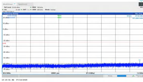
NTNV-n66-PC2-15-45-H-DFT-BPSK-Inner_1RB_Right-30-1000-P ASS
