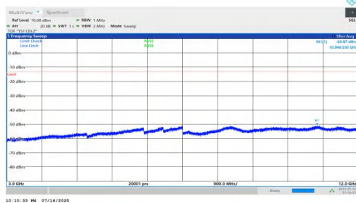
NTNV-n66-PC2-15-45-L-DFT-BPSK-Inner_1RB_Right-3000-1200 0-PASS
