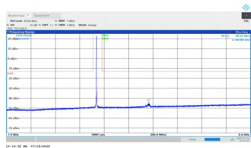
NTNV-n66-PC2-15-45-H-DFT-QPSK-Inner_1RB_Left-1000-3000-PASS
