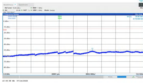
NTNV-n66-PC2-15-40-M-DFT-QPSK-Inner_1RB_Left-3000-1200 0-PASS
