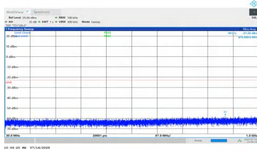
NTNV-n66-PC2-15-40-M-DFT-QPSK-Inner_1RB_Right-30-1000- PASS
