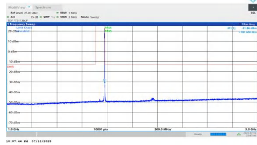
NTNV-n66-PC2-15-40-H-DFT-BPSK-Inner_1RB_Right-1000-3000-PASS
