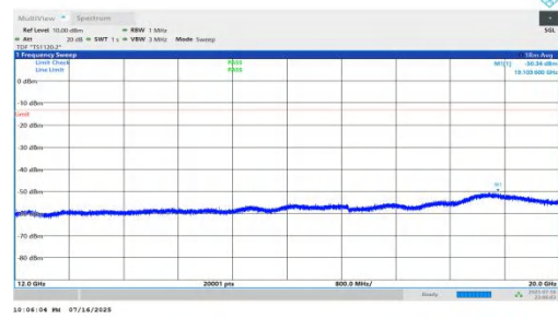
NTNV-n66-PC2-15-40-M-DFT-QPSK-Inner_1RB_Left-12000-2000 0-PASS
