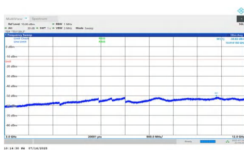
NTNV-n66-PC2-15-45-M-DFT-QPSK-Inner_1RB_Right-3000-120 00-PASS
