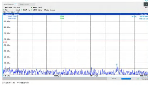
NTNV-n66-PC2-15-45-L-DFT-BPSK-Inner_1RB_Left-0.009-0.15- PASS
