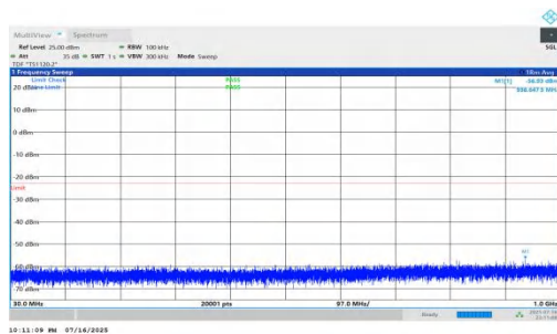
NTNV-n66-PC2-15-45-L-DFT-QPSK-Inner_1RB_Left-30-1000-PA SS
