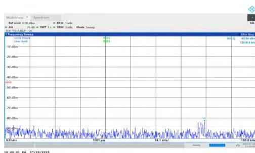
NTNV-n66-PC2-15-45-L-DFT-BPSK-Inner_1RB_Right-0.009-0.15 -PASS
