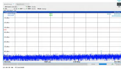
NTNV-n66-PC2-15-40-H-DFT-QPSK-Inner_1RB_Right-0.15-30-PA SS
