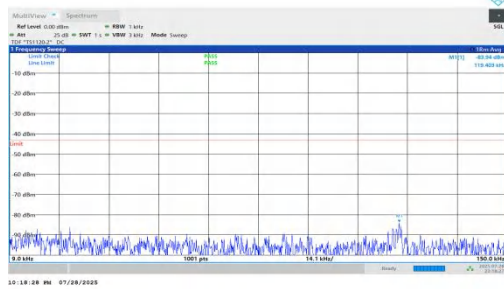
NTNV-n66-PC2-15-40-M-DFT-QPSK-Inner_1RB_Right-0.009-0.1 5-PASS
