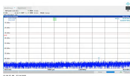
NTNV-n66-PC2-15-40-M-DFT-BPSK-Inner_1RB_Right-0.15-30-PASS
