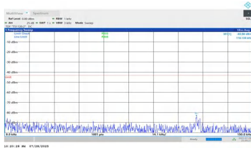
NTVN-n66-PC2-15-45-L-DFT-QPSK-Inner_1RB_Right-0.009-0.1 5-PASS
