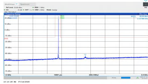
NTNV-n66-PC2-15-45-L-DFT-BPSK-Inner_1RB_Right-1000-3000-P PASS
