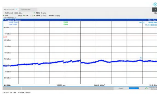
NTNV-n66-PC2-15-45-L-DFT-BPSK-Inner_1RB_Left-3000-12000 -PASS
