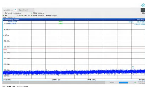
NTNV-n66-PC2-15-45-M-DFT-QPSK-Inner_1RB_Left-30-1000-PASS
