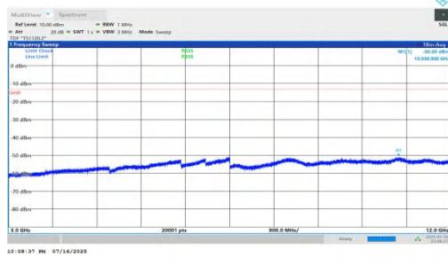
NTNV-n66-PC2-15-40-H-DFT-QPSK-Inner_1RB_Left-3000-1200 0-PASS
