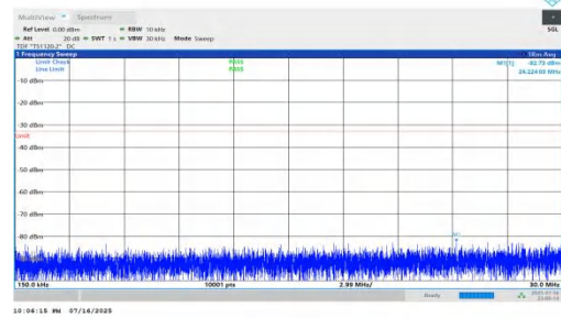
NTNV-n66-PC2-15-40-M-DFT-QPSK-Inner_1RB_Right-0.15-30-P ASS
