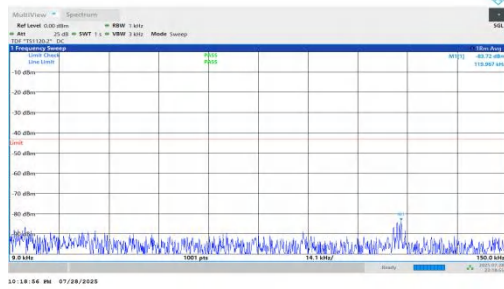
NTNV-n66-PC2-15-40-H-DFT-BPSK-Inner_1RB_Left-0.009-0.15-PASS
