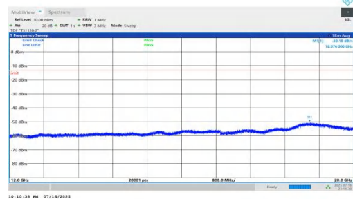
NTNV-n66-PC2-15-45-L-DFT-BPSK-Inner_1RB_Right-12000-200 00-PASS
