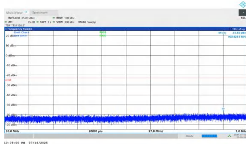
NTNV-n66-PC2-15-40-H-DFT-QPSK-Inner_1RB_Right-30-1000- PASS
