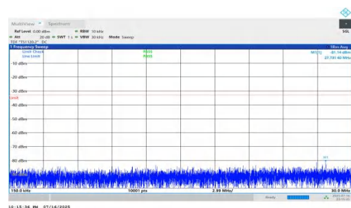
NTNV-n66-PC2-15-45-H-DFT-BPSK-Inner_1RB_Right-0.15-30-PASS
