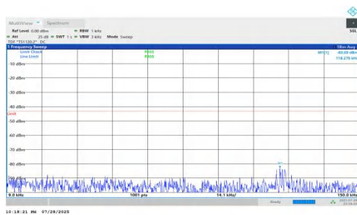
NTNV-n66-PC2-15-40-M-DFT-QPSK-Inner_1RB_Left-0.009-0.15-PASS
