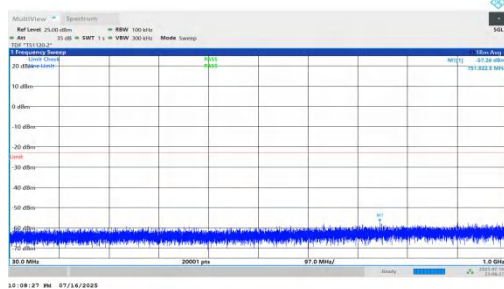
NTNV-n66-PC2-15-40-H-DFT-QPSK-Inner_1RB_Left-30-1000-PASS
