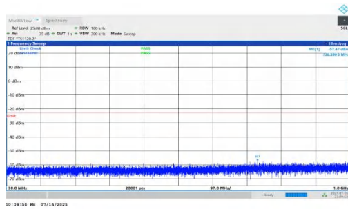
NTNV-n66-PC2-15-45-L-DFT-BPSK-Inner_1RB_Left-30-1000-PASS SS
