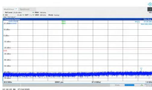
NTNV-n66-PC2-15-45-M-DFT-QPSK-Inner_1RB_Right-30-1000- PASS
