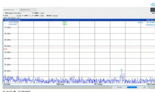
NTNV-n66-PC2-15-40-M-DFT-BPSK-Inner_1RB_Right-0.009-0.15-PASS
