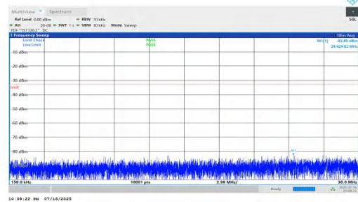
NTNV-n66-PC2-15-40-H-DFT-QPSK-Inner_1RB_Left-0.15-30-PASS
