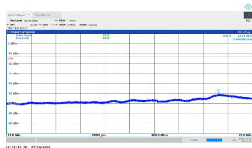
NTNV-n66-PC2-15-40-M-DFT-BPSK-Inner_1RB_Left-12000-20000-PASS
