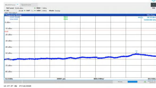
NTNV-n66-PC2-15-40-H-DFT-BPSK-Inner_1RB_Right-12000-20000-PASS
