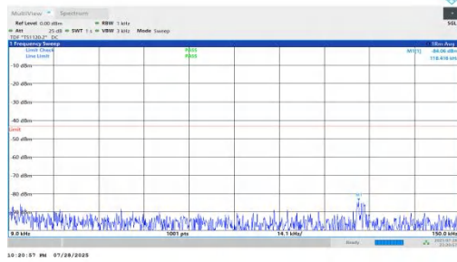
NTNV-n66-PC2-15-45-M-DFT-BPSK-Inner_1RB_Left-0.009-0.15-PASS
