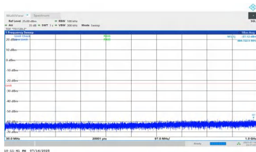
NTVN-n66-PC2-15-45-L-DFT-QPSK-Inner_1RB_Right-30-1000-PASS 5-PASS
