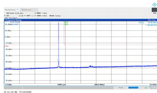
NTNV-n66-PC2-15-45-L-DFT-QPSK-Inner_1RB_Left-1000-3000-P ASS
