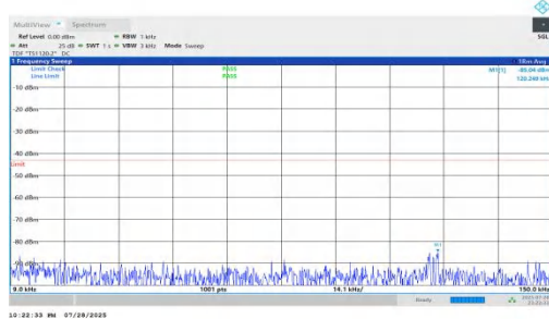
NTNV-n66-PC2-15-45-H-DFT-QPSK-Inner_1RB_Right-0.009-0.1 5-PASS
