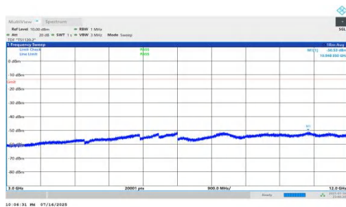
NTNV-n66-PC2-15-40-M-DFT-QPSK-Inner_1RB_Right-3000-12000- 00-PASS
