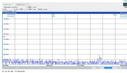
NTNV-n66-PC2-15-40-H-DFT-QPSK-Inner_1RB_Right-0.009-0.1 5-PASS
