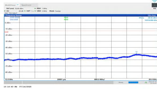
NTNV-n66-PC2-15-45-H-DFT-QPSK-Inner_1RB_Left-12000-2000 0-PASS
