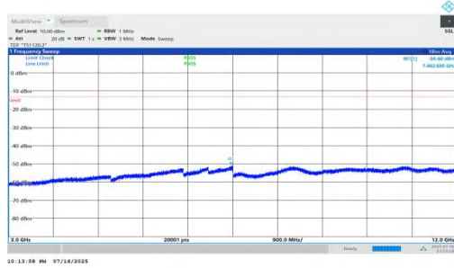
NTNV-n66-PC2-15-45-M-DFT-QPSK-Inner_1RB_Left-3000-1200 0-PASS
