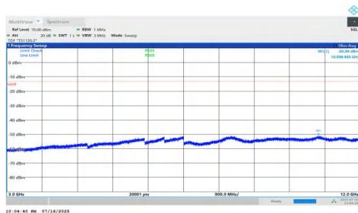
NTNV-n66-PC2-15-40-M-DFT-BPSK-Inner_1RB_Left-3000-12000-PASS
