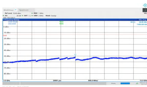
NTVN-n66-PC2-15-45-L-DFT-QPSK-Inner_1RB_Right-3000-12000-PASS 5-PASS
