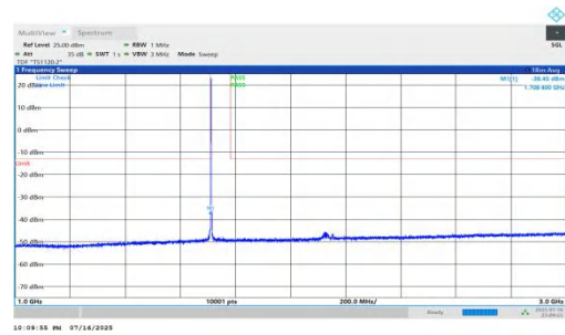
NTNV-n66-PC2-15-45-L-DFT-BPSK-Inner_1RB_Left-1000-3000-PASS ASS
