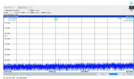
NTNV-n66-PC2-15-45-H-DFT-QPSK-Inner_1RB_Left-0.15-30-PASS
