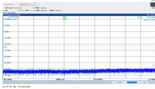
NTNV-n66-PC2-15-40-H-DFT-BPSK-Inner_1RB_Right-30-1000-PASS
