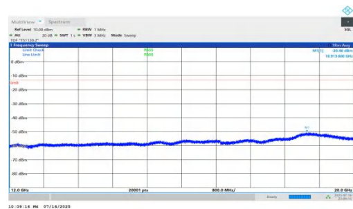
NTNV-n66-PC2-15-40-H-DFT-QPSK-Inner_1RB_Right-12000-20000-PASS
