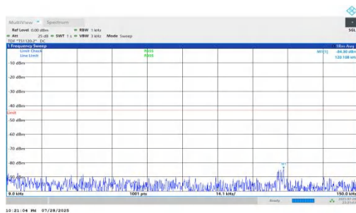
NTNV-n66-PC2-15-45-M-DFT-BPSK-Inner_1RB_Right-0.009-0.15-PASS
