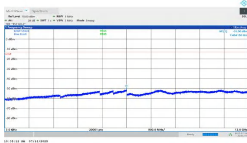
NTNV-n66-PC2-15-40-M-DFT-BPSK-Inner_1RB_Right-3000-12000-PASS
