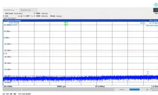
NTNV-n66-PC2-15-40-M-DFT-QPSK-Inner_1RB_Left-30-1000-PASS
