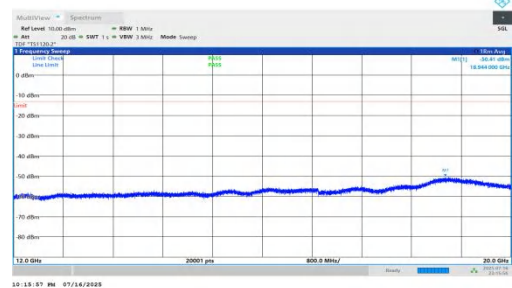
NTNV-n66-PC2-15-45-H-DFT-BPSK-Inner_1RB_Right-12000-20000-PASS
