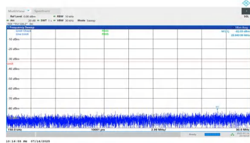
NTNV-n66-PC2-15-45-H-DFT-QPSK-Inner_1RB_Right-0.15-30-PA SS
