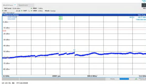
NTNV-n66-PC2-15-45-H-DFT-BPSK-Inner_1RB_Right-3000-12000-PASS
