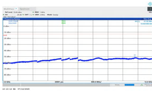
NTNV-n66-PC2-15-45-M-DFT-BPSK-Inner_1RB_Right-3000-12000-PASS
