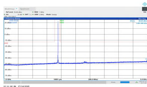
NTVN-n66-PC2-15-45-L-DFT-QPSK-Inner_1RB_Right-1000-3000-PASS 5-PASS
