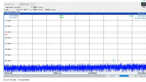
NTNV-n66-PC2-15-45-H-DFT-BPSK-Inner_1RB_Left-0.15-30-PAS
