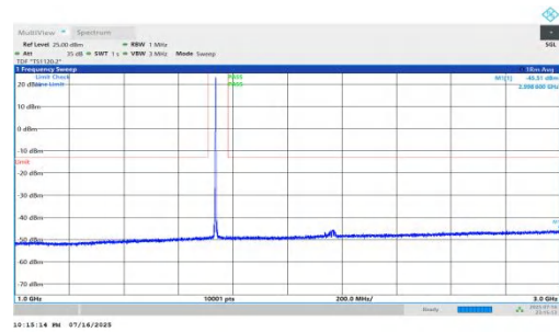
NTNV-n66-PC2-15-45-H-DFT-BPSK-Inner_1RB_Left-1000-3000-PASS
