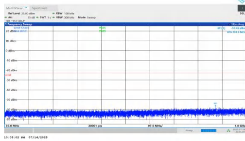
NTNV-n66-PC2-15-40-M-DFT-BPSK-Inner_1RB_Right-30-1000-PASS
