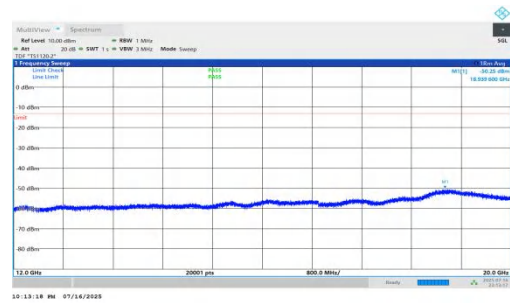
NTNV-n66-PC2-15-45-M-DFT-BPSK-Inner_1RB_Right-12000-20000-PASS
