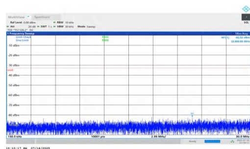
NTNV-n66-PC2-15-45-L-DFT-BPSK-Inner_1RB_Right-0.15-30-PASS SS
