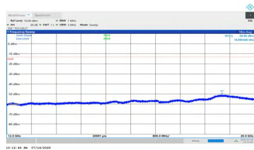
NTNV-n66-PC2-15-45-M-DFT-BPSK-Inner_1RB_Left-12000-20000-PASS
