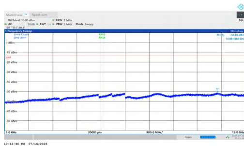
NTNV-n66-PC2-15-45-M-DFT-BPSK-Inner_1RB_Left-3000-12000-PASS
