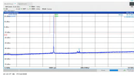
NTNV-n66-PC2-15-45-M-DFT-BPSK-Inner_1RB_Right-1000-3000-PASS
