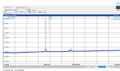
NTNV-n66-PC2-15-40-M-DFT-QPSK-Inner_1RB_Left-1000-3000-PASS
