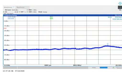
NTNV-n66-PC2-15-40-H-DFT-BPSK-Inner_1RB_Left-12000-20000-PASS
