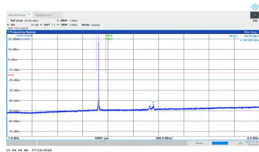
NTNV-n66-PC2-15-40-M-DFT-BPSK-Inner_1RB_Left-1000-3000-PASS
