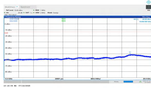
NTNV-n66-PC2-15-45-M-DFT-QPSK-Inner_1RB_Left-12000-2000 0-PASS
