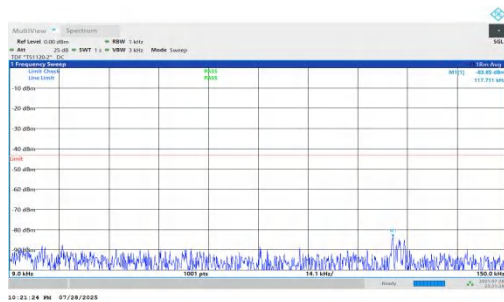
NTNV-n66-PC2-15-45-M-DFT-QPSK-Inner_1RB_Left-0.009-0.15-PASS
