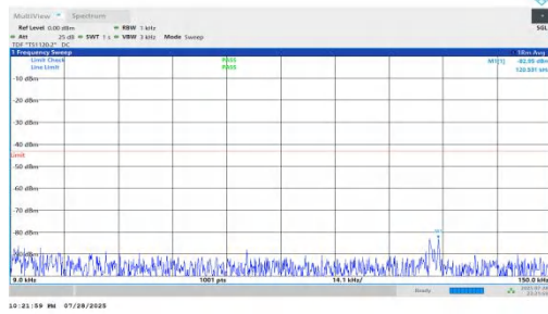
NTNV-n66-PC2-15-45-H-DFT-BPSK-Inner_1RB_Left-0.009-0.15-PASS
