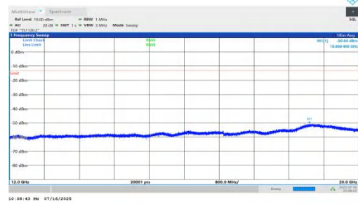
NTNV-n66-PC2-15-40-H-DFT-QPSK-Inner_1RB_Left-12000-2000 0-PASS
