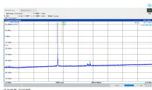
NTNV-n66-PC2-15-45-M-DFT-QPSK-Inner_1RB_Left-1000-3000-PASS
