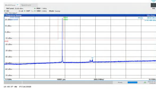
NTNV-n66-PC2-15-40-M-DFT-BPSK-Inner_1RB_Right-1000-3000-PASS
