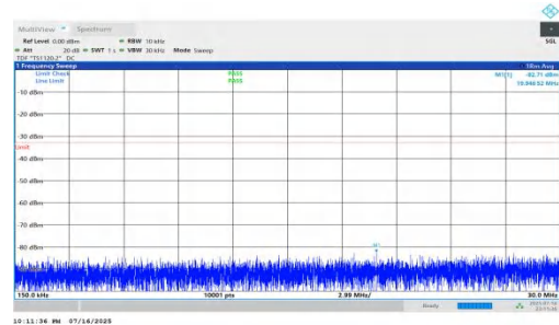
NTVN-n66-PC2-15-45-L-DFT-QPSK-Inner_1RB_Right-0.15-30-PASS 5-PASS
