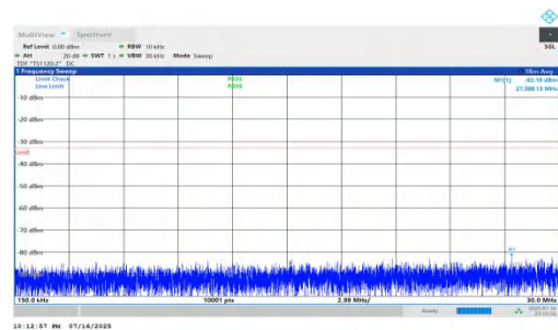
NTNV-n66-PC2-15-45-M-DFT-BPSK-Inner_1RB_Right-0.15-30-PASS
