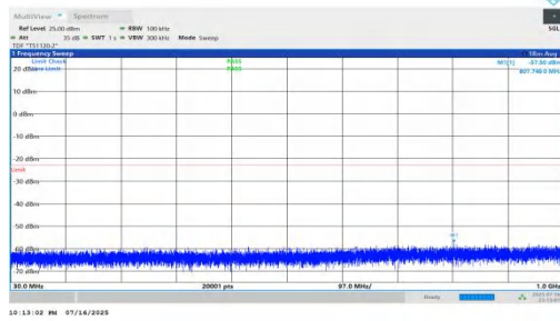
NTNV-n66-PC2-15-45-M-DFT-BPSK-Inner_1RB_Right-30-1000-PASS
