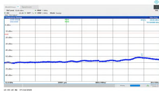
NTNV-n66-PC2-15-40-M-DFT-BPSK-Inner_1RB_Right-12000-20000-PASS
