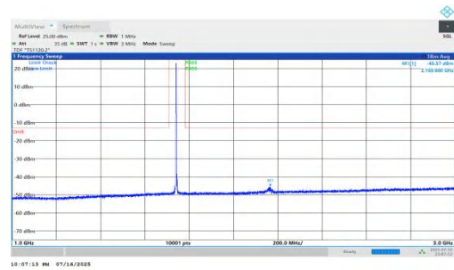
NTNV-n66-PC2-15-40-H-DFT-BPSK-Inner_1RB_Left-1000-3000-PASS
