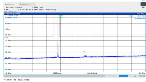
NTNV-n66-PC2-15-35-M-DFT-BPSK-Inner_1RB_Right-1000-3000-PASS
