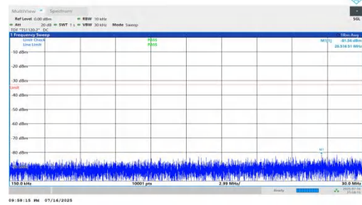
NTNV-n66-PC2-15-35-M-DFT-QPSK-Inner_1RB_Right-0.15-30-P ASS
