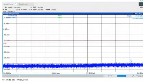
NTNV-n66-PC2-15-35-H-DFT-BPSK-Inner_1RB_Right-30-1000-P ASS
