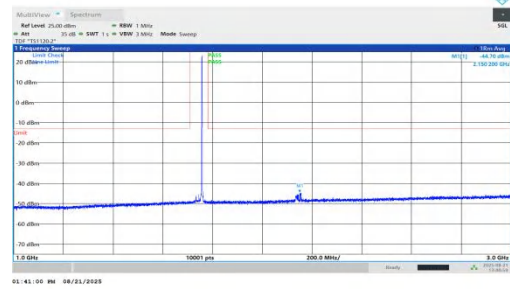
NTNV-n66-PC2-15-25-M-DFT-BPSK-Inner_1RB_Right-1000-3000-PASS
