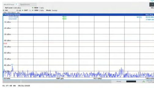
NTNV-n66-PC2-15-25-L-DFT-BPSK-Inner_1RB_Left-0.009-0.15- PASS
