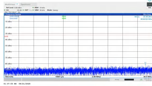
NTNV-n66-PC2-15-25-L-DFT-BPSK-Inner_1RB_Left-0.15-30-PAS S
