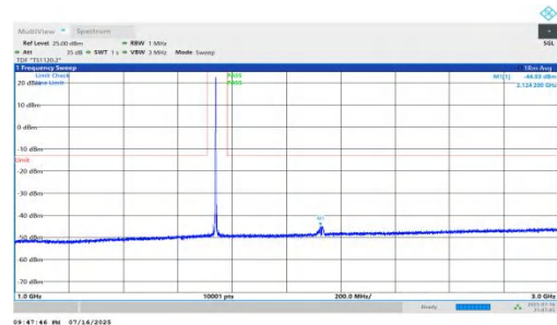
NTV-n66-PC2-15-30-L-DFT-QPSK-Inner_1RB_Right-1000-3000-PASS
