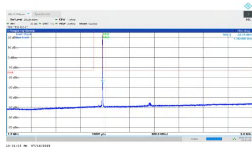
NTNV-n66-PC2-15-35-H-DFT-QPSK-Inner_1RB_Right-1000-3000 -PASS
