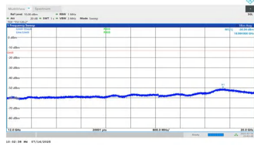
NTNV-n66-PC2-15-40-L-DFT-BPSK-Inner_1RB_Right-12000-200 00-PASS
