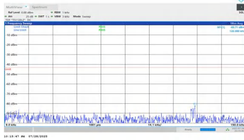
NTNV-n66-PC2-15-35-H-DFT-BPSK-Inner_1RB_Left-0.009-0.15-PASS
