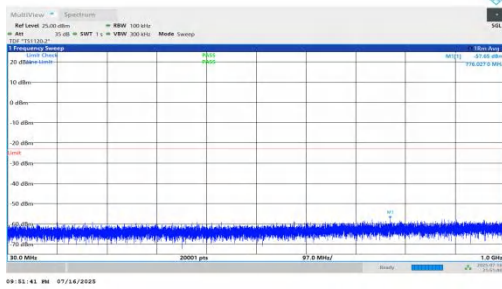
NTNV-n66-PC2-15-30-H-DFT-BPSK-Inner_1RB_Right-30-1000-P ASS
