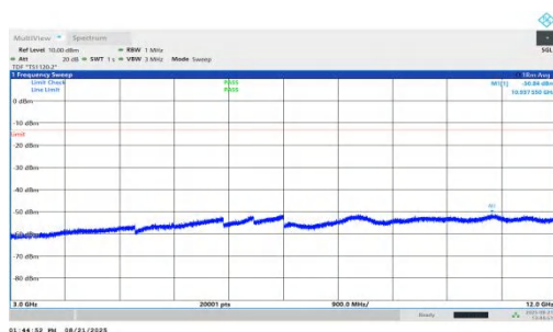
NTNV-n66-PC2-15-25-H-DFT-QPSK-Inner_1RB_Right-3000-120 00-PASS
