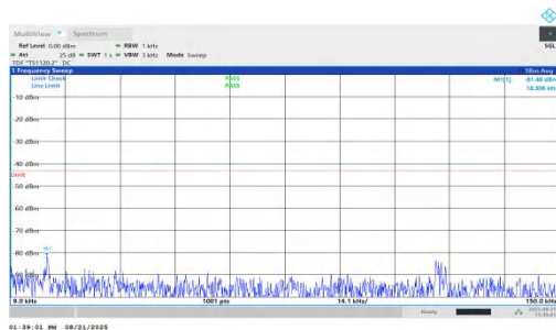
NTNV-n66-PC2-15-25-L-DFT-QPSK-Inner_1RB_Left-0.009-0.15- PASS
