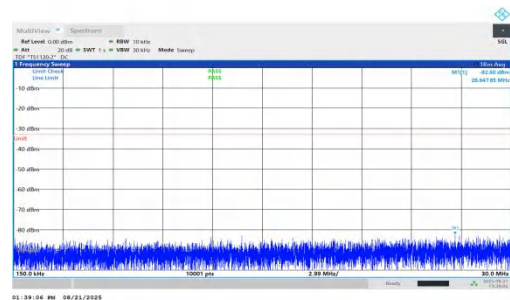
NTNV-n66-PC2-15-25-L-DFT-QPSK-Inner_1RB_Left-0.15-30-PAS S
