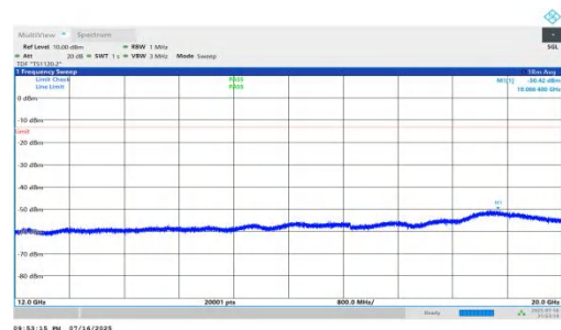
NTNV-n66-PC2-15-30-H-DFT-QPSK-Inner_1RB_Right-12000-200 00-PASS
