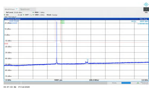
NTNV-n66-PC2-15-35-M-DFT-QPSK-Inner_1RB_Left-1000-3000-PASS
