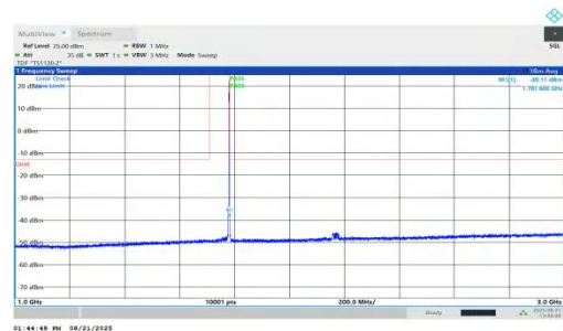
NTNV-n66-PC2-15-25-H-DFT-QPSK-Inner_1RB_Right-1000-3000 -PASS
