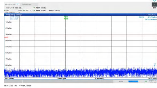
NTNV-n66-PC2-15-30-H-DFT-BPSK-Inner_1RB_Left-0.15-30-PAS
