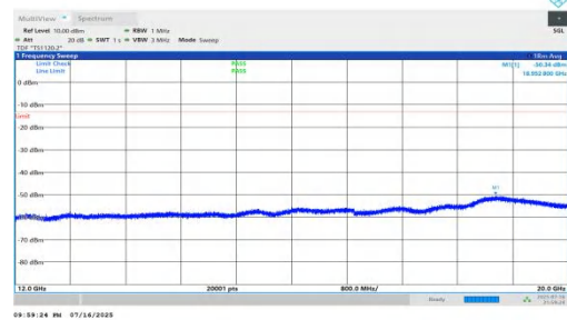
NTNV-n66-PC2-15-35-H-DFT-BPSK-Inner_1RB_Left-12000-20000-PASS
