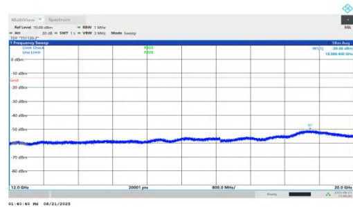
NTNV-n66-PC2-15-25-M-DFT-BPSK-Inner_1RB_Left-12000-20000-PASS
