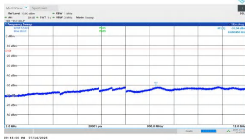
NTNV-n66-PC2-15-30-L-DFT-BPSK-Inner_1RB_Left-3000-12000-PASS
