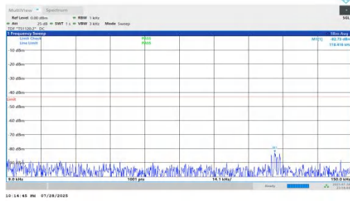
NTNV-n66-PC2-15-35-M-DFT-BPSK-Inner_1RB_Left-0.009-0.15-PASS
