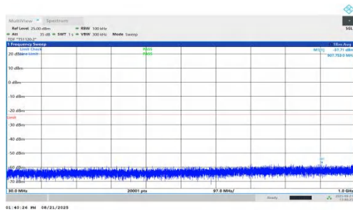
NTNV-n66-PC2-15-25-M-DFT-BPSK-Inner_1RB_Left-30-1000-PASS
