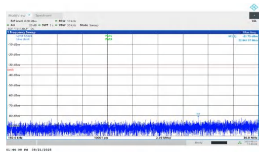
NTNV-n66-PC2-15-25-H-DFT-QPSK-Inner_1RB_Left-0.15-30-PAS S
