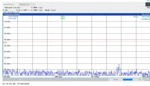
NTNV-n66-PC2-15-30-L-DFT-BPSK-Inner_1RB_Left-0.009-0.15-PASS
