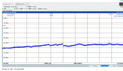
NTNV-n66-PC2-15-30-H-DFT-QPSK-Inner_1RB_Left-3000-1200 0-PASS
