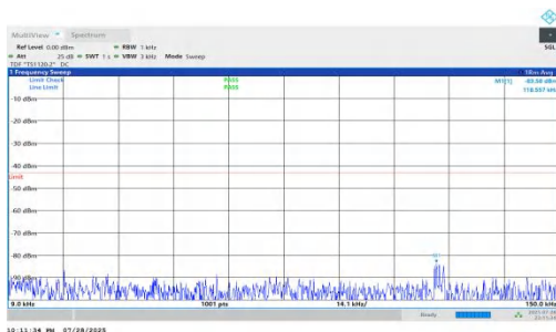
NTNV-n66-PC2-15-30-M-DFT-BPSK-Inner_1RB_Right-0.009-0.15-PASS
