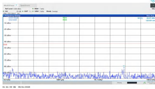
NTNV-n66-PC2-15-25-M-DFT-QPSK-Inner_1RB_Right-0.009-0.1 5-PASS
