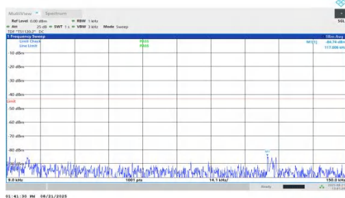
NTNV-n66-PC2-15-25-M-DFT-QPSK-Inner_1RB_Left-0.009-0.15-PASS
