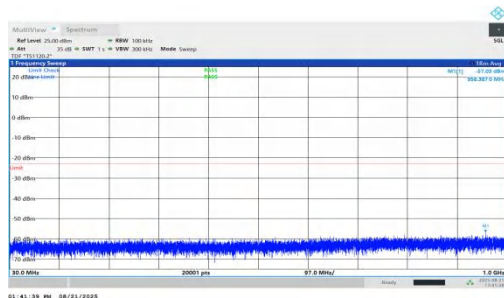
NTNV-n66-PC2-15-25-M-DFT-QPSK-Inner_1RB_Left-30-1000-PASS
