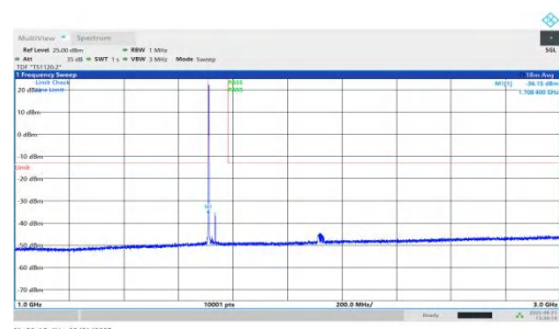
NTNV-n66-PC2-15-25-L-DFT-QPSK-Inner_1RB_Left-1000-3000-P ASS
