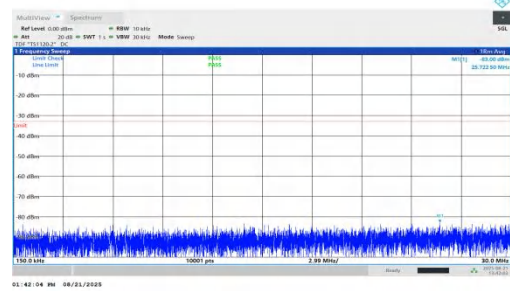
NTNV-n66-PC2-15-25-M-DFT-QPSK-Inner_1RB_Right-0.15-30-P ASS
