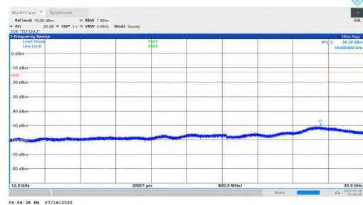
NTNV-n66-PC2-15-35-L-DFT-BPSK-Inner_1RB_Right-12000-200 00-PASS
