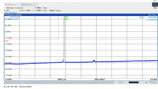
NTNV-n66-PC2-15-25-H-DFT-BPSK-Inner_1RB_Right-1000-3000- PASS
