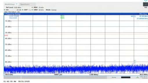
NTNV-n66-PC2-15-25-H-DFT-BPSK-Inner_1RB_Left-0.15-30-PAS
