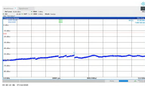
NTNV-n66-PC2-15-20-H-DFT-QPSK-Inner_1RB_Right-3000-12000-PASS
