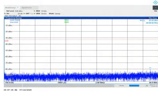
NTV-n66-PC2-15-30-L-DFT-QPSK-Inner_1RB_Right-0.15-30-PASS
