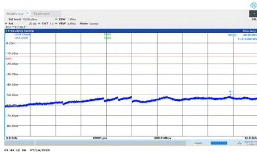
NTNV-n66-PC2-15-30-M-DFT-BPSK-Inner_1RB_Right-3000-12000-PASS
