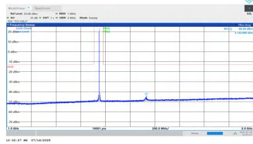
NTNV-n66-PC2-15-40-L-DFT-BPSK-Inner_1RB_Right-1000-3000-P PASS
