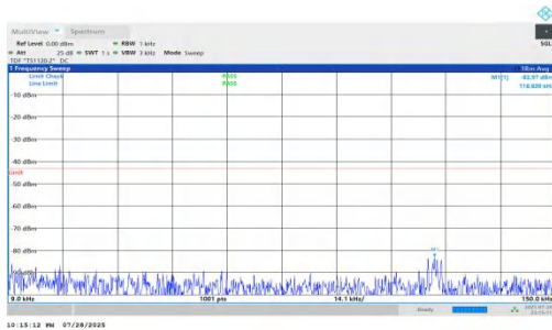
NTNV-n66-PC2-15-35-M-DFT-QPSK-Inner_1RB_Left-0.009-0.15-PASS
