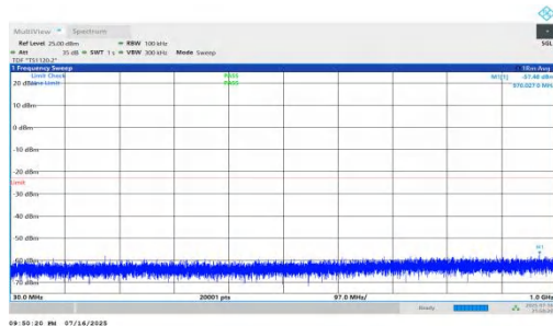
NTNV-n66-PC2-15-30-M-DFT-QPSK-Inner_1RB_Right-30-1000- PASS
