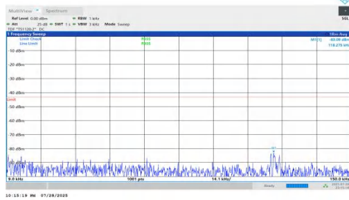
NTNV-n66-PC2-15-35-M-DFT-QPSK-Inner_1RB_Right-0.009-0.1 5-PASS
