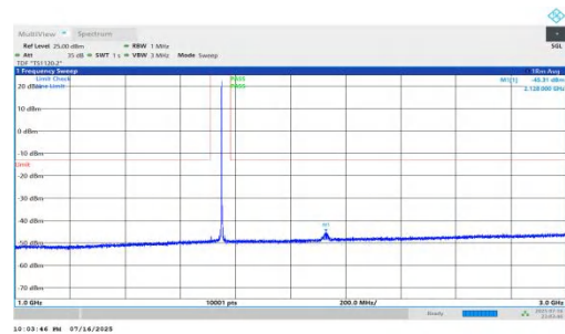
NTVN-n66-PC2-15-40-L-DFT-QPSK-Inner_1RB_Right-1000-3000-P PASS
