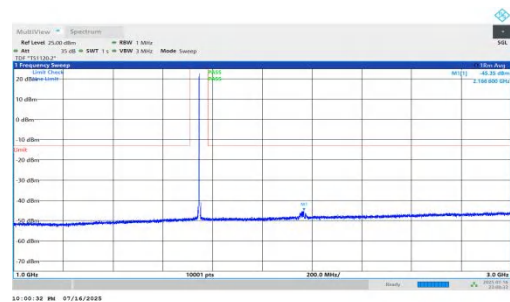
NTNV-n66-PC2-15-35-H-DFT-QPSK-Inner_1RB_Left-1000-3000- PASS
