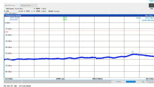
NTNV-n66-PC2-15-35-H-DFT-BPSK-Inner_1RB_Right-12000-200 00-PASS
