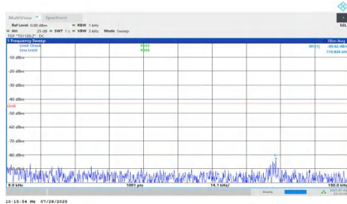
NTNV-n66-PC2-15-35-H-DFT-BPSK-Inner_1RB_Right-0.009-0.15-PASS
