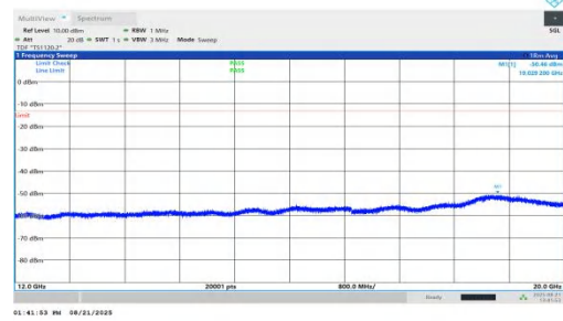
NTNV-n66-PC2-15-25-M-DFT-QPSK-Inner_1RB_Left-12000-2000 0-PASS
