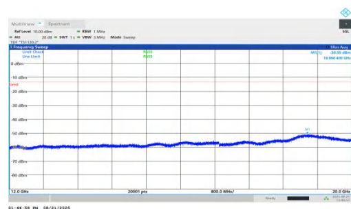
NTNV-n66-PC2-15-25-H-DFT-QPSK-Inner_1RB_Right-12000-200 00-PASS
