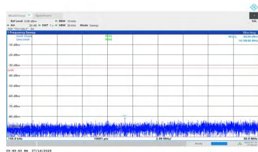
NTNV-n66-PC2-15-30-M-DFT-QPSK-Inner_1RB_Left-0.15-30-PASS
