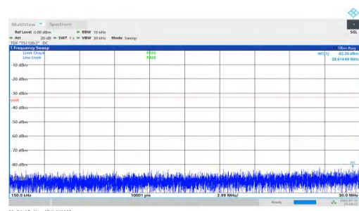
NTNV-n66-PC2-15-35-L-DFT-BPSK-Inner_1RB_Right-0.15-30-PASS
