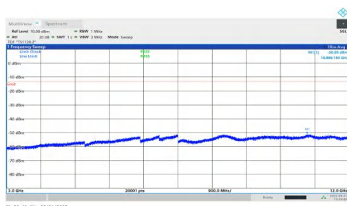
NTVN-n66-PC2-15-25-L-DFT-QPSK-Inner_1RB_Right-3000-12000- 00-PASS
