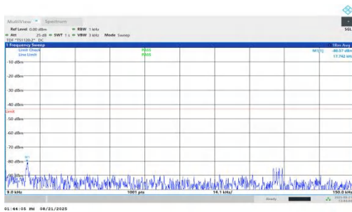
NTNV-n66-PC2-15-25-H-DFT-QPSK-Inner_1RB_Left-0.009-0.15- PASS
