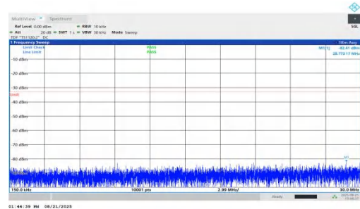
NTNV-n66-PC2-15-25-H-DFT-QPSK-Inner_1RB_Right-0.15-30-PA SS
