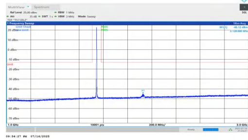
NTNV-n66-PC2-15-35-L-DFT-BPSK-Inner_1RB_Right-1000-3000-P PASS
