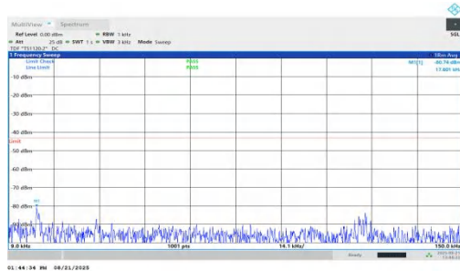
NTNV-n66-PC2-15-25-H-DFT-QPSK-Inner_1RB_Right-0.009-0.1 5-PASS
