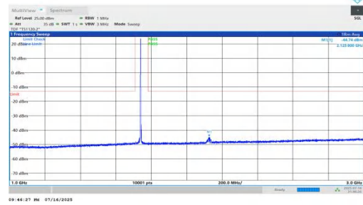
NTNV-n66-PC2-15-30-L-DFT-BPSK-Inner_1RB_Right-1000-3000-P PASS
