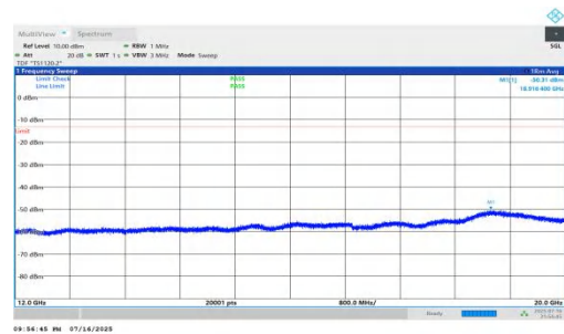
NTNV-n66-PC2-15-35-M-DFT-BPSK-Inner_1RB_Left-12000-20000-PASS
