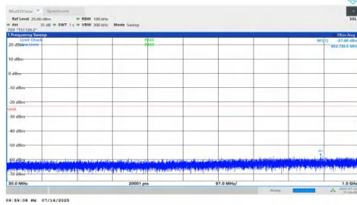
NTNV-n66-PC2-15-35-H-DFT-BPSK-Inner_1RB_Left-30-1000-PASS
