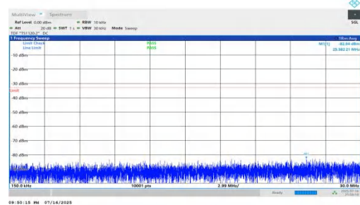
NTNV-n66-PC2-15-30-M-DFT-QPSK-Inner_1RB_Right-0.15-30-P ASS
