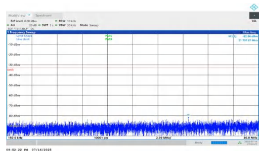
NTNV-n66-PC2-15-30-H-DFT-QPSK-Inner_1RB_Left-0.15-30-PAS S
