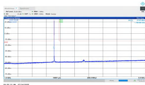
NTNV-n66-PC2-15-35-L-DFT-QPSK-Inner_1RB_Left-1000-3000-P ASS
