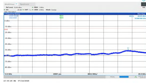
NTVN-n66-PC2-15-40-L-DFT-QPSK-Inner_1RB_Left-12000-2000 0-PASS
