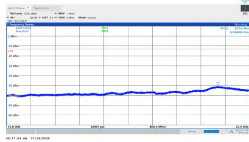
NTV-n66-PC2-15-30-L-DFT-QPSK-Inner_1RB_Left-12000-2000 0-PASS
