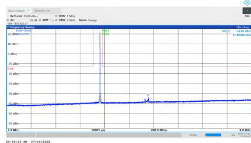
NTNV-n66-PC2-15-35-M-DFT-QPSK-Inner_1RB_Right-1000-3000 -PASS
