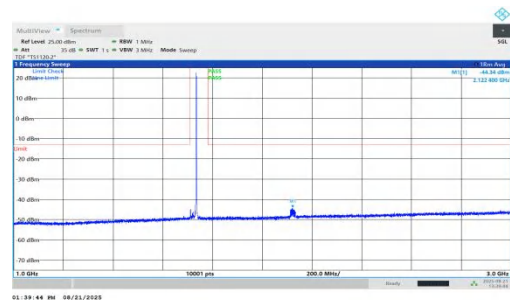
NTVN-n66-PC2-15-25-L-DFT-QPSK-Inner_1RB_Right-1000-3000- PASS
