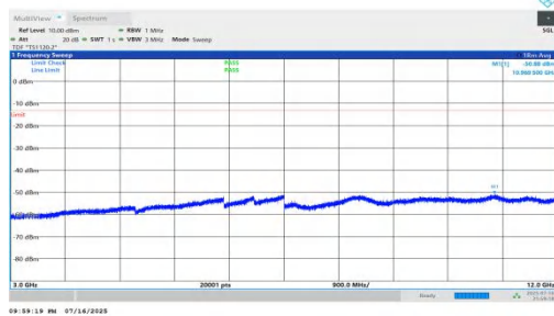
NTNV-n66-PC2-15-35-H-DFT-BPSK-Inner_1RB_Left-3000-12000-PASS
