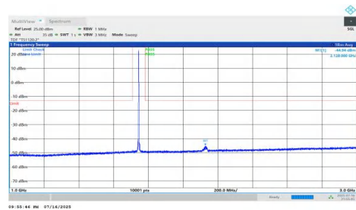
NTV-n66-PC2-15-35-L-DFT-QPSK-Inner_1RB_Right-1000-3000-P PASS
