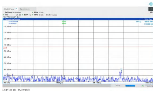
NTVN-n66-PC2-15-40-L-DFT-QPSK-Inner_1RB_Right-0.009-0.1 5-PASS
