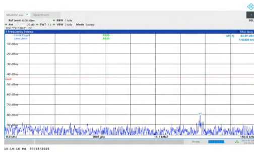
NTV-n66-PC2-15-35-L-DFT-QPSK-Inner_1RB_Right-0.009-0.1 5-PASS
