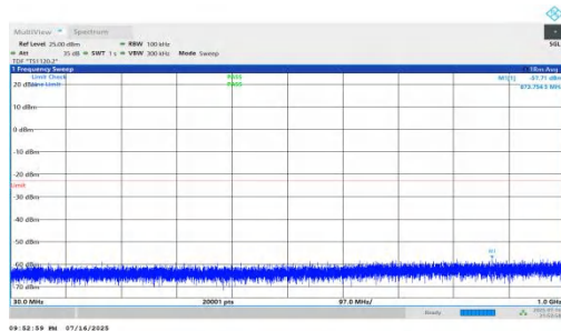
NTNV-n66-PC2-15-30-H-DFT-QPSK-Inner_1RB_Right-30-1000- PASS
