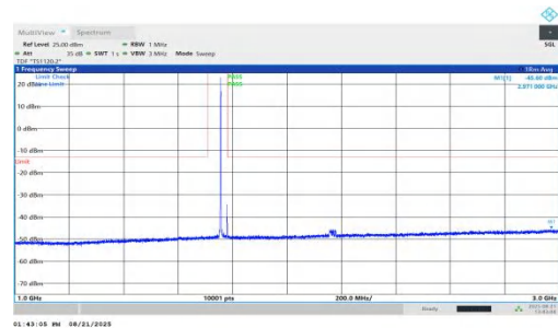
NTNV-n66-PC2-15-25-H-DFT-BPSK-Inner_1RB_Left-1000-3000-PASS
