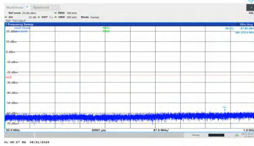
NTNV-n66-PC2-15-25-L-DFT-BPSK-Inner_1RB_Right-30-1000-P ASS
