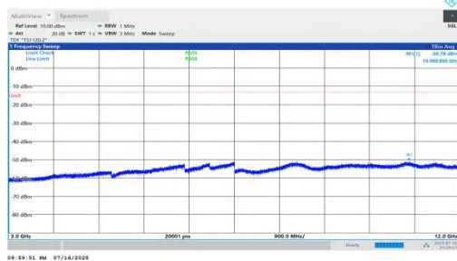
NTNV-n66-PC2-15-35-H-DFT-BPSK-Inner_1RB_Right-3000-120 00-PASS
