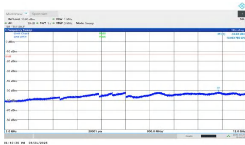
NTNV-n66-PC2-15-25-M-DFT-BPSK-Inner_1RB_Left-3000-12000-PASS
