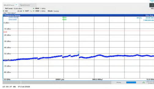
NTNV-n66-PC2-15-35-H-DFT-QPSK-Inner_1RB_Left-3000-1200 0-PASS
