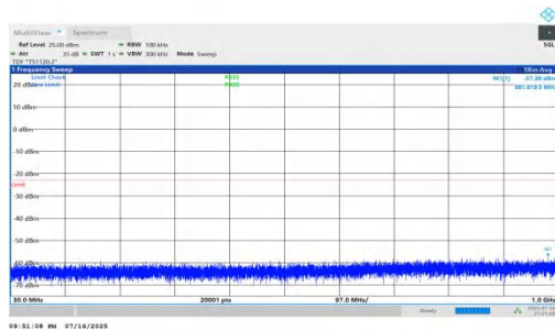
NTNV-n66-PC2-15-30-H-DFT-BPSK-Inner_1RB_Left-30-1000-PASS
