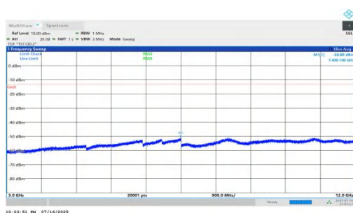
NTVN-n66-PC2-15-40-L-DFT-QPSK-Inner_1RB_Right-3000-12000 00-PASS
