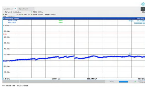
NTNV-n66-PC2-15-35-M-DFT-BPSK-Inner_1RB_Left-3000-12000-PASS
