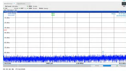
NTNV-n66-PC2-15-35-L-DFT-BPSK-Inner_1RB_Left-0.15-30-PASS
