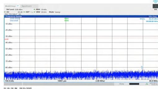
NTNV-n66-PC2-15-25-M-DFT-QPSK-Inner_1RB_Left-0.15-30-PASS
