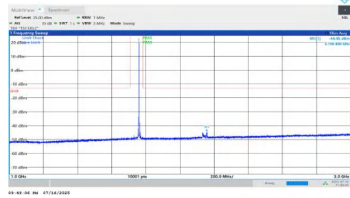
NTNV-n66-PC2-15-30-M-DFT-BPSK-Inner_1RB_Right-1000-3000-PASS
