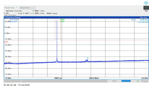
NTNV-n66-PC2-15-30-M-DFT-BPSK-Inner_1RB_Left-1000-3000-PASS
