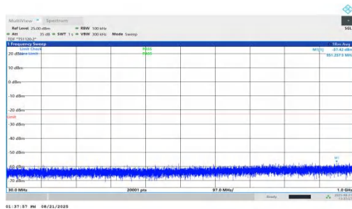
NTNV-n66-PC2-15-25-L-DFT-BPSK-Inner_1RB_Left-30-1000-PA SS
