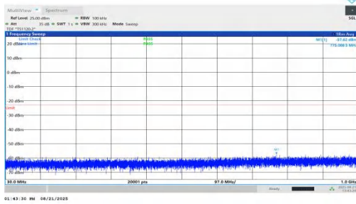
NTNV-n66-PC2-15-25-H-DFT-BPSK-Inner_1RB_Right-30-1000-P ASS
