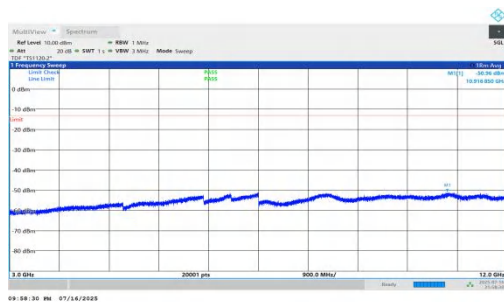
NTNV-n66-PC2-15-35-M-DFT-QPSK-Inner_1RB_Right-3000-120 00-PASS
