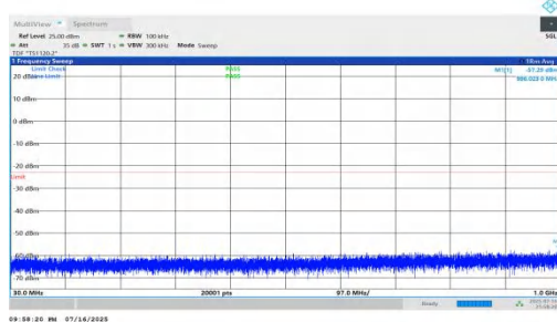
NTNV-n66-PC2-15-35-M-DFT-QPSK-Inner_1RB_Right-30-1000- PASS
