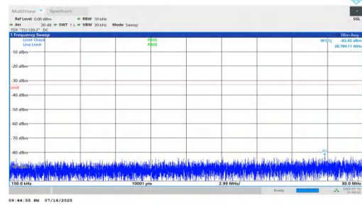
NTNV-n66-PC2-15-20-H-DFT-QPSK-Inner_1RB_Right-0.15-30-PA SS
