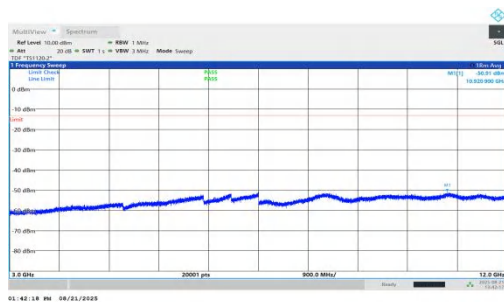
NTNV-n66-PC2-15-25-M-DFT-QPSK-Inner_1RB_Right-3000-120 00-PASS
