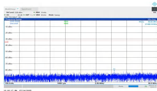
NTNV-n66-PC2-15-40-L-DFT-BPSK-Inner_1RB_Right-0.15-30-PA SS
