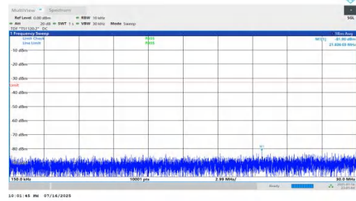
NTNV-n66-PC2-15-40-L-DFT-BPSK-Inner_1RB_Left-0.15-30-PAS S
