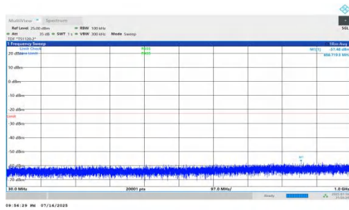
NTNV-n66-PC2-15-35-M-DFT-BPSK-Inner_1RB_Left-30-1000-PASS
