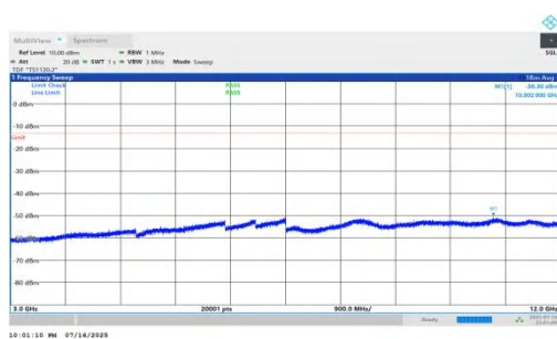
NTNV-n66-PC2-15-35-H-DFT-QPSK-Inner_1RB_Right-3000-12000-PASS
