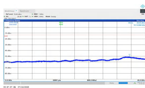
NTV-n66-PC2-15-30-L-DFT-QPSK-Inner_1RB_Right-12000-20000-00-PASS
