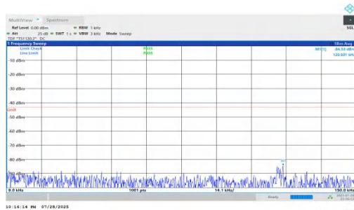
NTNV-n66-PC2-15-35-H-DFT-QPSK-Inner_1RB_Left-0.009-0.15- PASS
