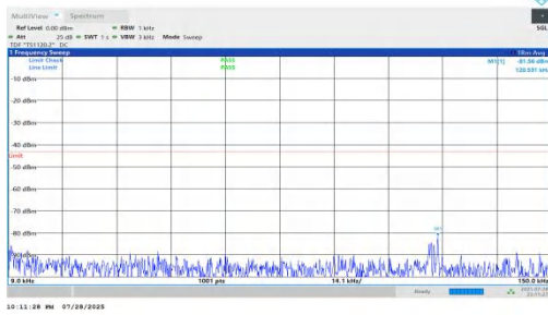
NTNV-n66-PC2-15-30-M-DFT-BPSK-Inner_1RB_Left-0.009-0.15-PASS
