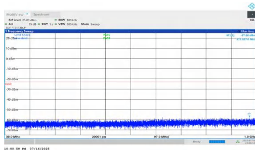
NTNV-n66-PC2-15-35-H-DFT-QPSK-Inner_1RB_Right-30-1000- PASS
