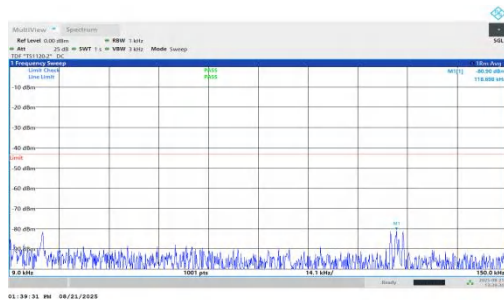
NTVN-n66-PC2-15-25-L-DFT-QPSK-Inner_1RB_Right-0.009-0.1 5-PASS
