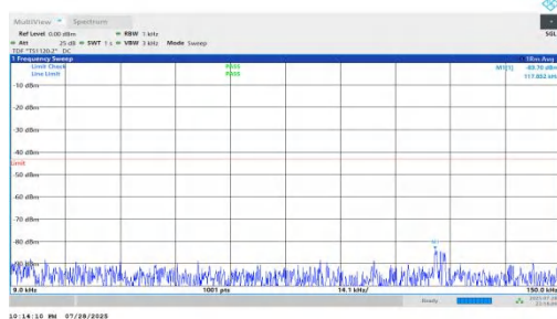
NTNV-n66-PC2-15-35-L-DFT-QPSK-Inner_1RB_Left-0.009-0.15- PASS
