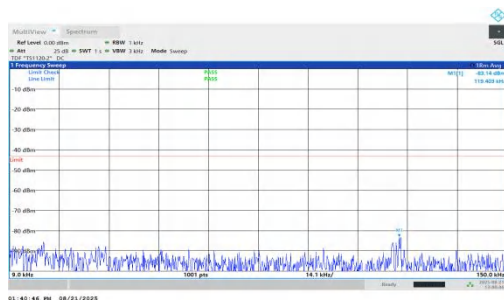
NTNV-n66-PC2-15-25-M-DFT-BPSK-Inner_1RB_Right-0.009-0.15-PASS
