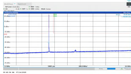
NTNV-n66-PC2-15-30-L-DFT-BPSK-Inner_1RB_Left-1000-3000-PASS
