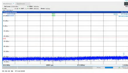
NTNV-n66-PC2-15-35-L-DFT-BPSK-Inner_1RB_Right-30-1000-P ASS
