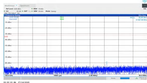
NTNV-n66-PC2-15-35-L-DFT-QPSK-Inner_1RB_Left-0.15-30-PAS S
