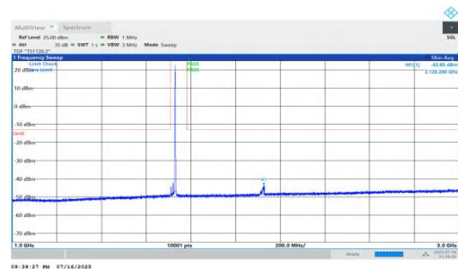
NTVN-n66-PC2-15-20-L-DFT-QPSK-Inner_1RB_Right-1000-3000- PASS
