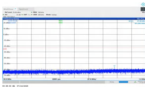
NTNV-n66-PC2-15-20-L-DFT-QPSK-Inner_1RB_Left-30-1000-PA SS
