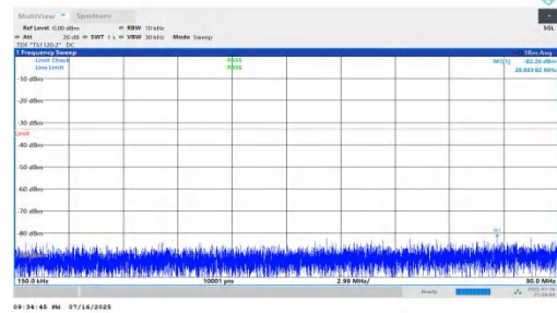
NTNV-n66-PC2-15-15-H-DFT-BPSK-Inner_1RB_Left-0.15-30-PAS
