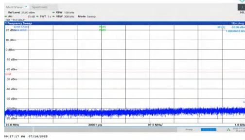
NTNV-n66-PC2-15-10-H-DFT-BPSK-Inner_1RB_Right-30-1000-P ASS
