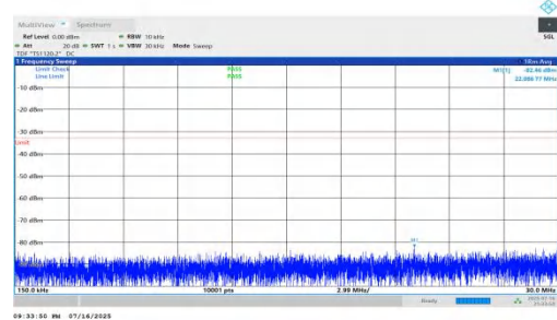
NTNV-n66-PC2-15-15-M-DFT-QPSK-Inner_1RB_Right-0.15-30-P ASS
