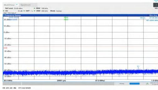
NTNV-n66-PC2-15-15-L-DFT-BPSK-Inner_1RB_Left-30-1000-PASS SS
