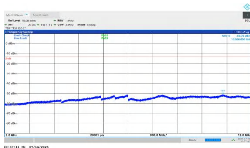
NTNV-n66-PC2-15-20-L-DFT-BPSK-Inner_1RB_Left-3000-12000-PASS
