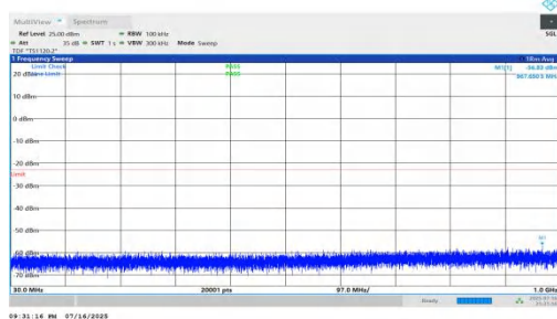
NTV-n66-PC2-15-15-L-DFT-QPSK-Inner_1RB_Right-30-1000-PASS
