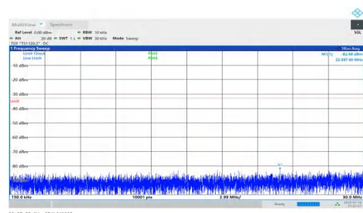
NTNV-n66-PC2-15-20-L-DFT-BPSK-Inner_1RB_Right-0.15-30-PASS
