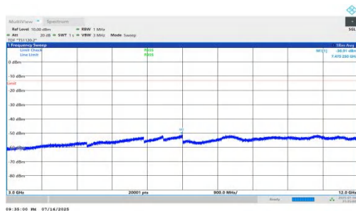
NTNV-n66-PC2-15-15-H-DFT-BPSK-Inner_1RB_Left-3000-12000-PASS
