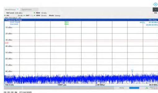
NTNV-n66-PC2-15-15-L-DFT-QPSK-Inner_1RB_Left-0.15-30-PAS S
