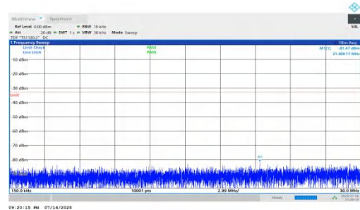
NTNV-n66-PC2-15-5-H-DFT-QPSK-Inner_1RB_Right-0.15-30-PA-SS
