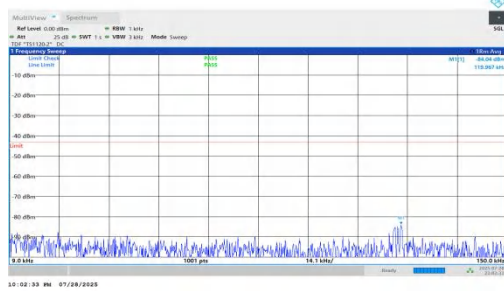
NTNV-n66-PC2-15-10-M-DFT-QPSK-Inner_1RB_Right-0.009-0.1 5-PASS
