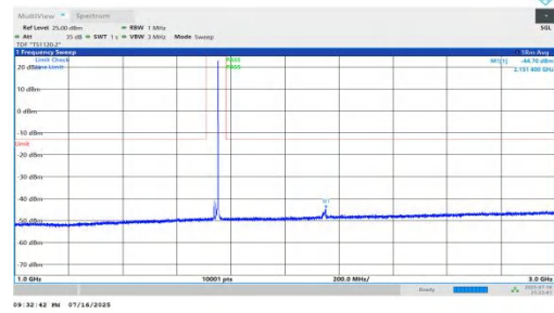
NTNV-n66-PC2-15-15-M-DFT-BPSK-Inner_1RB_Right-1000-3000-PASS
