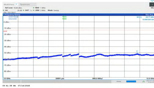
NTNV-n66-PC2-15-20-M-DFT-QPSK-Inner_1RB_Left-3000-1200 0-PASS
