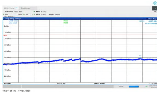
NTNV-n66-PC2-15-10-H-DFT-BPSK-Inner_1RB_Right-3000-120 00-PASS
