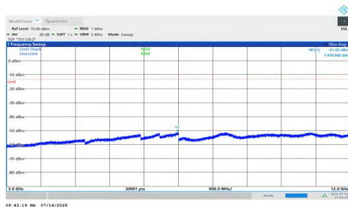
NTNV-n66-PC2-15-20-H-DFT-BPSK-Inner_1RB_Left-3000-12000-PASS
