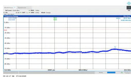
NTNV-n66-PC2-15-5-H-DFT-BPSK-Inner_1RB_Right-12000-2000 0-PASS
