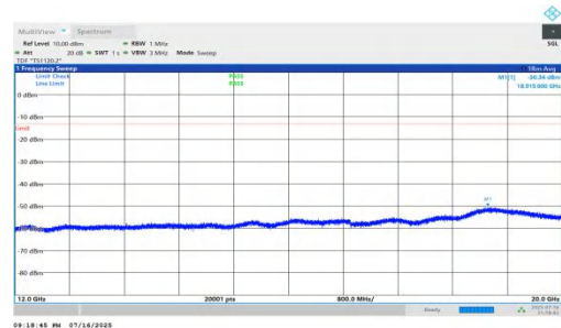
NTNV-n66-PC2-15-5-H-DFT-BPSK-Inner_1RB_Left-12000-20000- PASS
