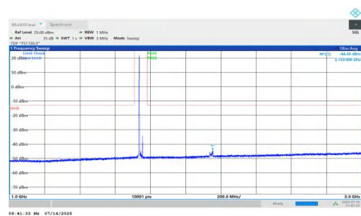
NTNV-n66-PC2-15-20-M-DFT-QPSK-Inner_1RB_Left-1000-3000-PASS
