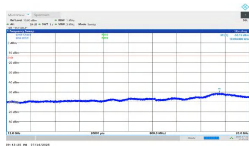
NTNV-n66-PC2-15-20-H-DFT-BPSK-Inner_1RB_Left-12000-20000-PASS
