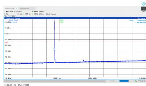
NTNV-n66-PC2-15-10-L-DFT-BPSK-Inner_1RB_Left-1000-3000-PASS
