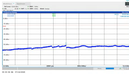
NTV-n66-PC2-15-15-L-DFT-QPSK-Inner_1RB_Left-3000-12000-PASS
