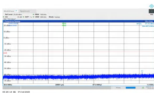
NTNV-n66-PC2-15-10-M-DFT-QPSK-Inner_1RB_Left-30-1000-PASS
