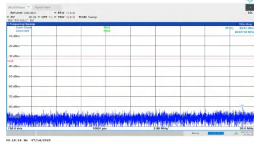
NTNV-n66-PC2-15-5-H-DFT-BPSK-Inner_1RB_Left-0.15-30-PASS
