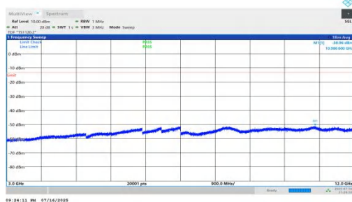
NTNV-n66-PC2-15-10-M-DFT-BPSK-Inner_1RB_Left-3000-12000-PASS
