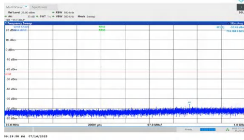
NTNV-n66-PC2-15-15-L-DFT-BPSK-Inner_1RB_Right-30-1000-P ASS
