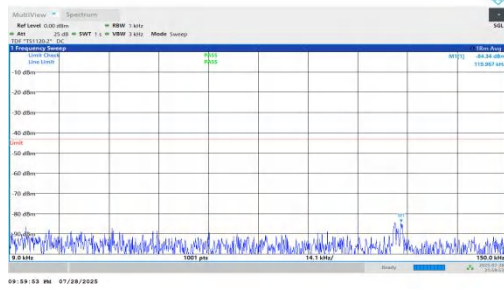
NTNV-n66-PC2-15-5-H-DFT-BPSK-Inner_1RB_Left-0.009-0.15-P ASS
