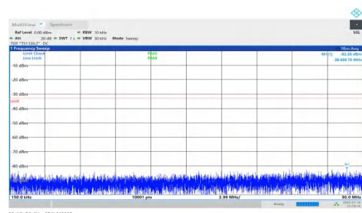
NTNV-n66-PC2-15-5-H-DFT-BPSK-Inner_1RB_Right-0.15-30-PAS S
