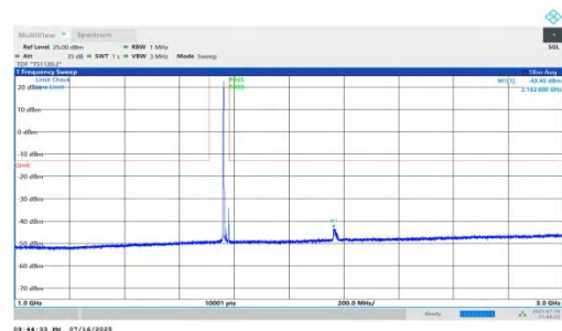
NTNV-n66-PC2-15-20-H-DFT-QPSK-Inner_1RB_Left-1000-3000- PASS
