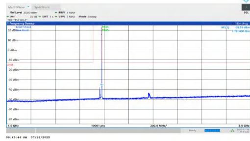
NTNV-n66-PC2-15-20-H-DFT-BPSK-Inner_1RB_Right-1000-3000-P PASS
