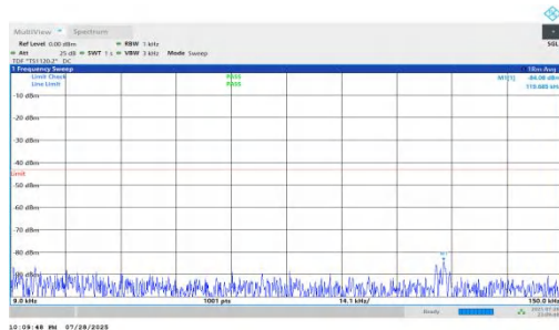
NTNV-n66-PC2-15-20-H-DFT-QPSK-Inner_1RB_Left-0.009-0.15- PASS
