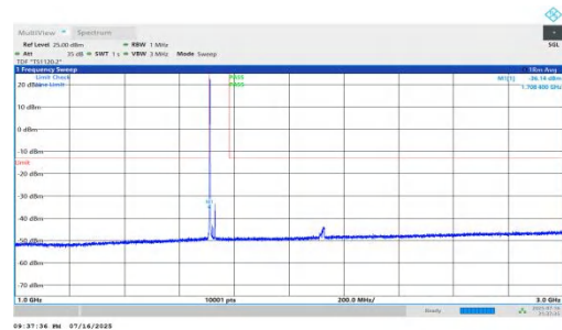
NTNV-n66-PC2-15-20-L-DFT-BPSK-Inner_1RB_Left-1000-3000-PASS
