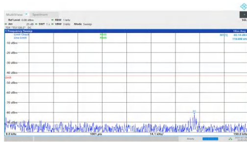
NTNV-n66-PC2-15-10-M-DFT-BPSK-Inner_1RB_Right-0.009-0.15-PASS
