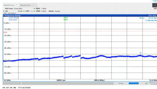
NTNV-n66-PC2-15-15-L-DFT-BPSK-Inner_1RB_Left-3000-12000 -PASS
