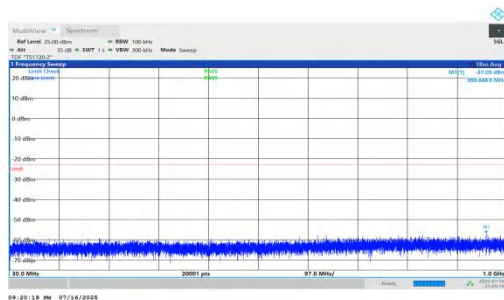
NTNV-n66-PC2-15-5-H-DFT-QPSK-Inner_1RB_Right-30-1000-PASS
