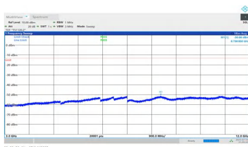
NTNV-n66-PC2-15-5-H-DFT-QPSK-Inner_1RB_Right-3000-12000-PASS
