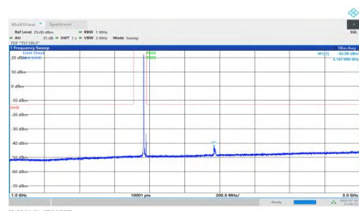
NTNV-n66-PC2-15-15-H-DFT-QPSK-Inner_1RB_Left-1000-3000-PASS
