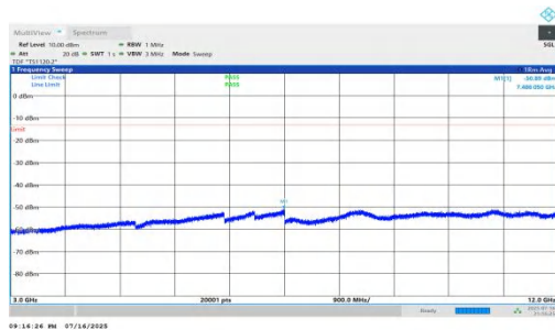
NTNV-n66-PC2-15-5-M-DFT-BPSK-Inner_1RB_Right-3000-1200 0-PASS
