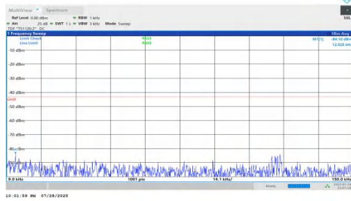
NTNV-n66-PC2-15-10-M-DFT-BPSK-Inner_1RB_Left-0.009-0.15-PASS
