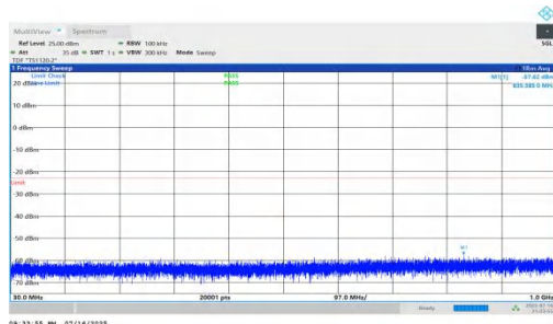
NTNV-n66-PC2-15-15-M-DFT-QPSK-Inner_1RB_Right-30-1000- PASS
