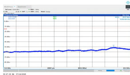
NTNV-n66-PC2-15-10-H-DFT-BPSK-Inner_1RB_Right-12000-200 00-PASS
