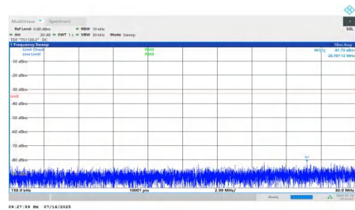
NTNV-n66-PC2-15-10-H-DFT-QPSK-Inner_1RB_Left-0.15-30-PAS S
