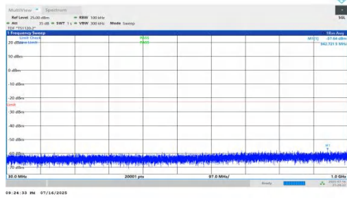
NTNV-n66-PC2-15-10-M-DFT-BPSK-Inner_1RB_Right-30-1000-PASS
