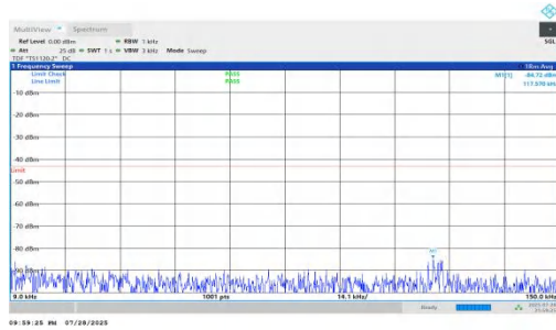
NTNV-n66-PC2-15-5-M-DFT-QPSK-Inner_1RB_Right-0.009-0.15 -PASS
