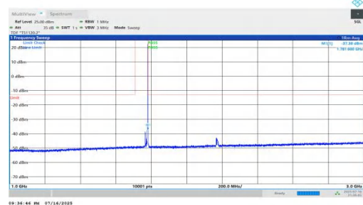
NTNV-n66-PC2-15-15-H-DFT-QPSK-Inner_1RB_Right-1000-3000 -PASS
