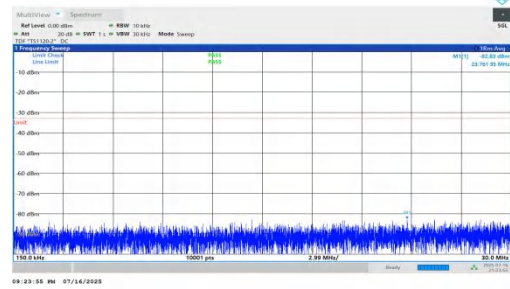
NTNV-n66-PC2-15-10-M-DFT-BPSK-Inner_1RB_Left-0.15-30-PASS
