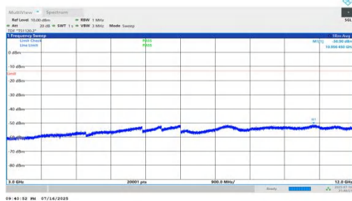
NTNV-n66-PC2-15-20-M-DFT-BPSK-Inner_1RB_Right-3000-12000-PASS
