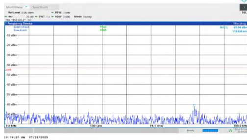
NTNV-n66-PC2-15-20-H-DFT-BPSK-Inner_1RB_Left-0.009-0.15-PASS
