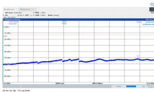
NTNV-n66-PC2-15-20-M-DFT-BPSK-Inner_1RB_Left-3000-12000-PASS
