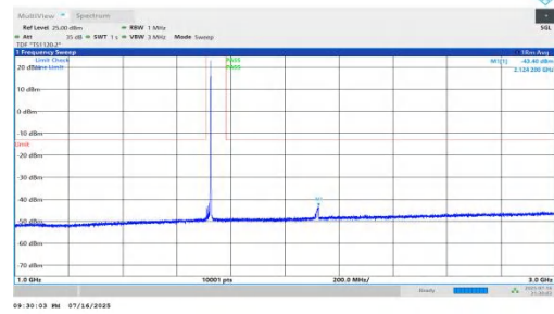
NTNV-n66-PC2-15-15-L-DFT-BPSK-Inner_1RB_Right-1000-3000-P PASS
