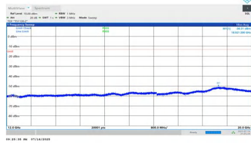
NTNV-n66-PC2-15-10-M-DFT-QPSK-Inner_1RB_Left-12000-2000 0-PASS
