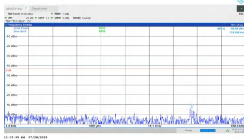
NTNV-n66-PC2-15-10-H-DFT-QPSK-Inner_1RB_Right-0.009-0.1 5-PASS
