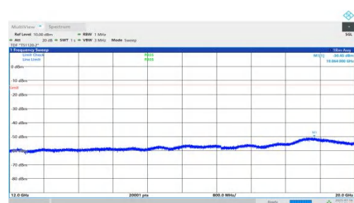
NTNV-n66-PC2-15-15-M-DFT-QPSK-Inner_1RB_Right-12000-20000-PASS
