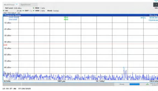
NTNV-n66-PC2-15-10-L-DFT-BPSK-Inner_1RB_Left-0.009-0.15-PASS
