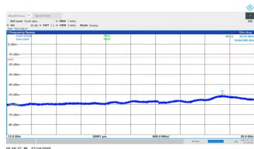
NTNV-n66-PC2-15-10-M-DFT-QPSK-Inner_1RB_Right-12000-20000- 00-PASS
