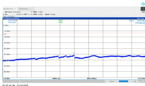
NTNV-n66-PC2-15-10-H-DFT-BPSK-Inner_1RB_Left-3000-12000-PASS
