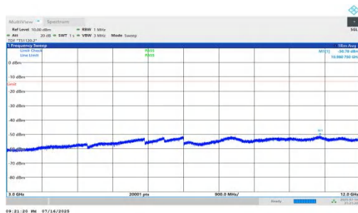
NTNV-n66-PC2-15-10-L-DFT-BPSK-Inner_1RB_Left-3000-12000-PASS
