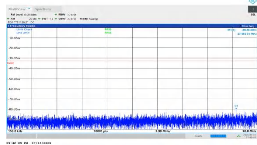
NTNV-n66-PC2-15-20-M-DFT-QPSK-Inner_1RB_Right-0.15-30-P ASS
