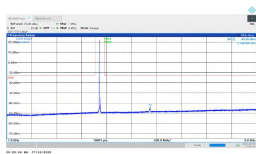
NTNV-n66-PC2-15-10-M-DFT-QPSK-Inner_1RB_Left-1000-3000-PASS
