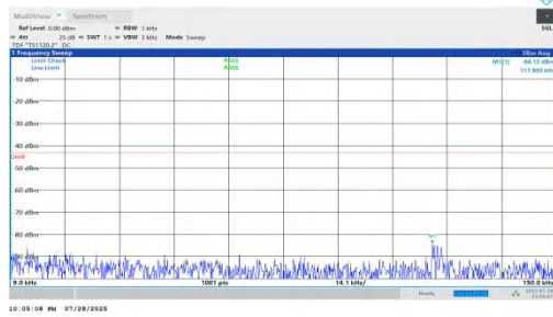
NTNV-n66-PC2-15-15-M-DFT-BPSK-Inner_1RB_Left-0.009-0.15-PASS
