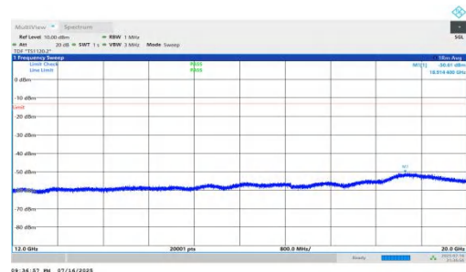
NTNV-n66-PC2-15-15-H-DFT-QPSK-Inner_1RB_Right-12000-200 00-PASS
