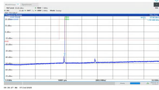
NTNV-n66-PC2-15-15-H-DFT-BPSK-Inner_1RB_Right-1000-3000-PASS
