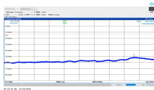
NTNV-n66-PC2-15-5-M-DFT-BPSK-Inner_1RB_Right-12000-2000 0-PASS
