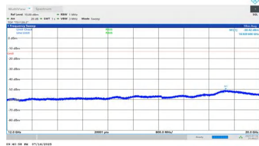
NTNV-n66-PC2-15-20-M-DFT-BPSK-Inner_1RB_Right-12000-20000-PASS
