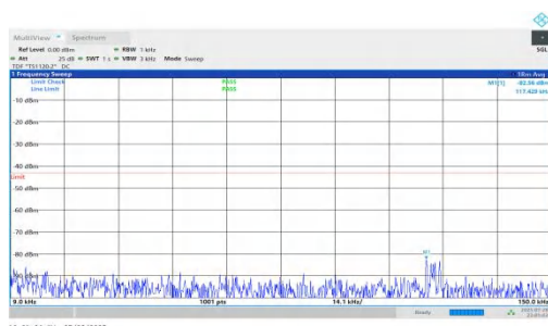
NTNV-n66-PC2-15-10-L-DFT-BPSK-Inner_1RB_Right-0.009-0.15-PASS
