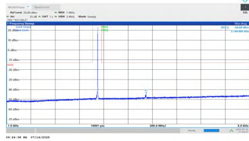
NTNV-n66-PC2-15-10-M-DFT-BPSK-Inner_1RB_Right-1000-3000-PASS
