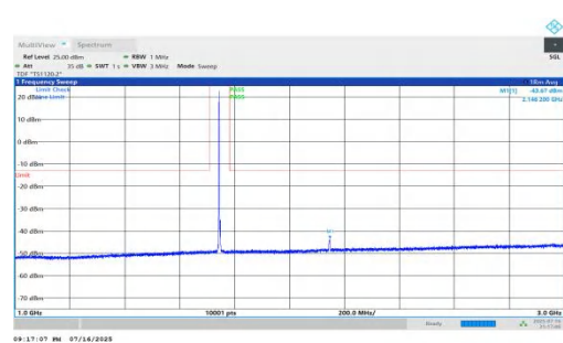
NTNV-n66-PC2-15-5-M-DFT-QPSK-Inner_1RB_Left-1000-3000-P ASS
