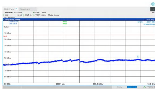
NTV-n66-PC2-15-15-L-DFT-QPSK-Inner_1RB_Right-3000-12000-PASS
