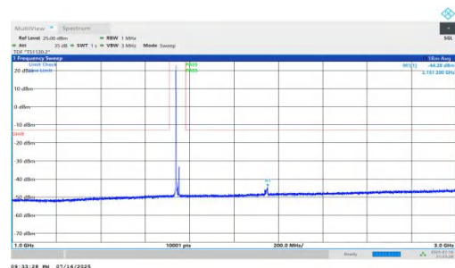
NTNV-n66-PC2-15-15-M-DFT-QPSK-Inner_1RB_Left-1000-3000-PASS
