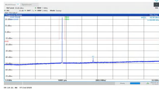
NTNV-n66-PC2-15-5-M-DFT-BPSK-Inner_1RB_Right-1000-3000-P PASS
