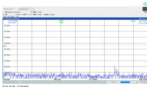
NTNV-n66-PC2-15-5-M-DFT-QPSK-Inner_1RB_Left-0.009-0.15- PASS
