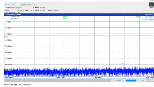
NTNV-n66-PC2-15-15-L-DFT-BPSK-Inner_1RB_Left-0.15-30-PAS S
