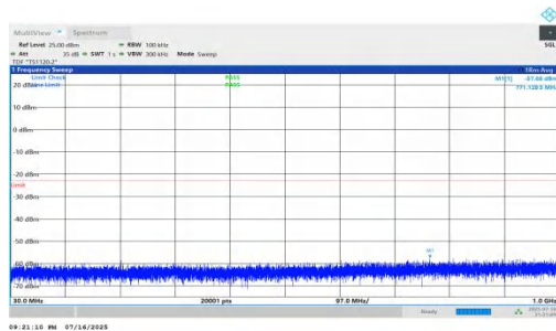
NTNV-n66-PC2-15-10-L-DFT-BPSK-Inner_1RB_Left-30-1000-PASS
