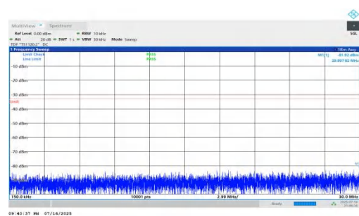
NTNV-n66-PC2-15-20-M-DFT-BPSK-Inner_1RB_Right-0.15-30-PASS
