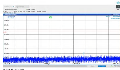
NTNV-n66-PC2-15-15-M-DFT-QPSK-Inner_1RB_Left-0.15-30-PASS
