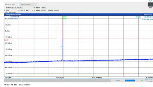
NTNV-n66-PC2-15-5-H-DFT-BPSK-Inner_1RB_Right-1000-3000-P PASS
