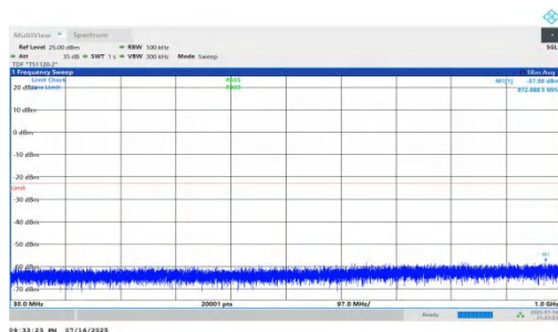
NTNV-n66-PC2-15-15-M-DFT-QPSK-Inner_1RB_Left-30-1000-PASS
