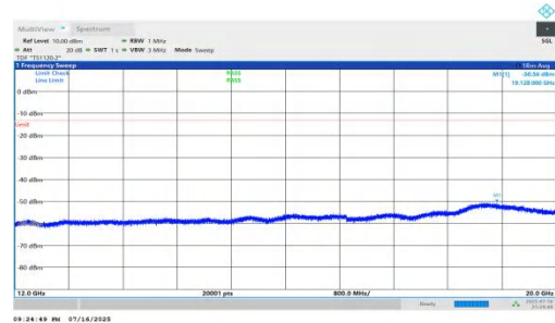
NTNV-n66-PC2-15-10-M-DFT-BPSK-Inner_1RB_Right-12000-20000-PASS
