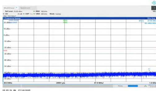
NTNV-n66-PC2-15-10-M-DFT-QPSK-Inner_1RB_Right-30-1000- PASS
