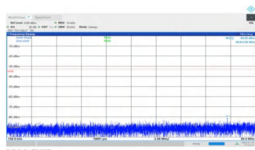
NTNV-n66-PC2-15-15-M-DFT-BPSK-Inner_1RB_Right-0.15-30-PASS
