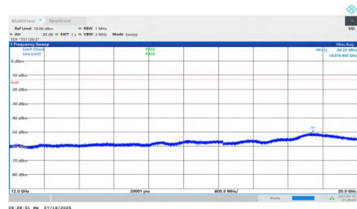
NTNV-n66-PC2-15-10-H-DFT-QPSK-Inner_1RB_Right-12000-20000- 00-PASS
