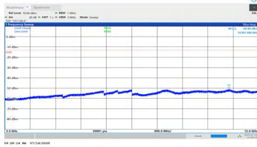
NTNV-n66-PC2-15-10-H-DFT-QPSK-Inner_1RB_Left-3000-1200 0-PASS
