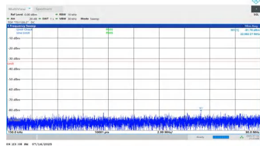
NTNV-n66-PC2-15-10-L-DFT-QPSK-Inner_1RB_Right-0.15-30-PA SS
