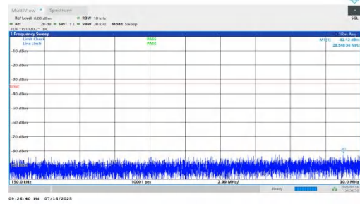
NTNV-n66-PC2-15-10-H-DFT-BPSK-Inner_1RB_Left-0.15-30-PAS
