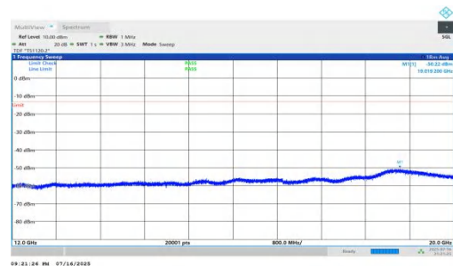
NTNV-n66-PC2-15-10-L-DFT-BPSK-Inner_1RB_Left-12000-20000-PASS
