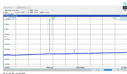
NTNV-n66-PC2-15-5-M-DFT-QPSK-Inner_1RB_Right-1000-3000- PASS
