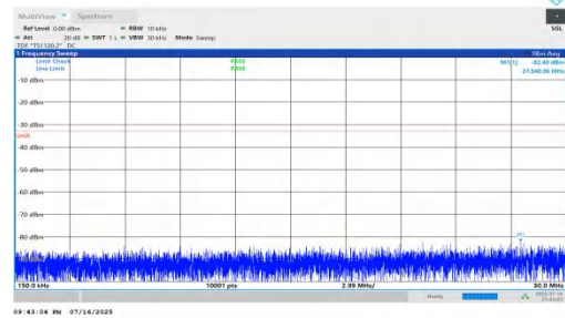
NTNV-n66-PC2-15-20-H-DFT-BPSK-Inner_1RB_Left-0.15-30-PAS
