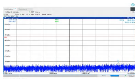
NTNV-n66-PC2-15-15-H-DFT-BPSK-Inner_1RB_Right-0.15-30-PASS
