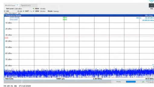
NTNV-n66-PC2-15-10-H-DFT-QPSK-Inner_1RB_Right-0.15-30-PA SS
