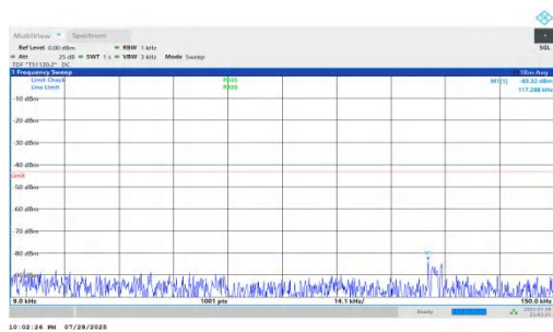
NTNV-n66-PC2-15-10-M-DFT-QPSK-Inner_1RB_Left-0.009-0.15-PASS
