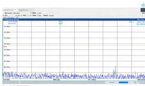
NTNV-n66-PC2-15-5-H-DFT-BPSK-Inner_1RB_Right-0.009-0.15- PASS
