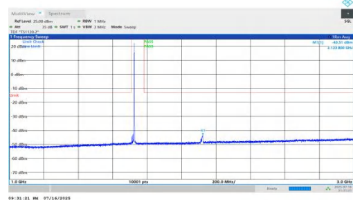
NTV-n66-PC2-15-15-L-DFT-QPSK-Inner_1RB_Right-1000-3000-PASS
