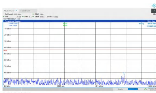
NTNV-n66-PC2-15-20-H-DFT-BPSK-Inner_1RB_Right-0.009-0.15-5-PASS
