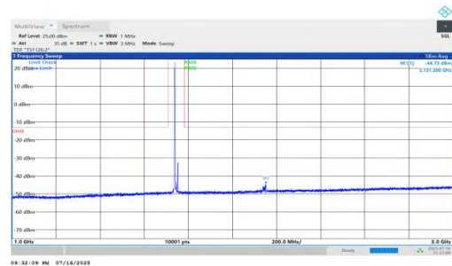
NTNV-n66-PC2-15-15-M-DFT-BPSK-Inner_1RB_Left-1000-3000-PASS
