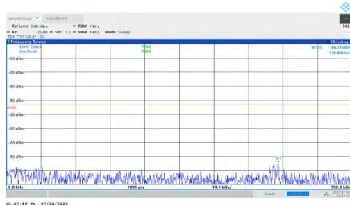
NTVN-n66-PC2-15-20-L-DFT-QPSK-Inner_1RB_Right-0.009-0.1 5-PASS
