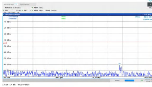
NTNV-n66-PC2-15-20-M-DFT-BPSK-Inner_1RB_Left-0.009-0.15-PASS
