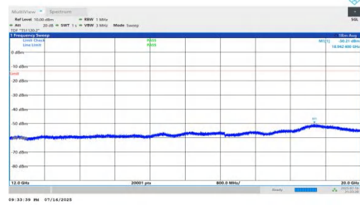
NTNV-n66-PC2-15-15-M-DFT-QPSK-Inner_1RB_Left-12000-2000 0-PASS
