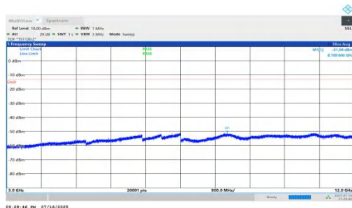
NTNV-n66-PC2-15-10-H-DFT-QPSK-Inner_1RB_Right-3000-12000- 00-PASS
