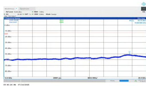
NTNV-n66-PC2-15-20-M-DFT-BPSK-Inner_1RB_Left-12000-20000-PASS
