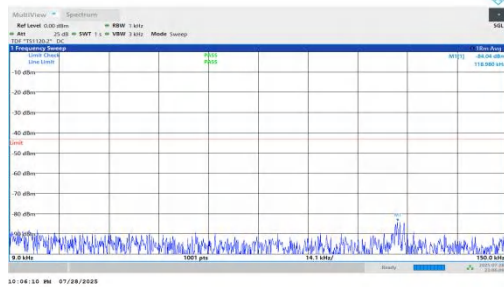
NTNV-n66-PC2-15-15-H-DFT-BPSK-Inner_1RB_Left-0.009-0.15-PASS
