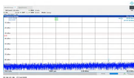
NTNV-n66-PC2-15-20-H-DFT-QPSK-Inner_1RB_Left-0.15-30-PAS S
