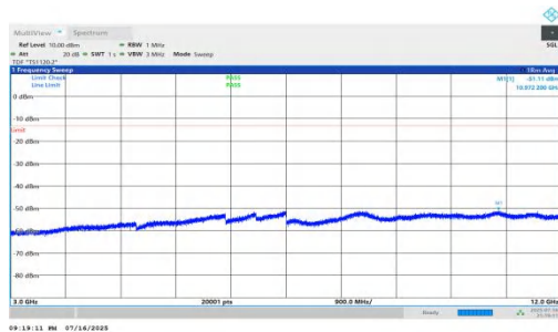
NTNV-n66-PC2-15-5-H-DFT-BPSK-Inner_1RB_Right-3000-1200 0-PASS
