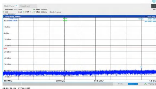
NTNV-n66-PC2-15-10-H-DFT-QPSK-Inner_1RB_Right-30-1000- PASS
