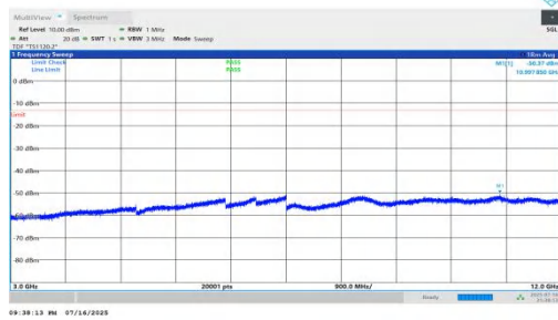
NTNV-n66-PC2-15-20-L-DFT-BPSK-Inner_1RB_Right-3000-1200 0-PASS
