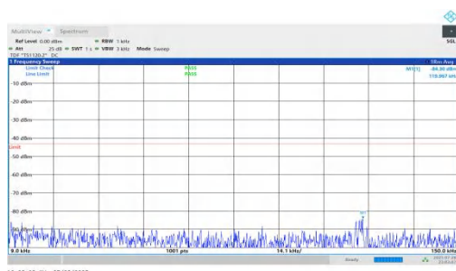
NTNV-n66-PC2-15-10-H-DFT-BPSK-Inner_1RB_Right-0.009-0.15-PASS
