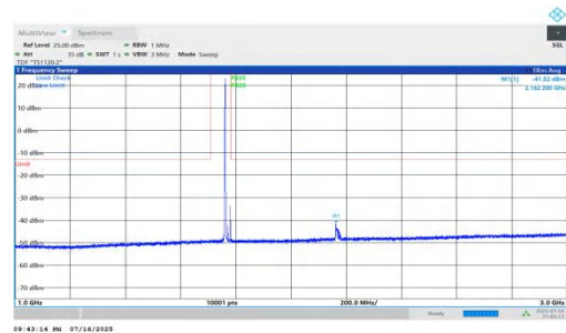
NTNV-n66-PC2-15-20-H-DFT-BPSK-Inner_1RB_Left-1000-3000-PASS
