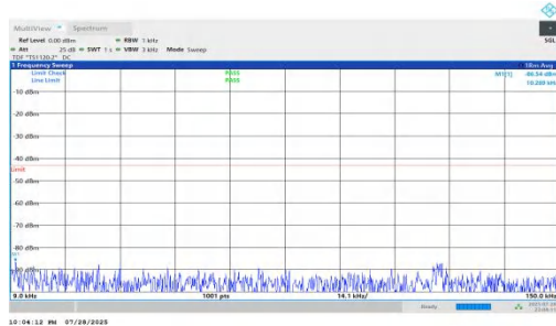
NTNV-n66-PC2-15-15-L-DFT-BPSK-Inner_1RB_Right-0.009-0.15 -PASS
