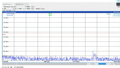
NTNV-n66-PC2-15-10-L-DFT-QPSK-Inner_1RB_Right-0.009-0.1 5-PASS
