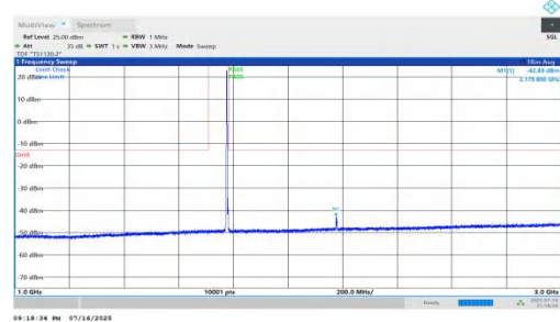
NTNV-n66-PC2-15-5-H-DFT-BPSK-Inner_1RB_Left-1000-3000-P ASS
