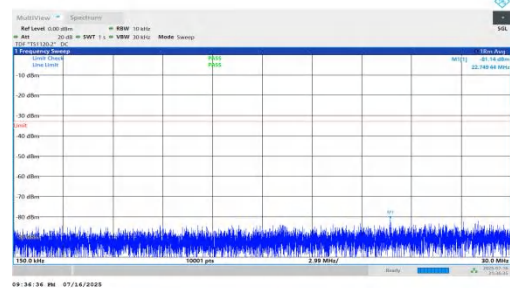
NTNV-n66-PC2-15-15-H-DFT-QPSK-Inner_1RB_Right-0.15-30-PA SS
