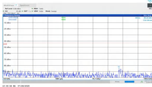
NTNV-n66-PC2-15-15-H-DFT-QPSK-Inner_1RB_Right-0.009-0.1 5-PASS
