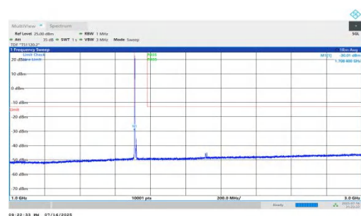
NTNV-n66-PC2-15-10-L-DFT-QPSK-Inner_1RB_Left-1000-3000-P ASS
