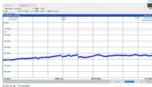
NTNV-n66-PC2-15-20-H-DFT-BPSK-Inner_1RB_Right-3000-120 00-PASS
