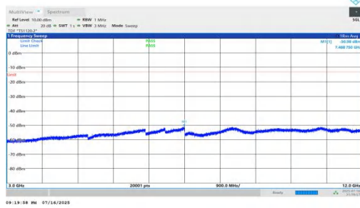
NTNV-n66-PC2-15-5-H-DFT-QPSK-Inner_1RB_Left-3000-12000-PASS
