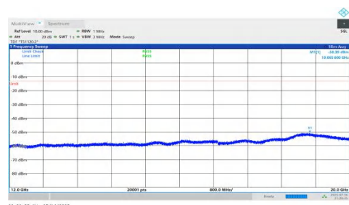
NTNV-n66-PC2-15-5-H-DFT-QPSK-Inner_1RB_Right-12000-20000-PASS
