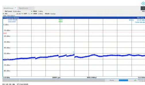
NTNV-n66-PC2-15-5-H-DFT-BPSK-Inner_1RB_Left-3000-12000- PASS
