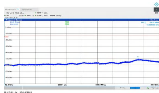
NTNV-n66-PC2-15-10-H-DFT-BPSK-Inner_1RB_Left-12000-20000-PASS
