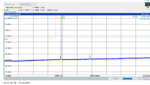
NTNV-n66-PC2-15-10-H-DFT-BPSK-Inner_1RB_Right-1000-3000- PASS
