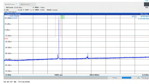
NTNV-n66-PC2-15-20-M-DFT-BPSK-Inner_1RB_Right-1000-3000-PASS
