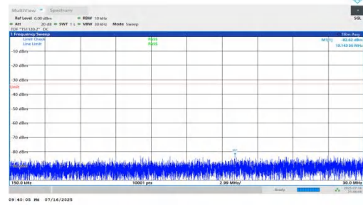
NTNV-n66-PC2-15-20-M-DFT-BPSK-Inner_1RB_Left-0.15-30-PASS
