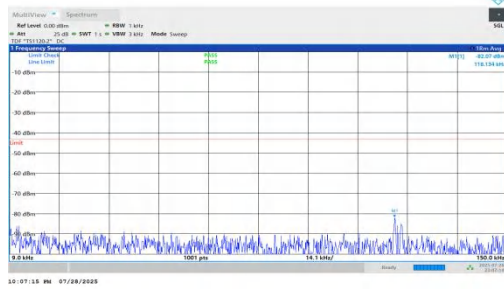
NTNV-n66-PC2-15-20-L-DFT-BPSK-Inner_1RB_Left-0.009-0.15-PASS
