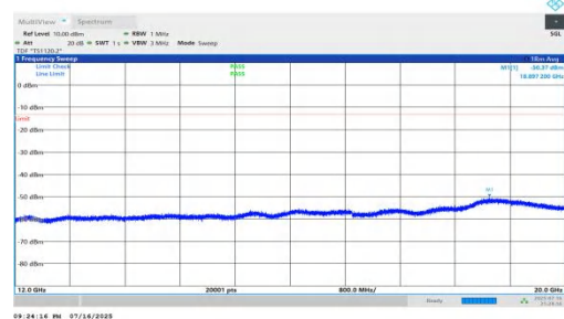
NTNV-n66-PC2-15-10-M-DFT-BPSK-Inner_1RB_Left-12000-20000-PASS
