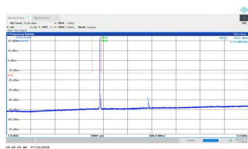
NTNV-n66-PC2-15-10-H-DFT-QPSK-Inner_1RB_Left-1000-3000- PASS
