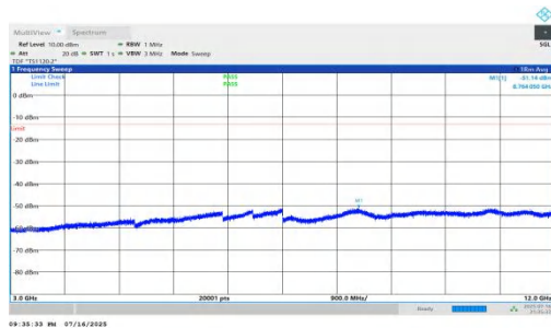
NTNV-n66-PC2-15-15-H-DFT-BPSK-Inner_1RB_Right-3000-12000-PASS
