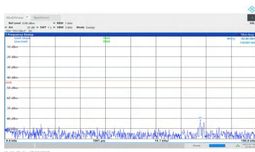
NTNV-n66-PC2-15-15-H-DFT-BPSK-Inner_1RB_Right-0.009-0.15-PASS
