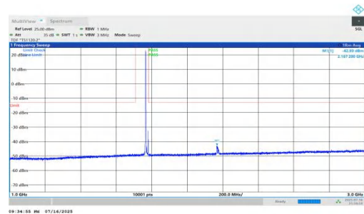
NTNV-n66-PC2-15-15-H-DFT-BPSK-Inner_1RB_Left-1000-3000-PASS
