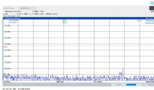
NTNV-n66-PC2-15-5-H-DFT-QPSK-Inner_1RB_Right-0.009-0.15-PASS
