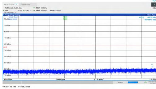
NTNV-n66-PC2-15-5-H-DFT-BPSK-Inner_1RB_Right-30-1000-P ASS
