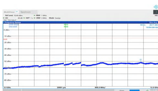
NTNV-n66-PC2-15-15-M-DFT-QPSK-Inner_1RB_Right-3000-12000-PASS
