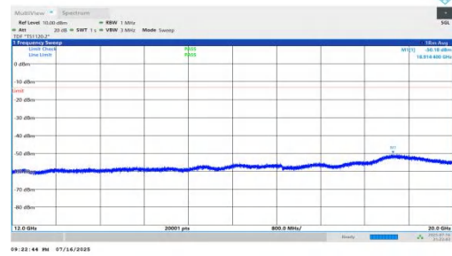
NTNV-n66-PC2-15-10-L-DFT-QPSK-Inner_1RB_Left-12000-20000 0-PASS
