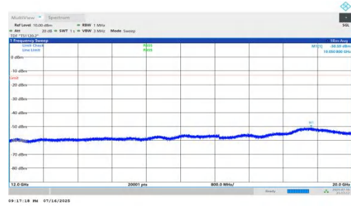
NTNV-n66-PC2-15-5-M-DFT-QPSK-Inner_1RB_Left-12000-20000 -PASS
