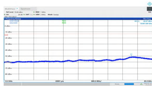
NTV-n66-PC2-15-15-L-DFT-QPSK-Inner_1RB_Right-12000-20000-PASS
