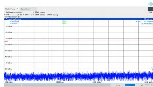
NTNV-n66-PC2-15-10-M-DFT-BPSK-Inner_1RB_Right-0.15-30-PASS
