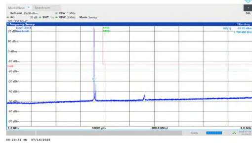
NTNV-n66-PC2-15-15-L-DFT-BPSK-Inner_1RB_Left-1000-3000-PASS ASS
