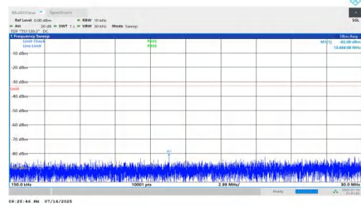
NTNV-n66-PC2-15-10-M-DFT-QPSK-Inner_1RB_Right-0.15-30-P ASS
