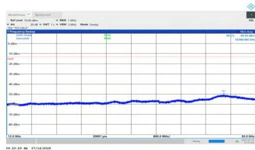
NTNV-n66-PC2-15-10-L-DFT-QPSK-Inner_1RB_Right-12000-20000 00-PASS
