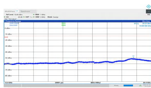
NTNV-n66-PC2-15-5-M-DFT-QPSK-Inner_1RB_Right-12000-2000 0-PASS
