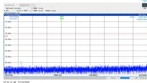
NTV-n66-PC2-15-15-L-DFT-QPSK-Inner_1RB_Right-0.15-30-PASS
