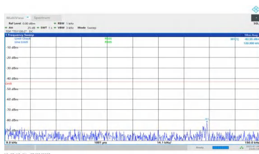
NTNV-n66-PC2-15-15-M-DFT-BPSK-Inner_1RB_Right-0.009-0.15-PASS
