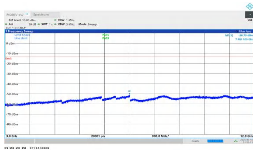
NTNV-n66-PC2-15-10-L-DFT-QPSK-Inner_1RB_Right-3000-12000 00-PASS
