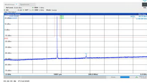
NTNV-n66-PC2-15-10-M-DFT-BPSK-Inner_1RB_Left-1000-3000-PASS
