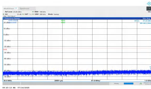
NTNV-n66-PC2-15-10-L-DFT-QPSK-Inner_1RB_Right-30-1000-P ASS
