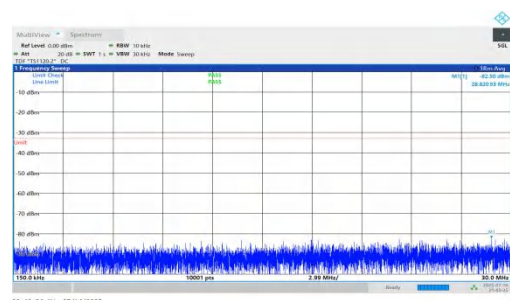
NTNV-n66-PC2-15-20-H-DFT-BPSK-Inner_1RB_Right-0.15-30-PASS
