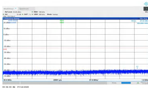
NTNV-n66-PC2-15-15-H-DFT-BPSK-Inner_1RB_Left-30-1000-PASS
