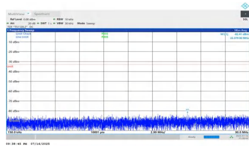
NTNV-n66-PC2-15-20-L-DFT-QPSK-Inner_1RB_Left-0.15-30-PAS S
