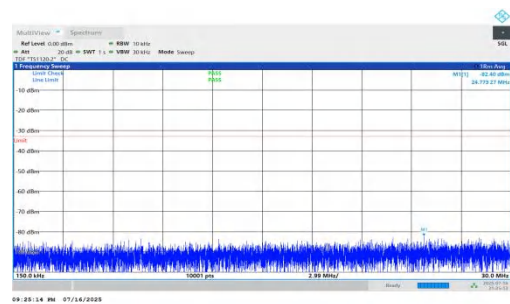
NTNV-n66-PC2-15-10-M-DFT-QPSK-Inner_1RB_Left-0.15-30-PASS
