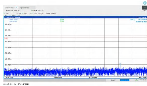
NTNV-n66-PC2-15-5-M-DFT-QPSK-Inner_1RB_Right-0.15-30-PA SS
