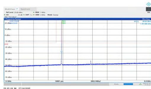
NTNV-n66-PC2-15-5-H-DFT-QPSK-Inner_1RB_Right-1000-3000-PASS
