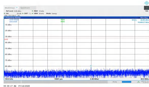
NTVN-n66-PC2-15-20-L-DFT-QPSK-Inner_1RB_Right-0.15-30-PA SS
