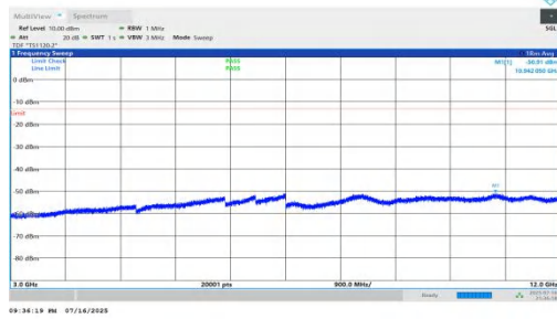
NTNV-n66-PC2-15-15-H-DFT-QPSK-Inner_1RB_Left-3000-1200 0-PASS
