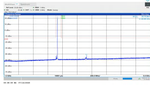
NTNV-n66-PC2-15-20-L-DFT-BPSK-Inner_1RB_Right-1000-3000-P PASS
