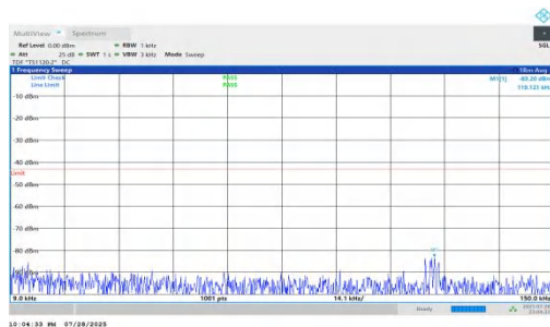
NTNV-n66-PC2-15-15-L-DFT-QPSK-Inner_1RB_Left-0.009-0.15- PASS
