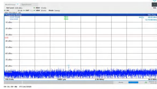
NTNV-n66-PC2-15-15-M-DFT-BPSK-Inner_1RB_Left-0.15-30-PASS
