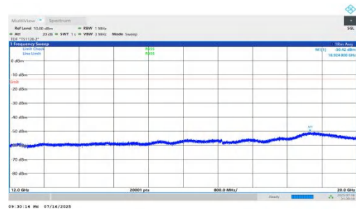
NTNV-n66-PC2-15-15-L-DFT-BPSK-Inner_1RB_Right-12000-200 00-PASS
