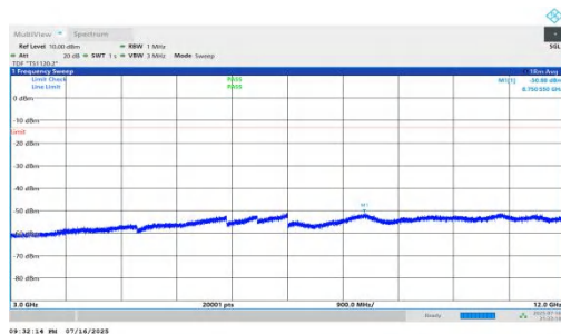
NTNV-n66-PC2-15-15-M-DFT-BPSK-Inner_1RB_Left-3000-12000-PASS
