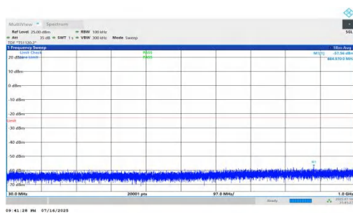
NTNV-n66-PC2-15-20-M-DFT-QPSK-Inner_1RB_Left-30-1000-PASS
