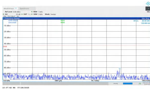
NTNV-n66-PC2-15-20-L-DFT-QPSK-Inner_1RB_Left-0.009-0.15- PASS
