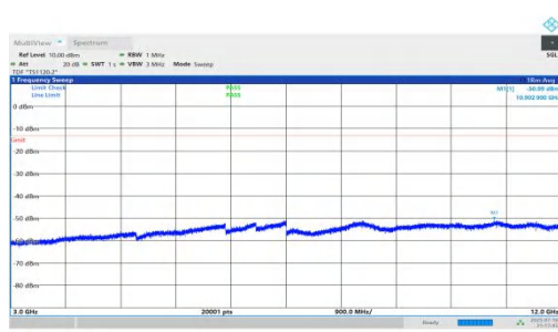
NTNV-n66-PC2-15-5-M-DFT-QPSK-Inner_1RB_Right-3000-1200 0-PASS
