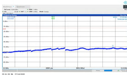
NTNV-n66-PC2-15-10-L-DFT-BPSK-Inner_1RB_Right-3000-1200 0-PASS
