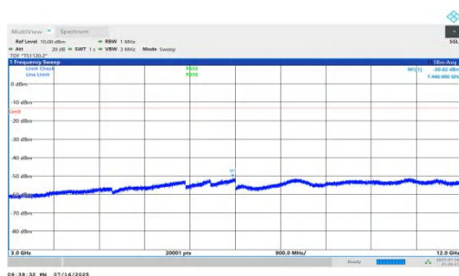
NTVN-n66-PC2-15-20-L-DFT-QPSK-Inner_1RB_Right-3000-12000- 00-PASS
