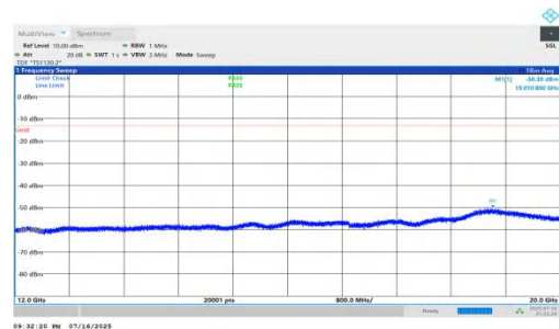
NTNV-n66-PC2-15-15-M-DFT-BPSK-Inner_1RB_Left-12000-20000-PASS
