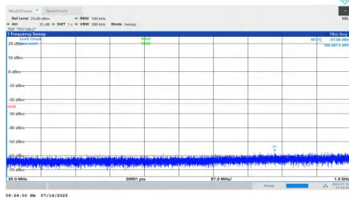
NTNV-n66-PC2-15-10-M-DFT-BPSK-Inner_1RB_Left-30-1000-PASS
