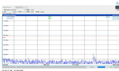
NTNV-n66-PC2-15-15-H-DFT-QPSK-Inner_1RB_Left-0.009-0.15-PASS
