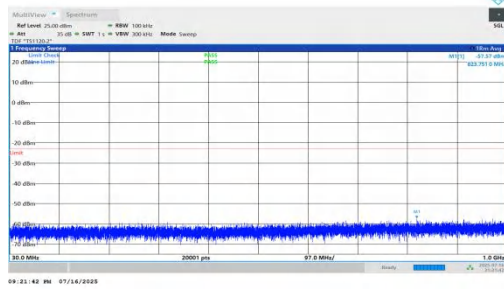
NTNV-n66-PC2-15-10-L-DFT-BPSK-Inner_1RB_Right-30-1000-P ASS
