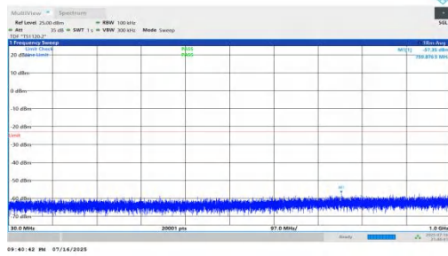
NTNV-n66-PC2-15-20-M-DFT-BPSK-Inner_1RB_Right-30-1000-PASS
