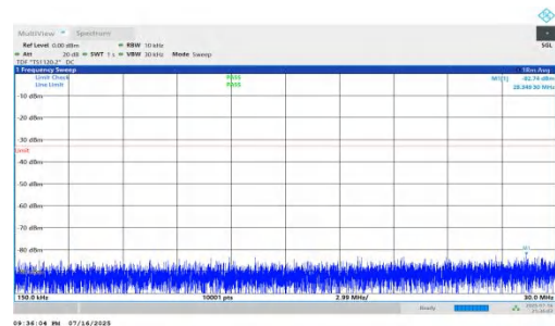
NTNV-n66-PC2-15-15-H-DFT-QPSK-Inner_1RB_Left-0.15-30-PASS
