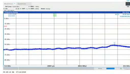
NTNV-n66-PC2-15-10-H-DFT-QPSK-Inner_1RB_Left-12000-2000 0-PASS
