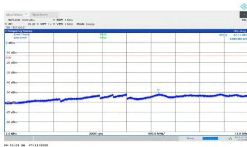
NTNV-n66-PC2-15-15-L-DFT-BPSK-Inner_1RB_Right-3000-1200 0-PASS
