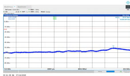
NTNV-n66-PC2-15-10-L-DFT-BPSK-Inner_1RB_Right-12000-200 00-PASS
