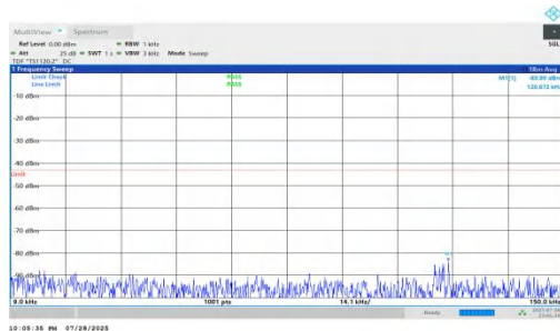
NTNV-n66-PC2-15-15-M-DFT-QPSK-Inner_1RB_Left-0.009-0.15-PASS
