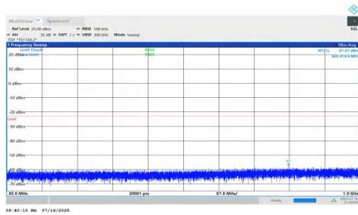
NTNV-n66-PC2-15-20-M-DFT-BPSK-Inner_1RB_Left-30-1000-PASS
