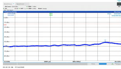
NTNV-n66-PC2-15-5-H-DFT-QPSK-Inner_1RB_Left-12000-20000-PASS
