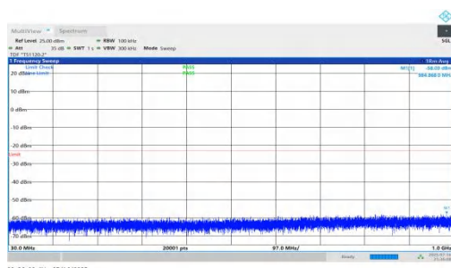
NTNV-n66-PC2-15-15-H-DFT-QPSK-Inner_1RB_Left-30-1000-PASS
