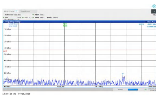
NTNV-n66-PC2-15-20-M-DFT-BPSK-Inner_1RB_Right-0.009-0.15-PASS
