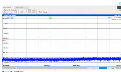
NTNV-n66-PC2-15-5-M-DFT-QPSK-Inner_1RB_Right-30-1000-P ASS
