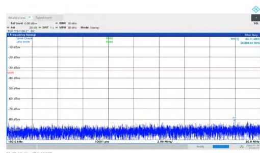
NTNV-n66-PC2-15-10-H-DFT-BPSK-Inner_1RB_Right-0.15-30-PASS
