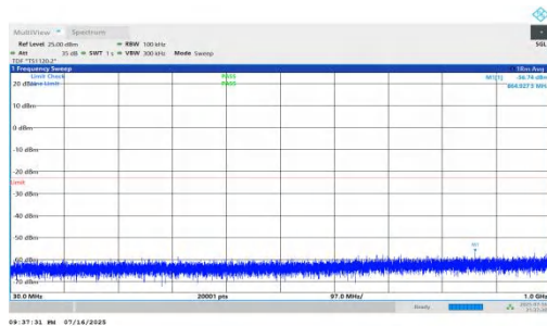
NTNV-n66-PC2-15-20-L-DFT-BPSK-Inner_1RB_Left-30-1000-PASS
