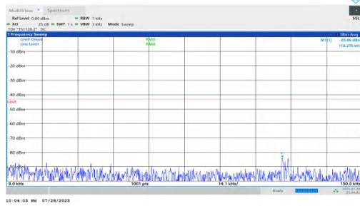
NTNV-n66-PC2-15-15-L-DFT-BPSK-Inner_1RB_Left-0.009-0.15- PASS
