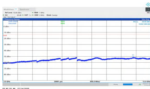
NTNV-n66-PC2-15-20-M-DFT-QPSK-Inner_1RB_Right-3000-120 00-PASS
