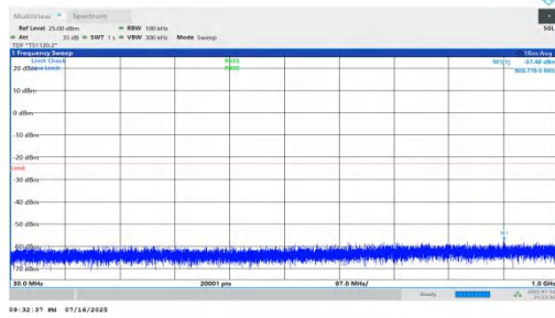
NTNV-n66-PC2-15-15-M-DFT-BPSK-Inner_1RB_Right-30-1000-PASS
