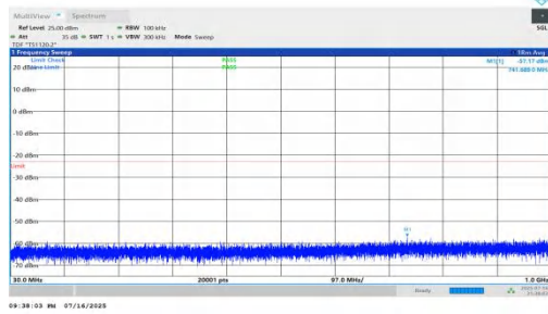
NTNV-n66-PC2-15-20-L-DFT-BPSK-Inner_1RB_Right-30-1000-P ASS
