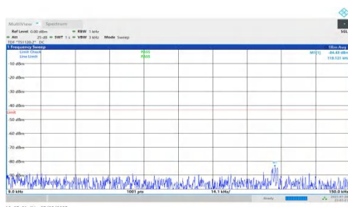
NTNV-n66-PC2-15-20-L-DFT-BPSK-Inner_1RB_Right-0.009-0.15-PASS
