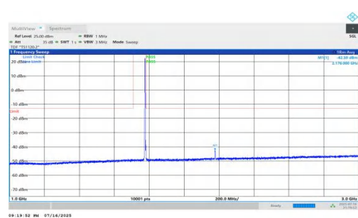
NTNV-n66-PC2-15-5-H-DFT-QPSK-Inner_1RB_Left-1000-3000-P ASS
