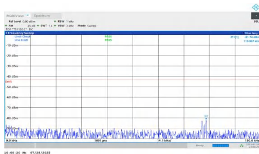
NTNV-n66-PC2-15-5-H-DFT-QPSK-Inner_1RB_Left-0.009-0.15-P ASS
