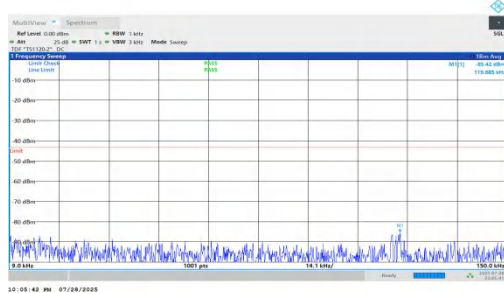
NTNV-n66-PC2-15-15-M-DFT-QPSK-Inner_1RB_Right-0.009-0.1 5-PASS
