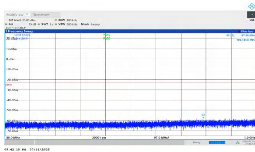
NTNV-n66-PC2-15-20-M-DFT-QPSK-Inner_1RB_Right-30-1000- PASS
