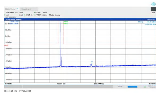
NTNV-n66-PC2-15-20-M-DFT-BPSK-Inner_1RB_Left-1000-3000-PASS
