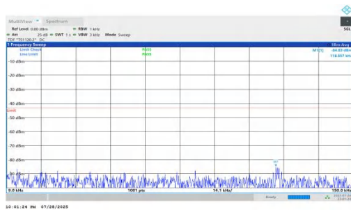
NTNV-n66-PC2-15-10-L-DFT-QPSK-Inner_1RB_Left-0.009-0.15- PASS
