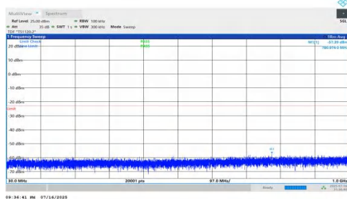
NTNV-n66-PC2-15-15-H-DFT-QPSK-Inner_1RB_Right-30-1000- PASS
