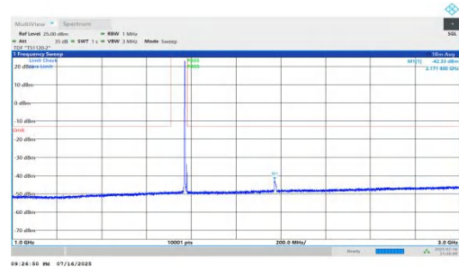
NTNV-n66-PC2-15-10-H-DFT-BPSK-Inner_1RB_Left-1000-3000-PASS
