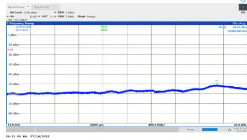
NTV-n66-PC2-15-15-L-DFT-QPSK-Inner_1RB_Left-12000-20000-PASS
