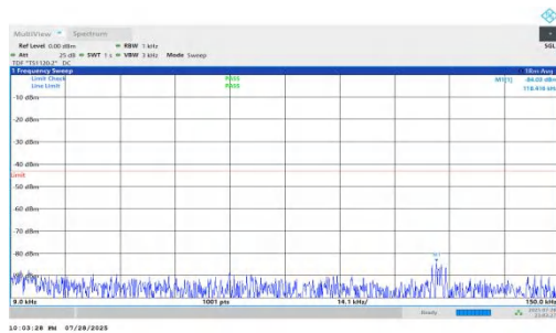
NTNV-n66-PC2-15-10-H-DFT-QPSK-Inner_1RB_Left-0.009-0.15- PASS
