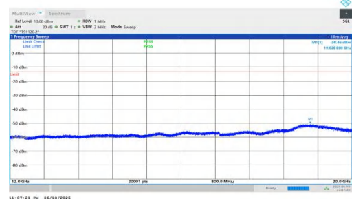
NTNV-n66-PC3-15-40-H-DFT-BPSK-Inner_1RB_Left-12000-20000-PASS
