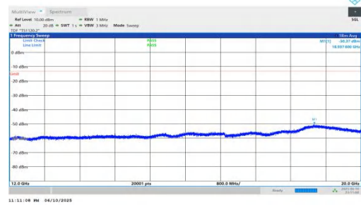
NTNV-n66-PC3-15-45-L-DFT-QPSK-Inner_1RB_Left-12000-2000 0-PASS
