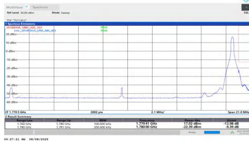
NTNV-n66-PC2-15-20-H-DFT-QPSK-Edge_1RB_Right-PASS
