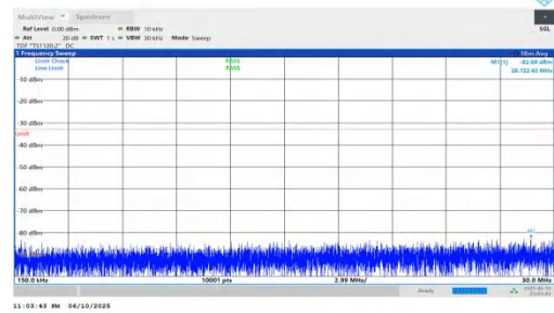
NTNV-n66-PC3-15-40-L-DFT-QPSK-Inner_1RB_Right-0.15-30-PA SS
