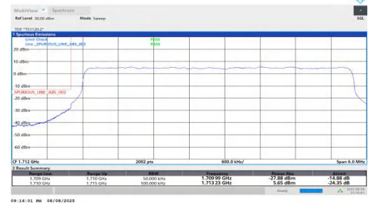
NTNV-n66-PC2-15-5-L-DFT-QPSK-Outer_Full-PASS
