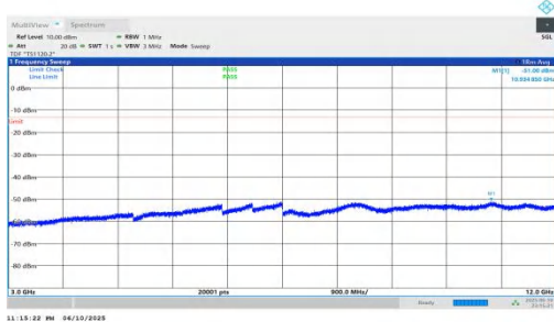
NTNV-n66-PC3-15-45-H-DFT-BPSK-Inner_1RB_Right-3000-120 00-PASS
