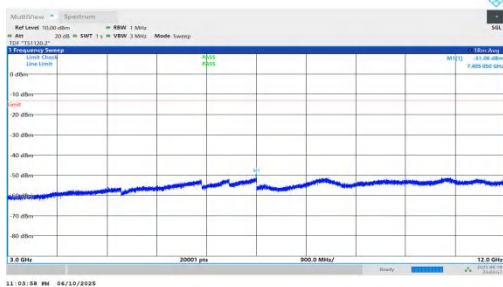
NTNV-n66-PC3-15-40-L-DFT-QPSK-Inner_1RB_Right-3000-120 00-PASS
