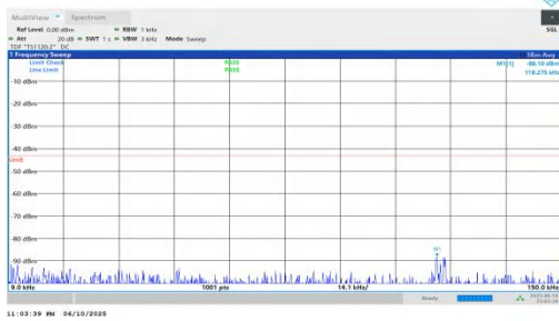
NTNV-n66-PC3-15-40-L-DFT-QPSK-Inner_1RB_Right-0.009-0.1 5-PASS
