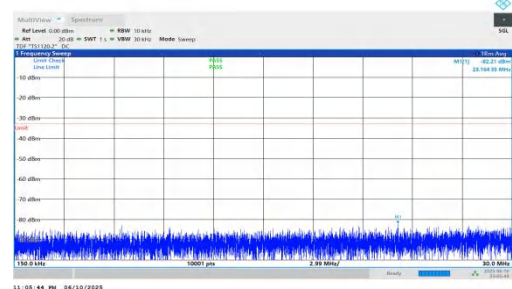
NTNV-n66-PC3-15-40-M-DFT-QPSK-Inner_1RB_Left-0.15-30-PASS
