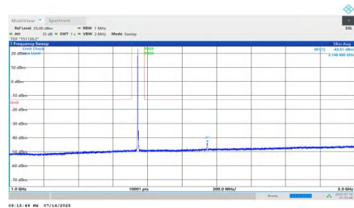
NTNV-n66-PC2-15-5-M-DFT-BPSK-Inner_1RB_Left-1000-3000-P ASS
