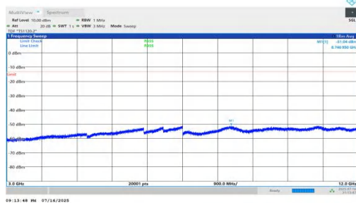
NTNV-n66-PC2-15-5-L-DFT-BPSK-Inner_1RB_Right-3000-12000 -PASS
