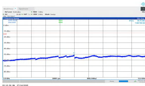
NTNV-n66-PC2-15-5-M-DFT-BPSK-Inner_1RB_Left-3000-12000-PASS
