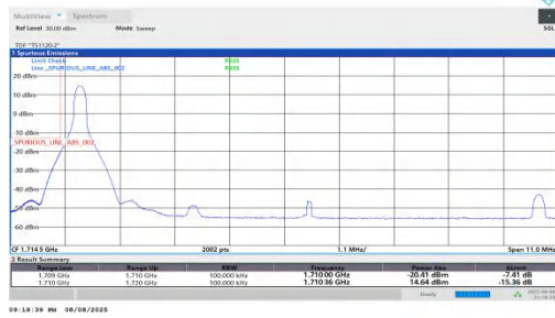
NTNV-n66-PC2-15-10-L-DFT-BPSK-Edge_1RB_Left-PASS
