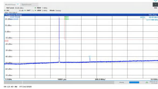
NTNV-n66-PC2-15-5-L-DFT-BPSK-Inner_1RB_Right-1000-3000-P ASS
