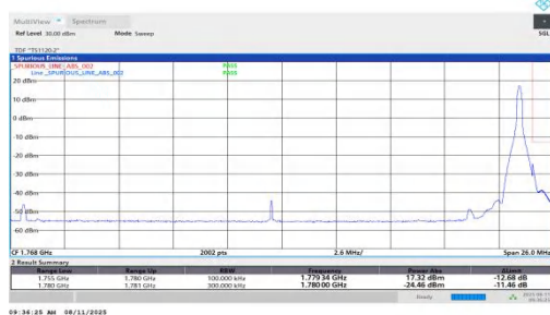
NTNV-n66-PC2-15-25-H-DFT-BPSK-Edge_1RB_Right-PASS
