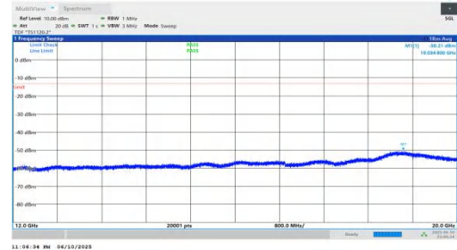
NTNV-n66-PC3-15-40-M-DFT-QPSK-Inner_1RB_Right-12000-20000- 00-PASS
