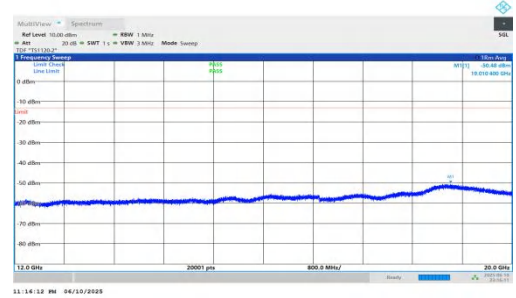
NTNV-n66-PC3-15-45-H-DFT-QPSK-Inner_1RB_Left-12000-2000 0-PASS
