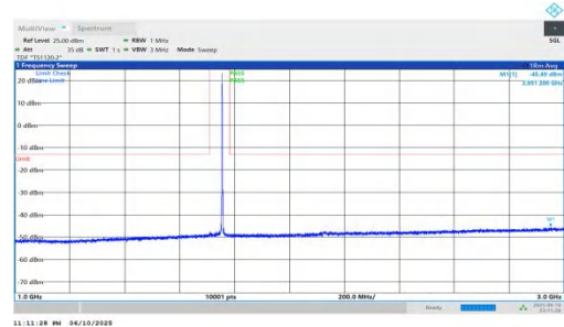
NTNV-n66-PC3-15-45-L-DFT-QPSK-Inner_1RB_Right-1000-3000-P PASS
