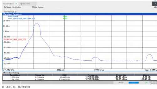
NTNV-n66-PC2-15-5-L-DFT-BPSK-Edge_1RB_Left-PASS
