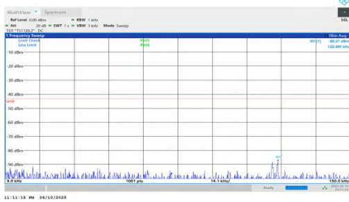
NTNV-n66-PC3-15-45-L-DFT-QPSK-Inner_1RB_Right-0.009-0.1 5-PASS
