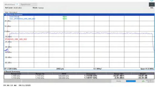
NTNV-n66-PC2-15-40-L-DFT-BPSK-Outer_Full-PASS
