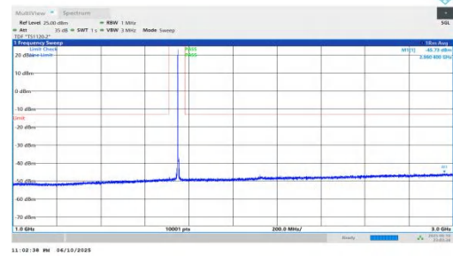
NTNV-n66-PC3-15-40-L-DFT-BPSK-Inner_1RB_Right-1000-3000-P PASS
