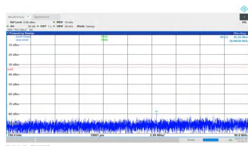
NTNV-n66-PC2-15-5-M-DFT-BPSK-Inner_1RB_Right-0.15-30-PASS SS
