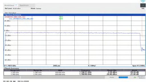
NTNV-n66-PC2-15-40-H-DFT-QPSK-Outer_Full-PASS
