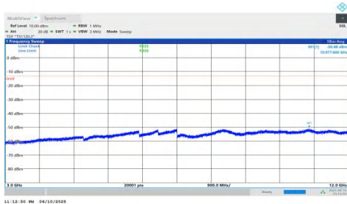
NTNV-n66-PC3-15-45-M-DFT-BPSK-Inner_1RB_Right-3000-12000-PASS
