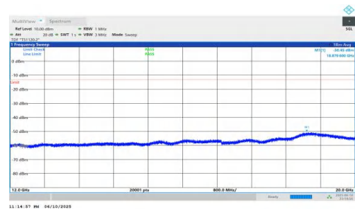
NTNV-n66-PC3-15-45-H-DFT-BPSK-Inner_1RB_Left-12000-20000-PASS
