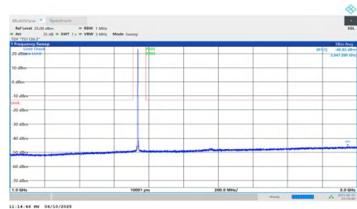
NTNV-n66-PC3-15-45-H-DFT-BPSK-Inner_1RB_Left-1000-3000-PASS
