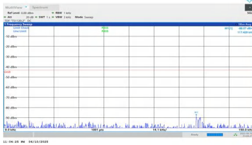
NTNV-n66-PC3-15-40-M-DFT-BPSK-Inner_1RB_Left-0.009-0.15-PASS
