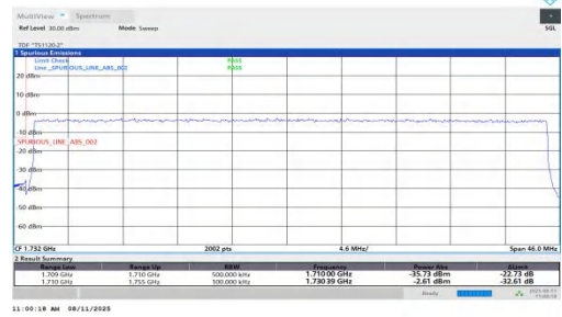
NTNV-n66-PC2-15-45-L-DFT-BPSK-Outer_Full-PASS
