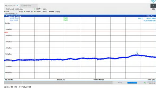
NTNV-n66-PC3-15-45-L-DFT-QPSK-Inner_1RB_Right-12000-2000 00-PASS
