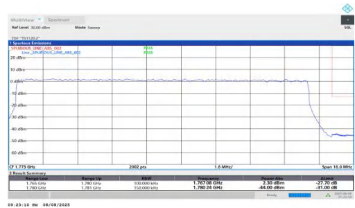
NTNV-n66-PC2-15-15-H-DFT-BPSK-Outer_Full-PASS
