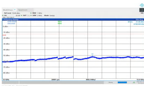
NTNV-n66-PC3-15-45-H-DFT-QPSK-Inner_1RB_Right-3000-120 00-PASS
