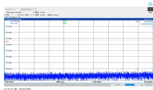
NTNV-n66-PC3-15-40-L-DFT-QPSK-Inner_1RB_Left-0.15-30-PAS S
