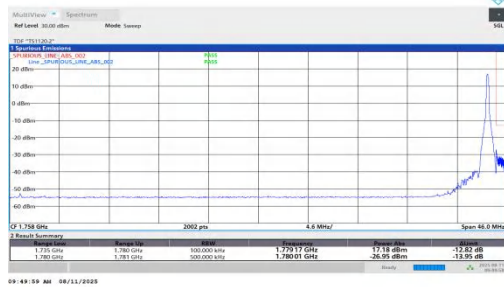
NTNV-n66-PC2-15-45-H-DFT-QPSK-Edge_1RB_Right-PASS
