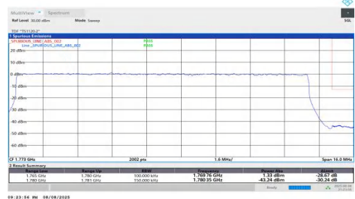
NTNV-n66-PC2-15-15-H-DFT-QPSK-Outer_Full-PASS
