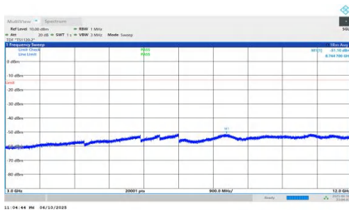
NTNV-n66-PC3-15-40-M-DFT-BPSK-Inner_1RB_Left-3000-12000-PASS
