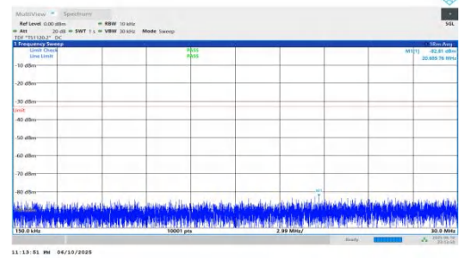
NTNV-n66-PC3-15-45-M-DFT-QPSK-Inner_1RB_Right-0.15-30-P ASS
