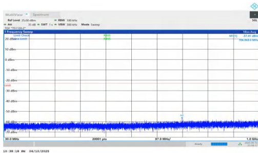
NTNV-n66-PC3-15-20-H-DFT-QPSK-Inner_1RB_Right-30-1000- PASS
