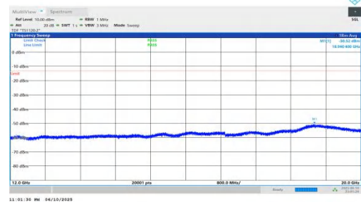
NTNV-n66-PC3-15-35-H-DFT-QPSK-Inner_1RB_Right-12000-200 00-PASS
