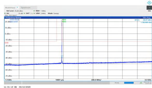
NTNV-n66-PC3-15-35-H-DFT-QPSK-Inner_1RB_Right-1000-3000 -PASS
