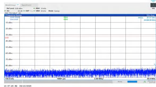
NTNV-n66-PC3-15-35-M-DFT-BPSK-Inner_1RB_Right-0.15-30-PASS
