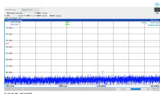
NTNV-n66-PC3-15-30-H-DFT-QPSK-Inner_1RB_Left-0.15-30-PASS
