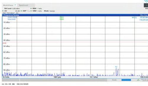
NTNV-n66-PC3-15-35-H-DFT-QPSK-Inner_1RB_Right-0.009-0.1 5-PASS
