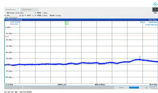
NTNV-n66-PC3-15-30-H-DFT-BPSK-Inner_1RB_Left-12000-20000-PASS
