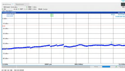
NTNV-n66-PC3-15-25-M-DFT-BPSK-Inner_1RB_Right-3000-12000-PASS
