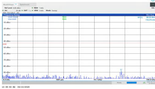
NTNV-n66-PC3-15-25-L-DFT-BPSK-Inner_1RB_Left-0.009-0.15-PASS
