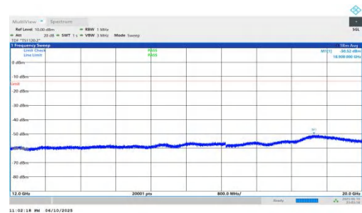
NTNV-n66-PC3-15-40-L-DFT-BPSK-Inner_1RB_Left-12000-20000-PASS
