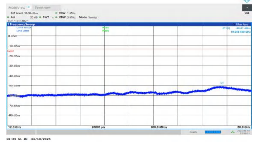
NTNV-n66-PC3-15-25-L-DFT-BPSK-Inner_1RB_Right-12000-200 00-PASS
