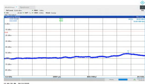
NTNV-n66-PC3-15-30-M-DFT-BPSK-Inner_1RB_Left-12000-20000-PASS
