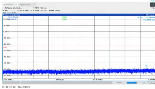
NTNV-n66-PC3-15-35-L-DFT-BPSK-Inner_1RB_Right-30-1000-P ASS
