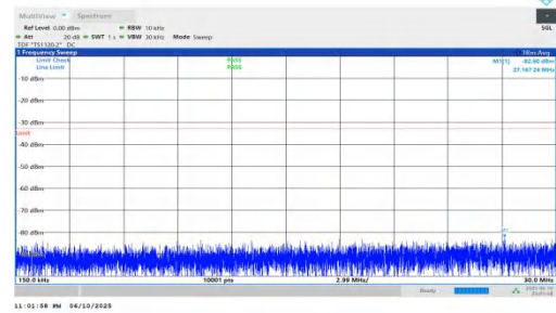
NTNV-n66-PC3-15-40-L-DFT-BPSK-Inner_1RB_Left-0.15-30-PAS
