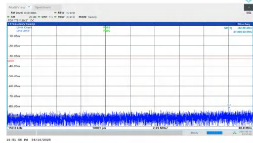
NTNV-n66-PC3-15-30-H-DFT-BPSK-Inner_1RB_Left-0.15-30-PAS
