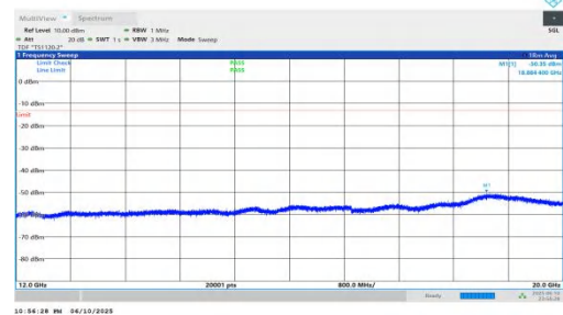
NTNV-n66-PC3-15-35-L-DFT-QPSK-Inner_1RB_Right-12000-20000 00-PASS
