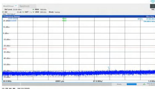
NTNV-n66-PC3-15-35-M-DFT-QPSK-Inner_1RB_Right-30-1000-PASS
