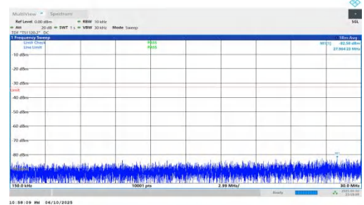
NTNV-n66-PC3-15-35-M-DFT-QPSK-Inner_1RB_Left-0.15-30-PASS
