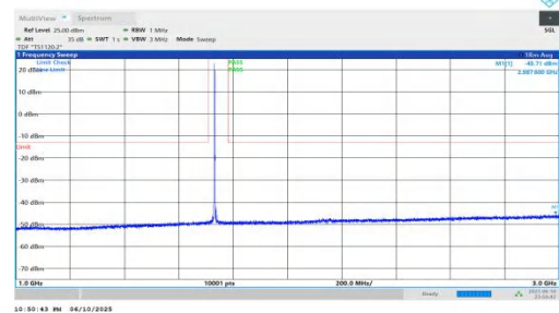
NTNV-n66-PC3-15-30-M-DFT-QPSK-Inner_1RB_Left-1000-3000-PASS
