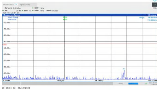
NTNV-n66-PC3-15-30-M-DFT-BPSK-Inner_1RB_Left-0.009-0.15-PASS
