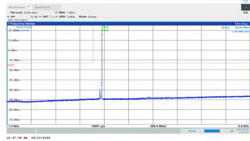
NTNV-n66-PC3-15-20-H-DFT-BPSK-Inner_1RB_Right-1000-3000- PASS
