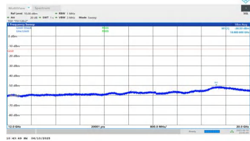
NTNV-n66-PC3-15-25-M-DFT-QPSK-Inner_1RB_Right-12000-20000- 00-PASS
