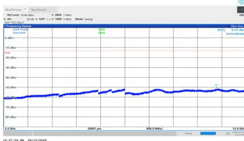
NTNV-n66-PC3-15-35-M-DFT-BPSK-Inner_1RB_Left-3000-12000-PASS
