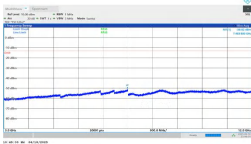
NTNV-n66-PC3-15-25-H-DFT-BPSK-Inner_1RB_Right-3000-120 00-PASS
