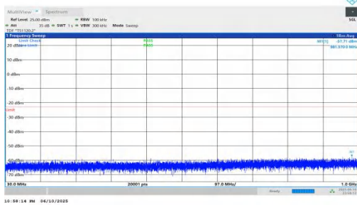
NTNV-n66-PC3-15-35-M-DFT-QPSK-Inner_1RB_Left-30-1000-PASS
