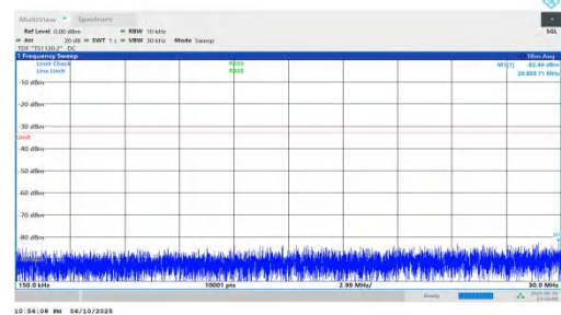
NTNV-n66-PC3-15-35-L-DFT-QPSK-Inner_1RB_Right-0.15-30-PA SS
