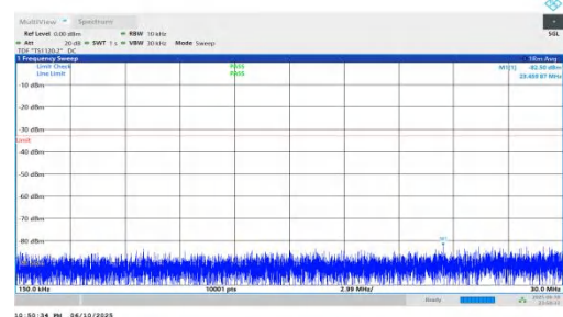
NTNV-n66-PC3-15-30-M-DFT-QPSK-Inner_1RB_Left-0.15-30-PASS
