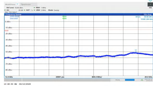
NTNV-n66-PC3-15-25-H-DFT-QPSK-Inner_1RB_Left-12000-2000 0-PASS
