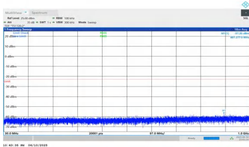
NTNV-n66-PC3-15-25-M-DFT-QPSK-Inner_1RB_Right-30-1000- PASS
