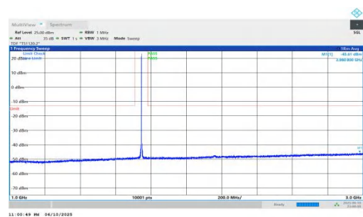
NTNV-n66-PC3-15-35-H-DFT-QPSK-Inner_1RB_Left-1000-3000- PASS
