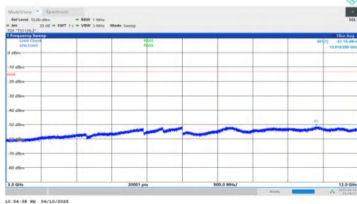
NTNV-n66-PC3-15-35-L-DFT-BPSK-Inner_1RB_Left-3000-12000-PASS
