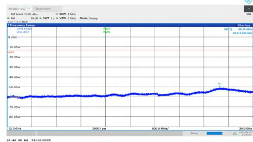
NTNV-n66-PC3-15-25-H-DFT-BPSK-Inner_1RB_Right-12000-200 00-PASS
