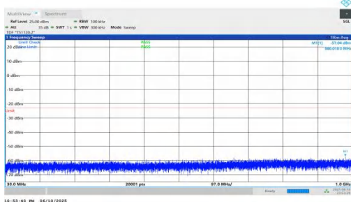
NTNV-n66-PC3-15-30-H-DFT-QPSK-Inner_1RB_Right-30-1000- PASS
