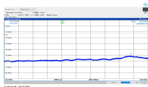
NTNV-n66-PC3-15-25-H-DFT-BPSK-Inner_1RB_Left-12000-20000-PASS
