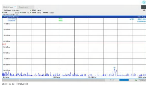
NTNV-n66-PC3-15-25-L-DFT-QPSK-Inner_1RB_Right-0.009-0.1 5-PASS
