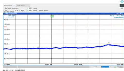
NTNV-n66-PC3-15-35-H-DFT-BPSK-Inner_1RB_Right-12000-200 00-PASS
