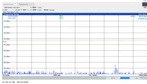
NTNV-n66-PC3-15-35-L-DFT-BPSK-Inner_1RB_Left-0.009-0.15-PASS
