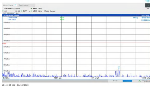
NTNV-n66-PC3-15-25-M-DFT-QPSK-Inner_1RB_Right-0.009-0.1 5-PASS
