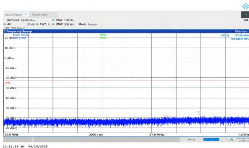
NTNV-n66-PC3-15-25-M-DFT-BPSK-Inner_1RB_Left-30-1000-PASS
