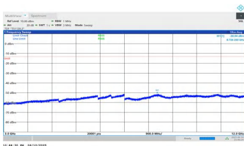
NTNV-n66-PC3-15-25-H-DFT-BPSK-Inner_1RB_Left-3000-12000-PASS
