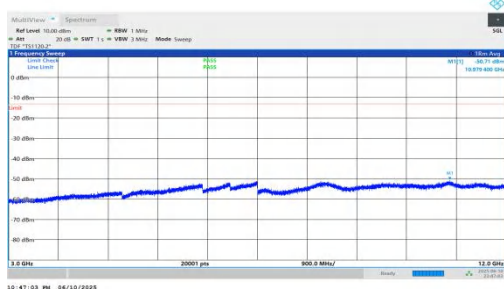
NTNV-n66-PC3-15-30-L-DFT-BPSK-Inner_1RB_Left-3000-12000-PASS
