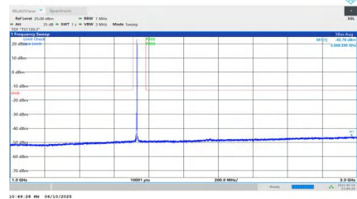
NTNV-n66-PC3-15-30-M-DFT-BPSK-Inner_1RB_Left-1000-3000-PASS
