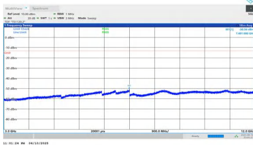
NTNV-n66-PC3-15-35-H-DFT-QPSK-Inner_1RB_Right-3000-120 00-PASS
