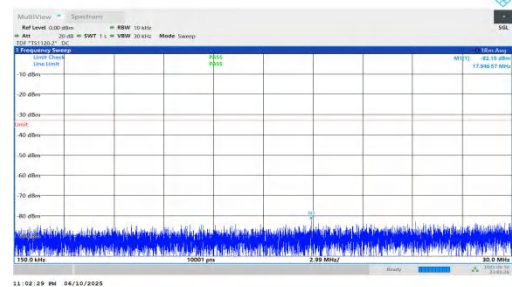
NTNV-n66-PC3-15-40-L-DFT-BPSK-Inner_1RB_Right-0.15-30-PASS
