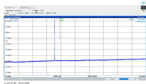
NTNV-n66-PC3-15-40-L-DFT-BPSK-Inner_1RB_Left-1000-3000-PASS
