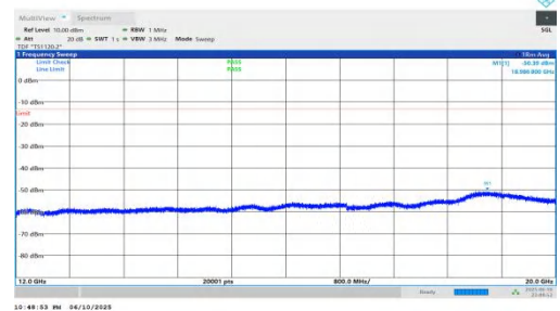
NTNV-n66-PC3-15-30-L-DFT-QPSK-Inner_1RB_Right-12000-20000 00-PASS
