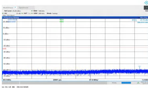
NTNV-n66-PC3-15-35-H-DFT-QPSK-Inner_1RB_Right-30-1000- PASS
