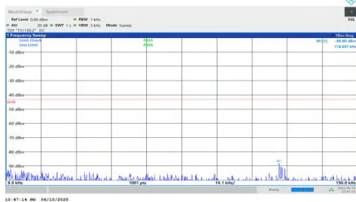
NTNV-n66-PC3-15-30-L-DFT-BPSK-Inner_1RB_Right-0.009-0.15-PASS
