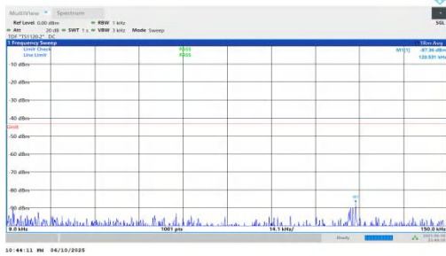
NTNV-n66-PC3-15-25-H-DFT-BPSK-Inner_1RB_Left-0.009-0.15-PASS
