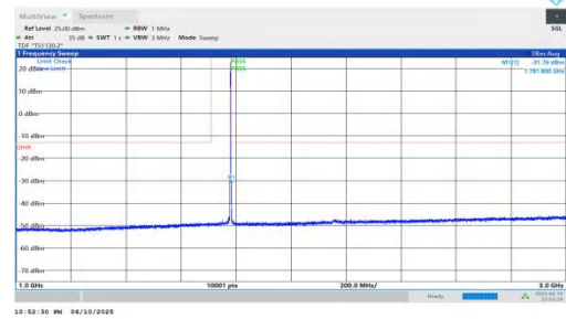
NTNV-n66-PC3-15-30-H-DFT-BPSK-Inner_1RB_Right-1000-3000-PASS
