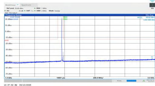
NTNV-n66-PC3-15-20-H-DFT-QPSK-Inner_1RB_Left-1000-3000- PASS
