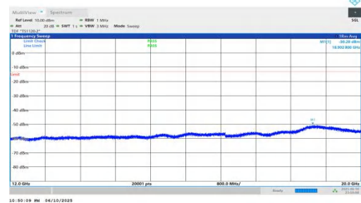
NTNV-n66-PC3-15-30-M-DFT-BPSK-Inner_1RB_Right-12000-20000-PASS
