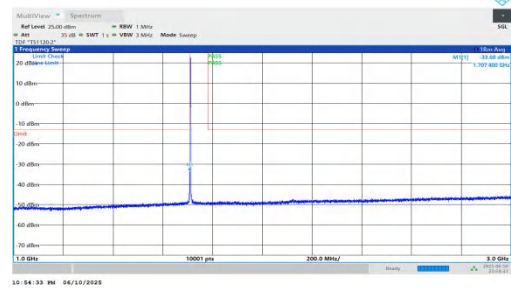
NTNV-n66-PC3-15-35-L-DFT-BPSK-Inner_1RB_Left-1000-3000-PASS
