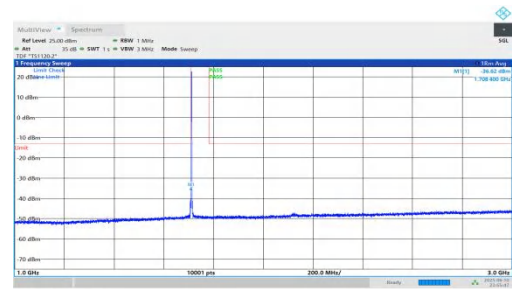
NTNV-n66-PC3-15-35-L-DFT-QPSK-Inner_1RB_Left-1000-3000-P ASS
