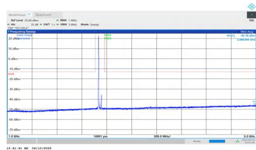
NTNV-n66-PC3-15-25-M-DFT-BPSK-Inner_1RB_Left-1000-3000-PASS
