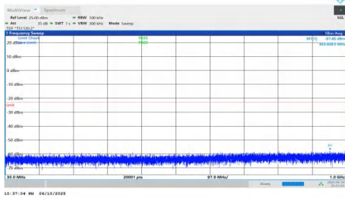
NTNV-n66-PC3-15-20-H-DFT-BPSK-Inner_1RB_Right-30-1000-P ASS
