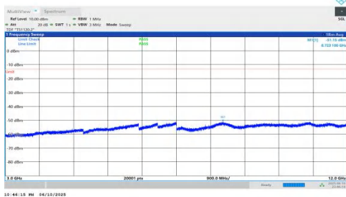
NTNV-n66-PC3-15-25-H-DFT-QPSK-Inner_1RB_Right-3000-120 00-PASS
