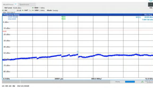
NTNV-n66-PC3-15-35-M-DFT-QPSK-Inner_1RB_Left-3000-1200 0-PASS
