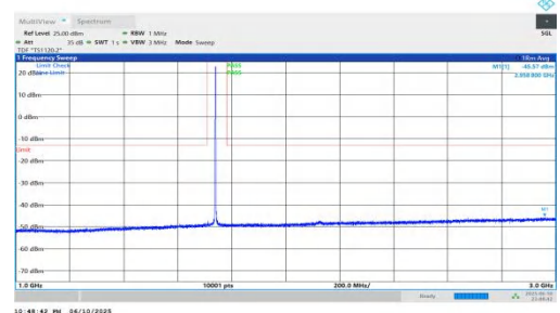
NTNV-n66-PC3-15-30-L-DFT-QPSK-Inner_1RB_Right-1000-3000-P PASS
