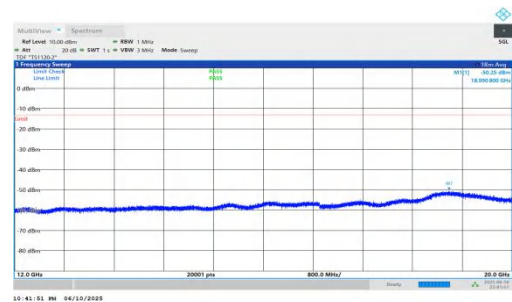
NTNV-n66-PC3-15-25-M-DFT-BPSK-Inner_1RB_Left-12000-20000-PASS
