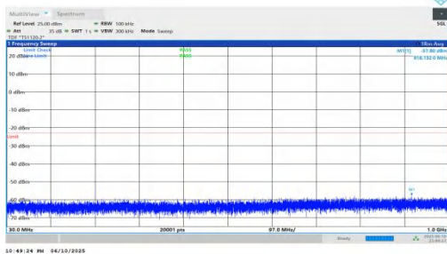
NTNV-n66-PC3-15-30-M-DFT-BPSK-Inner_1RB_Left-30-1000-PASS
