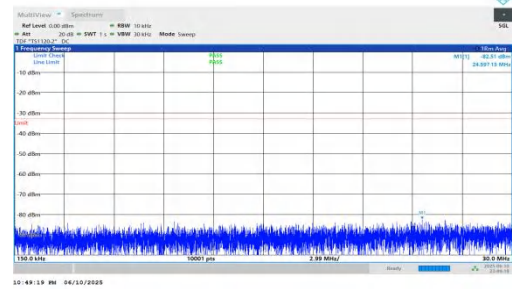
NTNV-n66-PC3-15-30-M-DFT-BPSK-Inner_1RB_Left-0.15-30-PASS
