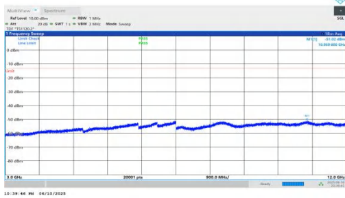
NTNV-n66-PC3-15-25-L-DFT-BPSK-Inner_1RB_Right-3000-1200 0-PASS
