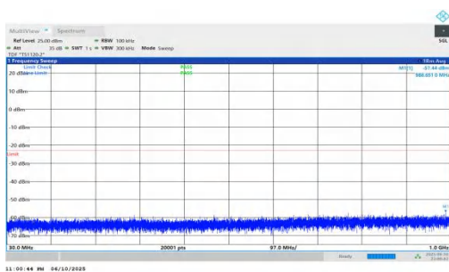
NTNV-n66-PC3-15-35-H-DFT-QPSK-Inner_1RB_Left-30-1000-P ASS
