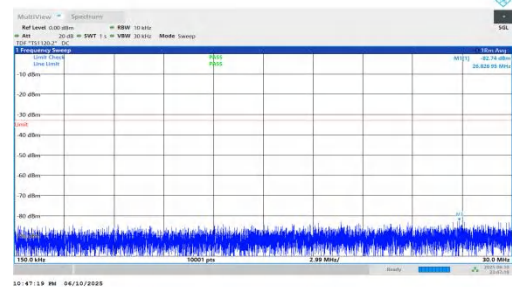
NTNV-n66-PC3-15-30-L-DFT-BPSK-Inner_1RB_Right-0.15-30-PASS
