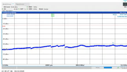
NTNV-n66-PC3-15-20-H-DFT-QPSK-Inner_1RB_Right-3000-120 00-PASS
