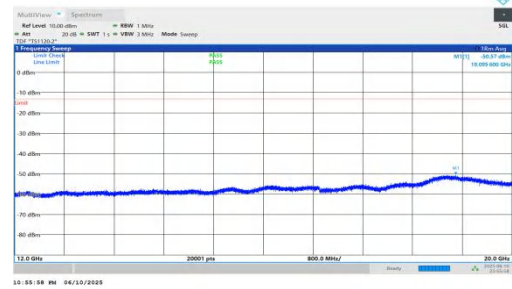
NTNV-n66-PC3-15-35-L-DFT-QPSK-Inner_1RB_Left-12000-2000 0-PASS
