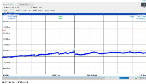
NTNV-n66-PC3-15-35-M-DFT-BPSK-Inner_1RB_Right-3000-12000-PASS
