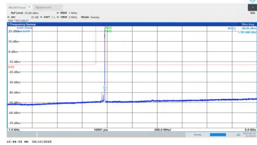
NTNV-n66-PC3-15-25-H-DFT-BPSK-Inner_1RB_Right-1000-3000- PASS
