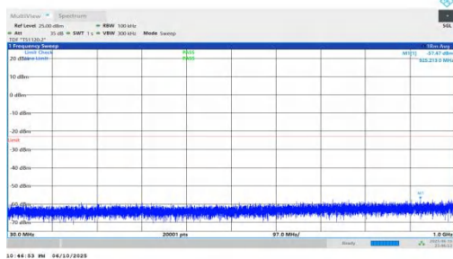
NTNV-n66-PC3-15-30-L-DFT-BPSK-Inner_1RB_Left-30-1000-PASS
