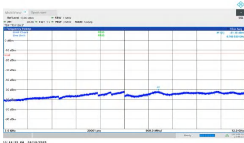
NTNV-n66-PC3-15-30-M-DFT-BPSK-Inner_1RB_Left-3000-12000-PASS
