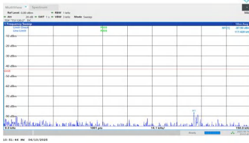
NTNV-n66-PC3-15-30-H-DFT-BPSK-Inner_1RB_Left-0.009-0.15-PASS
