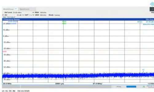
NTNV-n66-PC3-15-30-H-DFT-BPSK-Inner_1RB_Left-30-1000-PASS
