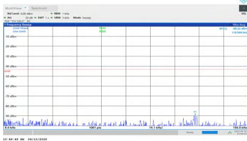
NTNV-n66-PC3-15-30-M-DFT-BPSK-Inner_1RB_Right-0.009-0.15-PASS
