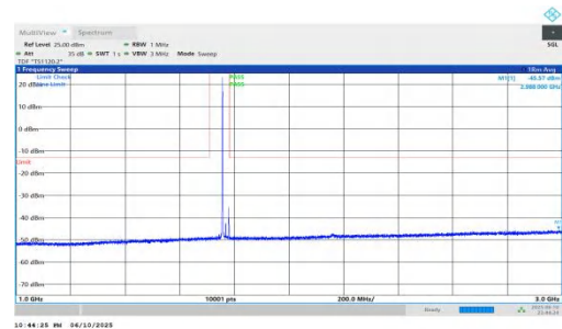
NTNV-n66-PC3-15-25-H-DFT-BPSK-Inner_1RB_Left-1000-3000-PASS
