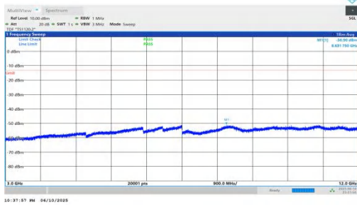
NTNV-n66-PC3-15-20-H-DFT-QPSK-Inner_1RB_Left-3000-1200 0-PASS
