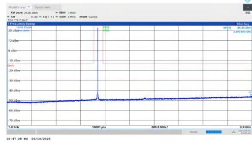
NTNV-n66-PC3-15-30-L-DFT-BPSK-Inner_1RB_Right-1000-3000-P PASS
