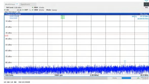
NTNV-n66-PC3-15-25-H-DFT-BPSK-Inner_1RB_Left-0.15-30-PAS
