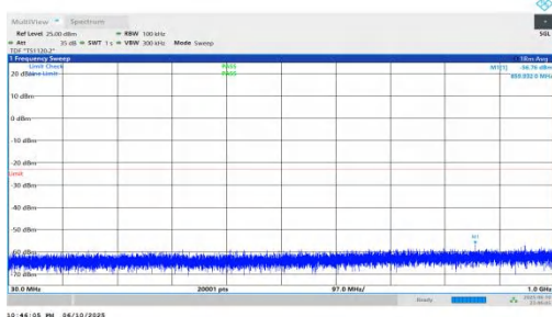
NTNV-n66-PC3-15-25-H-DFT-QPSK-Inner_1RB_Right-30-1000- PASS
