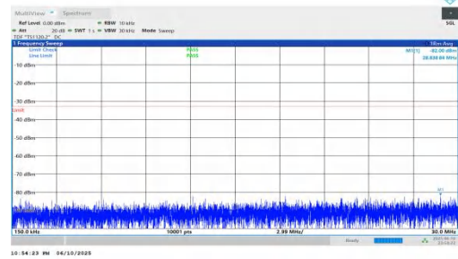
NTNV-n66-PC3-15-35-L-DFT-BPSK-Inner_1RB_Left-0.15-30-PAS
