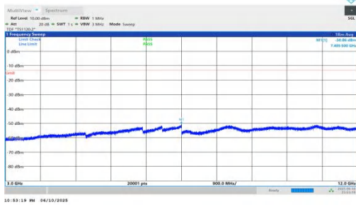
NTNV-n66-PC3-15-30-H-DFT-QPSK-Inner_1RB_Left-3000-1200 0-PASS
