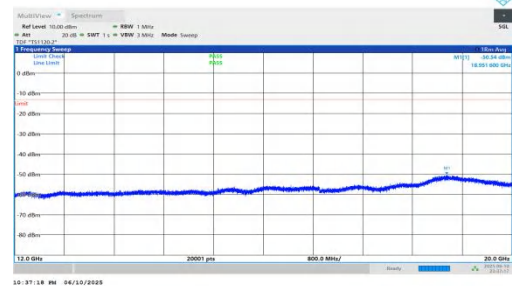
NTNV-n66-PC3-15-20-H-DFT-BPSK-Inner_1RB_Right-12000-200 00-PASS
