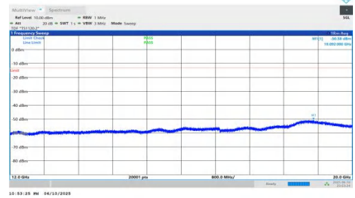
NTNV-n66-PC3-15-30-H-DFT-QPSK-Inner_1RB_Left-12000-2000 0-PASS
