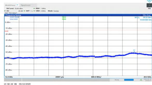
NTNV-n66-PC3-15-25-M-DFT-BPSK-Inner_1RB_Right-12000-20000-PASS
