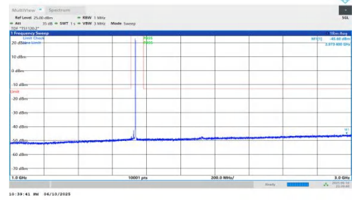
NTNV-n66-PC3-15-25-L-DFT-BPSK-Inner_1RB_Right-1000-3000-P PASS
