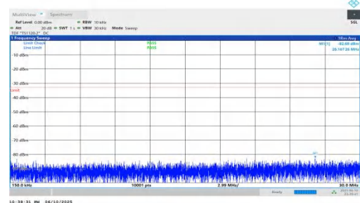
NTNV-n66-PC3-15-25-L-DFT-BPSK-Inner_1RB_Right-0.15-30-PASS
