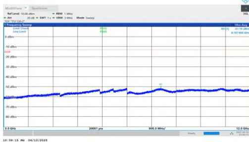
NTNV-n66-PC3-15-25-L-DFT-BPSK-Inner_1RB_Left-3000-12000-PASS
