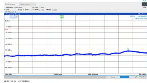
NTNV-n66-PC3-15-30-M-DFT-QPSK-Inner_1RB_Left-12000-2000 0-PASS
