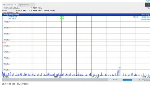
NTNV-n66-PC3-15-30-M-DFT-QPSK-Inner_1RB_Right-0.009-0.1 5-PASS
