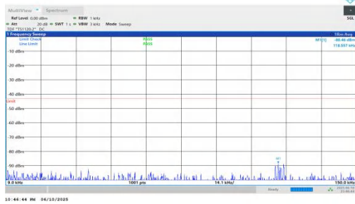
NTNV-n66-PC3-15-30-L-DFT-BPSK-Inner_1RB_Left-0.009-0.15-PASS
