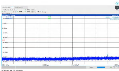
NTNV-n66-PC3-15-25-L-DFT-QPSK-Inner_1RB_Right-30-1000-P ASS
