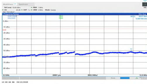
NTNV-n66-PC3-15-25-H-DFT-QPSK-Inner_1RB_Left-3000-1200 0-PASS
