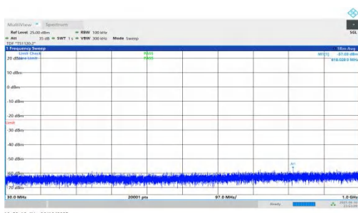
NTNV-n66-PC3-15-30-H-DFT-QPSK-Inner_1RB_Left-30-1000-PASS
