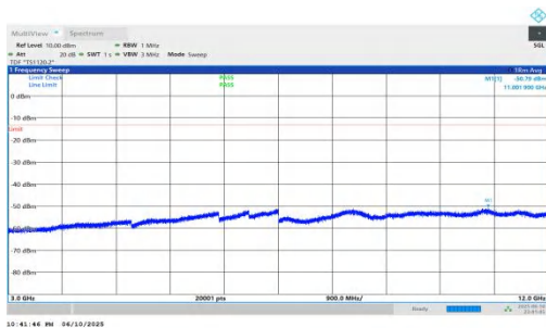
NTNV-n66-PC3-15-25-M-DFT-BPSK-Inner_1RB_Left-3000-12000-PASS
