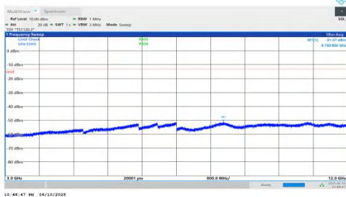
NTNV-n66-PC3-15-30-L-DFT-QPSK-Inner_1RB_Right-3000-12000 00-PASS
