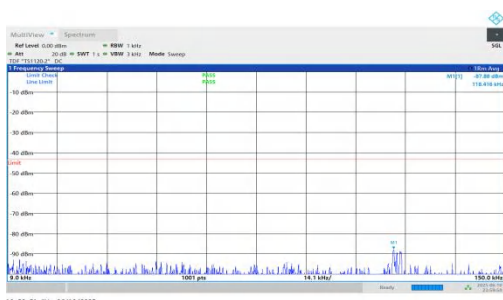
NTNV-n66-PC3-15-35-H-DFT-BPSK-Inner_1RB_Right-0.009-0.15-PASS
