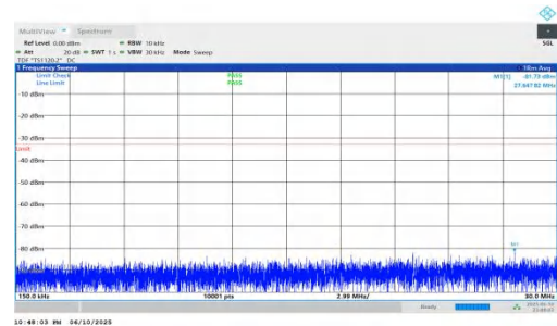
NTNV-n66-PC3-15-30-L-DFT-QPSK-Inner_1RB_Left-0.15-30-PAS S
