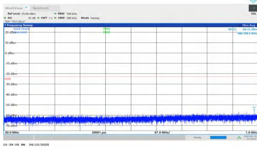
NTNV-n66-PC3-15-25-L-DFT-BPSK-Inner_1RB_Left-30-1000-PASS
