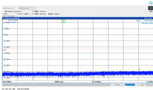
NTNV-n66-PC3-15-40-L-DFT-BPSK-Inner_1RB_Left-30-1000-PASS
