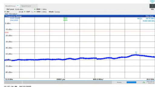
NTNV-n66-PC3-15-35-M-DFT-BPSK-Inner_1RB_Left-12000-20000-PASS
