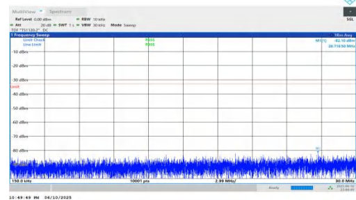
NTNV-n66-PC3-15-30-M-DFT-BPSK-Inner_1RB_Right-0.15-30-PASS
