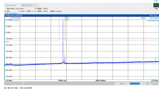
NTNV-n66-PC3-15-25-H-DFT-QPSK-Inner_1RB_Left-1000-3000- PASS
