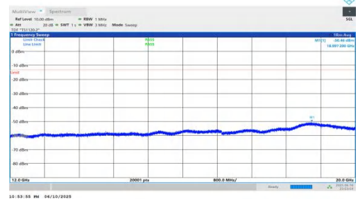
NTNV-n66-PC3-15-30-H-DFT-QPSK-Inner_1RB_Right-12000-20000- 00-PASS
