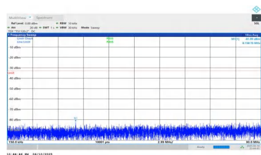
NTNV-n66-PC3-15-25-H-DFT-BPSK-Inner_1RB_Right-0.15-30-PASS
