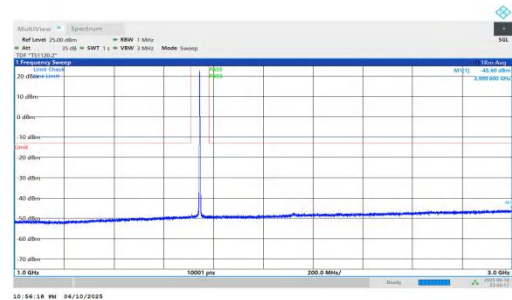
NTNV-n66-PC3-15-35-L-DFT-QPSK-Inner_1RB_Right-1000-3000-P PASS
