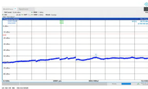
NTNV-n66-PC3-15-30-H-DFT-BPSK-Inner_1RB_Left-3000-12000-PASS
