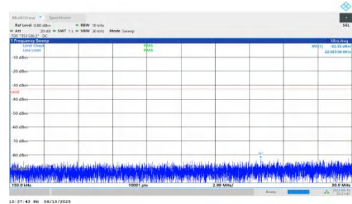
NTNV-n66-PC3-15-20-H-DFT-QPSK-Inner_1RB_Left-0.15-30-PAS S
