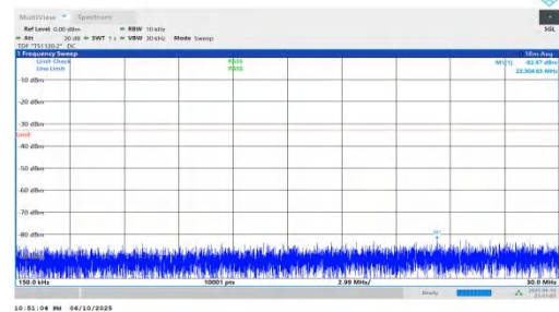
NTNV-n66-PC3-15-30-M-DFT-QPSK-Inner_1RB_Right-0.15-30-P ASS
