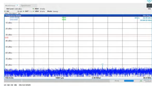
NTNV-n66-PC3-15-25-M-DFT-BPSK-Inner_1RB_Right-0.15-30-PASS
