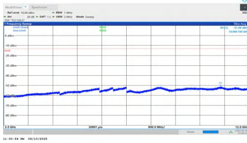
NTNV-n66-PC3-15-35-H-DFT-QPSK-Inner_1RB_Left-3000-1200 0-PASS
