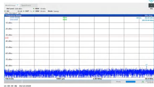
NTNV-n66-PC3-15-35-M-DFT-QPSK-Inner_1RB_Right-0.15-30-P ASS
