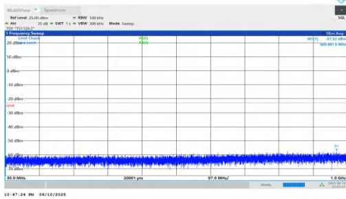
NTNV-n66-PC3-15-30-L-DFT-BPSK-Inner_1RB_Right-30-1000-P ASS
