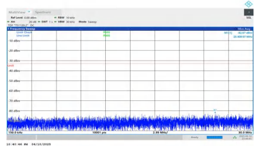
NTNV-n66-PC3-15-25-L-DFT-QPSK-Inner_1RB_Right-0.15-30-PA SS
