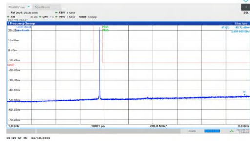
NTNV-n66-PC3-15-30-M-DFT-BPSK-Inner_1RB_Right-1000-3000-PASS
