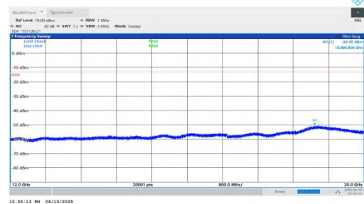
NTNV-n66-PC3-15-35-L-DFT-BPSK-Inner_1RB_Right-12000-200 00-PASS
