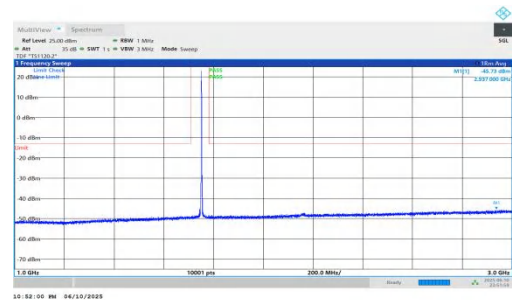
NTNV-n66-PC3-15-30-H-DFT-BPSK-Inner_1RB_Left-1000-3000-PASS
