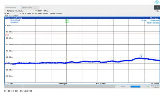
NTNV-n66-PC3-15-25-L-DFT-QPSK-Inner_1RB_Left-12000-2000 0-PASS
