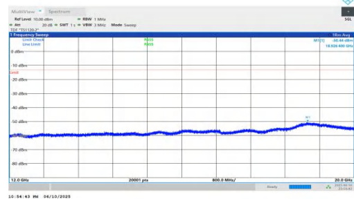
NTNV-n66-PC3-15-35-L-DFT-BPSK-Inner_1RB_Left-12000-20000-PASS
