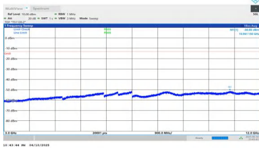
NTNV-n66-PC3-15-25-M-DFT-QPSK-Inner_1RB_Right-3000-12000- 00-PASS
