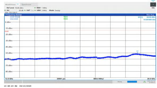
NTNV-n66-PC3-15-30-L-DFT-QPSK-Inner_1RB_Left-12000-2000 0-PASS
