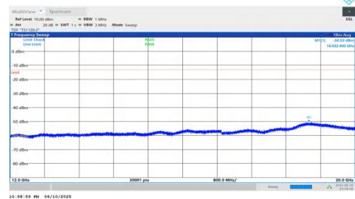
NTNV-n66-PC3-15-35-M-DFT-QPSK-Inner_1RB_Right-12000-20000-PASS
