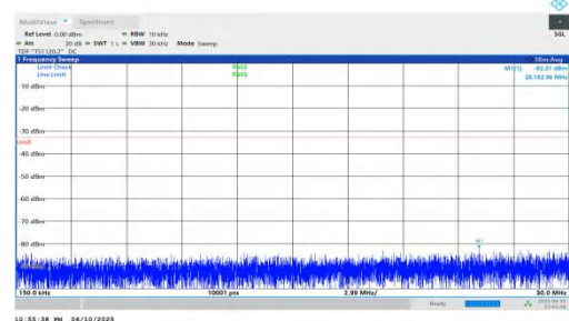
NTNV-n66-PC3-15-35-L-DFT-QPSK-Inner_1RB_Left-0.15-30-PAS S
