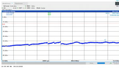
NTNV-n66-PC3-15-30-M-DFT-QPSK-Inner_1RB_Left-3000-1200 0-PASS
