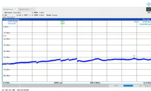
NTNV-n66-PC3-15-40-L-DFT-BPSK-Inner_1RB_Left-3000-12000-PASS
