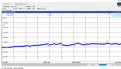
NTNV-n66-PC3-15-35-M-DFT-QPSK-Inner_1RB_Right-3000-12000-PASS
