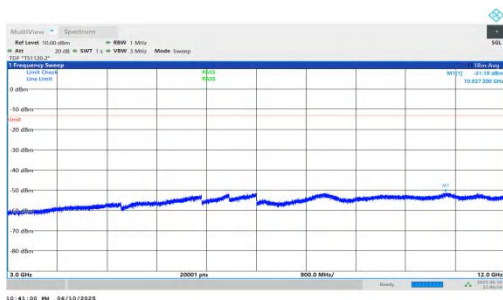
NTNV-n66-PC3-15-25-L-DFT-QPSK-Inner_1RB_Right-3000-12000 00-PASS
