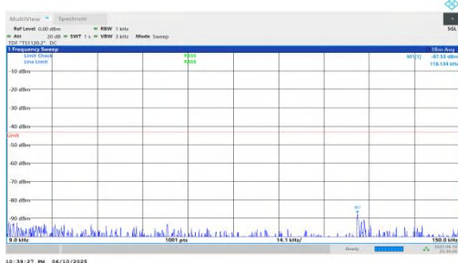
NTNV-n66-PC3-15-25-L-DFT-BPSK-Inner_1RB_Right-0.009-0.15-PASS
