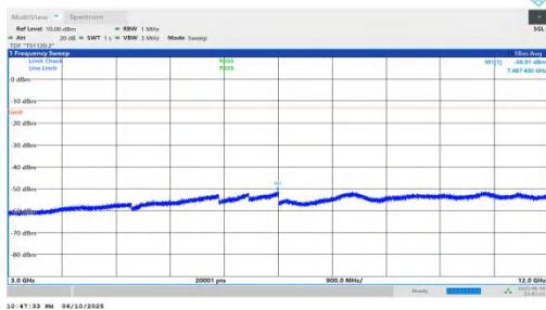
NTNV-n66-PC3-15-30-L-DFT-BPSK-Inner_1RB_Right-3000-1200 0-PASS
