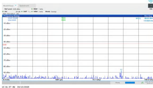
NTNV-n66-PC3-15-25-M-DFT-BPSK-Inner_1RB_Right-0.009-0.15-PASS
