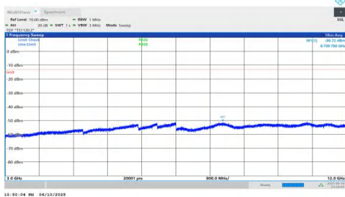
NTNV-n66-PC3-15-30-M-DFT-BPSK-Inner_1RB_Right-3000-12000-PASS
