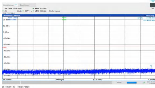
NTNV-n66-PC3-15-30-M-DFT-QPSK-Inner_1RB_Left-30-1000-PASS
