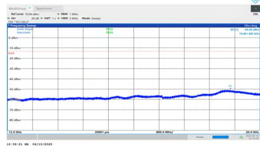
NTNV-n66-PC3-15-25-L-DFT-BPSK-Inner_1RB_Left-12000-20000-PASS
