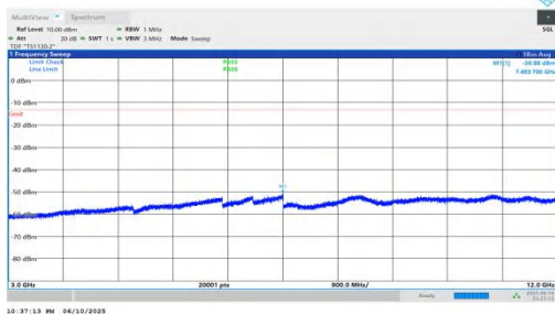
NTNV-n66-PC3-15-20-H-DFT-BPSK-Inner_1RB_Right-3000-120 00-PASS
