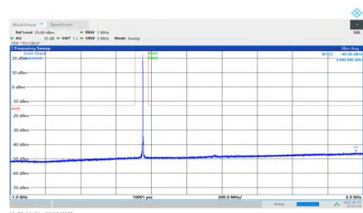
NTNV-n66-PC3-15-30-H-DFT-QPSK-Inner_1RB_Left-1000-3000-PASS
