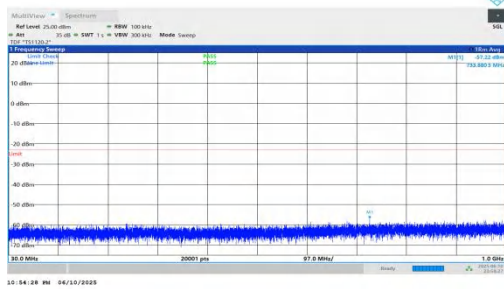
NTNV-n66-PC3-15-35-L-DFT-BPSK-Inner_1RB_Left-30-1000-PASS
