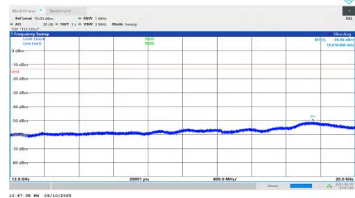
NTNV-n66-PC3-15-30-L-DFT-BPSK-Inner_1RB_Right-12000-200 00-PASS
