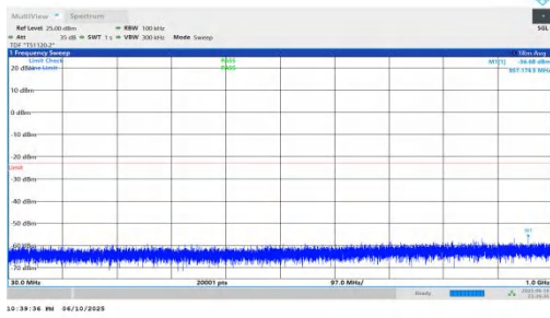
NTNV-n66-PC3-15-25-L-DFT-BPSK-Inner_1RB_Right-30-1000-P ASS
