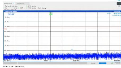
NTNV-n66-PC3-15-25-M-DFT-BPSK-Inner_1RB_Left-0.15-30-PASS
