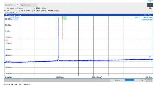
NTNV-n66-PC3-15-35-M-DFT-QPSK-Inner_1RB_Left-1000-3000-PASS
