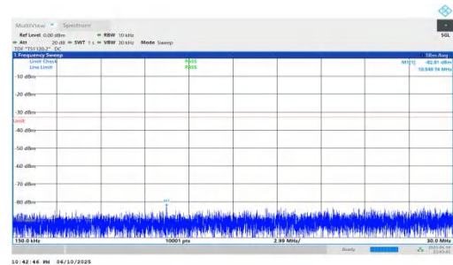
NTNV-n66-PC3-15-25-M-DFT-QPSK-Inner_1RB_Left-0.15-30-PASS
