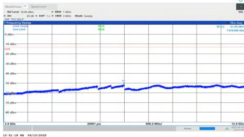
NTNV-n66-PC3-15-30-M-DFT-QPSK-Inner_1RB_Right-3000-12000- 00-PASS
