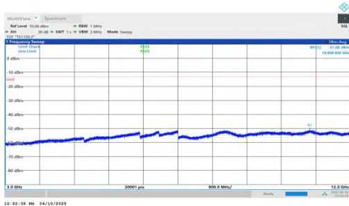
NTNV-n66-PC3-15-30-H-DFT-BPSK-Inner_1RB_Right-3000-12000-PASS
