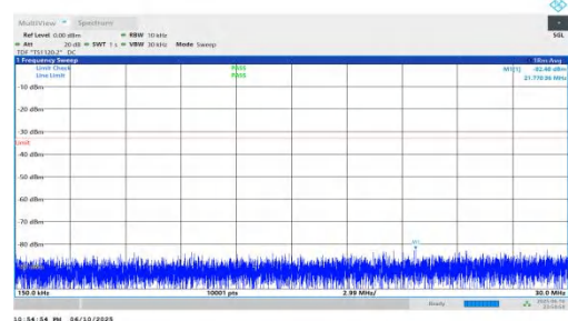
NTNV-n66-PC3-15-35-L-DFT-BPSK-Inner_1RB_Right-0.15-30-PASS
