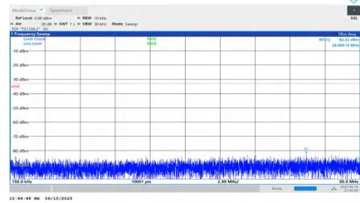
NTNV-n66-PC3-15-30-L-DFT-BPSK-Inner_1RB_Left-0.15-30-PASS
