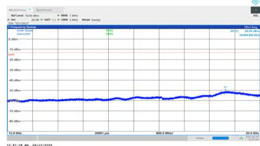
NTNV-n66-PC3-15-30-L-DFT-BPSK-Inner_1RB_Left-12000-20000-PASS
