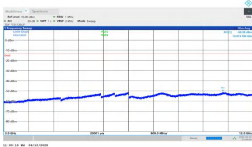
NTNV-n66-PC3-15-35-H-DFT-BPSK-Inner_1RB_Right-3000-120 00-PASS
