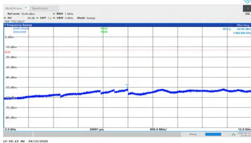
NTNV-n66-PC3-15-35-L-DFT-QPSK-Inner_1RB_Right-3000-12000 00-PASS
