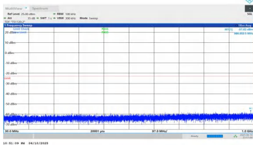
NTNV-n66-PC3-15-30-M-DFT-QPSK-Inner_1RB_Right-30-1000- PASS
