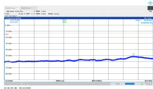
NTNV-n66-PC3-15-30-H-DFT-BPSK-Inner_1RB_Right-12000-20000-PASS
