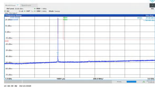
NTNV-n66-PC3-15-30-L-DFT-BPSK-Inner_1RB_Left-1000-3000-PASS
