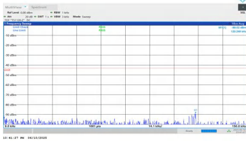
NTNV-n66-PC3-15-25-M-DFT-BPSK-Inner_1RB_Left-0.009-0.15-PASS
