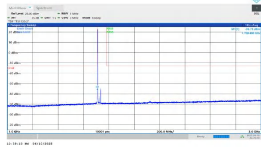
NTNV-n66-PC3-15-25-L-DFT-BPSK-Inner_1RB_Left-1000-3000-PASS
