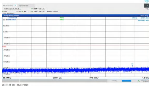
NTNV-n66-PC3-15-30-L-DFT-QPSK-Inner_1RB_Left-30-1000-PA SS
