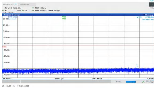
NTNV-n66-PC3-15-30-H-DFT-BPSK-Inner_1RB_Right-30-1000-P ASS
