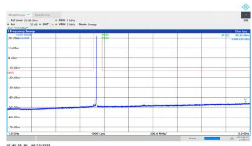
NTNV-n66-PC3-15-25-L-DFT-QPSK-Inner_1RB_Right-1000-3000-P PASS
