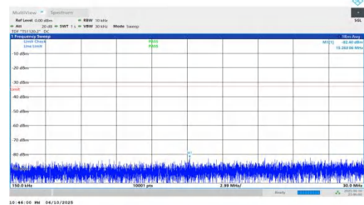
NTNV-n66-PC3-15-25-H-DFT-QPSK-Inner_1RB_Right-0.15-30-PA SS
