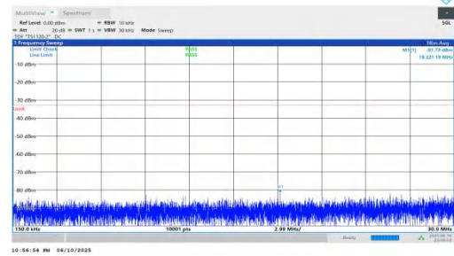
NTNV-n66-PC3-15-35-M-DFT-BPSK-Inner_1RB_Left-0.15-30-PASS
