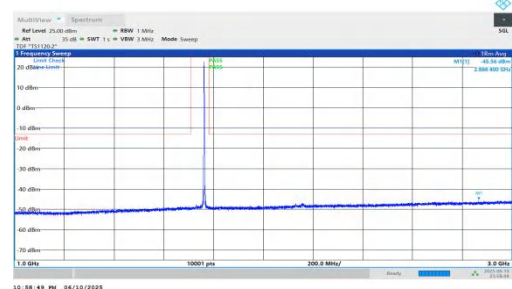
NTNV-n66-PC3-15-35-M-DFT-QPSK-Inner_1RB_Right-1000-3000-PASS
