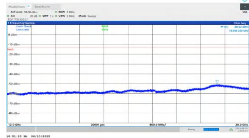
NTNV-n66-PC3-15-30-M-DFT-QPSK-Inner_1RB_Right-12000-20000- 00-PASS
