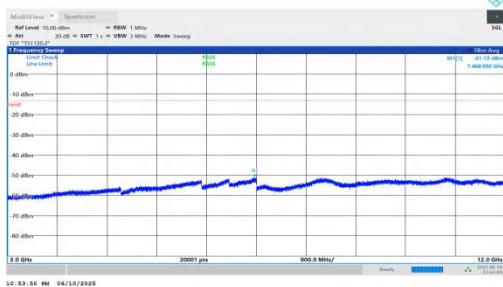
NTNV-n66-PC3-15-30-H-DFT-QPSK-Inner_1RB_Right-3000-12000- 00-PASS
