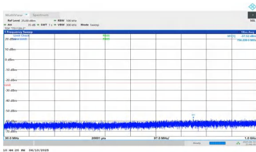
NTNV-n66-PC3-15-25-H-DFT-BPSK-Inner_1RB_Left-30-1000-PASS
