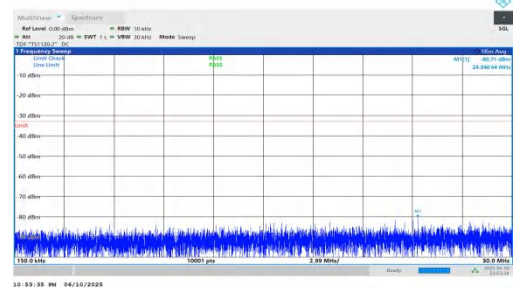
NTNV-n66-PC3-15-30-H-DFT-QPSK-Inner_1RB_Right-0.15-30-PA SS
