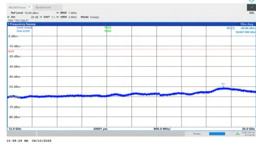
NTNV-n66-PC3-15-35-M-DFT-QPSK-Inner_1RB_Left-12000-2000 0-PASS
