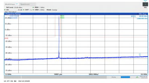
NTNV-n66-PC3-15-35-M-DFT-BPSK-Inner_1RB_Right-1000-3000-PASS
