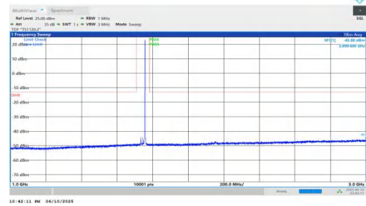
NTNV-n66-PC3-15-25-M-DFT-BPSK-Inner_1RB_Right-1000-3000-PASS
