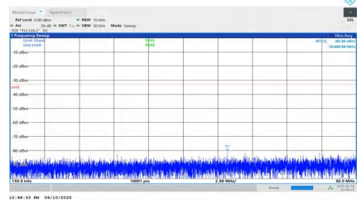
NTNV-n66-PC3-15-30-L-DFT-QPSK-Inner_1RB_Right-0.15-30-PA SS
