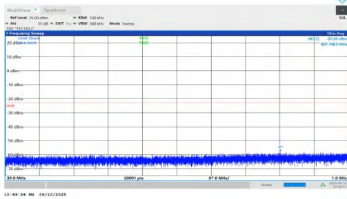
NTNV-n66-PC3-15-30-M-DFT-BPSK-Inner_1RB_Right-30-1000-PASS
