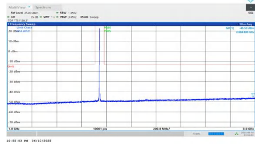
NTNV-n66-PC3-15-35-L-DFT-BPSK-Inner_1RB_Right-1000-3000-P PASS
