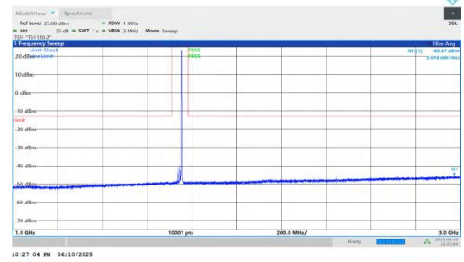
NTNV-n66-PC3-15-15-M-DFT-BPSK-Inner_1RB_Right-1000-3000-PASS
