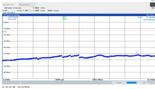
NTNV-n66-PC3-15-15-H-DFT-QPSK-Inner_1RB_Left-3000-1200 0-PASS
