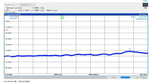
NTNV-n66-PC3-15-10-L-DFT-QPSK-Inner_1RB_Right-12000-200 00-PASS
