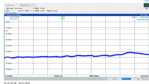
NTNV-n66-PC3-15-5-H-DFT-BPSK-Inner_1RB_Right-12000-2000 0-PASS
