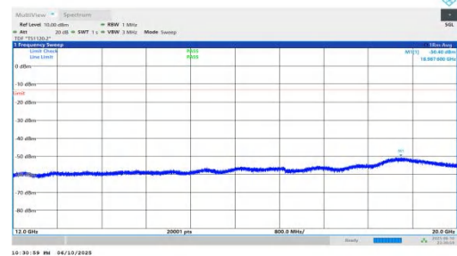
NTNV-n66-PC3-15-15-H-DFT-QPSK-Inner_1RB_Right-12000-20000-PASS
