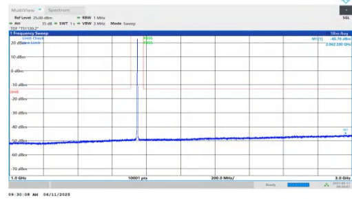
NTNV-n66-PC3-15-5-M-DFT-BPSK-Inner_1RB_Right-1000-3000-PASS
