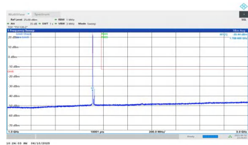
NTNV-n66-PC3-15-15-L-DFT-BPSK-Inner_1RB_Left-1000-3000-PASS
