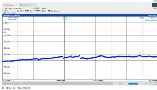
NTNV-n66-PC3-15-20-L-DFT-BPSK-Inner_1RB_Right-3000-12000-PASS
