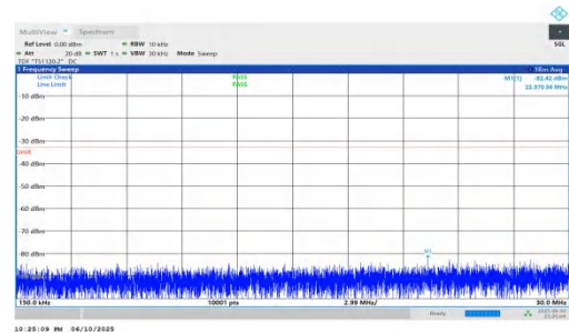
NTNV-n66-PC3-15-15-L-DFT-QPSK-Inner_1RB_Left-0.15-30-PASS
