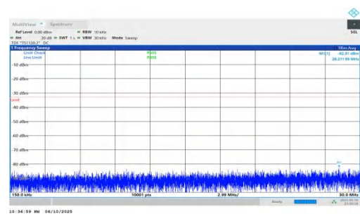
NTNV-n66-PC3-15-20-H-DFT-BPSK-Inner_1RB_Right-0.15-30-PASS
