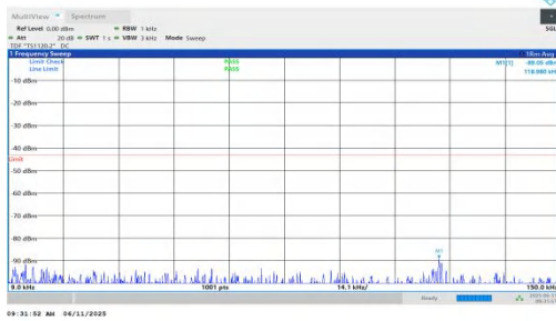
NTNV-n66-PC3-15-5-H-DFT-BPSK-Inner_1RB_Left-0.009-0.15-P ASS
