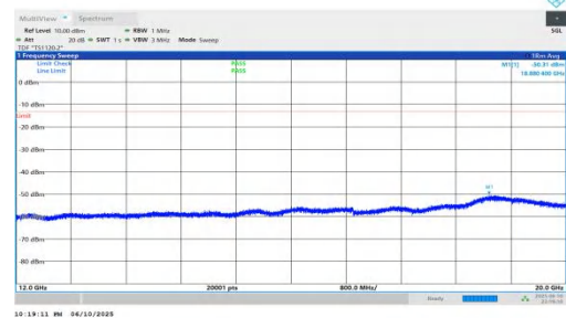
NTNV-n66-PC3-15-10-M-DFT-BPSK-Inner_1RB_Left-12000-20000-PASS
