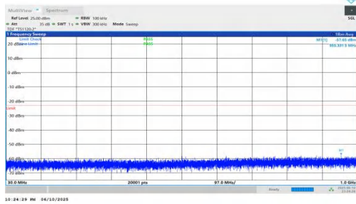
NTNV-n66-PC3-15-15-L-DFT-BPSK-Inner_1RB_Right-30-1000-PASS
