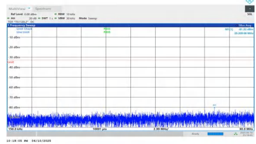
NTNV-n66-PC3-15-10-L-DFT-QPSK-Inner_1RB_Right-0.15-30-PA SS
