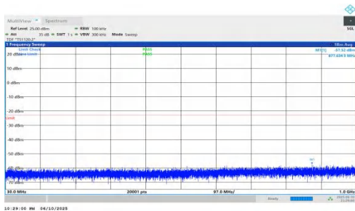
NTNV-n66-PC3-15-15-H-DFT-BPSK-Inner_1RB_Left-30-1000-PA
