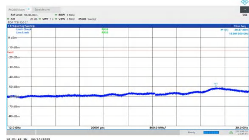
NTNV-n66-PC3-15-10-H-DFT-BPSK-Inner_1RB_Left-12000-20000-PASS 0-PASS
