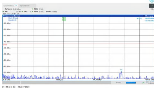
NTNV-n66-PC3-15-20-M-DFT-BPSK-Inner_1RB_Right-0.009-0.15-5-PASS
