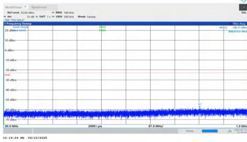
NTNV-n66-PC3-15-10-M-DFT-BPSK-Inner_1RB_Right-30-1000-PASS
