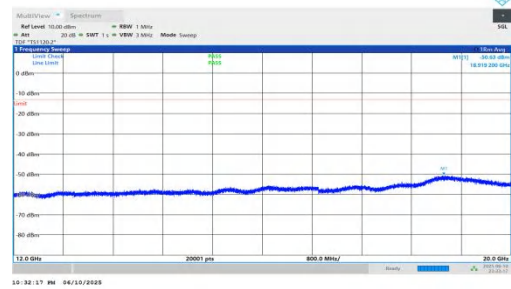
NTNV-n66-PC3-15-20-L-DFT-BPSK-Inner_1RB_Right-12000-20000-PASS
