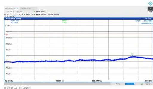
NTNV-n66-PC3-15-5-H-DFT-BPSK-Inner_1RB_Left-12000-20000- PASS
