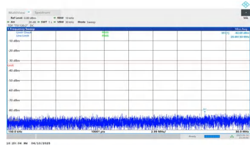
NTNV-n66-PC3-15-10-M-DFT-QPSK-Inner_1RB_Left-0.15-30-PASS
