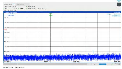
NTNV-n66-PC3-15-10-M-DFT-QPSK-Inner_1RB_Right-0.15-30-P ASS
