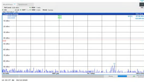
NTNV-n66-PC3-15-20-L-DFT-QPSK-Inner_1RB_Right-0.009-0.1 5-PASS
