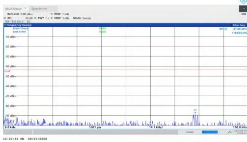
NTNV-n66-PC3-15-10-M-DFT-QPSK-Inner_1RB_Right-0.009-0.1 5-PASS
