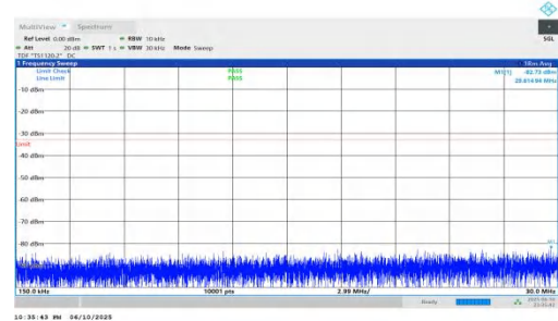
NTNV-n66-PC3-15-20-M-DFT-QPSK-Inner_1RB_Right-0.15-30-P ASS
