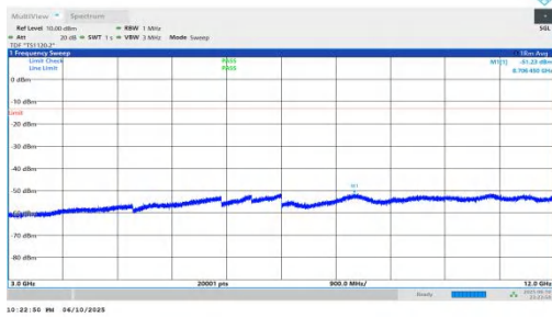
NTNV-n66-PC3-15-10-H-DFT-QPSK-Inner_1RB_Left-3000-1200 0-PASS
