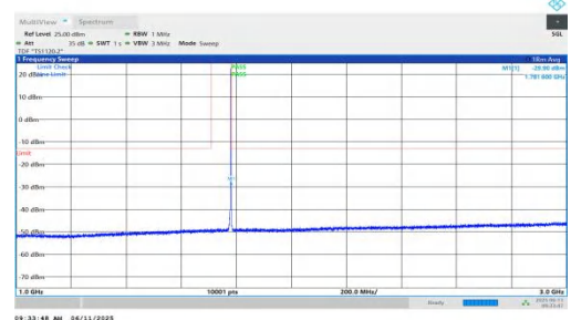
NTNV-n66-PC3-15-5-H-DFT-QPSK-Inner_1RB_Right-1000-3000-PASS
