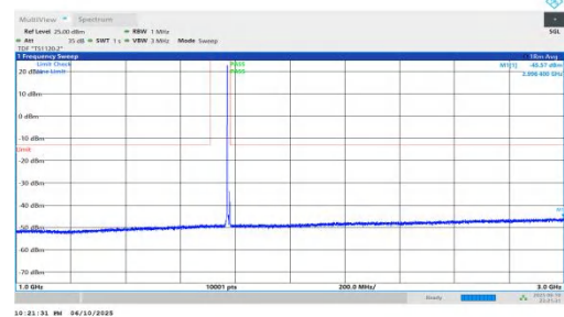
NTNV-n66-PC3-15-10-H-DFT-BPSK-Inner_1RB_Left-1000-3000-P ASS
