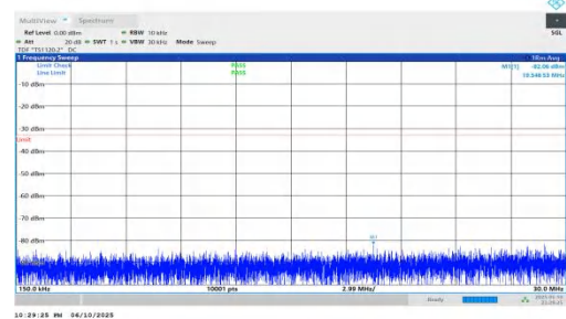
NTNV-n66-PC3-15-15-H-DFT-BPSK-Inner_1RB_Right-0.15-30-PASS
