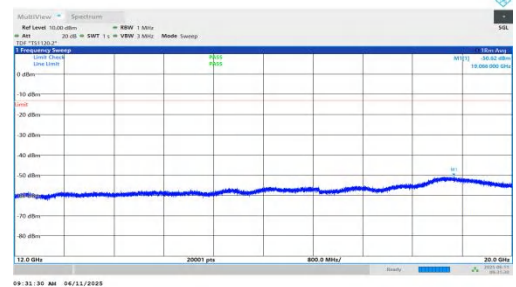
NTNV-n66-PC3-15-5-M-DFT-QPSK-Inner_1RB_Right-12000-2000 0-PASS
