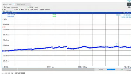
NTNV-n66-PC3-15-10-H-DFT-QPSK-Inner_1RB_Right-3000-12000-PASS
