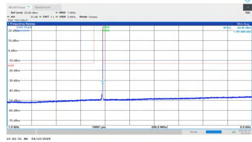
NTNV-n66-PC3-15-10-H-DFT-BPSK-Inner_1RB_Right-1000-3000-P PASS
