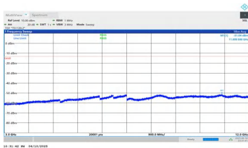
NTNV-n66-PC3-15-20-L-DFT-BPSK-Inner_1RB_Left-3000-12000-PASS
