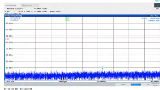
NTNV-n66-PC3-15-10-M-DFT-BPSK-Inner_1RB_Right-0.15-30-PASS
