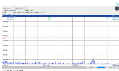
NTNV-n66-PC3-15-20-L-DFT-BPSK-Inner_1RB_Right-0.009-0.15-PASS
