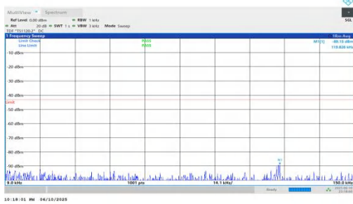
NTNV-n66-PC3-15-10-L-DFT-QPSK-Inner_1RB_Right-0.009-0.1 5-PASS
