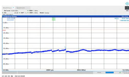
NTNV-n66-PC3-15-15-M-DFT-BPSK-Inner_1RB_Left-3000-12000-PASS
