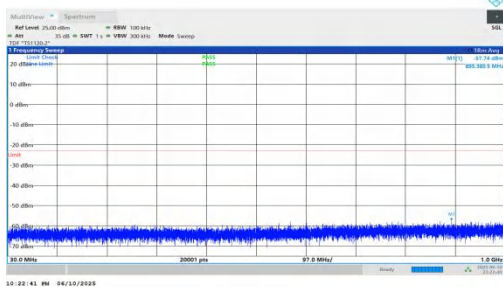
NTNV-n66-PC3-15-10-H-DFT-QPSK-Inner_1RB_Left-30-1000-P ASS
