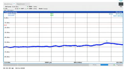
NTNV-n66-PC3-15-5-H-DFT-QPSK-Inner_1RB_Right-12000-20000-PASS
