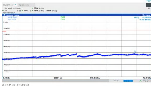
NTNV-n66-PC3-15-20-M-DFT-QPSK-Inner_1RB_Right-3000-12000-PASS
