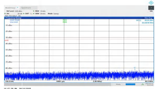
NTNV-n66-PC3-15-15-M-DFT-QPSK-Inner_1RB_Left-0.15-30-PASS
