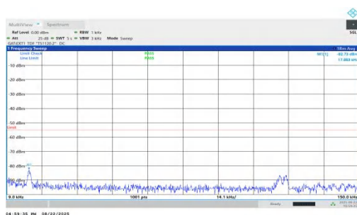
NTNV-n41-PC1.5-30-90-L-DFT-BPSK-Inner_1RB_Right-0.009-0.15-PASS
