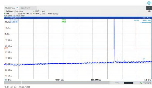
NTNV-n41-PC1.5-30-90-L-DFT-BPSK-Inner_1RB_Left-1000-3000-PASS
