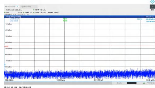
NTNV-n41-PC1.5-30-100-H-DFT-QPSK-Inner_1RB_Left-0.15-30- PASS
