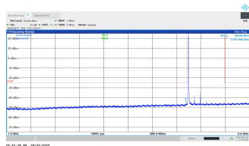
NTNV-n41-PC1.5-30-100-L-DFT-QPSK-Inner_1RB_Left-1000-300 0-PASS
