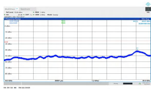
NTNV-n41-PC1.5-30-90-L-DFT-BPSK-Inner_1RB_Left-18000-30000-PASS
