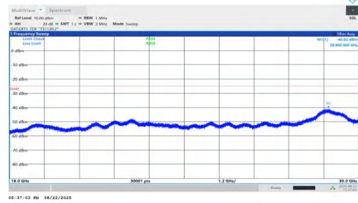
NTNV-n41-PC1.5-30-100-H-DFT-QPSK-Inner_1RB_Left-18000-3000-PASS
