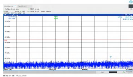
NTNV-n41-PC1.5-30-90-L-DFT-QPSK-Inner_1RB_Left-0.15-30-PA SS
