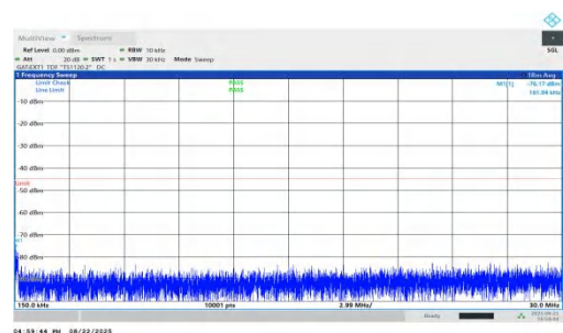
NTNV-n41-PC1.5-30-90-L-DFT-BPSK-Inner_1RB_Right-0.15-30-PA
