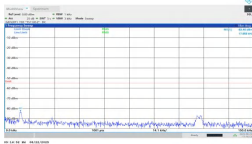
NTVN-n41-PC1.5-30-90-H-DFT-QPSK-Inner_1RB_Right-0.009-0.15-PASS
