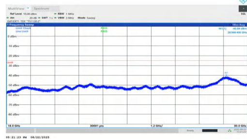
NTNV-n41-PC1.5-30-100-L-DFT-BPSK-Inner_1RB_Right-18000-3 0000-PASS
