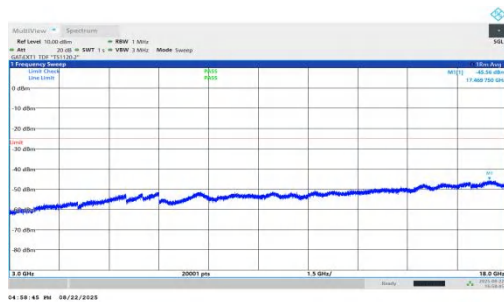
NTNV-n41-PC1.5-30-90-L-DFT-BPSK-Inner_1RB_Left-3000-18000-PASS
