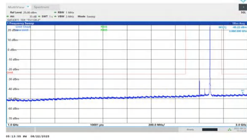
NTNV-n41-PC1.5-30-90-H-DFT-BPSK-Inner_1RB_Right-1000-300 0-PASS
