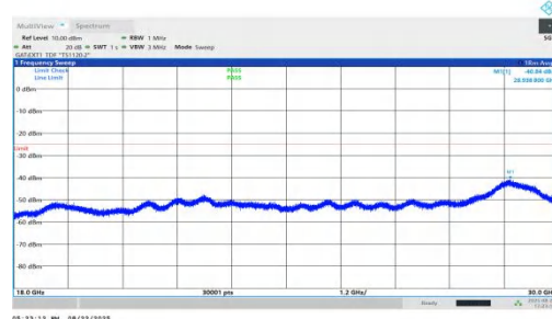
NTNV-n41-PC1.5-30-100-L-DFT-QPSK-Inner_1RB_Left-18000-30000-PASS
