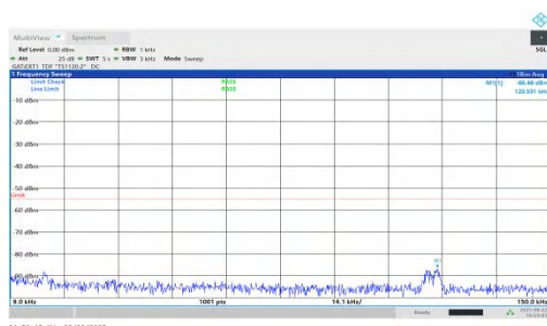
NTNV-n41-PC1.5-30-80-H-DFT-BPSK-Inner_1RB_Right-0.009-0.15-PASS
