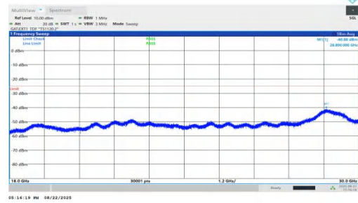
NTVN-n41-PC1.5-30-90-H-DFT-QPSK-Inner_1RB_Left-18000-30000-PASS
