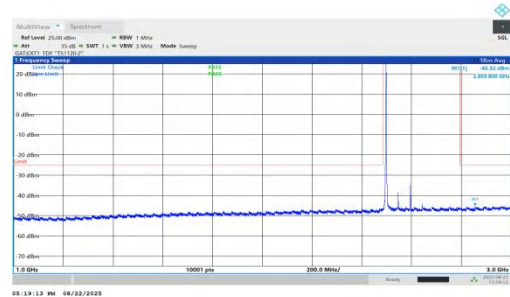
NTNV-n41-PC1.5-30-100-L-DFT-BPSK-Inner_1RB_Left-1000-300-PASS
