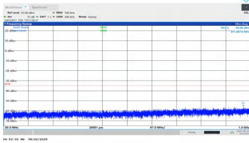
NTNV-n41-PC1.5-30-80-H-DFT-BPSK-Inner_1RB_Right-30-1000 -PASS
