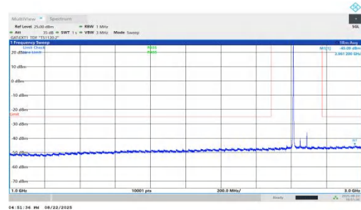
NTNV-n41-PC1.5-30-80-H-DFT-BPSK-Inner_1RB_Left-1000-3000-PASS
