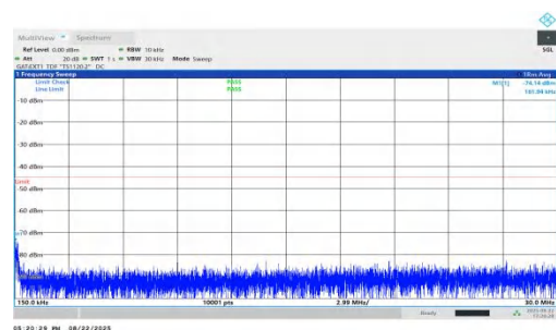
NTNV-n41-PC1.5-30-100-L-DFT-BPSK-Inner_1RB_Right-0.15-30-PASS
