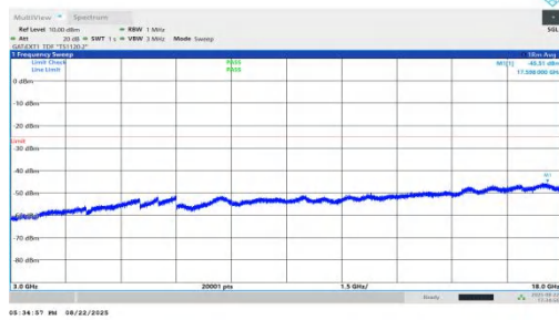
NTNV-n41-PC1.5-30-100-H-DFT-BPSK-Inner_1RB_Right-3000-1 8000-PASS
