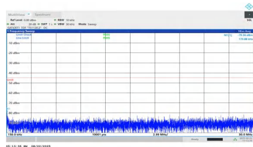
NTNV-n41-PC1.5-30-90-H-DFT-BPSK-Inner_1RB_Right-0.15-30- PASS
