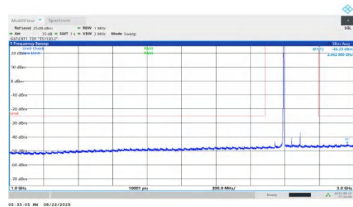
NTNV-n41-PC1.5-30-100-H-DFT-BPSK-Inner_1RB_Left-1000-3000-PASS
