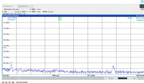
NTNV-n41-PC1.5-30-80-H-DFT-QPSK-Inner_1RB_Left-0.009-0.1 5-PASS
