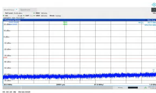
NTNV-n41-PC1.5-30-100-H-DFT-QPSK-Inner_1RB_Left-30-1000 -PASS
