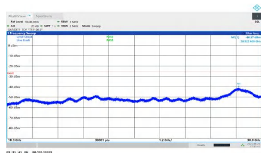
NTVN-n41-PC1.5-30-100-M-DFT-QPSK-Inner_1RB_Right-18000.0-30000.0-PASS
