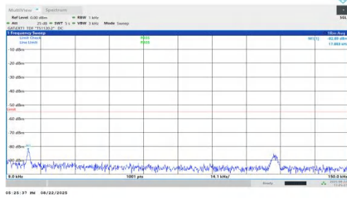
NTNV-n41-PC1.5-30-100-M-DFT-BPSK-Inner_1RB_Left-0.009-0.15-PASS
