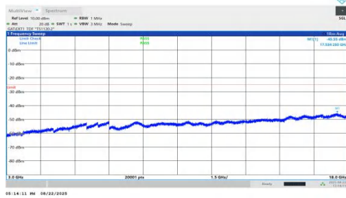
NTNV-n41-PC1.5-30-90-H-DFT-BPSK-Inner_1RB_Right-3000-18 000-PASS
