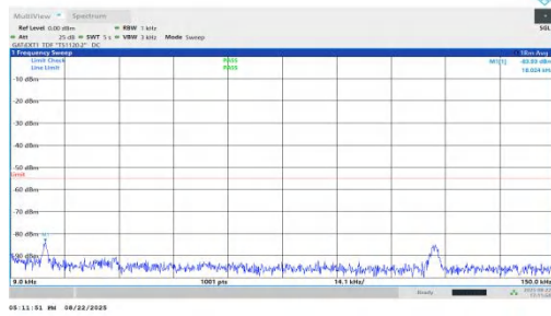
NTNV-n41-PC1.5-30-90-H-DFT-BPSK-Inner_1RB_Left-0.009-0.1 5-PASS
