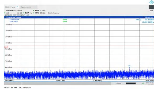
NTNV-n41-PC1.5-30-90-H-DFT-QPSK-Inner_1RB_Left-0.15-30-P ASS
