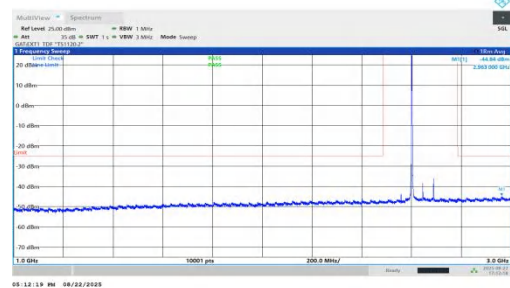
NTNV-n41-PC1.5-30-90-H-DFT-BPSK-Inner_1RB_Left-1000-3000 -PASS
