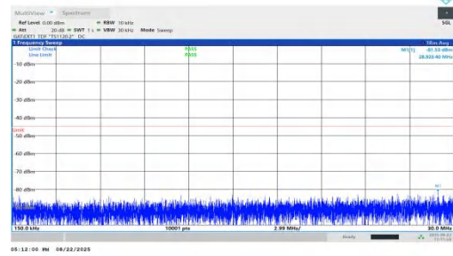
NTNV-n41-PC1.5-30-90-H-DFT-BPSK-Inner_1RB_Left-0.15-30-P ASS
