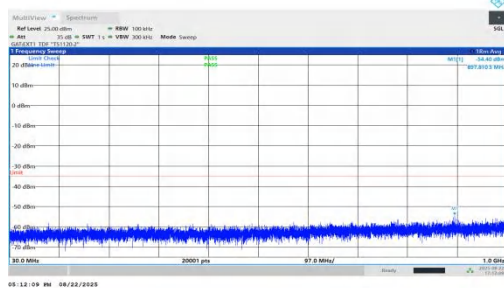
NTNV-n41-PC1.5-30-90-H-DFT-BPSK-Inner_1RB_Left-30-1000- PASS
