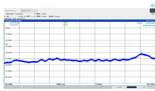
NTNV-n41-PC1.5-30-80-H-DFT-QPSK-Inner_1RB_Right-18000-30000-PASS
