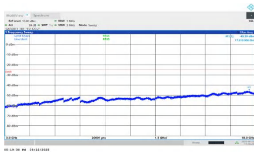
NTNV-n41-PC1.5-30-100-L-DFT-BPSK-Inner_1RB_Left-3000-18000-PASS
