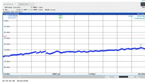
NTNV-n41-PC1.5-30-100-H-DFT-QPSK-Inner_1RB_Left-3000-18000-PASS
