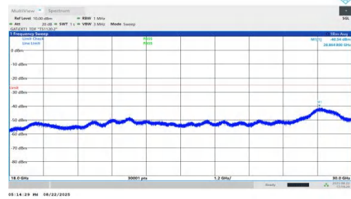
NTNV-n41-PC1.5-30-90-H-DFT-BPSK-Inner_1RB_Right-18000-30 000-PASS
