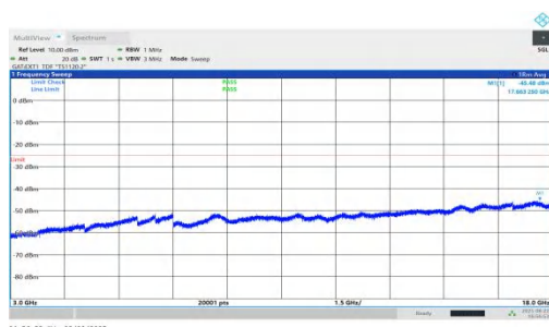
NTNV-n41-PC1.5-30-80-H-DFT-QPSK-Inner_1RB_Right-3000-18000-PASS
