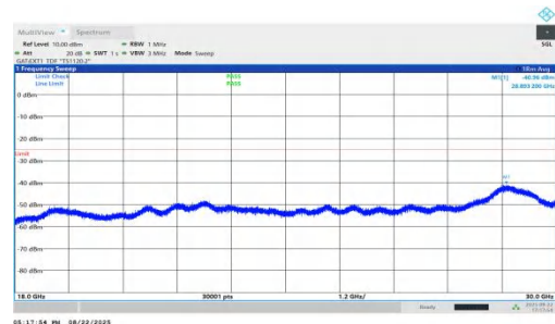
NTVN-n41-PC1.5-30-90-H-DFT-QPSK-Inner_1RB_Right-18000-30000-PASS
