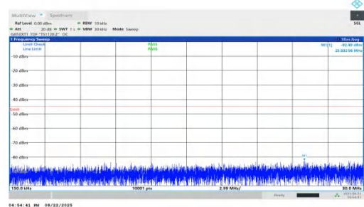
NTNV-n41-PC1.5-30-80-H-DFT-QPSK-Inner_1RB_Left-0.15-30-P ASS
