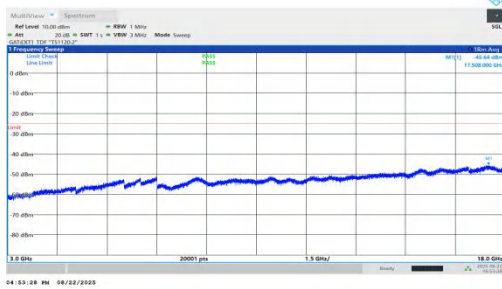
NTNV-n41-PC1.5-30-80-H-DFT-BPSK-Inner_1RB_Right-3000-18 000-PASS
