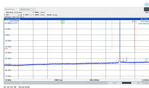
NTNV-n41-PC1.5-30-100-H-DFT-QPSK-Inner_1RB_Left-1000-300 0-PASS
