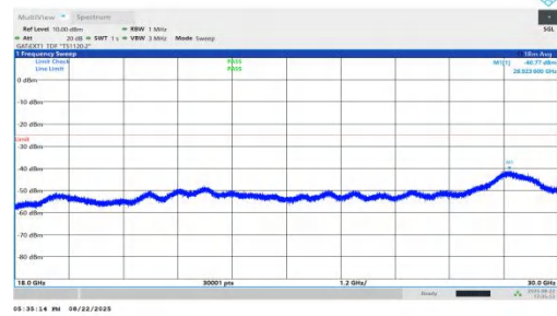
NTNV-n41-PC1.5-30-100-H-DFT-BPSK-Inner_1RB_Right-18000-3 0000-PASS
