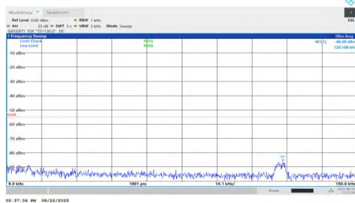
NTNV-n41-PC1.5-30-100-H-DFT-QPSK-Inner_1RB_Right-0.009-0.15-PASS
