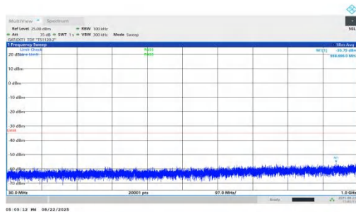
NTVN-n41-PC1.5-30-90-M-DFT-BPSK-Inner_1RB_Left-30-1000- PASS
