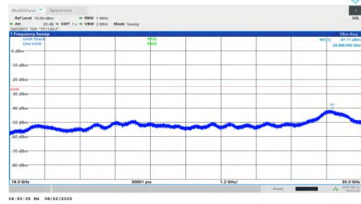
NTNV-n41-PC1.5-30-80-H-DFT-QPSK-Inner_1RB_Left-18000-30000-PASS
