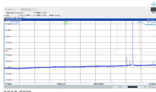
NTNV-n41-PC1.5-30-80-H-DFT-QPSK-Inner_1RB_Right-1000-3000-PASS
