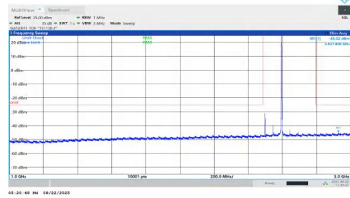
NTNV-n41-PC1.5-30-100-L-DFT-BPSK-Inner_1RB_Right-1000-30 00-PASS
