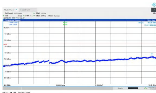
NTVN-n41-PC1.5-30-100-M-DFT-QPSK-Inner_1RB_Right-3000.0-18000.0-PASS
