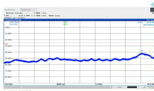
NTNV-n41-PC1.5-30-100-L-DFT-QPSK-Inner_1RB_Right-18000-30000-PASS
