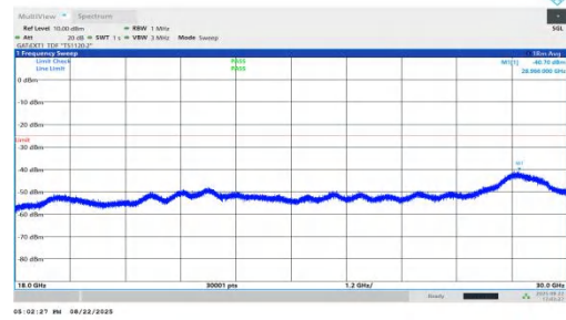
NTNV-n41-PC1.5-30-90-L-DFT-QPSK-Inner_1RB_Left-18000-30000-PASS
