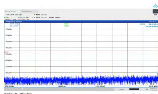
NTVN-n41-PC1.5-30-90-M-DFT-BPSK-Inner_1RB_Right-0.15-30- PASS
