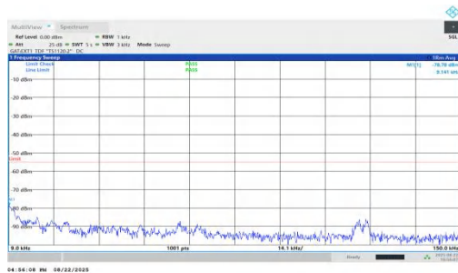
NTNV-n41-PC1.5-30-80-H-DFT-QPSK-Inner_1RB_Right-0.009-0.15-PASS
