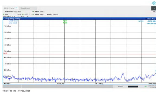
NTVN-n41-PC1.5-30-100-M-DFT-QPSK-Inner_1RB_Right-0.009-0.15-PASS
