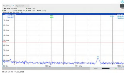
NTNV-n41-PC1.5-30-90-H-DFT-QPSK-Inner_1RB_Left-0.009-0.1 5-PASS
