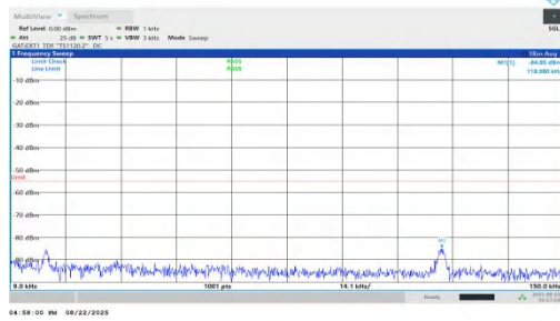
NTNV-n41-PC1.5-30-90-L-DFT-BPSK-Inner_1RB_Left-0.009-0.15-PASS
