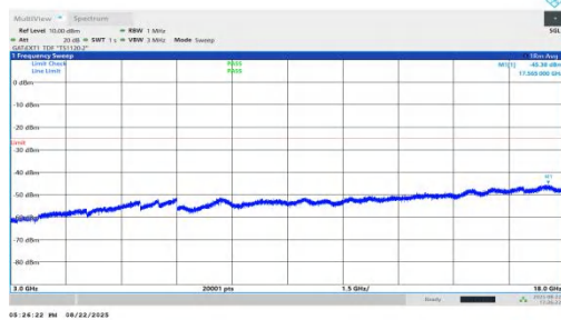
NTNV-n41-PC1.5-30-100-M-DFT-BPSK-Inner_1RB_Left-3000-18000-PASS
