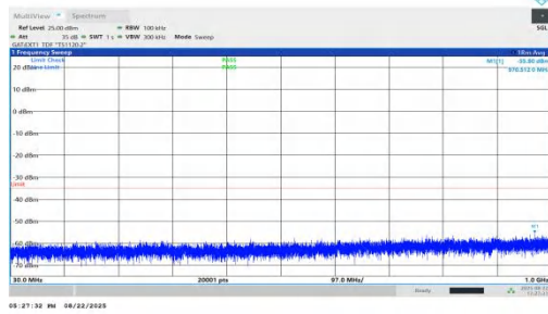
NTVN-n41-PC1.5-30-100-M-DFT-BPSK-Inner_1RB_Right-30-100 0-PASS
