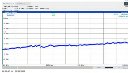
NTNV-n41-PC1.5-30-80-H-DFT-QPSK-Inner_1RB_Left-3000-18000-PASS
