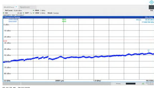
NTNV-n41-PC1.5-30-100-L-DFT-QPSK-Inner_1RB_Left-3000-18000-PASS
