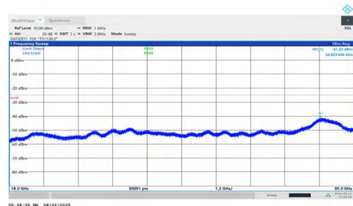
NTNV-n41-PC1.5-30-100-H-DFT-QPSK-Inner_1RB_Right-18000-30000-PASS
