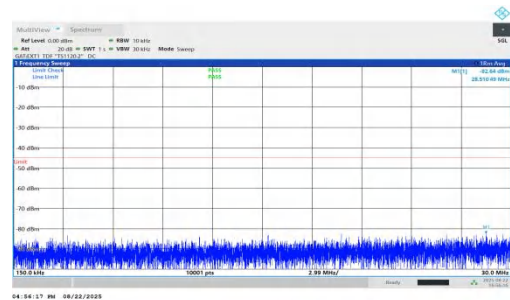
NTNV-n41-PC1.5-30-80-H-DFT-QPSK-Inner_1RB_Right-0.15-30-PASS
