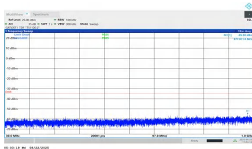
NTNV-n41-PC1.5-30-90-L-DFT-QPSK-Inner_1RB_Right-30-1000-PASS
