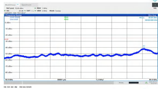
NTNV-n41-PC1.5-30-80-H-DFT-BPSK-Inner_1RB_Right-18000-30 000-PASS
