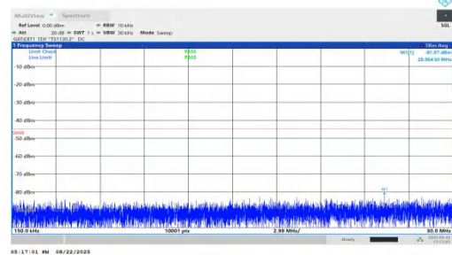
NTVN-n41-PC1.5-30-90-H-DFT-QPSK-Inner_1RB_Right-0.15-30-PASS
