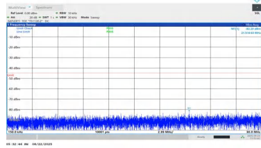
NTNV-n41-PC1.5-30-100-H-DFT-BPSK-Inner_1RB_Left-0.15-30-PASS
