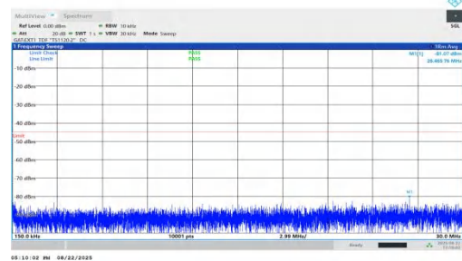
NTVN-n41-PC1.5-30-90-M-DFT-QPSK-Inner_1RB_Right-0.15-30-PASS
