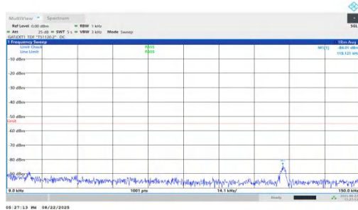
NTNV-n41-PC1.5-30-100-M-DFT-BPSK-Inner_1RB_Right-0.009-0.15-PASS
