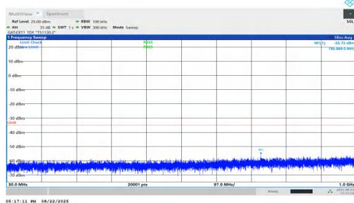
NTVN-n41-PC1.5-30-90-H-DFT-QPSK-Inner_1RB_Right-30-1000-PASS
