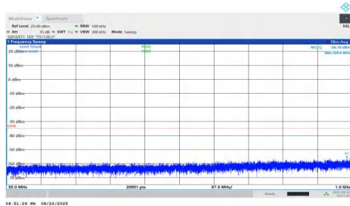
NTNV-n41-PC1.5-30-80-H-DFT-BPSK-Inner_1RB_Left-30-1000-PASS
