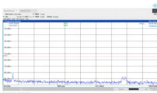
NTNV-n41-PC1.5-30-100-H-DFT-BPSK-Inner_1RB_Right-0.009-0.15-PASS
