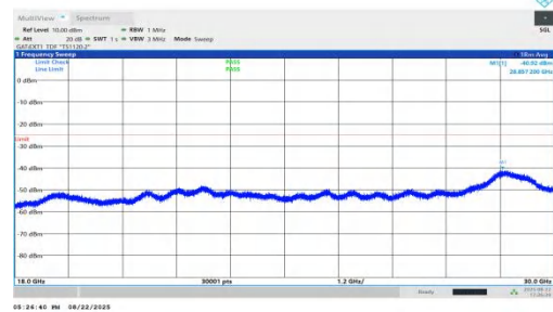
NTNV-n41-PC1.5-30-100-M-DFT-BPSK-Inner_1RB_Left-18000-30000-PASS
