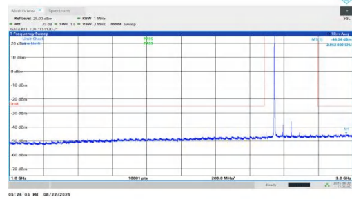
NTNV-n41-PC1.5-30-100-M-DFT-BPSK-Inner_1RB_Left-1000-3000-PASS
