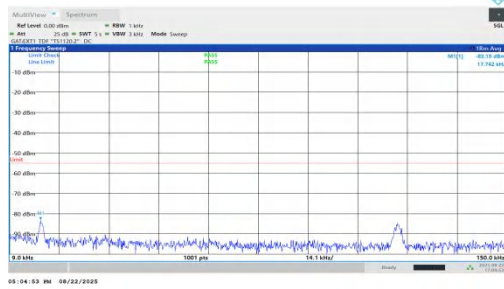
NTVN-n41-PC1.5-30-90-M-DFT-BPSK-Inner_1RB_Left-0.009-0.1 5-PASS
