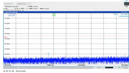
NTNV-n41-PC1.5-30-90-L-DFT-BPSK-Inner_1RB_Left-0.15-30-PA
