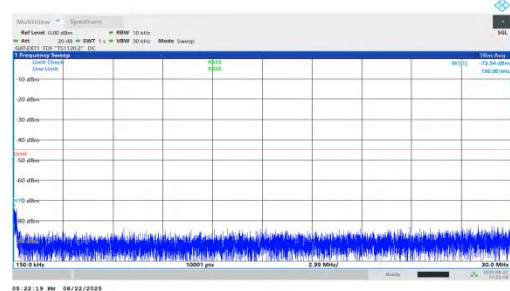
NTNV-n41-PC1.5-30-100-L-DFT-QPSK-Inner_1RB_Left-0.15-30-P ASS
