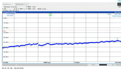
NTNV-n41-PC1.5-30-100-L-DFT-BPSK-Inner_1RB_Right-3000-1 8000-PASS
