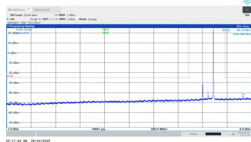
NTVN-n41-PC1.5-30-90-H-DFT-QPSK-Inner_1RB_Right-1000-3000-PASS
