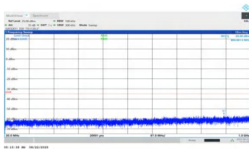
NTNV-n41-PC1.5-30-90-H-DFT-QPSK-Inner_1RB_Left-30-1000- PASS
