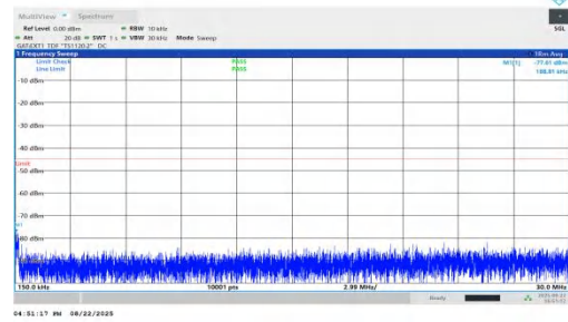
NTNV-n41-PC1.5-30-80-H-DFT-BPSK-Inner_1RB_Left-0.15-30-PASS
