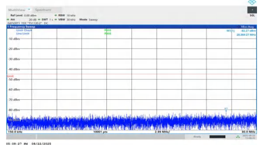
NTNV-n41-PC1.5-30-90-M-DFT-QPSK-Inner_1RB_Left-0.15-30-PASS
