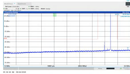
NTNV-n41-PC1.5-30-100-H-DFT-BPSK-Inner_1RB_Right-1000-30 00-PASS
