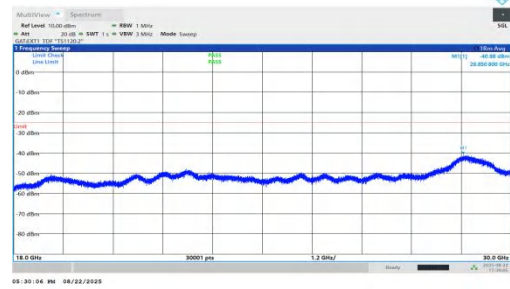
NTVN-n41-PC1.5-30-100-M-DFT-QPSK-Inner_1RB_Left-18000-30000-PASS
