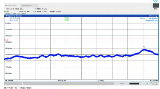
NTNV-n41-PC1.5-30-90-M-DFT-BPSK-Inner_1RB_Right-18000-30000-PASS
