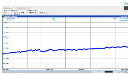
NTNV-n41-PC1.5-30-100-L-DFT-QPSK-Inner_1RB_Right-3000-18000-PASS
