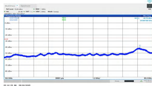
NTNV-n41-PC1.5-30-90-H-DFT-BPSK-Inner_1RB_Left-18000-300 00-PASS
