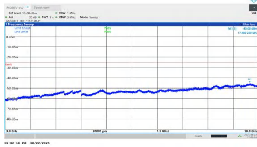
NTNV-n41-PC1.5-30-90-L-DFT-QPSK-Inner_1RB_Left-3000-18000-PASS
