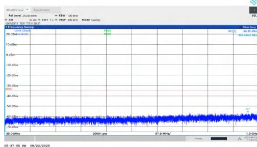
NTNV-n41-PC1.5-30-100-H-DFT-QPSK-Inner_1RB_Right-30-1000-PASS
