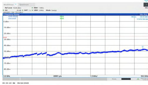
NTNV-n41-PC1.5-30-90-L-DFT-BPSK-Inner_1RB_Right-3000-18 000-PASS
