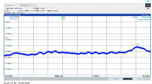
NTVN-n41-PC1.5-30-100-M-DFT-BPSK-Inner_1RB_Right-18000-3 0000-PASS
