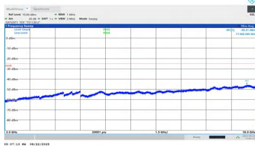
NTNV-n41-PC1.5-30-90-M-DFT-BPSK-Inner_1RB_Right-3000-18000-PASS
