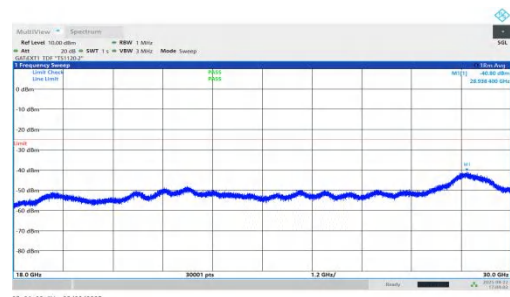
NTNV-n41-PC1.5-30-90-L-DFT-QPSK-Inner_1RB_Right-18000-30000-PASS
