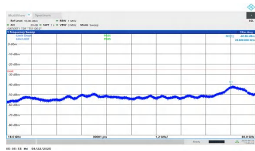
NTVN-n41-PC1.5-30-90-M-DFT-BPSK-Inner_1RB_Left-18000-300 00-PASS
