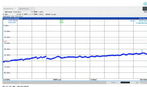
NTVN-n41-PC1.5-30-90-H-DFT-QPSK-Inner_1RB_Right-3000-18000-PASS
