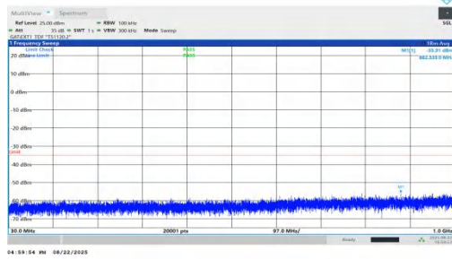
NTNV-n41-PC1.5-30-90-L-DFT-BPSK-Inner_1RB_Right-30-1000 -PASS
