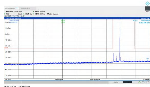
NTNV-n41-PC1.5-30-90-L-DFT-QPSK-Inner_1RB_Right-1000-3000-PASS
