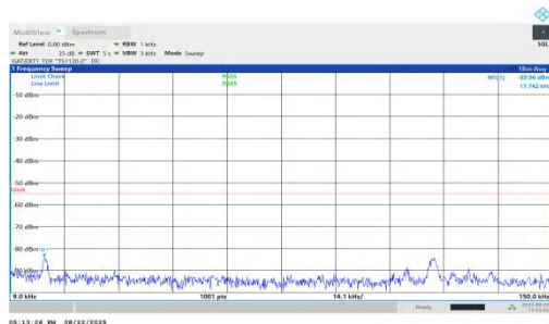
NTNV-n41-PC1.5-30-90-H-DFT-BPSK-Inner_1RB_Right-0.009-0. 15-PASS
