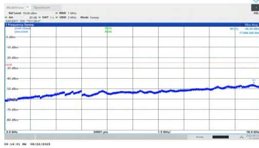
NTVN-n41-PC1.5-30-90-H-DFT-QPSK-Inner_1RB_Left-3000-18000-PASS
