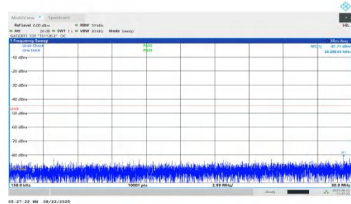
NTNV-n41-PC1.5-30-100-M-DFT-BPSK-Inner_1RB_Right-0.15-30-PASS
