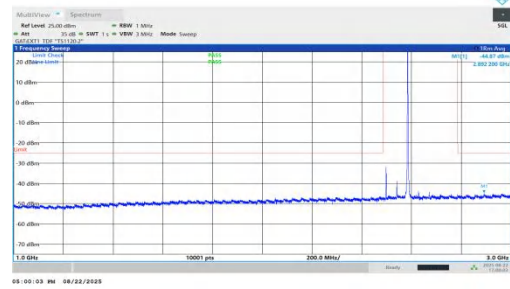
NTNV-n41-PC1.5-30-90-L-DFT-BPSK-Inner_1RB_Right-1000-300 0-PASS
