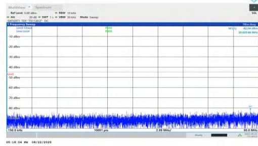
NTNV-n41-PC1.5-30-100-L-DFT-BPSK-Inner_1RB_Left-0.15-30-PASS
