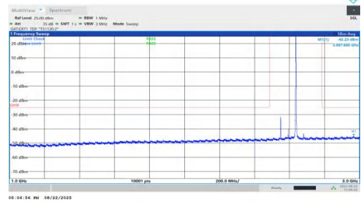
NTNV-n41-PC1.5-30-90-M-DFT-BPSK-Inner_1RB_Right-1000-3000-PASS
