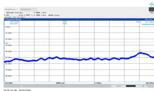
NTNV-n41-PC1.5-30-80-H-DFT-BPSK-Inner_1RB_Left-18000-30000-PASS
