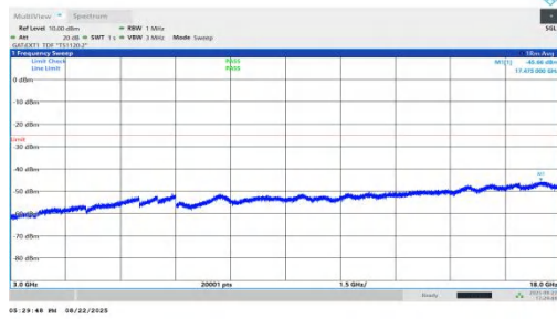
NTVN-n41-PC1.5-30-100-M-DFT-QPSK-Inner_1RB_Left-3000-18000-PASS
