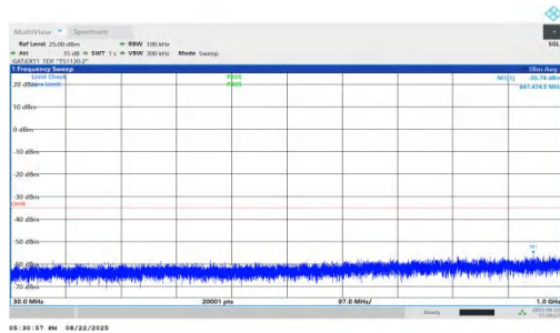
NTVN-n41-PC1.5-30-100-M-DFT-QPSK-Inner_1RB_Right-30.0-1000.0-PASS
