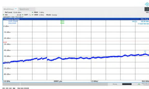
NTNV-n41-PC1.5-30-100-H-DFT-BPSK-Inner_1RB_Left-3000-18000-PASS
