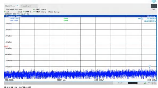
NTVN-n41-PC1.5-30-100-M-DFT-QPSK-Inner_1RB_Left-0.15-30- 00-PASS
