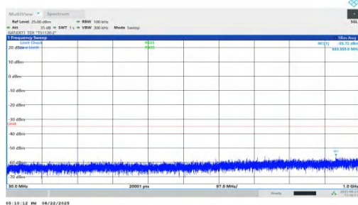
NTVN-n41-PC1.5-30-90-M-DFT-QPSK-Inner_1RB_Right-30-1000-PASS
