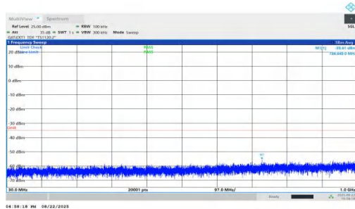
NTNV-n41-PC1.5-30-90-L-DFT-BPSK-Inner_1RB_Left-30-1000-P
