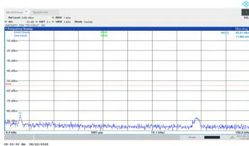
NTNV-n41-PC1.5-30-90-L-DFT-QPSK-Inner_1RB_Right-0.009-0.15-PASS
