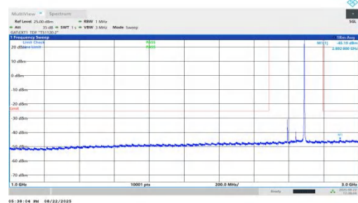
NTNV-n41-PC1.5-30-100-H-DFT-QPSK-Inner_1RB_Right-1000-3000-PASS
