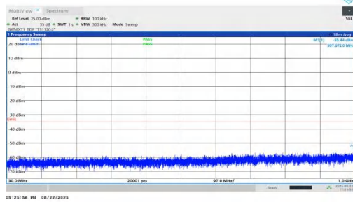
NTNV-n41-PC1.5-30-100-M-DFT-BPSK-Inner_1RB_Left-30-1000-PASS
