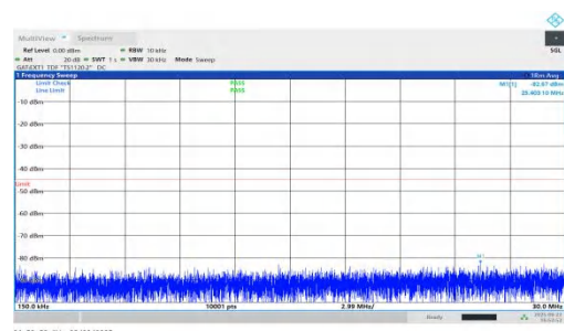
NTNV-n41-PC1.5-30-80-H-DFT-BPSK-Inner_1RB_Right-0.15-30-PASS
