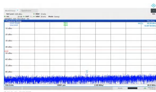
NTNV-n41-PC1.5-30-100-H-DFT-BPSK-Inner_1RB_Right-0.15-30-PASS
