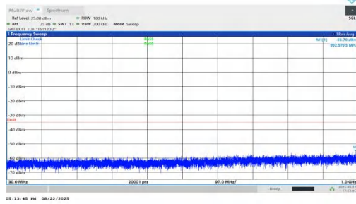
NTNV-n41-PC1.5-30-90-H-DFT-BPSK-Inner_1RB_Right-30-1000 -PASS
