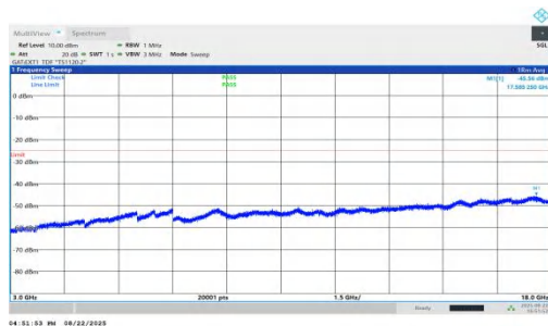
NTNV-n41-PC1.5-30-80-H-DFT-BPSK-Inner_1RB_Left-3000-18000-PASS
