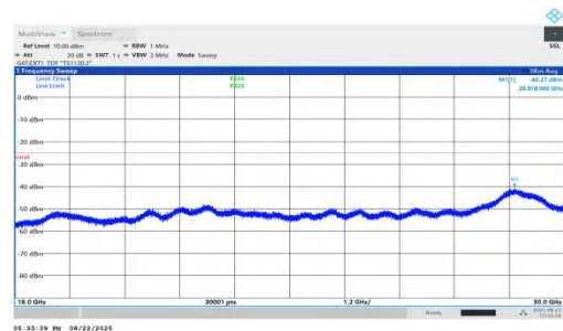
NTNV-n41-PC1.5-30-100-H-DFT-BPSK-Inner_1RB_Left-18000-30000-PASS
