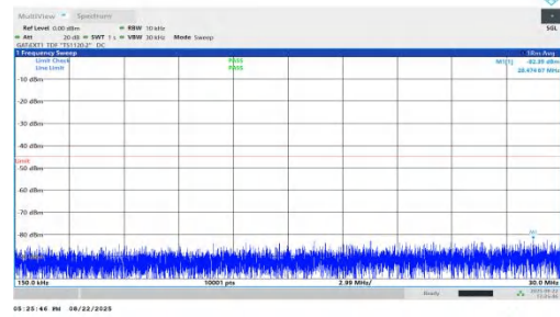
NTNV-n41-PC1.5-30-100-M-DFT-BPSK-Inner_1RB_Left-0.15-30-PASS
