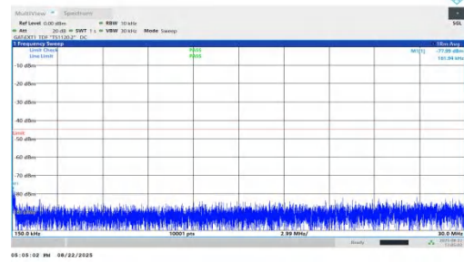
NTVN-n41-PC1.5-30-90-M-DFT-BPSK-Inner_1RB_Left-0.15-30-P ASS
