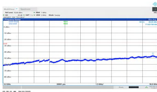
NTNV-n41-PC1.5-30-100-H-DFT-QPSK-Inner_1RB_Right-3000-18000-PASS
