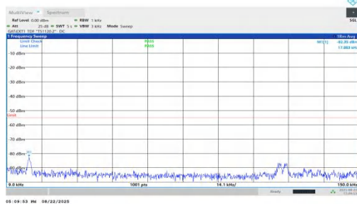
NTVN-n41-PC1.5-30-90-M-DFT-QPSK-Inner_1RB_Right-0.009-0.15-PASS
