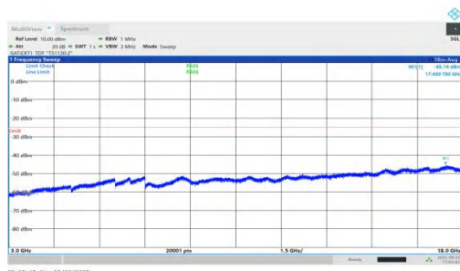
NTNV-n41-PC1.5-30-90-L-DFT-QPSK-Inner_1RB_Right-3000-18000-PASS
