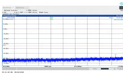
NTNV-n41-PC1.5-30-90-L-DFT-QPSK-Inner_1RB_Left-30-1000- PASS
