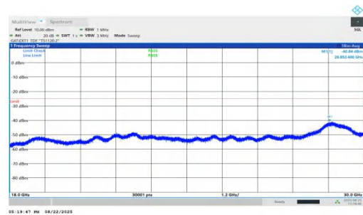
NTNV-n41-PC1.5-30-100-L-DFT-BPSK-Inner_1RB_Left-18000-30000-PASS
