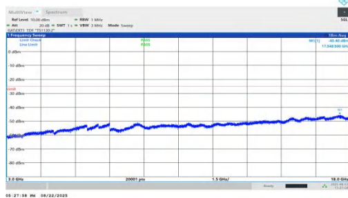
NTVN-n41-PC1.5-30-100-M-DFT-BPSK-Inner_1RB_Right-3000-1 8000-PASS
