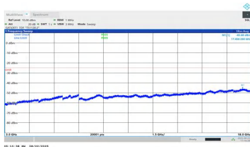
NTVN-n41-PC1.5-30-90-M-DFT-QPSK-Inner_1RB_Right-3000-18000-PASS
