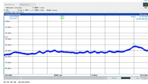
NTNV-n41-PC1.5-30-90-L-DFT-BPSK-Inner_1RB_Right-18000-30 000-PASS
