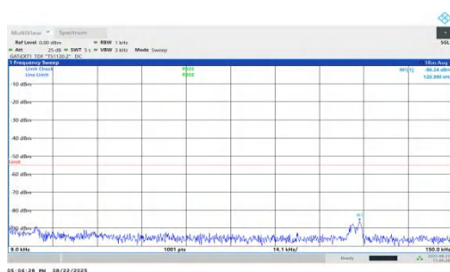
NTVN-n41-PC1.5-30-90-M-DFT-BPSK-Inner_1RB_Right-0.009-0. 15-PASS
