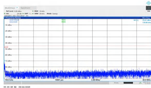
NTVN-n41-PC1.5-30-100-M-DFT-QPSK-Inner_1RB_Right-0.15-30.0-PASS
