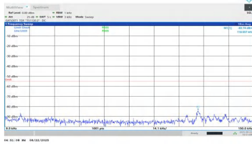
NTNV-n41-PC1.5-30-80-H-DFT-BPSK-Inner_1RB_Left-0.009-0.15-PASS
