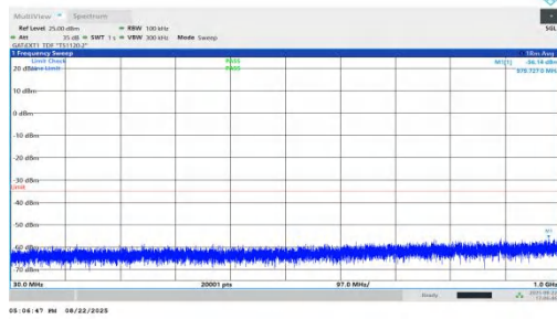
NTNV-n41-PC1.5-30-90-M-DFT-BPSK-Inner_1RB_Right-30-1000-PASS
