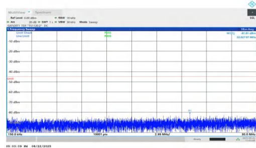
NTNV-n41-PC1.5-30-90-L-DFT-QPSK-Inner_1RB_Right-0.15-30-PASS
