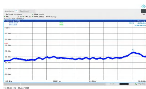
NTVN-n41-PC1.5-30-80-M-DFT-QPSK-Inner_1RB_Right-18000-30000-PASS
