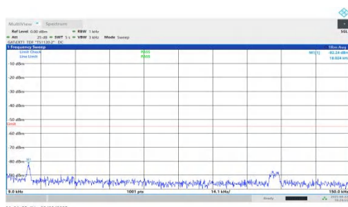
NTNV-n41-PC1.5-30-70-M-DFT-BPSK-Inner_1RB_Right-0.009-0. 15-PASS
