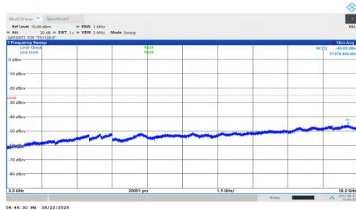
NTVN-n41-PC1.5-30-80-M-DFT-BPSK-Inner_1RB_Right-3000-18000-PASS
