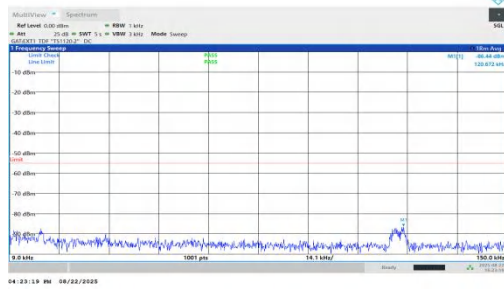
NTNV-n41-PC1.5-30-70-M-DFT-BPSK-Inner_1RB_Left-0.009-0.1 5-PASS
