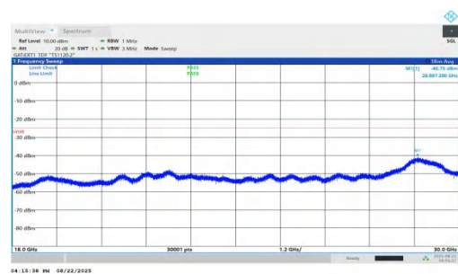
NTVN-n41-PC1.5-30-60-H-DFT-QPSK-Inner_1RB_Right-18000-30000-PASS
