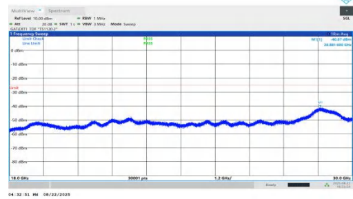
NTNV-n41-PC1.5-30-70-H-DFT-BPSK-Inner_1RB_Right-18000-30 000-PASS
