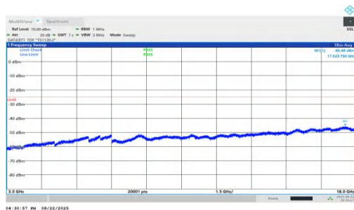
NTNV-n41-PC1.5-30-70-H-DFT-BPSK-Inner_1RB_Left-3000-180 00-PASS
