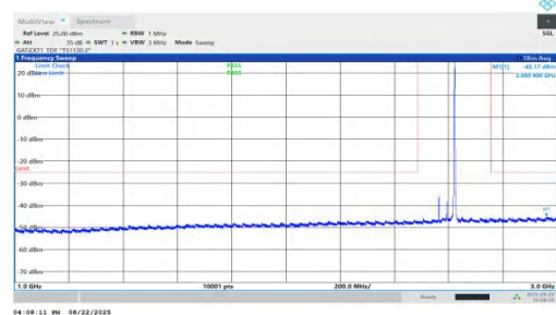
NTVN-n41-PC1.5-30-60-M-DFT-QPSK-Inner_1RB_Right-1000-3000-PASS
