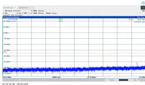
NTNV-n41-PC1.5-30-60-H-DFT-BPSK-Inner_1RB_Left-30-1000- PASS
