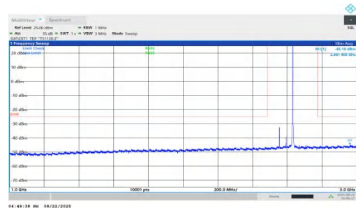
NTVN-n41-PC1.5-30-80-M-DFT-QPSK-Inner_1RB_Right-1000-3000-PASS
