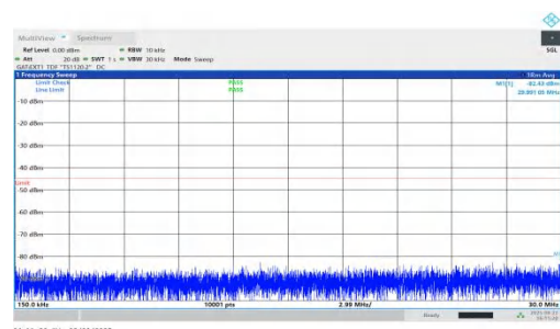
NTNV-n41-PC1.5-30-60-H-DFT-BPSK-Inner_1RB_Right-0.15-30- PASS
