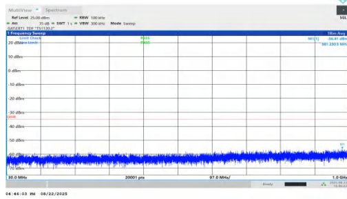
NTVN-n41-PC1.5-30-80-M-DFT-BPSK-Inner_1RB_Right-30-1000-PASS
