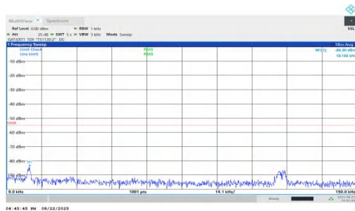
NTNV-n41-PC1.5-30-80-M-DFT-BPSK-Inner_1RB_Right-0.009-0. 15-PASS
