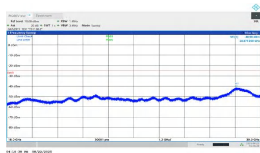
NTNV-n41-PC1.5-30-60-H-DFT-BPSK-Inner_1RB_Left-18000-300 00-PASS
