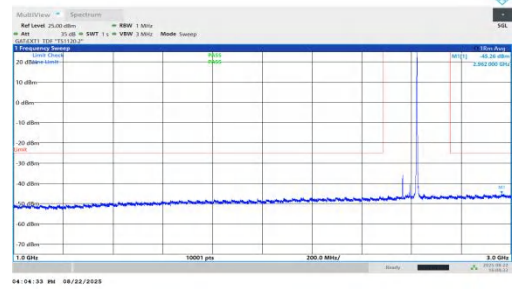
NTVN-n41-PC1.5-30-60-M-DFT-BPSK-Inner_1RB_Right-1000-30 00-PASS
