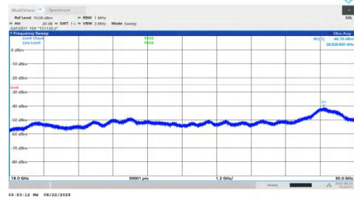
NTVN-n41-PC1.5-30-50-H-DFT-QPSK-Inner_1RB_Left-18000-30000-PASS
