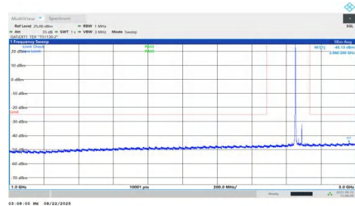
NTNV-n41-PC1.5-30-40-H-DFT-BPSK-Inner_1RB_Left-1000-3000 -PASS
