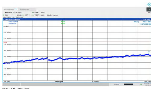
NTNV-n41-PC1.5-30-40-H-DFT-QPSK-Inner_1RB_Right-3000-18000-PASS
