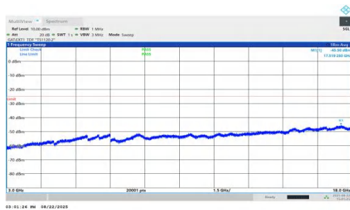
NTNV-n41-PC1.5-30-40-M-DFT-BPSK-Inner_1RB_Left-3000-180 00-PASS
