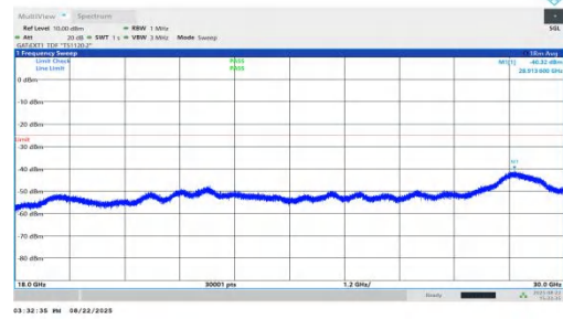
NTVN-n41-PC1.5-30-45-H-DFT-QPSK-Inner_1RB_Left-18000-30000-PASS
