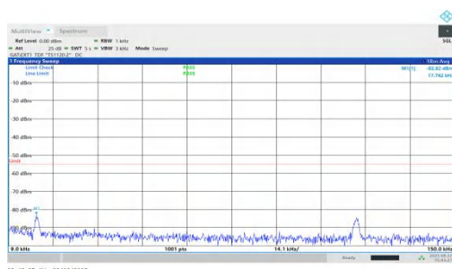
NTVN-n41-PC1.5-30-50-M-DFT-BPSK-Inner_1RB_Right-0.009-0. 15-PASS
