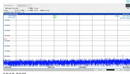
NTVN-n41-PC1.5-30-50-M-DFT-QPSK-Inner_1RB_Left-0.15-30-PASS
