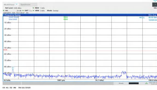
NTVN-n41-PC1.5-30-50-M-DFT-BPSK-Inner_1RB_Left-0.009-0.1 5-PASS
