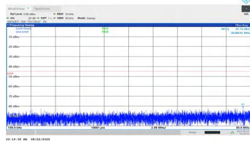
NTNV-n41-PC1.5-30-45-L-DFT-QPSK-Inner_1RB_Right-0.15-30-PASS
