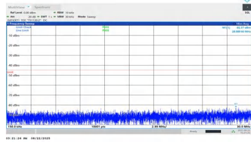
NTVN-n41-PC1.5-30-45-M-DFT-BPSK-Inner_1RB_Left-0.15-30-P ASS
