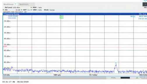
NTVN-n41-PC1.5-30-45-M-DFT-BPSK-Inner_1RB_Left-0.009-0.1 5-PASS
