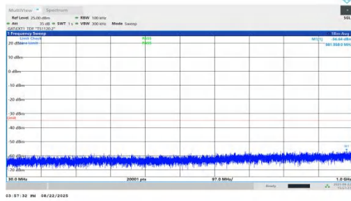
NTNV-n41-PC1.5-30-60-L-DFT-BPSK-Inner_1RB_Right-30-1000 -PASS
