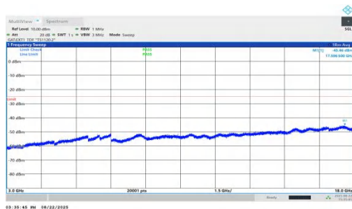
NTNV-n41-PC1.5-30-50-L-DFT-BPSK-Inner_1RB_Left-3000-18000-PASS
