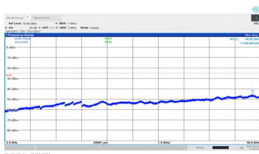
NTNV-n41-PC1.5-30-50-L-DFT-QPSK-Inner_1RB_Right-3000-18000-PASS
