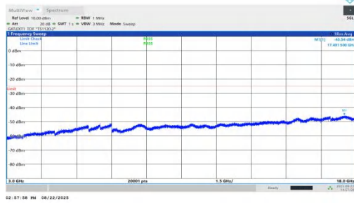
NTNV-n41-PC1.5-30-40-L-DFT-QPSK-Inner_1RB_Left-3000-18000-PASS
