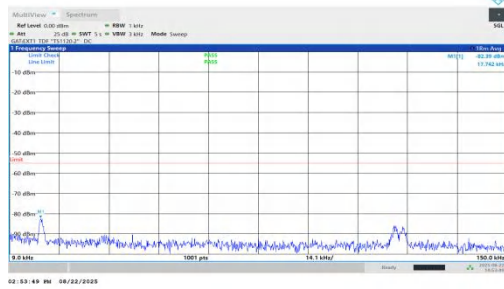
NTNV-n41-PC1.5-30-40-L-DFT-BPSK-Inner_1RB_Left-0.009-0.1 5-PASS
