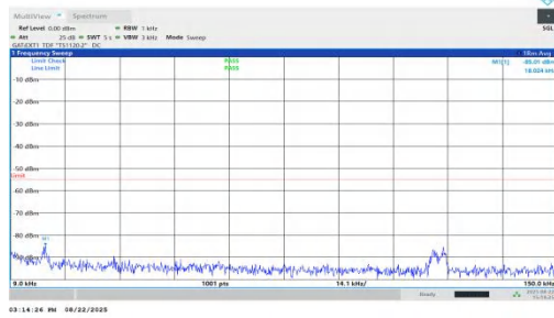
NTNV-n41-PC1.5-30-45-L-DFT-BPSK-Inner_1RB_Left-0.009-0.15-PASS
