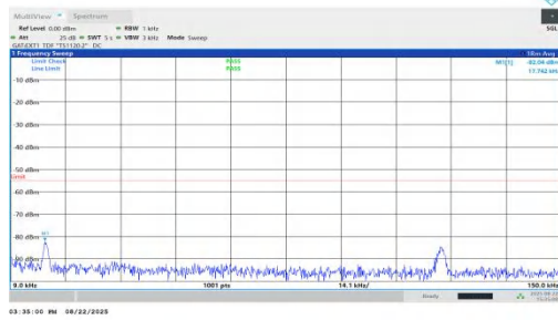
NTNV-n41-PC1.5-30-50-L-DFT-BPSK-Inner_1RB_Left-0.009-0.15-PASS
