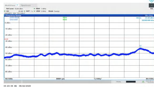
NTVN-n41-PC1.5-30-45-M-DFT-BPSK-Inner_1RB_Right-18000-30000-PASS
