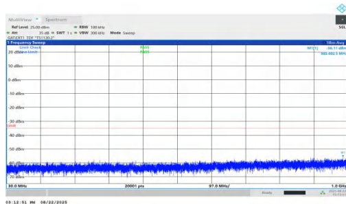
NTNV-n41-PC1.5-30-40-H-DFT-QPSK-Inner_1RB_Right-30-1000-PASS
