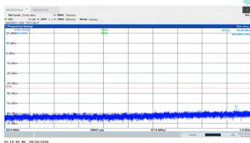
NTNV-n41-PC1.5-30-45-L-DFT-QPSK-Inner_1RB_Right-30-1000-PASS
