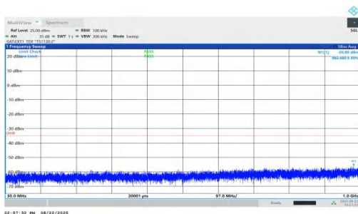
NTNV-n41-PC1.5-30-40-L-DFT-QPSK-Inner_1RB_Left-30-1000-PASS
