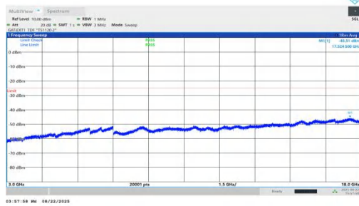
NTNV-n41-PC1.5-30-60-L-DFT-BPSK-Inner_1RB_Right-3000-18 000-PASS
