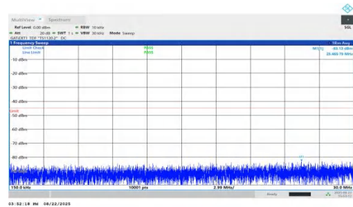
NTNV-n41-PC1.5-30-50-H-DFT-QPSK-Inner_1RB_Left-0.15-30-P ASS
