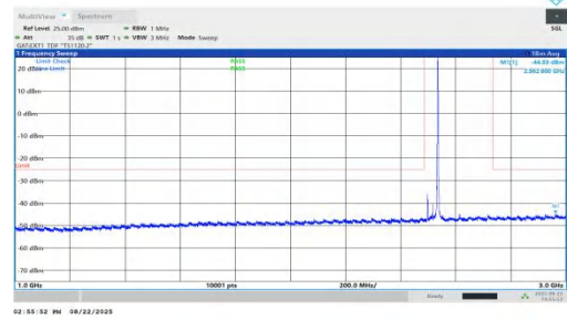
NTNV-n41-PC1.5-30-40-L-DFT-BPSK-Inner_1RB_Right-1000-300-PASS
