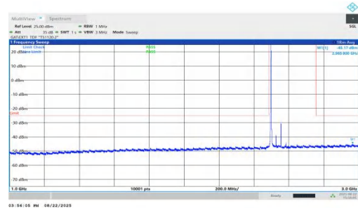
NTNV-n41-PC1.5-30-60-L-DFT-BPSK-Inner_1RB_Left-1000-3000-PASS
