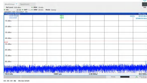
NTNV-n41-PC1.5-30-50-L-DFT-BPSK-Inner_1RB_Left-0.15-30-PA-SS
