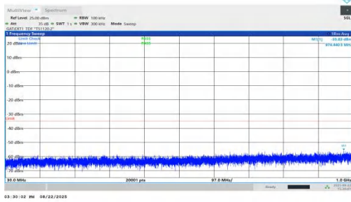
NTNV-n41-PC1.5-30-45-H-DFT-BPSK-Inner_1RB_Right-30-1000 -PASS
