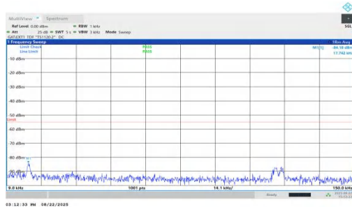
NTNV-n41-PC1.5-30-40-H-DFT-QPSK-Inner_1RB_Right-0.009-0.15-PASS
