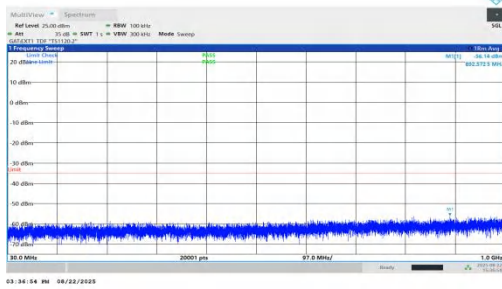
NTNV-n41-PC1.5-30-50-L-DFT-BPSK-Inner_1RB_Right-30-1000 -PASS
