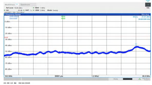
NTNV-n41-PC1.5-30-60-L-DFT-BPSK-Inner_1RB_Right-18000-30 000-PASS
