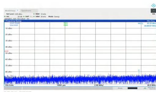
NTNV-n41-PC1.5-30-60-L-DFT-BPSK-Inner_1RB_Right-0.15-30-PA-ASS
