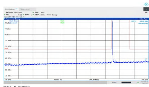
NTNV-n41-PC1.5-30-40-L-DFT-QPSK-Inner_1RB_Left-1000-3000-PASS
