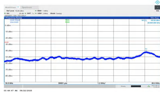
NTNV-n41-PC1.5-30-50-H-DFT-BPSK-Inner_1RB_Left-18000-300 00-PASS
