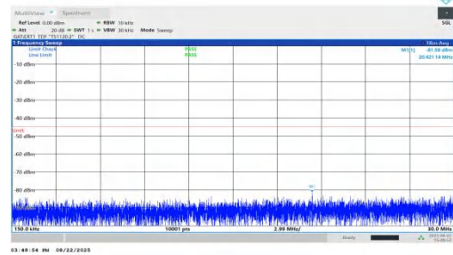
NTNV-n41-PC1.5-30-50-H-DFT-BPSK-Inner_1RB_Left-0.15-30-P ASS
