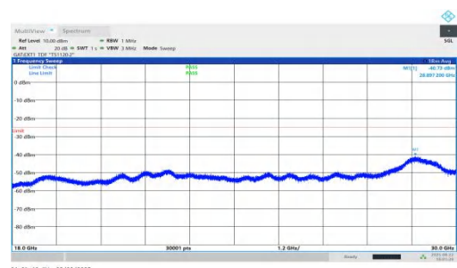
NTNV-n41-PC1.5-30-60-L-DFT-QPSK-Inner_1RB_Right-18000-30000-PASS
