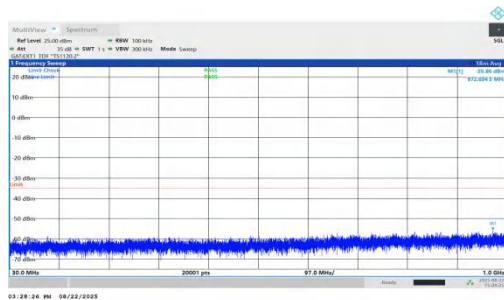
NTNV-n41-PC1.5-30-45-H-DFT-BPSK-Inner_1RB_Left-30-1000- PASS
