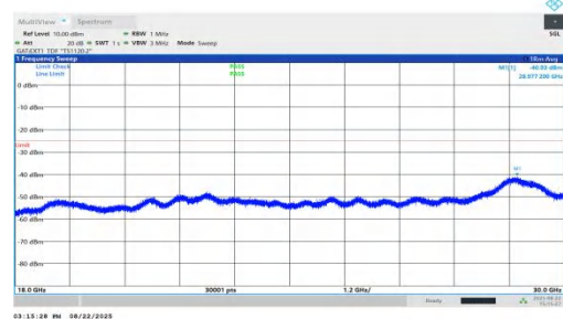
NTNV-n41-PC1.5-30-45-L-DFT-BPSK-Inner_1RB_Left-18000-30000-PASS
