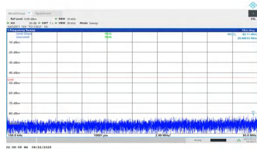
NTNV-n41-PC1.5-30-40-L-DFT-QPSK-Inner_1RB_Right-0.15-0.30-PASS
