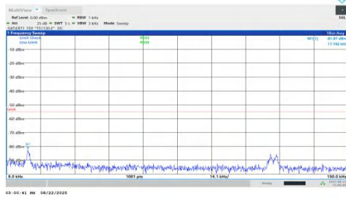
NTNV-n41-PC1.5-30-40-M-DFT-BPSK-Inner_1RB_Left-0.009-0.1 5-PASS
