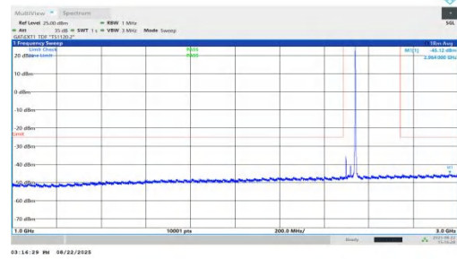
NTNV-n41-PC1.5-30-45-L-DFT-BPSK-Inner_1RB_Right-1000-300 0-PASS
