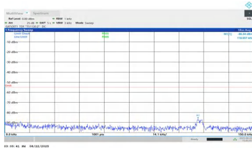
NTVN-n41-PC1.5-30-40-M-DFT-QPSK-Inner_1RB_Right-0.009-0.15-PASS
