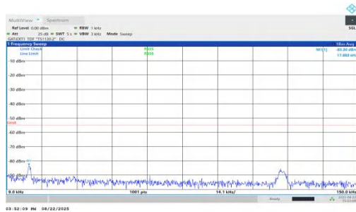
NTNV-n41-PC1.5-30-50-H-DFT-QPSK-Inner_1RB_Left-0.009-0.1 5-PASS
