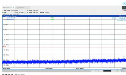
NTVN-n41-PC1.5-30-50-H-DFT-QPSK-Inner_1RB_Right-30-1000-PASS
