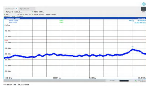
NTNV-n41-PC1.5-30-45-H-DFT-BPSK-Inner_1RB_Left-18000-300 00-PASS
