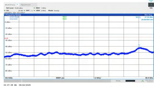
NTNV-n41-PC1.5-30-50-L-DFT-BPSK-Inner_1RB_Right-18000-30000 000-PASS
