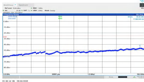
NTVN-n41-PC1.5-30-50-M-DFT-BPSK-Inner_1RB_Right-3000-18000-PASS
