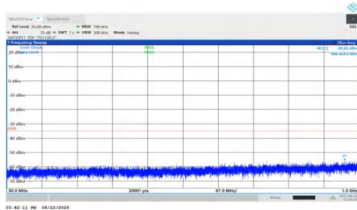
NTVN-n41-PC1.5-30-50-M-DFT-BPSK-Inner_1RB_Left-30-1000- PASS
