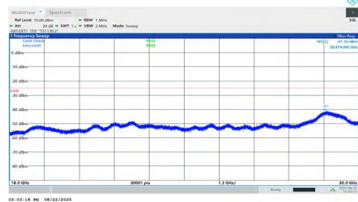
NTVN-n41-PC1.5-30-40-M-DFT-BPSK-Inner_1RB_Right-18000-30000-PASS
