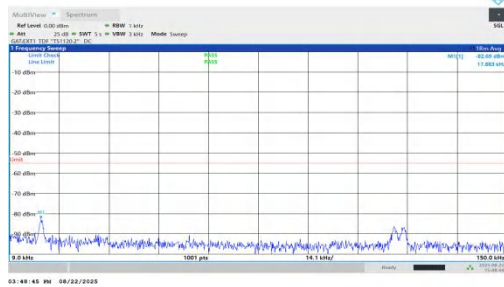
NTNV-n41-PC1.5-30-50-H-DFT-BPSK-Inner_1RB_Left-0.009-0.1 5-PASS
