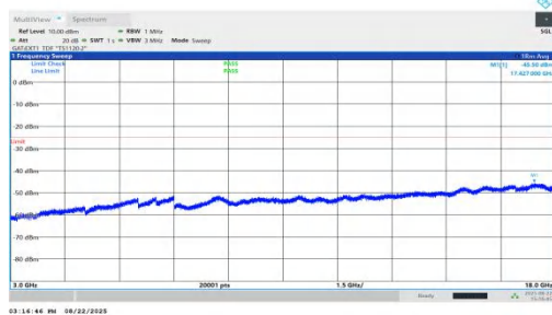
NTNV-n41-PC1.5-30-45-L-DFT-BPSK-Inner_1RB_Right-3000-18 000-PASS
