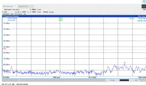
NTNV-n41-PC1.5-30-40-L-DFT-QPSK-Inner_1RB_Left-0.009-0.15-PASS
