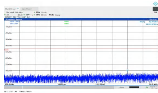
NTNV-n41-PC1.5-30-40-H-DFT-QPSK-Inner_1RB_Left-0.15-30-P ASS
