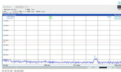
NTNV-n41-PC1.5-30-60-L-DFT-QPSK-Inner_1RB_Left-0.009-0.1 5-PASS
