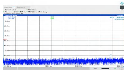
NTNV-n41-PC1.5-30-45-L-DFT-BPSK-Inner_1RB_Right-0.15-30-PA-ASS
