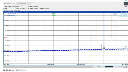
NTVN-n41-PC1.5-30-40-M-DFT-BPSK-Inner_1RB_Right-1000-3000-PASS
