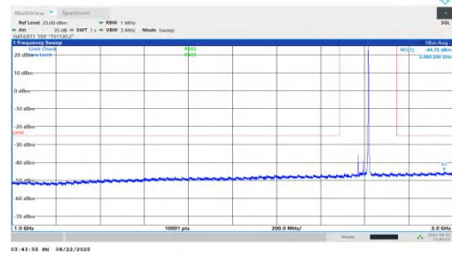
NTVN-n41-PC1.5-30-50-M-DFT-BPSK-Inner_1RB_Right-1000-3000-PASS
