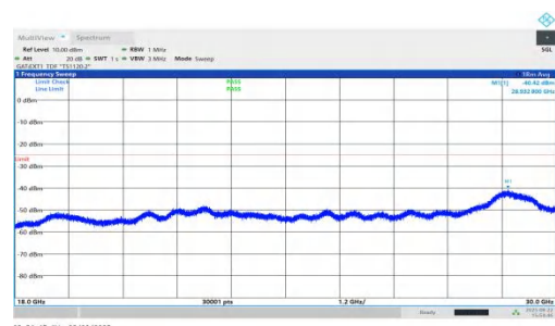
NTVN-n41-PC1.5-30-50-H-DFT-QPSK-Inner_1RB_Right-18000-30000-PASS
