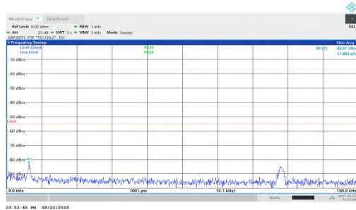
NTVN-n41-PC1.5-30-50-H-DFT-QPSK-Inner_1RB_Right-0.009-0.15-PASS
