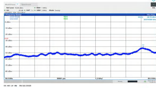
NTVN-n41-PC1.5-30-50-M-DFT-QPSK-Inner_1RB_Left-18000-30000-PASS
