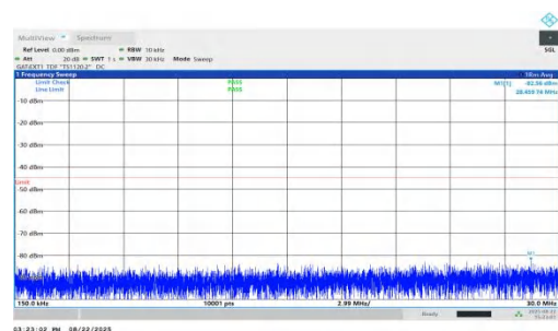
NTVN-n41-PC1.5-30-45-M-DFT-BPSK-Inner_1RB_Right-0.15-30- PASS
