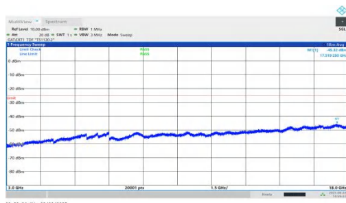
NTNV-n41-PC1.5-30-40-L-DFT-QPSK-Inner_1RB_Right-3000-18000-PASS
