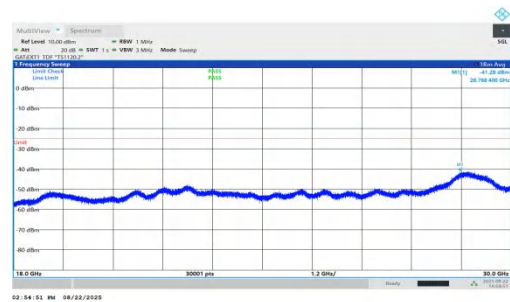
NTNV-n41-PC1.5-30-40-L-DFT-BPSK-Inner_1RB_Left-18000-300 00-PASS
