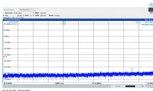
NTNV-n41-PC1.5-30-45-L-DFT-QPSK-Inner_1RB_Left-30-1000- PASS
