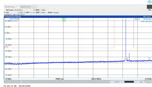
NTNV-n41-PC1.5-30-50-H-DFT-BPSK-Inner_1RB_Left-1000-3000 -PASS
