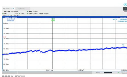
NTVN-n41-PC1.5-30-45-H-DFT-QPSK-Inner_1RB_Right-3000-18000-PASS
