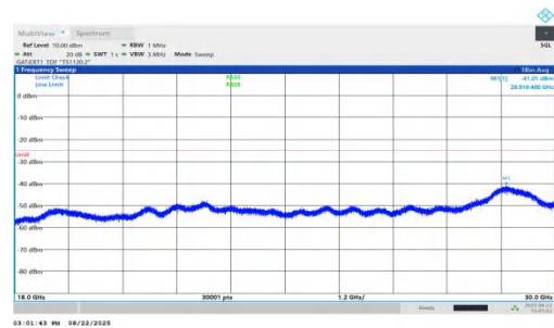
NTNV-n41-PC1.5-30-40-M-DFT-BPSK-Inner_1RB_Left-18000-300 00-PASS
