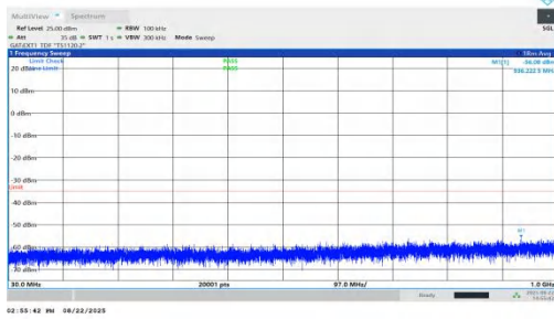
NTNV-n41-PC1.5-30-40-L-DFT-BPSK-Inner_1RB_Right-30-1000-PASS
