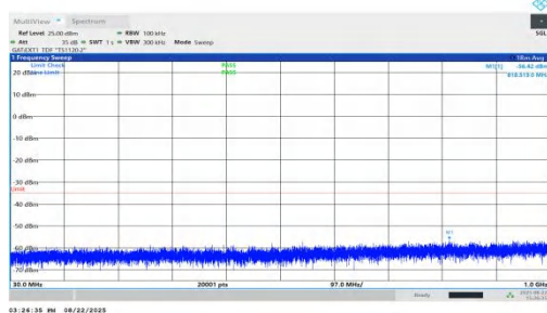
NTVN-n41-PC1.5-30-45-M-DFT-QPSK-Inner_1RB_Right-30-1000-PASS
