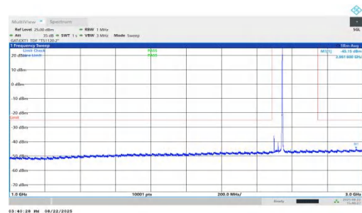
NTNV-n41-PC1.5-30-50-L-DFT-QPSK-Inner_1RB_Right-1000-3000-PASS
