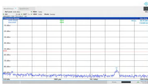
NTNV-n41-PC1.5-30-45-L-DFT-BPSK-Inner_1RB_Right-0.009-0.15-PASS
