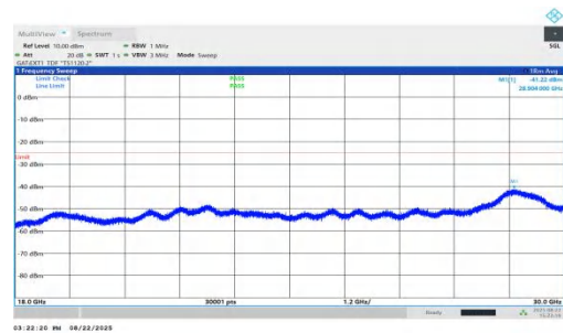
NTVN-n41-PC1.5-30-45-M-DFT-BPSK-Inner_1RB_Left-18000-300 00-PASS
