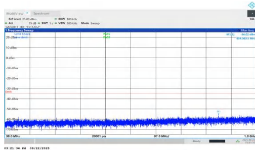
NTVN-n41-PC1.5-30-45-M-DFT-BPSK-Inner_1RB_Left-30-1000- PASS
