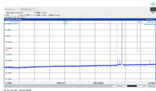
NTNV-n41-PC1.5-30-60-L-DFT-QPSK-Inner_1RB_Right-1000-3000-PASS
