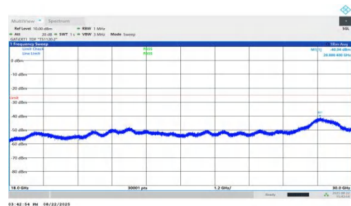
NTVN-n41-PC1.5-30-50-M-DFT-BPSK-Inner_1RB_Left-18000-300 00-PASS
