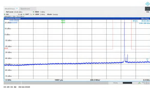
NTNV-n41-PC1.5-30-45-H-DFT-BPSK-Inner_1RB_Left-1000-3000 -PASS
