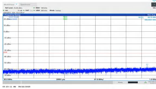
NTVN-n41-PC1.5-30-45-M-DFT-BPSK-Inner_1RB_Right-30-1000-PASS
