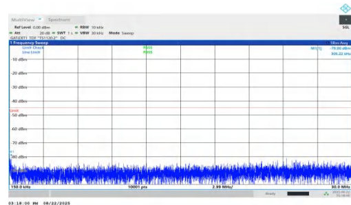
NTNV-n41-PC1.5-30-45-L-DFT-QPSK-Inner_1RB_Left-0.15-30-PA SS
