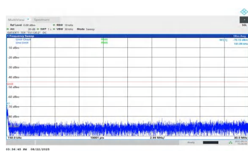
NTNV-n41-PC1.5-30-50-L-DFT-BPSK-Inner_1RB_Right-0.15-30-PA-ASS
