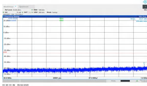
NTNV-n41-PC1.5-30-50-H-DFT-BPSK-Inner_1RB_Left-30-1000- PASS
