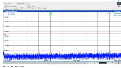
NTNV-n41-PC1.5-30-45-H-DFT-BPSK-Inner_1RB_Left-0.15-30-P ASS
