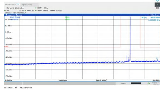
NTVN-n41-PC1.5-30-45-M-DFT-BPSK-Inner_1RB_Right-1000-3000-PASS
