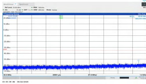
NTNV-n41-PC1.5-30-50-H-DFT-BPSK-Inner_1RB_Right-30-1000 -PASS
