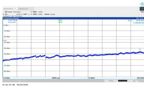
NTVN-n41-PC1.5-30-45-M-DFT-BPSK-Inner_1RB_Left-3000-180 00-PASS
