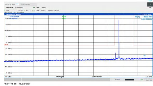
NTNV-n41-PC1.5-30-50-L-DFT-BPSK-Inner_1RB_Right-1000-300 0-PASS
