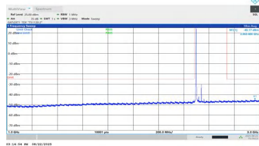
NTNV-n41-PC1.5-30-45-L-DFT-BPSK-Inner_1RB_Left-1000-3000-PASS
