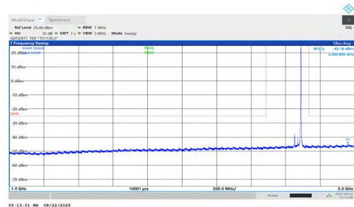
NTNV-n41-PC1.5-30-40-H-DFT-QPSK-Inner_1RB_Right-1000-3000-PASS
