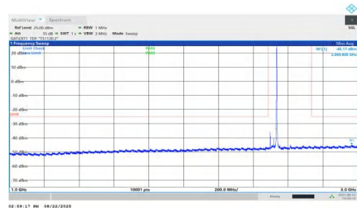
NTNV-n41-PC1.5-30-40-L-DFT-QPSK-Inner_1RB_Right-1000-3000-PASS
