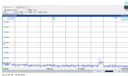
NTNV-n41-PC1.5-30-40-H-DFT-QPSK-Inner_1RB_Left-0.009-0.1 5-PASS
