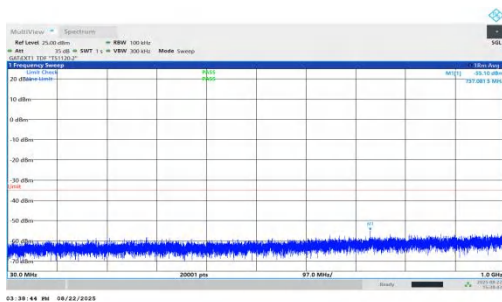
NTNV-n41-PC1.5-30-50-L-DFT-QPSK-Inner_1RB_Left-30-1000 PASS
