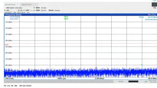
NTNV-n41-PC1.5-30-45-L-DFT-BPSK-Inner_1RB_Left-0.15-30-PA-SS
