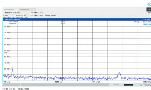
NTNV-n41-PC1.5-30-50-H-DFT-BPSK-Inner_1RB_Right-0.009-0. 15-PASS
