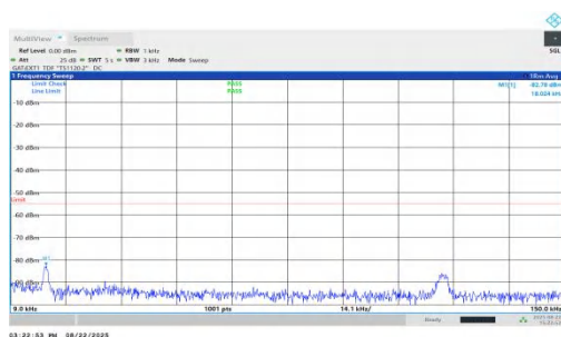
NTVN-n41-PC1.5-30-45-M-DFT-BPSK-Inner_1RB_Right-0.009-0. 15-PASS
