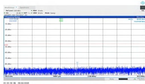
NTVN-n41-PC1.5-30-50-H-DFT-QPSK-Inner_1RB_Right-0.15-30-PASS
