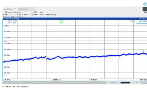
NTNV-n41-PC1.5-30-45-H-DFT-BPSK-Inner_1RB_Left-3000-180 00-PASS
