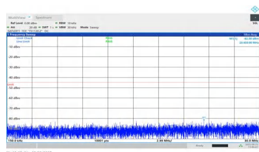
NTNV-n41-PC1.5-30-25-M-DFT-BPSK-Inner_1RB_Right-0.15-30- PASS
