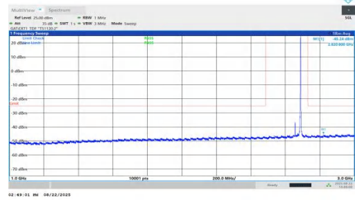
NTNV-n41-PC1.5-30-35-H-DFT-BPSK-Inner_1RB_Right-1000-300 0-PASS
