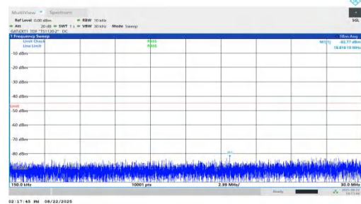
NTNV-n41-PC1.5-30-30-L-DFT-QPSK-Inner_1RB_Right-0.15-30-PASS
