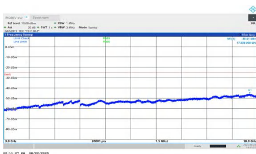
NTVN-n41-PC1.5-30-25-H-DFT-QPSK-Inner_1RB_Right-3000-18000-PASS
