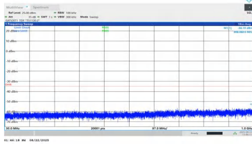
NTVN-n41-PC1.5-30-25-M-DFT-BPSK-Inner_1RB_Right-30-1000-PASS
