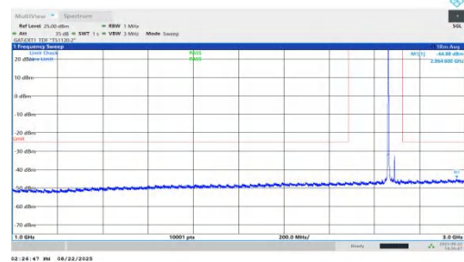
NTNV-n41-PC1.5-30-30-H-DFT-BPSK-Inner_1RB_Left-1000-3000 -PASS
