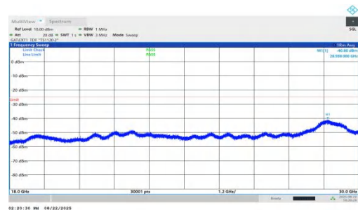
NTNV-n41-PC1.5-30-30-M-DFT-BPSK-Inner_1RB_Left-18000-300 00-PASS
