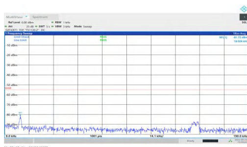
NTNV-n41-PC1.5-30-25-L-DFT-BPSK-Inner_1RB_Right-0.009-0.15-PASS
