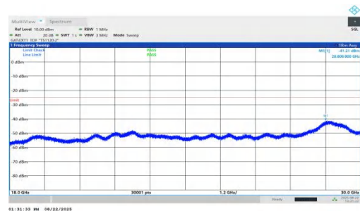
NTNV-n41-PC1.5-30-20-H-DFT-BPSK-Inner_1RB_Left-18000-300 00-PASS
