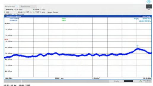
NTNV-n41-PC1.5-30-30-L-DFT-BPSK-Inner_1RB_Left-18000-30000-PASS
