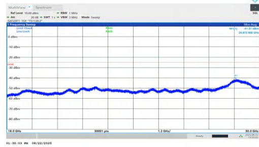
NTVN-n41-PC1.5-30-20-H-DFT-QPSK-Inner_1RB_Left-18000-30000-PASS
