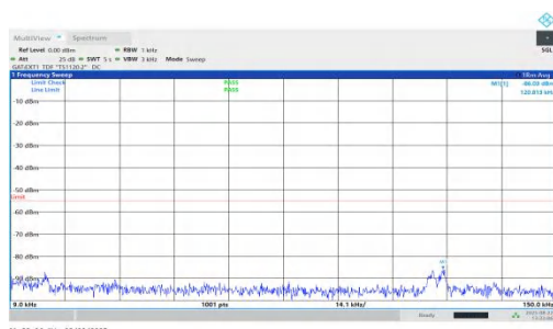
NTNV-n41-PC1.5-30-20-H-DFT-BPSK-Inner_1RB_Right-0.009-0. 15-PASS
