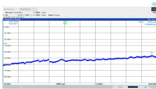
NTNV-n41-PC1.5-30-30-L-DFT-QPSK-Inner_1RB_Right-3000-18000-PASS
