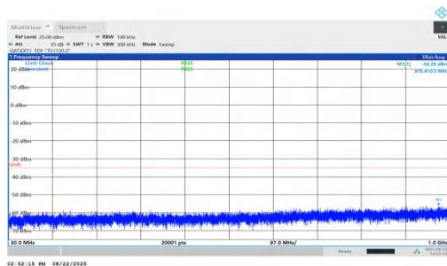
NTNV-n41-PC1.5-30-35-H-DFT-QPSK-Inner_1RB_Right-30-1000-PASS
