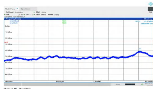
NTNV-n41-PC1.5-30-35-L-DFT-QPSK-Inner_1RB_Right-18000-30000-PASS
