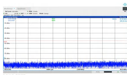
NTNV-n41-PC1.5-30-25-L-DFT-BPSK-Inner_1RB_Right-0.15-30-PA-ASS
