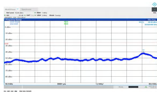
NTNV-n41-PC1.5-30-25-M-DFT-BPSK-Inner_1RB_Left-18000-300 00-PASS
