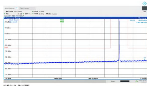
NTNV-n41-PC1.5-30-35-M-DFT-QPSK-Inner_1RB_Right-1000-3000-PASS
