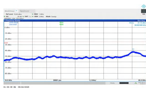
NTVN-n41-PC1.5-30-20-H-DFT-QPSK-Inner_1RB_Right-18000-30000-PASS
