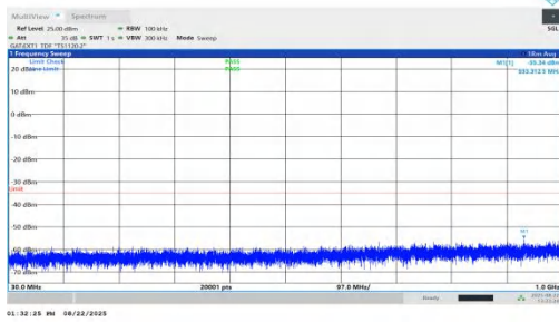
NTVN-n41-PC1.5-30-20-H-DFT-BPSK-Inner_1RB_Right-30-1000 -PASS
