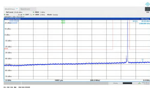
NTVN-n41-PC1.5-30-20-H-DFT-QPSK-Inner_1RB_Right-1000-3000-PASS
