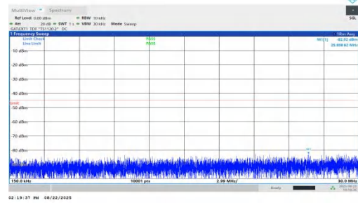
NTNV-n41-PC1.5-30-30-M-DFT-BPSK-Inner_1RB_Left-0.15-30-P ASS
