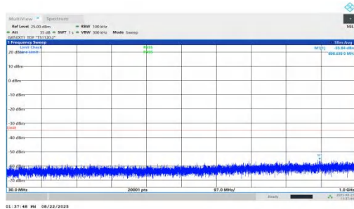
NTNV-n41-PC1.5-30-25-L-DFT-BPSK-Inner_1RB_Left-30-1000-PASS
