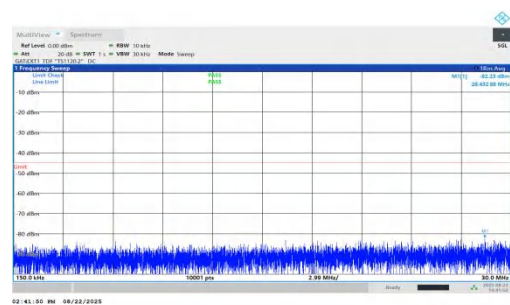
NTNV-n41-PC1.5-30-35-M-DFT-BPSK-Inner_1RB_Right-0.15-30- PASS
