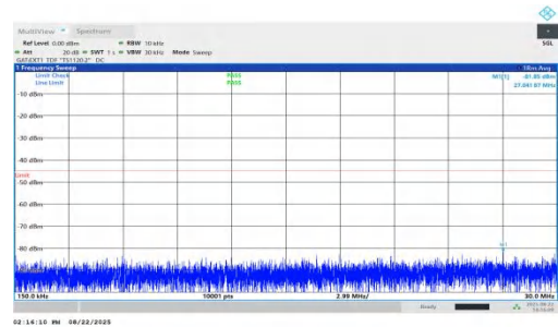
NTNV-n41-PC1.5-30-30-L-DFT-QPSK-Inner_1RB_Left-0.15-30-PA SS
