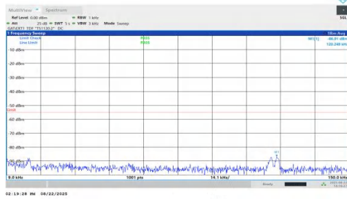
NTNV-n41-PC1.5-30-30-M-DFT-BPSK-Inner_1RB_Left-0.009-0.1 5-PASS
