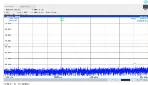
NTNV-n41-PC1.5-30-30-H-DFT-QPSK-Inner_1RB_Right-0.15-30-PASS
