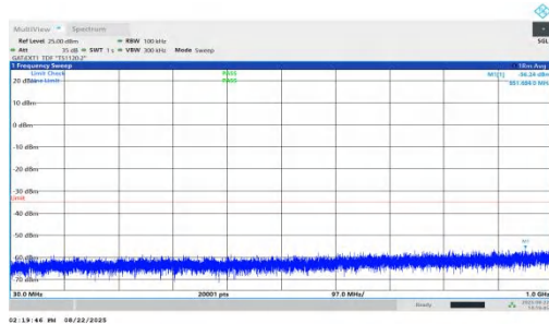
NTNV-n41-PC1.5-30-30-M-DFT-BPSK-Inner_1RB_Left-30-1000- PASS
