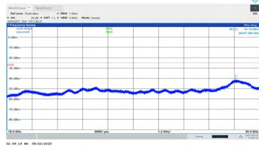
NTNV-n41-PC1.5-30-25-H-DFT-BPSK-Inner_1RB_Right-18000-30 000-PASS
