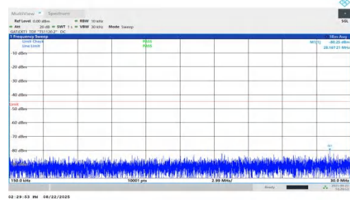
NTNV-n41-PC1.5-30-30-H-DFT-QPSK-Inner_1RB_Left-0.15-30-P ASS
