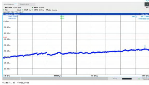
NTNV-n41-PC1.5-30-25-L-DFT-QPSK-Inner_1RB_Left-3000-18000-PASS
