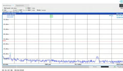
NTNV-n41-PC1.5-30-30-H-DFT-QPSK-Inner_1RB_Right-0.009-0.15-PASS
