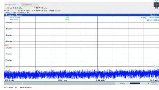
NTNV-n41-PC1.5-30-35-H-DFT-BPSK-Inner_1RB_Left-0.15-30-P ASS
