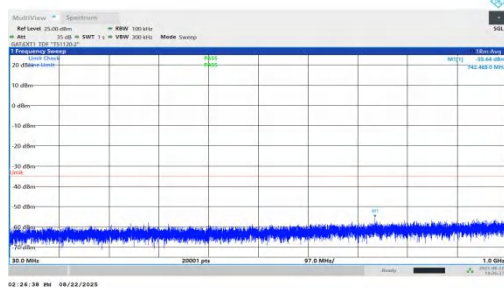
NTNV-n41-PC1.5-30-30-H-DFT-BPSK-Inner_1RB_Left-30-1000- PASS
