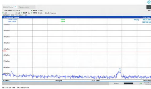
NTVN-n41-PC1.5-30-20-H-DFT-QPSK-Inner_1RB_Left-0.009-0.1 5-PASS
