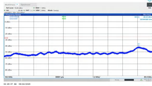
NTNV-n41-PC1.5-30-30-H-DFT-BPSK-Inner_1RB_Right-18000-30 000-PASS
