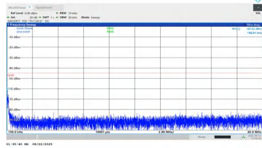
NTNV-n41-PC1.5-30-20-H-DFT-BPSK-Inner_1RB_Left-0.15-30-P ASS
