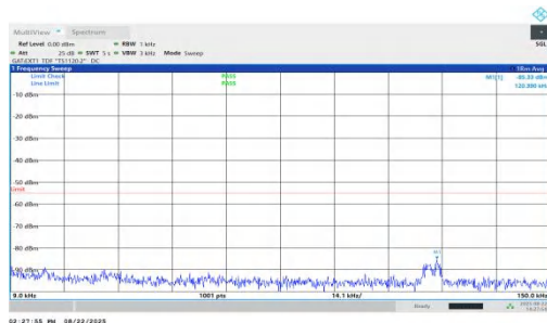
NTNV-n41-PC1.5-30-30-H-DFT-BPSK-Inner_1RB_Right-0.009-0. 15-PASS
