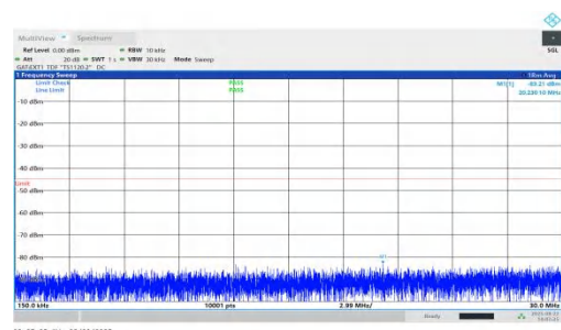
NTNV-n41-PC1.5-30-25-H-DFT-BPSK-Inner_1RB_Right-0.15-30- PASS
