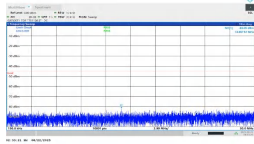
NTNV-n41-PC1.5-30-35-L-DFT-BPSK-Inner_1RB_Left-0.15-30-PA-SS
