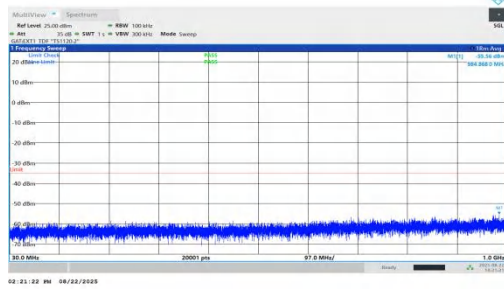
NTVN-n41-PC1.5-30-30-M-DFT-BPSK-Inner_1RB_Right-30-1000-PASS
