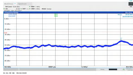
NTNV-n41-PC1.5-30-25-L-DFT-QPSK-Inner_1RB_Left-18000-30000-PASS
