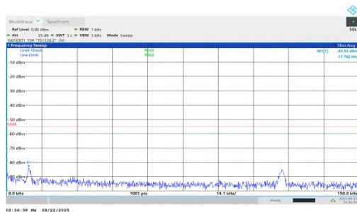
NTNV-n41-PC1.5-30-35-L-DFT-QPSK-Inner_1RB_Left-0.009-0.1 5-PASS
