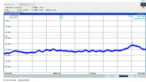
NTVN-n41-PC1.5-30-20-H-DFT-BPSK-Inner_1RB_Right-18000-30 000-PASS
