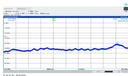
NTNV-n41-PC1.5-30-30-H-DFT-QPSK-Inner_1RB_Right-18000-30000-PASS
