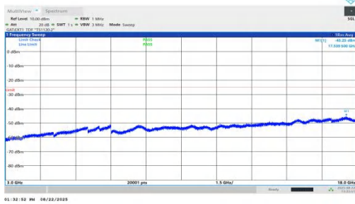
NTVN-n41-PC1.5-30-20-H-DFT-BPSK-Inner_1RB_Right-3000-18 000-PASS
