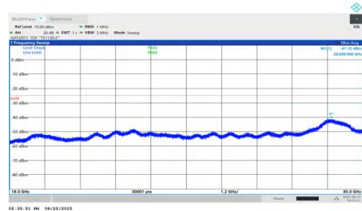
NTNV-n41-PC1.5-30-35-L-DFT-BPSK-Inner_1RB_Right-18000-30 000-PASS
