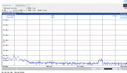
NTNV-n41-PC1.5-30-35-H-DFT-QPSK-Inner_1RB_Left-0.009-0.1 5-PASS
