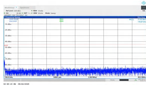
NTNV-n41-PC1.5-30-35-M-DFT-QPSK-Inner_1RB_Right-0.15-30-PASS
