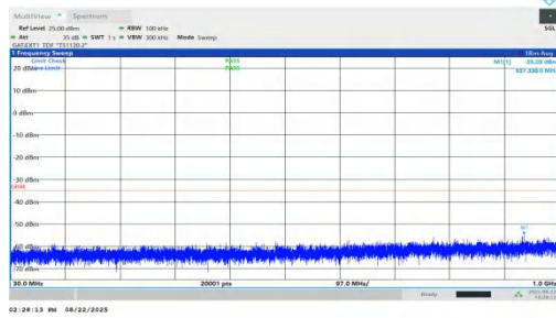
NTNV-n41-PC1.5-30-30-H-DFT-BPSK-Inner_1RB_Right-30-1000 -PASS
