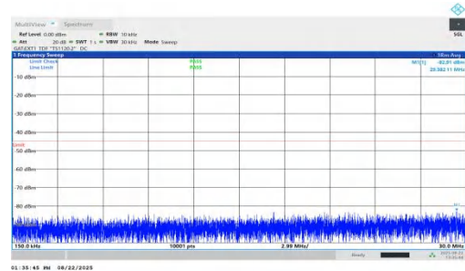
NTVN-n41-PC1.5-30-20-H-DFT-QPSK-Inner_1RB_Right-0.15-30-PASS
