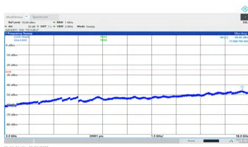
NTVN-n41-PC1.5-30-25-M-DFT-QPSK-Inner_1RB_Right-3000-18000-PASS
