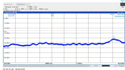
NTNV-n41-PC1.5-30-35-H-DFT-BPSK-Inner_1RB_Right-18000-30 000-PASS
