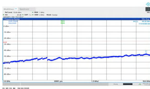
NTNV-n41-PC1.5-30-25-M-DFT-BPSK-Inner_1RB_Left-3000-180 00-PASS
