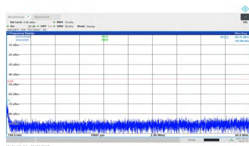
NTNV-n41-PC1.5-30-30-M-DFT-BPSK-Inner_1RB_Right-0.15-30- PASS
