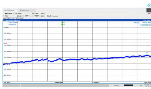
NTNV-n41-PC1.5-30-35-H-DFT-QPSK-Inner_1RB_Right-3000-18000-PASS
