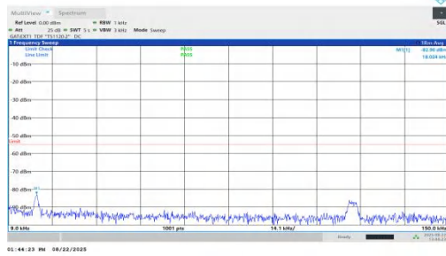
NTNV-n41-PC1.5-30-25-M-DFT-BPSK-Inner_1RB_Left-0.009-0.1 5-PASS
