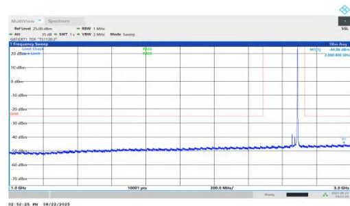
NTNV-n41-PC1.5-30-35-H-DFT-QPSK-Inner_1RB_Right-1000-3000-PASS
