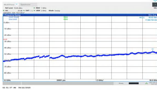
NTNV-n41-PC1.5-30-35-H-DFT-QPSK-Inner_1RB_Left-3000-18000-PASS
