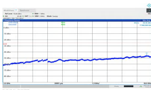
NTNV-n41-PC1.5-30-25-L-DFT-QPSK-Inner_1RB_Right-3000-18000-PASS
