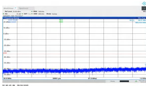
NTNV-n41-PC1.5-30-35-M-DFT-QPSK-Inner_1RB_Right-30-1000-PASS
