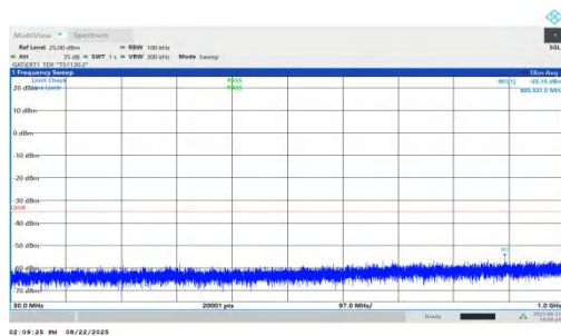
NTNV-n41-PC1.5-30-25-H-DFT-QPSK-Inner_1RB_Left-30-1000- PASS
