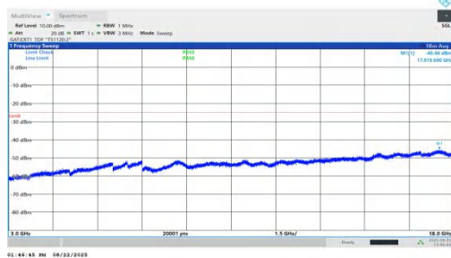
NTVN-n41-PC1.5-30-25-M-DFT-BPSK-Inner_1RB_Right-3000-18000-PASS
