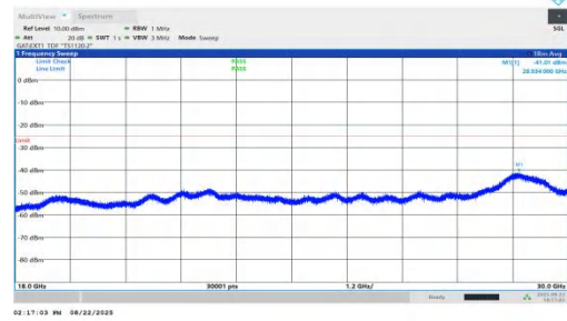
NTNV-n41-PC1.5-30-30-L-DFT-QPSK-Inner_1RB_Left-18000-30000-PASS
