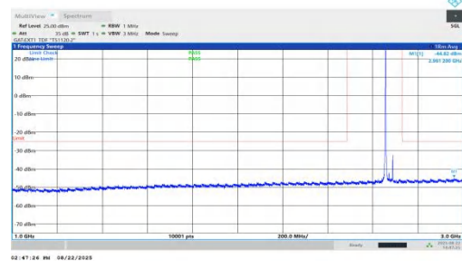
NTNV-n41-PC1.5-30-35-H-DFT-BPSK-Inner_1RB_Left-1000-3000 -PASS
