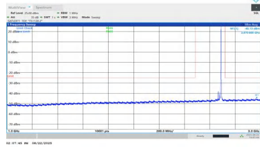
NTNV-n41-PC1.5-30-25-H-DFT-BPSK-Inner_1RB_Right-1000-300 0-PASS
