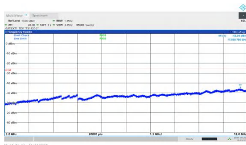
NTNV-n41-PC1.5-30-35-M-DFT-QPSK-Inner_1RB_Right-3000-18000-PASS
