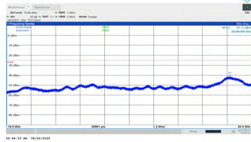
NTNV-n41-PC1.5-30-35-M-DFT-QPSK-Inner_1RB_Left-18000-30000-PASS
