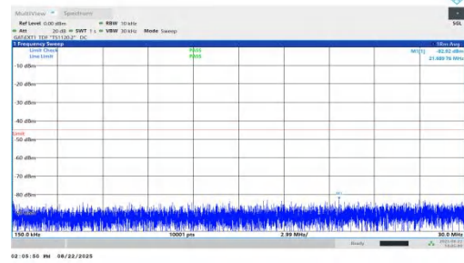
NTNV-n41-PC1.5-30-25-H-DFT-BPSK-Inner_1RB_Left-0.15-30-P ASS
