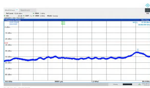
NTNV-n41-PC1.5-30-25-L-DFT-QPSK-Inner_1RB_Right-18000-30000-PASS
