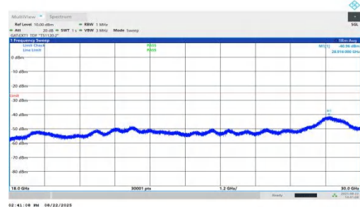
NTNV-n41-PC1.5-30-35-M-DFT-BPSK-Inner_1RB_Left-18000-300 00-PASS
