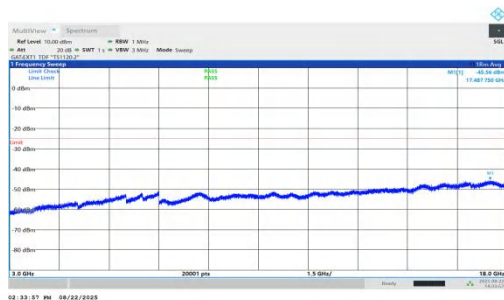
NTNV-n41-PC1.5-30-35-L-DFT-BPSK-Inner_1RB_Left-3000-18000-PASS
