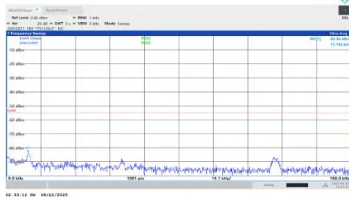
NTNV-n41-PC1.5-30-35-L-DFT-BPSK-Inner_1RB_Left-0.009-0.15-PASS
