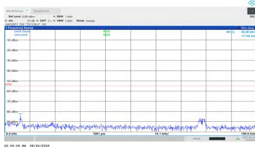
NTNV-n41-PC1.5-30-25-H-DFT-QPSK-Inner_1RB_Left-0.009-0.1 5-PASS
