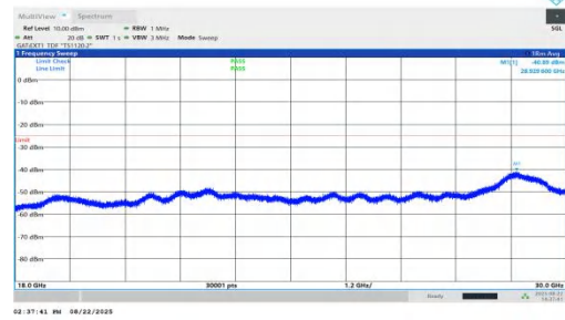
NTNV-n41-PC1.5-30-35-L-DFT-QPSK-Inner_1RB_Left-18000-30000-PASS
