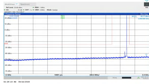
NTNV-n41-PC1.5-30-30-H-DFT-BPSK-Inner_1RB_Right-1000-300 0-PASS
