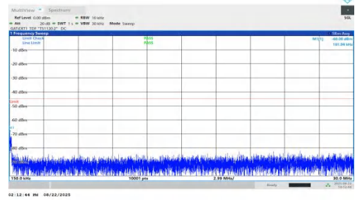
NTNV-n41-PC1.5-30-30-L-DFT-BPSK-Inner_1RB_Left-0.15-30-PA SS
