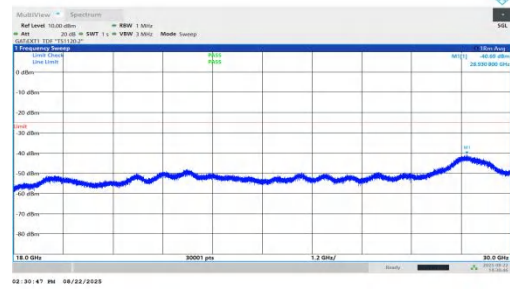
NTNV-n41-PC1.5-30-30-H-DFT-QPSK-Inner_1RB_Left-18000-30000-PASS
