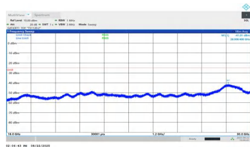
NTNV-n41-PC1.5-30-25-H-DFT-BPSK-Inner_1RB_Left-18000-300 00-PASS
