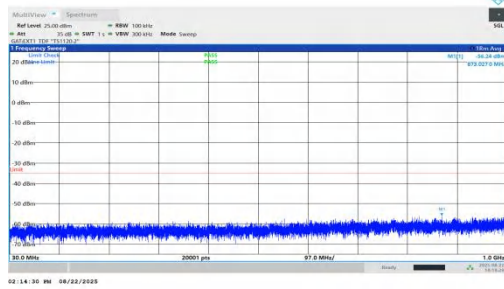
NTNV-n41-PC1.5-30-30-L-DFT-BPSK-Inner_1RB_Right-30-1000 -PASS
