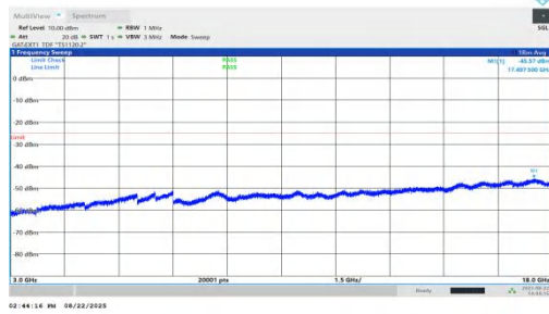
NTNV-n41-PC1.5-30-35-M-DFT-QPSK-Inner_1RB_Left-3000-18000-PASS
