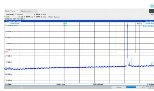
NTNV-n41-PC2-30-50-H-DFT-QPSK-Inner_1RB_Left-1000-3000- PASS
