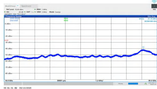
NTNV-n41-PC2-30-60-L-DFT-BPSK-Inner_1RB_Left-18000-30000 -PASS
