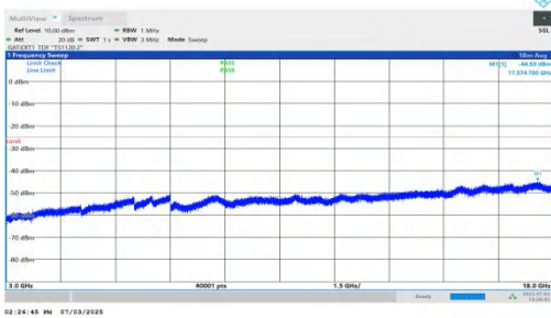
NTNV-n41-PC2-30-80-H-DFT-QPSK-Inner_1RB_Right-3000-18000-PASS
