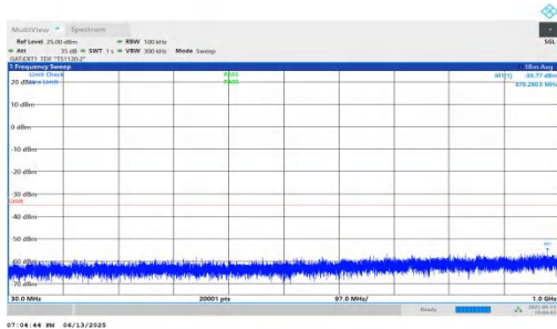
NTNV-n41-PC2-30-70-M-DFT-BPSK-Inner_1RB_Left-30-1000-PASS
