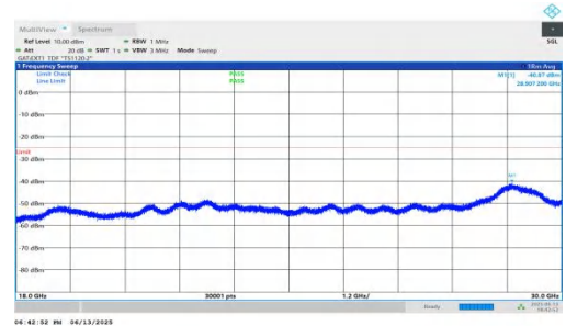
NTNV-n41-PC2-30-60-L-DFT-BPSK-Inner_1RB_Right-18000-30000-PASS
