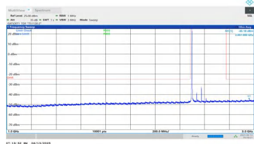
NTNV-n41-PC2-30-80-L-DFT-QPSK-Inner_1RB_Left-1000-3000-PASS
