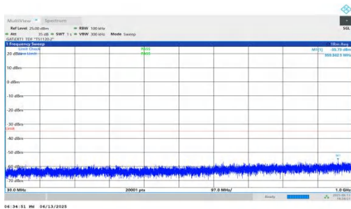
NTNV-n41-PC2-30-50-H-DFT-BPSK-Inner_1RB_Left-30-1000-PA
