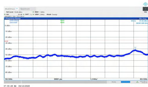
NTNV-n41-PC2-30-70-M-DFT-BPSK-Inner_1RB_Left-18000-30000-PASS
