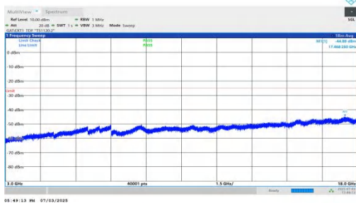
NTNV-n41-PC2-30-70-L-DFT-QPSK-Inner_1RB_Right-3000-18000-PASS 00-PASS
