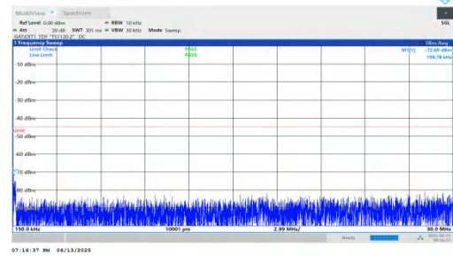
NTNV-n41-PC2-30-80-L-DFT-BPSK-Inner_1RB_Left-0.15-30-PAS
