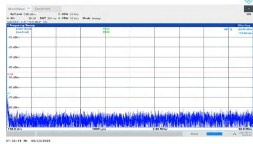
NTNV-n41-PC2-30-80-H-DFT-QPSK-Inner_1RB_Right-0.15-30-PA SS
