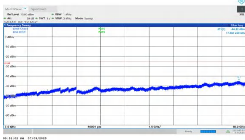
NTNV-n41-PC2-30-70-M-DFT-QPSK-Inner_1RB_Right-3000-18000- 00-PASS
