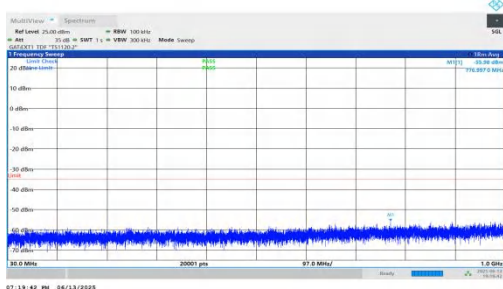
NTNV-n41-PC2-30-80-L-DFT-QPSK-Inner_1RB_Left-30-1000-PASS
