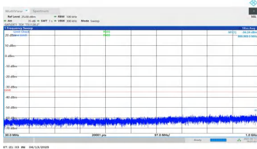
NTNV-n41-PC2-30-80-L-DFT-QPSK-Inner_1RB_Right-30-1000-PASS ASS
