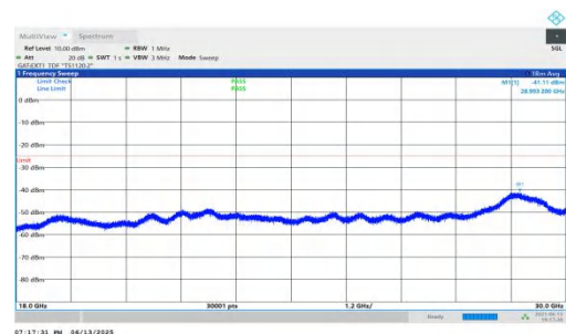
NTNV-n41-PC2-30-80-L-DFT-BPSK-Inner_1RB_Left-18000-30000-PASS
