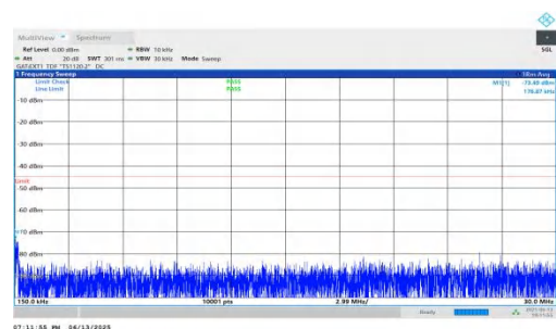
NTNV-n41-PC2-30-70-H-DFT-BPSK-Inner_1RB_Right-0.15-30-PASS
