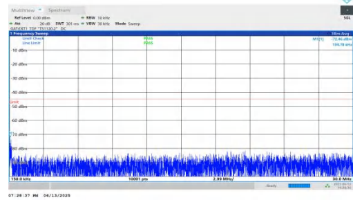
NTNV-n41-PC2-30-80-H-DFT-BPSK-Inner_1RB_Left-0.15-30-PAS S
