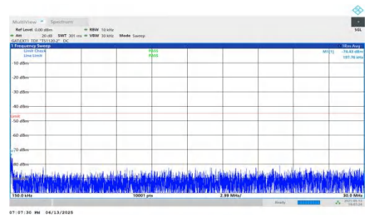
NTNV-n41-PC2-30-70-M-DFT-QPSK-Inner_1RB_Left-0.15-30-PASS
