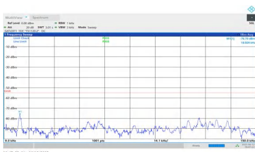
NTNV-n41-PC2-30-60-M-DFT-BPSK-Inner_1RB_Right-0.009-0.15-PASS
