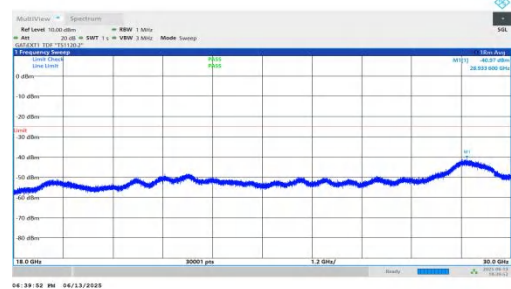
NTNV-n41-PC2-30-50-H-DFT-QPSK-Inner_1RB_Right-18000-300 00-PASS
