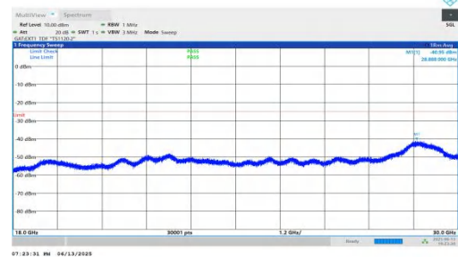
NTNV-n41-PC2-30-80-M-DFT-BPSK-Inner_1RB_Left-18000-30000-PASS
