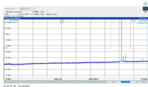
NTNV-n41-PC2-30-60-H-DFT-BPSK-Inner_1RB_Left-1000-3000-PASS
