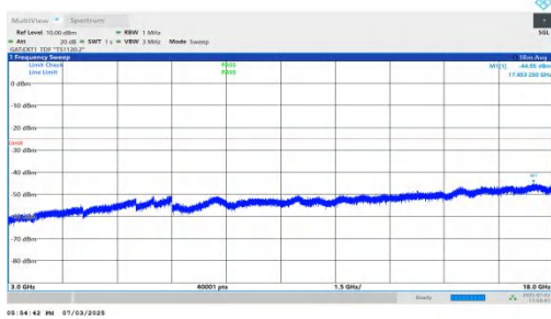
NTNV-n41-PC2-30-80-L-DFT-QPSK-Inner_1RB_Right-3000-18000-PASS 00-PASS
