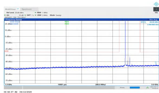
NTNV-n41-PC2-30-60-M-DFT-BPSK-Inner_1RB_Left-1000-3000-PASS
