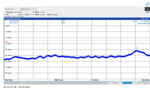
NTNV-n41-PC2-30-60-H-DFT-BPSK-Inner_1RB_Left-18000-30000-PASS
