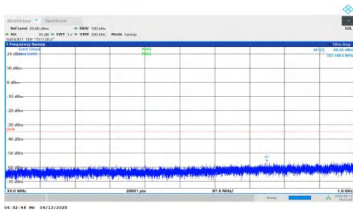
NTNV-n41-PC2-30-60-H-DFT-BPSK-Inner_1RB_Left-30-1000-PASS
