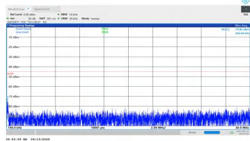
NTNV-n41-PC2-30-60-H-DFT-BPSK-Inner_1RB_Right-0.15-30-PASS
