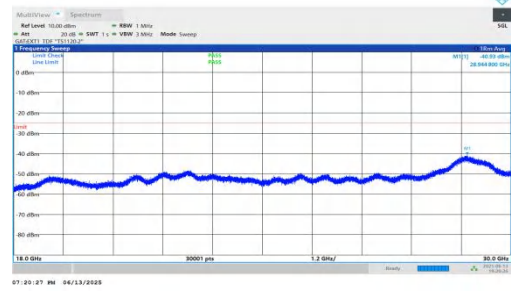
NTNV-n41-PC2-30-80-L-DFT-QPSK-Inner_1RB_Left-18000-3000 0-PASS
