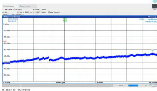
NTNV-n41-PC2-30-60-L-DFT-BPSK-Inner_1RB_Left-3000-18000 -PASS
