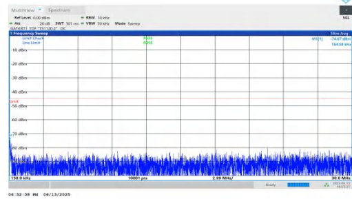
NTNV-n41-PC2-30-60-H-DFT-BPSK-Inner_1RB_Left-0.15-30-PASS
