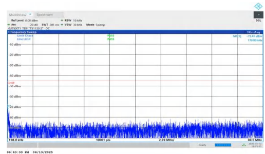
NTNV-n41-PC2-30-60-L-DFT-QPSK-Inner_1RB_Left-0.15-30-PASS
