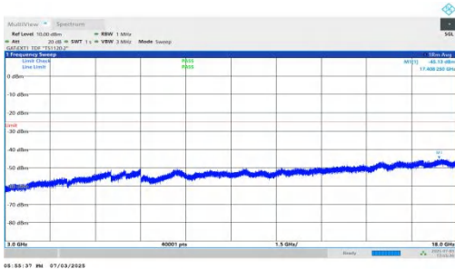
NTNV-n41-PC2-30-80-M-DFT-BPSK-Inner_1RB_Right-3000-18000-PASS
