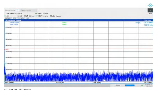
NTNV-n41-PC2-30-80-L-DFT-BPSK-Inner_1RB_Right-0.15-30-PASS
