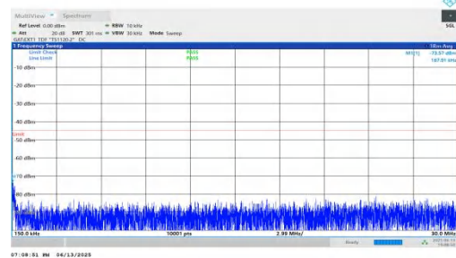
NTNV-n41-PC2-30-70-M-DFT-QPSK-Inner_1RB_Right-0.15-30-P ASS
