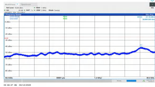
NTNV-n41-PC2-30-60-L-DFT-QPSK-Inner_1RB_Left-18000-3000 0-PASS
