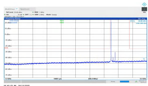
NTNV-n41-PC2-30-60-L-DFT-QPSK-Inner_1RB_Left-1000-3000-PASS
