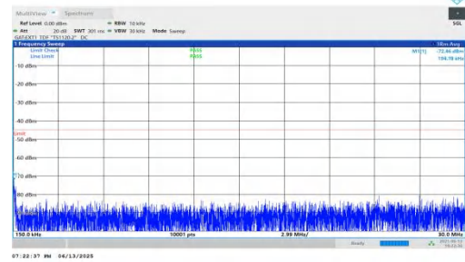
NTNV-n41-PC2-30-80-M-DFT-BPSK-Inner_1RB_Left-0.15-30-PASS
