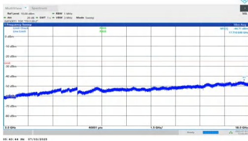
NTNV-n41-PC2-30-60-L-DFT-QPSK-Inner_1RB_Right-3000-18000 00-PASS
