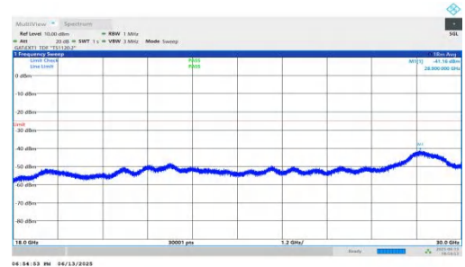
NTNV-n41-PC2-30-60-H-DFT-BPSK-Inner_1RB_Right-18000-300 00-PASS
