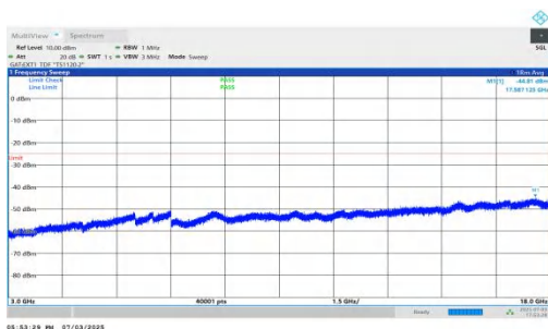
NTNV-n41-PC2-30-80-L-DFT-BPSK-Inner_1RB_Left-3000-18000-PASS
