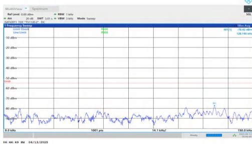
NTNV-n41-PC2-30-60-L-DFT-QPSK-Inner_1RB_Right-0.009-0.1 5-PASS
