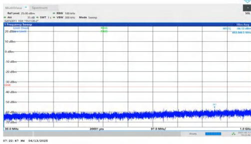
NTNV-n41-PC2-30-80-M-DFT-BPSK-Inner_1RB_Left-30-1000-PASS
