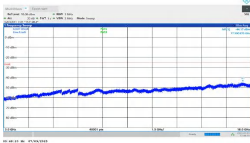
NTNV-n41-PC2-30-70-L-DFT-BPSK-Inner_1RB_Right-3000-18000-P PASS
