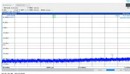
NTNV-n41-PC2-30-60-M-DFT-QPSK-Inner_1RB_Right-30-1000-P PASS
