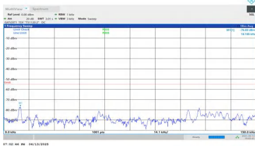
NTNV-n41-PC2-30-70-L-DFT-QPSK-Inner_1RB_Right-0.009-0.1 5-PASS
