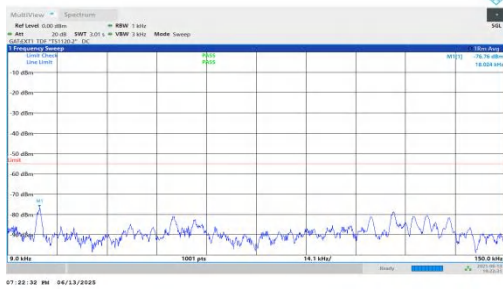
NTNV-n41-PC2-30-80-M-DFT-BPSK-Inner_1RB_Left-0.009-0.15-PASS
