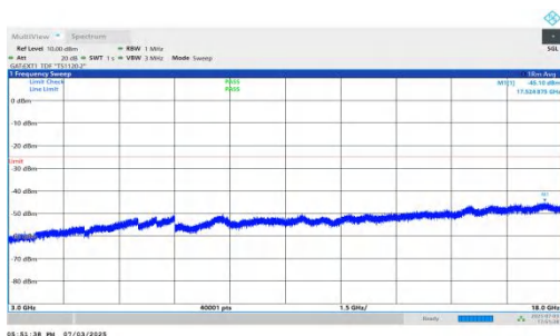
NTNV-n41-PC2-30-70-H-DFT-BPSK-Inner_1RB_Left-3000-18000-PASS
