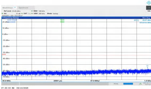
NTNV-n41-PC2-30-80-H-DFT-QPSK-Inner_1RB_Right-30-1000-PASS
