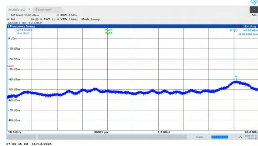
NTNV-n41-PC2-30-70-M-DFT-QPSK-Inner_1RB_Right-18000-300 00-PASS
