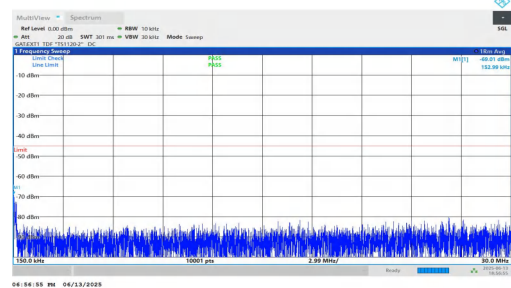
NTNV-n41-PC2-30-60-H-DFT-QPSK-Inner_1RB_Right-0.15-30-PA SS
