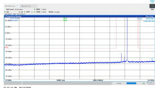
NTNV-n41-PC2-30-80-M-DFT-QPSK-Inner_1RB_Right-1000-3000- -PASS
