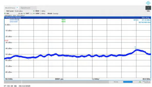
NTNV-n41-PC2-30-70-M-DFT-BPSK-Inner_1RB_Right-18000-30000-PASS
