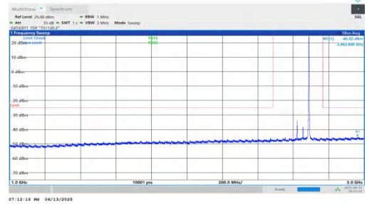
NTNV-n41-PC2-30-70-H-DFT-BPSK-Inner_1RB_Right-1000-3000 -PASS
