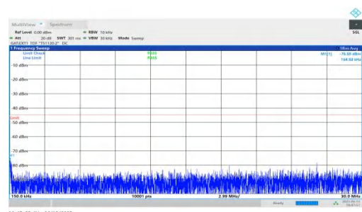
NTNV-n41-PC2-30-60-M-DFT-BPSK-Inner_1RB_Right-0.15-30-PASS
