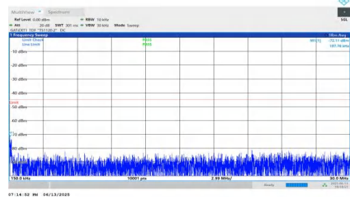
NTNV-n41-PC2-30-70-H-DFT-QPSK-Inner_1RB_Right-0.15-30-PA SS
