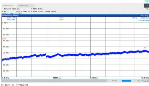
NTNV-n41-PC2-30-50-H-DFT-QPSK-Inner_1RB_Right-3000-180 00-PASS
