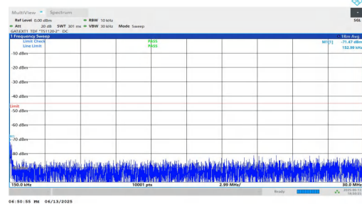
NTNV-n41-PC2-30-60-M-DFT-QPSK-Inner_1RB_Right-0.15-30-P ASS
