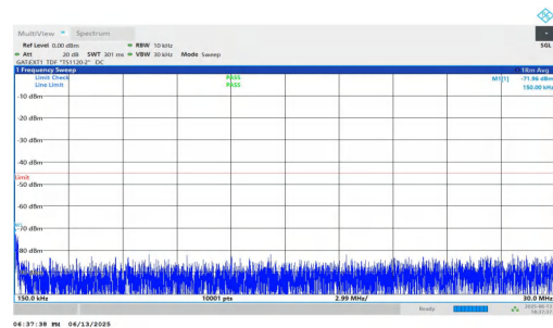
NTNV-n41-PC2-30-50-H-DFT-QPSK-Inner_1RB_Left-0.15-30-PAS S
