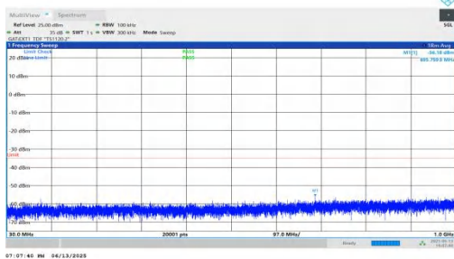
NTNV-n41-PC2-30-70-M-DFT-QPSK-Inner_1RB_Left-30-1000-PASS
