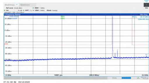
NTNV-n41-PC2-30-70-L-DFT-QPSK-Inner_1RB_Left-1000-3000-P PASS
