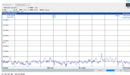
NTNV-n41-PC2-30-80-M-DFT-BPSK-Inner_1RB_Right-0.009-0.15-PASS
