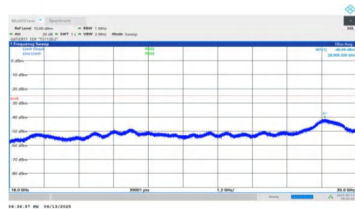
NTNV-n41-PC2-30-50-H-DFT-BPSK-Inner_1RB_Right-18000-300 00-PASS
