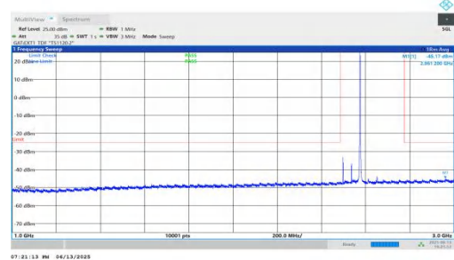
NTNV-n41-PC2-30-80-L-DFT-QPSK-Inner_1RB_Right-1000-3000-PASS PASS
