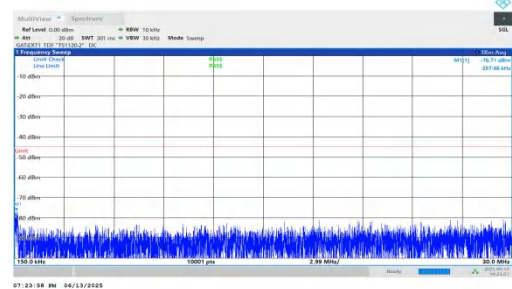
NTNV-n41-PC2-30-80-M-DFT-BPSK-Inner_1RB_Right-0.15-30-PASS
