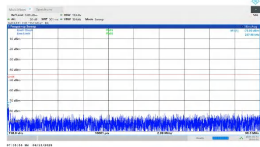
NTNV-n41-PC2-30-70-M-DFT-BPSK-Inner_1RB_Right-0.15-30-PASS
