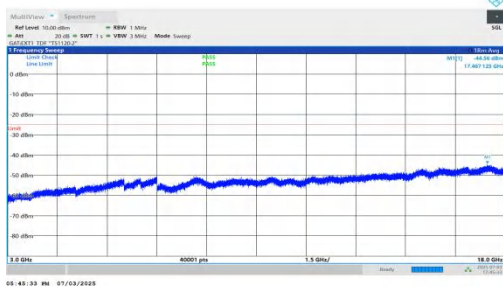
NTNV-n41-PC2-30-60-M-DFT-QPSK-Inner_1RB_Right-3000-1800 00-PASS
