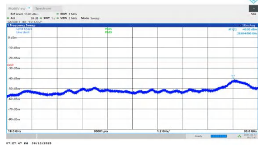
NTNV-n41-PC2-30-80-M-DFT-QPSK-Inner_1RB_Right-18000-30000- 00-PASS
