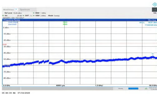
NTNV-n41-PC2-30-60-H-DFT-BPSK-Inner_1RB_Left-3000-18000-PASS
