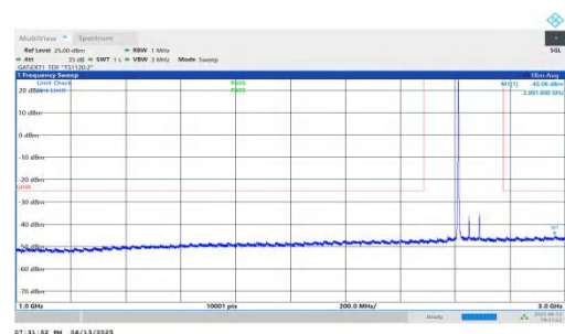
NTNV-n41-PC2-30-80-H-DFT-QPSK-Inner_1RB_Left-1000-3000- PASS
