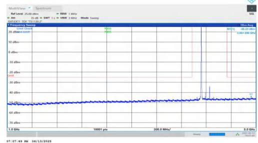
NTNV-n41-PC2-30-70-M-DFT-QPSK-Inner_1RB_Left-1000-3000-PASS
