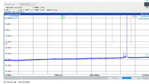
NTNV-n41-PC2-30-50-H-DFT-BPSK-Inner_1RB_Right-1000-3000 -PASS
