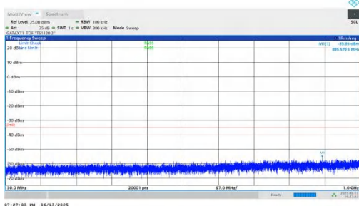
NTNV-n41-PC2-30-80-M-DFT-QPSK-Inner_1RB_Right-30-1000- PASS
