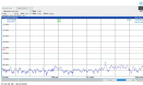
NTNV-n41-PC2-30-80-M-DFT-QPSK-Inner_1RB_Left-0.009-0.15-PASS
