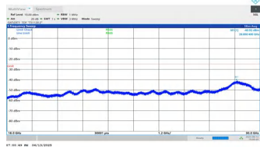
NTNV-n41-PC2-30-70-L-DFT-BPSK-Inner_1RB_Right-18000-30000-P PASS
