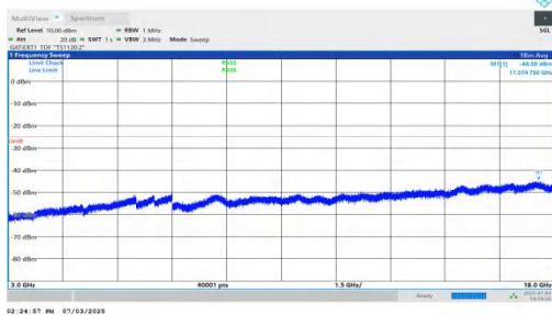
NTNV-n41-PC2-30-80-M-DFT-QPSK-Inner_1RB_Right-3000-18000- 00-PASS
