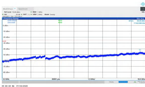
NTNV-n41-PC2-30-70-M-DFT-BPSK-Inner_1RB_Left-3000-18000-PASS
