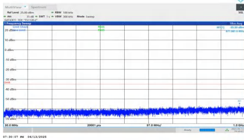
NTNV-n41-PC2-30-80-H-DFT-BPSK-Inner_1RB_Right-30-1000-P ASS
