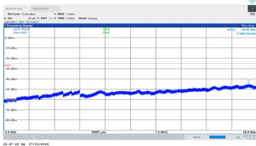
NTNV-n41-PC2-30-60-H-DFT-QPSK-Inner_1RB_Right-3000-180 00-PASS
