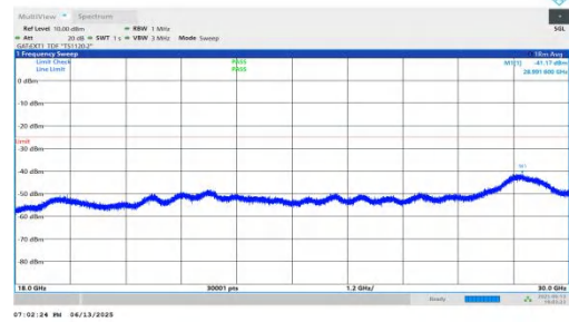
NTNV-n41-PC2-30-70-L-DFT-QPSK-Inner_1RB_Left-18000-3000 0-PASS
