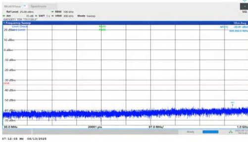
NTNV-n41-PC2-30-70-H-DFT-BPSK-Inner_1RB_Right-30-1000-P ASS
