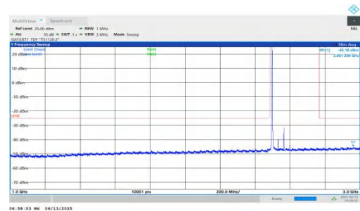
NTNV-n41-PC2-30-70-L-DFT-BPSK-Inner_1RB_Left-1000-3000-PASS
