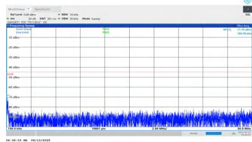
NTNV-n41-PC2-30-50-H-DFT-BPSK-Inner_1RB_Right-0.15-30-PA
