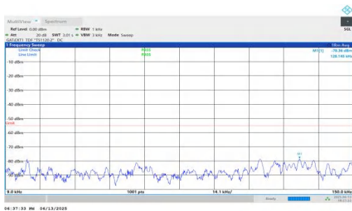
NTNV-n41-PC2-30-50-H-DFT-QPSK-Inner_1RB_Left-0.009-0.15- PASS
