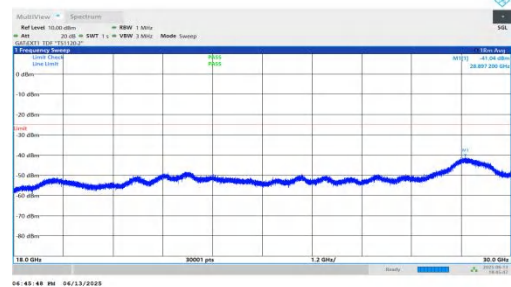
NTNV-n41-PC2-30-60-L-DFT-QPSK-Inner_1RB_Right-18000-3000 00-PASS
