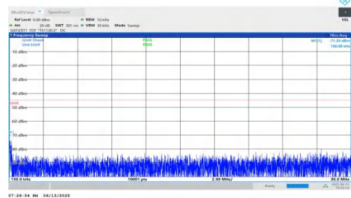
NTNV-n41-PC2-30-80-M-DFT-QPSK-Inner_1RB_Right-0.15-30-P ASS
