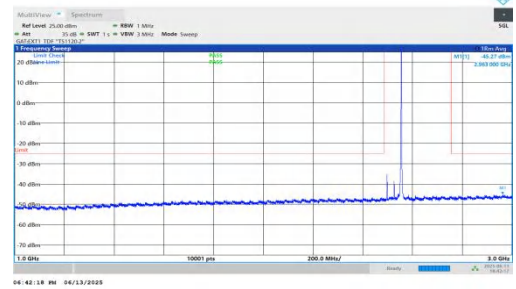
NTNV-n41-PC2-30-60-L-DFT-BPSK-Inner_1RB_Right-1000-3000-PASS
