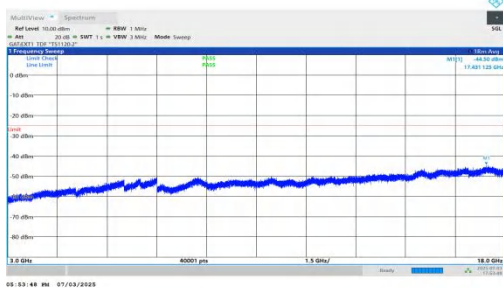
NTNV-n41-PC2-30-80-L-DFT-BPSK-Inner_1RB_Right-3000-18000-PASS
