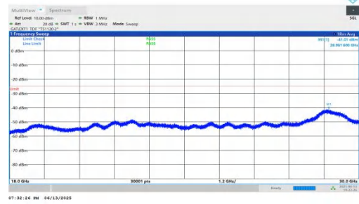
NTNV-n41-PC2-30-80-H-DFT-QPSK-Inner_1RB_Left-18000-3000 0-PASS
