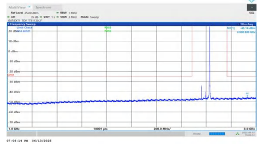
NTNV-n41-PC2-30-70-M-DFT-BPSK-Inner_1RB_Right-1000-3000-PASS
