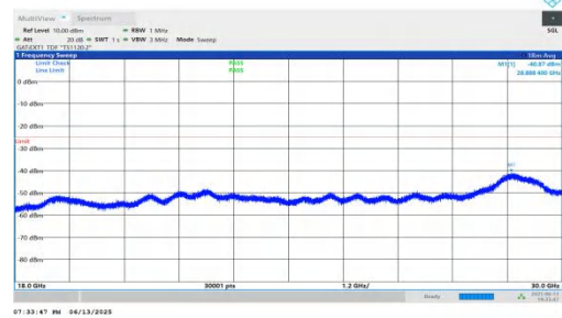
NTNV-n41-PC2-30-80-H-DFT-QPSK-Inner_1RB_Right-18000-30000-PASS
