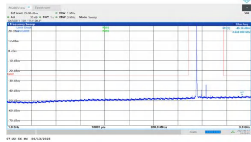
NTNV-n41-PC2-30-80-M-DFT-BPSK-Inner_1RB_Left-1000-3000-PASS
