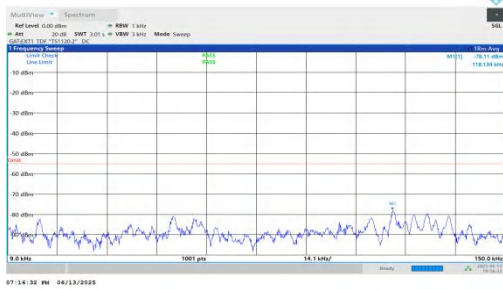
NTNV-n41-PC2-30-80-L-DFT-BPSK-Inner_1RB_Left-0.009-0.15-PASS
