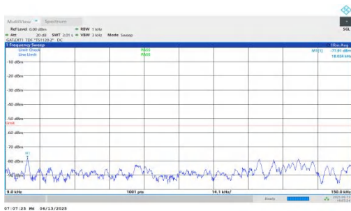
NTNV-n41-PC2-30-70-M-DFT-QPSK-Inner_1RB_Left-0.009-0.15-PASS
