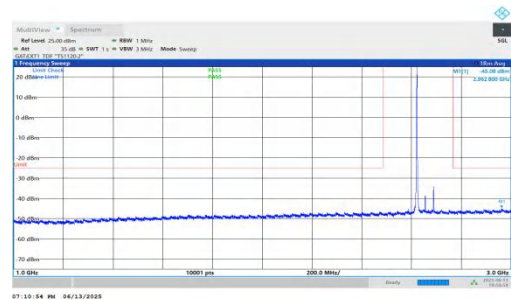
NTNV-n41-PC2-30-70-H-DFT-BPSK-Inner_1RB_Left-1000-3000-PASS
