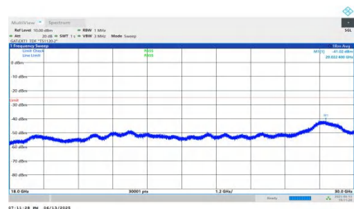
NTNV-n41-PC2-30-70-H-DFT-BPSK-Inner_1RB_Left-18000-30000-PASS
