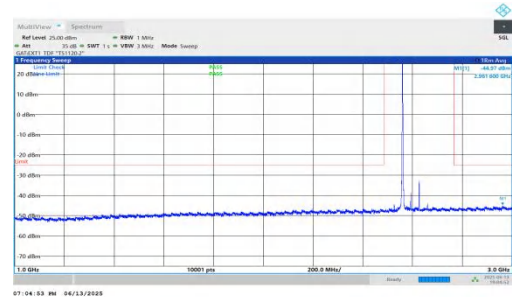
NTNV-n41-PC2-30-70-M-DFT-BPSK-Inner_1RB_Left-1000-3000-PASS
