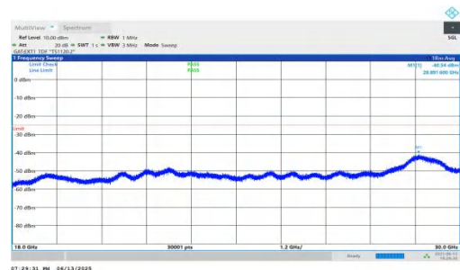
NTNV-n41-PC2-30-80-H-DFT-BPSK-Inner_1RB_Left-18000-30000-PASS 0-PASS
