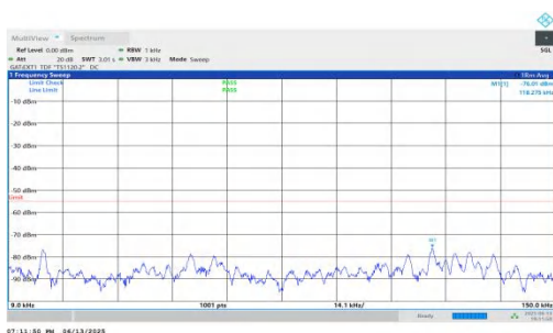
NTNV-n41-PC2-30-70-H-DFT-BPSK-Inner_1RB_Right-0.009-0.15-PASS
