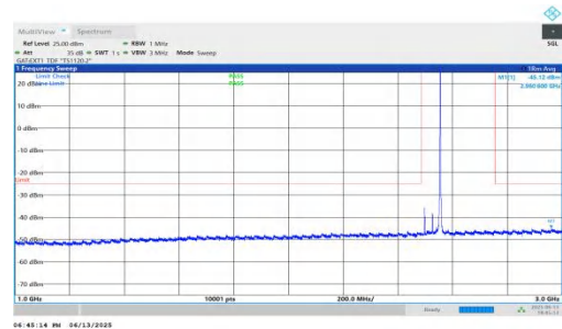
NTNV-n41-PC2-30-60-L-DFT-QPSK-Inner_1RB_Right-1000-3000-P PASS
