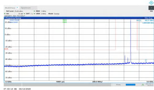
NTNV-n41-PC2-30-80-H-DFT-QPSK-Inner_1RB_Right-1000-3000-PASS
