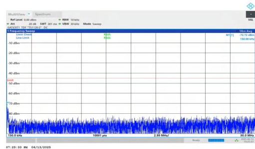
NTNV-n41-PC2-30-80-M-DFT-QPSK-Inner_1RB_Left-0.15-30-PASS
