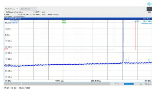
NTNV-n41-PC2-30-80-H-DFT-BPSK-Inner_1RB_Left-1000-3000-PASS ASS
