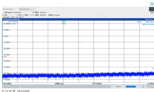
NTNV-n41-PC2-30-70-H-DFT-BPSK-Inner_1RB_Left-30-1000-PASS
