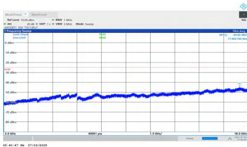
NTNV-n41-PC2-30-50-H-DFT-BPSK-Inner_1RB_Right-3000-180 00-PASS
