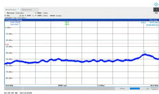
NTNV-n41-PC2-30-70-L-DFT-BPSK-Inner_1RB_Left-18000-30000-PASS
