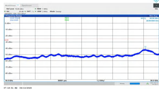
NTNV-n41-PC2-30-80-L-DFT-BPSK-Inner_1RB_Right-18000-30000-PASS
