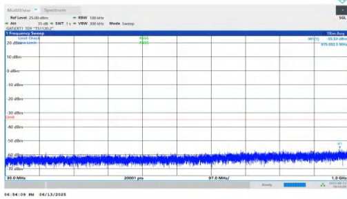
NTNV-n41-PC2-30-60-H-DFT-BPSK-Inner_1RB_Right-30-1000-P ASS
