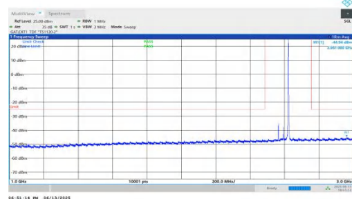
NTNV-n41-PC2-30-60-M-DFT-QPSK-Inner_1RB_Right-1000-3000 -PASS
