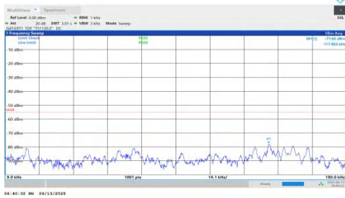
NTNV-n41-PC2-30-60-L-DFT-BPSK-Inner_1RB_Left-0.009-0.15- PASS
