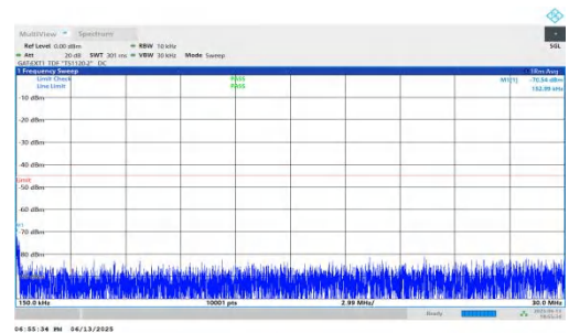
NTNV-n41-PC2-30-60-H-DFT-QPSK-Inner_1RB_Left-0.15-30-PAS S
