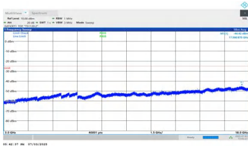
NTNV-n41-PC2-30-60-L-DFT-BPSK-Inner_1RB_Right-3000-18000-PASS
