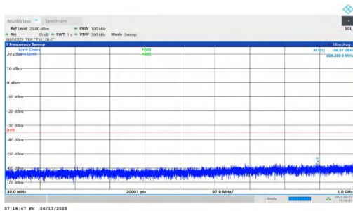
NTNV-n41-PC2-30-80-L-DFT-BPSK-Inner_1RB_Left-30-1000-PASS
