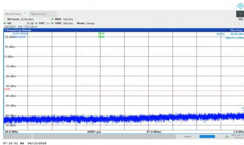
NTNV-n41-PC2-30-70-H-DFT-QPSK-Inner_1RB_Right-30-1000-PASS
