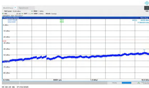
NTNV-n41-PC2-30-60-H-DFT-BPSK-Inner_1RB_Right-3000-180 00-PASS
