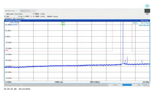
NTNV-n41-PC2-30-60-H-DFT-QPSK-Inner_1RB_Left-1000-3000- PASS
