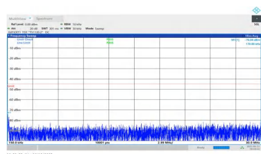
NTNV-n41-PC2-30-70-L-DFT-BPSK-Inner_1RB_Right-0.15-30-PASS
