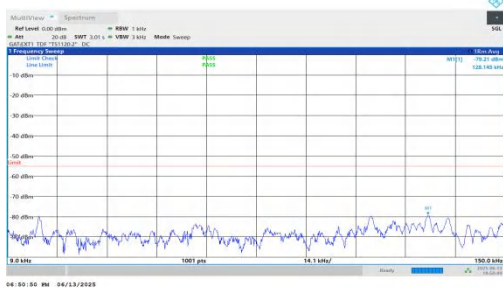
NTNV-n41-PC2-30-60-M-DFT-QPSK-Inner_1RB_Right-0.009-0.1 5-PASS
