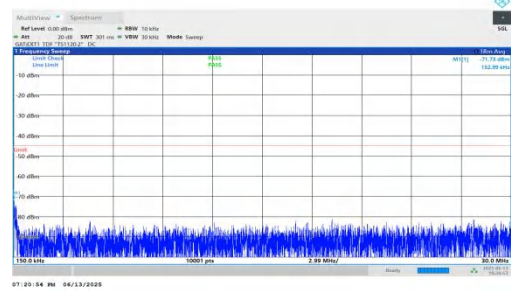
NTNV-n41-PC2-30-80-L-DFT-QPSK-Inner_1RB_Right-0.15-30-PASS SS
