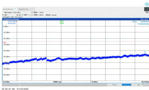
NTNV-n41-PC2-30-50-H-DFT-BPSK-Inner_1RB_Left-3000-1800
