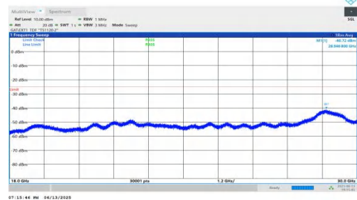
NTNV-n41-PC2-30-70-H-DFT-QPSK-Inner_1RB_Right-18000-30000-PASS
