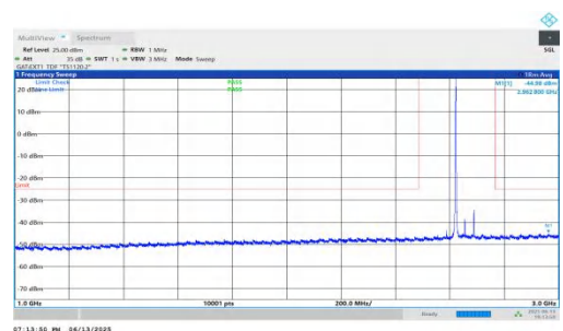
NTNV-n41-PC2-30-70-H-DFT-QPSK-Inner_1RB_Left-1000-3000- PASS
