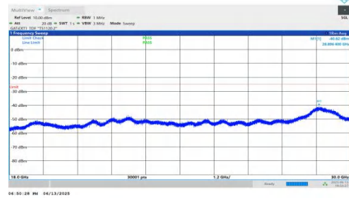
NTNV-n41-PC2-30-60-M-DFT-QPSK-Inner_1RB_Left-18000-3000 0-PASS
