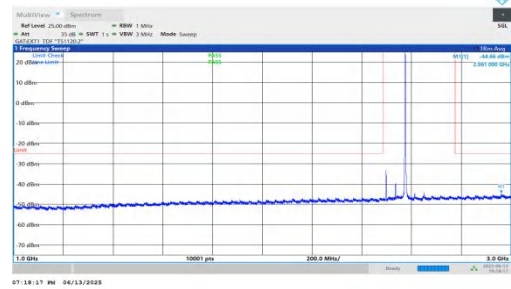
NTNV-n41-PC2-30-80-L-DFT-BPSK-Inner_1RB_Right-1000-3000-PASS
