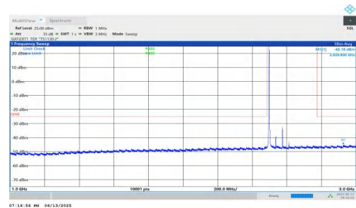
NTNV-n41-PC2-30-80-L-DFT-BPSK-Inner_1RB_Left-1000-3000-PASS
