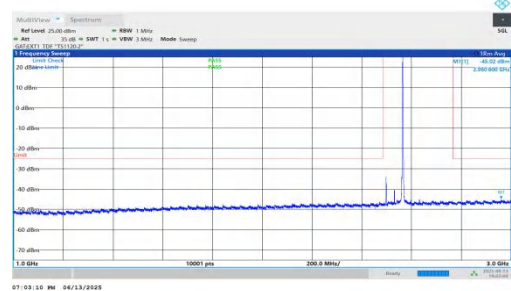
NTNV-n41-PC2-30-70-L-DFT-QPSK-Inner_1RB_Right-1000-3000-PASS PASS
