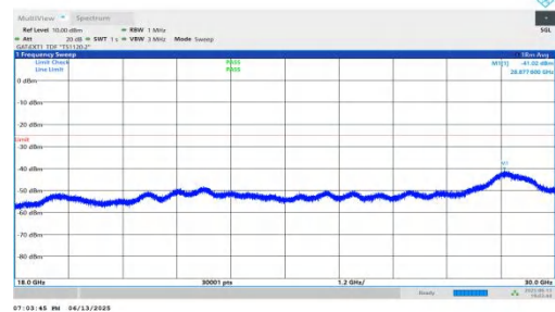
NTNV-n41-PC2-30-70-L-DFT-QPSK-Inner_1RB_Right-18000-3000-PASS 00-PASS
