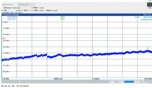
NTNV-n41-PC2-30-50-H-DFT-QPSK-Inner_1RB_Left-3000-1800 0-PASS
