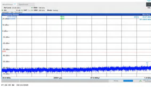
NTNV-n41-PC2-30-80-M-DFT-BPSK-Inner_1RB_Right-30-1000-PASS
