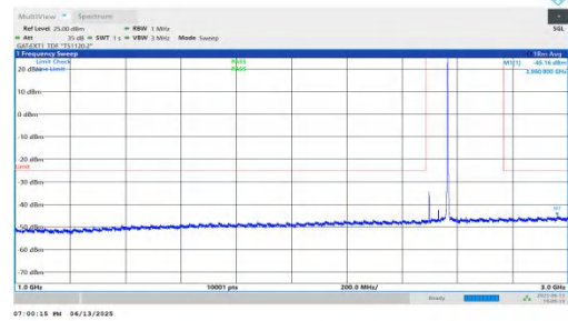
NTNV-n41-PC2-30-70-L-DFT-BPSK-Inner_1RB_Right-1000-3000-P PASS
