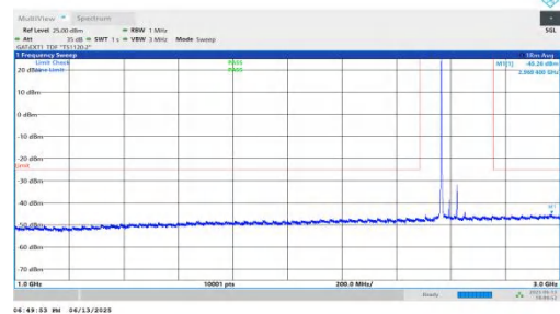
NTNV-n41-PC2-30-60-M-DFT-QPSK-Inner_1RB_Left-1000-3000-PASS
