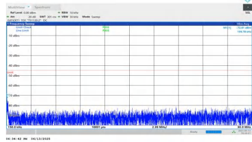
NTNV-n41-PC2-30-50-H-DFT-BPSK-Inner_1RB_Left-0.15-30-PAS
