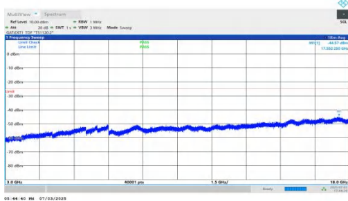
NTNV-n41-PC2-30-60-M-DFT-BPSK-Inner_1RB_Right-3000-18000-PASS
