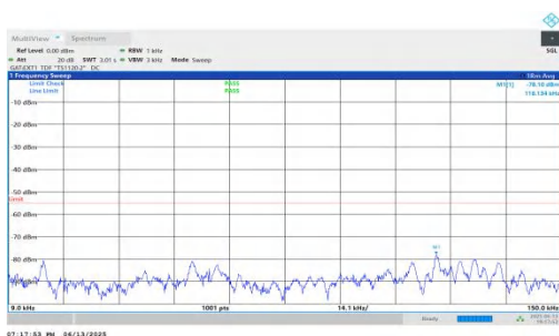
NTNV-n41-PC2-30-80-L-DFT-BPSK-Inner_1RB_Right-0.009-0.15-PASS
