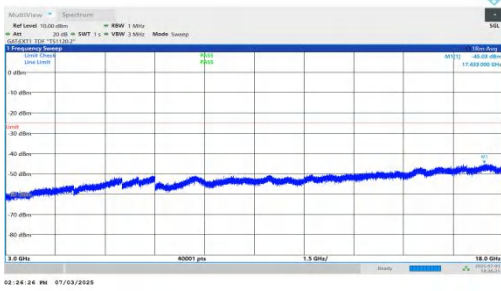
NTNV-n41-PC2-30-80-H-DFT-QPSK-Inner_1RB_Left-3000-1800 0-PASS
