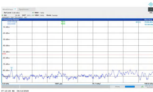
NTNV-n41-PC2-30-70-H-DFT-QPSK-Inner_1RB_Left-0.009-0.15- PASS
