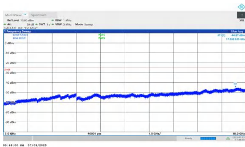
NTNV-n41-PC2-30-70-L-DFT-BPSK-Inner_1RB_Left-3000-18000-PASS
