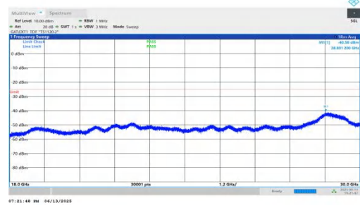
NTNV-n41-PC2-30-80-L-DFT-QPSK-Inner_1RB_Right-18000-30000-PASS 00-PASS
