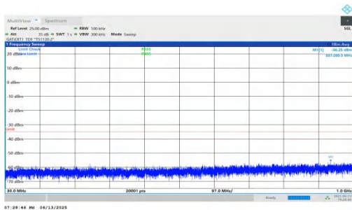
NTNV-n41-PC2-30-80-H-DFT-BPSK-Inner_1RB_Left-30-1000-PASS SS
