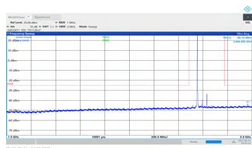
NTNV-n41-PC2-30-80-M-DFT-QPSK-Inner_1RB_Left-1000-3000-PASS
