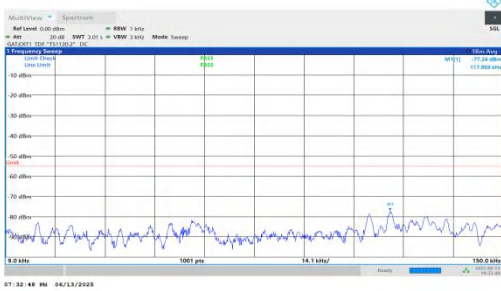
NTNV-n41-PC2-30-80-H-DFT-QPSK-Inner_1RB_Right-0.009-0.1 5-PASS
