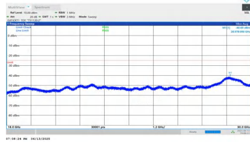
NTNV-n41-PC2-30-70-M-DFT-QPSK-Inner_1RB_Left-18000-3000 0-PASS
