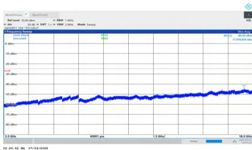
NTNV-n41-PC2-30-80-H-DFT-BPSK-Inner_1RB_Right-3000-180 00-PASS
