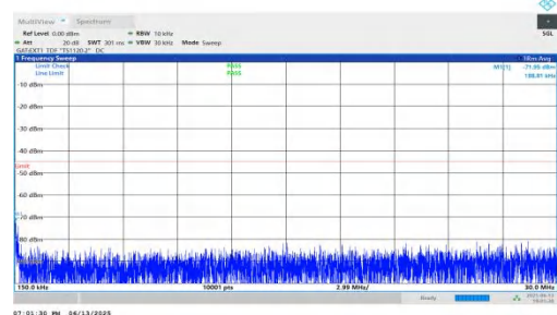
NTNV-n41-PC2-30-70-L-DFT-QPSK-Inner_1RB_Left-0.15-30-P PASS
