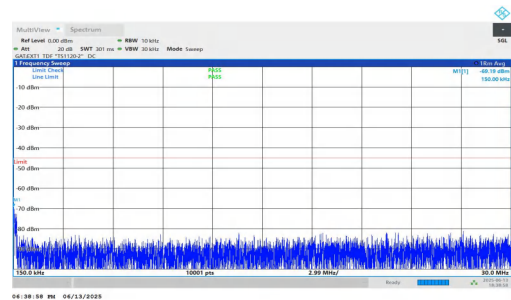
NTNV-n41-PC2-30-50-H-DFT-QPSK-Inner_1RB_Right-0.15-30-PA SS
