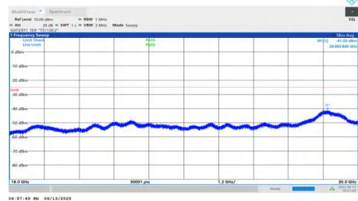
NTNV-n41-PC2-30-60-H-DFT-QPSK-Inner_1RB_Right-18000-300 00-PASS
