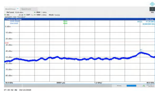
NTNV-n41-PC2-30-80-H-DFT-BPSK-Inner_1RB_Right-18000-300 00-PASS
