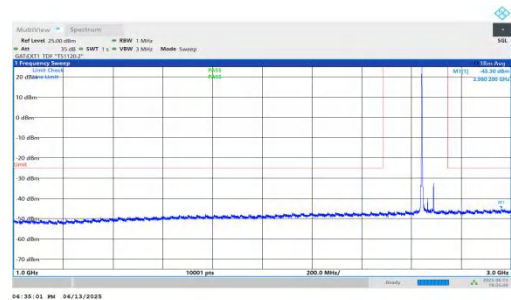
NTNV-n41-PC2-30-50-H-DFT-BPSK-Inner_1RB_Left-1000-3000-P
