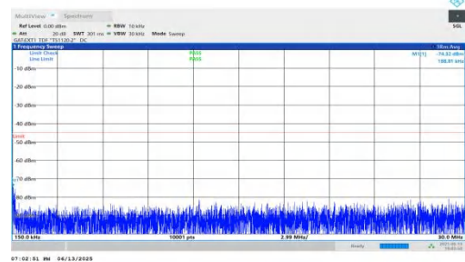
NTNV-n41-PC2-30-70-L-DFT-QPSK-Inner_1RB_Right-0.15-30-PASS SS
