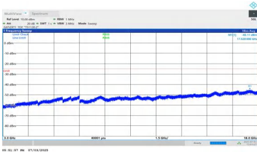
NTNV-n41-PC2-30-70-H-DFT-BPSK-Inner_1RB_Right-3000-180 00-PASS
