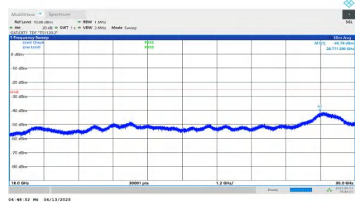
NTNV-n41-PC2-30-60-M-DFT-BPSK-Inner_1RB_Right-18000-30000-PASS
