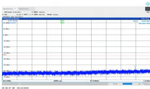
NTNV-n41-PC2-30-60-M-DFT-BPSK-Inner_1RB_Left-30-1000-PASS
