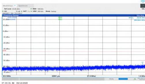
NTNV-n41-PC2-30-70-L-DFT-QPSK-Inner_1RB_Right-30-1000-PASS ASS
