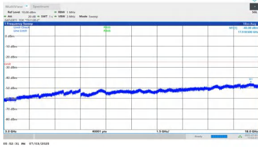
NTNV-n41-PC2-30-70-H-DFT-QPSK-Inner_1RB_Left-3000-1800 0-PASS
