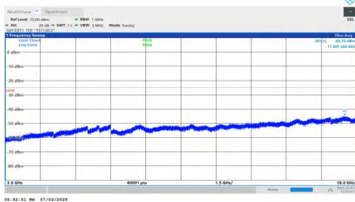
NTNV-n41-PC2-30-70-H-DFT-QPSK-Inner_1RB_Right-3000-18000-PASS
