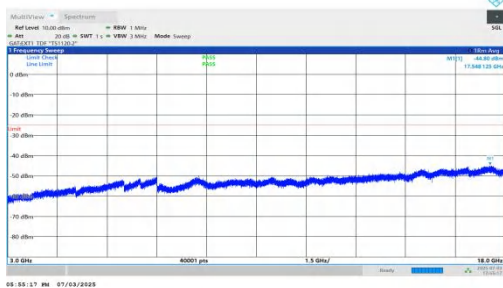
NTNV-n41-PC2-30-80-M-DFT-BPSK-Inner_1RB_Left-3000-18000-PASS
