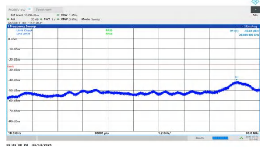
NTNV-n41-PC2-30-35-L-DFT-QPSK-Inner_1RB_Right-18000-3000-PASS 00-PASS
