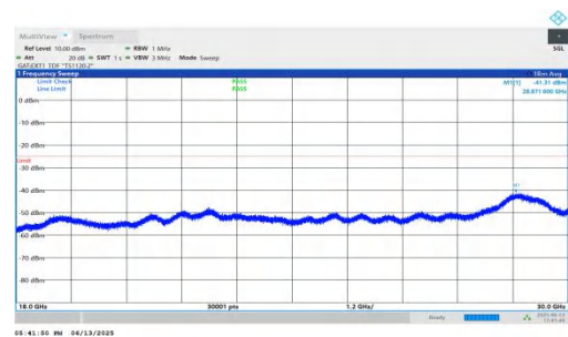
NTNV-n41-PC2-30-35-H-DFT-BPSK-Inner_1RB_Left-18000-30000-PASS
