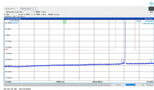
NTNV-n41-PC2-30-50-M-DFT-QPSK-Inner_1RB_Right-1000-3000- -PASS
