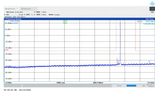
NTNV-n41-PC2-30-45-L-DFT-QPSK-Inner_1RB_Right-1000-3000-P PASS
