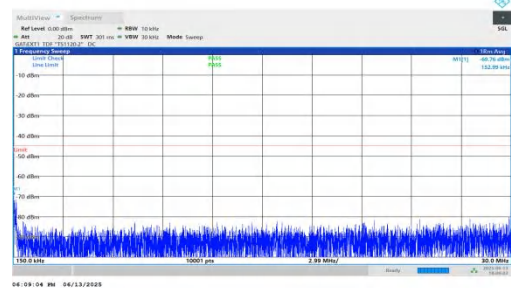
NTNV-n41-PC2-30-45-L-DFT-QPSK-Inner_1RB_Right-0.15-30-PA SS
