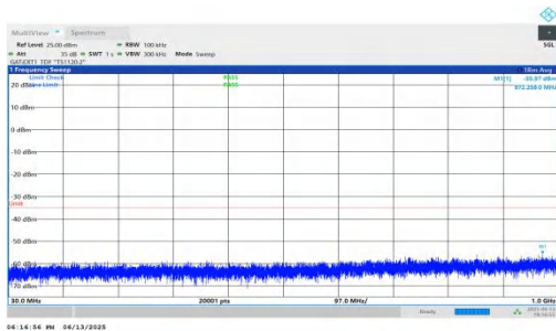
NTNV-n41-PC2-30-45-H-DFT-BPSK-Inner_1RB_Left-30-1000-PASS
