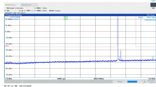
NTNV-n41-PC2-30-40-L-DFT-BPSK-Inner_1RB_Left-1000-3000-PASS
