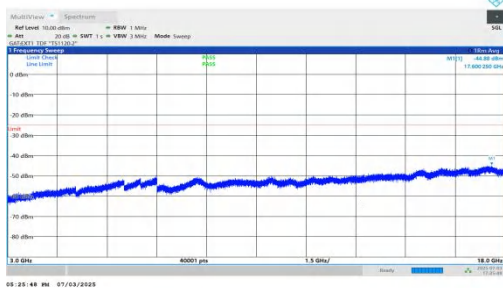
NTNV-n41-PC2-30-40-L-DFT-BPSK-Inner_1RB_Left-3000-18000-PASS
