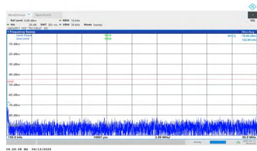
NTNV-n41-PC2-30-50-L-DFT-QPSK-Inner_1RB_Right-0.15-30-PASS SS
