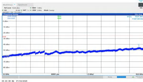
NTNV-n41-PC2-30-40-H-DFT-QPSK-Inner_1RB_Right-3000-18000- 00-PASS
