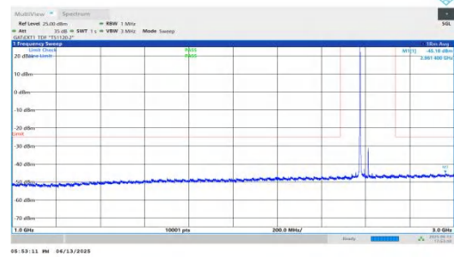
NTNV-n41-PC2-30-40-M-DFT-BPSK-Inner_1RB_Left-1000-3000-PASS
