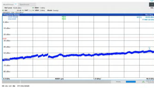
NTNV-n41-PC2-30-35-L-DFT-QPSK-Inner_1RB_Left-3000-18000 -PASS
