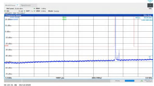
NTNV-n41-PC2-30-50-L-DFT-BPSK-Inner_1RB_Left-1000-3000-P ASS
