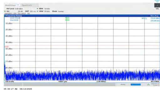
NTNV-n41-PC2-30-35-M-DFT-BPSK-Inner_1RB_Right-0.15-30-PASS
