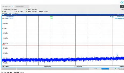
NTNV-n41-PC2-30-45-M-DFT-BPSK-Inner_1RB_Left-30-1000-PASS
