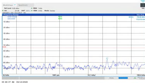
NTNV-n41-PC2-30-35-H-DFT-QPSK-Inner_1RB_Right-0.009-0.1 5-PASS
