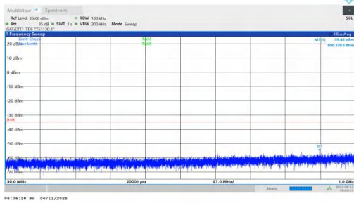
NTNV-n41-PC2-30-45-L-DFT-BPSK-Inner_1RB_Right-30-1000-P ASS
