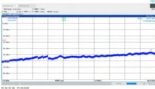
NTNV-n41-PC2-30-45-L-DFT-QPSK-Inner_1RB_Right-3000-180 00-PASS
