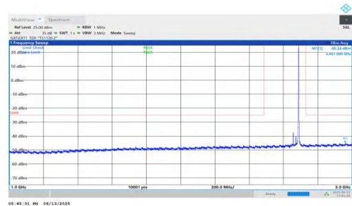
NTNV-n41-PC2-30-35-H-DFT-QPSK-Inner_1RB_Right-1000-3000 -PASS
