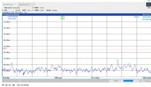
NTNV-n41-PC2-30-35-H-DFT-BPSK-Inner_1RB_Left-0.009-0.15-PASS
