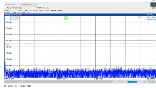
NTNV-n41-PC2-30-35-H-DFT-BPSK-Inner_1RB_Left-0.15-30-PAS
