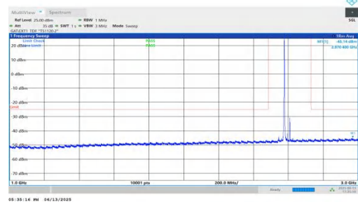
NTNV-n41-PC2-30-35-M-DFT-BPSK-Inner_1RB_Left-1000-3000-PASS
