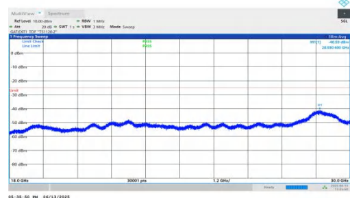
NTNV-n41-PC2-30-35-M-DFT-BPSK-Inner_1RB_Left-18000-30000-PASS
