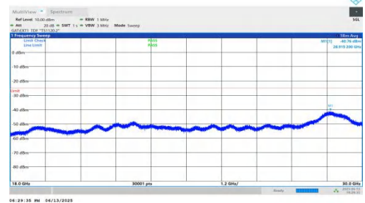
NTNV-n41-PC2-30-50-M-DFT-BPSK-Inner_1RB_Left-18000-30000-PASS
