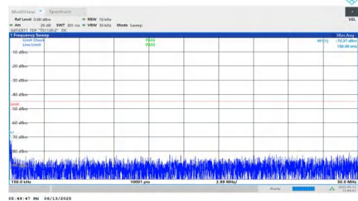
NTNV-n41-PC2-30-40-L-DFT-QPSK-Inner_1RB_Left-0.15-30-P PASS
