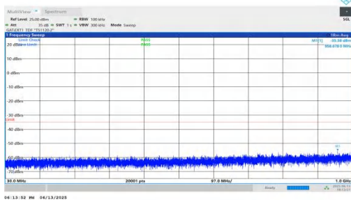
NTNV-n41-PC2-30-45-M-DFT-QPSK-Inner_1RB_Left-30-1000-PASS
