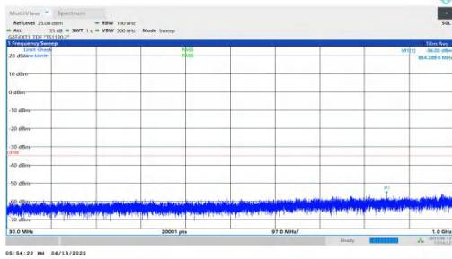
NTNV-n41-PC2-30-40-M-DFT-BPSK-Inner_1RB_Right-30-1000-PASS
