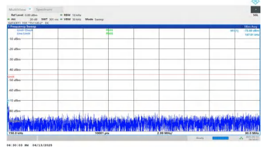
NTNV-n41-PC2-30-50-M-DFT-BPSK-Inner_1RB_Right-0.15-30-PASS
