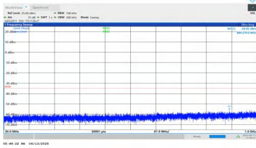
NTNV-n41-PC2-30-40-L-DFT-BPSK-Inner_1RB_Right-30-1000-P ASS
