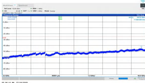
NTNV-n41-PC2-30-45-H-DFT-QPSK-Inner_1RB_Right-3000-18000- 00-PASS
