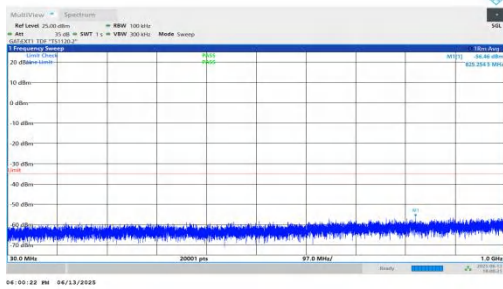
NTNV-n41-PC2-30-40-H-DFT-BPSK-Inner_1RB_Right-30-1000-P ASS
