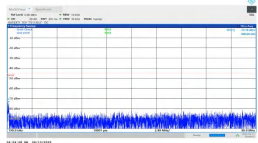
NTNV-n41-PC2-30-45-L-DFT-BPSK-Inner_1RB_Right-0.15-30-PA SS
