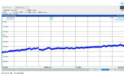
NTNV-n41-PC2-30-45-L-DFT-BPSK-Inner_1RB_Left-3000-18000 -PASS
