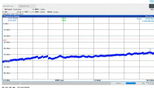
NTNV-n41-PC2-30-35-M-DFT-BPSK-Inner_1RB_Left-3000-18000-PASS
