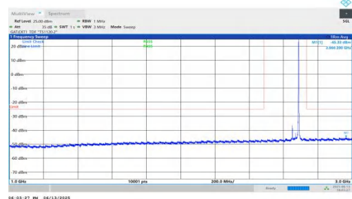
NTNV-n41-PC2-30-40-H-DFT-QPSK-Inner_1RB_Right-1000-3000- -PASS
