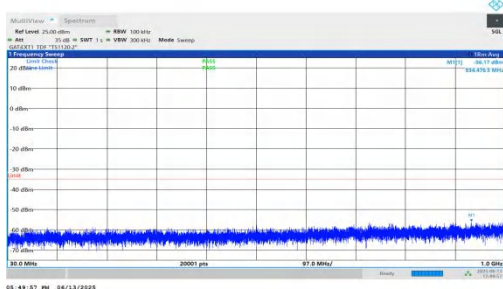
NTNV-n41-PC2-30-40-L-DFT-QPSK-Inner_1RB_Left-30-1000-P PASS
