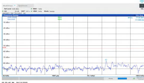
NTNV-n41-PC2-30-40-M-DFT-QPSK-Inner_1RB_Left-0.009-0.15-PASS
