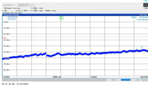
NTNV-n41-PC2-30-40-M-DFT-BPSK-Inner_1RB_Left-3000-18000-PASS
