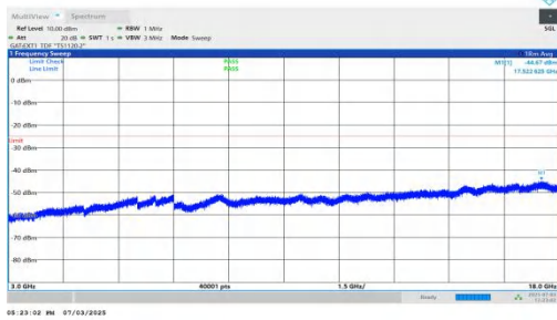
NTNV-n41-PC2-30-35-M-DFT-QPSK-Inner_1RB_Left-3000-1800 0-PASS
