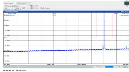
NTNV-n41-PC2-30-45-M-DFT-BPSK-Inner_1RB_Right-1000-3000-PASS
