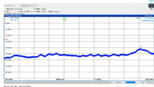
NTNV-n41-PC2-30-45-H-DFT-QPSK-Inner_1RB_Right-18000-3000- 00-PASS
