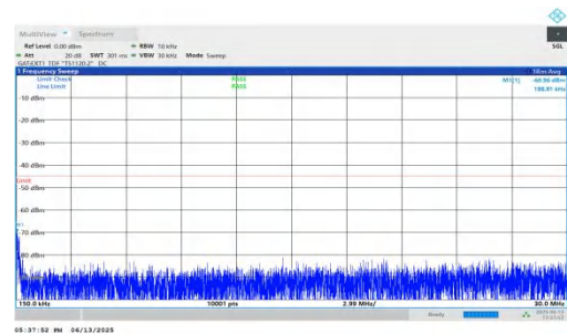
NTNV-n41-PC2-30-35-M-DFT-QPSK-Inner_1RB_Left-0.15-30-PASS
