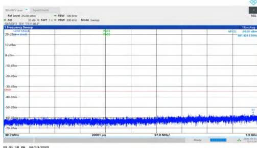
NTNV-n41-PC2-30-40-L-DFT-QPSK-Inner_1RB_Right-30-1000-PASS ASS
