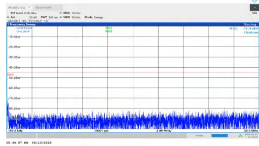
NTNV-n41-PC2-30-35-M-DFT-BPSK-Inner_1RB_Left-0.15-30-PASS
