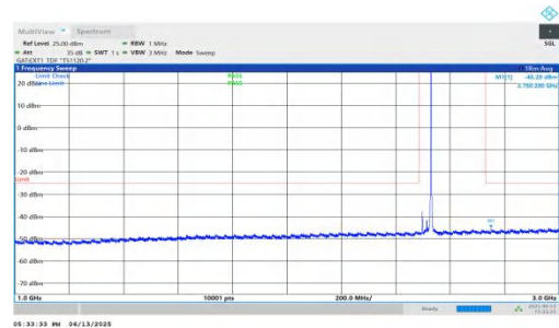
NTNV-n41-PC2-30-35-L-DFT-QPSK-Inner_1RB_Right-1000-3000-PASS PASS
