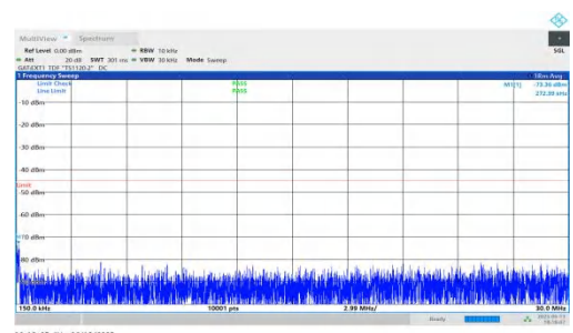
NTNV-n41-PC2-30-45-H-DFT-BPSK-Inner_1RB_Right-0.15-30-PASS
