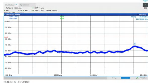
NTNV-n41-PC2-30-40-L-DFT-QPSK-Inner_1RB_Right-18000-3000-PASS 00-PASS
