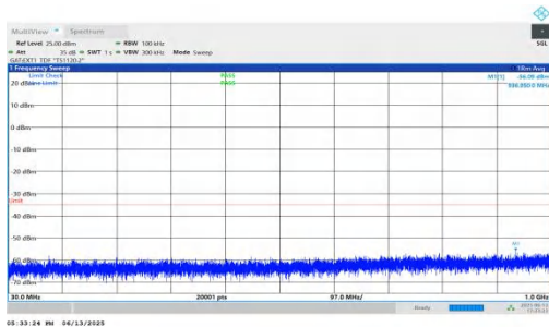
NTNV-n41-PC2-30-35-L-DFT-QPSK-Inner_1RB_Right-30-1000-PASS ASS
