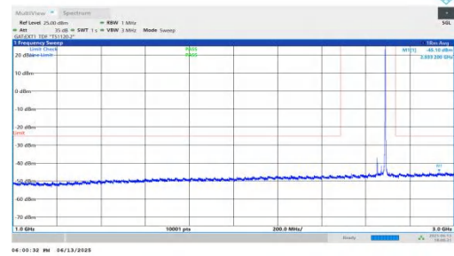
NTNV-n41-PC2-30-40-H-DFT-BPSK-Inner_1RB_Right-1000-3000 -PASS
