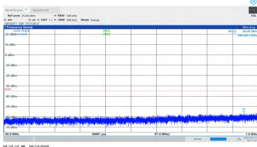
NTNV-n41-PC2-30-45-M-DFT-QPSK-Inner_1RB_Right-30-1000- PASS
