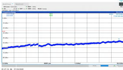
NTNV-n41-PC2-30-40-L-DFT-QPSK-Inner_1RB_Right-3000-18000-PASS 00-PASS
