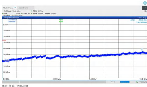
NTNV-n41-PC2-30-50-M-DFT-BPSK-Inner_1RB_Right-3000-18000-PASS
