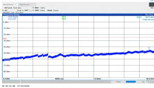
NTNV-n41-PC2-30-45-M-DFT-QPSK-Inner_1RB_Left-3000-1800 0-PASS
