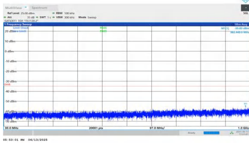
NTNV-n41-PC2-30-40-M-DFT-BPSK-Inner_1RB_Left-30-1000-PASS
