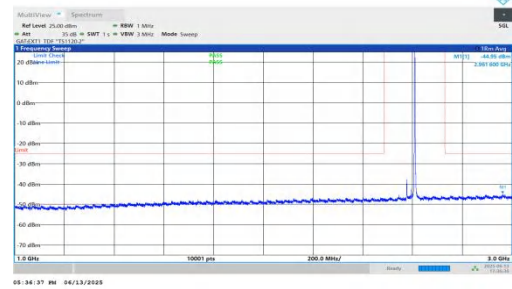
NTNV-n41-PC2-30-35-M-DFT-BPSK-Inner_1RB_Right-1000-3000-PASS
