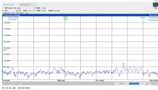
NTNV-n41-PC2-30-45-H-DFT-BPSK-Inner_1RB_Left-0.009-0.15-PASS
