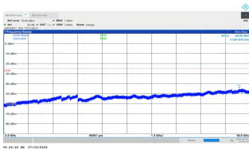
NTNV-n41-PC2-30-40-H-DFT-BPSK-Inner_1RB_Left-3000-18000-PASS
