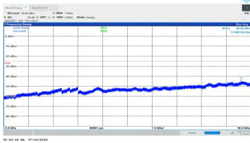
NTNV-n41-PC2-30-40-L-DFT-BPSK-Inner_1RB_Right-3000-18000-P PASS
