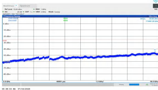
NTNV-n41-PC2-30-50-L-DFT-QPSK-Inner_1RB_Right-3000-18000-PASS 00-PASS
