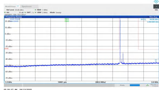
NTNV-n41-PC2-30-40-L-DFT-QPSK-Inner_1RB_Left-1000-3000-P PASS
