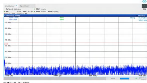
NTNV-n41-PC2-30-40-M-DFT-BPSK-Inner_1RB_Right-0.15-30-PASS
