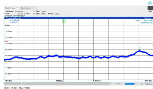
NTNV-n41-PC2-30-50-M-DFT-BPSK-Inner_1RB_Right-18000-30000-PASS
