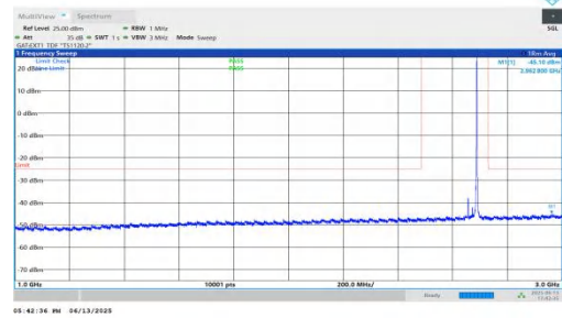
NTNV-n41-PC2-30-35-H-DFT-BPSK-Inner_1RB_Right-1000-3000 -PASS
