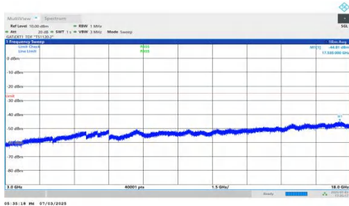
NTNV-n41-PC2-30-45-H-DFT-BPSK-Inner_1RB_Right-3000-180 00-PASS
