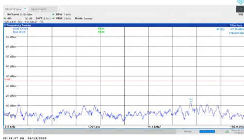
NTNV-n41-PC2-30-40-L-DFT-BPSK-Inner_1RB_Right-0.009-0.15-PASS
