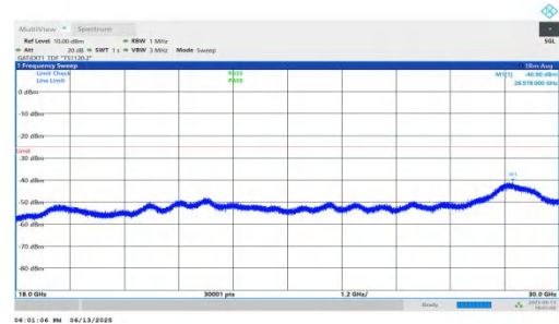
NTNV-n41-PC2-30-40-H-DFT-BPSK-Inner_1RB_Right-18000-300 00-PASS
