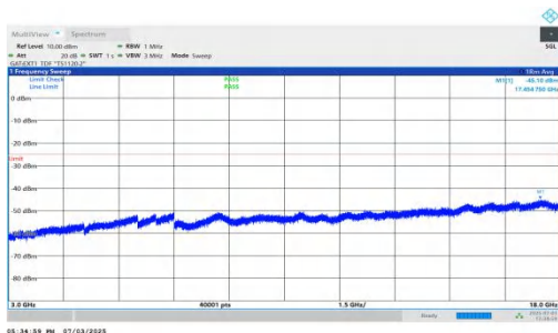
NTNV-n41-PC2-30-45-H-DFT-BPSK-Inner_1RB_Left-3000-18000-PASS
