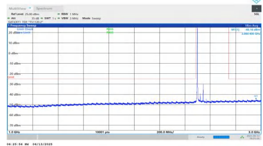
NTNV-n41-PC2-30-50-L-DFT-QPSK-Inner_1RB_Left-1000-3000-PASS
