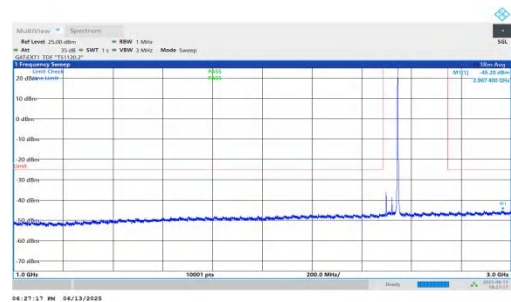
NTNV-n41-PC2-30-50-L-DFT-QPSK-Inner_1RB_Right-1000-3000-PASS PASS
