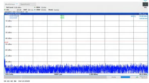
NTNV-n41-PC2-30-50-L-DFT-BPSK-Inner_1RB_Left-0.15-30-PAS S
