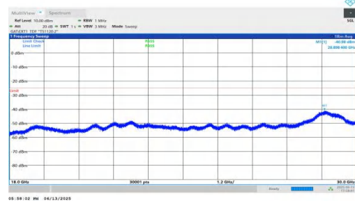
NTNV-n41-PC2-30-40-M-DFT-QPSK-Inner_1RB_Right-18000-3000- 00-PASS
