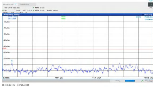
NTNV-n41-PC2-30-40-H-DFT-BPSK-Inner_1RB_Left-0.009-0.15-PASS
