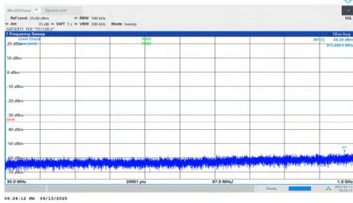
NTNV-n41-PC2-30-50-L-DFT-BPSK-Inner_1RB_Right-30-1000-PASS
