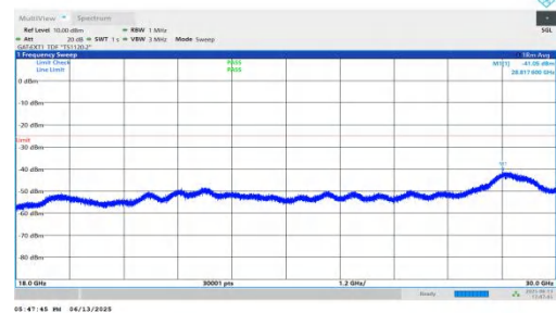
NTNV-n41-PC2-30-40-L-DFT-BPSK-Inner_1RB_Left-18000-30000-PASS
