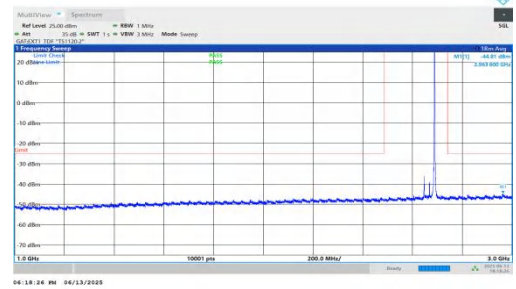
NTNV-n41-PC2-30-45-H-DFT-BPSK-Inner_1RB_Right-1000-3000 -PASS
