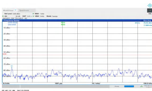
NTNV-n41-PC2-30-35-H-DFT-BPSK-Inner_1RB_Right-0.009-0.15-PASS
