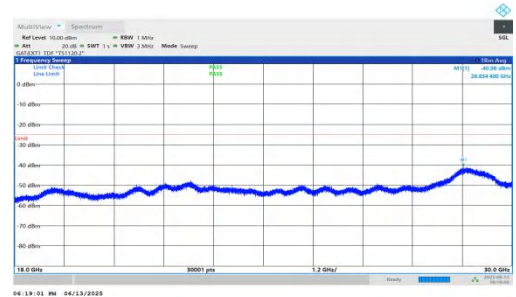
NTNV-n41-PC2-30-45-H-DFT-BPSK-Inner_1RB_Right-18000-300 00-PASS
