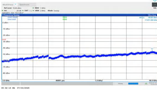
NTNV-n41-PC2-30-45-L-DFT-QPSK-Inner_1RB_Left-3000-18000 -PASS
