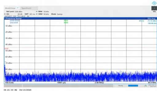
NTNV-n41-PC2-30-45-H-DFT-QPSK-Inner_1RB_Right-0.15-30-PA SS
