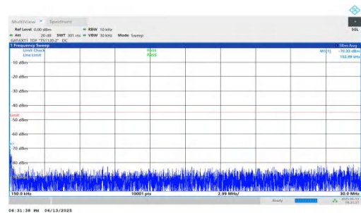
NTNV-n41-PC2-30-50-M-DFT-QPSK-Inner_1RB_Left-0.15-30-PASS
