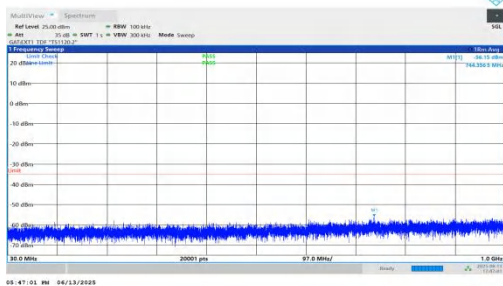
NTNV-n41-PC2-30-40-L-DFT-BPSK-Inner_1RB_Left-30-1000-PASS
