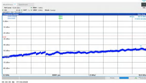
NTNV-n41-PC2-30-45-M-DFT-BPSK-Inner_1RB_Right-3000-18000-PASS
