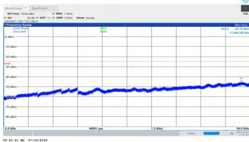
NTNV-n41-PC2-30-35-M-DFT-QPSK-Inner_1RB_Right-3000-18000- 00-PASS
