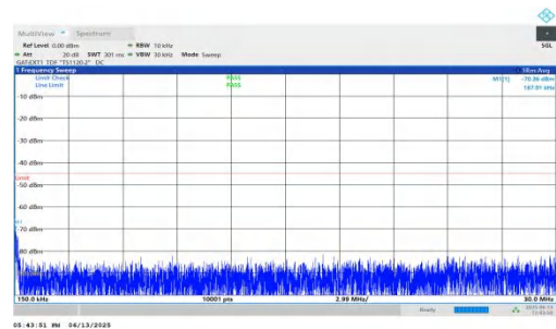
NTNV-n41-PC2-30-35-H-DFT-QPSK-Inner_1RB_Left-0.15-30-PAS S
