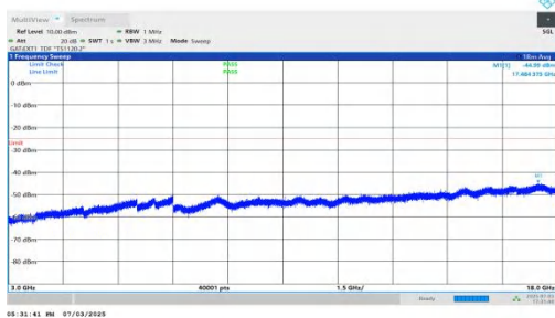
NTNV-n41-PC2-30-45-L-DFT-BPSK-Inner_1RB_Right-3000-18000-PASS
