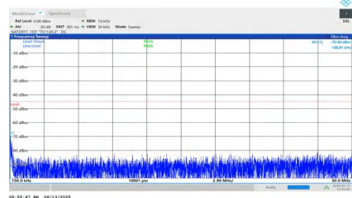
NTNV-n41-PC2-30-40-M-DFT-QPSK-Inner_1RB_Left-0.15-30-PASS
