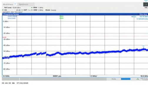
NTNV-n41-PC2-30-35-H-DFT-QPSK-Inner_1RB_Left-3000-1800 0-PASS
