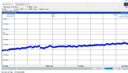
NTNV-n41-PC2-30-35-H-DFT-QPSK-Inner_1RB_Right-3000-180 00-PASS
