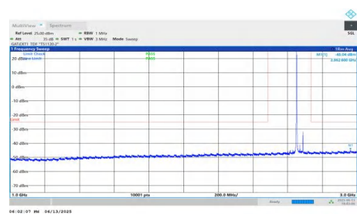
NTNV-n41-PC2-30-40-H-DFT-QPSK-Inner_1RB_Left-1000-3000- PASS
