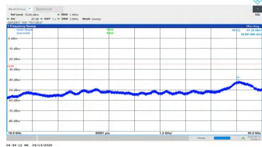
NTNV-n41-PC2-30-20-H-DFT-BPSK-Inner_1RB_Right-18000-300 00-PASS
