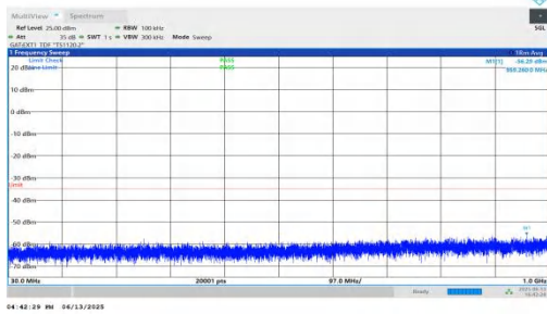
NTNV-n41-PC2-30-20-M-DFT-BPSK-Inner_1RB_Right-30-1000-PASS
