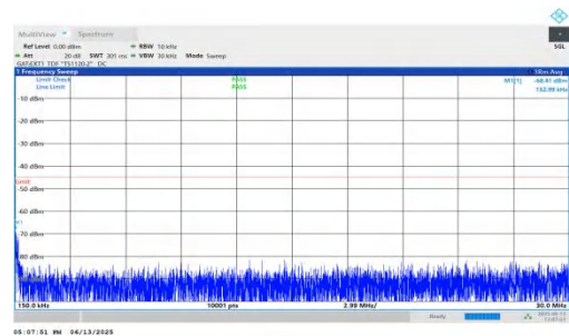
NTNV-n41-PC2-30-25-H-DFT-QPSK-Inner_1RB_Left-0.15-30-PAS S
