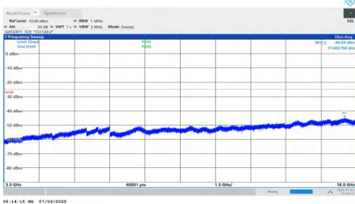
NTNV-n41-PC2-30-25-H-DFT-QPSK-Inner_1RB_Right-3000-18000- 00-PASS
