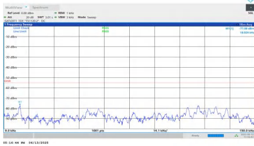
NTNV-n41-PC2-30-30-M-DFT-BPSK-Inner_1RB_Left-0.009-0.15-PASS
