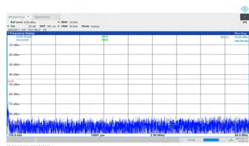
NTNV-n41-PC2-30-25-H-DFT-BPSK-Inner_1RB_Right-0.15-30-PASS
