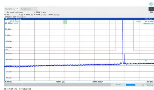
NTNV-n41-PC2-30-30-M-DFT-BPSK-Inner_1RB_Left-1000-3000-PASS
