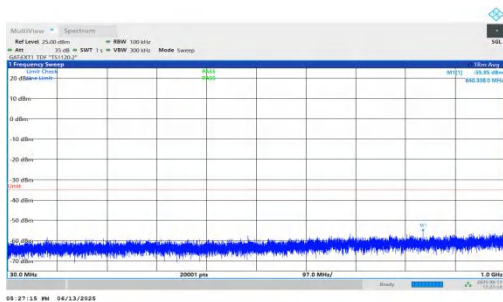
NTNV-n41-PC2-30-30-H-DFT-QPSK-Inner_1RB_Right-30-1000- PASS
