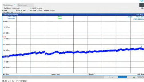
NTNV-n41-PC2-30-25-L-DFT-BPSK-Inner_1RB_Right-3000-18000-PASS
