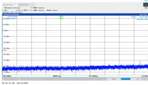
NTNV-n41-PC2-30-20-L-DFT-BPSK-Inner_1RB_Left-30-1000-PA
