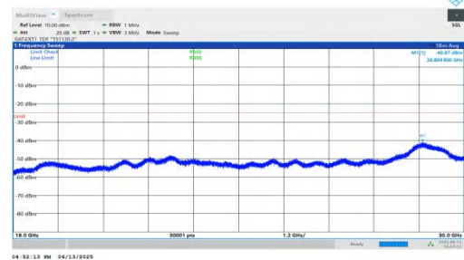
NTNV-n41-PC2-30-20-H-DFT-QPSK-Inner_1RB_Right-18000-30000-PASS
