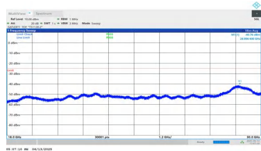
NTNV-n41-PC2-30-25-H-DFT-BPSK-Inner_1RB_Right-18000-300 00-PASS
