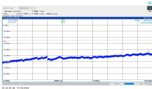
NTNV-n41-PC2-30-30-H-DFT-BPSK-Inner_1RB_Right-3000-180 00-PASS
