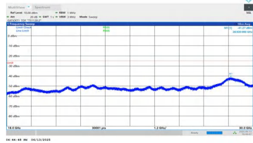
NTNV-n41-PC2-30-20-M-DFT-QPSK-Inner_1RB_Left-18000-3000 0-PASS
