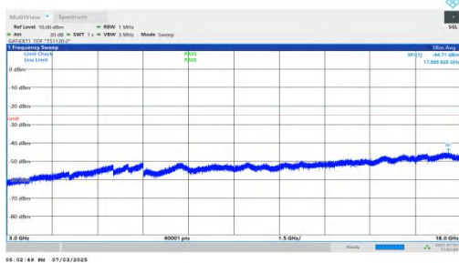
NTNV-n41-PC2-30-15-H-DFT-QPSK-Inner_1RB_Right-3000-18000-PASS
