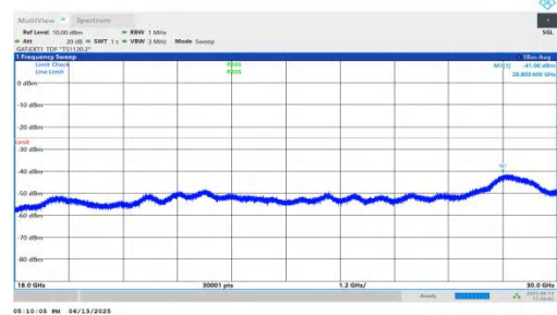
NTNV-n41-PC2-30-25-H-DFT-QPSK-Inner_1RB_Right-18000-30000- 00-PASS
