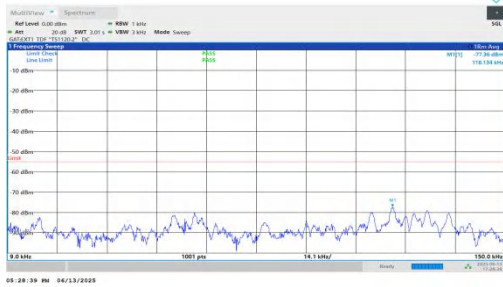
NTNV-n41-PC2-30-35-L-DFT-BPSK-Inner_1RB_Left-0.009-0.15- PASS
