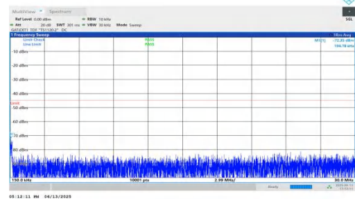
NTNV-n41-PC2-30-30-L-DFT-BPSK-Inner_1RB_Right-0.15-30-PA SS
