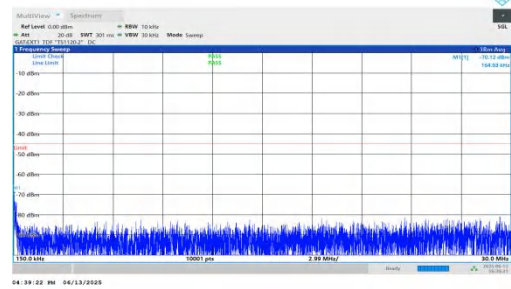
NTNV-n41-PC2-30-20-L-DFT-QPSK-Inner_1RB_Right-0.15-30-PASS SS
