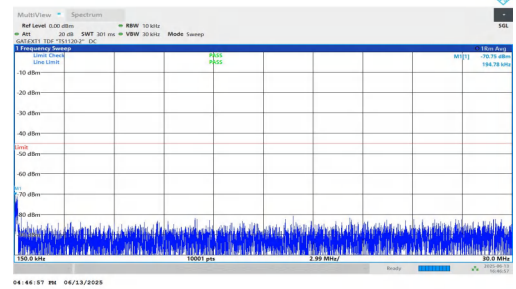
NTNV-n41-PC2-30-20-H-DFT-BPSK-Inner_1RB_Left-0.15-30-PAS
