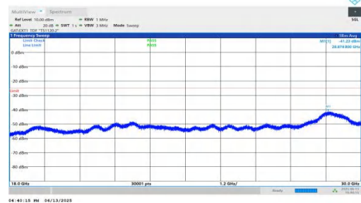
NTNV-n41-PC2-30-20-L-DFT-QPSK-Inner_1RB_Right-18000-3000-PASS 00-PASS
