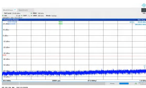
NTNV-n41-PC2-30-30-H-DFT-QPSK-Inner_1RB_Left-30-1000-P ASS
