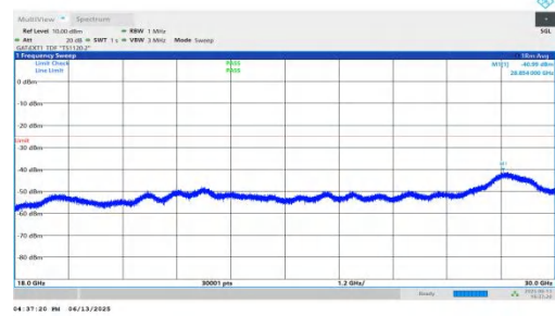
NTNV-n41-PC2-30-20-L-DFT-BPSK-Inner_1RB_Right-18000-3000-PASS
