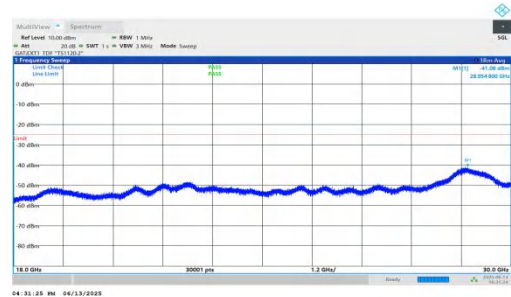
NTNV-n41-PC2-30-15-H-DFT-BPSK-Inner_1RB_Right-18000-300 00-PASS
