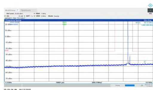
NTNV-n41-PC2-30-30-H-DFT-QPSK-Inner_1RB_Left-1000-3000- PASS
