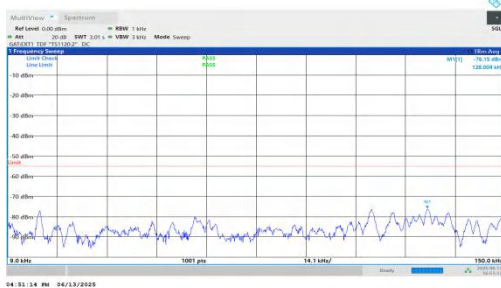
NTNV-n41-PC2-30-20-H-DFT-QPSK-Inner_1RB_Right-0.009-0.1 5-PASS
