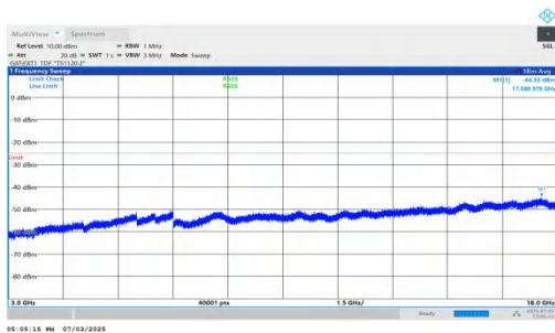
NTNV-n41-PC2-30-20-M-DFT-BPSK-Inner_1RB_Left-3000-18000-PASS
