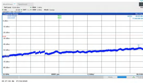
NTNV-n41-PC2-30-20-H-DFT-QPSK-Inner_1RB_Left-3000-1800 0-PASS
