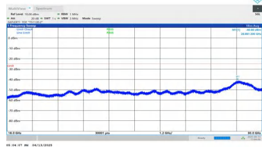
NTNV-n41-PC2-30-25-M-DFT-QPSK-Inner_1RB_Right-18000-3000- 00-PASS
