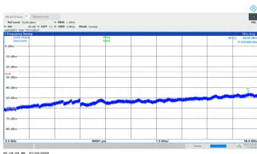
NTNV-n41-PC2-30-30-H-DFT-BPSK-Inner_1RB_Left-3000-18000-PASS
