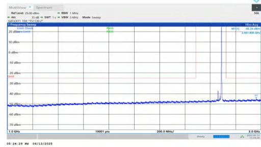
NTNV-n41-PC2-30-30-H-DFT-BPSK-Inner_1RB_Right-1000-3000 -PASS
