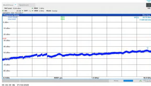
NTNV-n41-PC2-30-20-L-DFT-QPSK-Inner_1RB_Right-3000-18000-PASS 00-PASS
