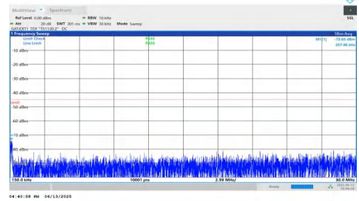
NTNV-n41-PC2-30-20-M-DFT-BPSK-Inner_1RB_Left-0.15-30-PASS
