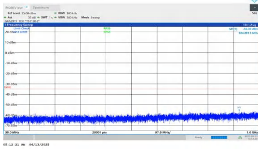
NTNV-n41-PC2-30-30-L-DFT-BPSK-Inner_1RB_Right-30-1000-P ASS
