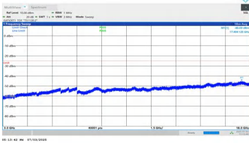
NTNV-n41-PC2-30-25-H-DFT-QPSK-Inner_1RB_Left-3000-1800 0-PASS
