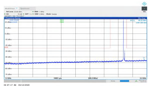
NTNV-n41-PC2-30-20-H-DFT-BPSK-Inner_1RB_Left-1000-3000-PASS
