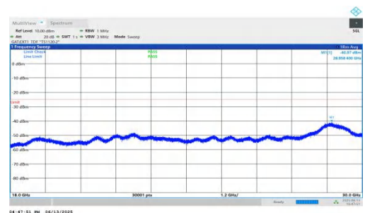
NTNV-n41-PC2-30-20-H-DFT-BPSK-Inner_1RB_Left-18000-30000-PASS
