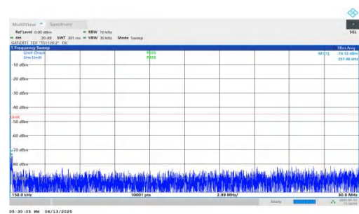
NTNV-n41-PC2-30-35-L-DFT-BPSK-Inner_1RB_Right-0.15-30-PASS
