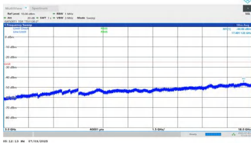
NTNV-n41-PC2-30-25-M-DFT-QPSK-Inner_1RB_Right-3000-18000- 00-PASS
