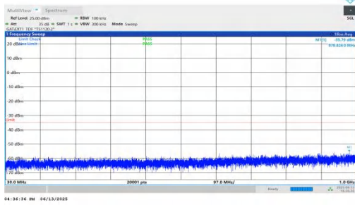
NTNV-n41-PC2-30-20-L-DFT-BPSK-Inner_1RB_Right-30-1000-P ASS
