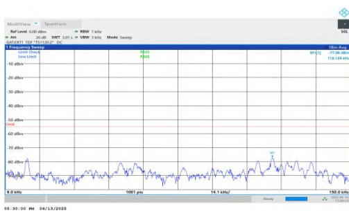
NTNV-n41-PC2-30-35-L-DFT-BPSK-Inner_1RB_Right-0.009-0.15- PASS
