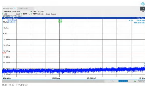
NTNV-n41-PC2-30-25-H-DFT-BPSK-Inner_1RB_Left-30-1000-PASS
