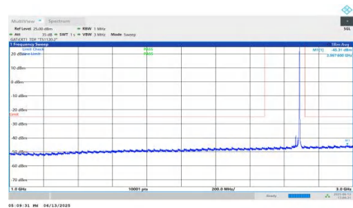
NTNV-n41-PC2-30-25-H-DFT-QPSK-Inner_1RB_Right-1000-3000- -PASS
