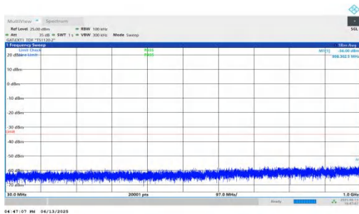
NTNV-n41-PC2-30-20-H-DFT-BPSK-Inner_1RB_Left-30-1000-PASS
