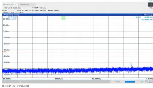
NTNV-n41-PC2-30-25-M-DFT-BPSK-Inner_1RB_Right-30-1000-PASS
