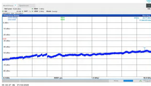
NTNV-n41-PC2-30-20-M-DFT-QPSK-Inner_1RB_Right-3000-18000- 00-PASS
