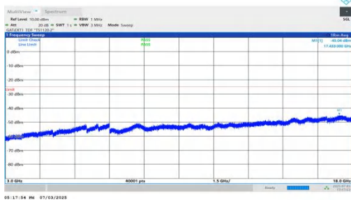
NTNV-n41-PC2-30-30-M-DFT-QPSK-Inner_1RB_Right-3000-18000- 00-PASS
