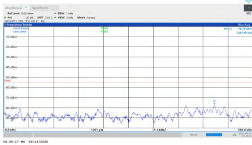
NTNV-n41-PC2-30-20-L-DFT-QPSK-Inner_1RB_Right-0.009-0.1 5-PASS
