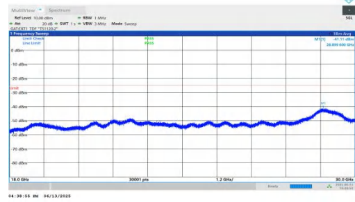
NTNV-n41-PC2-30-20-L-DFT-QPSK-Inner_1RB_Left-18000-3000 0-PASS
