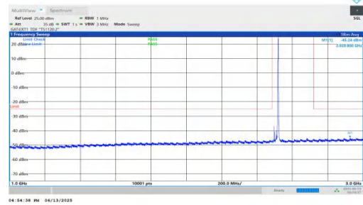
NTNV-n41-PC2-30-25-L-DFT-BPSK-Inner_1RB_Right-1000-3000-PASS
