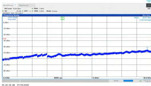
NTNV-n41-PC2-30-20-M-DFT-BPSK-Inner_1RB_Right-3000-18000-PASS
