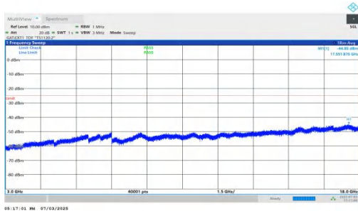
NTNV-n41-PC2-30-30-M-DFT-BPSK-Inner_1RB_Right-3000-18000-PASS
