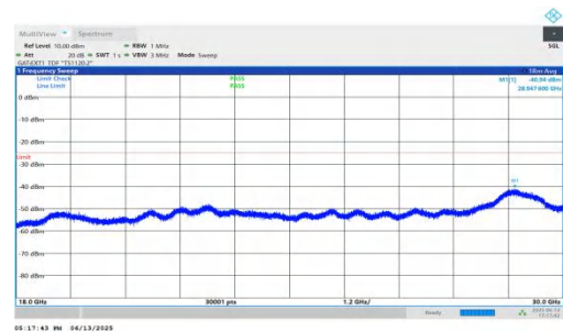
NTNV-n41-PC2-30-30-M-DFT-BPSK-Inner_1RB_Left-18000-30000-PASS
