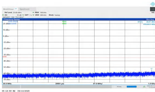
NTNV-n41-PC2-30-30-M-DFT-BPSK-Inner_1RB_Left-30-1000-PASS
