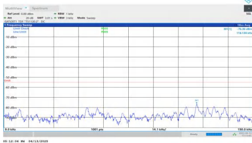
NTNV-n41-PC2-30-30-L-DFT-BPSK-Inner_1RB_Right-0.009-0.15 -PASS
