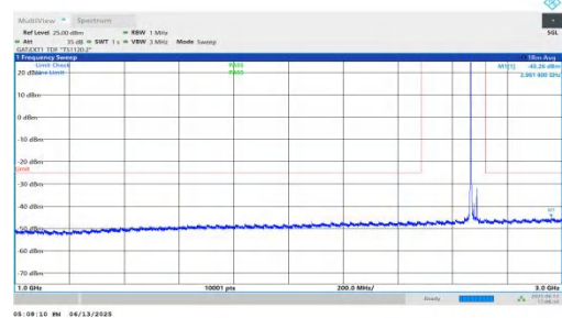
NTNV-n41-PC2-30-25-H-DFT-QPSK-Inner_1RB_Left-1000-3000- PASS
