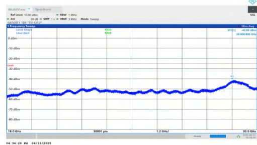
NTNV-n41-PC2-30-15-H-DFT-QPSK-Inner_1RB_Right-18000-30000-PASS
