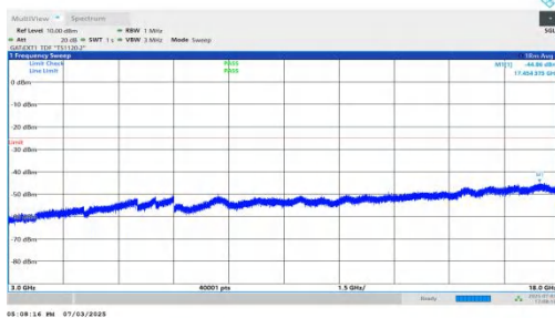
NTNV-n41-PC2-30-20-H-DFT-QPSK-Inner_1RB_Right-3000-18000-PASS
