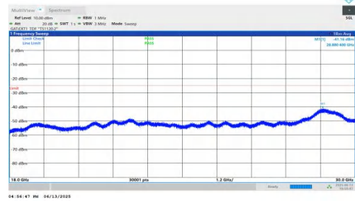
NTNV-n41-PC2-30-25-L-DFT-QPSK-Inner_1RB_Left-18000-3000 0-PASS
