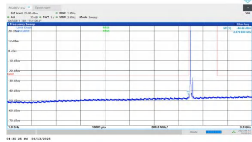
NTNV-n41-PC2-30-20-L-DFT-BPSK-Inner_1RB_Left-1000-3000-P
