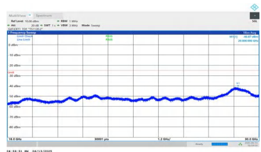
NTNV-n41-PC2-30-25-M-DFT-BPSK-Inner_1RB_Left-18000-30000-PASS
