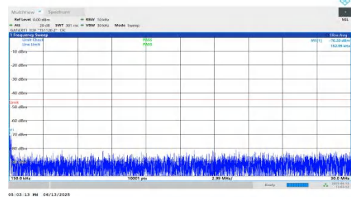
NTNV-n41-PC2-30-25-M-DFT-QPSK-Inner_1RB_Right-0.15-30-P ASS
