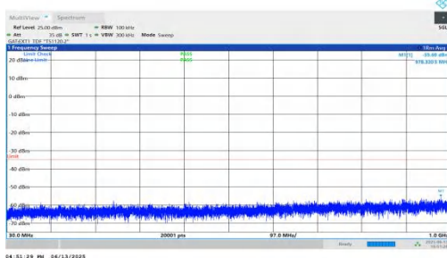
NTNV-n41-PC2-30-20-H-DFT-QPSK-Inner_1RB_Right-30-1000-PASS
