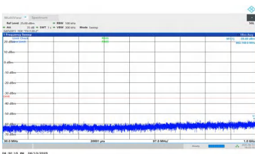
NTNV-n41-PC2-30-15-H-DFT-QPSK-Inner_1RB_Left-30-1000-P ASS
