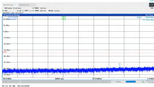
NTNV-n41-PC2-30-30-L-DFT-BPSK-Inner_1RB_Left-30-1000-PA SS
