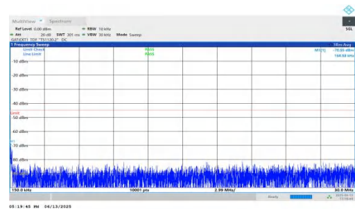
NTNV-n41-PC2-30-30-M-DFT-QPSK-Inner_1RB_Left-0.15-30-PASS
