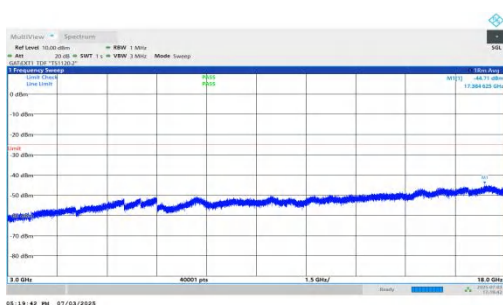
NTNV-n41-PC2-30-30-H-DFT-QPSK-Inner_1RB_Right-3000-18000- 00-PASS
