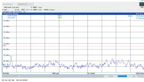
NTNV-n41-PC2-30-30-H-DFT-BPSK-Inner_1RB_Left-0.009-0.15-PASS
