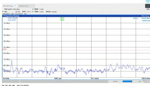
NTNV-n41-PC2-30-25-L-DFT-QPSK-Inner_1RB_Left-0.009-0.15-PASS
