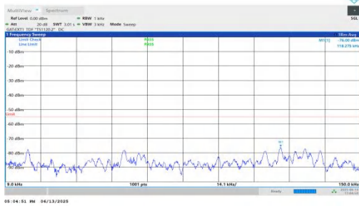
NTNV-n41-PC2-30-25-H-DFT-BPSK-Inner_1RB_Left-0.009-0.15-PASS
