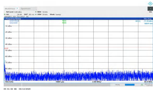
NTNV-n41-PC2-30-25-M-DFT-QPSK-Inner_1RB_Left-0.15-30-PASS
