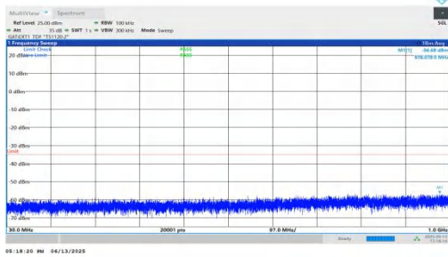
NTNV-n41-PC2-30-30-M-DFT-BPSK-Inner_1RB_Right-30-1000-PASS
