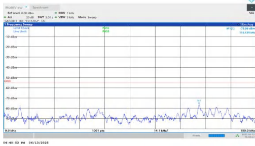
NTNV-n41-PC2-30-20-M-DFT-BPSK-Inner_1RB_Left-0.009-0.15-PASS
