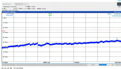
NTNV-n41-PC2-30-25-L-DFT-QPSK-Inner_1RB_Right-3000-18000 00-PASS
