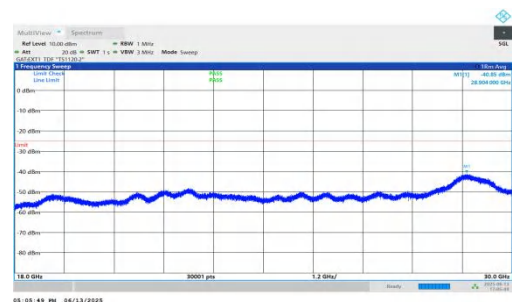
NTNV-n41-PC2-30-25-H-DFT-BPSK-Inner_1RB_Left-18000-30000-PASS
