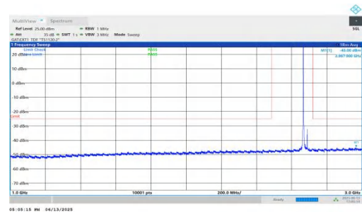
NTNV-n41-PC2-30-25-H-DFT-BPSK-Inner_1RB_Left-1000-3000-PASS
