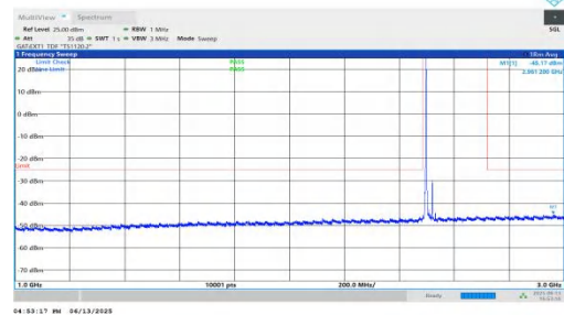
NTNV-n41-PC2-30-25-L-DFT-BPSK-Inner_1RB_Left-1000-3000-P ASS
