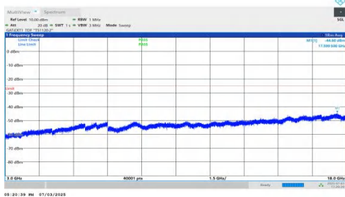
NTNV-n41-PC2-30-35-L-DFT-BPSK-Inner_1RB_Right-3000-18000-PASS
