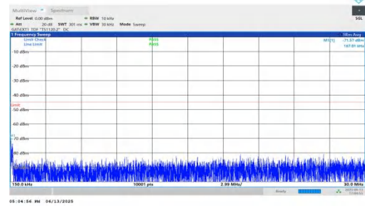
NTNV-n41-PC2-30-25-H-DFT-BPSK-Inner_1RB_Left-0.15-30-PAS
