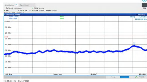
NTNV-n41-PC2-30-25-L-DFT-BPSK-Inner_1RB_Right-18000-3000-PASS
