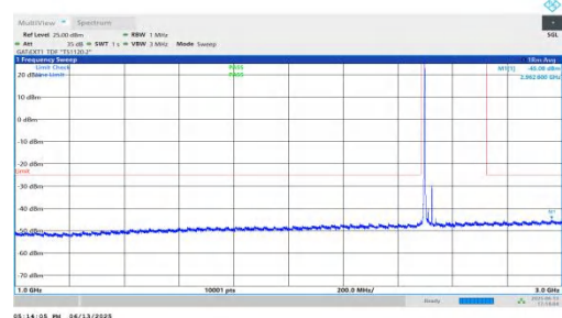
NTNV-n41-PC2-30-30-L-DFT-QPSK-Inner_1RB_Left-1000-3000-P PASS
