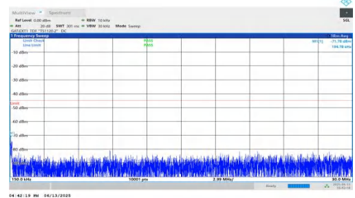
NTNV-n41-PC2-30-20-M-DFT-BPSK-Inner_1RB_Right-0.15-30-PASS
