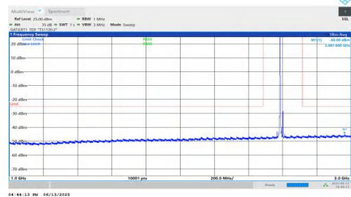
NTNV-n41-PC2-30-20-M-DFT-QPSK-Inner_1RB_Left-1000-3000-PASS
