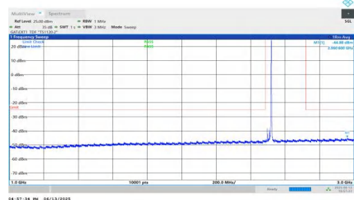
NTNV-n41-PC2-30-25-L-DFT-QPSK-Inner_1RB_Right-1000-3000- PASS
