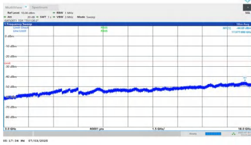
NTNV-n41-PC2-30-30-M-DFT-QPSK-Inner_1RB_Left-3000-1800 0-PASS
