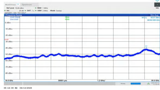
NTNV-n41-PC2-30-30-L-DFT-QPSK-Inner_1RB_Left-18000-3000 0-PASS
