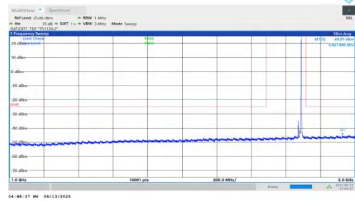
NTNV-n41-PC2-30-20-H-DFT-BPSK-Inner_1RB_Right-1000-3000 -PASS
