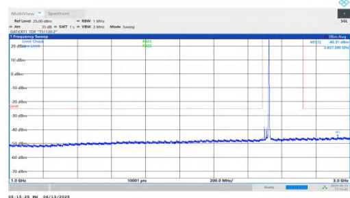
NTNV-n41-PC2-30-30-L-DFT-QPSK-Inner_1RB_Right-1000-3000-PASS PASS
