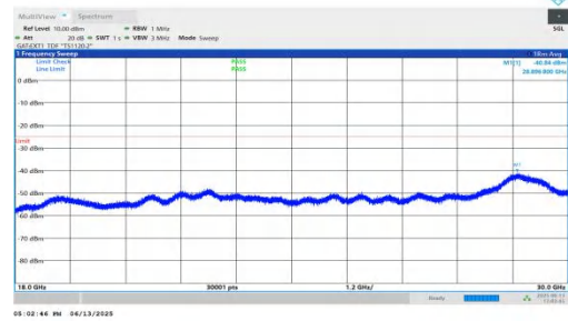
NTNV-n41-PC2-30-25-M-DFT-QPSK-Inner_1RB_Left-18000-3000 0-PASS
