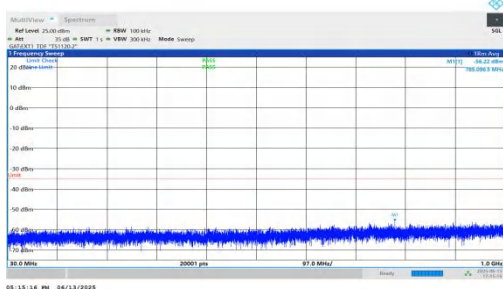
NTNV-n41-PC2-30-30-L-DFT-QPSK-Inner_1RB_Right-30-1000-PASS ASS
