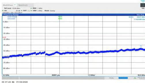
NTNV-n41-PC2-30-20-H-DFT-BPSK-Inner_1RB_Right-3000-180 00-PASS
