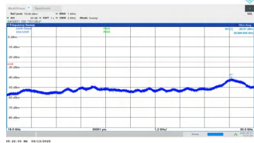
NTNV-n41-PC2-30-30-M-DFT-QPSK-Inner_1RB_Right-18000-3000- 00-PASS
