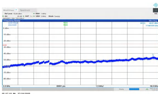
NTNV-n41-PC2-30-20-H-DFT-BPSK-Inner_1RB_Left-3000-18000-PASS
