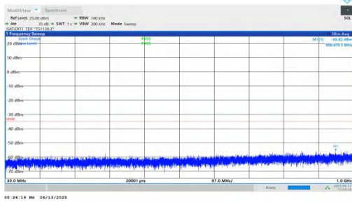
NTNV-n41-PC2-30-30-H-DFT-BPSK-Inner_1RB_Right-30-1000-P ASS
