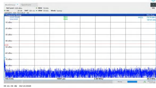
NTNV-n41-PC2-30-30-M-DFT-QPSK-Inner_1RB_Right-0.15-30-P ASS
