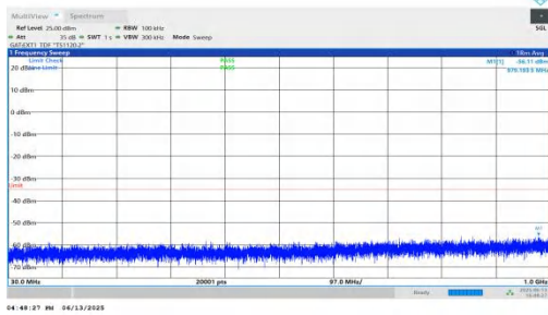
NTNV-n41-PC2-30-20-H-DFT-BPSK-Inner_1RB_Right-30-1000-P ASS
