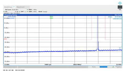
NTNV-n41-PC2-30-20-M-DFT-BPSK-Inner_1RB_Left-1000-3000-PASS
