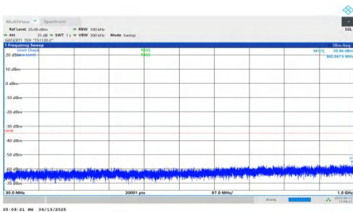
NTNV-n41-PC2-30-25-H-DFT-QPSK-Inner_1RB_Right-30-1000- PASS
