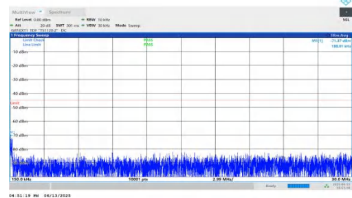
NTNV-n41-PC2-30-20-H-DFT-QPSK-Inner_1RB_Right-0.15-30-PA SS
