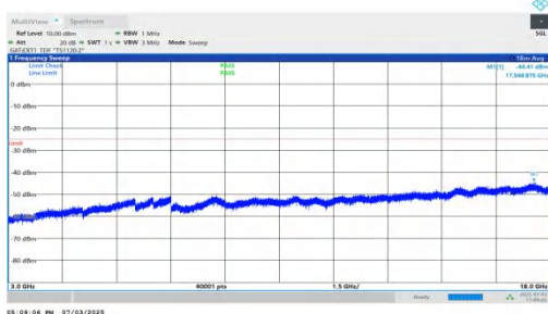
NTNV-n41-PC2-30-25-L-DFT-BPSK-Inner_1RB_Left-3000-18000 -PASS
