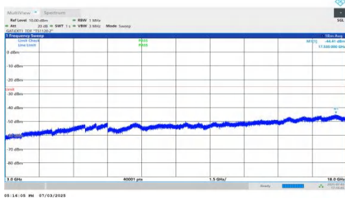
NTNV-n41-PC2-30-30-L-DFT-QPSK-Inner_1RB_Right-3000-18000-PASS 00-PASS
