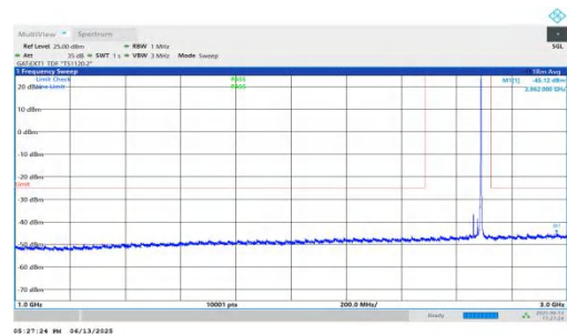
NTNV-n41-PC2-30-30-H-DFT-QPSK-Inner_1RB_Right-1000-3000- -PASS
