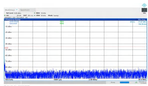
NTNV-n41-PC2-30-30-H-DFT-BPSK-Inner_1RB_Right-0.15-30-PASS
