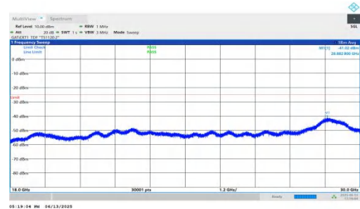
NTNV-n41-PC2-30-30-M-DFT-BPSK-Inner_1RB_Right-18000-3000-PASS
