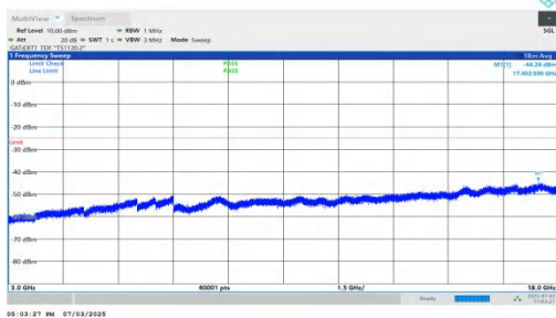
NTNV-n41-PC2-30-20-L-DFT-BPSK-Inner_1RB_Left-3000-18000-PASS
