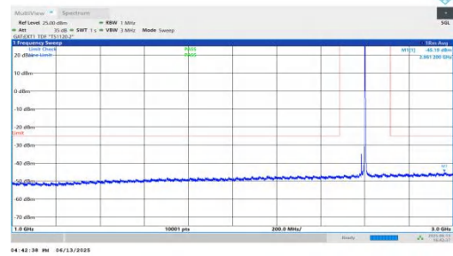
NTNV-n41-PC2-30-20-M-DFT-BPSK-Inner_1RB_Right-1000-3000-PASS
