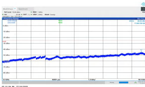
NTNV-n41-PC2-30-25-M-DFT-BPSK-Inner_1RB_Left-3000-18000-PASS
