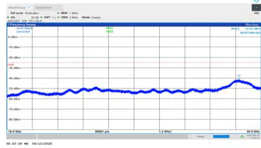
NTNV-n41-PC2-30-30-M-DFT-QPSK-Inner_1RB_Left-18000-3000 0-PASS
