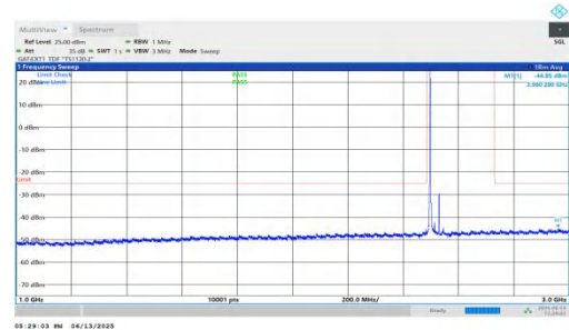
NTNV-n41-PC2-30-35-L-DFT-BPSK-Inner_1RB_Left-1000-3000-PASS
