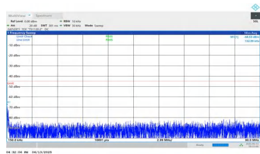
NTNV-n41-PC2-30-15-H-DFT-QPSK-Inner_1RB_Left-0.15-30-PAS S
