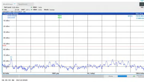
NTNV-n41-PC2-30-20-L-DFT-BPSK-Inner_1RB_Left-0.009-0.15-PASS
