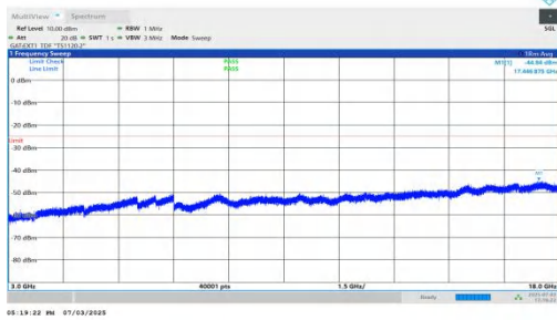
NTNV-n41-PC2-30-30-H-DFT-QPSK-Inner_1RB_Left-3000-1800 0-PASS
