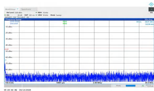
NTNV-n41-PC2-30-30-H-DFT-QPSK-Inner_1RB_Left-0.15-30-PAS S
