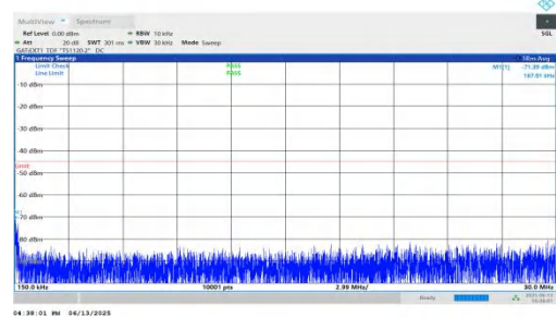
NTNV-n41-PC2-30-20-L-DFT-QPSK-Inner_1RB_Left-0.15-30-PASS
