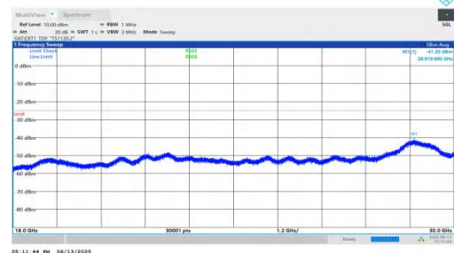
NTNV-n41-PC2-30-30-L-DFT-BPSK-Inner_1RB_Left-18000-30000 -PASS
