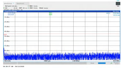
NTNV-n41-PC2-30-25-M-DFT-BPSK-Inner_1RB_Left-0.15-30-PASS
