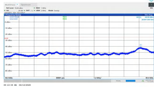
NTNV-n41-PC2-30-30-L-DFT-BPSK-Inner_1RB_Right-18000-30000-P PASS
