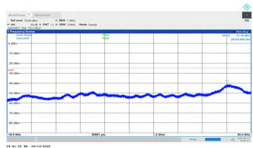
NTNV-n41-PC2-30-20-M-DFT-BPSK-Inner_1RB_Left-18000-30000-PASS
