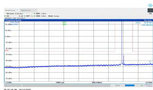
NTNV-n41-PC2-30-30-M-DFT-QPSK-Inner_1RB_Left-1000-3000-PASS
