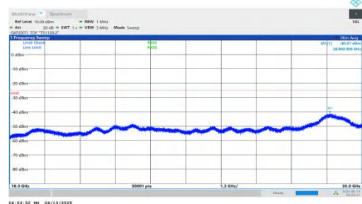
NTNV-n41-PC2-30-25-L-DFT-BPSK-Inner_1RB_Left-18000-30000 -PASS
