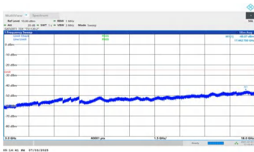
NTNV-n41-PC2-30-30-M-DFT-BPSK-Inner_1RB_Left-3000-18000-PASS
