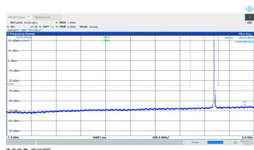
NTNV-n41-PC2-30-15-H-DFT-QPSK-Inner_1RB_Left-1000-3000- PASS
