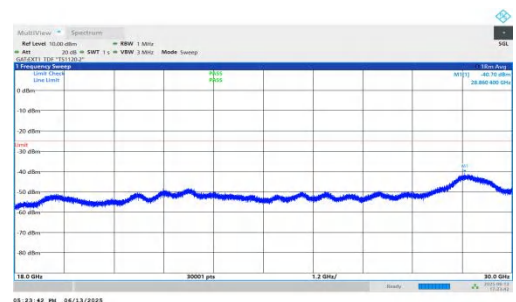
NTNV-n41-PC2-30-30-H-DFT-BPSK-Inner_1RB_Left-18000-30000-PASS
