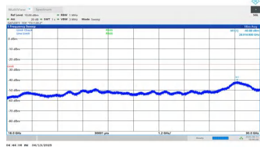
NTNV-n41-PC2-30-20-M-DFT-QPSK-Inner_1RB_Right-18000-300 00-PASS
