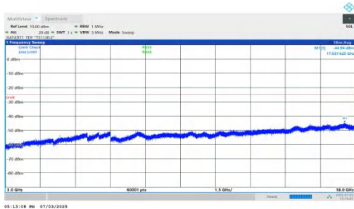
NTNV-n41-PC2-30-25-H-DFT-BPSK-Inner_1RB_Right-3000-180 00-PASS
