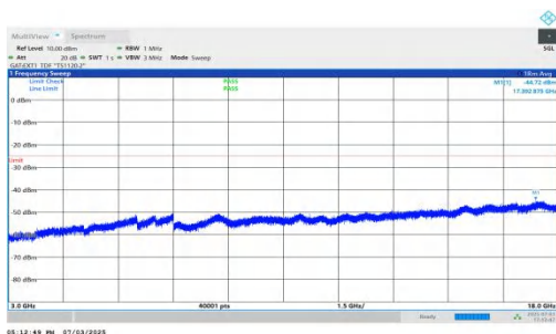
NTNV-n41-PC2-30-25-H-DFT-BPSK-Inner_1RB_Left-3000-18000-PASS
