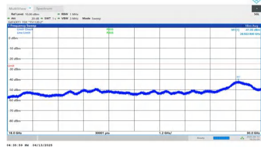
NTNV-n41-PC2-30-20-L-DFT-BPSK-Inner_1RB_Left-18000-30000-PASS
