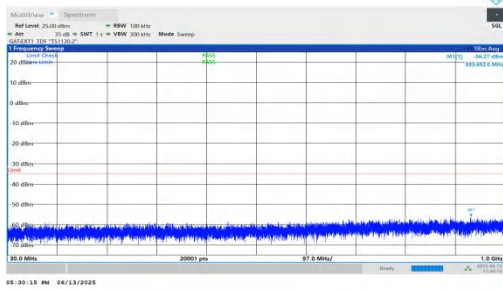
NTNV-n41-PC2-30-35-L-DFT-BPSK-Inner_1RB_Right-30-1000-P ASS
