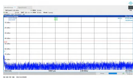
NTNV-n41-PC2-30-20-H-DFT-QPSK-Inner_1RB_Left-0.15-30-PAS S
