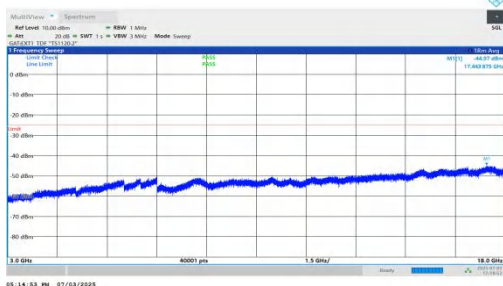
NTNV-n41-PC2-30-30-L-DFT-BPSK-Inner_1RB_Left-3000-18000 -PASS
