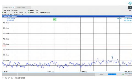
NTNV-n41-PC2-30-25-M-DFT-QPSK-Inner_1RB_Left-0.009-0.15-PASS
