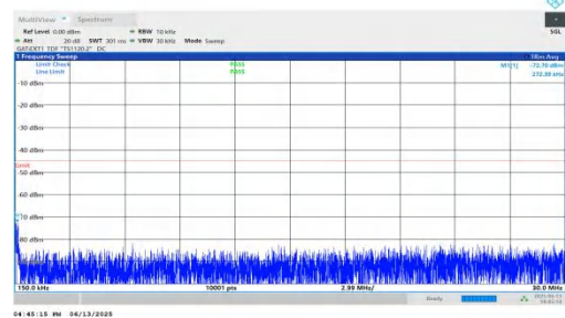
NTNV-n41-PC2-30-20-M-DFT-QPSK-Inner_1RB_Right-0.15-30-P ASS
