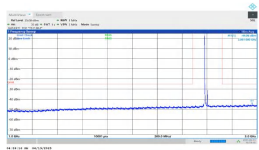
NTNV-n41-PC2-30-25-M-DFT-BPSK-Inner_1RB_Left-1000-3000-PASS
