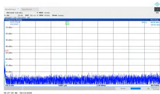
NTNV-n41-PC2-30-30-H-DFT-QPSK-Inner_1RB_Right-0.15-30-PA SS
