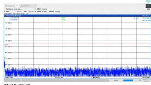
NTNV-n41-PC2-30-20-M-DFT-QPSK-Inner_1RB_Left-0.15-30-PASS
