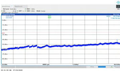
NTNV-n41-PC2-30-15-H-DFT-BPSK-Inner_1RB_Right-3000-180 00-PASS
