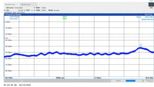
NTNV-n41-PC2-30-30-H-DFT-QPSK-Inner_1RB_Left-18000-3000 0-PASS
