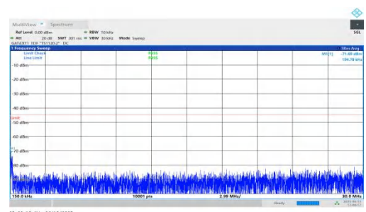
NTNV-n41-PC2-30-25-M-DFT-BPSK-Inner_1RB_Right-0.15-30-PASS
