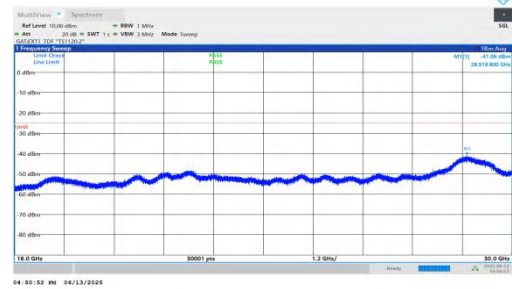
NTNV-n41-PC2-30-20-H-DFT-QPSK-Inner_1RB_Left-18000-3000 0-PASS
