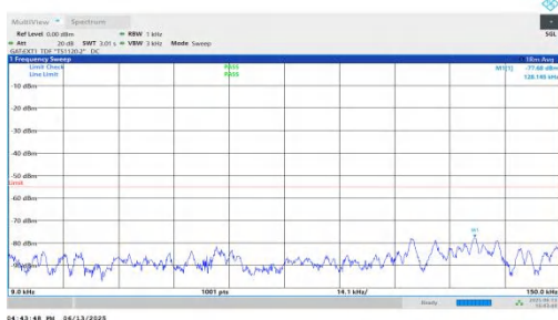
NTNV-n41-PC2-30-20-M-DFT-QPSK-Inner_1RB_Left-0.009-0.15-PASS
