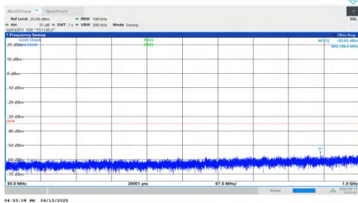
NTNV-n41-PC2-30-25-L-DFT-BPSK-Inner_1RB_Left-30-1000-PA SS
