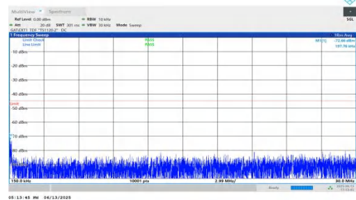
NTNV-n41-PC2-30-30-L-DFT-QPSK-Inner_1RB_Left-0.15-30-P PASS
