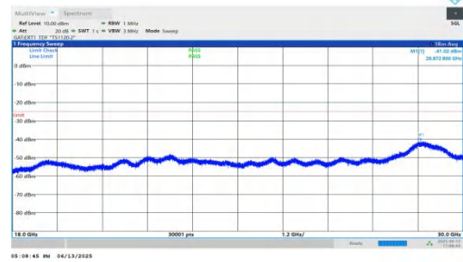
NTNV-n41-PC2-30-25-H-DFT-QPSK-Inner_1RB_Left-18000-3000 0-PASS
