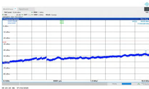
NTNV-n41-PC2-30-35-L-DFT-BPSK-Inner_1RB_Left-3000-18000- PASS
