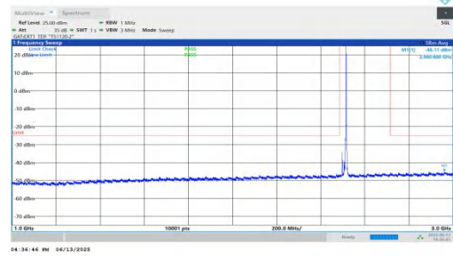
NTNV-n41-PC2-30-20-L-DFT-BPSK-Inner_1RB_Right-1000-3000-PASS
