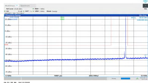
NTNV-n41-PC2-30-20-H-DFT-QPSK-Inner_1RB_Right-1000-3000-PASS
