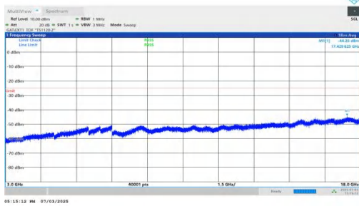
NTNV-n41-PC2-30-30-L-DFT-BPSK-Inner_1RB_Right-3000-18000-P PASS
