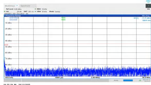
NTNV-n41-PC2-30-25-L-DFT-QPSK-Inner_1RB_Left-0.15-30-PASS
