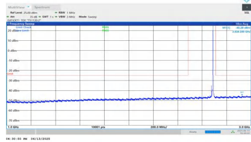
NTNV-n41-PC2-30-15-H-DFT-BPSK-Inner_1RB_Right-1000-3000 -PASS
