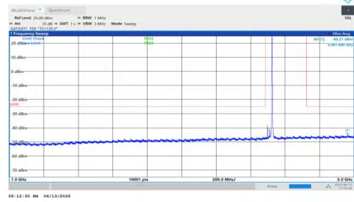
NTNV-n41-PC2-30-30-L-DFT-BPSK-Inner_1RB_Right-1000-3000-P PASS
