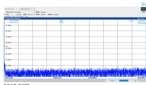
NTNV-n41-PC2-30-30-M-DFT-BPSK-Inner_1RB_Right-0.15-30-PASS
