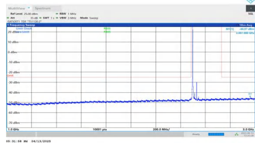
NTNV-n41-PC2-30-35-L-DFT-QPSK-Inner_1RB_Left-1000-3000-PASS
