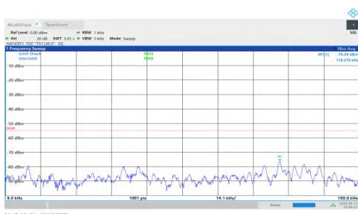
NTNV-n41-PC2-30-20-H-DFT-BPSK-Inner_1RB_Right-0.009-0.15-PASS
