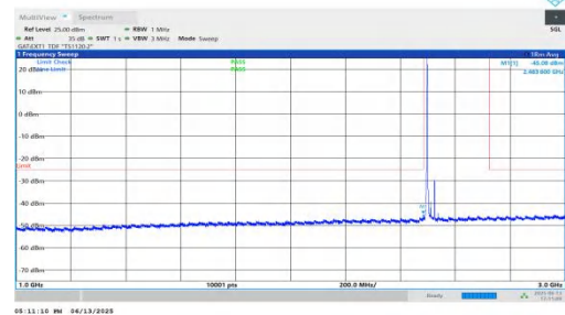
NTNV-n41-PC2-30-30-L-DFT-BPSK-Inner_1RB_Left-1000-3000-P ASS
