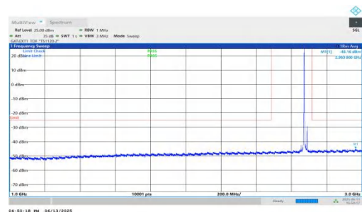
NTNV-n41-PC2-30-20-H-DFT-QPSK-Inner_1RB_Left-1000-3000- PASS
