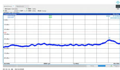
NTNV-n41-PC2-30-25-M-DFT-BPSK-Inner_1RB_Right-18000-30000-PASS
