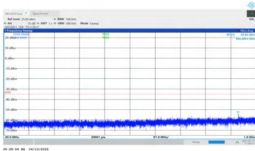
NTNV-n41-PC2-30-35-L-DFT-BPSK-Inner_1RB_Left-30-1000-PASS
