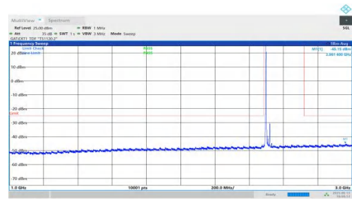
NTNV-n41-PC2-30-25-L-DFT-QPSK-Inner_1RB_Left-1000-3000-PASS
