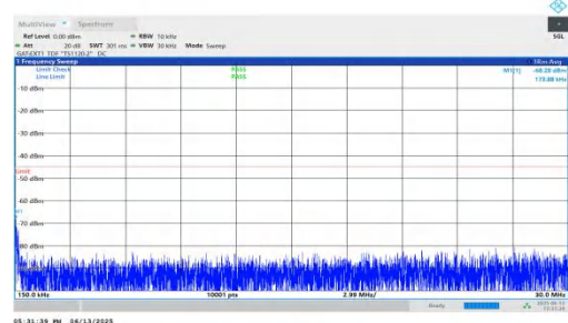
NTNV-n41-PC2-30-35-L-DFT-QPSK-Inner_1RB_Left-0.15-30-PASS
