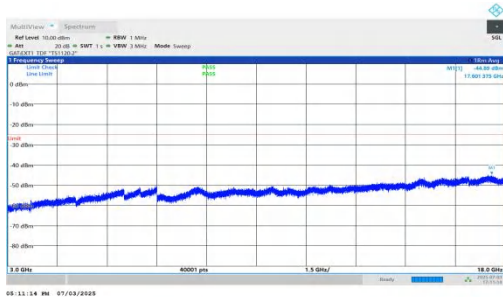
NTNV-n41-PC2-30-25-M-DFT-BPSK-Inner_1RB_Right-3000-18000-PASS
