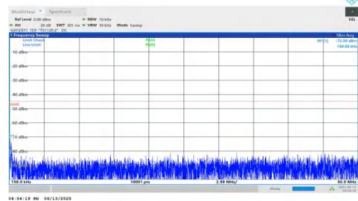
NTNV-n41-PC2-30-25-L-DFT-BPSK-Inner_1RB_Right-0.15-30-PA SS
