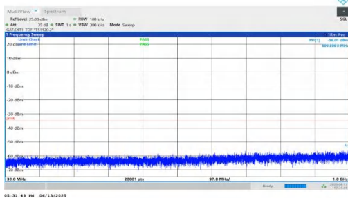
NTNV-n41-PC2-30-35-L-DFT-QPSK-Inner_1RB_Left-30-1000-PASS
