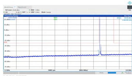
NTNV-n41-PC2-30-20-L-DFT-QPSK-Inner_1RB_Left-1000-3000-PASS
