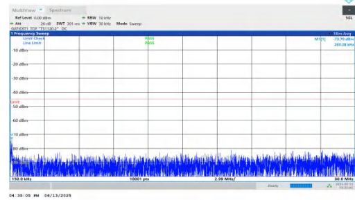
NTNV-n41-PC2-30-20-L-DFT-BPSK-Inner_1RB_Left-0.15-30-PAS
