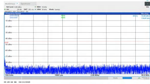
NTNV-n41-PC2-30-35-L-DFT-BPSK-Inner_1RB_Left-0.15-30-PAS S
