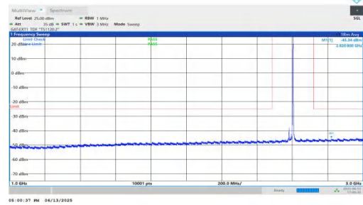
NTNV-n41-PC2-30-25-M-DFT-BPSK-Inner_1RB_Right-1000-3000-PASS
