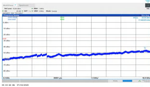
NTNV-n41-PC2-30-20-L-DFT-BPSK-Inner_1RB_Right-3000-18000-PASS
