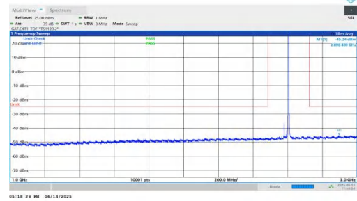
NTNV-n41-PC2-30-30-M-DFT-BPSK-Inner_1RB_Right-1000-3000-PASS
