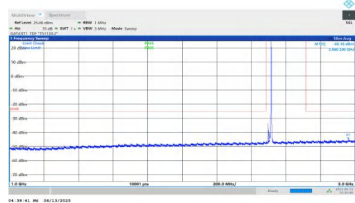
NTNV-n41-PC2-30-20-L-DFT-QPSK-Inner_1RB_Right-1000-3000-PASS PASS
