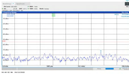
NTNV-n41-PC2-30-20-H-DFT-BPSK-Inner_1RB_Left-0.009-0.15-PASS
