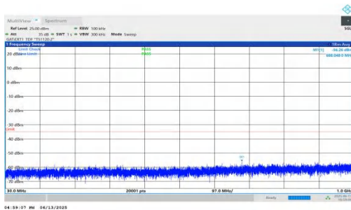
NTNV-n41-PC2-30-25-M-DFT-BPSK-Inner_1RB_Left-30-1000-PASS
