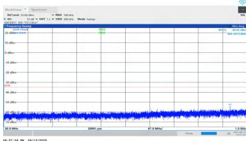
NTNV-n41-PC2-30-25-L-DFT-QPSK-Inner_1RB_Right-30-1000-P ASS
