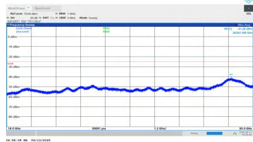
NTNV-n41-PC2-30-25-L-DFT-QPSK-Inner_1RB_Right-18000-3000 00-PASS
