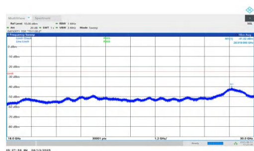
NTNV-n41-PC2-30-30-H-DFT-QPSK-Inner_1RB_Right-18000-30000- 00-PASS
