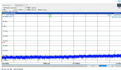
NTNV-n41-PC2-30-30-M-DFT-QPSK-Inner_1RB_Right-30-1000- PASS
