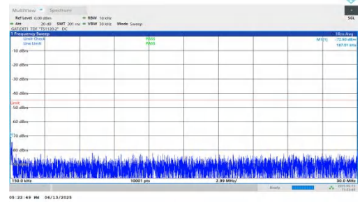
NTNV-n41-PC2-30-30-H-DFT-BPSK-Inner_1RB_Left-0.15-30-PAS
