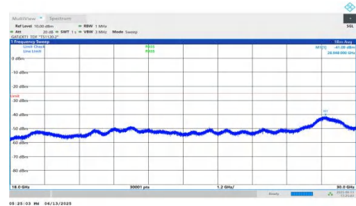
NTNV-n41-PC2-30-30-H-DFT-BPSK-Inner_1RB_Right-18000-300 00-PASS
