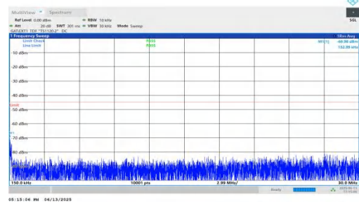
NTNV-n41-PC2-30-30-L-DFT-QPSK-Inner_1RB_Right-0.15-30-PASS SS
