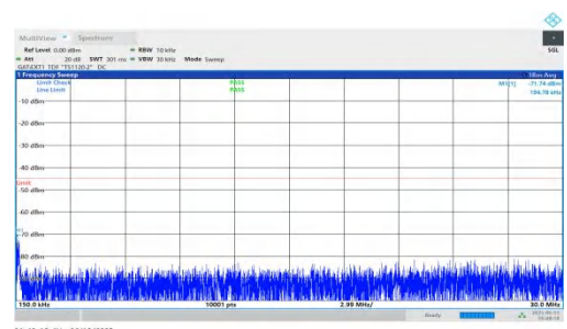
NTNV-n41-PC2-30-20-H-DFT-BPSK-Inner_1RB_Right-0.15-30-PASS
