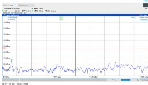
NTNV-n41-PC2-30-25-L-DFT-QPSK-Inner_1RB_Right-0.009-0.1 5-PASS
