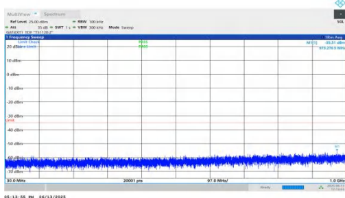
NTNV-n41-PC2-30-30-L-DFT-QPSK-Inner_1RB_Left-30-1000-P PASS
