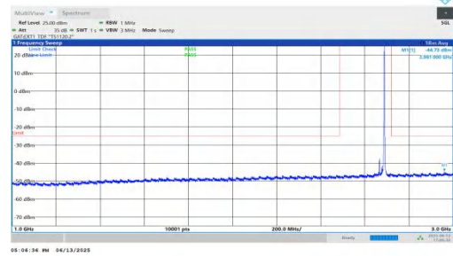
NTNV-n41-PC2-30-25-H-DFT-BPSK-Inner_1RB_Right-1000-3000 -PASS
