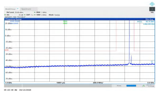
NTNV-n41-PC2-30-30-H-DFT-BPSK-Inner_1RB_Left-1000-3000-PASS
