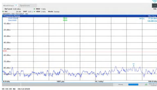
NTNV-n41-PC2-30-25-M-DFT-QPSK-Inner_1RB_Right-0.009-0.1 5-PASS
