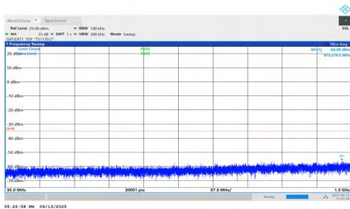
NTNV-n41-PC2-30-30-H-DFT-BPSK-Inner_1RB_Left-30-1000-PASS
