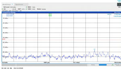
NTNV-n41-PC2-30-20-M-DFT-BPSK-Inner_1RB_Right-0.009-0.15-PASS
