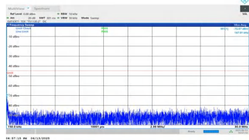
NTNV-n41-PC2-30-25-L-DFT-QPSK-Inner_1RB_Right-0.15-30-PA SS
