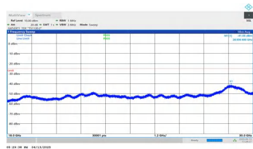
NTNV-n41-PC2-30-35-L-DFT-BPSK-Inner_1RB_Left-18000-30000- PASS
