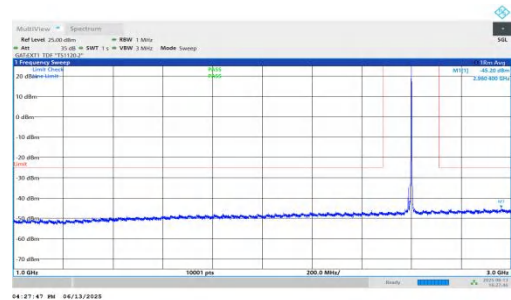
NTNV-n41-PC2-30-15-M-DFT-QPSK-Inner_1RB_Right-1000-3000 -PASS
