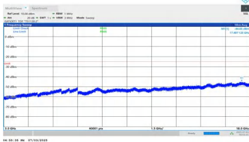
NTNV-n41-PC2-30-10-M-DFT-QPSK-Inner_1RB_Right-3000-18000- 00-PASS
