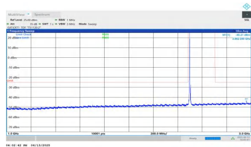
NTNV-n41-PC2-30-10-L-DFT-QPSK-Inner_1RB_Left-1000-3000-P PASS
