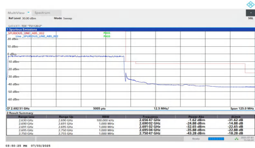
NTVN-n41-PC2-30-60-H-DFT-BPSK-Outer_Full-PASS
