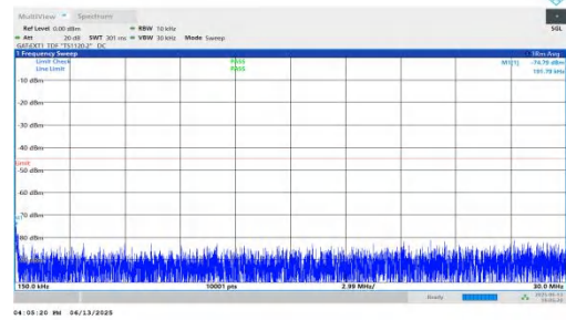
NTNV-n41-PC2-30-10-M-DFT-BPSK-Inner_1RB_Left-0.15-30-PASS
