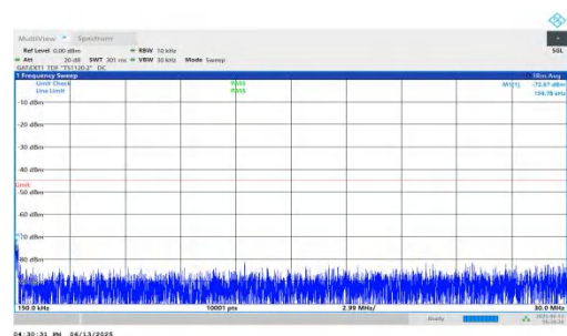
NTNV-n41-PC2-30-15-H-DFT-BPSK-Inner_1RB_Right-0.15-30-PASS
