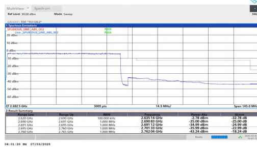
NTNV-n41-PC2-30-70-H-DFT-QPSK-Outer_Full-PASS
