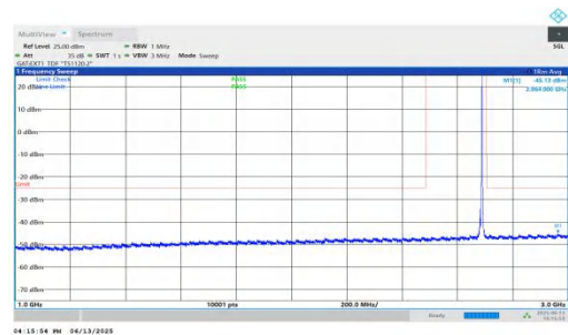
NTNV-n41-PC2-30-10-H-DFT-QPSK-Inner_1RB_Right-1000-3000- -PASS
