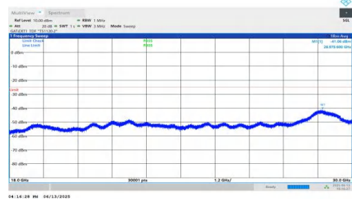
NTNV-n41-PC2-30-10-H-DFT-QPSK-Inner_1RB_Right-18000-30000- 00-PASS
