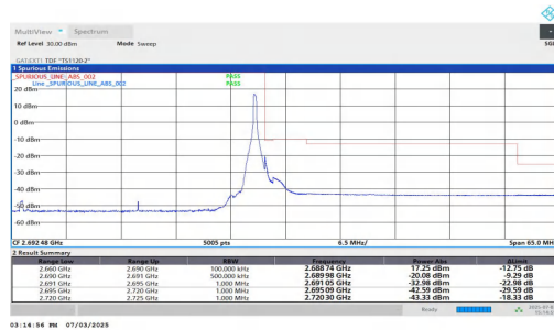
NTVN-n41-PC2-30-30-H-DFT-BPSK-Edge_1RB_Right-PASS
