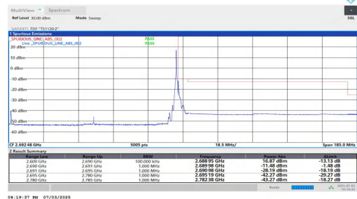
NTVN-n41-PC2-30-90-H-DFT-QPSK-Edge_1RB_Right-PASS
