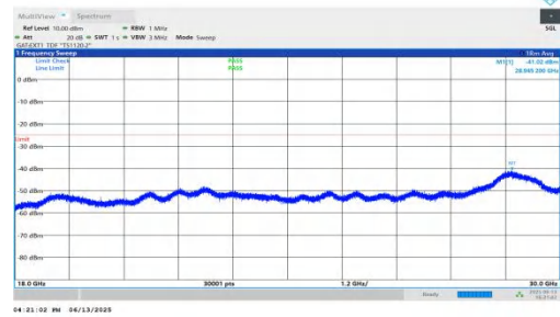
NTNV-n41-PC2-30-15-L-DFT-QPSK-Inner_1RB_Left-18000-3000 0-PASS
