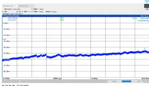
NTNV-n41-PC2-30-15-M-DFT-BPSK-Inner_1RB_Left-3000-18000-PASS
