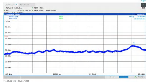
NTNV-n41-PC2-30-15-M-DFT-QPSK-Inner_1RB_Right-18000-300 00-PASS
