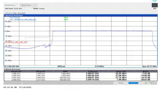
NTVN-n41-PC2-30-25-L-DFT-BPSK-Outer_Full-PASS
