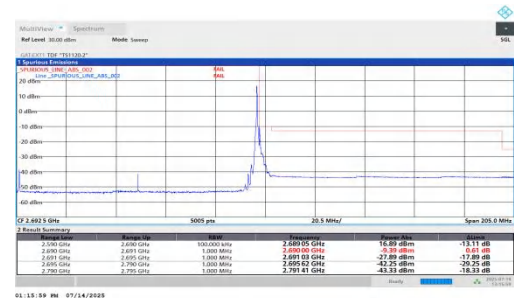
NTV-n41-PC2-30-100-H-DFT-QPSK-Edge_1RB_Right
