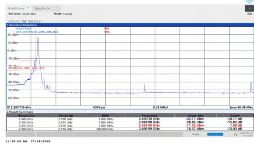
NTNV-n41-PC2-30-80-L-DFT-BPSK-Edge_1RB_Left
