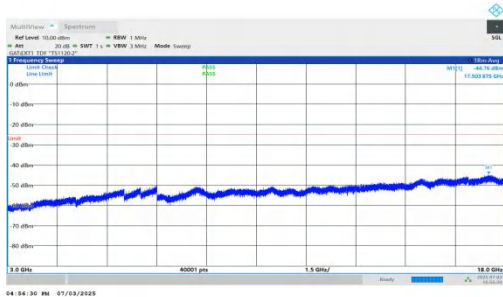
NTNV-n41-PC2-30-10-H-DFT-BPSK-Inner_1RB_Right-3000-180 00-PASS
