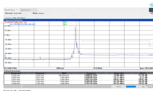
NTNV-n41-PC2-30-70-H-DFT-QPSK-Edge 1RB Right-PASS
