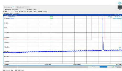
NTNV-n41-PC2-30-15-H-DFT-BPSK-Inner_1RB_Left-1000-3000-PASS
