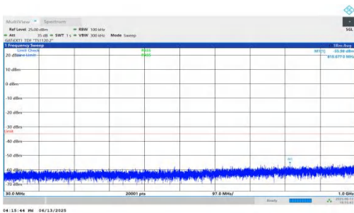
NTNV-n41-PC2-30-10-H-DFT-QPSK-Inner_1RB_Right-30-1000- PASS
