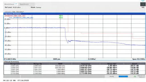
NTVN-n41-PC2-30-25-H-DFT-QPSK-Outer_Full-PASS
