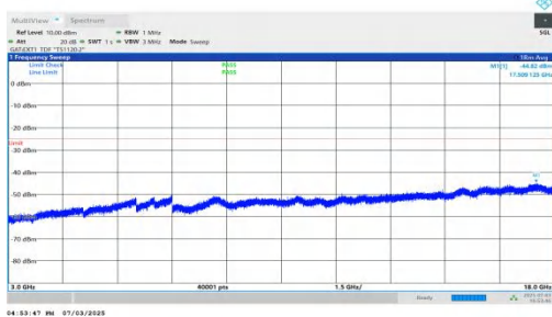
NTNV-n41-PC2-30-10-L-DFT-QPSK-Inner_1RB_Right-3000-18000-PASS
