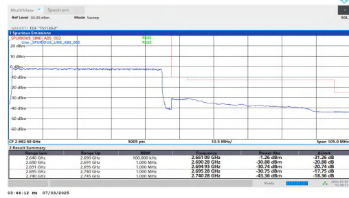
NTVN-n41-PC2-30-50-H-DFT-QPSK-Outer_Full-PASS
