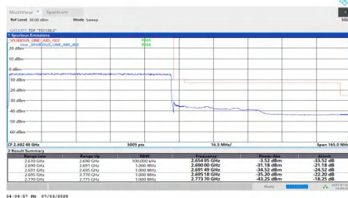
NTVN-n41-PC2-30-80-H-DFT-QPSK-Outer_Full-PASS
