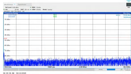
NTNV-n41-PC2-30-10-M-DFT-QPSK-Inner_1RB_Right-0.15-30-P ASS
