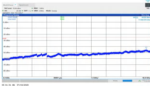
NTNV-n41-PC2-30-15-M-DFT-QPSK-Inner_1RB_Right-3000-1800 00-PASS
