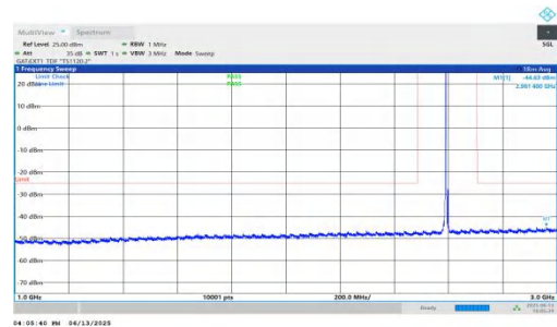
NTNV-n41-PC2-30-10-M-DFT-BPSK-Inner_1RB_Left-1000-3000-PASS
