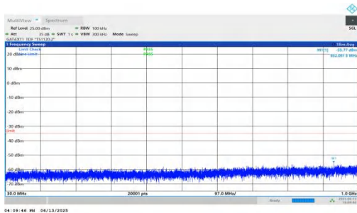
NTNV-n41-PC2-30-10-M-DFT-QPSK-Inner_1RB_Right-30-1000- PASS
