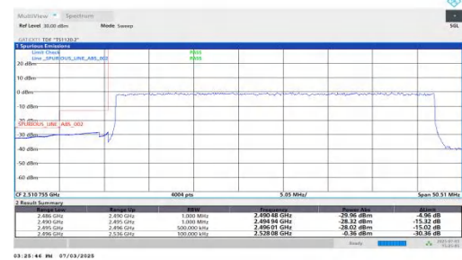
NTVN-n41-PC2-30-40-L-DFT-QPSK-Outer_Full-PASS
