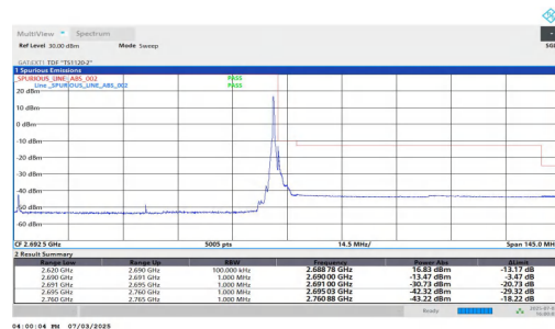
NTNV-n41-PC2-30-70-H-DFT-BPSK-Edge 1RB Right-PASS
