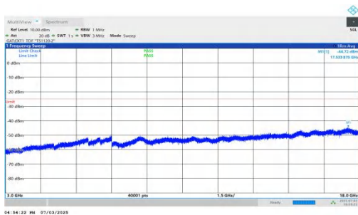
NTNV-n41-PC2-30-10-M-DFT-BPSK-Inner_1RB_Left-3000-18000-PASS
