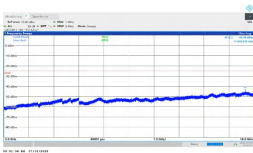
NTNV-n41-PC2-30-15-H-DFT-BPSK-Inner_1RB_Left-3000-18000-PASS
