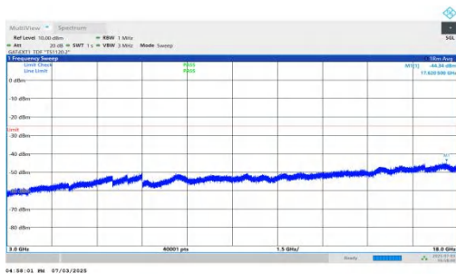
NTNV-n41-PC2-30-15-L-DFT-BPSK-Inner_1RB_Left-3000-18000-PASS
