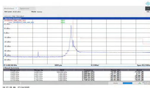
NTNV-n41-PC2-30-45-H-DFT-BPSK-Edge 1RB Right-PASS
