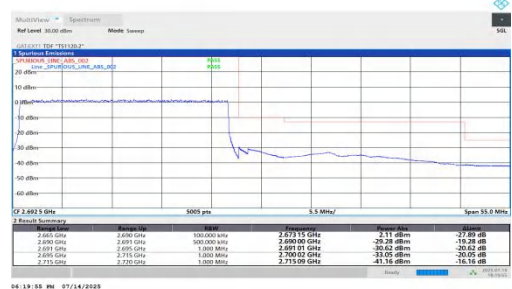
NTVN-n41-PC2-30-25-H-DFT-BPSK-Outer_Full-PASS
