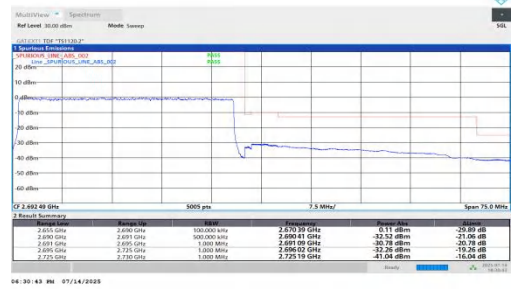
NTVN-n41-PC2-30-35-H-DFT-QPSK-Outer_Full-PASS
