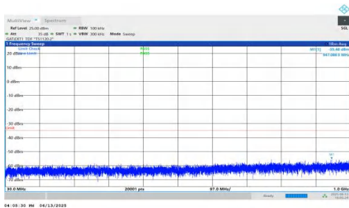
NTNV-n41-PC2-30-10-M-DFT-BPSK-Inner_1RB_Left-30-1000-PASS
