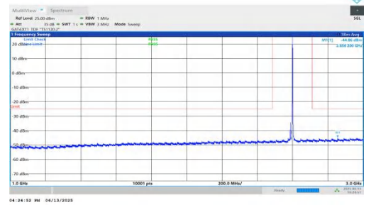
NTNV-n41-PC2-30-15-M-DFT-BPSK-Inner_1RB_Right-1000-3000-PASS
