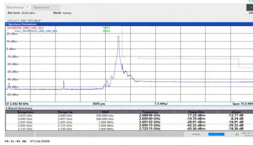
NTVN-n41-PC2-30-35-H-DFT-QPSK-Edge_1RB_Right-PASS
