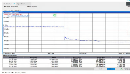
NTVN-n41-PC2-30-80-H-DFT-BPSK-Outer_Full-PASS
