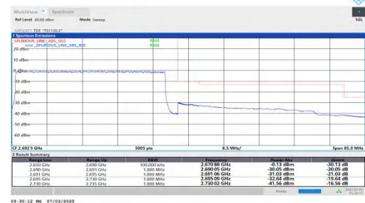
NTVN-n41-PC2-30-40-H-DFT-QPSK-Outer_Full-PASS
