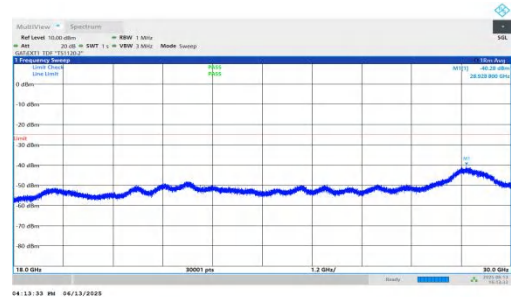
NTNV-n41-PC2-30-10-H-DFT-BPSK-Inner_1RB_Right-18000-300 00-PASS
