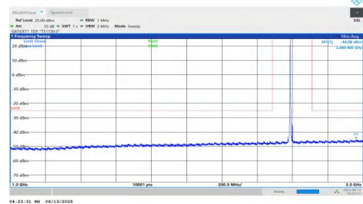
NTNV-n41-PC2-30-15-M-DFT-BPSK-Inner_1RB_Left-1000-3000-PASS
