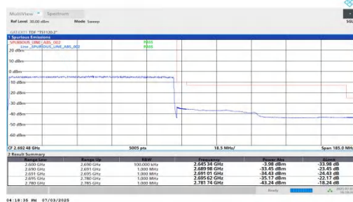
NTVN-n41-PC2-30-90-H-DFT-QPSK-Outer_Full-PASS
