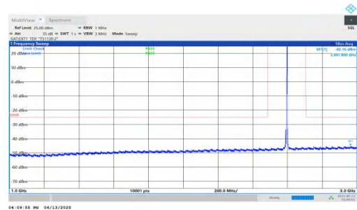
NTNV-n41-PC2-30-10-M-DFT-QPSK-Inner_1RB_Right-1000-3000- -PASS
