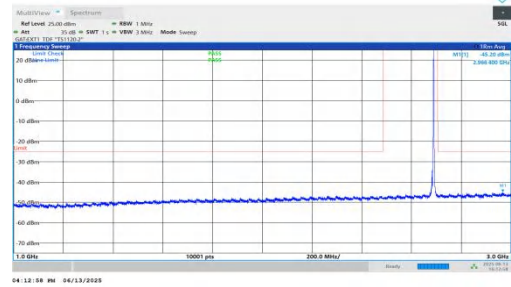
NTNV-n41-PC2-30-10-H-DFT-BPSK-Inner_1RB_Right-1000-3000 -PASS
