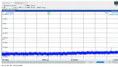
NTNV-n41-PC2-30-10-H-DFT-BPSK-Inner_1RB_Right-30-1000-P ASS
