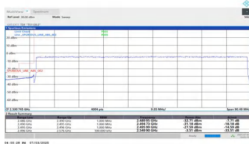
NTNV-n41-PC2-30-80-L-DFT-QPSK-Outer_Full-PASS
