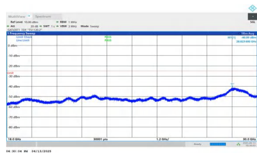
NTNV-n41-PC2-30-15-H-DFT-BPSK-Inner_1RB_Left-18000-30000-PASS
