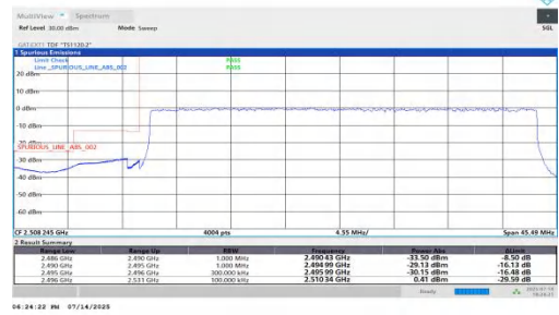
NTVN-n41-PC2-30-35-L-DFT-BPSK-Outer_Full-PASS
