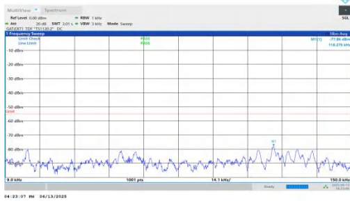
NTNV-n41-PC2-30-15-M-DFT-BPSK-Inner_1RB_Left-0.009-0.15-PASS
