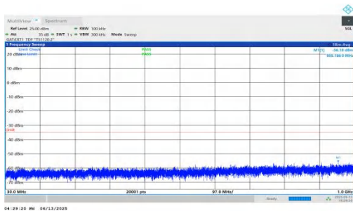
NTNV-n41-PC2-30-15-H-DFT-BPSK-Inner_1RB_Left-30-1000-PASS
