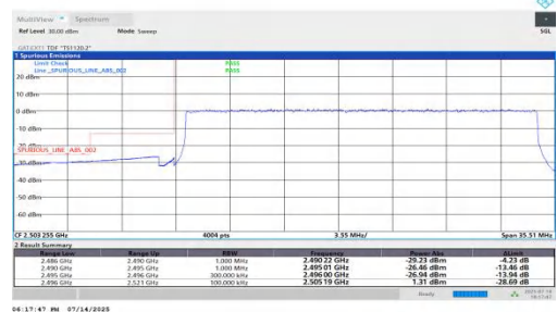
NTVN-n41-PC2-30-25-L-DFT-QPSK-Outer_Full-PASS
