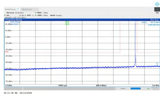
NTNV-n41-PC2-30-10-H-DFT-BPSK-Inner_1RB_Left-1000-3000-PASS
