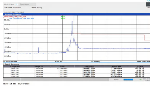
NTVN-n41-PC2-30-50-H-DFT-QPSK-Edge_1RB_Right-PASS
