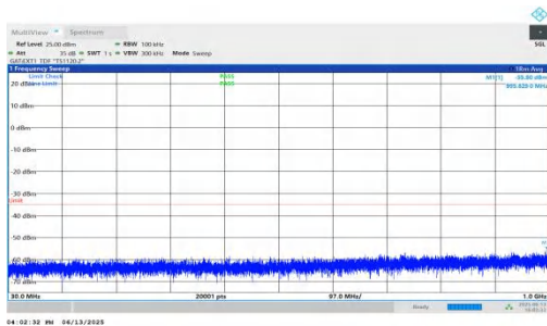
NTNV-n41-PC2-30-10-L-DFT-QPSK-Inner_1RB_Left-30-1000-P PASS
