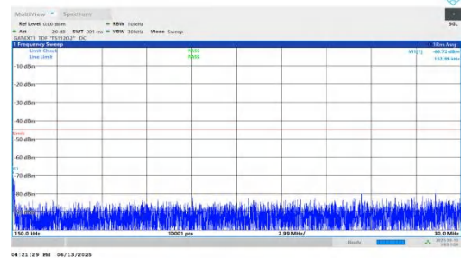
NTNV-n41-PC2-30-15-L-DFT-QPSK-Inner_1RB_Right-0.15-30-PA SS
