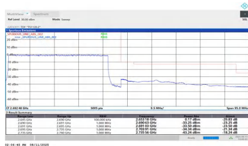
NTNV-n41-PC2-30-45-H-DFT-BPSK-Outer Full-PASS
