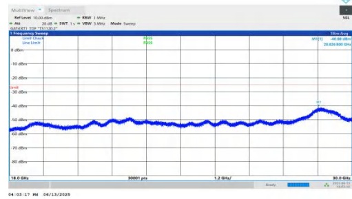
NTNV-n41-PC2-30-10-L-DFT-QPSK-Inner_1RB_Left-18000-3000 0-PASS
