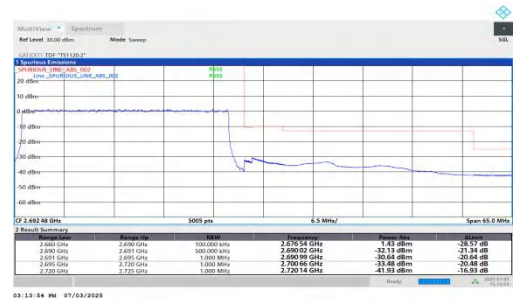
NTVN-n41-PC2-30-30-H-DFT-BPSK-Outer_Full-PASS
