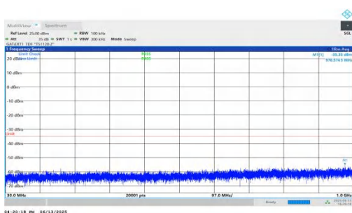
NTNV-n41-PC2-30-15-L-DFT-QPSK-Inner_1RB_Left-30-1000-PA SS
