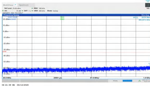
NTNV-n41-PC2-30-15-L-DFT-QPSK-Inner_1RB_Right-30-1000-P ASS
