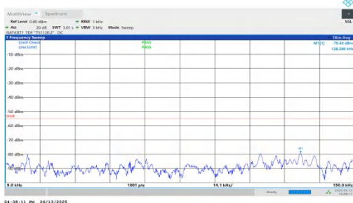
NTNV-n41-PC2-30-10-M-DFT-QPSK-Inner_1RB_Left-0.009-0.15-PASS
