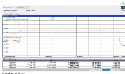
NTNV-n41-PC2-30-70-L-DFT-QPSK-Outer Full-PASS
