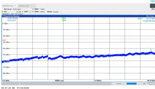
NTNV-n41-PC2-30-10-H-DFT-QPSK-Inner_1RB_Right-3000-18000- 00-PASS
