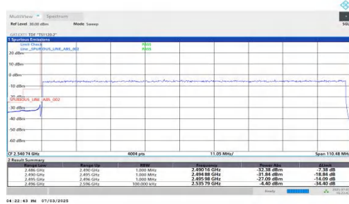
NTV-n41-PC2-30-100-L-DFT-QPSK-Outer_Full-PASS
