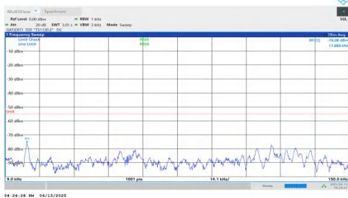
NTNV-n41-PC2-30-15-M-DFT-BPSK-Inner_1RB_Right-0.009-0.15-PASS
