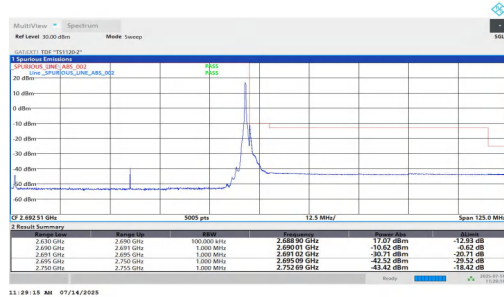
NTVN-n41-PC2-30-60-H-DFT-BPSK-Edge_1RB_Right-PASS
