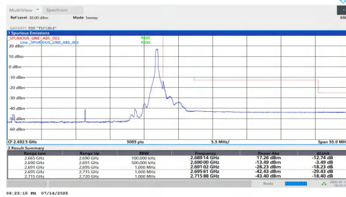
NTVN-n41-PC2-30-25-H-DFT-QPSK-Edge_1RB_Right-PASS
