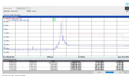
NTNV-n41-PC2-30-45-H-DFT-QPSK-Edge 1RB Right-PASS
