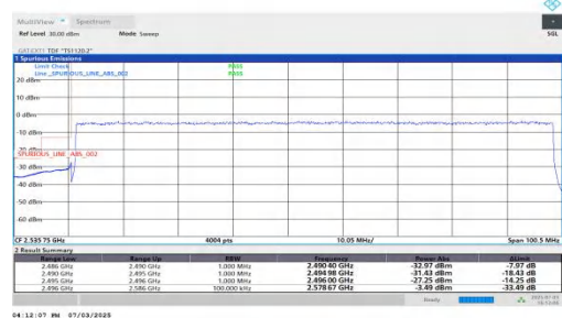
NTVN-n41-PC2-30-90-L-DFT-BPSK-Outer_Full-PASS
