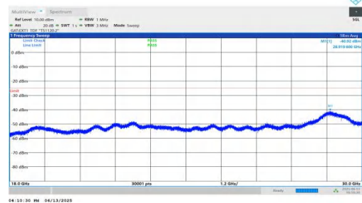
NTNV-n41-PC2-30-10-M-DFT-QPSK-Inner_1RB_Right-18000-300 00-PASS
