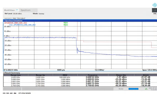
NTNV-n41-PC2-30-60-H-DFT-QPSK-Outer Full-PASS
