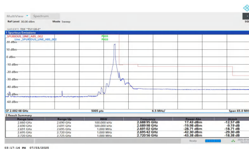
NTVN-n41-PC2-30-30-H-DFT-QPSK-Edge_1RB_Right-PASS
