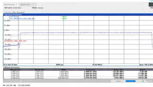
NTVN-n41-PC2-30-90-L-DFT-QPSK-Outer_Full-PASS
