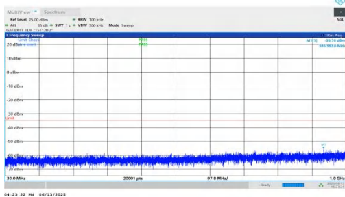
NTNV-n41-PC2-30-15-M-DFT-BPSK-Inner_1RB_Left-30-1000-PASS
