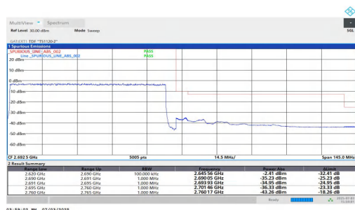
NTNV-n41-PC2-30-70-H-DFT-BPSK-Outer Full-PASS
