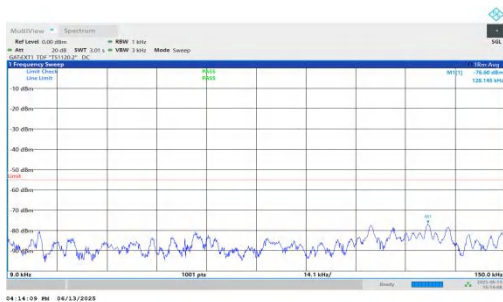
NTNV-n41-PC2-30-10-H-DFT-QPSK-Inner_1RB_Left-0.009-0.15- PASS
