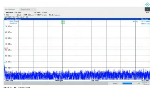
NTNV-n41-PC2-30-10-M-DFT-BPSK-Inner_1RB_Right-0.15-30-PASS
