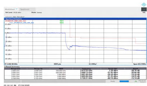
NTVN-n41-PC2-30-30-H-DFT-QPSK-Outer_Full-PASS
