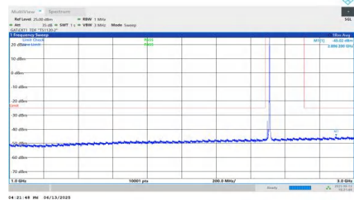
NTNV-n41-PC2-30-15-L-DFT-QPSK-Inner_1RB_Right-1000-3000-P PASS
