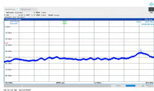
NTNV-n41-PC2-30-10-H-DFT-BPSK-Inner_1RB_Left-18000-30000-PASS
