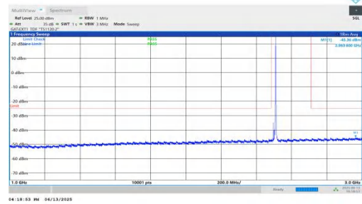
NTNV-n41-PC2-30-15-L-DFT-BPSK-Inner_1RB_Right-1000-3000-P PASS
