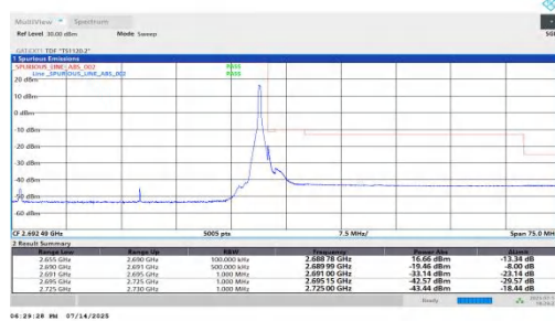
NTVN-n41-PC2-30-35-H-DFT-BPSK-Edge_1RB_Right-PASS
