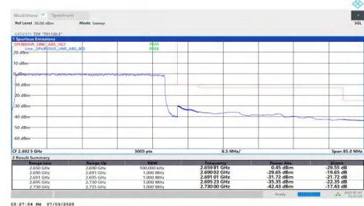
NTVN-n41-PC2-30-40-H-DFT-BPSK-Outer_Full-PASS
