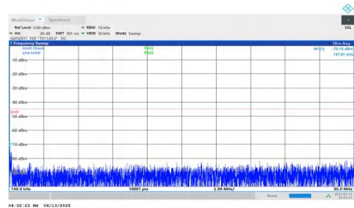
NTNV-n41-PC2-30-10-L-DFT-QPSK-Inner_1RB_Left-0.15-30-P PASS
