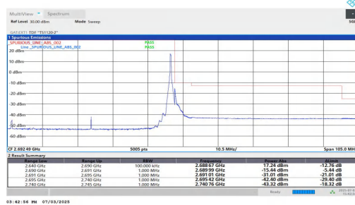
NTVN-n41-PC2-30-50-H-DFT-BPSK-Edge_1RB_Right-PASS
