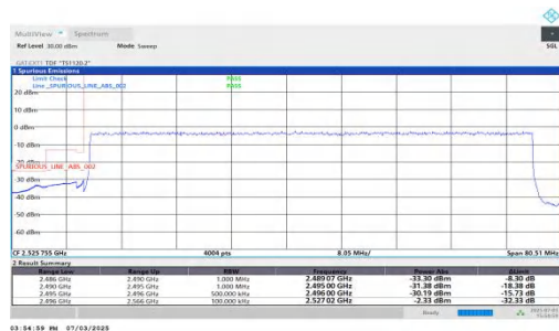
NTNV-n41-PC2-30-70-L-DFT-BPSK-Outer Full-PASS
