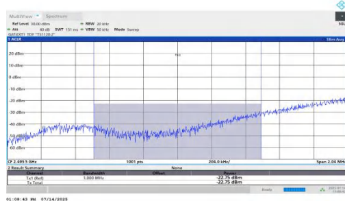
NTVN-n41-PC2-30-100-L-DFT-BPSK-Edge_1RB_Left-PASS
