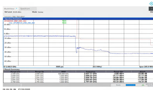
NTV-n41-PC2-30-100-H-DFT-BPSK-Outer_Full-PASS
