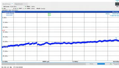
NTNV-n41-PC2-30-15-L-DFT-QPSK-Inner_1RB_Right-3000-180 00-PASS
