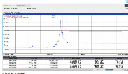
NTVN-n41-PC2-30-40-H-DFT-BPSK-Edge_1RB_Right-PASS
