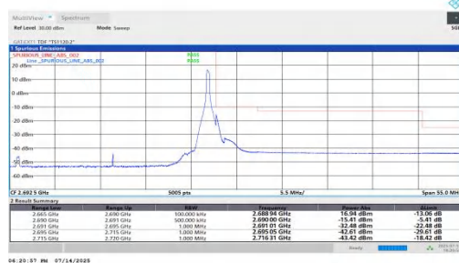
NTVN-n41-PC2-30-25-H-DFT-BPSK-Edge_1RB_Right-PASS
