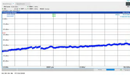
NTNV-n41-PC2-30-15-L-DFT-QPSK-Inner_1RB_Left-3000-18000 -PASS
