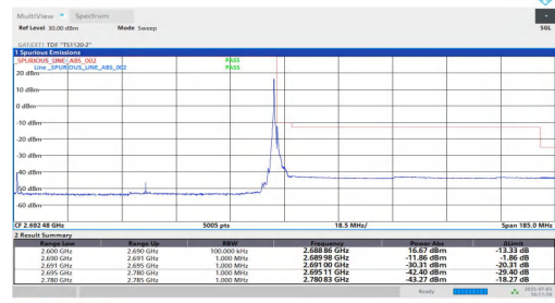
NTVN-n41-PC2-30-90-H-DFT-BPSK-Edge_1RB_Right-PASS
