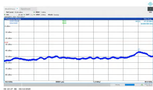
NTNV-n41-PC2-30-15-L-DFT-BPSK-Inner_1RB_Right-18000-300 00-PASS
