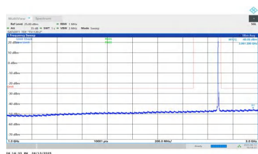
NTNV-n41-PC2-30-10-H-DFT-QPSK-Inner_1RB_Left-1000-3000- PASS
