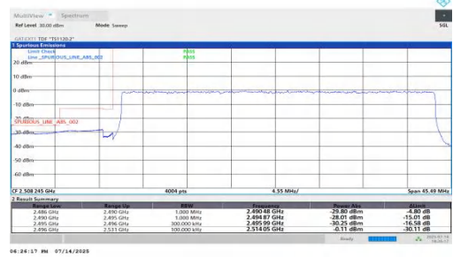
NTVN-n41-PC2-30-35-L-DFT-QPSK-Outer_Full-PASS
