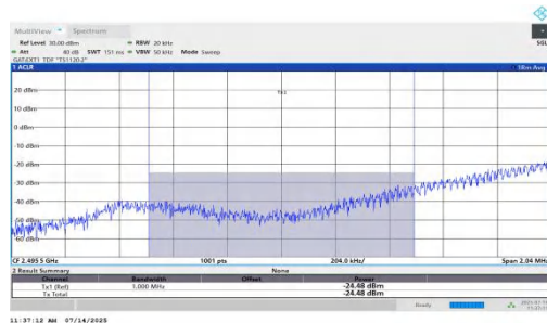
NTNV-n41-PC2-30-80-L-DFT-BPSK-Edge_1RB_Left-PASS
