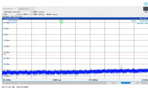
NTNV-n41-PC2-30-15-L-DFT-BPSK-Inner_1RB_Left-30-1000-PASS
