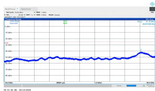
NTNV-n41-PC2-30-10-L-DFT-BPSK-Inner_1RB_Right-18000-30000-P PASS
