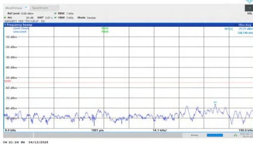
NTNV-n41-PC2-30-15-L-DFT-QPSK-Inner_1RB_Right-0.009-0.1 5-PASS
