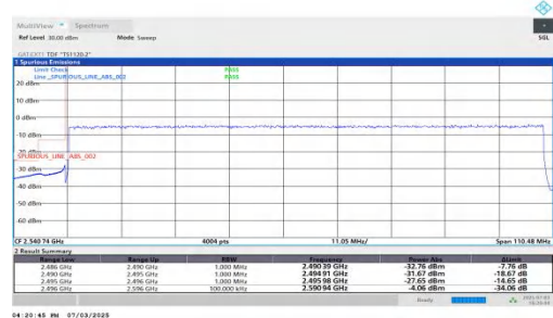
NTVN-n41-PC2-30-100-L-DFT-BPSK-Outer_Full-PASS
