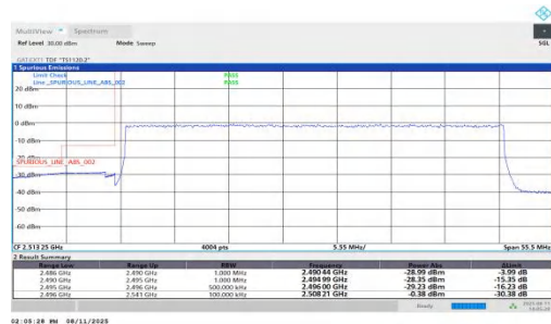
NTNV-n41-PC2-30-45-L-DFT-QPSK-Outer Full-PASS
