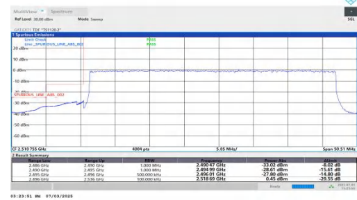
NTVN-n41-PC2-30-40-L-DFT-BPSK-Outer_Full-PASS
