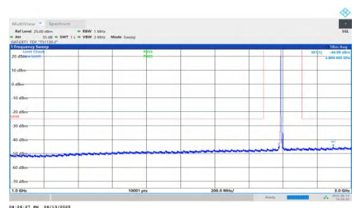
NTNV-n41-PC2-30-15-M-DFT-QPSK-Inner_1RB_Left-1000-3000-PASS
