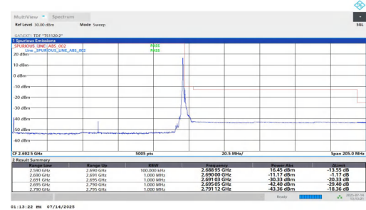
NTV-n41-PC2-30-100-H-DFT-BPSK-Edge_1RB_Right-PASS
