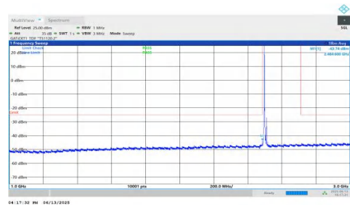
NTNV-n41-PC2-30-15-L-DFT-BPSK-Inner_1RB_Left-1000-3000-PASS
