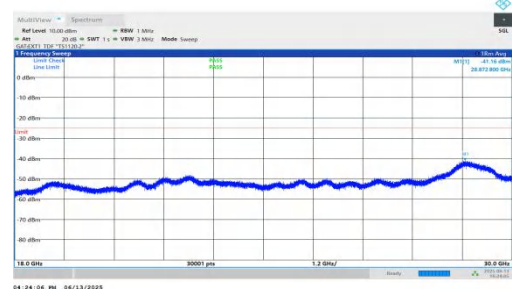
NTNV-n41-PC2-30-15-M-DFT-BPSK-Inner_1RB_Left-18000-30000-PASS
