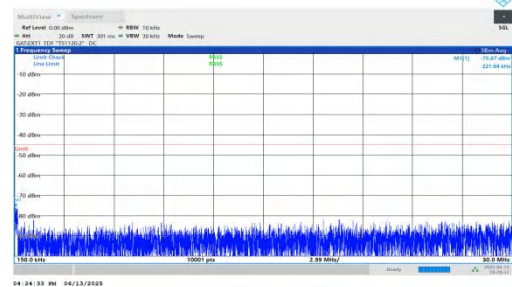
NTNV-n41-PC2-30-15-M-DFT-BPSK-Inner_1RB_Right-0.15-30-PASS
