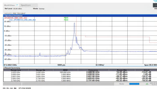
NTVN-n41-PC2-30-40-H-DFT-QPSK-Edge_1RB_Right-PASS
