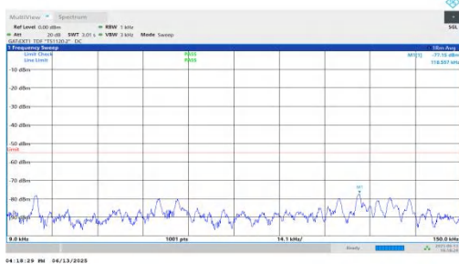
NTNV-n41-PC2-30-15-L-DFT-BPSK-Inner_1RB_Right-0.009-0.15-PASS
