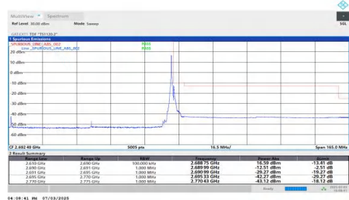
NTNV-n41-PC2-30-80-H-DFT-BPSK-Edge 1RB_Right-PASS
