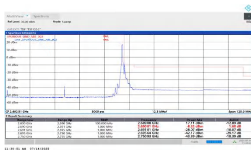
NTVN-n41-PC2-30-60-H-DFT-QPSK-Edge_1RB_Right
