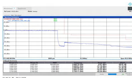
NTNV-n41-PC2-30-45-H-DFT-QPSK-Outer Full-PASS
