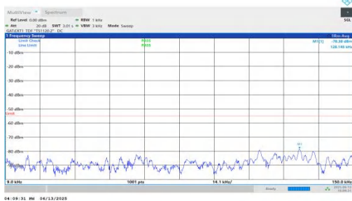
NTNV-n41-PC2-30-10-M-DFT-QPSK-Inner_1RB_Right-0.009-0.1 5-PASS
