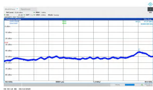
NTNV-n41-PC2-30-10-M-DFT-BPSK-Inner_1RB_Left-18000-30000-PASS
