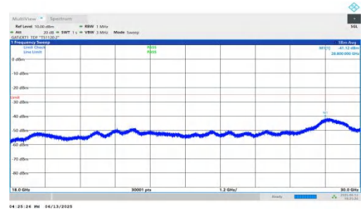
NTNV-n41-PC2-30-15-M-DFT-BPSK-Inner_1RB_Right-18000-30000-PASS
