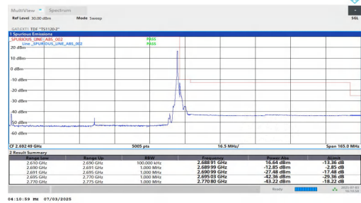
NTVN-n41-PC2-30-80-H-DFT-QPSK-Edge_1RB_Right-PASS
