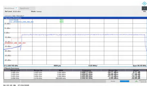
NTNV-n41-PC2-30-80-L-DFT-BPSK-Outer_Full-PASS
