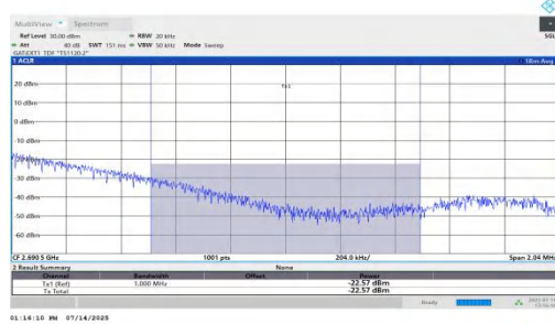
NTV-n41-PC2-30-100-H-DFT-QPSK-Edge_1RB_Right-PASS
