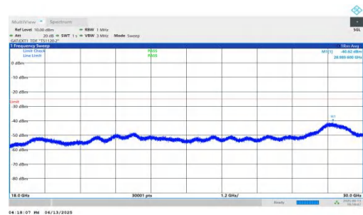
NTNV-n41-PC2-30-15-L-DFT-BPSK-Inner_1RB_Left-18000-30000-PASS
