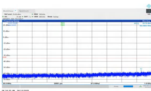
NTNV-n41-PC2-30-10-H-DFT-QPSK-Inner_1RB_Left-30-1000-P ASS
