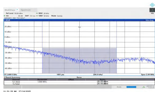
NTVN-n41-PC2-30-60-H-DFT-QPSK-Edge_1RB_Right-PASS
