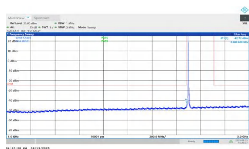
NTNV-n41-PC2-30-15-L-DFT-QPSK-Inner_1RB_Left-1000-3000-P ASS
