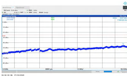
NTNV-n41-PC2-30-10-L-DFT-BPSK-Inner_1RB_Right-3000-18000-P PASS
