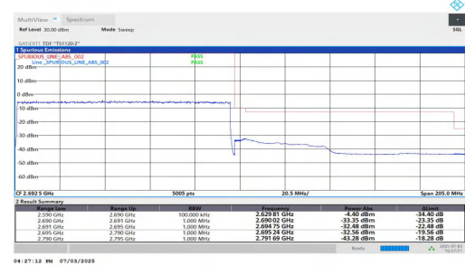
NTV-n41-PC2-30-100-H-DFT-QPSK-Outer_Full-PASS
