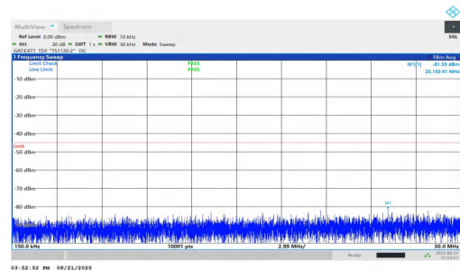
NTVN-n38-PC1.5-30-40-H-DFT-QPSK-Inner_1RB_Right-0.15-30-PASS
