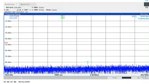
NTNV-n38-PC1.5-30-40-H-DFT-BPSK-Inner_1RB_Left-0.15-30-P ASS
