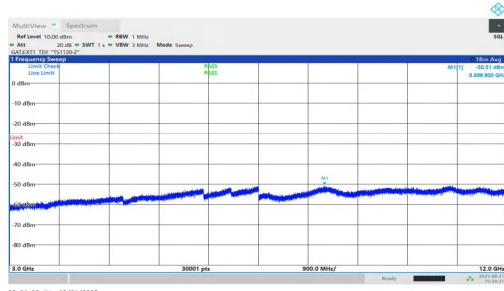
NTNV-n38-PC1.5-30-30-H-DFT-QPSK-Inner_1RB_Right-3000-12000-PASS
