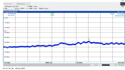
NTNV-n38-PC1.5-30-40-L-DFT-BPSK-Inner_1RB_Right-12000-26 500-PASS
