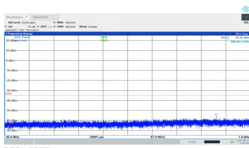
NTVN-n38-PC1.5-30-40-M-DFT-QPSK-Inner_1RB_Left-30-1000-PASS
