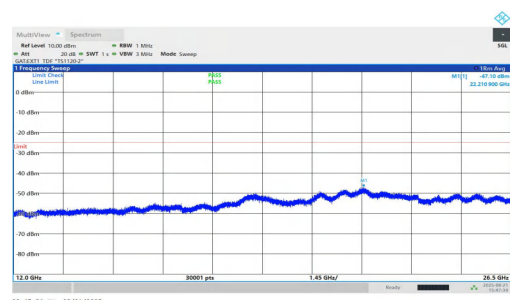
NTVN-n38-PC1.5-30-40-M-DFT-QPSK-Inner_1RB_Right-12000-26500-PASS
