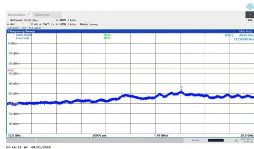
NTVN-n38-PC1.5-30-40-M-DFT-BPSK-Inner_1RB_Right-12000-26500-PASS
