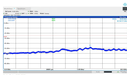
NTNV-n38-PC1.5-30-40-L-DFT-QPSK-Inner_1RB_Right-12000-26500-PASS
