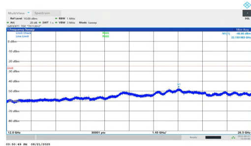
NTNV-n38-PC1.5-30-40-H-DFT-BPSK-Inner_1RB_Right-12000-26 500-PASS
