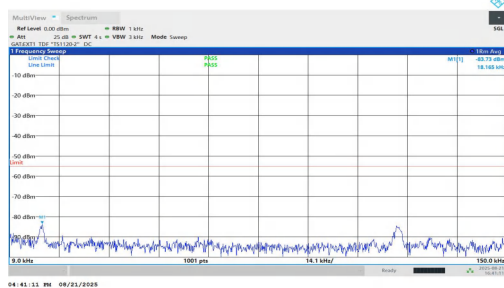
NTNV-n38-PC1.5-30-30-H-DFT-QPSK-Inner_1RB_Right-0.009-0.15-PASS
