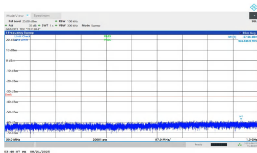
NTNV-n38-PC1.5-30-40-L-DFT-QPSK-Inner_1RB_Right-30-1000-PASS
