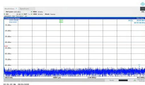
NTNV-n38-PC1.5-30-40-H-DFT-QPSK-Inner_1RB_Left-0.15-30-P ASS
