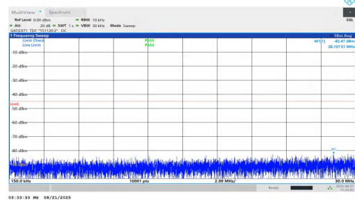
NTNV-n38-PC1.5-30-30-H-DFT-QPSK-Inner_1RB_Right-0.15-30-PASS
