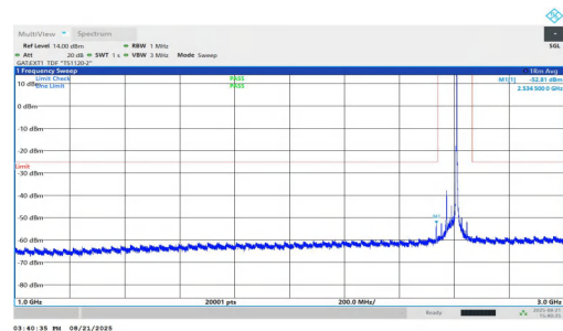
NTNV-n38-PC1.5-30-40-L-DFT-QPSK-Inner_1RB_Right-1000-3000-PASS
