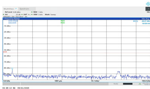
NTVN-n38-PC1.5-30-40-H-DFT-QPSK-Inner_1RB_Right-0.009-0.15-PASS
