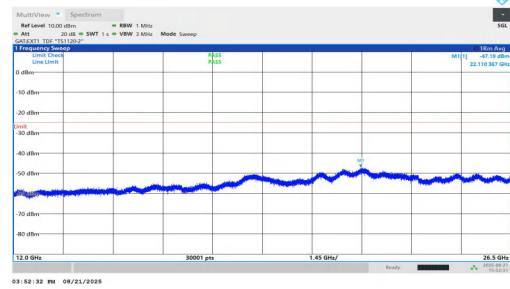
NTVN-n38-PC1.5-30-40-H-DFT-QPSK-Inner_1RB_Left-12000-26500-PASS
