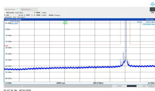
NTVN-n38-PC1.5-30-40-M-DFT-QPSK-Inner_1RB_Right-1000-3000-PASS
