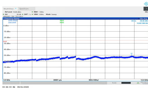
NTVN-n38-PC1.5-30-40-M-DFT-BPSK-Inner_1RB_Right-3000-12000-PASS
