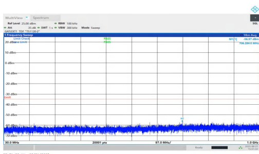
NTNV-n38-PC1.5-30-40-H-DFT-QPSK-Inner_1RB_Left-30-1000- PASS
