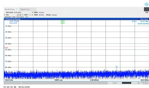
NTNV-n38-PC1.5-30-40-H-DFT-BPSK-Inner_1RB_Right-0.15-30- PASS
