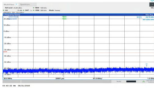
NTVN-n38-PC1.5-30-40-M-DFT-BPSK-Inner_1RB_Right-30-1000-PASS
