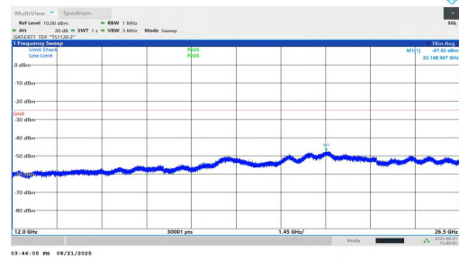
NTVN-n38-PC1.5-30-40-M-DFT-QPSK-Inner_1RB_Left-12000-26500-PASS
