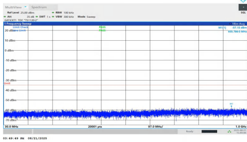
NTNV-n38-PC1.5-30-40-H-DFT-BPSK-Inner_1RB_Right-30-1000 -PASS
