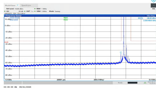
NTNV-n38-PC1.5-30-40-L-DFT-BPSK-Inner_1RB_Left-1000-3000 -PASS
