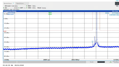
NTVN-n38-PC1.5-30-40-M-DFT-BPSK-Inner_1RB_Right-1000-3000-PASS
