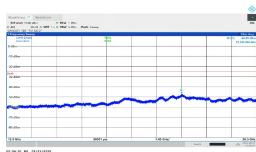
NTVN-n38-PC1.5-30-40-H-DFT-QPSK-Inner_1RB_Right-12000-26500-PASS
