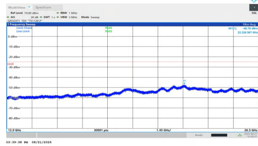
NTNV-n38-PC1.5-30-40-L-DFT-QPSK-Inner_1RB_Left-12000-26500-PASS
