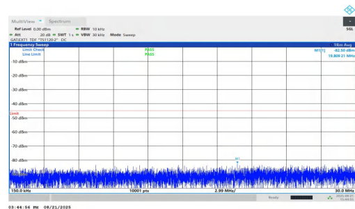
NTVN-n38-PC1.5-30-40-M-DFT-QPSK-Inner_1RB_Left-0.15-30-PASS
