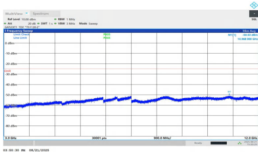
NTNV-n38-PC1.5-30-40-H-DFT-BPSK-Inner_1RB_Right-3000-12 000-PASS
