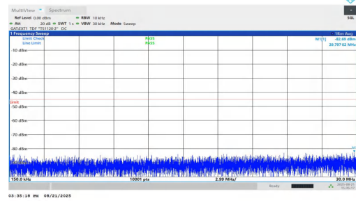
NTNV-n38-PC1.5-30-40-L-DFT-BPSK-Inner_1RB_Left-0.15-30-PA SS
