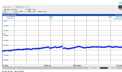
NTNV-n38-PC1.5-30-40-M-DFT-BPSK-Inner_1RB_Left-3000-120 00-PASS
