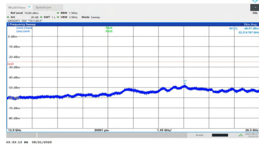
NTNV-n38-PC1.5-30-30-H-DFT-QPSK-Inner_1RB_Left-12000-26500-PASS
