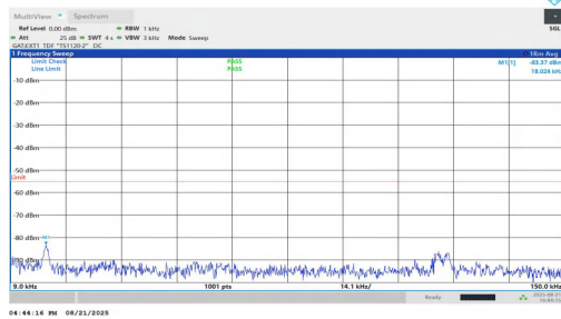
NTNV-n38-PC1.5-30-40-M-DFT-BPSK-Inner_1RB_Left-0.009-0.1 5-PASS
