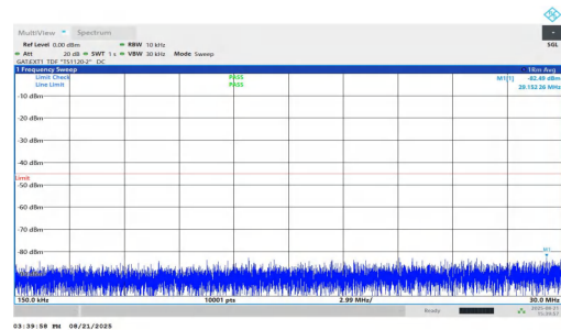
NTNV-n38-PC1.5-30-40-L-DFT-QPSK-Inner_1RB_Right-0.15-30-PASS
