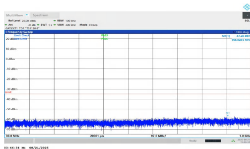
NTVN-n38-PC1.5-30-40-M-DFT-QPSK-Inner_1RB_Right-30-1000-PASS
