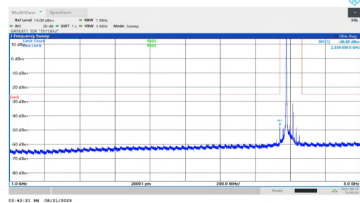
NTNV-n38-PC1.5-30-40-M-DFT-BPSK-Inner_1RB_Left-1000-3000 -PASS
