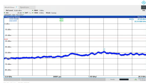
NTNV-n38-PC1.5-30-30-H-DFT-QPSK-Inner_1RB_Right-12000-26500-PASS
