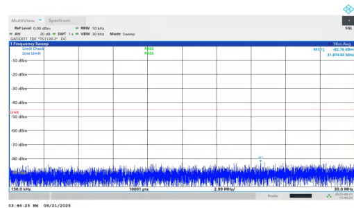
NTVN-n38-PC1.5-30-40-M-DFT-QPSK-Inner_1RB_Right-0.15-30-PASS
