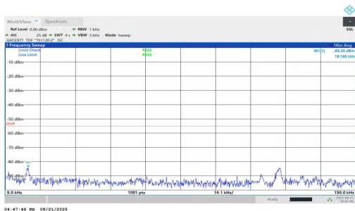
NTNV-n38-PC1.5-30-40-H-DFT-QPSK-Inner_1RB_Left-0.009-0.1 5-PASS
