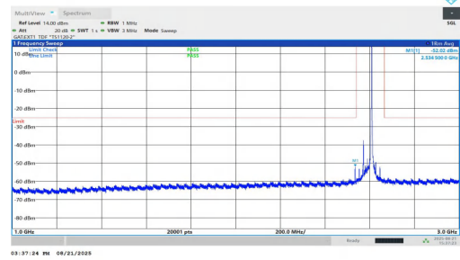
NTNV-n38-PC1.5-30-40-L-DFT-BPSK-Inner_1RB_Right-1000-300 0-PASS
