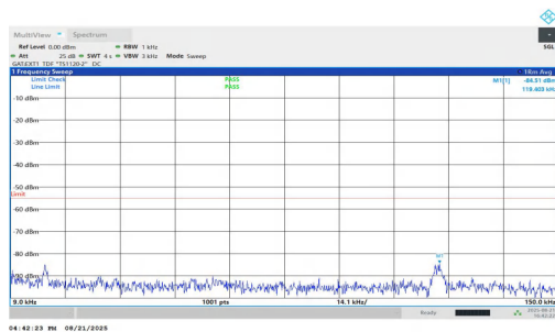
NTNV-n38-PC1.5-30-40-L-DFT-BPSK-Inner_1RB_Right-0.009-0. 15-PASS
