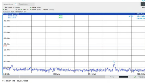
NTNV-n38-PC1.5-30-40-H-DFT-BPSK-Inner_1RB_Left-0.009-0.1 5-PASS
