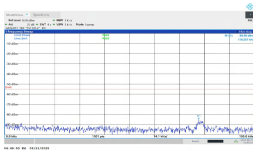
NTVN-n38-PC1.5-30-40-M-DFT-QPSK-Inner_1RB_Right-0.009-0.15-PASS
