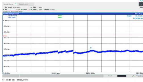
NTVN-n38-PC1.5-30-40-M-DFT-QPSK-Inner_1RB_Left-3000-12000-PASS
