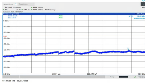
NTNV-n38-PC1.5-30-40-L-DFT-QPSK-Inner_1RB_Left-3000-12000-PASS
