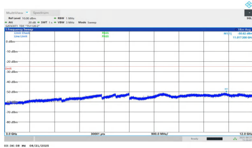
NTNV-n38-PC1.5-30-40-L-DFT-BPSK-Inner_1RB_Left-3000-120 00-PASS
