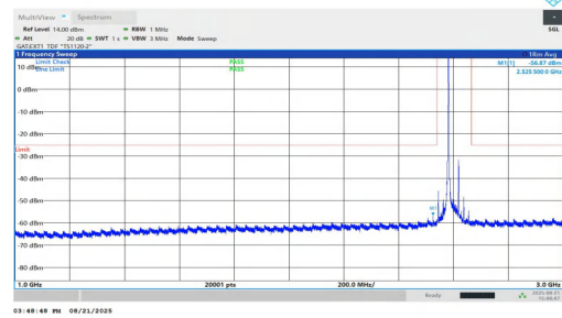
NTNV-n38-PC1.5-30-40-H-DFT-BPSK-Inner_1RB_Left-1000-3000 -PASS
