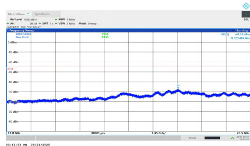
NTNV-n38-PC1.5-30-40-M-DFT-BPSK-Inner_1RB_Left-12000-265 00-PASS
