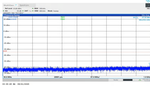
NTNV-n38-PC1.5-30-40-L-DFT-BPSK-Inner_1RB_Left-30-1000-P ASS
