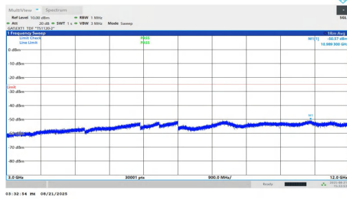
NTNV-n38-PC1.5-30-30-H-DFT-QPSK-Inner_1RB_Left-3000-12000-PASS
