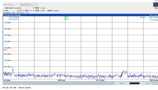
NTNV-n38-PC1.5-30-40-L-DFT-BPSK-Inner_1RB_Left-0.009-0.1 5-PASS
