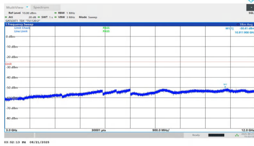
NTVN-n38-PC1.5-30-40-H-DFT-QPSK-Inner_1RB_Left-3000-12000-PASS
