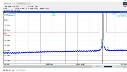
NTNV-n38-PC1.5-30-40-H-DFT-BPSK-Inner_1RB_Right-1000-300 0-PASS
