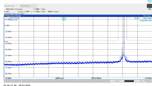
NTNV-n38-PC1.5-30-30-H-DFT-QPSK-Inner_1RB_Right-1000-3000-PASS
