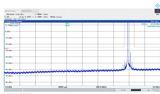
NTNV-n38-PC1.5-30-40-H-DFT-QPSK-Inner_1RB_Left-1000-3000 -PASS
