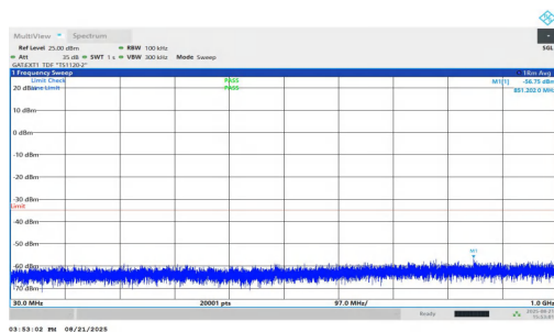
NTVN-n38-PC1.5-30-40-H-DFT-QPSK-Inner_1RB_Right-30-1000-PASS
