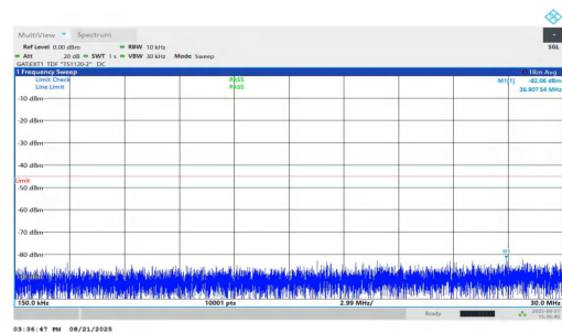
NTNV-n38-PC1.5-30-40-L-DFT-BPSK-Inner_1RB_Right-0.15-30-P ASS
