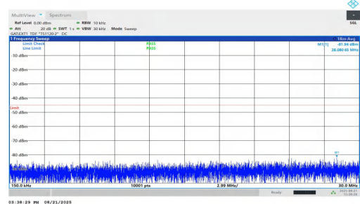
NTNV-n38-PC1.5-30-40-L-DFT-QPSK-Inner_1RB_Left-0.15-30-PA SS
