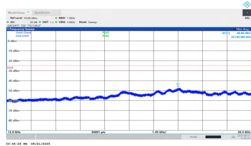
NTNV-n38-PC1.5-30-40-L-DFT-BPSK-Inner_1RB_Left-12000-265 00-PASS
