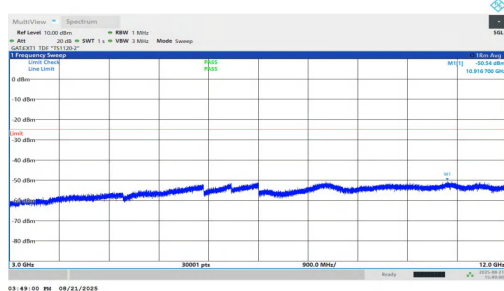
NTNV-n38-PC1.5-30-40-H-DFT-BPSK-Inner_1RB_Left-3000-120 00-PASS
