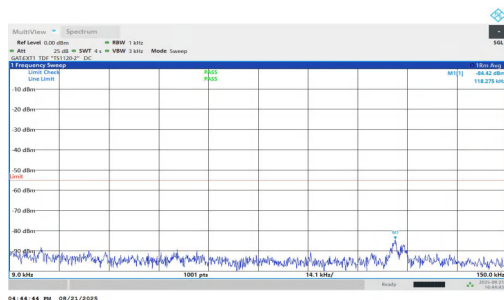
NTNV-n38-PC1.5-30-40-M-DFT-BPSK-Inner_1RB_Right-0.009-0. 15-PASS
