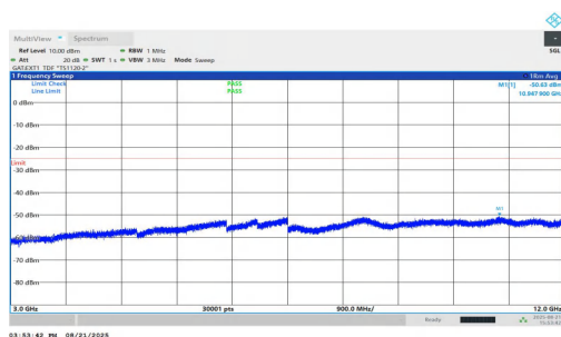
NTVN-n38-PC1.5-30-40-H-DFT-QPSK-Inner_1RB_Right-3000-12000-PASS
