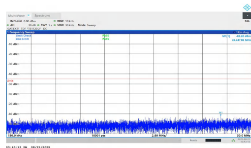
NTNV-n38-PC1.5-30-40-M-DFT-BPSK-Inner_1RB_Right-0.15-30- PASS
