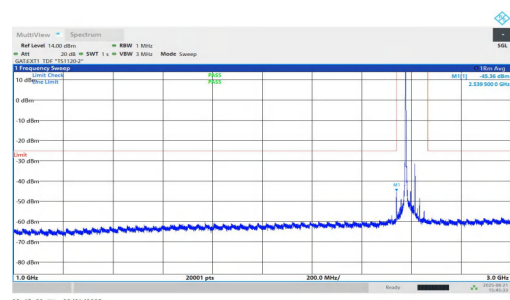
NTVN-n38-PC1.5-30-40-M-DFT-QPSK-Inner_1RB_Left-1000-3000-PASS
