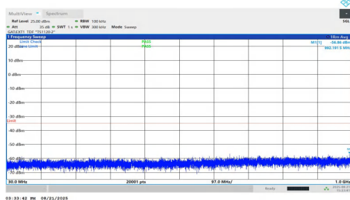
NTNV-n38-PC1.5-30-30-H-DFT-QPSK-Inner_1RB_Right-30-1000-PASS
