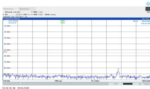
NTNV-n38-PC1.5-30-40-L-DFT-QPSK-Inner_1RB_Right-0.009-0.15-PASS
