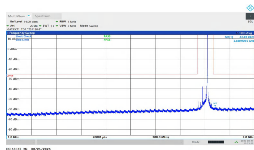
NTVN-n38-PC1.5-30-40-H-DFT-QPSK-Inner_1RB_Right-1000-3000-PASS
