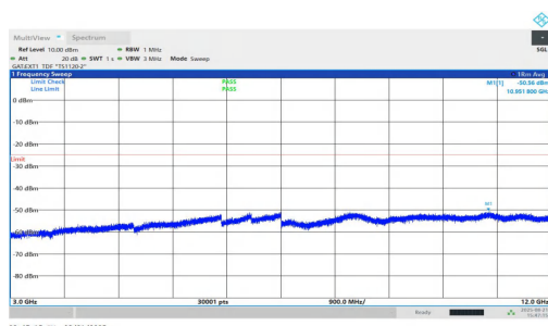
NTVN-n38-PC1.5-30-40-M-DFT-QPSK-Inner_1RB_Right-3000-12000-PASS
