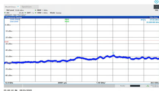
NTNV-n38-PC1.5-30-40-H-DFT-BPSK-Inner_1RB_Left-12000-265 00-PASS
