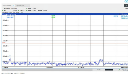
NTNV-n38-PC1.5-30-40-L-DFT-QPSK-Inner_1RB_Left-0.009-0.1 5-PASS
