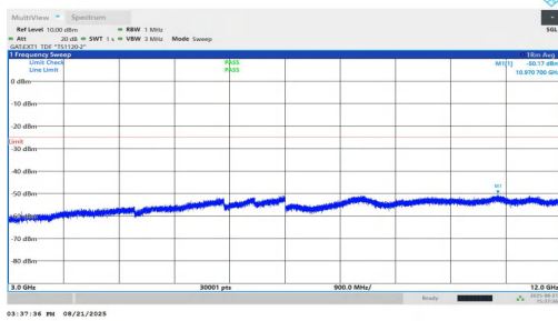
NTNV-n38-PC1.5-30-40-L-DFT-BPSK-Inner_1RB_Right-3000-12 000-PASS
