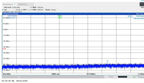
NTNV-n38-PC1.5-30-40-L-DFT-BPSK-Inner_1RB_Right-30-1000 -PASS
