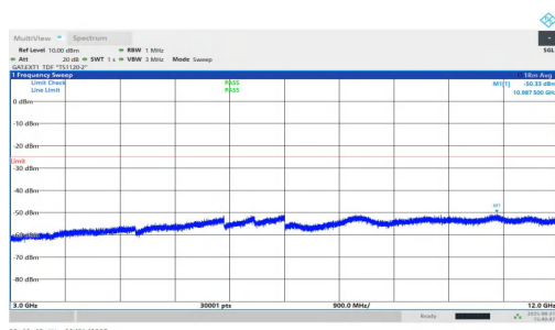
NTNV-n38-PC1.5-30-40-L-DFT-QPSK-Inner_1RB_Right-3000-12000-PASS
