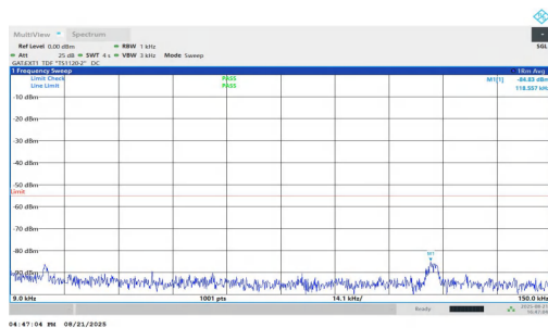
NTNV-n38-PC1.5-30-40-H-DFT-BPSK-Inner_1RB_Right-0.009-0. 15-PASS
