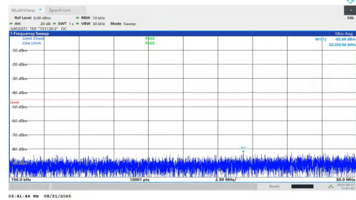
NTNV-n38-PC1.5-30-40-M-DFT-BPSK-Inner_1RB_Left-0.15-30-P ASS
