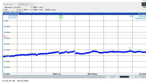
NTNV-n38-PC1.5-30-30-M-DFT-QPSK-Inner_1RB_Left-3000-12000-PASS
