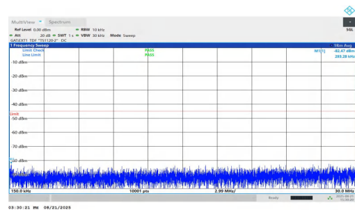
NTNV-n38-PC1.5-30-30-H-DFT-BPSK-Inner_1RB_Right-0.15-30- PASS
