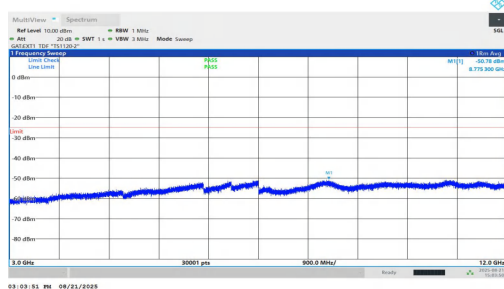
NTNV-n38-PC1.5-30-25-M-DFT-BPSK-Inner_1RB_Left-3000-120 00-PASS
