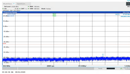
NTVN-n38-PC1.5-30-30-M-DFT-BPSK-Inner_1RB_Right-30-1000-PASS
