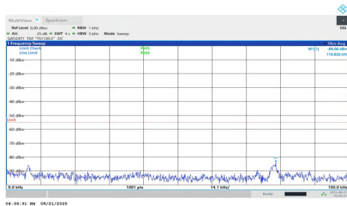
NTNV-n38-PC1.5-30-30-L-DFT-QPSK-Inner_1RB_Right-0.009-0.15-PASS
