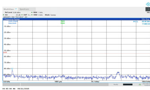
NTVN-n38-PC1.5-30-30-H-DFT-QPSK-Inner_1RB_Left-0.009-0.1 5-PASS
