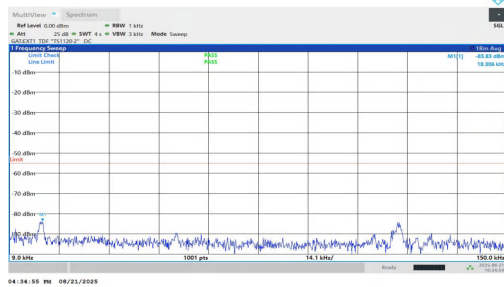
NTNV-n38-PC1.5-30-30-L-DFT-BPSK-Inner_1RB_Left-0.009-0.1 5-PASS
