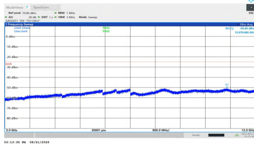
NTVN-n38-PC1.5-30-25-H-DFT-QPSK-Inner_1RB_Left-3000-12000-PASS
