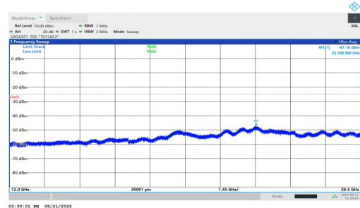
NTNV-n38-PC1.5-30-30-H-DFT-BPSK-Inner_1RB_Left-12000-265 00-PASS
