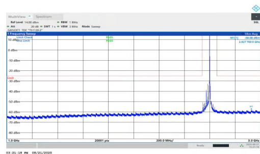
NTNV-n38-PC1.5-30-30-L-DFT-QPSK-Inner_1RB_Right-1000-3000-PASS
