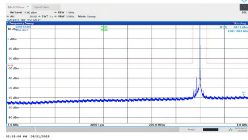
NTNV-n38-PC1.5-30-30-L-DFT-BPSK-Inner_1RB_Right-1000-300 0-PASS
