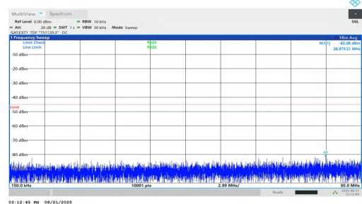
NTVN-n38-PC1.5-30-25-H-DFT-QPSK-Inner_1RB_Left-0.15-30-P ASS
