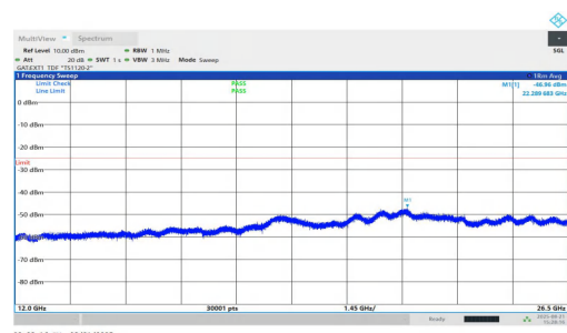
NTNV-n38-PC1.5-30-30-M-DFT-QPSK-Inner_1RB_Right-12000-26500-PASS
