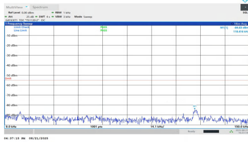
NTNV-n38-PC1.5-30-30-M-DFT-BPSK-Inner_1RB_Left-0.009-0.1 5-PASS
