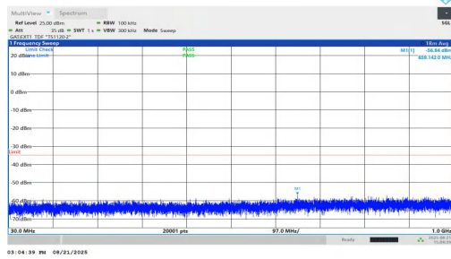
NTVN-n38-PC1.5-30-25-M-DFT-BPSK-Inner_1RB_Right-30-1000-PASS
