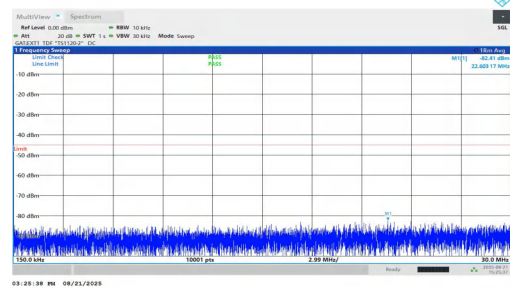
NTVN-n38-PC1.5-30-30-M-DFT-QPSK-Inner_1RB_Left-0.15-30-PASS
