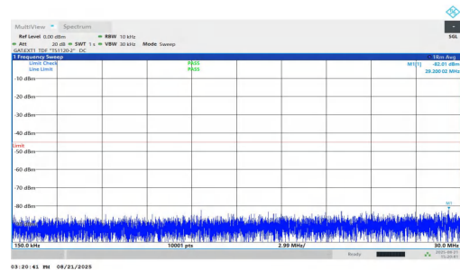
NTNV-n38-PC1.5-30-30-L-DFT-QPSK-Inner_1RB_Right-0.15-30-PASS
