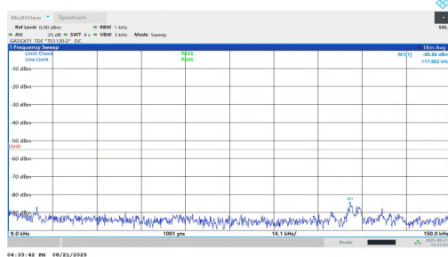
NTVN-n38-PC1.5-30-25-H-DFT-QPSK-Inner_1RB_Left-0.009-0.1 5-PASS
