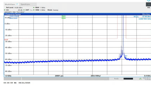
NTVN-n38-PC1.5-30-30-H-DFT-BPSK-Inner_1RB_Right-1000-300 0-PASS
