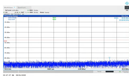
NTNV-n38-PC1.5-30-30-M-DFT-QPSK-Inner_1RB_Right-0.15-30-PASS
