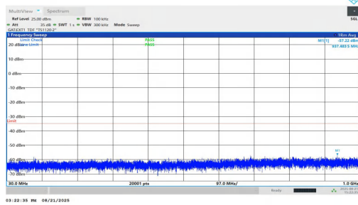
NTNV-n38-PC1.5-30-30-M-DFT-BPSK-Inner_1RB_Left-30-1000- PASS
