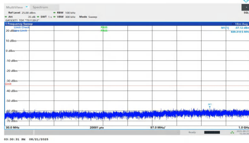
NTVN-n38-PC1.5-30-30-H-DFT-BPSK-Inner_1RB_Right-30-1000 -PASS
