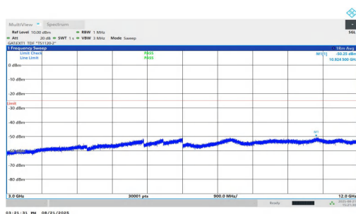
NTNV-n38-PC1.5-30-30-L-DFT-QPSK-Inner_1RB_Right-3000-12000-PASS
