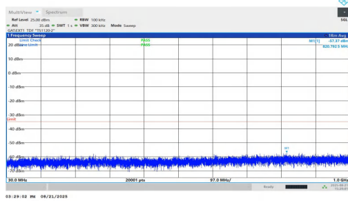
NTNV-n38-PC1.5-30-30-H-DFT-BPSK-Inner_1RB_Left-30-1000- PASS
