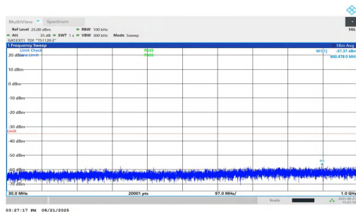
NTNV-n38-PC1.5-30-30-M-DFT-QPSK-Inner_1RB_Right-30-1000-PASS
