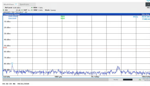
NTNV-n38-PC1.5-30-25-H-DFT-BPSK-Inner_1RB_Left-0.009-0.1 5-PASS
