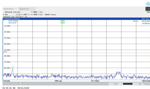
NTNV-n38-PC1.5-30-30-L-DFT-BPSK-Inner_1RB_Right-0.009-0. 15-PASS
