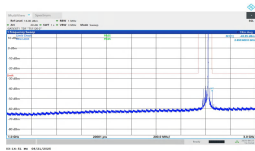
NTVN-n38-PC1.5-30-25-H-DFT-QPSK-Inner_1RB_Right-1000-3000-PASS
