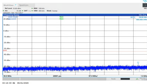
NTNV-n38-PC1.5-30-30-L-DFT-BPSK-Inner_1RB_Left-30-1000-P ASS
