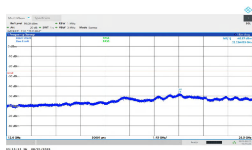
NTVN-n38-PC1.5-30-25-H-DFT-QPSK-Inner_1RB_Right-12000-26500-PASS
