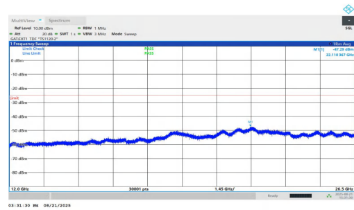
NTVN-n38-PC1.5-30-30-H-DFT-BPSK-Inner_1RB_Right-12000-26 500-PASS
