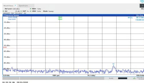
NTNV-n38-PC1.5-30-30-L-DFT-QPSK-Inner_1RB_Left-0.009-0.1 5-PASS
