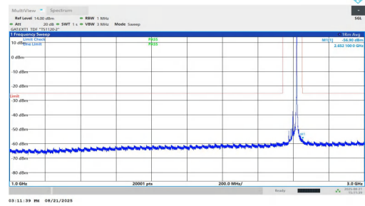
NTVN-n38-PC1.5-30-25-H-DFT-BPSK-Inner_1RB_Right-1000-300 0-PASS
