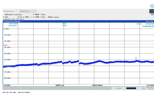
NTVN-n38-PC1.5-30-25-H-DFT-QPSK-Inner_1RB_Right-3000-12000-PASS
