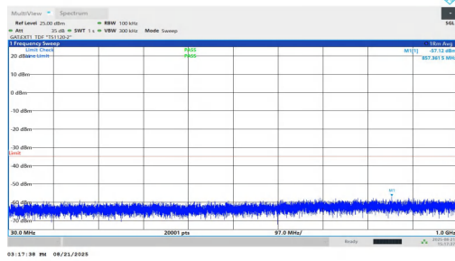
NTNV-n38-PC1.5-30-30-L-DFT-BPSK-Inner_1RB_Right-30-1000 -PASS
