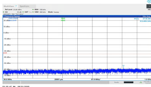
NTVN-n38-PC1.5-30-30-M-DFT-QPSK-Inner_1RB_Left-30-1000-PASS
