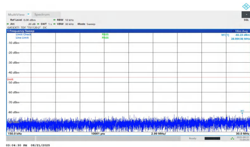
NTNV-n38-PC1.5-30-25-M-DFT-BPSK-Inner_1RB_Right-0.15-30- PASS
