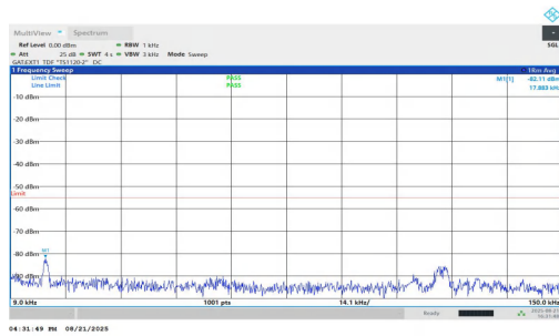
NTVN-n38-PC1.5-30-25-M-DFT-QPSK-Inner_1RB_Right-0.009-0.15-PASS
