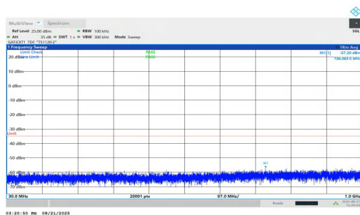
NTNV-n38-PC1.5-30-30-L-DFT-QPSK-Inner_1RB_Right-30-1000-PASS
