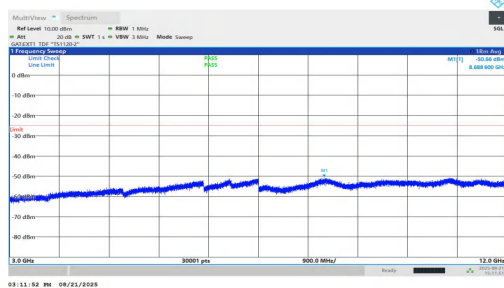
NTVN-n38-PC1.5-30-25-H-DFT-BPSK-Inner_1RB_Right-3000-12 000-PASS
