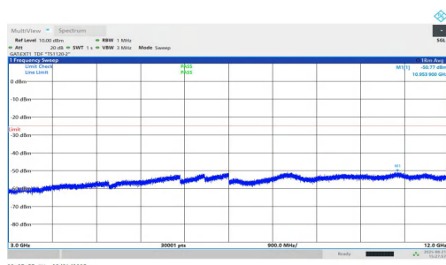
NTNV-n38-PC1.5-30-30-M-DFT-QPSK-Inner_1RB_Right-3000-12000-PASS
