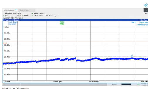
NTVN-n38-PC1.5-30-25-M-DFT-QPSK-Inner_1RB_Right-3000-12000-PASS
