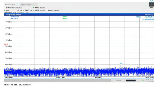
NTNV-n38-PC1.5-30-25-M-DFT-BPSK-Inner_1RB_Left-0.15-30-P ASS
