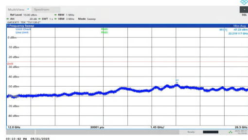
NTNV-n38-PC1.5-30-25-H-DFT-BPSK-Inner_1RB_Left-12000-265 00-PASS
