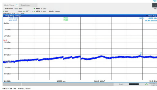
NTNV-n38-PC1.5-30-30-M-DFT-BPSK-Inner_1RB_Left-3000-120 00-PASS
