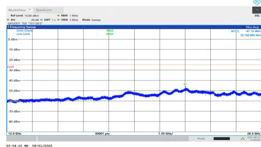
NTNV-n38-PC1.5-30-25-M-DFT-BPSK-Inner_1RB_Left-12000-265 00-PASS
