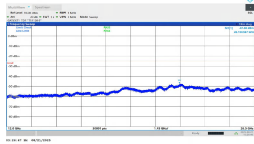
NTNV-n38-PC1.5-30-30-M-DFT-QPSK-Inner_1RB_Left-12000-26500-PASS
