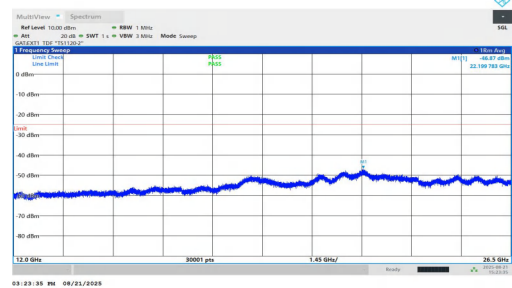
NTNV-n38-PC1.5-30-30-M-DFT-BPSK-Inner_1RB_Left-12000-265 00-PASS
