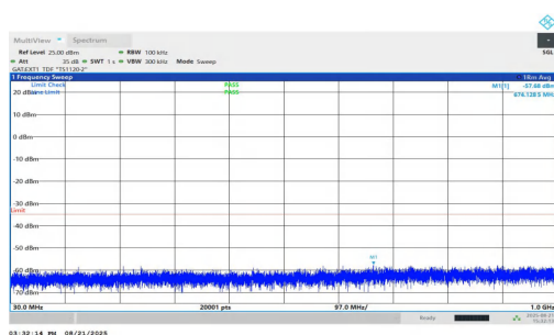
NTVN-n38-PC1.5-30-30-H-DFT-QPSK-Inner_1RB_Left-30-1000- PASS
