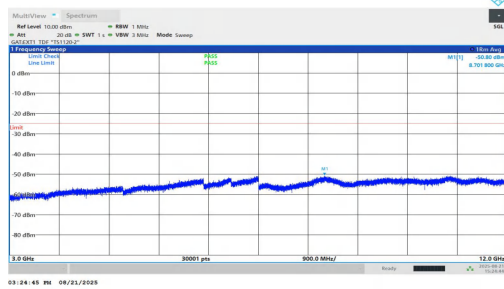
NTVN-n38-PC1.5-30-30-M-DFT-BPSK-Inner_1RB_Right-3000-12000-PASS
