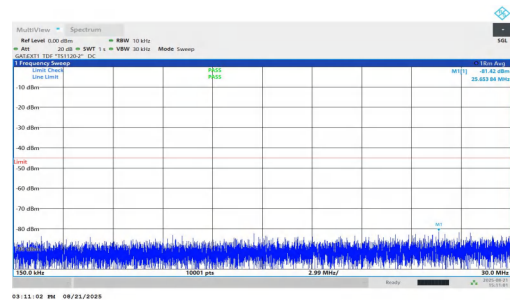
NTNV-n38-PC1.5-30-25-H-DFT-BPSK-Inner_1RB_Right-0.15-30- PASS
