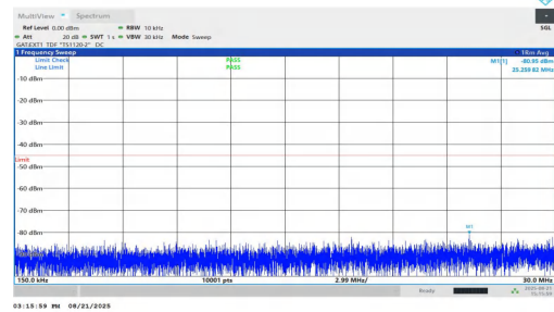
NTNV-n38-PC1.5-30-30-L-DFT-BPSK-Inner_1RB_Left-0.15-30-PA SS
