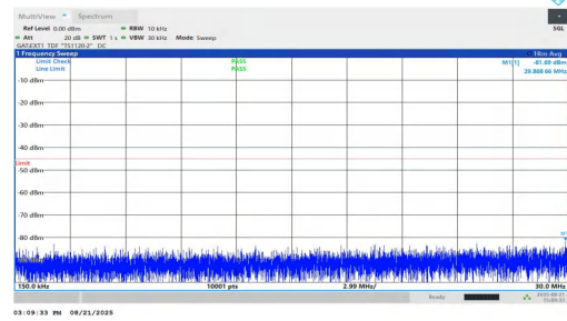
NTNV-n38-PC1.5-30-25-H-DFT-BPSK-Inner_1RB_Left-0.15-30-P ASS
