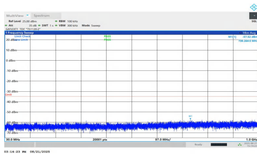
NTVN-n38-PC1.5-30-25-H-DFT-QPSK-Inner_1RB_Right-30-1000-PASS
