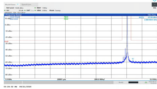
NTVN-n38-PC1.5-30-30-M-DFT-BPSK-Inner_1RB_Right-1000-3000-PASS
