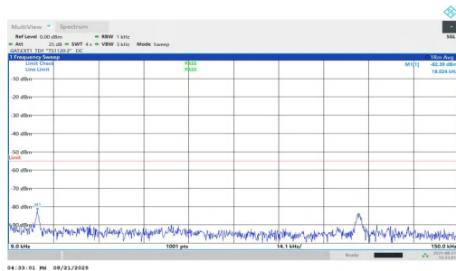
NTNV-n38-PC1.5-30-25-H-DFT-BPSK-Inner_1RB_Right-0.009-0. 15-PASS
