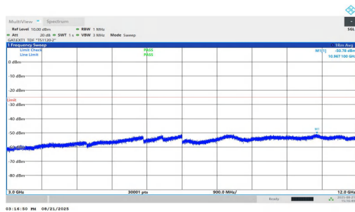
NTNV-n38-PC1.5-30-30-L-DFT-BPSK-Inner_1RB_Left-3000-120 00-PASS
