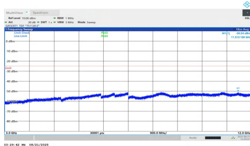
NTNV-n38-PC1.5-30-30-H-DFT-BPSK-Inner_1RB_Left-3000-120 00-PASS
