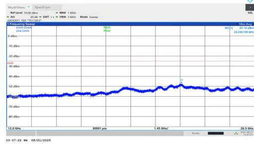
NTVN-n38-PC1.5-30-25-M-DFT-QPSK-Inner_1RB_Left-12000-26500-PASS
