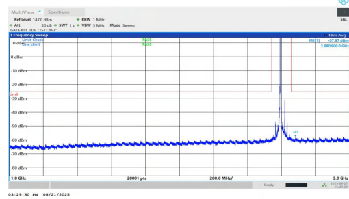
NTNV-n38-PC1.5-30-30-H-DFT-BPSK-Inner_1RB_Left-1000-3000 -PASS
