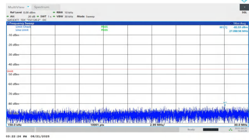
NTNV-n38-PC1.5-30-30-M-DFT-BPSK-Inner_1RB_Left-0.15-30-P ASS
