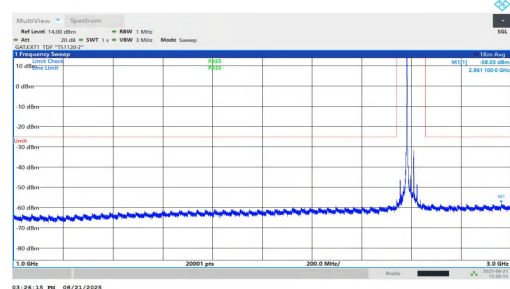
NTVN-n38-PC1.5-30-30-M-DFT-QPSK-Inner_1RB_Left-1000-3000-PASS
