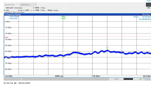
NTVN-n38-PC1.5-30-30-M-DFT-BPSK-Inner_1RB_Right-12000-26500-PASS
