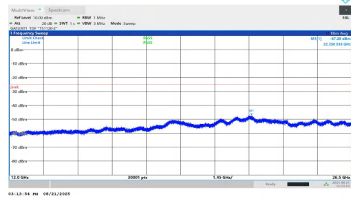
NTVN-n38-PC1.5-30-25-H-DFT-QPSK-Inner_1RB_Left-12000-26500-PASS
