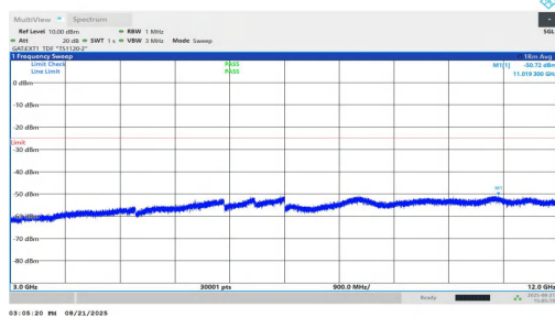
NTVN-n38-PC1.5-30-25-M-DFT-BPSK-Inner_1RB_Right-3000-12000-PASS
