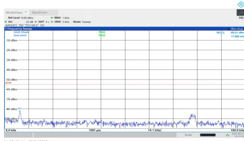
NTNV-n38-PC1.5-30-30-M-DFT-BPSK-Inner_1RB_Right-0.009-0. 15-PASS
