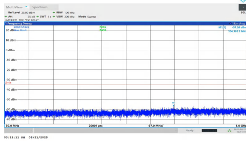
NTVN-n38-PC1.5-30-25-H-DFT-BPSK-Inner_1RB_Right-30-1000 -PASS
