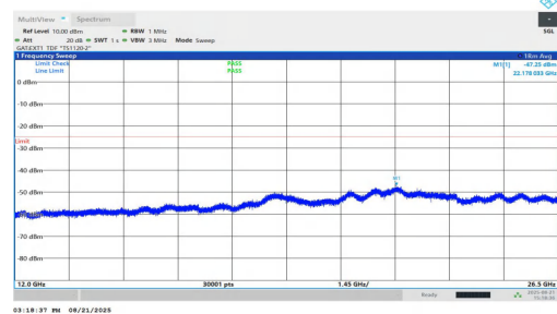
NTNV-n38-PC1.5-30-30-L-DFT-BPSK-Inner_1RB_Right-12000-26 500-PASS
