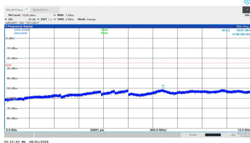
NTNV-n38-PC1.5-30-25-H-DFT-BPSK-Inner_1RB_Left-3000-120 00-PASS
