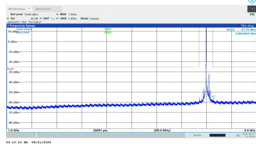
NTNV-n38-PC1.5-30-25-H-DFT-BPSK-Inner_1RB_Left-1000-3000 -PASS
