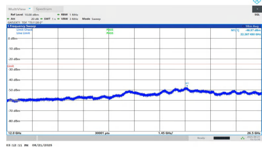
NTVN-n38-PC1.5-30-25-H-DFT-BPSK-Inner_1RB_Right-12000-26 500-PASS
