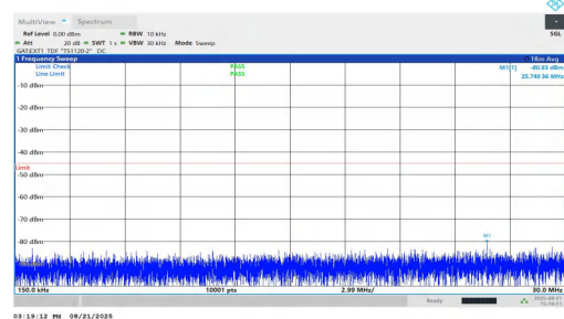
NTNV-n38-PC1.5-30-30-L-DFT-QPSK-Inner_1RB_Left-0.15-30-PA SS
