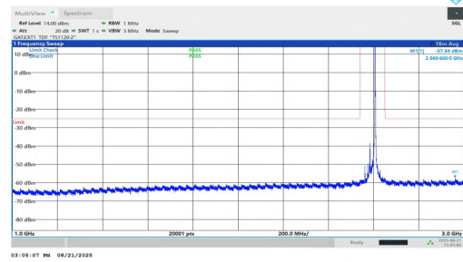
NTVN-n38-PC1.5-30-25-M-DFT-BPSK-Inner_1RB_Right-1000-3000-PASS
