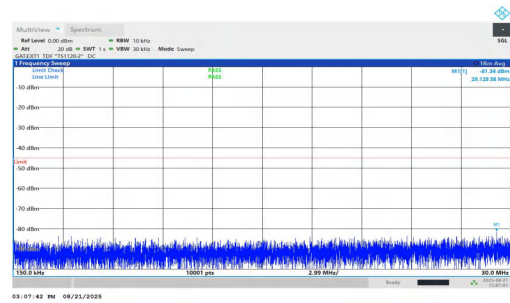
NTVN-n38-PC1.5-30-25-M-DFT-QPSK-Inner_1RB_Right-0.15-30-PASS
