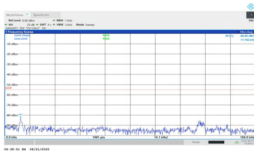
NTNV-n38-PC1.5-30-30-M-DFT-QPSK-Inner_1RB_Right-0.009-0.15-PASS
