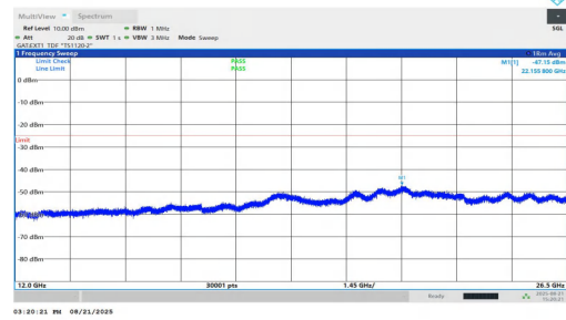
NTNV-n38-PC1.5-30-30-L-DFT-QPSK-Inner_1RB_Left-12000-26500-PASS
