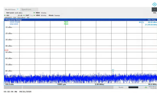
NTVN-n38-PC1.5-30-30-H-DFT-QPSK-Inner_1RB_Left-0.15-30-P ASS
