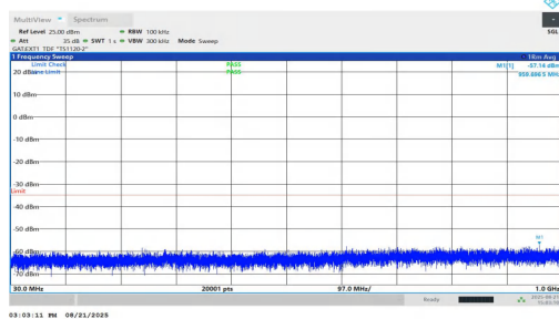
NTNV-n38-PC1.5-30-25-M-DFT-BPSK-Inner_1RB_Left-30-1000- PASS
