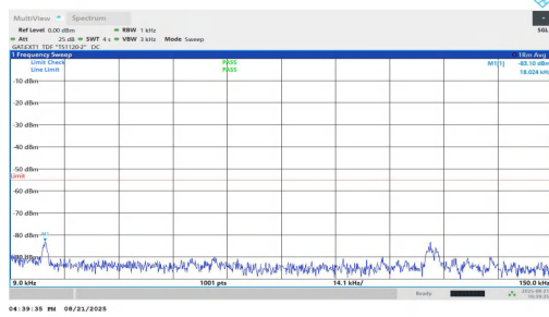
NTNV-n38-PC1.5-30-30-H-DFT-BPSK-Inner_1RB_Left-0.009-0.1 5-PASS
