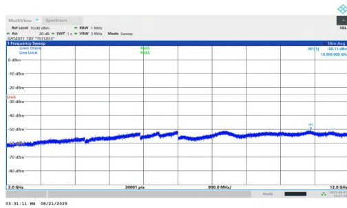
NTVN-n38-PC1.5-30-30-H-DFT-BPSK-Inner_1RB_Right-3000-12 000-PASS
