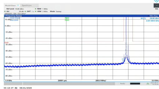
NTNV-n38-PC1.5-30-30-L-DFT-BPSK-Inner_1RB_Left-1000-3000 -PASS
