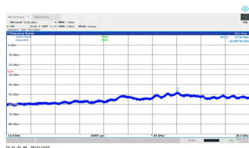
NTNV-n38-PC1.5-30-30-L-DFT-QPSK-Inner_1RB_Right-12000-26500-PASS
