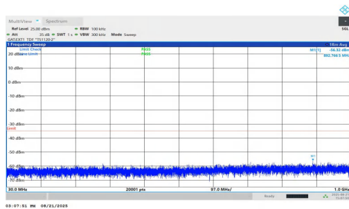
NTVN-n38-PC1.5-30-25-M-DFT-QPSK-Inner_1RB_Right-30-1000-PASS
