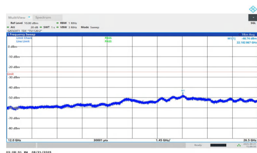
NTVN-n38-PC1.5-30-25-M-DFT-QPSK-Inner_1RB_Right-12000-26500-PASS
