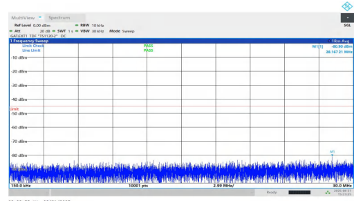
NTNV-n38-PC1.5-30-30-M-DFT-BPSK-Inner_1RB_Right-0.15-30- PASS
