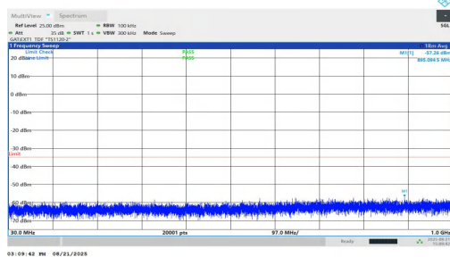
NTNV-n38-PC1.5-30-25-H-DFT-BPSK-Inner_1RB_Left-30-1000- PASS
