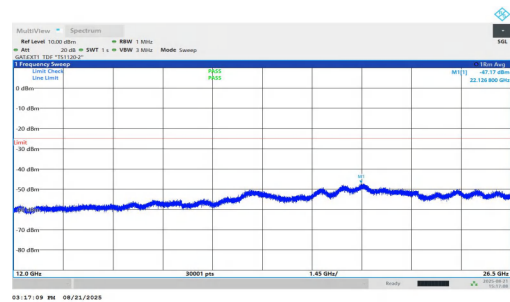
NTNV-n38-PC1.5-30-30-L-DFT-BPSK-Inner_1RB_Left-12000-265 00-PASS
