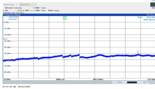
NTVN-n38-PC1.5-30-25-M-DFT-QPSK-Inner_1RB_Left-3000-12000-PASS
