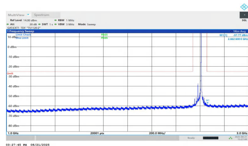
NTNV-n38-PC1.5-30-30-M-DFT-QPSK-Inner_1RB_Right-1000-3000-PASS
