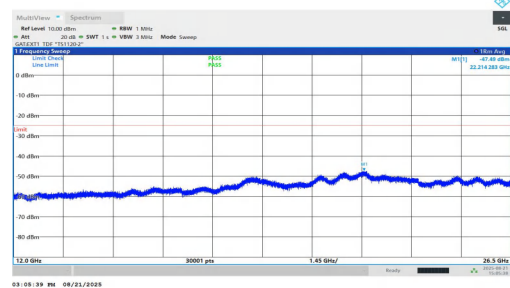
NTVN-n38-PC1.5-30-25-M-DFT-BPSK-Inner_1RB_Right-12000-26500-PASS
