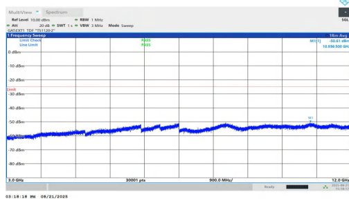
NTNV-n38-PC1.5-30-30-L-DFT-BPSK-Inner_1RB_Right-3000-12 000-PASS
