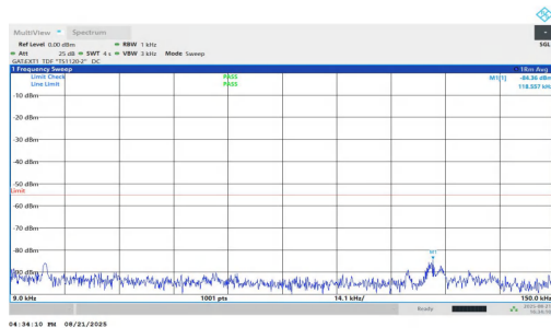
NTVN-n38-PC1.5-30-25-H-DFT-QPSK-Inner_1RB_Right-0.009-0.15-PASS
