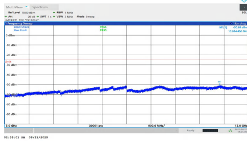
NTVN-n38-PC1.5-30-15-H-DFT-QPSK-Inner_1RB_Left-3000-12000-PASS
