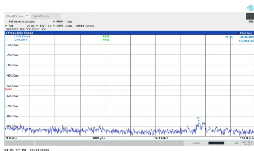
NTNV-n38-PC1.5-30-20-L-DFT-BPSK-Inner_1RB_Right-0.009-0. 15-PASS
