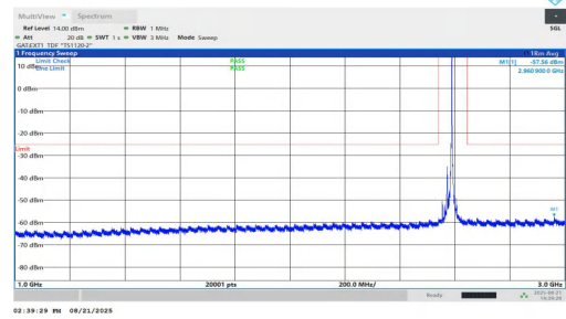
NTNV-n38-PC1.5-30-20-L-DFT-BPSK-Inner_1RB_Right-1000-300 0-PASS
