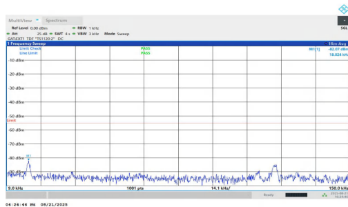
NTVN-n38-PC1.5-30-20-M-DFT-QPSK-Inner_1RB_Right-0.009-0.15-PASS
