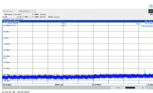
NTVN-n38-PC1.5-30-20-H-DFT-QPSK-Inner_1RB_Left-30-1000- PASS
