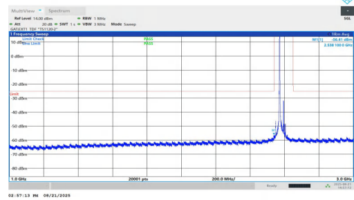
NTNV-n38-PC1.5-30-25-L-DFT-BPSK-Inner_1RB_Left-1000-3000-PASS
