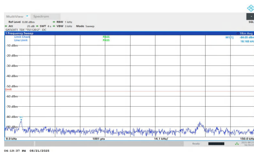
NTNV-n38-PC1.5-30-15-H-DFT-QPSK-Inner_1RB_Left-0.009-0.1 5-PASS
