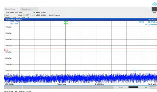
NTNV-n38-PC1.5-30-20-M-DFT-BPSK-Inner_1RB_Right-0.15-30- PASS
