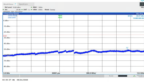
NTNV-n38-PC1.5-30-25-L-DFT-QPSK-Inner_1RB_Left-3000-12000-PASS
