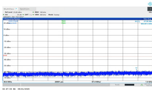
NTVN-n38-PC1.5-30-20-M-DFT-QPSK-Inner_1RB_Left-30-1000-PASS
