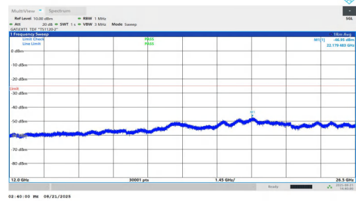
NTNV-n38-PC1.5-30-20-L-DFT-BPSK-Inner_1RB_Right-12000-26 500-PASS
