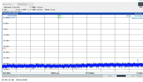
NTNV-n38-PC1.5-30-25-L-DFT-BPSK-Inner_1RB_Right-30-1000 -PASS
