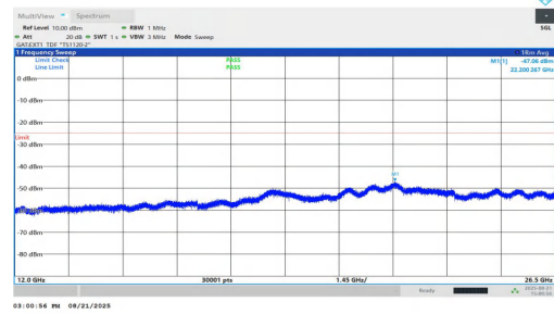
NTNV-n38-PC1.5-30-25-L-DFT-QPSK-Inner_1RB_Left-12000-26500-PASS
