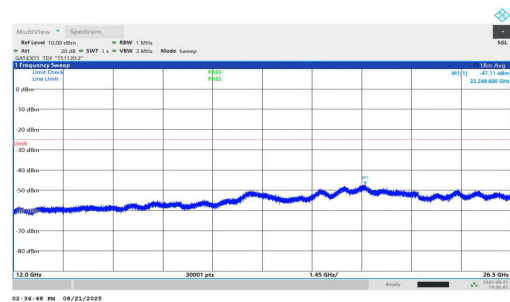
NTVN-n38-PC1.5-30-15-H-DFT-QPSK-Inner_1RB_Right-12000-26500-PASS
