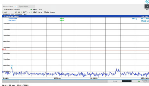
NTNV-n38-PC1.5-30-20-L-DFT-QPSK-Inner_1RB_Left-0.009-0.1 5-PASS
