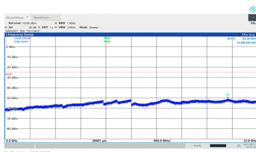
NTVN-n38-PC1.5-30-20-H-DFT-QPSK-Inner_1RB_Right-3000-12000-PASS
