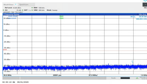
NTNV-n38-PC1.5-30-20-H-DFT-BPSK-Inner_1RB_Left-30-1000- PASS
