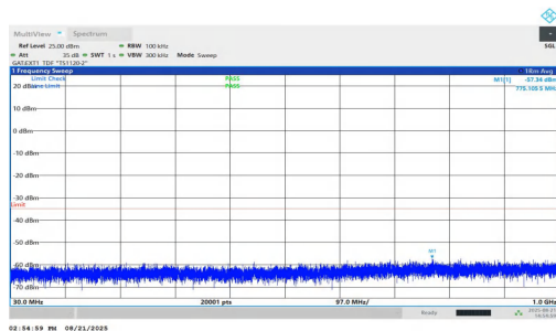
NTVN-n38-PC1.5-30-20-H-DFT-QPSK-Inner_1RB_Right-30-1000-PASS
