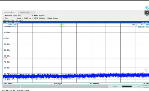
NTNV-n38-PC1.5-30-15-H-DFT-QPSK-Inner_1RB_Left-30-1000- PASS
