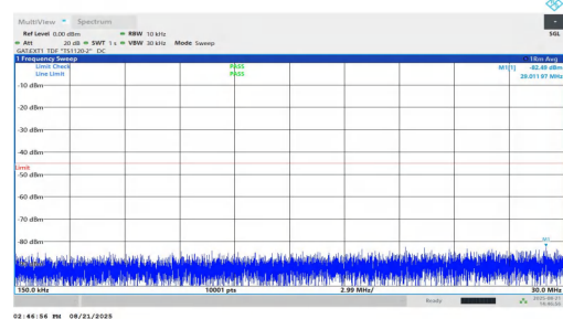
NTVN-n38-PC1.5-30-20-M-DFT-QPSK-Inner_1RB_Left-0.15-30-PASS
