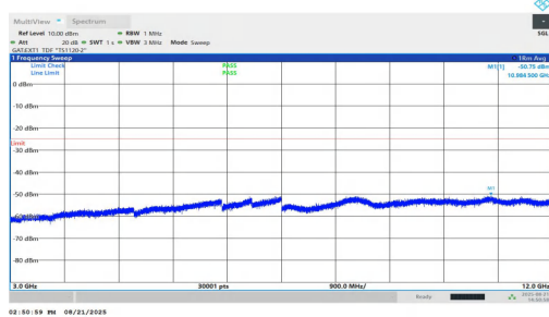
NTNV-n38-PC1.5-30-20-H-DFT-BPSK-Inner_1RB_Left-3000-120 00-PASS
