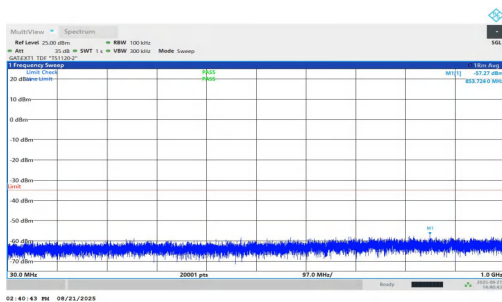
NTNV-n38-PC1.5-30-20-L-DFT-QPSK-Inner_1RB_Left-30-1000- PASS
