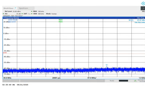
NTVN-n38-PC1.5-30-15-H-DFT-QPSK-Inner_1RB_Right-30-1000-PASS
