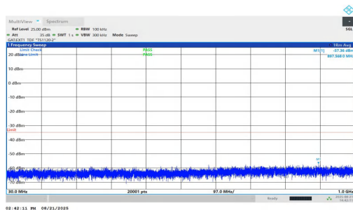
NTNV-n38-PC1.5-30-20-L-DFT-QPSK-Inner_1RB_Right-30-1000-PASS
