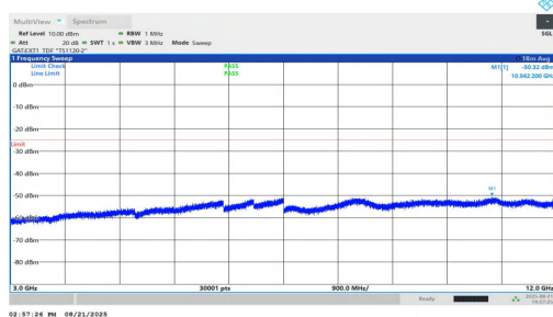
NTNV-n38-PC1.5-30-25-L-DFT-BPSK-Inner_1RB_Left-3000-12000-PASS
