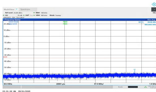
NTNV-n38-PC1.5-30-25-L-DFT-QPSK-Inner_1RB_Right-30-1000-PASS
