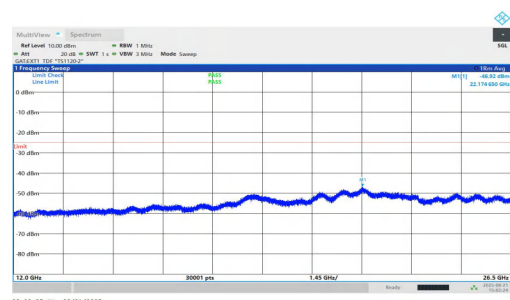
NTNV-n38-PC1.5-30-25-L-DFT-QPSK-Inner_1RB_Right-12000-26500-PASS
