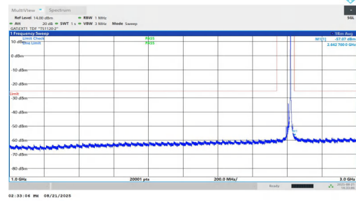
NTNV-n38-PC1.5-30-15-H-DFT-BPSK-Inner_1RB_Right-1000-300 0-PASS
