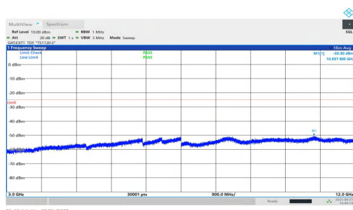
NTVN-n38-PC1.5-30-20-M-DFT-QPSK-Inner_1RB_Right-3000-12000-PASS
