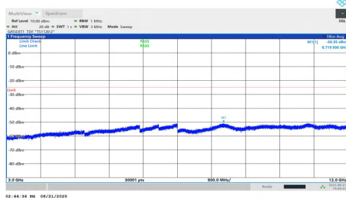
NTNV-n38-PC1.5-30-20-M-DFT-BPSK-Inner_1RB_Left-3000-120 00-PASS
