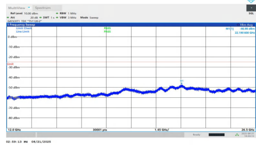
NTNV-n38-PC1.5-30-25-L-DFT-BPSK-Inner_1RB_Right-12000-26 500-PASS
