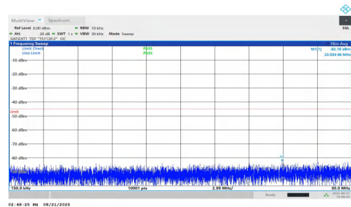
NTVN-n38-PC1.5-30-20-M-DFT-QPSK-Inner_1RB_Right-0.15-30-PASS
