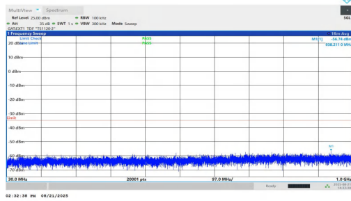
NTNV-n38-PC1.5-30-15-H-DFT-BPSK-Inner_1RB_Right-30-1000 -PASS
