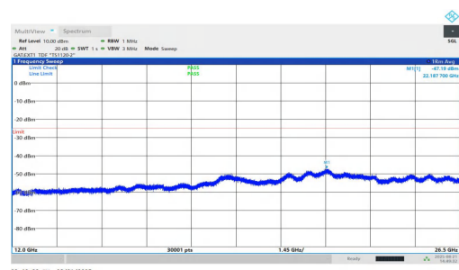
NTVN-n38-PC1.5-30-20-M-DFT-QPSK-Inner_1RB_Right-12000-26500-PASS
