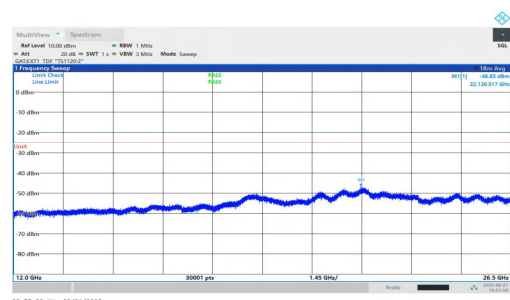
NTVN-n38-PC1.5-30-20-H-DFT-QPSK-Inner_1RB_Right-12000-26500-PASS
