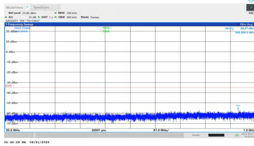
NTVN-n38-PC1.5-30-20-M-DFT-BPSK-Inner_1RB_Right-30-1000-PASS
