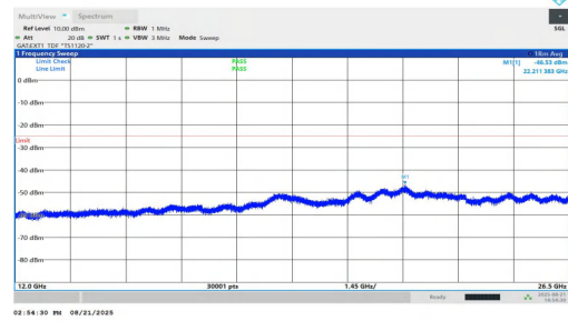
NTVN-n38-PC1.5-30-20-H-DFT-QPSK-Inner_1RB_Left-12000-26500-PASS
