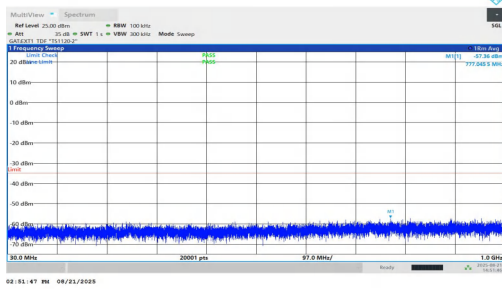
NTVN-n38-PC1.5-30-20-H-DFT-BPSK-Inner_1RB_Right-30-1000 -PASS
