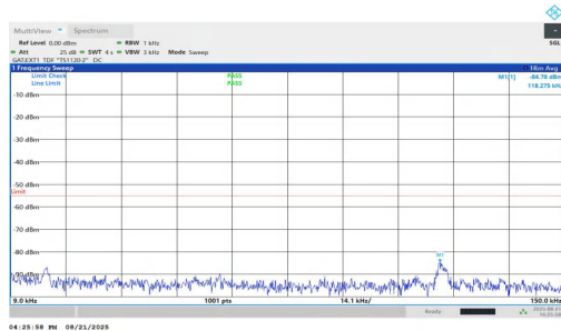
NTNV-n38-PC1.5-30-20-H-DFT-BPSK-Inner_1RB_Right-0.009-0. 15-PASS
