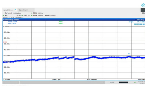
NTNV-n38-PC1.5-30-20-L-DFT-QPSK-Inner_1RB_Right-3000-12000-PASS
