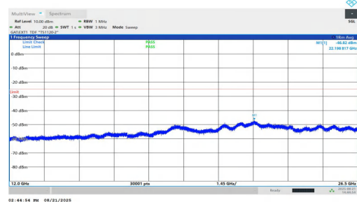
NTNV-n38-PC1.5-30-20-M-DFT-BPSK-Inner_1RB_Left-12000-265 00-PASS
