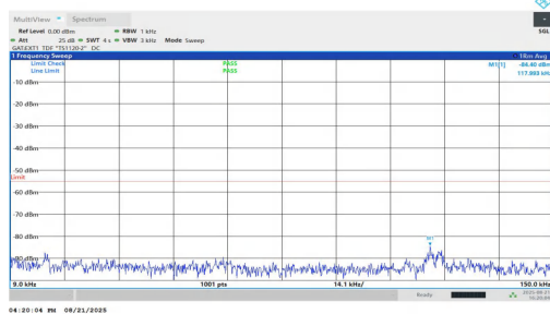
NTVN-n38-PC1.5-30-15-H-DFT-QPSK-Inner_1RB_Right-0.009-0.15-PASS
