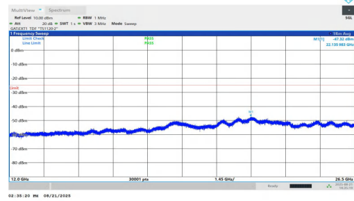
NTVN-n38-PC1.5-30-15-H-DFT-QPSK-Inner_1RB_Left-12000-265-PASS
