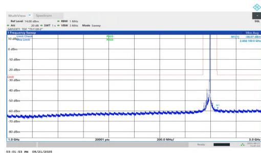
NTNV-n38-PC1.5-30-25-L-DFT-QPSK-Inner_1RB_Right-1000-3000-PASS
