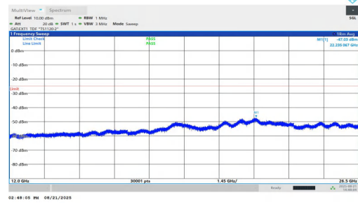
NTVN-n38-PC1.5-30-20-M-DFT-QPSK-Inner_1RB_Left-12000-26500-PASS
