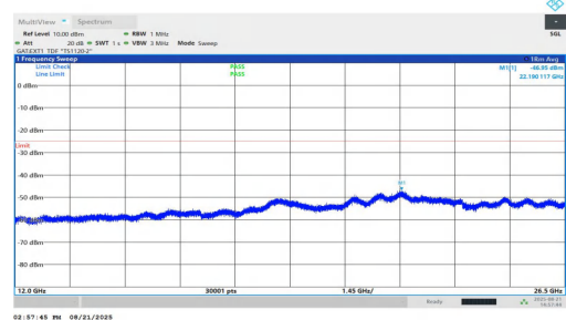
NTNV-n38-PC1.5-30-25-L-DFT-BPSK-Inner_1RB_Left-12000-26500-PASS
