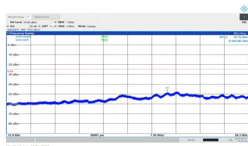
NTNV-n38-PC1.5-30-20-L-DFT-QPSK-Inner_1RB_Right-12000-26500-PASS
