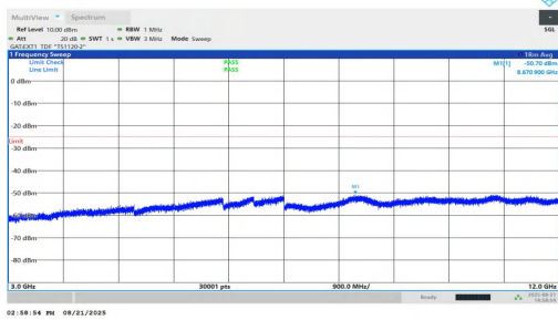
NTNV-n38-PC1.5-30-25-L-DFT-BPSK-Inner_1RB_Right-3000-12 000-PASS
