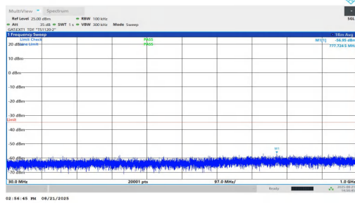
NTNV-n38-PC1.5-30-25-L-DFT-BPSK-Inner_1RB_Left-30-1000-P ASS
