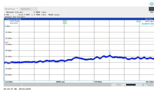
NTNV-n38-PC1.5-30-15-H-DFT-BPSK-Inner_1RB_Right-12000-26 500-PASS
