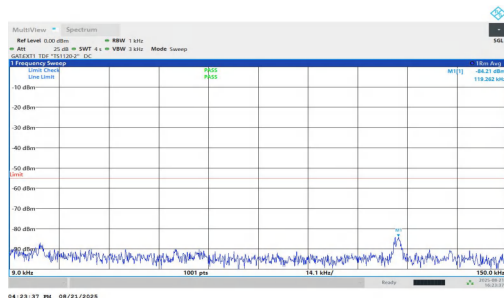
NTNV-n38-PC1.5-30-20-M-DFT-BPSK-Inner_1RB_Right-0.009-0. 15-PASS
