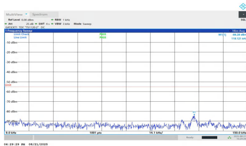
NTNV-n38-PC1.5-30-25-L-DFT-QPSK-Inner_1RB_Right-0.009-0.15-PASS
