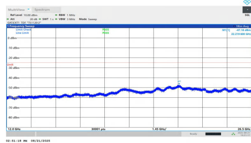
NTNV-n38-PC1.5-30-20-H-DFT-BPSK-Inner_1RB_Left-12000-265 00-PASS
