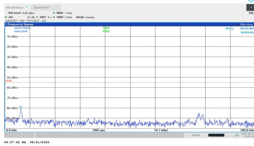
NTNV-n38-PC1.5-30-25-L-DFT-BPSK-Inner_1RB_Left-0.009-0.15-PASS
