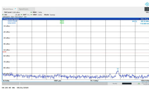
NTVN-n38-PC1.5-30-20-H-DFT-QPSK-Inner_1RB_Left-0.009-0.1 5-PASS
