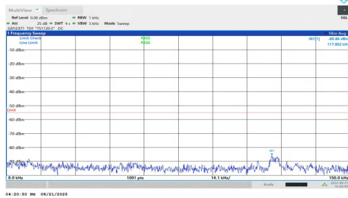
NTNV-n38-PC1.5-30-20-L-DFT-BPSK-Inner_1RB_Left-0.009-0.1 5-PASS
