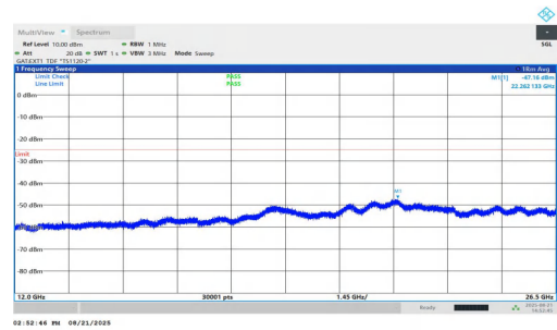
NTVN-n38-PC1.5-30-20-H-DFT-BPSK-Inner_1RB_Right-12000-26 500-PASS
