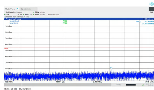
NTNV-n38-PC1.5-30-25-L-DFT-QPSK-Inner_1RB_Right-0.15-30-PASS
