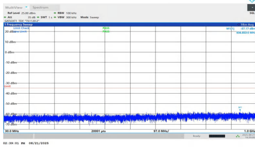
NTNV-n38-PC1.5-30-20-L-DFT-BPSK-Inner_1RB_Right-30-1000 -PASS
