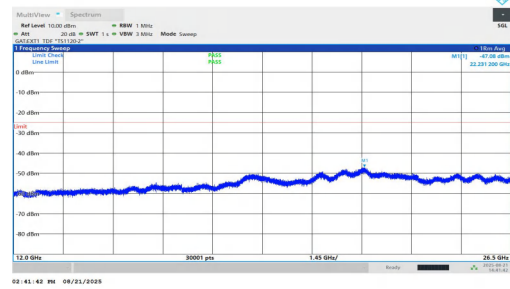
NTNV-n38-PC1.5-30-20-L-DFT-QPSK-Inner_1RB_Left-12000-26500-PASS
