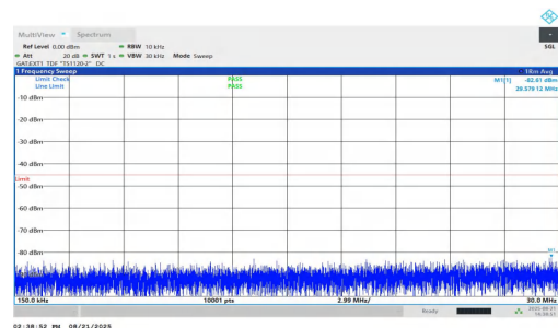
NTNV-n38-PC1.5-30-20-L-DFT-BPSK-Inner_1RB_Right-0.15-30-P ASS
