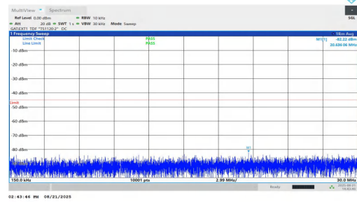
NTNV-n38-PC1.5-30-20-M-DFT-BPSK-Inner_1RB_Left-0.15-30-P ASS
