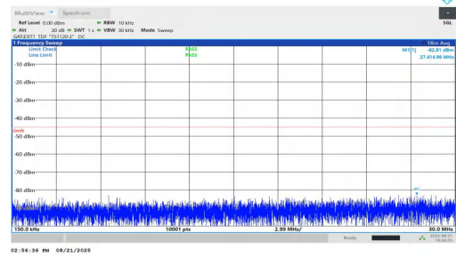
NTNV-n38-PC1.5-30-25-L-DFT-BPSK-Inner_1RB_Left-0.15-30-PA-SS
