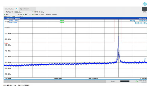
NTVN-n38-PC1.5-30-20-M-DFT-QPSK-Inner_1RB_Right-1000-3000-PASS
