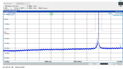
NTNV-n38-PC1.5-30-25-L-DFT-BPSK-Inner_1RB_Right-1000-300 0-PASS
