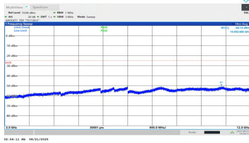
NTVN-n38-PC1.5-30-20-H-DFT-QPSK-Inner_1RB_Left-3000-12000-PASS
