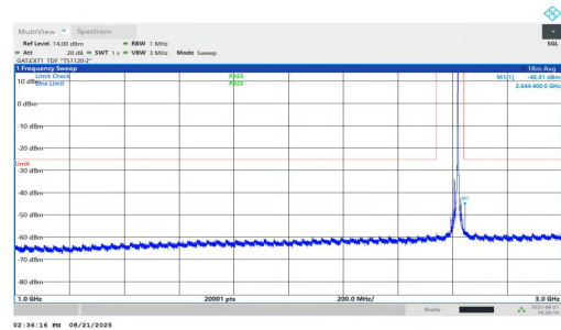
NTVN-n38-PC1.5-30-15-H-DFT-QPSK-Inner_1RB_Right-1000-3000-PASS
