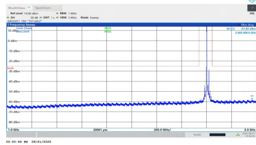
NTNV-n38-PC1.5-30-20-H-DFT-BPSK-Inner_1RB_Left-1000-3000 -PASS
