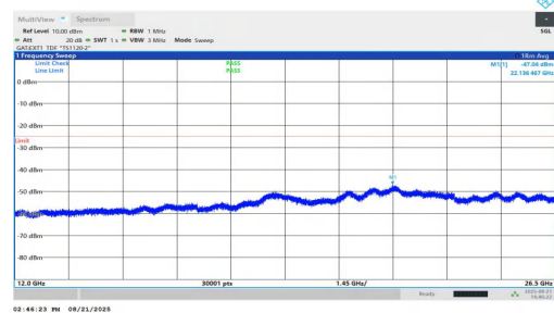
NTVN-n38-PC1.5-30-20-M-DFT-BPSK-Inner_1RB_Right-12000-26500-PASS
