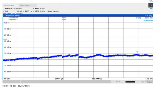
NTVN-n38-PC1.5-30-20-M-DFT-BPSK-Inner_1RB_Right-3000-12000-PASS
