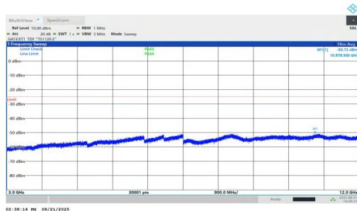
NTNV-n38-PC1.5-30-20-L-DFT-BPSK-Inner_1RB_Left-3000-120 00-PASS
