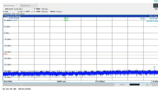
NTNV-n38-PC1.5-30-20-M-DFT-BPSK-Inner_1RB_Left-30-1000- PASS
