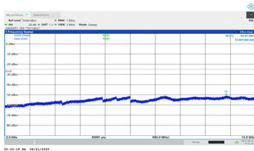
NTNV-n38-PC1.5-30-15-H-DFT-BPSK-Inner_1RB_Right-3000-12 000-PASS
