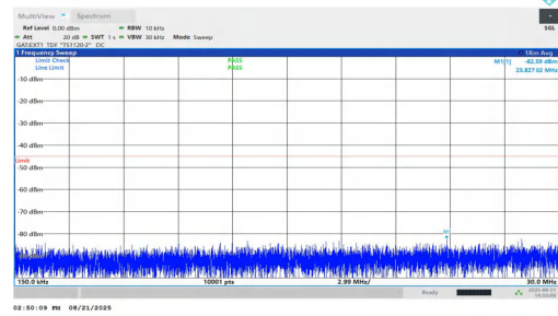
NTNV-n38-PC1.5-30-20-H-DFT-BPSK-Inner_1RB_Left-0.15-30-P ASS
