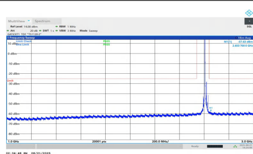
NTNV-n38-PC1.5-30-15-H-DFT-QPSK-Inner_1RB_Left-1000-3000 -PASS
