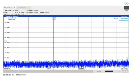
NTVN-n38-PC1.5-30-20-H-DFT-QPSK-Inner_1RB_Left-0.15-30-P ASS
