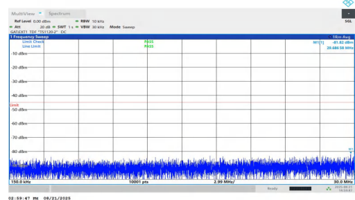
NTNV-n38-PC1.5-30-25-L-DFT-QPSK-Inner_1RB_Left-0.15-30-PA SS
