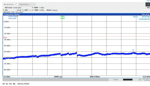
NTNV-n38-PC1.5-30-20-L-DFT-QPSK-Inner_1RB_Left-3000-12000-PASS
