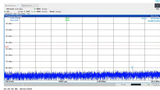
NTVN-n38-PC1.5-30-15-H-DFT-QPSK-Inner_1RB_Right-0.15-30-PASS
