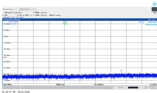
NTNV-n38-PC1.5-30-25-L-DFT-QPSK-Inner_1RB_Left-30-1000- PASS
