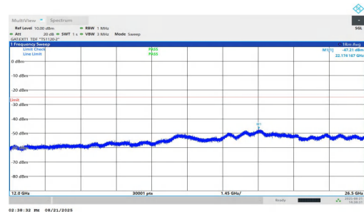
NTNV-n38-PC1.5-30-20-L-DFT-BPSK-Inner_1RB_Left-12000-265 00-PASS
