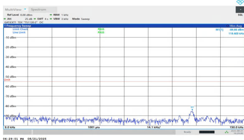
NTNV-n38-PC1.5-30-25-L-DFT-QPSK-Inner_1RB_Left-0.009-0.1 5-PASS
