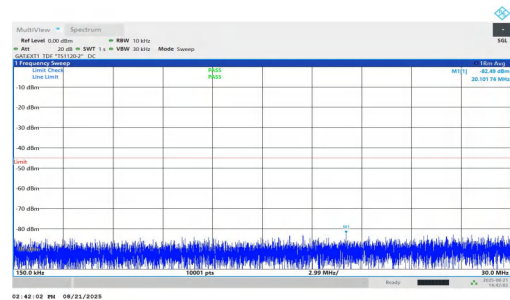
NTNV-n38-PC1.5-30-20-L-DFT-QPSK-Inner_1RB_Right-0.15-30-PASS
