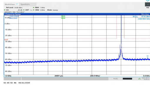
NTVN-n38-PC1.5-30-20-M-DFT-BPSK-Inner_1RB_Right-1000-3000-PASS
