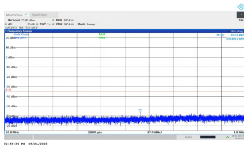
NTVN-n38-PC1.5-30-20-M-DFT-QPSK-Inner_1RB_Right-30-1000-PASS
