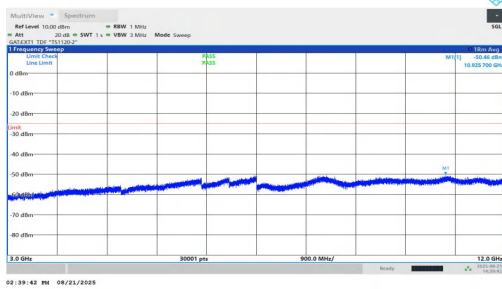
NTNV-n38-PC1.5-30-20-L-DFT-BPSK-Inner_1RB_Right-3000-12 000-PASS
