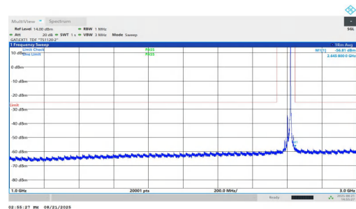
NTVN-n38-PC1.5-30-20-H-DFT-QPSK-Inner_1RB_Right-1000-3000-PASS
