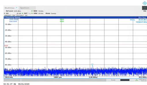
NTNV-n38-PC1.5-30-20-H-DFT-BPSK-Inner_1RB_Right-0.15-30- PASS
