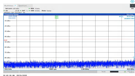
NTNV-n38-PC1.5-30-20-L-DFT-QPSK-Inner_1RB_Left-0.15-30-PA SS
