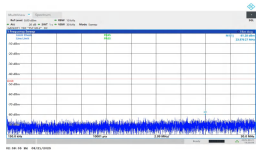
NTNV-n38-PC1.5-30-25-L-DFT-BPSK-Inner_1RB_Right-0.15-30-P ASS
