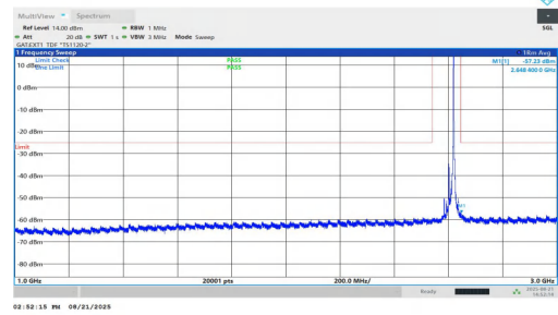
NTVN-n38-PC1.5-30-20-H-DFT-BPSK-Inner_1RB_Right-1000-300 0-PASS
