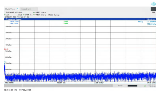
NTVN-n38-PC1.5-30-20-H-DFT-QPSK-Inner_1RB_Right-0.15-30-PASS
