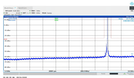
NTNV-n38-PC1.5-30-20-L-DFT-QPSK-Inner_1RB_Right-1000-3000-PASS
