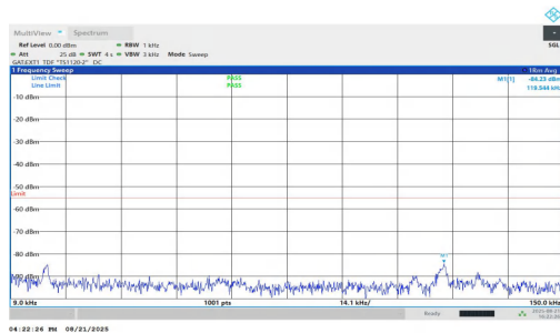
NTNV-n38-PC1.5-30-20-L-DFT-QPSK-Inner_1RB_Right-0.009-0.15-PASS
