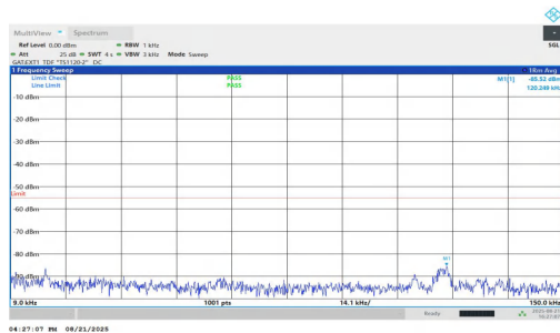
NTVN-n38-PC1.5-30-20-H-DFT-QPSK-Inner_1RB_Right-0.009-0.15-PASS
