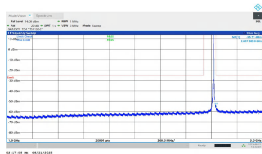
NTVN-n38-PC1.5-30-10-H-DFT-QPSK-Inner_1RB_Right-1000-3000-PASS
