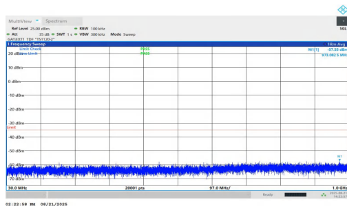
NTNV-n38-PC1.5-30-15-L-DFT-QPSK-Inner_1RB_Right-30-1000-PASS
