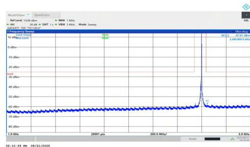
NTVN-n38-PC1.5-30-10-M-DFT-QPSK-Inner_1RB_Right-1000-3000-PASS
