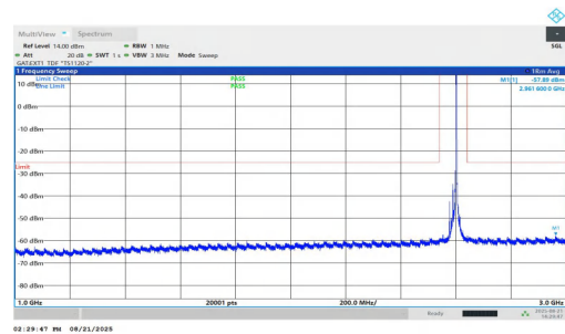
NTNV-n38-PC1.5-30-15-M-DFT-QPSK-Inner_1RB_Right-1000-3000-PASS
