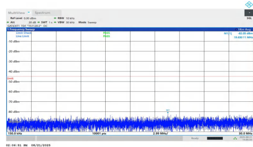
NTNV-n38-PC1.5-30-10-M-DFT-BPSK-Inner_1RB_Right-0.15-30- PASS
