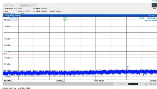
NTVN-n38-PC1.5-30-15-M-DFT-BPSK-Inner_1RB_Right-30-1000-PASS
