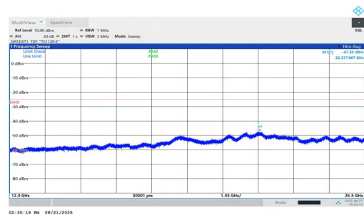
NTNV-n38-PC1.5-30-15-M-DFT-QPSK-Inner_1RB_Right-12000-26500-PASS
