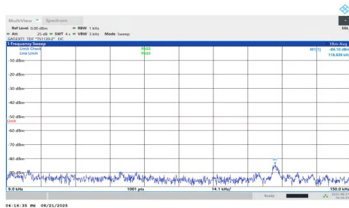
NTNV-n38-PC1.5-30-15-M-DFT-BPSK-Inner_1RB_Right-0.009-0. 15-PASS
