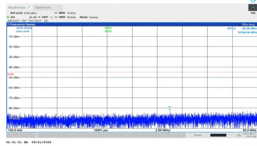
NTNV-n38-PC1.5-30-15-H-DFT-BPSK-Inner_1RB_Left-0.15-30-P ASS
