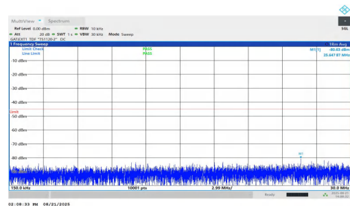
NTVN-n38-PC1.5-30-10-M-DFT-QPSK-Inner_1RB_Left-0.15-30-PASS
