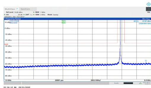
NTNV-n38-PC1.5-30-10-L-DFT-QPSK-Inner_1RB_Right-1000-3000-PASS
