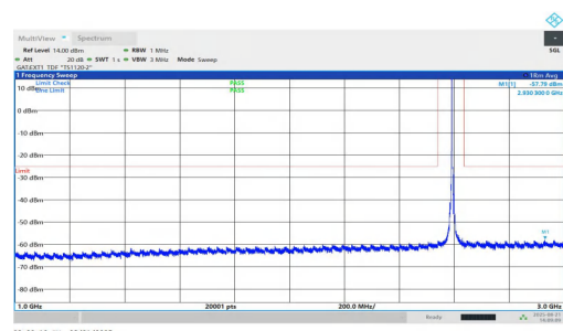
NTVN-n38-PC1.5-30-10-M-DFT-QPSK-Inner_1RB_Left-1000-3000-PASS
