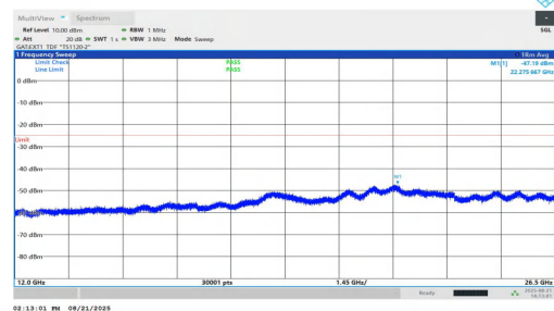
NTNV-n38-PC1.5-30-10-H-DFT-BPSK-Inner_1RB_Left-12000-26500-PASS
