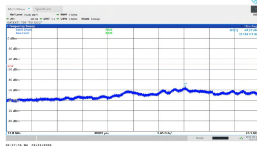
NTVN-n38-PC1.5-30-15-M-DFT-BPSK-Inner_1RB_Right-12000-26500-PASS
