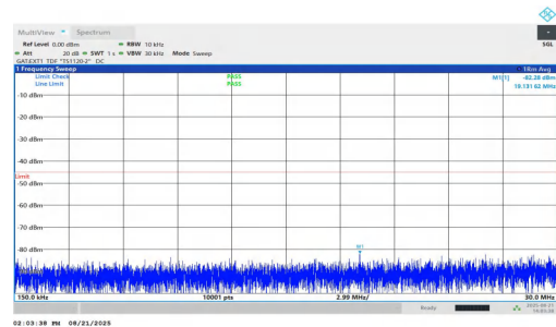
NTNV-n38-PC1.5-30-10-L-DFT-QPSK-Inner_1RB_Right-0.15-30-PASS
