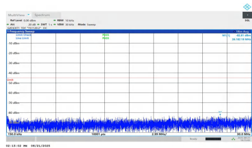
NTNV-n38-PC1.5-30-10-H-DFT-QPSK-Inner_1RB_Left-0.15-30-P ASS
