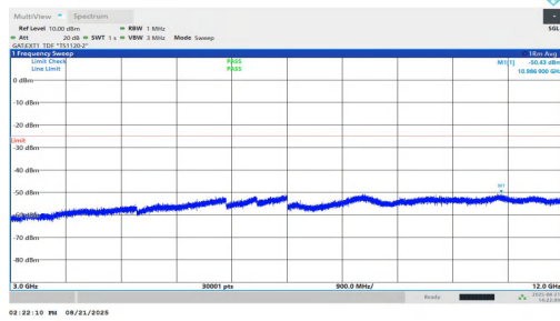
NTNV-n38-PC1.5-30-15-L-DFT-QPSK-Inner_1RB_Left-3000-12000-PASS
