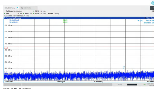
NTVN-n38-PC1.5-30-15-M-DFT-QPSK-Inner_1RB_Left-0.15-30-PASS
