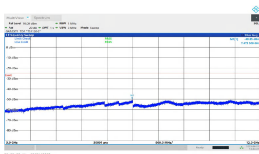
NTNV-n38-PC1.5-30-15-L-DFT-QPSK-Inner_1RB_Right-3000-12000-PASS
