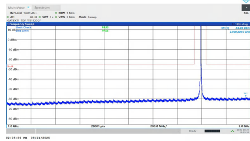
NTNV-n38-PC1.5-30-10-M-DFT-BPSK-Inner_1RB_Left-1000-3000 -PASS
