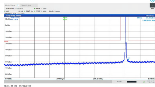
NTNV-n38-PC1.5-30-15-H-DFT-BPSK-Inner_1RB_Left-1000-3000 -PASS
