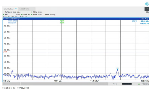
NTNV-n38-PC1.5-30-15-L-DFT-QPSK-Inner_1RB_Right-0.009-0.15-PASS
