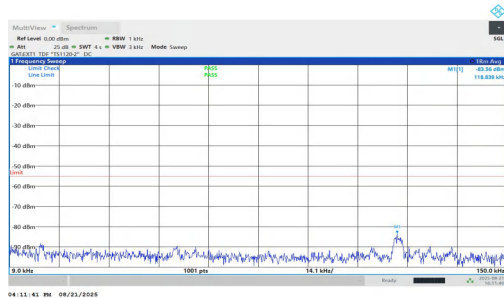
NTNV-n38-PC1.5-30-10-H-DFT-BPSK-Inner_1RB_Right-0.009-0.15-PASS
