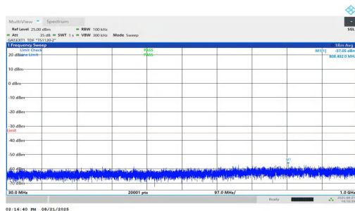
NTVN-n38-PC1.5-30-10-H-DFT-QPSK-Inner_1RB_Right-30-1000-PASS
