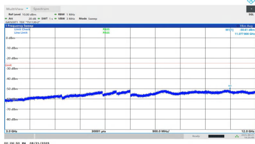
NTVN-n38-PC1.5-30-15-M-DFT-BPSK-Inner_1RB_Right-3000-12000-PASS
