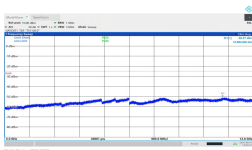
NTNV-n38-PC1.5-30-10-L-DFT-QPSK-Inner_1RB_Right-3000-12000-PASS
