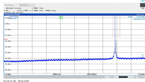
NTNV-n38-PC1.5-30-15-L-DFT-BPSK-Inner_1RB_Left-1000-3000 -PASS
