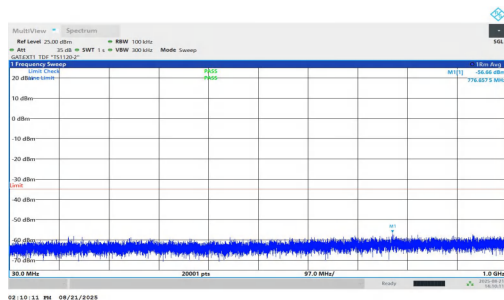
NTVN-n38-PC1.5-30-10-M-DFT-QPSK-Inner_1RB_Right-30-1000-PASS
