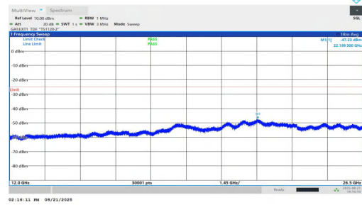
NTVN-n38-PC1.5-30-10-H-DFT-QPSK-Inner_1RB_Left-12000-26500-PASS
