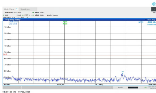
NTVN-n38-PC1.5-30-10-M-DFT-QPSK-Inner_1RB_Right-0.009-0.15-PASS
