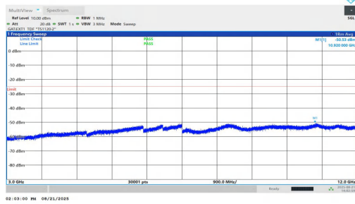
NTNV-n38-PC1.5-30-10-L-DFT-QPSK-Inner_1RB_Left-3000-12000-PASS
