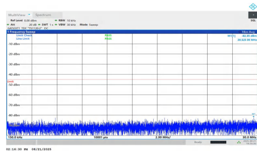
NTVN-n38-PC1.5-30-10-H-DFT-QPSK-Inner_1RB_Right-0.15-30-PASS
