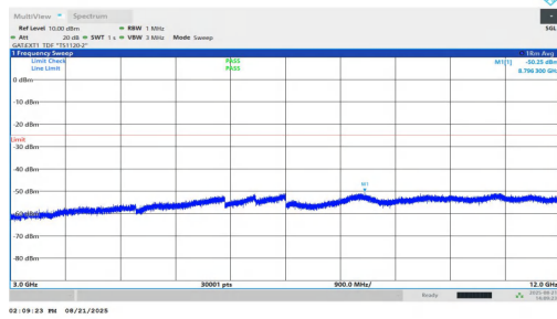
NTVN-n38-PC1.5-30-10-M-DFT-QPSK-Inner_1RB_Left-3000-12000-PASS
