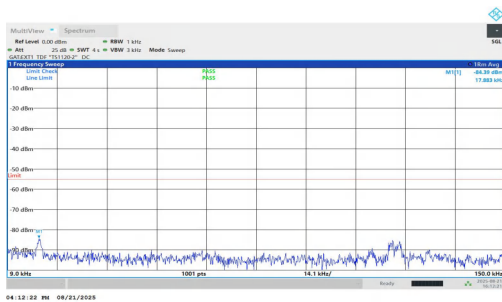
NTNV-n38-PC1.5-30-10-H-DFT-QPSK-Inner_1RB_Left-0.009-0.1 5-PASS
