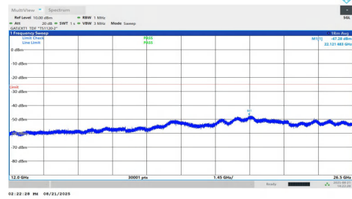
NTNV-n38-PC1.5-30-15-L-DFT-QPSK-Inner_1RB_Left-12000-26500-PASS
