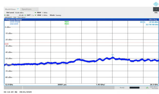
NTNV-n38-PC1.5-30-10-H-DFT-BPSK-Inner_1RB_Right-12000-26 500-PASS
