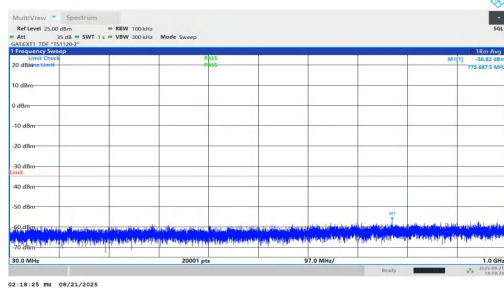
NTNV-n38-PC1.5-30-15-L-DFT-BPSK-Inner_1RB_Left-30-1000-P ASS
