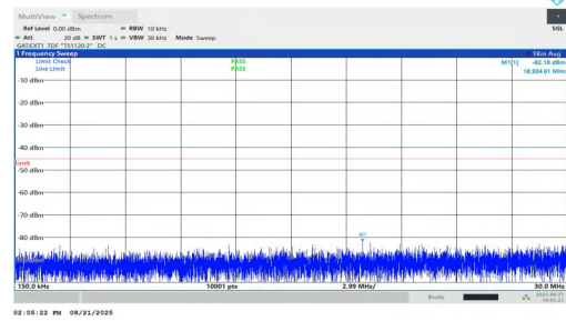
NTNV-n38-PC1.5-30-10-M-DFT-BPSK-Inner_1RB_Left-0.15-30-P ASS
