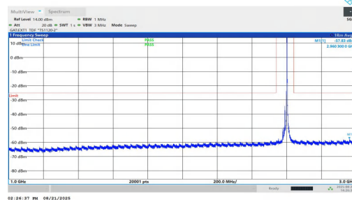
NTVN-n38-PC1.5-30-15-M-DFT-BPSK-Inner_1RB_Right-1000-3000-PASS
