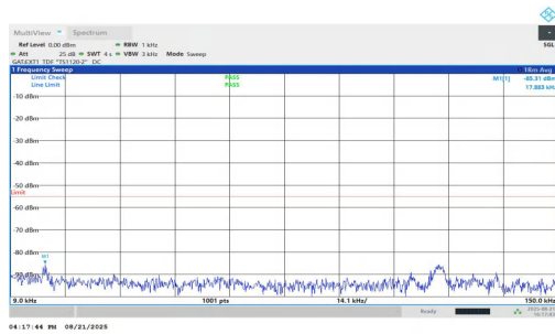
NTNV-n38-PC1.5-30-15-M-DFT-QPSK-Inner_1RB_Right-0.009-0.15-PASS
