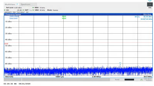
NTNV-n38-PC1.5-30-15-M-DFT-BPSK-Inner_1RB_Left-0.15-30-P ASS
