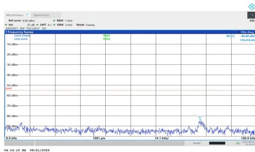
NTNV-n38-PC1.5-30-15-L-DFT-BPSK-Inner_1RB_Right-0.009-0. 15-PASS
