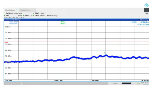
NTVN-n38-PC1.5-30-10-M-DFT-QPSK-Inner_1RB_Right-12000-26500-PASS
