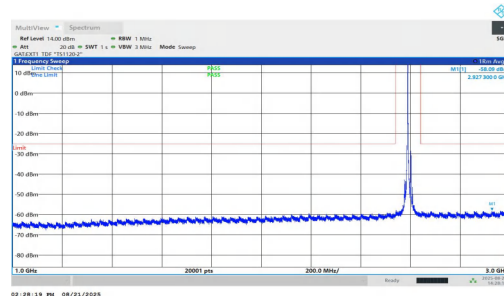
NTVN-n38-PC1.5-30-15-M-DFT-QPSK-Inner_1RB_Left-1000-3000-PASS
