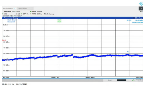
NTNV-n38-PC1.5-30-10-H-DFT-BPSK-Inner_1RB_Right-3000-12 000-PASS
