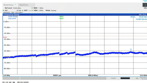
NTNV-n38-PC1.5-30-10-H-DFT-BPSK-Inner_1RB_Left-3000-12000-PASS
