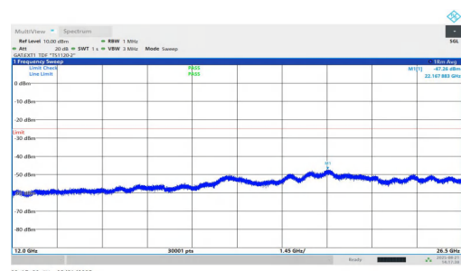
NTVN-n38-PC1.5-30-10-H-DFT-QPSK-Inner_1RB_Right-12000-26500-PASS
