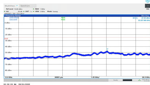
NTNV-n38-PC1.5-30-15-H-DFT-BPSK-Inner_1RB_Left-12000-265 00-PASS
