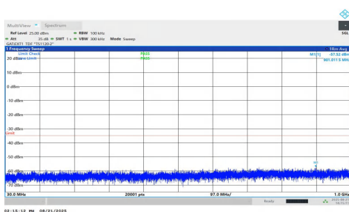
NTNV-n38-PC1.5-30-10-H-DFT-QPSK-Inner_1RB_Left-30-1000- PASS
