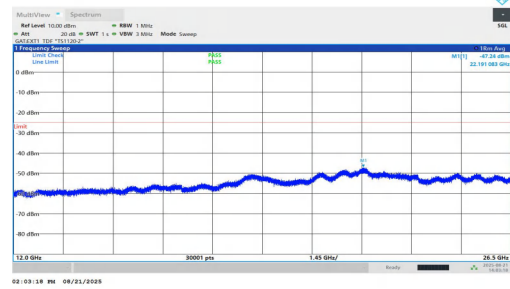
NTNV-n38-PC1.5-30-10-L-DFT-QPSK-Inner_1RB_Left-12000-26500-PASS
