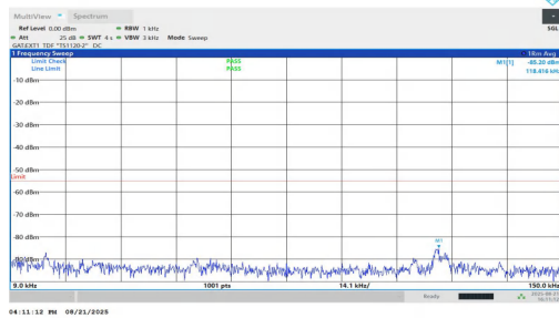
NTNV-n38-PC1.5-30-10-H-DFT-BPSK-Inner_1RB_Left-0.009-0.15-PASS
