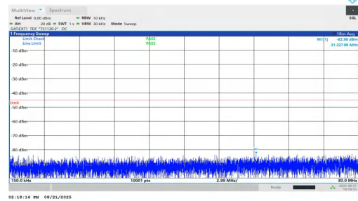
NTNV-n38-PC1.5-30-15-L-DFT-BPSK-Inner_1RB_Left-0.15-30-PA SS
