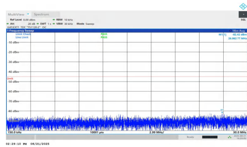
NTNV-n38-PC1.5-30-15-M-DFT-QPSK-Inner_1RB_Right-0.15-30-PASS
