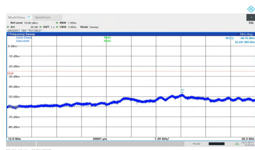
NTNV-n38-PC1.5-30-10-L-DFT-QPSK-Inner_1RB_Right-12000-26500-PASS
