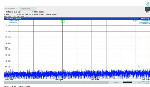
NTNV-n38-PC1.5-30-15-H-DFT-BPSK-Inner_1RB_Right-0.15-30- PASS
