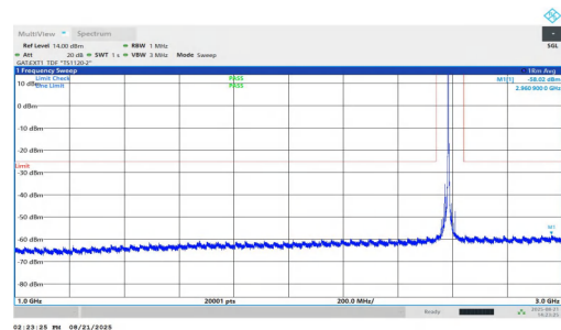
NTNV-n38-PC1.5-30-15-L-DFT-QPSK-Inner_1RB_Right-1000-3000-PASS
