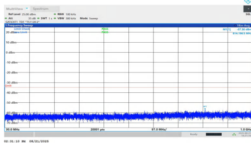
NTNV-n38-PC1.5-30-15-H-DFT-BPSK-Inner_1RB_Left-30-1000- PASS
