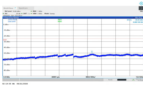
NTNV-n38-PC1.5-30-15-L-DFT-BPSK-Inner_1RB_Left-3000-120 00-PASS
