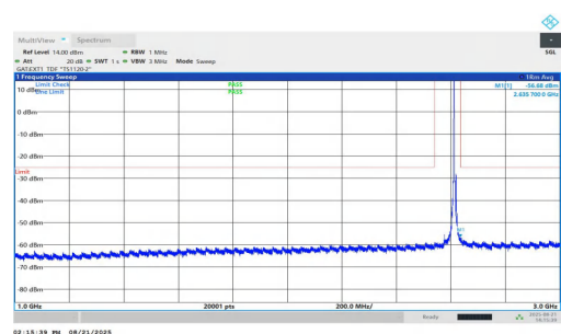
NTNV-n38-PC1.5-30-10-H-DFT-QPSK-Inner_1RB_Left-1000-3000 -PASS
