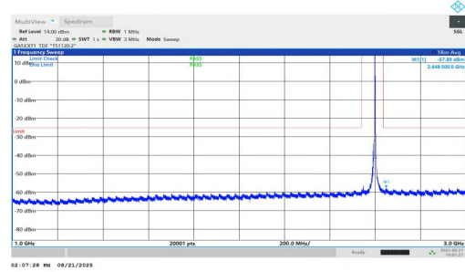
NTVN-n38-PC1.5-30-10-M-DFT-BPSK-Inner_1RB_Right-1000-3000-PASS
