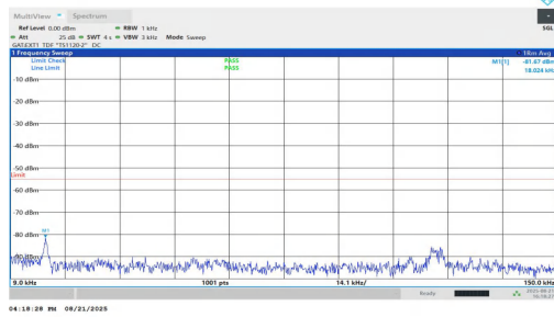
NTNV-n38-PC1.5-30-15-H-DFT-BPSK-Inner_1RB_Left-0.009-0.1 5-PASS
