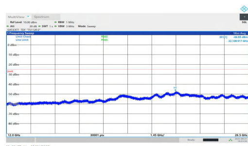
NTNV-n38-PC1.5-30-15-L-DFT-QPSK-Inner_1RB_Right-12000-26500-PASS
