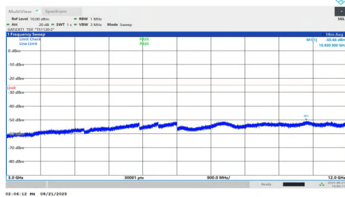
NTNV-n38-PC1.5-30-10-M-DFT-BPSK-Inner_1RB_Left-3000-120 00-PASS
