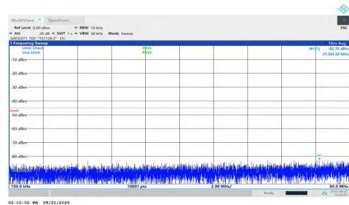
NTVN-n38-PC1.5-30-10-M-DFT-QPSK-Inner_1RB_Right-0.15-30-PASS
