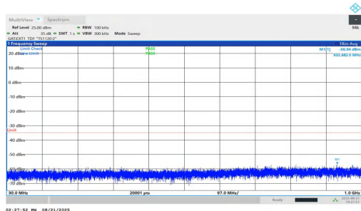
NTVN-n38-PC1.5-30-15-M-DFT-QPSK-Inner_1RB_Left-30-1000-PASS
