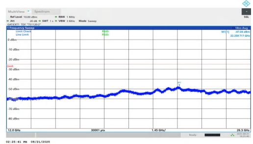
NTNV-n38-PC1.5-30-15-M-DFT-BPSK-Inner_1RB_Left-12000-265 00-PASS
