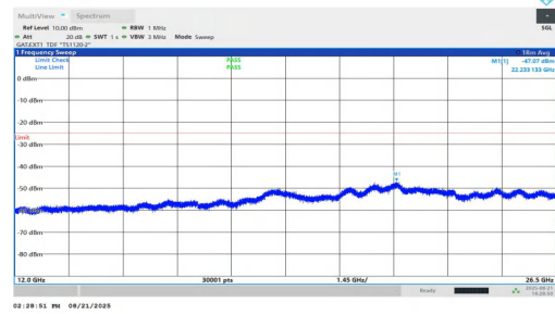
NTNV-n38-PC1.5-30-15-M-DFT-QPSK-Inner_1RB_Left-12000-26500-PASS
