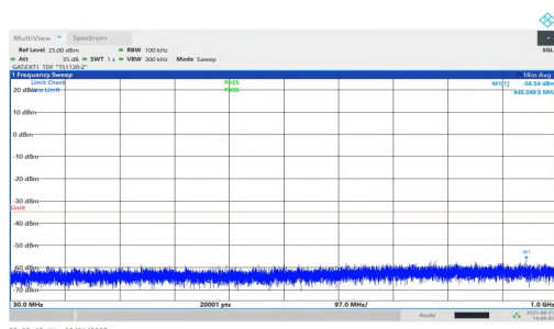
NTVN-n38-PC1.5-30-10-M-DFT-QPSK-Inner_1RB_Left-30-1000-PASS
