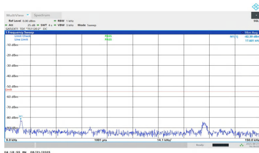
NTNV-n38-PC1.5-30-15-H-DFT-BPSK-Inner_1RB_Right-0.009-0. 15-PASS
