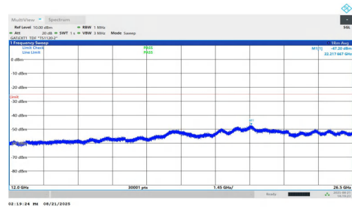
NTNV-n38-PC1.5-30-15-L-DFT-BPSK-Inner_1RB_Left-12000-265 00-PASS
