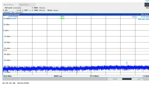
NTNV-n38-PC1.5-30-10-M-DFT-BPSK-Inner_1RB_Left-30-1000- PASS
