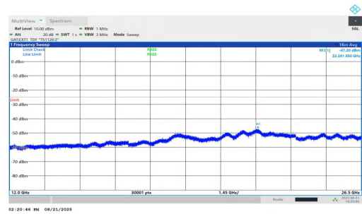
NTNV-n38-PC1.5-30-15-L-DFT-BPSK-Inner_1RB_Right-12000-26 500-PASS
