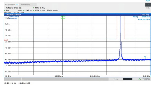
NTNV-n38-PC1.5-30-15-M-DFT-BPSK-Inner_1RB_Left-1000-3000 -PASS
