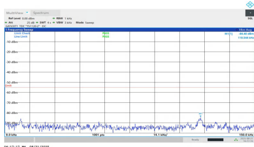
NTVN-n38-PC1.5-30-15-M-DFT-QPSK-Inner_1RB_Left-0.009-0.15-PASS
