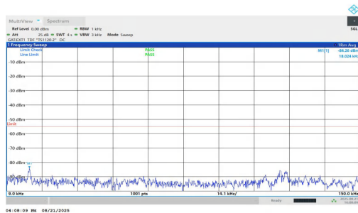
NTNV-n38-PC1.5-30-10-L-DFT-QPSK-Inner_1RB_Right-0.009-0.15-PASS
