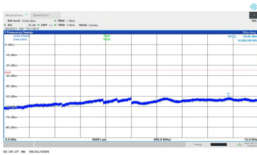
NTNV-n38-PC1.5-30-15-L-DFT-BPSK-Inner_1RB_Right-3000-12 000-PASS
