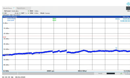
NTNV-n38-PC1.5-30-15-M-DFT-QPSK-Inner_1RB_Right-3000-12000-PASS
