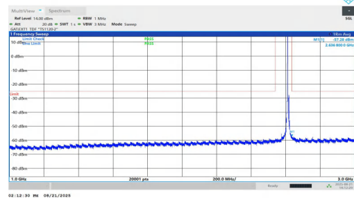
NTNV-n38-PC1.5-30-10-H-DFT-BPSK-Inner_1RB_Left-1000-3000-PASS
