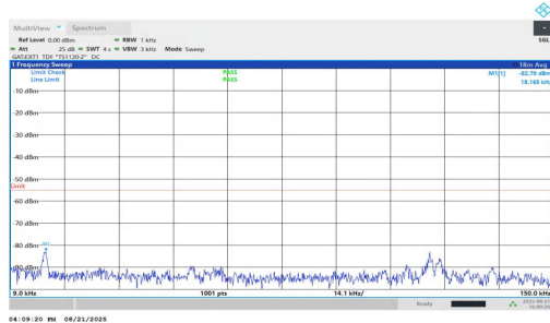
NTNV-n38-PC1.5-30-10-M-DFT-BPSK-Inner_1RB_Right-0.009-0. 15-PASS
