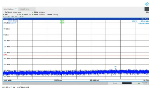
NTNV-n38-PC1.5-30-10-L-DFT-QPSK-Inner_1RB_Right-30-1000-PASS
