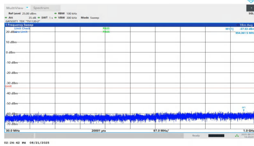
NTNV-n38-PC1.5-30-15-M-DFT-BPSK-Inner_1RB_Left-30-1000- PASS
