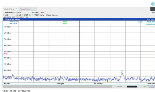
NTVN-n38-PC1.5-30-10-H-DFT-QPSK-Inner_1RB_Right-0.009-0.15-PASS
