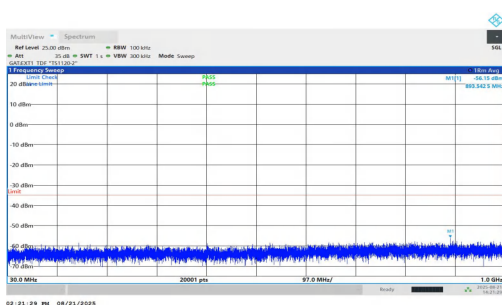
NTNV-n38-PC1.5-30-15-L-DFT-QPSK-Inner_1RB_Left-30-1000- PASS
