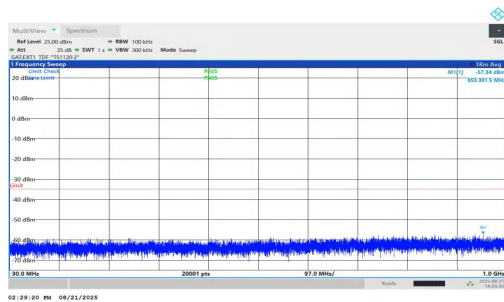
NTNV-n38-PC1.5-30-15-M-DFT-QPSK-Inner_1RB_Right-30-1000-PASS
