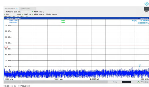
NTNV-n38-PC1.5-30-15-L-DFT-BPSK-Inner_1RB_Right-0.15-30-P ASS
