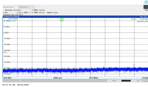
NTVN-n38-PC1.5-30-10-M-DFT-BPSK-Inner_1RB_Right-30-1000-PASS
