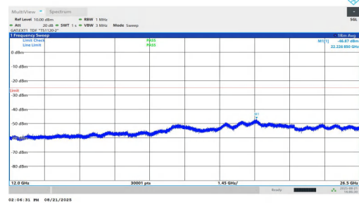
NTNV-n38-PC1.5-30-10-M-DFT-BPSK-Inner_1RB_Left-12000-265 00-PASS
