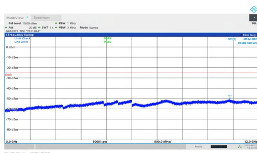
NTVN-n38-PC1.5-30-10-H-DFT-QPSK-Inner_1RB_Right-3000-12000-PASS
