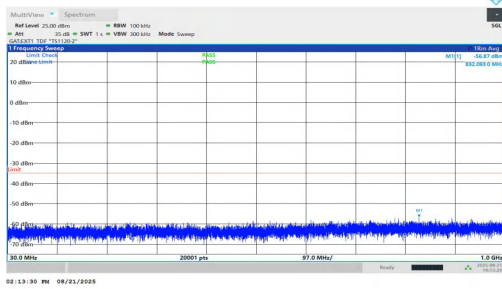
NTNV-n38-PC1.5-30-10-H-DFT-BPSK-Inner_1RB_Right-30-1000 -PASS
