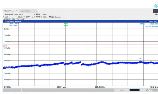
NTVN-n38-PC1.5-30-10-M-DFT-QPSK-Inner_1RB_Right-3000-12000-PASS
