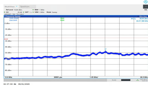
NTVN-n38-PC1.5-30-10-M-DFT-BPSK-Inner_1RB_Right-12000-26500-PASS
