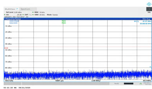
NTNV-n38-PC1.5-30-15-L-DFT-QPSK-Inner_1RB_Left-0.15-30-PA SS
