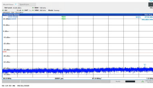
NTNV-n38-PC1.5-30-15-L-DFT-BPSK-Inner_1RB_Right-30-1000 -PASS
