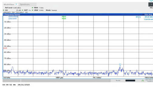
NTNV-n38-PC1.5-30-10-M-DFT-BPSK-Inner_1RB_Left-0.009-0.1 5-PASS
