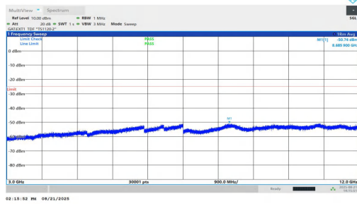
NTVN-n38-PC1.5-30-10-H-DFT-QPSK-Inner_1RB_Left-3000-12000-PASS
