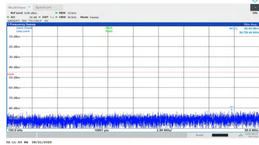
NTNV-n38-PC1.5-30-10-H-DFT-BPSK-Inner_1RB_Left-0.15-30-PASS
