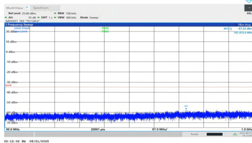
NTNV-n38-PC1.5-30-10-H-DFT-BPSK-Inner_1RB_Left-30-1000-PASS
