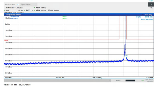
NTNV-n38-PC1.5-30-10-H-DFT-BPSK-Inner_1RB_Right-1000-300 0-PASS
