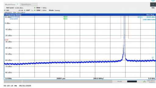
NTNV-n38-PC1.5-30-15-L-DFT-BPSK-Inner_1RB_Right-1000-300 0-PASS
