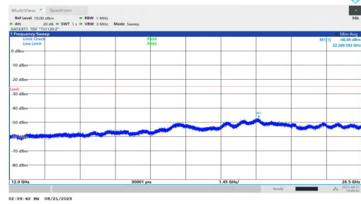
NTVN-n38-PC1.5-30-10-M-DFT-QPSK-Inner_1RB_Left-12000-26500-PASS
