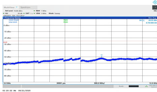
NTNV-n38-PC1.5-30-15-M-DFT-BPSK-Inner_1RB_Left-3000-120 00-PASS
