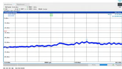
NTNV-n38-PC2-30-20-L-DFT-QPSK-Inner_1RB_Right-12000-265 00-PASS
