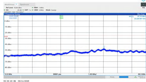
NTNV-n38-PC2-30-25-L-DFT-BPSK-Inner_1RB_Right-12000-265 00-PASS
