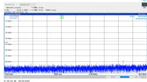
NTNV-n38-PC2-30-15-M-DFT-QPSK-Inner_1RB_Right-0.15-30-P ASS
