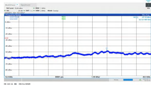
NTNV-n38-PC2-30-25-H-DFT-BPSK-Inner_1RB_Left-12000-26500-PASS
