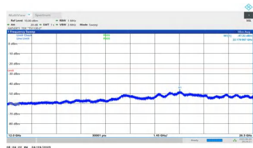
NTNV-n38-PC2-30-30-L-DFT-BPSK-Inner_1RB_Left-12000-26500-PASS
