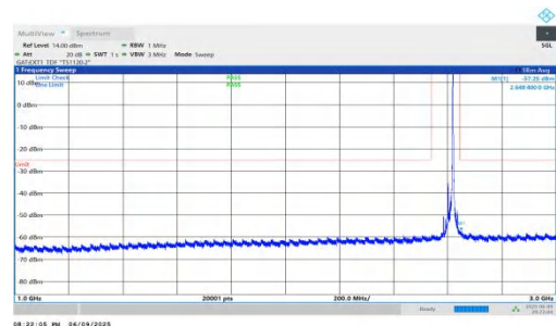
NTNV-n38-PC2-30-20-H-DFT-QPSK-Inner_1RB_Right-1000-3000 -PASS
