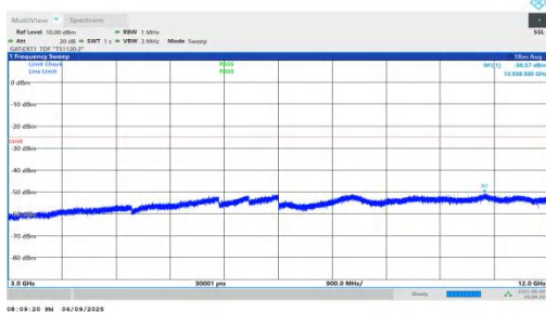
NTNV-n38-PC2-30-20-L-DFT-QPSK-Inner_1RB_Right-3000-120 00-PASS
