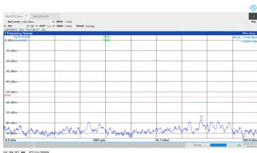
NTNV-n38-PC2-30-15-M-DFT-BPSK-Inner_1RB_Right-0.009-0.15-PASS
