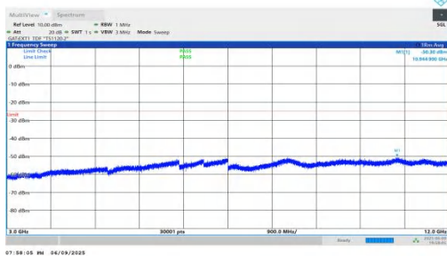
NTNV-n38-PC2-30-15-H-DFT-BPSK-Inner_1RB_Left-3000-12000-PASS
