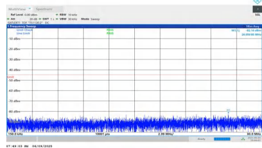
NTNV-n38-PC2-30-15-L-DFT-QPSK-Inner_1RB_Right-0.15-30-PA SS
