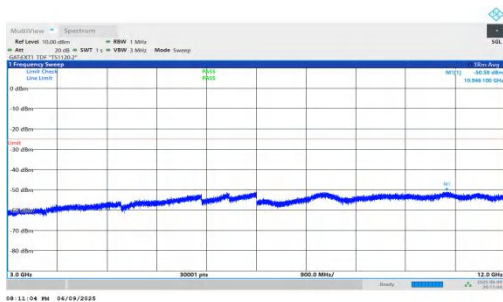
NTNV-n38-PC2-30-20-M-DFT-BPSK-Inner_1RB_Left-3000-12000-PASS
