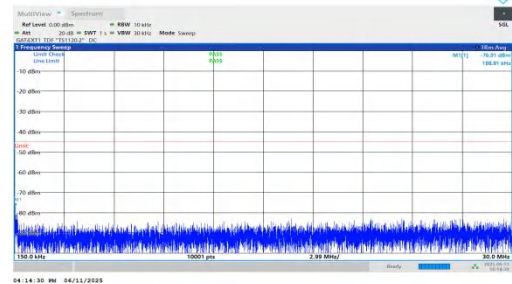
NTNV-n38-PC2-30-25-H-DFT-BPSK-Inner_1RB_Right-0.15-30-PASS
