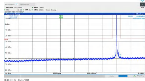
NTNV-n38-PC2-30-25-H-DFT-BPSK-Inner_1RB_Left-1000-3000-PASS
