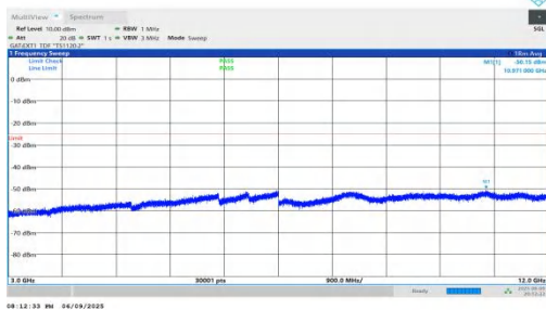
NTNV-n38-PC2-30-20-M-DFT-BPSK-Inner_1RB_Right-3000-12000-PASS
