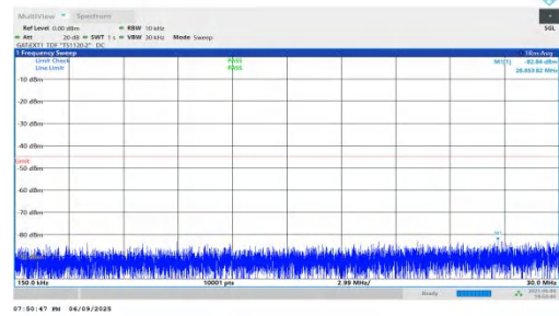
NTNV-n38-PC2-30-15-M-DFT-BPSK-Inner_1RB_Left-0.15-30-PASS
