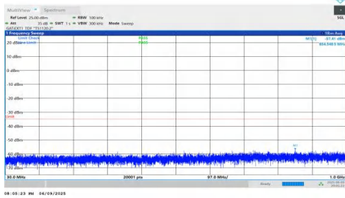
NTNV-n38-PC2-30-20-L-DFT-BPSK-Inner_1RB_Right-30-1000-P ASS
