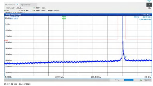
NTNV-n38-PC2-30-15-H-DFT-BPSK-Inner_1RB_Left-1000-3000-PASS
