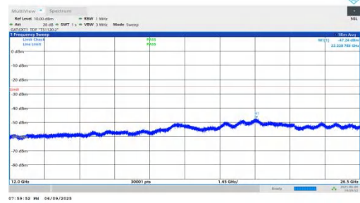
NTNV-n38-PC2-30-15-H-DFT-BPSK-Inner_1RB_Right-12000-26500-PASS
