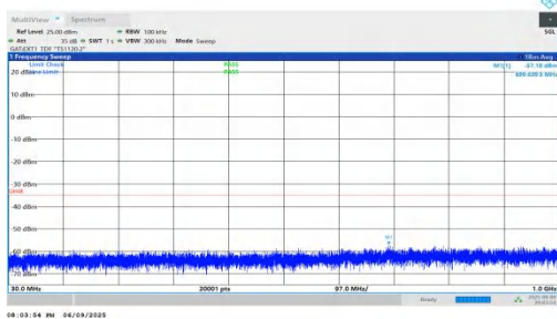
NTNV-n38-PC2-30-20-L-DFT-BPSK-Inner_1RB_Left-30-1000-PASS SS
