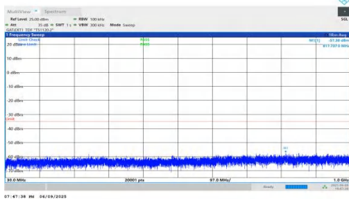
NTNV-n38-PC2-30-15-L-DFT-QPSK-Inner_1RB_Left-30-1000-PA SS
