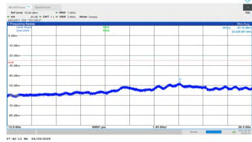
NTNV-n38-PC2-30-10-H-DFT-QPSK-Inner_1RB_Left-12000-2650 0-PASS
