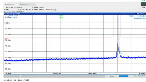
NTNV-n38-PC2-30-20-H-DFT-BPSK-Inner_1RB_Right-1000-3000-P PASS
