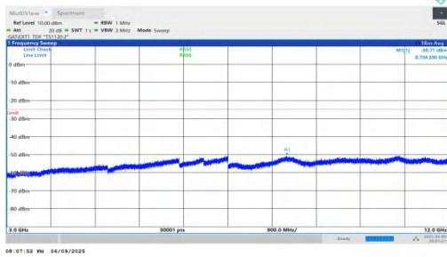
NTNV-n38-PC2-30-20-L-DFT-QPSK-Inner_1RB_Left-3000-12000 -PASS
