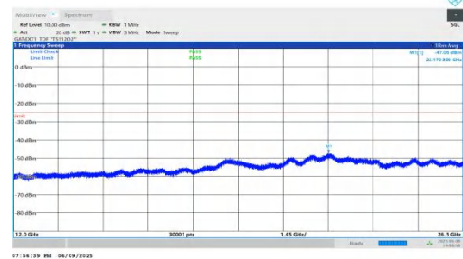
NTNV-n38-PC2-30-15-M-DFT-QPSK-Inner_1RB_Right-12000-26500- 00-PASS
