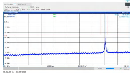
NTNV-n38-PC2-30-15-H-DFT-QPSK-Inner_1RB_Left-1000-3000-PASS
