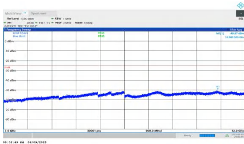
NTNV-n38-PC2-30-15-H-DFT-QPSK-Inner_1RB_Right-3000-12000-PASS
