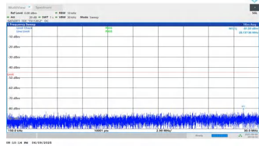
NTNV-n38-PC2-30-20-M-DFT-BPSK-Inner_1RB_Left-0.15-30-PASS
