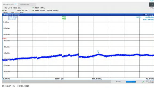
NTNV-n38-PC2-30-15-M-DFT-QPSK-Inner_1RB_Left-3000-1200 0-PASS
