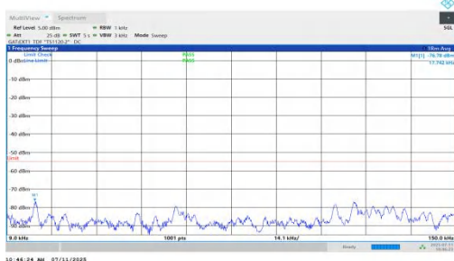
NTNV-n38-PC2-30-20-L-DFT-QPSK-Inner_1RB_Left-0.009-0.15- PASS
