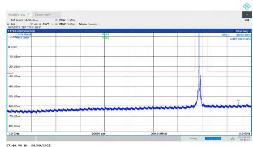
NTNV-n38-PC2-30-15-L-DFT-BPSK-Inner_1RB_Left-1000-3000-P ASS
