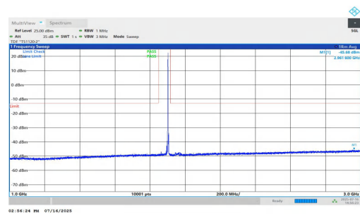
NTNV-n25-PC2-15-40-M-DFT-QPSK-Inner_1RB_Right-1000-3000 -PASS
