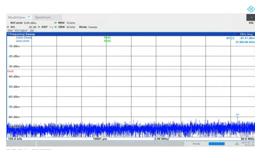
NTNV-n25-PC2-15-40-H-DFT-BPSK-Inner_1RB_Right-0.15-30-PASS
