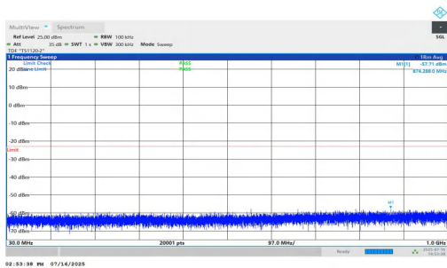
NTNV-n25-PC2-15-40-L-DFT-QPSK-Inner_1RB_Right-30-1000-PASS
