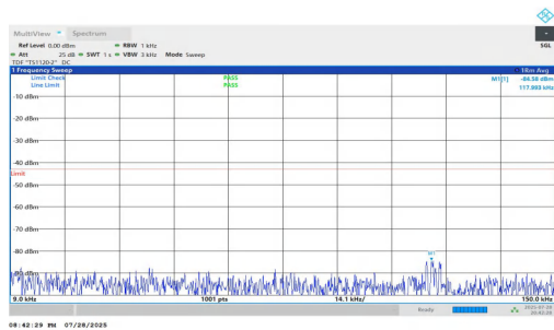
NTNV-n25-PC2-15-40-M-DFT-QPSK-Inner_1RB_Left-0.009-0.15-PASS
