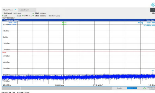
NTNV-n25-PC2-15-40-H-DFT-QPSK-Inner_1RB_Left-30-1000-PASS
