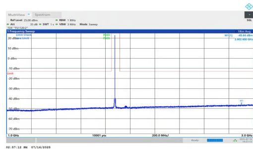
NTNV-n25-PC2-15-40-H-DFT-BPSK-Inner_1RB_Left-1000-3000-PASS
