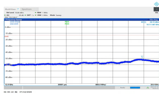
NTNV-n25-PC2-15-40-M-DFT-BPSK-Inner_1RB_Right-12000-20000-PASS
