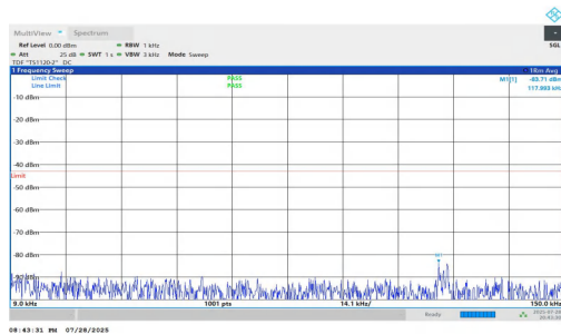
NTNV-n25-PC2-15-40-H-DFT-QPSK-Inner_1RB_Right-0.009-0.1 5-PASS
