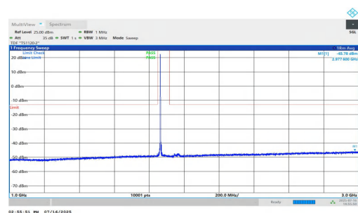
NTNV-n25-PC2-15-40-M-DFT-QPSK-Inner_1RB_Left-1000-3000-PASS
