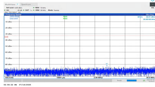
NTNV-n25-PC2-15-40-M-DFT-BPSK-Inner_1RB_Left-0.15-30-PASS
