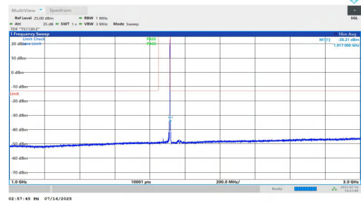
NTNV-n25-PC2-15-40-H-DFT-BPSK-Inner_1RB_Right-1000-3000-PASS
