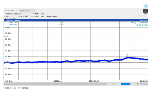
NTNV-n25-PC2-15-40-M-DFT-QPSK-Inner_1RB_Right-12000-200 00-PASS
