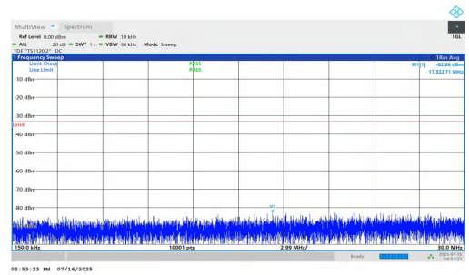
NTNV-n25-PC2-15-40-L-DFT-QPSK-Inner_1RB_Right-0.15-30-PASS
