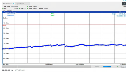
NTNV-n25-PC2-15-40-H-DFT-QPSK-Inner_1RB_Left-3000-1200 0-PASS
