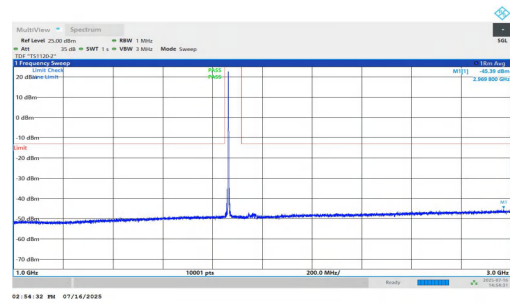
NTNV-n25-PC2-15-40-M-DFT-BPSK-Inner_1RB_Left-1000-3000-PASS
