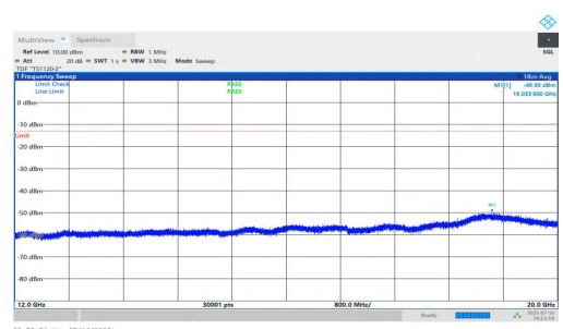
NTNV-n25-PC2-15-40-L-DFT-QPSK-Inner_1RB_Right-12000-20000-PASS
