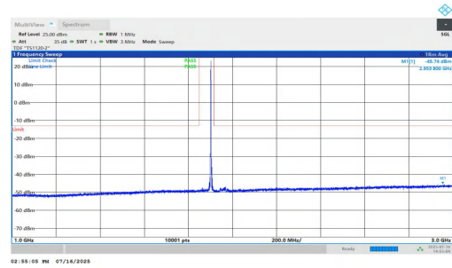
NTNV-n25-PC2-15-40-M-DFT-BPSK-Inner_1RB_Right-1000-3000-PASS
