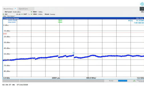
NTNV-n25-PC2-15-40-M-DFT-BPSK-Inner_1RB_Left-3000-12000-PASS
