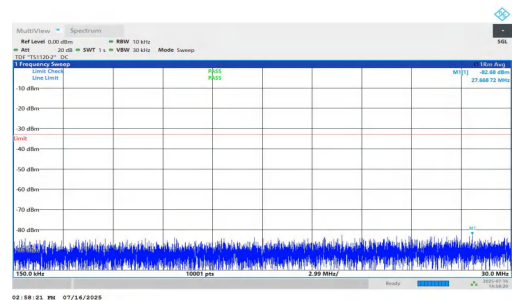
NTNV-n25-PC2-15-40-H-DFT-QPSK-Inner_1RB_Left-0.15-30-PASS
