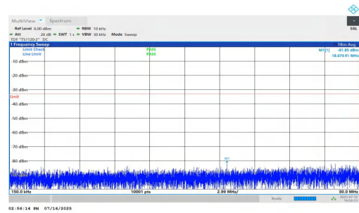
NTNV-n25-PC2-15-40-M-DFT-QPSK-Inner_1RB_Right-0.15-30-P ASS
