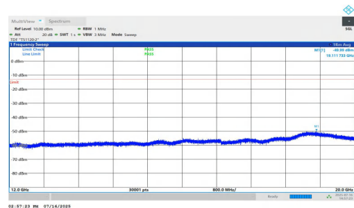
NTNV-n25-PC2-15-40-H-DFT-BPSK-Inner_1RB_Left-12000-20000-PASS
