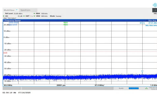
NTNV-n25-PC2-15-40-M-DFT-QPSK-Inner_1RB_Right-30-1000- PASS
