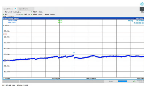
NTNV-n25-PC2-15-40-H-DFT-BPSK-Inner_1RB_Left-3000-12000-PASS
