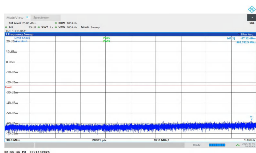
NTNV-n25-PC2-15-40-M-DFT-QPSK-Inner_1RB_Left-30-1000-PASS
