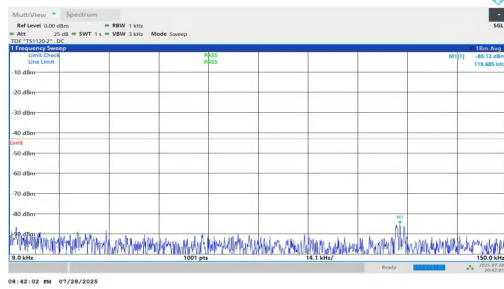
NTNV-n25-PC2-15-40-M-DFT-BPSK-Inner_1RB_Left-0.009-0.15-PASS
