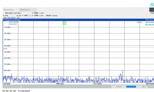
NTNV-n25-PC2-15-40-M-DFT-BPSK-Inner_1RB_Right-0.009-0.15-PASS
