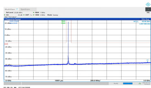
NTNV-n25-PC2-15-40-H-DFT-QPSK-Inner_1RB_Left-1000-3000-PASS
