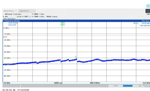
NTNV-n25-PC2-15-40-M-DFT-QPSK-Inner_1RB_Right-3000-120 00-PASS
