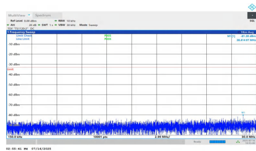
NTNV-n25-PC2-15-40-M-DFT-QPSK-Inner_1RB_Left-0.15-30-PASS
