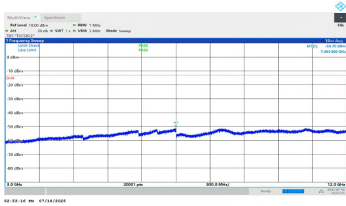
NTNV-n25-PC2-15-40-L-DFT-QPSK-Inner_1RB_Left-3000-12000 -PASS
