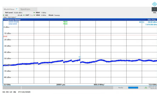
NTNV-n25-PC2-15-40-M-DFT-BPSK-Inner_1RB_Right-3000-12000-PASS
