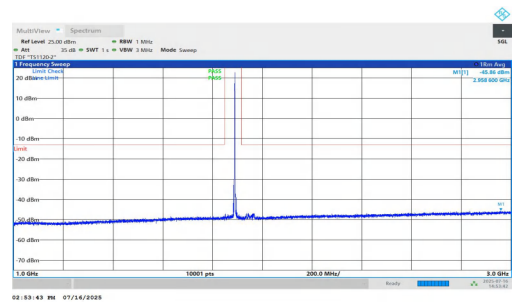
NTNV-n25-PC2-15-40-L-DFT-QPSK-Inner_1RB_Right-1000-3000-PASS
