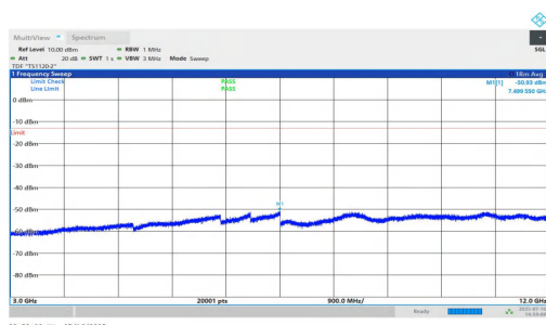
NTNV-n25-PC2-15-40-H-DFT-QPSK-Inner_1RB_Right-3000-12000- 00-PASS
