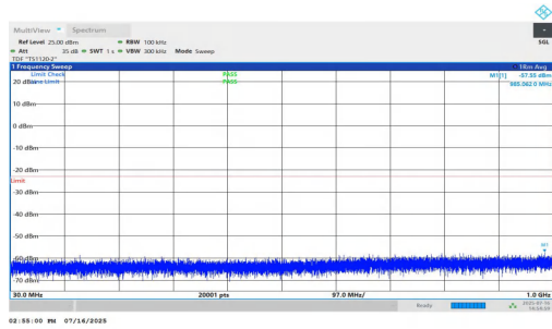
NTNV-n25-PC2-15-40-M-DFT-BPSK-Inner_1RB_Right-30-1000-PASS
