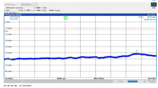
NTNV-n25-PC2-15-40-H-DFT-QPSK-Inner_1RB_Left-12000-2000 0-PASS
