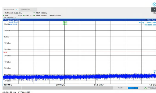
NTNV-n25-PC2-15-40-H-DFT-QPSK-Inner_1RB_Right-30-1000- PASS
