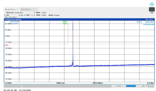
NTNV-n25-PC2-15-40-H-DFT-QPSK-Inner_1RB_Right-1000-3000- -PASS
