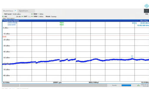
NTNV-n25-PC2-15-40-L-DFT-QPSK-Inner_1RB_Right-3000-12000-PASS
