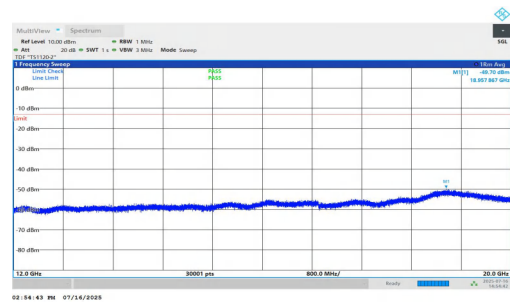
NTNV-n25-PC2-15-40-M-DFT-BPSK-Inner_1RB_Left-12000-20000-PASS
