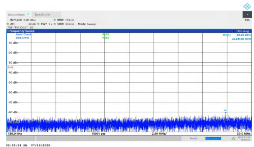
NTNV-n25-PC2-15-40-H-DFT-QPSK-Inner_1RB_Right-0.15-30-PA SS
