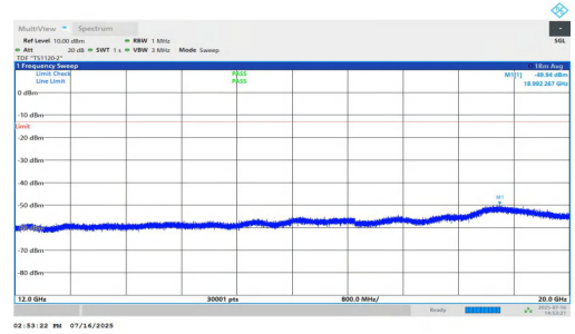
NTNV-n25-PC2-15-40-L-DFT-QPSK-Inner_1RB_Left-12000-20000 0-PASS
