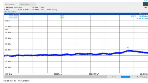
NTNV-n25-PC2-15-40-M-DFT-QPSK-Inner_1RB_Left-12000-2000 0-PASS
