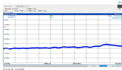
NTNV-n25-PC2-15-40-H-DFT-BPSK-Inner_1RB_Right-12000-20000-PASS
