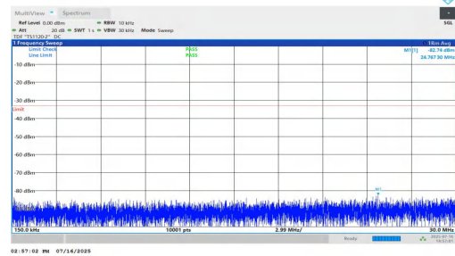
NTNV-n25-PC2-15-40-H-DFT-BPSK-Inner_1RB_Left-0.15-30-PAS
