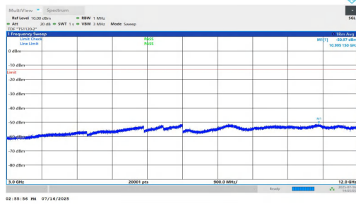
NTNV-n25-PC2-15-40-M-DFT-QPSK-Inner_1RB_Left-3000-1200 0-PASS
