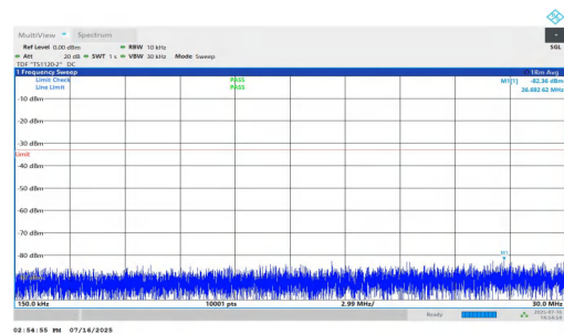
NTNV-n25-PC2-15-40-M-DFT-BPSK-Inner_1RB_Right-0.15-30-PASS
