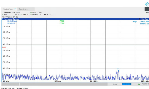
NTNV-n25-PC2-15-40-H-DFT-QPSK-Inner_1RB_Left-0.009-0.15-PASS
