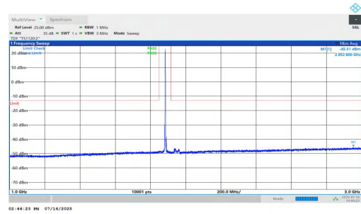
NTNV-n25-PC2-15-35-L-DFT-BPSK-Inner_1RB_Right-1000-3000-P PASS
