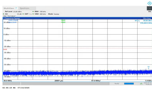
NTNV-n25-PC2-15-35-L-DFT-BPSK-Inner_1RB_Right-30-1000-P ASS
