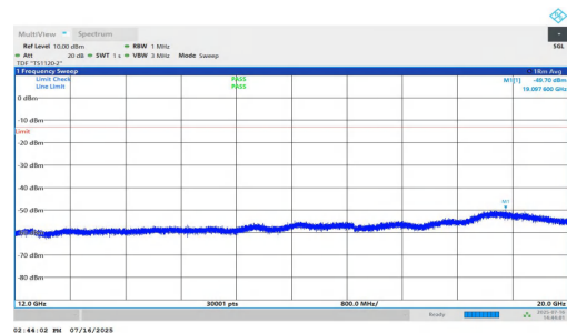
NTNV-n25-PC2-15-35-L-DFT-BPSK-Inner_1RB_Left-12000-20000-PASS
