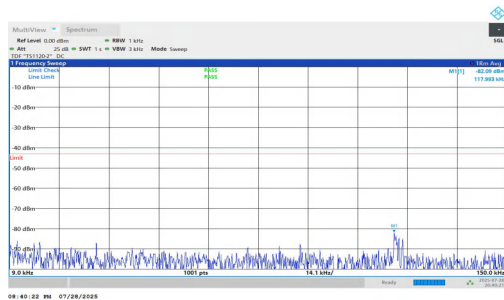
NTNV-n25-PC2-15-35-H-DFT-QPSK-Inner_1RB_Right-0.009-0.1 5-PASS
