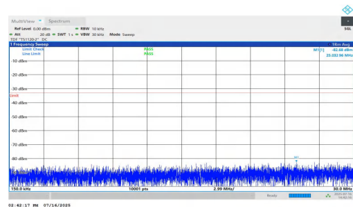
NTNV-n25-PC2-15-30-H-DFT-QPSK-Inner_1RB_Left-0.15-30-PAS S
