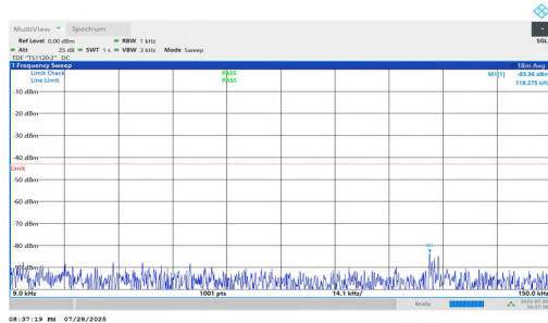
NTNV-n25-PC2-15-30-H-DFT-QPSK-Inner_1RB_Right-0.009-0.1 5-PASS
