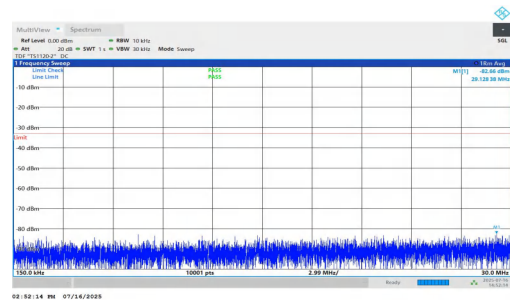
NTNV-n25-PC2-15-40-L-DFT-BPSK-Inner_1RB_Right-0.15-30-PASS SS
