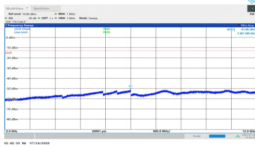
NTNV-n25-PC2-15-30-H-DFT-QPSK-Inner_1RB_Left-3000-1200 0-PASS
