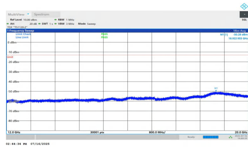
NTNV-n25-PC2-15-35-L-DFT-BPSK-Inner_1RB_Right-12000-200 00-PASS
