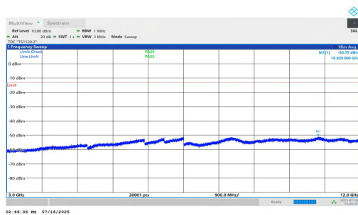
NTNV-n25-PC2-15-35-M-DFT-BPSK-Inner_1RB_Left-3000-12000-PASS
