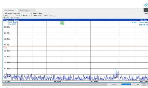
NTNV-n25-PC2-15-35-L-DFT-BPSK-Inner_1RB_Right-0.009-0.15-PASS
