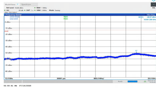
NTNV-n25-PC2-15-35-H-DFT-QPSK-Inner_1RB_Left-12000-2000 0-PASS
