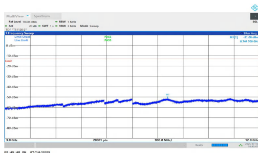
NTNV-n25-PC2-15-35-L-DFT-QPSK-Inner_1RB_Right-3000-12000-PASS 00-PASS
