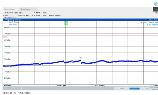
NTNV-n25-PC2-15-40-L-DFT-BPSK-Inner_1RB_Right-3000-1200 0-PASS
