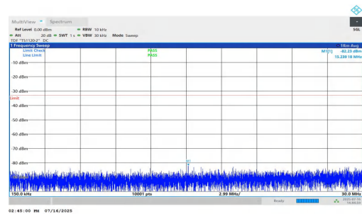
NTNV-n25-PC2-15-35-L-DFT-QPSK-Inner_1RB_Left-0.15-30-PAS S
