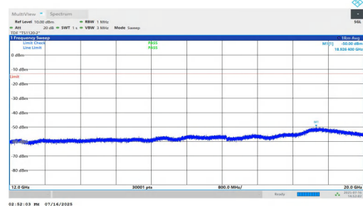
NTNV-n25-PC2-15-40-L-DFT-BPSK-Inner_1RB_Left-12000-20000 -PASS
