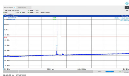
NTNV-n25-PC2-15-35-L-DFT-BPSK-Inner_1RB_Left-1000-3000-PASS
