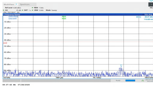
NTNV-n25-PC2-15-35-L-DFT-BPSK-Inner_1RB_Left-0.009-0.15-PASS
