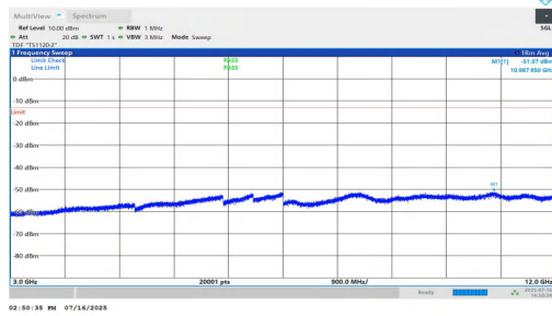
NTNV-n25-PC2-15-35-H-DFT-QPSK-Inner_1RB_Left-3000-1200 0-PASS
