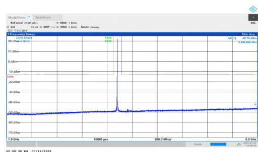
NTNV-n25-PC2-15-35-H-DFT-QPSK-Inner_1RB_Left-1000-3000- PASS
