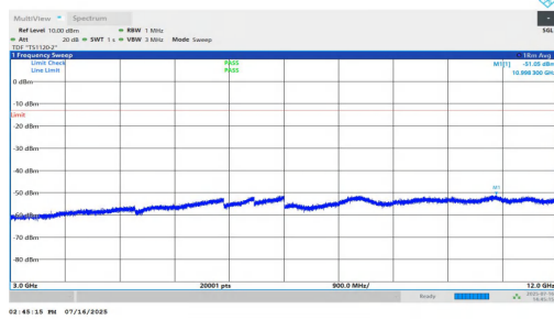
NTNV-n25-PC2-15-35-L-DFT-QPSK-Inner_1RB_Left-3000-12000 -PASS
