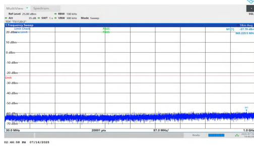
NTNV-n25-PC2-15-35-M-DFT-BPSK-Inner_1RB_Right-30-1000-PASS
