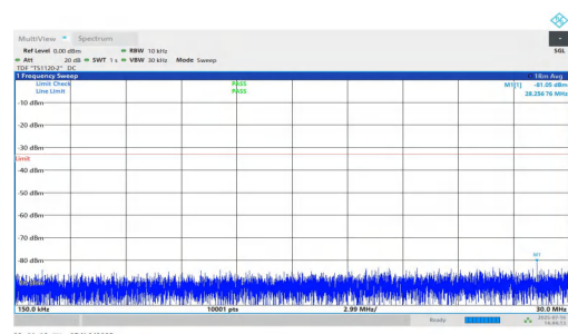
NTNV-n25-PC2-15-35-L-DFT-BPSK-Inner_1RB_Right-0.15-30-PASS
