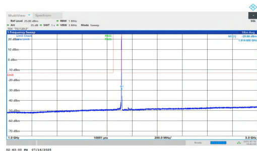
NTNV-n25-PC2-15-30-H-DFT-QPSK-Inner_1RB_Right-1000-3000- -PASS
