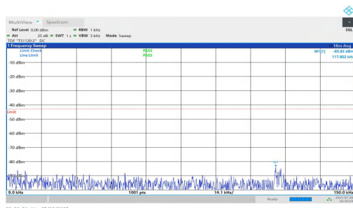
NTNV-n25-PC2-15-35-H-DFT-BPSK-Inner_1RB_Right-0.009-0.15-PASS
