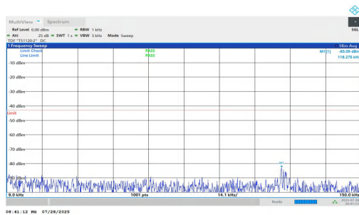
NTNV-n25-PC2-15-40-L-DFT-QPSK-Inner_1RB_Left-0.009-0.15- PASS
