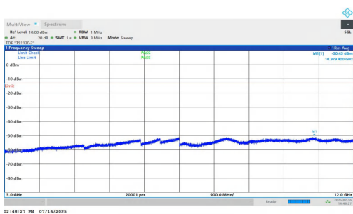
NTNV-n25-PC2-15-35-M-DFT-QPSK-Inner_1RB_Right-3000-120 00-PASS
