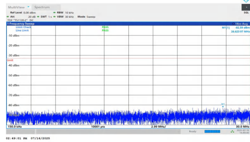
NTNV-n25-PC2-15-35-H-DFT-BPSK-Inner_1RB_Left-0.15-30-PASS
