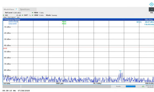
NTNV-n25-PC2-15-35-L-DFT-QPSK-Inner_1RB_Left-0.009-0.15- PASS
