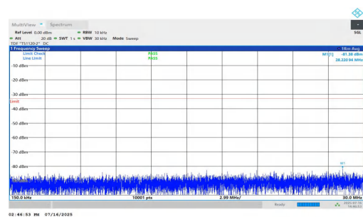
NTNV-n25-PC2-15-35-M-DFT-BPSK-Inner_1RB_Right-0.15-30-PASS
