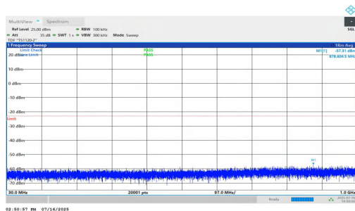
NTNV-n25-PC2-15-35-H-DFT-QPSK-Inner_1RB_Right-30-1000-PASS
