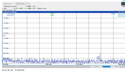
NTNV-n25-PC2-15-35-H-DFT-BPSK-Inner_1RB_Left-0.009-0.15-PASS
