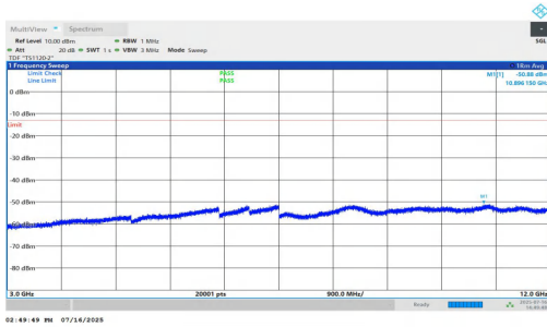
NTNV-n25-PC2-15-35-H-DFT-BPSK-Inner_1RB_Right-3000-120 00-PASS
