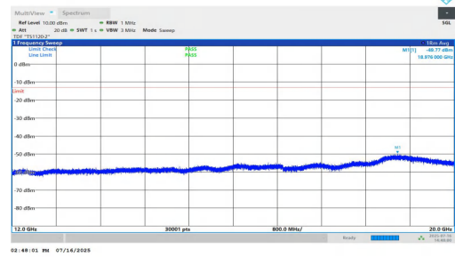
NTNV-n25-PC2-15-35-M-DFT-QPSK-Inner_1RB_Left-12000-2000 0-PASS
