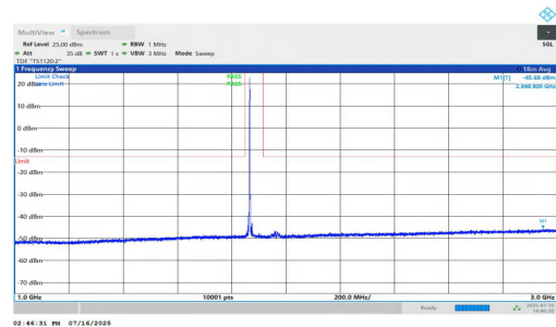
NTNV-n25-PC2-15-35-M-DFT-BPSK-Inner_1RB_Left-1000-3000-PASS
