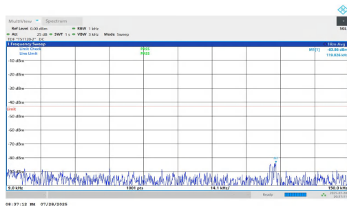
NTNV-n25-PC2-15-30-H-DFT-QPSK-Inner_1RB_Left-0.009-0.15- PASS
