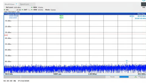
NTNV-n25-PC2-15-35-L-DFT-BPSK-Inner_1RB_Left-0.15-30-PASS
