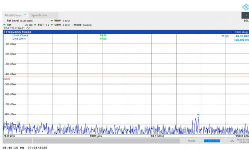
NTNV-n25-PC2-15-35-H-DFT-QPSK-Inner_1RB_Left-0.009-0.15- PASS
