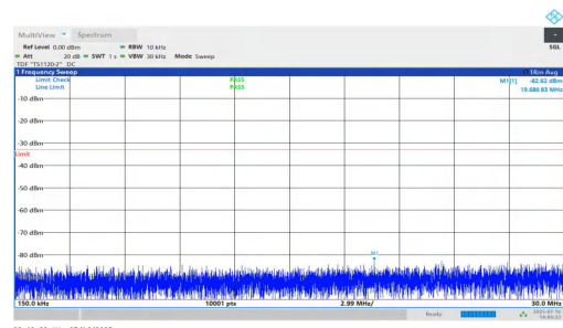
NTNV-n25-PC2-15-35-H-DFT-BPSK-Inner_1RB_Right-0.15-30-PASS
