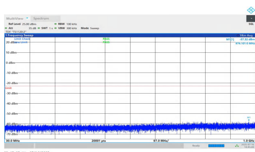
NTNV-n25-PC2-15-35-L-DFT-QPSK-Inner_1RB_Left-30-1000-PA SS
