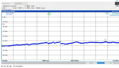
NTNV-n25-PC2-15-35-M-DFT-QPSK-Inner_1RB_Left-3000-1200 0-PASS
