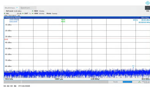
NTNV-n25-PC2-15-30-H-DFT-QPSK-Inner_1RB_Right-0.15-30-PA SS
