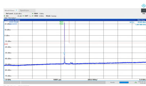
NTNV-n25-PC2-15-35-L-DFT-QPSK-Inner_1RB_Left-1000-3000-P ASS
