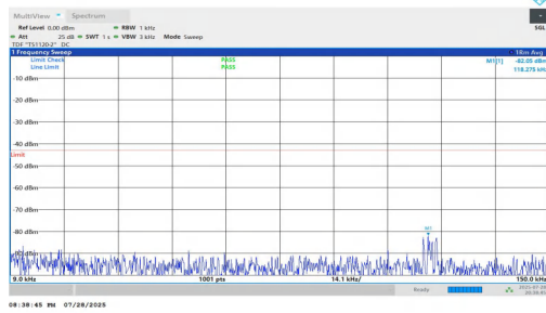
NTNV-n25-PC2-15-35-M-DFT-BPSK-Inner_1RB_Left-0.009-0.15-PASS
