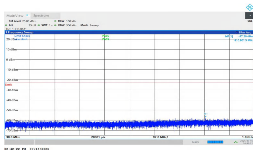
NTNV-n25-PC2-15-30-H-DFT-QPSK-Inner_1RB_Left-30-1000-P ASS
