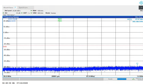
NTNV-n25-PC2-15-35-H-DFT-BPSK-Inner_1RB_Left-30-1000-PASS
