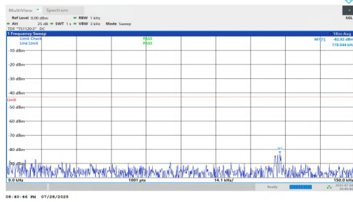
NTNV-n25-PC2-15-40-L-DFT-BPSK-Inner_1RB_Left-0.009-0.15- PASS
