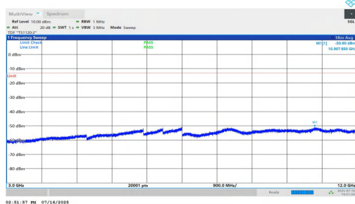
NTNV-n25-PC2-15-40-L-DFT-BPSK-Inner_1RB_Left-3000-12000 -PASS
