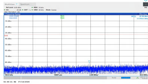
NTNV-n25-PC2-15-35-M-DFT-BPSK-Inner_1RB_Left-0.15-30-PASS
