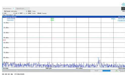
NTNV-n25-PC2-15-35-M-DFT-BPSK-Inner_1RB_Right-0.009-0.15-PASS
