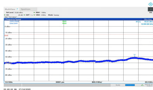
NTNV-n25-PC2-15-35-H-DFT-BPSK-Inner_1RB_Left-12000-20000-PASS
