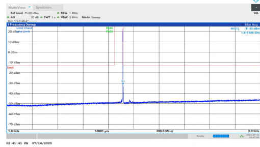
NTNV-n25-PC2-15-30-H-DFT-BPSK-Inner_1RB_Right-1000-3000-P PASS
