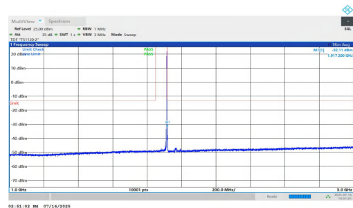
NTNV-n25-PC2-15-35-H-DFT-QPSK-Inner_1RB_Right-1000-3000-PASS
