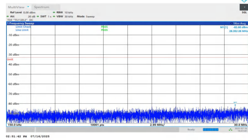
NTNV-n25-PC2-15-40-L-DFT-BPSK-Inner_1RB_Left-0.15-30-PAS S
