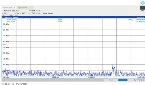
NTNV-n25-PC2-15-35-M-DFT-QPSK-Inner_1RB_Right-0.009-0.1 5-PASS
