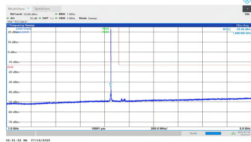
NTNV-n25-PC2-15-40-L-DFT-BPSK-Inner_1RB_Left-1000-3000-PASS ASS
