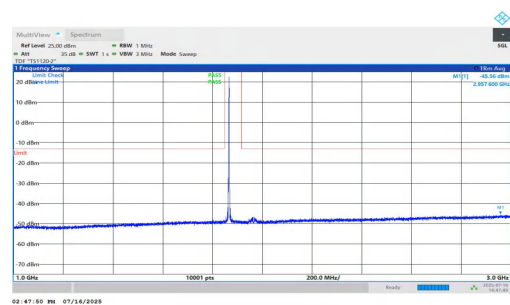
NTNV-n25-PC2-15-35-M-DFT-QPSK-Inner_1RB_Left-1000-3000-PASS
