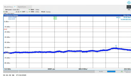
NTNV-n25-PC2-15-30-H-DFT-BPSK-Inner_1RB_Right-12000-200 00-PASS
