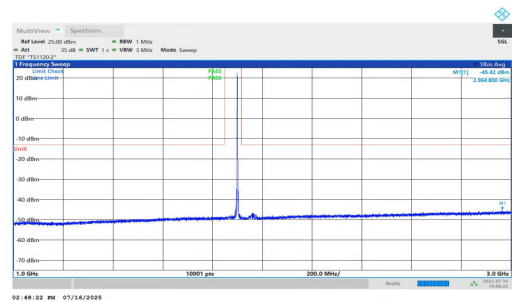
NTNV-n25-PC2-15-35-M-DFT-QPSK-Inner_1RB_Right-1000-3000 -PASS
