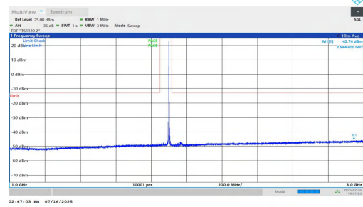
NTNV-n25-PC2-15-35-M-DFT-BPSK-Inner_1RB_Right-1000-3000-PASS
