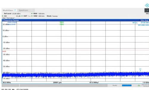
NTNV-n25-PC2-15-35-H-DFT-QPSK-Inner_1RB_Left-30-1000-P ASS
