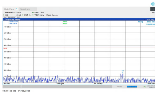
NTNV-n25-PC2-15-40-L-DFT-BPSK-Inner_1RB_Right-0.009-0.15 -PASS
