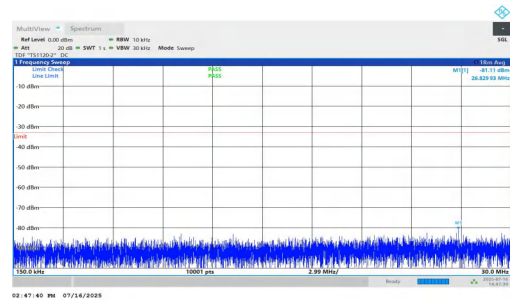
NTNV-n25-PC2-15-35-M-DFT-QPSK-Inner_1RB_Left-0.15-30-PASS
