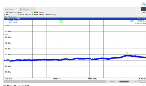
NTNV-n25-PC2-15-30-H-DFT-QPSK-Inner_1RB_Right-12000-20000- 00-PASS
