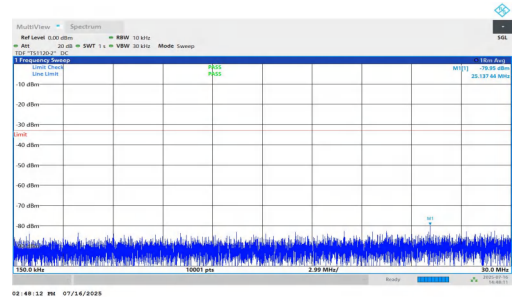
NTNV-n25-PC2-15-35-M-DFT-QPSK-Inner_1RB_Right-0.15-30-P ASS
