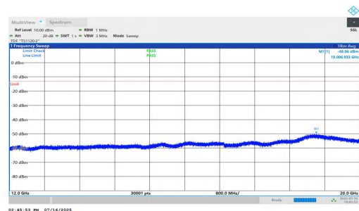
NTNV-n25-PC2-15-35-L-DFT-QPSK-Inner_1RB_Right-12000-20000-PASS 00-PASS
