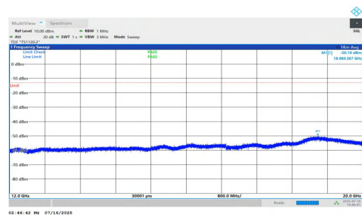
NTNV-n25-PC2-15-35-M-DFT-BPSK-Inner_1RB_Left-12000-20000-PASS
