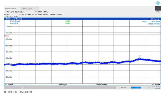
NTNV-n25-PC2-15-35-H-DFT-BPSK-Inner_1RB_Right-12000-200 00-PASS
