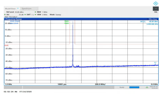
NTNV-n25-PC2-15-40-L-DFT-BPSK-Inner_1RB_Right-1000-3000-P PASS
