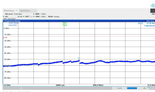
NTNV-n25-PC2-15-35-H-DFT-QPSK-Inner_1RB_Right-3000-12000-PASS
