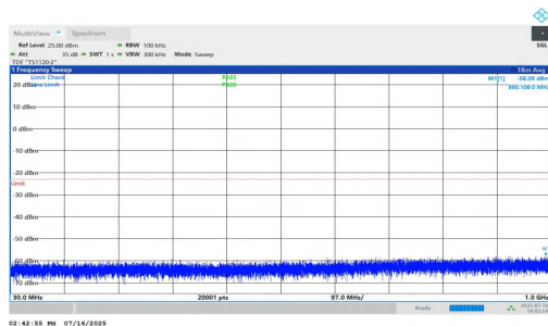
NTNV-n25-PC2-15-30-H-DFT-QPSK-Inner_1RB_Right-30-1000- PASS
