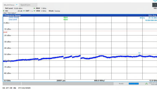
NTNV-n25-PC2-15-35-M-DFT-BPSK-Inner_1RB_Right-3000-12000-PASS
