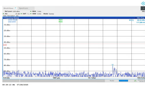
NTNV-n25-PC2-15-35-M-DFT-QPSK-Inner_1RB_Left-0.009-0.15-PASS
