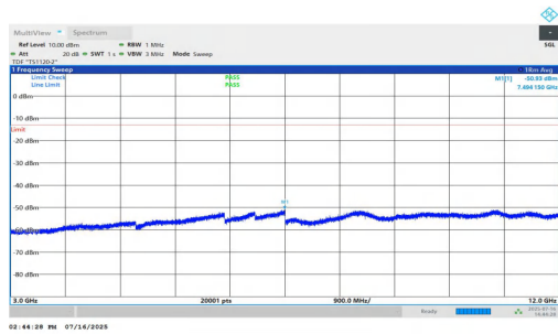
NTNV-n25-PC2-15-35-L-DFT-BPSK-Inner_1RB_Right-3000-1200 0-PASS
