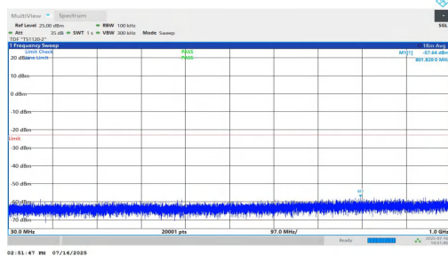
NTNV-n25-PC2-15-40-L-DFT-BPSK-Inner_1RB_Left-30-1000-PASS SS
