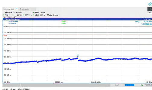
NTNV-n25-PC2-15-35-H-DFT-BPSK-Inner_1RB_Left-3000-12000-PASS
