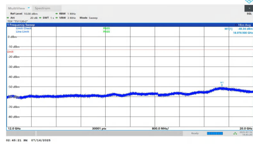
NTNV-n25-PC2-15-35-L-DFT-QPSK-Inner_1RB_Left-12000-20000 0-PASS
