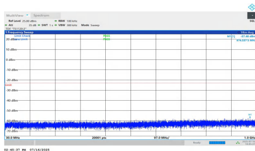
NTNV-n25-PC2-15-35-L-DFT-QPSK-Inner_1RB_Right-30-1000-PASS ASS
