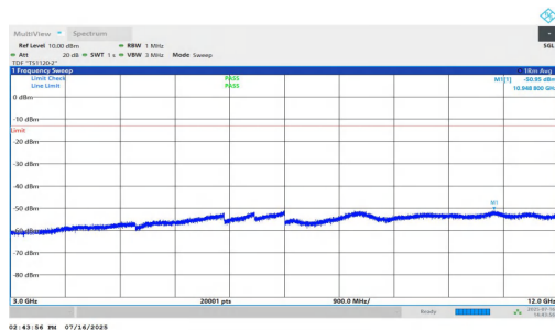
NTNV-n25-PC2-15-35-L-DFT-BPSK-Inner_1RB_Left-3000-12000-PASS
