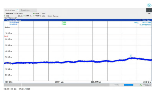
NTNV-n25-PC2-15-35-M-DFT-QPSK-Inner_1RB_Right-12000-200 00-PASS
