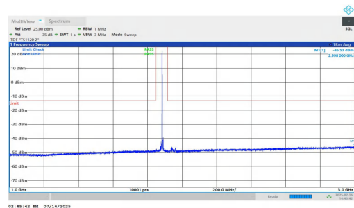
NTNV-n25-PC2-15-35-L-DFT-QPSK-Inner_1RB_Right-1000-3000-PASS PASS
