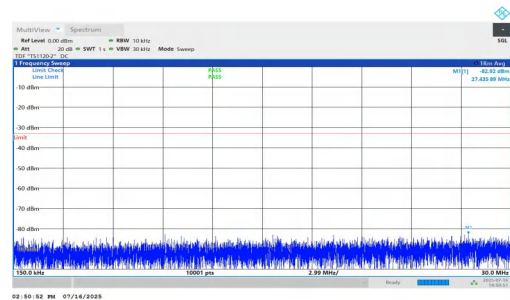
NTNV-n25-PC2-15-35-H-DFT-QPSK-Inner_1RB_Right-0.15-30-PA SS
