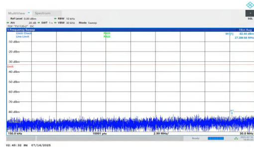
NTNV-n25-PC2-15-35-L-DFT-QPSK-Inner_1RB_Right-0.15-30-PASS SS
