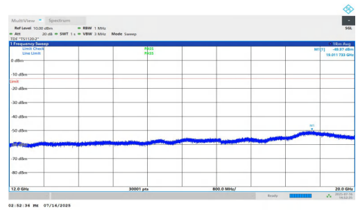
NTNV-n25-PC2-15-40-L-DFT-BPSK-Inner_1RB_Right-12000-200 00-PASS
