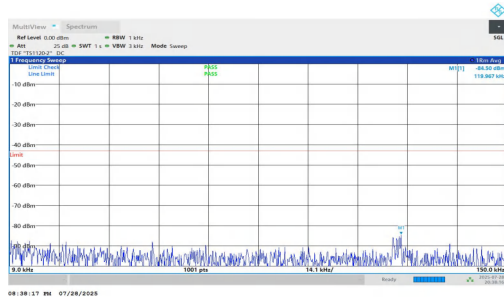
NTNV-n25-PC2-15-35-L-DFT-QPSK-Inner_1RB_Right-0.009-0.1 5-PASS
