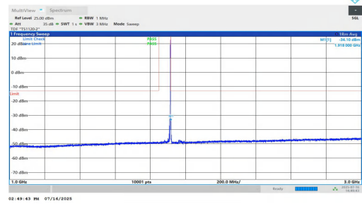
NTNV-n25-PC2-15-35-H-DFT-BPSK-Inner_1RB_Right-1000-3000-P PASS
