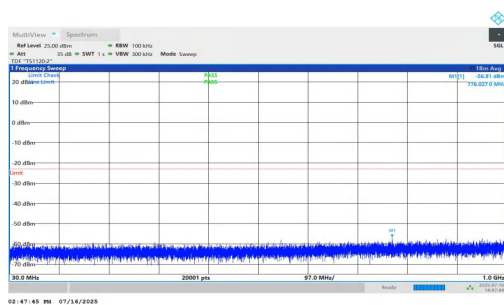
NTNV-n25-PC2-15-35-M-DFT-QPSK-Inner_1RB_Left-30-1000-PASS
