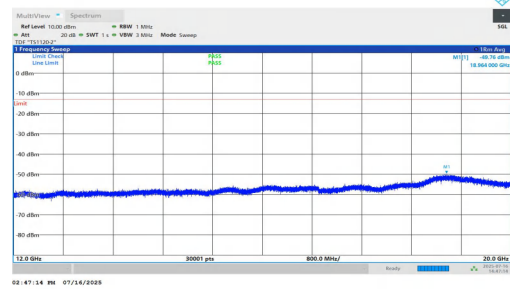
NTNV-n25-PC2-15-35-M-DFT-BPSK-Inner_1RB_Right-12000-20000-PASS
