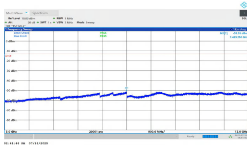
NTNV-n25-PC2-15-30-H-DFT-BPSK-Inner_1RB_Right-3000-120 00-PASS
