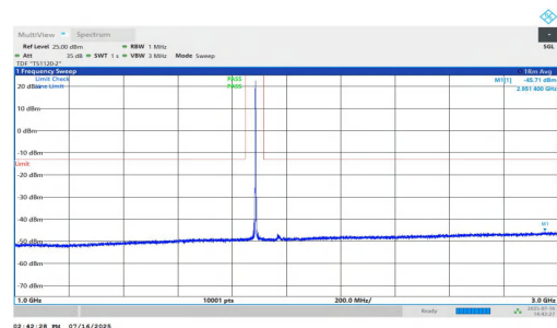
NTNV-n25-PC2-15-30-H-DFT-QPSK-Inner_1RB_Left-1000-3000- PASS
