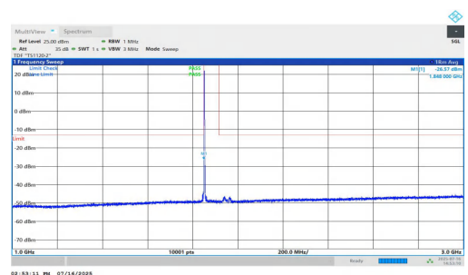
NTNV-n25-PC2-15-40-L-DFT-QPSK-Inner_1RB_Left-1000-3000-P ASS
