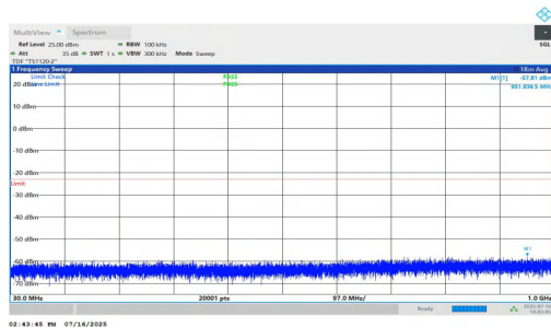
NTNV-n25-PC2-15-35-L-DFT-BPSK-Inner_1RB_Left-30-1000-PASS
