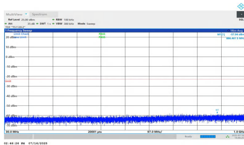
NTNV-n25-PC2-15-35-M-DFT-BPSK-Inner_1RB_Left-30-1000-PASS
