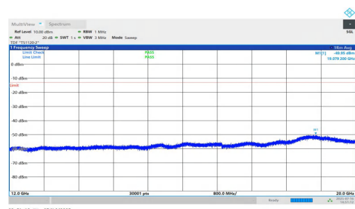
NTNV-n25-PC2-15-35-H-DFT-QPSK-Inner_1RB_Right-12000-20000-PASS
