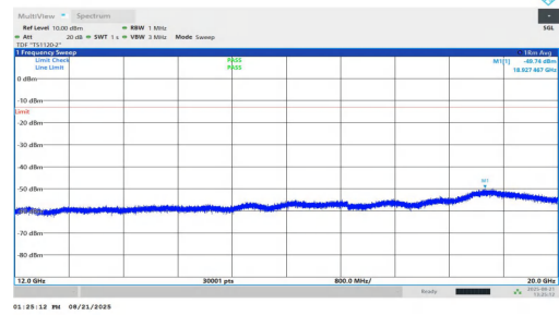
NTNV-n25-PC2-15-25-H-DFT-QPSK-Inner_1RB_Left-12000-2000 0-PASS
