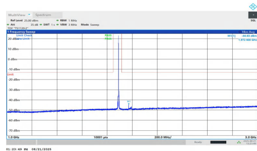
NTNV-n25-PC2-15-25-H-DFT-BPSK-Inner_1RB_Left-1000-3000-P ASS
