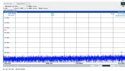
NTNV-n25-PC2-15-25-M-DFT-BPSK-Inner_1RB_Left-0.15-30-PASS
