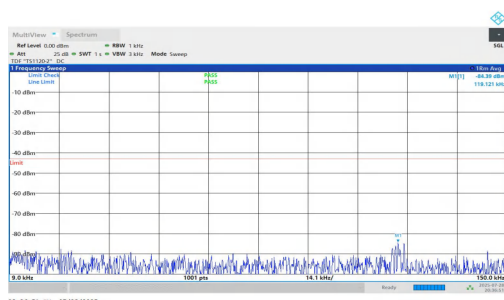
NTNV-n25-PC2-15-30-H-DFT-BPSK-Inner_1RB_Right-0.009-0.15-PASS
