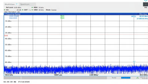
NTNV-n25-PC2-15-30-L-DFT-BPSK-Inner_1RB_Left-0.15-30-PAS S
