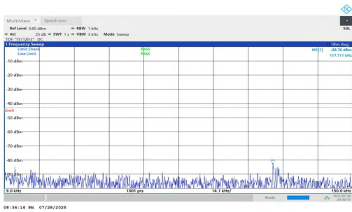
NTNV-n25-PC2-15-30-M-DFT-QPSK-Inner_1RB_Right-0.009-0.1 5-PASS
