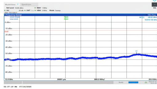
NTNV-n25-PC2-15-30-L-DFT-QPSK-Inner_1RB_Left-12000-20000 0-PASS
