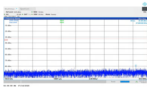
NTNV-n25-PC2-15-30-L-DFT-QPSK-Inner_1RB_Left-0.15-30-PAS S
