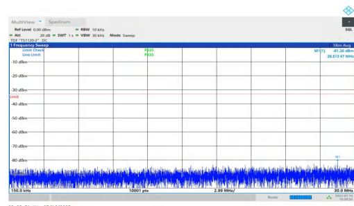
NTNV-n25-PC2-15-30-M-DFT-BPSK-Inner_1RB_Right-0.15-30-PASS
