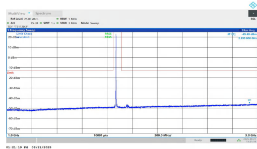
NTNV-n25-PC2-15-25-M-DFT-BPSK-Inner_1RB_Left-1000-3000-PASS
