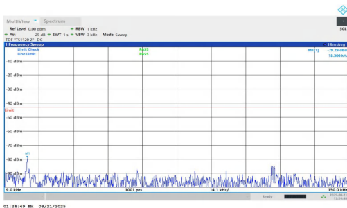
NTNV-n25-PC2-15-25-H-DFT-QPSK-Inner_1RB_Left-0.009-0.15- PASS
