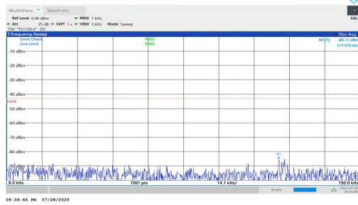
NTNV-n25-PC2-15-30-H-DFT-BPSK-Inner_1RB_Left-0.009-0.15-PASS
