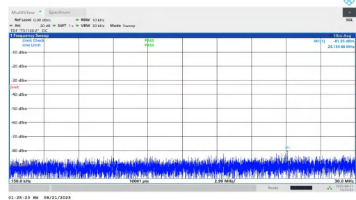
NTNV-n25-PC2-15-25-H-DFT-QPSK-Inner_1RB_Right-0.15-30-PA SS
