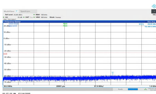
NTNV-n25-PC2-15-30-L-DFT-QPSK-Inner_1RB_Left-30-1000-PA SS
