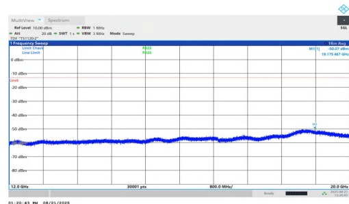
NTNV-n25-PC2-15-25-L-DFT-QPSK-Inner_1RB_Right-12000-20000-PASS
