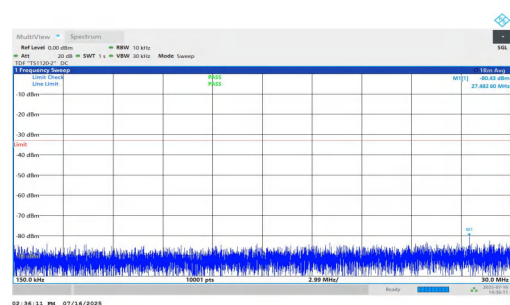
NTNV-n25-PC2-15-30-L-DFT-BPSK-Inner_1RB_Right-0.15-30-PASS SS
