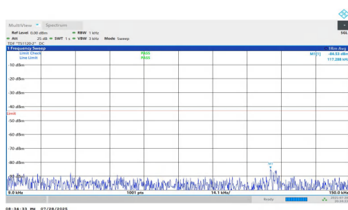
NTNV-n25-PC2-15-30-L-DFT-BPSK-Inner_1RB_Right-0.009-0.15 -PASS
