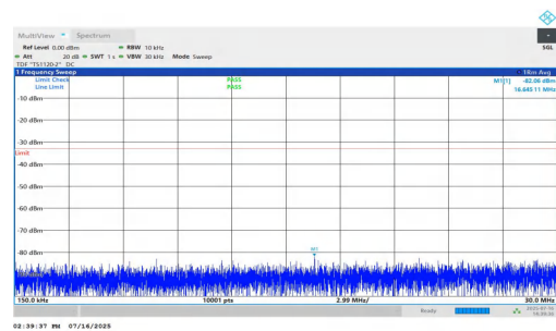
NTNV-n25-PC2-15-30-M-DFT-QPSK-Inner_1RB_Left-0.15-30-PASS
