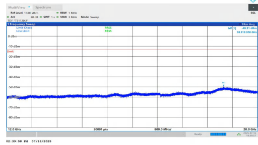
NTNV-n25-PC2-15-30-M-DFT-QPSK-Inner_1RB_Left-12000-2000 0-PASS
