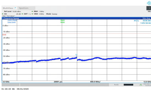
NTNV-n25-PC2-15-25-H-DFT-BPSK-Inner_1RB_Right-3000-120 00-PASS
