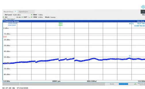
NTNV-n25-PC2-15-30-L-DFT-QPSK-Inner_1RB_Right-3000-12000- 00-PASS
