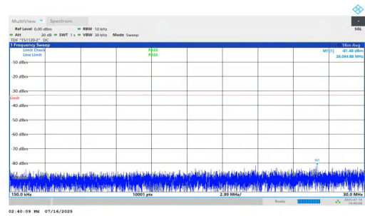
NTNV-n25-PC2-15-30-M-DFT-QPSK-Inner_1RB_Right-0.15-30-P ASS
