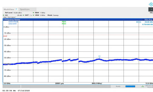
NTNV-n25-PC2-15-30-L-DFT-BPSK-Inner_1RB_Left-3000-12000 -PASS
