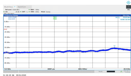
NTNV-n25-PC2-15-25-H-DFT-BPSK-Inner_1RB_Right-12000-200 00-PASS
