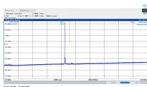
NTNV-n25-PC2-15-30-L-DFT-QPSK-Inner_1RB_Left-1000-3000-P ASS
