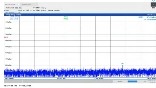
NTNV-n25-PC2-15-30-M-DFT-BPSK-Inner_1RB_Left-0.15-30-PASS
