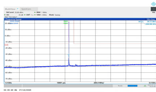
NTNV-n25-PC2-15-30-L-DFT-BPSK-Inner_1RB_Left-1000-3000-P ASS
