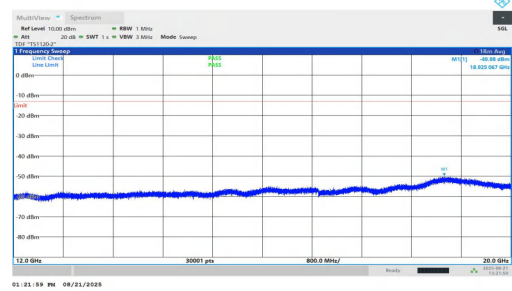
NTNV-n25-PC2-15-25-M-DFT-BPSK-Inner_1RB_Right-12000-20000-PASS
