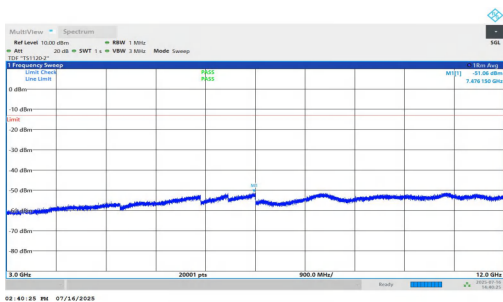
NTNV-n25-PC2-15-30-M-DFT-QPSK-Inner_1RB_Right-3000-12000-PASS
