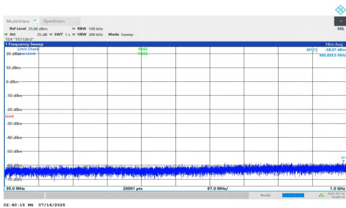
NTNV-n25-PC2-15-30-M-DFT-QPSK-Inner_1RB_Right-30-1000-PASS
