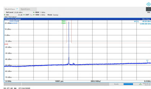
NTNV-n25-PC2-15-30-L-DFT-QPSK-Inner_1RB_Right-1000-3000- PASS
