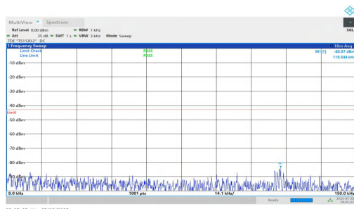
NTNV-n25-PC2-15-30-M-DFT-BPSK-Inner_1RB_Right-0.009-0.15-PASS
