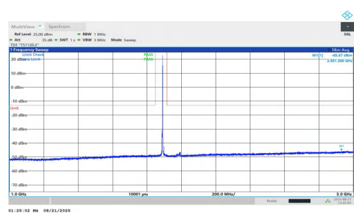
NTNV-n25-PC2-15-25-H-DFT-QPSK-Inner_1RB_Left-1000-3000- PASS
