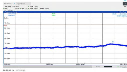
NTNV-n25-PC2-15-25-L-DFT-QPSK-Inner_1RB_Left-12000-20000-PASS
