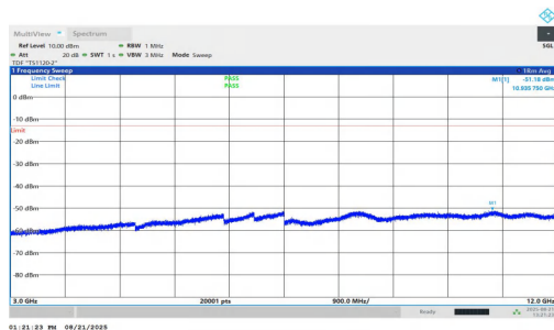
NTNV-n25-PC2-15-25-M-DFT-BPSK-Inner_1RB_Left-3000-12000-PASS
