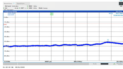
NTNV-n25-PC2-15-25-M-DFT-QPSK-Inner_1RB_Left-12000-2000 0-PASS
