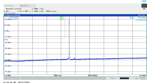
NTNV-n25-PC2-15-25-H-DFT-QPSK-Inner_1RB_Right-1000-3000 -PASS
