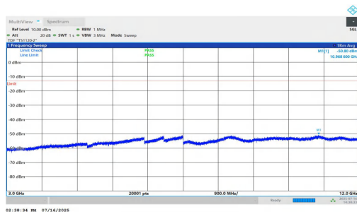
NTNV-n25-PC2-15-30-M-DFT-BPSK-Inner_1RB_Left-3000-12000-PASS
