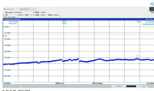
NTNV-n25-PC2-15-25-L-DFT-QPSK-Inner_1RB_Right-3000-12000-PASS
