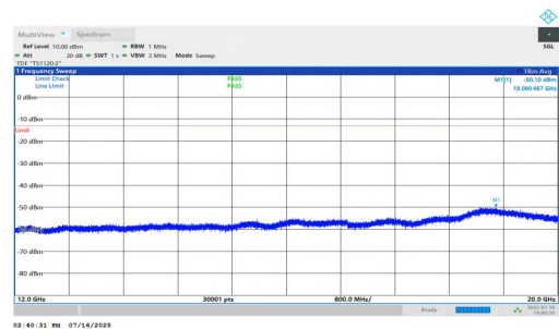
NTNV-n25-PC2-15-30-M-DFT-QPSK-Inner_1RB_Right-12000-20000-PASS
