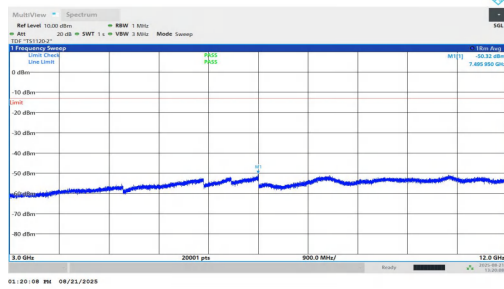
NTNV-n25-PC2-15-25-L-DFT-QPSK-Inner_1RB_Left-3000-12000-PASS
