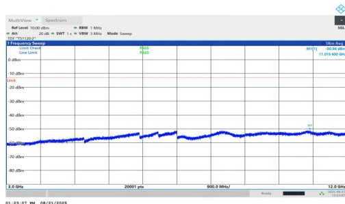
NTNV-n25-PC2-15-25-M-DFT-QPSK-Inner_1RB_Right-3000-120 00-PASS
