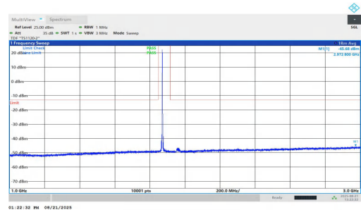
NTNV-n25-PC2-15-25-M-DFT-QPSK-Inner_1RB_Left-1000-3000-PASS
