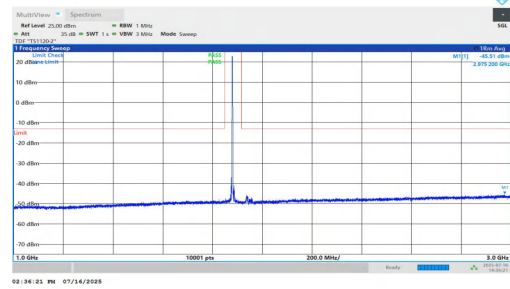
NTNV-n25-PC2-15-30-L-DFT-BPSK-Inner_1RB_Right-1000-3000-P PASS
