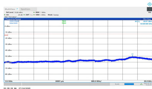
NTNV-n25-PC2-15-30-M-DFT-BPSK-Inner_1RB_Left-12000-20000-PASS
