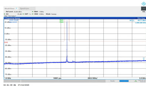
NTNV-n25-PC2-15-30-H-DFT-BPSK-Inner_1RB_Left-1000-3000-PASS
