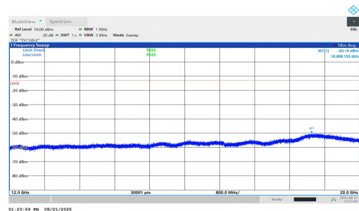
NTNV-n25-PC2-15-25-H-DFT-BPSK-Inner_1RB_Left-12000-20000-PASS 0-PASS
