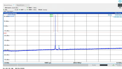
NTNV-n25-PC2-15-25-L-DFT-QPSK-Inner_1RB_Right-1000-3000-PASS
