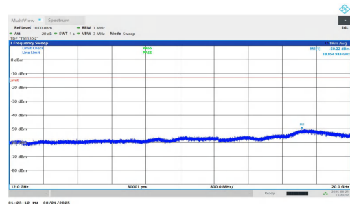
NTNV-n25-PC2-15-25-M-DFT-QPSK-Inner_1RB_Right-12000-200 00-PASS
