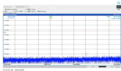
NTNV-n25-PC2-15-25-M-DFT-QPSK-Inner_1RB_Left-0.15-30-PASS
