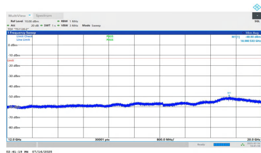
NTNV-n25-PC2-15-30-H-DFT-BPSK-Inner_1RB_Left-12000-20000-PASS
