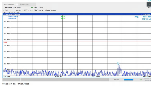
NTNV-n25-PC2-15-30-M-DFT-BPSK-Inner_1RB_Left-0.009-0.15-PASS
