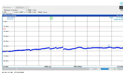
NTNV-n25-PC2-15-30-H-DFT-BPSK-Inner_1RB_Left-3000-12000-PASS
