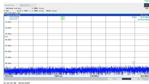
NTNV-n25-PC2-15-25-M-DFT-QPSK-Inner_1RB_Right-0.15-30-P ASS
