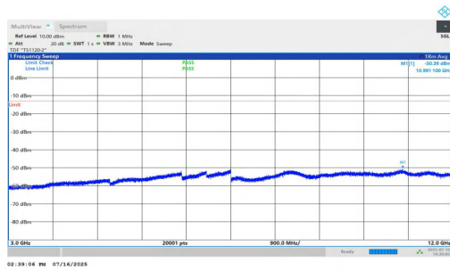
NTNV-n25-PC2-15-30-M-DFT-BPSK-Inner_1RB_Right-3000-12000-PASS
