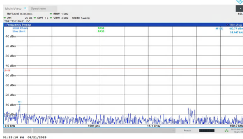
NTNV-n25-PC2-15-25-H-DFT-QPSK-Inner_1RB_Right-0.009-0.1 5-PASS
