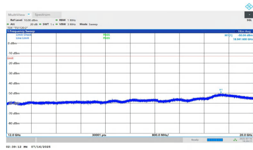
NTNV-n25-PC2-15-30-M-DFT-BPSK-Inner_1RB_Right-12000-20000-PASS
