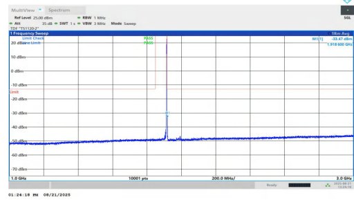
NTNV-n25-PC2-15-25-H-DFT-BPSK-Inner_1RB_Right-1000-3000- PASS
