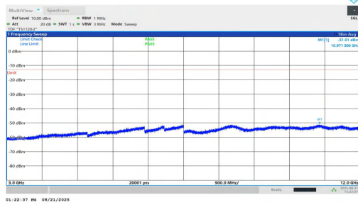
NTNV-n25-PC2-15-25-M-DFT-QPSK-Inner_1RB_Left-3000-1200 0-PASS
