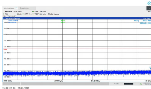
NTNV-n25-PC2-15-25-M-DFT-QPSK-Inner_1RB_Left-30-1000-PASS
