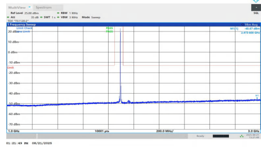
NTNV-n25-PC2-15-25-M-DFT-BPSK-Inner_1RB_Right-1000-3000-PASS
