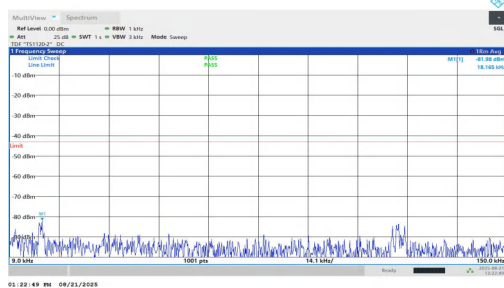
NTNV-n25-PC2-15-25-M-DFT-QPSK-Inner_1RB_Right-0.009-0.1 5-PASS
