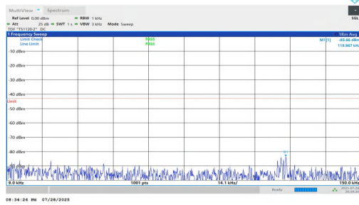
NTNV-n25-PC2-15-30-L-DFT-BPSK-Inner_1RB_Left-0.009-0.15- PASS
