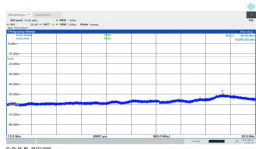
NTNV-n25-PC2-15-25-H-DFT-QPSK-Inner_1RB_Right-12000-200 00-PASS
