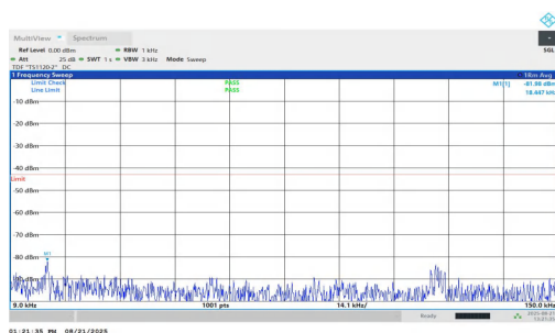
NTNV-n25-PC2-15-25-M-DFT-BPSK-Inner_1RB_Right-0.009-0.15-PASS
