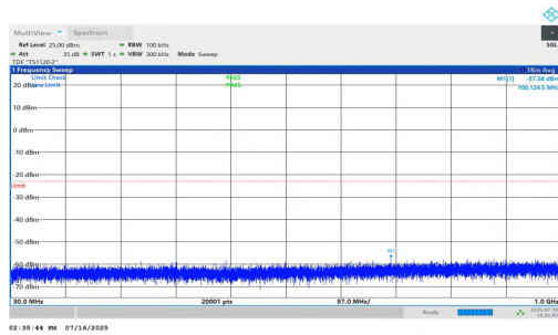
NTNV-n25-PC2-15-30-L-DFT-BPSK-Inner_1RB_Left-30-1000-PASS SS
