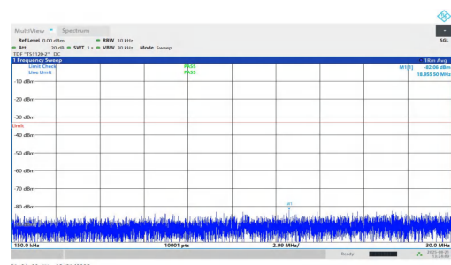
NTNV-n25-PC2-15-25-H-DFT-BPSK-Inner_1RB_Right-0.15-30-PASS SS
