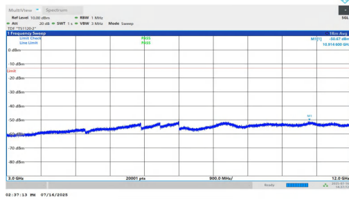
NTNV-n25-PC2-15-30-L-DFT-QPSK-Inner_1RB_Left-3000-12000 -PASS
