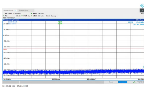
NTNV-n25-PC2-15-30-M-DFT-QPSK-Inner_1RB_Left-30-1000-PASS
