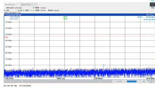
NTNV-n25-PC2-15-30-H-DFT-BPSK-Inner_1RB_Left-0.15-30-PASS
