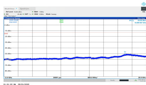
NTNV-n25-PC2-15-25-M-DFT-BPSK-Inner_1RB_Left-12000-20000-PASS
