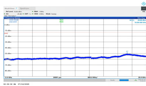
NTNV-n25-PC2-15-30-L-DFT-BPSK-Inner_1RB_Right-12000-200 00-PASS
