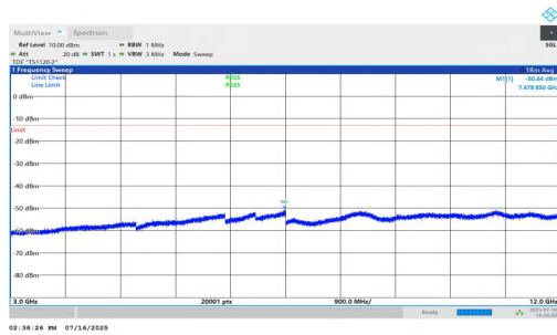
NTNV-n25-PC2-15-30-L-DFT-BPSK-Inner_1RB_Right-3000-1200 0-PASS
