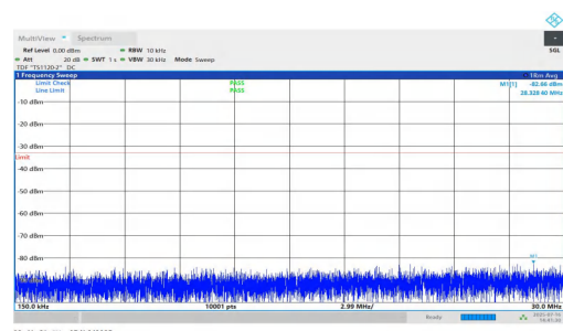
NTNV-n25-PC2-15-30-H-DFT-BPSK-Inner_1RB_Right-0.15-30-PASS
