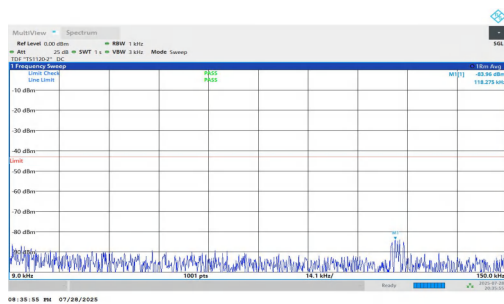
NTNV-n25-PC2-15-30-M-DFT-QPSK-Inner_1RB_Left-0.009-0.15-PASS
