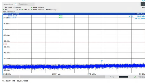
NTNV-n25-PC2-15-25-M-DFT-BPSK-Inner_1RB_Right-30-1000-PASS
