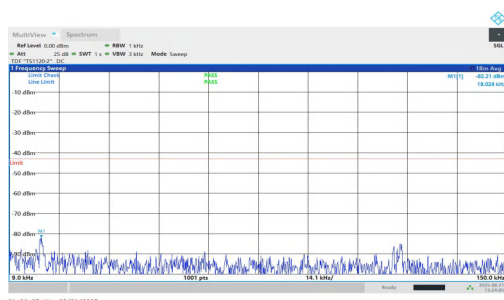
NTNV-n25-PC2-15-25-H-DFT-BPSK-Inner_1RB_Right-0.009-0.15-PASS 5-PASS
