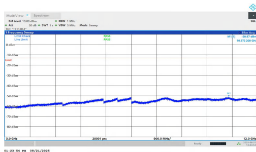
NTNV-n25-PC2-15-25-H-DFT-BPSK-Inner_1RB_Left-3000-12000-PASS 0-PASS
