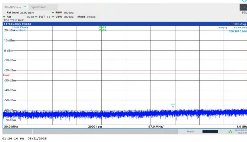
NTNV-n25-PC2-15-25-H-DFT-BPSK-Inner_1RB_Right-30-1000-P ASS
