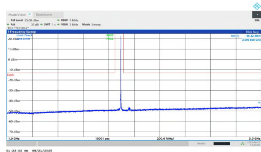
NTNV-n25-PC2-15-25-M-DFT-QPSK-Inner_1RB_Right-1000-3000 -PASS
