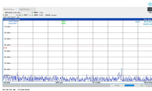
NTNV-n25-PC2-15-30-L-DFT-QPSK-Inner_1RB_Left-0.009-0.15- PASS
