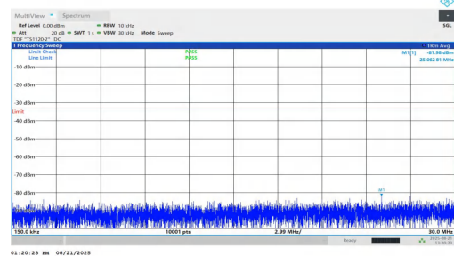
NTNV-n25-PC2-15-25-L-DFT-QPSK-Inner_1RB_Right-0.15-30-PASS
