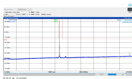
NTNV-n25-PC2-15-30-M-DFT-QPSK-Inner_1RB_Left-1000-3000-PASS
