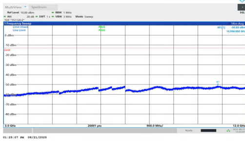
NTNV-n25-PC2-15-25-H-DFT-QPSK-Inner_1RB_Left-3000-1200 0-PASS
