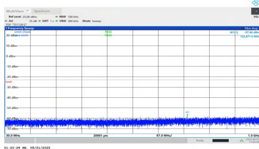
NTNV-n25-PC2-15-25-L-DFT-QPSK-Inner_1RB_Right-30-1000-PASS
