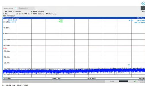
NTNV-n25-PC2-15-25-M-DFT-QPSK-Inner_1RB_Right-30-1000- PASS
