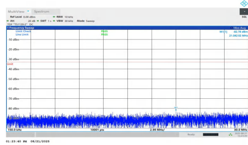
NTNV-n25-PC2-15-25-H-DFT-BPSK-Inner_1RB_Left-0.15-30-PAS S
