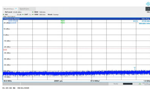
NTNV-n25-PC2-15-25-H-DFT-BPSK-Inner_1RB_Left-30-1000-PASS SS
