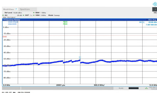
NTNV-n25-PC2-15-25-H-DFT-QPSK-Inner_1RB_Right-3000-120 00-PASS
