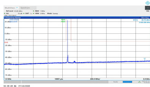
NTNV-n25-PC2-15-30-M-DFT-BPSK-Inner_1RB_Left-1000-3000-PASS
