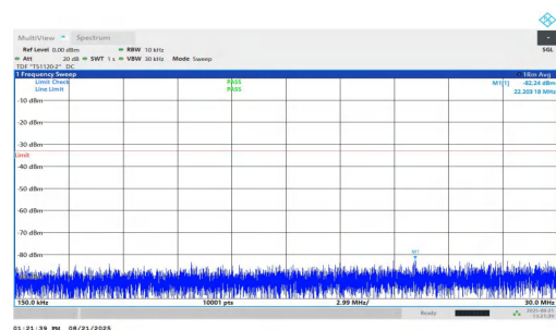
NTNV-n25-PC2-15-25-M-DFT-BPSK-Inner_1RB_Right-0.15-30-PASS
