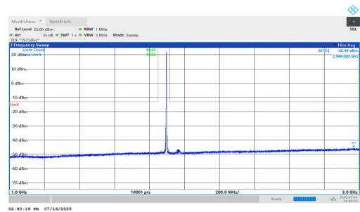
NTNV-n25-PC2-15-30-M-DFT-QPSK-Inner_1RB_Right-1000-3000-PASS
