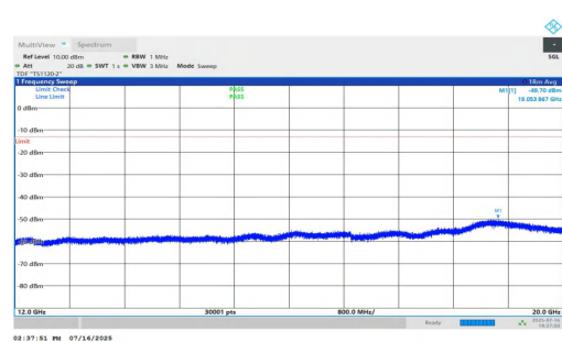
NTNV-n25-PC2-15-30-L-DFT-QPSK-Inner_1RB_Right-12000-20000- 00-PASS
