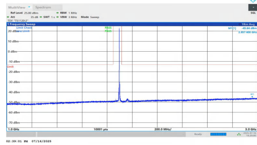
NTNV-n25-PC2-15-30-M-DFT-BPSK-Inner_1RB_Right-1000-3000-PASS
