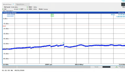
NTNV-n25-PC2-15-25-M-DFT-BPSK-Inner_1RB_Right-3000-12000-PASS
