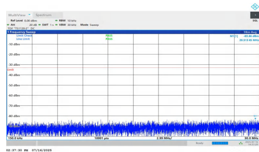
NTNV-n25-PC2-15-30-L-DFT-QPSK-Inner_1RB_Right-0.15-30-PA SS
