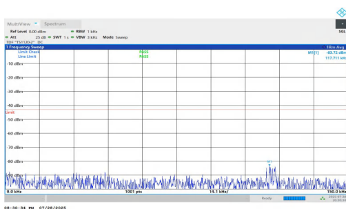
NTNV-n25-PC2-15-15-H-DFT-BPSK-Inner_1RB_Right-0.009-0.15-PASS
