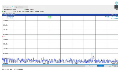
NTNV-n25-PC2-15-15-H-DFT-QPSK-Inner_1RB_Right-0.009-0.1 5-PASS
