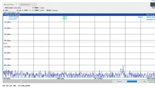
NTNV-n25-PC2-15-20-M-DFT-BPSK-Inner_1RB_Left-0.009-0.15-PASS
