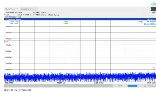
NTNV-n25-PC2-15-20-L-DFT-QPSK-Inner_1RB_Right-0.15-30-PASS
