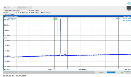
NTNV-n25-PC2-15-20-M-DFT-QPSK-Inner_1RB_Right-1000-3000- -PASS
