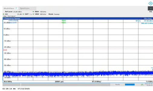
NTNV-n25-PC2-15-20-L-DFT-BPSK-Inner_1RB_Right-30-1000-P ASS
