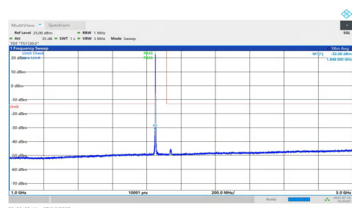
NTNV-n25-PC2-15-20-L-DFT-QPSK-Inner_1RB_Left-1000-3000-P ASS
