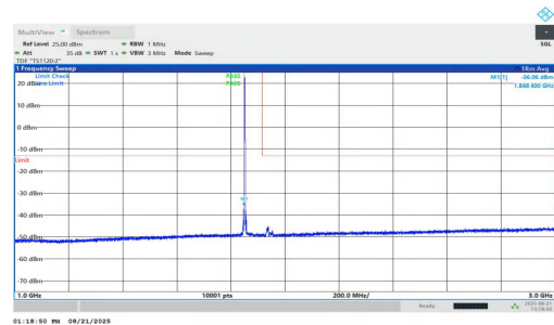
NTNV-n25-PC2-15-25-L-DFT-BPSK-Inner_1RB_Left-1000-3000-P ASS
