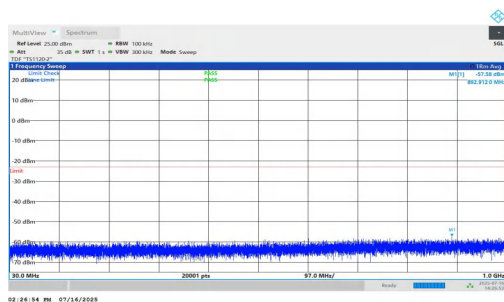
NTNV-n25-PC2-15-15-H-DFT-QPSK-Inner_1RB_Right-30-1000- PASS
