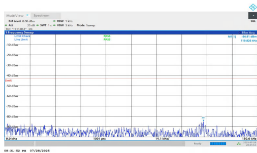
NTNV-n25-PC2-15-20-L-DFT-QPSK-Inner_1RB_Left-0.009-0.15- PASS
