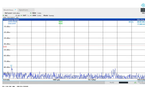
NTNV-n25-PC2-15-25-L-DFT-BPSK-Inner_1RB_Right-0.009-0.15 -PASS
