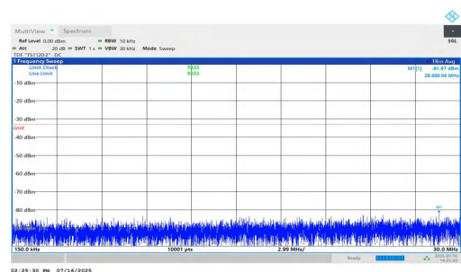
NTNV-n25-PC2-15-15-H-DFT-BPSK-Inner_1RB_Right-0.15-30-PASS
