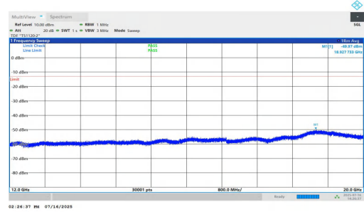
NTNV-n25-PC2-15-15-H-DFT-QPSK-Inner_1RB_Left-12000-2000 0-PASS
