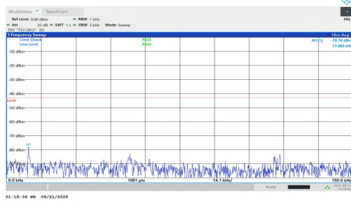
NTNV-n25-PC2-15-25-L-DFT-BPSK-Inner_1RB_Left-0.009-0.15- PASS
