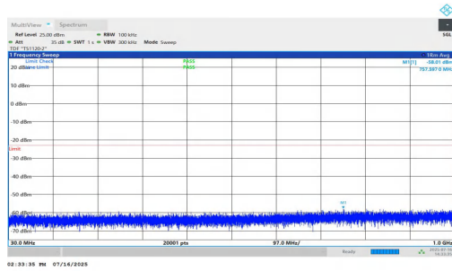
NTNV-n25-PC2-15-20-H-DFT-BPSK-Inner_1RB_Right-30-1000-PASS
