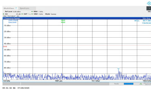
NTNV-n25-PC2-15-20-L-DFT-BPSK-Inner_1RB_Right-0.009-0.15 -PASS
