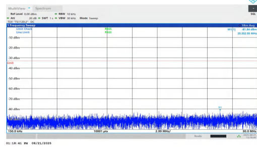
NTNV-n25-PC2-15-25-L-DFT-BPSK-Inner_1RB_Left-0.15-30-PAS S
