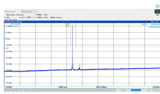
NTNV-n25-PC2-15-20-M-DFT-QPSK-Inner_1RB_Left-1000-3000-PASS
