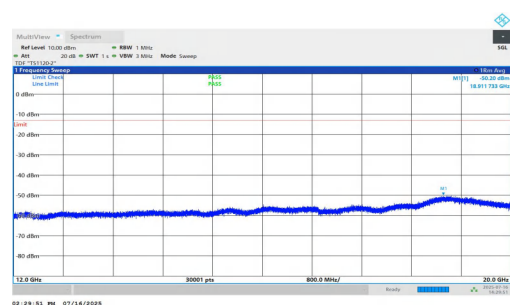
NTNV-n25-PC2-15-20-L-DFT-QPSK-Inner_1RB_Right-12000-20000-00-PASS
