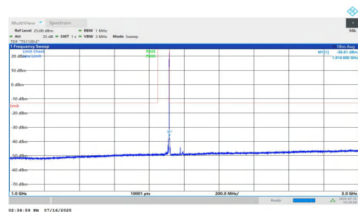
NTNV-n25-PC2-15-20-H-DFT-QPSK-Inner_1RB_Right-1000-3000 -PASS
