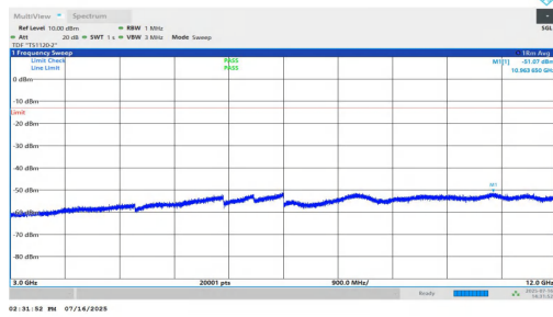
NTNV-n25-PC2-15-20-M-DFT-QPSK-Inner_1RB_Left-3000-1200 0-PASS
