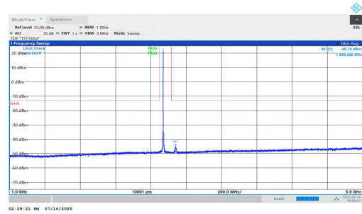
NTNV-n25-PC2-15-20-L-DFT-BPSK-Inner_1RB_Right-1000-3000-P PASS
