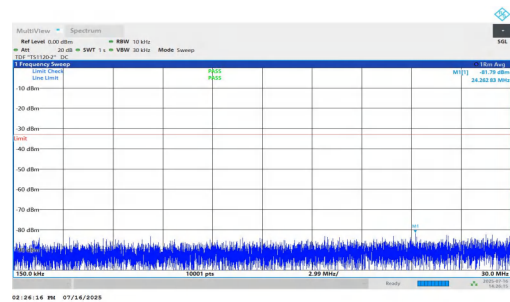
NTNV-n25-PC2-15-15-H-DFT-QPSK-Inner_1RB_Left-0.15-30-PAS S
