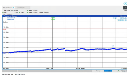
NTNV-n25-PC2-15-20-M-DFT-BPSK-Inner_1RB_Left-3000-12000-PASS
