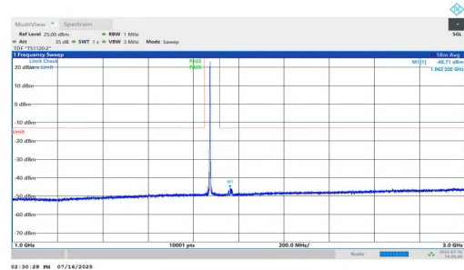
NTNV-n25-PC2-15-20-M-DFT-BPSK-Inner_1RB_Left-1000-3000-PASS
