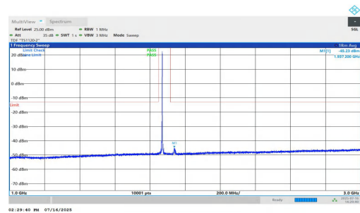
NTNV-n25-PC2-15-20-L-DFT-QPSK-Inner_1RB_Right-1000-3000-PASS
