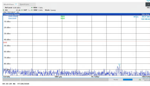
NTNV-n25-PC2-15-20-H-DFT-BPSK-Inner_1RB_Left-0.009-0.15-PASS
