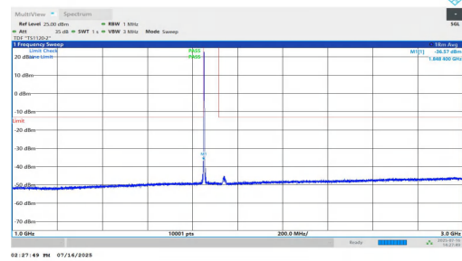
NTNV-n25-PC2-15-20-L-DFT-BPSK-Inner_1RB_Left-1000-3000-P ASS
