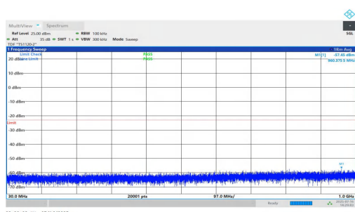
NTNV-n25-PC2-15-20-L-DFT-QPSK-Inner_1RB_Left-30-1000-PA SS
