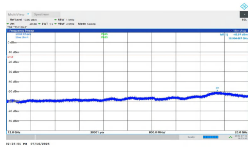
NTNV-n25-PC2-15-15-H-DFT-BPSK-Inner_1RB_Right-12000-200 00-PASS
