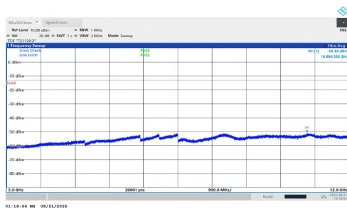
NTNV-n25-PC2-15-25-L-DFT-BPSK-Inner_1RB_Left-3000-12000 -PASS
