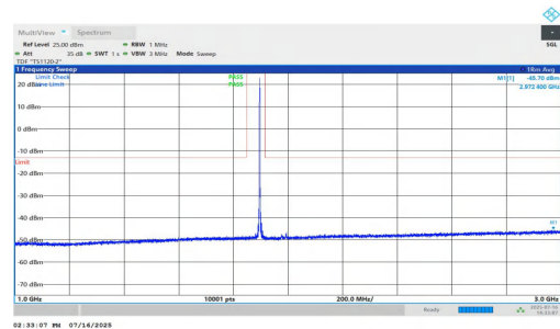
NTNV-n25-PC2-15-20-H-DFT-BPSK-Inner_1RB_Left-1000-3000-PASS ASS
