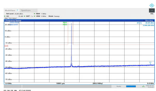
NTNV-n25-PC2-15-20-H-DFT-QPSK-Inner_1RB_Left-1000-3000-PASS
