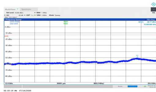
NTNV-n25-PC2-15-20-H-DFT-BPSK-Inner_1RB_Left-12000-20000-PASS 0-PASS
