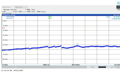
NTNV-n25-PC2-15-25-L-DFT-BPSK-Inner_1RB_Right-3000-12000-PASS
