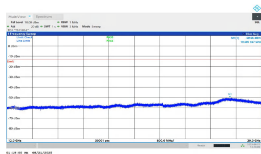
NTNV-n25-PC2-15-25-L-DFT-BPSK-Inner_1RB_Left-12000-20000 -PASS
