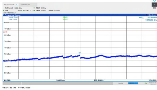
NTNV-n25-PC2-15-20-H-DFT-QPSK-Inner_1RB_Left-3000-1200 0-PASS
