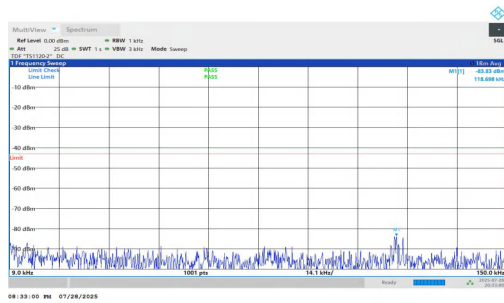
NTNV-n25-PC2-15-20-M-DFT-QPSK-Inner_1RB_Right-0.009-0.1 5-PASS
