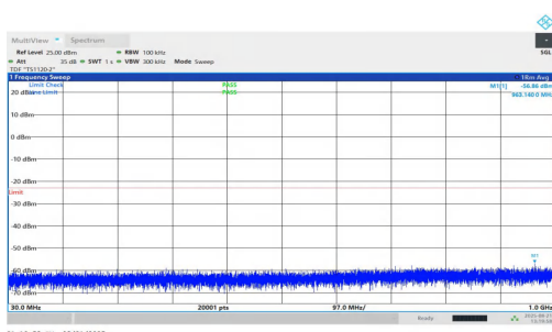
NTNV-n25-PC2-15-25-L-DFT-QPSK-Inner_1RB_Left-30-1000-PASS
