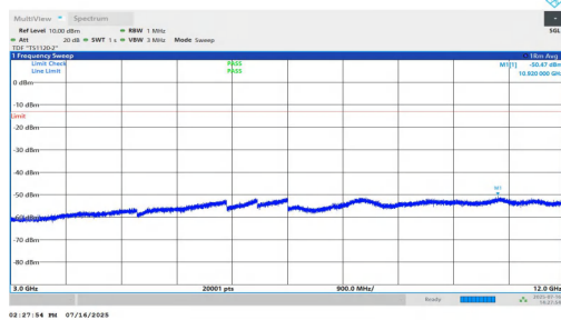
NTNV-n25-PC2-15-20-L-DFT-BPSK-Inner_1RB_Left-3000-12000 -PASS
