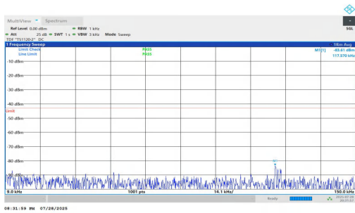
NTNV-n25-PC2-15-20-L-DFT-QPSK-Inner_1RB_Right-0.009-0.1 5-PASS
