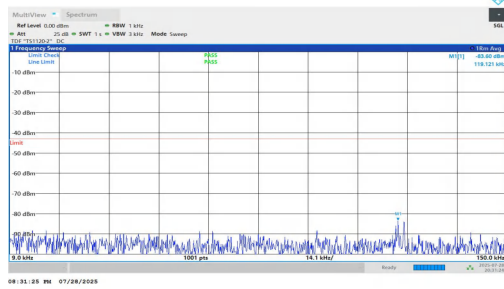
NTNV-n25-PC2-15-20-L-DFT-BPSK-Inner_1RB_Left-0.009-0.15- PASS
