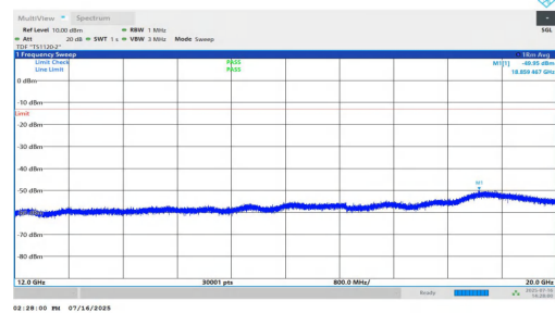
NTNV-n25-PC2-15-20-L-DFT-BPSK-Inner_1RB_Left-12000-20000 -PASS
