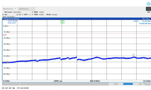
NTNV-n25-PC2-15-15-H-DFT-BPSK-Inner_1RB_Right-3000-120 00-PASS
