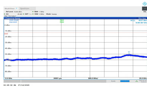
NTNV-n25-PC2-15-20-L-DFT-BPSK-Inner_1RB_Right-12000-200 00-PASS
