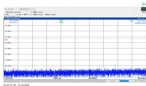
NTNV-n25-PC2-15-20-H-DFT-BPSK-Inner_1RB_Right-0.15-30-PASS SS
