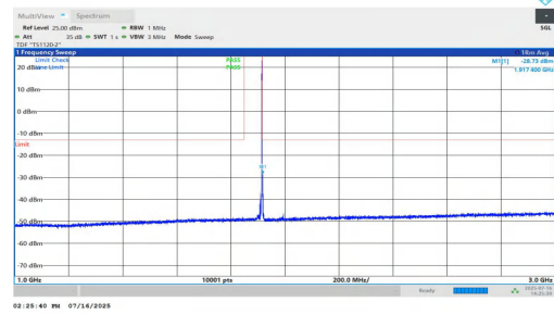
NTNV-n25-PC2-15-15-H-DFT-BPSK-Inner_1RB_Right-1000-3000-P PASS
