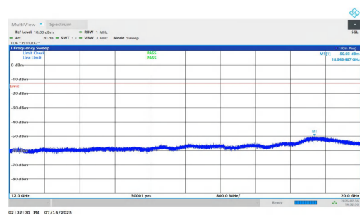
NTNV-n25-PC2-15-20-M-DFT-QPSK-Inner_1RB_Right-12000-20000- 00-PASS
