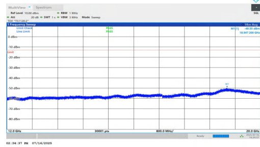
NTNV-n25-PC2-15-20-H-DFT-QPSK-Inner_1RB_Left-12000-2000 0-PASS
