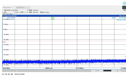
NTNV-n25-PC2-15-25-L-DFT-BPSK-Inner_1RB_Left-30-1000-PA SS
