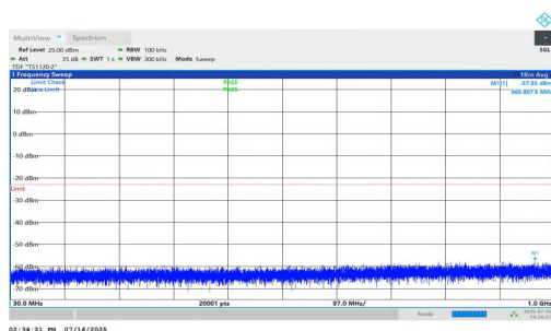
NTNV-n25-PC2-15-20-H-DFT-QPSK-Inner_1RB_Left-30-1000-PASS
