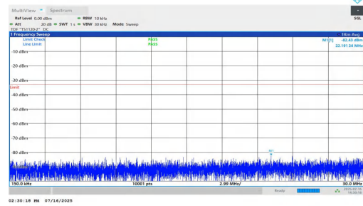
NTNV-n25-PC2-15-20-M-DFT-BPSK-Inner_1RB_Left-0.15-30-PASS
