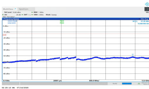
NTNV-n25-PC2-15-15-H-DFT-BPSK-Inner_1RB_Left-3000-12000-PASS
