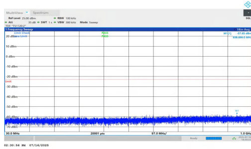
NTNV-n25-PC2-15-20-M-DFT-BPSK-Inner_1RB_Right-30-1000-PASS
