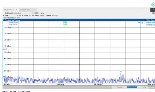
NTNV-n25-PC2-15-20-M-DFT-BPSK-Inner_1RB_Right-0.009-0.15-PASS
