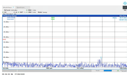
NTNV-n25-PC2-15-20-H-DFT-QPSK-Inner_1RB_Right-0.009-0.1 5-PASS
