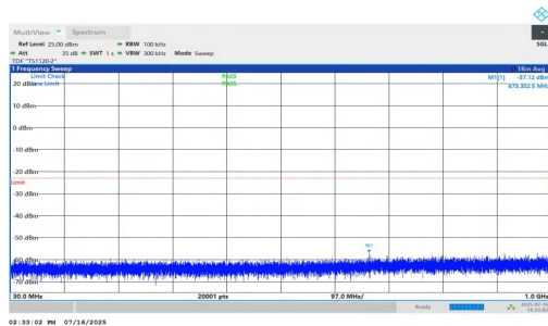
NTNV-n25-PC2-15-20-H-DFT-BPSK-Inner_1RB_Left-30-1000-PASS SS
