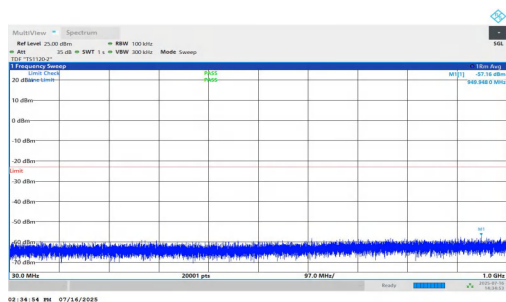
NTNV-n25-PC2-15-20-H-DFT-QPSK-Inner_1RB_Right-30-1000- PASS
