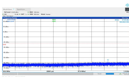
NTNV-n25-PC2-15-20-M-DFT-QPSK-Inner_1RB_Left-30-1000-PASS
