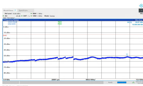
NTNV-n25-PC2-15-15-H-DFT-QPSK-Inner_1RB_Right-3000-12000- 00-PASS
