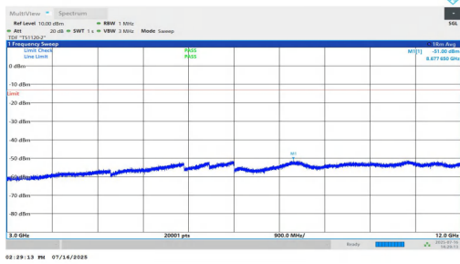
NTNV-n25-PC2-15-20-L-DFT-QPSK-Inner_1RB_Left-3000-12000 -PASS
