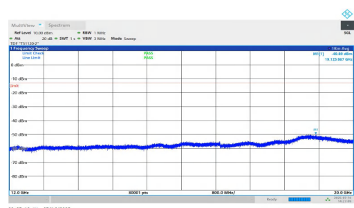
NTNV-n25-PC2-15-15-H-DFT-QPSK-Inner_1RB_Right-12000-20000- 00-PASS
