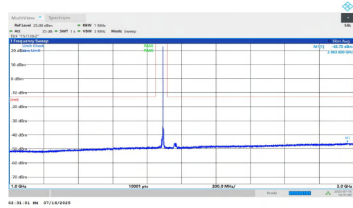
NTNV-n25-PC2-15-20-M-DFT-BPSK-Inner_1RB_Right-1000-3000-PASS
