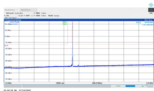
NTNV-n25-PC2-15-15-H-DFT-QPSK-Inner_1RB_Right-1000-3000- -PASS
