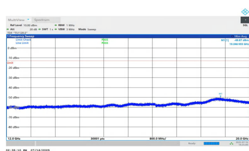
NTNV-n25-PC2-15-20-H-DFT-QPSK-Inner_1RB_Right-12000-20000- 00-PASS
