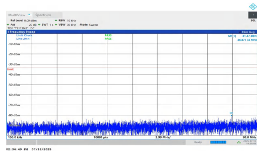
NTNV-n25-PC2-15-20-H-DFT-QPSK-Inner_1RB_Right-0.15-30-PA SS
