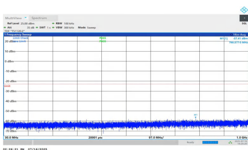
NTNV-n25-PC2-15-15-H-DFT-QPSK-Inner_1RB_Left-30-1000-P ASS
