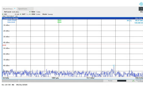
NTNV-n25-PC2-15-25-L-DFT-QPSK-Inner_1RB_Left-0.009-0.15-PASS
