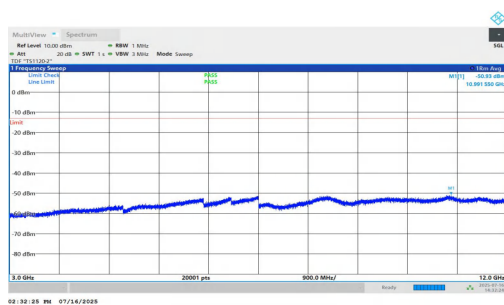
NTNV-n25-PC2-15-20-M-DFT-QPSK-Inner_1RB_Right-3000-12000- 00-PASS
