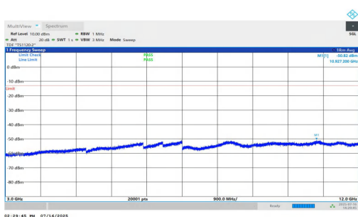
NTNV-n25-PC2-15-20-L-DFT-QPSK-Inner_1RB_Right-3000-12000-00-PASS
