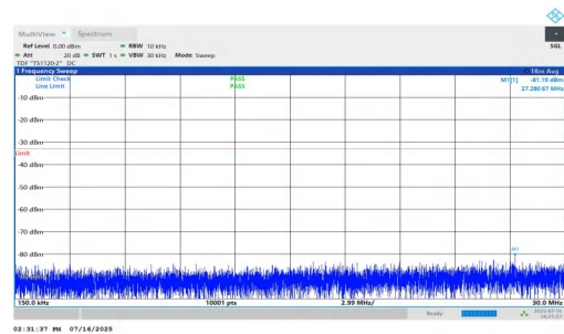
NTNV-n25-PC2-15-20-M-DFT-QPSK-Inner_1RB_Left-0.15-30-PASS
