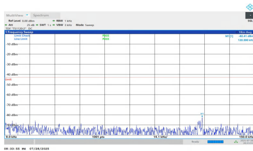
NTNV-n25-PC2-15-20-H-DFT-QPSK-Inner_1RB_Left-0.009-0.15-PASS
