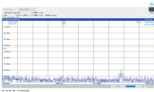
NTNV-n25-PC2-15-15-H-DFT-QPSK-Inner_1RB_Left-0.009-0.15- PASS
