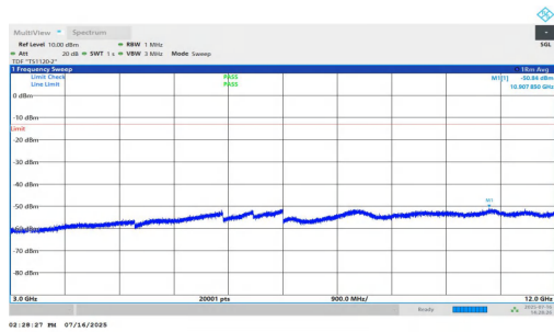
NTNV-n25-PC2-15-20-L-DFT-BPSK-Inner_1RB_Right-3000-1200 0-PASS
