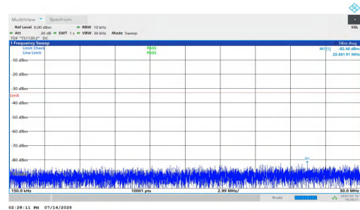
NTNV-n25-PC2-15-20-L-DFT-BPSK-Inner_1RB_Right-0.15-30-PA SS
