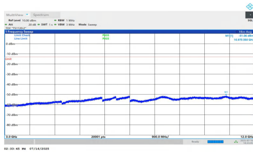
NTNV-n25-PC2-15-20-H-DFT-BPSK-Inner_1RB_Right-3000-12000-PASS
