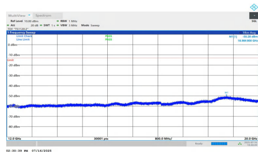
NTNV-n25-PC2-15-20-M-DFT-BPSK-Inner_1RB_Left-12000-20000-PASS
