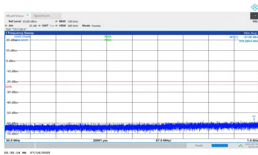
NTNV-n25-PC2-15-20-M-DFT-QPSK-Inner_1RB_Right-30-1000- PASS
