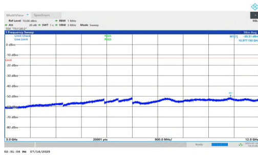
NTNV-n25-PC2-15-20-M-DFT-BPSK-Inner_1RB_Right-3000-12000-PASS
