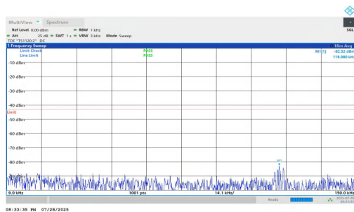
NTNV-n25-PC2-15-20-H-DFT-BPSK-Inner_1RB_Right-0.009-0.15-PASS 5-PASS
