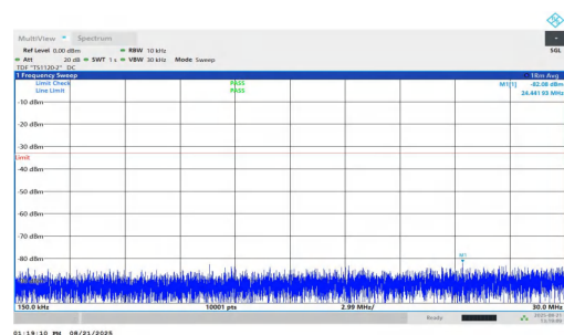
NTNV-n25-PC2-15-25-L-DFT-BPSK-Inner_1RB_Right-0.15-30-PA SS
