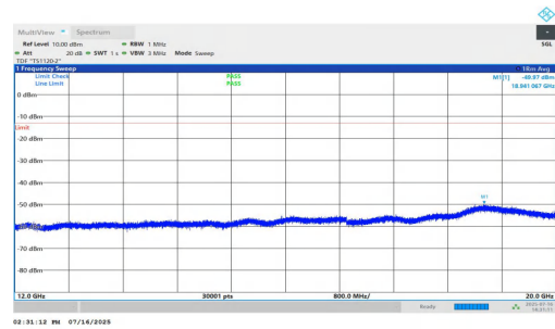
NTNV-n25-PC2-15-20-M-DFT-BPSK-Inner_1RB_Right-12000-20000-PASS
