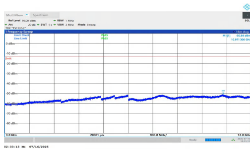
NTNV-n25-PC2-15-20-H-DFT-BPSK-Inner_1RB_Left-3000-12000-PASS 0-PASS
