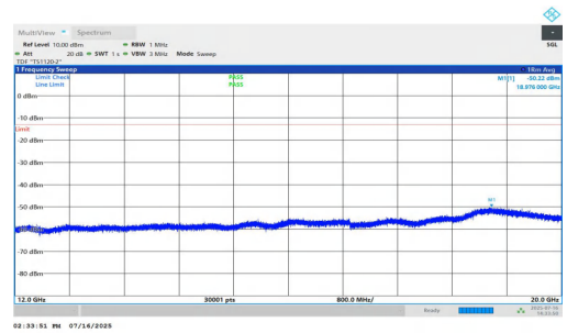
NTNV-n25-PC2-15-20-H-DFT-BPSK-Inner_1RB_Right-12000-20000-PASS
