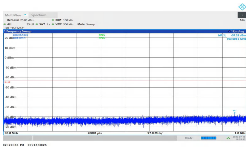
NTNV-n25-PC2-15-20-L-DFT-QPSK-Inner_1RB_Right-30-1000-PASS
