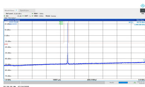
NTNV-n25-PC2-15-15-H-DFT-QPSK-Inner_1RB_Left-1000-3000- PASS
