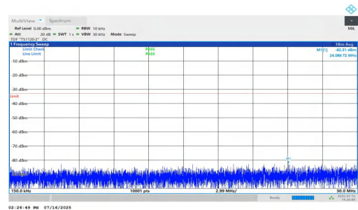
NTNV-n25-PC2-15-15-H-DFT-QPSK-Inner_1RB_Right-0.15-30-PA SS
