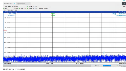
NTNV-n25-PC2-15-20-L-DFT-BPSK-Inner_1RB_Left-0.15-30-PAS S
