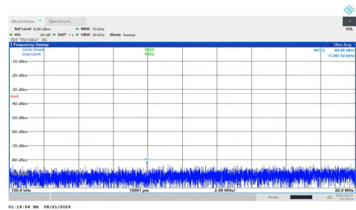
NTNV-n25-PC2-15-25-L-DFT-QPSK-Inner_1RB_Left-0.15-30-PASS
