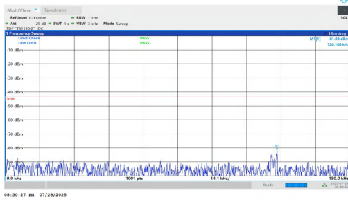
NTNV-n25-PC2-15-15-H-DFT-BPSK-Inner_1RB_Left-0.009-0.15-PASS
