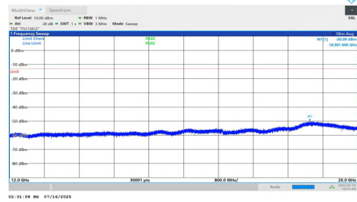
NTNV-n25-PC2-15-20-M-DFT-QPSK-Inner_1RB_Left-12000-2000 0-PASS
