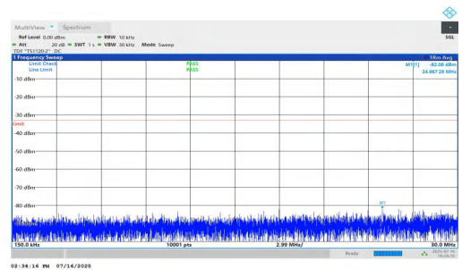
NTNV-n25-PC2-15-20-H-DFT-QPSK-Inner_1RB_Left-0.15-30-PASS
