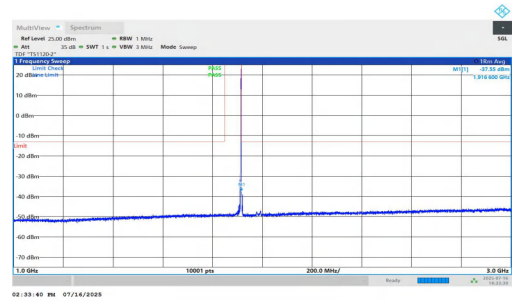
NTNV-n25-PC2-15-20-H-DFT-BPSK-Inner_1RB_Right-1000-3000-PASS
