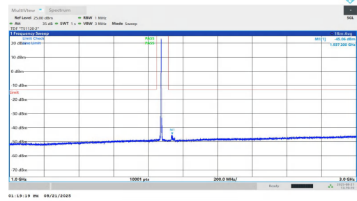
NTNV-n25-PC2-15-25-L-DFT-BPSK-Inner_1RB_Right-1000-3000-PASS
