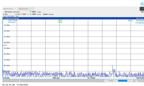
NTNV-n25-PC2-15-20-M-DFT-QPSK-Inner_1RB_Left-0.009-0.15-PASS
