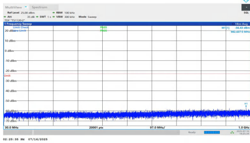
NTNV-n25-PC2-15-15-H-DFT-BPSK-Inner_1RB_Right-30-1000-P ASS
