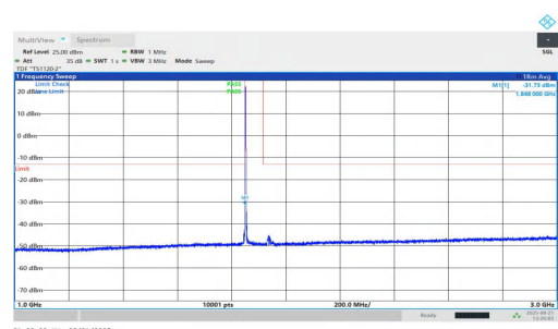
NTNV-n25-PC2-15-25-L-DFT-QPSK-Inner_1RB_Left-1000-3000-PASS
