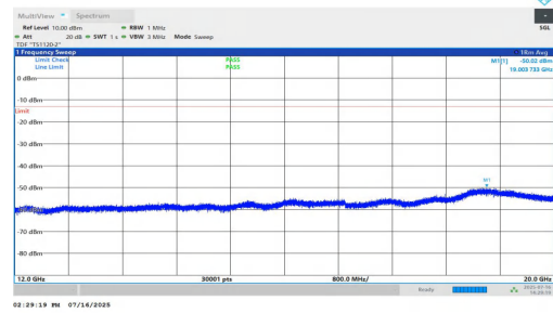
NTNV-n25-PC2-15-20-L-DFT-QPSK-Inner_1RB_Left-12000-20000 0-PASS
