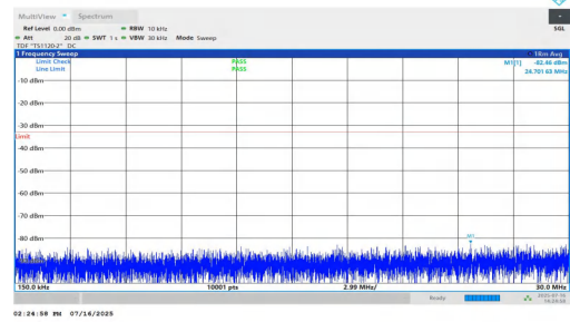
NTNV-n25-PC2-15-15-H-DFT-BPSK-Inner_1RB_Left-0.15-30-PAS S
