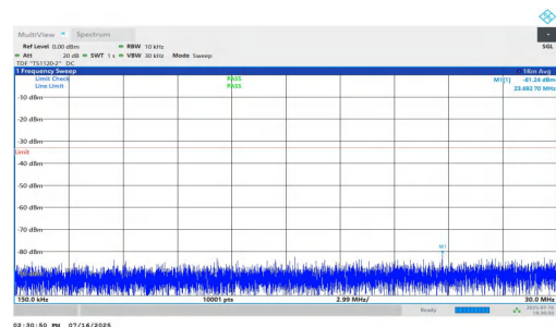
NTNV-n25-PC2-15-20-M-DFT-BPSK-Inner_1RB_Right-0.15-30-PASS
