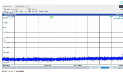
NTNV-n25-PC2-15-20-M-DFT-BPSK-Inner_1RB_Left-30-1000-PASS
