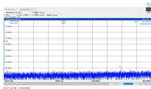
NTNV-n25-PC2-15-10-H-DFT-BPSK-Inner_1RB_Right-0.15-30-PASS SS
