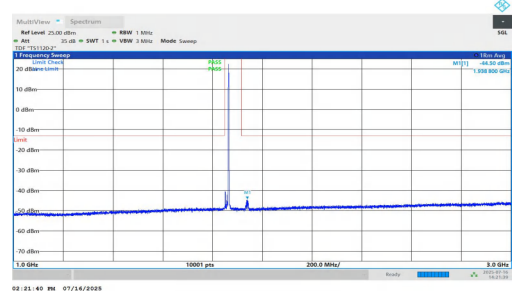
NTVN-n25-PC2-15-15-L-DFT-QPSK-Inner_1RB_Right-1000-3000- PASS
