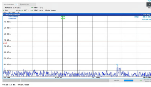
NTNV-n25-PC2-15-10-L-DFT-BPSK-Inner_1RB_Left-0.009-0.15-PASS
