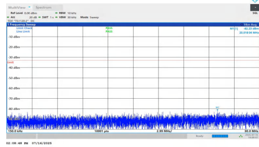
NTNV-n25-PC2-15-5-H-DFT-BPSK-Inner_1RB_Left-0.15-30-PASS
