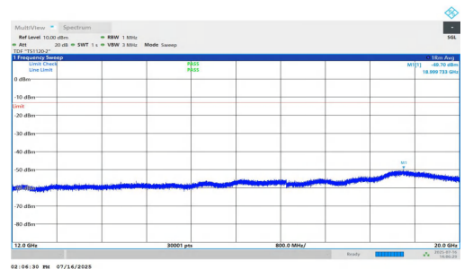
NTNV-n25-PC2-15-5-M-DFT-BPSK-Inner_1RB_Left-12000-20000-PASS
