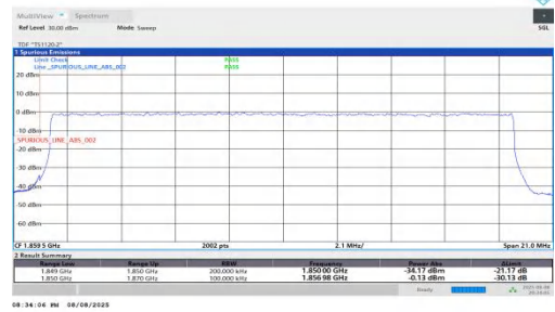
NTNV-n25-PC2-15-20-L-DFT-QPSK-Outer_Full-PASS
