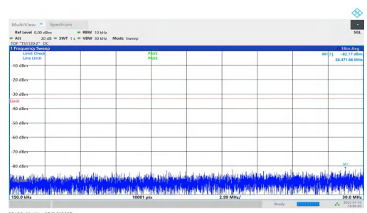
NTNV-n25-PC2-15-5-M-DFT-BPSK-Inner_1RB_Right-0.15-30-PASS
