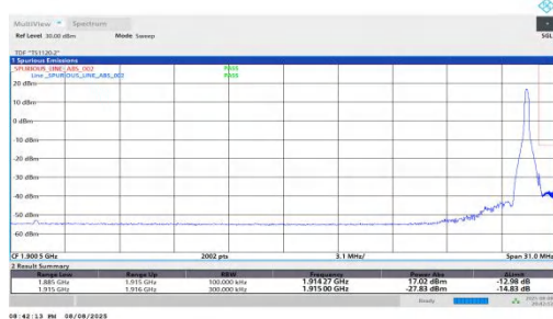
NTNV-n25-PC2-15-30-H-DFT-QPSK-Edge_1RB_Right-PASS
