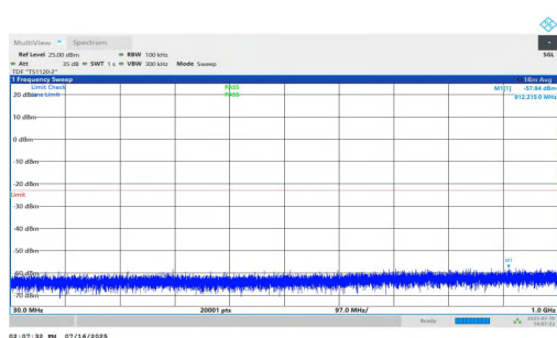
NTNV-n25-PC2-15-5-M-DFT-QPSK-Inner_1RB_Left-30-1000-PA SS
