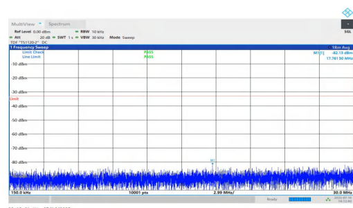
NTNV-n25-PC2-15-10-L-DFT-BPSK-Inner_1RB_Right-0.15-30-PASS
