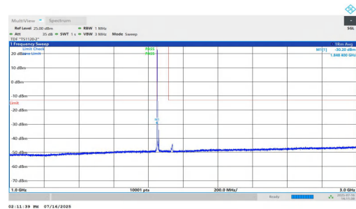
NTNV-n25-PC2-15-10-L-DFT-BPSK-Inner_1RB_Left-1000-3000-PASS
