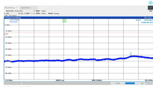
NTNV-n25-PC2-15-5-L-DFT-QPSK-Inner_1RB_Right-12000-20000-PASS
