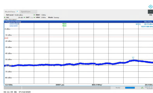
NTNV-n25-PC2-15-5-H-DFT-QPSK-Inner_1RB_Right-12000-20000-PASS
