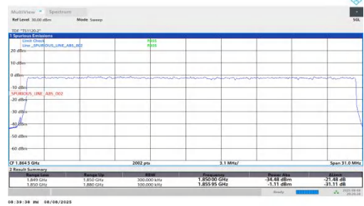
NTNV-n25-PC2-15-30-L-DFT-BPSK-Outer_Full-PASS
