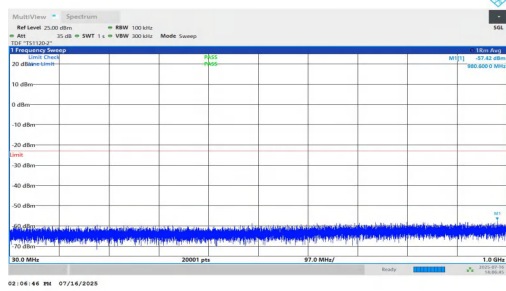
NTNV-n25-PC2-15-5-M-DFT-BPSK-Inner_1RB_Right-30-1000-P ASS
