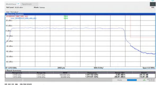
NTNV-n25-PC2-15-5-H-DFT-QPSK-Outer_Full-PASS
