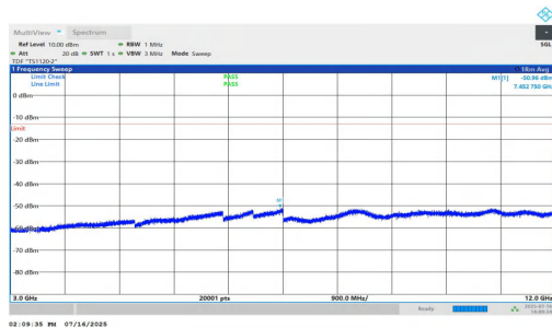
NTNV-n25-PC2-15-5-H-DFT-BPSK-Inner_1RB_Right-3000-12000-PASS
