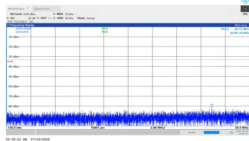
NTNV-n25-PC2-15-5-L-DFT-QPSK-Inner_1RB_Right-0.15-30-PASS
