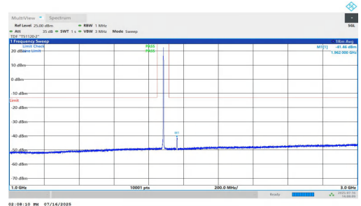
NTNV-n25-PC2-15-5-M-DFT-QPSK-Inner_1RB_Right-1000-3000- PASS
