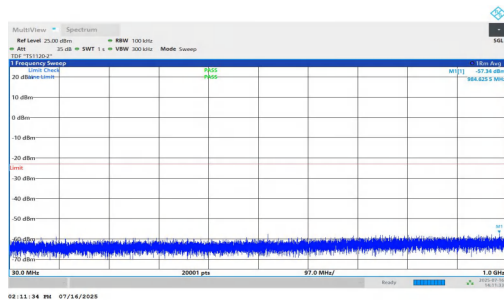
NTNV-n25-PC2-15-10-L-DFT-BPSK-Inner_1RB_Left-30-1000-PASS
