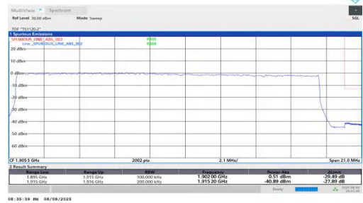
NTNV-n25-PC2-15-20-H-DFT-QPSK-Outer_Full-PASS
