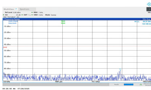
NTNV-n25-PC2-15-5-H-DFT-QPSK-Inner_1RB_Left-0.009-0.15-P ASS
