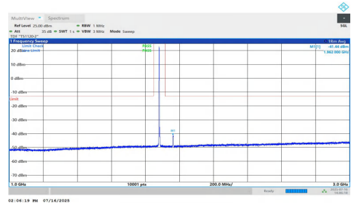
NTNV-n25-PC2-15-5-M-DFT-BPSK-Inner_1RB_Left-1000-3000-PASS
