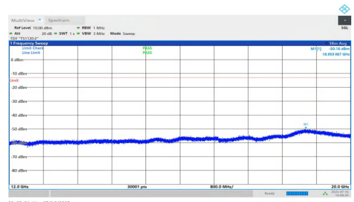
NTNV-n25-PC2-15-5-M-DFT-QPSK-Inner_1RB_Right-12000-2000 0-PASS
