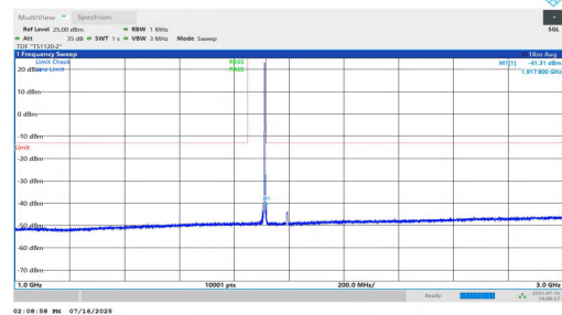
NTNV-n25-PC2-15-5-H-DFT-BPSK-Inner_1RB_Left-1000-3000-P ASS
