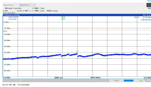
NTNV-n25-PC2-15-5-M-DFT-QPSK-Inner_1RB_Left-3000-12000 -PASS
