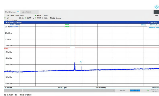
NTNV-n25-PC2-15-5-H-DFT-QPSK-Inner_1RB_Left-1000-3000-PASS
