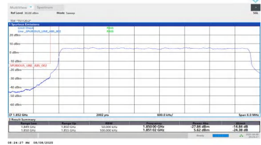
NTNV-n25-PC2-15-5-L-DFT-QPSK-Outer_Full-PASS
