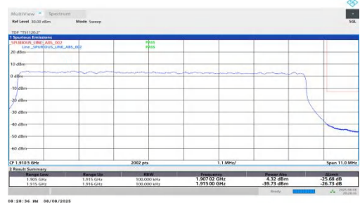
NTNV-n25-PC2-15-10-H-DFT-BPSK-Outer_Full-PASS
