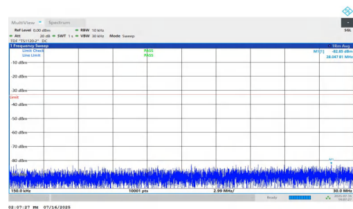
NTNV-n25-PC2-15-5-M-DFT-QPSK-Inner_1RB_Left-0.15-30-PAS S
