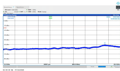
NTNV-n25-PC2-15-5-H-DFT-BPSK-Inner_1RB_Left-12000-20000- PASS
