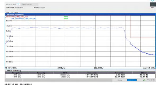
NTNV-n25-PC2-15-5-H-DFT-BPSK-Outer_Full-PASS
