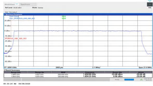
NTNV-n25-PC2-15-20-L-DFT-BPSK-Outer_Full-PASS
