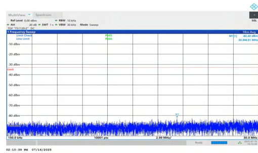
NTNV-n25-PC2-15-5-H-DFT-QPSK-Inner_1RB_Right-0.15-30-PA-SS
