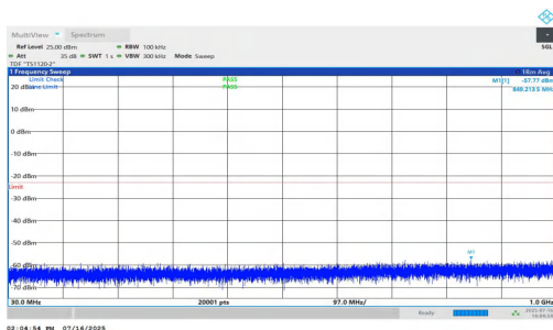
NTNV-n25-PC2-15-5-L-DFT-QPSK-Inner_1RB_Left-30-1000-PA SS
