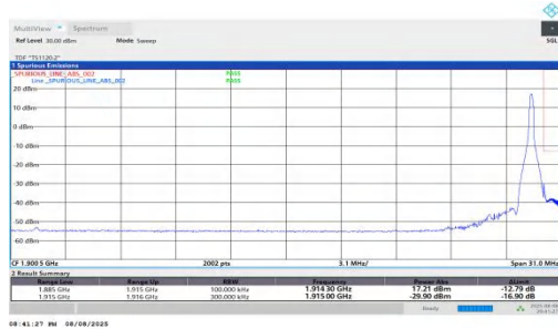
NTNV-n25-PC2-15-30-H-DFT-BPSK-Edge_1RB_Right-PASS
