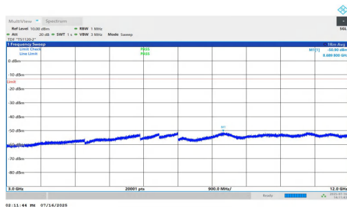
NTNV-n25-PC2-15-10-L-DFT-BPSK-Inner_1RB_Left-3000-12000-PASS
