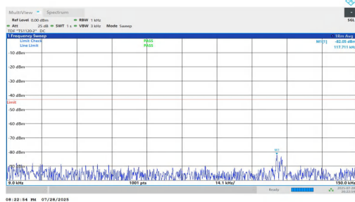
NTNV-n25-PC2-15-5-L-DFT-QPSK-Inner_1RB_Right-0.009-0.15-PASS
