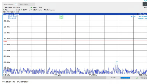
NTNV-n25-PC2-15-5-H-DFT-BPSK-Inner_1RB_Left-0.009-0.15-P ASS
