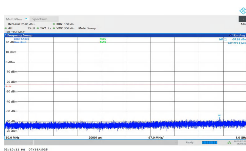
NTNV-n25-PC2-15-5-H-DFT-QPSK-Inner_1RB_Left-30-1000-PASS
