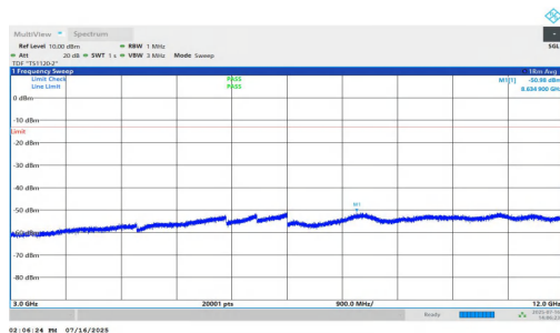
NTNV-n25-PC2-15-5-M-DFT-BPSK-Inner_1RB_Left-3000-12000-PASS
