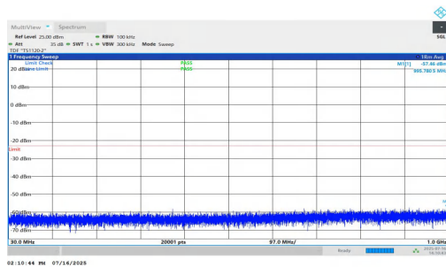
NTNV-n25-PC2-15-5-H-DFT-QPSK-Inner_1RB_Right-30-1000-PASS
