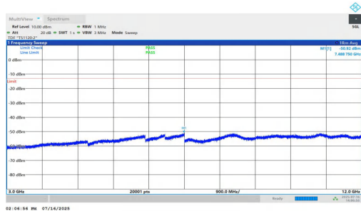
NTNV-n25-PC2-15-5-M-DFT-BPSK-Inner_1RB_Right-3000-1200 0-PASS
