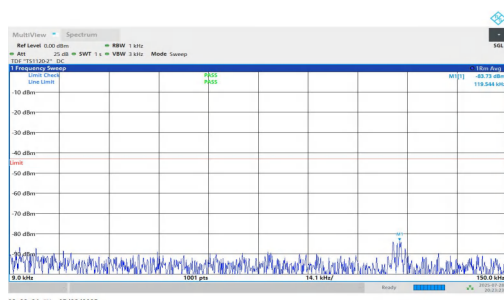
NTNV-n25-PC2-15-5-M-DFT-BPSK-Inner_1RB_Right-0.009-0.15-PASS
