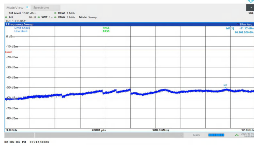
NTNV-n25-PC2-15-5-L-DFT-QPSK-Inner_1RB_Left-3000-12000-PASS
