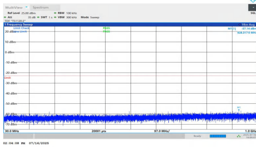
NTNV-n25-PC2-15-5-L-DFT-BPSK-Inner_1RB_Right-30-1000-PA SS
