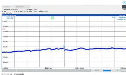
NTNV-n25-PC2-15-5-L-DFT-BPSK-Inner_1RB_Right-3000-12000 -PASS
