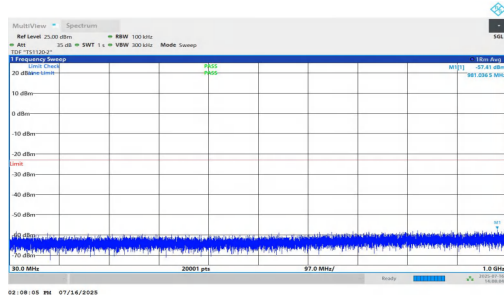
NTNV-n25-PC2-15-5-M-DFT-QPSK-Inner_1RB_Right-30-1000-P ASS
