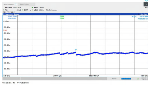
NTNV-n25-PC2-15-5-H-DFT-QPSK-Inner_1RB_Left-3000-12000-PASS
