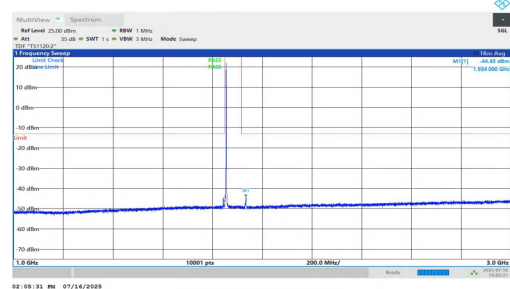
NTNV-n25-PC2-15-5-L-DFT-QPSK-Inner_1RB_Right-1000-3000-PASS
