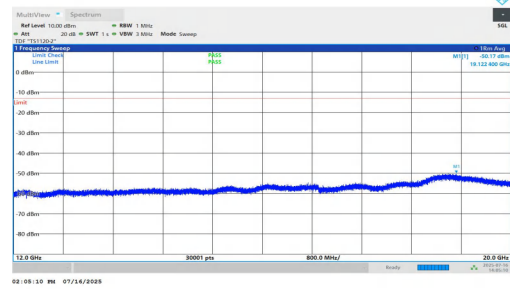
NTNV-n25-PC2-15-5-L-DFT-QPSK-Inner_1RB_Left-12000-20000-PASS
