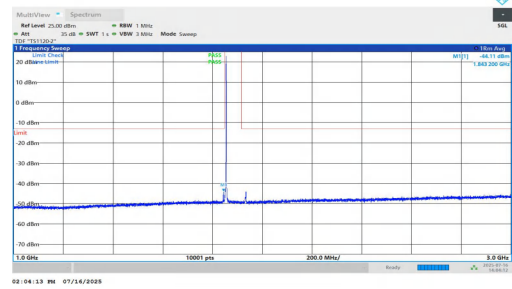
NTNV-n25-PC2-15-5-L-DFT-BPSK-Inner_1RB_Right-1000-3000-P ASS
