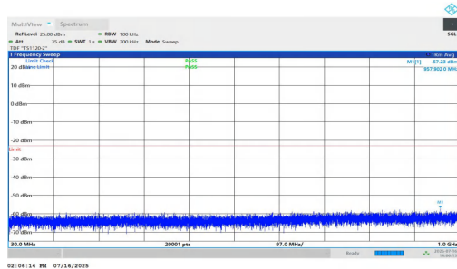
NTNV-n25-PC2-15-5-M-DFT-BPSK-Inner_1RB_Left-30-1000-PASS
