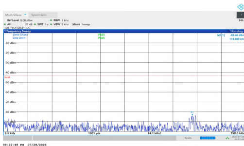
NTNV-n25-PC2-15-5-L-DFT-QPSK-Inner_1RB_Left-0.009-0.15-P ASS
