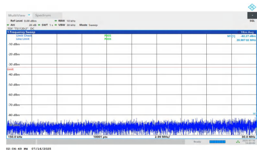
NTNV-n25-PC2-15-5-L-DFT-QPSK-Inner_1RB_Left-0.15-30-PASS
