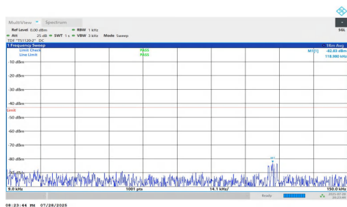
NTNV-n25-PC2-15-5-M-DFT-QPSK-Inner_1RB_Left-0.009-0.15- PASS
