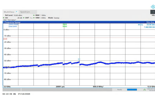
NTNV-n25-PC2-15-5-H-DFT-QPSK-Inner_1RB_Right-3000-12000-PASS
