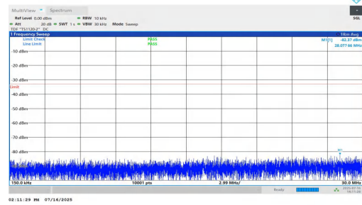
NTNV-n25-PC2-15-10-L-DFT-BPSK-Inner_1RB_Left-0.15-30-PASS
