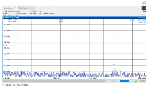
NTNV-n25-PC2-15-5-H-DFT-BPSK-Inner_1RB_Right-0.009-0.15- PASS
