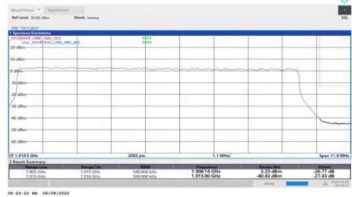
NTNV-n25-PC2-15-10-H-DFT-QPSK-Outer_Full-PASS
