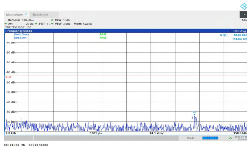
NTNV-n25-PC2-15-5-H-DFT-QPSK-Inner_1RB_Right-0.009-0.15-PASS
