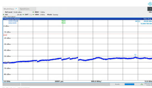
NTNV-n25-PC2-15-5-M-DFT-QPSK-Inner_1RB_Right-3000-1200 0-PASS
