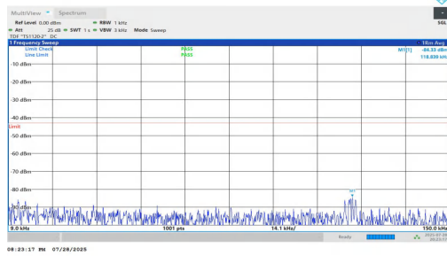
NTNV-n25-PC2-15-5-M-DFT-BPSK-Inner_1RB_Left-0.009-0.15-PASS
