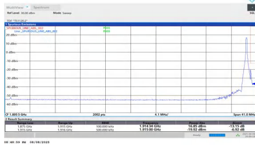
NTNV-n25-PC2-15-40-H-DFT-QPSK-Edge_1RB_Right-PASS
