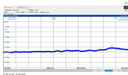
NTNV-n25-PC2-15-5-H-DFT-BPSK-Inner_1RB_Right-12000-20000-PASS
