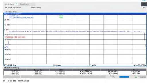
NTNV-n25-PC2-15-40-L-DFT-BPSK-Outer_Full-PASS
