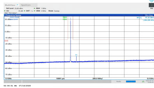
NTNV-n25-PC2-15-5-M-DFT-BPSK-Inner_1RB_Right-1000-3000-P PASS
