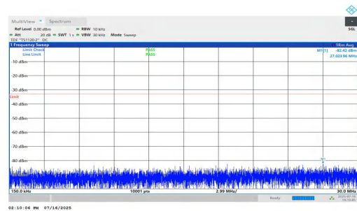
NTNV-n25-PC2-15-5-H-DFT-QPSK-Inner_1RB_Left-0.15-30-PASS
