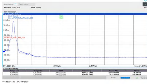
NTNV-n25-PC2-15-20-L-DFT-BPSK-Edge_1RB_Left-PASS
