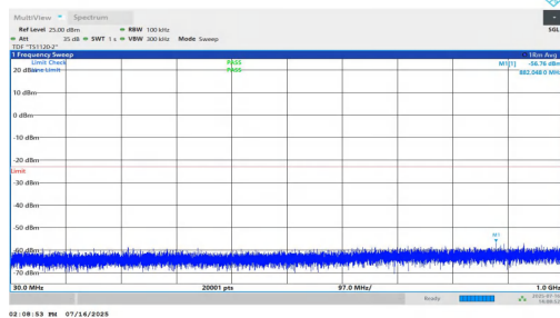
NTNV-n25-PC2-15-5-H-DFT-BPSK-Inner_1RB_Left-30-1000-P ASS
