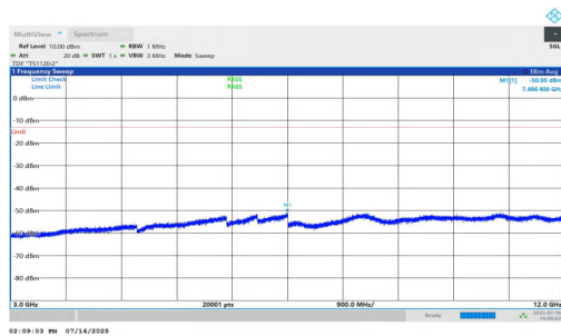
NTNV-n25-PC2-15-5-H-DFT-BPSK-Inner_1RB_Left-3000-12000- PASS
