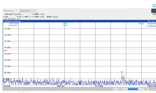
NTNV-n25-PC2-15-10-L-DFT-BPSK-Inner_1RB_Right-0.009-0.15-PASS
