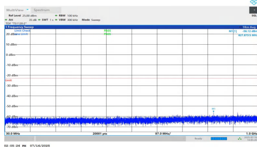
NTNV-n25-PC2-15-5-L-DFT-QPSK-Inner_1RB_Right-30-1000-PASS
