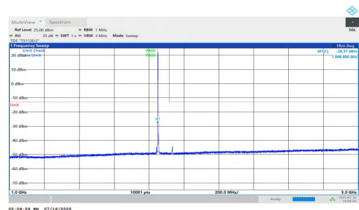
NTNV-n25-PC2-15-5-L-DFT-QPSK-Inner_1RB_Left-1000-3000-PA SS
