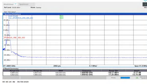
NTNV-n25-PC2-15-40-L-DFT-BPSK-Edge_1RB_Left-PASS
