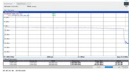
NTNV-n25-PC2-15-40-H-DFT-QPSK-Outer_Full-PASS
