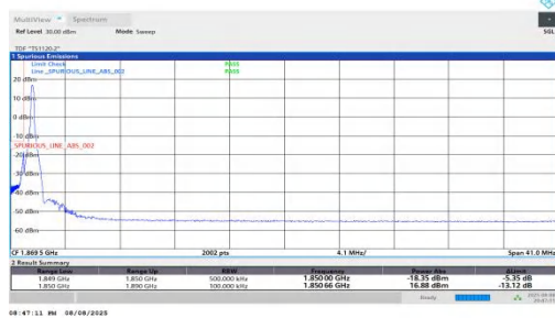
NTNV-n25-PC2-15-40-L-DFT-QPSK-Edge_1RB_Left-PASS
