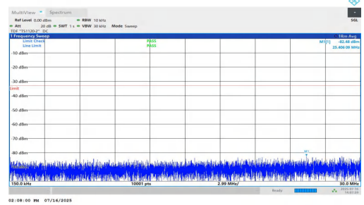
NTNV-n25-PC2-15-5-M-DFT-QPSK-Inner_1RB_Right-0.15-30-PA SS
