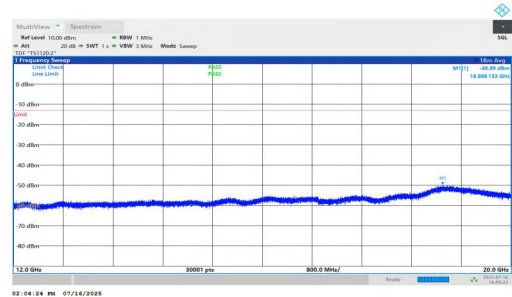
NTNV-n25-PC2-15-5-L-DFT-BPSK-Inner_1RB_Right-12000-2000 0-PASS
