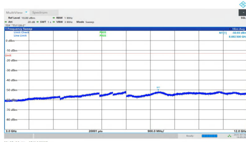
NTNV-n25-PC2-15-5-L-DFT-QPSK-Inner_1RB_Right-3000-12000-PASS
