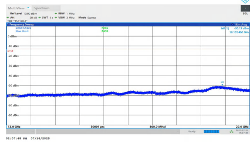
NTNV-n25-PC2-15-5-M-DFT-QPSK-Inner_1RB_Left-12000-20000 -PASS
