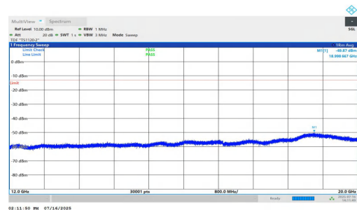
NTNV-n25-PC2-15-10-L-DFT-BPSK-Inner_1RB_Left-12000-20000-PASS
