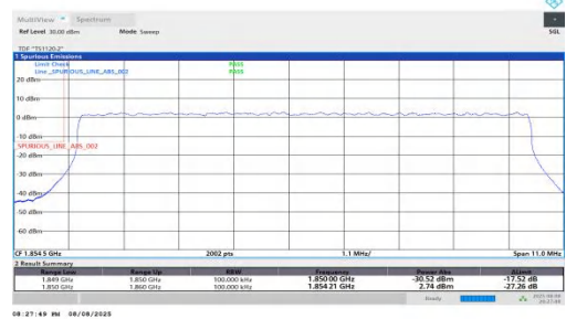
NTNV-n25-PC2-15-10-L-DFT-QPSK-Outer_Full-PASS
