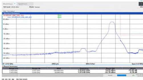
NTNV-n25-PC2-15-5-H-DFT-QPSK-Edge_1RB_Right-PASS
