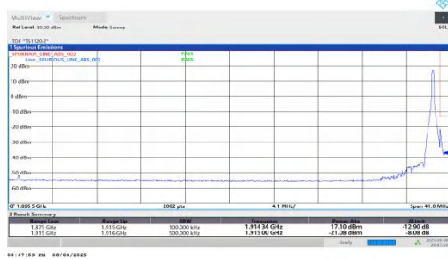
NTNV-n25-PC2-15-40-H-DFT-BPSK-Edge_1RB_Right-PASS
