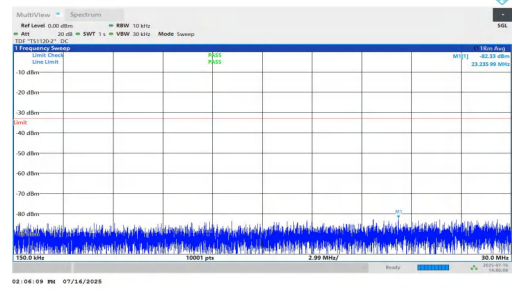
NTNV-n25-PC2-15-5-M-DFT-BPSK-Inner_1RB_Left-0.15-30-PASS
