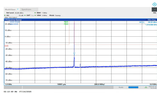
NTNV-n25-PC2-15-5-H-DFT-QPSK-Inner_1RB_Right-1000-3000-PASS
