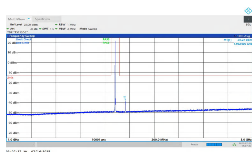
NTNV-n25-PC2-15-5-M-DFT-QPSK-Inner_1RB_Left-1000-3000-P ASS
