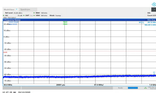
NTNV-n25-PC3-15-40-H-DFT-QPSK-Inner_1RB_Right-30-1000- PASS
