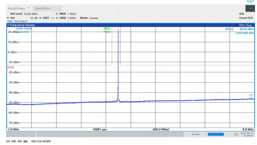
NTNV-n25-PC3-15-35-M-DFT-BPSK-Inner_1RB_Right-1000-3000-PASS
