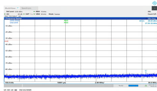
NTNV-n25-PC3-15-40-M-DFT-QPSK-Inner_1RB_Right-0.15-30-P ASS
