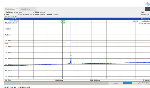
NTNV-n25-PC3-15-40-H-DFT-QPSK-Inner_1RB_Right-1000-3000- -PASS
