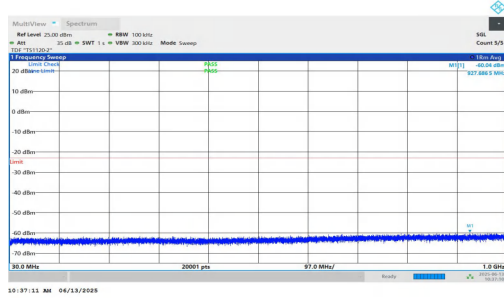
NTNV-n25-PC3-15-40-L-DFT-BPSK-Inner_1RB_Right-30-1000-P ASS
