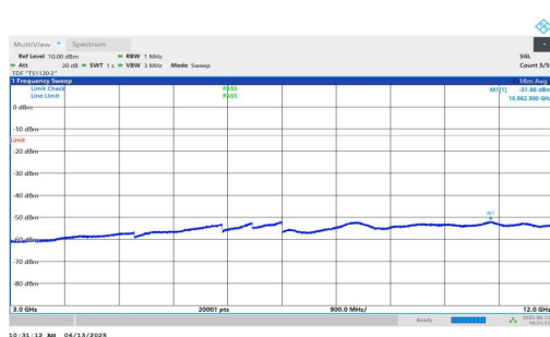
NTNV-n25-PC3-15-35-M-DFT-QPSK-Inner_1RB_Right-3000-12000-PASS
