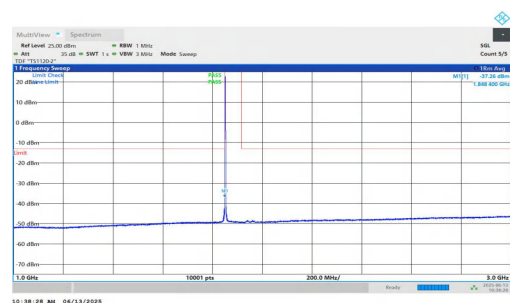
NTNV-n25-PC3-15-40-L-DFT-QPSK-Inner_1RB_Left-1000-3000-P ASS
