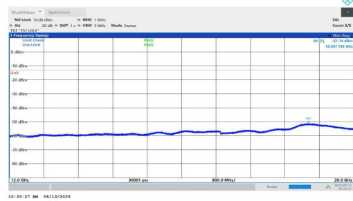
NTNV-n25-PC3-15-35-H-DFT-BPSK-Inner_1RB_Right-12000-20000-PASS
