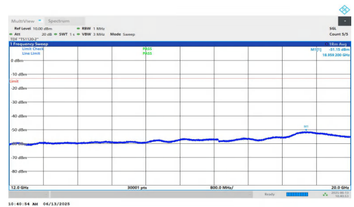
NTNV-n25-PC3-15-40-M-DFT-BPSK-Inner_1RB_Left-12000-20000-PASS
