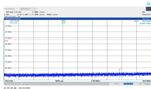
NTNV-n25-PC3-15-35-M-DFT-QPSK-Inner_1RB_Right-0.15-30-P ASS
