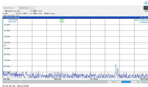
NTNV-n25-PC3-15-40-M-DFT-QPSK-Inner_1RB_Right-0.009-0.1 5-PASS
