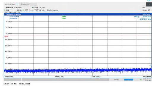
NTNV-n25-PC3-15-35-M-DFT-BPSK-Inner_1RB_Left-0.15-30-PASS
