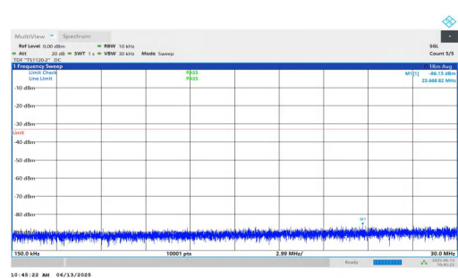
NTNV-n25-PC3-15-40-H-DFT-BPSK-Inner_1RB_Right-0.15-30-PASS
