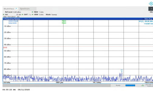
NTNV-n25-PC3-15-35-H-DFT-QPSK-Inner_1RB_Left-0.009-0.15-PASS
