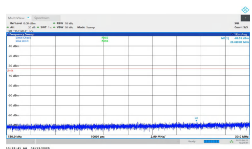
NTNV-n25-PC3-15-35-M-DFT-BPSK-Inner_1RB_Right-0.15-30-PASS
