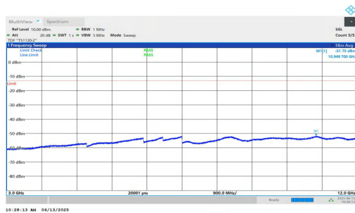
NTNV-n25-PC3-15-35-M-DFT-BPSK-Inner_1RB_Left-3000-12000-PASS
