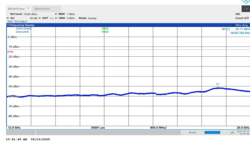
NTNV-n25-PC3-15-40-M-DFT-BPSK-Inner_1RB_Right-12000-20000-PASS
