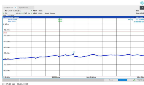
NTNV-n25-PC3-15-40-L-DFT-BPSK-Inner_1RB_Right-3000-1200 0-PASS
