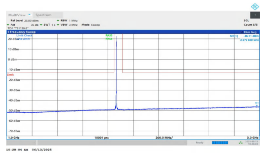
NTNV-n25-PC3-15-35-M-DFT-BPSK-Inner_1RB_Left-1000-3000-PASS
