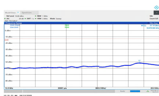
NTNV-n25-PC3-15-35-M-DFT-QPSK-Inner_1RB_Right-12000-20000-PASS
