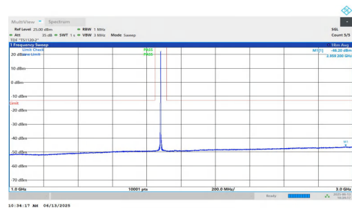
NTNV-n25-PC3-15-35-H-DFT-QPSK-Inner_1RB_Left-1000-3000-PASS
