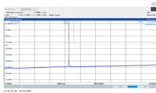
NTNV-n25-PC3-15-40-L-DFT-BPSK-Inner_1RB_Left-1000-3000-P ASS
