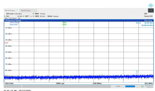
NTNV-n25-PC3-15-40-M-DFT-BPSK-Inner_1RB_Right-0.15-30-PASS
