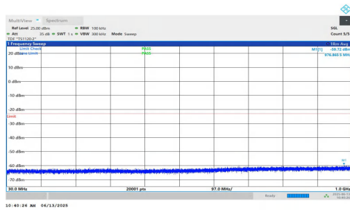
NTNV-n25-PC3-15-40-M-DFT-BPSK-Inner_1RB_Left-30-1000-PASS
