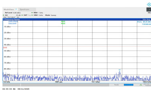
NTNV-n25-PC3-15-35-H-DFT-BPSK-Inner_1RB_Right-0.009-0.15-PASS
