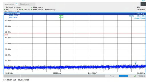
NTNV-n25-PC3-15-40-H-DFT-BPSK-Inner_1RB_Left-0.15-30-PAS
