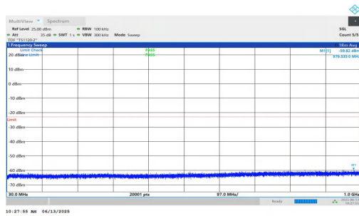
NTNV-n25-PC3-15-35-M-DFT-BPSK-Inner_1RB_Left-30-1000-PASS
