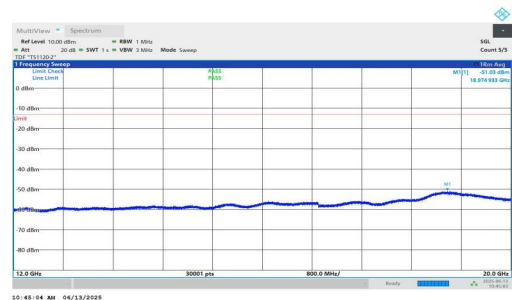
NTNV-n25-PC3-15-40-H-DFT-BPSK-Inner_1RB_Left-12000-20000-PASS
