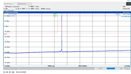
NTNV-n25-PC3-15-40-H-DFT-BPSK-Inner_1RB_Right-1000-3000-PASS
