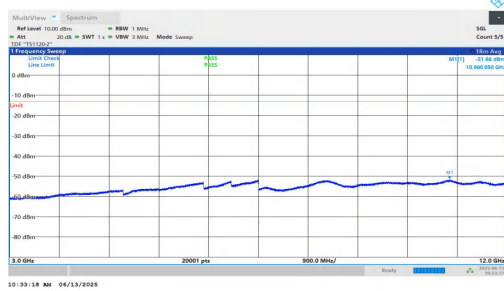
NTNV-n25-PC3-15-35-H-DFT-BPSK-Inner_1RB_Right-3000-12000-PASS
