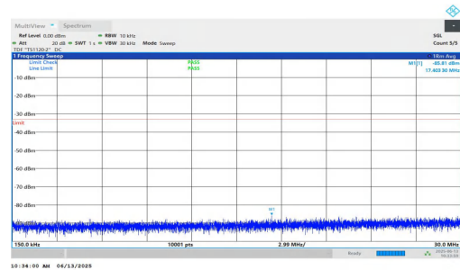
NTNV-n25-PC3-15-35-H-DFT-QPSK-Inner_1RB_Left-0.15-30-PASS
