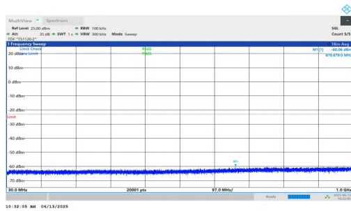
NTNV-n25-PC3-15-35-H-DFT-BPSK-Inner_1RB_Left-30-1000-PASS
