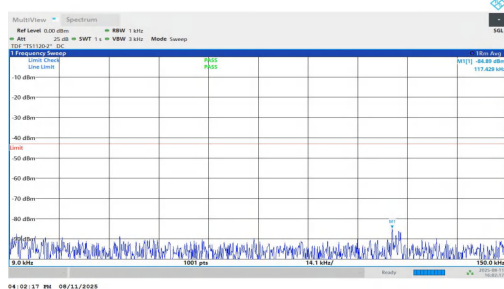
NTNV-n25-PC3-15-40-M-DFT-QPSK-Inner_1RB_Left-0.009-0.15-PASS
