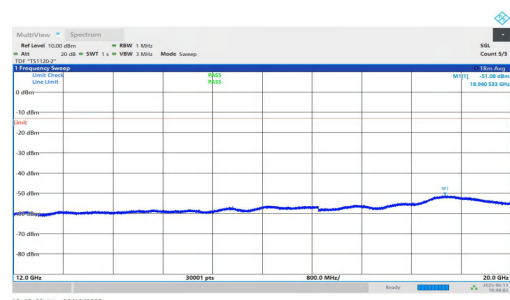
NTNV-n25-PC3-15-40-H-DFT-QPSK-Inner_1RB_Right-12000-20000- 00-PASS
