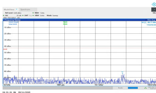
NTNV-n25-PC3-15-40-L-DFT-QPSK-Inner_1RB_Left-0.009-0.15- PASS
