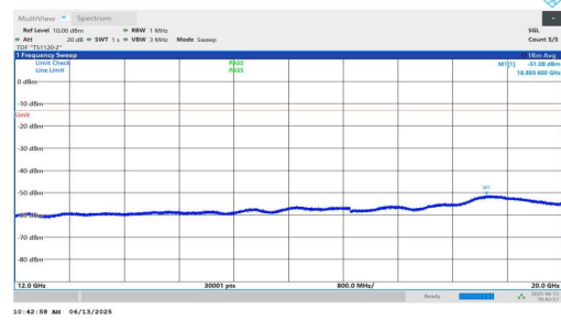
NTNV-n25-PC3-15-40-M-DFT-QPSK-Inner_1RB_Left-12000-2000 0-PASS
