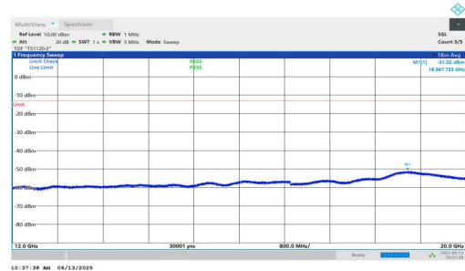
NTNV-n25-PC3-15-40-L-DFT-BPSK-Inner_1RB_Right-12000-200 00-PASS
