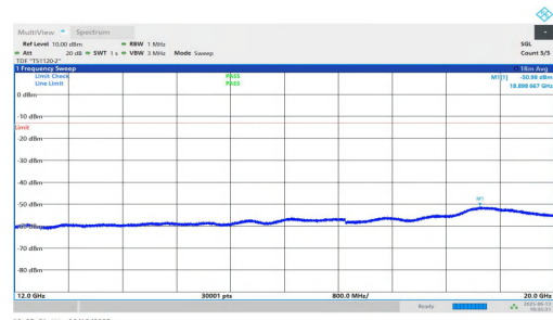
NTNV-n25-PC3-15-35-H-DFT-QPSK-Inner_1RB_Right-12000-20000-PASS
