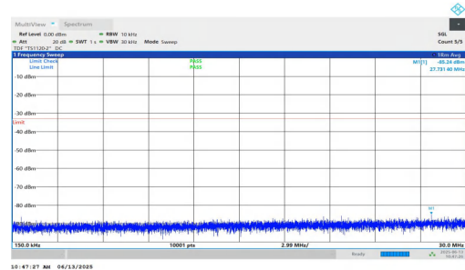
NTNV-n25-PC3-15-40-H-DFT-QPSK-Inner_1RB_Right-0.15-30-PA SS
