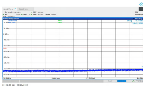
NTNV-n25-PC3-15-35-H-DFT-QPSK-Inner_1RB_Left-30-1000-PASS
