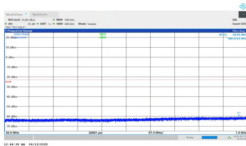
NTNV-n25-PC3-15-40-H-DFT-BPSK-Inner_1RB_Left-30-1000-PASS
