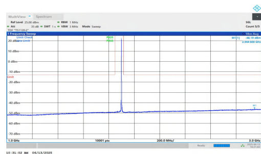
NTNV-n25-PC3-15-35-M-DFT-QPSK-Inner_1RB_Right-1000-3000-PASS
