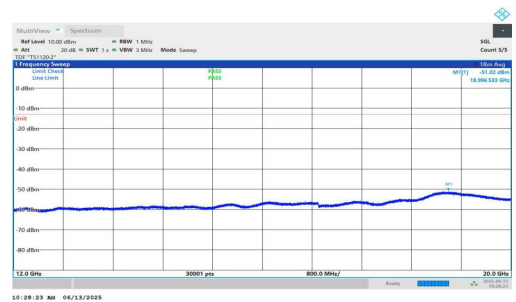
NTNV-n25-PC3-15-35-M-DFT-BPSK-Inner_1RB_Left-12000-20000-PASS
