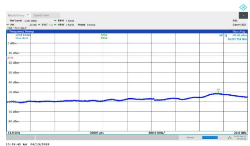
NTNV-n25-PC3-15-40-L-DFT-QPSK-Inner_1RB_Right-12000-20000-00-PASS
