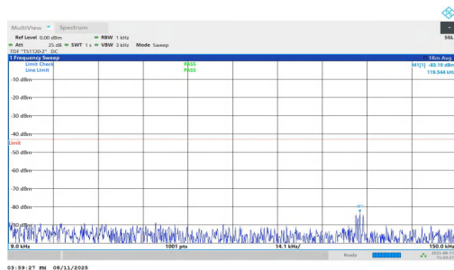
NTNV-n25-PC3-15-35-M-DFT-QPSK-Inner_1RB_Left-0.009-0.15-PASS
