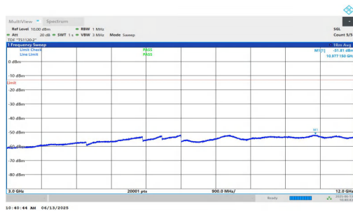
NTNV-n25-PC3-15-40-M-DFT-BPSK-Inner_1RB_Left-3000-12000-PASS
