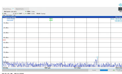
NTNV-n25-PC3-15-40-L-DFT-BPSK-Inner_1RB_Right-0.009-0.15 -PASS
