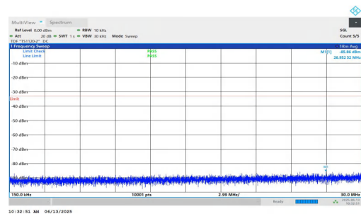
NTNV-n25-PC3-15-35-H-DFT-BPSK-Inner_1RB_Right-0.15-30-PASS
