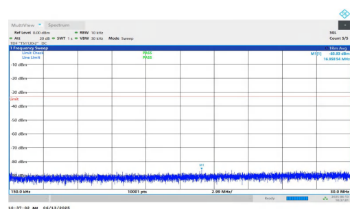
NTNV-n25-PC3-15-40-L-DFT-BPSK-Inner_1RB_Right-0.15-30-PASS SS
