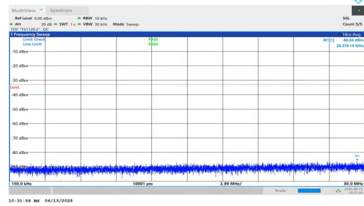
NTNV-n25-PC3-15-35-H-DFT-BPSK-Inner_1RB_Left-0.15-30-PAS
