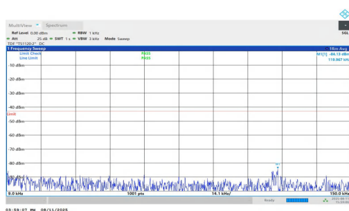
NTNV-n25-PC3-15-35-M-DFT-BPSK-Inner_1RB_Right-0.009-0.15-PASS
