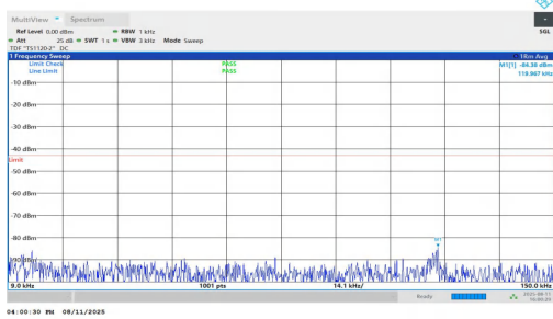
NTNV-n25-PC3-15-35-H-DFT-QPSK-Inner_1RB_Right-0.009-0.1 5-PASS
