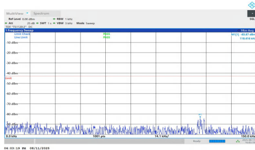
NTNV-n25-PC3-15-40-H-DFT-QPSK-Inner_1RB_Right-0.009-0.1 5-PASS
