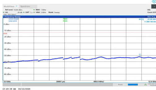
NTNV-n25-PC3-15-35-M-DFT-BPSK-Inner_1RB_Right-3000-12000-PASS
