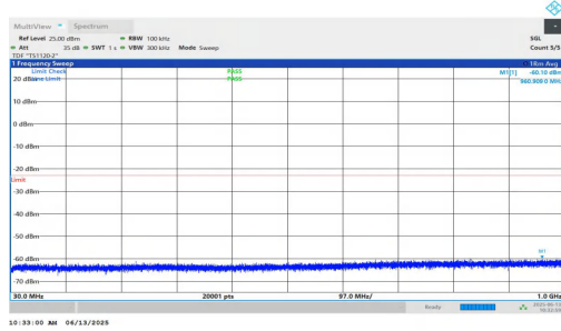
NTNV-n25-PC3-15-35-H-DFT-BPSK-Inner_1RB_Right-30-1000-PASS
