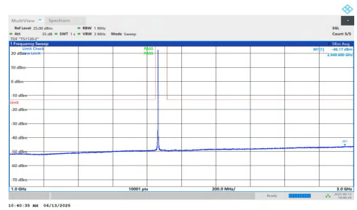
NTNV-n25-PC3-15-40-M-DFT-BPSK-Inner_1RB_Left-1000-3000-PASS
