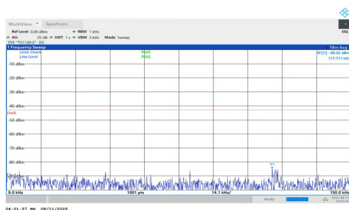
NTNV-n25-PC3-15-40-M-DFT-BPSK-Inner_1RB_Right-0.009-0.15-PASS
