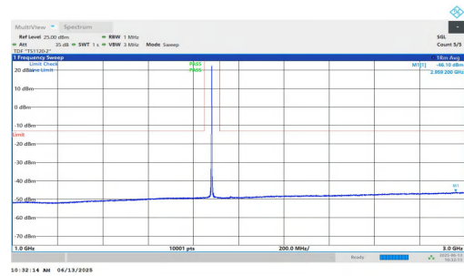
NTNV-n25-PC3-15-35-H-DFT-BPSK-Inner_1RB_Left-1000-3000-PASS
