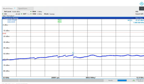
NTNV-n25-PC3-15-35-H-DFT-QPSK-Inner_1RB_Right-3000-12000-PASS
