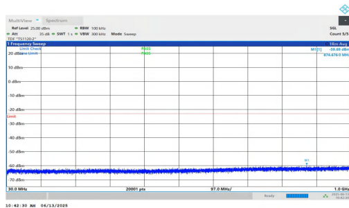
NTNV-n25-PC3-15-40-M-DFT-QPSK-Inner_1RB_Left-30-1000-PASS
