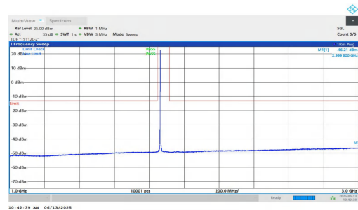
NTNV-n25-PC3-15-40-M-DFT-QPSK-Inner_1RB_Left-1000-3000-PASS
