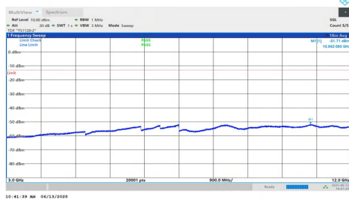
NTNV-n25-PC3-15-40-M-DFT-BPSK-Inner_1RB_Right-3000-12000-PASS
