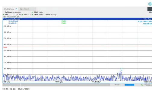
NTNV-n25-PC3-15-35-M-DFT-QPSK-Inner_1RB_Right-0.009-0.1 5-PASS
