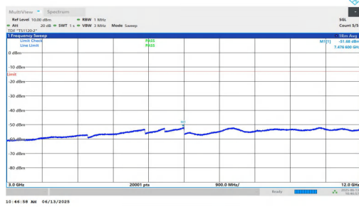
NTNV-n25-PC3-15-40-H-DFT-QPSK-Inner_1RB_Left-3000-1200 0-PASS
