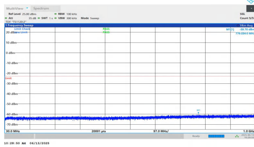
NTNV-n25-PC3-15-35-M-DFT-BPSK-Inner_1RB_Right-30-1000-PASS
