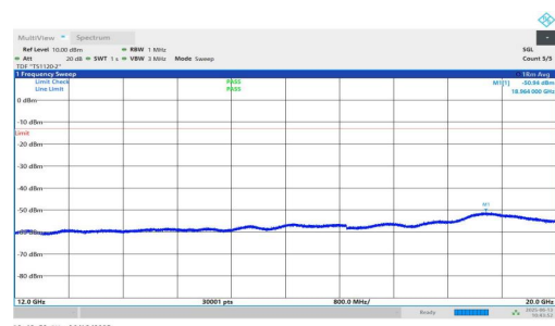
NTNV-n25-PC3-15-40-M-DFT-QPSK-Inner_1RB_Right-12000-20000- 00-PASS
