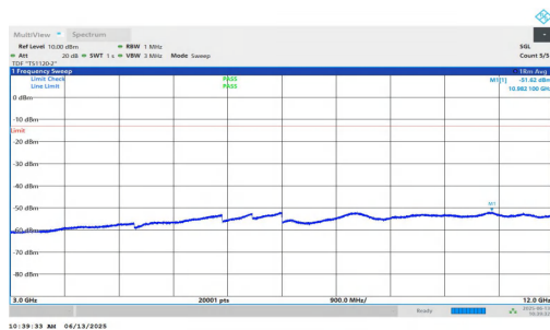
NTNV-n25-PC3-15-40-L-DFT-QPSK-Inner_1RB_Right-3000-12000-00-PASS
