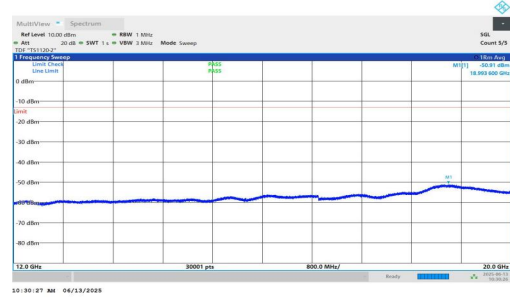
NTNV-n25-PC3-15-35-M-DFT-QPSK-Inner_1RB_Left-12000-2000 0-PASS
