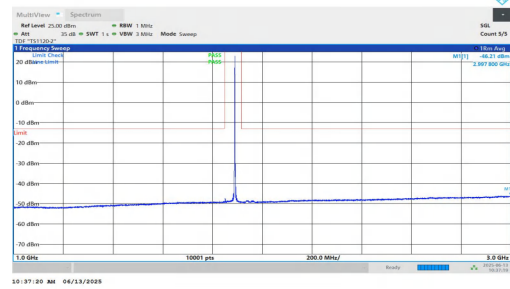
NTNV-n25-PC3-15-40-L-DFT-BPSK-Inner_1RB_Right-1000-3000-P PASS
