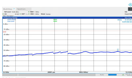
NTNV-n25-PC3-15-40-M-DFT-QPSK-Inner_1RB_Right-3000-12000- 00-PASS
