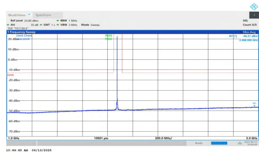
NTNV-n25-PC3-15-40-H-DFT-BPSK-Inner_1RB_Left-1000-3000-PASS
