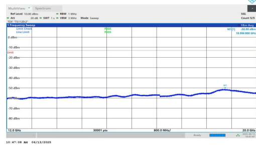
NTNV-n25-PC3-15-40-H-DFT-QPSK-Inner_1RB_Left-12000-2000 0-PASS
