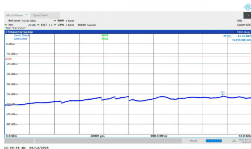
NTNV-n25-PC3-15-40-H-DFT-BPSK-Inner_1RB_Left-3000-12000-PASS
