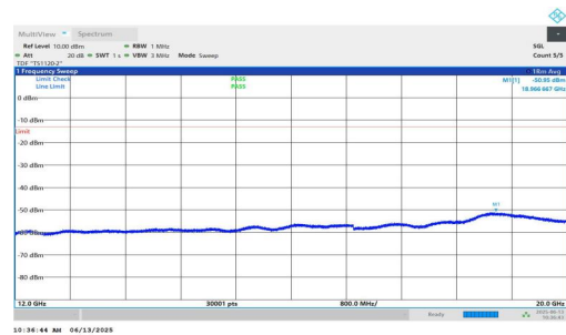
NTNV-n25-PC3-15-40-L-DFT-BPSK-Inner_1RB_Left-12000-20000 -PASS
