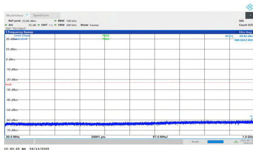
NTNV-n25-PC3-15-40-M-DFT-QPSK-Inner_1RB_Right-30-1000- PASS
