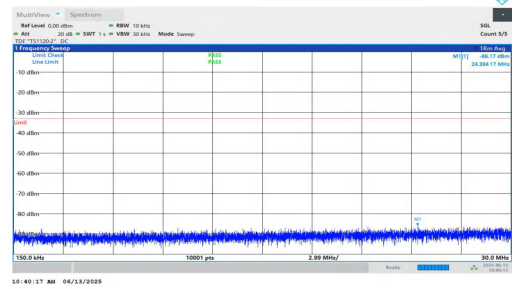
NTNV-n25-PC3-15-40-M-DFT-BPSK-Inner_1RB_Left-0.15-30-PASS
