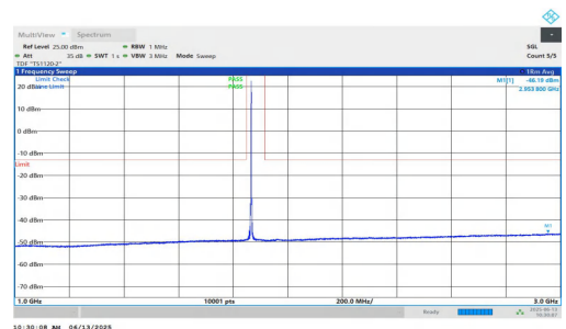
NTNV-n25-PC3-15-35-M-DFT-QPSK-Inner_1RB_Left-1000-3000-PASS
