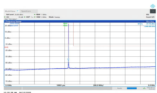
NTNV-n25-PC3-15-35-L-DFT-QPSK-Inner_1RB_Left-1000-3000-P ASS
