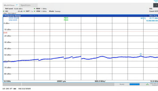
NTNV-n25-PC3-15-35-L-DFT-QPSK-Inner_1RB_Left-3000-12000 -PASS
