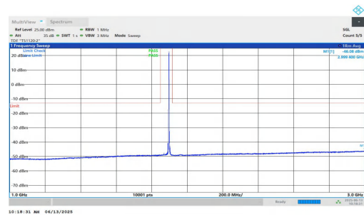
NTNV-n25-PC3-15-30-M-DFT-QPSK-Inner_1RB_Right-1000-3000- -PASS
