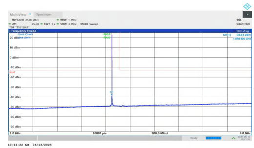
NTNV-n25-PC3-15-30-L-DFT-BPSK-Inner_1RB_Left-1000-3000-PASS ASS
