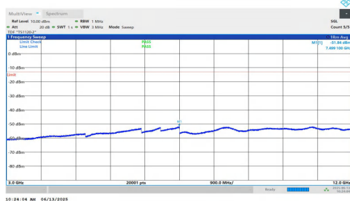
NTNV-n25-PC3-15-35-L-DFT-BPSK-Inner_1RB_Left-3000-12000 -PASS
