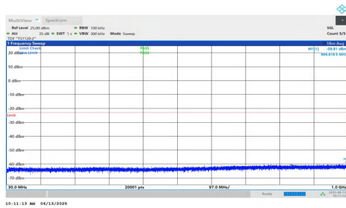
NTNV-n25-PC3-15-30-L-DFT-BPSK-Inner_1RB_Left-30-1000-PASS SS
