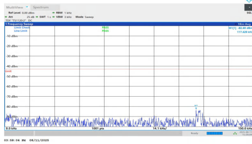
NTNV-n25-PC3-15-35-L-DFT-BPSK-Inner_1RB_Left-0.009-0.15- PASS
