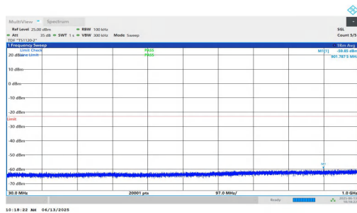
NTNV-n25-PC3-15-30-M-DFT-QPSK-Inner_1RB_Right-30-1000- PASS
