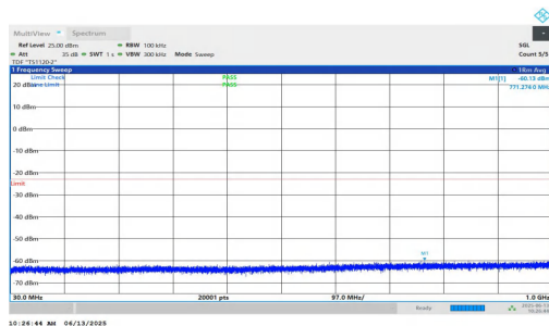
NTNV-n25-PC3-15-35-L-DFT-QPSK-Inner_1RB_Right-30-1000-P ASS
