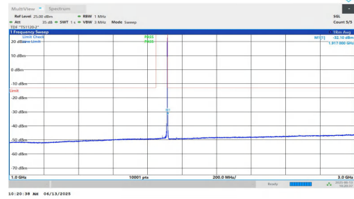
NTNV-n25-PC3-15-30-H-DFT-BPSK-Inner_1RB_Right-1000-3000-PASS
