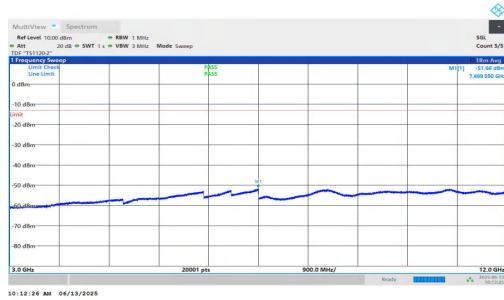
NTNV-n25-PC3-15-30-L-DFT-BPSK-Inner_1RB_Right-3000-1200 0-PASS
