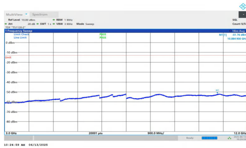
NTNV-n25-PC3-15-35-L-DFT-BPSK-Inner_1RB_Right-3000-1200 0-PASS
