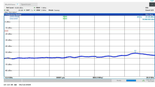
NTNV-n25-PC3-15-30-L-DFT-QPSK-Inner_1RB_Left-12000-2000 0-PASS
