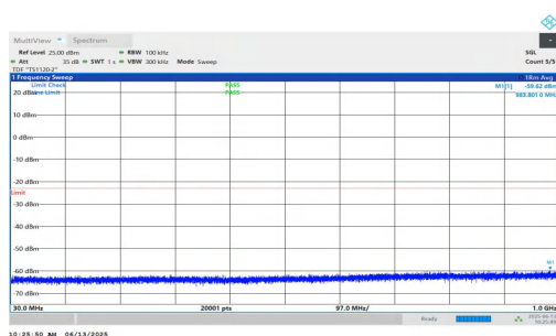
NTNV-n25-PC3-15-35-L-DFT-QPSK-Inner_1RB_Left-30-1000-PA SS
