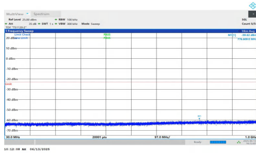
NTNV-n25-PC3-15-30-L-DFT-BPSK-Inner_1RB_Right-30-1000-P ASS
