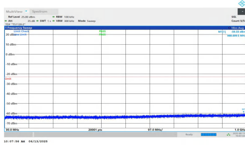
NTNV-n25-PC3-15-25-H-DFT-BPSK-Inner_1RB_Right-30-1000-P ASS
