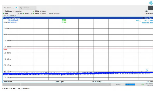
NTNV-n25-PC3-15-30-M-DFT-BPSK-Inner_1RB_Right-30-1000-PASS
