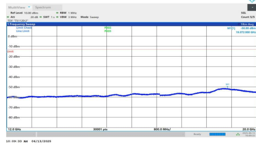
NTNV-n25-PC3-15-25-H-DFT-QPSK-Inner_1RB_Left-12000-2000 0-PASS
