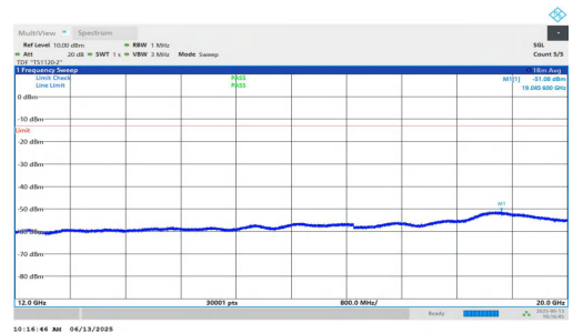
NTNV-n25-PC3-15-30-M-DFT-BPSK-Inner_1RB_Right-12000-20000-PASS
