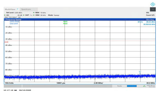
NTNV-n25-PC3-15-30-M-DFT-QPSK-Inner_1RB_Left-0.15-30-PASS
