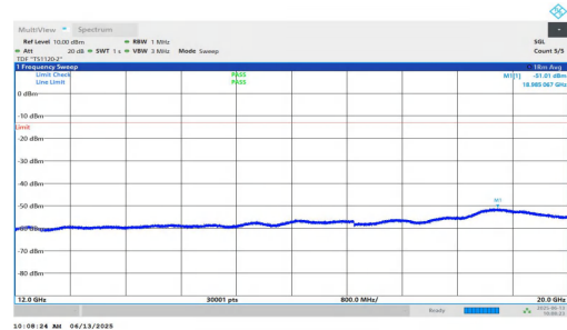
NTNV-n25-PC3-15-25-H-DFT-BPSK-Inner_1RB_Right-12000-200 00-PASS
