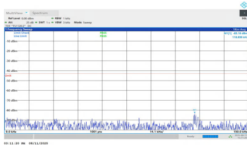
NTNV-n25-PC3-15-30-M-DFT-QPSK-Inner_1RB_Right-0.009-0.1 5-PASS
