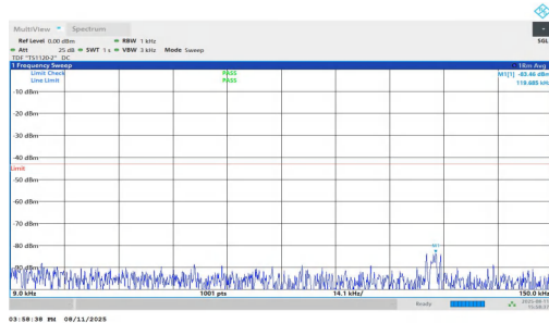
NTNV-n25-PC3-15-35-L-DFT-QPSK-Inner_1RB_Right-0.009-0.1 5-PASS
