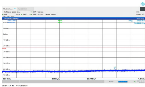
NTNV-n25-PC3-15-30-L-DFT-QPSK-Inner_1RB_Right-30-1000-P ASS
