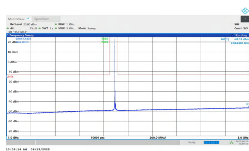
NTNV-n25-PC3-15-25-H-DFT-QPSK-Inner_1RB_Left-1000-3000- PASS
