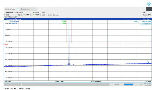
NTNV-n25-PC3-15-30-L-DFT-QPSK-Inner_1RB_Right-1000-3000-P PASS
