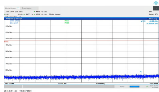
NTNV-n25-PC3-15-30-L-DFT-QPSK-Inner_1RB_Right-0.15-30-PA SS
