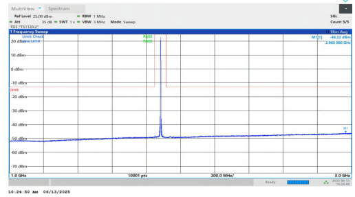
NTNV-n25-PC3-15-35-L-DFT-BPSK-Inner_1RB_Right-1000-3000-P PASS
