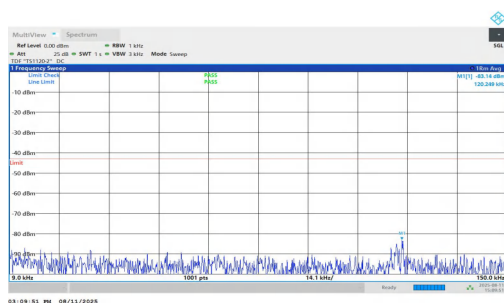
NTNV-n25-PC3-15-30-L-DFT-BPSK-Inner_1RB_Right-0.009-0.15 -PASS
