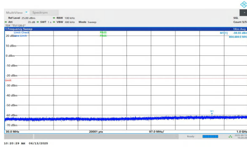
NTNV-n25-PC3-15-30-H-DFT-BPSK-Inner_1RB_Right-30-1000-PASS
