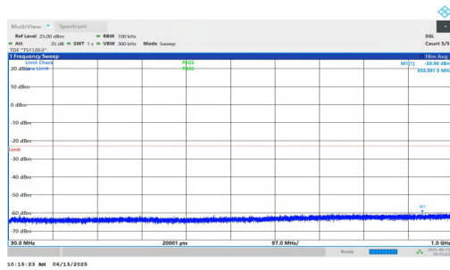
NTNV-n25-PC3-15-30-M-DFT-BPSK-Inner_1RB_Left-30-1000-PASS
