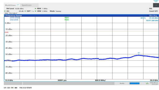
NTNV-n25-PC3-15-30-H-DFT-QPSK-Inner_1RB_Left-12000-2000 0-PASS
