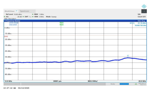
NTNV-n25-PC3-15-35-L-DFT-QPSK-Inner_1RB_Right-12000-200 00-PASS
