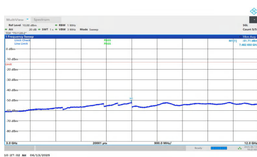
NTNV-n25-PC3-15-35-L-DFT-QPSK-Inner_1RB_Right-3000-120 00-PASS
