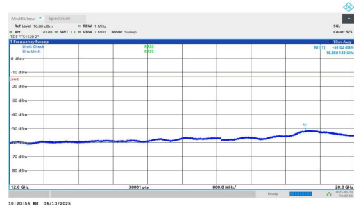
NTNV-n25-PC3-15-30-H-DFT-BPSK-Inner_1RB_Right-12000-20000-PASS
