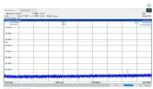
NTNV-n25-PC3-15-25-H-DFT-BPSK-Inner_1RB_Right-0.15-30-PASS SS
