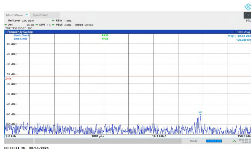
NTNV-n25-PC3-15-25-H-DFT-QPSK-Inner_1RB_Left-0.009-0.15- PASS
