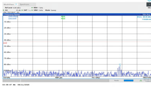
NTNV-n25-PC3-15-25-H-DFT-BPSK-Inner_1RB_Left-0.009-0.15-PASS
