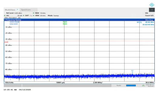
NTNV-n25-PC3-15-35-L-DFT-QPSK-Inner_1RB_Left-0.15-30-PAS S
