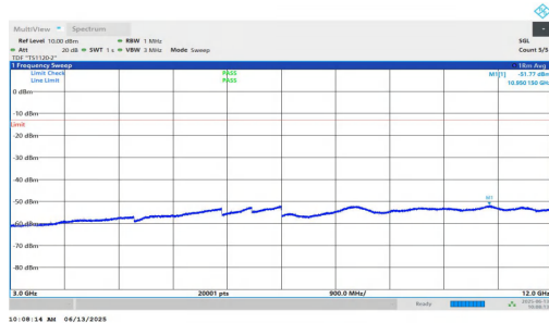
NTNV-n25-PC3-15-25-H-DFT-BPSK-Inner_1RB_Right-3000-120 00-PASS
