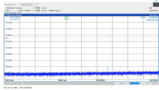
NTNV-n25-PC3-15-30-M-DFT-BPSK-Inner_1RB_Left-0.15-30-PASS
