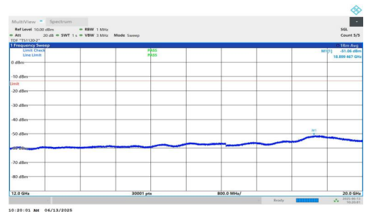
NTNV-n25-PC3-15-30-H-DFT-BPSK-Inner_1RB_Left-12000-20000-PASS
