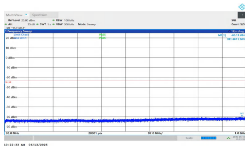
NTNV-n25-PC3-15-30-H-DFT-QPSK-Inner_1RB_Right-30-1000- PASS
