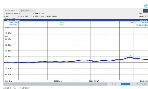
NTNV-n25-PC3-15-30-M-DFT-QPSK-Inner_1RB_Right-12000-20000- 00-PASS
