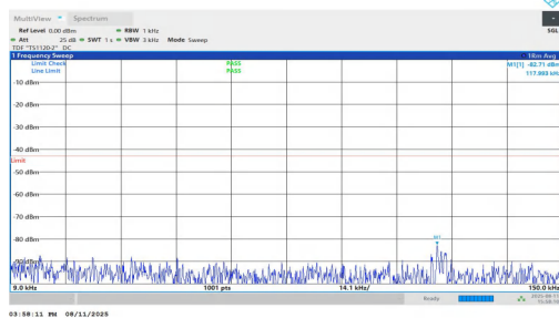
NTNV-n25-PC3-15-35-L-DFT-BPSK-Inner_1RB_Right-0.009-0.15 -PASS
