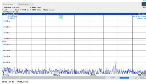
NTNV-n25-PC3-15-30-H-DFT-BPSK-Inner_1RB_Left-0.009-0.15-PASS
