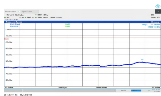
NTNV-n25-PC3-15-30-L-DFT-QPSK-Inner_1RB_Right-12000-20000 00-PASS
