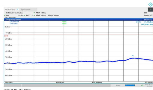
NTNV-n25-PC3-15-25-H-DFT-QPSK-Inner_1RB_Right-12000-20000-PASS
