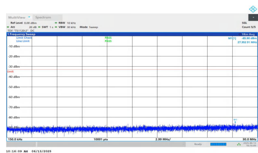
NTNV-n25-PC3-15-30-M-DFT-BPSK-Inner_1RB_Right-0.15-30-PASS
