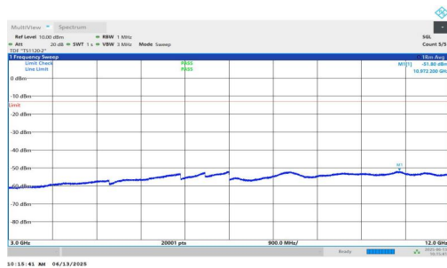
NTNV-n25-PC3-15-30-M-DFT-BPSK-Inner_1RB_Left-3000-12000-PASS
