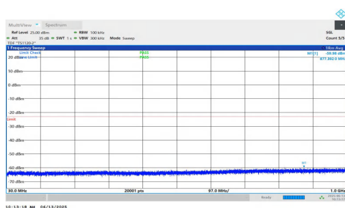
NTNV-n25-PC3-15-30-L-DFT-QPSK-Inner_1RB_Left-30-1000-PA SS
