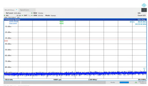
NTNV-n25-PC3-15-30-H-DFT-BPSK-Inner_1RB_Right-0.15-30-PASS
