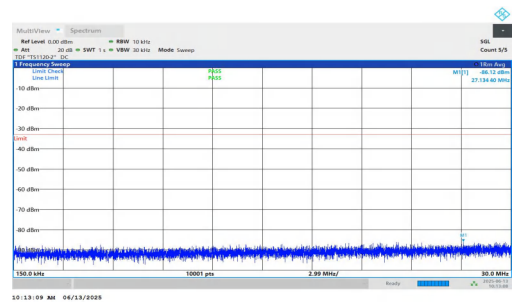
NTNV-n25-PC3-15-30-L-DFT-QPSK-Inner_1RB_Left-0.15-30-PAS S
