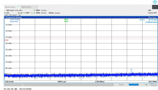
NTNV-n25-PC3-15-30-H-DFT-QPSK-Inner_1RB_Right-0.15-30-PA SS
