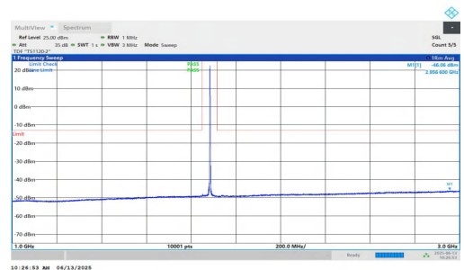
NTNV-n25-PC3-15-35-L-DFT-QPSK-Inner_1RB_Right-1000-3000- PASS
