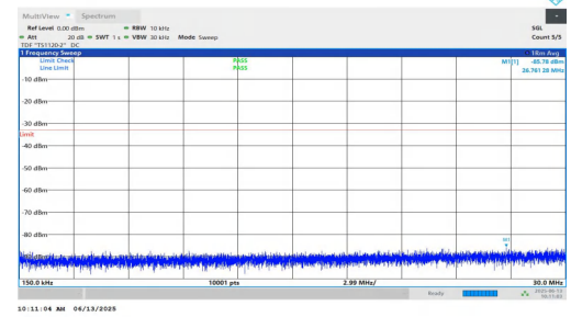
NTNV-n25-PC3-15-30-L-DFT-BPSK-Inner_1RB_Left-0.15-30-PAS S
