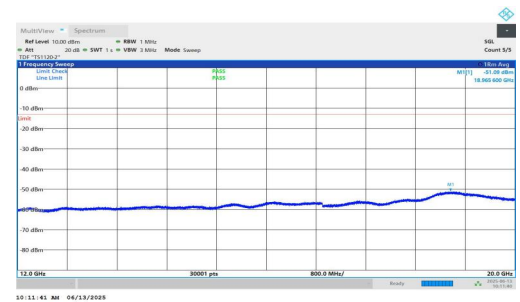
NTNV-n25-PC3-15-30-L-DFT-BPSK-Inner_1RB_Left-12000-20000 -PASS
