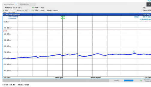
NTNV-n25-PC3-15-25-H-DFT-QPSK-Inner_1RB_Left-3000-1200 0-PASS
