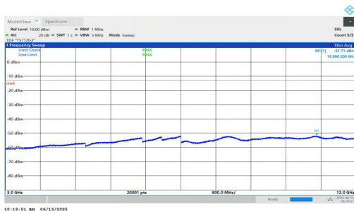
NTNV-n25-PC3-15-30-H-DFT-BPSK-Inner_1RB_Left-3000-12000-PASS
