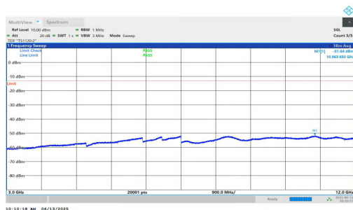
NTNV-n25-PC3-15-25-H-DFT-QPSK-Inner_1RB_Right-3000-12000-PASS
