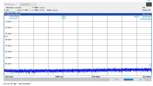
NTNV-n25-PC3-15-30-H-DFT-BPSK-Inner_1RB_Left-0.15-30-PASS
