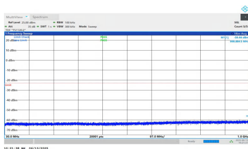
NTNV-n25-PC3-15-30-H-DFT-QPSK-Inner_1RB_Left-30-1000-PASS
