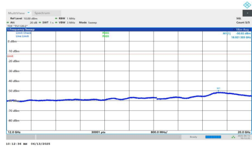
NTNV-n25-PC3-15-30-L-DFT-BPSK-Inner_1RB_Right-12000-200 00-PASS
