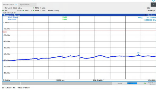
NTNV-n25-PC3-15-30-L-DFT-QPSK-Inner_1RB_Left-3000-12000 -PASS
