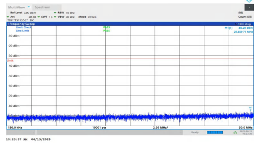
NTNV-n25-PC3-15-35-L-DFT-BPSK-Inner_1RB_Left-0.15-30-PAS S
