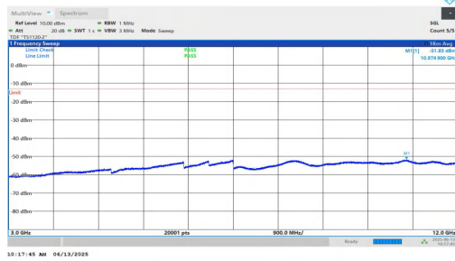
NTNV-n25-PC3-15-30-M-DFT-QPSK-Inner_1RB_Left-3000-1200 0-PASS
