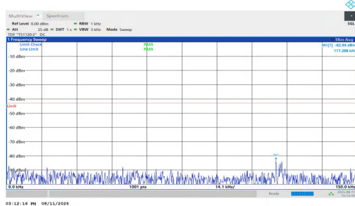
NTNV-n25-PC3-15-30-H-DFT-QPSK-Inner_1RB_Right-0.009-0.1 5-PASS
