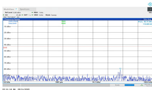
NTNV-n25-PC3-15-30-M-DFT-QPSK-Inner_1RB_Left-0.009-0.15-PASS
