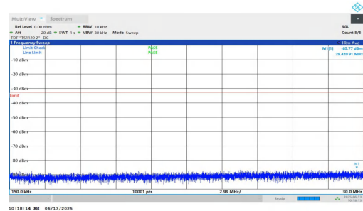
NTNV-n25-PC3-15-30-M-DFT-QPSK-Inner_1RB_Right-0.15-30-P ASS
