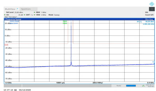
NTNV-n25-PC3-15-25-H-DFT-BPSK-Inner_1RB_Left-1000-3000-PASS ASS
