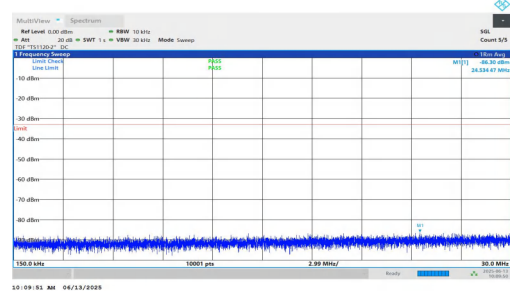
NTNV-n25-PC3-15-25-H-DFT-QPSK-Inner_1RB_Right-0.15-30-PA SS
