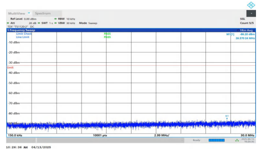
NTNV-n25-PC3-15-35-L-DFT-QPSK-Inner_1RB_Right-0.15-30-PA SS
