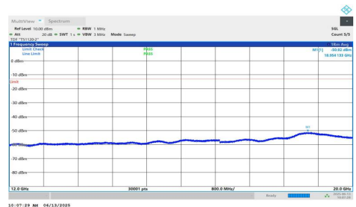
NTNV-n25-PC3-15-25-H-DFT-BPSK-Inner_1RB_Left-12000-20000-PASS 0-PASS
