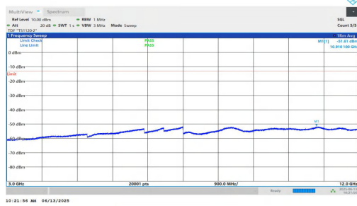
NTNV-n25-PC3-15-30-H-DFT-QPSK-Inner_1RB_Left-3000-1200 0-PASS
