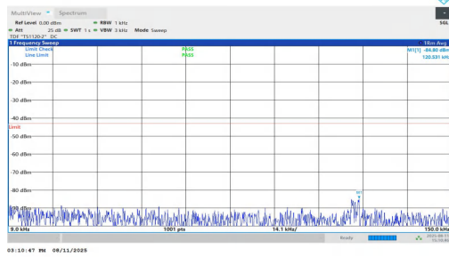
NTNV-n25-PC3-15-30-M-DFT-BPSK-Inner_1RB_Left-0.009-0.15-PASS
