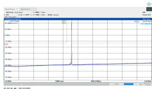
NTNV-n25-PC3-15-30-H-DFT-QPSK-Inner_1RB_Right-1000-3000- -PASS
