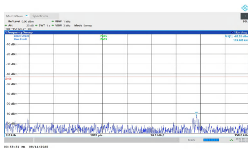
NTNV-n25-PC3-15-35-L-DFT-QPSK-Inner_1RB_Left-0.009-0.15- PASS
