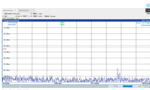
NTNV-n25-PC3-15-30-H-DFT-BPSK-Inner_1RB_Right-0.009-0.15-PASS
