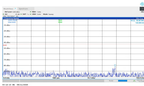
NTNV-n25-PC3-15-30-H-DFT-QPSK-Inner_1RB_Left-0.009-0.15-PASS
