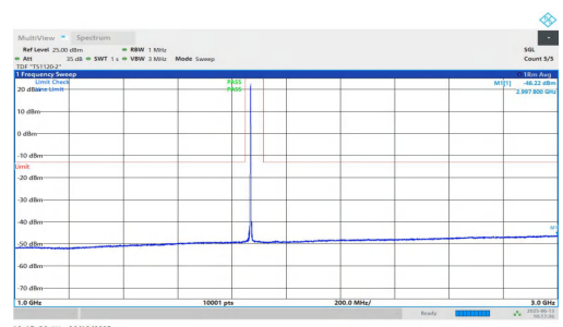
NTNV-n25-PC3-15-30-M-DFT-QPSK-Inner_1RB_Left-1000-3000-PASS
