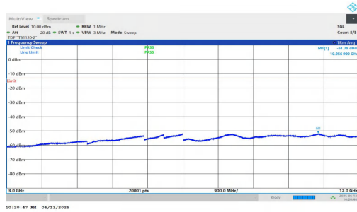
NTNV-n25-PC3-15-30-H-DFT-BPSK-Inner_1RB_Right-3000-12000-PASS
