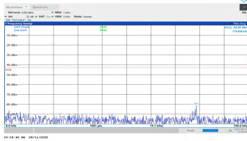
NTNV-n25-PC3-15-30-L-DFT-BPSK-Inner_1RB_Left-0.009-0.15- PASS
