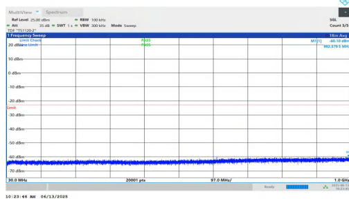
NTNV-n25-PC3-15-35-L-DFT-BPSK-Inner_1RB_Left-30-1000-PA SS
