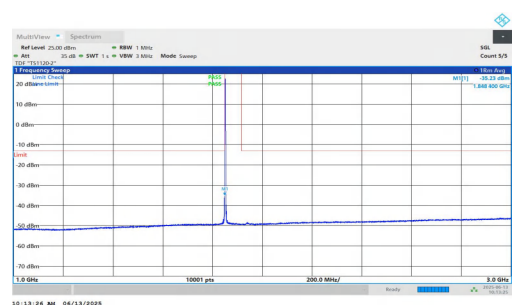
NTNV-n25-PC3-15-30-L-DFT-QPSK-Inner_1RB_Left-1000-3000-P ASS
