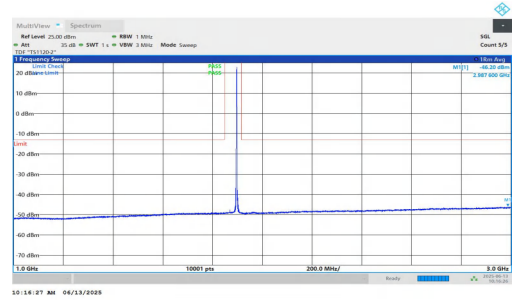
NTNV-n25-PC3-15-30-M-DFT-BPSK-Inner_1RB_Right-1000-3000-PASS
