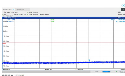
NTNV-n25-PC3-15-25-H-DFT-QPSK-Inner_1RB_Left-30-1000-P ASS
