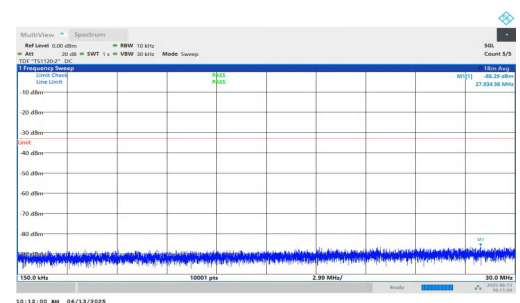
NTNV-n25-PC3-15-30-L-DFT-BPSK-Inner_1RB_Right-0.15-30-PASS SS
