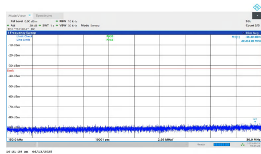
NTNV-n25-PC3-15-30-H-DFT-QPSK-Inner_1RB_Left-0.15-30-PASS
