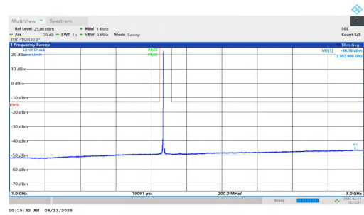
NTNV-n25-PC3-15-30-M-DFT-BPSK-Inner_1RB_Left-1000-3000-PASS
