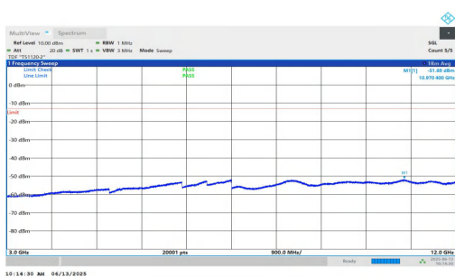
NTNV-n25-PC3-15-30-L-DFT-QPSK-Inner_1RB_Right-3000-12000 00-PASS
