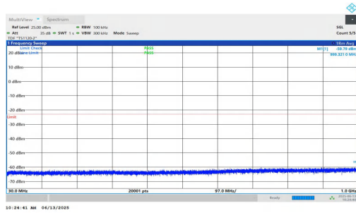
NTNV-n25-PC3-15-35-L-DFT-BPSK-Inner_1RB_Right-30-1000-P ASS
