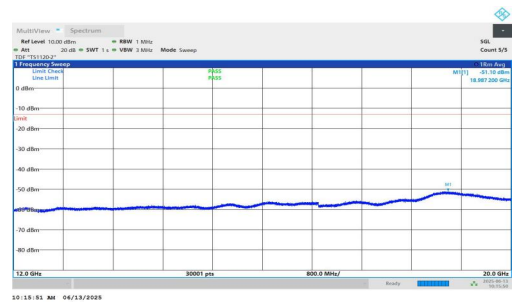
NTNV-n25-PC3-15-30-M-DFT-BPSK-Inner_1RB_Left-12000-20000-PASS
