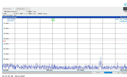
NTNV-n25-PC3-15-30-M-DFT-BPSK-Inner_1RB_Right-0.009-0.15-PASS
