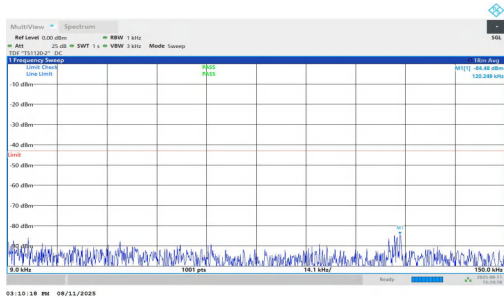
NTNV-n25-PC3-15-30-L-DFT-QPSK-Inner_1RB_Right-0.009-0.1 5-PASS
