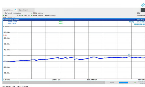
NTNV-n25-PC3-15-30-H-DFT-QPSK-Inner_1RB_Right-3000-12000- 00-PASS
