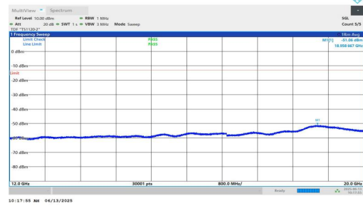
NTNV-n25-PC3-15-30-M-DFT-QPSK-Inner_1RB_Left-12000-2000 0-PASS
