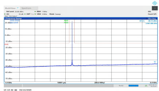
NTNV-n25-PC3-15-30-H-DFT-BPSK-Inner_1RB_Left-1000-3000-PASS
