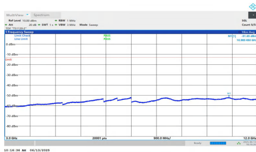
NTNV-n25-PC3-15-30-M-DFT-BPSK-Inner_1RB_Right-3000-12000-PASS
