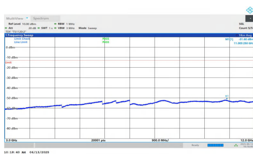
NTNV-n25-PC3-15-30-M-DFT-QPSK-Inner_1RB_Right-3000-12000- 00-PASS
