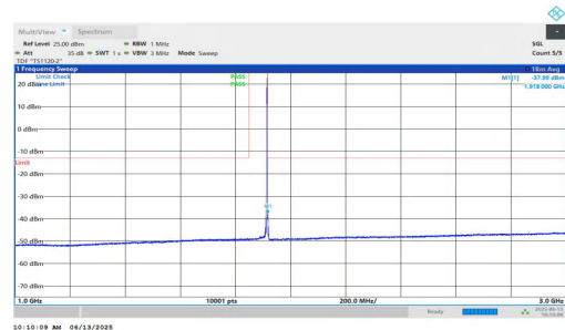
NTNV-n25-PC3-15-25-H-DFT-QPSK-Inner_1RB_Right-1000-3000-PASS
