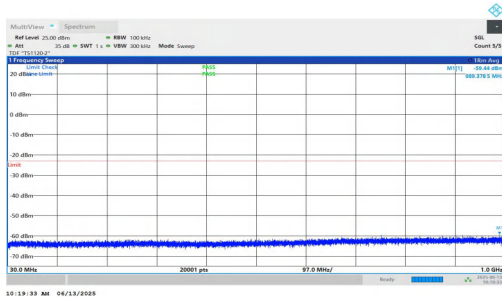
NTNV-n25-PC3-15-30-H-DFT-BPSK-Inner_1RB_Left-30-1000-PASS
