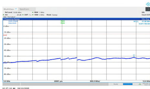
NTNV-n25-PC3-15-25-H-DFT-BPSK-Inner_1RB_Left-3000-12000-PASS 0-PASS
