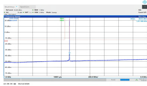
NTNV-n25-PC3-15-25-H-DFT-BPSK-Inner_1RB_Right-1000-3000-P PASS
