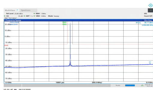
NTNV-n25-PC3-15-30-H-DFT-QPSK-Inner_1RB_Left-1000-3000-PASS
