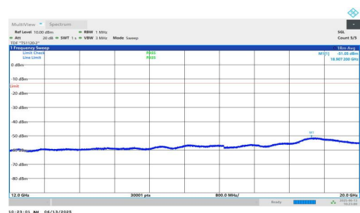
NTNV-n25-PC3-15-30-H-DFT-QPSK-Inner_1RB_Right-12000-20000- 00-PASS
