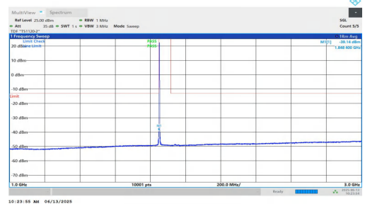
NTNV-n25-PC3-15-35-L-DFT-BPSK-Inner_1RB_Left-1000-3000-P ASS
