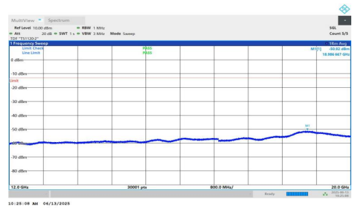
NTNV-n25-PC3-15-35-L-DFT-BPSK-Inner_1RB_Right-12000-200 00-PASS
