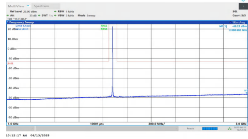
NTNV-n25-PC3-15-30-L-DFT-BPSK-Inner_1RB_Right-1000-3000-P PASS
