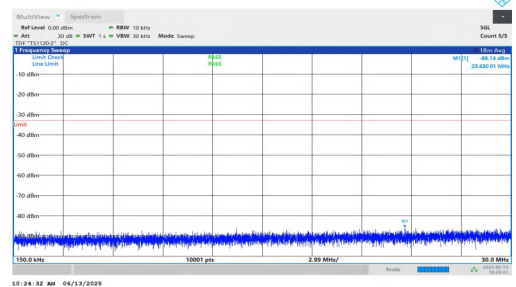
NTNV-n25-PC3-15-35-L-DFT-BPSK-Inner_1RB_Right-0.15-30-PA SS
