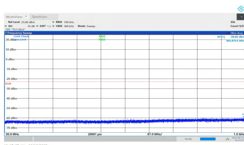
NTNV-n25-PC3-15-30-M-DFT-QPSK-Inner_1RB_Left-30-1000-PASS
