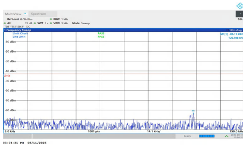
NTNV-n25-PC3-15-20-L-DFT-QPSK-Inner_1RB_Left-0.009-0.15- PASS
