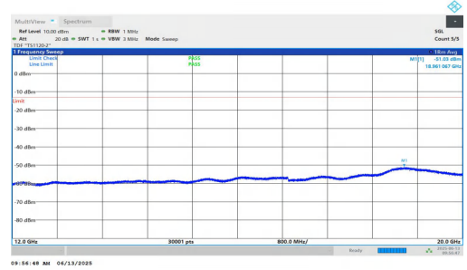
NTNV-n25-PC3-15-20-H-DFT-QPSK-Inner_1RB_Left-12000-2000 0-PASS
