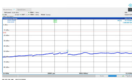
NTNV-n25-PC3-15-20-M-DFT-QPSK-Inner_1RB_Right-3000-12000-PASS
