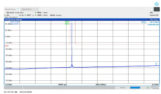
NTNV-n25-PC3-15-25-M-DFT-BPSK-Inner_1RB_Left-1000-3000-PASS
