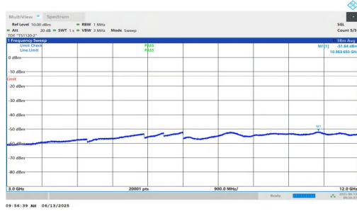
NTNV-n25-PC3-15-20-H-DFT-QPSK-Inner_1RB_Left-3000-1200 0-PASS
