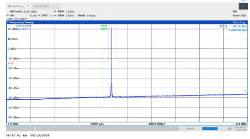
NTNV-n25-PC3-15-20-L-DFT-BPSK-Inner_1RB_Right-1000-3000-P PASS
