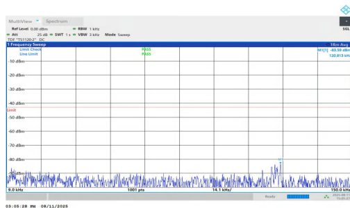
NTNV-n25-PC3-15-20-M-DFT-QPSK-Inner_1RB_Left-0.009-0.15-PASS
