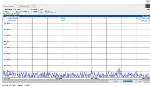
NTNV-n25-PC3-15-20-H-DFT-BPSK-Inner_1RB_Right-0.009-0.15-PASS
