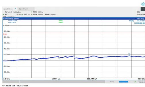
NTNV-n25-PC3-15-20-L-DFT-BPSK-Inner_1RB_Left-3000-12000 -PASS
