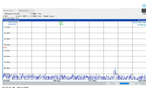
NTNV-n25-PC3-15-25-M-DFT-BPSK-Inner_1RB_Right-0.009-0.15-PASS
