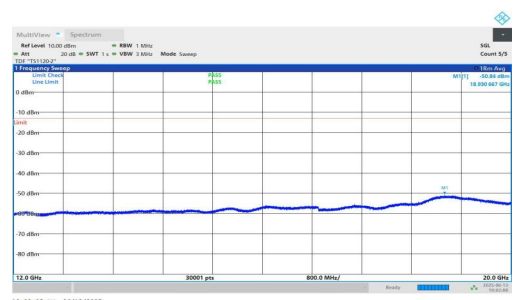
NTNV-n25-PC3-15-25-L-DFT-QPSK-Inner_1RB_Right-12000-20000 00-PASS
