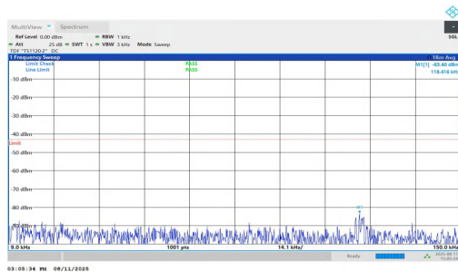
NTNV-n25-PC3-15-20-M-DFT-QPSK-Inner_1RB_Right-0.009-0.1 5-PASS
