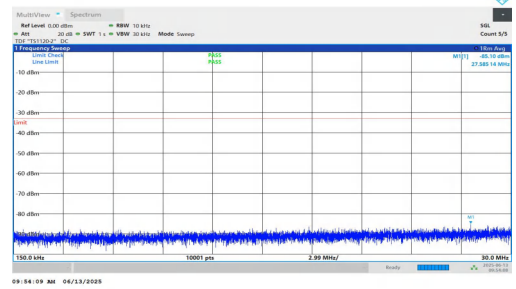
NTNV-n25-PC3-15-20-H-DFT-BPSK-Inner_1RB_Left-0.15-30-PASS
