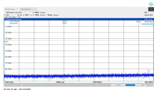
NTNV-n25-PC3-15-20-H-DFT-QPSK-Inner_1RB_Left-0.15-30-PASS
