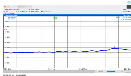
NTNV-n25-PC3-15-20-M-DFT-BPSK-Inner_1RB_Right-12000-20000-PASS
