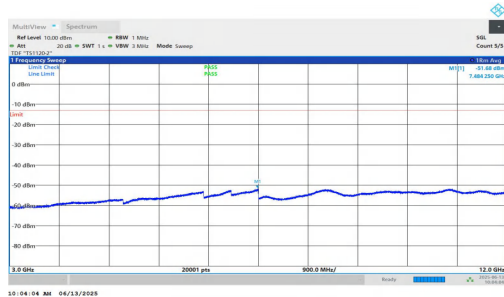
NTNV-n25-PC3-15-25-M-DFT-BPSK-Inner_1RB_Right-3000-12000-PASS
