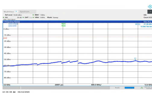
NTNV-n25-PC3-15-25-M-DFT-QPSK-Inner_1RB_Right-3000-12000- 00-PASS
