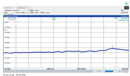
NTNV-n25-PC3-15-25-M-DFT-BPSK-Inner_1RB_Left-12000-20000-PASS
