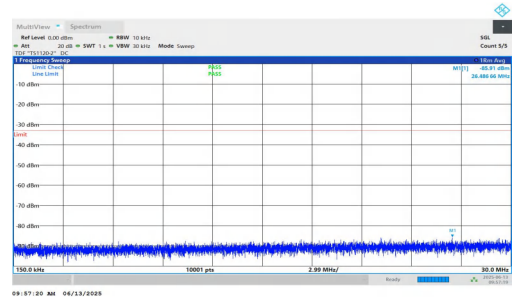
NTNV-n25-PC3-15-20-H-DFT-QPSK-Inner_1RB_Right-0.15-30-PA SS
