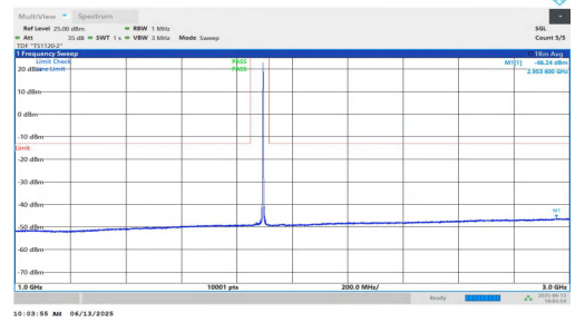
NTNV-n25-PC3-15-25-M-DFT-BPSK-Inner_1RB_Right-1000-3000-PASS
