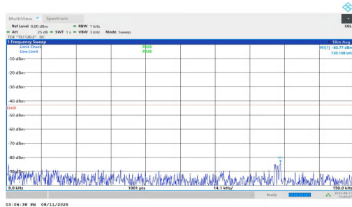
NTNV-n25-PC3-15-20-L-DFT-QPSK-Inner_1RB_Right-0.009-0.1 5-PASS
