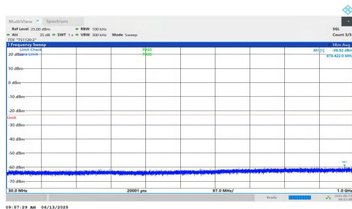
NTNV-n25-PC3-15-20-H-DFT-QPSK-Inner_1RB_Right-30-1000-PASS
