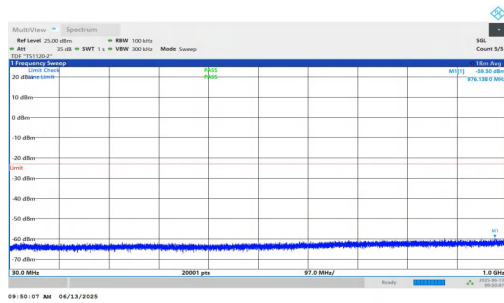
NTNV-n25-PC3-15-20-M-DFT-BPSK-Inner_1RB_Left-30-1000-PASS
