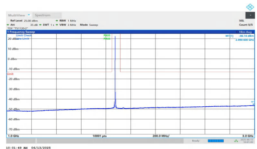
NTNV-n25-PC3-15-25-L-DFT-QPSK-Inner_1RB_Right-1000-3000-P PASS
