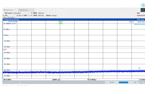
NTNV-n25-PC3-15-20-M-DFT-QPSK-Inner_1RB_Left-30-1000-PASS
