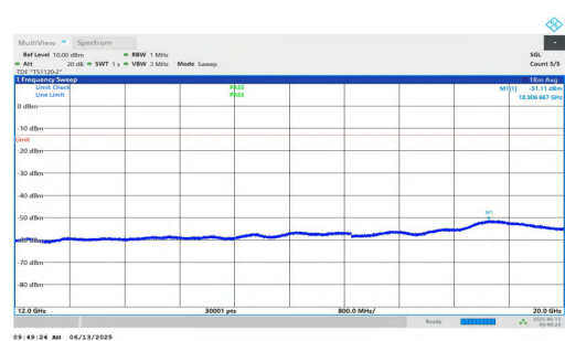
NTNV-n25-PC3-15-20-L-DFT-QPSK-Inner_1RB_Right-12000-20000 00-PASS
