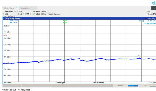
NTNV-n25-PC3-15-25-L-DFT-BPSK-Inner_1RB_Right-3000-1200 0-PASS
