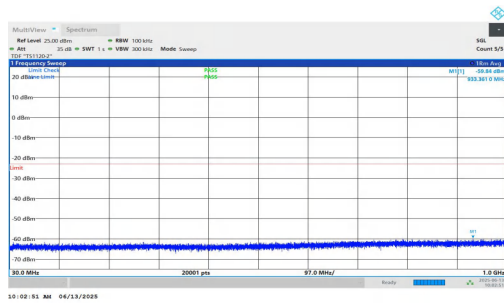
NTNV-n25-PC3-15-25-M-DFT-BPSK-Inner_1RB_Left-30-1000-PASS
