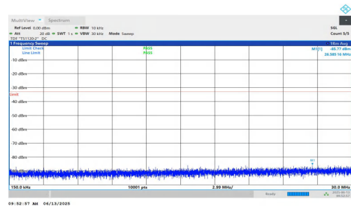
NTNV-n25-PC3-15-20-M-DFT-QPSK-Inner_1RB_Right-0.15-30-P ASS
