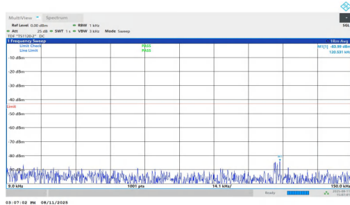
NTNV-n25-PC3-15-25-L-DFT-BPSK-Inner_1RB_Right-0.009-0.15-PASS
