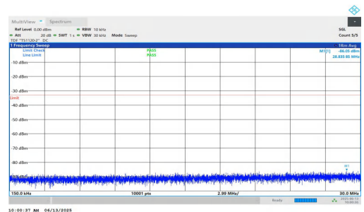
NTNV-n25-PC3-15-25-L-DFT-QPSK-Inner_1RB_Left-0.15-30-PAS S
