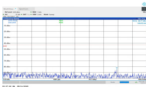
NTNV-n25-PC3-15-25-L-DFT-QPSK-Inner_1RB_Left-0.009-0.15- PASS
