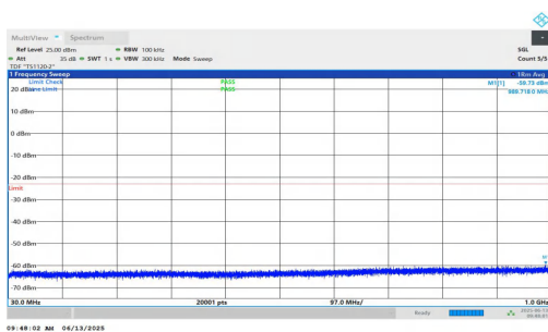
NTNV-n25-PC3-15-20-L-DFT-QPSK-Inner_1RB_Left-30-1000-PA SS
