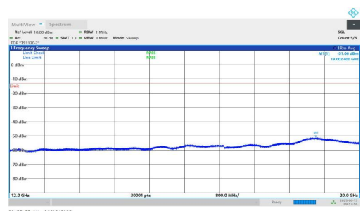
NTNV-n25-PC3-15-20-H-DFT-QPSK-Inner_1RB_Right-12000-20000-PASS
