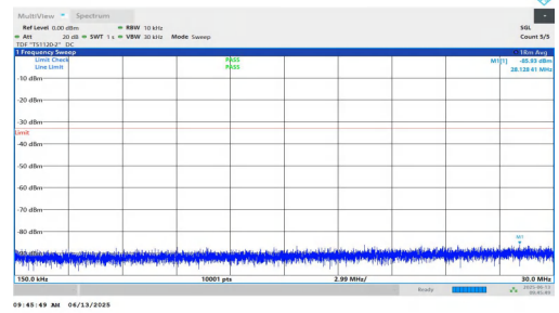
NTNV-n25-PC3-15-20-L-DFT-BPSK-Inner_1RB_Left-0.15-30-PAS S
