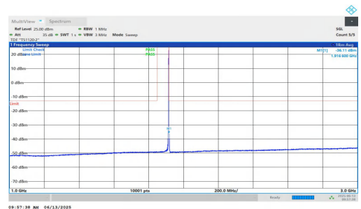
NTNV-n25-PC3-15-20-H-DFT-QPSK-Inner_1RB_Right-1000-3000-PASS
