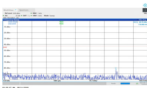
NTNV-n25-PC3-15-20-M-DFT-BPSK-Inner_1RB_Right-0.009-0.15-PASS
