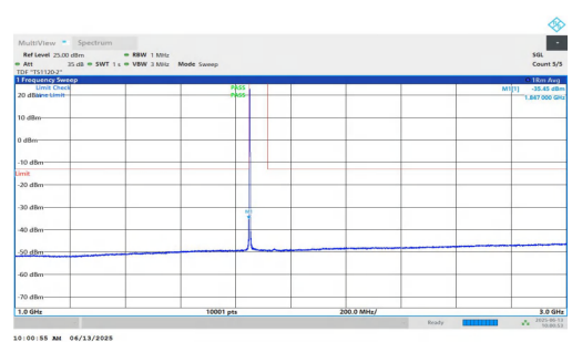
NTNV-n25-PC3-15-25-L-DFT-QPSK-Inner_1RB_Left-1000-3000-P ASS
