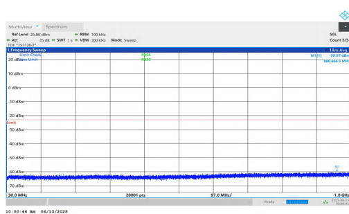
NTNV-n25-PC3-15-25-L-DFT-QPSK-Inner_1RB_Left-30-1000-PA SS
