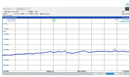
NTNV-n25-PC3-15-20-H-DFT-QPSK-Inner_1RB_Right-3000-12000-PASS
