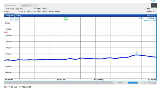
NTNV-n25-PC3-15-20-L-DFT-BPSK-Inner_1RB_Right-12000-200 00-PASS
