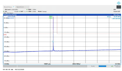
NTNV-n25-PC3-15-20-L-DFT-BPSK-Inner_1RB_Left-1000-3000-P ASS
