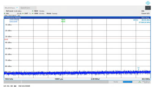
NTNV-n25-PC3-15-25-L-DFT-QPSK-Inner_1RB_Right-0.15-30-PA SS
