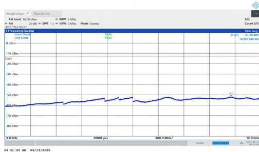
NTNV-n25-PC3-15-20-M-DFT-BPSK-Inner_1RB_Right-3000-12000-PASS
