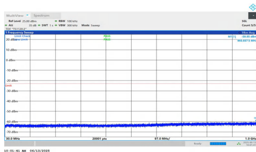
NTNV-n25-PC3-15-25-L-DFT-QPSK-Inner_1RB_Right-30-1000-P ASS
