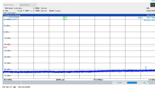
NTNV-n25-PC3-15-20-H-DFT-BPSK-Inner_1RB_Left-30-1000-PASS
