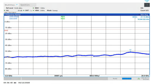
NTNV-n25-PC3-15-20-H-DFT-BPSK-Inner_1RB_Left-12000-20000-PASS
