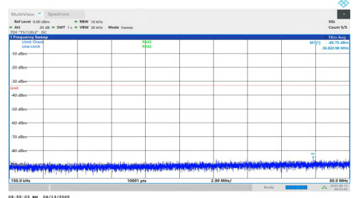
NTNV-n25-PC3-15-20-H-DFT-BPSK-Inner_1RB_Right-0.15-30-PASS
