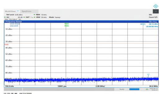
NTNV-n25-PC3-15-25-M-DFT-BPSK-Inner_1RB_Right-0.15-30-PASS
