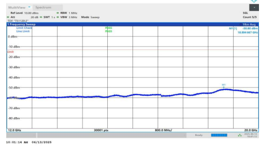
NTNV-n25-PC3-15-25-L-DFT-QPSK-Inner_1RB_Left-12000-2000 0-PASS
