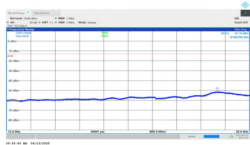
NTNV-n25-PC3-15-20-H-DFT-BPSK-Inner_1RB_Right-12000-20000-PASS
