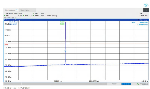
NTNV-n25-PC3-15-20-L-DFT-QPSK-Inner_1RB_Left-1000-3000-P ASS
