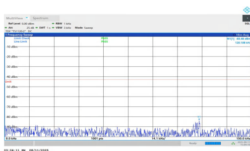
NTNV-n25-PC3-15-20-L-DFT-BPSK-Inner_1RB_Right-0.009-0.15 -PASS
