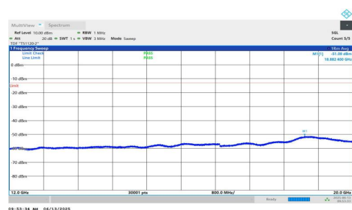
NTNV-n25-PC3-15-20-M-DFT-QPSK-Inner_1RB_Right-12000-20000-PASS
