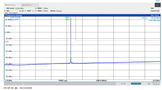
NTNV-n25-PC3-15-25-L-DFT-BPSK-Inner_1RB_Left-1000-3000-PASS
