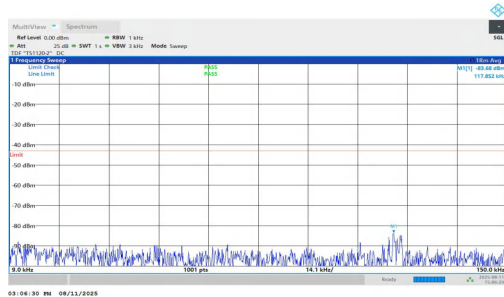
NTNV-n25-PC3-15-20-H-DFT-QPSK-Inner_1RB_Right-0.009-0.1 5-PASS
