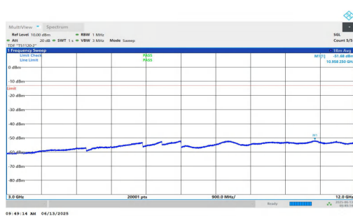
NTNV-n25-PC3-15-20-L-DFT-QPSK-Inner_1RB_Right-3000-12000 00-PASS
