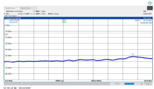
NTNV-n25-PC3-15-25-M-DFT-BPSK-Inner_1RB_Right-12000-20000-PASS
