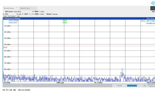
NTNV-n25-PC3-15-25-L-DFT-QPSK-Inner_1RB_Right-0.009-0.1 5-PASS
