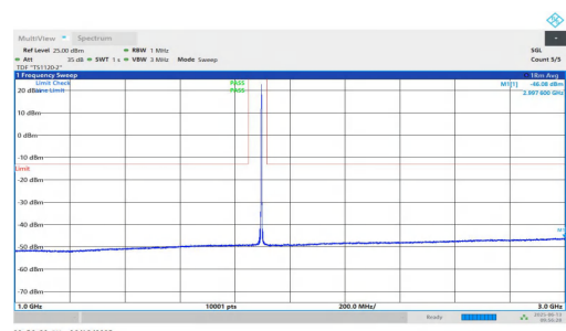
NTNV-n25-PC3-15-20-H-DFT-QPSK-Inner_1RB_Left-1000-3000-PASS
