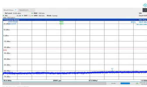
NTNV-n25-PC3-15-20-H-DFT-QPSK-Inner_1RB_Left-30-1000-PASS
