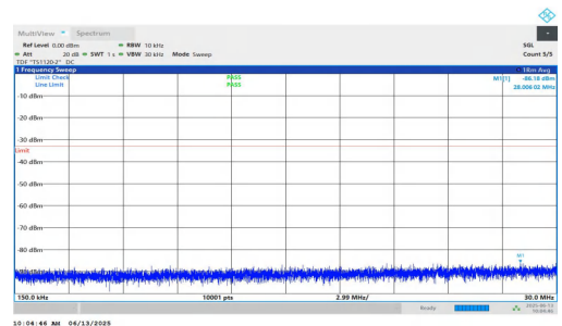
NTNV-n25-PC3-15-25-M-DFT-QPSK-Inner_1RB_Left-0.15-30-PASS
