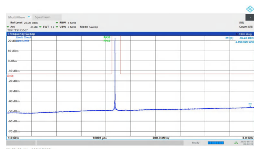
NTNV-n25-PC3-15-20-M-DFT-QPSK-Inner_1RB_Left-1000-3000-PASS
