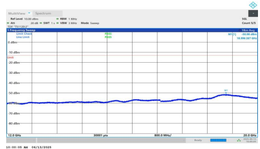
NTNV-n25-PC3-15-25-L-DFT-BPSK-Inner_1RB_Right-12000-200 00-PASS
