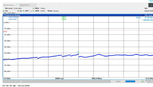
NTNV-n25-PC3-15-20-H-DFT-BPSK-Inner_1RB_Left-3000-12000-PASS
