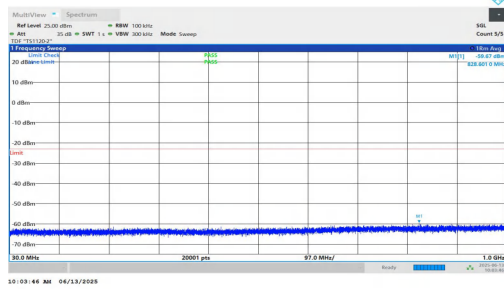
NTNV-n25-PC3-15-25-M-DFT-BPSK-Inner_1RB_Right-30-1000-PASS
