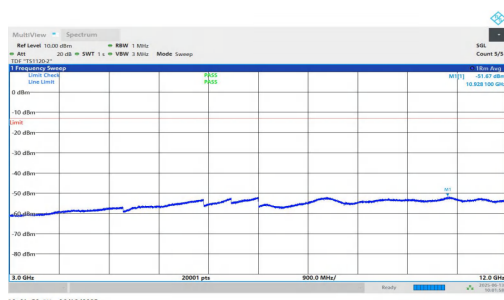
NTNV-n25-PC3-15-25-L-DFT-QPSK-Inner_1RB_Right-3000-12000 00-PASS
