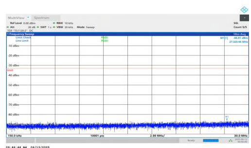
NTNV-n25-PC3-15-20-L-DFT-BPSK-Inner_1RB_Right-0.15-30-PASS SS
