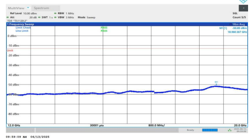
NTNV-n25-PC3-15-25-L-DFT-BPSK-Inner_1RB_Left-12000-20000-PASS
