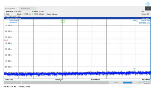
NTNV-n25-PC3-15-20-L-DFT-QPSK-Inner_1RB_Left-0.15-30-PAS S
