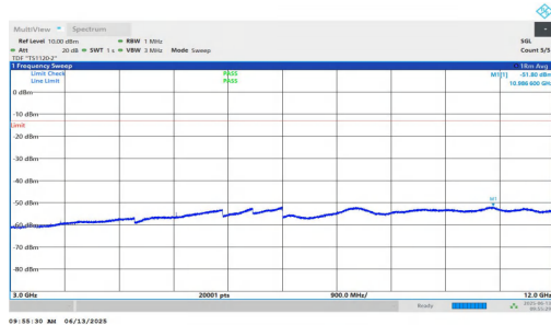
NTNV-n25-PC3-15-20-H-DFT-BPSK-Inner_1RB_Right-3000-12000-PASS
