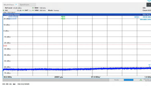
NTNV-n25-PC3-15-25-L-DFT-BPSK-Inner_1RB_Left-30-1000-PASS
