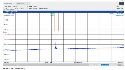
NTNV-n25-PC3-15-25-L-DFT-BPSK-Inner_1RB_Right-1000-3000-P PASS
