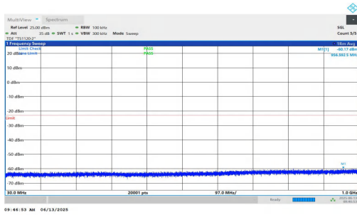
NTNV-n25-PC3-15-20-L-DFT-BPSK-Inner_1RB_Right-30-1000-P ASS
