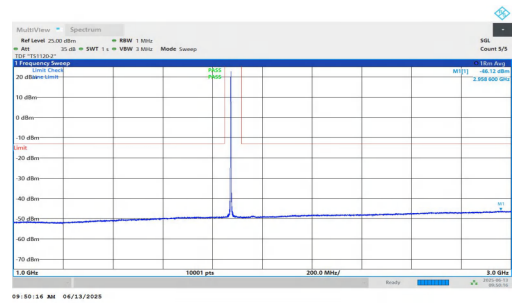
NTNV-n25-PC3-15-20-M-DFT-BPSK-Inner_1RB_Left-1000-3000-PASS
