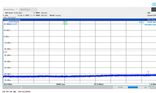
NTNV-n25-PC3-15-20-M-DFT-QPSK-Inner_1RB_Right-30-1000-PASS
