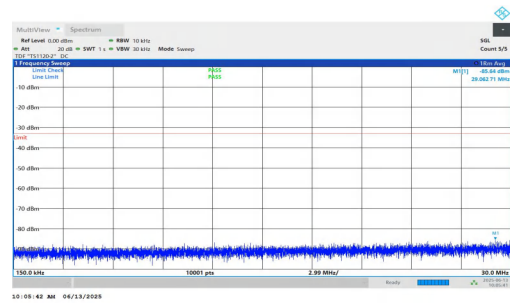
NTNV-n25-PC3-15-25-M-DFT-QPSK-Inner_1RB_Right-0.15-30-P ASS
