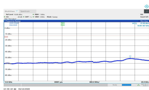
NTNV-n25-PC3-15-25-M-DFT-QPSK-Inner_1RB_Right-12000-20000- 00-PASS
