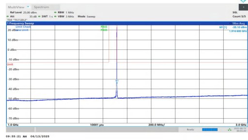
NTNV-n25-PC3-15-20-H-DFT-BPSK-Inner_1RB_Right-1000-3000-PASS
