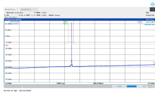
NTNV-n25-PC3-15-20-M-DFT-QPSK-Inner_1RB_Right-1000-3000-PASS
