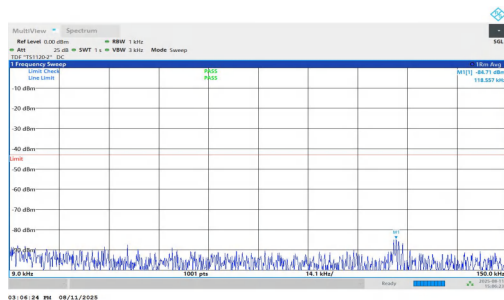
NTNV-n25-PC3-15-20-H-DFT-QPSK-Inner_1RB_Left-0.009-0.15-PASS
