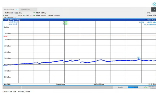
NTNV-n25-PC3-15-25-M-DFT-BPSK-Inner_1RB_Left-3000-12000-PASS
