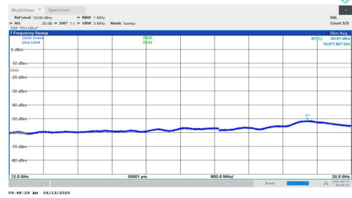
NTNV-n25-PC3-15-20-L-DFT-QPSK-Inner_1RB_Left-12000-20000 0-PASS
