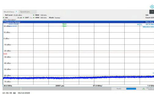
NTNV-n25-PC3-15-25-M-DFT-QPSK-Inner_1RB_Left-30-1000-PASS
