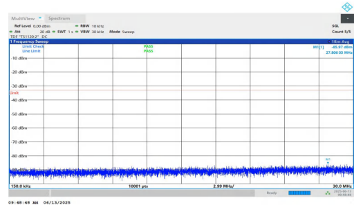
NTNV-n25-PC3-15-20-L-DFT-QPSK-Inner_1RB_Right-0.15-30-PA SS
