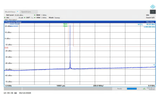
NTNV-n25-PC3-15-25-M-DFT-QPSK-Inner_1RB_Left-1000-3000-PASS
