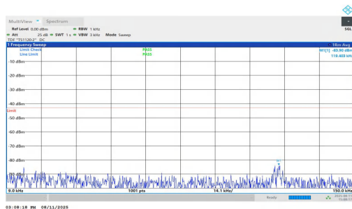
NTNV-n25-PC3-15-25-M-DFT-QPSK-Inner_1RB_Left-0.009-0.15-PASS
