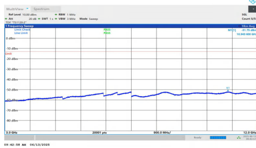
NTNV-n25-PC3-15-15-H-DFT-BPSK-Inner_1RB_Right-3000-120 00-PASS
