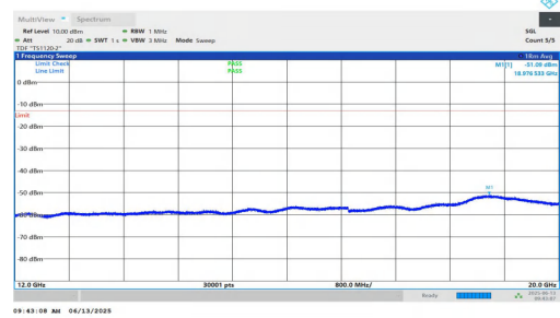
NTNV-n25-PC3-15-15-H-DFT-BPSK-Inner_1RB_Right-12000-200 00-PASS
