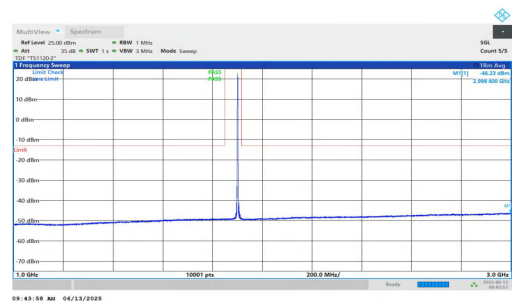
NTNV-n25-PC3-15-15-H-DFT-QPSK-Inner_1RB_Left-1000-3000- PASS
