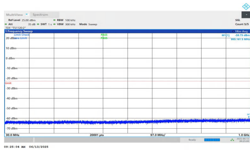
NTNV-n25-PC3-15-10-M-DFT-BPSK-Inner_1RB_Left-30-1000-PASS
