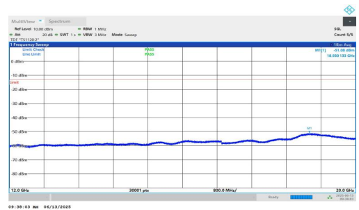
NTNV-n25-PC3-15-15-M-DFT-BPSK-Inner_1RB_Left-12000-20000-PASS
