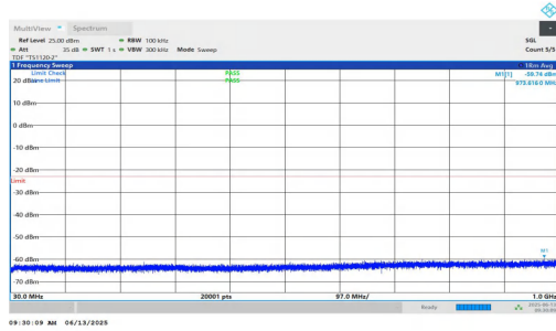
NTNV-n25-PC3-15-10-H-DFT-BPSK-Inner_1RB_Right-30-1000-P ASS
