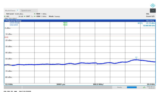
NTNV-n25-PC3-15-10-M-DFT-QPSK-Inner_1RB_Right-12000-200 00-PASS
