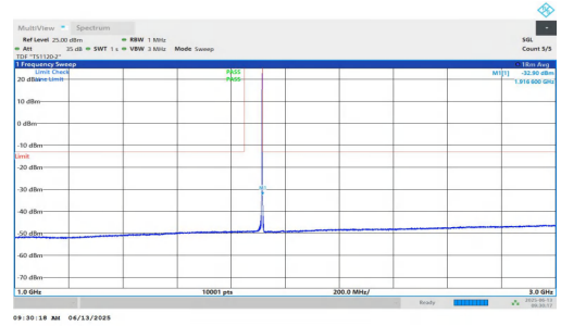
NTNV-n25-PC3-15-10-H-DFT-BPSK-Inner_1RB_Right-1000-3000- PASS
