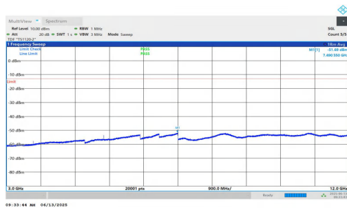
NTNV-n25-PC3-15-15-L-DFT-BPSK-Inner_1RB_Left-3000-12000 -PASS
