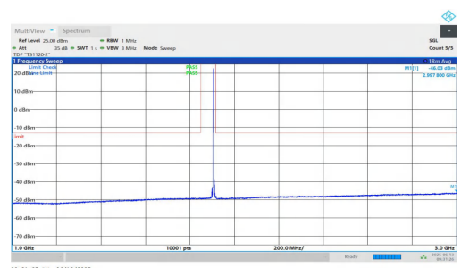
NTNV-n25-PC3-15-10-H-DFT-QPSK-Inner_1RB_Left-1000-3000- PASS
