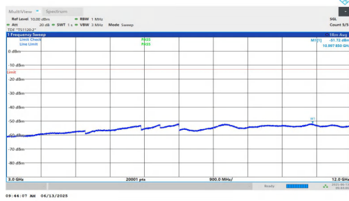
NTNV-n25-PC3-15-15-H-DFT-QPSK-Inner_1RB_Left-3000-1200 0-PASS
