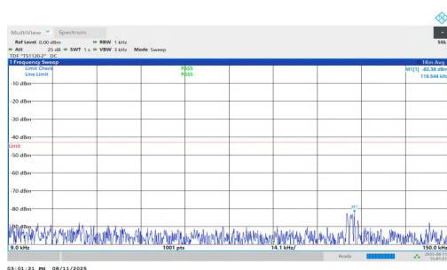
NTNV-n25-PC3-15-15-L-DFT-BPSK-Inner_1RB_Right-0.009-0.15 -PASS
