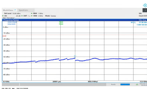
NTNV-n25-PC3-15-10-M-DFT-QPSK-Inner_1RB_Right-3000-120 00-PASS
