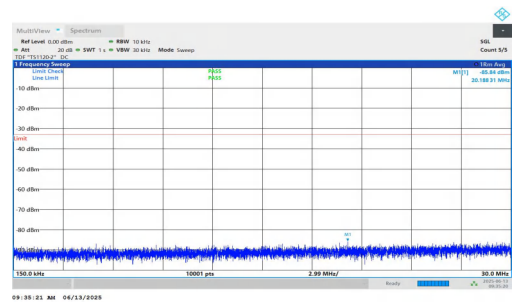
NTNV-n25-PC3-15-15-L-DFT-QPSK-Inner_1RB_Left-0.15-30-PAS S
