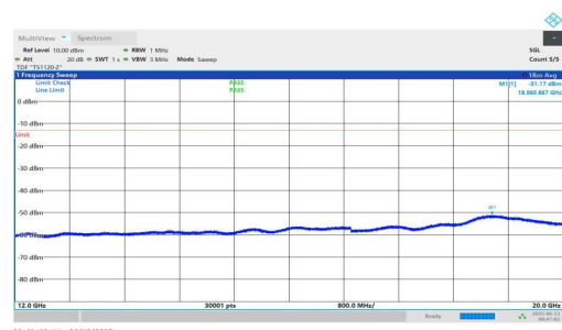
NTNV-n25-PC3-15-15-M-DFT-QPSK-Inner_1RB_Right-12000-20000-P 00-PASS
