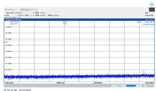
NTNV-n25-PC3-15-10-H-DFT-BPSK-Inner_1RB_Right-0.15-30-PASS SS
