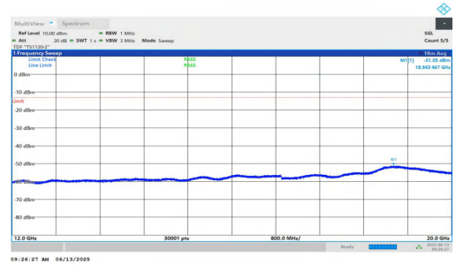
NTNV-n25-PC3-15-10-M-DFT-BPSK-Inner_1RB_Right-12000-20000-PASS
