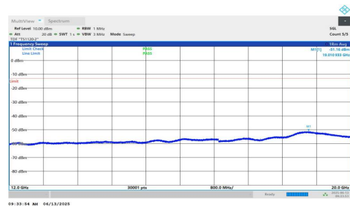
NTNV-n25-PC3-15-15-L-DFT-BPSK-Inner_1RB_Left-12000-20000 -PASS
