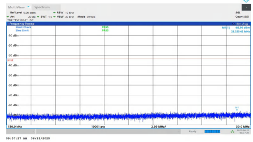
NTNV-n25-PC3-15-15-M-DFT-BPSK-Inner_1RB_Left-0.15-30-PASS
