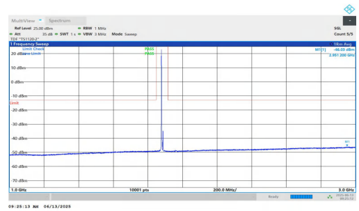
NTNV-n25-PC3-15-10-M-DFT-BPSK-Inner_1RB_Left-1000-3000-PASS
