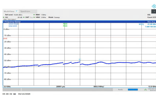
NTNV-n25-PC3-15-15-H-DFT-QPSK-Inner_1RB_Right-3000-12000-PASS
