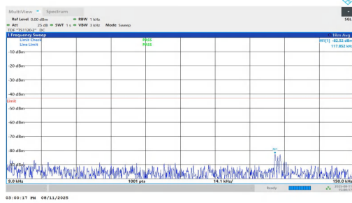
NTNV-n25-PC3-15-10-H-DFT-BPSK-Inner_1RB_Left-0.009-0.15-PASS
