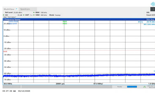
NTNV-n25-PC3-15-15-M-DFT-BPSK-Inner_1RB_Left-30-1000-PASS
