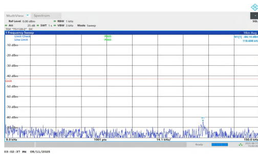
NTNV-n25-PC3-15-15-M-DFT-QPSK-Inner_1RB_Left-0.009-0.15-PASS
