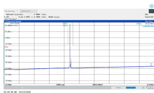
NTNV-n25-PC3-15-15-M-DFT-QPSK-Inner_1RB_Left-1000-3000-PASS
