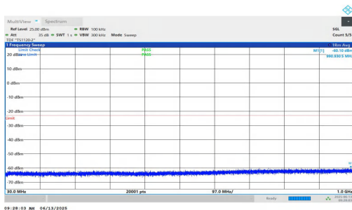
NTNV-n25-PC3-15-10-M-DFT-QPSK-Inner_1RB_Right-30-1000- PASS
