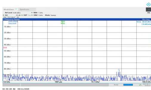
NTNV-n25-PC3-15-10-M-DFT-BPSK-Inner_1RB_Right-0.009-0.15-PASS
