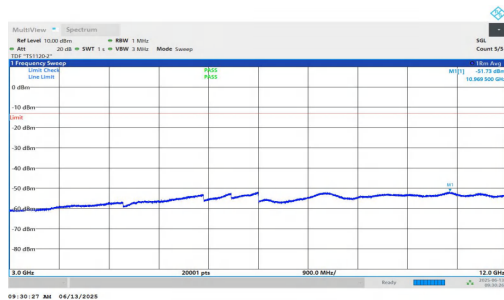
NTNV-n25-PC3-15-10-H-DFT-BPSK-Inner_1RB_Right-3000-120 00-PASS
