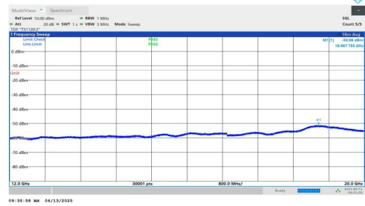
NTNV-n25-PC3-15-15-L-DFT-QPSK-Inner_1RB_Left-12000-20000 0-PASS
