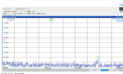
NTNV-n25-PC3-15-15-M-DFT-BPSK-Inner_1RB_Right-0.009-0.15-PASS
