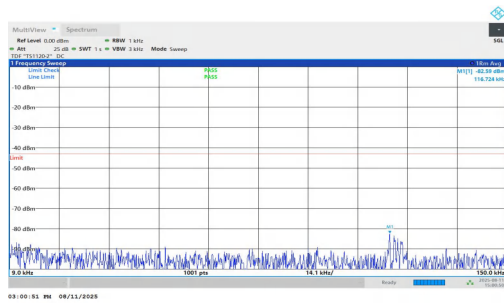
NTNV-n25-PC3-15-10-H-DFT-QPSK-Inner_1RB_Right-0.009-0.1 5-PASS
