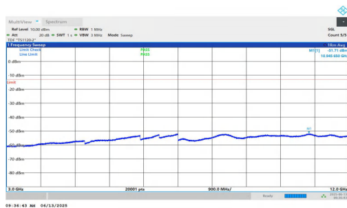
NTNV-n25-PC3-15-15-L-DFT-QPSK-Inner_1RB_Right-3000-12000 00-PASS
