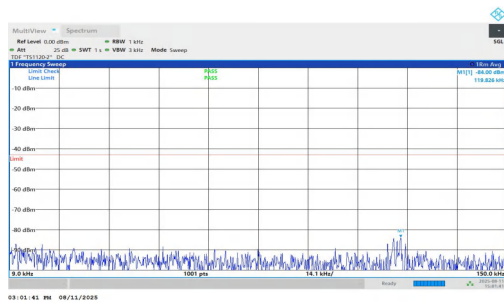
NTNV-n25-PC3-15-15-L-DFT-QPSK-Inner_1RB_Left-0.009-0.15- PASS
