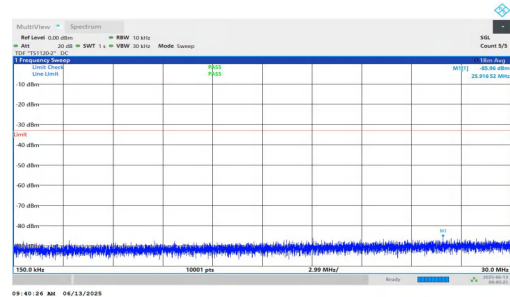
NTNV-n25-PC3-15-15-M-DFT-QPSK-Inner_1RB_Right-0.15-30-P ASS
