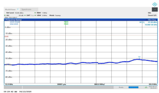
NTNV-n25-PC3-15-10-H-DFT-BPSK-Inner_1RB_Left-12000-20000-PASS 0-PASS
