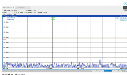
NTNV-n25-PC3-15-10-H-DFT-QPSK-Inner_1RB_Left-0.009-0.15- PASS
