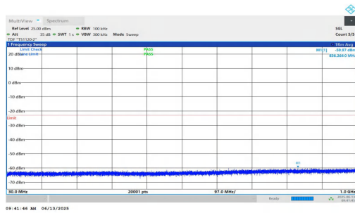
NTNV-n25-PC3-15-15-H-DFT-BPSK-Inner_1RB_Left-30-1000-PASS SS
