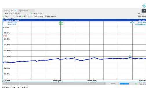
NTNV-n25-PC3-15-10-H-DFT-QPSK-Inner_1RB_Right-3000-12000- 00-PASS
