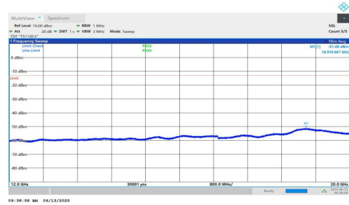
NTNV-n25-PC3-15-15-M-DFT-BPSK-Inner_1RB_Right-12000-20000-PASS
