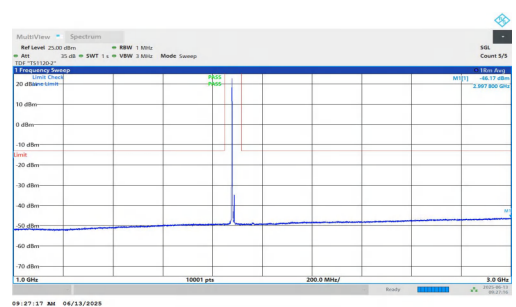
NTNV-n25-PC3-15-10-M-DFT-QPSK-Inner_1RB_Left-1000-3000-PASS
