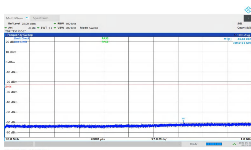
NTNV-n25-PC3-15-15-L-DFT-QPSK-Inner_1RB_Left-30-1000-PA SS
