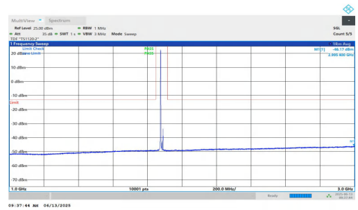
NTNV-n25-PC3-15-15-M-DFT-BPSK-Inner_1RB_Left-1000-3000-PASS
