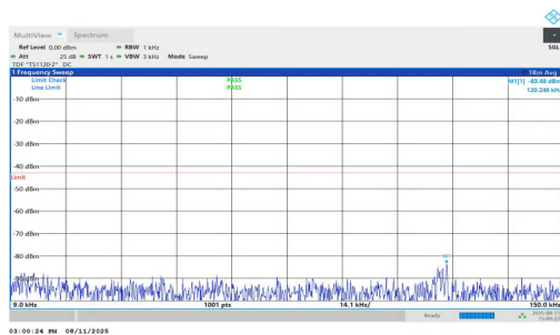
NTNV-n25-PC3-15-10-H-DFT-BPSK-Inner_1RB_Right-0.009-0.15-PASS 5-PASS
