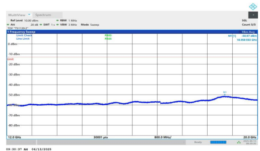
NTNV-n25-PC3-15-10-H-DFT-BPSK-Inner_1RB_Right-12000-200 00-PASS
