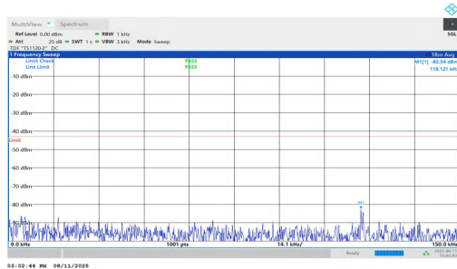
NTNV-n25-PC3-15-15-M-DFT-QPSK-Inner_1RB_Right-0.009-0.1 5-PASS
