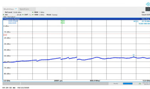
NTNV-n25-PC3-15-10-H-DFT-BPSK-Inner_1RB_Left-3000-12000-PASS 0-PASS
