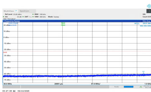
NTNV-n25-PC3-15-10-M-DFT-QPSK-Inner_1RB_Left-30-1000-PASS
