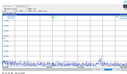
NTNV-n25-PC3-15-15-H-DFT-QPSK-Inner_1RB_Right-0.009-0.1 5-PASS
