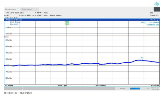
NTNV-n25-PC3-15-15-L-DFT-BPSK-Inner_1RB_Right-12000-200 00-PASS
