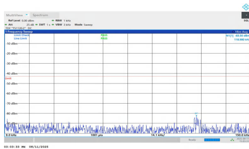
NTNV-n25-PC3-15-15-H-DFT-QPSK-Inner_1RB_Left-0.009-0.15- PASS
