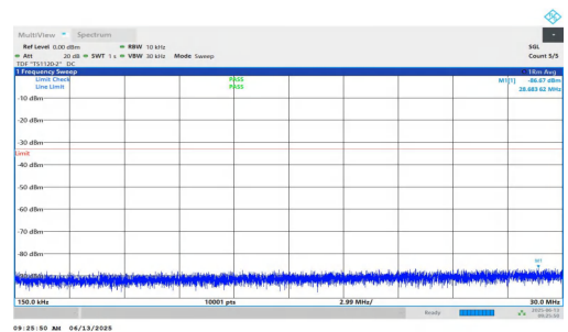
NTNV-n25-PC3-15-10-M-DFT-BPSK-Inner_1RB_Right-0.15-30-PASS
