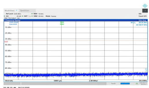
NTNV-n25-PC3-15-15-M-DFT-BPSK-Inner_1RB_Right-0.15-30-PASS
