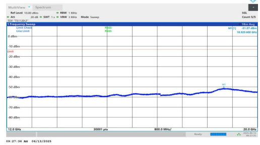
NTNV-n25-PC3-15-10-M-DFT-QPSK-Inner_1RB_Left-12000-2000 0-PASS
