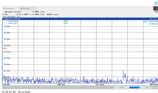
NTNV-n25-PC3-15-10-M-DFT-QPSK-Inner_1RB_Right-0.009-0.1 5-PASS
