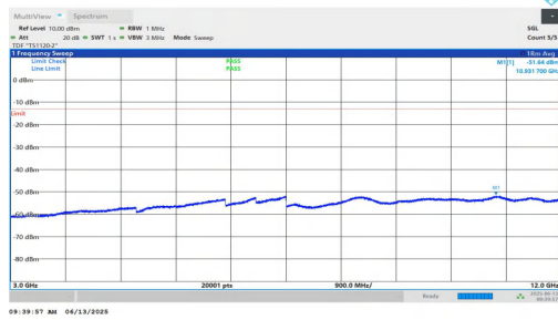
NTNV-n25-PC3-15-15-M-DFT-QPSK-Inner_1RB_Left-3000-1200 0-PASS
