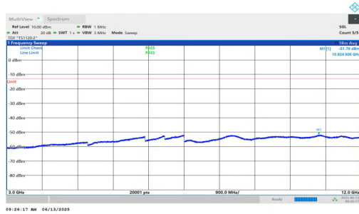
NTNV-n25-PC3-15-10-M-DFT-BPSK-Inner_1RB_Right-3000-12000-PASS
