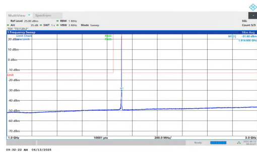
NTNV-n25-PC3-15-10-H-DFT-QPSK-Inner_1RB_Right-1000-3000- -PASS
