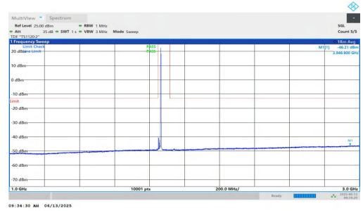
NTNV-n25-PC3-15-15-L-DFT-BPSK-Inner_1RB_Right-1000-3000-P PASS
