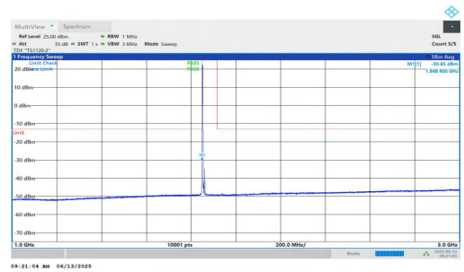
NTNV-n25-PC3-15-10-L-DFT-BPSK-Inner_1RB_Left-1000-3000-PASS
