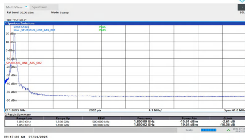
NTNV-n25-PC3-15-40-L-DFT-QPSK-Edge_1RB_Left-PASS
