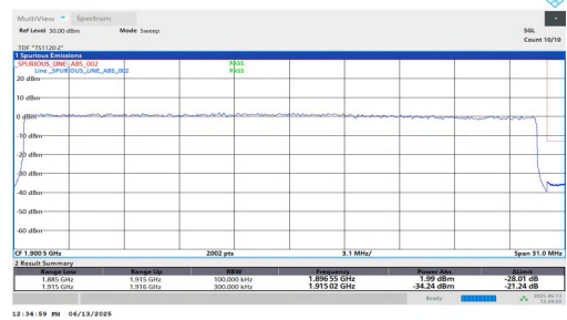
NTNV-n25-PC3-15-30-H-DFT-QPSK-Outer_Full-PASS
