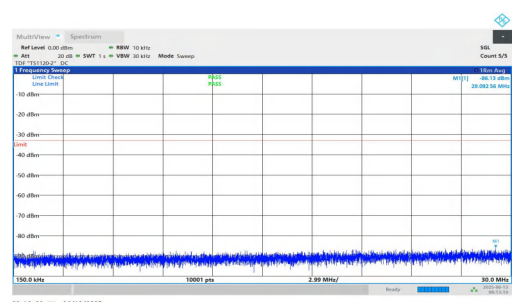
NTNV-n25-PC3-15-5-M-DFT-BPSK-Inner_1RB_Right-0.15-30-PASS
