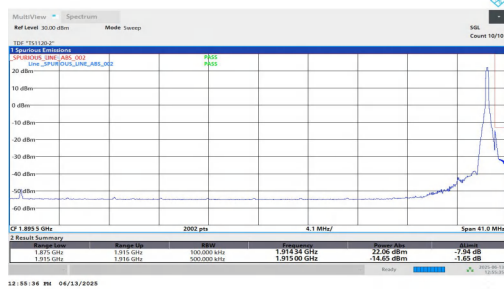
NTNV-n25-PC3-15-40-H-DFT-QPSK-Edge_1RB_Right-PASS
