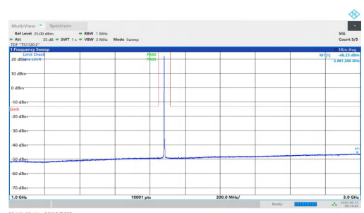
NTNV-n25-PC3-15-5-M-DFT-QPSK-Inner_1RB_Left-1000-3000-P PASS
