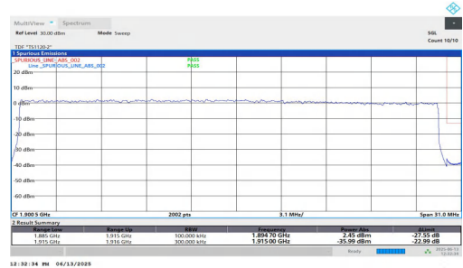
NTNV-n25-PC3-15-30-H-DFT-BPSK-Outer_Full-PASS
