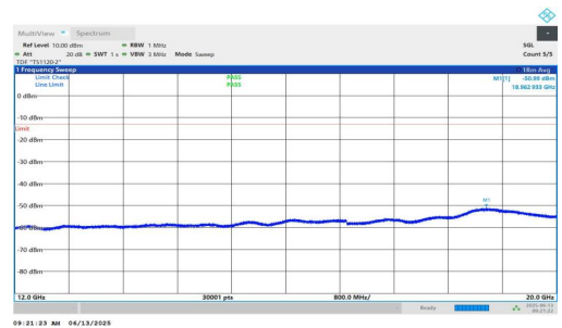
NTNV-n25-PC3-15-10-L-DFT-BPSK-Inner_1RB_Left-12000-20000-PASS
