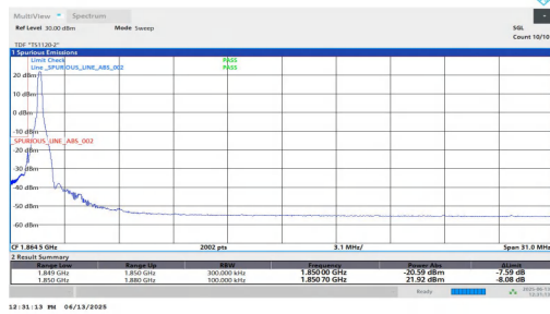
NTNV-n25-PC3-15-30-L-DFT-QPSK-Edge_1RB_Left-PASS
