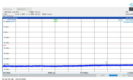
NTNV-n25-PC3-15-10-L-DFT-QPSK-Inner_1RB_Left-30-1000-PA SS
