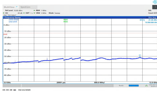
NTVN-n25-PC3-15-5-L-DFT-BPSK-Inner_1RB_Right-3000-12000 -PASS
