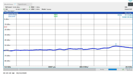
NTNV-n25-PC3-15-10-L-DFT-QPSK-Inner_1RB_Left-12000-20000-0-PASS
