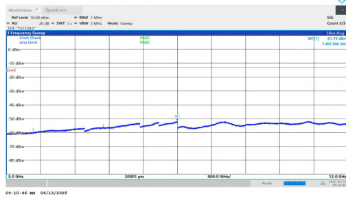
NTNV-n25-PC3-15-5-L-DFT-QPSK-Inner_1RB_Left-3000-12000-PASS
