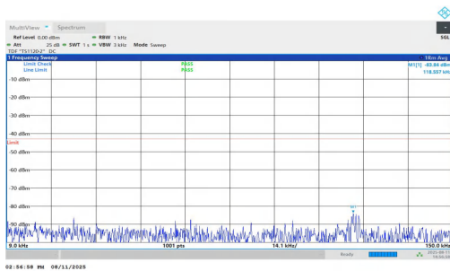
NTNV-n25-PC3-15-5-M-DFT-QPSK-Inner_1RB_Left-0.009-0.15-P PASS
