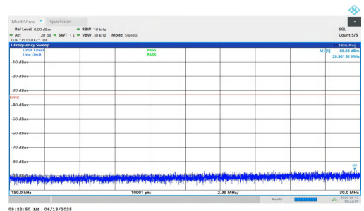
NTNV-n25-PC3-15-10-L-DFT-QPSK-Inner_1RB_Left-0.15-30-PAS S
