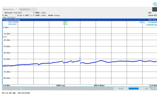
NTNV-n25-PC3-15-5-M-DFT-BPSK-Inner_1RB_Right-3000-12000-P PASS
