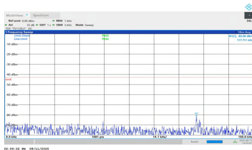
NTVN-n25-PC3-15-5-L-DFT-QPSK-Inner_1RB_Left-0.009-0.15-P ASS
