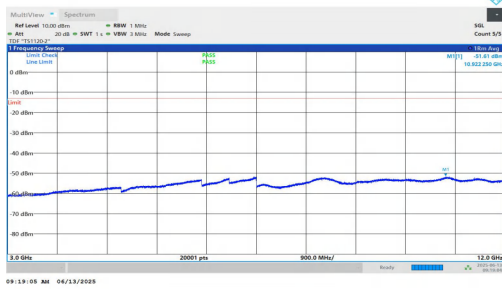
NTNV-n25-PC3-15-5-H-DFT-QPSK-Inner_1RB_Left-3000-12000-PASS
