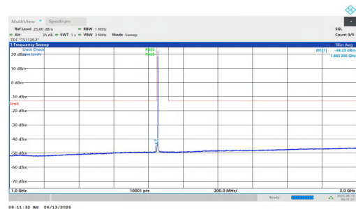
NTNV-n25-PC3-15-5-L-DFT-QPSK-Inner_1RB_Right-1000-3000-PASS
