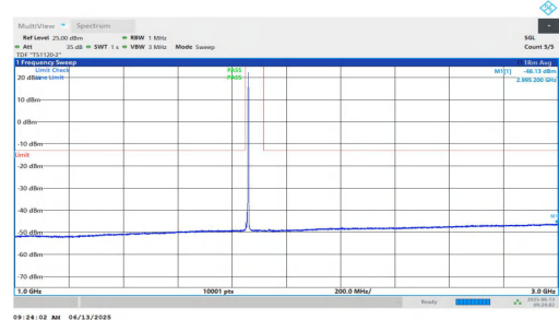
NTNV-n25-PC3-15-10-L-DFT-QPSK-Inner_1RB_Right-1000-3000-PASS
