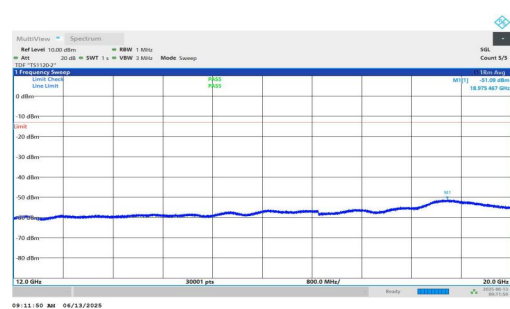
NTNV-n25-PC3-15-5-L-DFT-QPSK-Inner_1RB_Right-12000-20000-PASS
