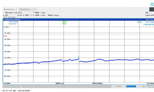
NTNV-n25-PC3-15-5-H-DFT-BPSK-Inner_1RB_Left-3000-12000-PASS
