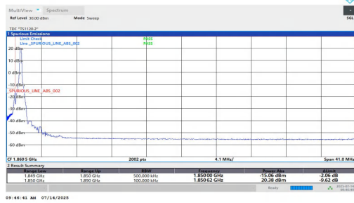
NTNV-n25-PC3-15-40-L-DFT-BPSK-Edge_1RB_Left-PASS
