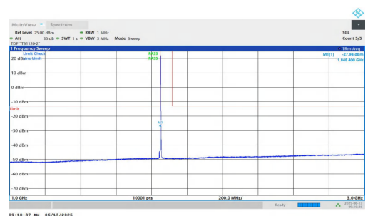
NTVN-n25-PC3-15-5-L-DFT-QPSK-Inner_1RB_Left-1000-3000-PA SS
