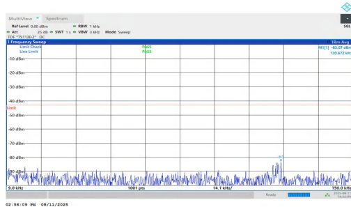
NTNV-n25-PC3-15-5-L-DFT-QPSK-Inner_1RB_Right-0.009-0.15-PASS
