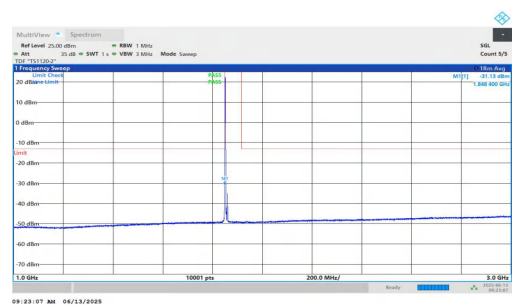
NTNV-n25-PC3-15-10-L-DFT-QPSK-Inner_1RB_Left-1000-3000-P ASS
