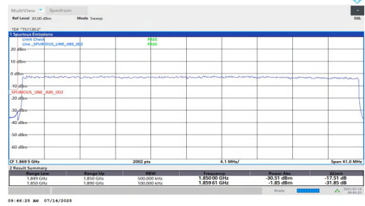
NTNV-n25-PC3-15-40-L-DFT-BPSK-Outer_Full-PASS
