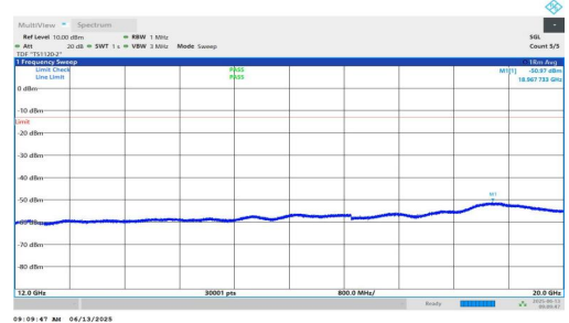
NTVN-n25-PC3-15-5-L-DFT-BPSK-Inner_1RB_Right-12000-2000 0-PASS
