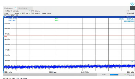
NTNV-n25-PC3-15-5-H-DFT-QPSK-Inner_1RB_Left-0.15-30-PAS S
