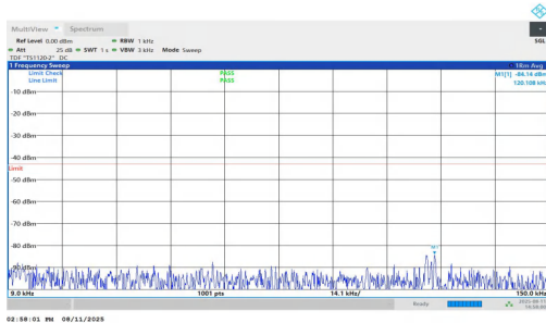
NTNV-n25-PC3-15-5-H-DFT-QPSK-Inner_1RB_Right-0.009-0.15-PASS
