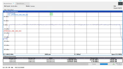
NTNV-n25-PC3-15-30-L-DFT-QPSK-Outer_Full-PASS
