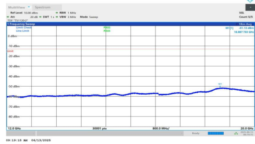
NTNV-n25-PC3-15-5-H-DFT-QPSK-Inner_1RB_Left-12000-20000-PASS
