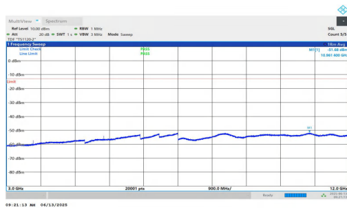
NTNV-n25-PC3-15-10-L-DFT-BPSK-Inner_1RB_Left-3000-12000-PASS
