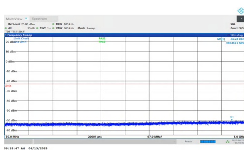
NTNV-n25-PC3-15-5-H-DFT-QPSK-Inner_1RB_Left-30-1000-PA SS
