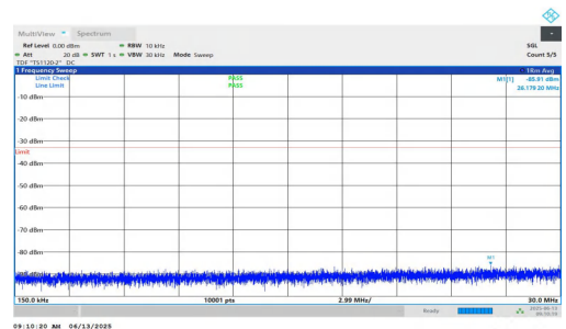
NTVN-n25-PC3-15-5-L-DFT-QPSK-Inner_1RB_Left-0.15-30-PASS
