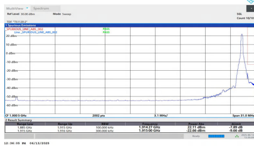
NTNV-n25-PC3-15-30-H-DFT-QPSK-Edge_1RB_Right-PASS
