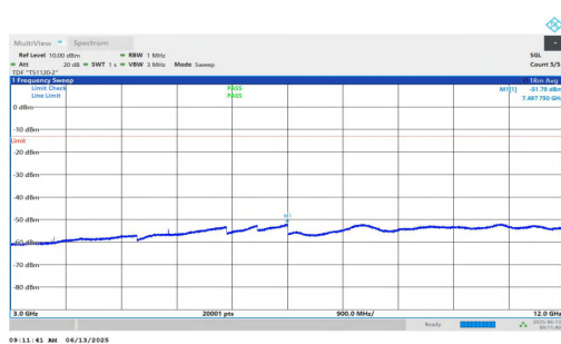
NTNV-n25-PC3-15-5-L-DFT-QPSK-Inner_1RB_Right-3000-12000-PASS
