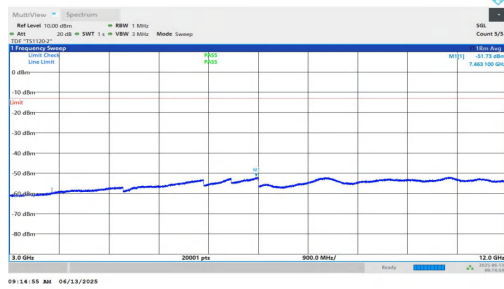
NTNV-n25-PC3-15-5-M-DFT-QPSK-Inner_1RB_Left-3000-12000 -PASS
