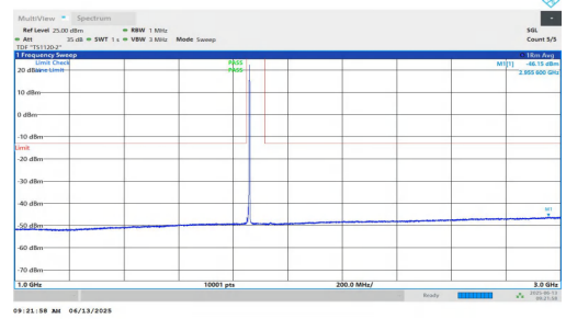
NTNV-n25-PC3-15-10-L-DFT-BPSK-Inner_1RB_Right-1000-3000-P PASS
