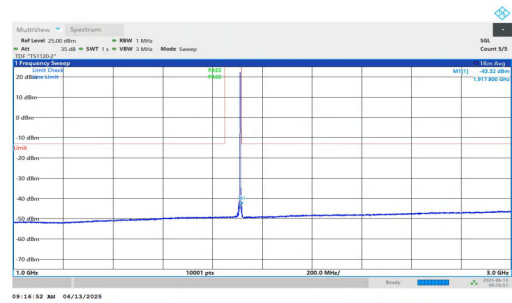
NTNV-n25-PC3-15-5-H-DFT-BPSK-Inner_1RB_Left-1000-3000-PASS
