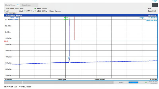
NTVN-n25-PC3-15-5-L-DFT-BPSK-Inner_1RB_Right-1000-3000-P ASS
