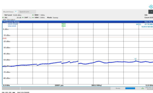
NTNV-n25-PC3-15-5-H-DFT-QPSK-Inner_1RB_Right-3000-12000-PASS
