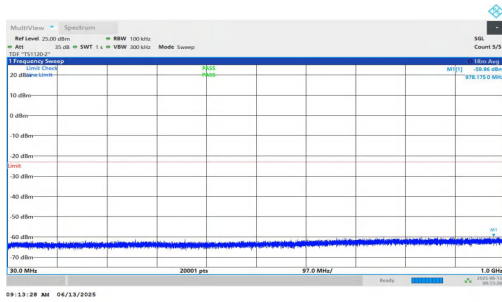
NTNV-n25-PC3-15-5-M-DFT-BPSK-Inner_1RB_Right-30-1000-P ASS
