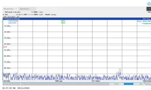
NTNV-n25-PC3-15-5-M-DFT-QPSK-Inner_1RB_Right-0.009-0.15 -PASS
