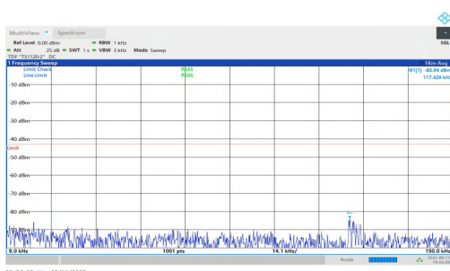
NTNV-n25-PC3-15-5-M-DFT-BPSK-Inner_1RB_Right-0.009-0.15-PASS
