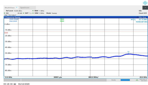
NTNV-n25-PC3-15-5-H-DFT-BPSK-Inner_1RB_Right-12000-2000 0-PASS
