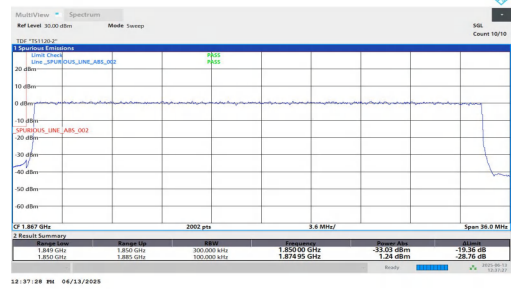
NTNV-n25-PC3-15-35-L-DFT-BPSK-Outer_Full-PASS
