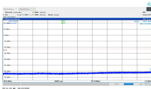
NTNV-n25-PC3-15-5-L-DFT-QPSK-Inner_1RB_Right-30-1000-PASS
