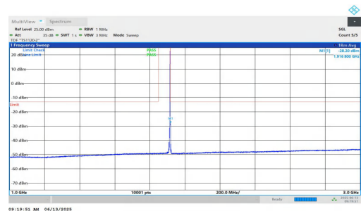
NTNV-n25-PC3-15-5-H-DFT-QPSK-Inner_1RB_Right-1000-3000-PASS
