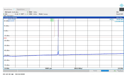
NTNV-n25-PC3-15-5-H-DFT-QPSK-Inner_1RB_Left-1000-3000-P ASS
