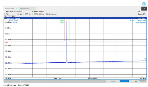
NTNV-n25-PC3-15-5-M-DFT-BPSK-Inner_1RB_Left-1000-3000-PASS
