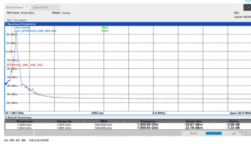
NTNV-n25-PC3-15-35-L-DFT-BPSK-Edge_1RB_Left-PASS
