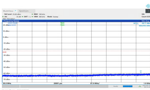
NTNV-n25-PC3-15-5-M-DFT-QPSK-Inner_1RB_Left-30-1000-P PASS
