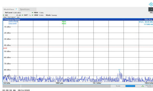
NTNV-n25-PC3-15-10-L-DFT-QPSK-Inner_1RB_Left-0.009-0.15- PASS
