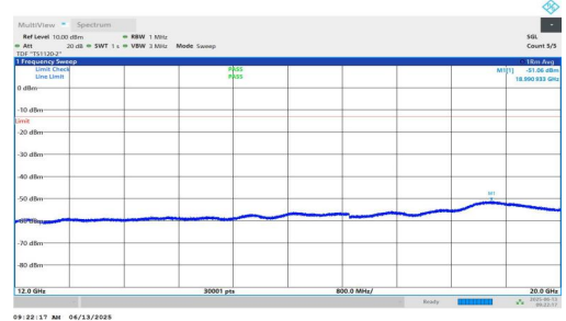
NTNV-n25-PC3-15-10-L-DFT-BPSK-Inner_1RB_Right-12000-200 00-PASS
