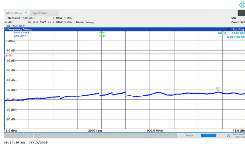
NTNV-n25-PC3-15-5-H-DFT-BPSK-Inner_1RB_Right-3000-1200 0-PASS
