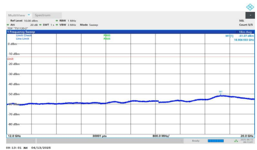
NTNV-n25-PC3-15-5-M-DFT-BPSK-Inner_1RB_Left-12000-20000-PASS
