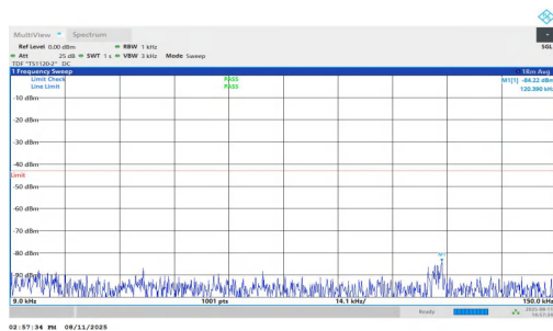
NTNV-n25-PC3-15-5-H-DFT-BPSK-Inner_1RB_Right-0.009-0.15-PASS
