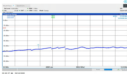
NTNV-n25-PC3-15-10-L-DFT-BPSK-Inner_1RB_Right-3000-1200 0-PASS
