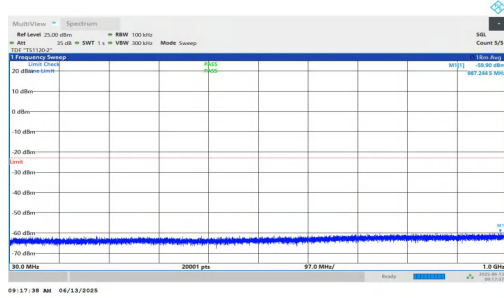
NTNV-n25-PC3-15-5-H-DFT-BPSK-Inner_1RB_Right-30-1000-P ASS
