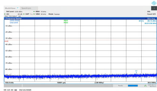
NTNV-n25-PC3-15-5-H-DFT-QPSK-Inner_1RB_Right-0.15-30-PA-SS
