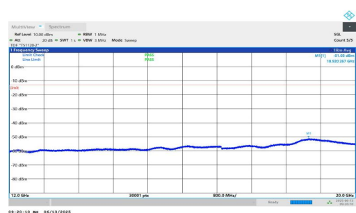
NTNV-n25-PC3-15-5-H-DFT-QPSK-Inner_1RB_Right-12000-20000-PASS
