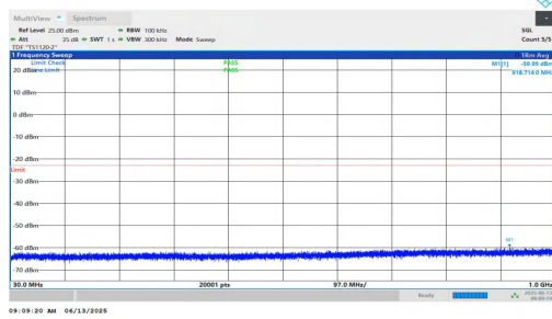
NTVN-n25-PC3-15-5-L-DFT-BPSK-Inner_1RB_Right-30-1000-PA SS
