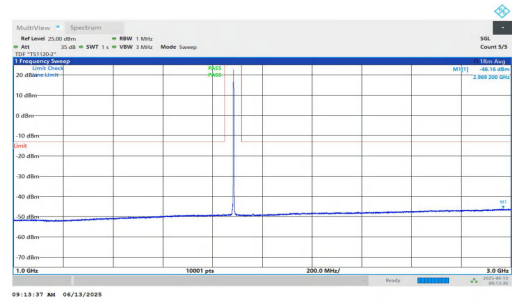
NTNV-n25-PC3-15-5-M-DFT-BPSK-Inner_1RB_Right-1000-3000-P PASS
