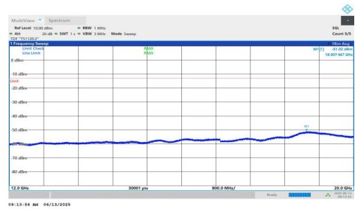
NTNV-n25-PC3-15-5-M-DFT-BPSK-Inner_1RB_Right-12000-20000-P PASS
