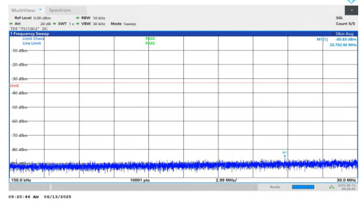
NTNV-n25-PC3-15-10-L-DFT-BPSK-Inner_1RB_Left-0.15-30-PASS
