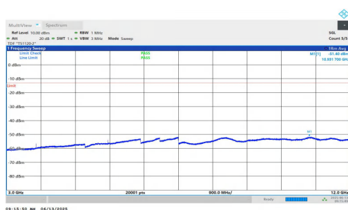
NTNV-n25-PC3-15-5-M-DFT-QPSK-Inner_1RB_Right-3000-1200 0-PASS
