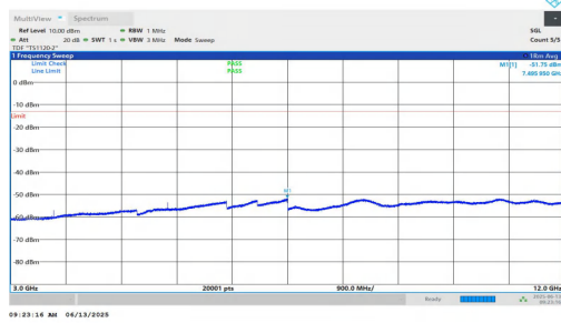
NTNV-n25-PC3-15-10-L-DFT-QPSK-Inner_1RB_Left-3000-12000-PASS
