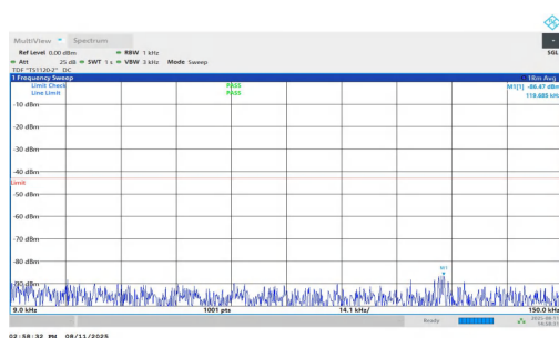
NTNV-n25-PC3-15-10-L-DFT-BPSK-Inner_1RB_Right-0.009-0.15-PASS
