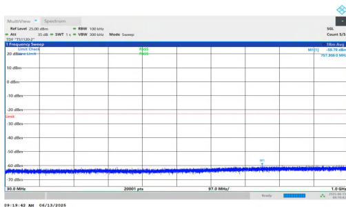
NTNV-n25-PC3-15-5-H-DFT-QPSK-Inner_1RB_Right-30-1000-PASS
