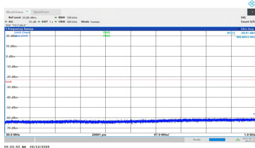
NTNV-n25-PC3-15-10-L-DFT-QPSK-Inner_1RB_Right-30-1000-P-ASS
