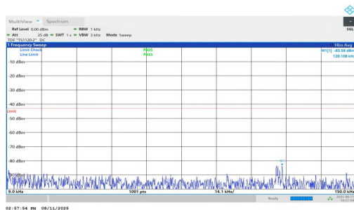
NTNV-n25-PC3-15-5-H-DFT-QPSK-Inner_1RB_Left-0.009-0.15-P ASS
