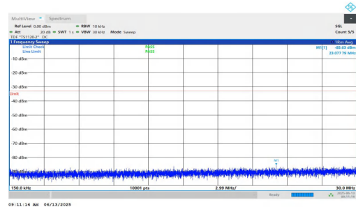
NTNV-n25-PC3-15-5-L-DFT-QPSK-Inner_1RB_Right-0.15-30-PASS
