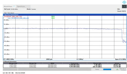
NTNV-n25-PC3-15-40-H-DFT-BPSK-Outer_Full-PASS
