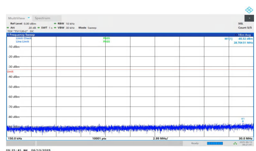
NTNV-n25-PC3-15-10-L-DFT-BPSK-Inner_1RB_Right-0.15-30-PASS
