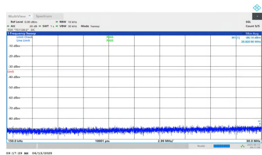
NTNV-n25-PC3-15-5-H-DFT-BPSK-Inner_1RB_Right-0.15-30-PASS
