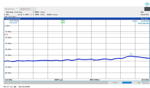
NTNV-n25-PC3-15-5-H-DFT-BPSK-Inner_1RB_Left-12000-20000-PASS
