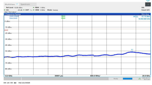
NTNV-n25-PC3-15-5-M-DFT-QPSK-Inner_1RB_Left-12000-20000 -PASS
