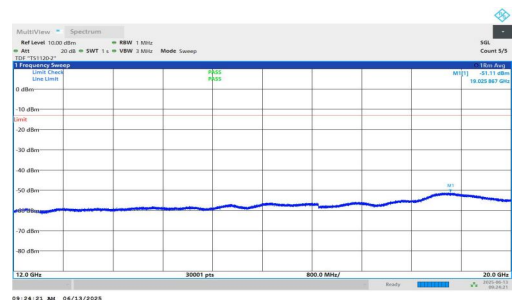
NTNV-n25-PC3-15-10-L-DFT-QPSK-Inner_1RB_Right-12000-20000-00-PASS
