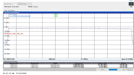
NTNV-n25-PC3-15-40-L-DFT-QPSK-Outer_Full-PASS
