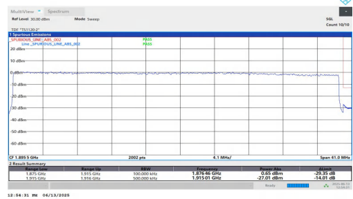
NTNV-n25-PC3-15-40-H-DFT-QPSK-Outer_Full-PASS
