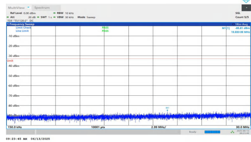
NTNV-n25-PC3-15-10-L-DFT-QPSK-Inner_1RB_Right-0.15-30-PA-SS
