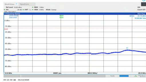
NTNV-n25-PC3-15-5-L-DFT-QPSK-Inner_1RB_Left-12000-20000-PASS
