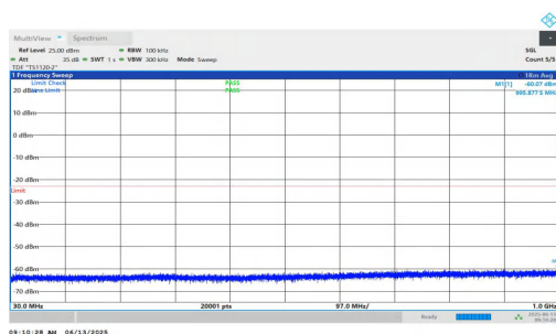
NTVN-n25-PC3-15-5-L-DFT-QPSK-Inner_1RB_Left-30-1000-PA SS
