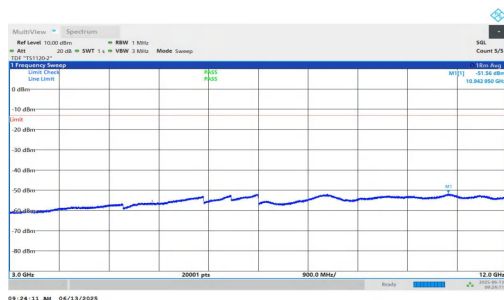
NTNV-n25-PC3-15-10-L-DFT-QPSK-Inner_1RB_Right-3000-12000-00-PASS
