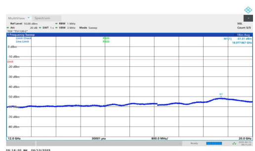
NTNV-n25-PC3-15-5-M-DFT-QPSK-Inner_1RB_Right-12000-2000 0-PASS
