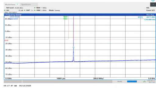
NTNV-n25-PC3-15-5-H-DFT-BPSK-Inner_1RB_Right-1000-3000-P PASS
