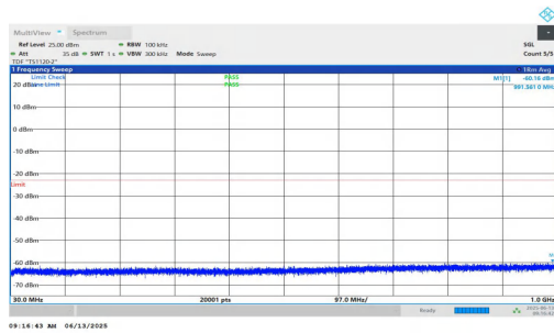
NTNV-n25-PC3-15-5-H-DFT-BPSK-Inner_1RB_Left-30-1000-PASS
